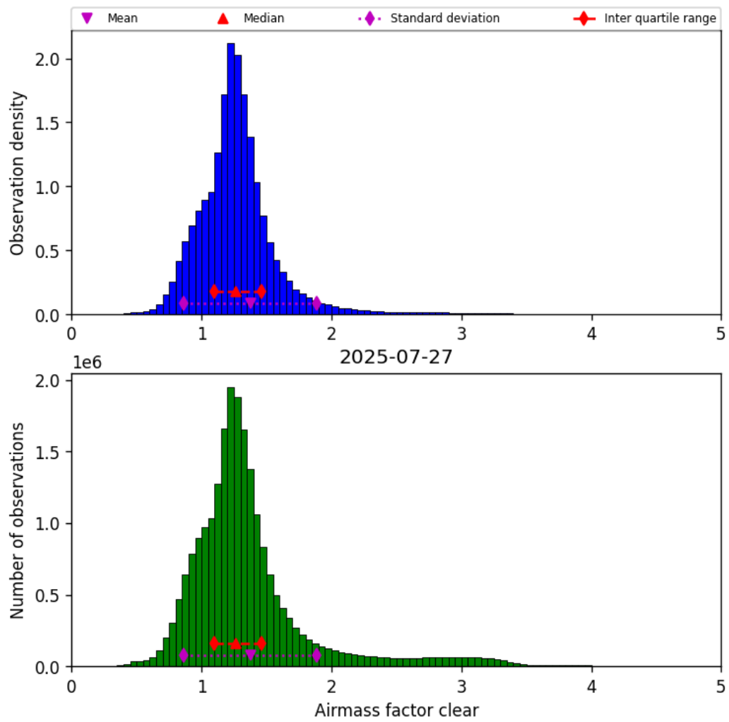
Figure 40: Histogram of “Airmass factor clear” for 2025-07-27 to 2025-07-27
