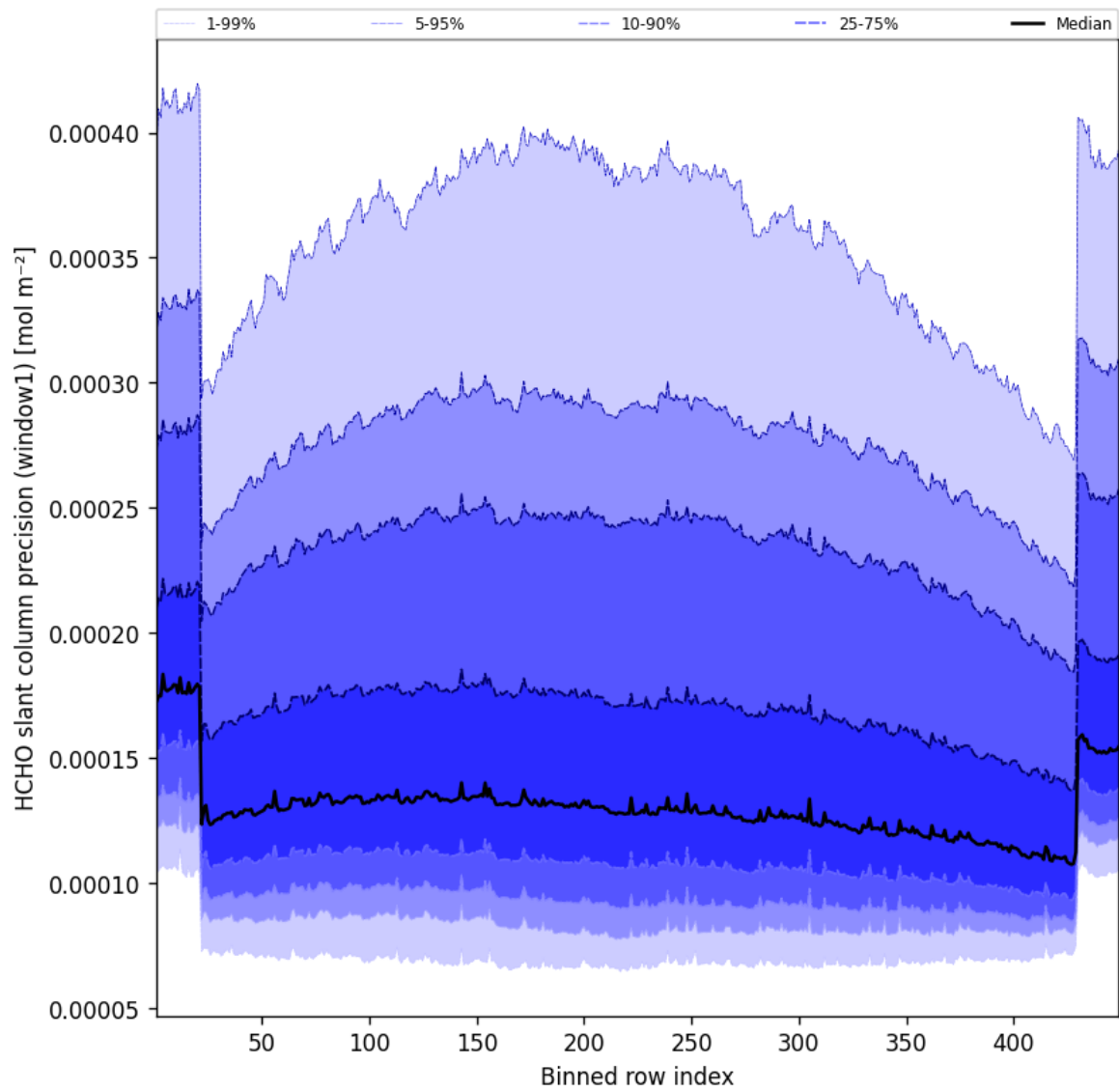
Figure 51: Along track statistics of “HCHO slant column precision (window1)” for 2025-07-27 to 2025-07-27
