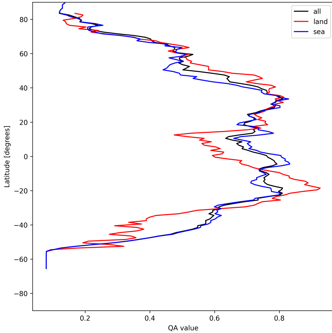
Figure 18: Zonal average of “QA value” for 2025-07-27 to 2025-07-27.
