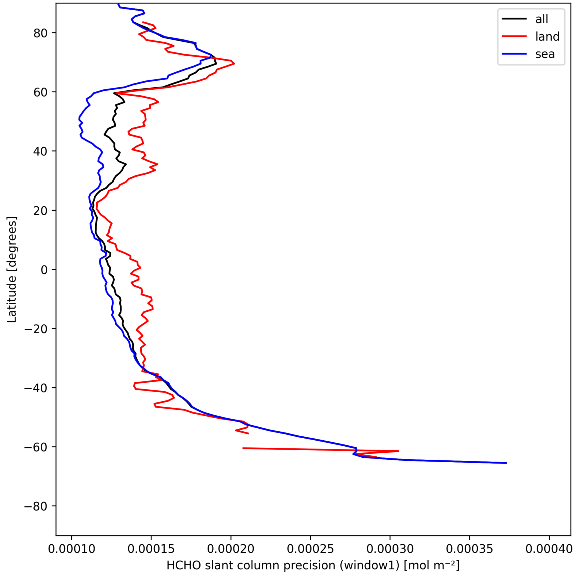
Figure 23: Zonal average of “HCHO slant column precision (window1)” for 2025-07-27 to 2025-07-27.
