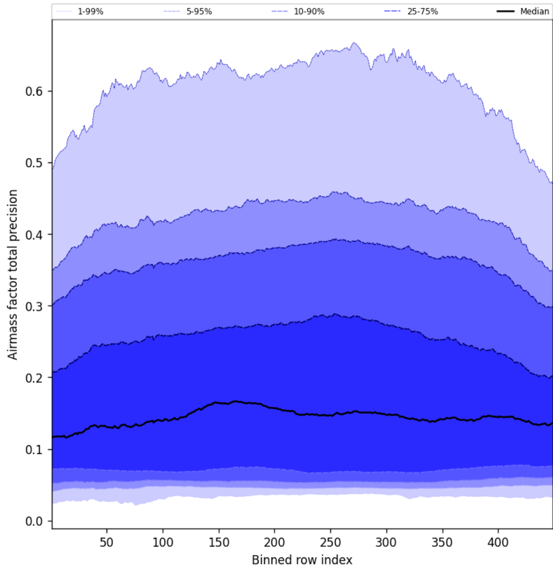
Figure 53: Along track statistics of “Airmass factor total precision” for 2025-07-27 to 2025-07-27
