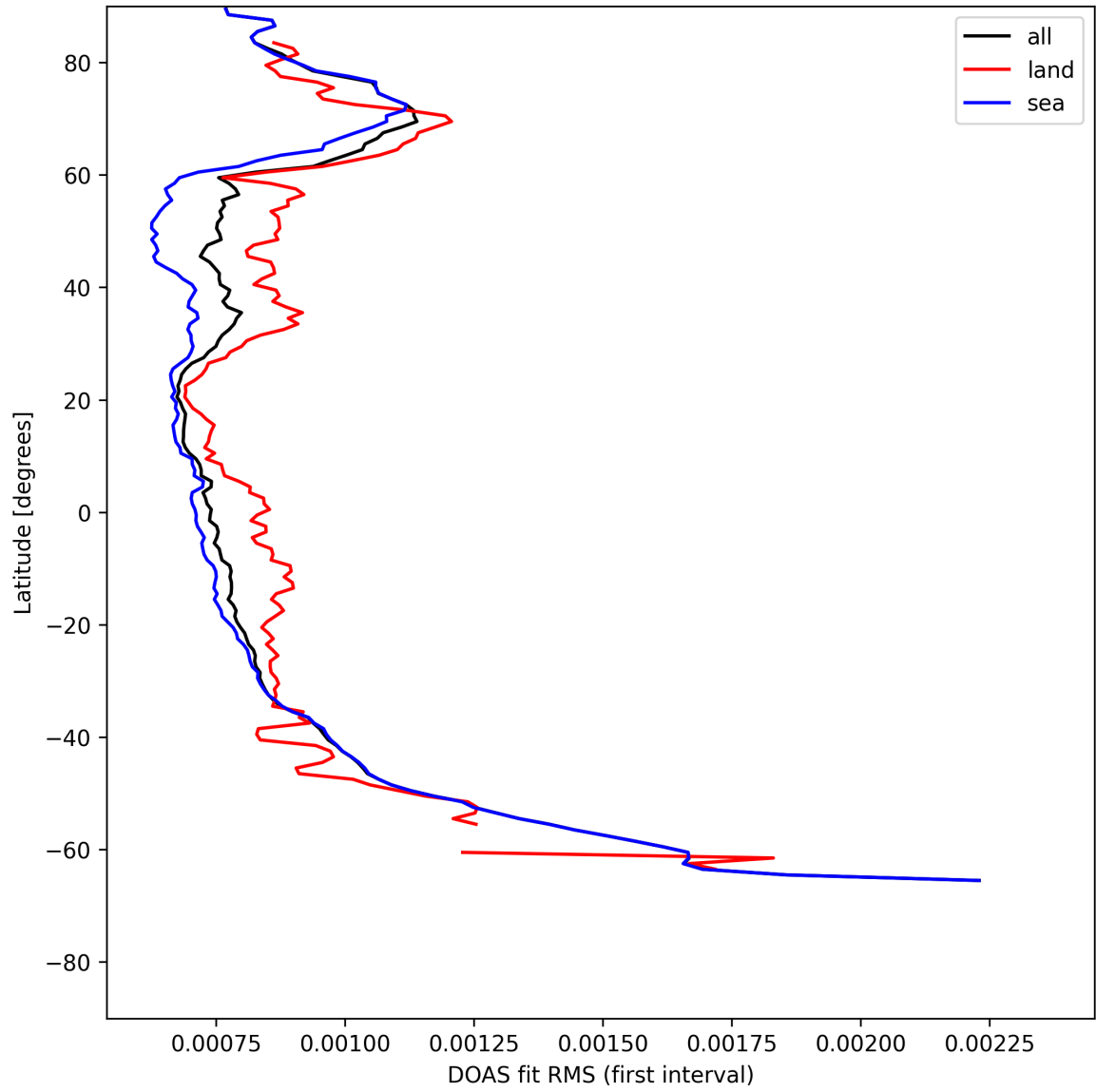
Figure 30: Zonal average of “DOAS fit RMS (first interval)” for 2025-07-27 to 2025-07-27.
