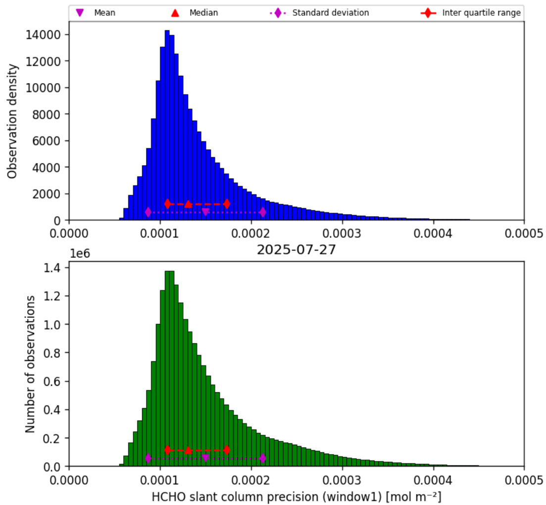
Figure 37: Histogram of “HCHO slant column precision (window1)” for 2025-07-27 to 2025-07-27
