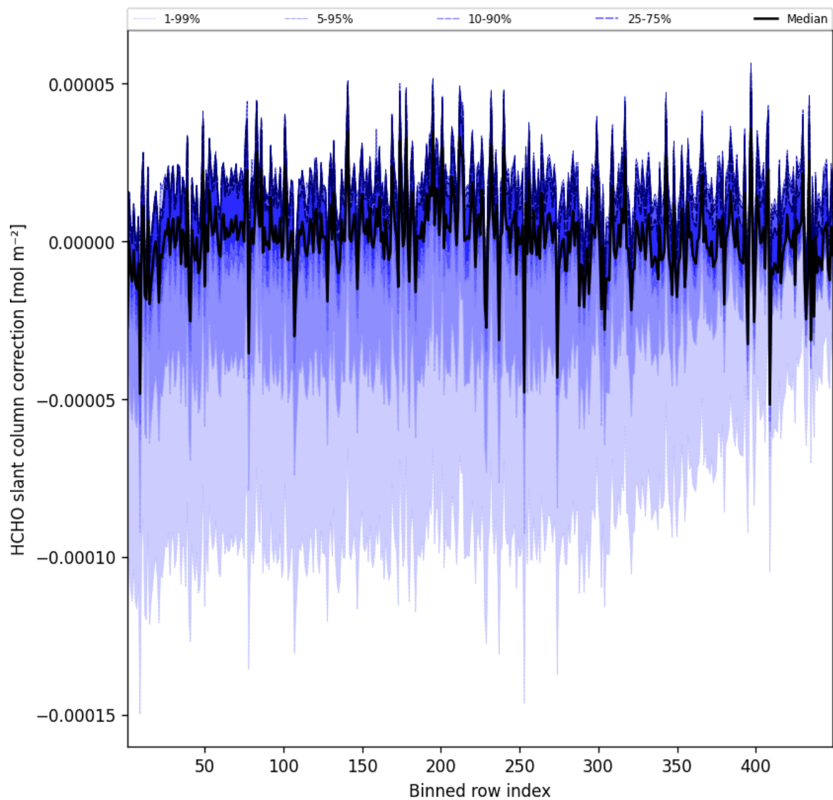
Figure 59: Along track statistics of “HCHO slant column correction” for 2025-07-27 to 2025-07-27
