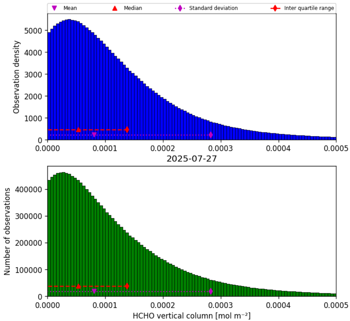
Figure 33: Histogram of “HCHO vertical column” for 2025-07-27 to 2025-07-27
