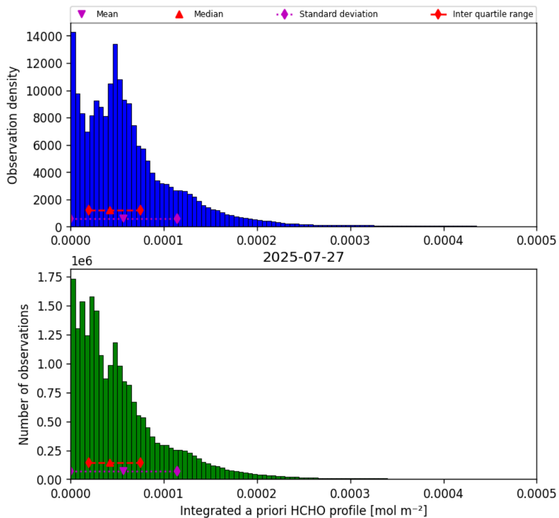
Figure 41: Histogram of “Integrated a priori HCHO profile” for 2025-07-27 to 2025-07-27
