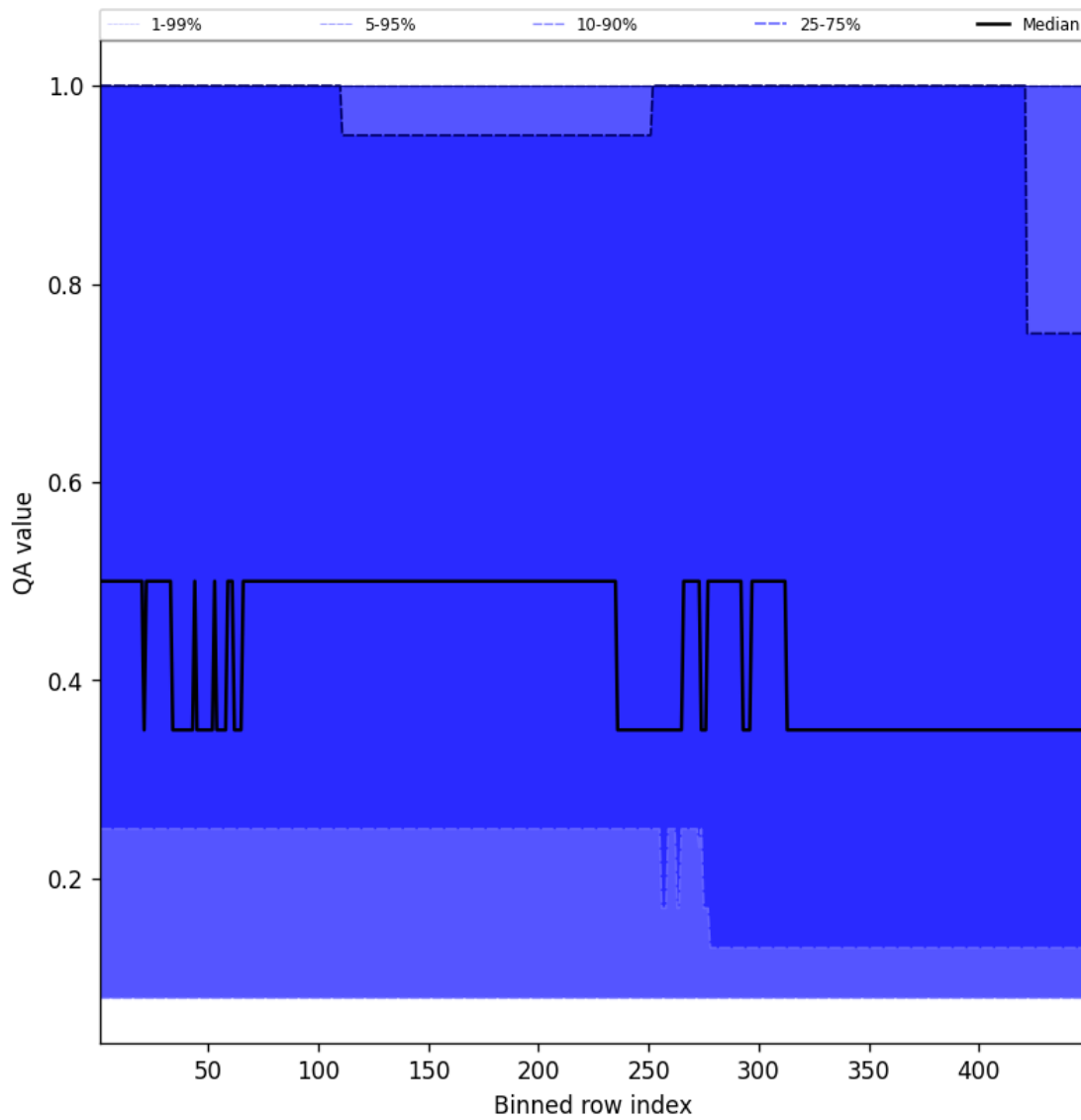
Figure 46: Along track statistics of “QA value” for 2025-07-27 to 2025-07-27
