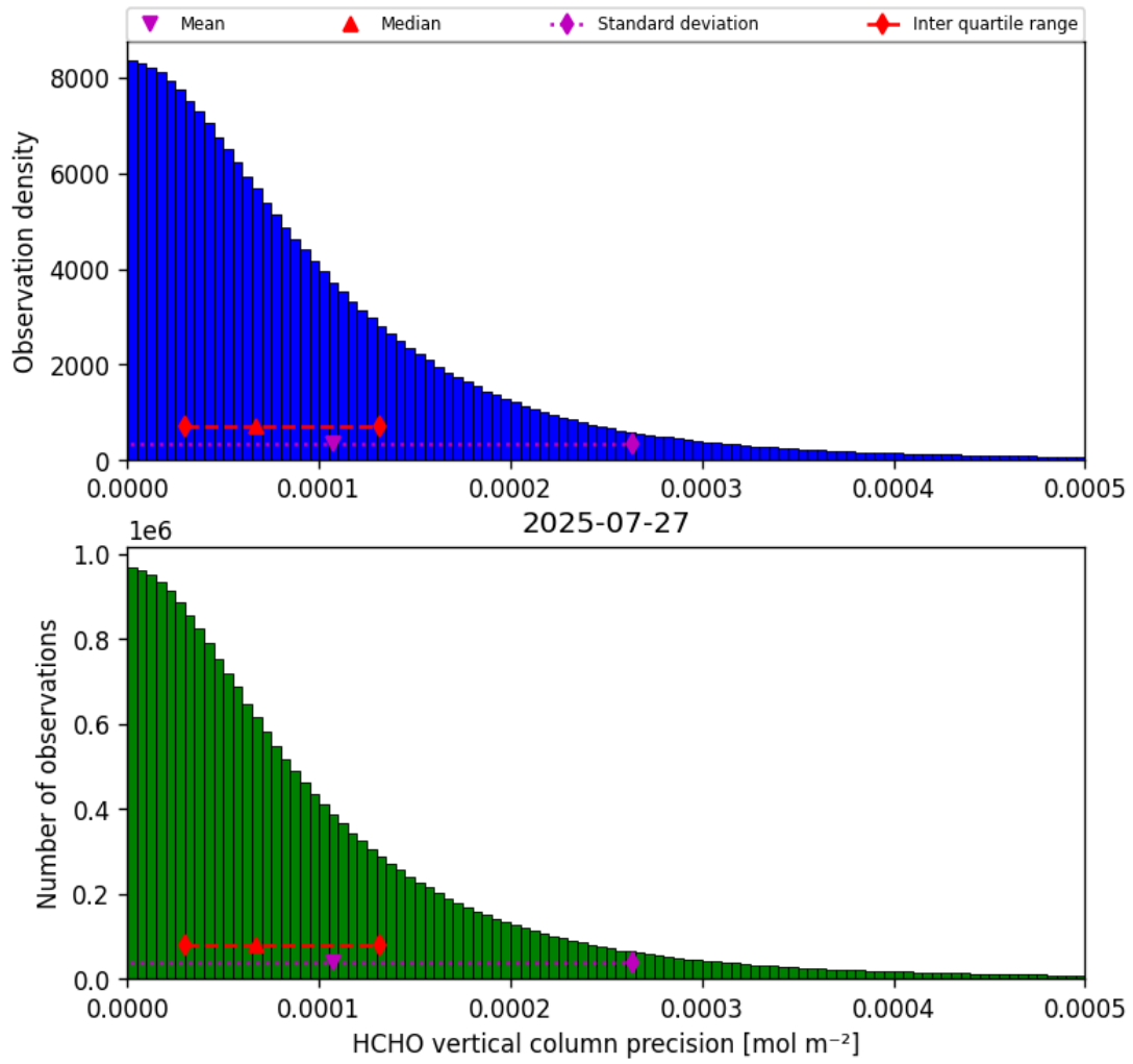
Figure 34: Histogram of “HCHO vertical column precision” for 2025-07-27 to 2025-07-27
