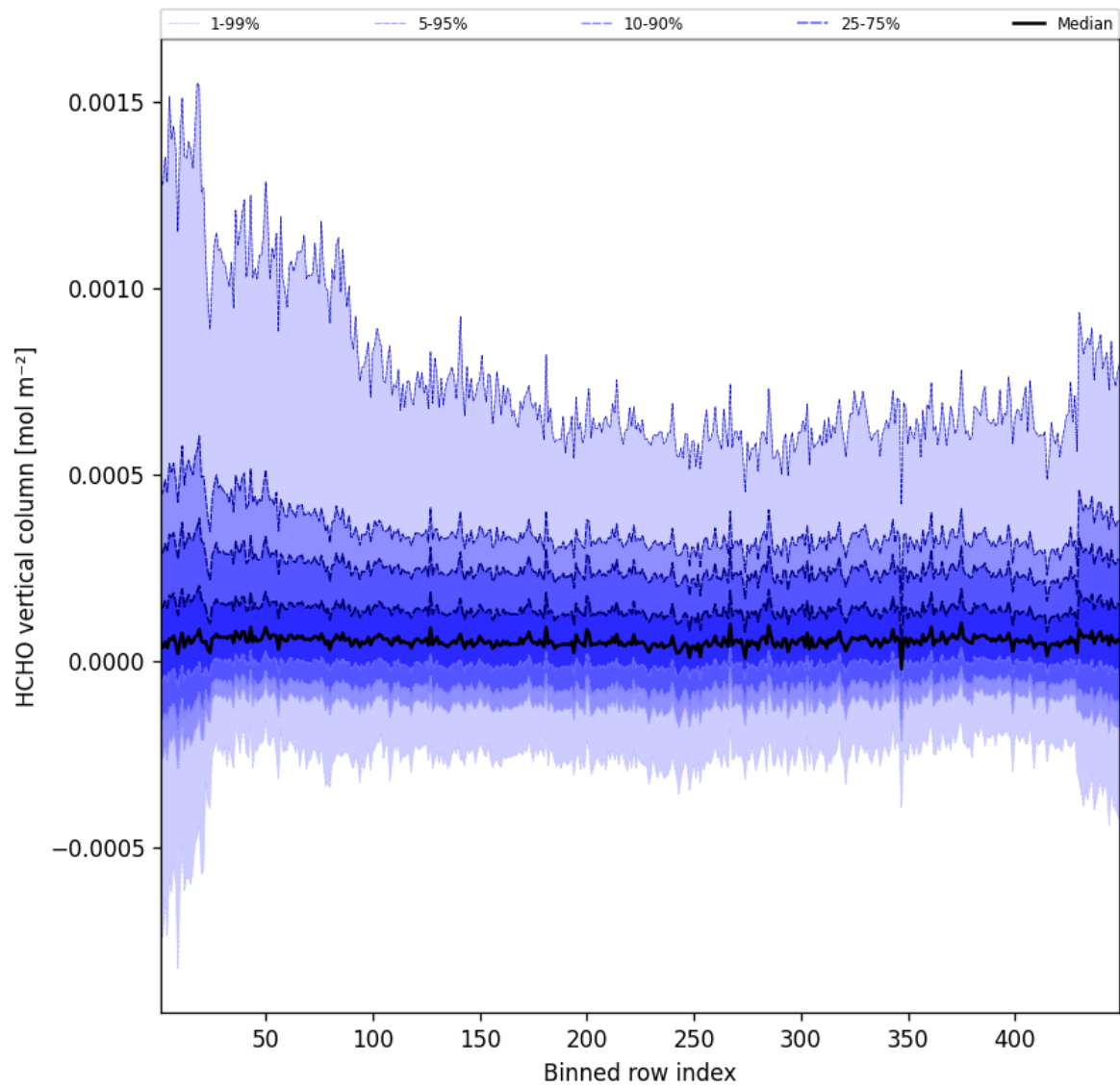
Figure 47: Along track statistics of “HCHO vertical column” for 2025-07-27 to 2025-07-27
