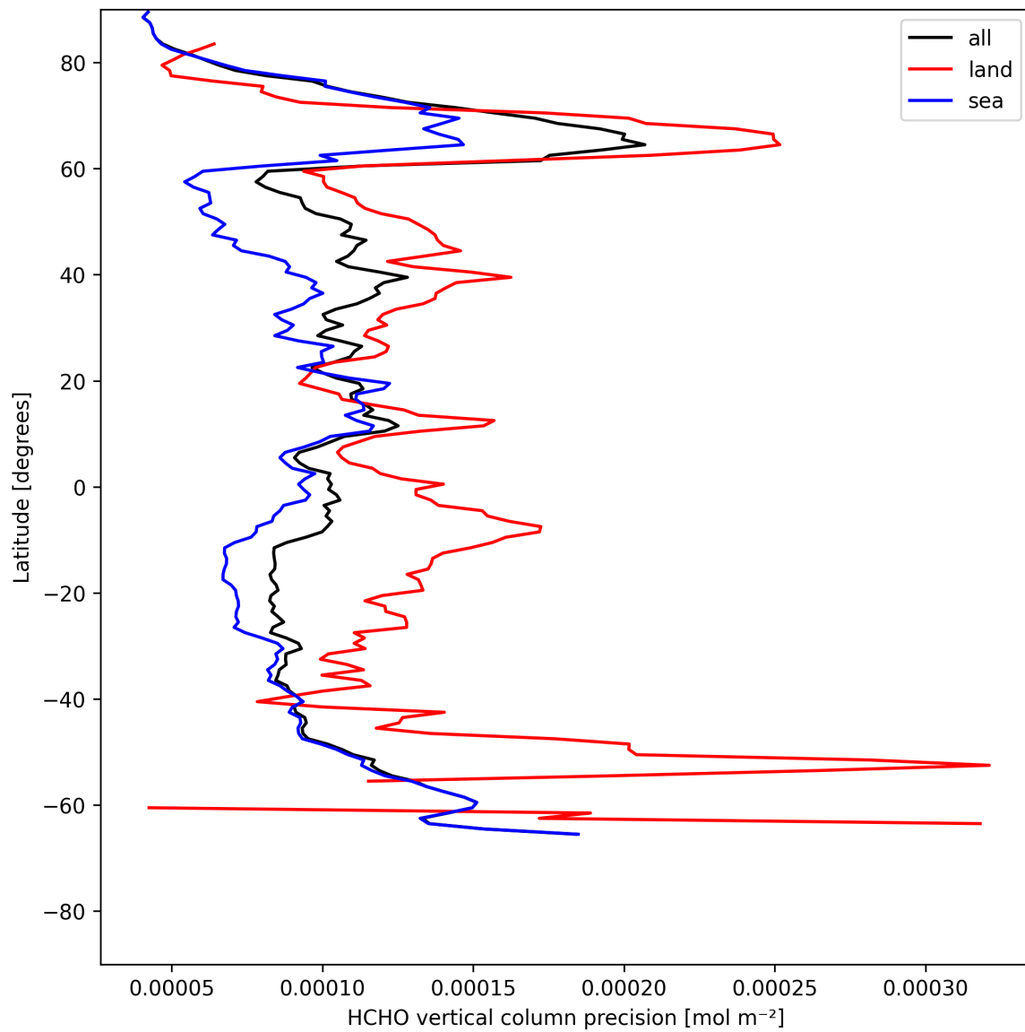
Figure 20: Zonal average of “HCHO vertical column precision” for 2025-07-27 to 2025-07-27.
