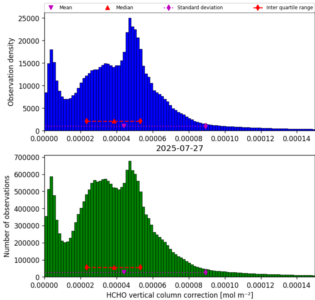
Figure 35: Histogram of “HCHO vertical column correction” for 2025-07-27 to 2025-07-27
