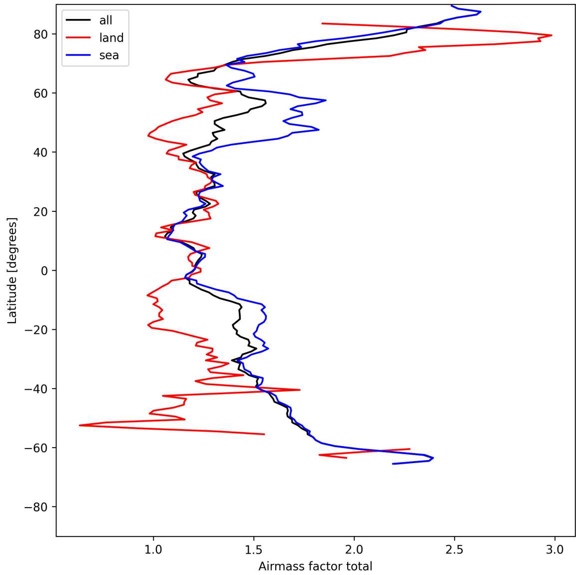
Figure 24: Zonal average of “Airmass factor total” for 2025-07-27 to 2025-07-27.
