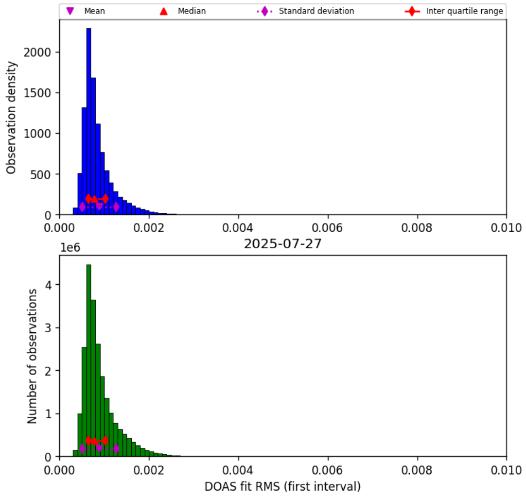
Figure 44: Histogram of “DOAS fit RMS (first interval)” for 2025-07-27 to 2025-07-27
