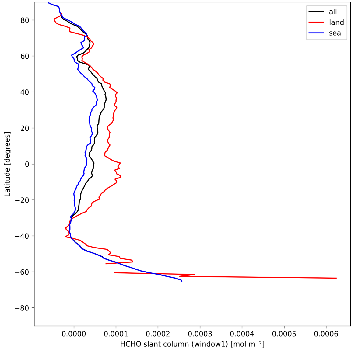
Figure 22: Zonal average of “HCHO slant column (window1)” for 2025-07-27 to 2025-07-27.
