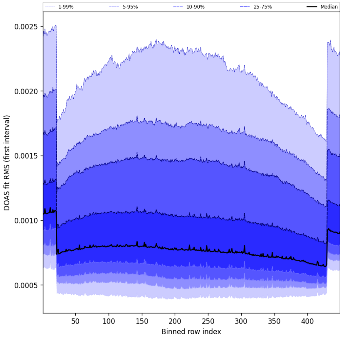
Figure 58: Along track statistics of “DOAS fit RMS (first interval)” for 2025-07-27 to 2025-07-27
