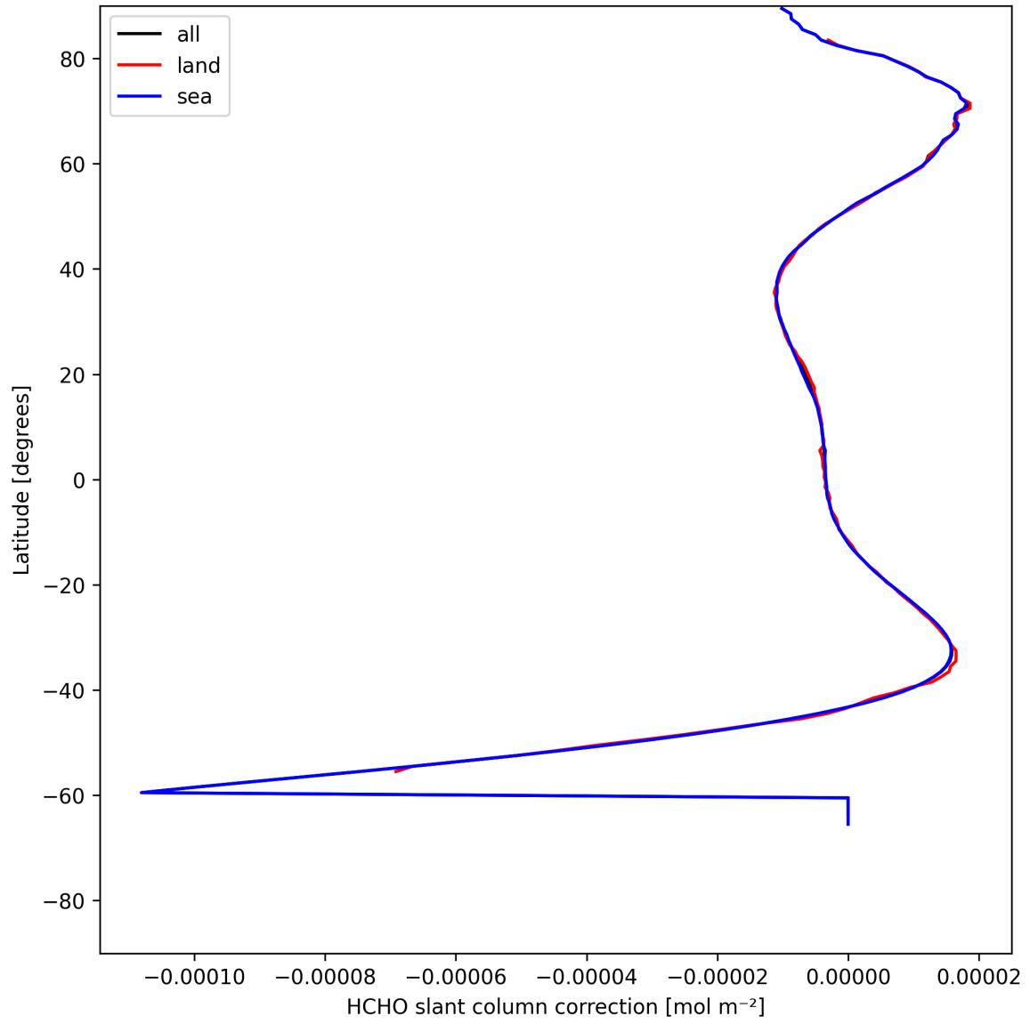
Figure 31: Zonal average of “HCHO slant column correction” for 2025-07-27 to 2025-07-27.
