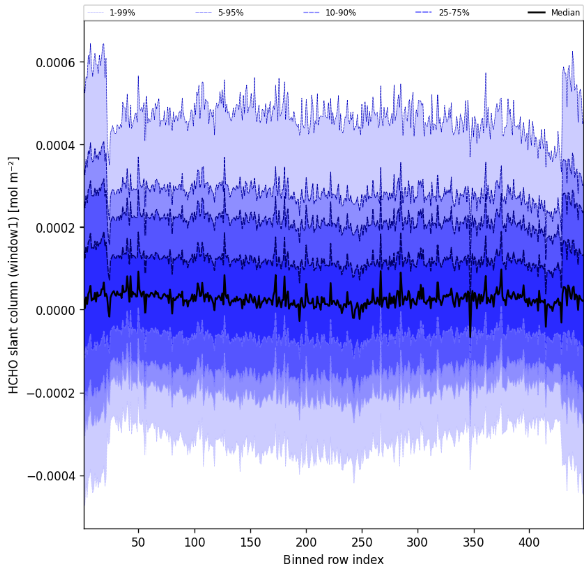
Figure 50: Along track statistics of “HCHO slant column (window1)” for 2025-07-27 to 2025-07-27
