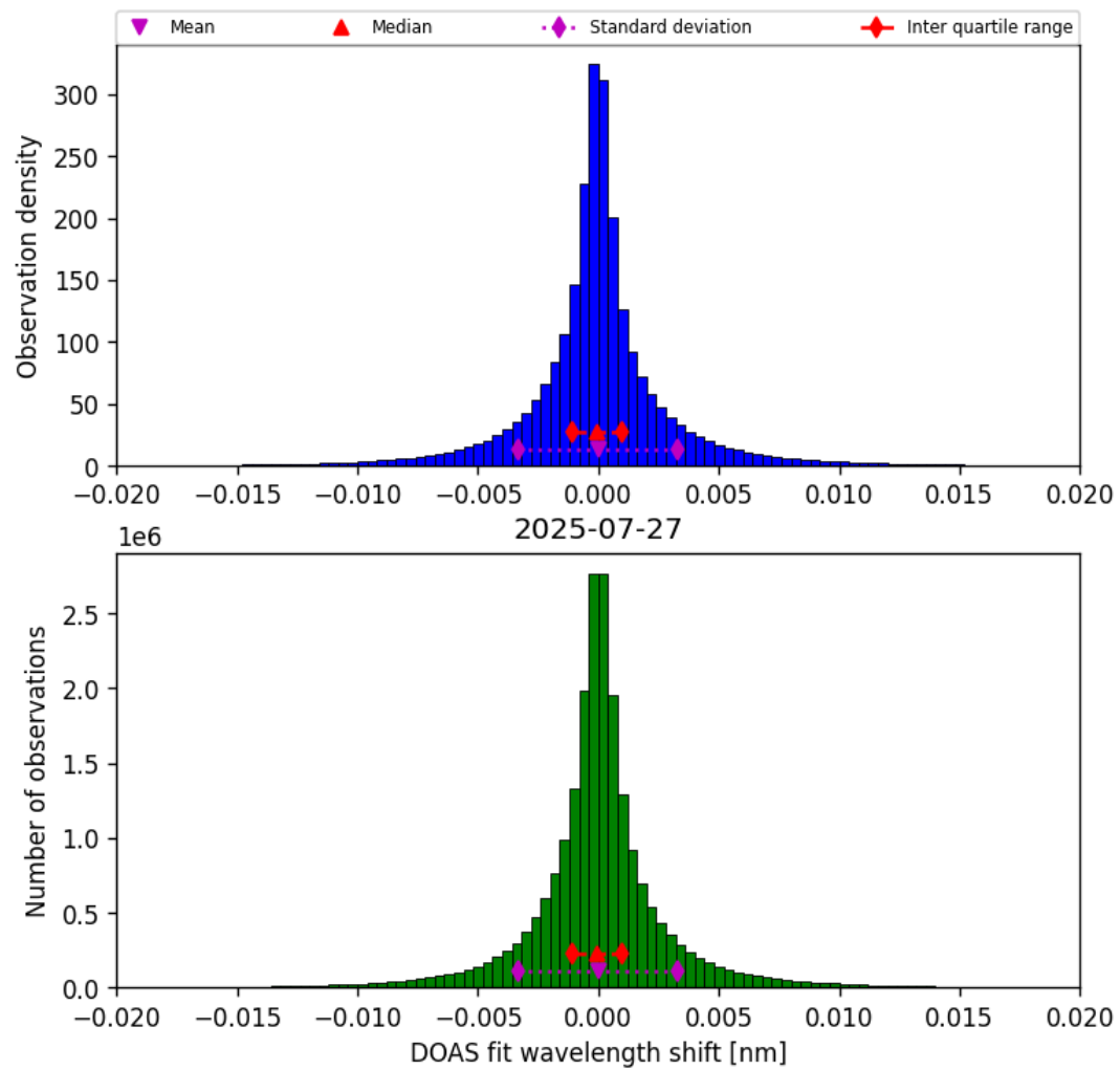
Figure 42: Histogram of “DOAS fit wavelength shift” for 2025-07-27 to 2025-07-27
