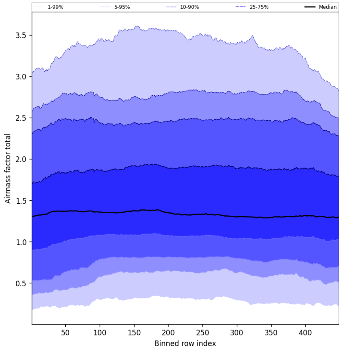
Figure 52: Along track statistics of “Airmass factor total” for 2025-07-27 to 2025-07-27
