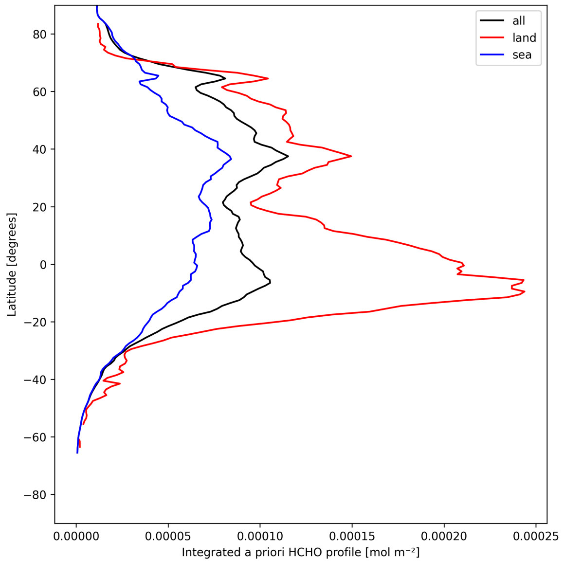
Figure 27: Zonal average of “Integrated a priori HCHO profile” for 2025-07-27 to 2025-07-27.
