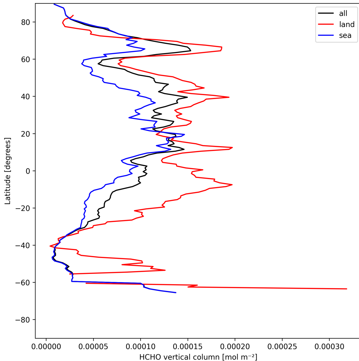
Figure 19: Zonal average of “HCHO vertical column” for 2025-07-27 to 2025-07-27.
