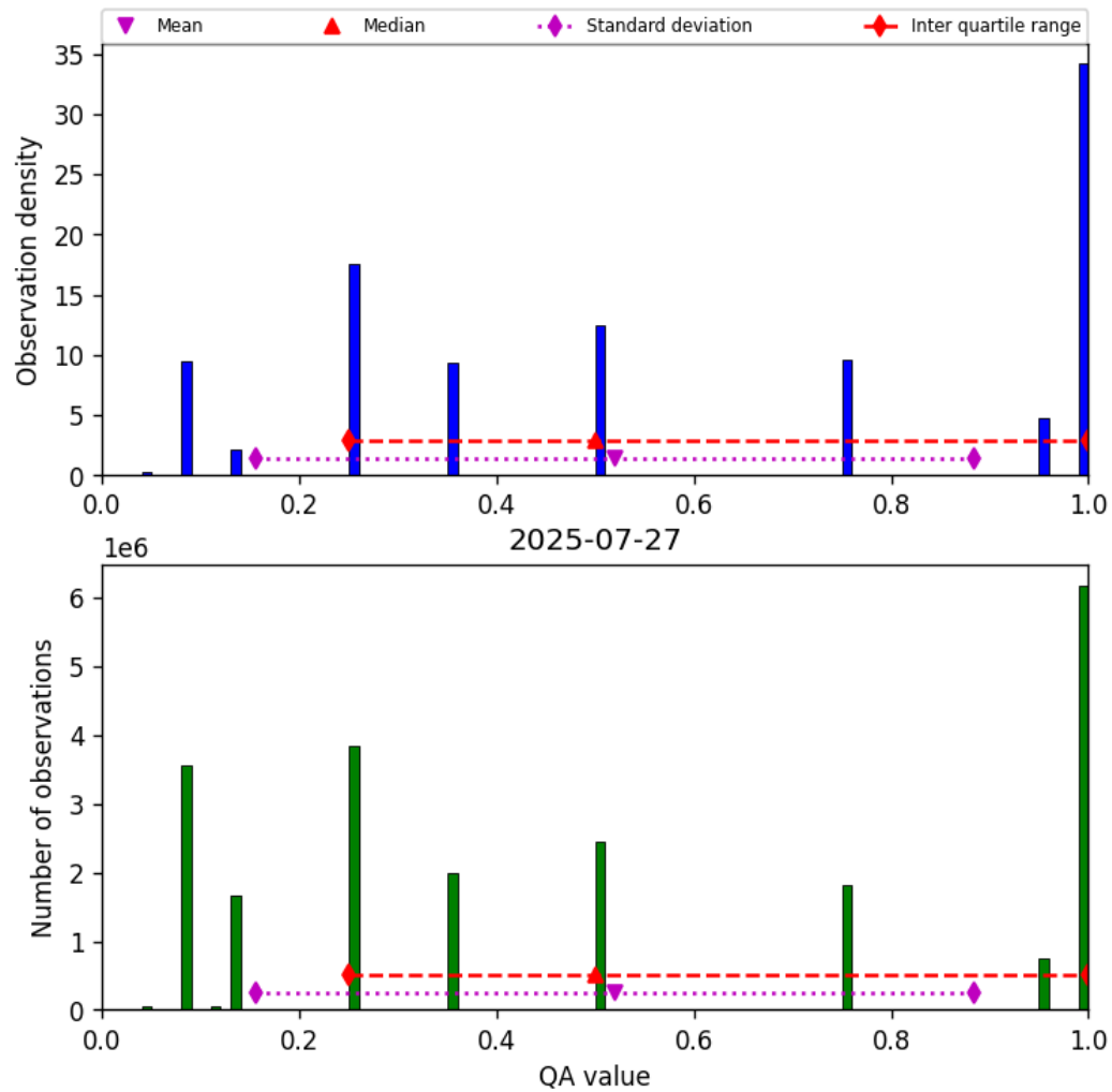
Figure 32: Histogram of “QA value” for 2025-07-27 to 2025-07-27
