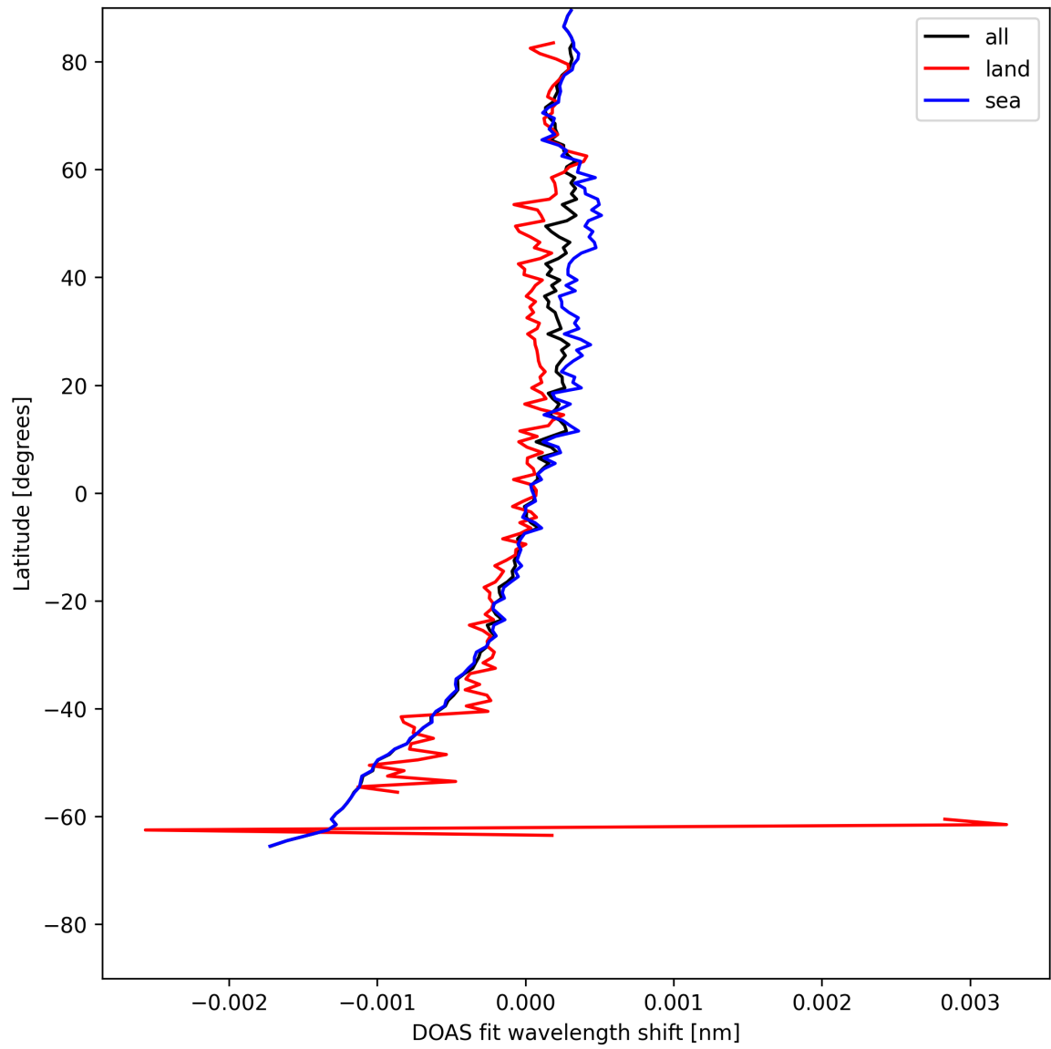
Figure 28: Zonal average of “DOAS fit wavelength shift” for 2025-07-27 to 2025-07-27.
