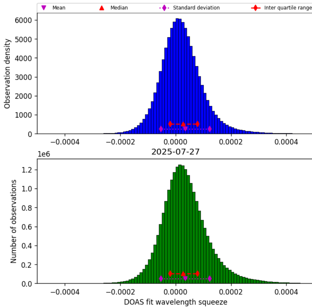
Figure 43: Histogram of “DOAS fit wavelength squeeze” for 2025-07-27 to 2025-07-27
