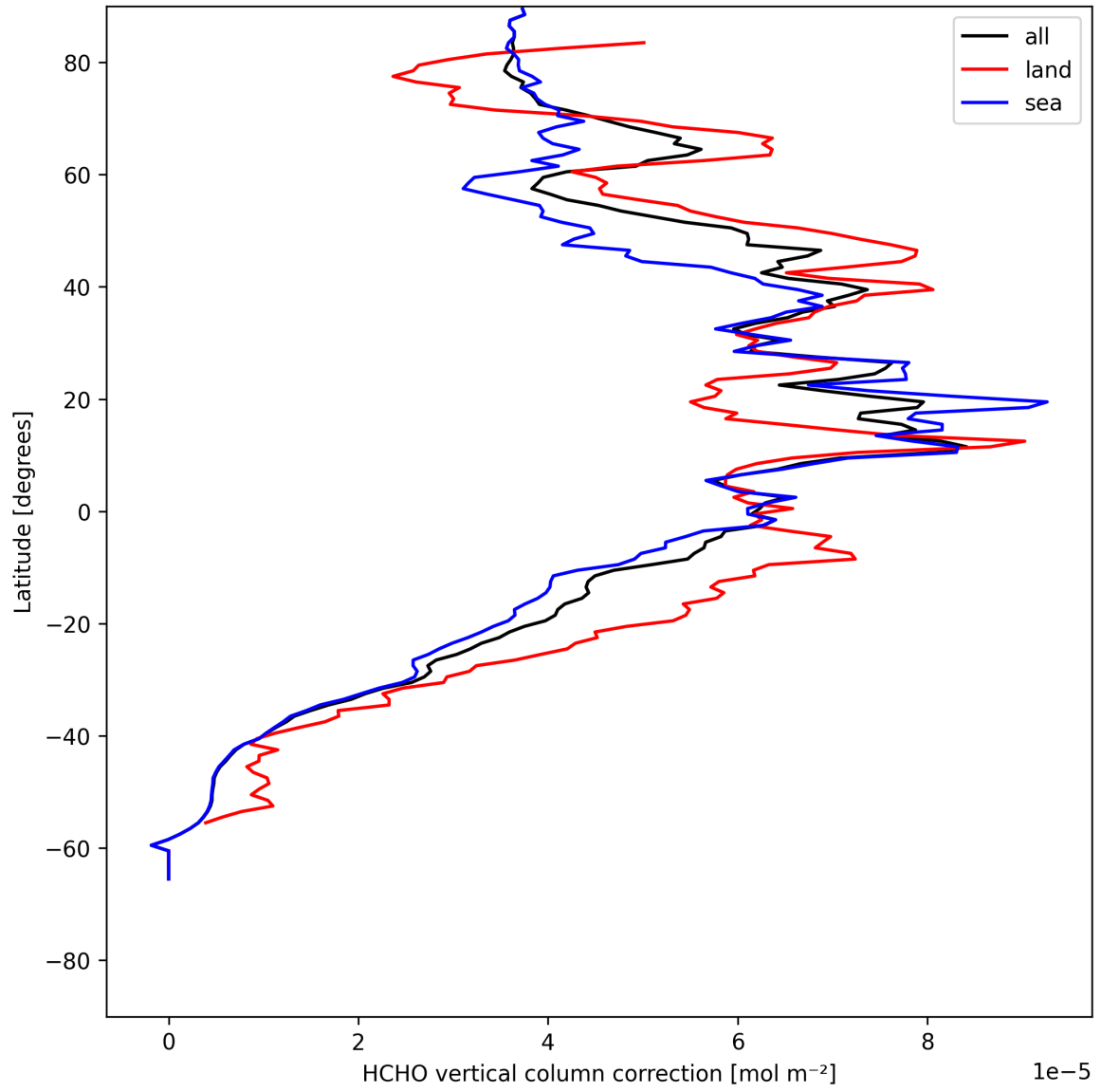
Figure 21: Zonal average of “HCHO vertical column correction” for 2025-07-27 to 2025-07-27.
