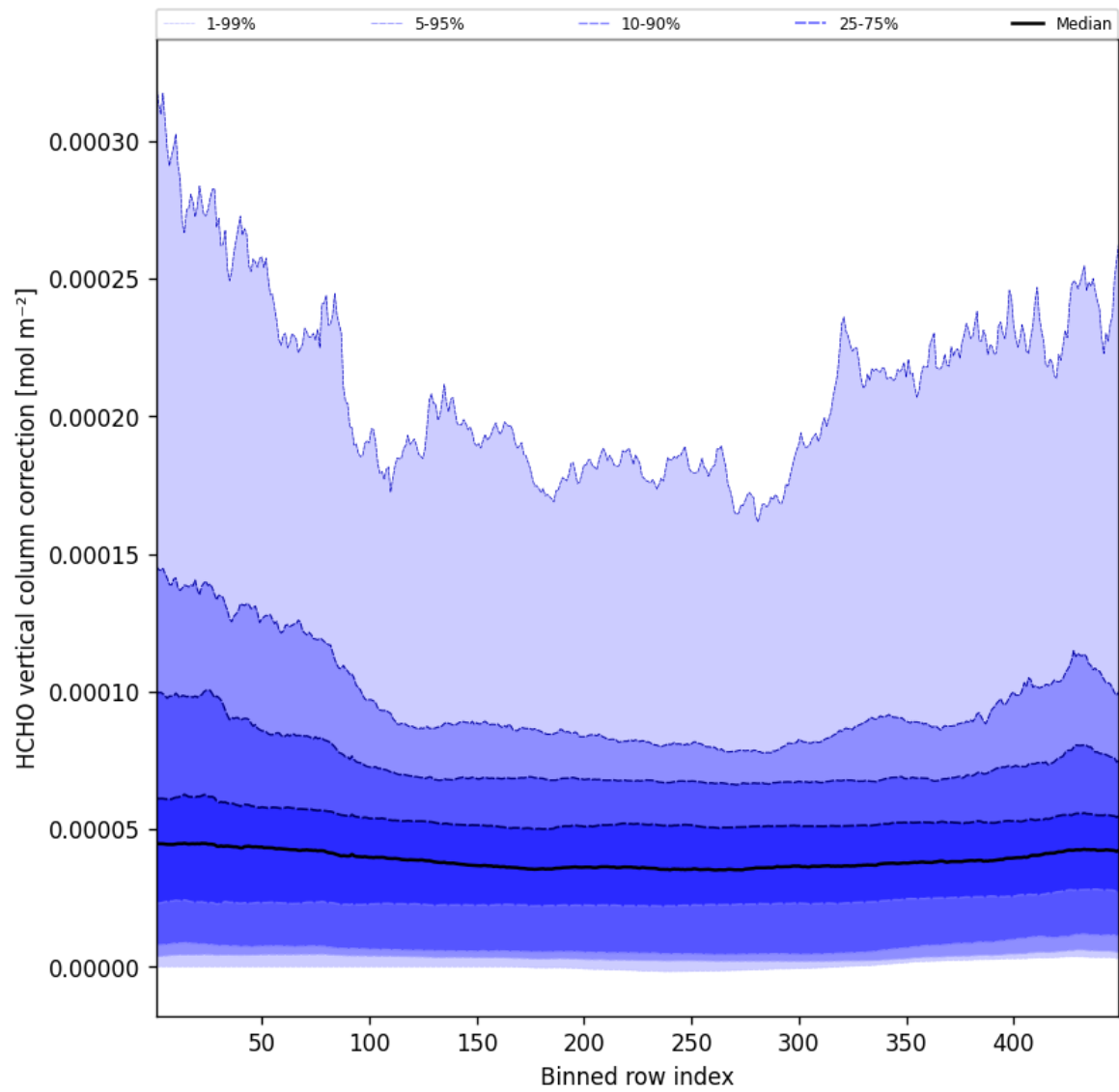
Figure 49: Along track statistics of “HCHO vertical column correction” for 2025-07-27 to 2025-07-27
