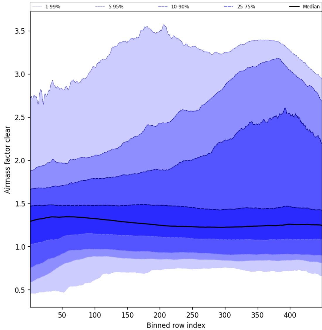
Figure 54: Along track statistics of “Airmass factor clear” for 2025-07-27 to 2025-07-27
