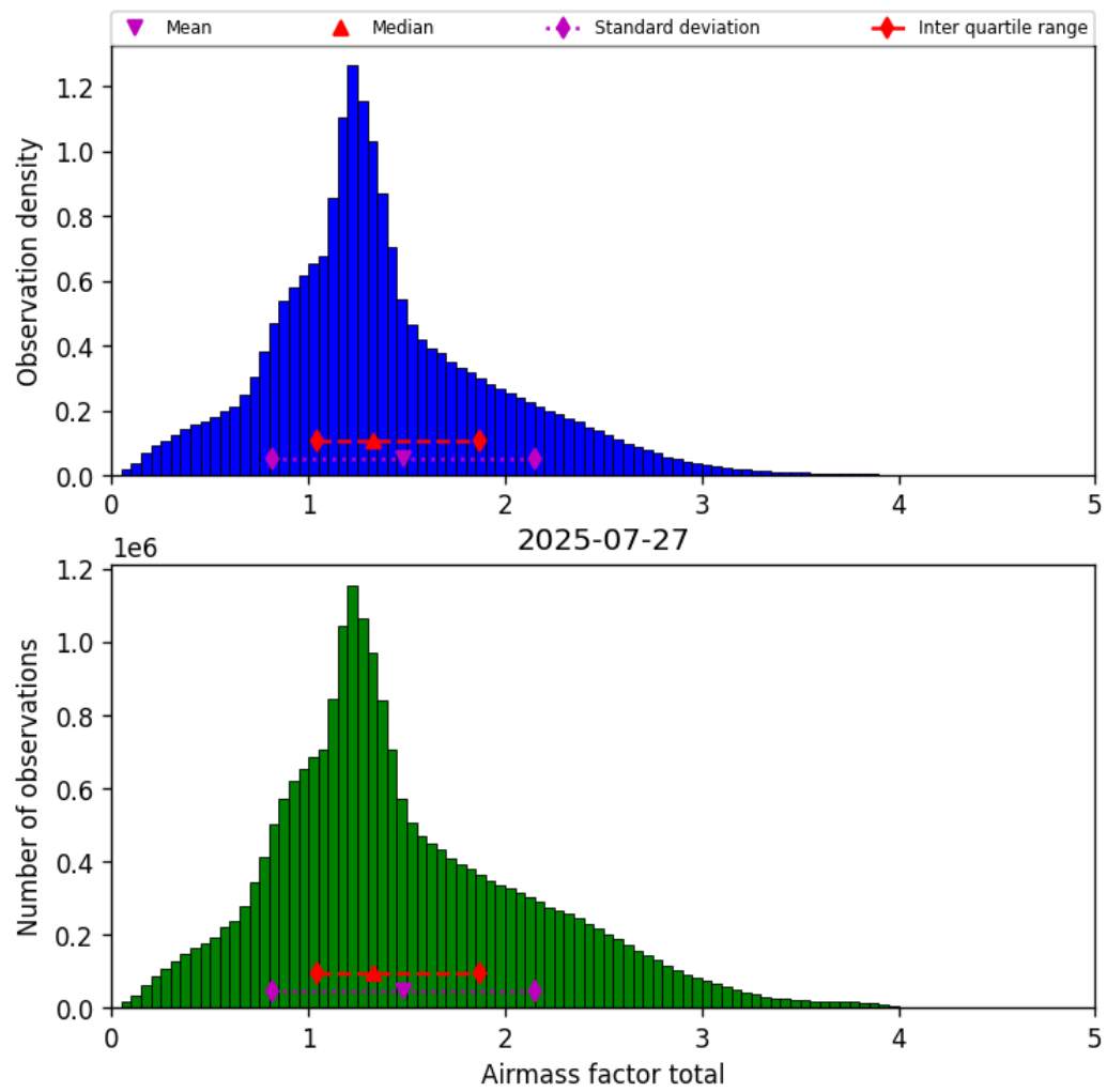
Figure 38: Histogram of “Airmass factor total” for 2025-07-27 to 2025-07-27
