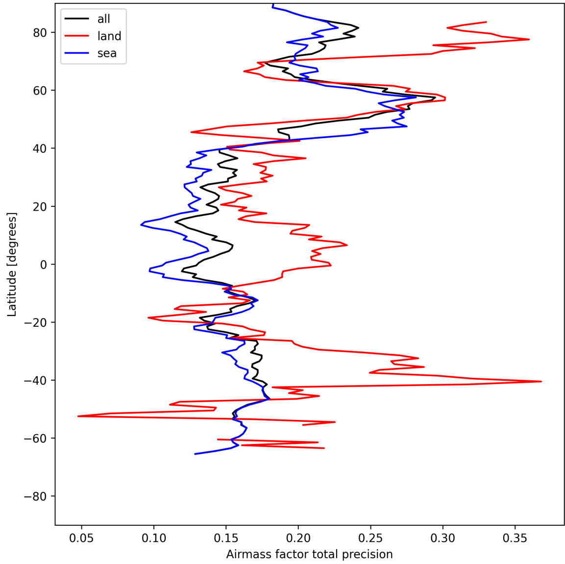
Figure 25: Zonal average of “Airmass factor total precision” for 2025-07-27 to 2025-07-27.
