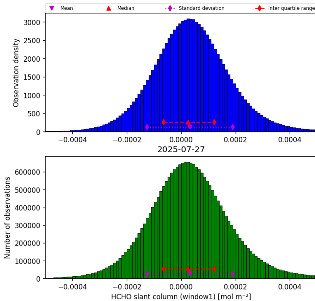
Figure 36: Histogram of “HCHO slant column (window1)” for 2025-07-27 to 2025-07-27
