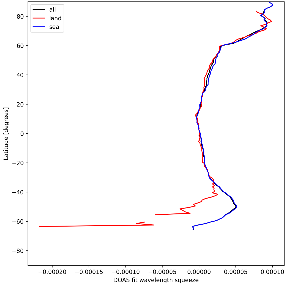
Figure 29: Zonal average of “DOAS fit wavelength squeeze” for 2025-07-27 to 2025-07-27.
