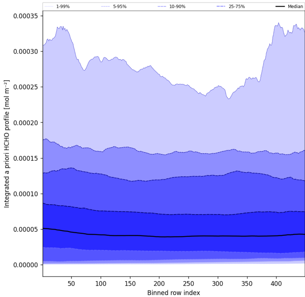
Figure 55: Along track statistics of “Integrated a priori HCHO profile” for 2025-07-27 to 2025-07-27
