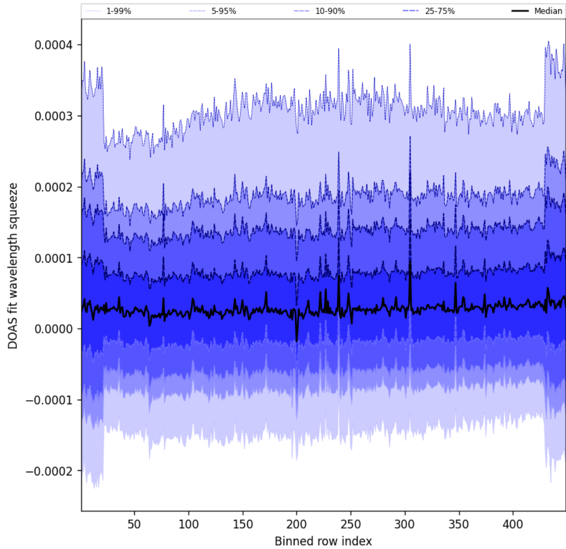
Figure 57: Along track statistics of “DOAS fit wavelength squeeze” for 2025-07-27 to 2025-07-27
