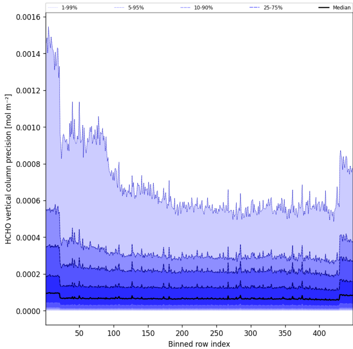
Figure 48: Along track statistics of “HCHO vertical column precision” for 2025-07-27 to 2025-07-27
