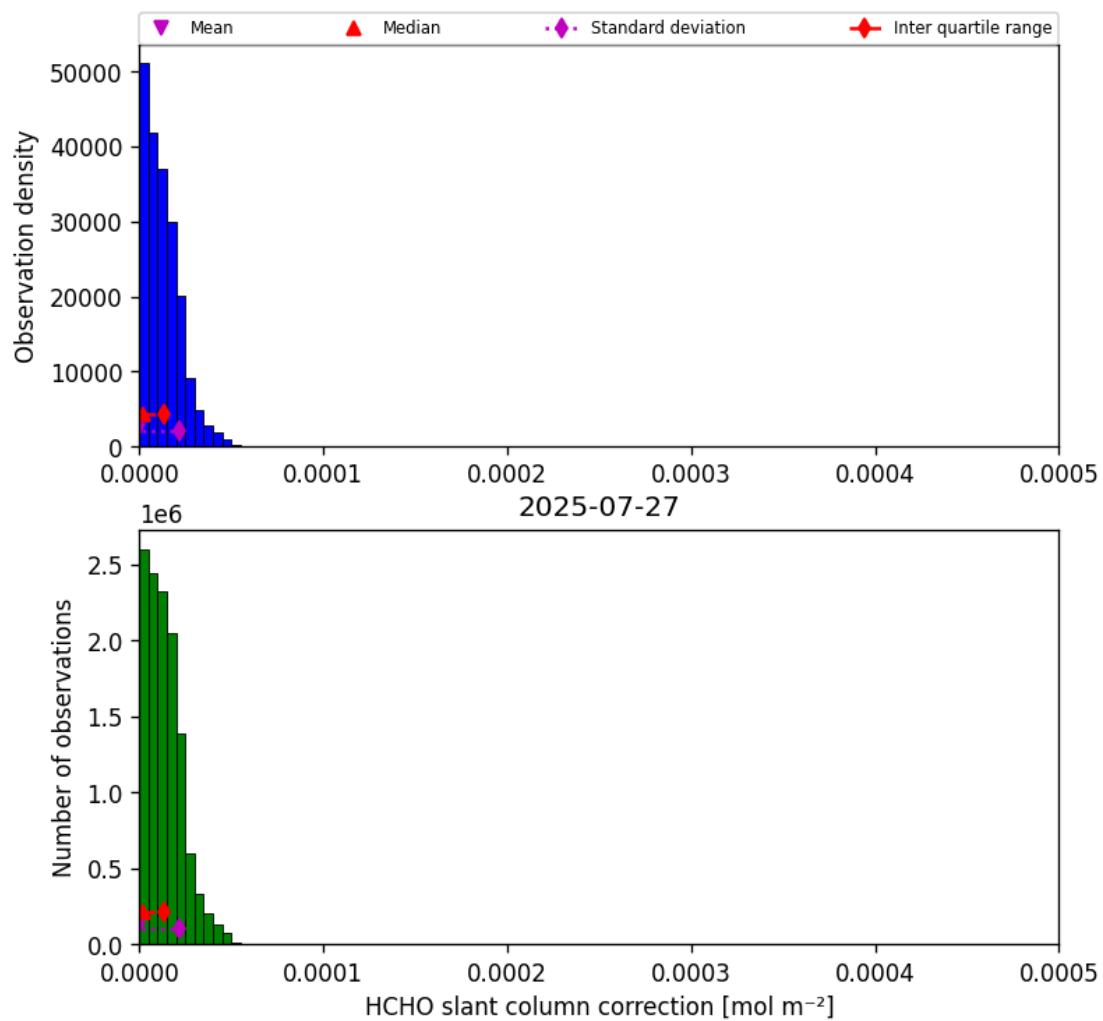
Figure 45: Histogram of “HCHO slant column correction” for 2025-07-27 to 2025-07-27
