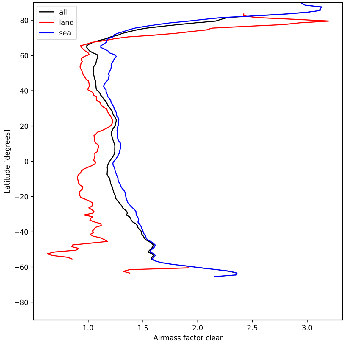
Figure 26: Zonal average of “Airmass factor clear” for 2025-07-27 to 2025-07-27.
