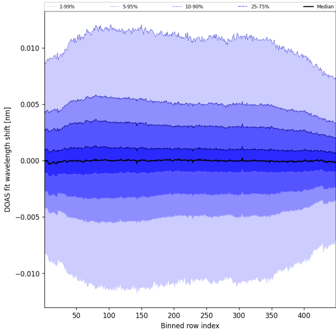
Figure 56: Along track statistics of “DOAS fit wavelength shift” for 2025-07-27 to 2025-07-27
