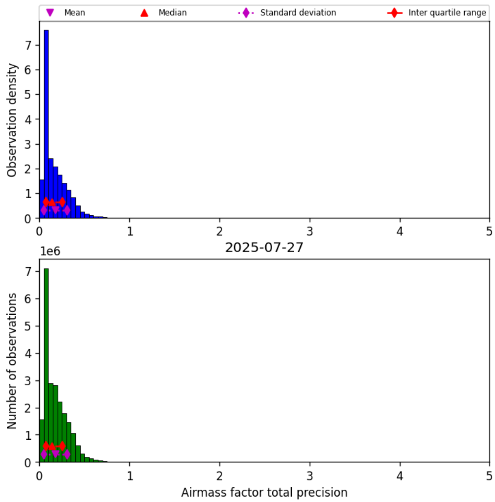
Figure 39: Histogram of “Airmass factor total precision” for 2025-07-27 to 2025-07-27
