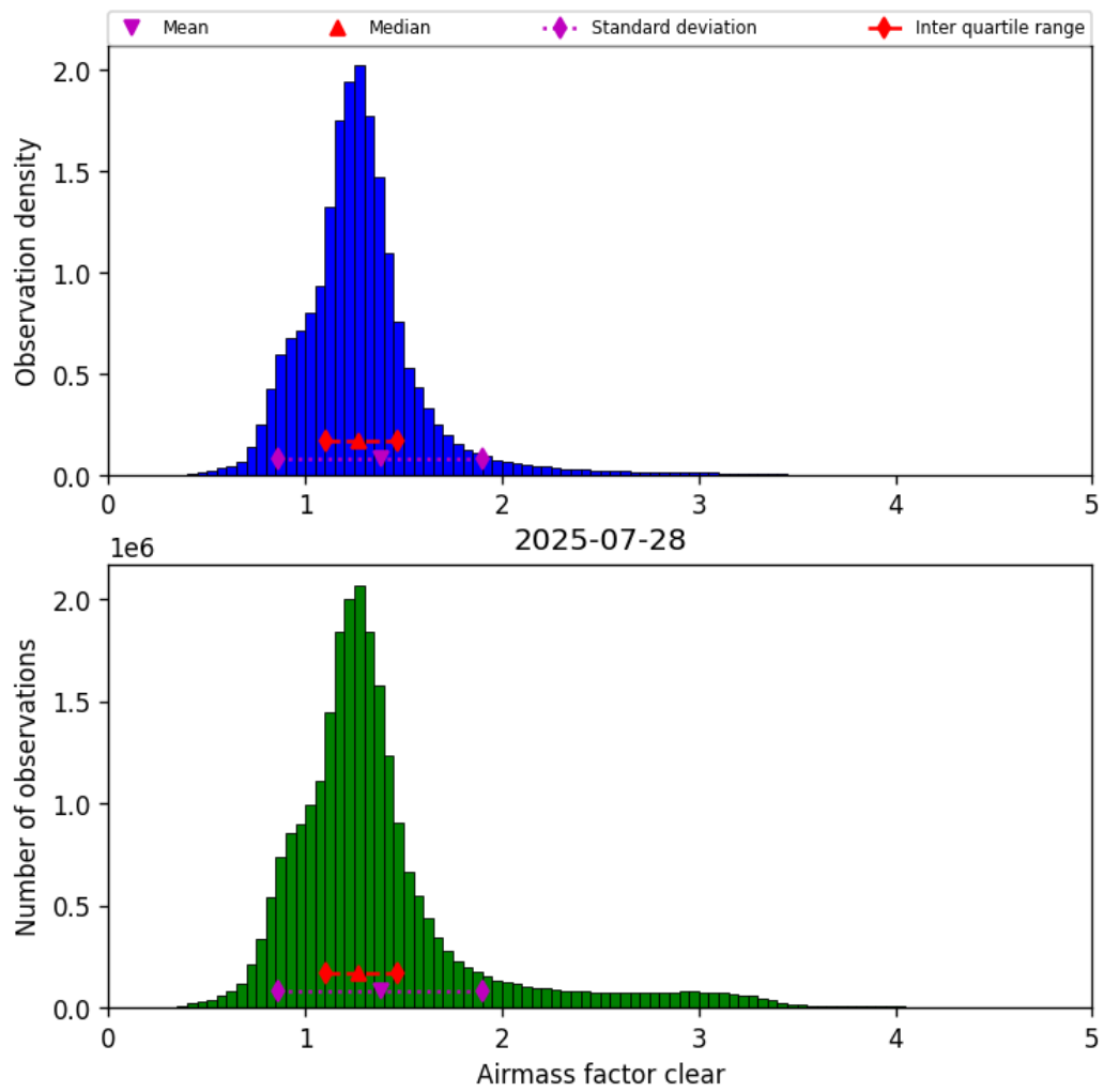
Figure 40: Histogram of “Airmass factor clear” for 2025-07-28 to 2025-07-29
