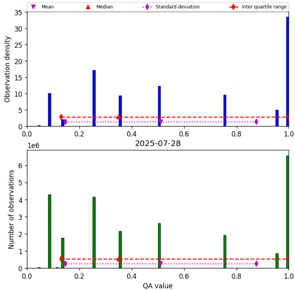
Figure 32: Histogram of “QA value” for 2025-07-28 to 2025-07-29
