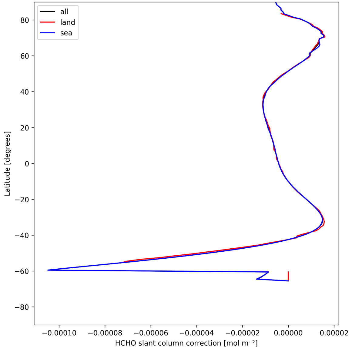
Figure 31: Zonal average of “HCHO slant column correction” for 2025-07-28 to 2025-07-29.
