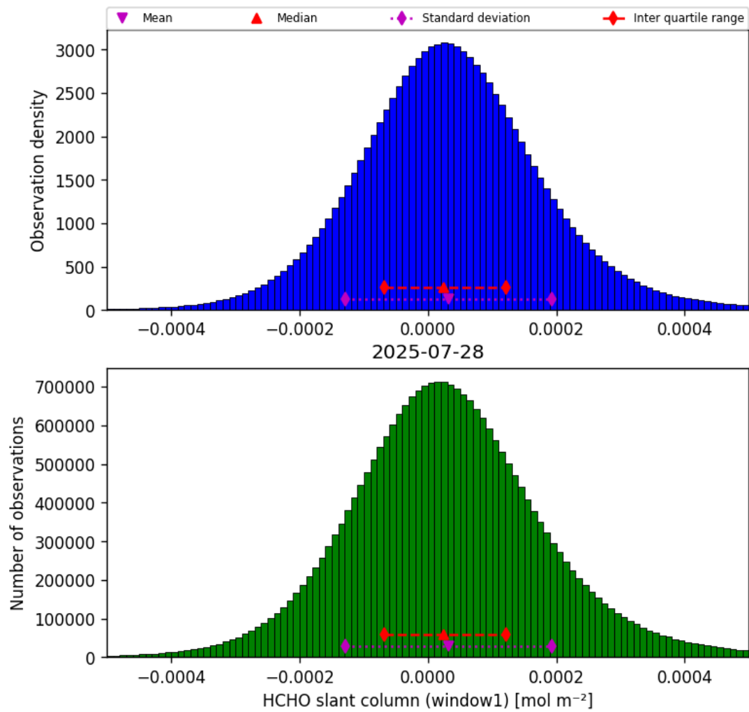
Figure 36: Histogram of “HCHO slant column (window1)” for 2025-07-28 to 2025-07-29
