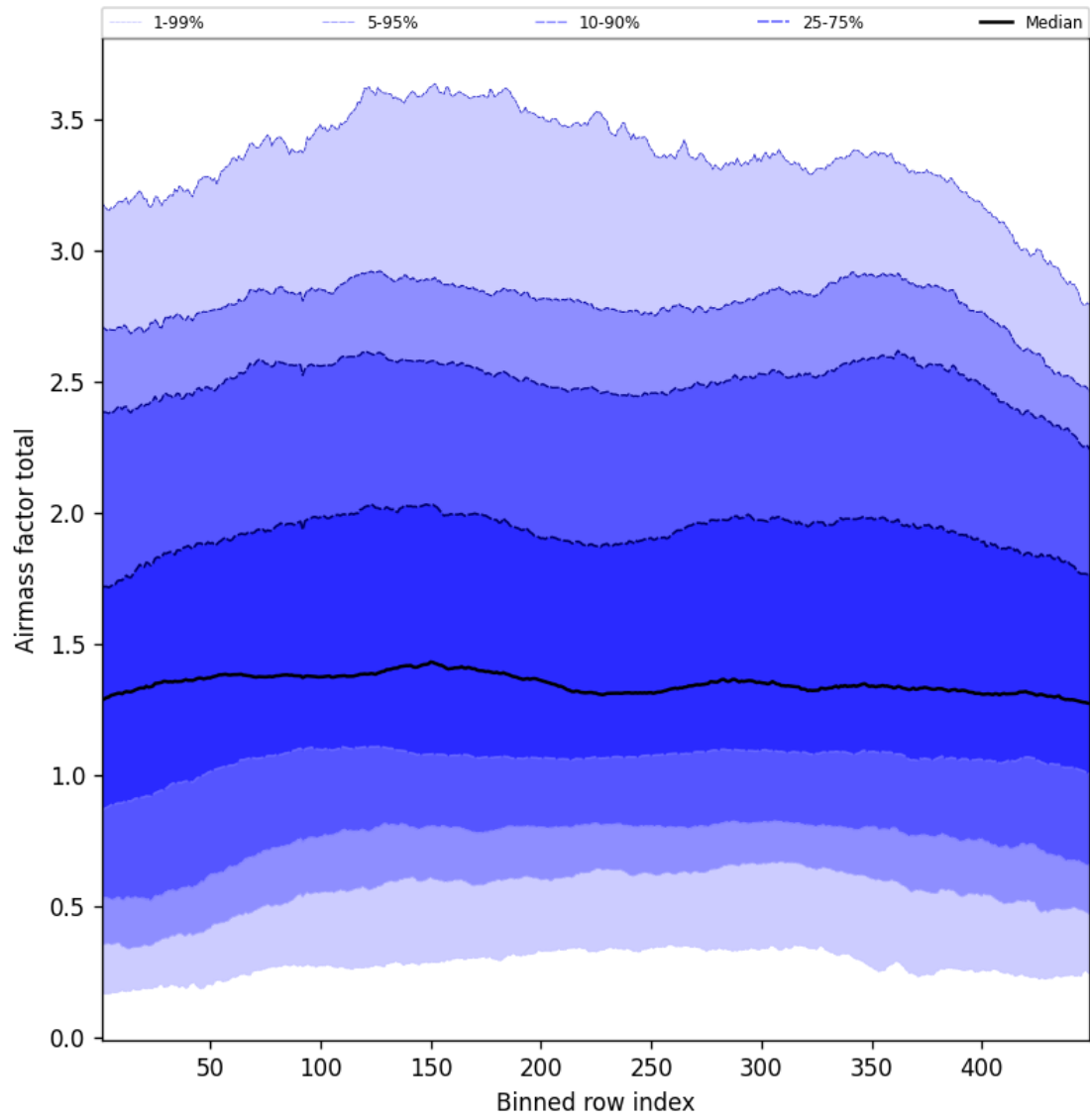
Figure 52: Along track statistics of “Airmass factor total” for 2025-07-28 to 2025-07-29
