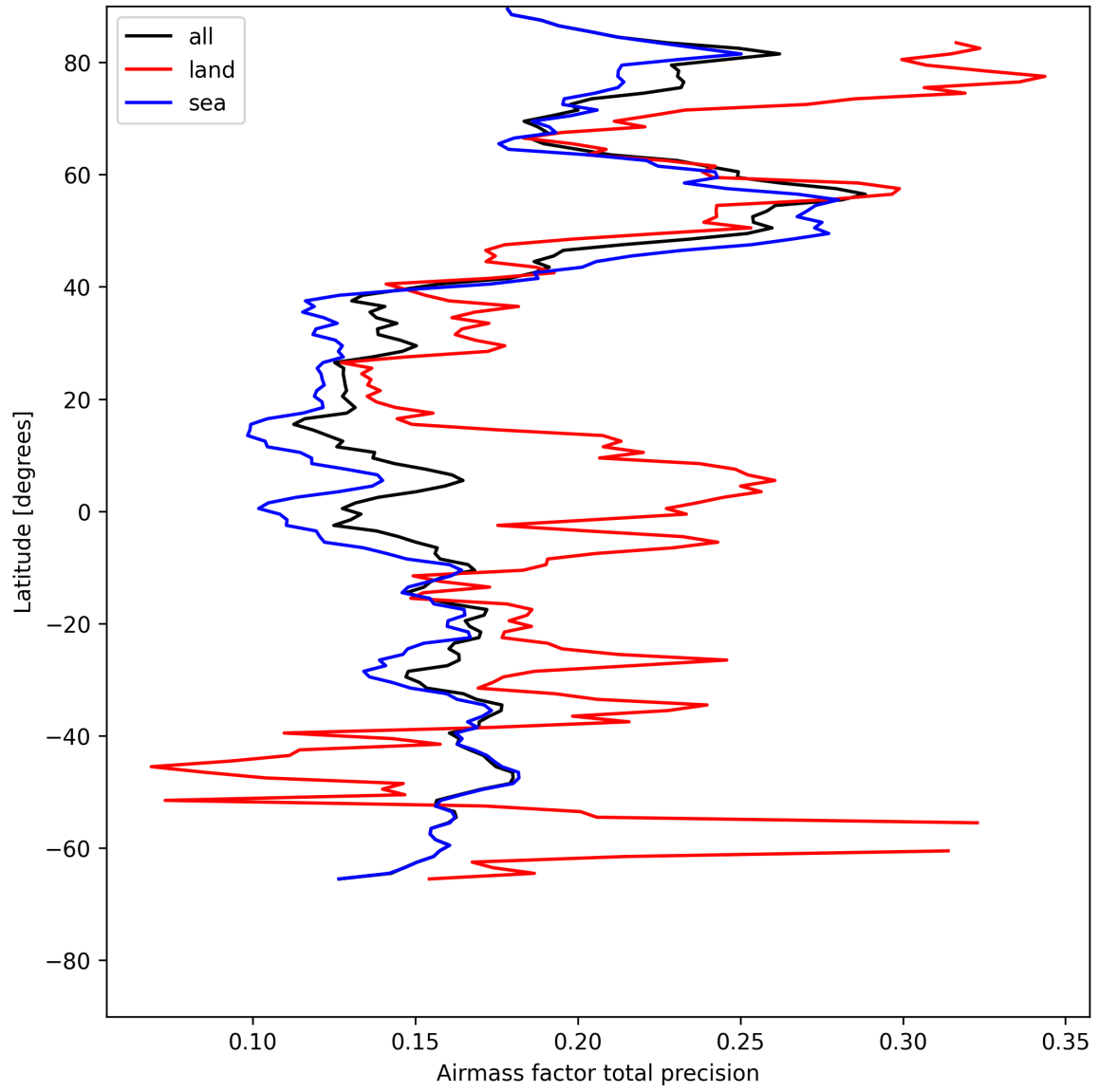
Figure 25: Zonal average of “Airmass factor total precision” for 2025-07-28 to 2025-07-29.
