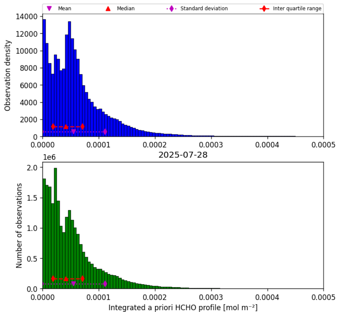
Figure 41: Histogram of “Integrated a priori HCHO profile” for 2025-07-28 to 2025-07-29
