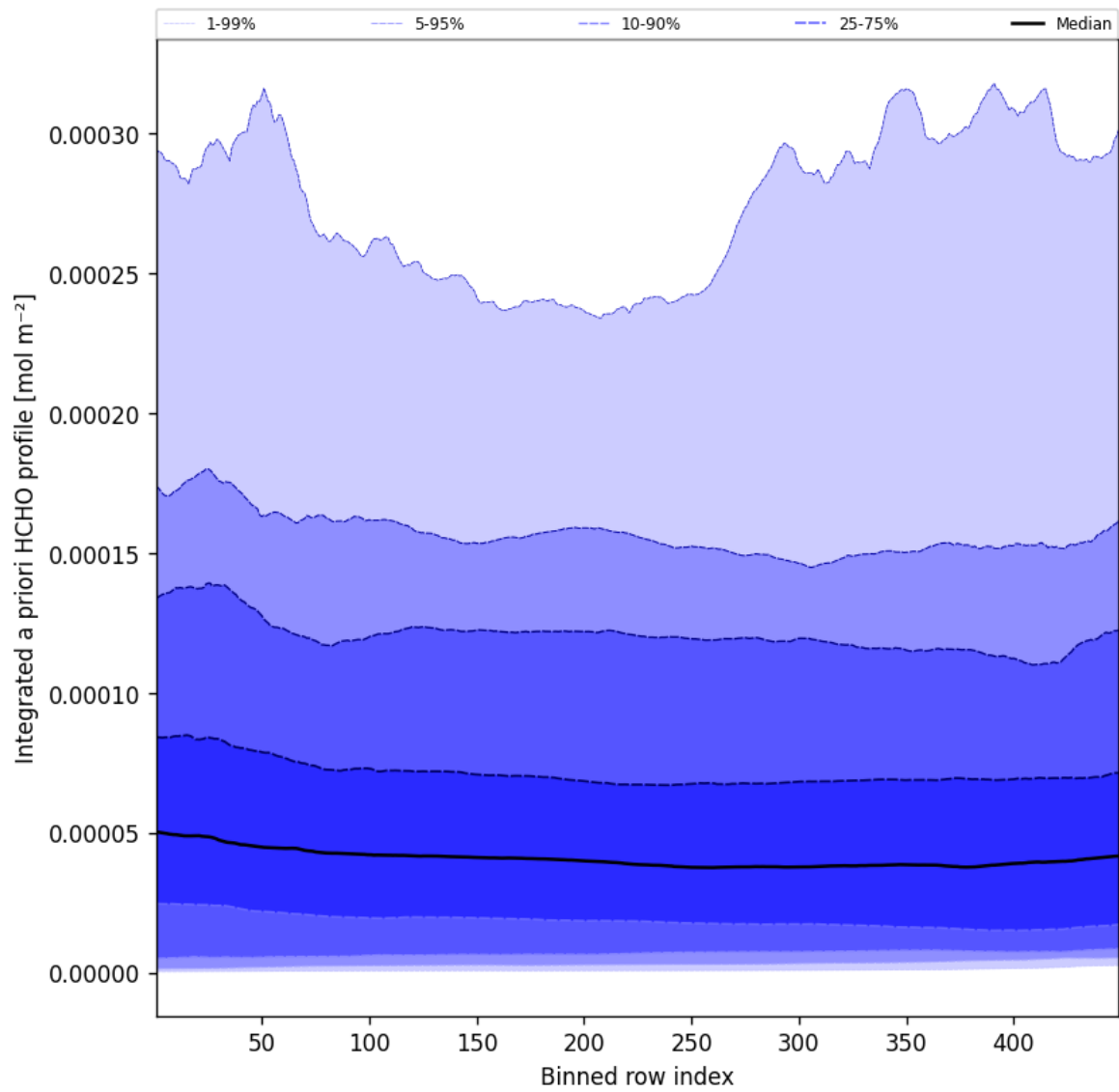
Figure 55: Along track statistics of "Integrated a priori HCHO profile" for 2025-07-28 to 2025-07-29
