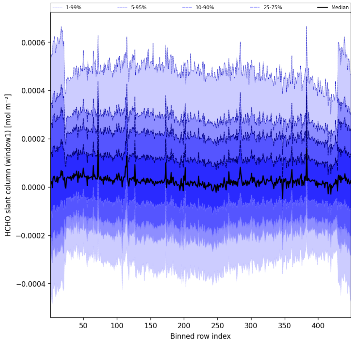
Figure 50: Along track statistics of “HCHO slant column (window1)” for 2025-07-28 to 2025-07-29
