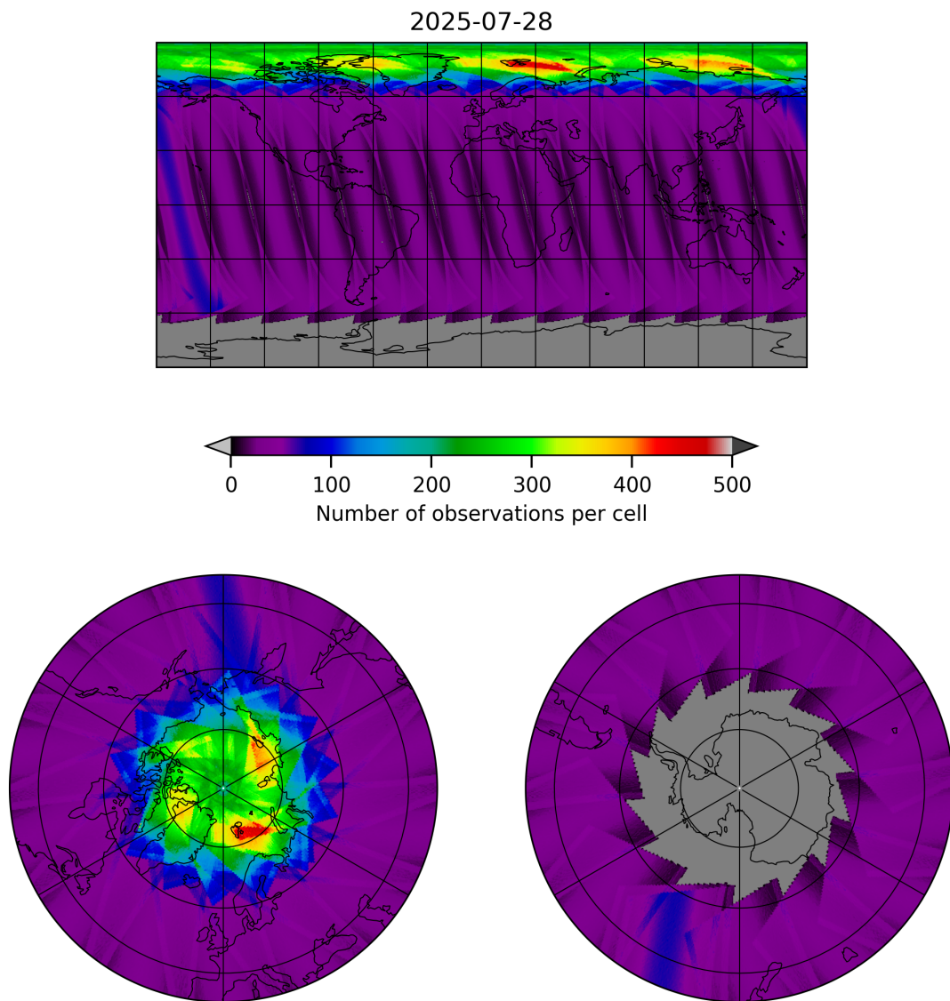
Figure 17: Map of the number of observations for 2025-07-28 to 2025-07-29
