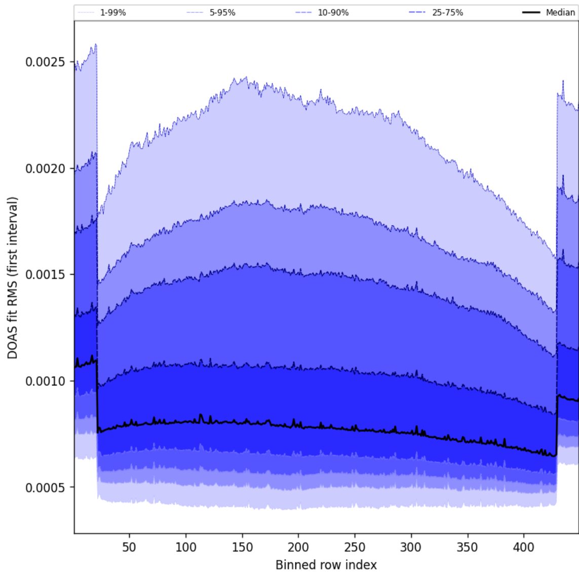
Figure 58: Along track statistics of “DOAS fit RMS (first interval)” for 2025-07-28 to 2025-07-29
