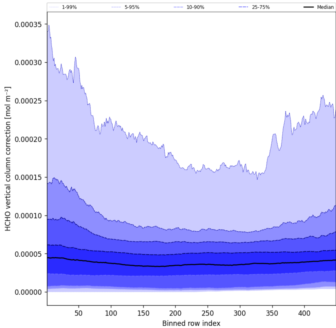
Figure 49: Along track statistics of “HCHO vertical column correction” for 2025-07-28 to 2025-07-29
