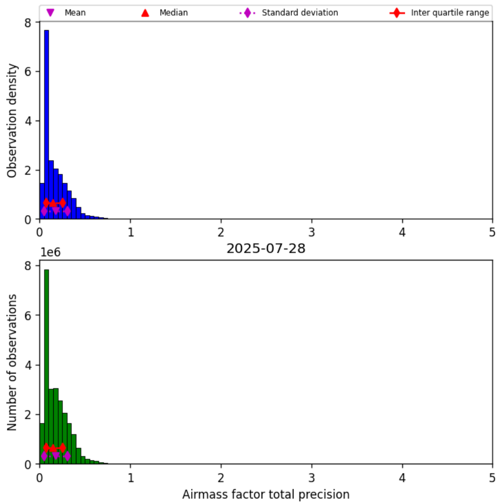
Figure 39: Histogram of “Airmass factor total precision” for 2025-07-28 to 2025-07-29
