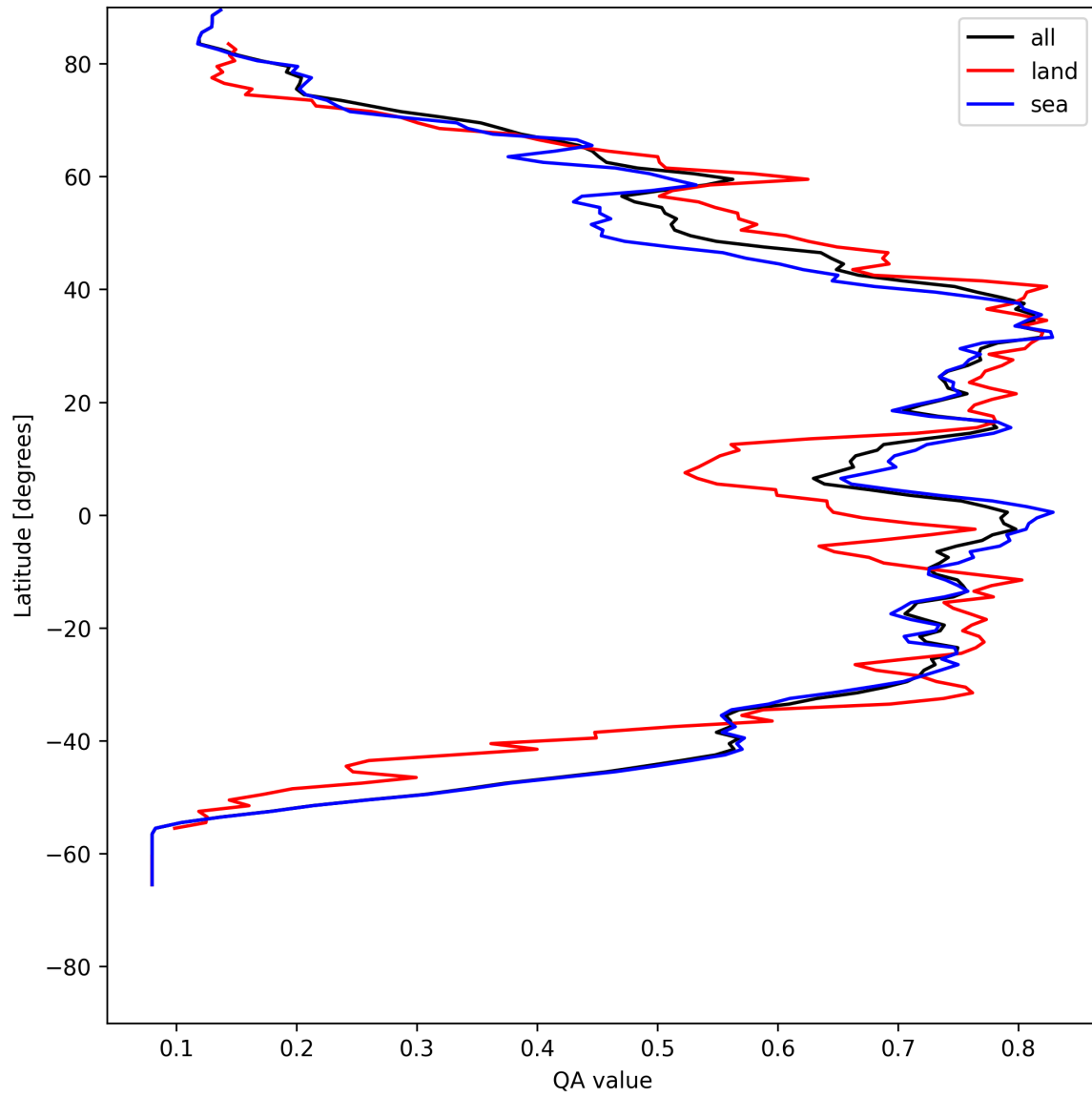
Figure 18: Zonal average of “QA value” for 2025-07-28 to 2025-07-29.
