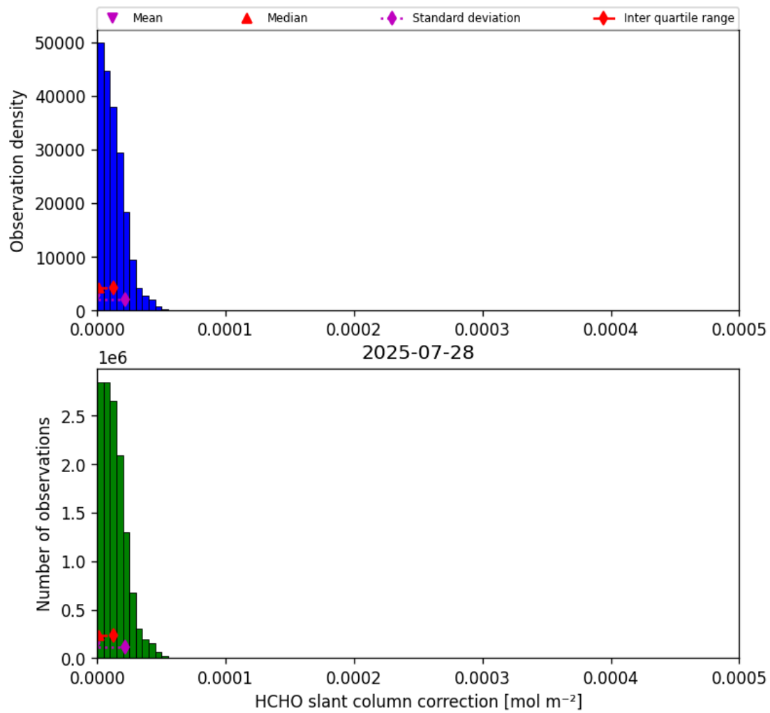
Figure 45: Histogram of “HCHO slant column correction” for 2025-07-28 to 2025-07-29
