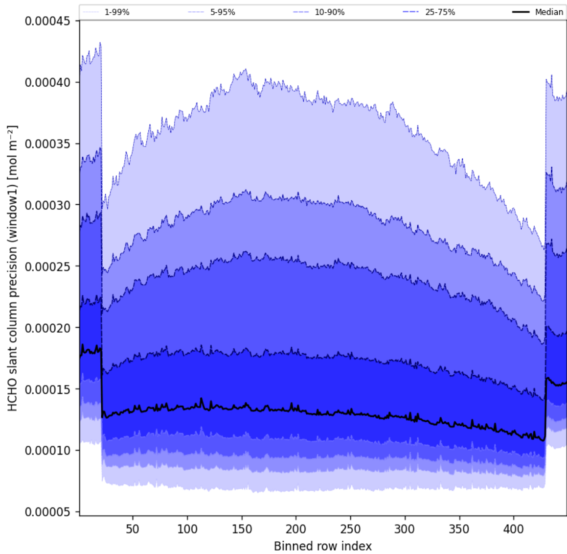
Figure 51: Along track statistics of “HCHO slant column precision (window1)” for 2025-07-28 to 2025-07-29
