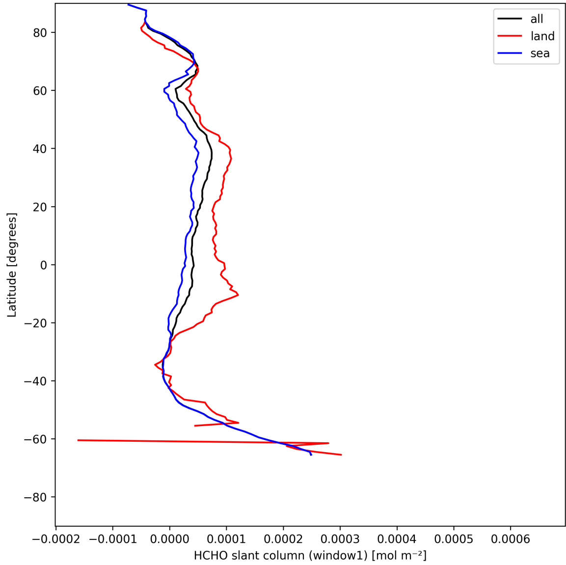
Figure 22: Zonal average of “HCHO slant column (window1)” for 2025-07-28 to 2025-07-29.
