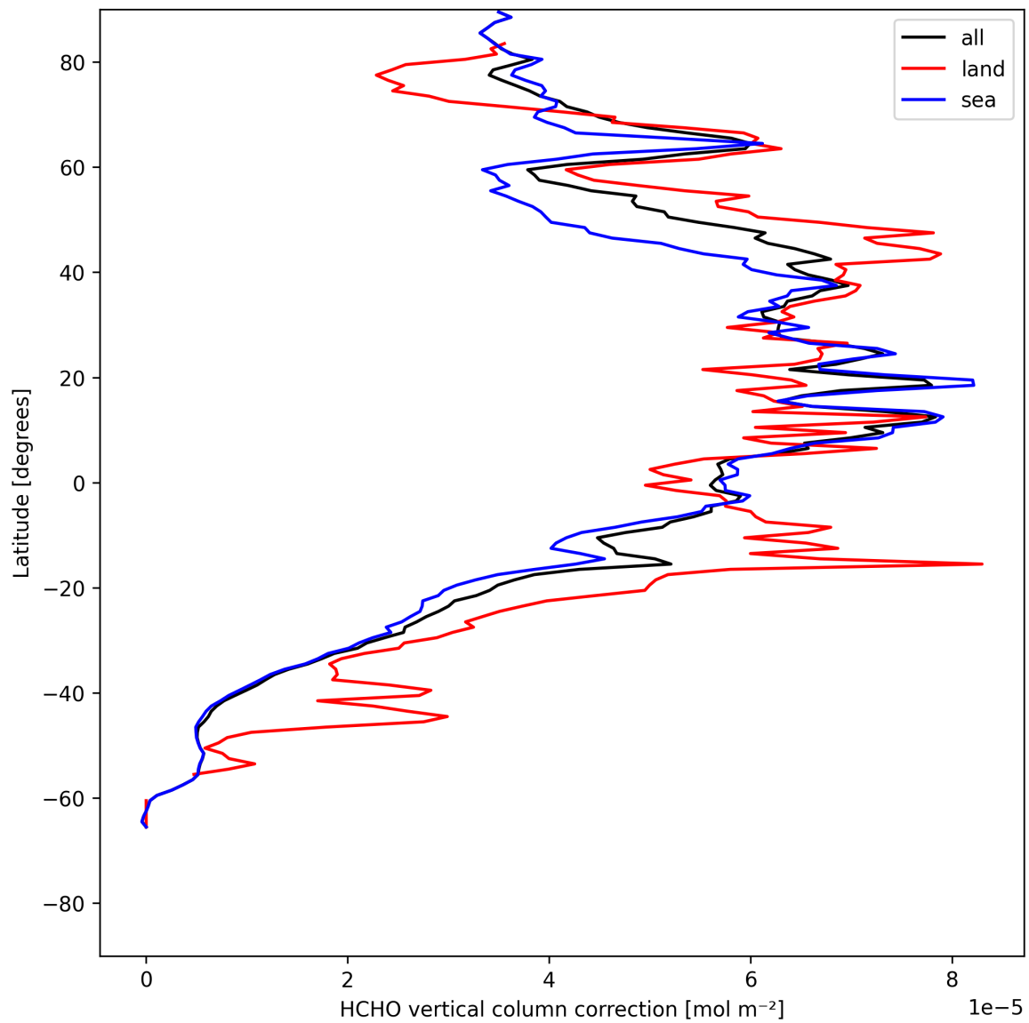
Figure 21: Zonal average of “HCHO vertical column correction” for 2025-07-28 to 2025-07-29.
