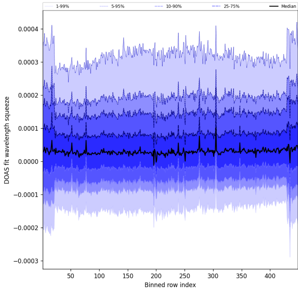
Figure 57: Along track statistics of “DOAS fit wavelength squeeze” for 2025-07-28 to 2025-07-29
