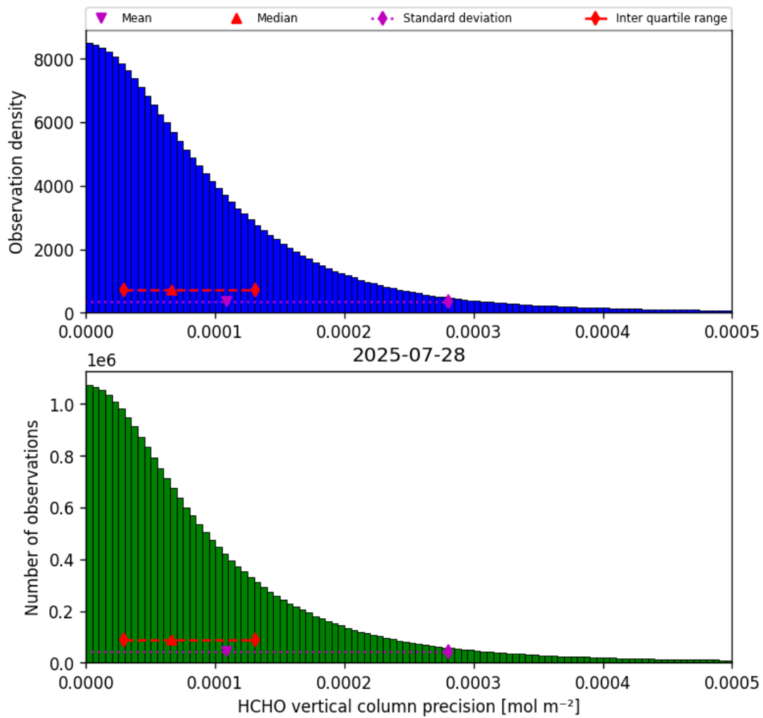
Figure 34: Histogram of “HCHO vertical column precision” for 2025-07-28 to 2025-07-29
