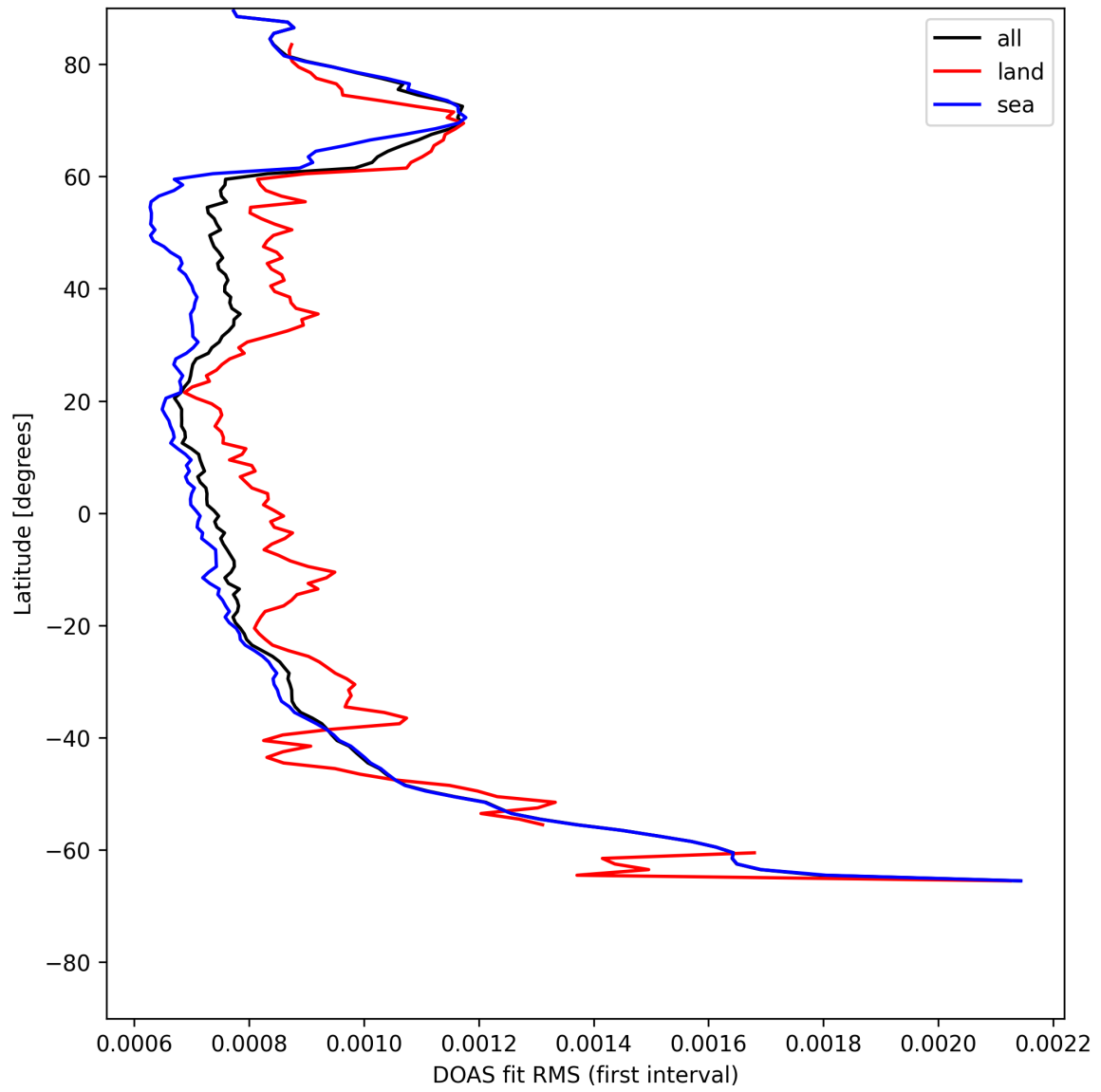
Figure 30: Zonal average of "DOAS fit RMS (first interval)" for 2025-07-28 to 2025-07-29.
