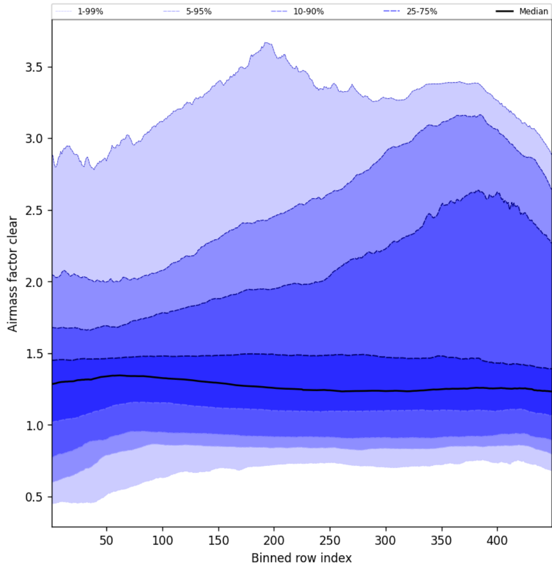
Figure 54: Along track statistics of “Airmass factor clear” for 2025-07-28 to 2025-07-29
