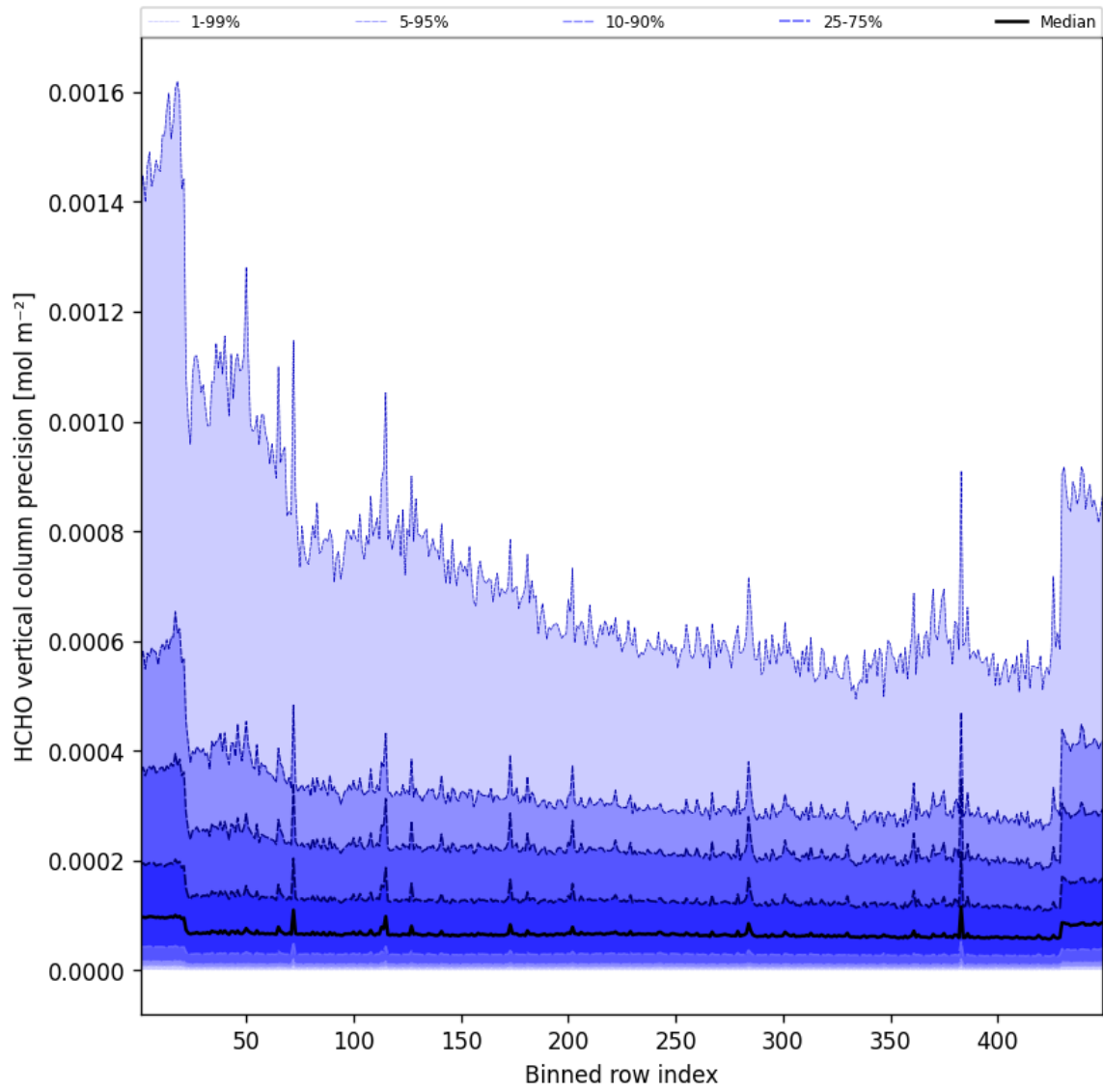
Figure 48: Along track statistics of “HCHO vertical column precision” for 2025-07-28 to 2025-07-29
