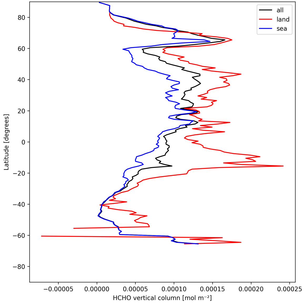
Figure 19: Zonal average of “HCHO vertical column” for 2025-07-28 to 2025-07-29.
