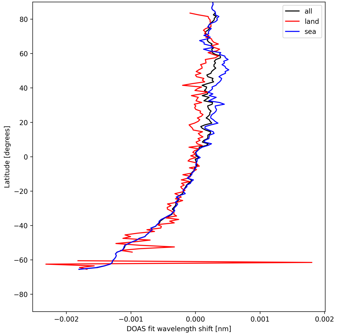
Figure 28: Zonal average of “DOAS fit wavelength shift” for 2025-07-28 to 2025-07-29.
