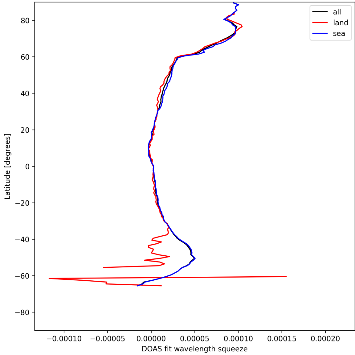
Figure 29: Zonal average of “DOAS fit wavelength squeeze” for 2025-07-28 to 2025-07-29.
