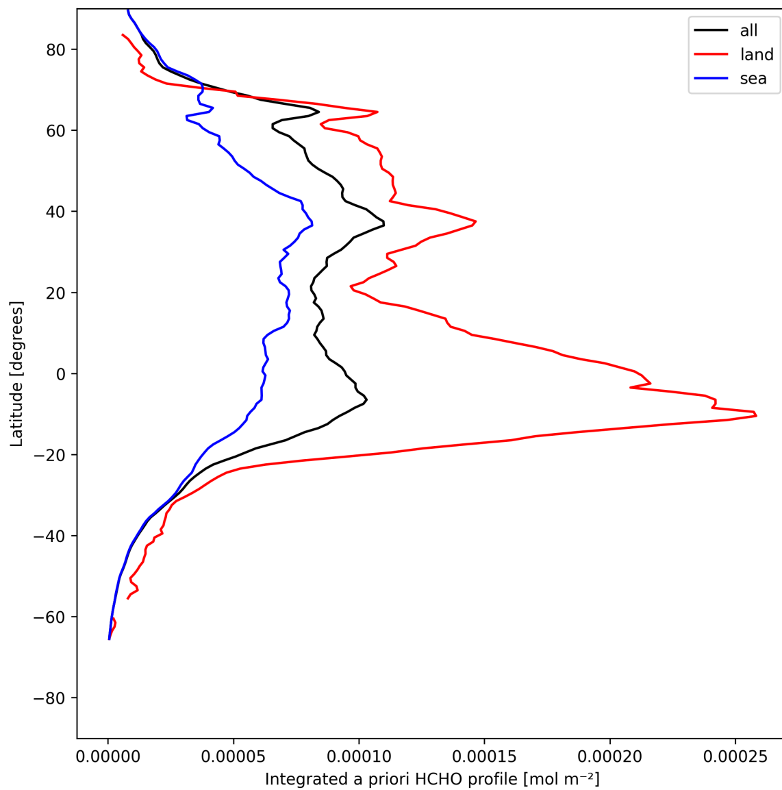
Figure 27: Zonal average of “Integrated a priori HCHO profile” for 2025-07-28 to 2025-07-29.
