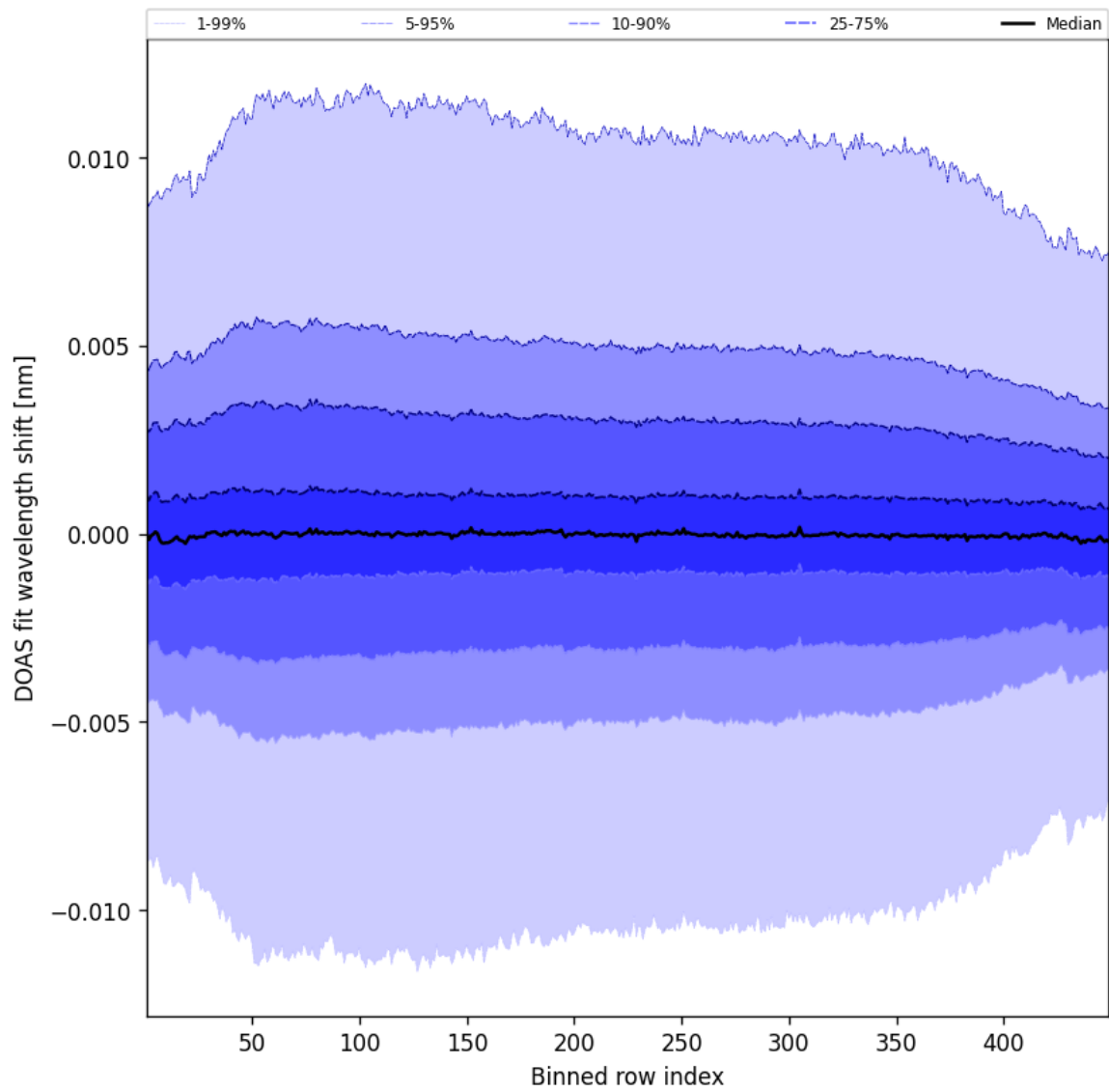
Figure 56: Along track statistics of “DOAS fit wavelength shift” for 2025-07-28 to 2025-07-29
