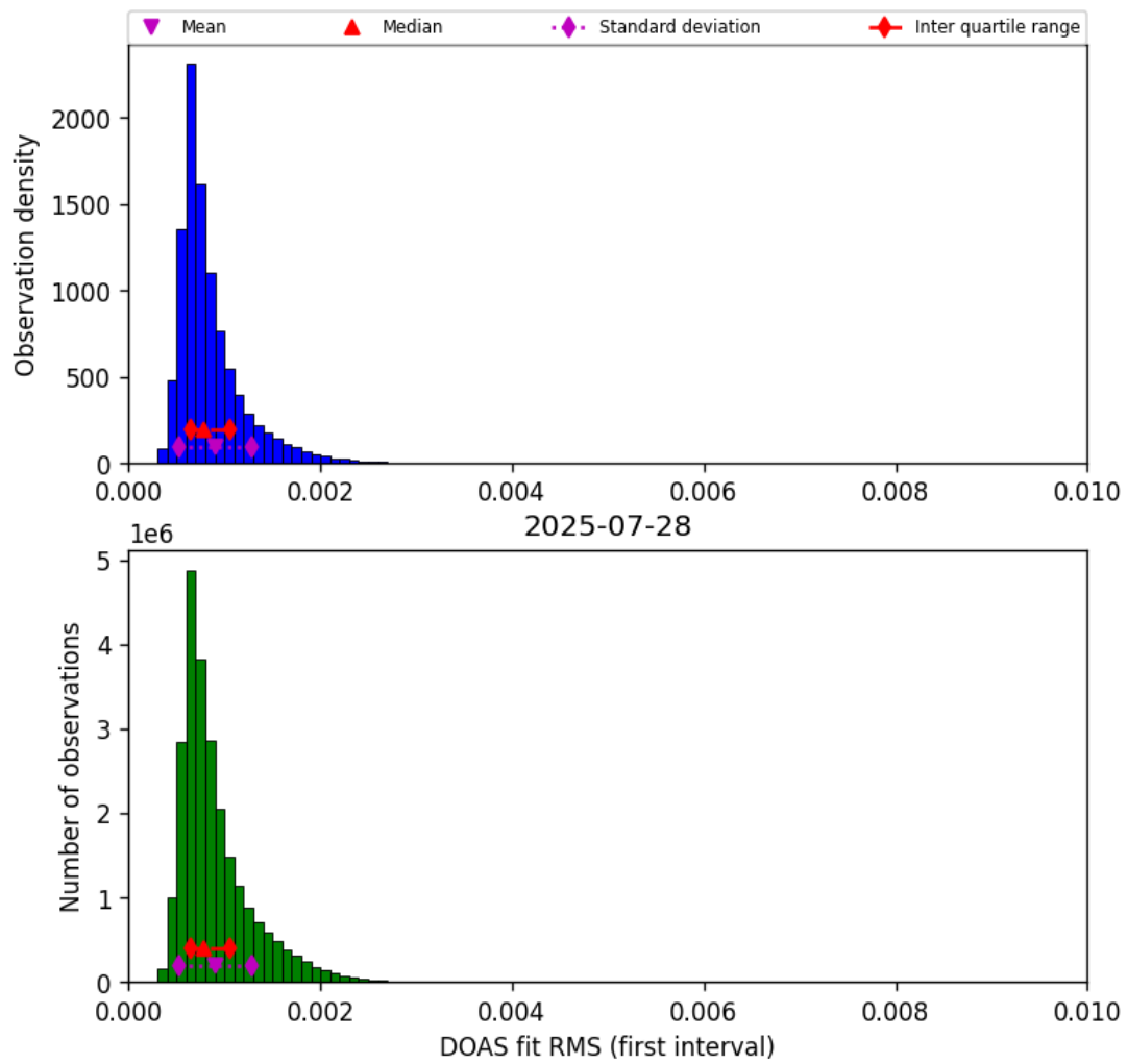
Figure 44: Histogram of “DOAS fit RMS (first interval)” for 2025-07-28 to 2025-07-29
