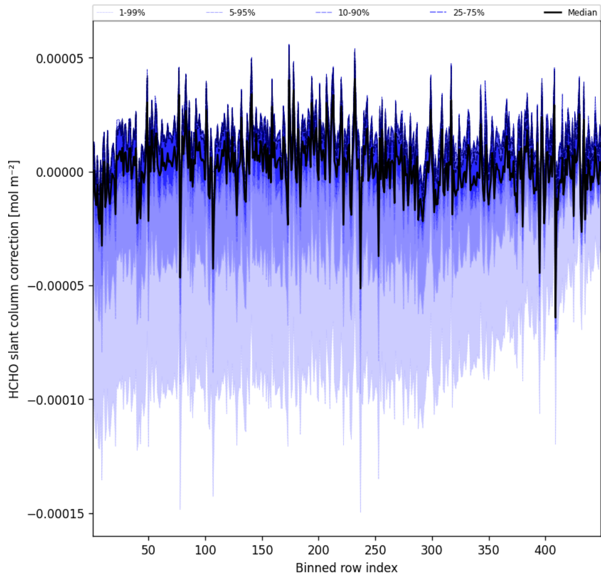
Figure 59: Along track statistics of “HCHO slant column correction” for 2025-07-28 to 2025-07-29
