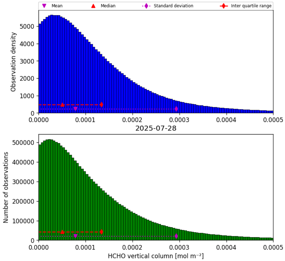
Figure 33: Histogram of “HCHO vertical column” for 2025-07-28 to 2025-07-29
