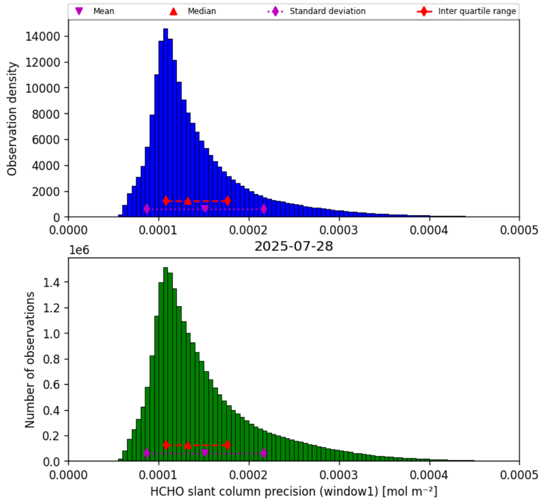
Figure 37: Histogram of “HCHO slant column precision (window1)” for 2025-07-28 to 2025-07-29
