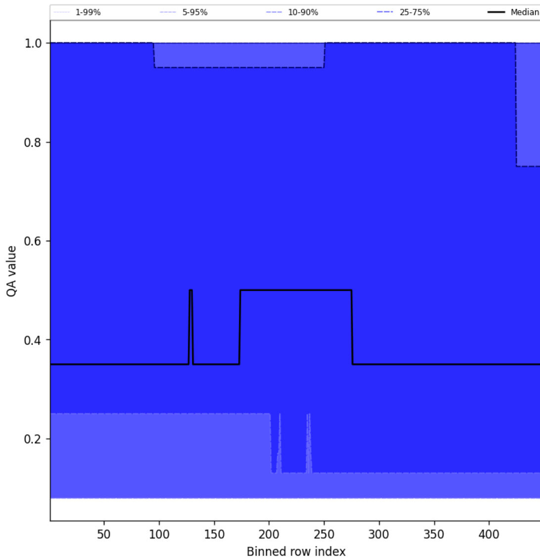
Figure 46: Along track statistics of “QA value” for 2025-07-28 to 2025-07-29
