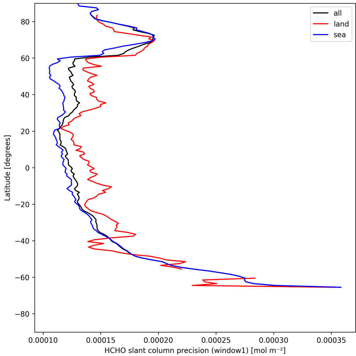
Figure 23: Zonal average of “HCHO slant column precision (window1)” for 2025-07-28 to 2025-07-29.
