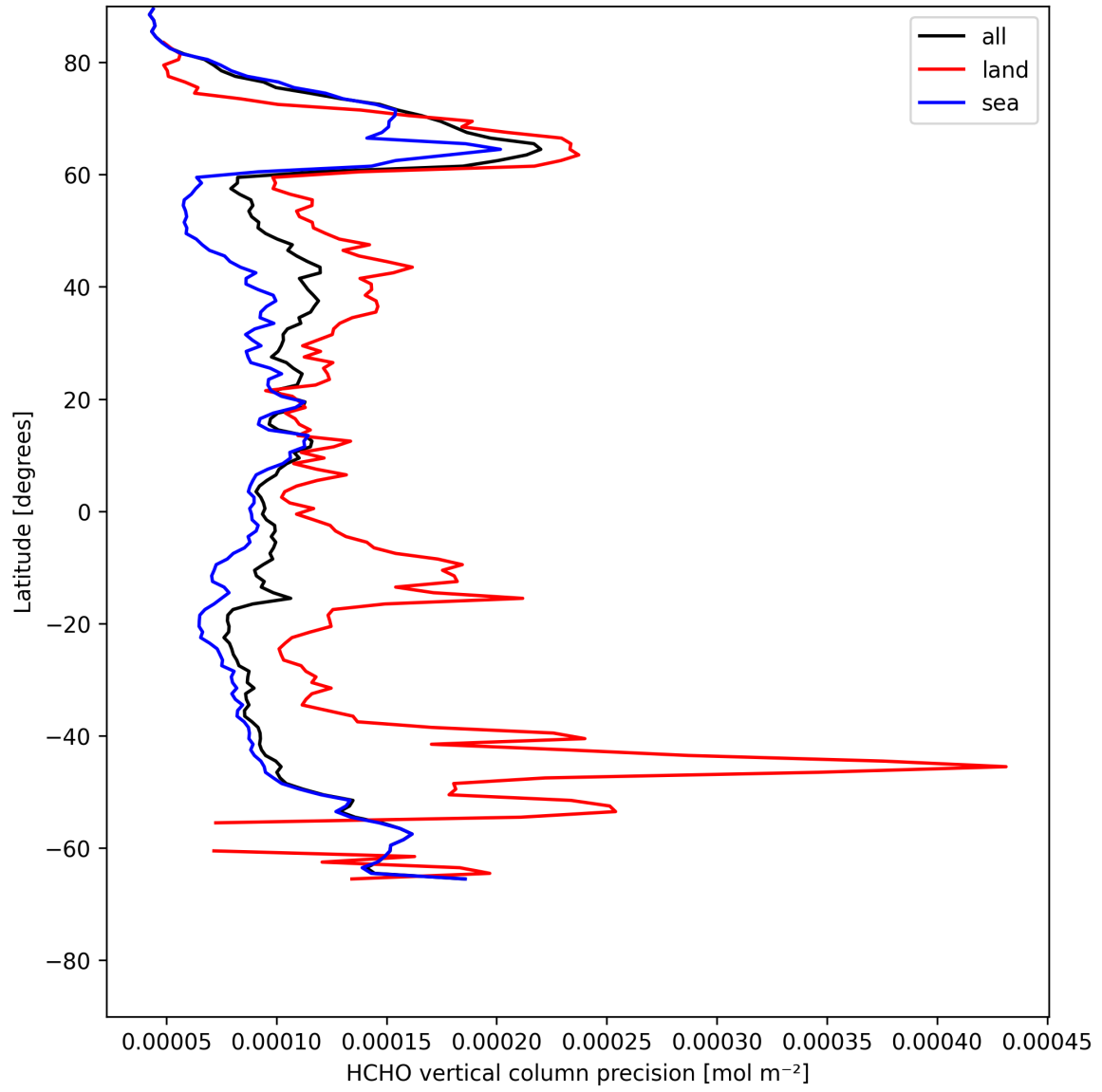
Figure 20: Zonal average of "HCHO vertical column precision" for 2025-07-28 to 2025-07-29.
