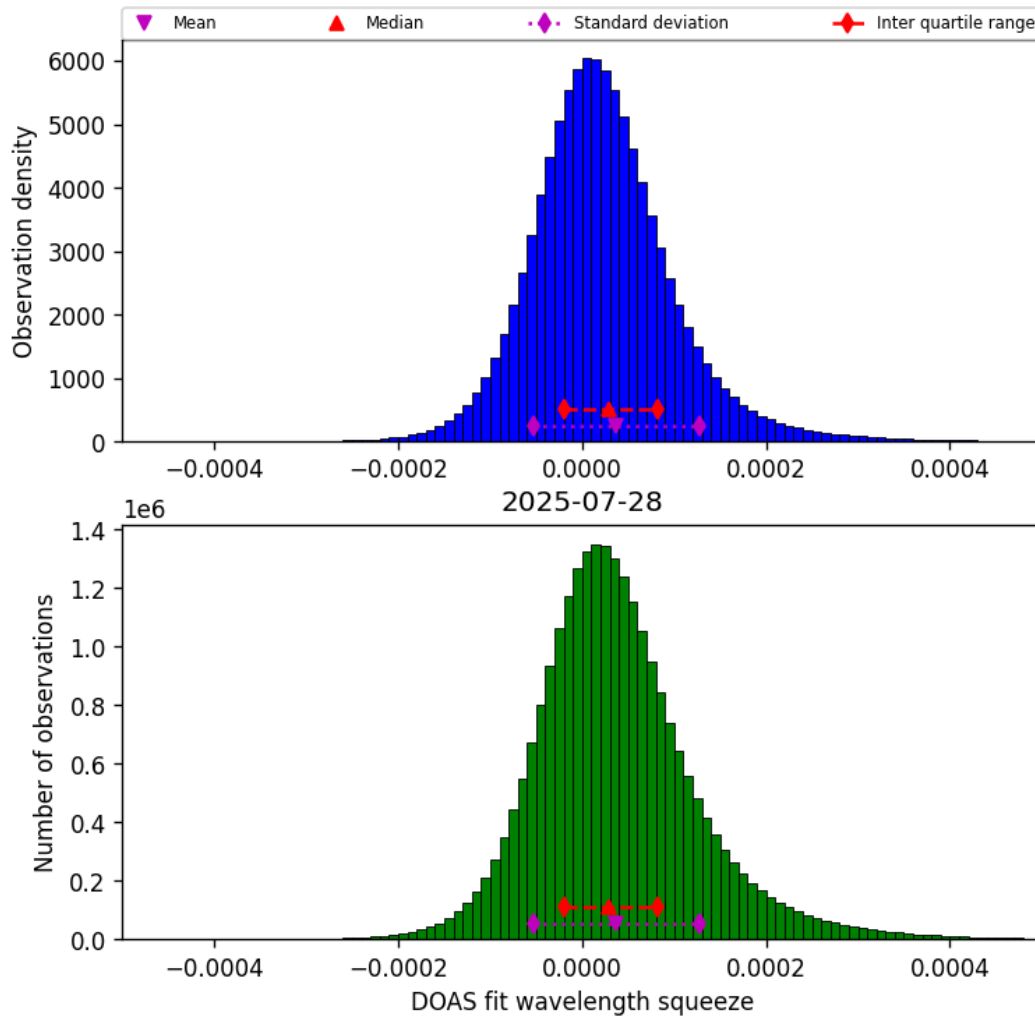
Figure 43: Histogram of “DOAS fit wavelength squeeze” for 2025-07-28 to 2025-07-29
