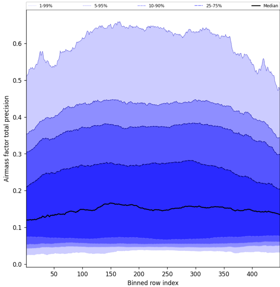
Figure 53: Along track statistics of “Airmass factor total precision” for 2025-07-28 to 2025-07-29
