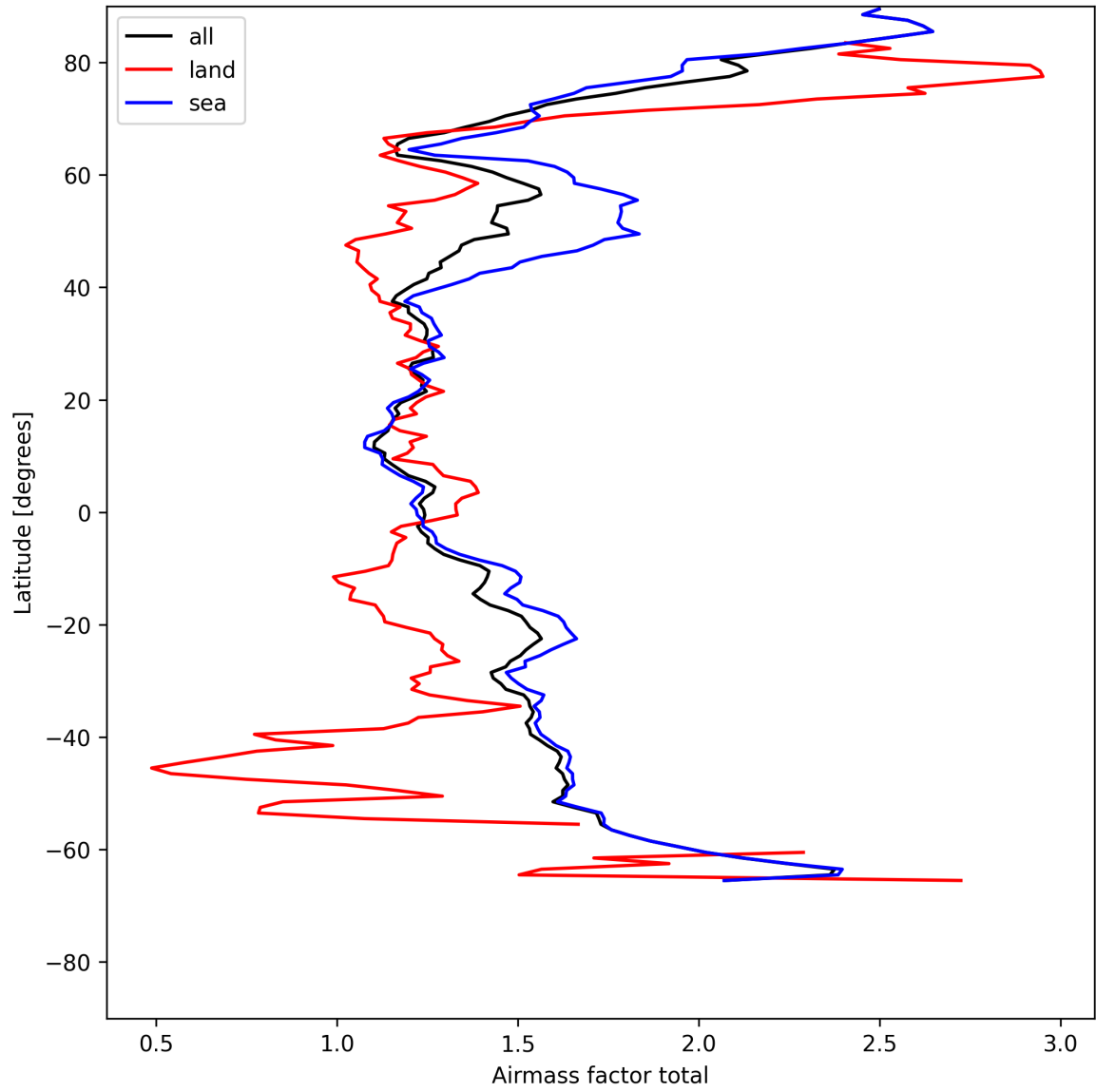
Figure 24: Zonal average of “Airmass factor total” for 2025-07-28 to 2025-07-29.
