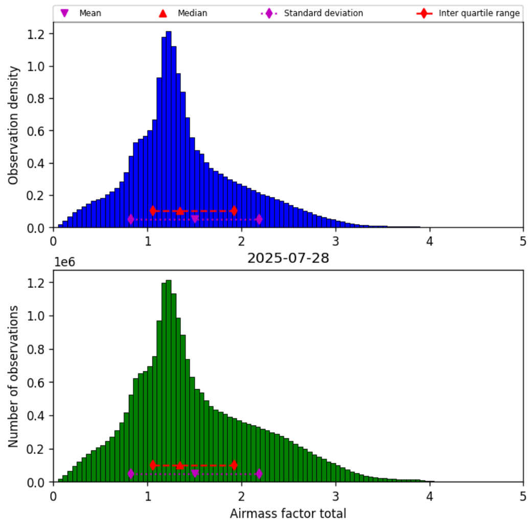
Figure 38: Histogram of “Airmass factor total” for 2025-07-28 to 2025-07-29
