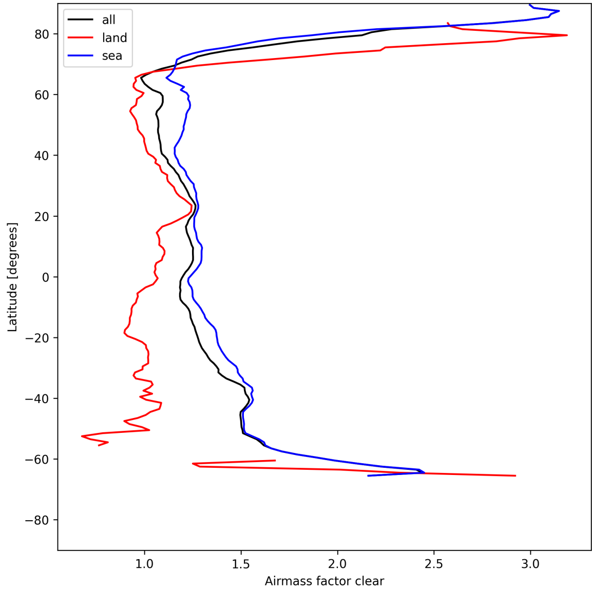
Figure 26: Zonal average of “Airmass factor clear” for 2025-07-28 to 2025-07-29.
