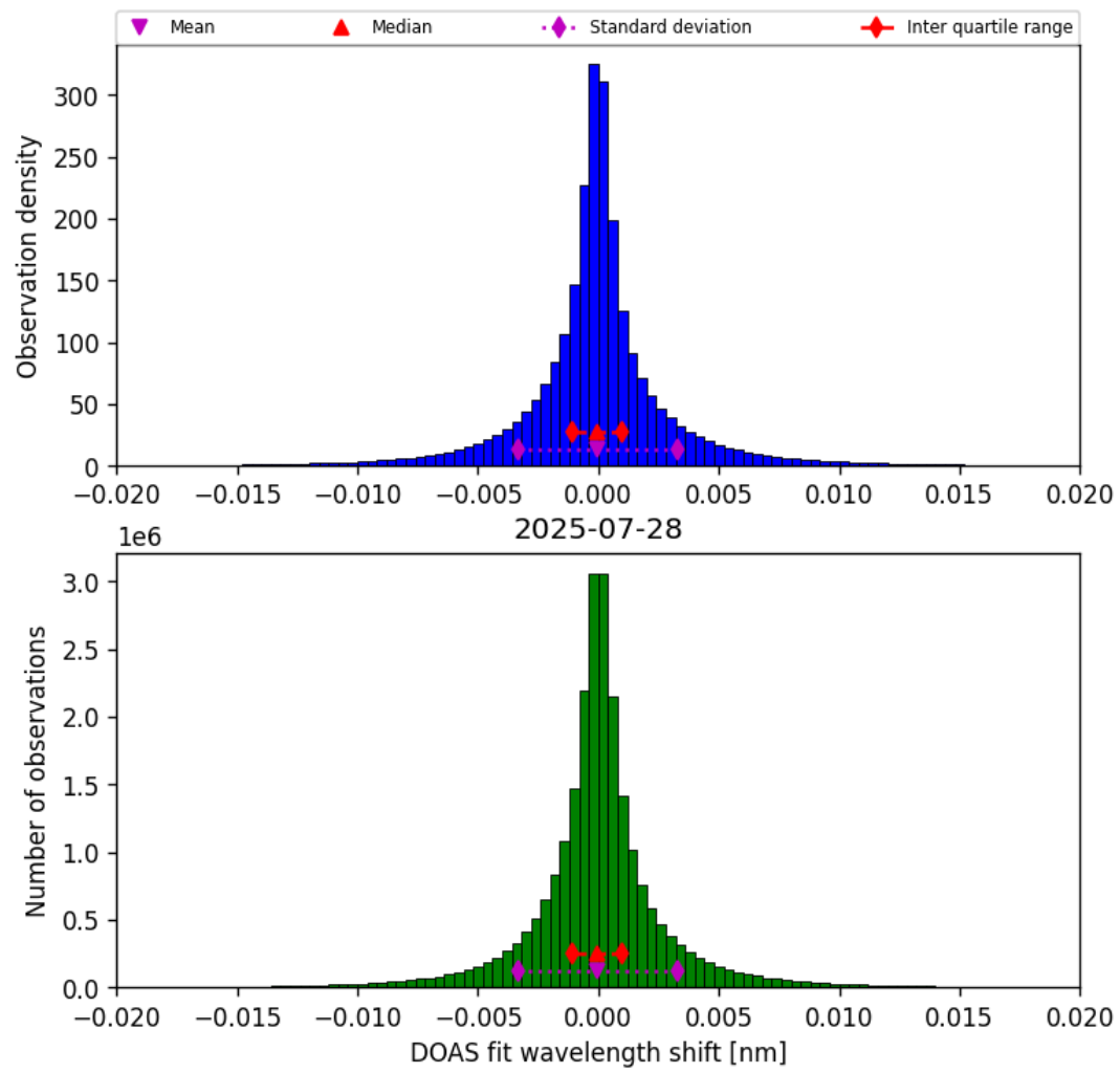
Figure 42: Histogram of “DOAS fit wavelength shift” for 2025-07-28 to 2025-07-29
