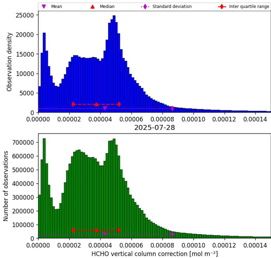
Figure 35: Histogram of “HCHO vertical column correction” for 2025-07-28 to 2025-07-29
