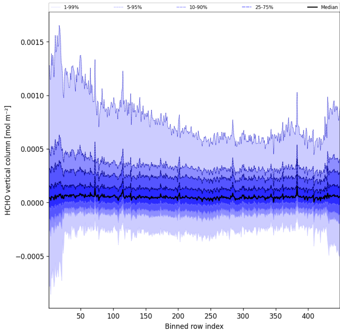
Figure 47: Along track statistics of “HCHO vertical column” for 2025-07-28 to 2025-07-29
