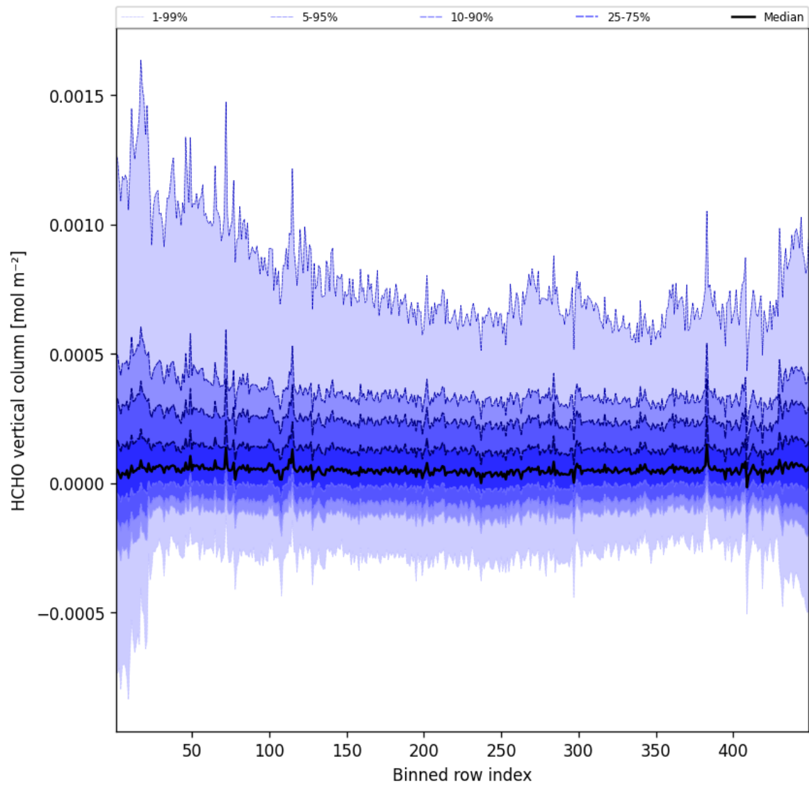
Figure 47: Along track statistics of “HCHO vertical column” for 2025-07-29 to 2025-07-30
