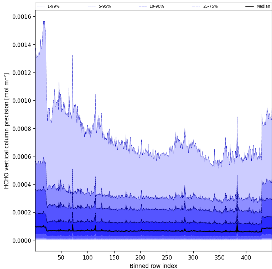
Figure 48: Along track statistics of “HCHO vertical column precision” for 2025-07-29 to 2025-07-30
