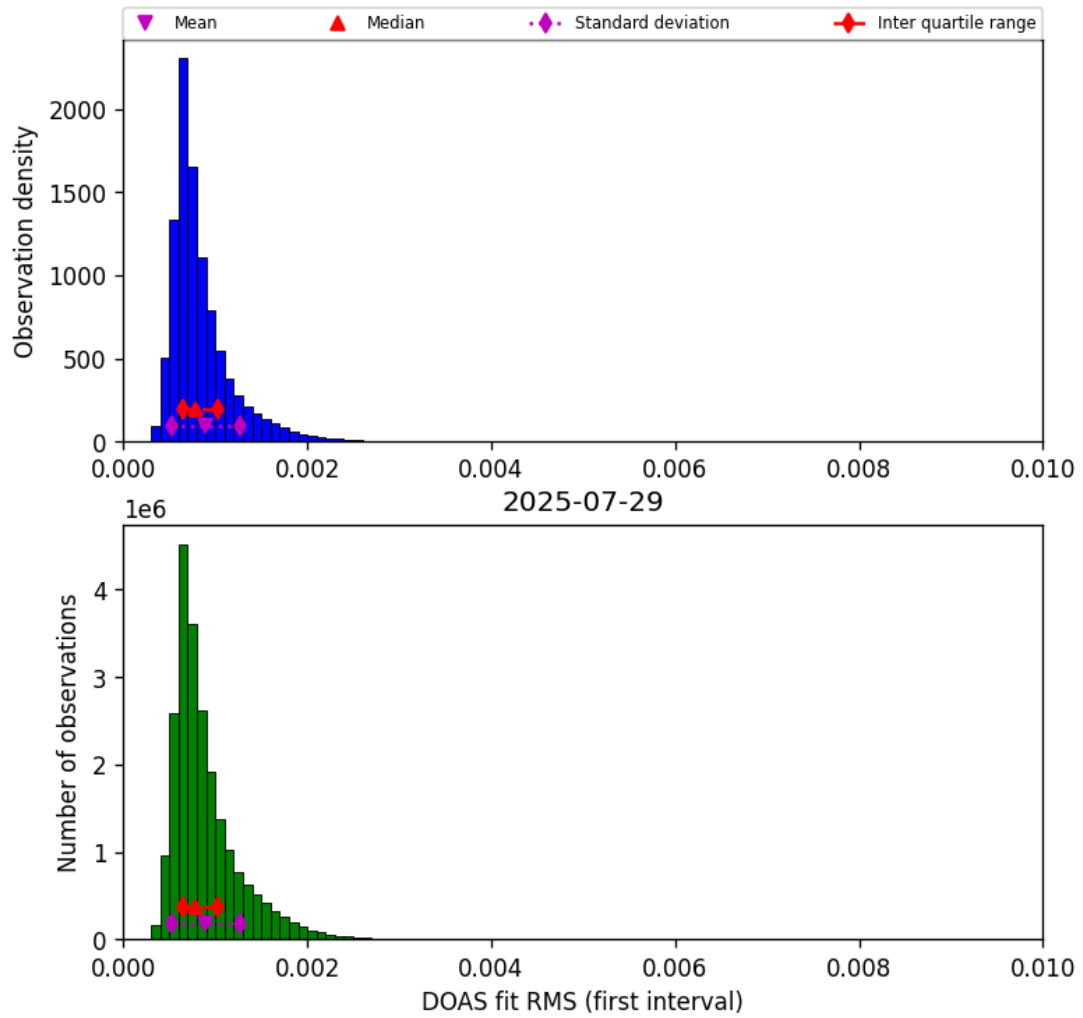
Figure 44: Histogram of “DOAS fit RMS (first interval)” for 2025-07-29 to 2025-07-30
