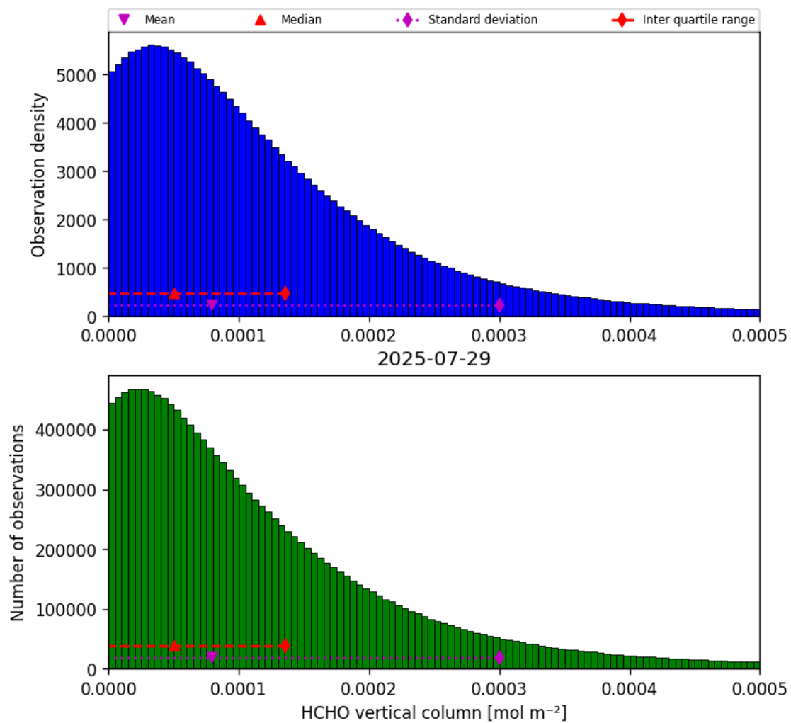
Figure 33: Histogram of “HCHO vertical column” for 2025-07-29 to 2025-07-30
