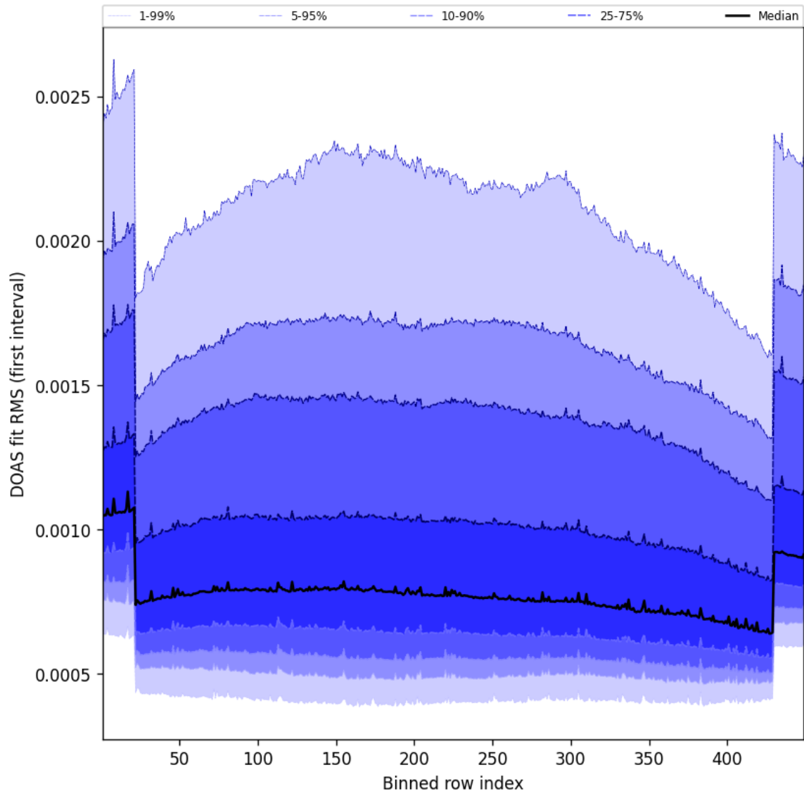
Figure 58: Along track statistics of “DOAS fit RMS (first interval)” for 2025-07-29 to 2025-07-30
