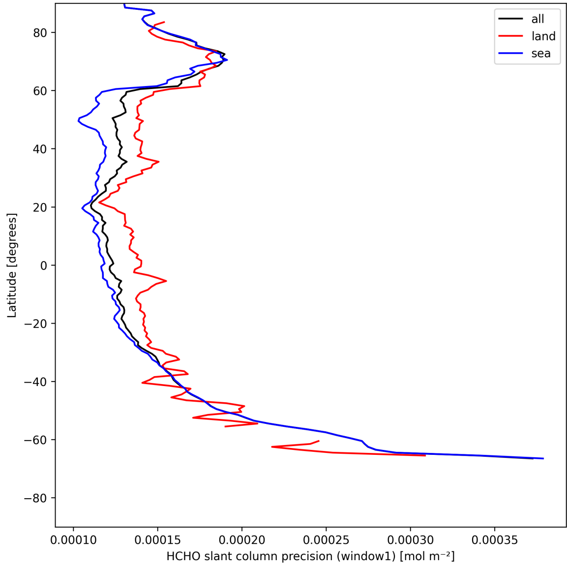
Figure 23: Zonal average of "HCHO slant column precision (window1)" for 2025-07-29 to 2025-07-30.
