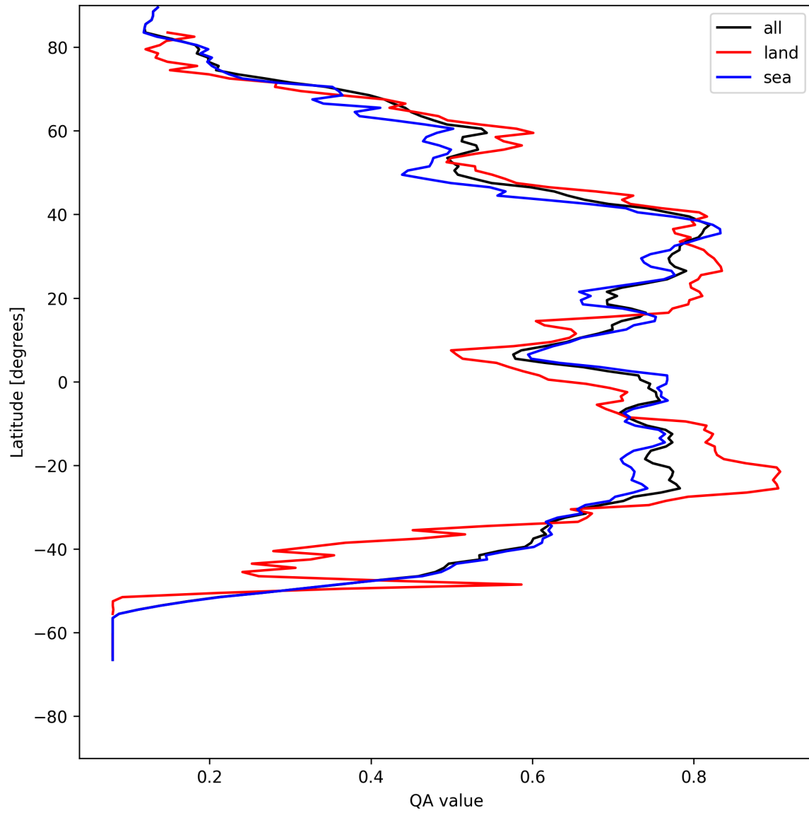
Figure 18: Zonal average of “QA value” for 2025-07-29 to 2025-07-30.
