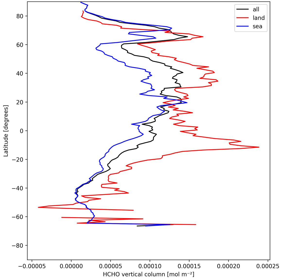
Figure 19: Zonal average of “HCHO vertical column” for 2025-07-29 to 2025-07-30.
