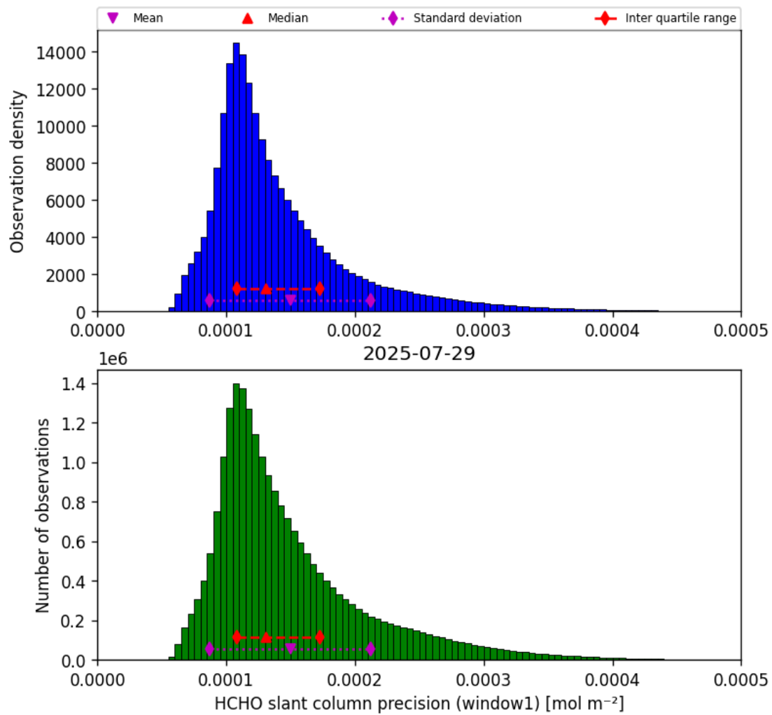
Figure 37: Histogram of “HCHO slant column precision (window1)” for 2025-07-29 to 2025-07-30
