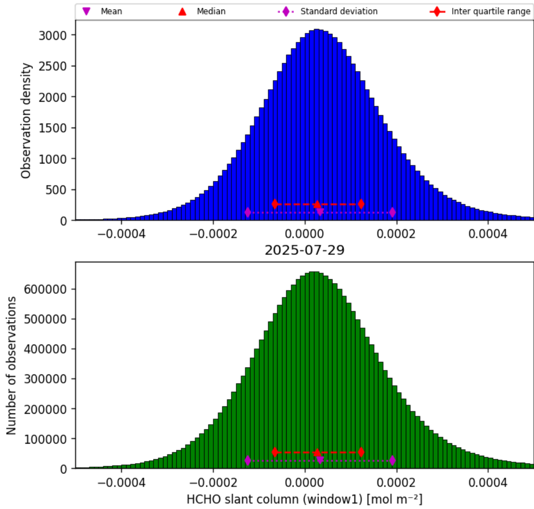
Figure 36: Histogram of “HCHO slant column (window1)” for 2025-07-29 to 2025-07-30
