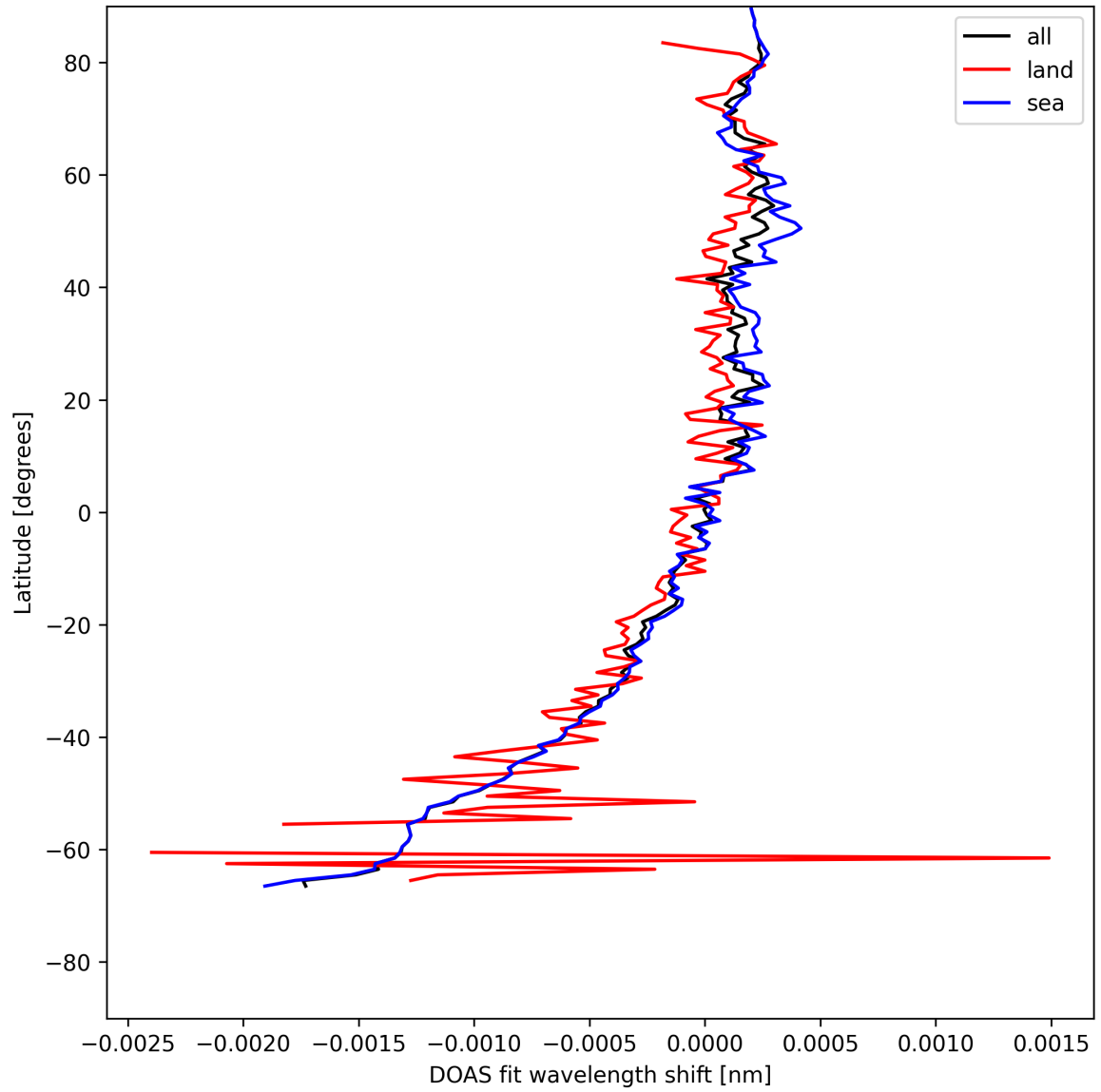
Figure 28: Zonal average of “DOAS fit wavelength shift” for 2025-07-29 to 2025-07-30.
