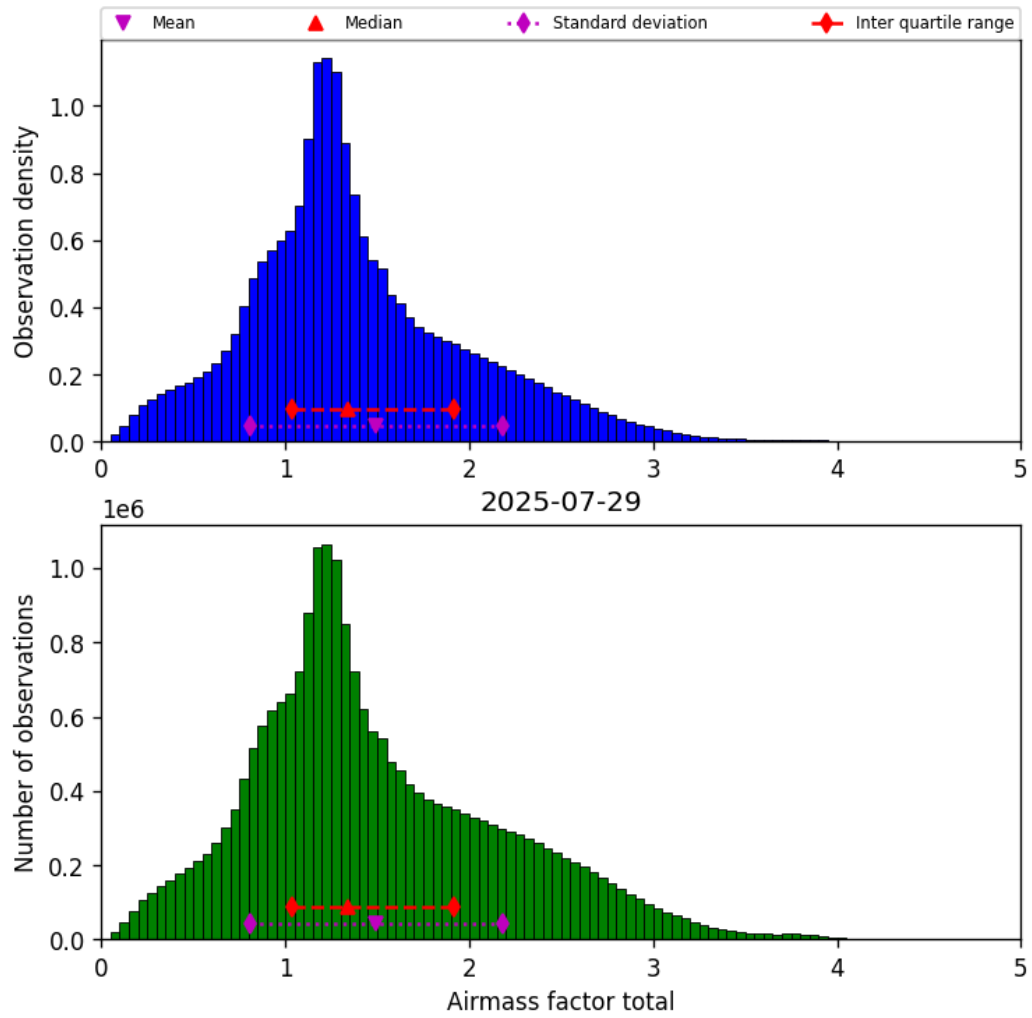
Figure 38: Histogram of “Airmass factor total” for 2025-07-29 to 2025-07-30
