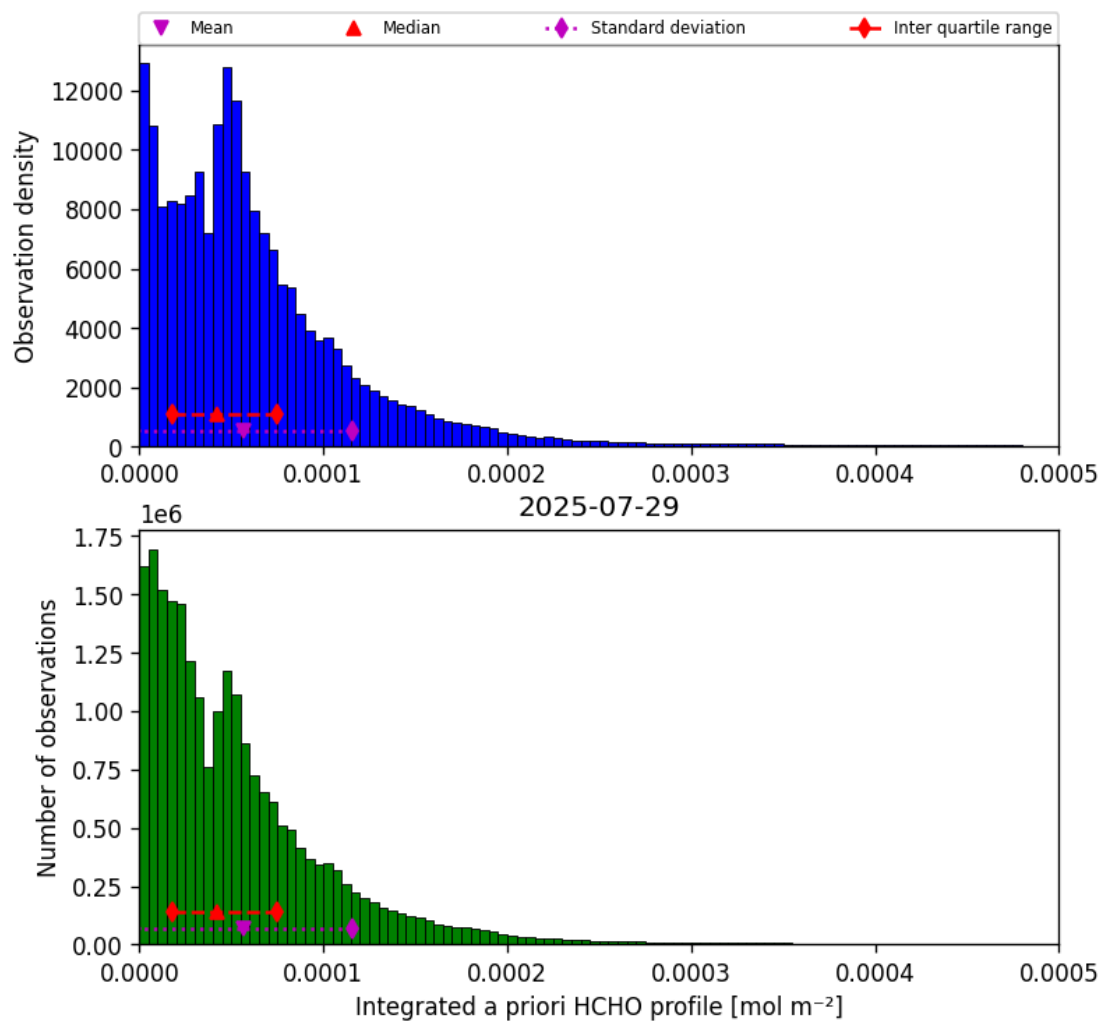
Figure 41: Histogram of “Integrated a priori HCHO profile” for 2025-07-29 to 2025-07-30
