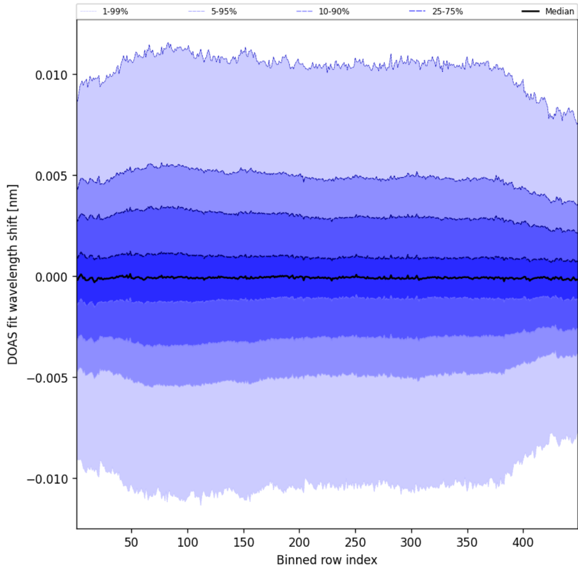
Figure 56: Along track statistics of “DOAS fit wavelength shift” for 2025-07-29 to 2025-07-30
