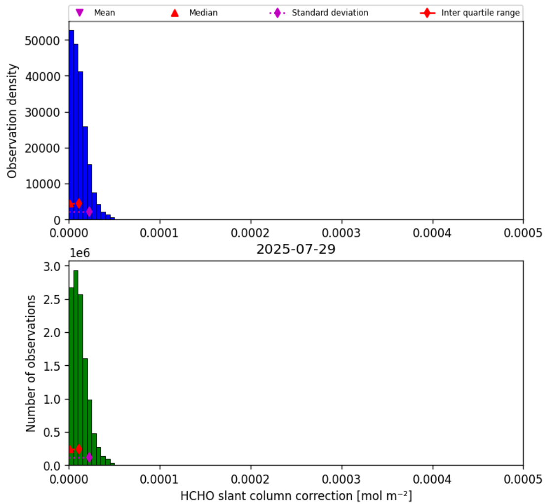
Figure 45: Histogram of “HCHO slant column correction” for 2025-07-29 to 2025-07-30
