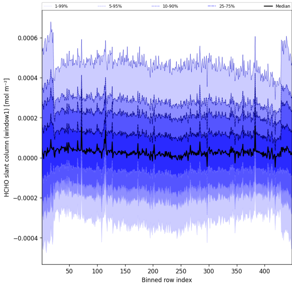
Figure 50: Along track statistics of “HCHO slant column (window1)” for 2025-07-29 to 2025-07-30
