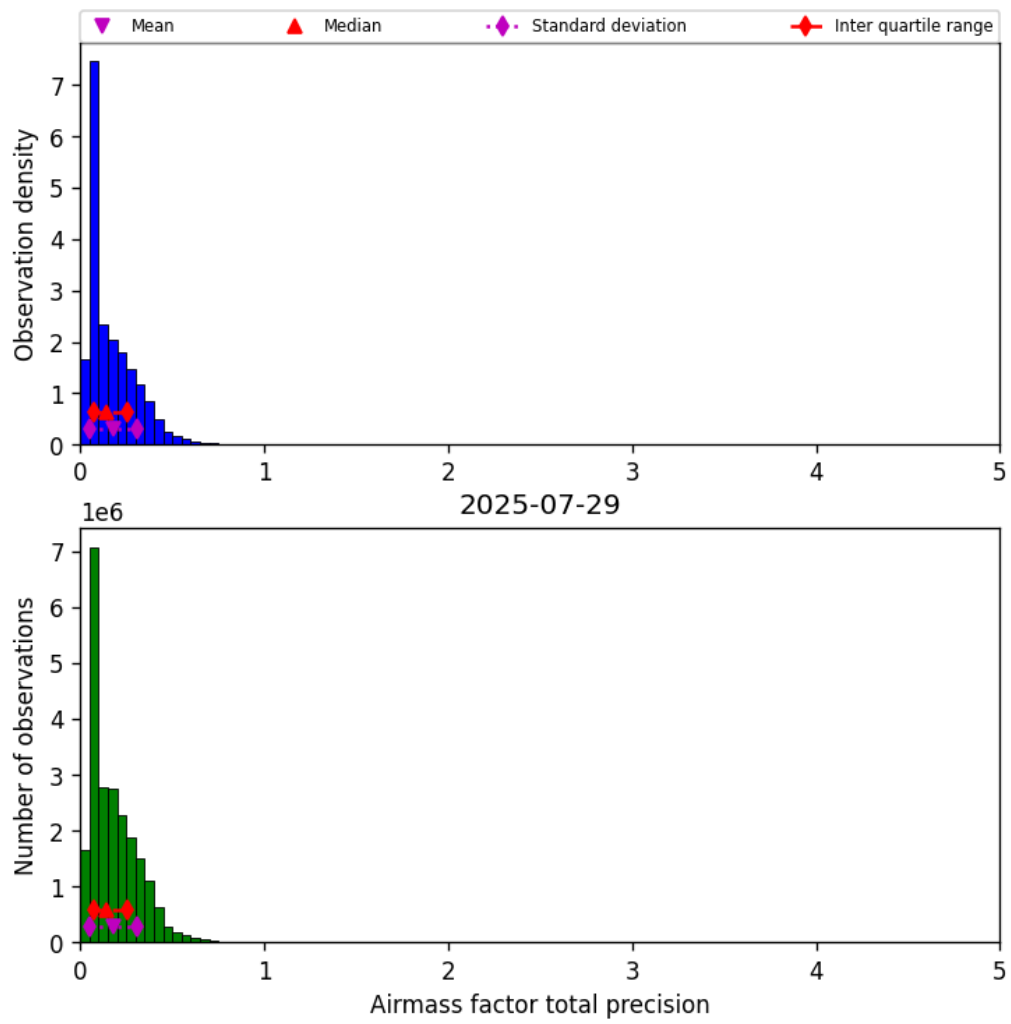
Figure 39: Histogram of “Airmass factor total precision” for 2025-07-29 to 2025-07-30
