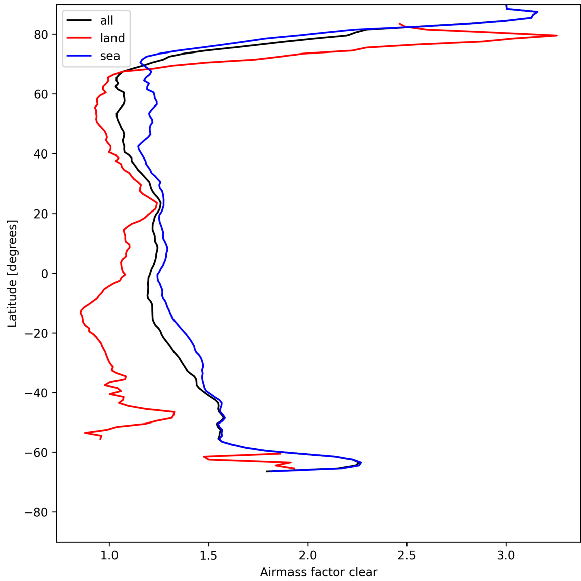
Figure 26: Zonal average of “Airmass factor clear” for 2025-07-29 to 2025-07-30.
