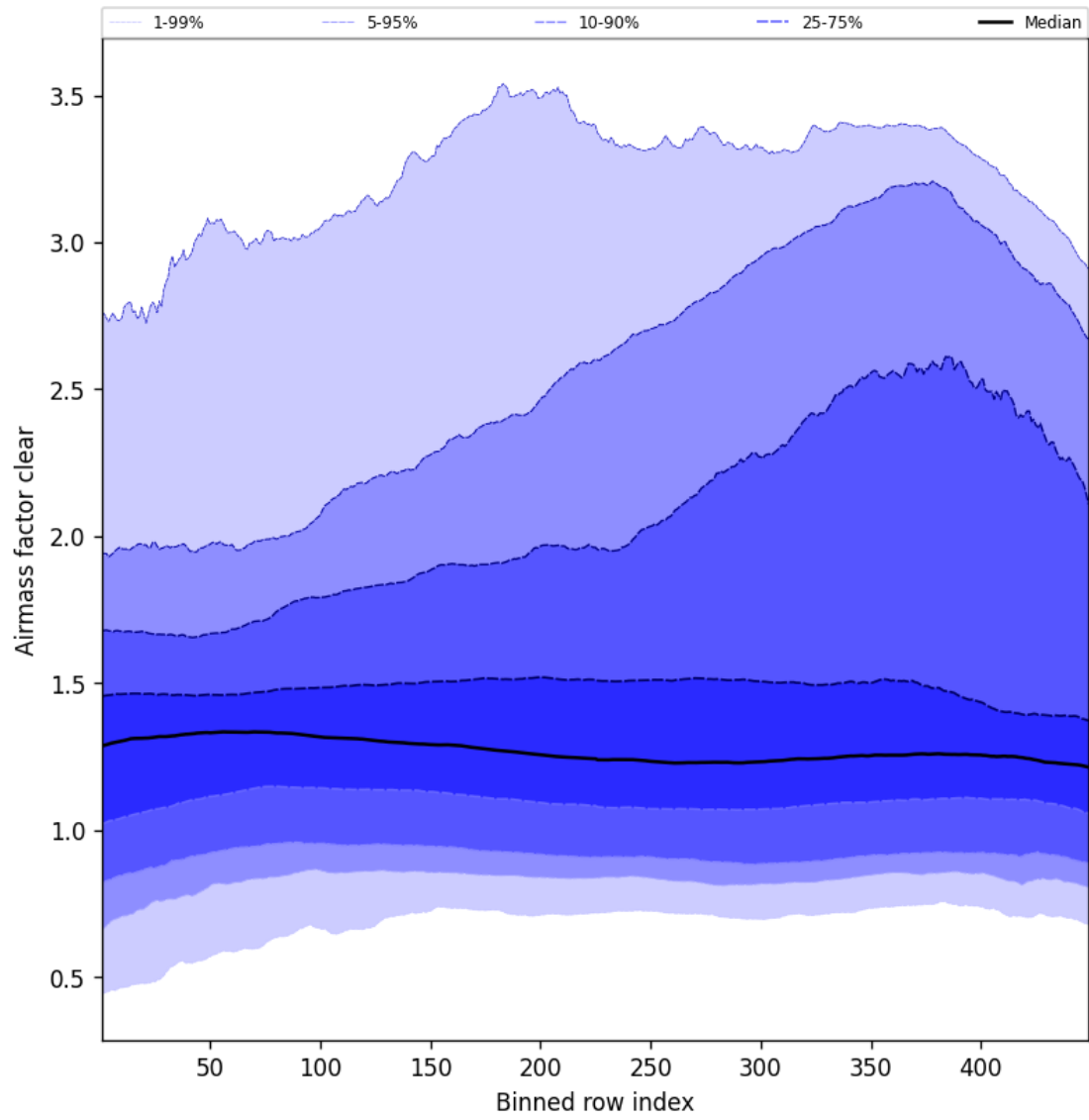
Figure 54: Along track statistics of “Airmass factor clear” for 2025-07-29 to 2025-07-30
