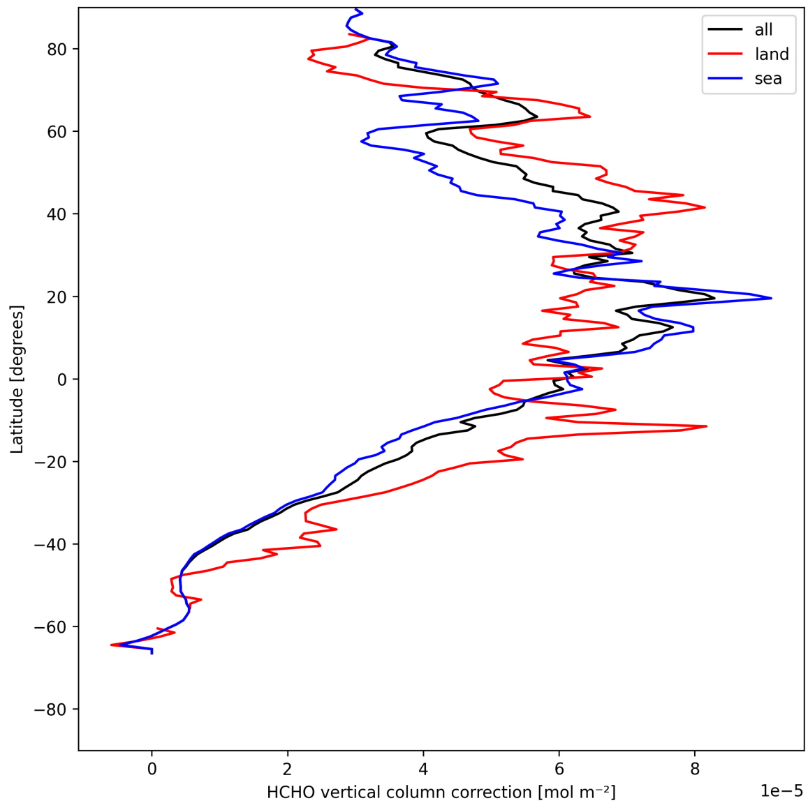
Figure 21: Zonal average of “HCHO vertical column correction” for 2025-07-29 to 2025-07-30.
