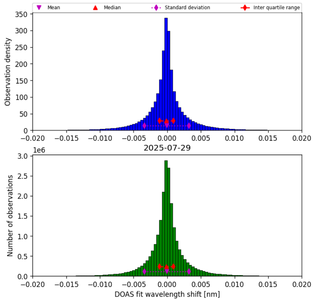
Figure 42: Histogram of “DOAS fit wavelength shift” for 2025-07-29 to 2025-07-30
