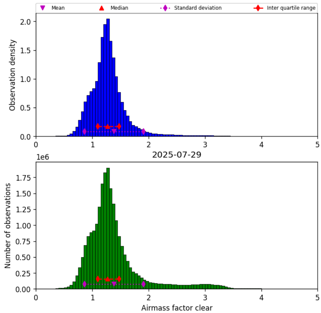
Figure 40: Histogram of “Airmass factor clear” for 2025-07-29 to 2025-07-30
