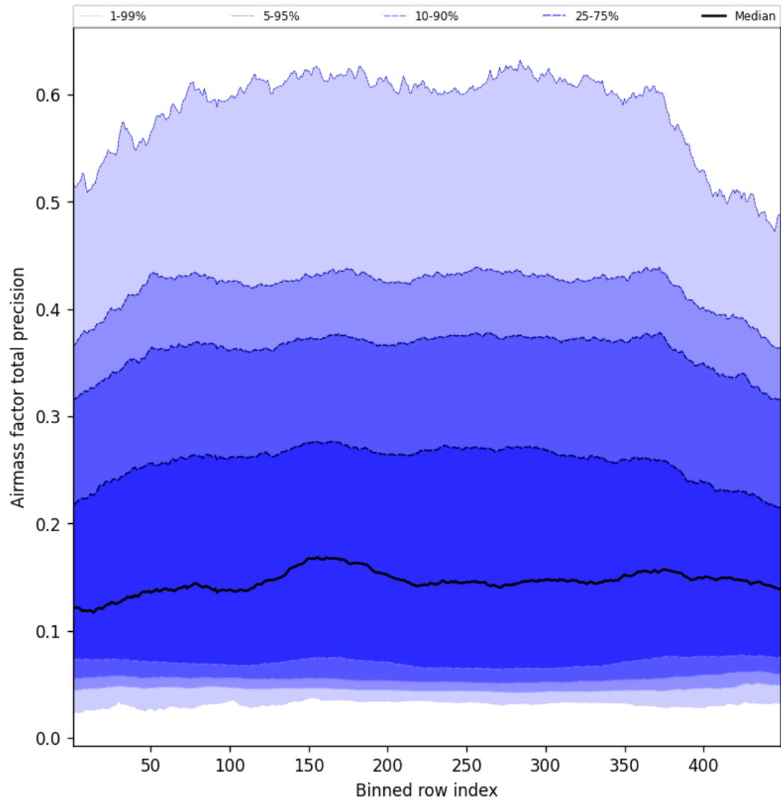
Figure 53: Along track statistics of “Airmass factor total precision” for 2025-07-29 to 2025-07-30
