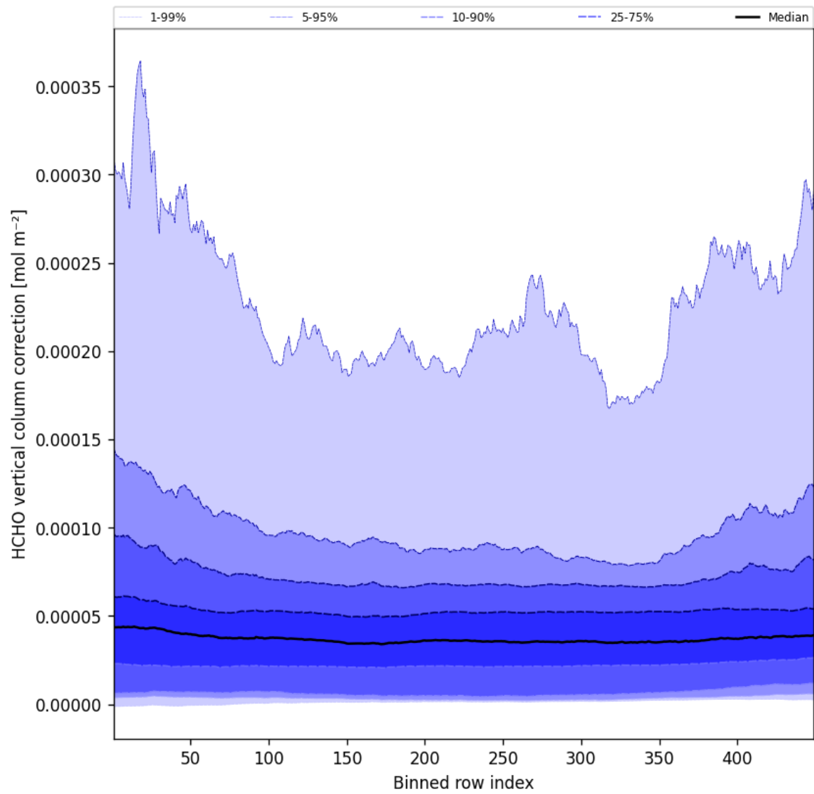
Figure 49: Along track statistics of “HCHO vertical column correction” for 2025-07-29 to 2025-07-30
