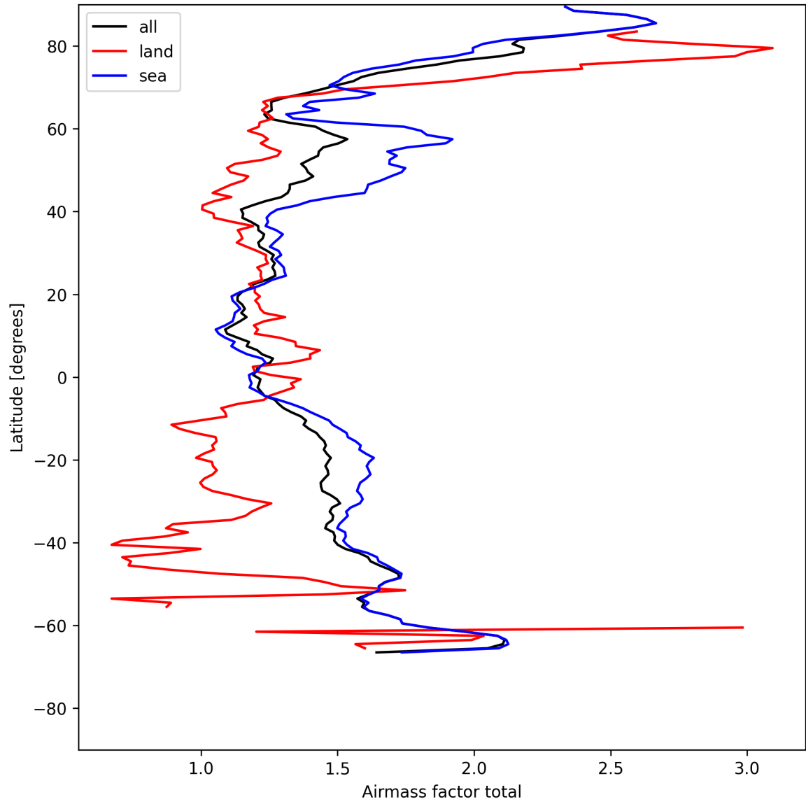
Figure 24: Zonal average of “Airmass factor total” for 2025-07-29 to 2025-07-30.
