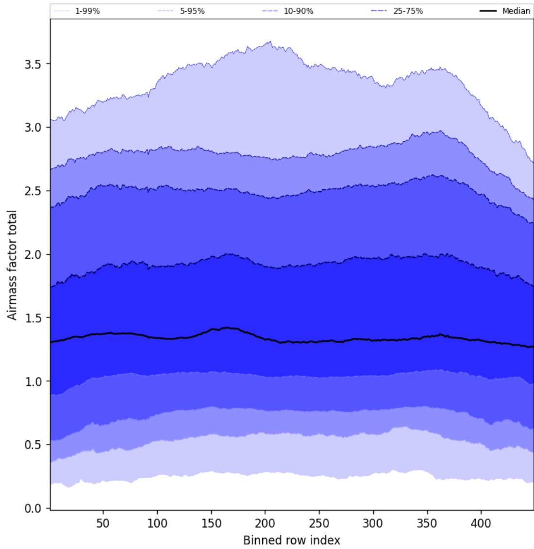
Figure 52: Along track statistics of “Airmass factor total” for 2025-07-29 to 2025-07-30
