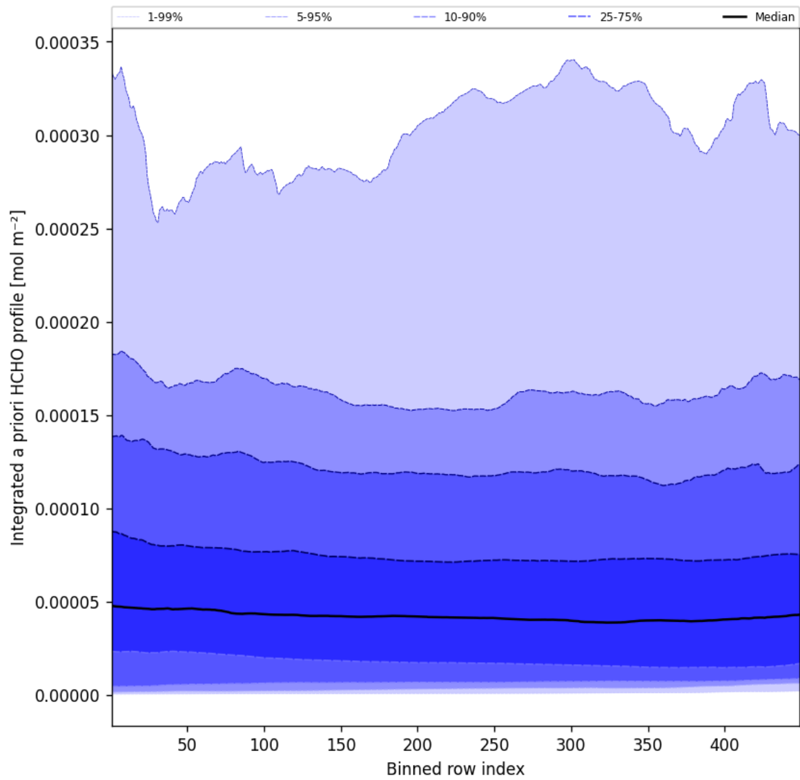
Figure 55: Along track statistics of “Integrated a priori HCHO profile” for 2025-07-29 to 2025-07-30
