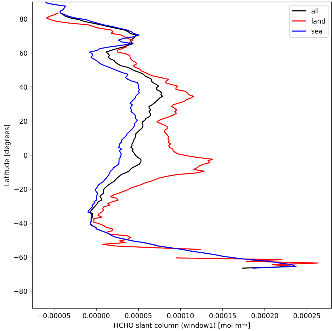
Figure 22: Zonal average of “HCHO slant column (window1)” for 2025-07-29 to 2025-07-30.
