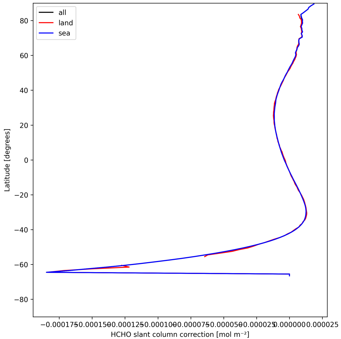
Figure 31: Zonal average of “HCHO slant column correction” for 2025-07-29 to 2025-07-30.
