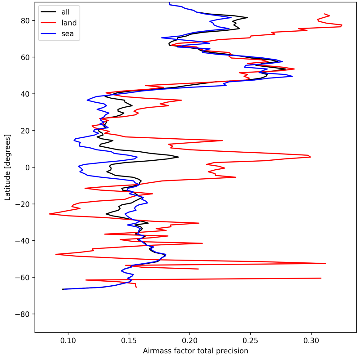
Figure 25: Zonal average of “Airmass factor total precision” for 2025-07-29 to 2025-07-30.
