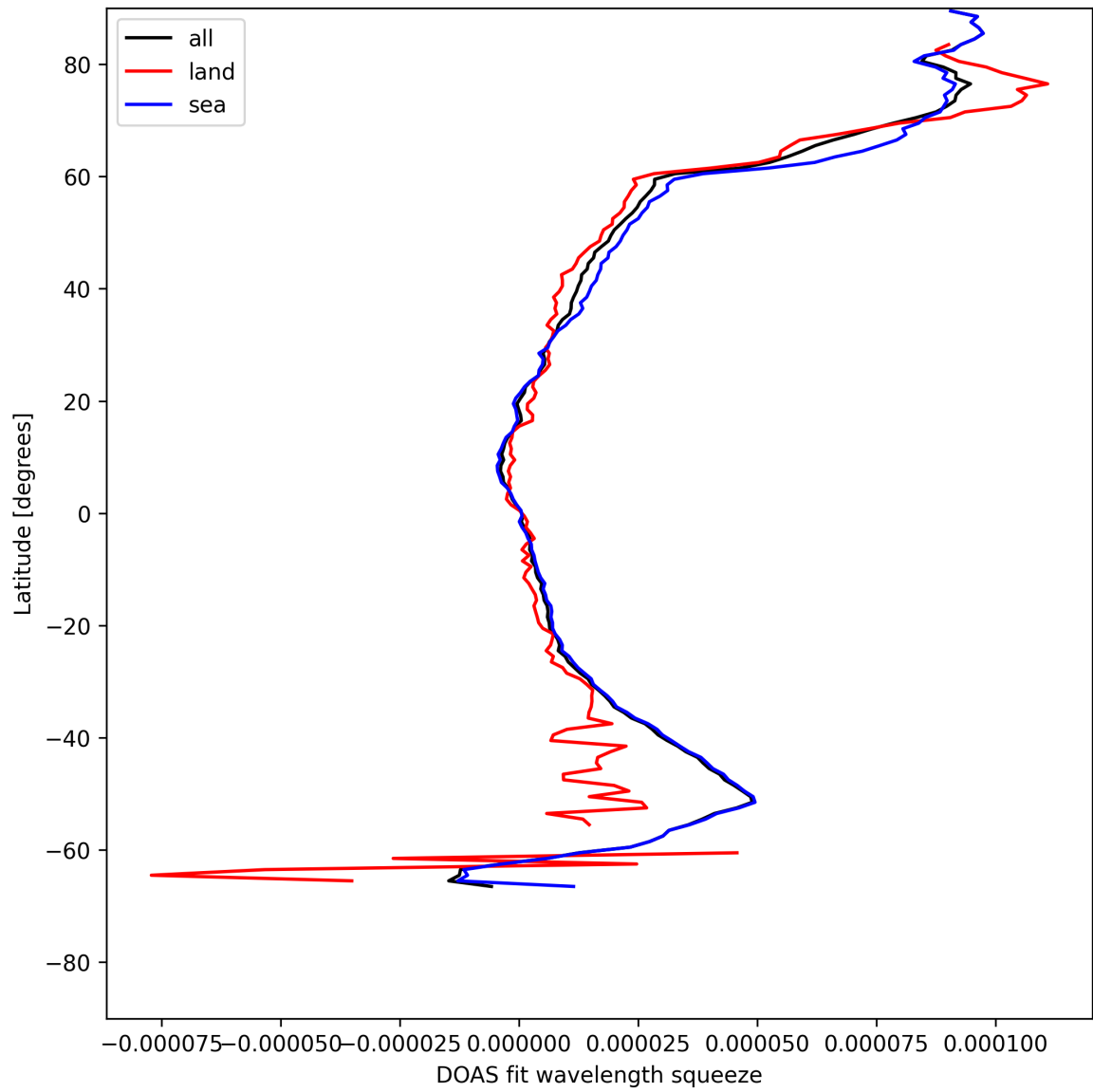
Figure 29: Zonal average of “DOAS fit wavelength squeeze” for 2025-07-29 to 2025-07-30.
