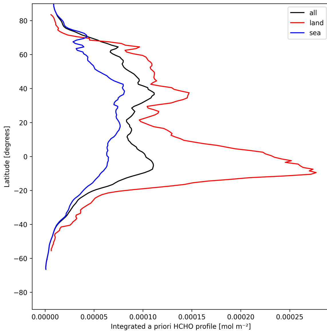
Figure 27: Zonal average of “Integrated a priori HCHO profile” for 2025-07-29 to 2025-07-30.
