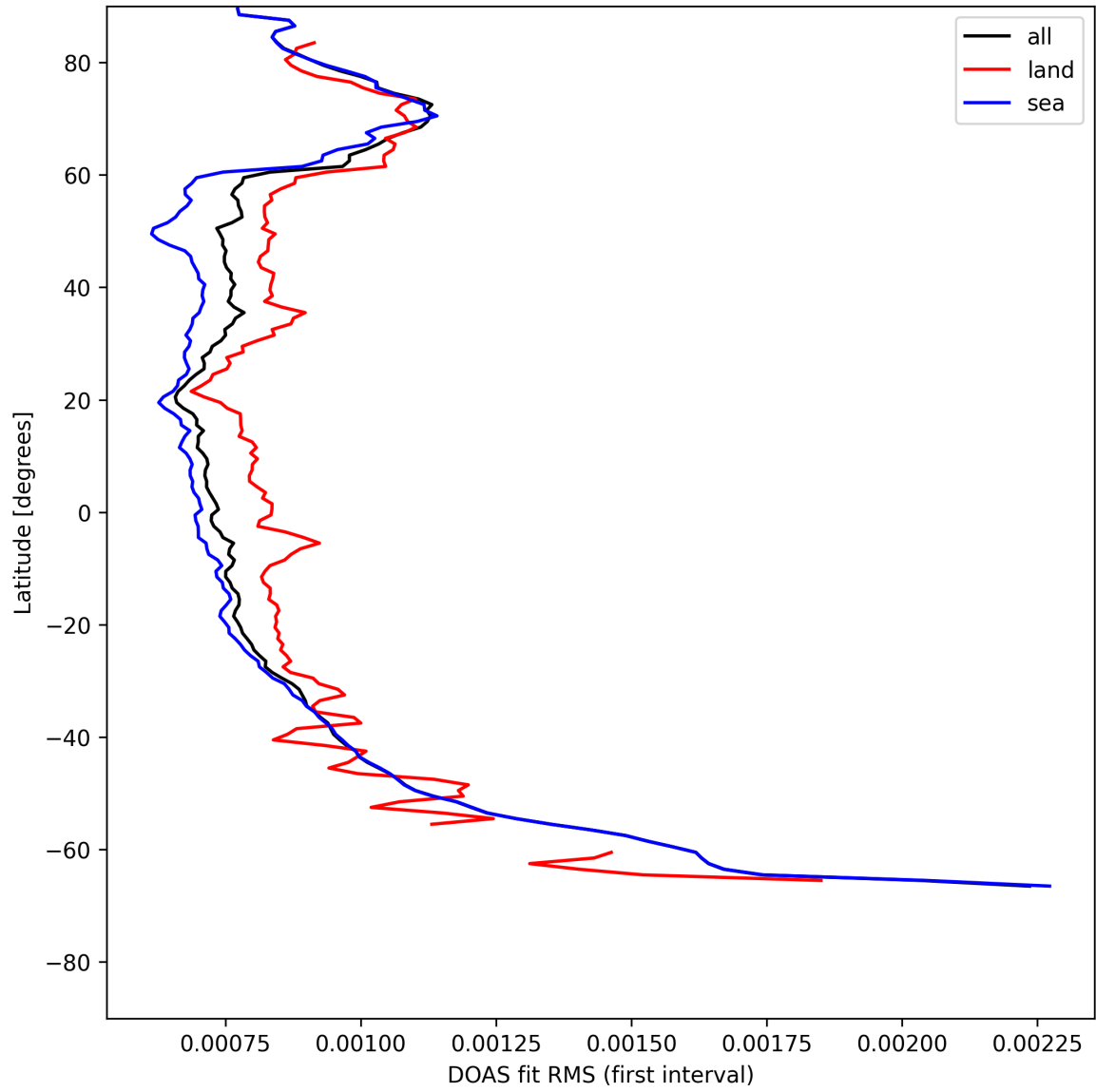
Figure 30: Zonal average of "DOAS fit RMS (first interval)" for 2025-07-29 to 2025-07-30.
