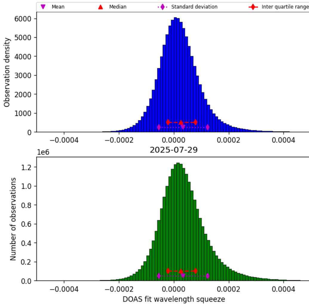
Figure 43: Histogram of “DOAS fit wavelength squeeze” for 2025-07-29 to 2025-07-30
