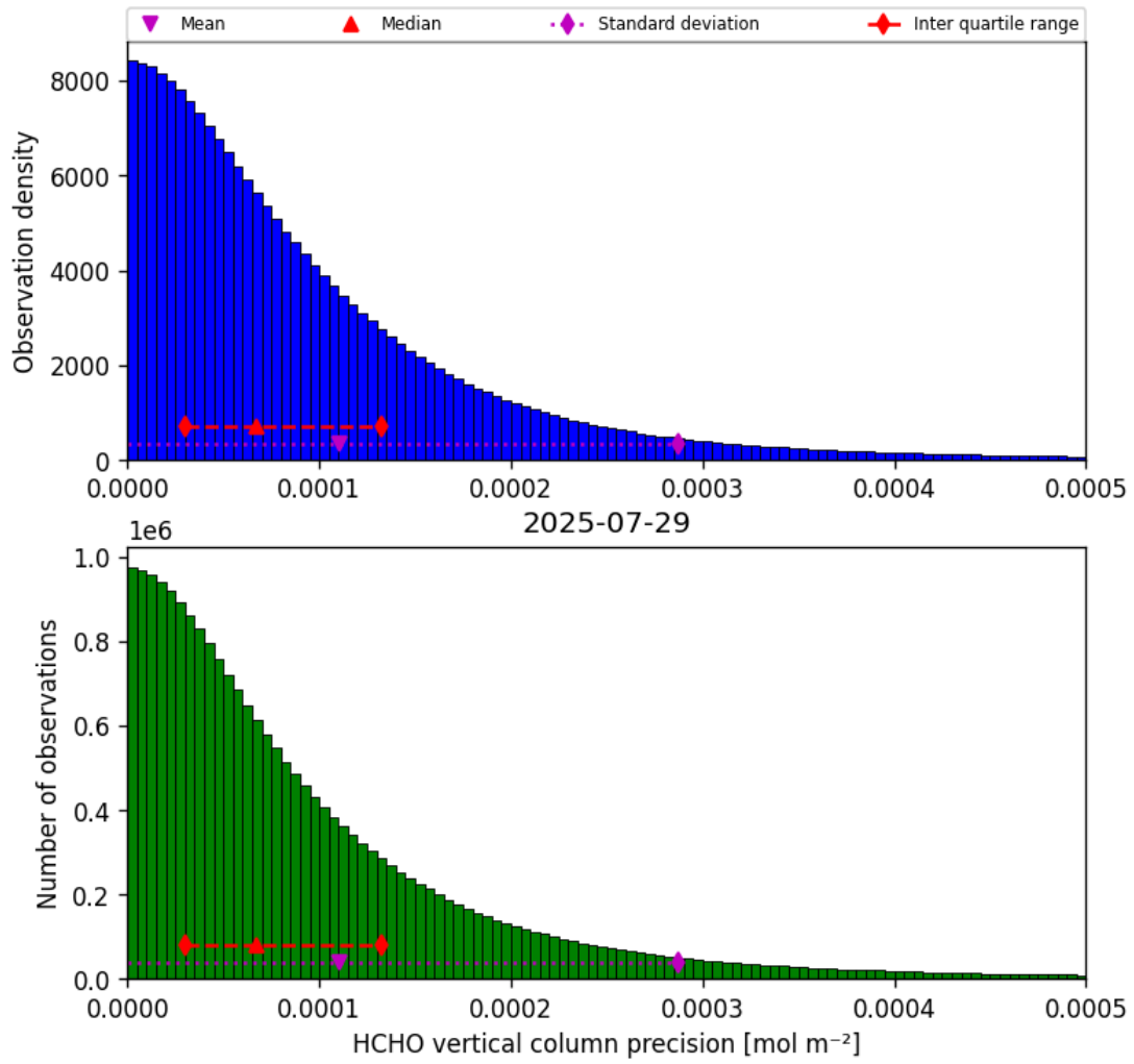
Figure 34: Histogram of “HCHO vertical column precision” for 2025-07-29 to 2025-07-30
