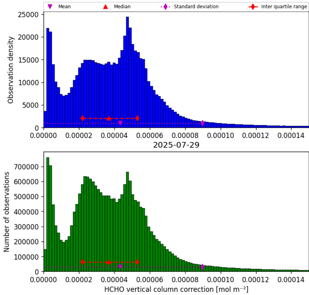
Figure 35: Histogram of “HCHO vertical column correction” for 2025-07-29 to 2025-07-30
