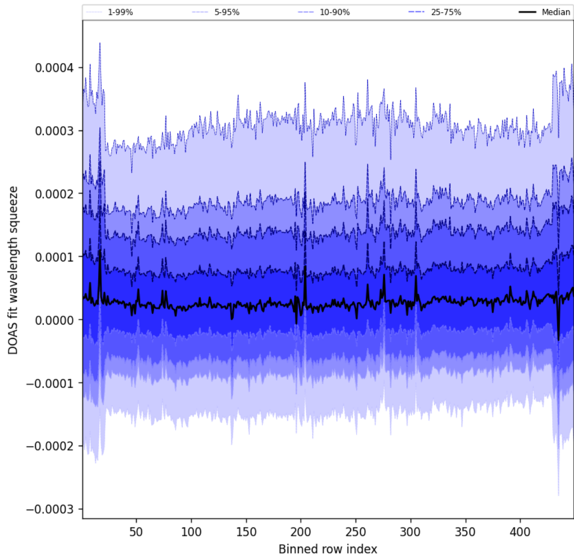
Figure 57: Along track statistics of “DOAS fit wavelength squeeze” for 2025-07-29 to 2025-07-30
