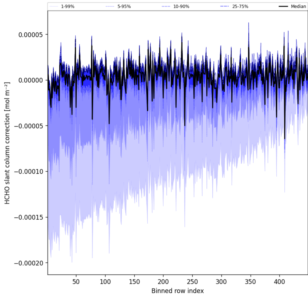
Figure 59: Along track statistics of “HCHO slant column correction” for 2025-07-29 to 2025-07-30
