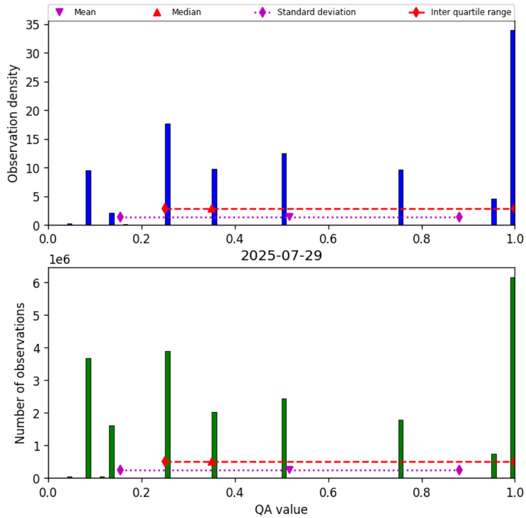
Figure 32: Histogram of “QA value” for 2025-07-29 to 2025-07-30
