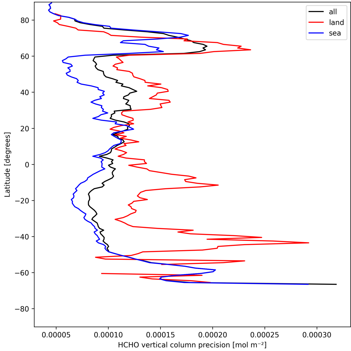
Figure 20: Zonal average of “HCHO vertical column precision” for 2025-07-29 to 2025-07-30.
