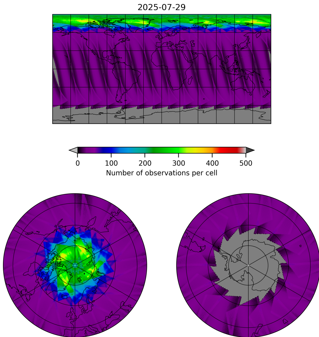
Figure 17: Map of the number of observations for 2025-07-29 to 2025-07-30
