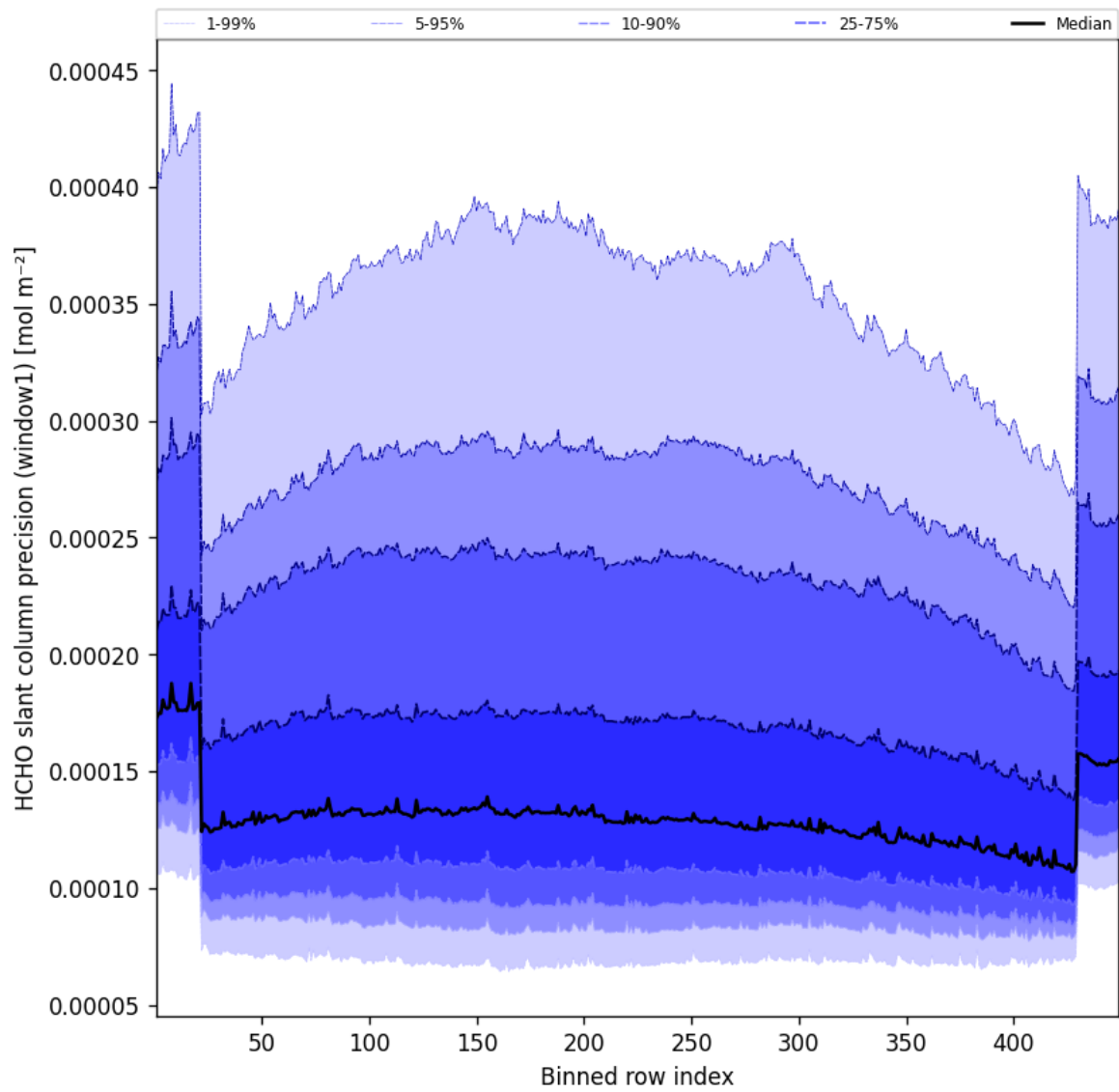
Figure 51: Along track statistics of “HCHO slant column precision (window1)” for 2025-07-29 to 2025-07-30
