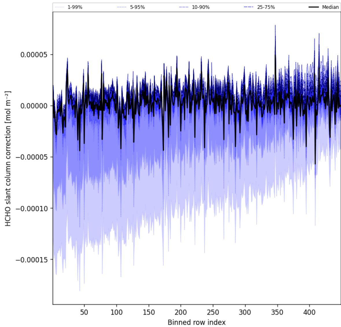
Figure 59: Along track statistics of “HCHO slant column correction” for 2025-07-30 to 2025-07-31
