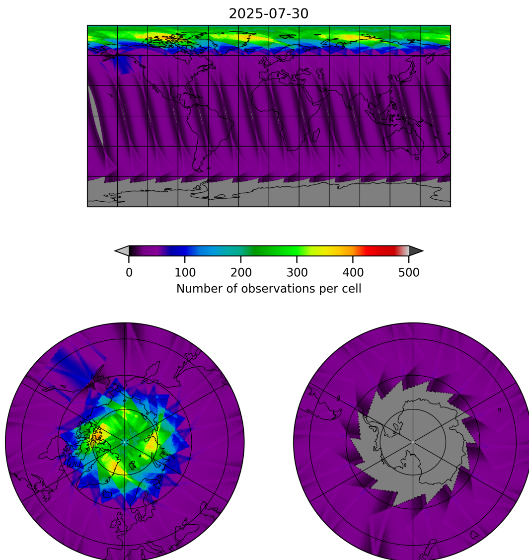
Figure 17: Map of the number of observations for 2025-07-30 to 2025-07-31
