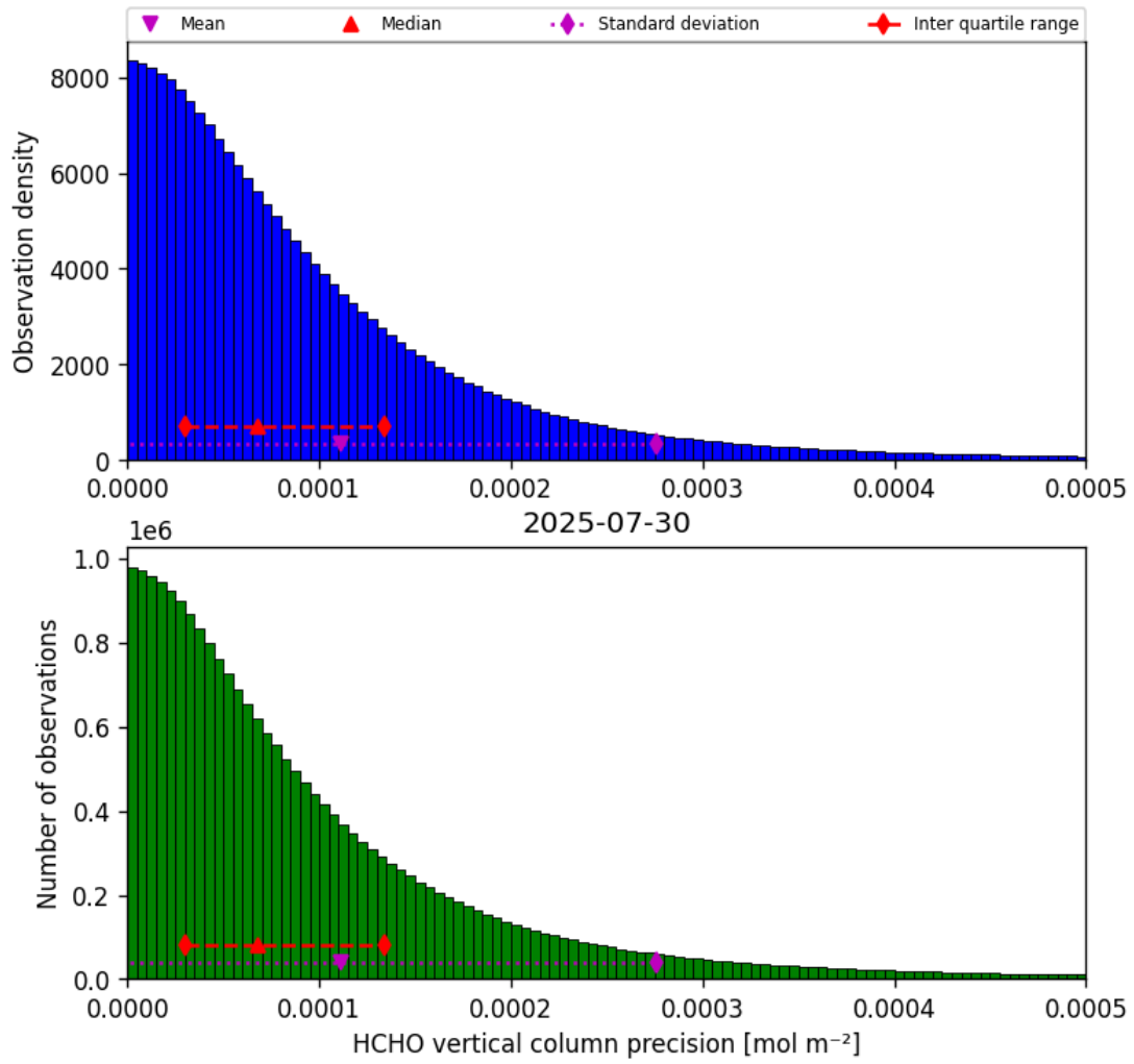
Figure 34: Histogram of “HCHO vertical column precision” for 2025-07-30 to 2025-07-31
