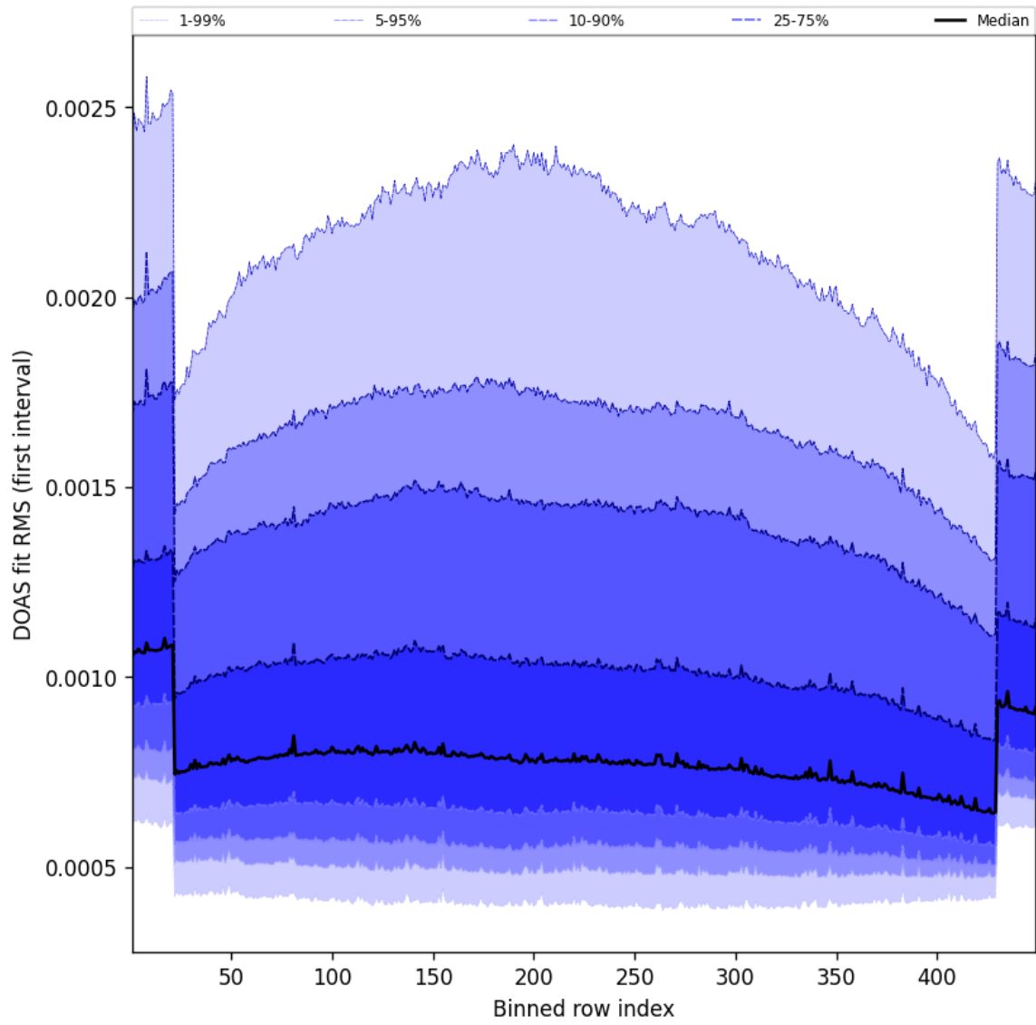
Figure 58: Along track statistics of “DOAS fit RMS (first interval)” for 2025-07-30 to 2025-07-31
