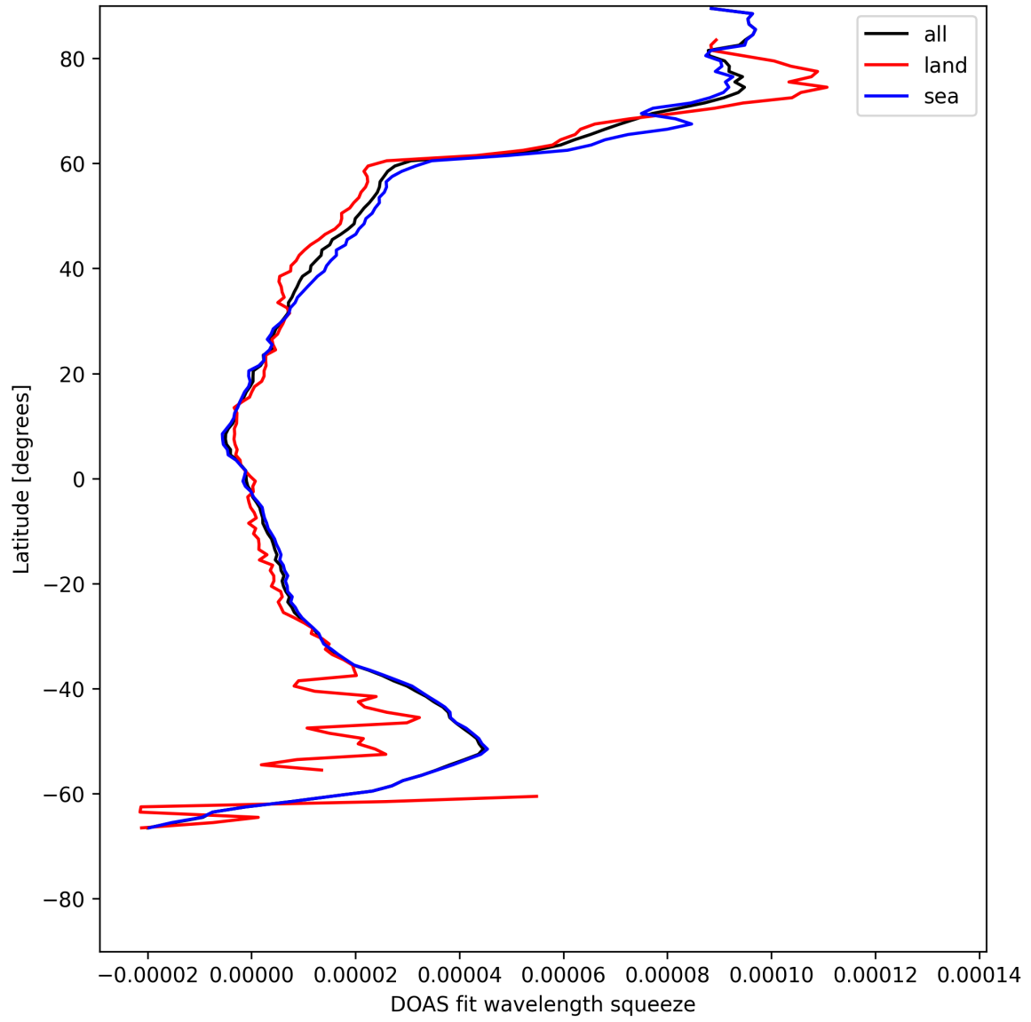
Figure 29: Zonal average of “DOAS fit wavelength squeeze” for 2025-07-30 to 2025-07-31.
