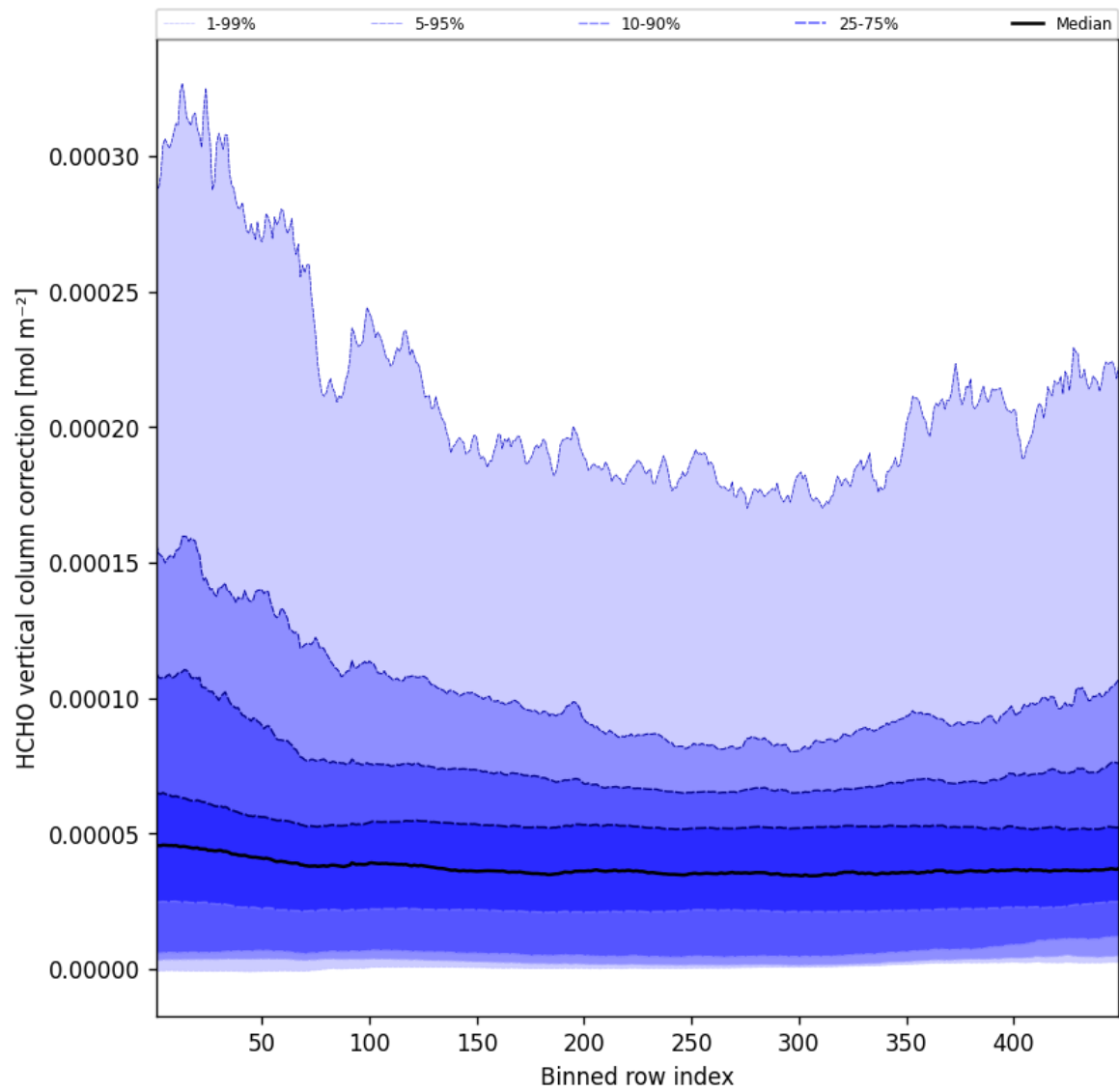
Figure 49: Along track statistics of “HCHO vertical column correction” for 2025-07-30 to 2025-07-31
