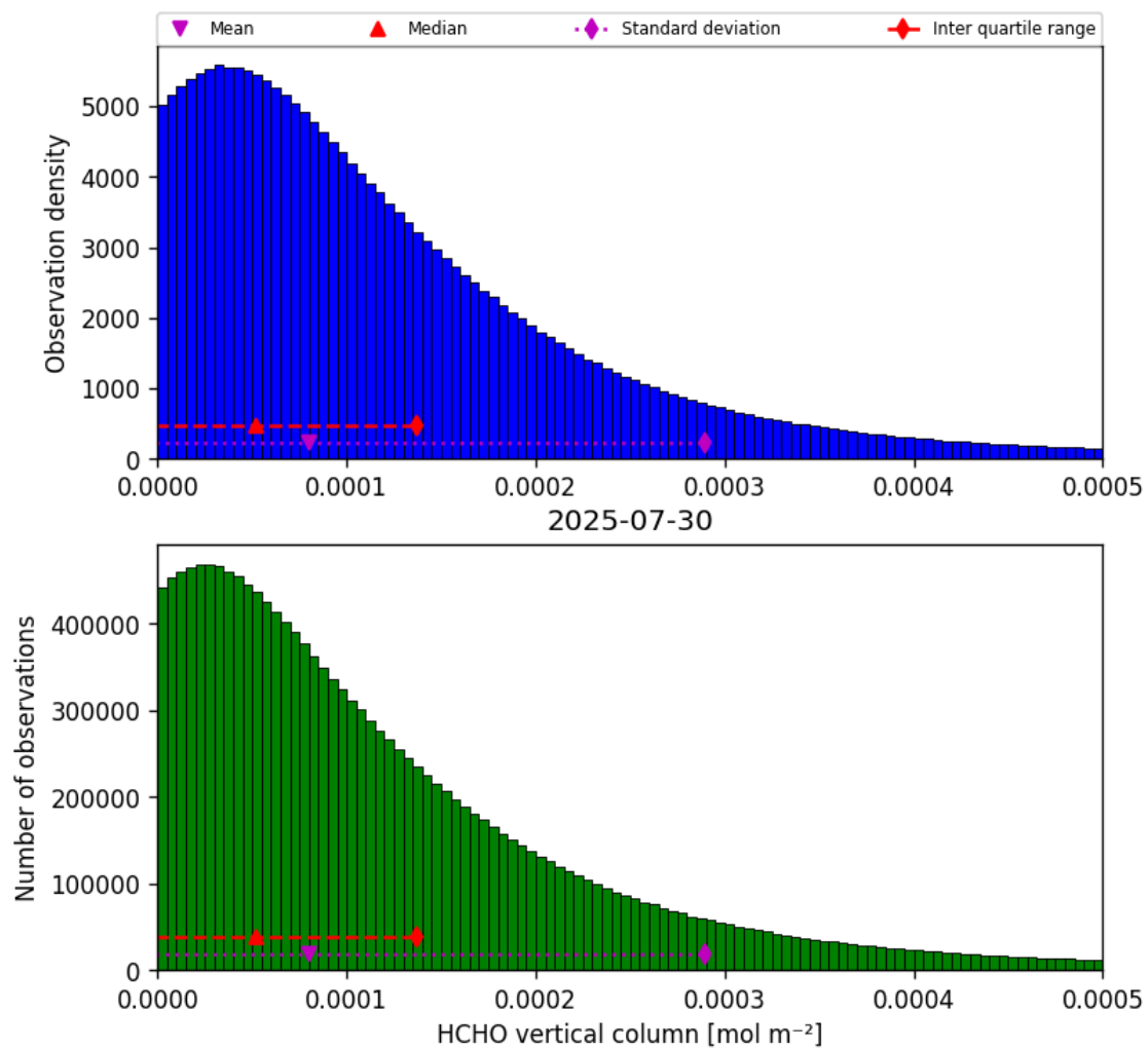
Figure 33: Histogram of “HCHO vertical column” for 2025-07-30 to 2025-07-31
