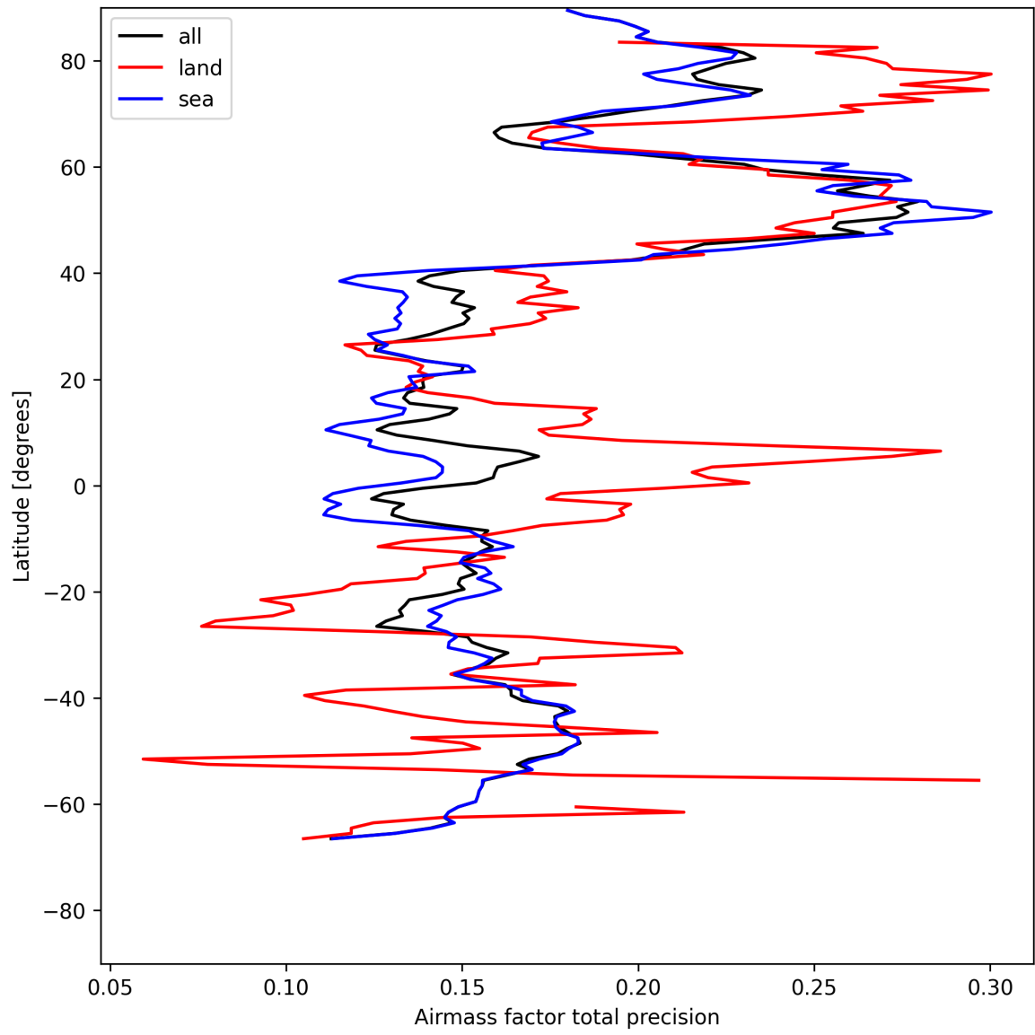
Figure 25: Zonal average of “Airmass factor total precision” for 2025-07-30 to 2025-07-31.
