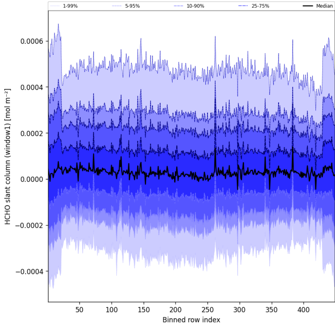
Figure 50: Along track statistics of “HCHO slant column (window1)” for 2025-07-30 to 2025-07-31
