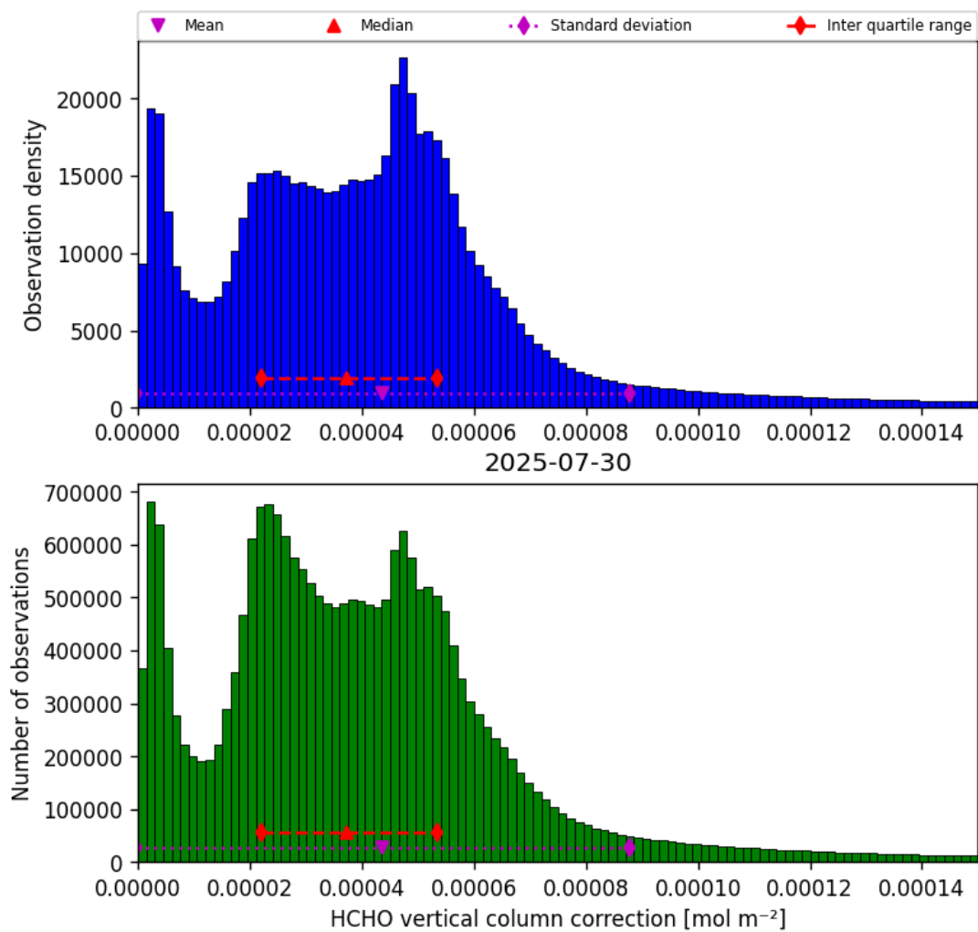
Figure 35: Histogram of “HCHO vertical column correction” for 2025-07-30 to 2025-07-31
