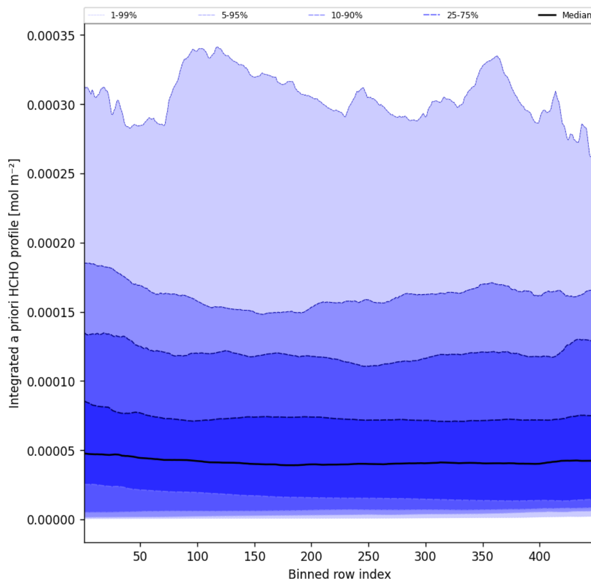
Figure 55: Along track statistics of "Integrated a priori HCHO profile" for 2025-07-30 to 2025-07-31
