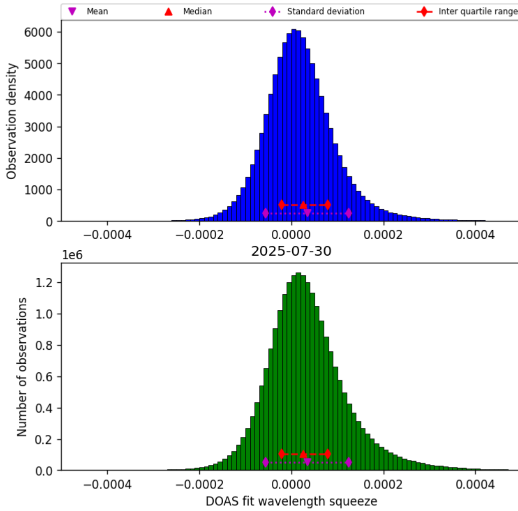
Figure 43: Histogram of “DOAS fit wavelength squeeze” for 2025-07-30 to 2025-07-31
