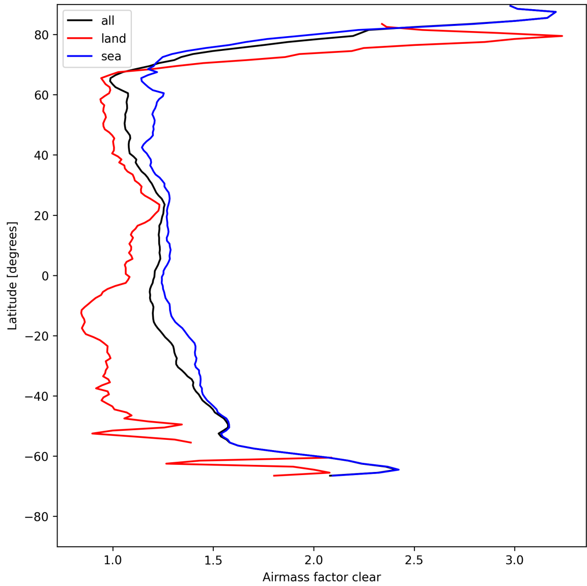
Figure 26: Zonal average of “Airmass factor clear” for 2025-07-30 to 2025-07-31.
