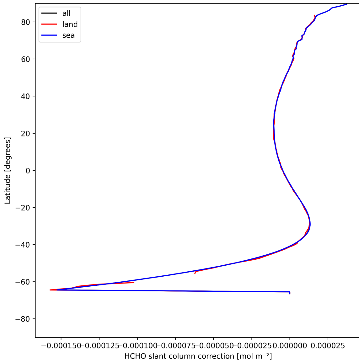
Figure 31: Zonal average of “HCHO slant column correction” for 2025-07-30 to 2025-07-31.
