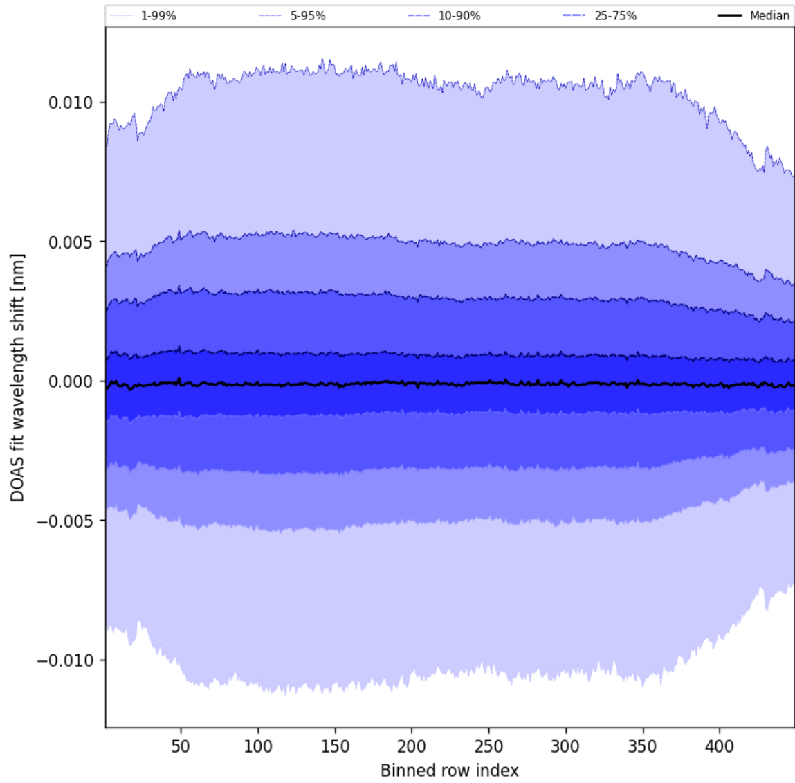
Figure 56: Along track statistics of “DOAS fit wavelength shift” for 2025-07-30 to 2025-07-31
