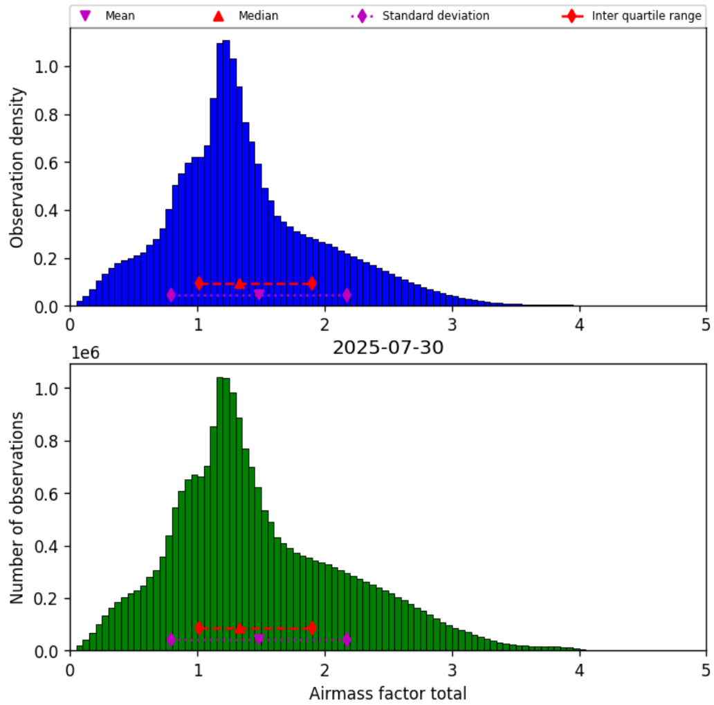
Figure 38: Histogram of “Airmass factor total” for 2025-07-30 to 2025-07-31
