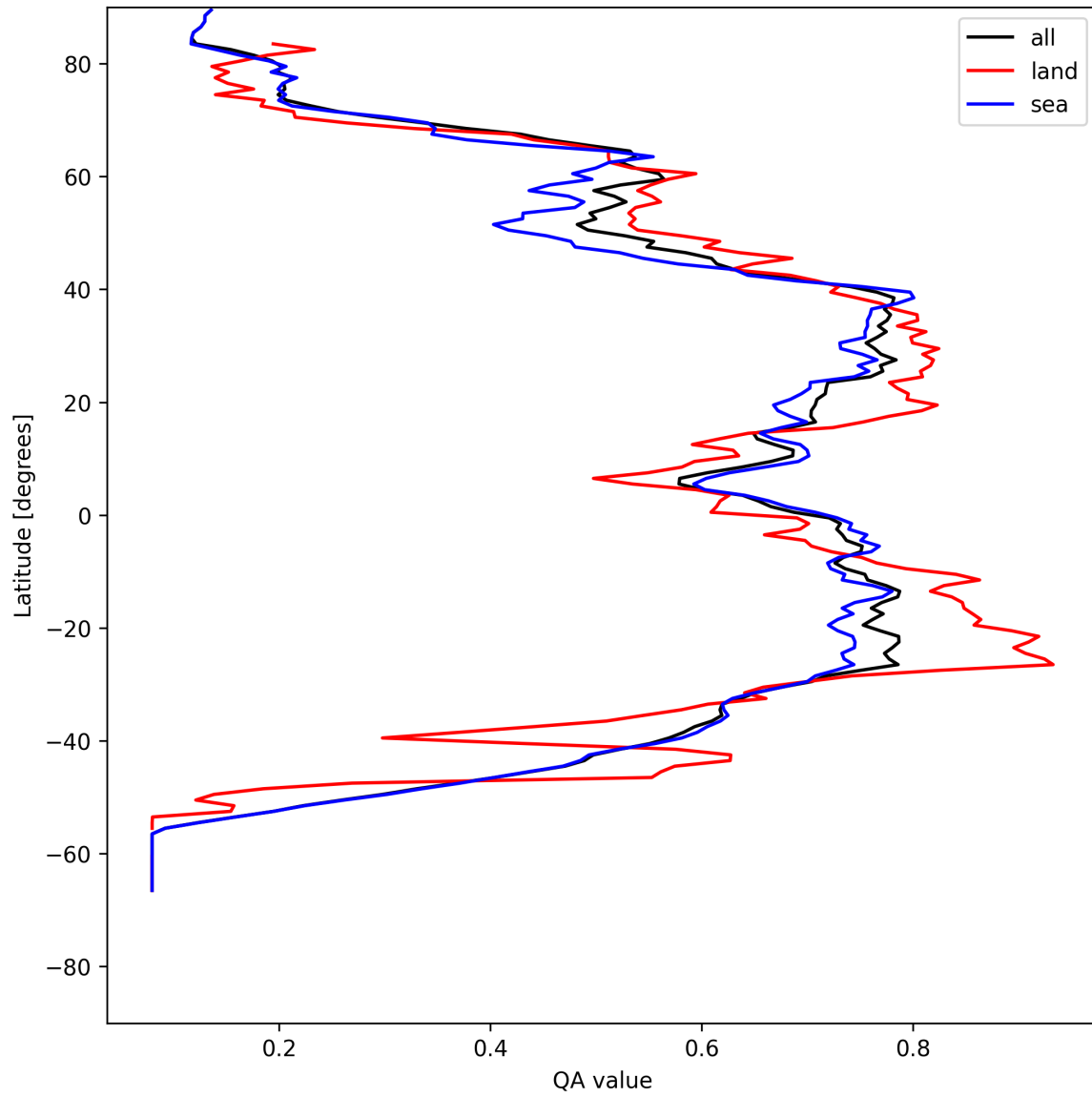
Figure 18: Zonal average of “QA value” for 2025-07-30 to 2025-07-31.
