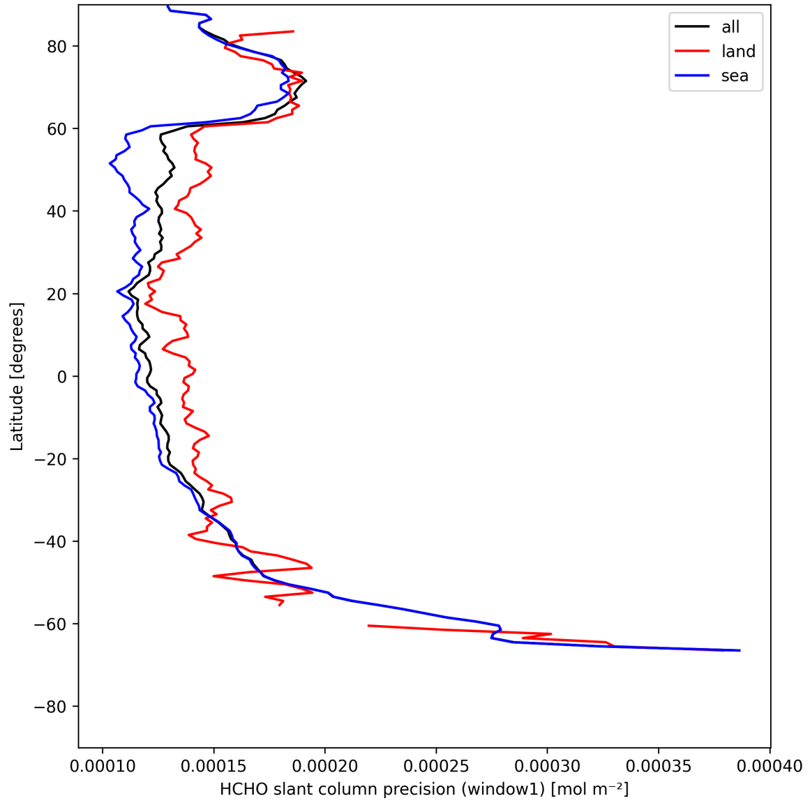
Figure 23: Zonal average of “HCHO slant column precision (window1)” for 2025-07-30 to 2025-07-31.
