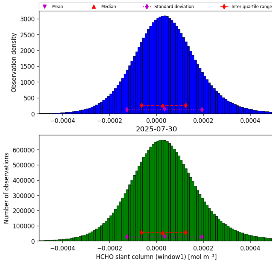
Figure 36: Histogram of “HCHO slant column (window1)” for 2025-07-30 to 2025-07-31
