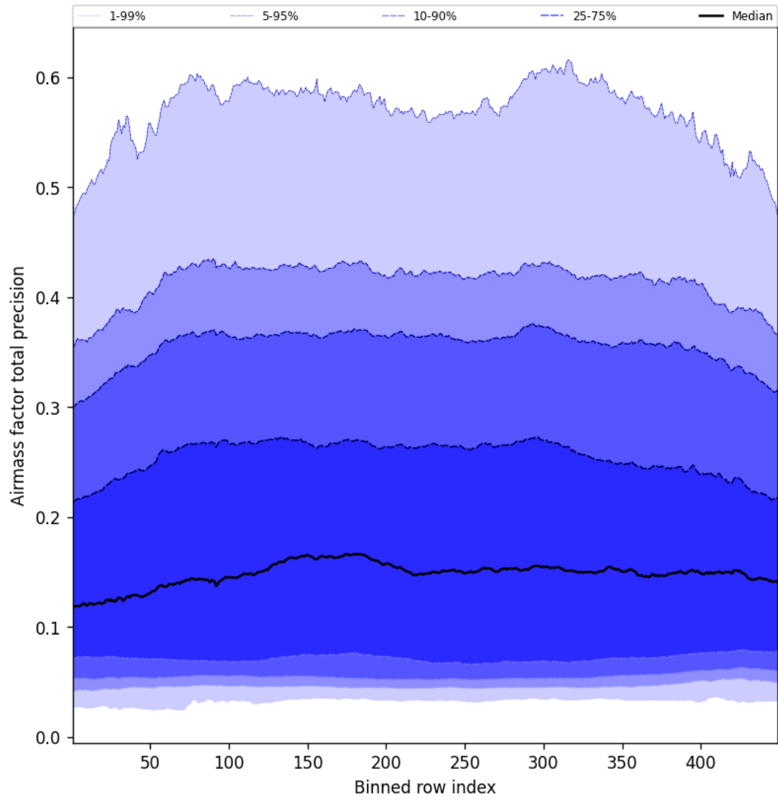
Figure 53: Along track statistics of “Airmass factor total precision” for 2025-07-30 to 2025-07-31
