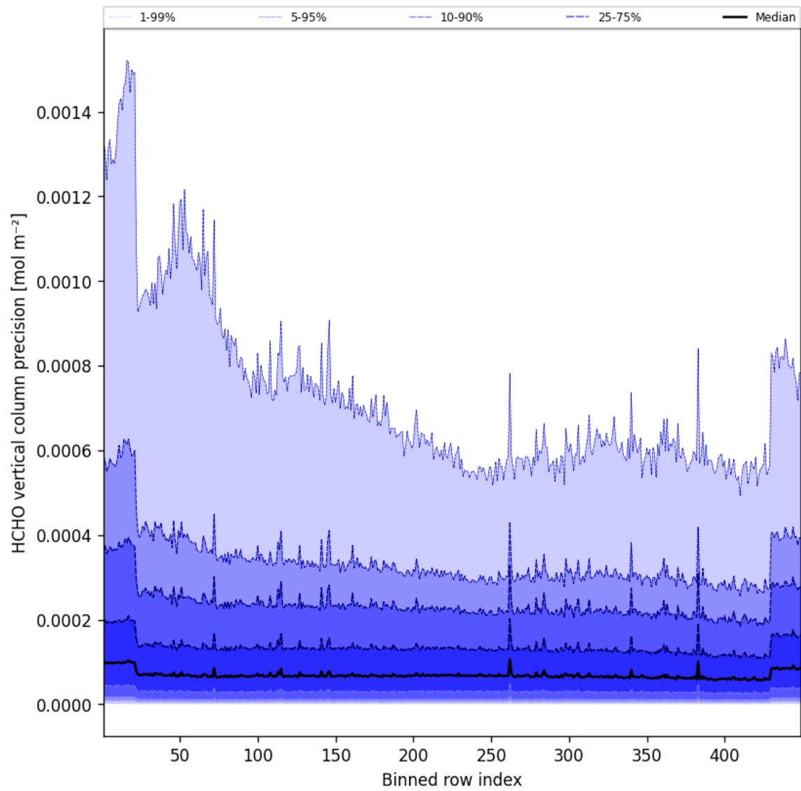
Figure 48: Along track statistics of “HCHO vertical column precision” for 2025-07-30 to 2025-07-31
