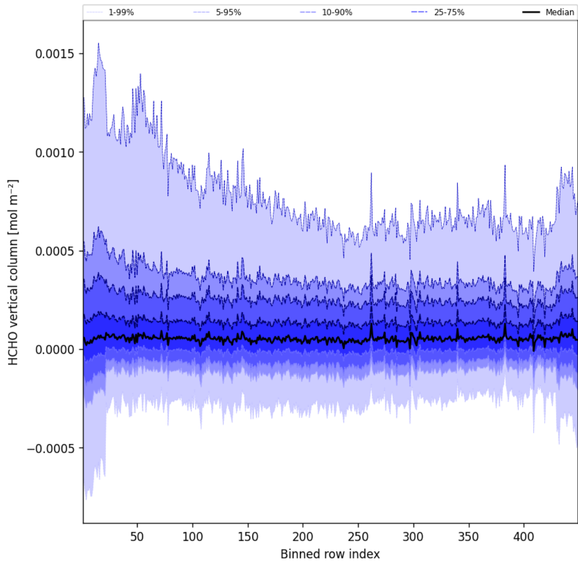
Figure 47: Along track statistics of “HCHO vertical column” for 2025-07-30 to 2025-07-31
