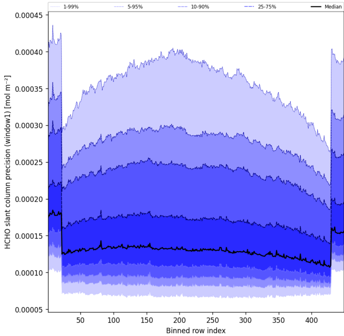
Figure 51: Along track statistics of “HCHO slant column precision (window1)” for 2025-07-30 to 2025-07-31
