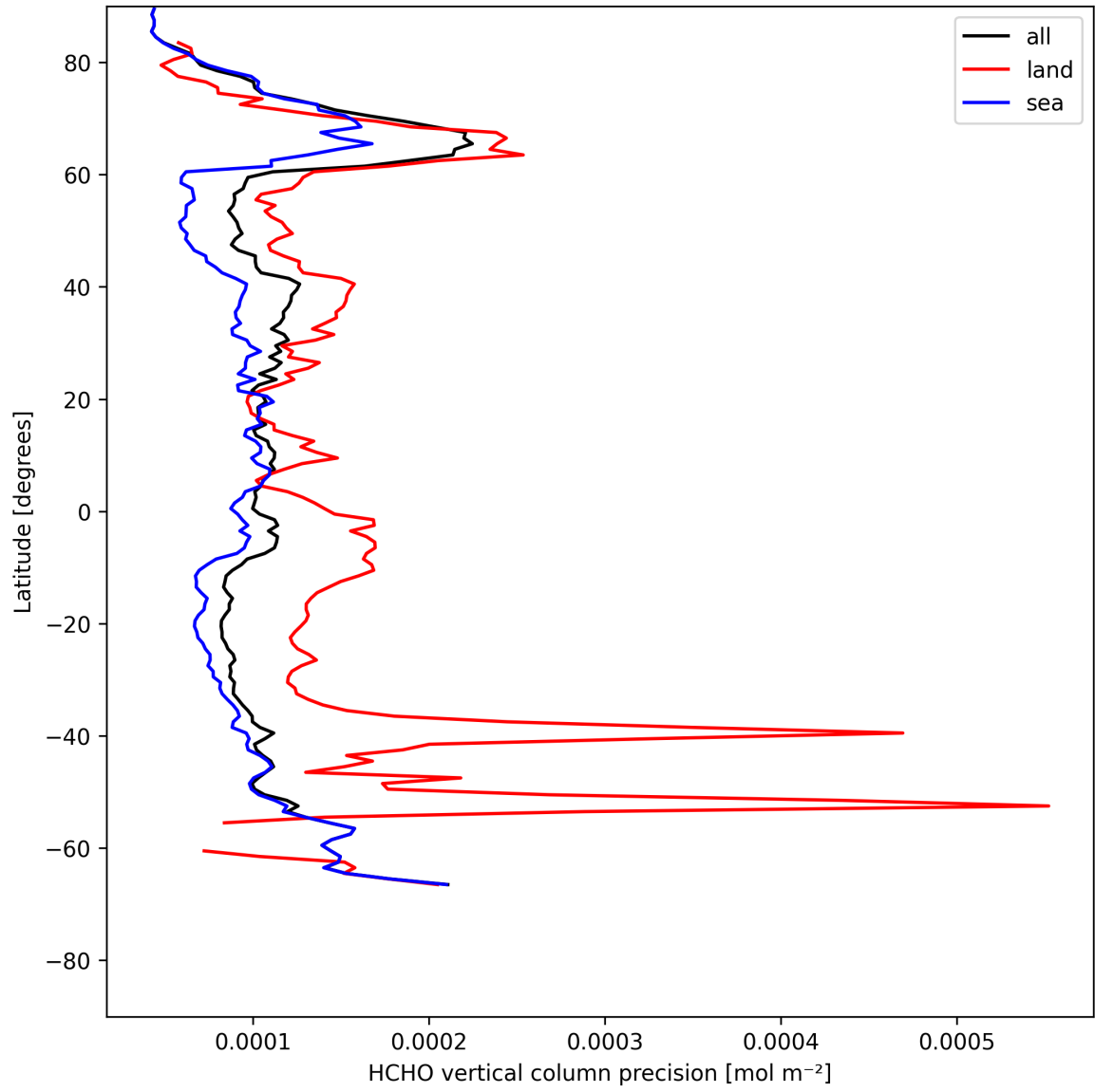
Figure 20: Zonal average of “HCHO vertical column precision” for 2025-07-30 to 2025-07-31.
