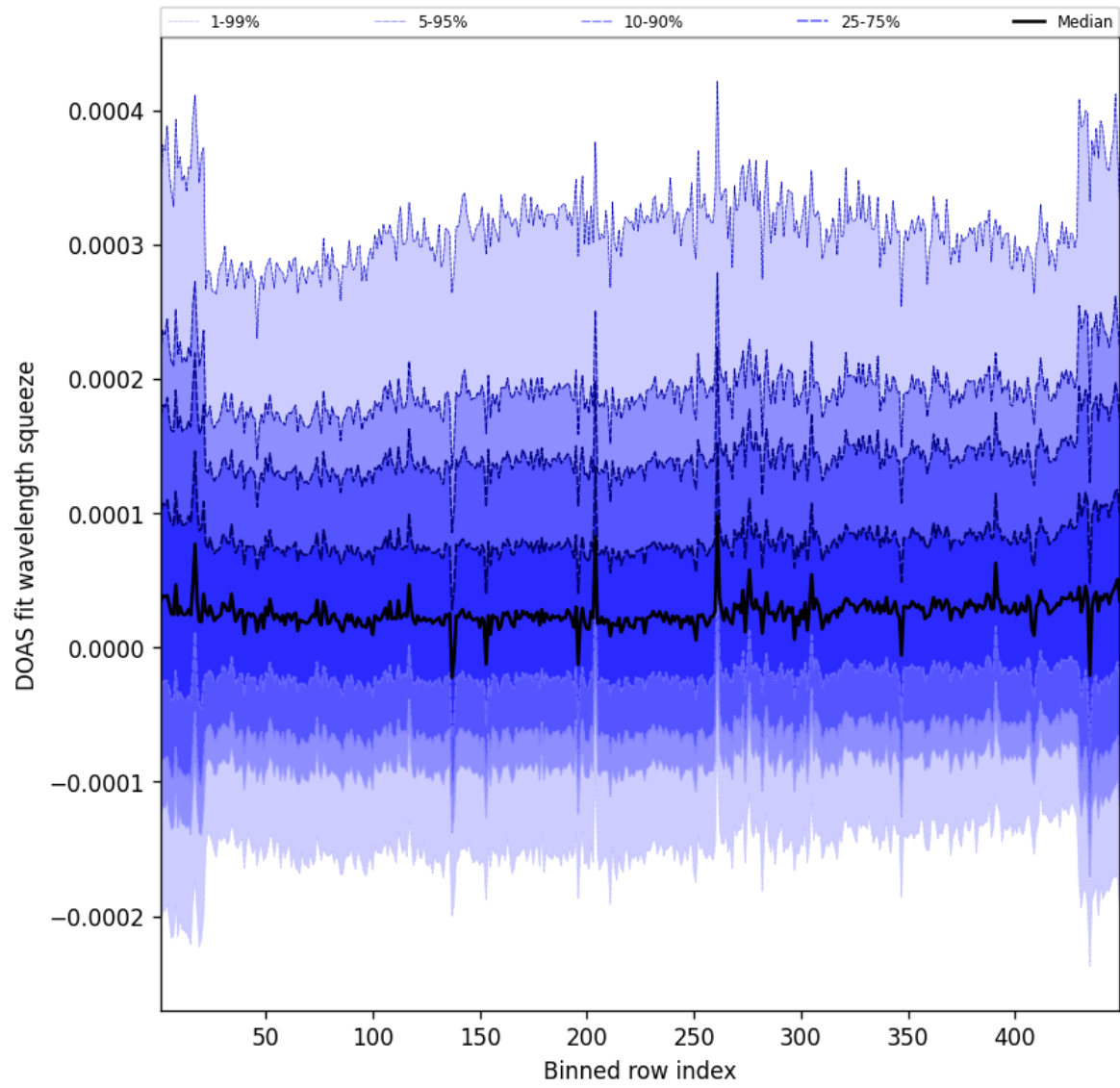
Figure 57: Along track statistics of “DOAS fit wavelength squeeze” for 2025-07-30 to 2025-07-31
