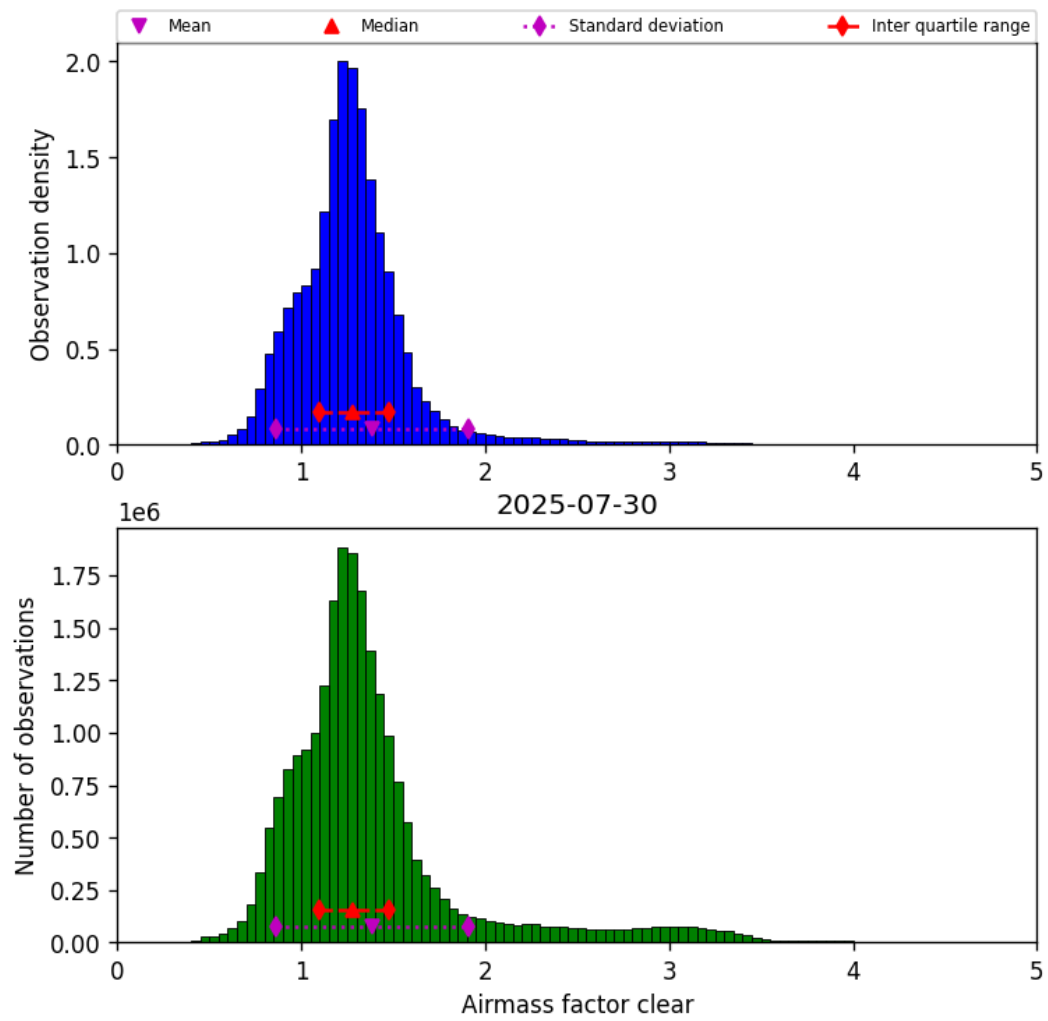
Figure 40: Histogram of “Airmass factor clear” for 2025-07-30 to 2025-07-31
