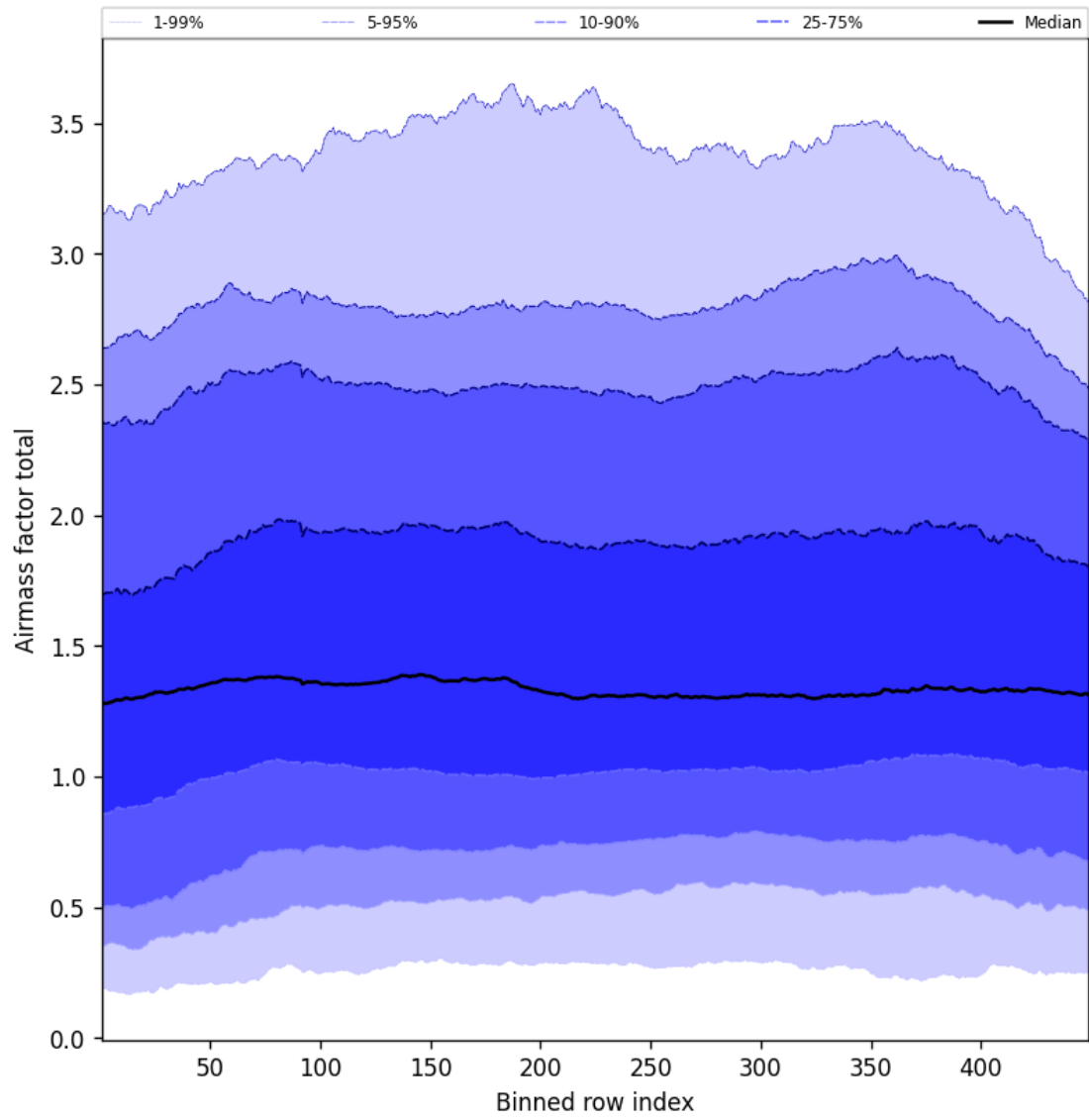
Figure 52: Along track statistics of “Airmass factor total” for 2025-07-30 to 2025-07-31
