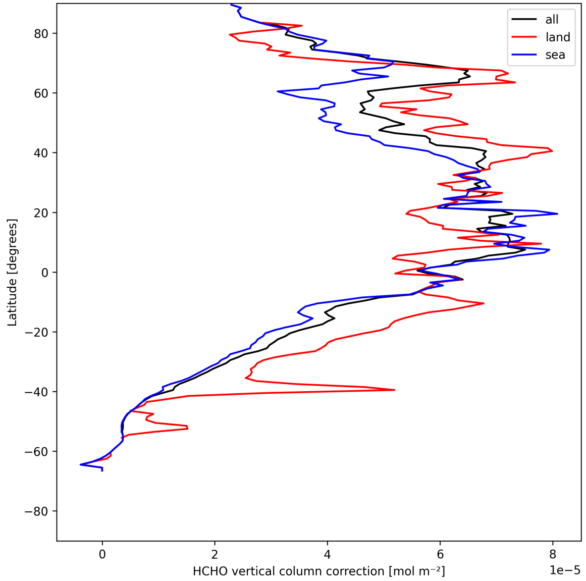
Figure 21: Zonal average of “HCHO vertical column correction” for 2025-07-30 to 2025-07-31.
