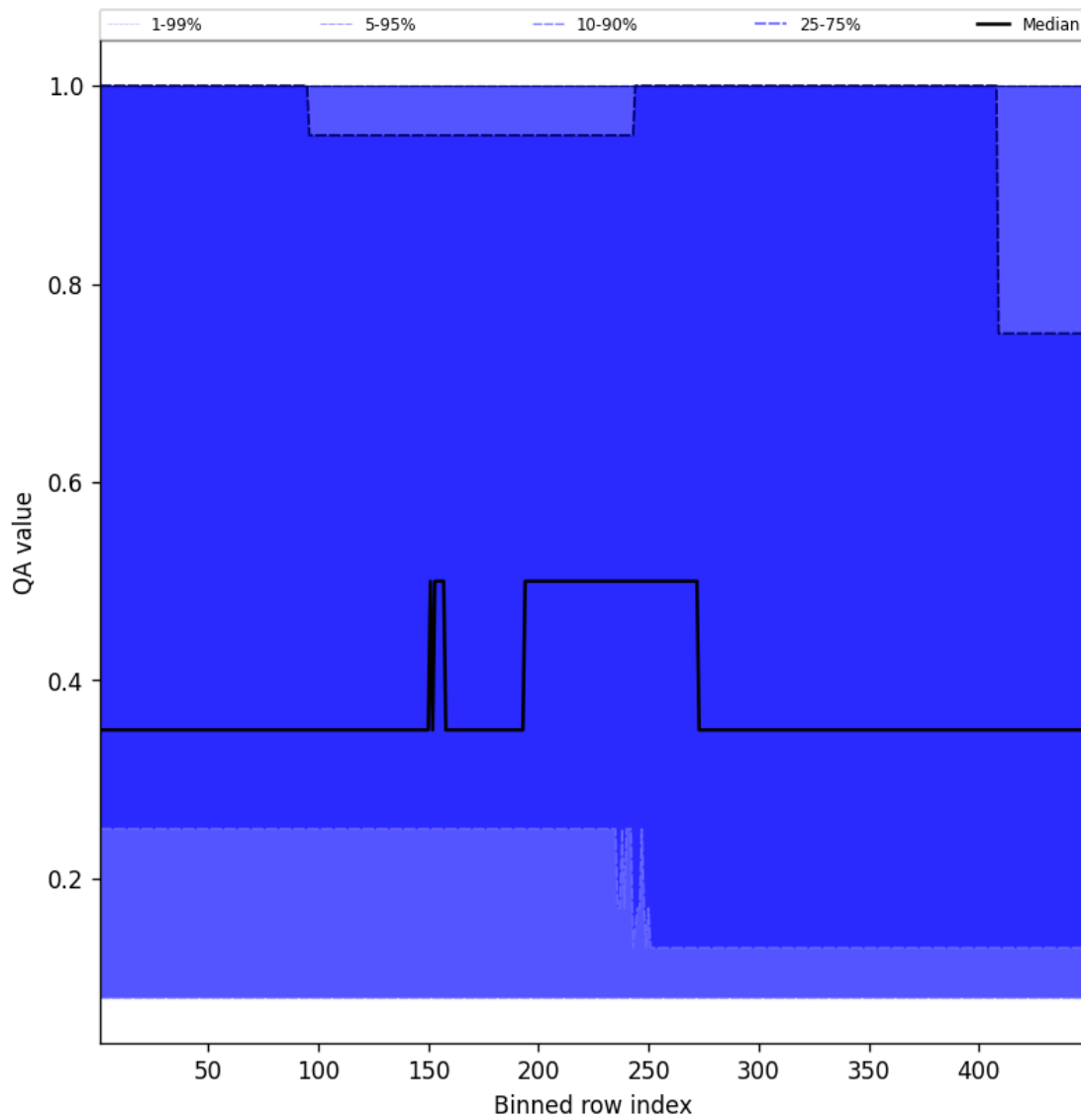
Figure 46: Along track statistics of “QA value” for 2025-07-30 to 2025-07-31
