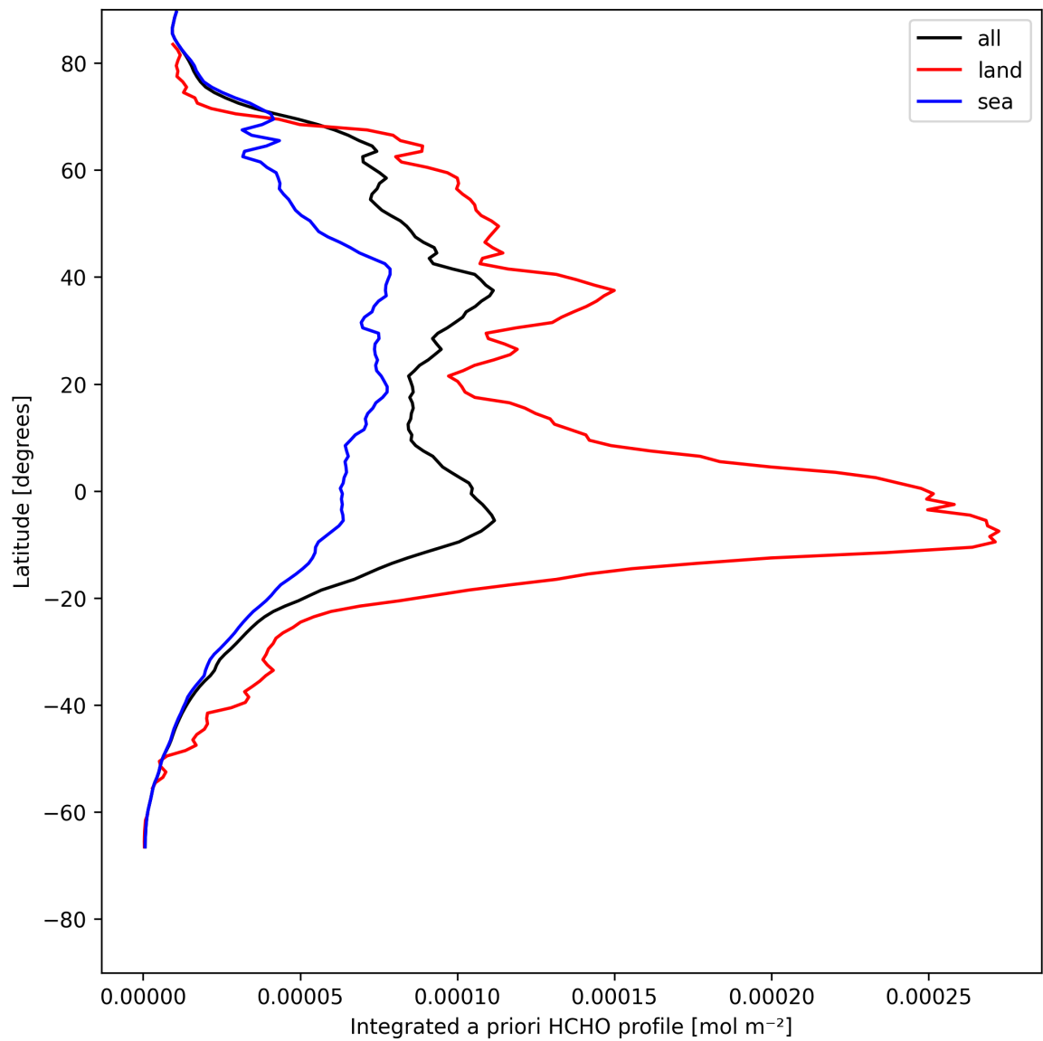
Figure 27: Zonal average of “Integrated a priori HCHO profile” for 2025-07-30 to 2025-07-31.
