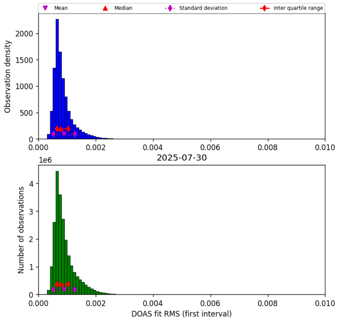
Figure 44: Histogram of “DOAS fit RMS (first interval)” for 2025-07-30 to 2025-07-31
