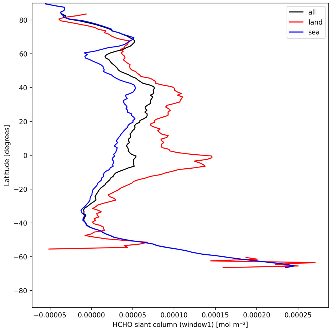
Figure 22: Zonal average of “HCHO slant column (window1)” for 2025-07-30 to 2025-07-31.
