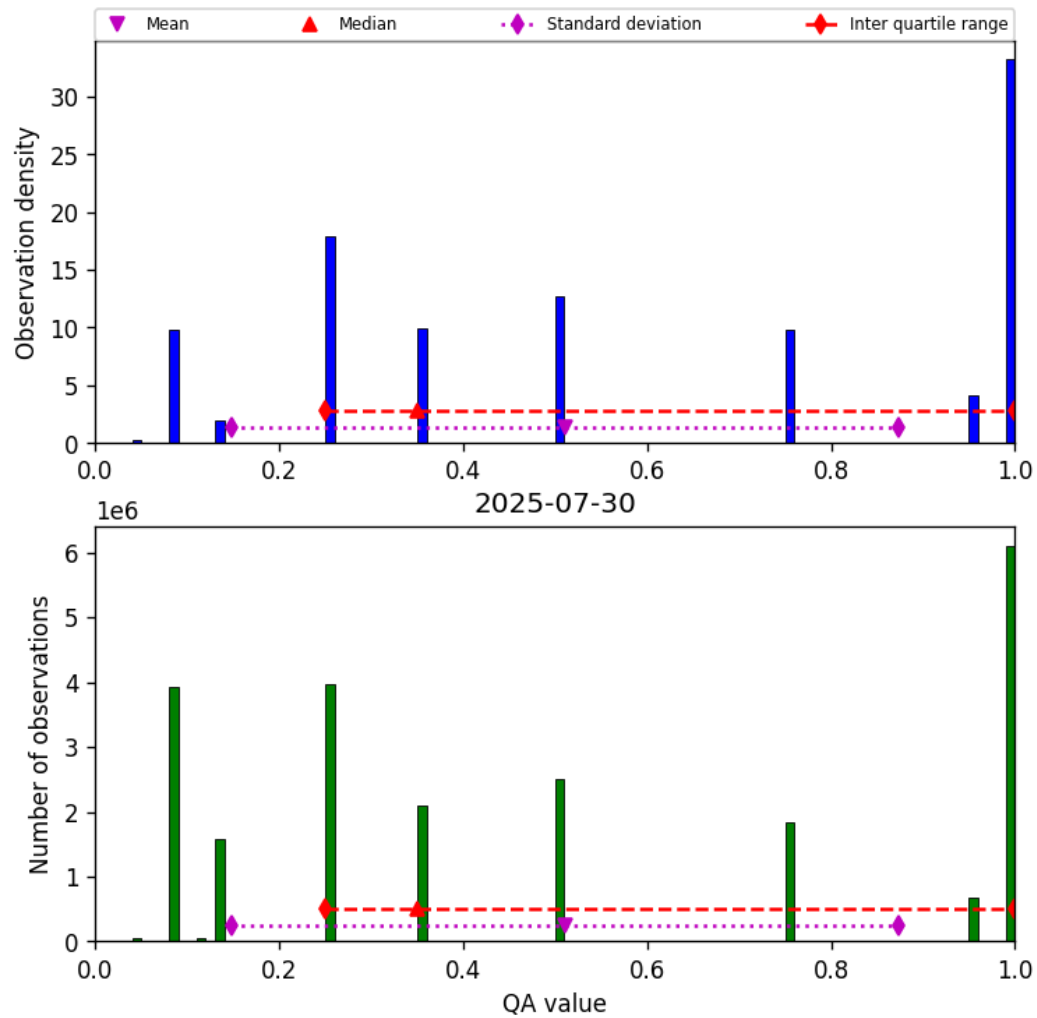
Figure 32: Histogram of “QA value” for 2025-07-30 to 2025-07-31
