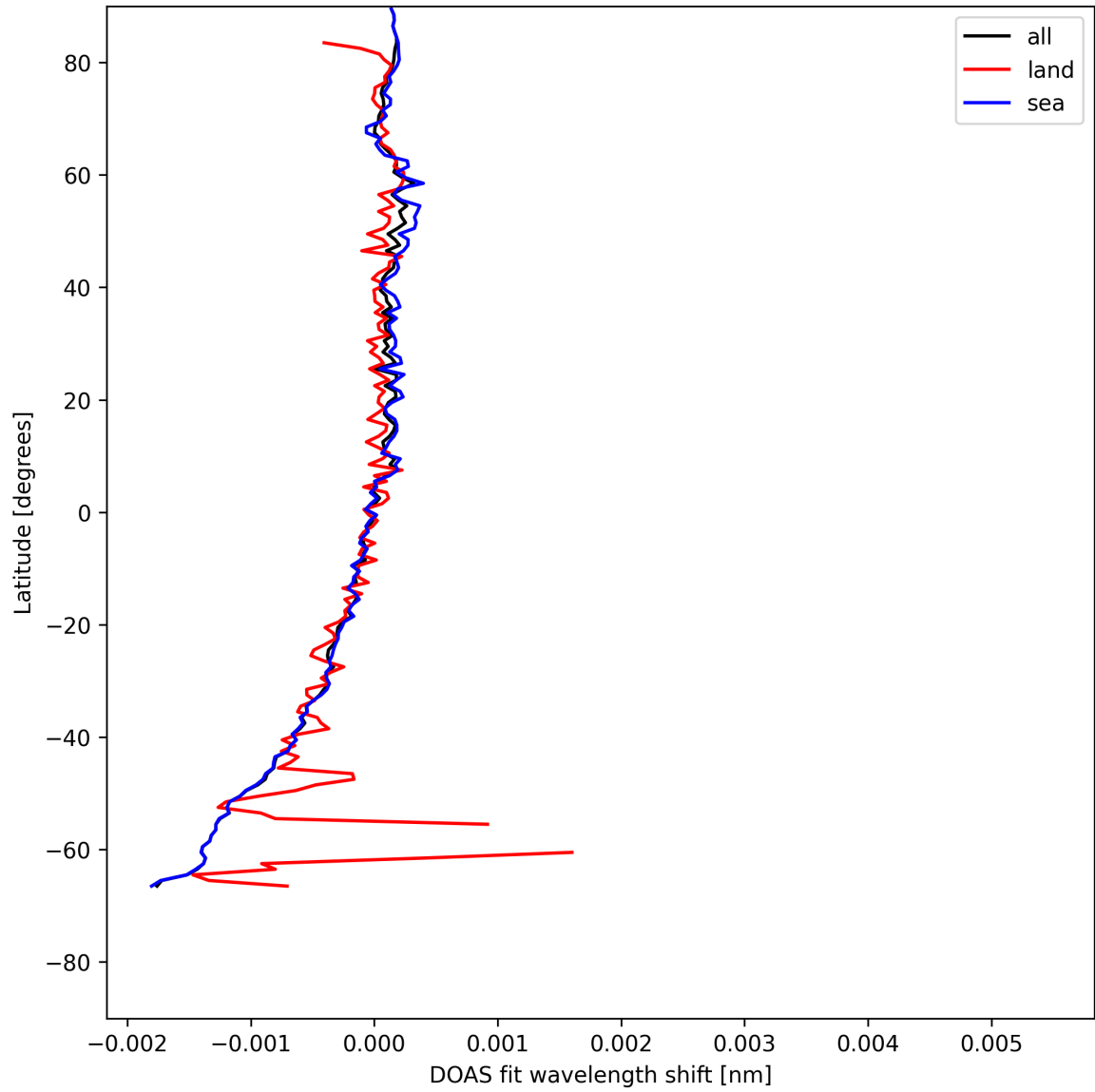
Figure 28: Zonal average of "DOAS fit wavelength shift" for 2025-07-30 to 2025-07-31.
