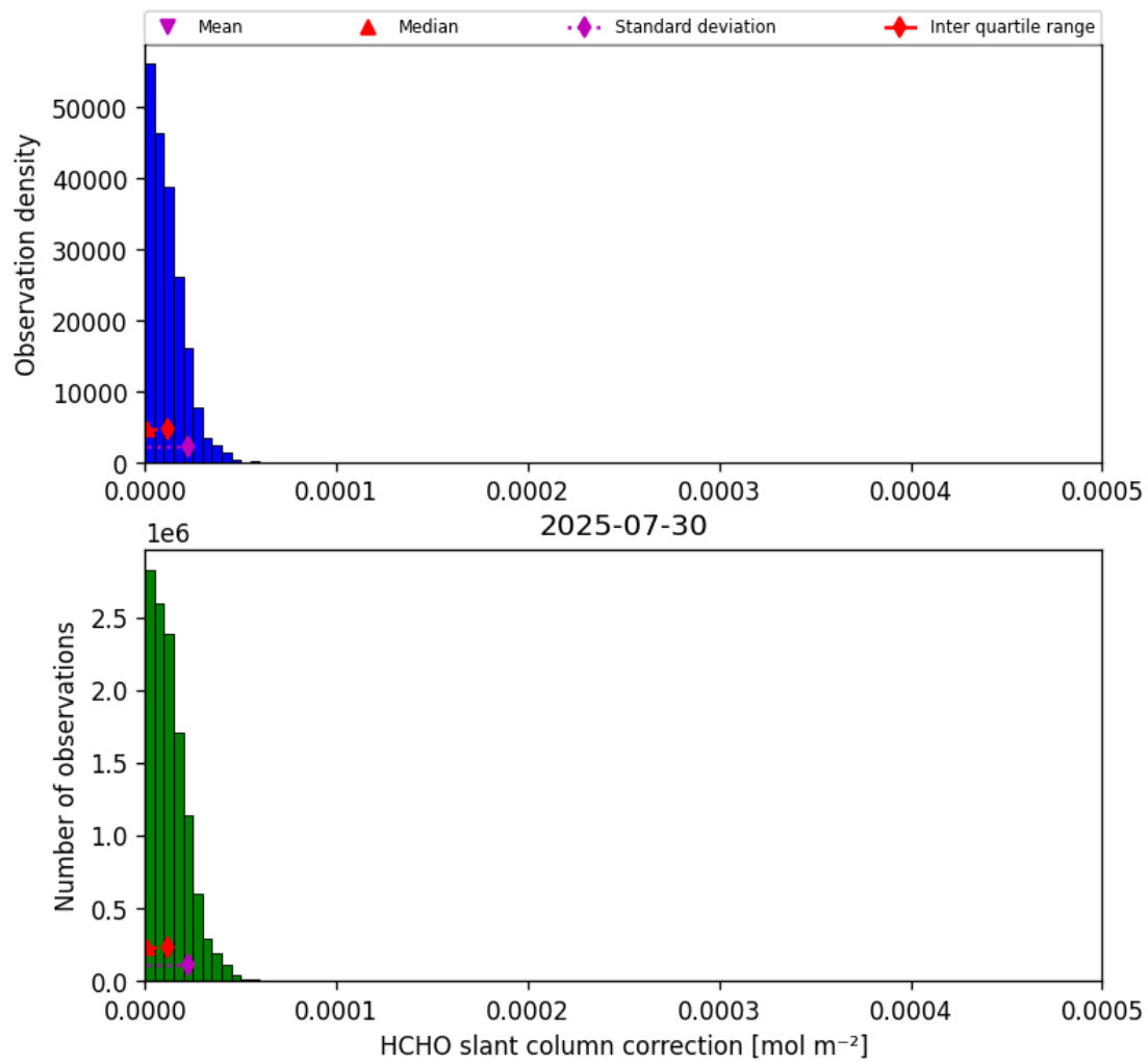
Figure 45: Histogram of “HCHO slant column correction” for 2025-07-30 to 2025-07-31
