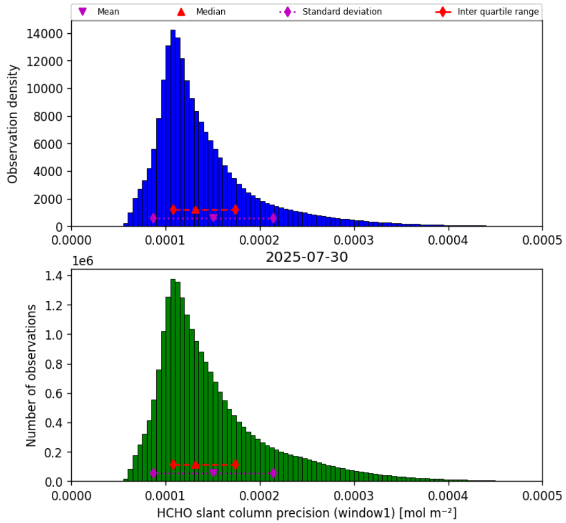
Figure 37: Histogram of “HCHO slant column precision (window1)” for 2025-07-30 to 2025-07-31
