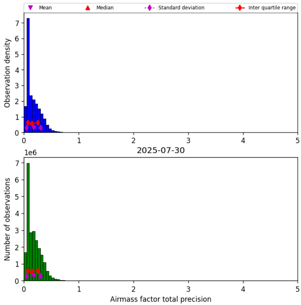
Figure 39: Histogram of “Airmass factor total precision” for 2025-07-30 to 2025-07-31
