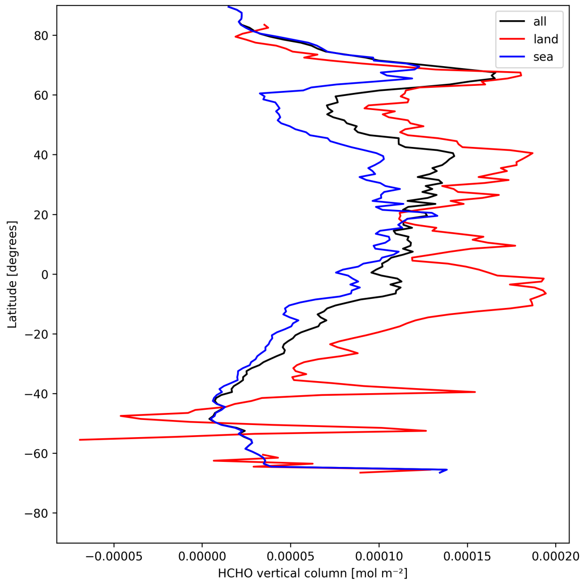
Figure 19: Zonal average of “HCHO vertical column” for 2025-07-30 to 2025-07-31.
