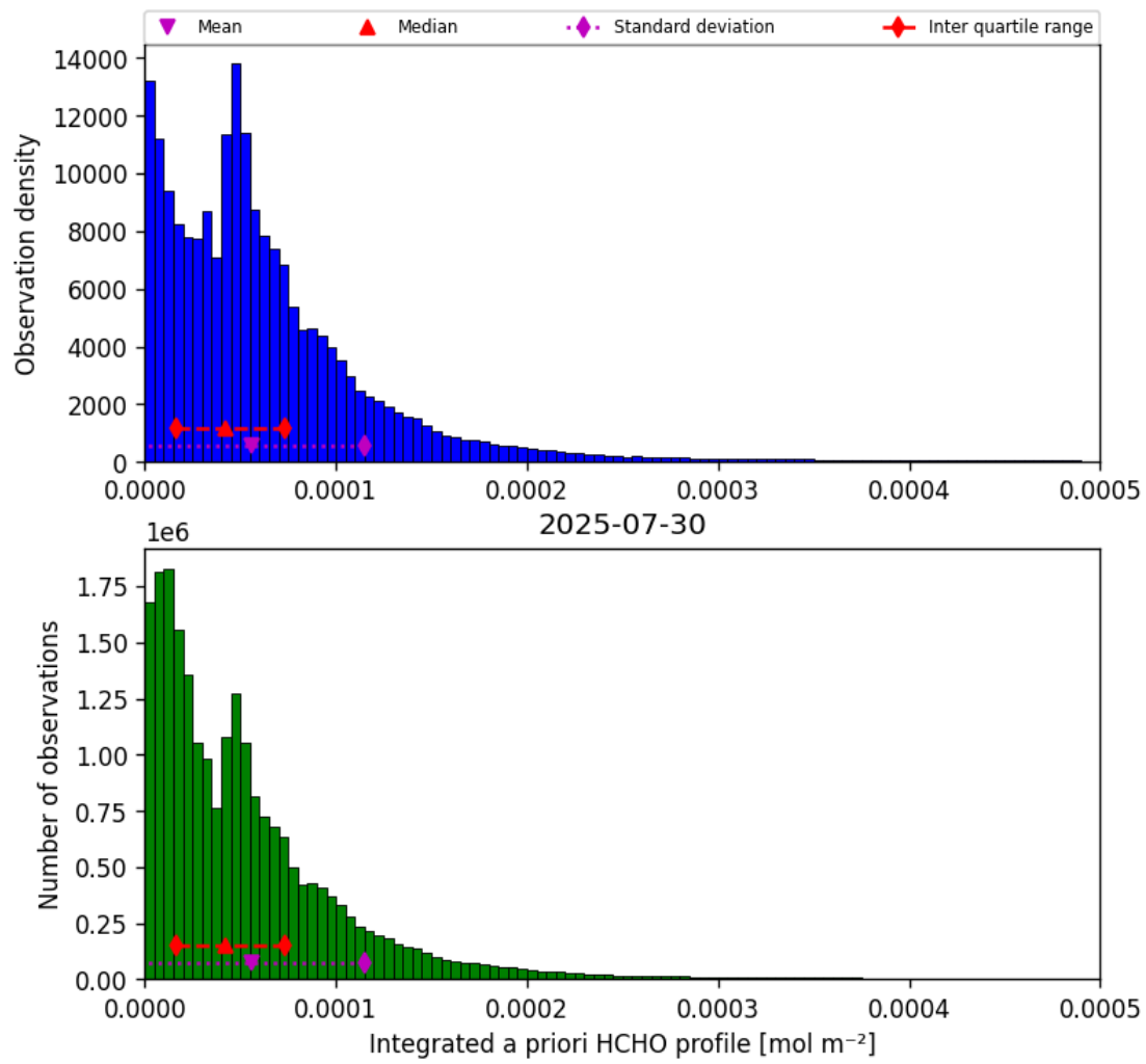
Figure 41: Histogram of “Integrated a priori HCHO profile” for 2025-07-30 to 2025-07-31
