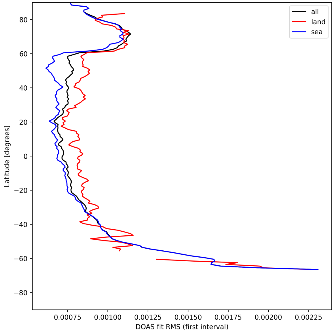
Figure 30: Zonal average of "DOAS fit RMS (first interval)" for 2025-07-30 to 2025-07-31.
