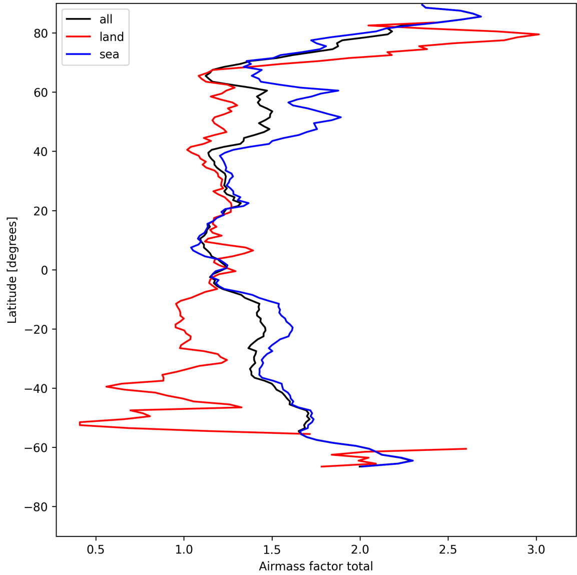
Figure 24: Zonal average of “Airmass factor total” for 2025-07-30 to 2025-07-31.
