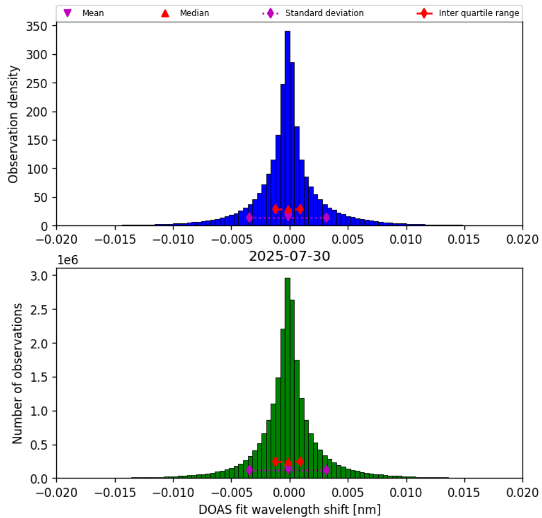
Figure 42: Histogram of “DOAS fit wavelength shift” for 2025-07-30 to 2025-07-31
