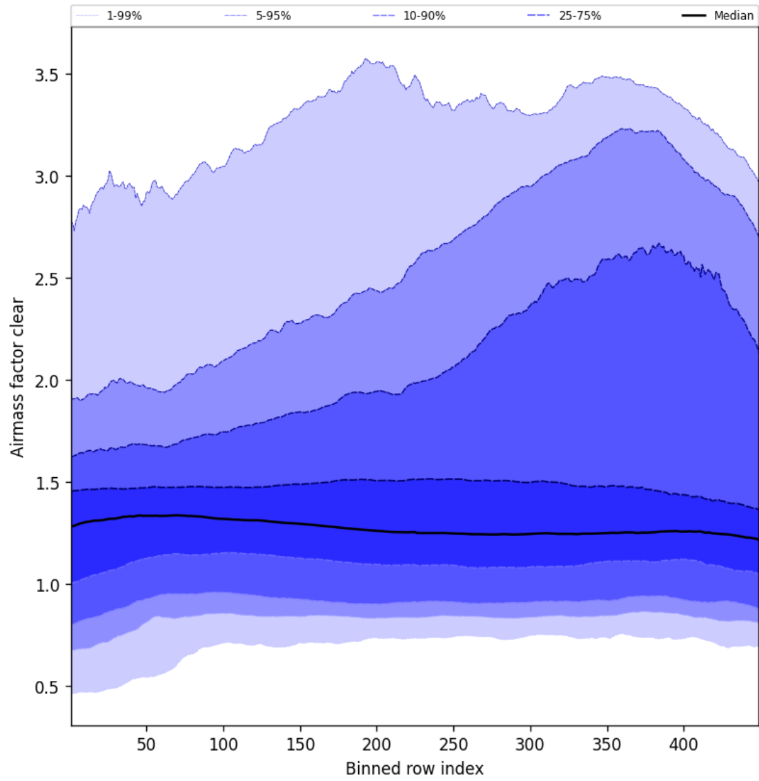
Figure 54: Along track statistics of “Airmass factor clear” for 2025-07-30 to 2025-07-31
