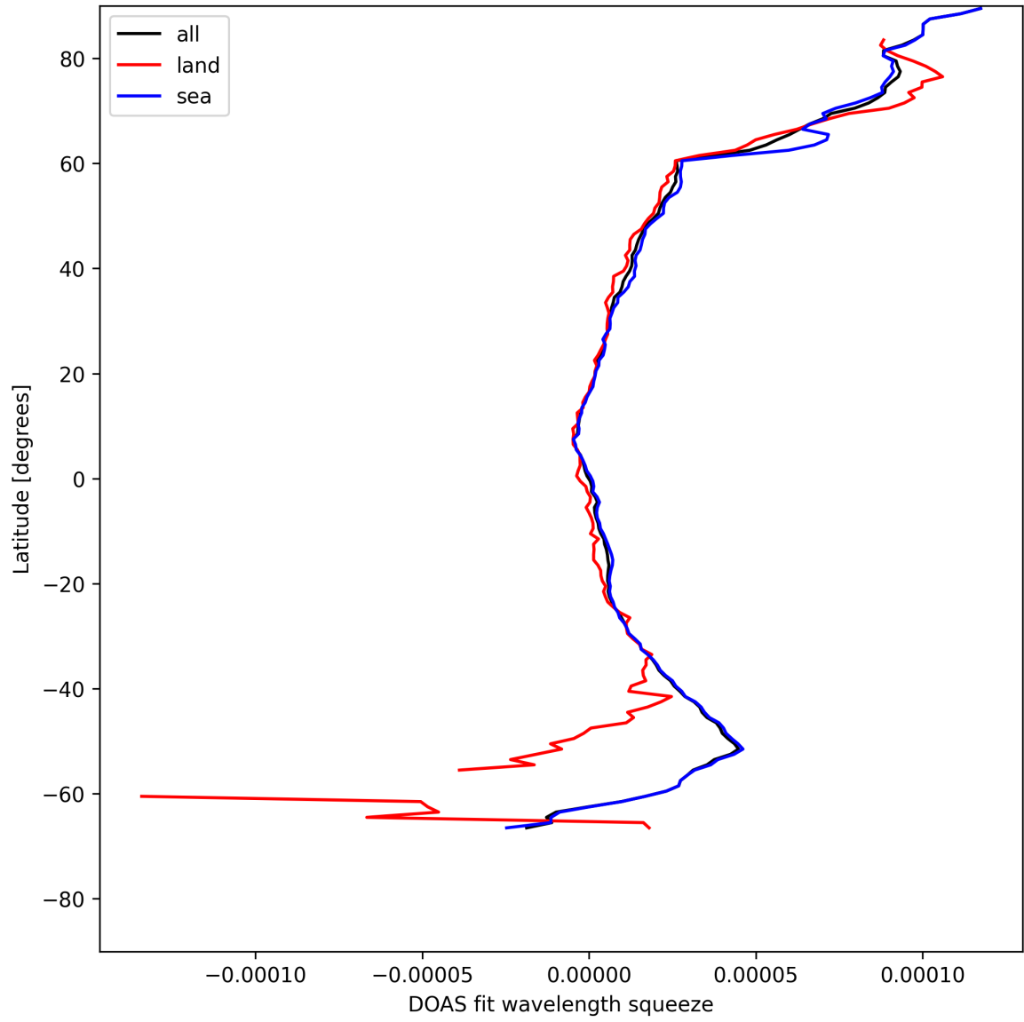
Figure 29: Zonal average of “DOAS fit wavelength squeeze” for 2025-08-01 to 2025-08-01.
