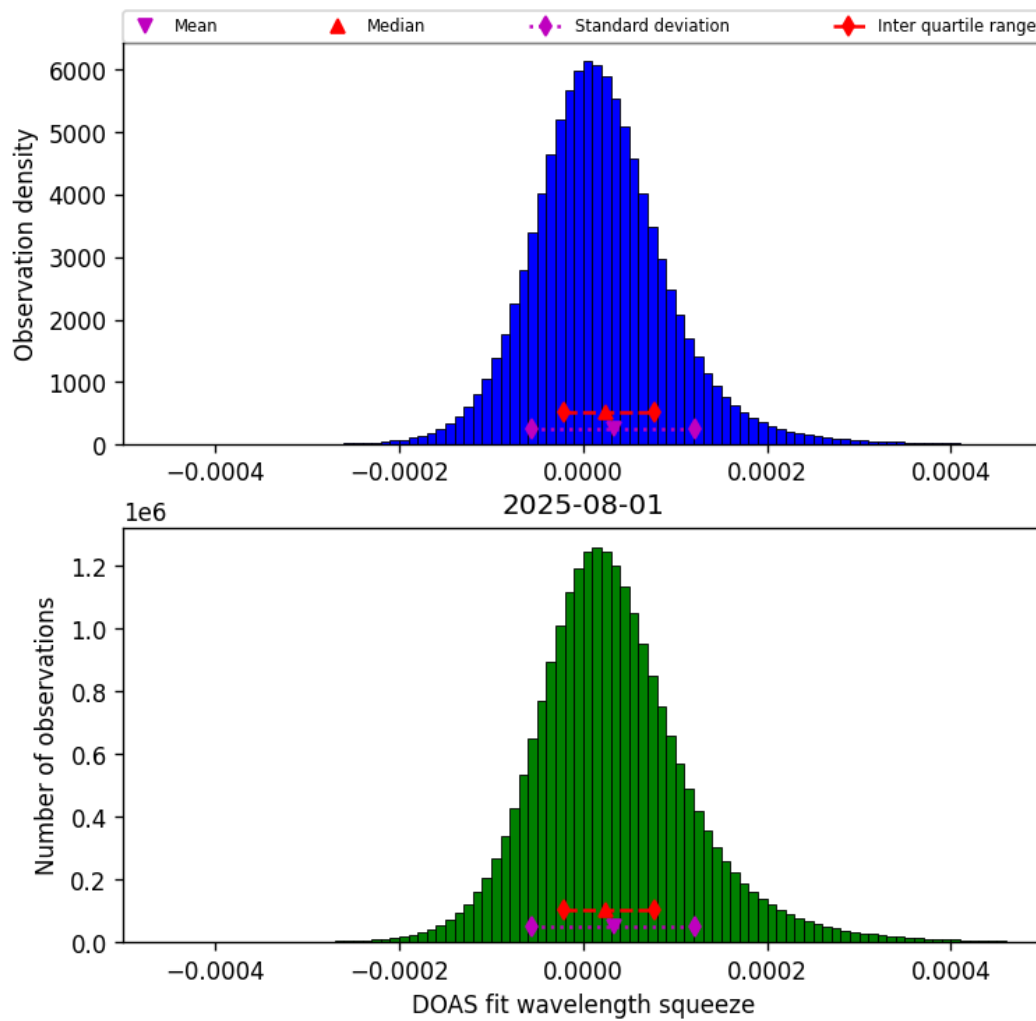
Figure 43: Histogram of “DOAS fit wavelength squeeze” for 2025-08-01 to 2025-08-01
