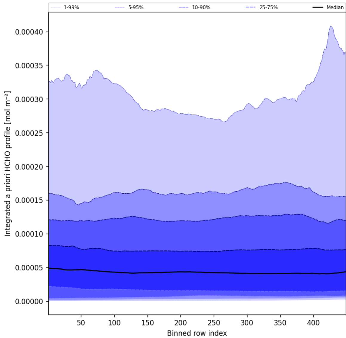
Figure 55: Along track statistics of "Integrated a priori HCHO profile" for 2025-08-01 to 2025-08-01
