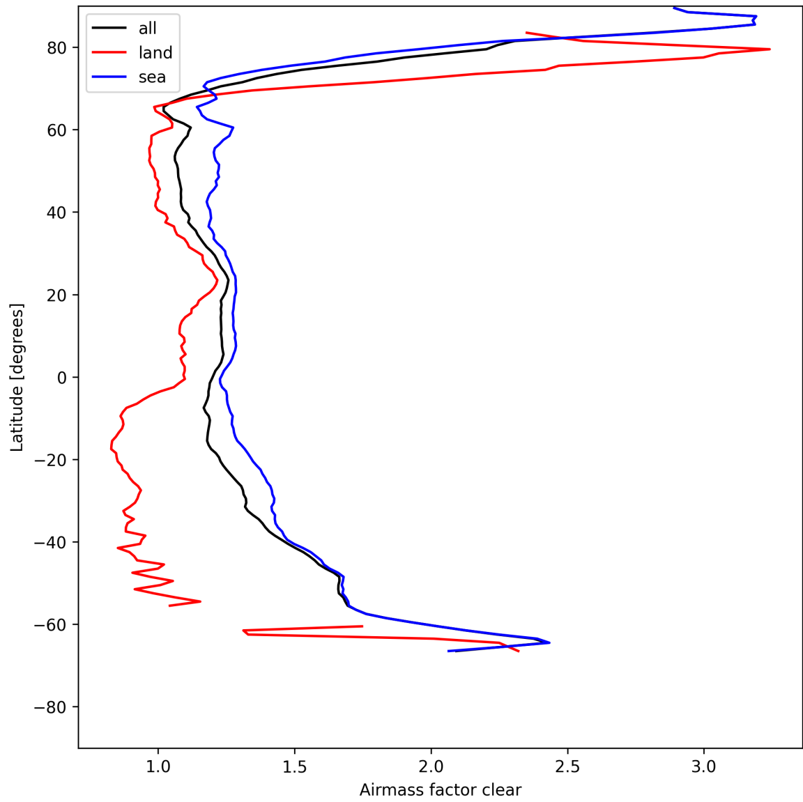
Figure 26: Zonal average of “Airmass factor clear” for 2025-08-01 to 2025-08-01.
