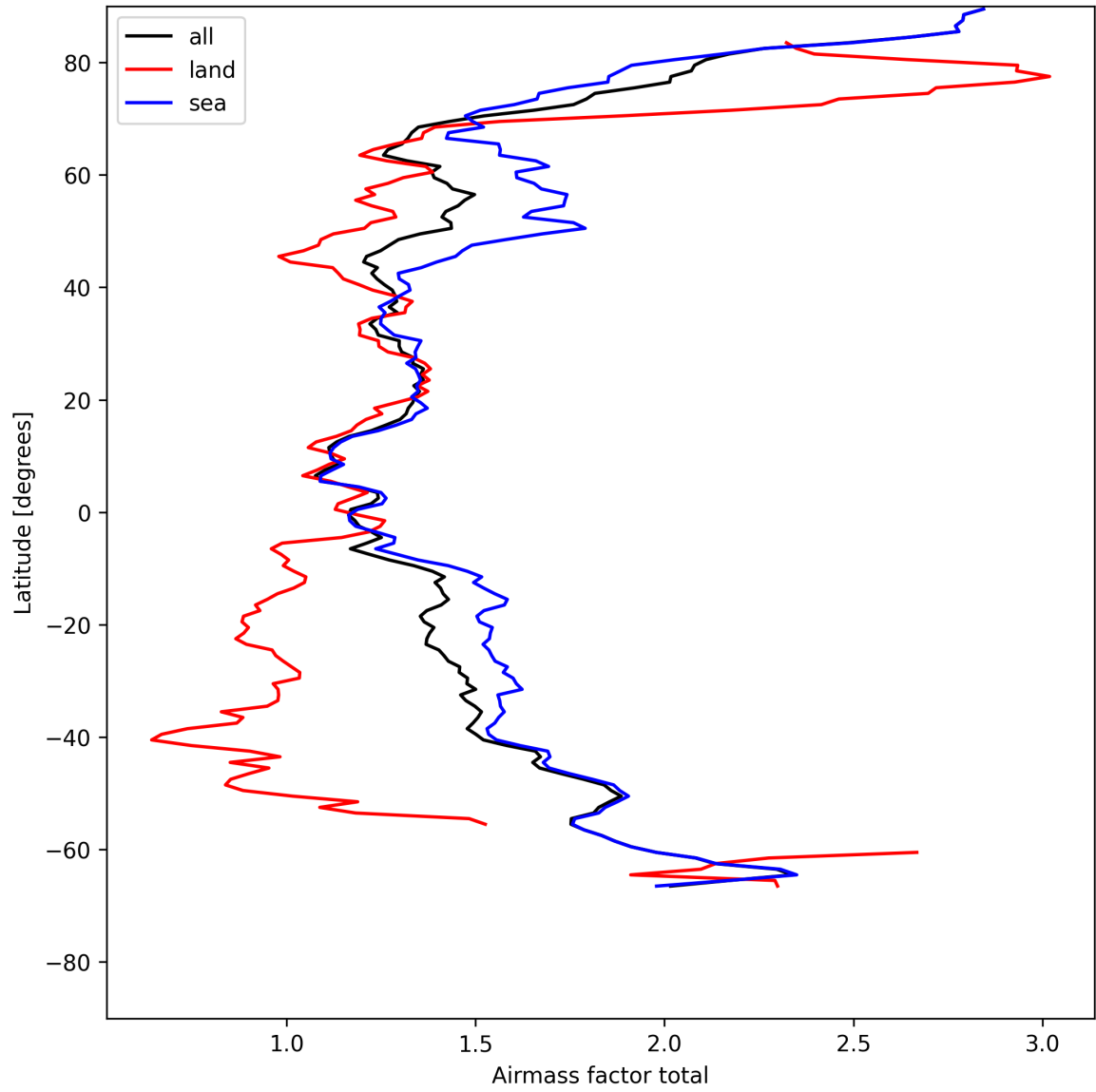
Figure 24: Zonal average of “Airmass factor total” for 2025-08-01 to 2025-08-01.
