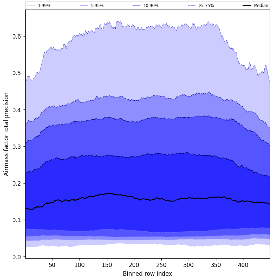
Figure 53: Along track statistics of “Airmass factor total precision” for 2025-08-01 to 2025-08-01
