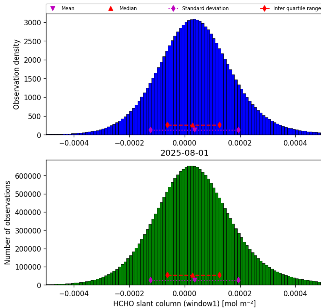
Figure 36: Histogram of “HCHO slant column (window1)” for 2025-08-01 to 2025-08-01
