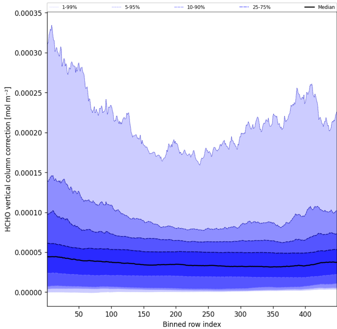
Figure 49: Along track statistics of “HCHO vertical column correction” for 2025-08-01 to 2025-08-01
