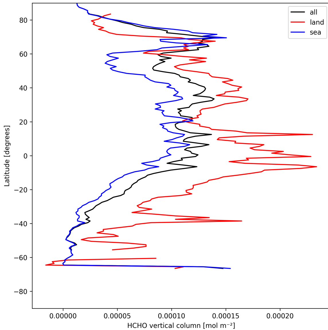
Figure 19: Zonal average of “HCHO vertical column” for 2025-08-01 to 2025-08-01.
