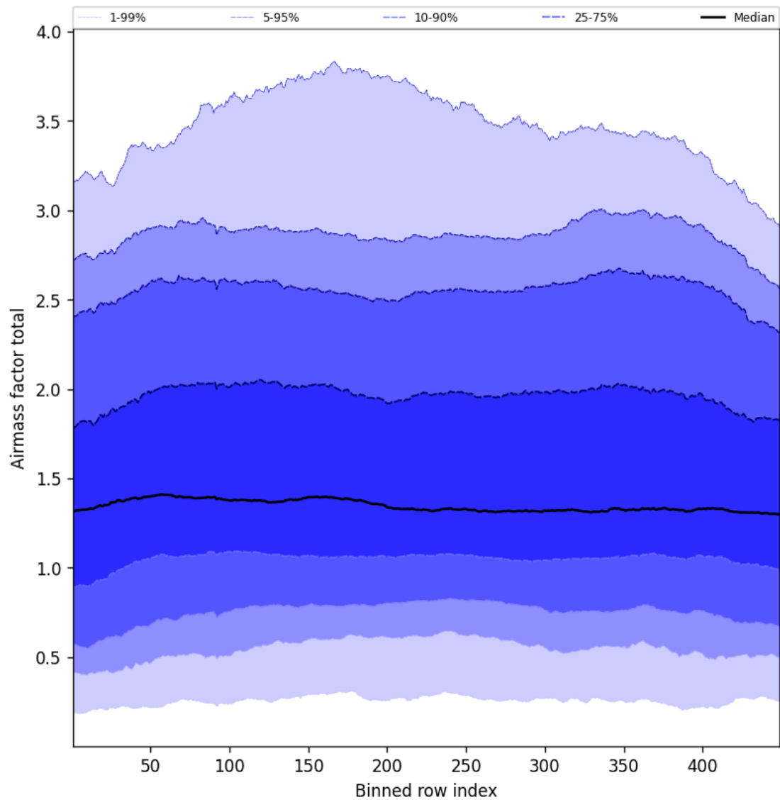
Figure 52: Along track statistics of “Airmass factor total” for 2025-08-01 to 2025-08-01
