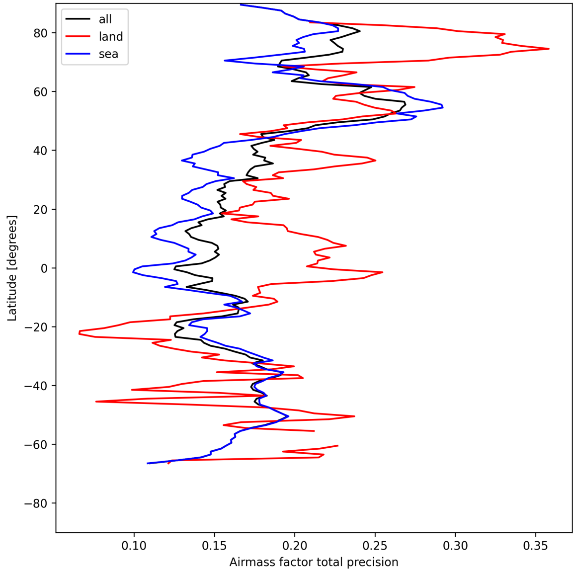
Figure 25: Zonal average of “Airmass factor total precision” for 2025-08-01 to 2025-08-01.
