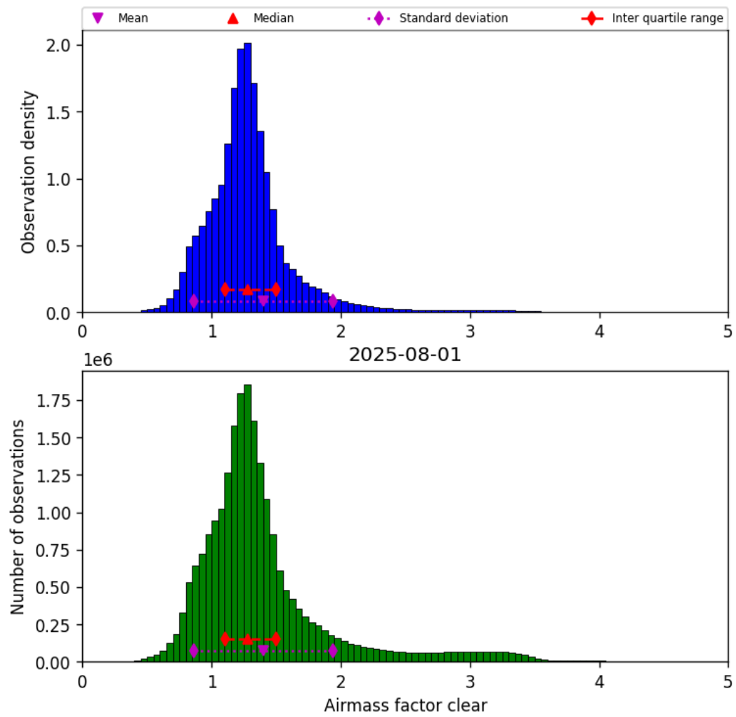
Figure 40: Histogram of “Airmass factor clear” for 2025-08-01 to 2025-08-01
