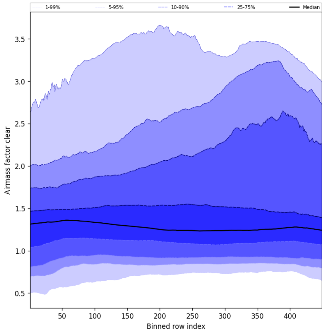
Figure 54: Along track statistics of “Airmass factor clear” for 2025-08-01 to 2025-08-01
