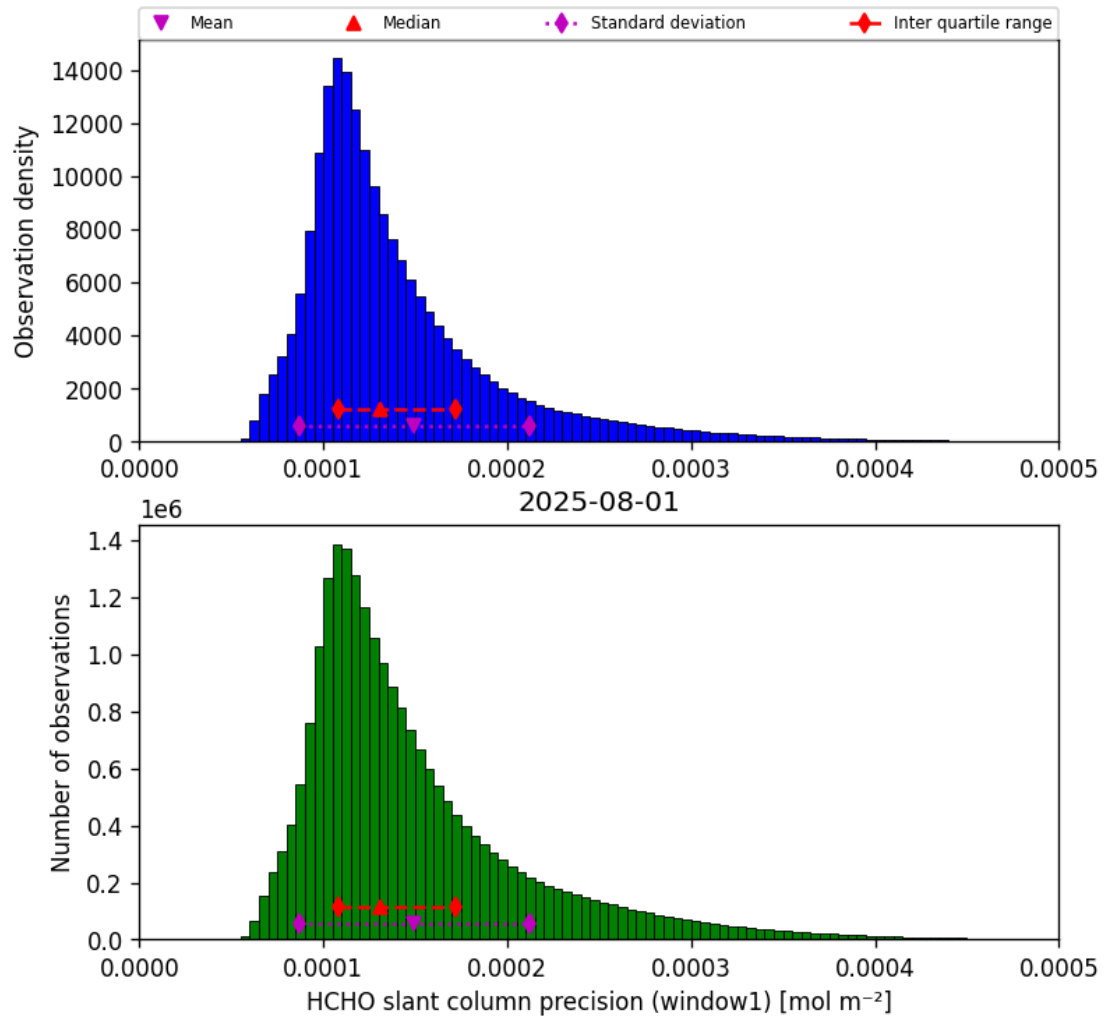
Figure 37: Histogram of “HCHO slant column precision (window1)” for 2025-08-01 to 2025-08-01
