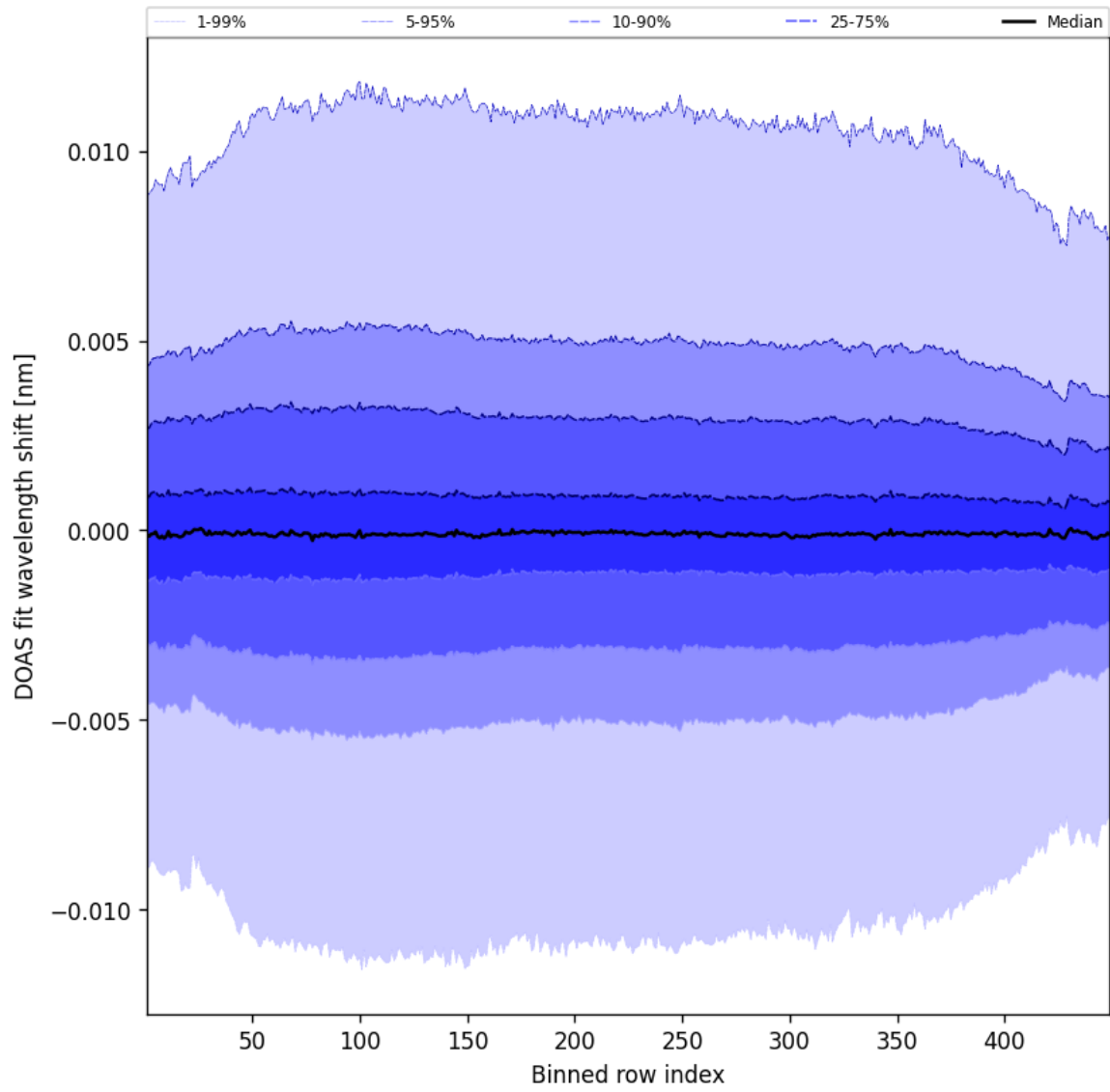
Figure 56: Along track statistics of “DOAS fit wavelength shift” for 2025-08-01 to 2025-08-01
