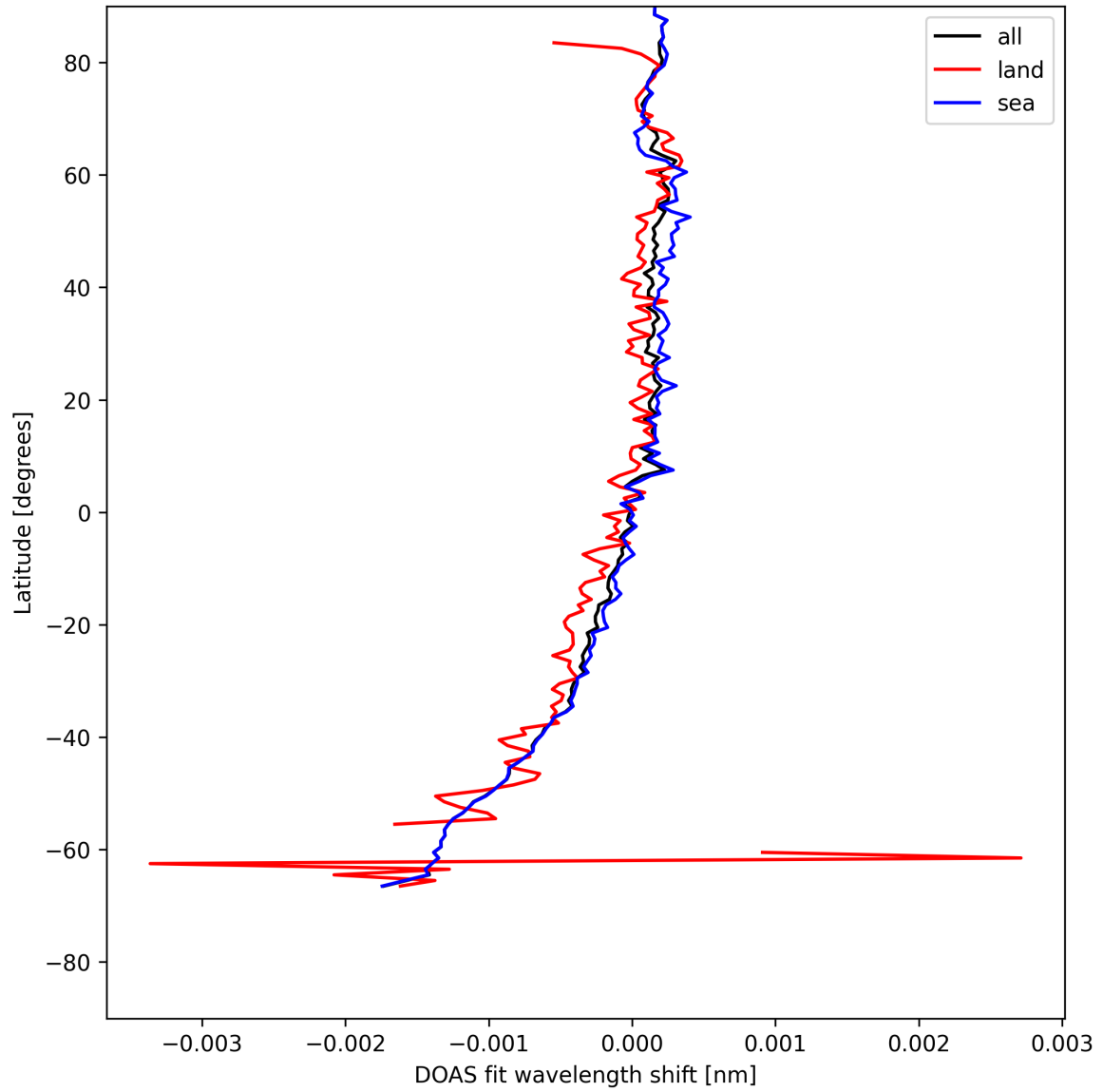
Figure 28: Zonal average of “DOAS fit wavelength shift” for 2025-08-01 to 2025-08-01.
