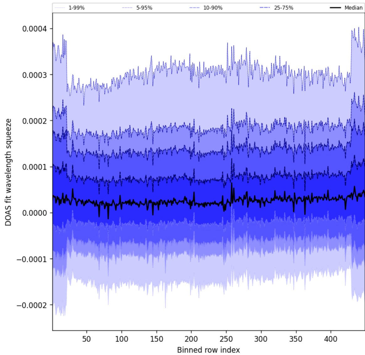
Figure 57: Along track statistics of “DOAS fit wavelength squeeze” for 2025-08-01 to 2025-08-01
