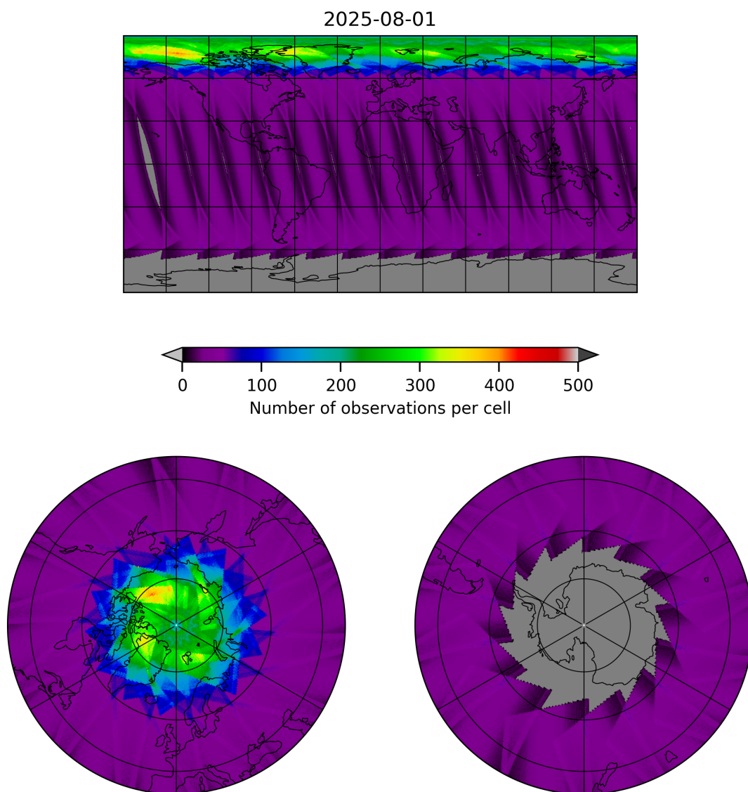
Figure 17: Map of the number of observations for 2025-08-01 to 2025-08-01
