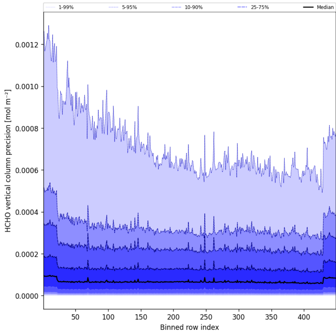
Figure 48: Along track statistics of “HCHO vertical column precision” for 2025-08-01 to 2025-08-01
