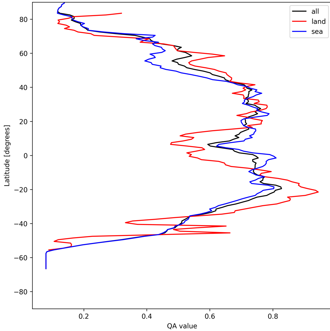
Figure 18: Zonal average of “QA value” for 2025-08-01 to 2025-08-01.
