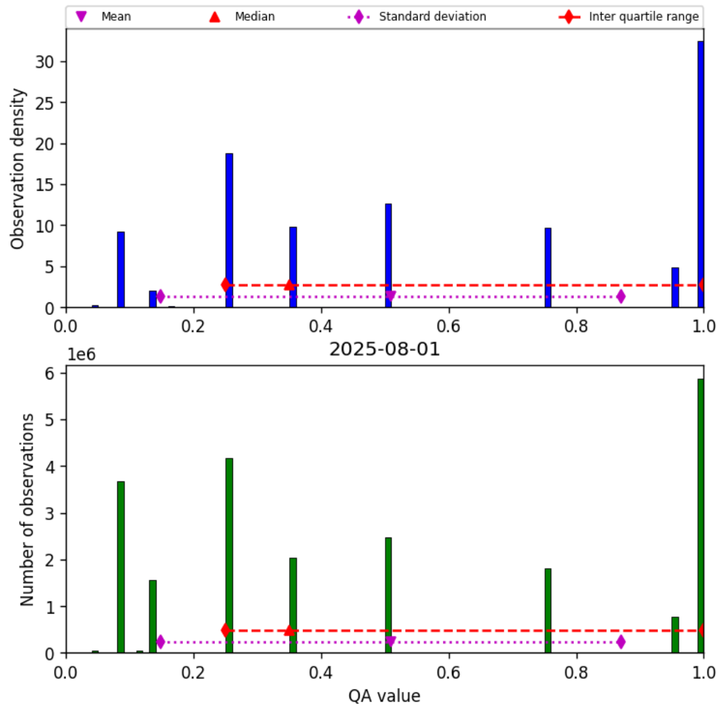
Figure 32: Histogram of “QA value” for 2025-08-01 to 2025-08-01
