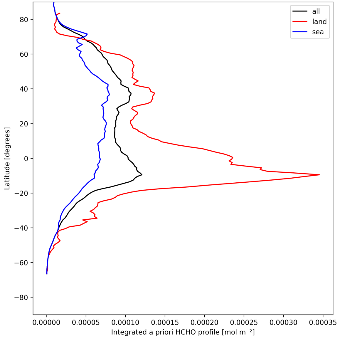
Figure 27: Zonal average of “Integrated a priori HCHO profile” for 2025-08-01 to 2025-08-01.
