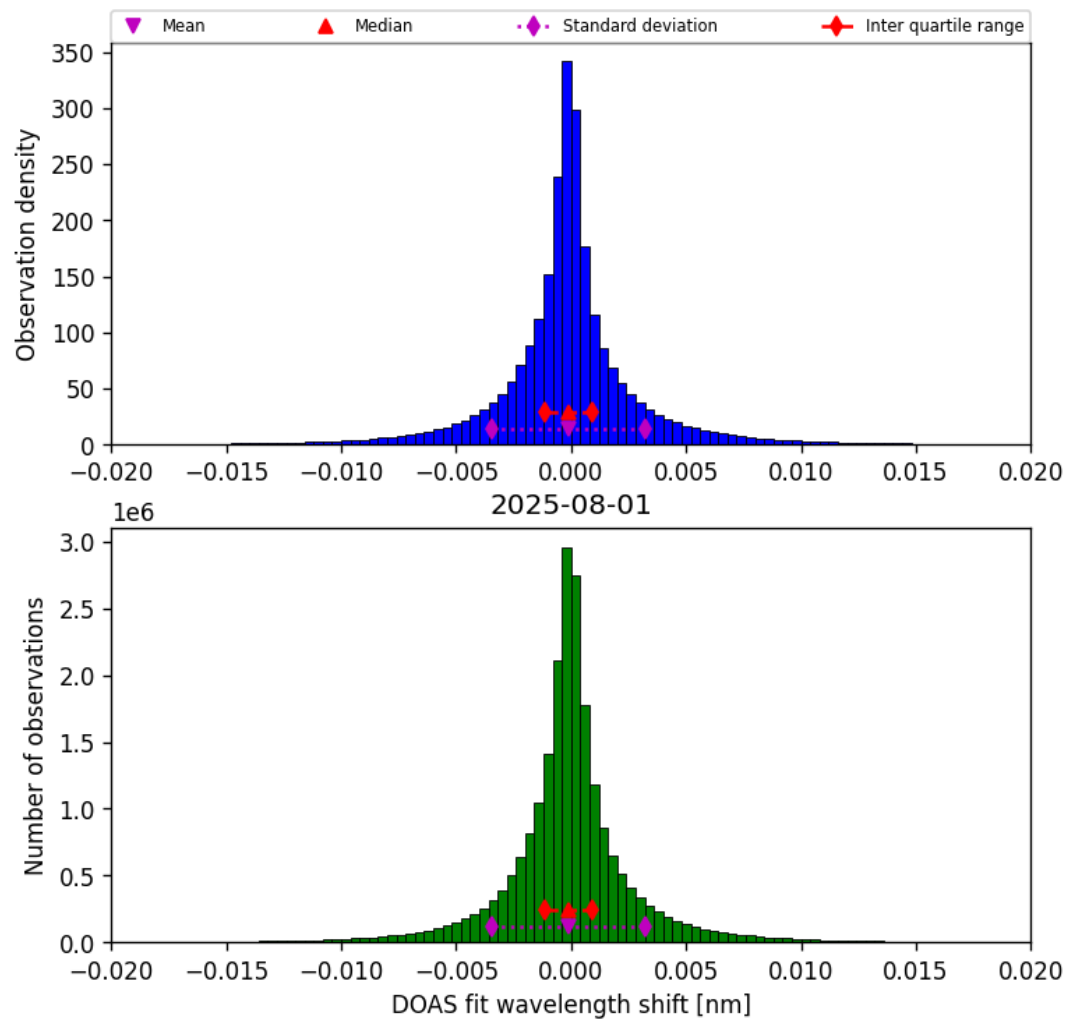
Figure 42: Histogram of “DOAS fit wavelength shift” for 2025-08-01 to 2025-08-01
