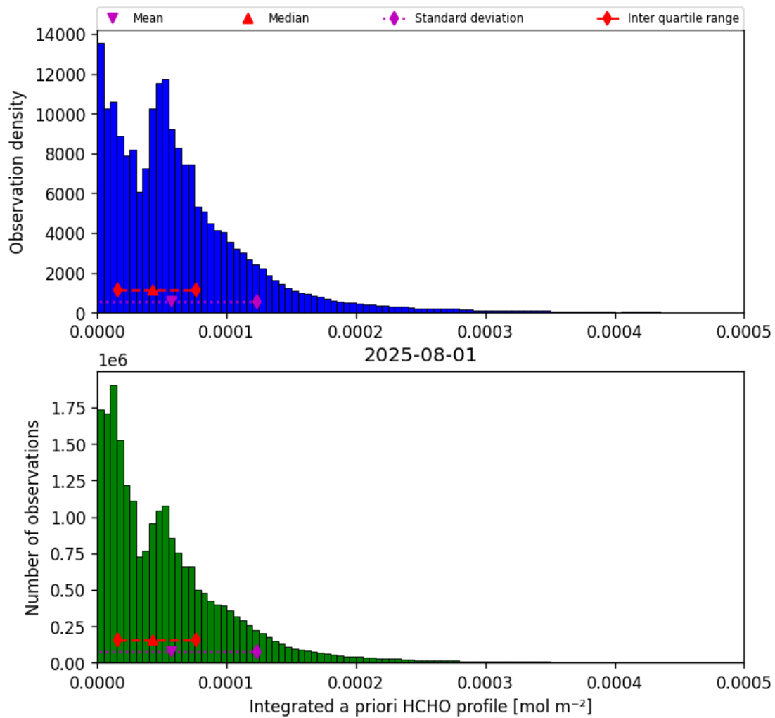
Figure 41: Histogram of “Integrated a priori HCHO profile” for 2025-08-01 to 2025-08-01
