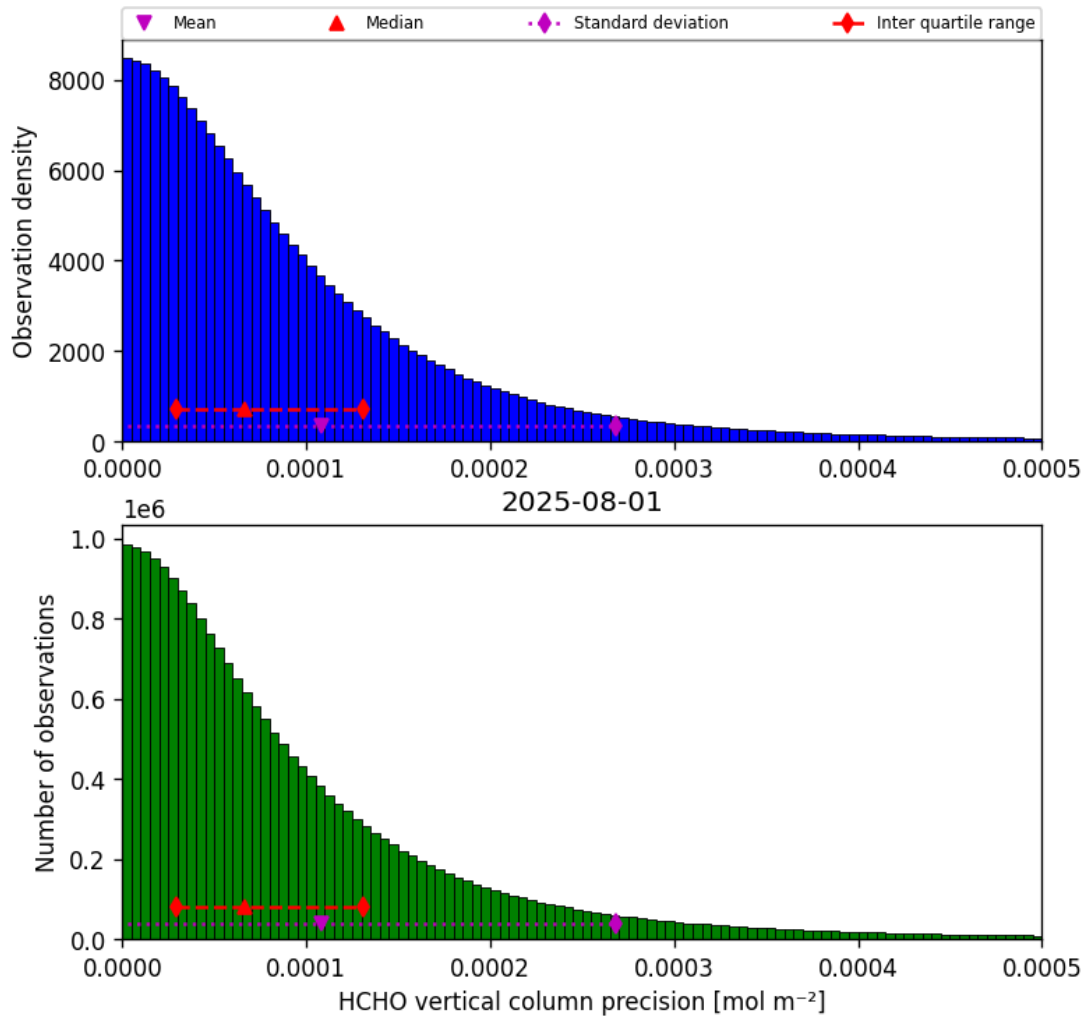
Figure 34: Histogram of “HCHO vertical column precision” for 2025-08-01 to 2025-08-01
