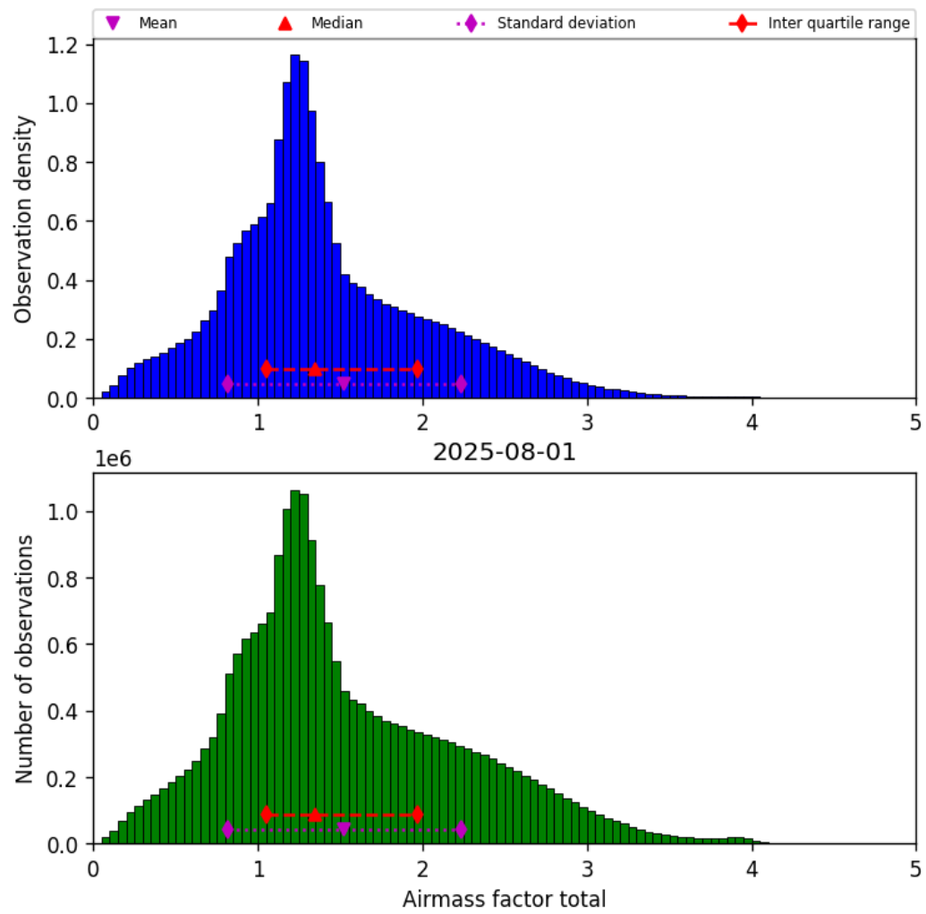
Figure 38: Histogram of “Airmass factor total” for 2025-08-01 to 2025-08-01
