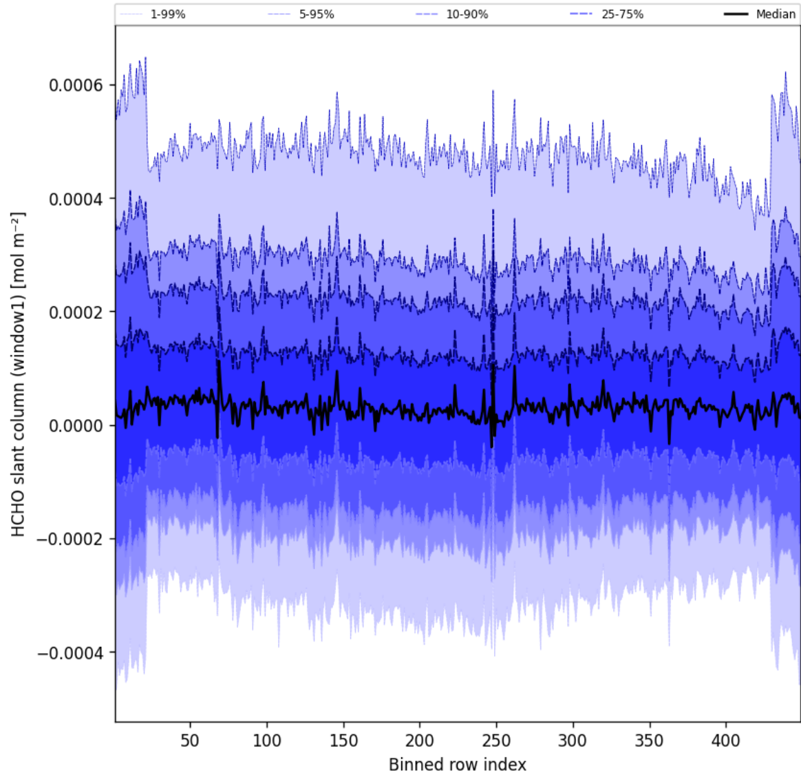
Figure 50: Along track statistics of “HCHO slant column (window1)” for 2025-08-01 to 2025-08-01
