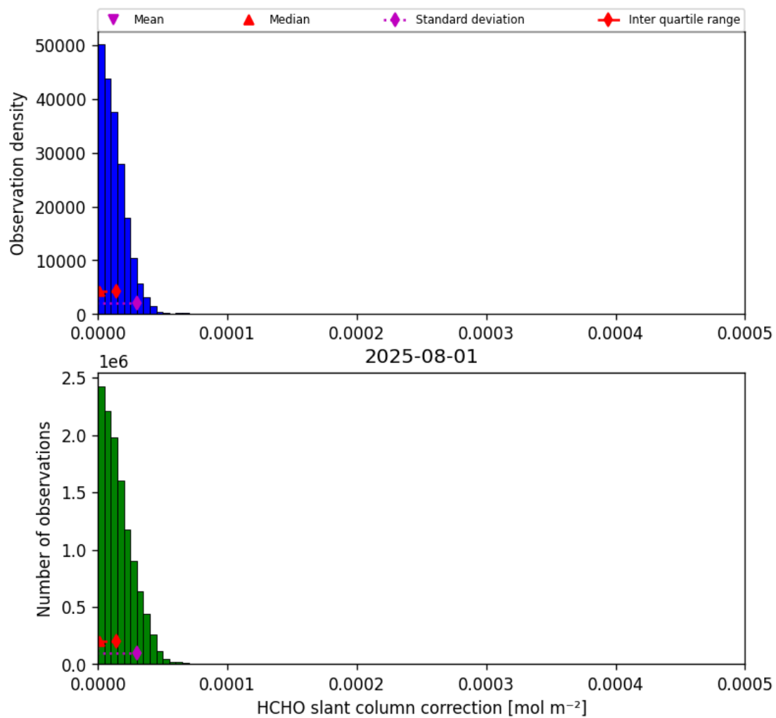
Figure 45: Histogram of “HCHO slant column correction” for 2025-08-01 to 2025-08-01
