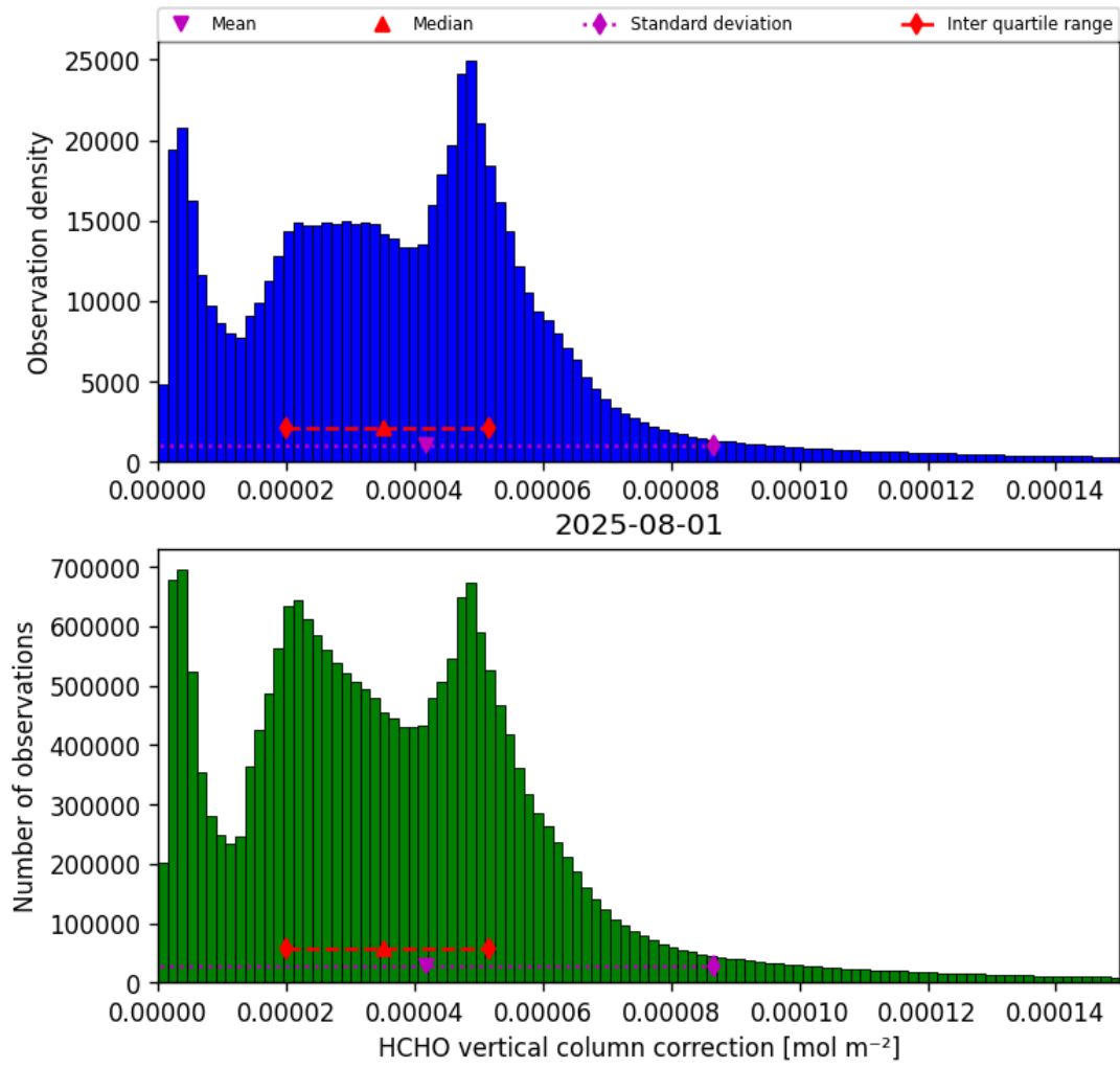
Figure 35: Histogram of “HCHO vertical column correction” for 2025-08-01 to 2025-08-01
