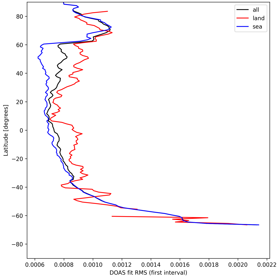
Figure 30: Zonal average of "DOAS fit RMS (first interval)" for 2025-08-01 to 2025-08-01.
