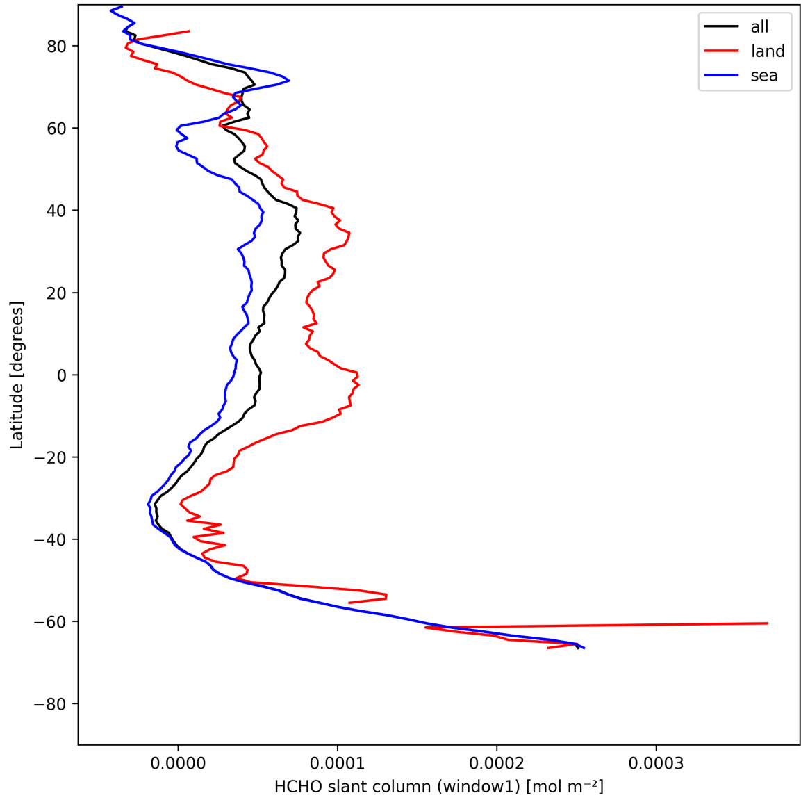
Figure 22: Zonal average of “HCHO slant column (window1)” for 2025-08-01 to 2025-08-01.
