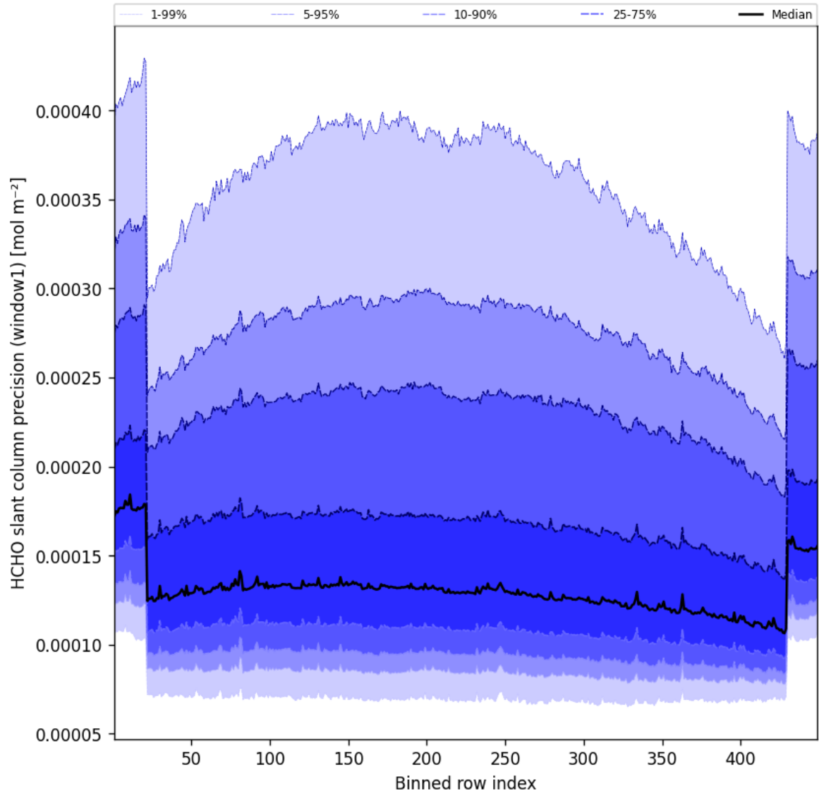
Figure 51: Along track statistics of “HCHO slant column precision (window1)” for 2025-08-01 to 2025-08-01
