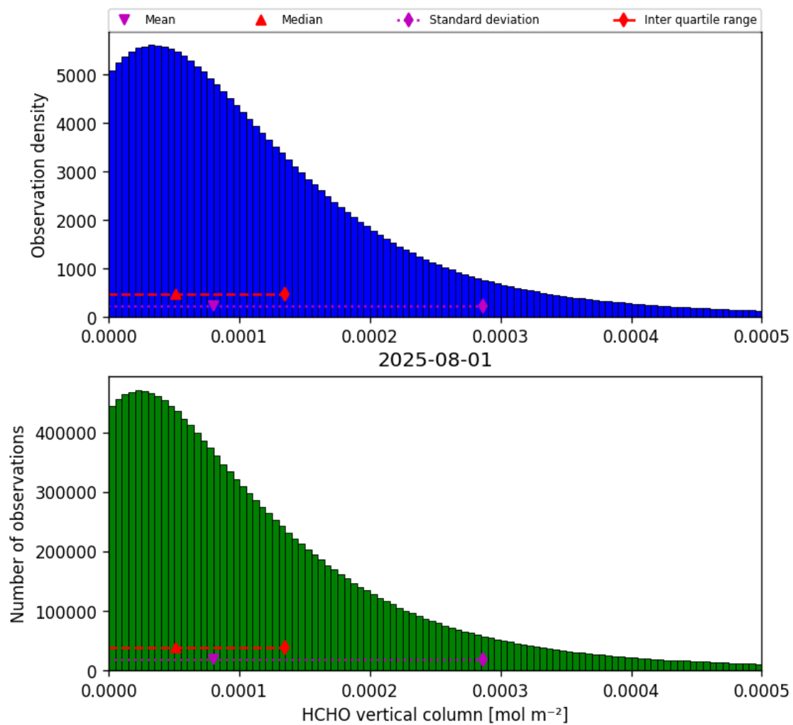
Figure 33: Histogram of “HCHO vertical column” for 2025-08-01 to 2025-08-01
