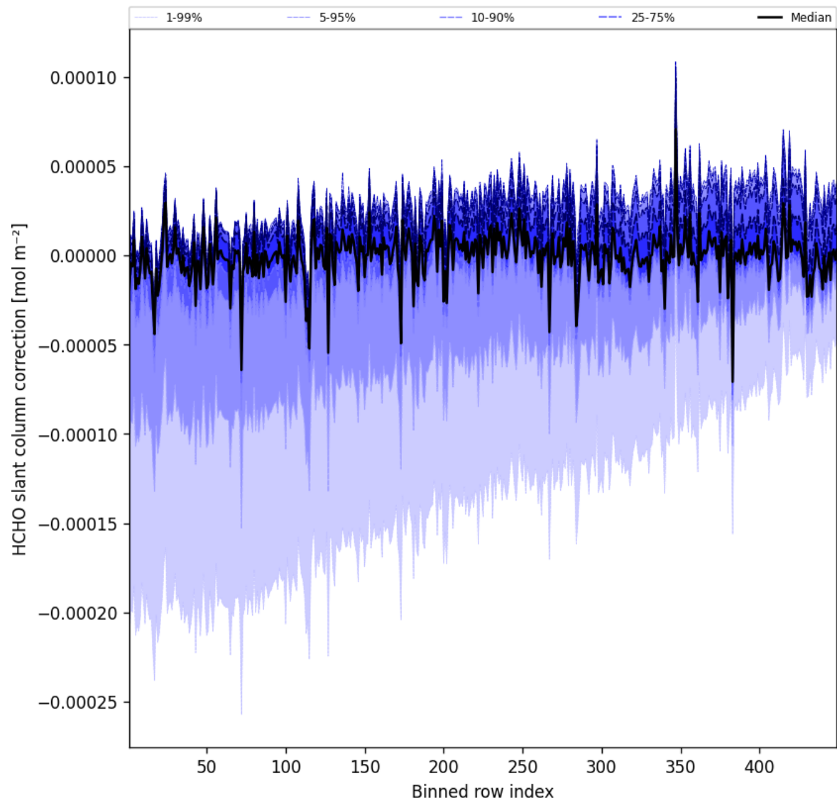
Figure 59: Along track statistics of “HCHO slant column correction” for 2025-08-01 to 2025-08-01
