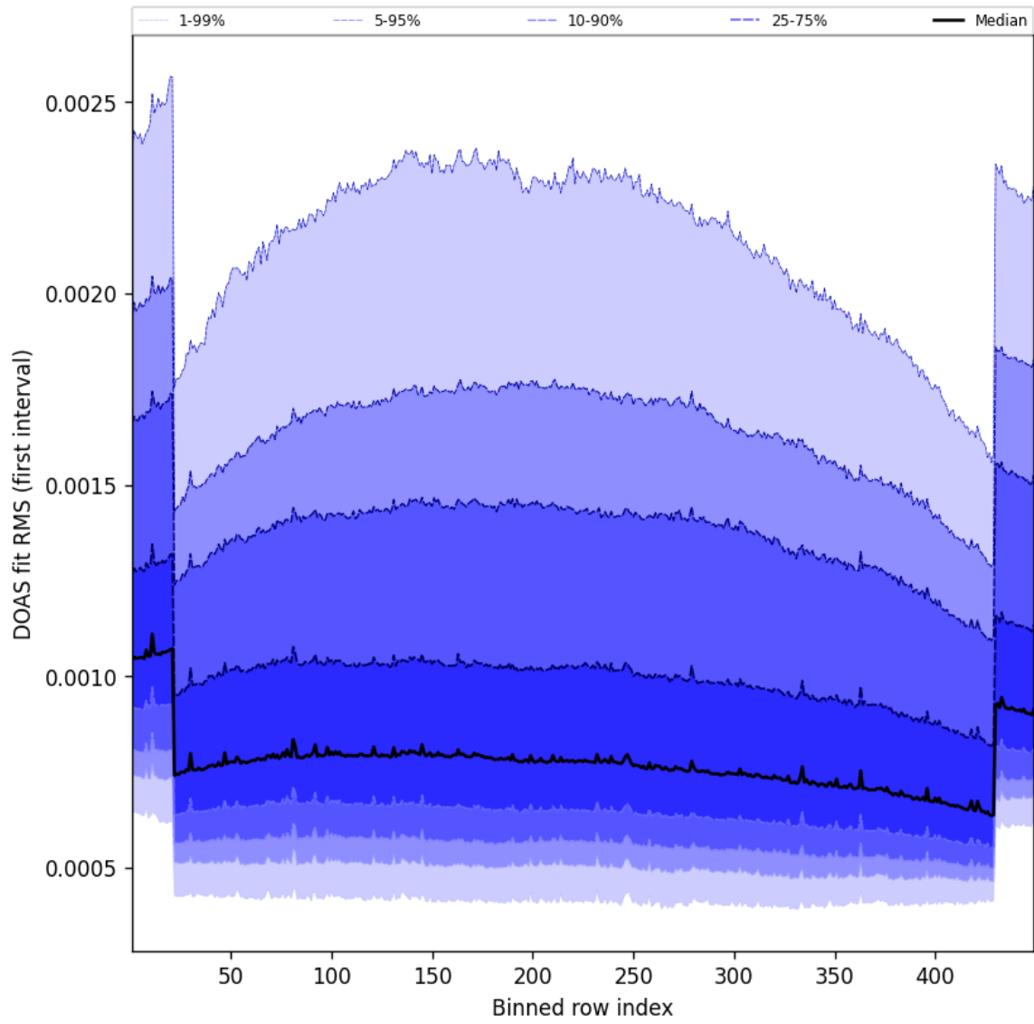
Figure 58: Along track statistics of “DOAS fit RMS (first interval)” for 2025-08-01 to 2025-08-01
