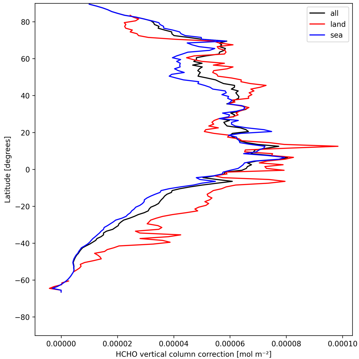
Figure 21: Zonal average of “HCHO vertical column correction” for 2025-08-01 to 2025-08-01.
