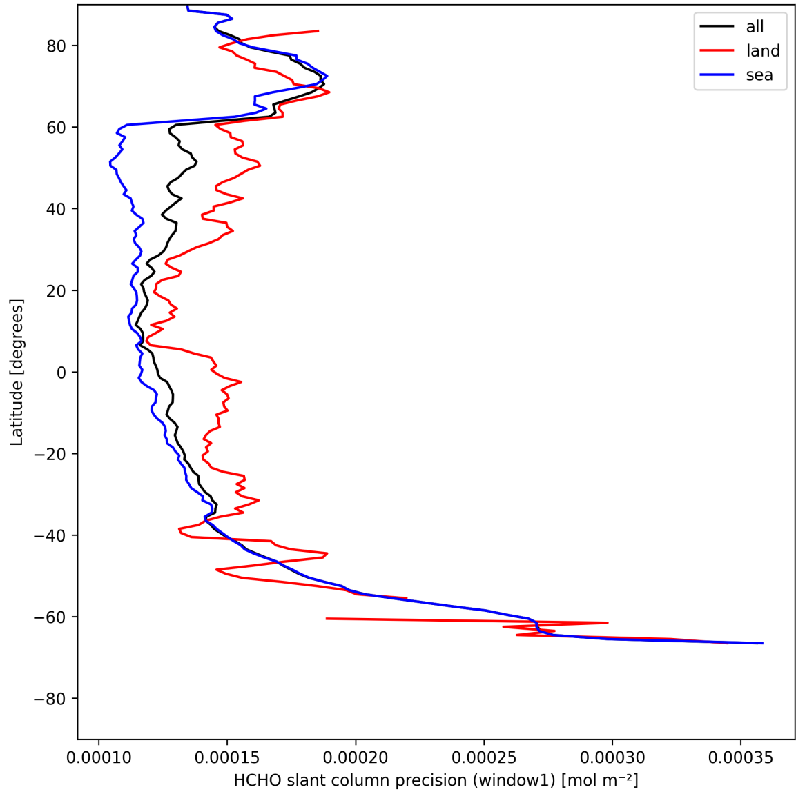
Figure 23: Zonal average of “HCHO slant column precision (window1)” for 2025-08-01 to 2025-08-01.
