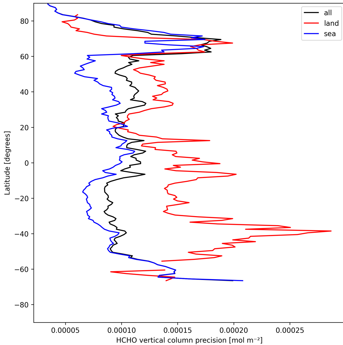
Figure 20: Zonal average of “HCHO vertical column precision” for 2025-08-01 to 2025-08-01.
