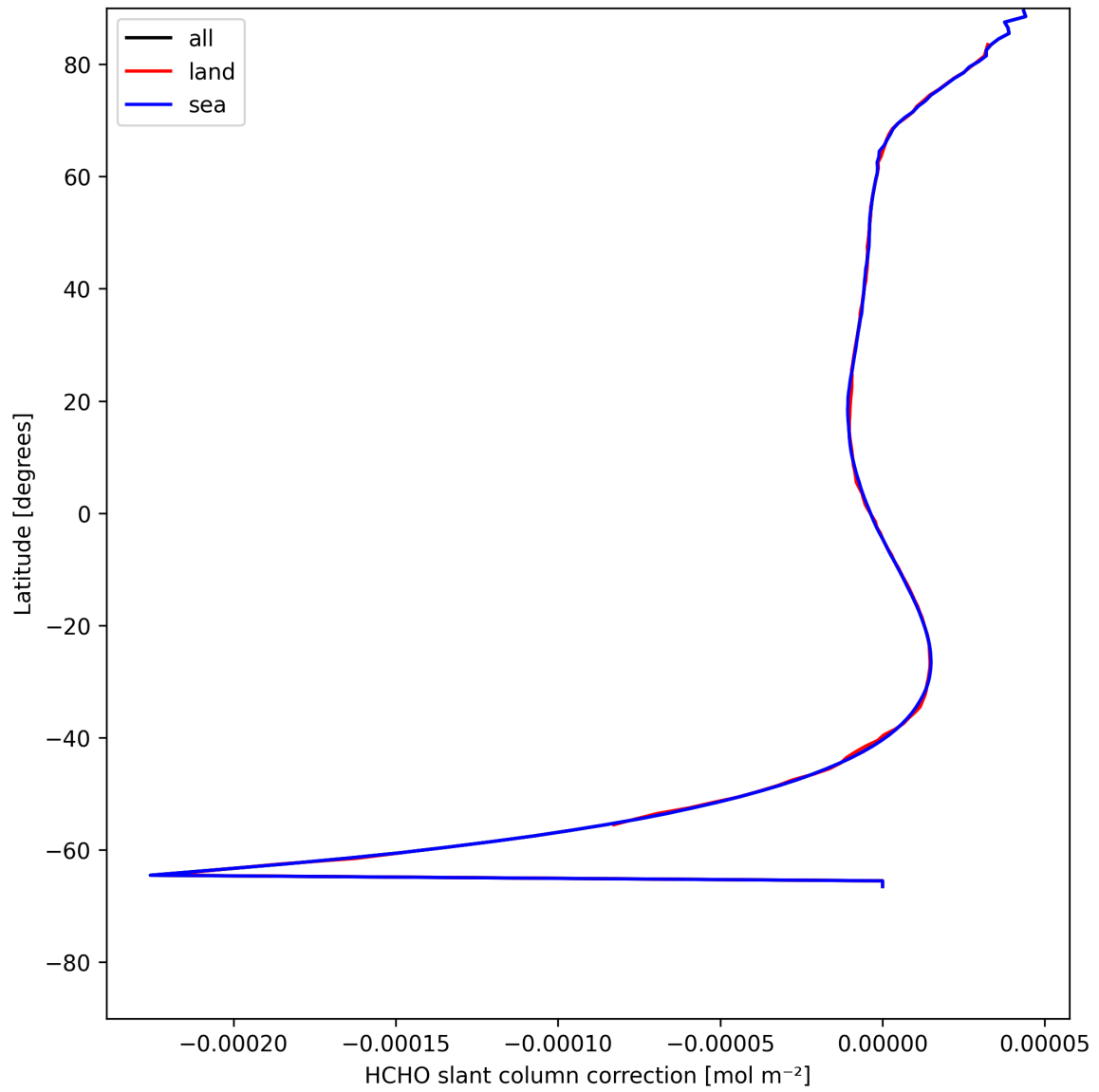
Figure 31: Zonal average of “HCHO slant column correction” for 2025-08-01 to 2025-08-01.
