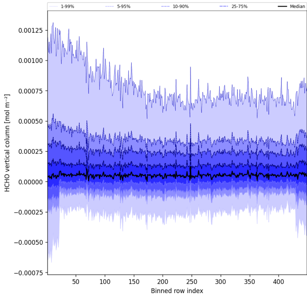
Figure 47: Along track statistics of “HCHO vertical column” for 2025-08-01 to 2025-08-01
