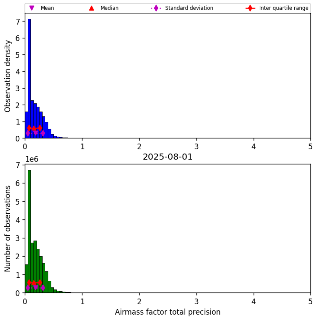
Figure 39: Histogram of “Airmass factor total precision” for 2025-08-01 to 2025-08-01
