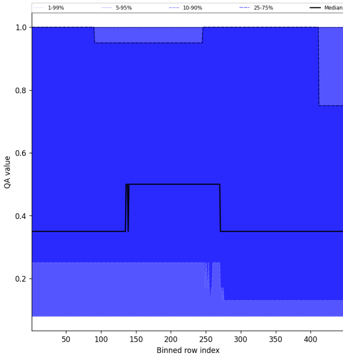
Figure 46: Along track statistics of “QA value” for 2025-08-01 to 2025-08-01
