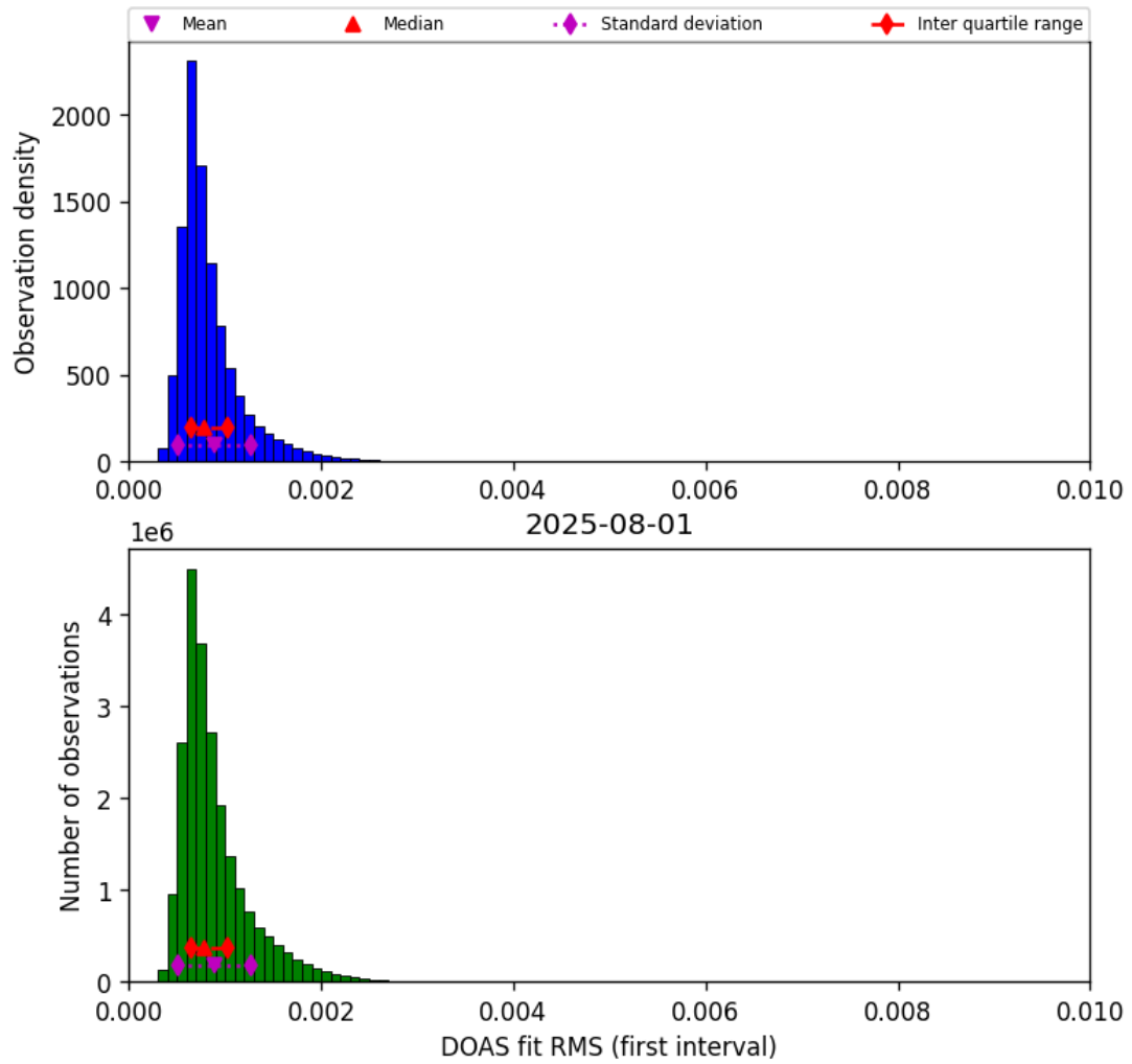
Figure 44: Histogram of “DOAS fit RMS (first interval)” for 2025-08-01 to 2025-08-01
