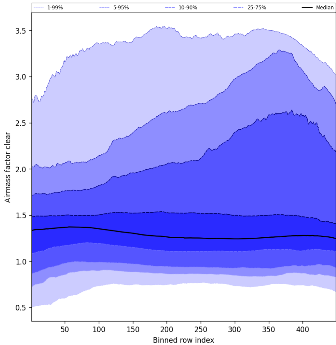
Figure 54: Along track statistics of “Airmass factor clear” for 2025-08-02 to 2025-08-03
