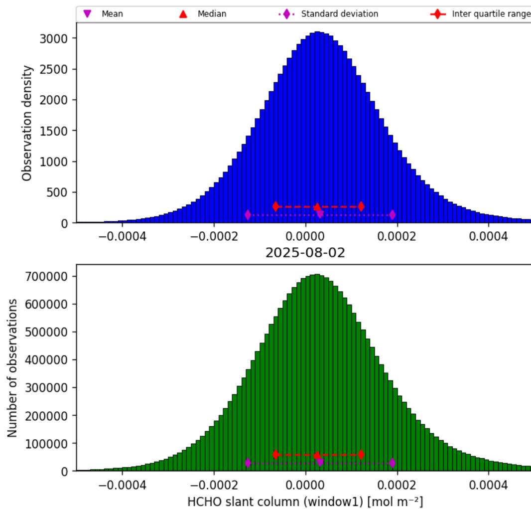
Figure 36: Histogram of “HCHO slant column (window1)” for 2025-08-02 to 2025-08-03
