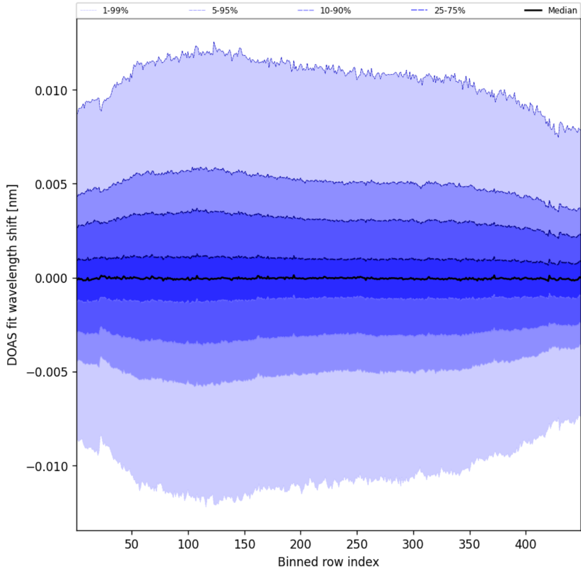
Figure 56: Along track statistics of “DOAS fit wavelength shift” for 2025-08-02 to 2025-08-03
