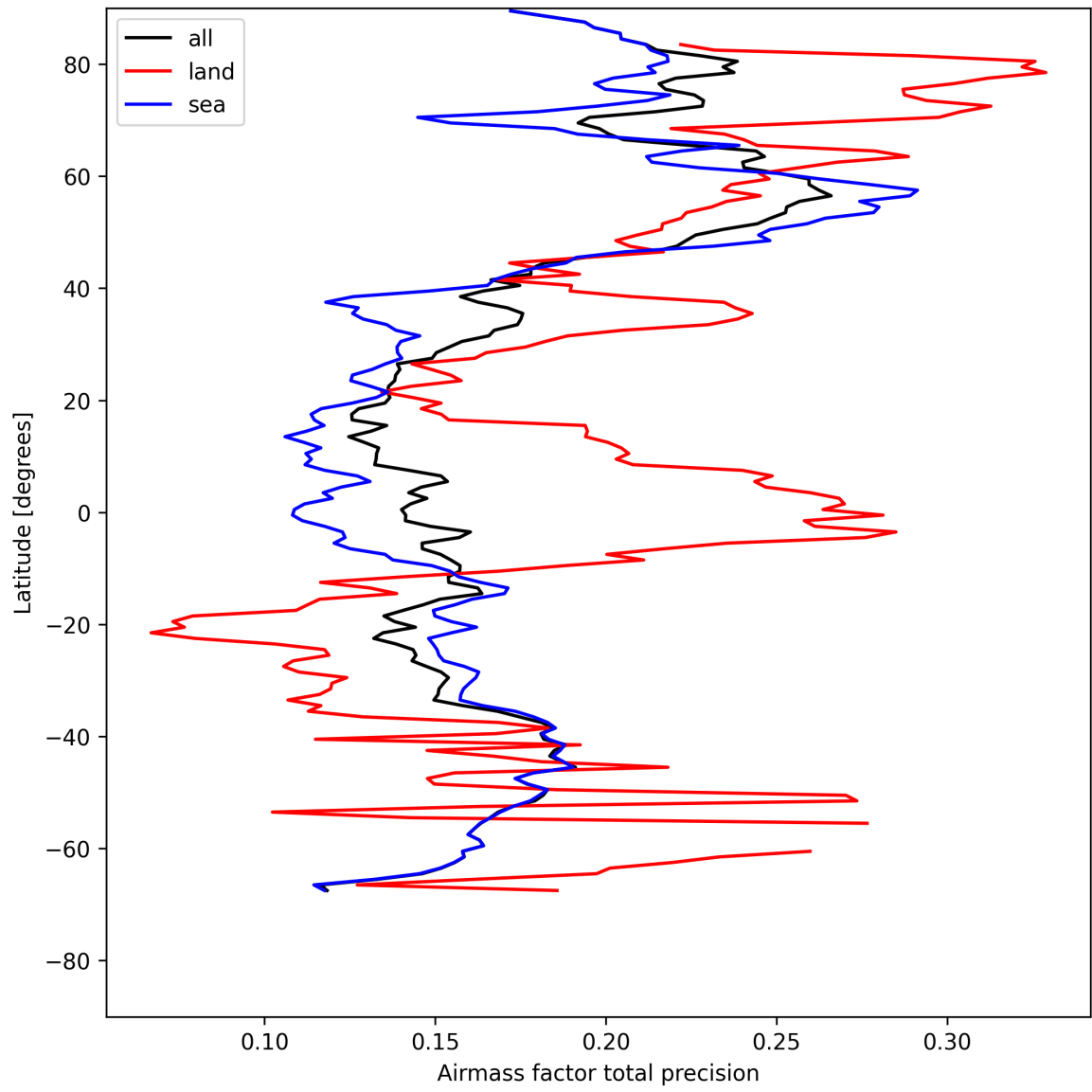
Figure 25: Zonal average of “Airmass factor total precision” for 2025-08-02 to 2025-08-03.
