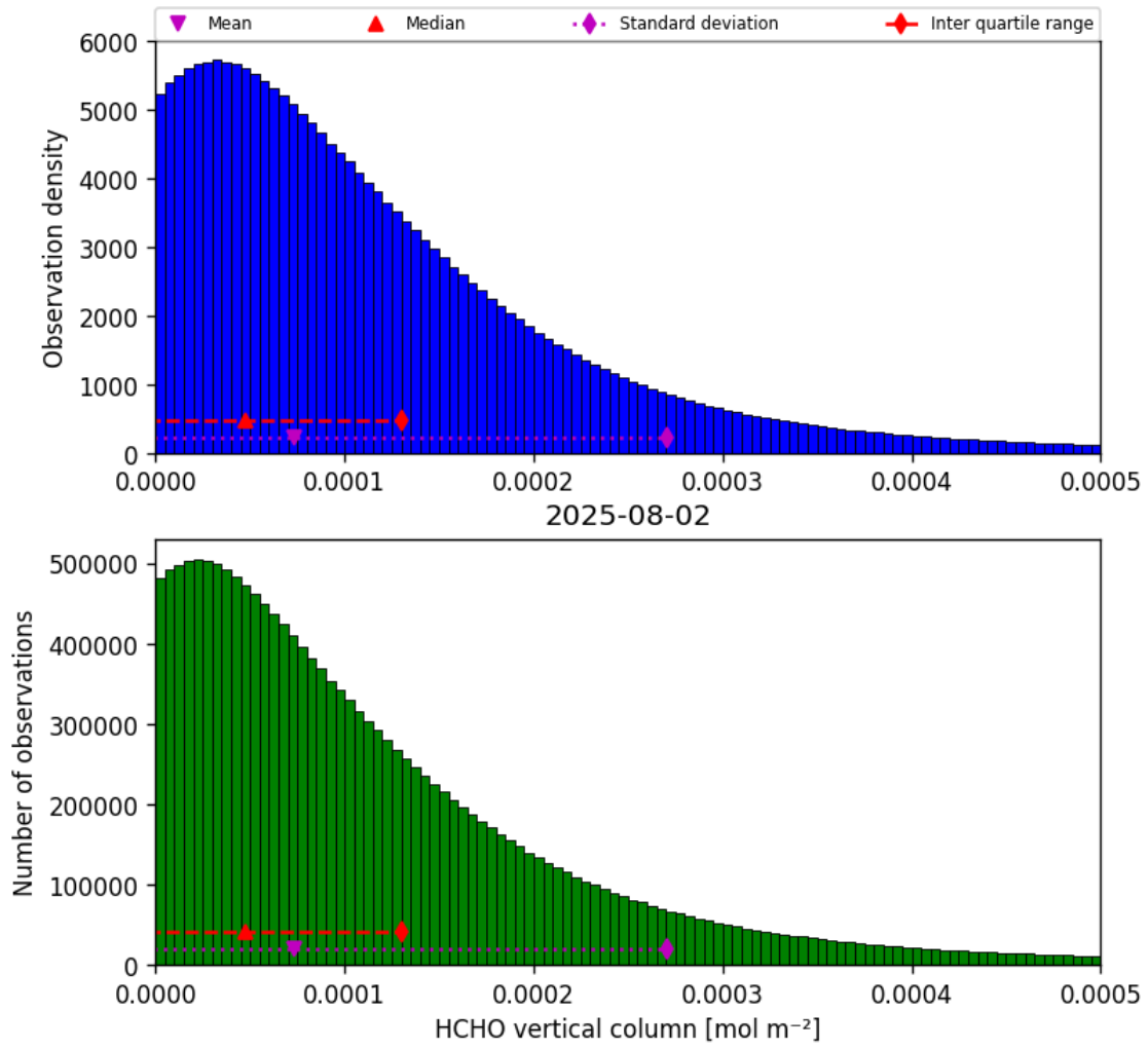
Figure 33: Histogram of “HCHO vertical column” for 2025-08-02 to 2025-08-03
