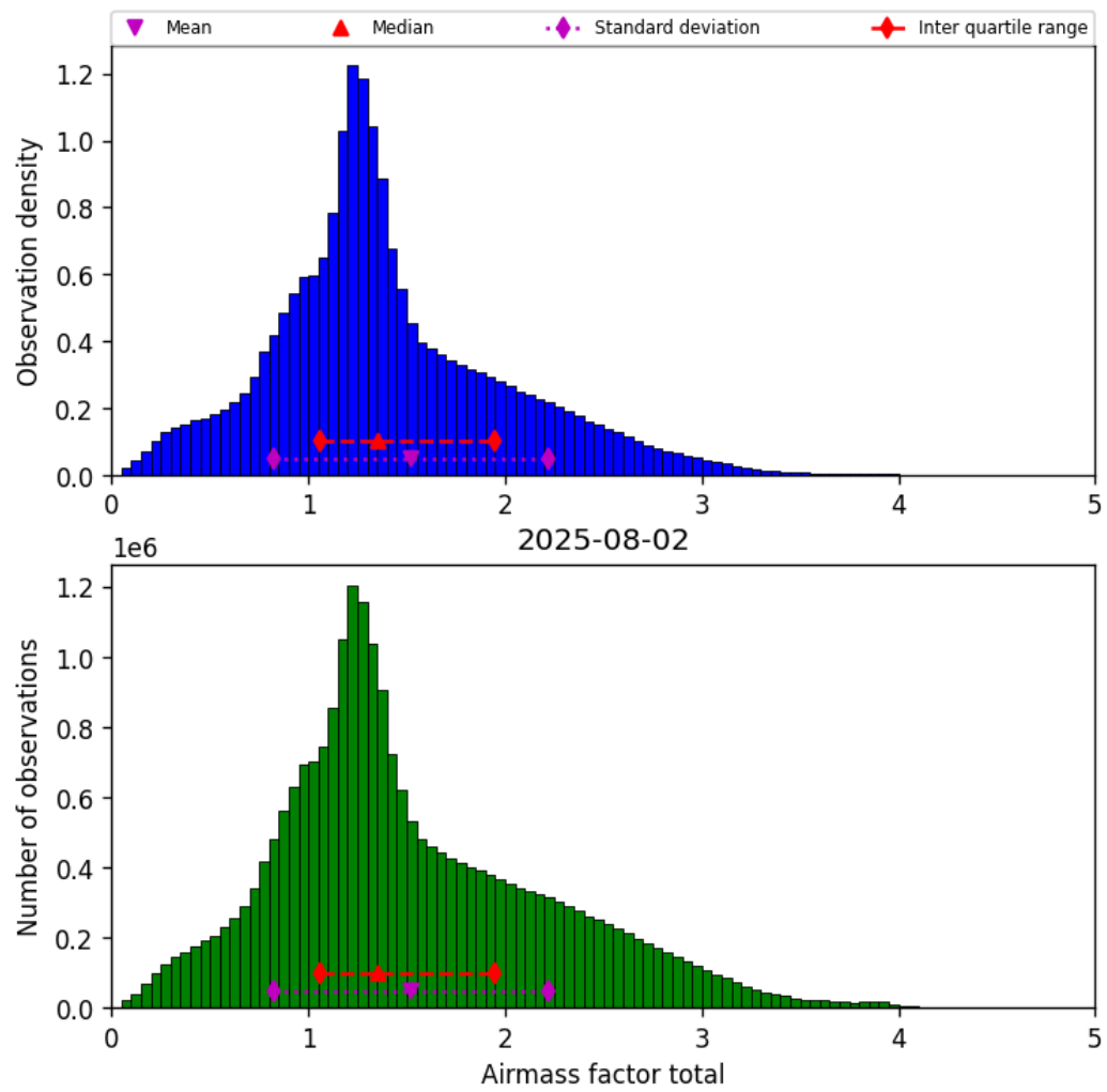
Figure 38: Histogram of “Airmass factor total” for 2025-08-02 to 2025-08-03
