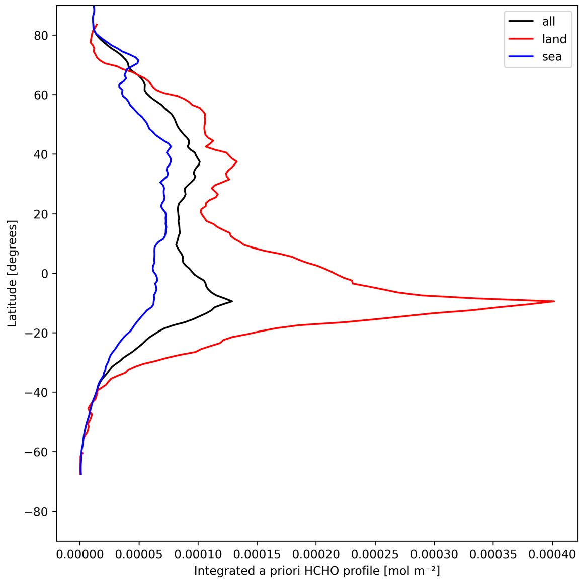
Figure 27: Zonal average of “Integrated a priori HCHO profile” for 2025-08-02 to 2025-08-03.
