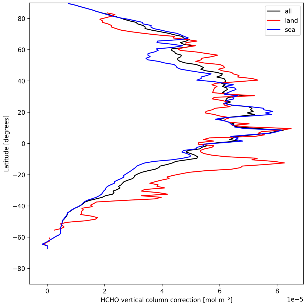
Figure 21: Zonal average of “HCHO vertical column correction” for 2025-08-02 to 2025-08-03.
