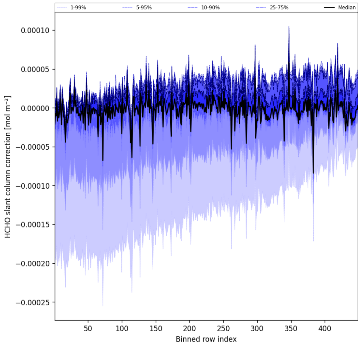
Figure 59: Along track statistics of “HCHO slant column correction” for 2025-08-02 to 2025-08-03
