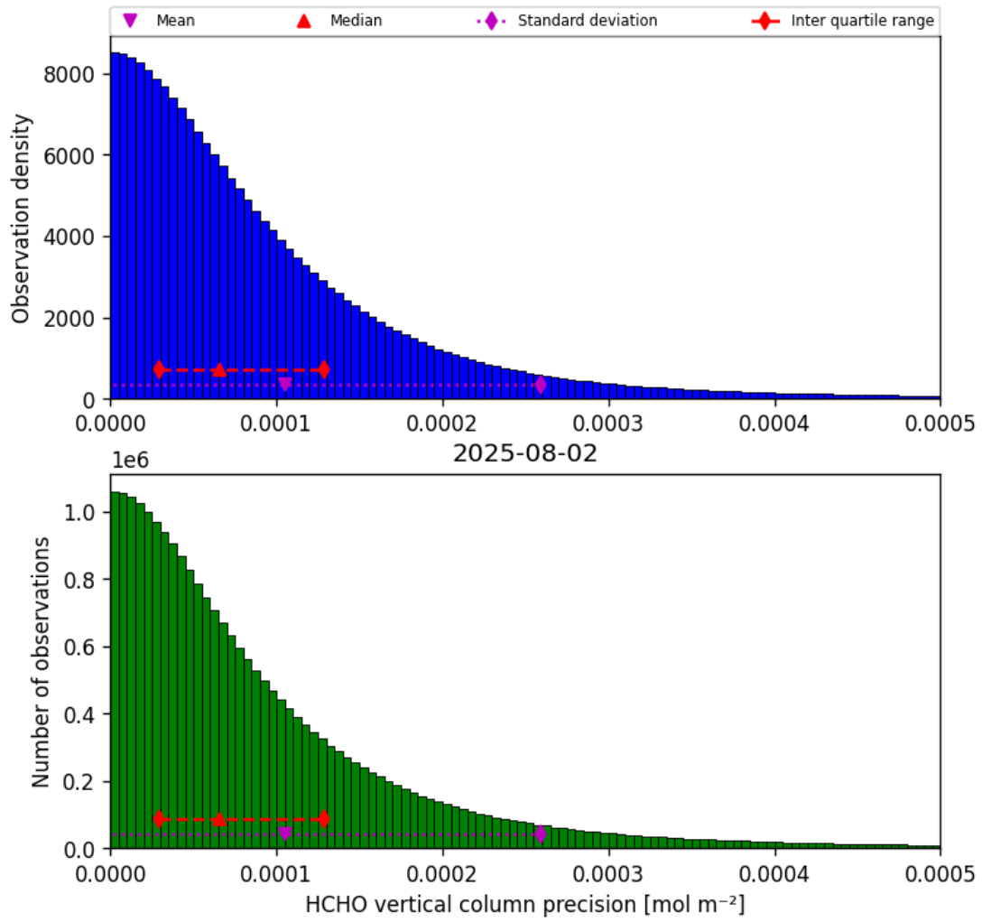
Figure 34: Histogram of “HCHO vertical column precision” for 2025-08-02 to 2025-08-03
