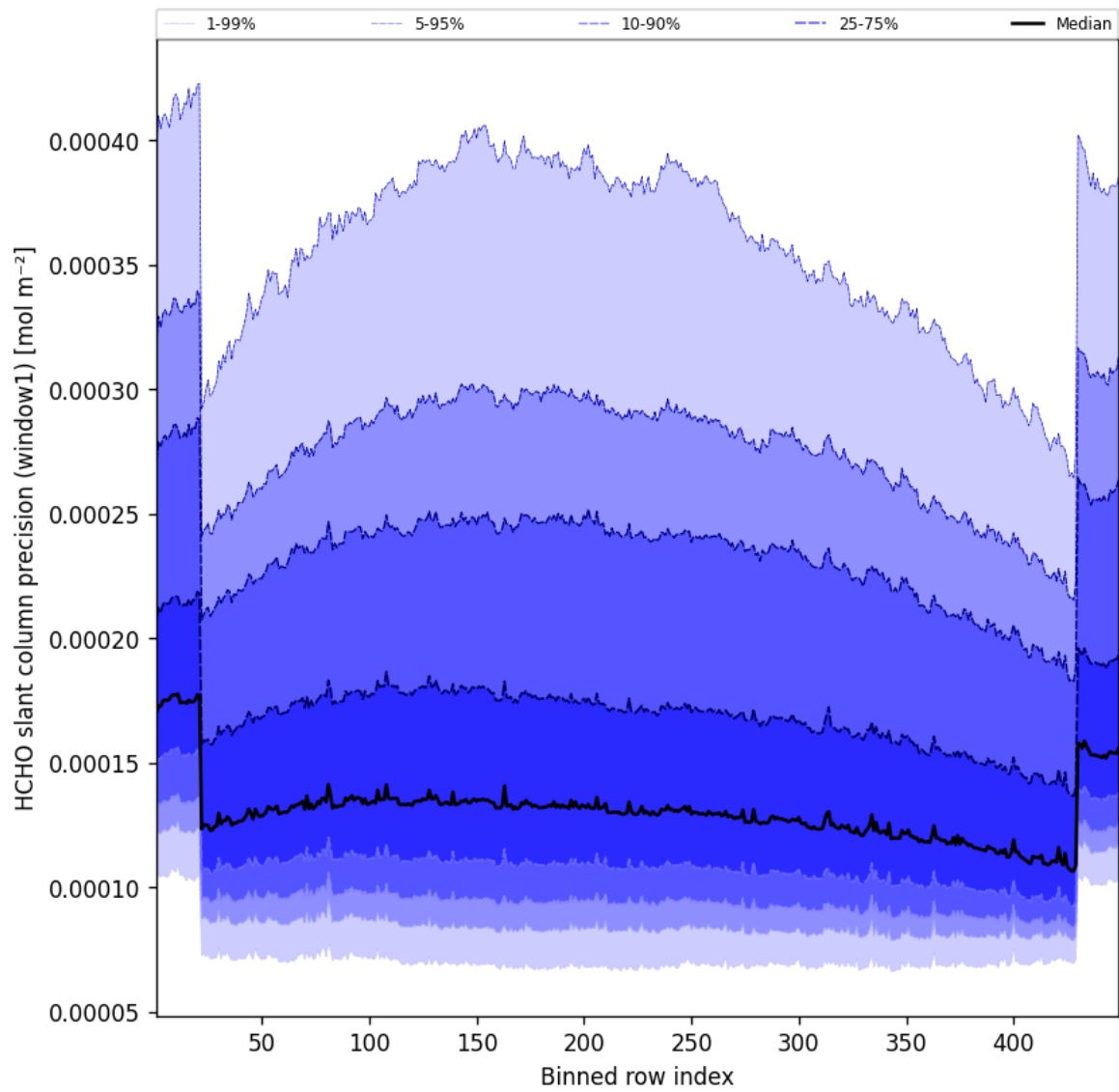
Figure 51: Along track statistics of “HCHO slant column precision (window1)” for 2025-08-02 to 2025-08-03
