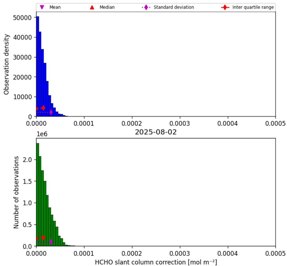
Figure 45: Histogram of “HCHO slant column correction” for 2025-08-02 to 2025-08-03
