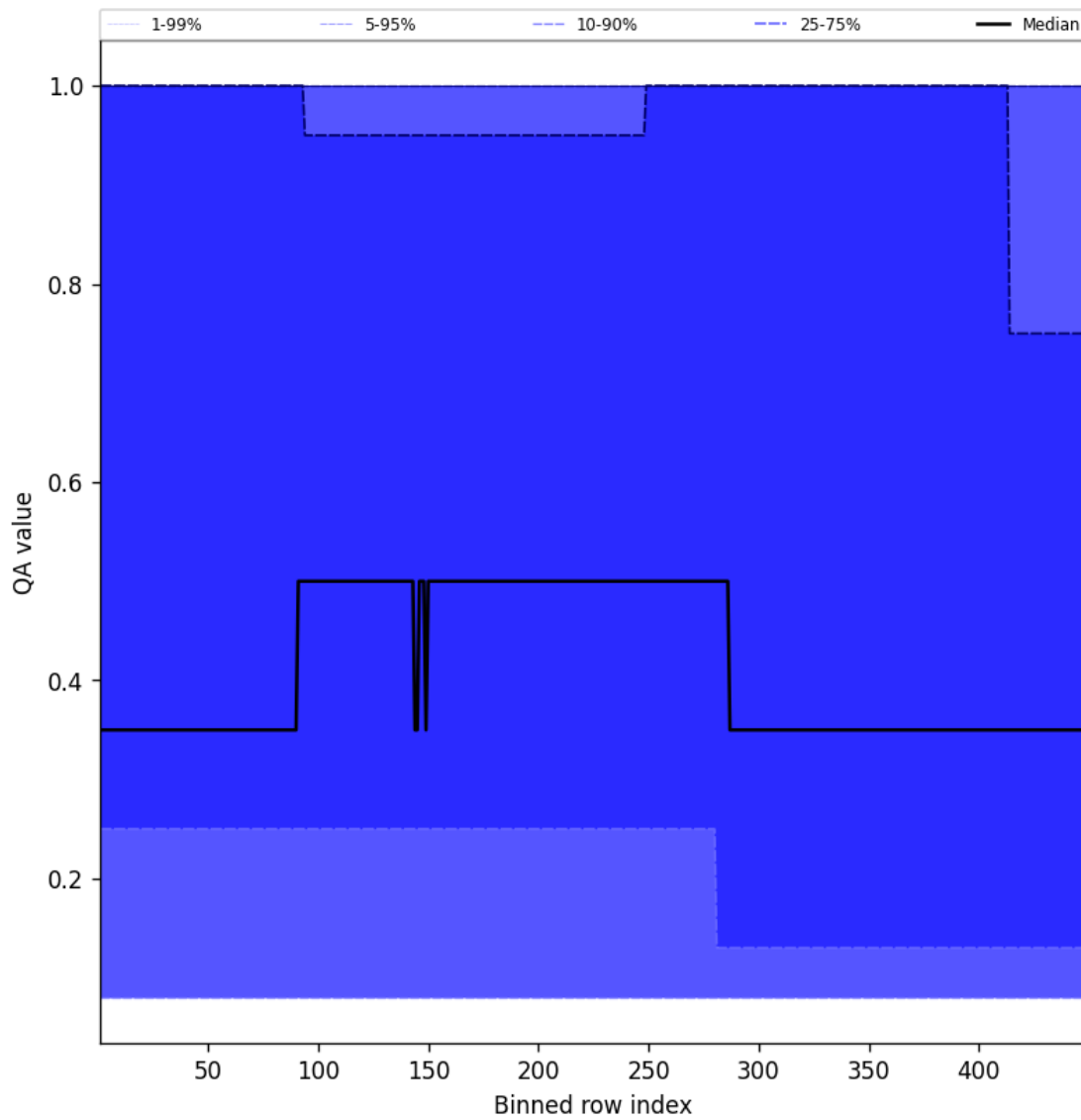
Figure 46: Along track statistics of “QA value” for 2025-08-02 to 2025-08-03
