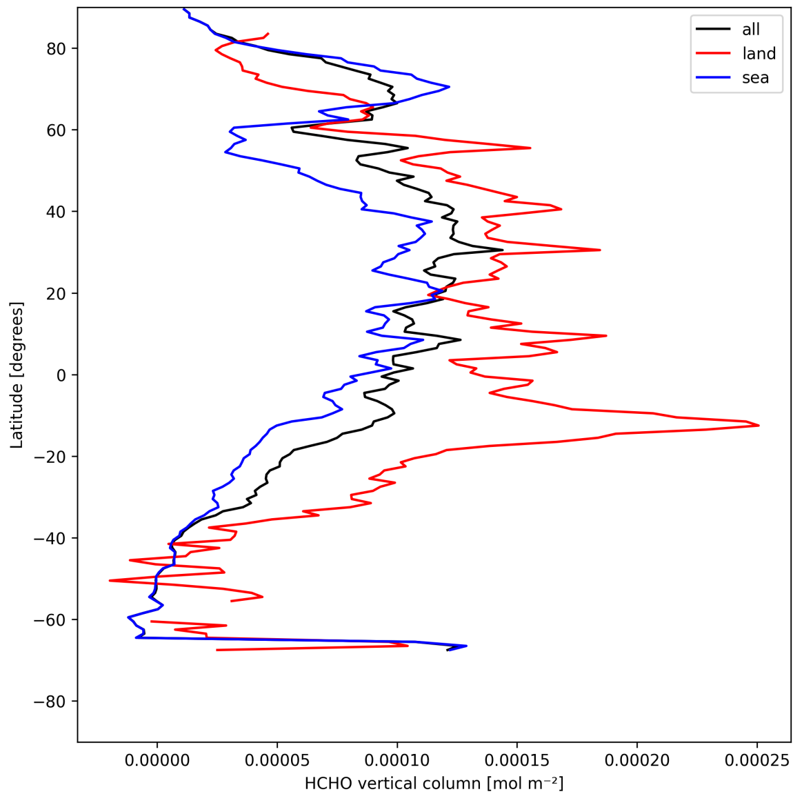
Figure 19: Zonal average of “HCHO vertical column” for 2025-08-02 to 2025-08-03.
