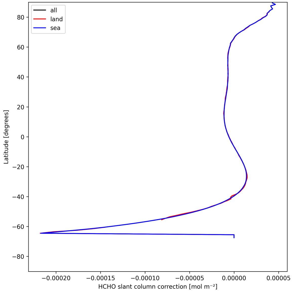
Figure 31: Zonal average of “HCHO slant column correction” for 2025-08-02 to 2025-08-03.
