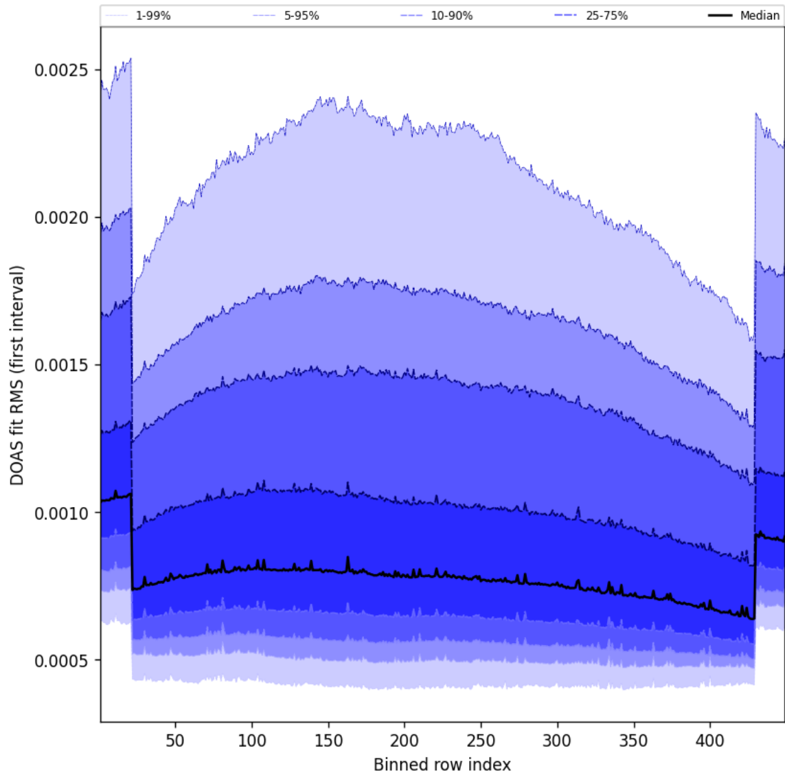
Figure 58: Along track statistics of “DOAS fit RMS (first interval)” for 2025-08-02 to 2025-08-03
