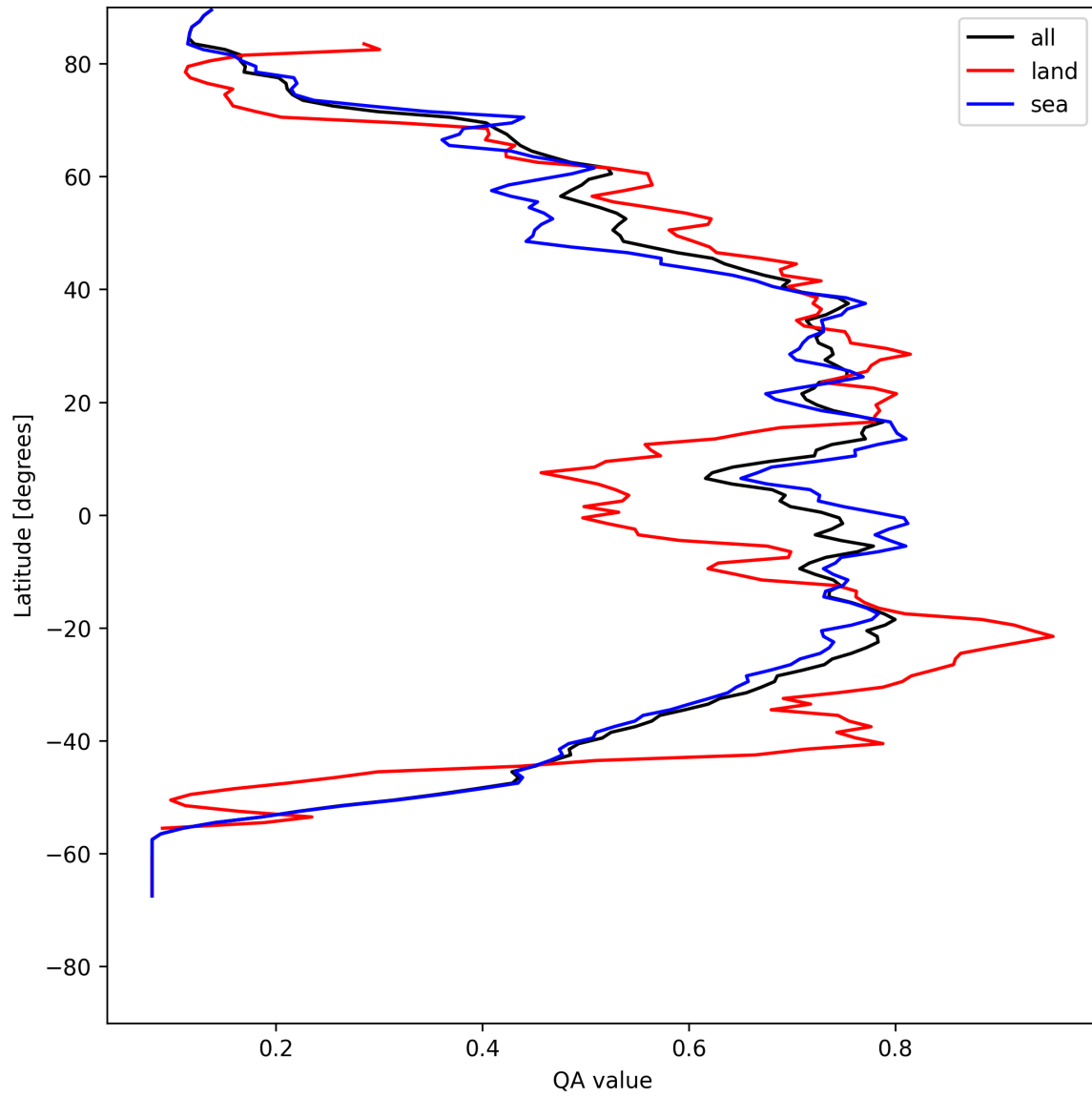
Figure 18: Zonal average of “QA value” for 2025-08-02 to 2025-08-03.
