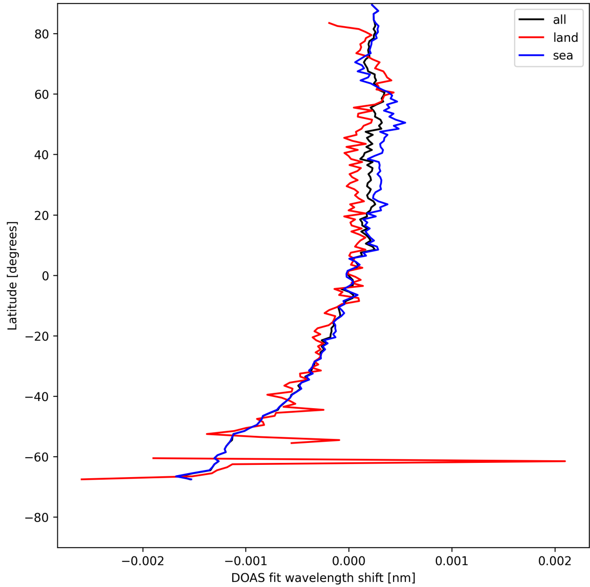
Figure 28: Zonal average of “DOAS fit wavelength shift” for 2025-08-02 to 2025-08-03.
