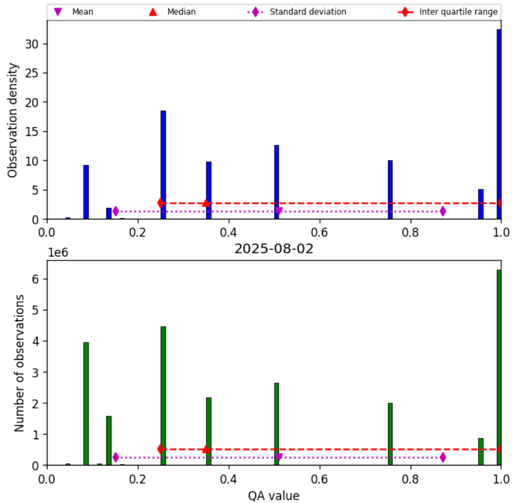
Figure 32: Histogram of “QA value” for 2025-08-02 to 2025-08-03
