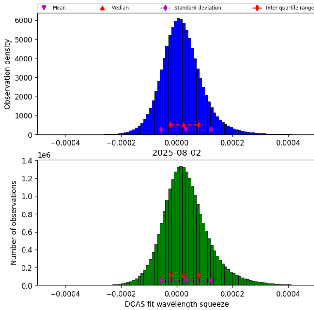
Figure 43: Histogram of “DOAS fit wavelength squeeze” for 2025-08-02 to 2025-08-03
