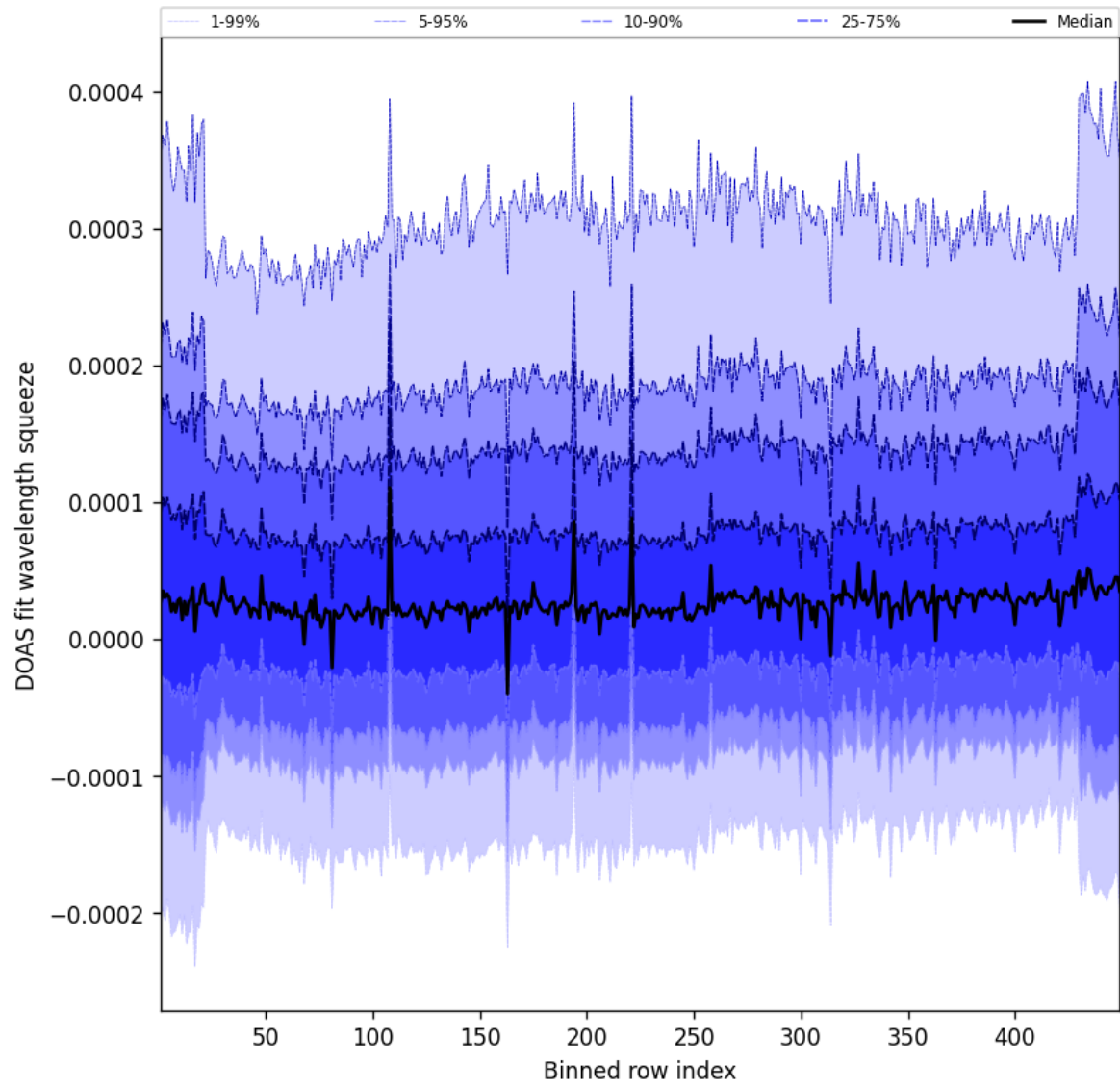
Figure 57: Along track statistics of “DOAS fit wavelength squeeze” for 2025-08-02 to 2025-08-03
