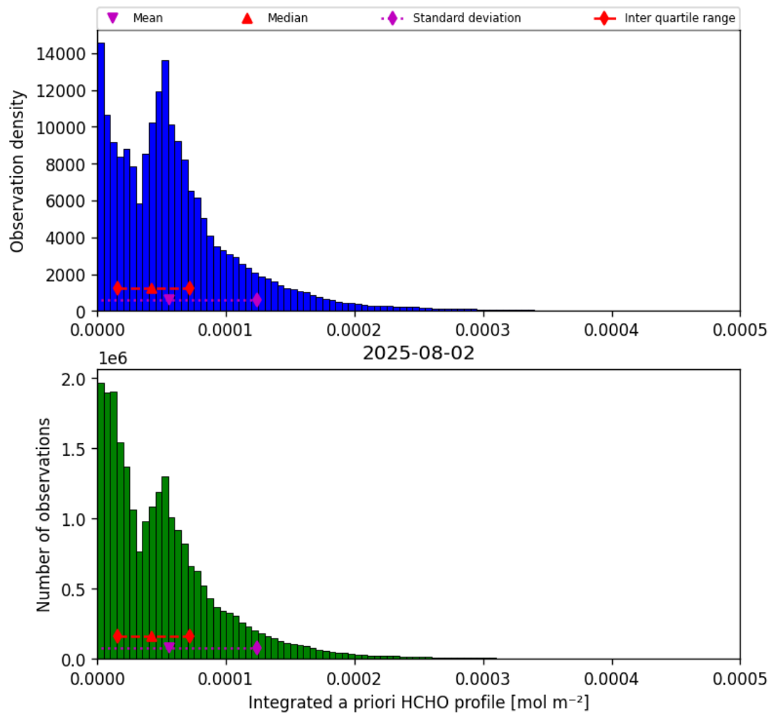
Figure 41: Histogram of “Integrated a priori HCHO profile” for 2025-08-02 to 2025-08-03
