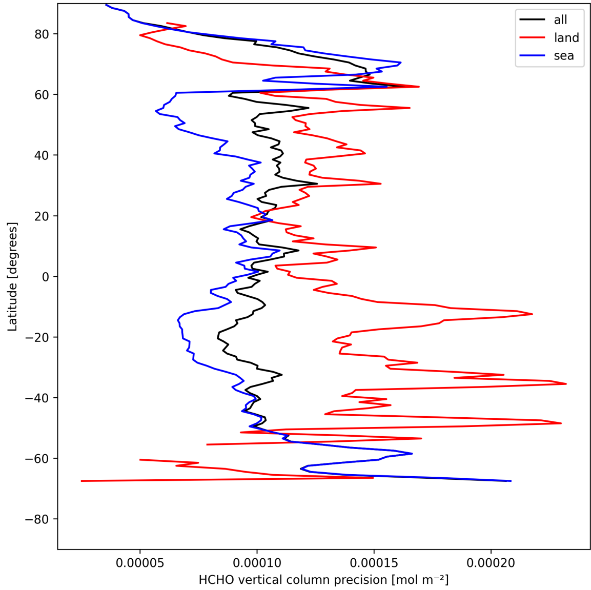
Figure 20: Zonal average of “HCHO vertical column precision” for 2025-08-02 to 2025-08-03.
