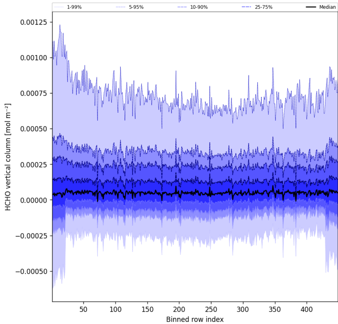
Figure 47: Along track statistics of “HCHO vertical column” for 2025-08-02 to 2025-08-03
