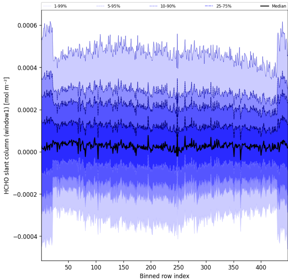
Figure 50: Along track statistics of “HCHO slant column (window1)” for 2025-08-02 to 2025-08-03
