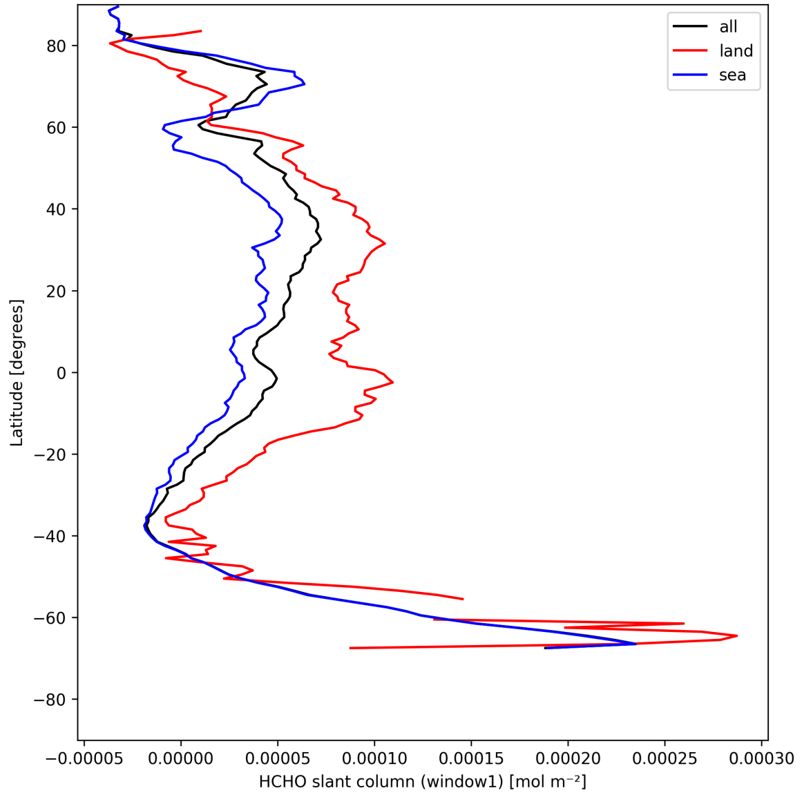
Figure 22: Zonal average of “HCHO slant column (window1)” for 2025-08-02 to 2025-08-03.
