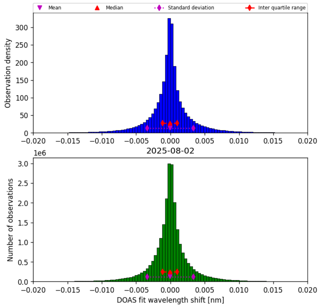
Figure 42: Histogram of “DOAS fit wavelength shift” for 2025-08-02 to 2025-08-03
