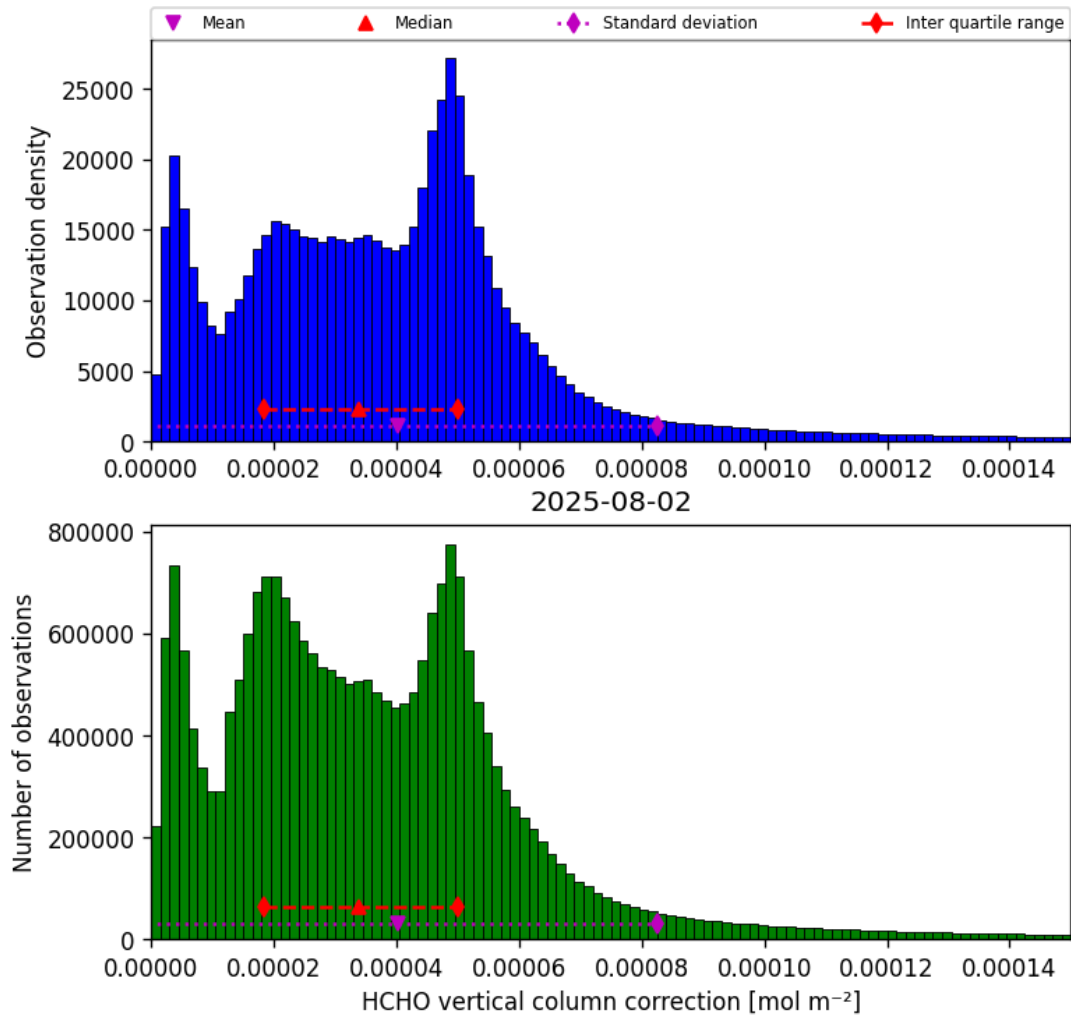
Figure 35: Histogram of “HCHO vertical column correction” for 2025-08-02 to 2025-08-03
