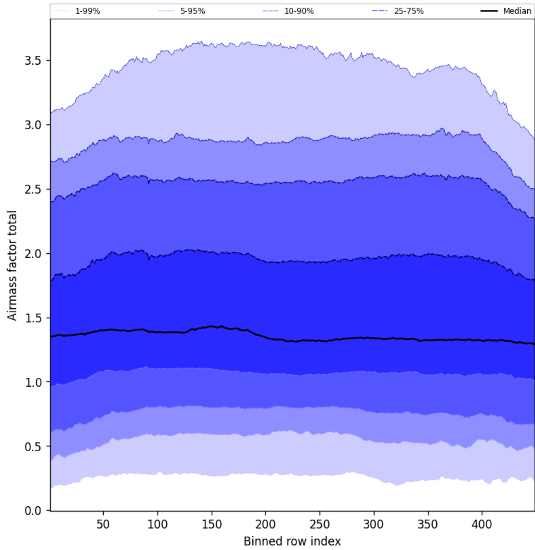
Figure 52: Along track statistics of “Air mass factor total” for 2025-08-02 to 2025-08-03
