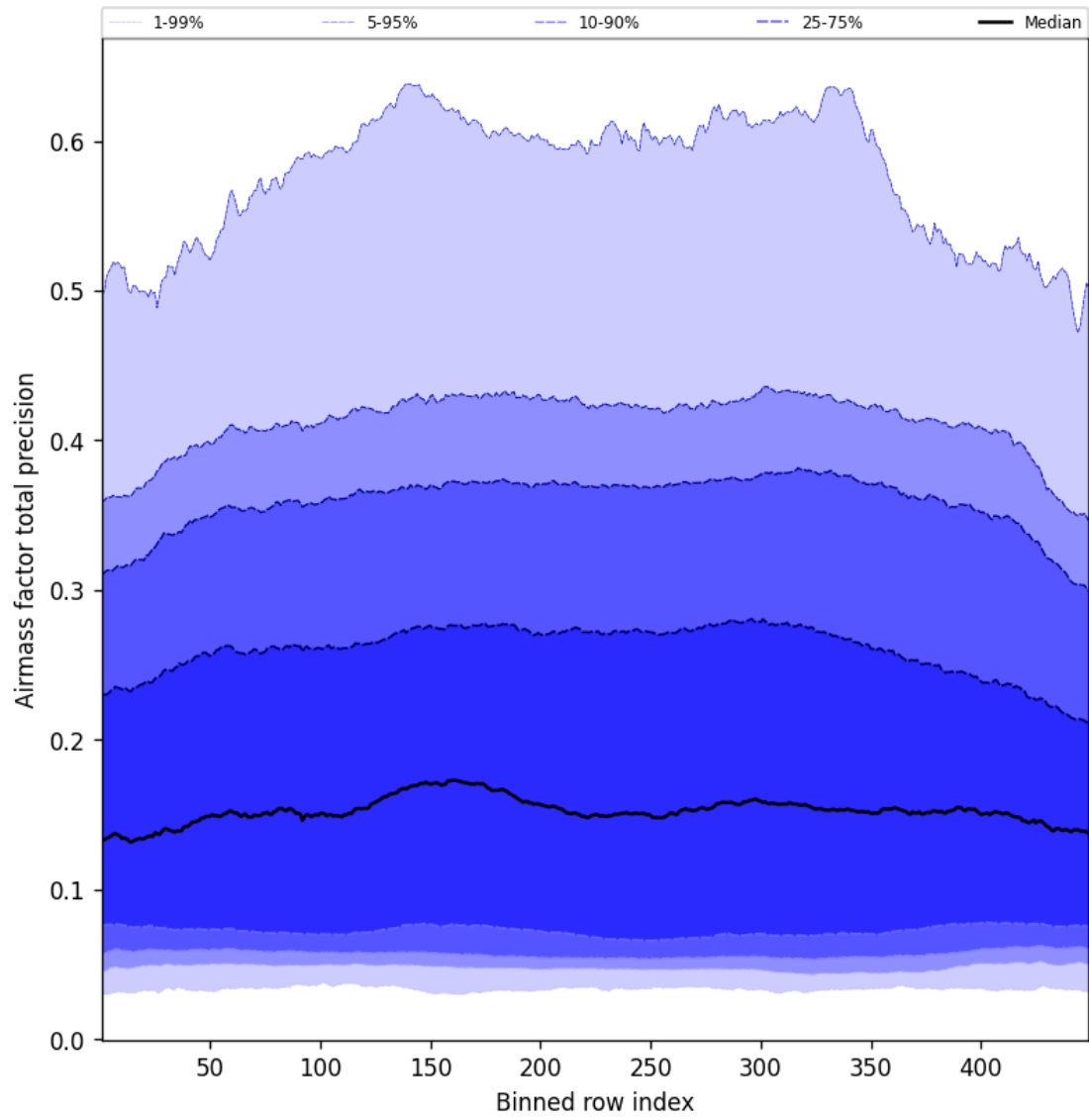
Figure 53: Along track statistics of “Airmass factor total precision” for 2025-08-02 to 2025-08-03
