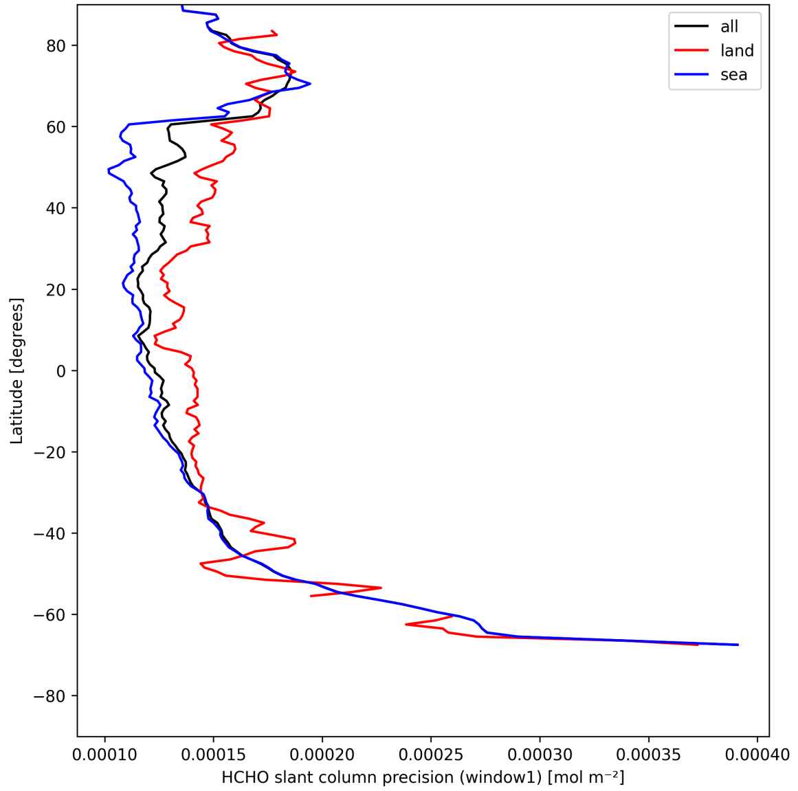
Figure 23: Zonal average of “HCHO slant column precision (window1)” for 2025-08-02 to 2025-08-03.
