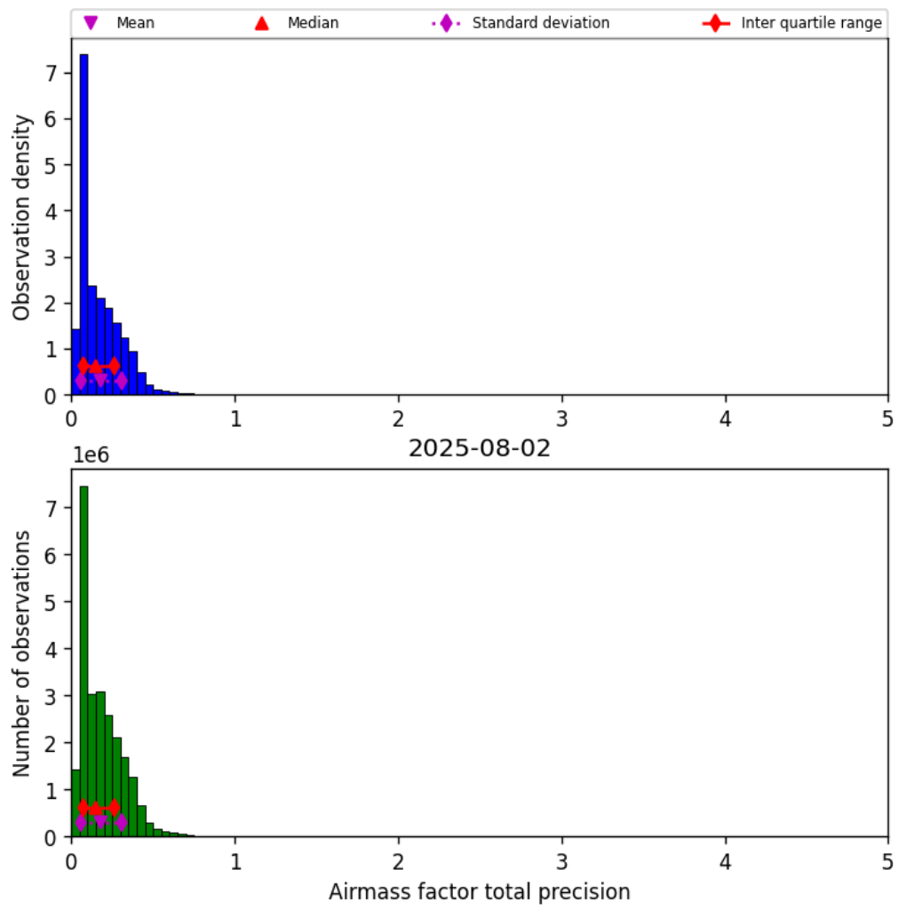
Figure 39: Histogram of “Airmass factor total precision” for 2025-08-02 to 2025-08-03
