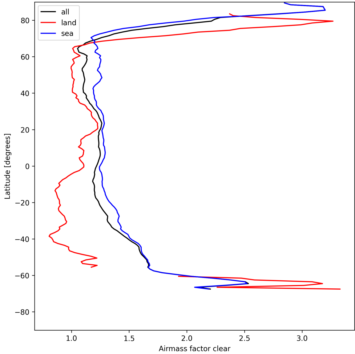
Figure 26: Zonal average of “Airmass factor clear” for 2025-08-02 to 2025-08-03.
