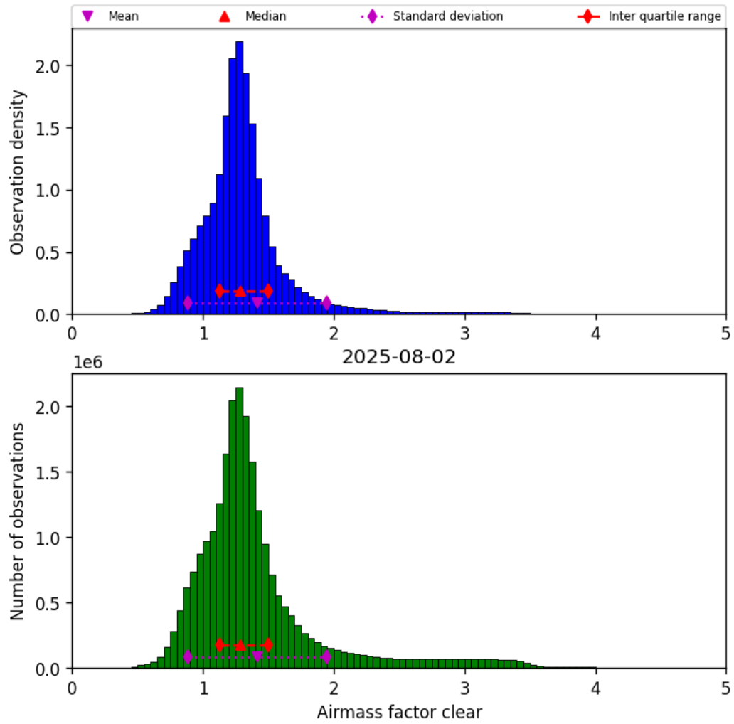
Figure 40: Histogram of “Airmass factor clear” for 2025-08-02 to 2025-08-03
