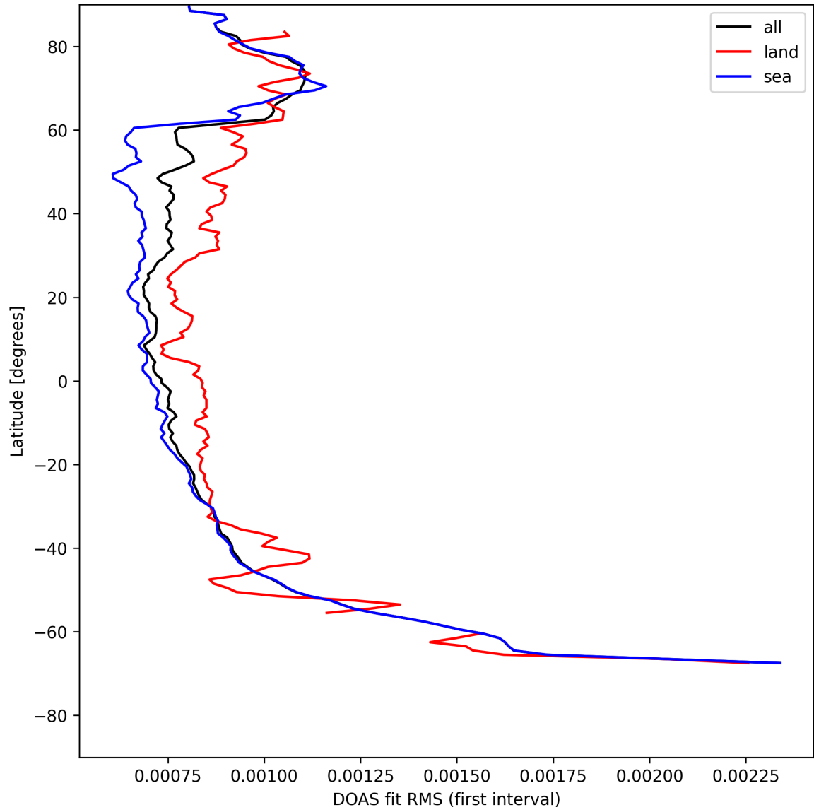
Figure 30: Zonal average of “DOAS fit RMS (first interval)” for 2025-08-02 to 2025-08-03.
