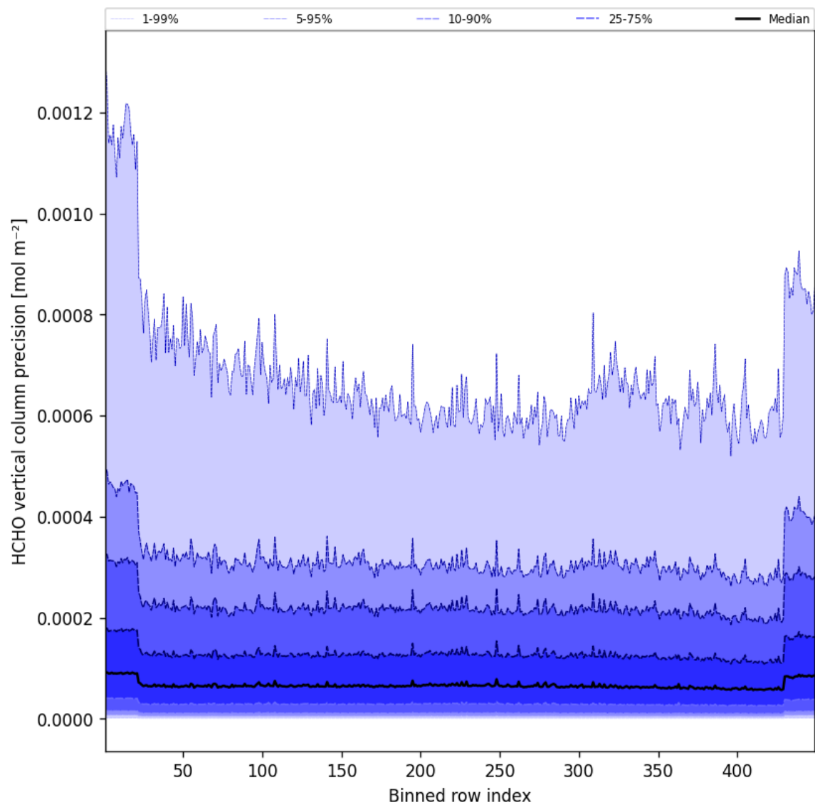
Figure 48: Along track statistics of “HCHO vertical column precision” for 2025-08-02 to 2025-08-03
