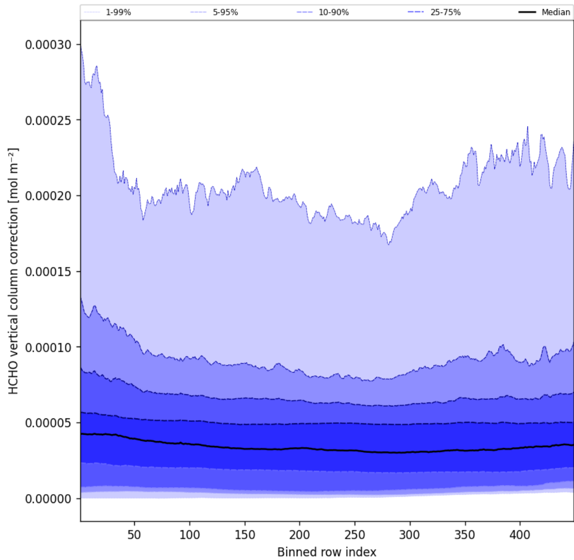
Figure 49: Along track statistics of “HCHO vertical column correction” for 2025-08-02 to 2025-08-03
