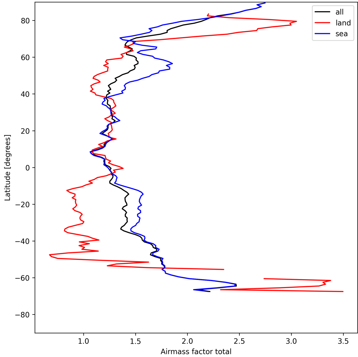
Figure 24: Zonal average of “Airmass factor total” for 2025-08-02 to 2025-08-03.
