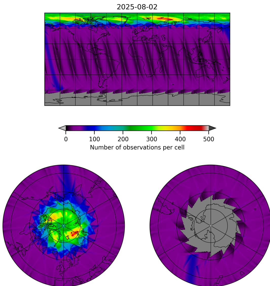
Figure 17: Map of the number of observations for 2025-08-02 to 2025-08-03
