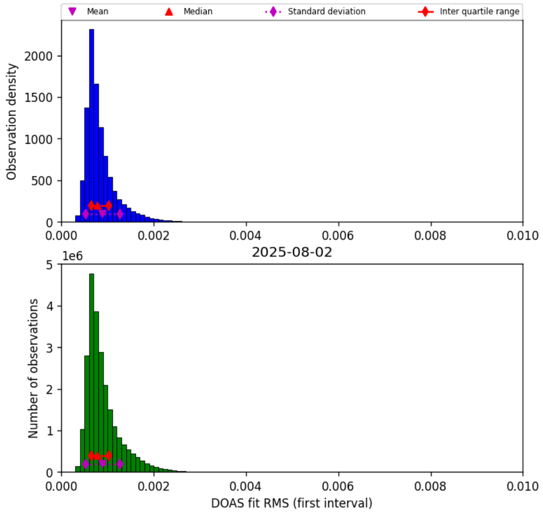
Figure 44: Histogram of “DOAS fit RMS (first interval)” for 2025-08-02 to 2025-08-03
