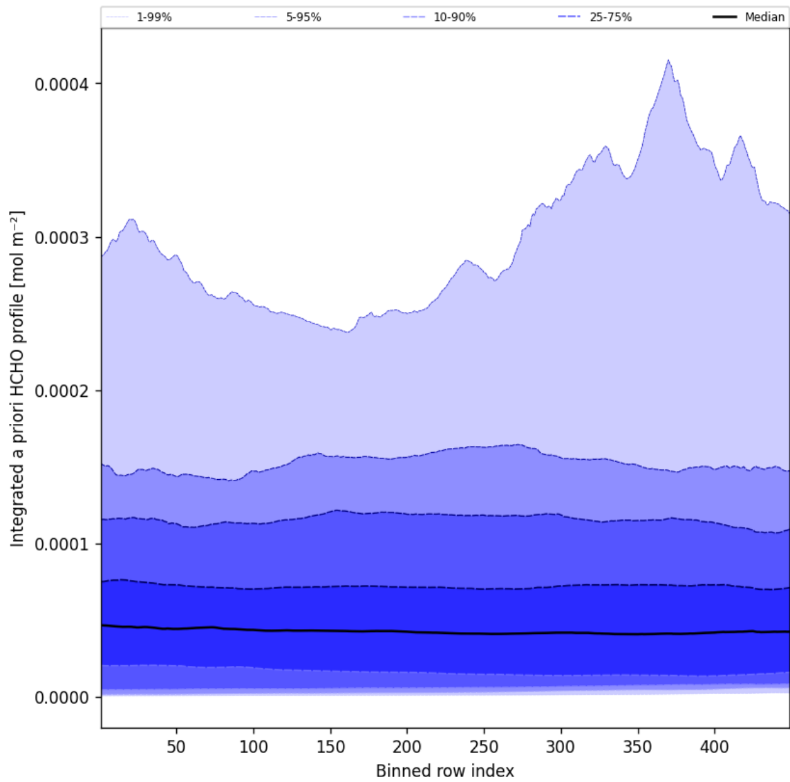
Figure 55: Along track statistics of “Integrated a priori HCHO profile” for 2025-08-02 to 2025-08-03
