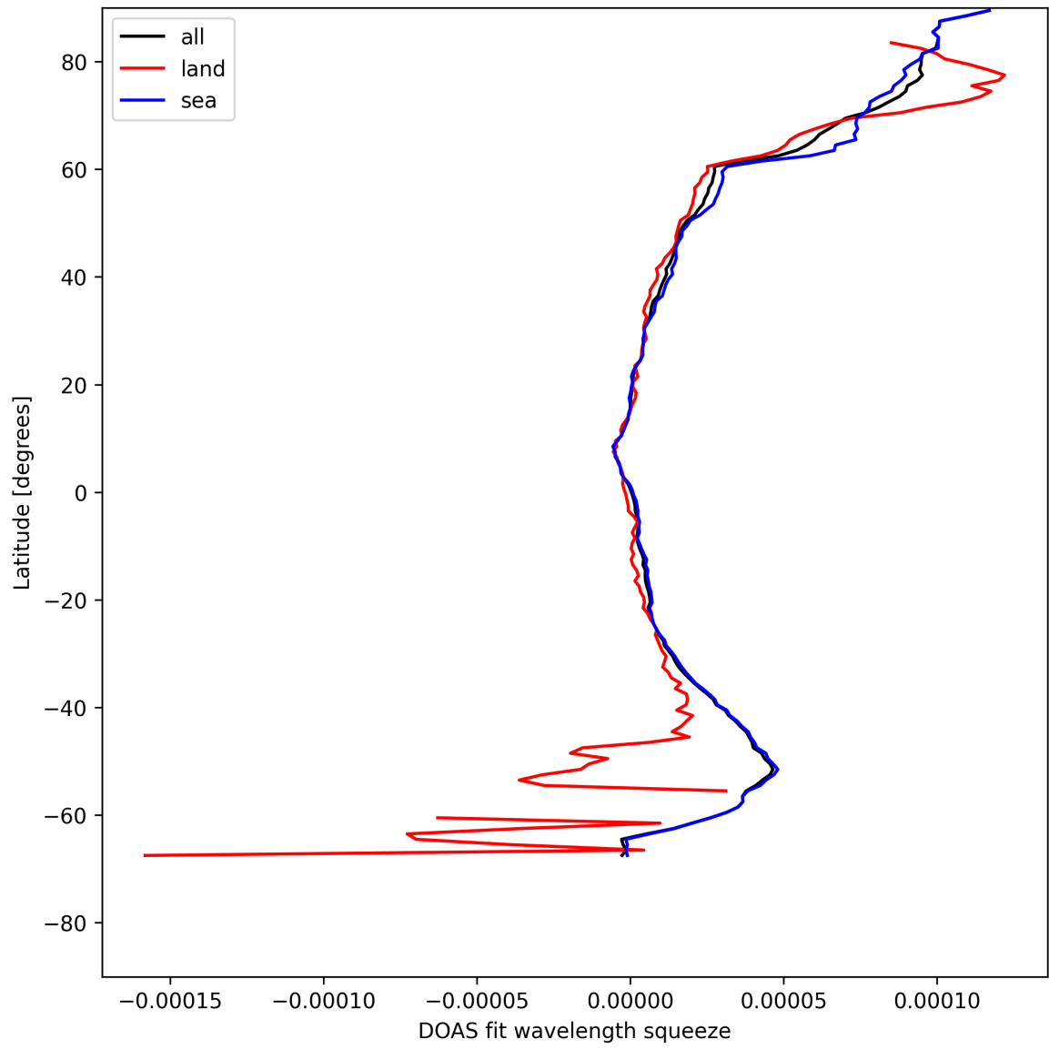
Figure 29: Zonal average of “DOAS fit wavelength squeeze” for 2025-08-02 to 2025-08-03.
