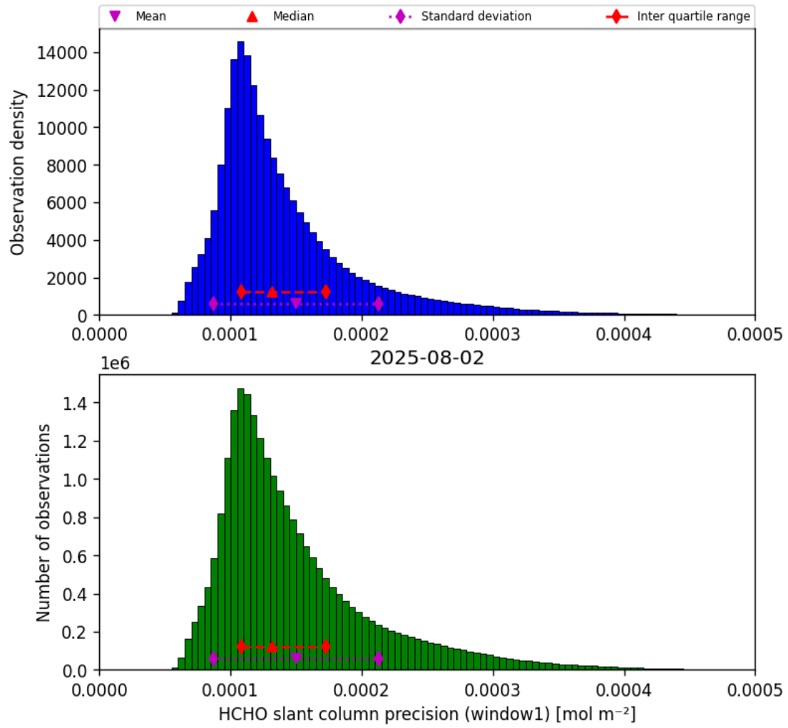
Figure 37: Histogram of “HCHO slant column precision (window1)” for 2025-08-02 to 2025-08-03
