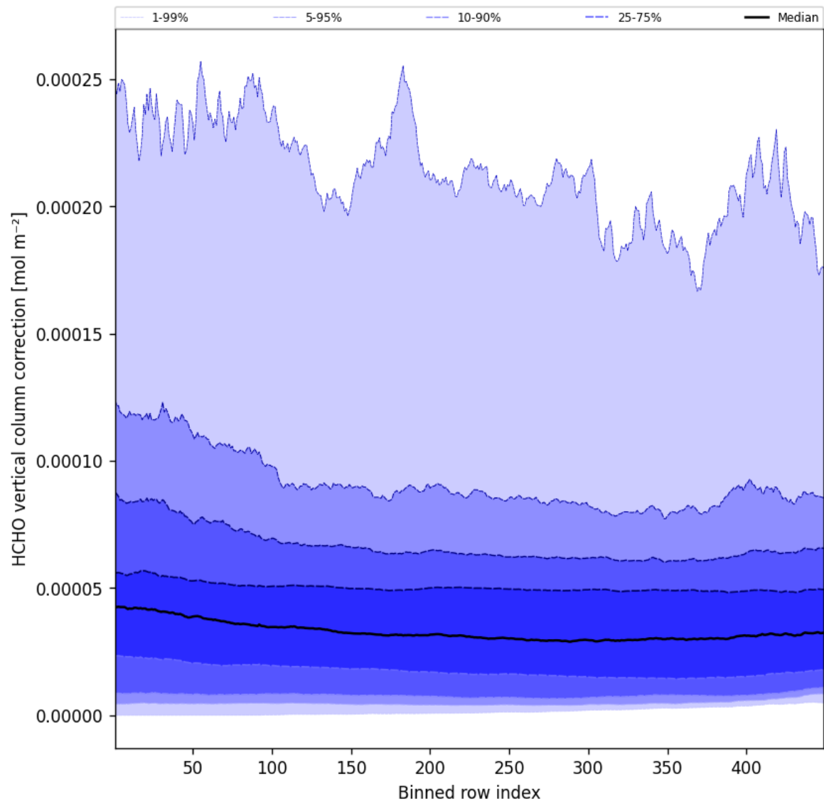
Figure 49: Along track statistics of “HCHO vertical column correction” for 2025-08-03 to 2025-08-04
