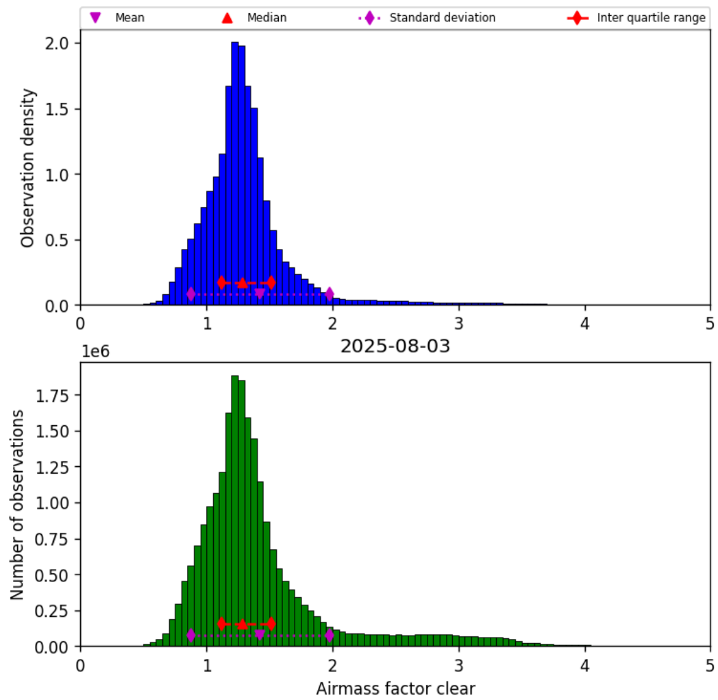
Figure 40: Histogram of “Airmass factor clear” for 2025-08-03 to 2025-08-04
