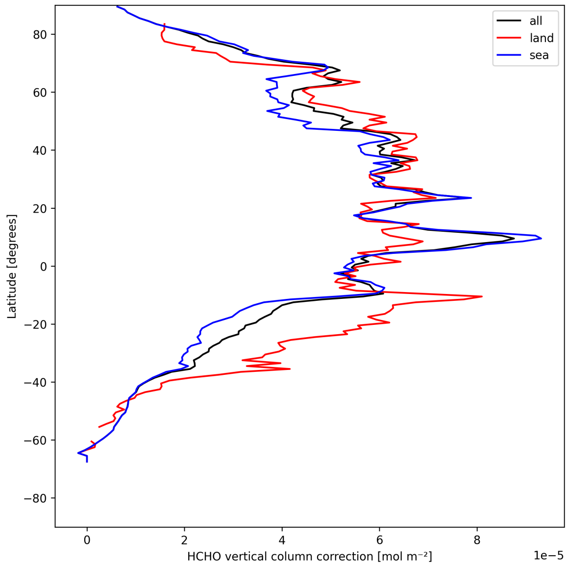
Figure 21: Zonal average of “HCHO vertical column correction” for 2025-08-03 to 2025-08-04.
