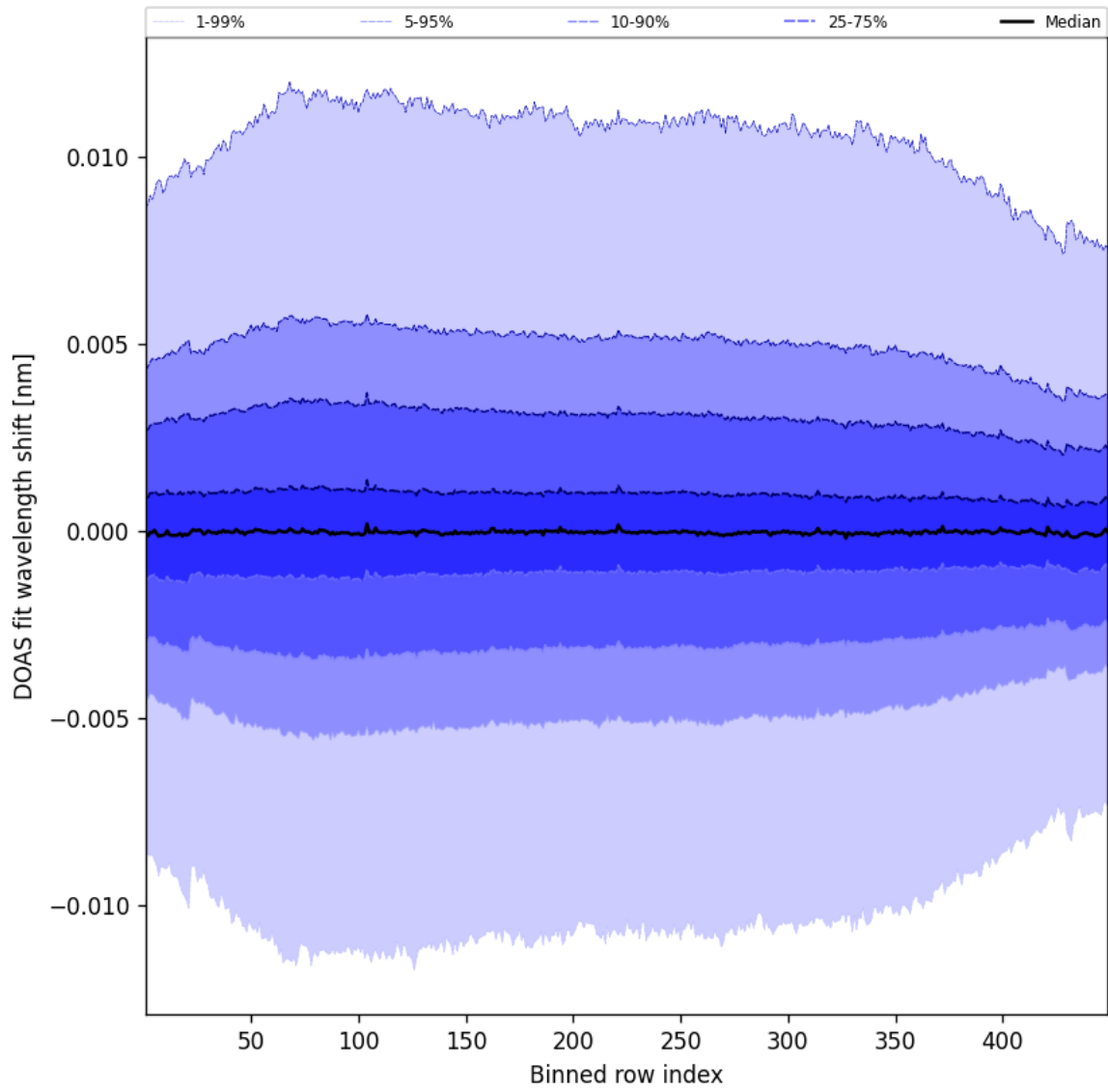
Figure 56: Along track statistics of “DOAS fit wavelength shift” for 2025-08-03 to 2025-08-04
