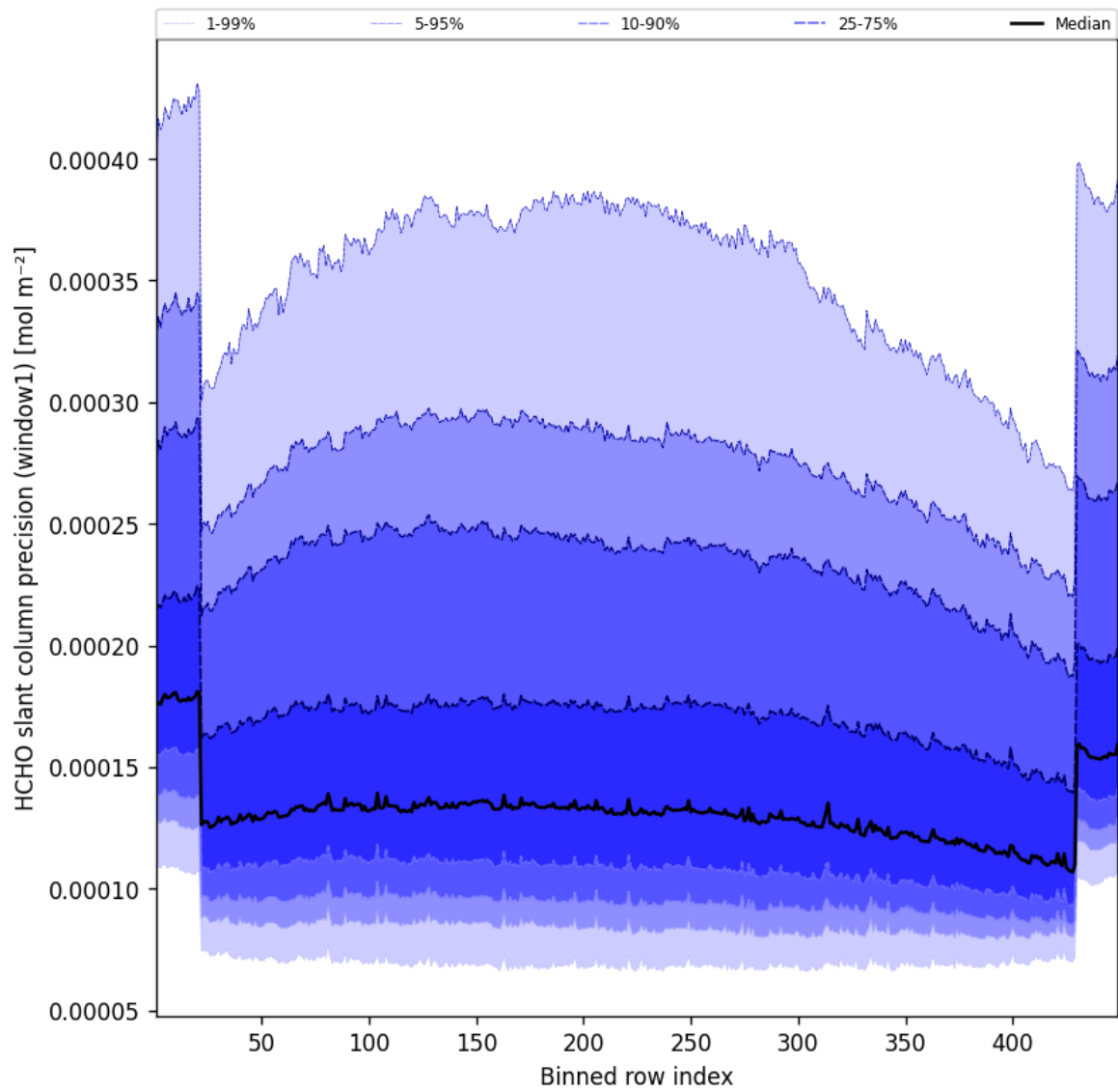
Figure 51: Along track statistics of “HCHO slant column precision (window1)” for 2025-08-03 to 2025-08-04
