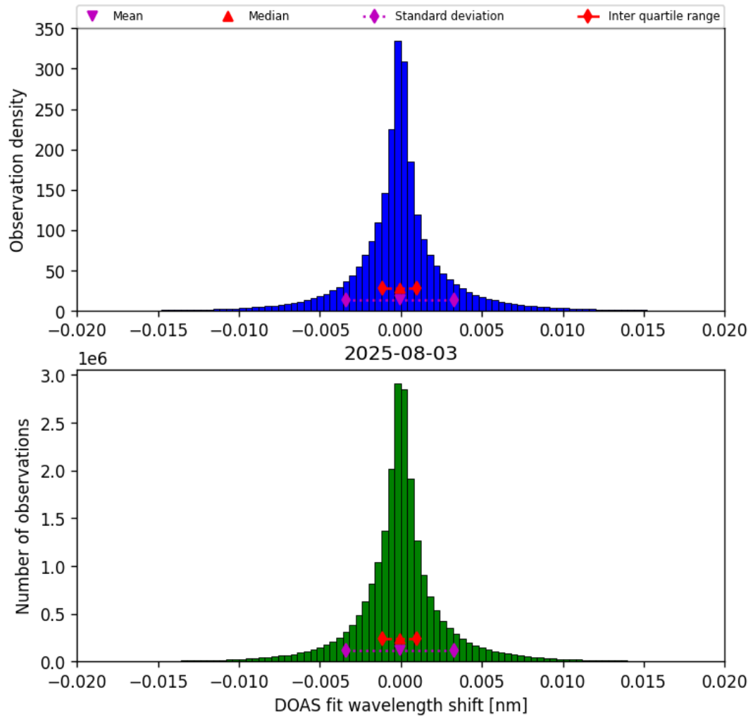
Figure 42: Histogram of “DOAS fit wavelength shift” for 2025-08-03 to 2025-08-04
