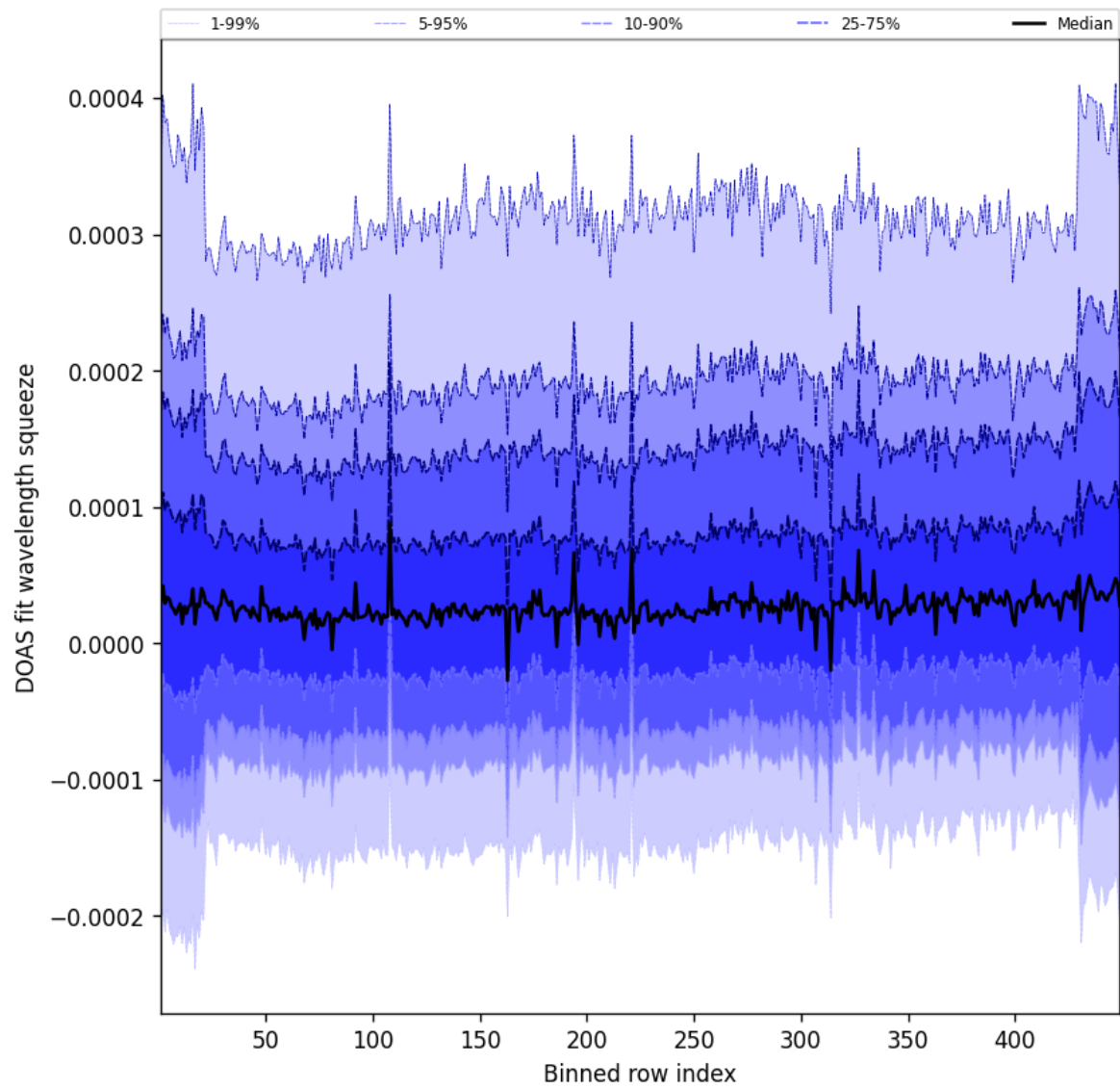
Figure 57: Along track statistics of “DOAS fit wavelength squeeze” for 2025-08-03 to 2025-08-04
