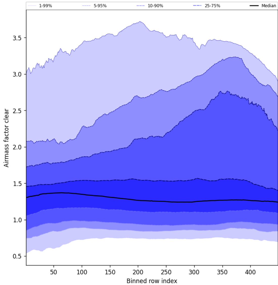
Figure 54: Along track statistics of “Airmass factor clear” for 2025-08-03 to 2025-08-04
