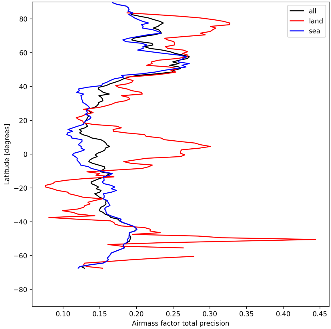
Figure 25: Zonal average of “Airmass factor total precision” for 2025-08-03 to 2025-08-04.
