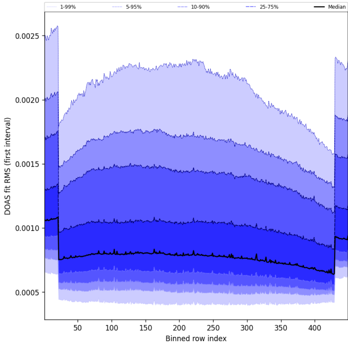
Figure 58: Along track statistics of “DOAS fit RMS (first interval)” for 2025-08-03 to 2025-08-04
