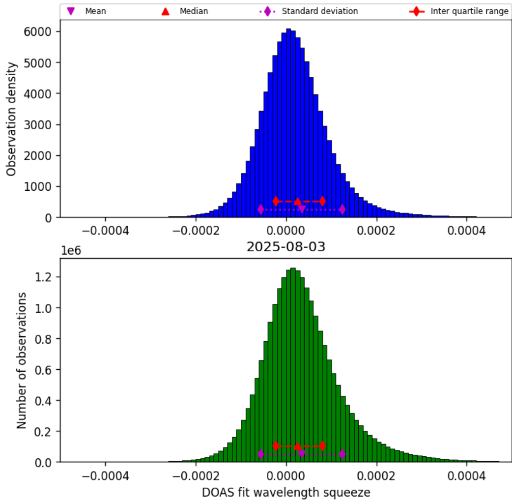
Figure 43: Histogram of “DOAS fit wavelength squeeze” for 2025-08-03 to 2025-08-04
