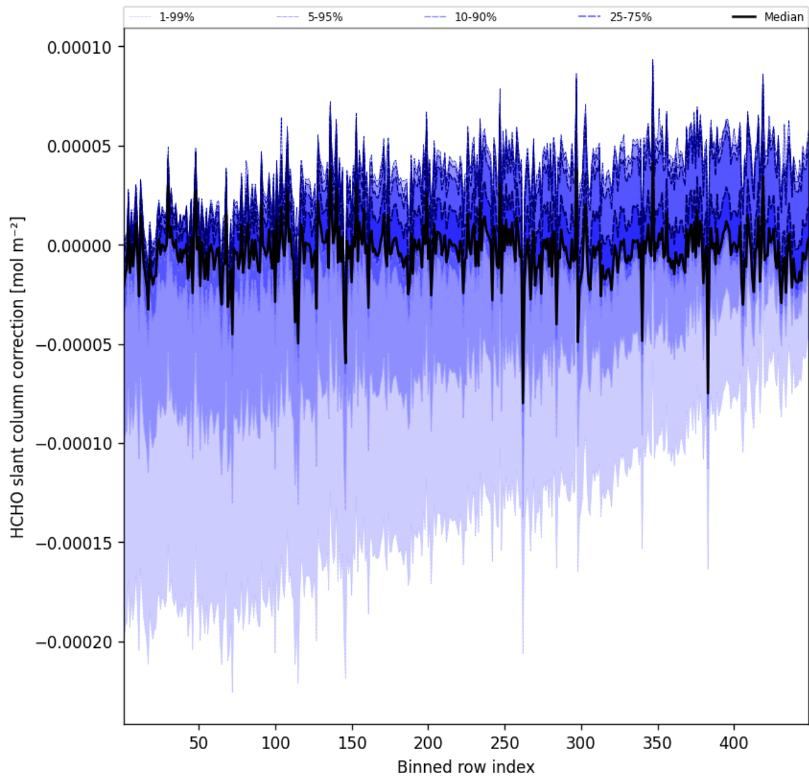
Figure 59: Along track statistics of “HCHO slant column correction” for 2025-08-03 to 2025-08-04
