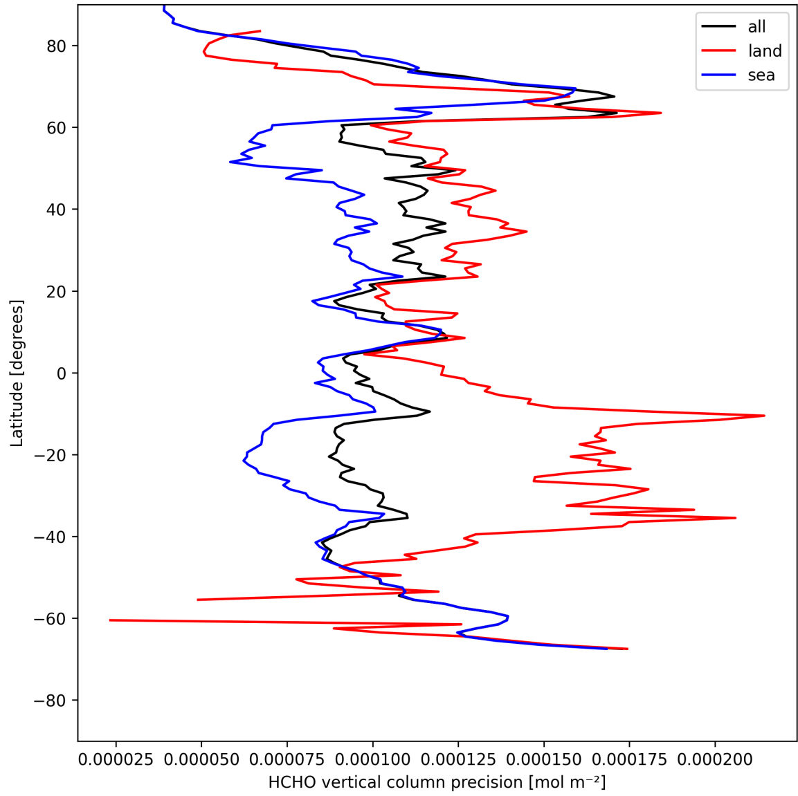
Figure 20: Zonal average of "HCHO vertical column precision" for 2025-08-03 to 2025-08-04.
