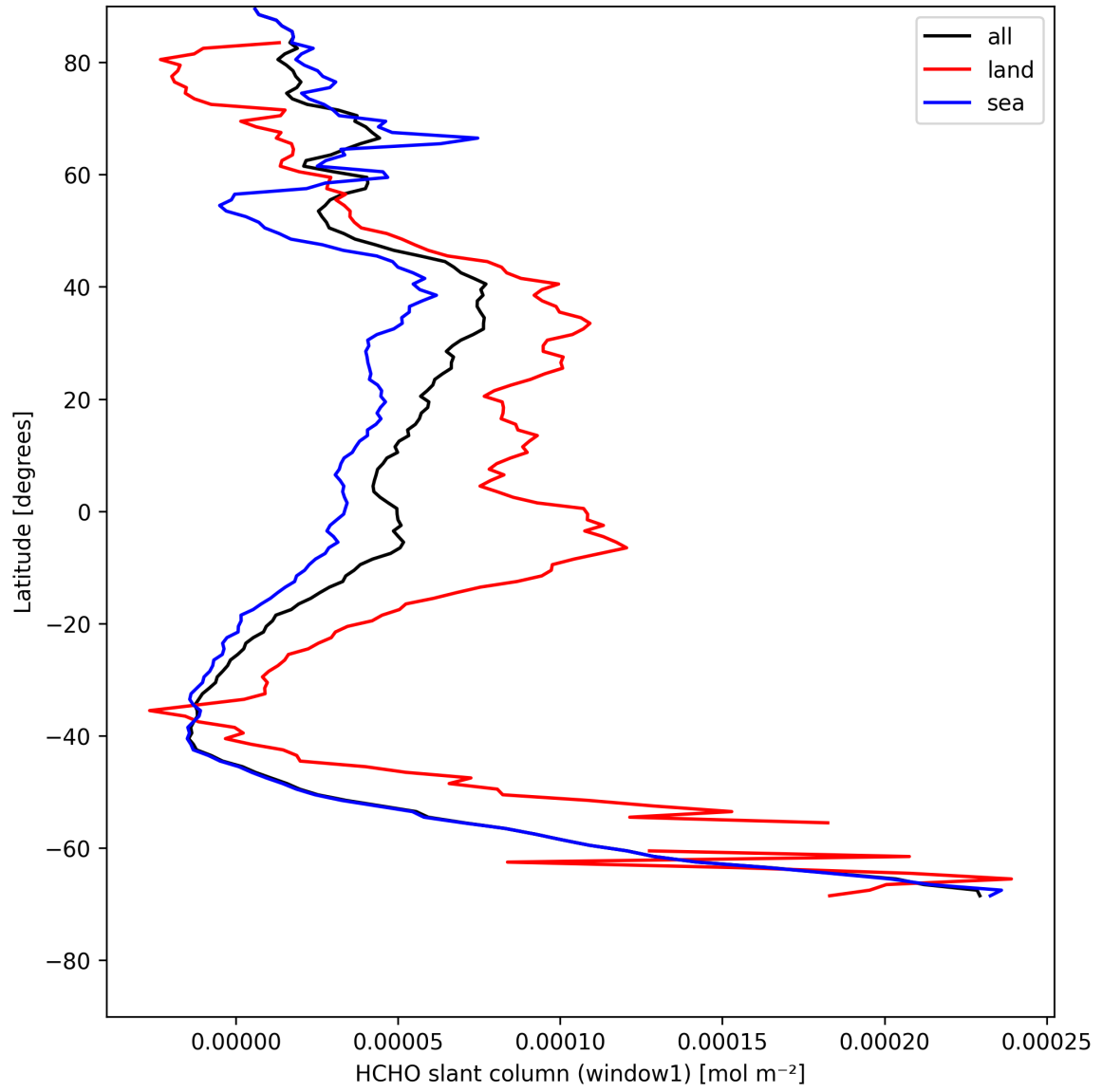
Figure 22: Zonal average of “HCHO slant column (window1)” for 2025-08-06 to 2025-08-07.
