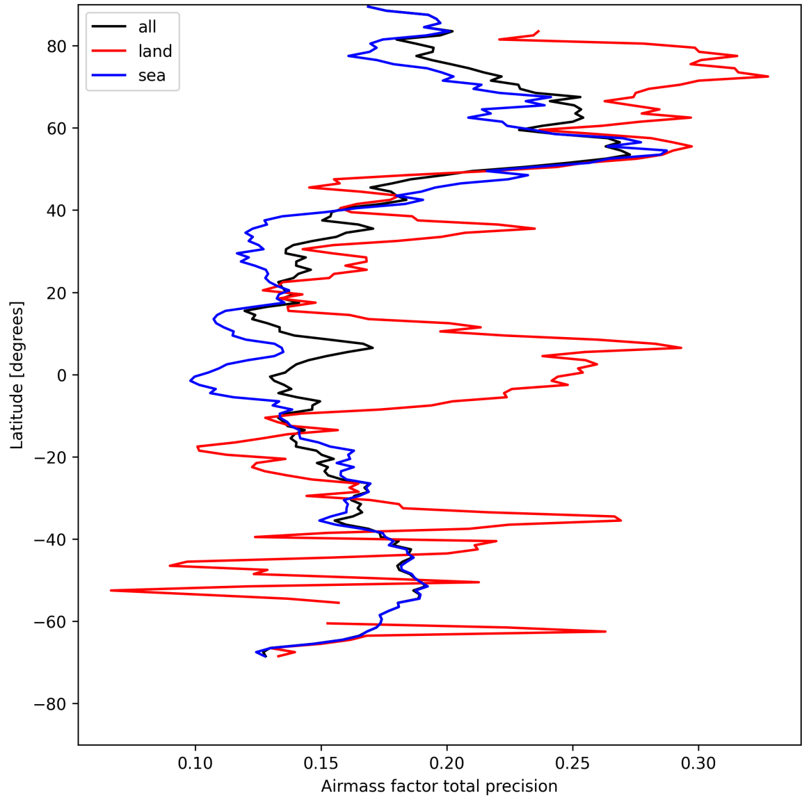
Figure 25: Zonal average of “Airmass factor total precision” for 2025-08-06 to 2025-08-07.
