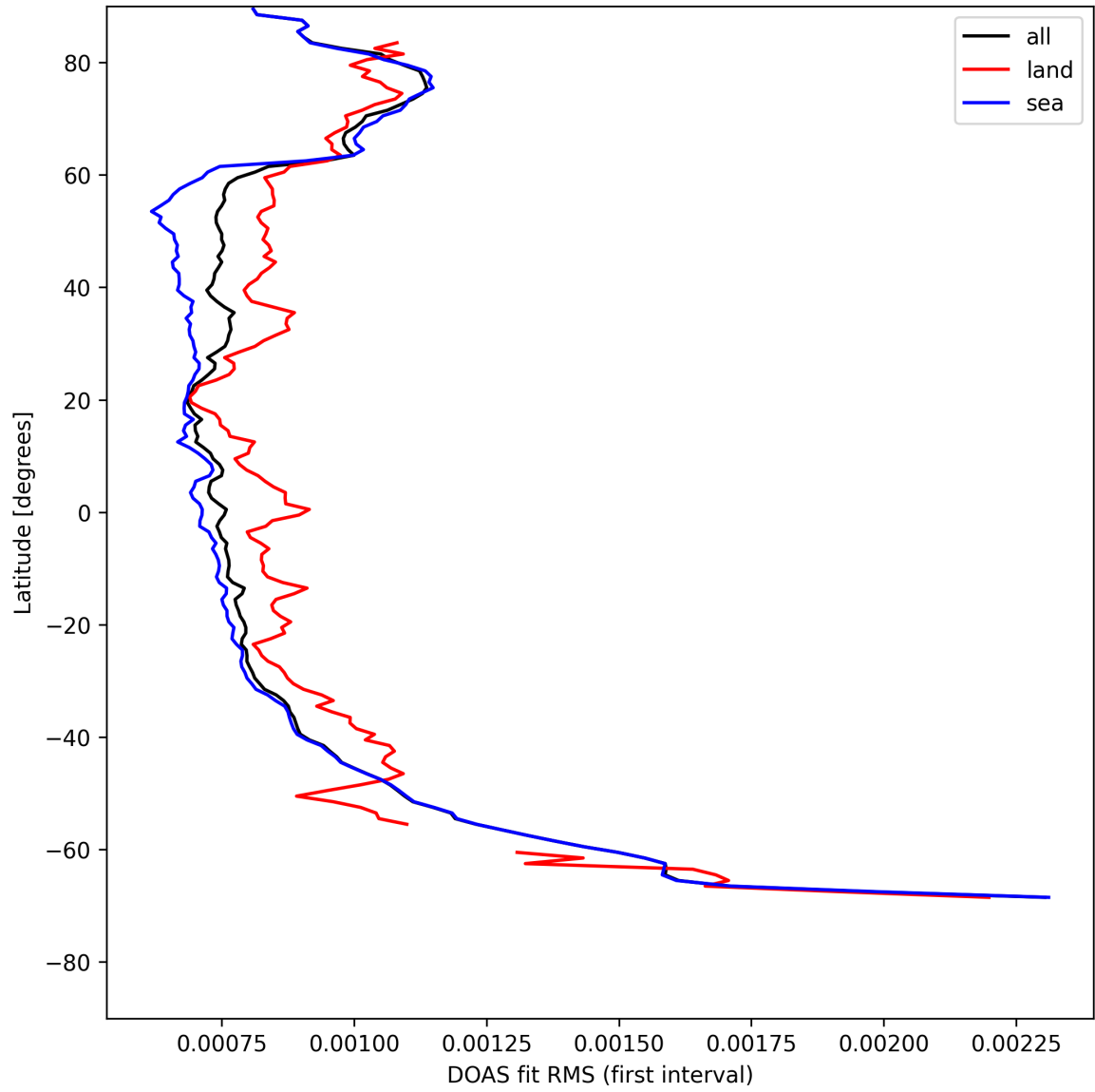
Figure 30: Zonal average of “DOAS fit RMS (first interval)” for 2025-08-06 to 2025-08-07.
