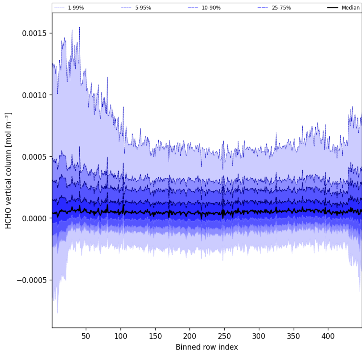
Figure 47: Along track statistics of “HCHO vertical column” for 2025-08-06 to 2025-08-07
