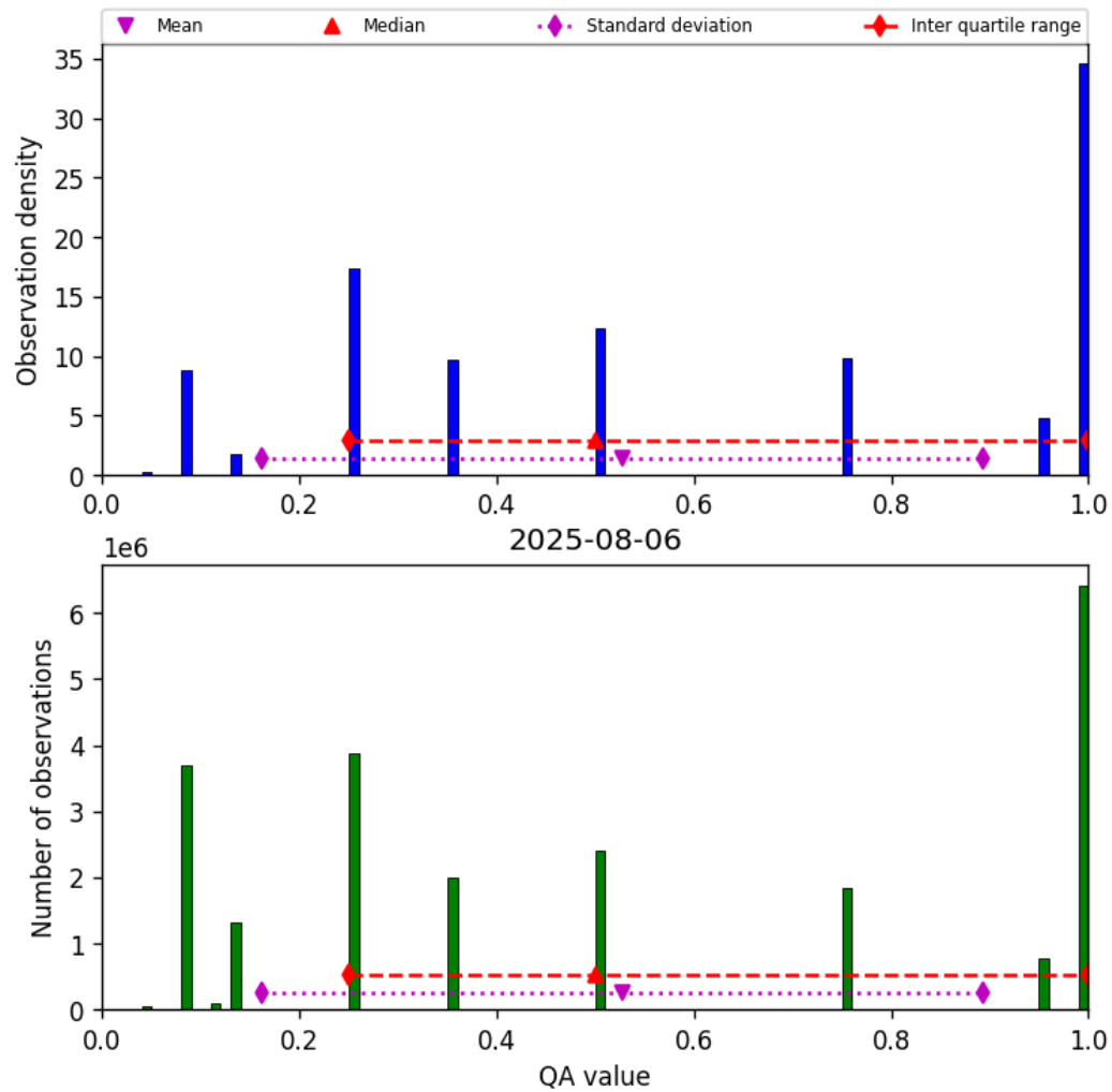
Figure 32: Histogram of “QA value” for 2025-08-06 to 2025-08-07
