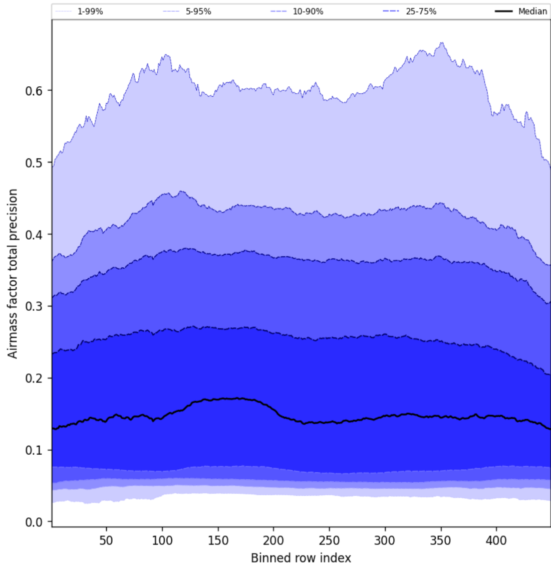
Figure 53: Along track statistics of “Airmass factor total precision” for 2025-08-06 to 2025-08-07
