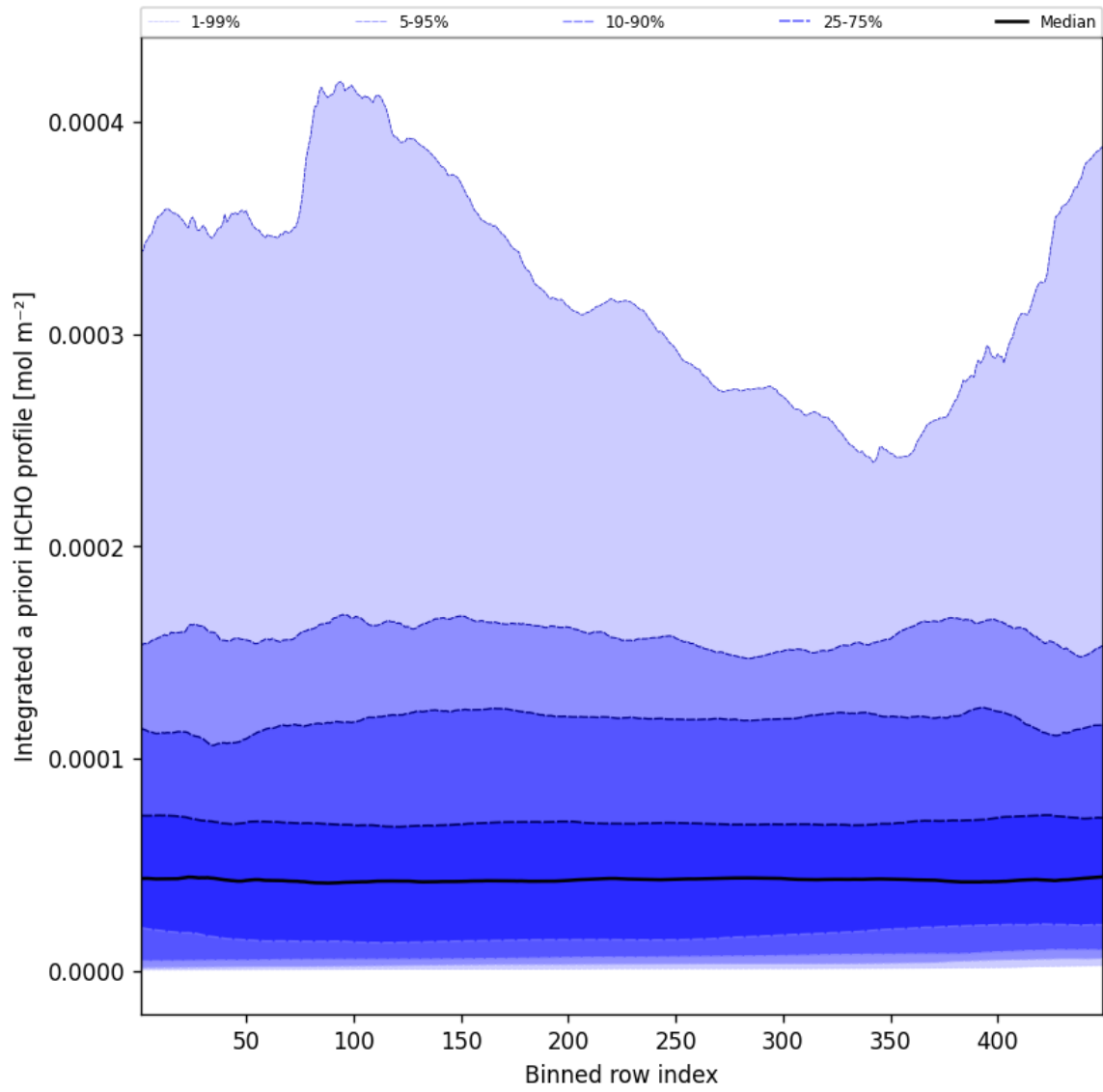
Figure 55: Along track statistics of “Integrated a priori HCHO profile” for 2025-08-06 to 2025-08-07
