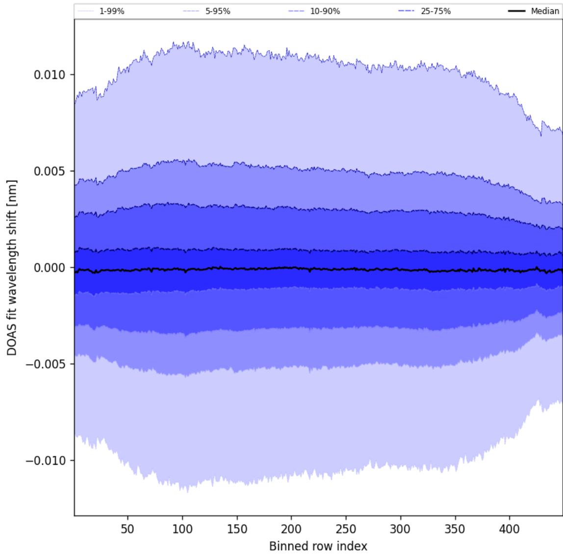
Figure 56: Along track statistics of “DOAS fit wavelength shift” for 2025-08-06 to 2025-08-07
