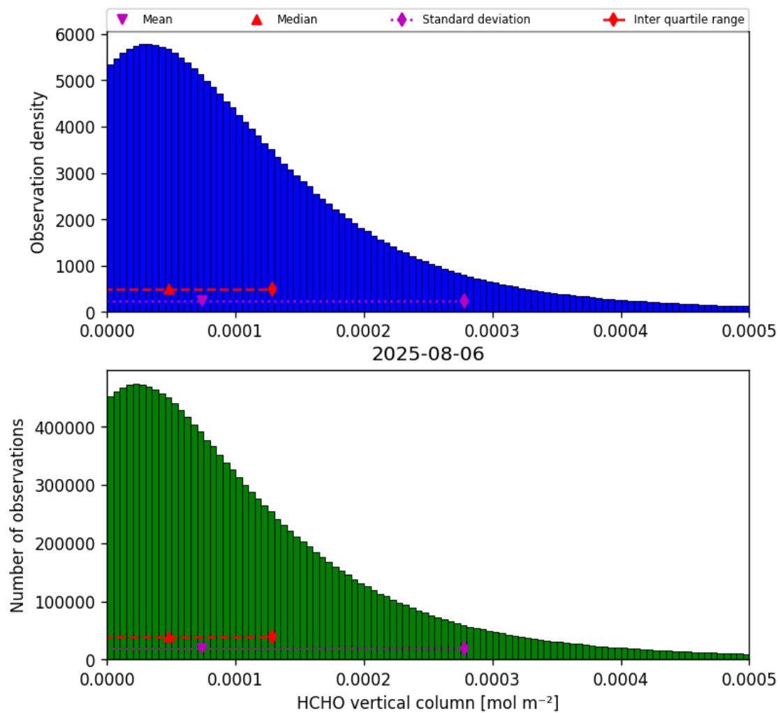
Figure 33: Histogram of “HCHO vertical column” for 2025-08-06 to 2025-08-07
