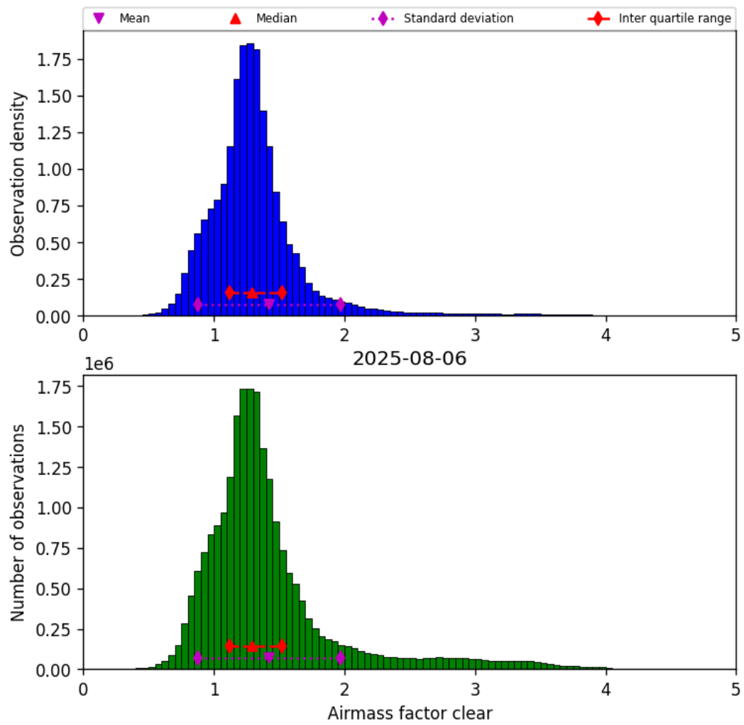
Figure 40: Histogram of “Airmass factor clear” for 2025-08-06 to 2025-08-07
