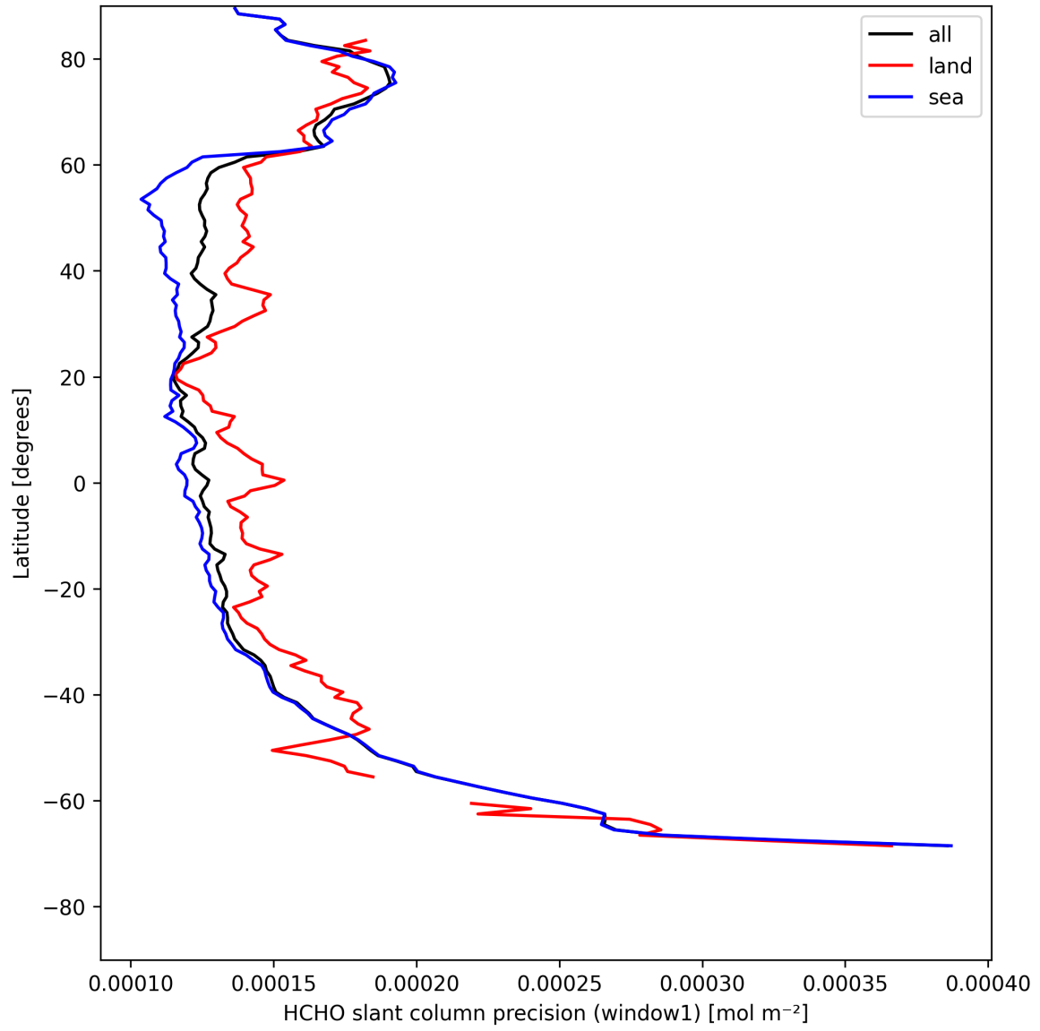
Figure 23: Zonal average of “HCHO slant column precision (window1)” for 2025-08-06 to 2025-08-07.
