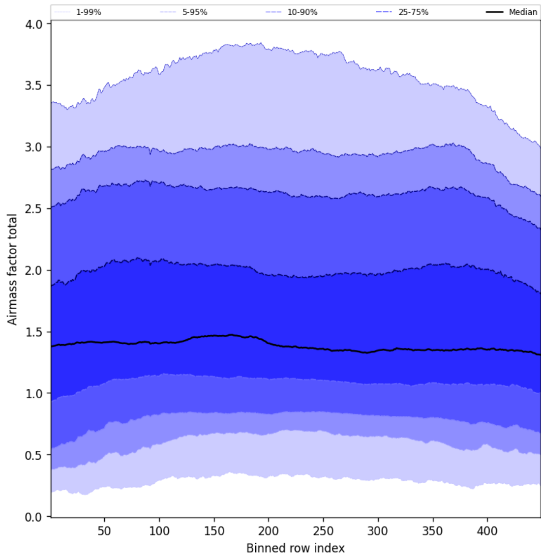
Figure 52: Along track statistics of “Airmass factor total” for 2025-08-06 to 2025-08-07
