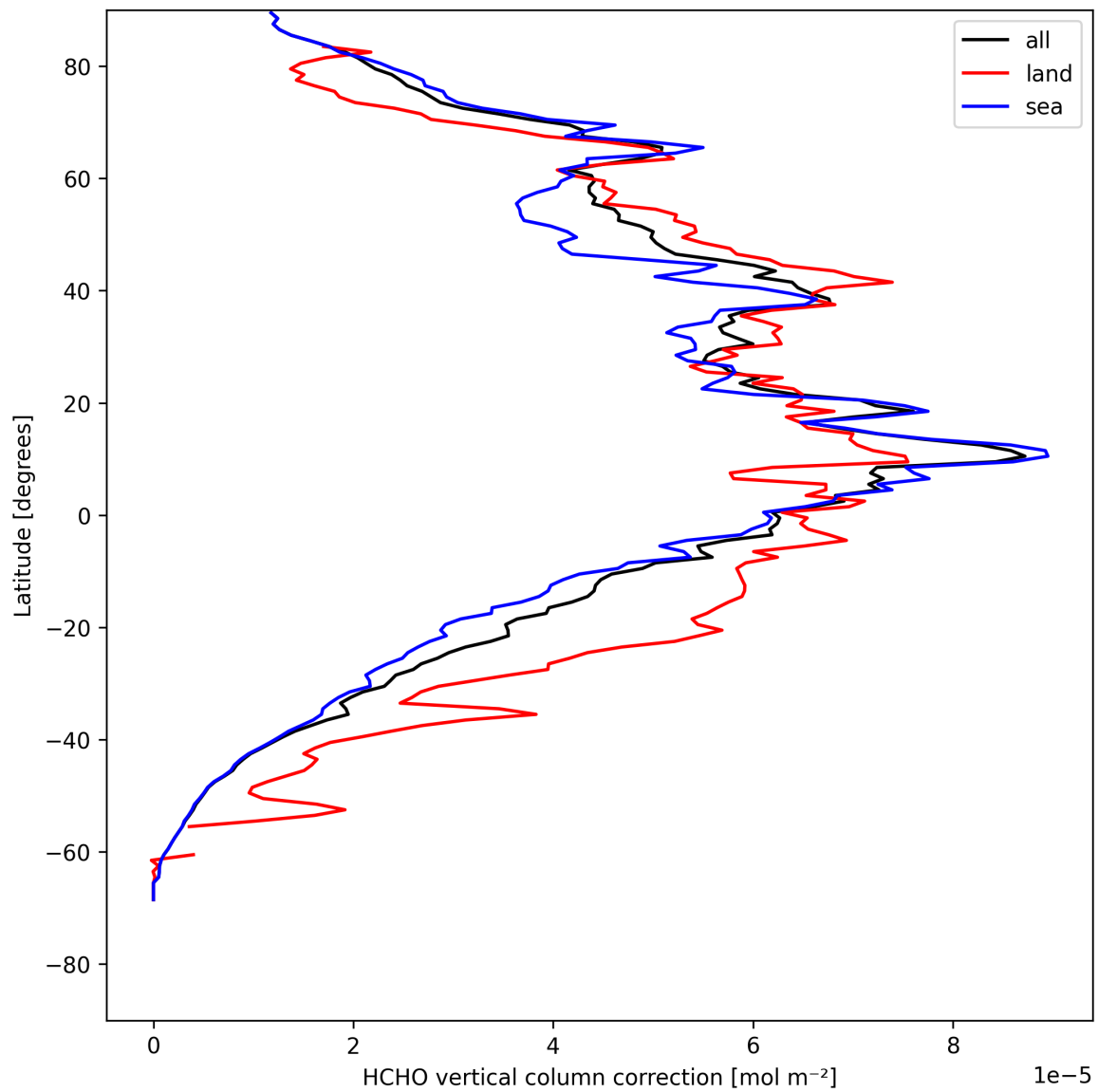
Figure 21: Zonal average of “HCHO vertical column correction” for 2025-08-06 to 2025-08-07.
