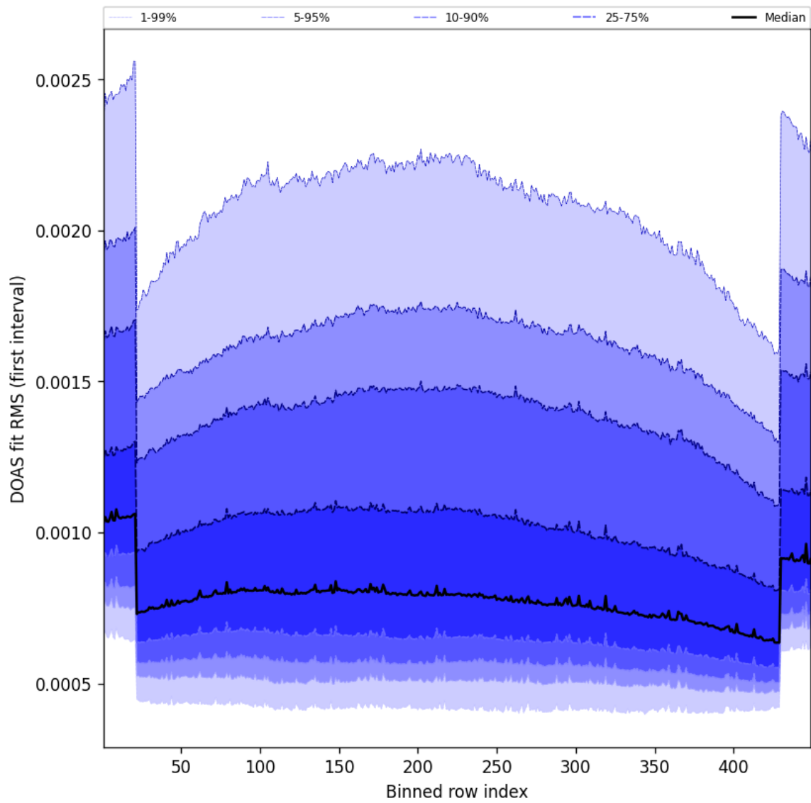
Figure 58: Along track statistics of “DOAS fit RMS (first interval)” for 2025-08-06 to 2025-08-07
