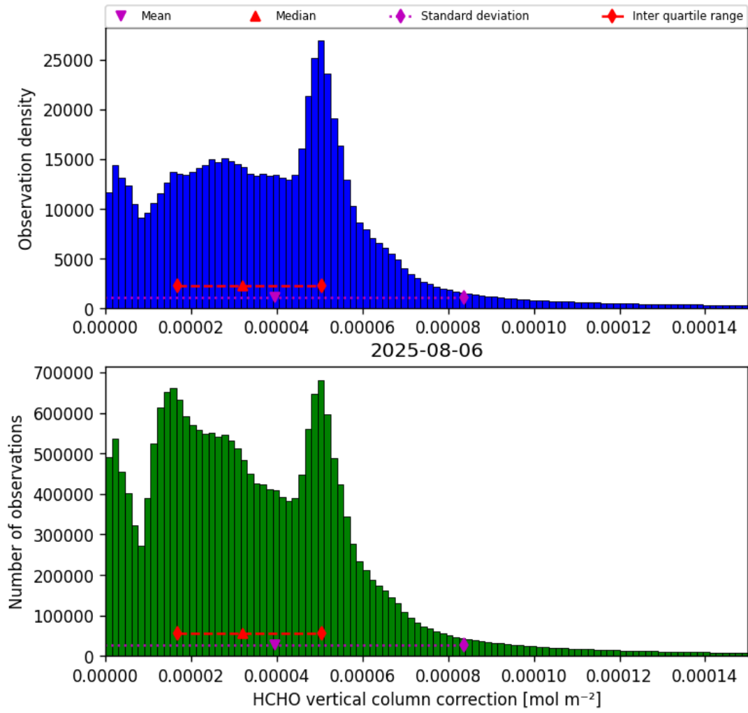
Figure 35: Histogram of “HCHO vertical column correction” for 2025-08-06 to 2025-08-07
