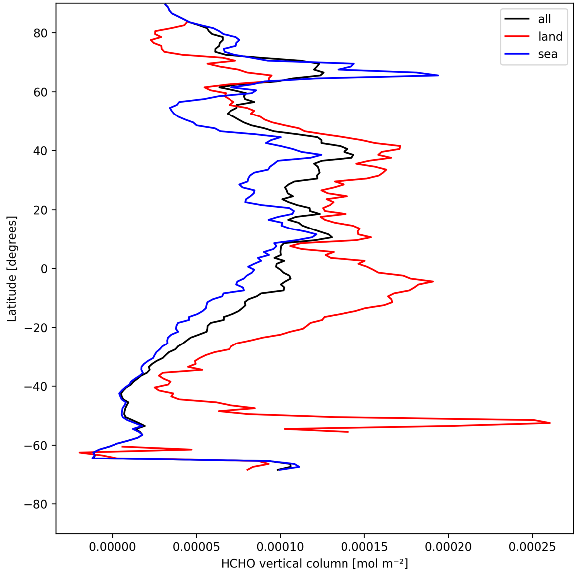
Figure 19: Zonal average of “HCHO vertical column” for 2025-08-06 to 2025-08-07.
