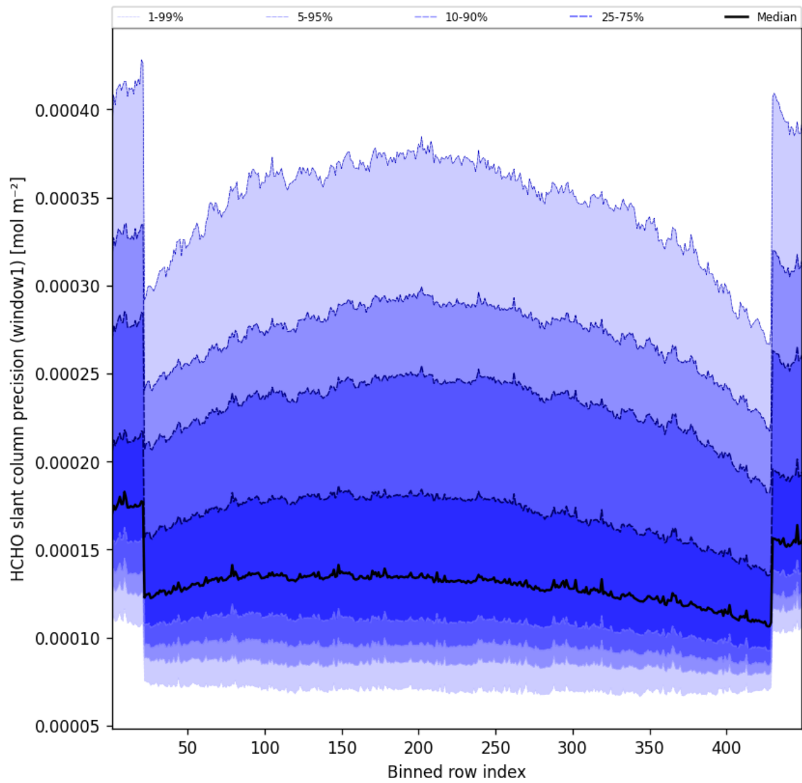
Figure 51: Along track statistics of “HCHO slant column precision (window1)” for 2025-08-06 to 2025-08-07
