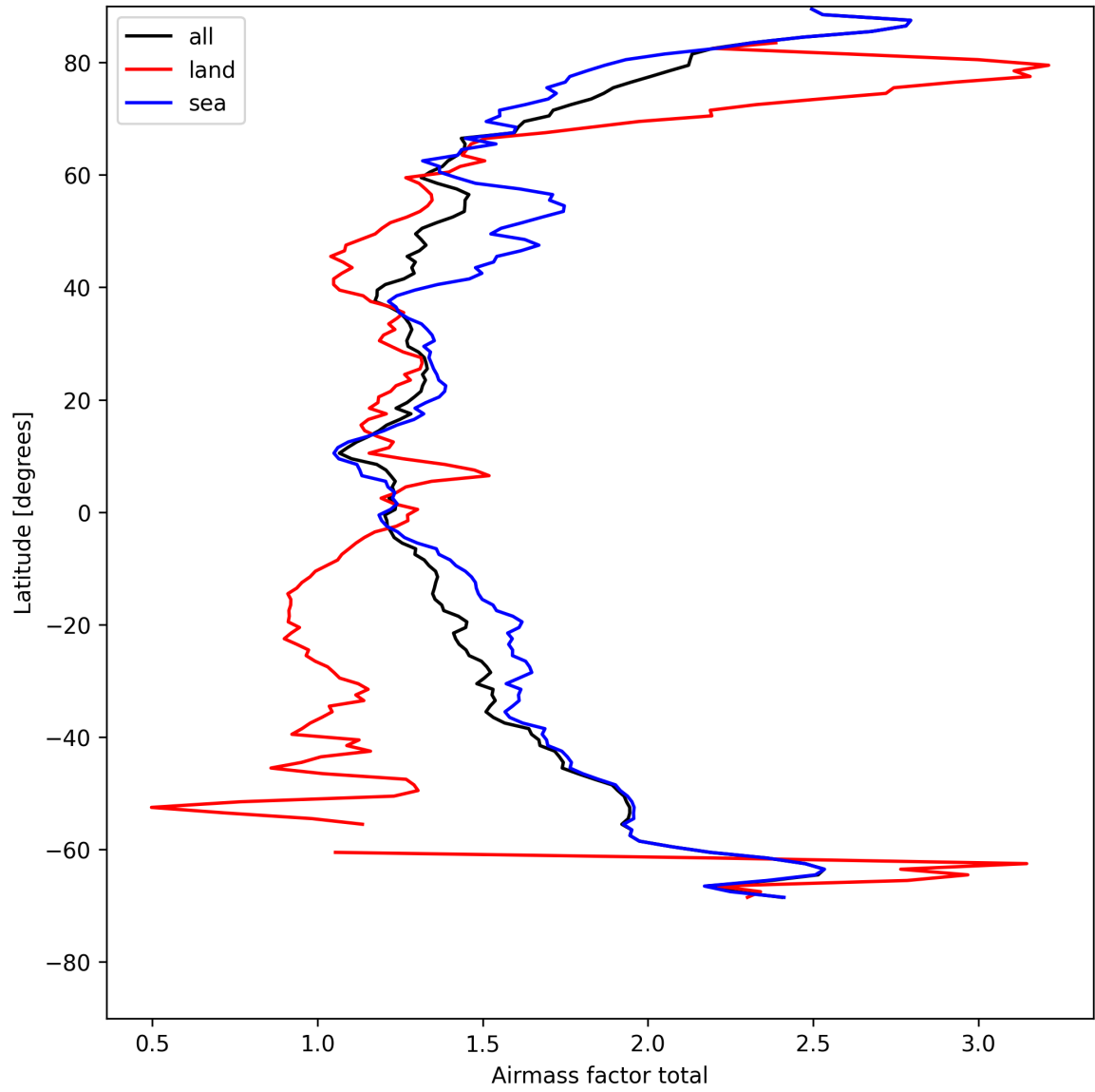
Figure 24: Zonal average of “Airmass factor total” for 2025-08-06 to 2025-08-07.
