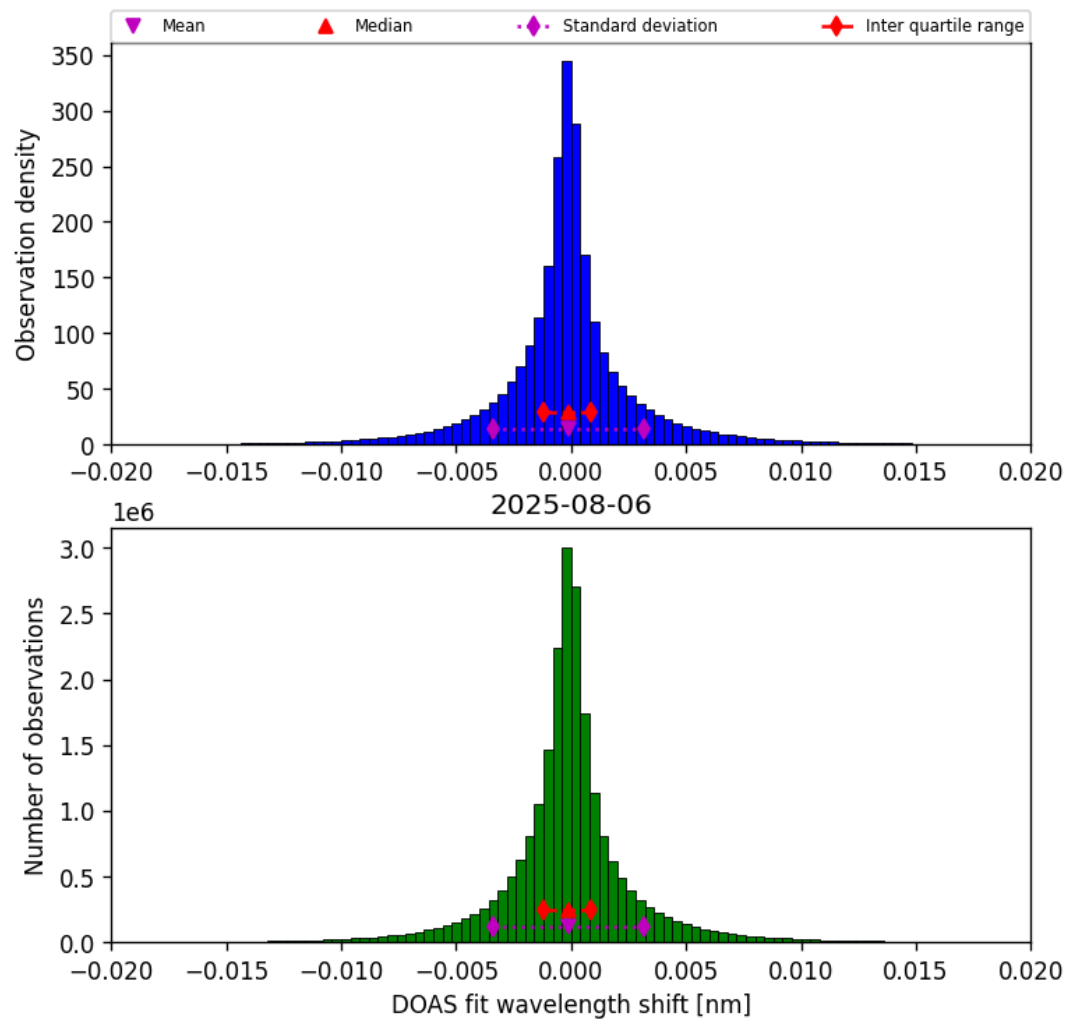
Figure 42: Histogram of “DOAS fit wavelength shift” for 2025-08-06 to 2025-08-07
