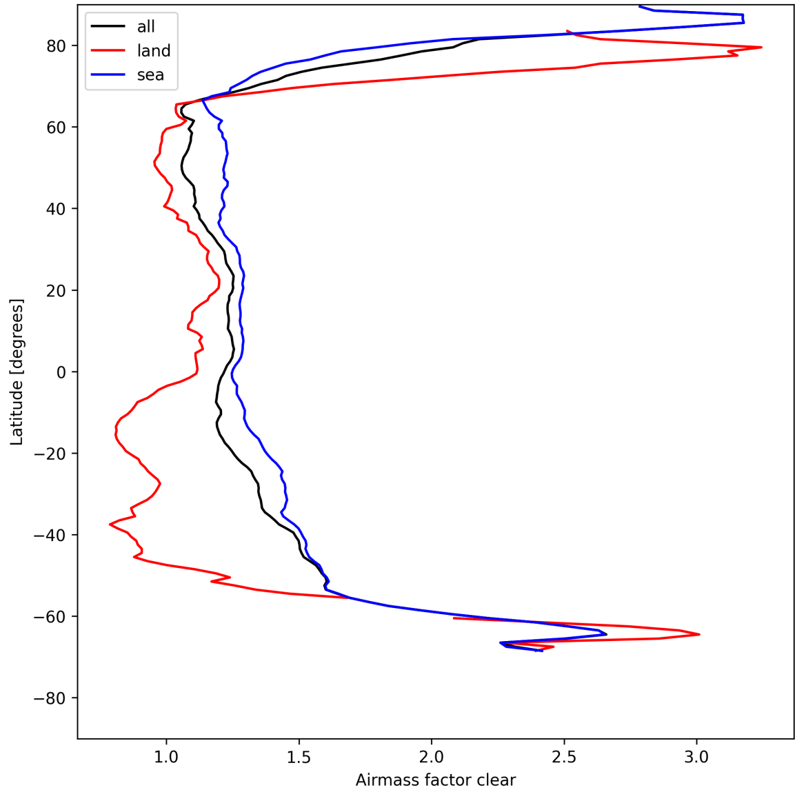
Figure 26: Zonal average of “Airmass factor clear” for 2025-08-06 to 2025-08-07.
