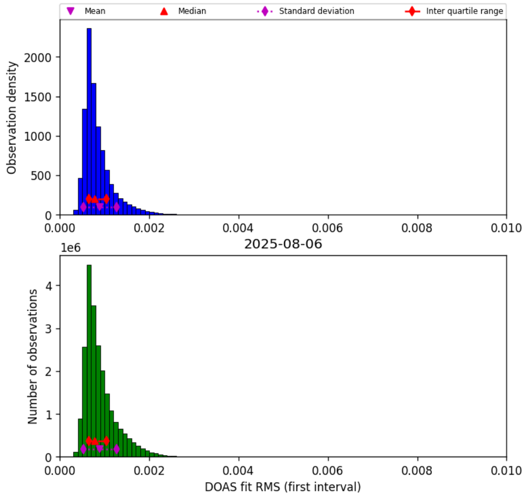
Figure 44: Histogram of “DOAS fit RMS (first interval)” for 2025-08-06 to 2025-08-07
