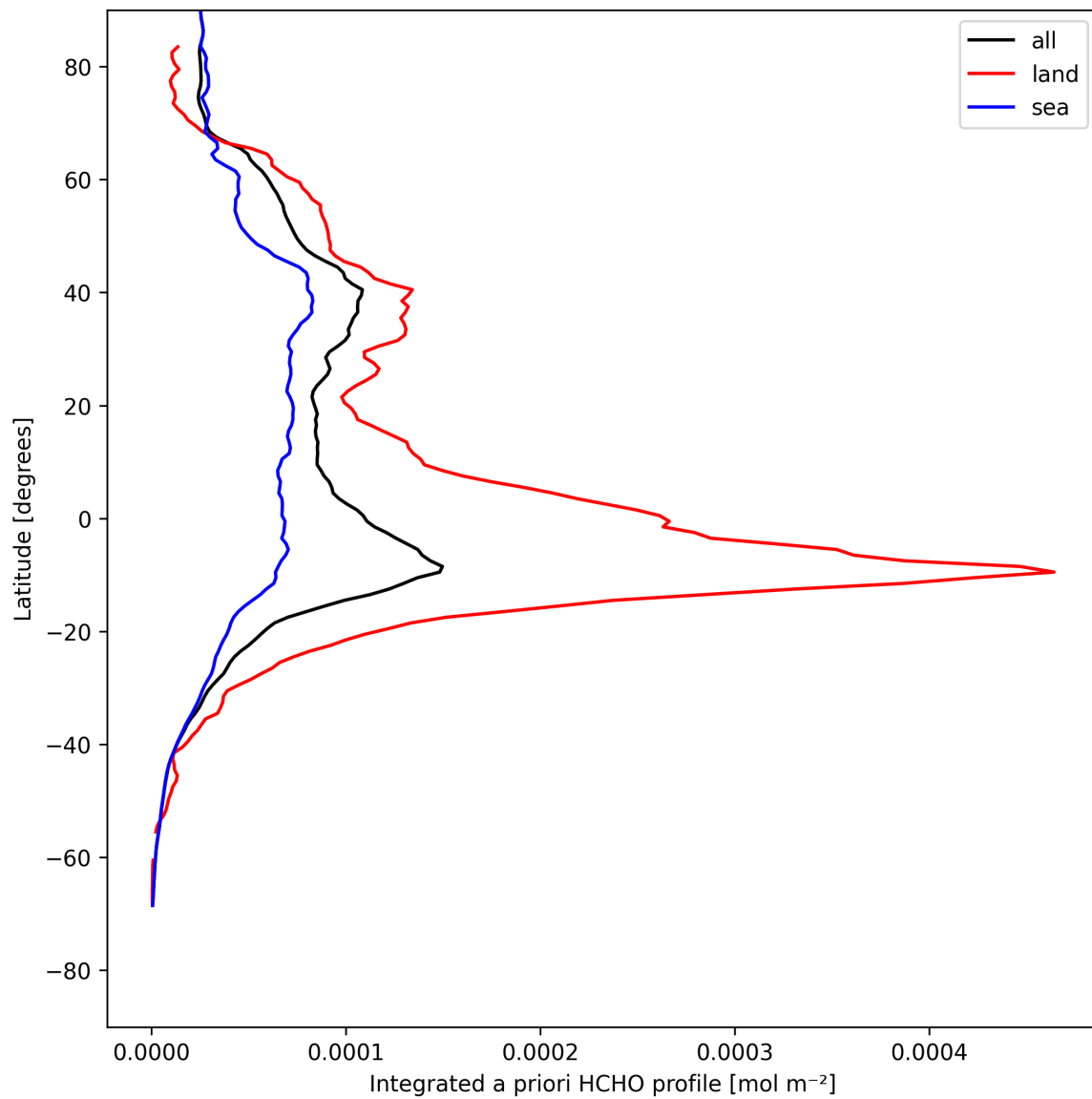
Figure 27: Zonal average of “Integrated a priori HCHO profile” for 2025-08-06 to 2025-08-07.
