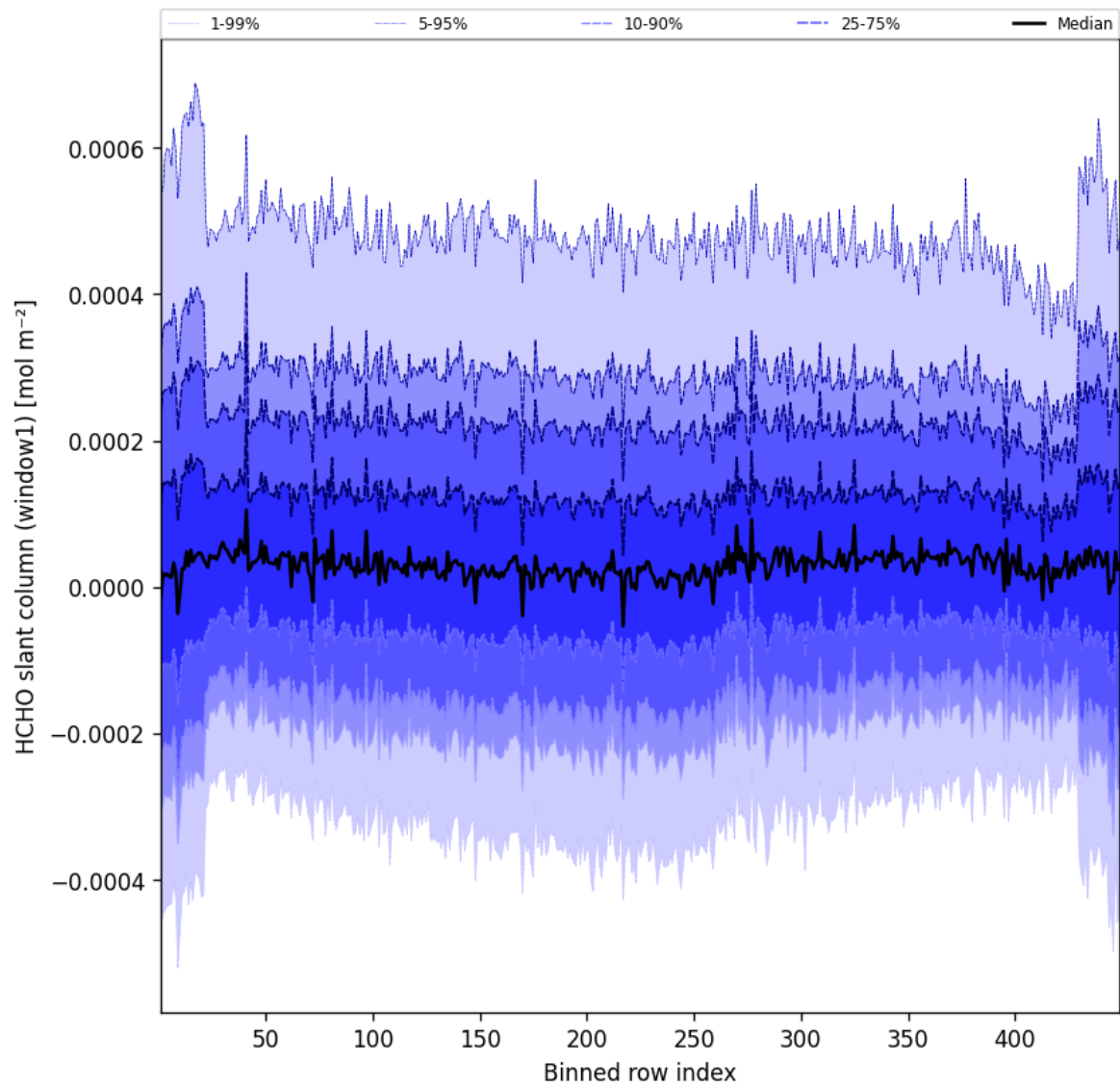
Figure 50: Along track statistics of “HCHO slant column (window1)” for 2025-08-06 to 2025-08-07
