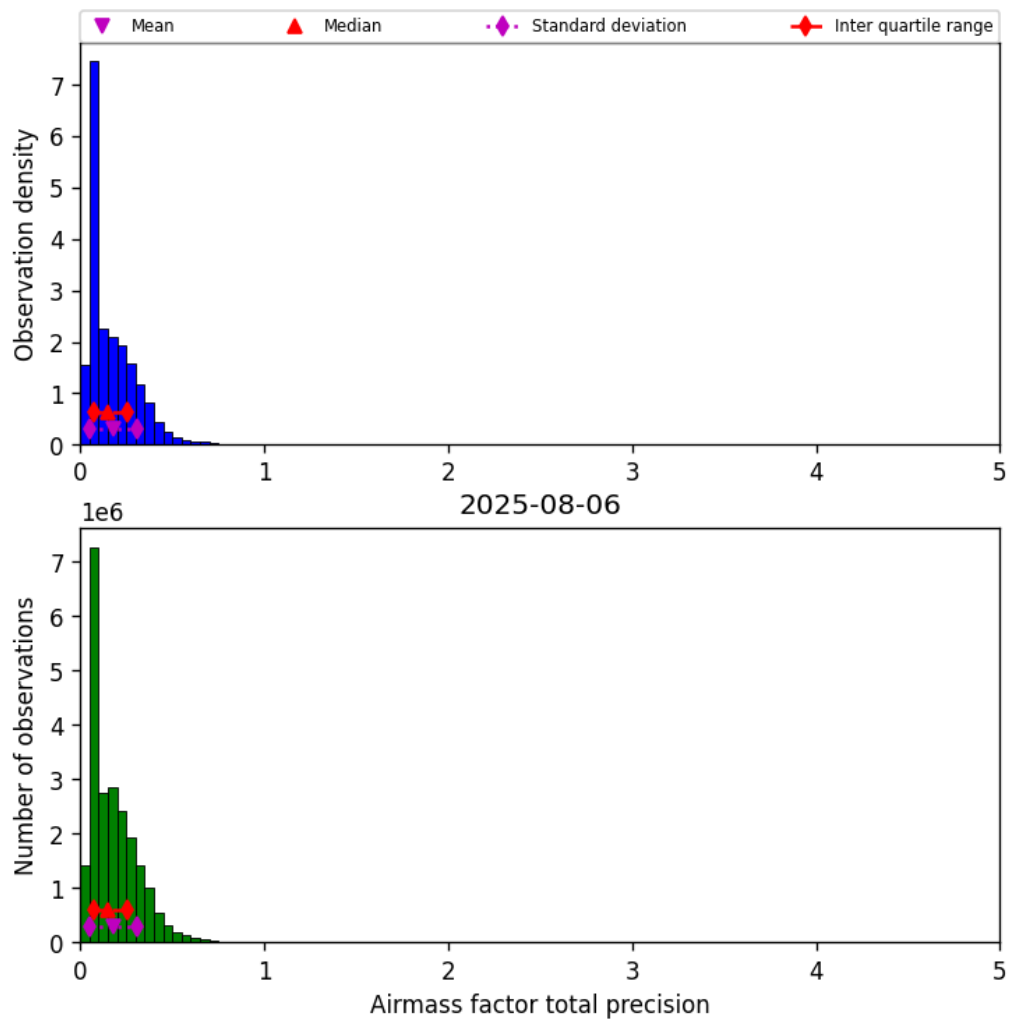
Figure 39: Histogram of “Airmass factor total precision” for 2025-08-06 to 2025-08-07
