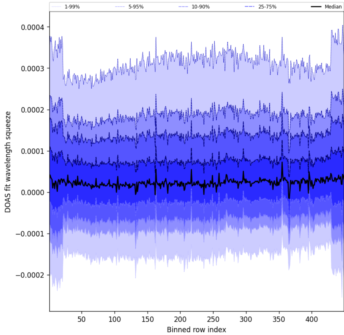
Figure 57: Along track statistics of “DOAS fit wavelength squeeze” for 2025-08-06 to 2025-08-07
