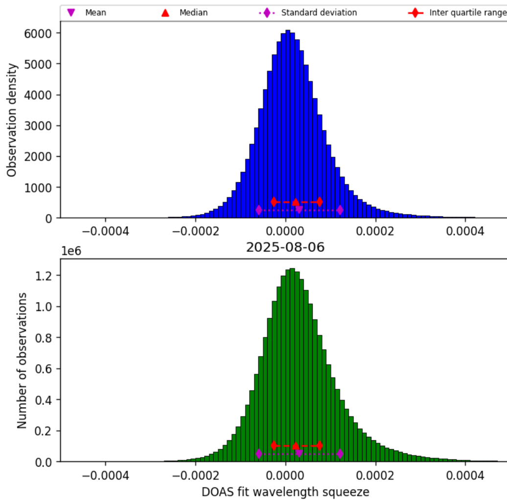
Figure 43: Histogram of “DOAS fit wavelength squeeze” for 2025-08-06 to 2025-08-07
