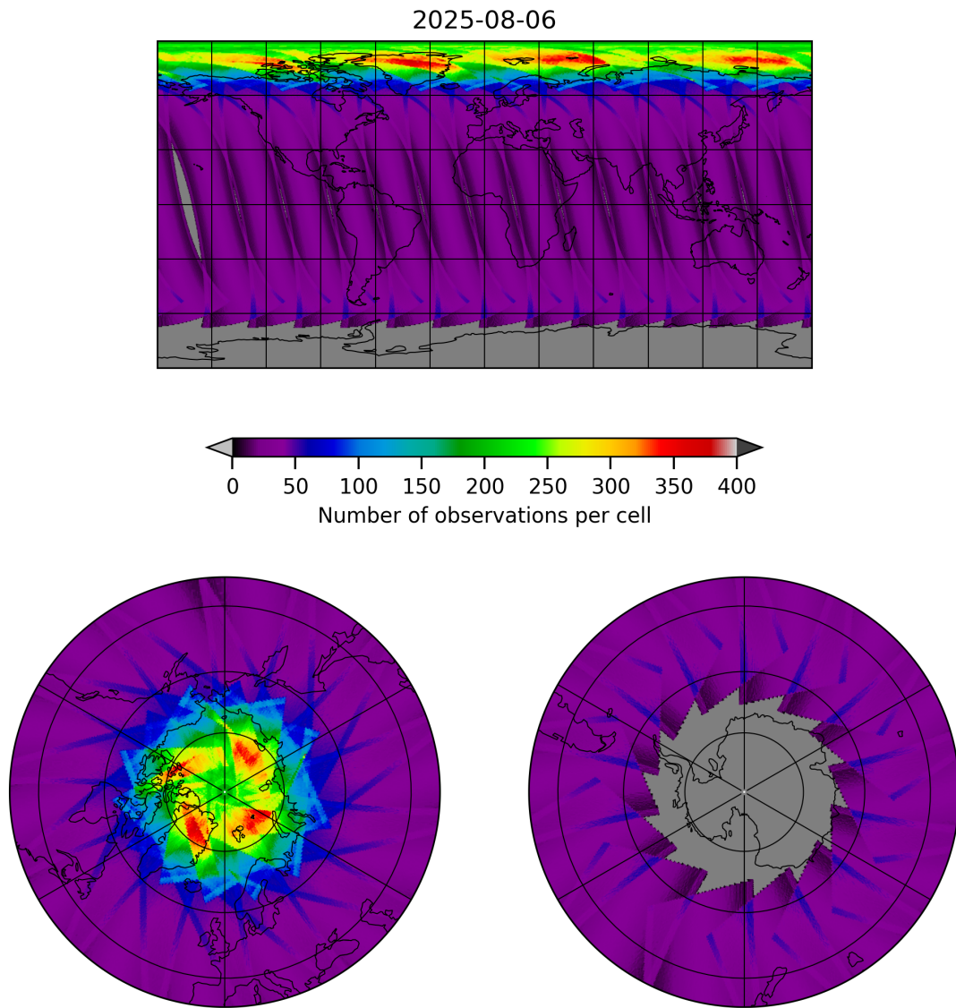
Figure 17: Map of the number of observations for 2025-08-06 to 2025-08-07
