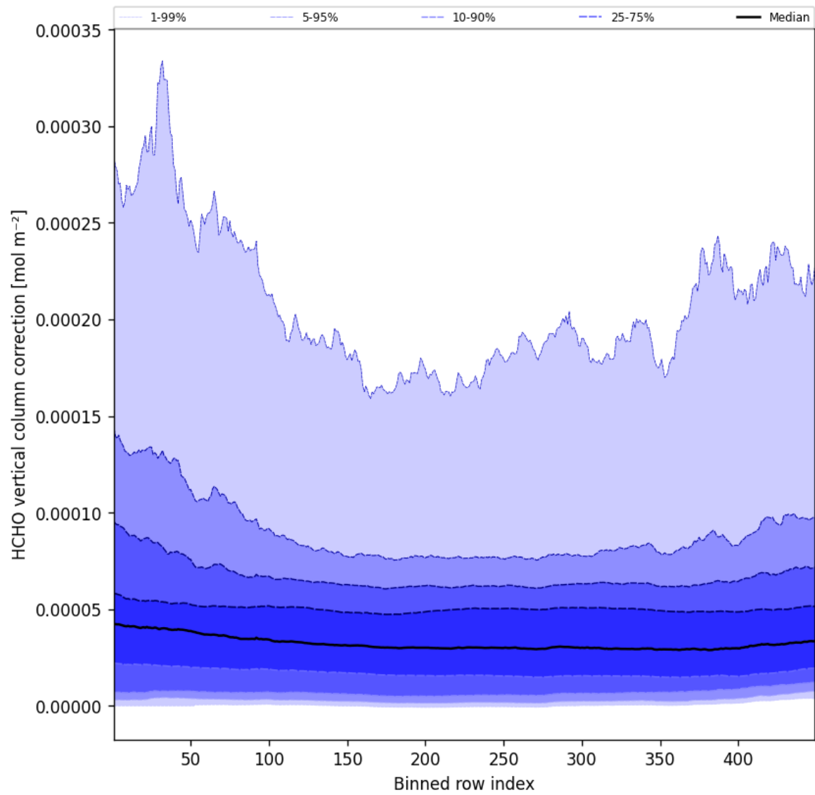
Figure 49: Along track statistics of “HCHO vertical column correction” for 2025-08-06 to 2025-08-07
