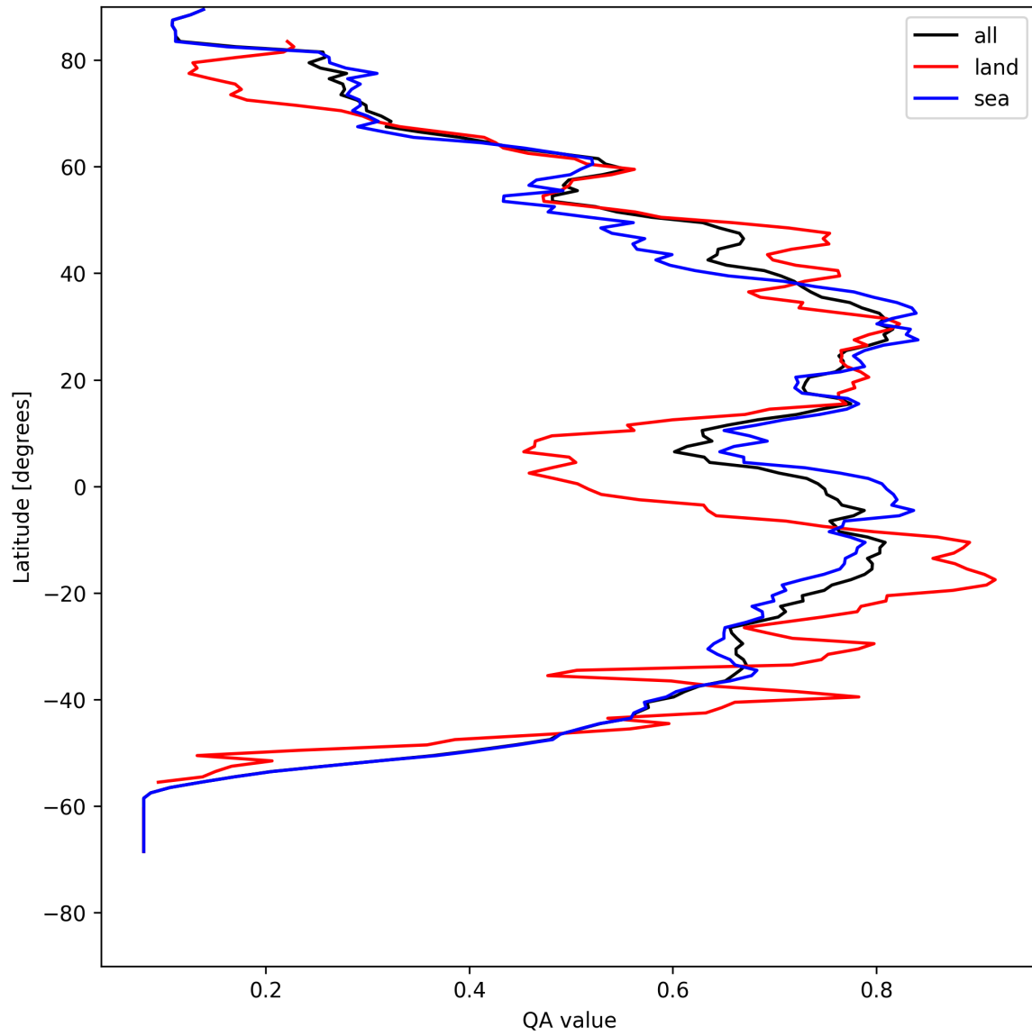
Figure 18: Zonal average of “QA value” for 2025-08-06 to 2025-08-07.
