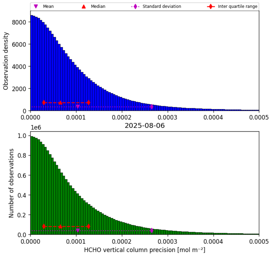
Figure 34: Histogram of “HCHO vertical column precision” for 2025-08-06 to 2025-08-07
