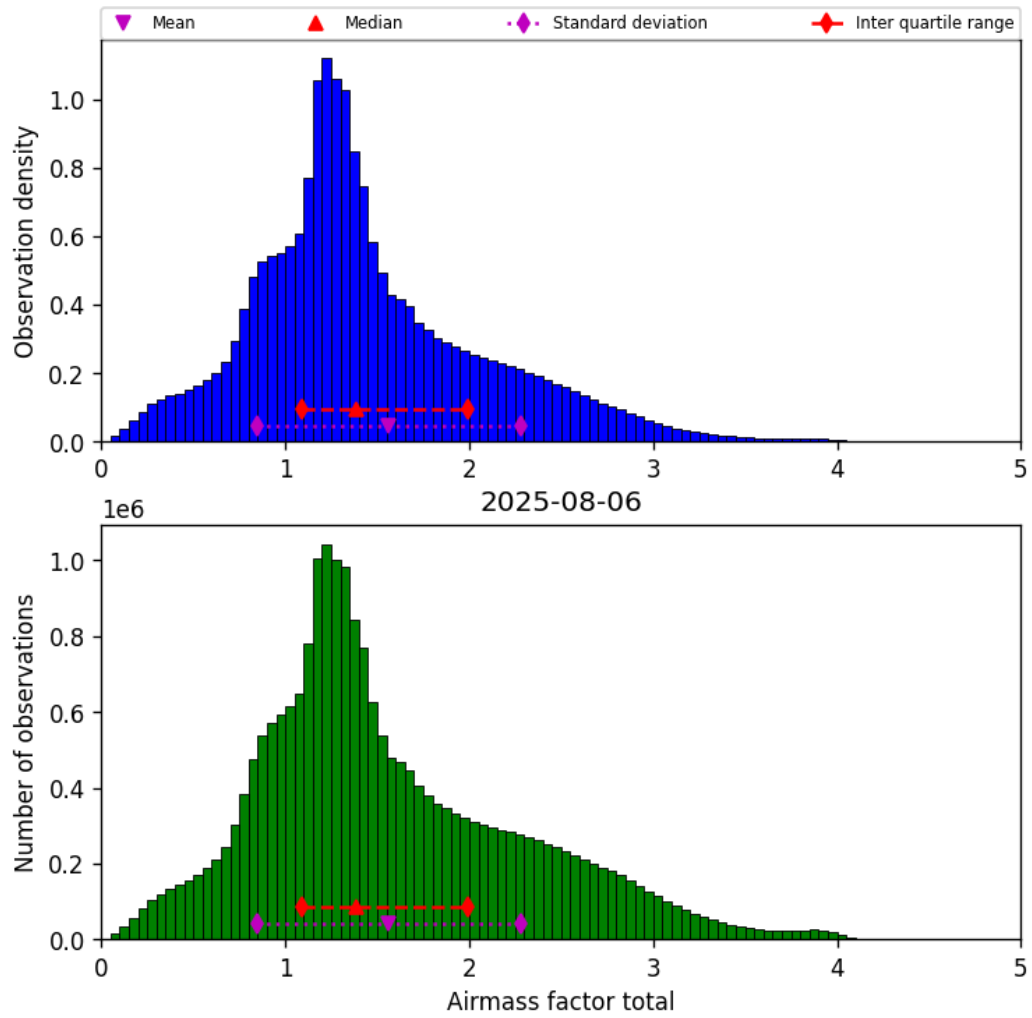
Figure 38: Histogram of “Airmass factor total” for 2025-08-06 to 2025-08-07
