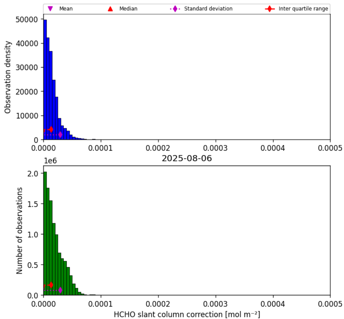
Figure 45: Histogram of “HCHO slant column correction” for 2025-08-06 to 2025-08-07
