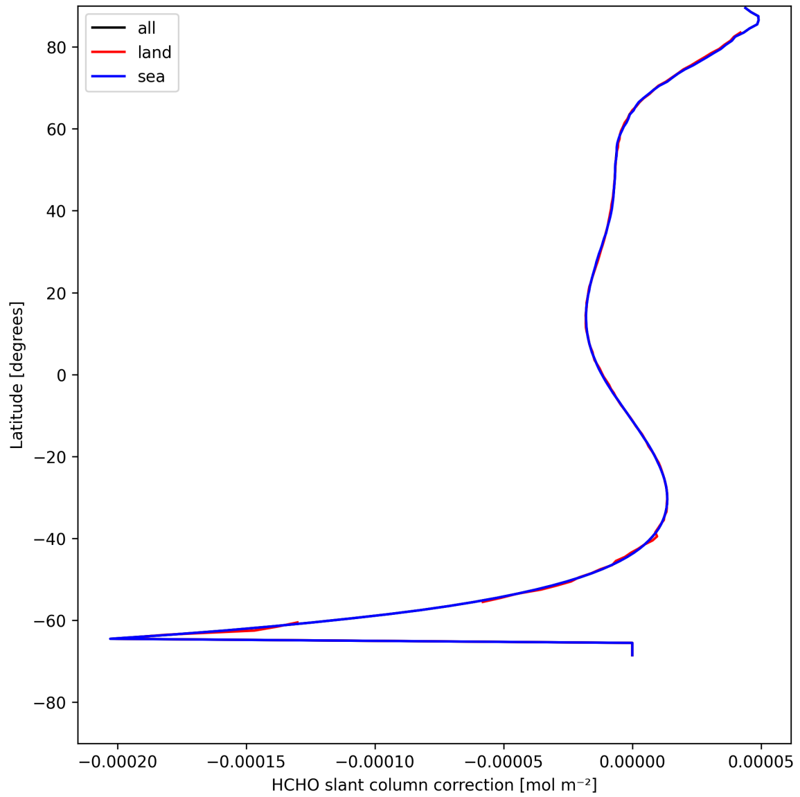
Figure 31: Zonal average of “HCHO slant column correction” for 2025-08-06 to 2025-08-07.
