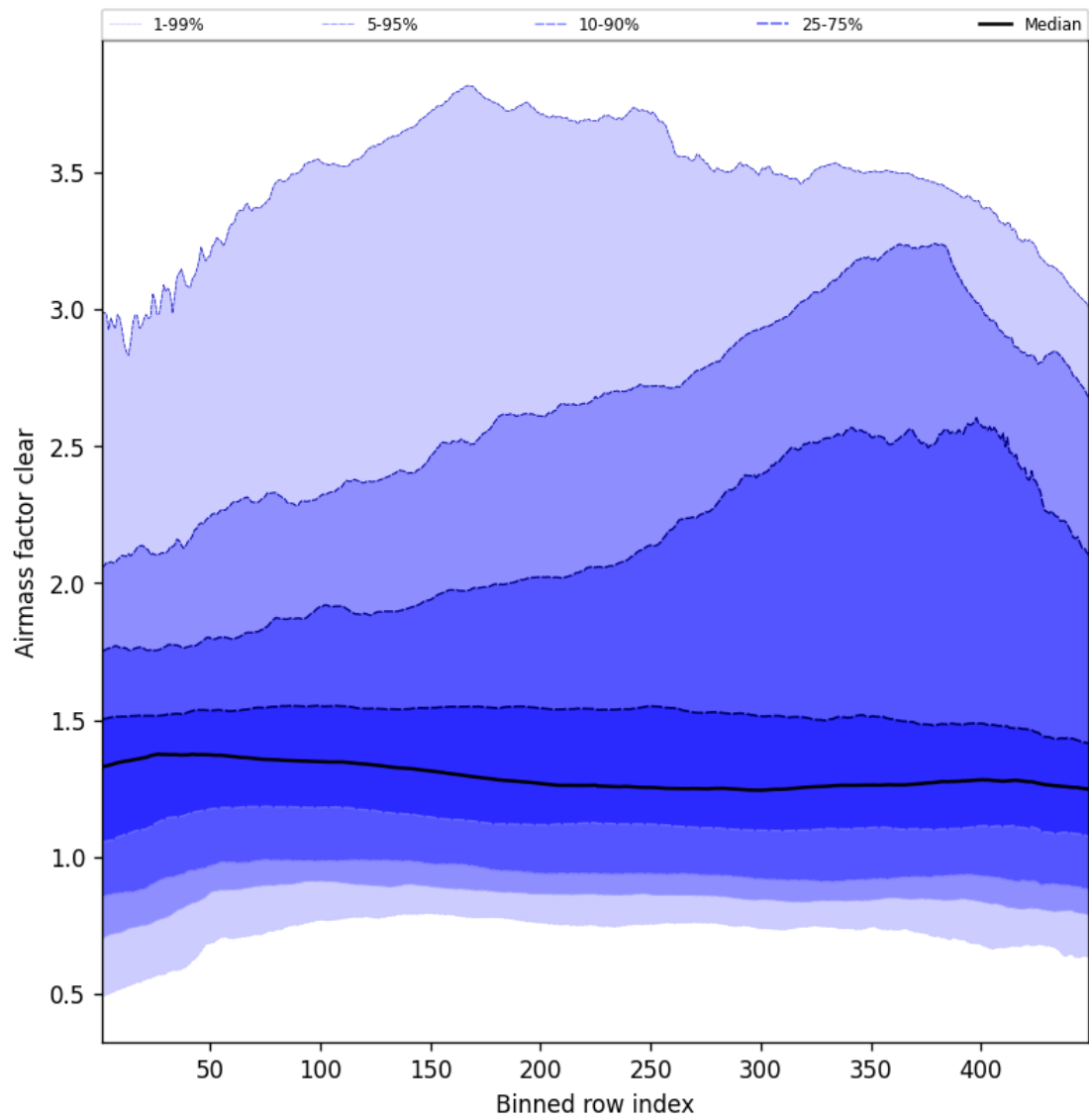
Figure 54: Along track statistics of “Airmass factor clear” for 2025-08-06 to 2025-08-07
