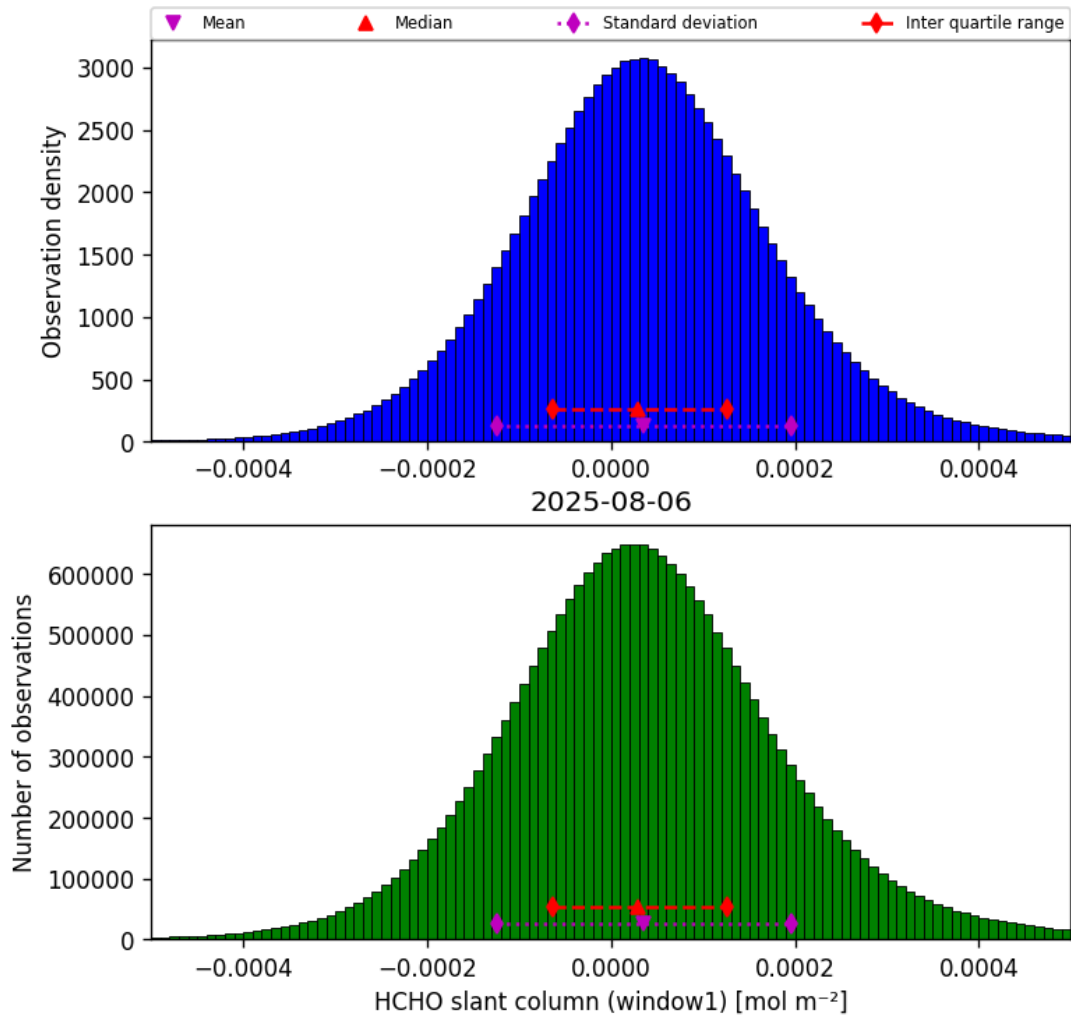
Figure 36: Histogram of “HCHO slant column (window1)” for 2025-08-06 to 2025-08-07
