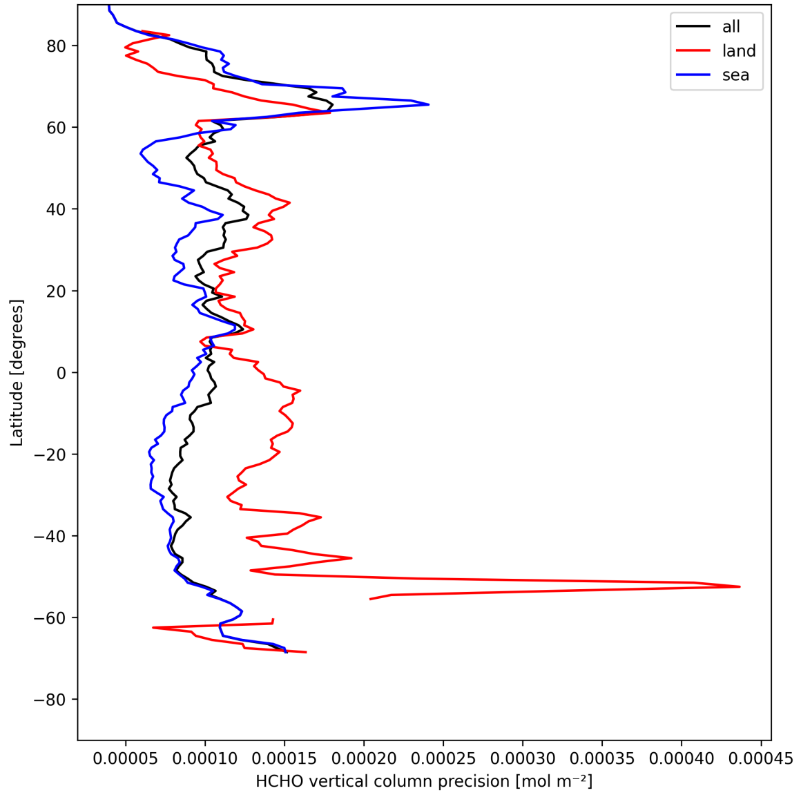
Figure 20: Zonal average of "HCHO vertical column precision" for 2025-08-06 to 2025-08-07.
