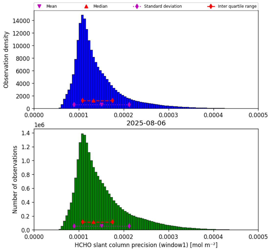
Figure 37: Histogram of “HCHO slant column precision (window1)” for 2025-08-06 to 2025-08-07
