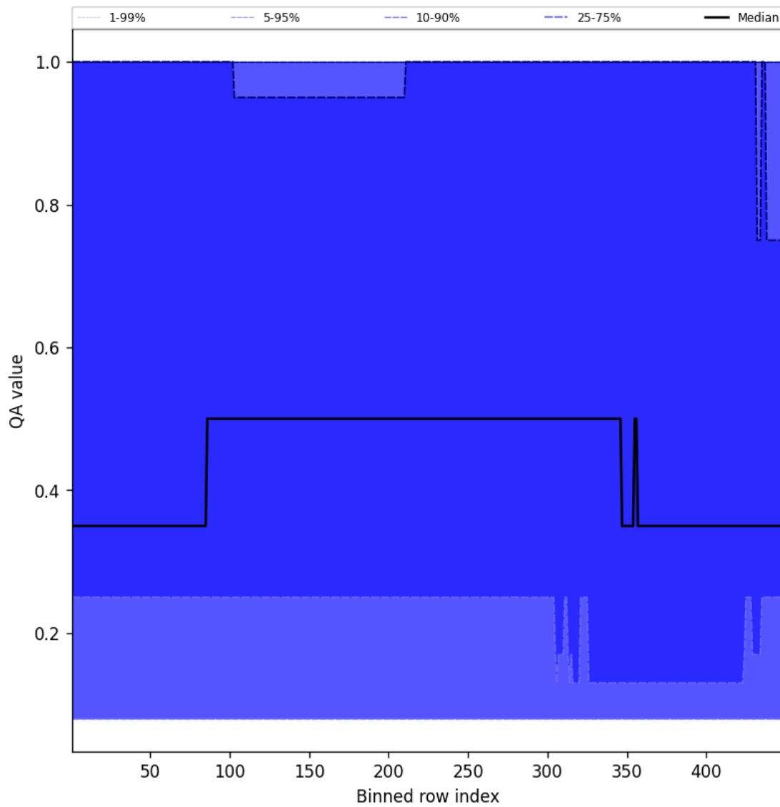
Figure 46: Along track statistics of “QA value” for 2025-08-06 to 2025-08-07
