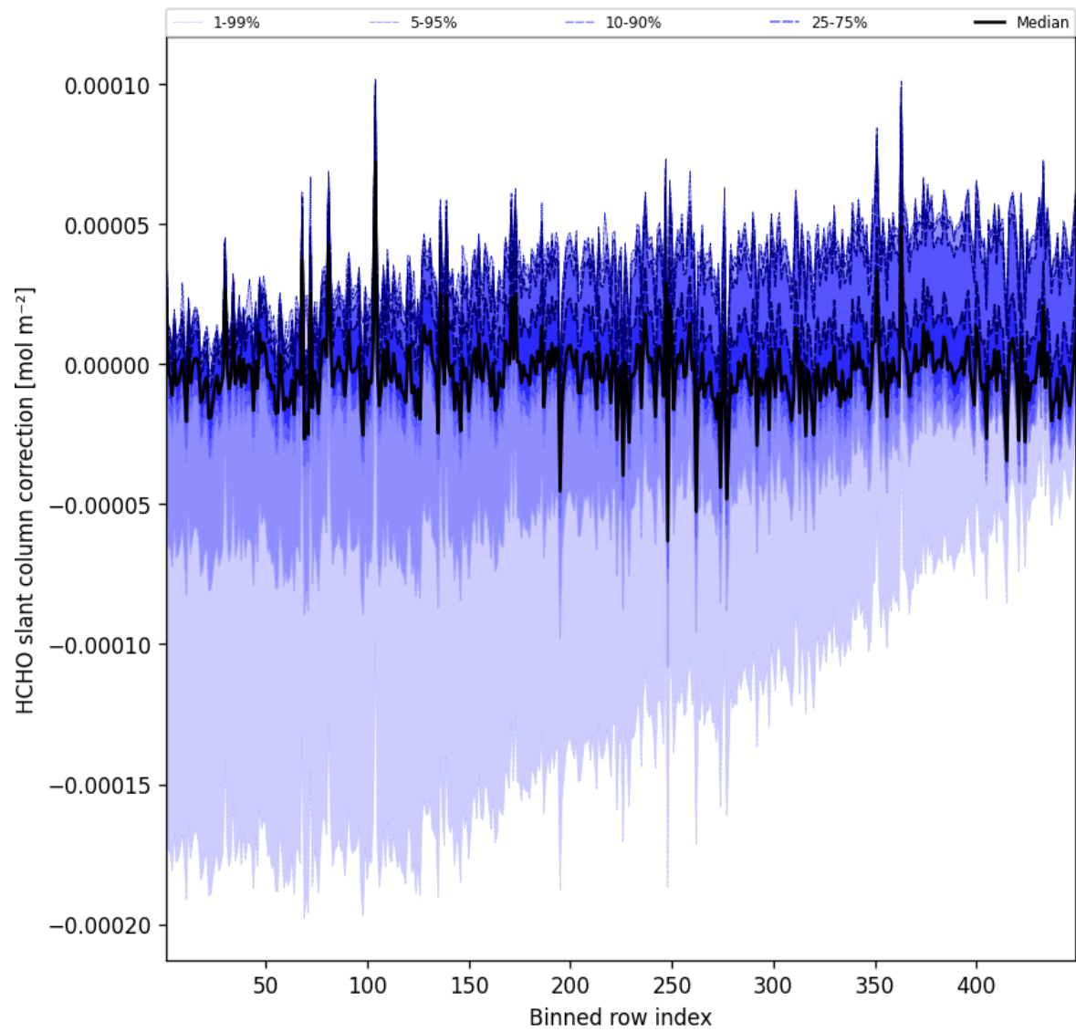
Figure 59: Along track statistics of “HCHO slant column correction” for 2025-08-06 to 2025-08-07
