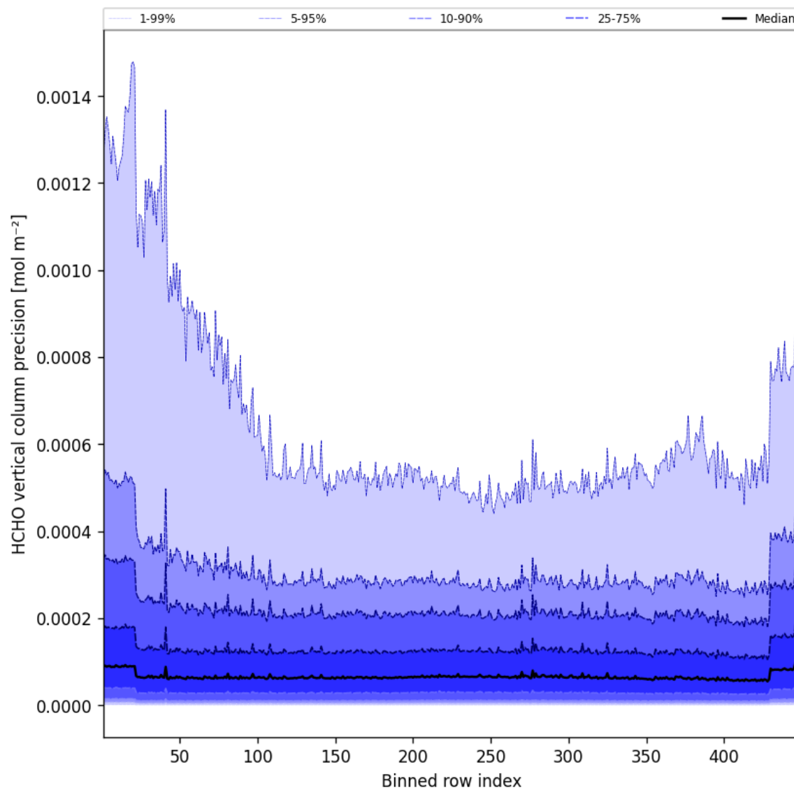
Figure 48: Along track statistics of “HCHO vertical column precision” for 2025-08-06 to 2025-08-07
