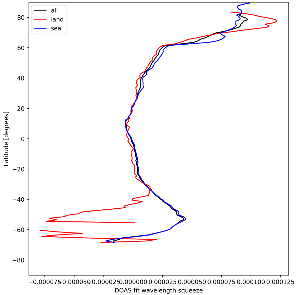
Figure 29: Zonal average of “DOAS fit wavelength squeeze” for 2025-08-06 to 2025-08-07.
