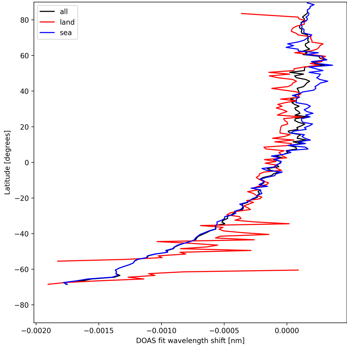
Figure 28: Zonal average of "DOAS fit wavelength shift" for 2025-08-06 to 2025-08-07.
