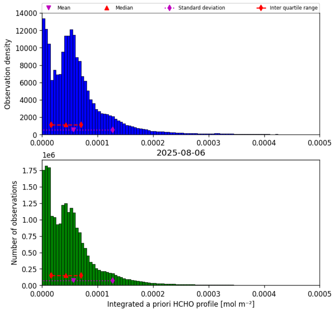
Figure 41: Histogram of “Integrated a priori HCHO profile” for 2025-08-06 to 2025-08-07
