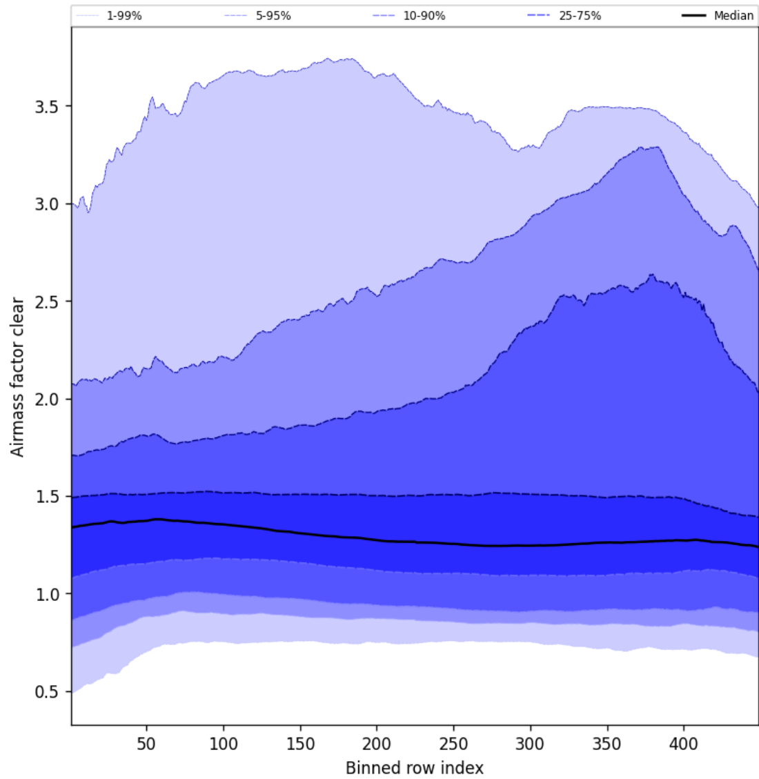
Figure 54: Along track statistics of “Airmass factor clear” for 2025-08-07 to 2025-08-07
