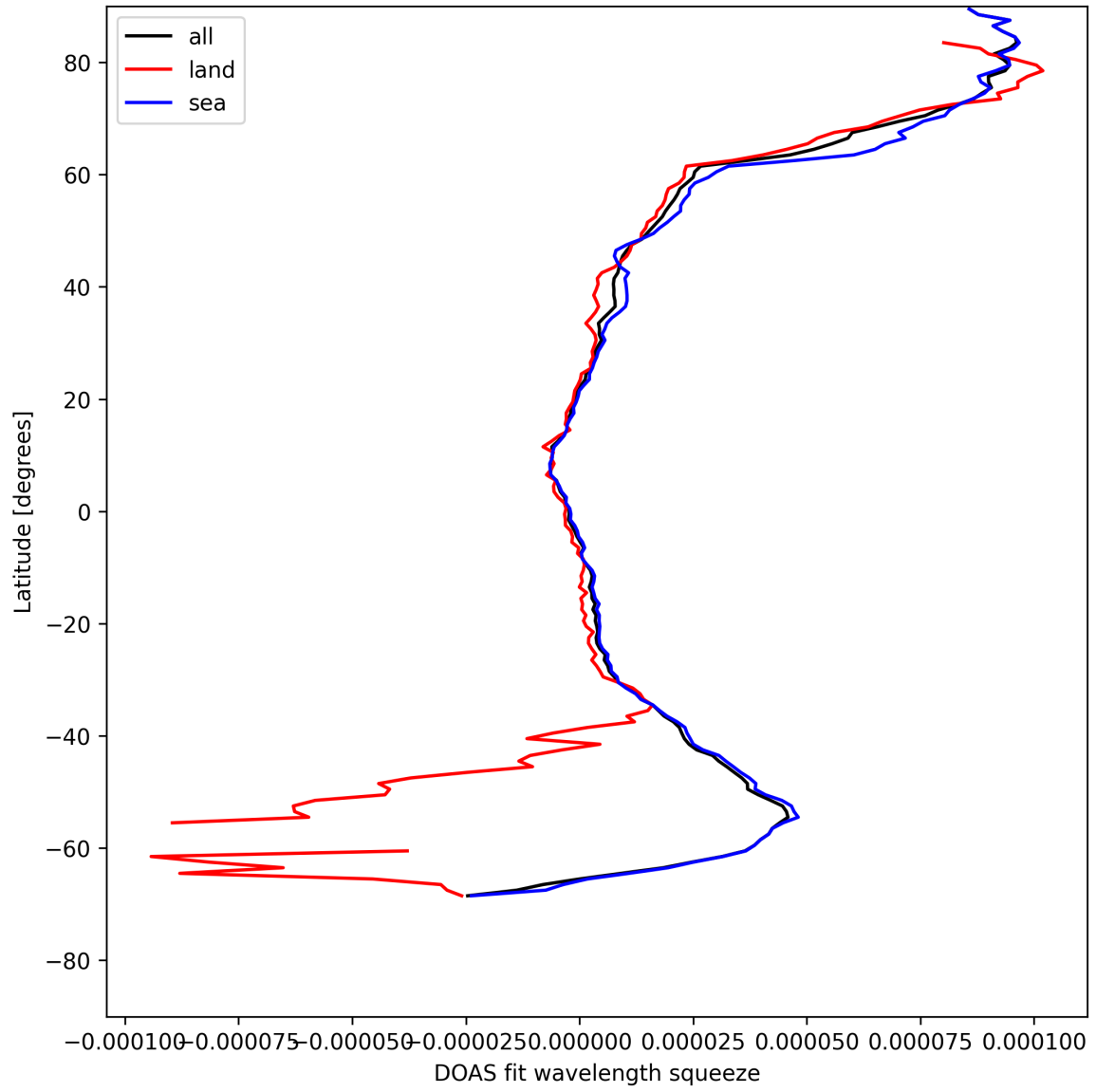
Figure 29: Zonal average of “DOAS fit wavelength squeeze” for 2025-08-07 to 2025-08-07.
