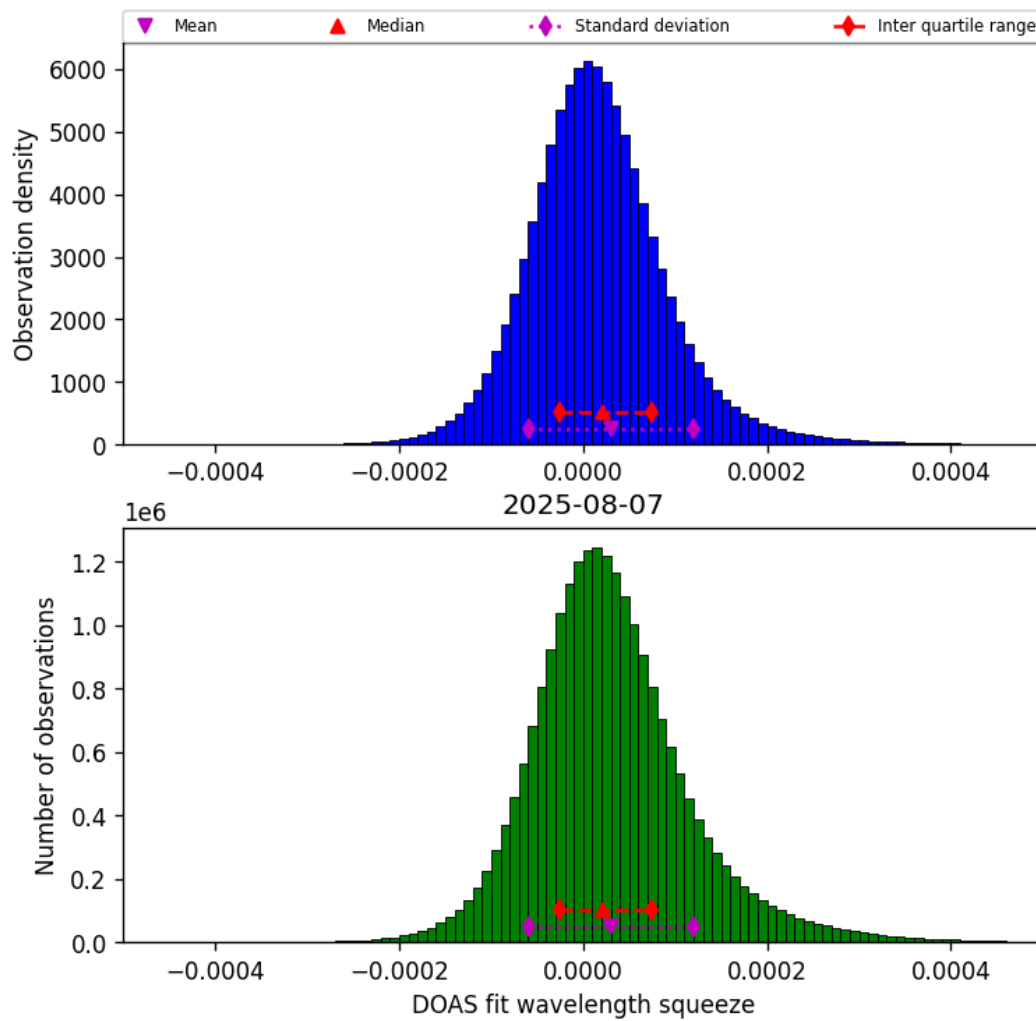
Figure 43: Histogram of “DOAS fit wavelength squeeze” for 2025-08-07 to 2025-08-07
