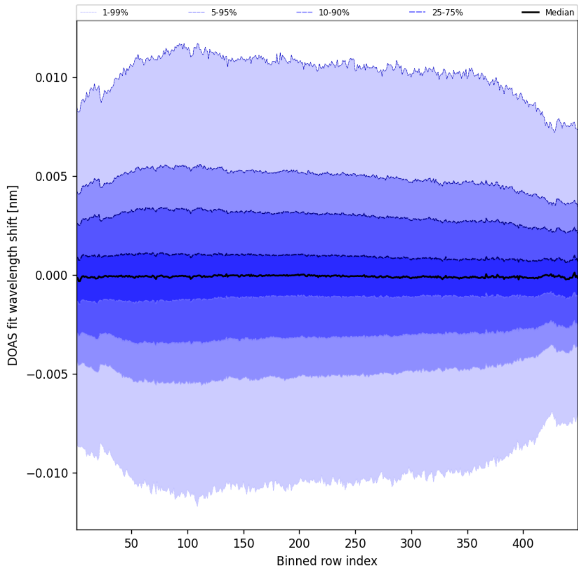
Figure 56: Along track statistics of “DOAS fit wavelength shift” for 2025-08-07 to 2025-08-07
