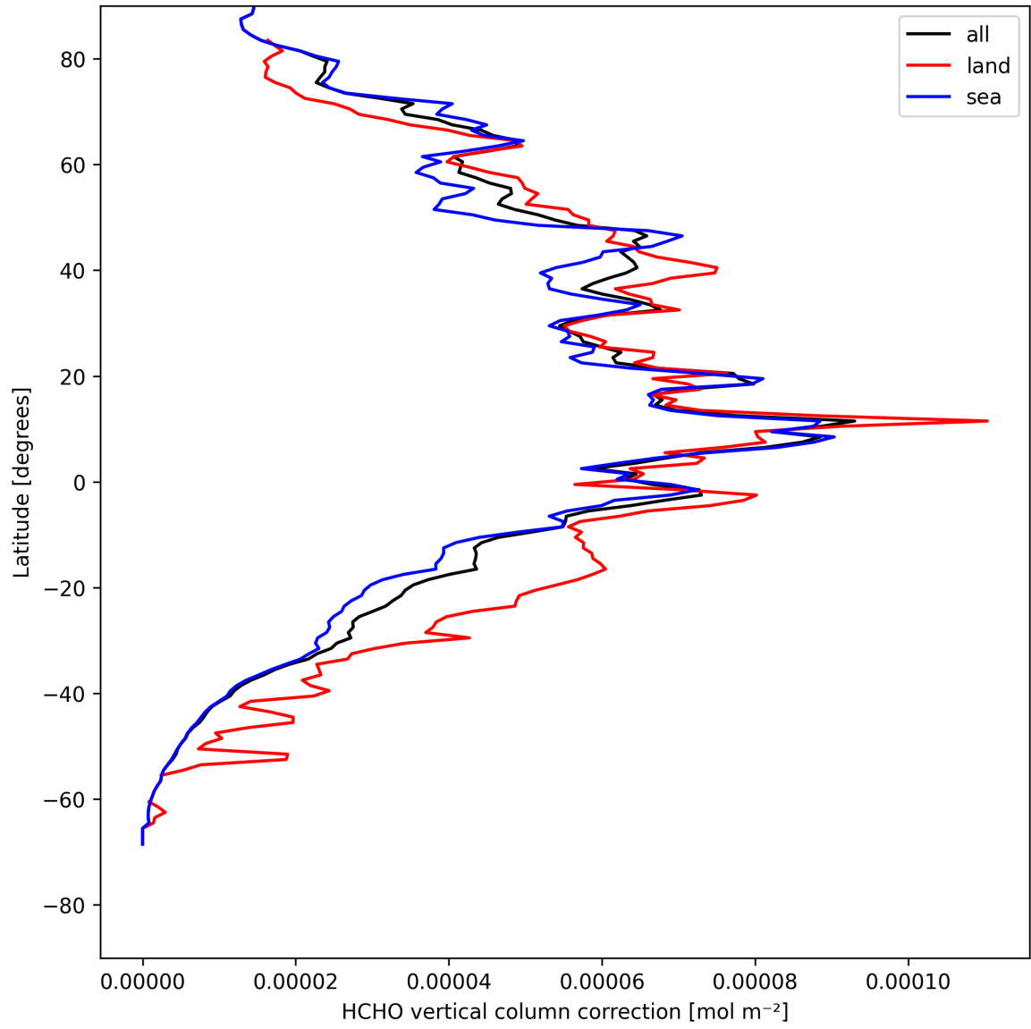
Figure 21: Zonal average of “HCHO vertical column correction” for 2025-08-07 to 2025-08-07.
