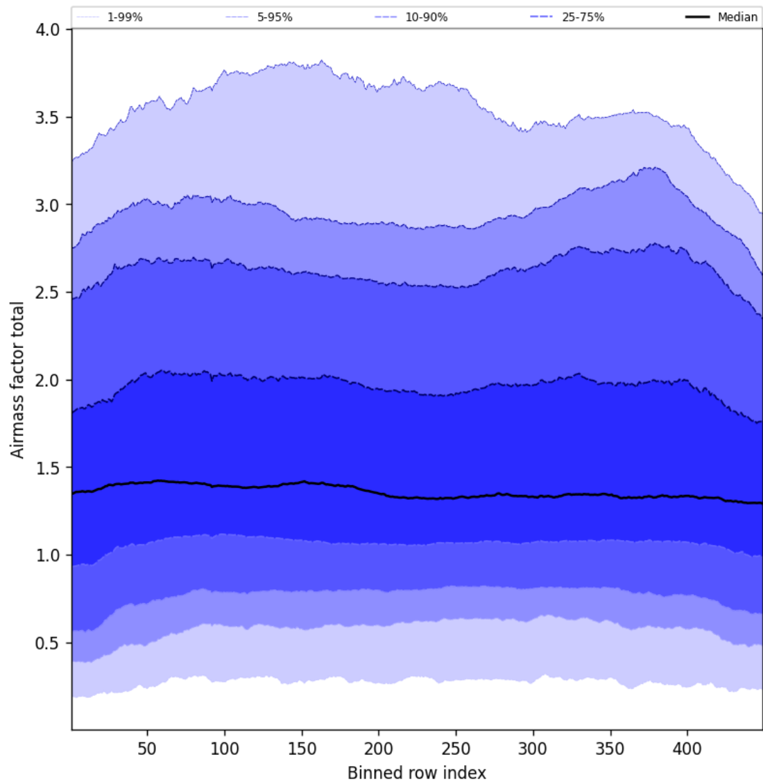
Figure 52: Along track statistics of “Airmass factor total” for 2025-08-07 to 2025-08-07
