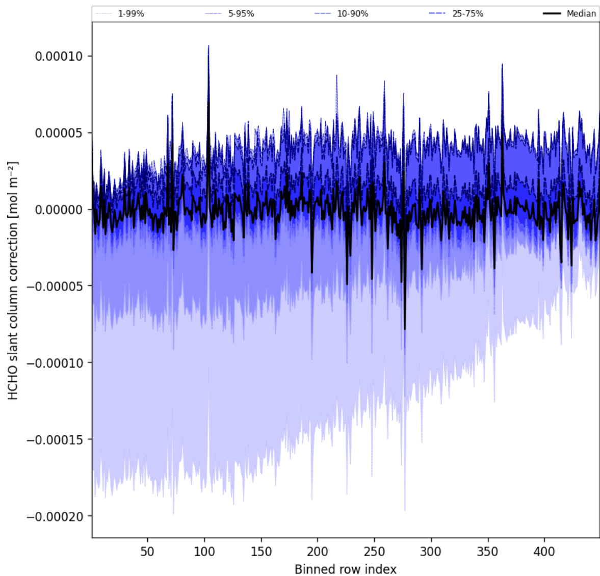
Figure 59: Along track statistics of “HCHO slant column correction” for 2025-08-07 to 2025-08-07
