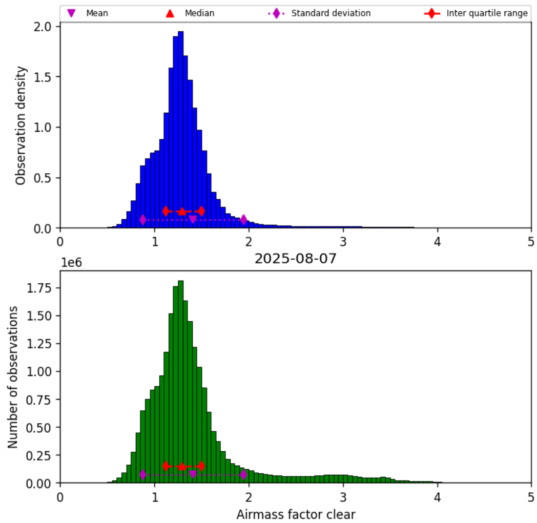
Figure 40: Histogram of “Airmass factor clear” for 2025-08-07 to 2025-08-07
