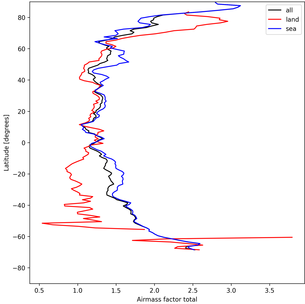
Figure 24: Zonal average of “Airmass factor total” for 2025-08-07 to 2025-08-07.
