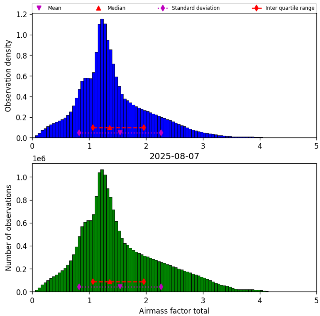
Figure 38: Histogram of “Airmass factor total” for 2025-08-07 to 2025-08-07
