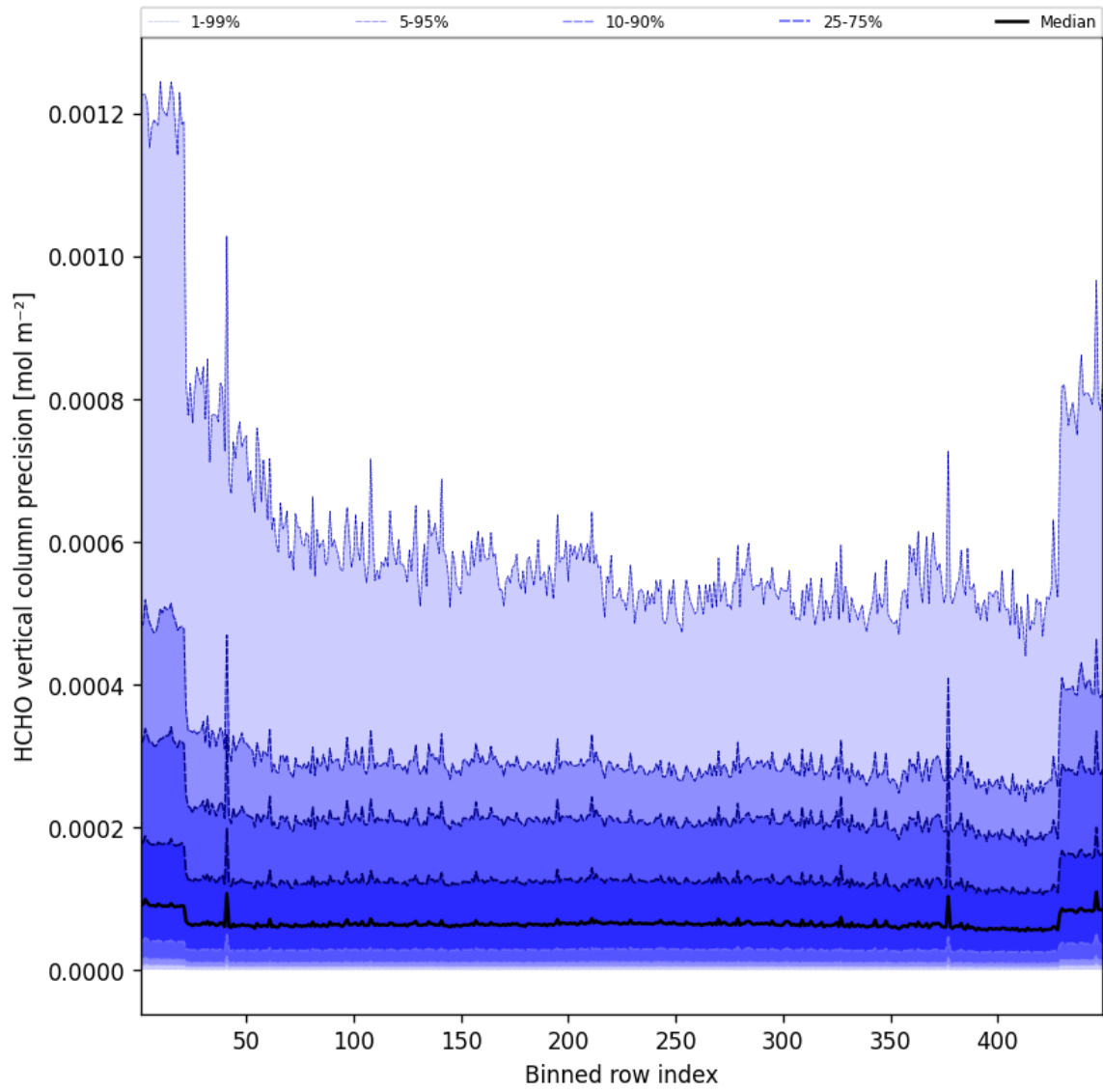
Figure 48: Along track statistics of “HCHO vertical column precision” for 2025-08-07 to 2025-08-07
