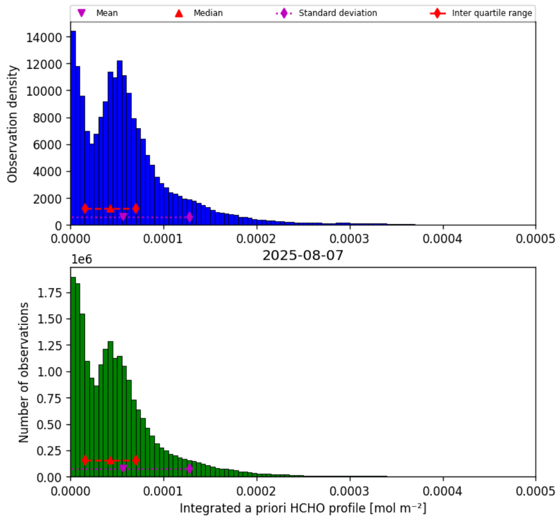
Figure 41: Histogram of “Integrated a priori HCHO profile” for 2025-08-07 to 2025-08-07
