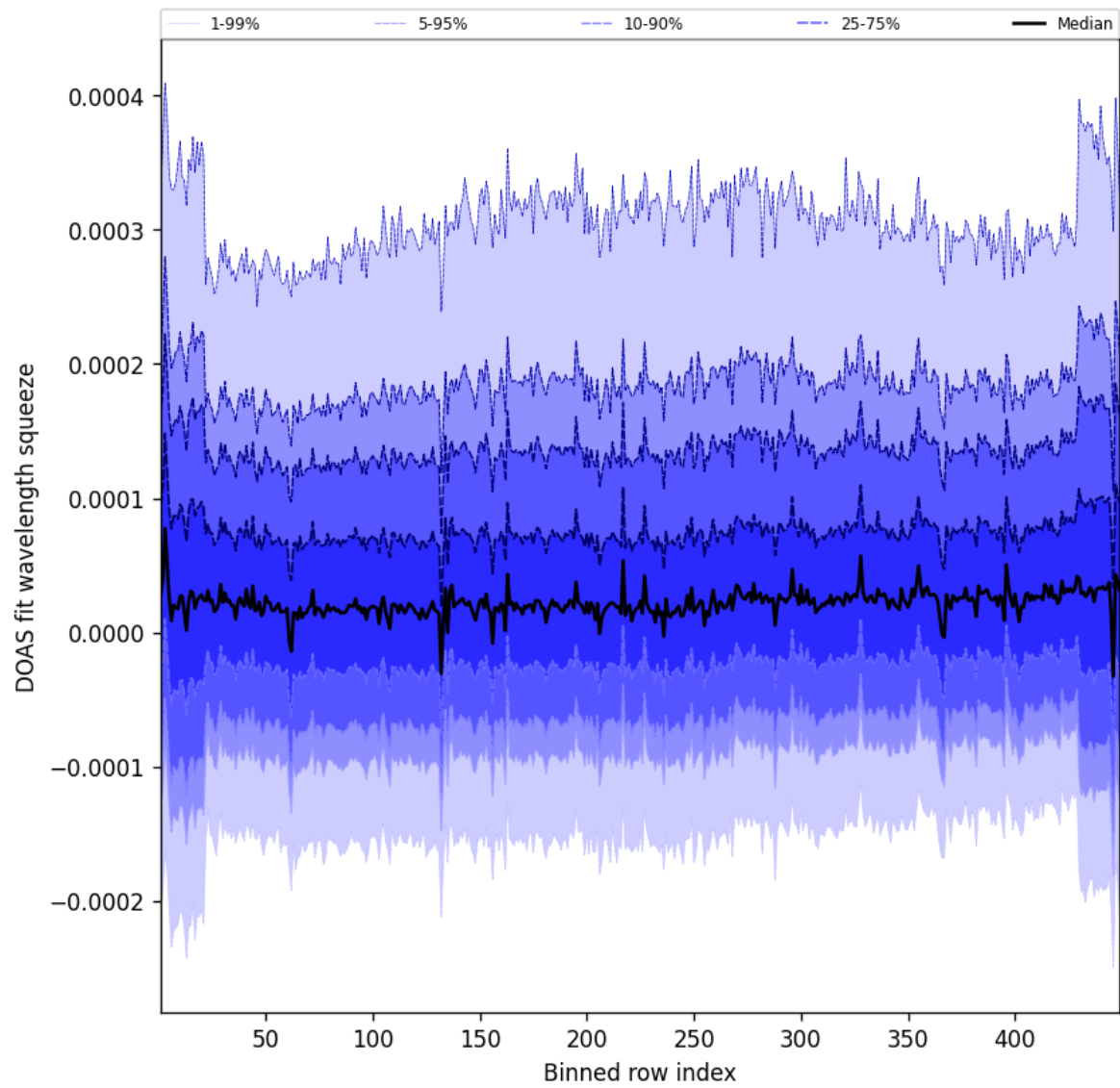
Figure 57: Along track statistics of “DOAS fit wavelength squeeze” for 2025-08-07 to 2025-08-07
