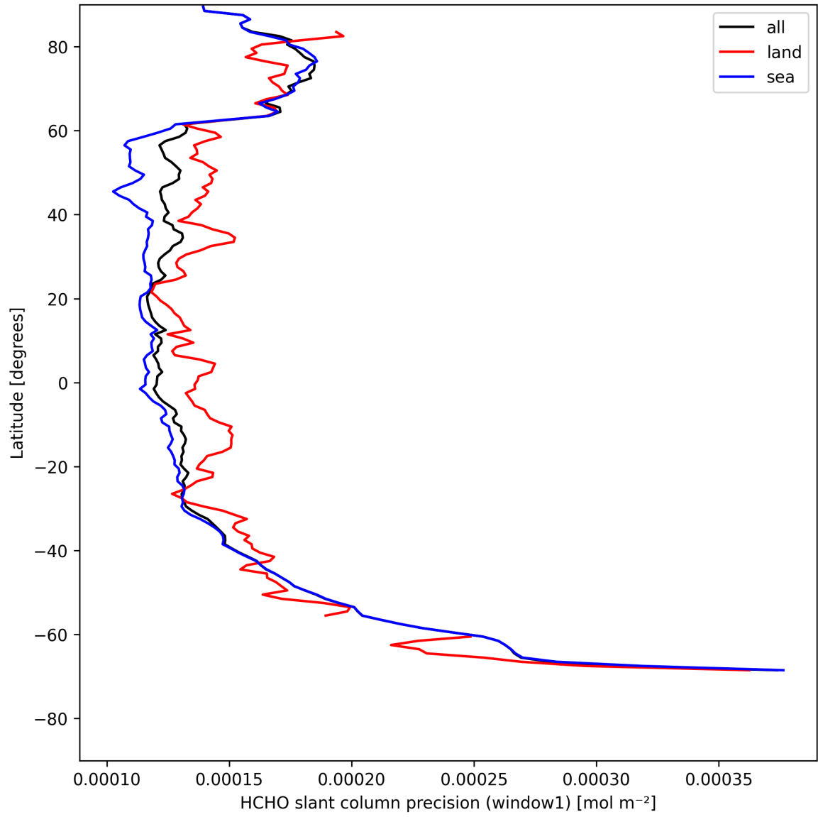
Figure 23: Zonal average of “HCHO slant column precision (window1)” for 2025-08-07 to 2025-08-07.
