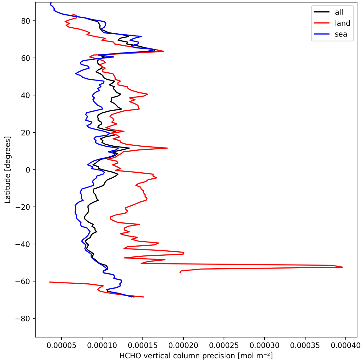
Figure 20: Zonal average of “HCHO vertical column precision” for 2025-08-07 to 2025-08-07.
