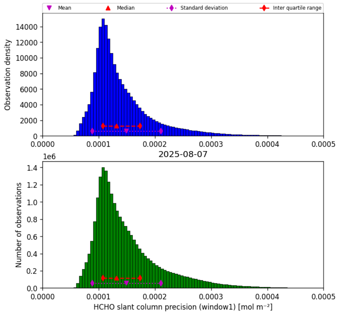
Figure 37: Histogram of “HCHO slant column precision (window1)” for 2025-08-07 to 2025-08-07
