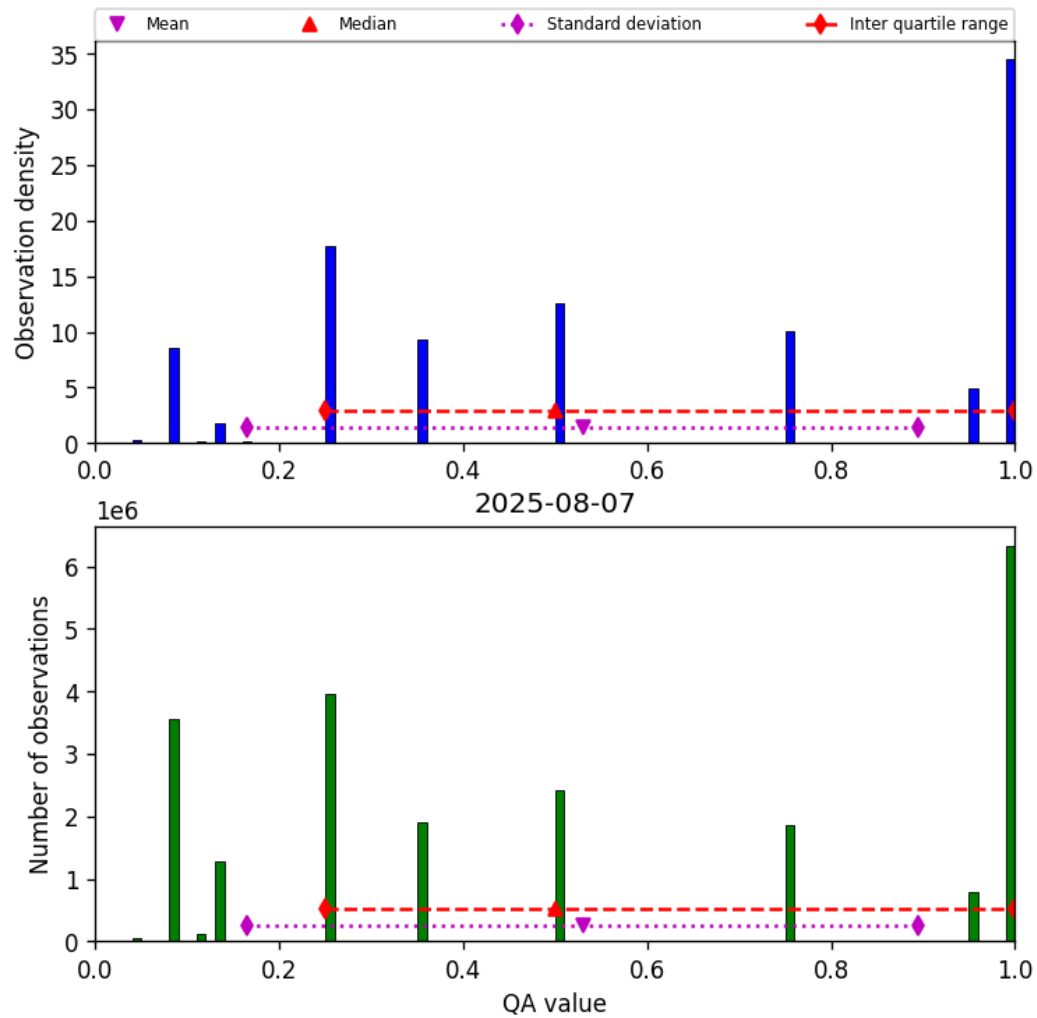
Figure 32: Histogram of “QA value” for 2025-08-07 to 2025-08-07
