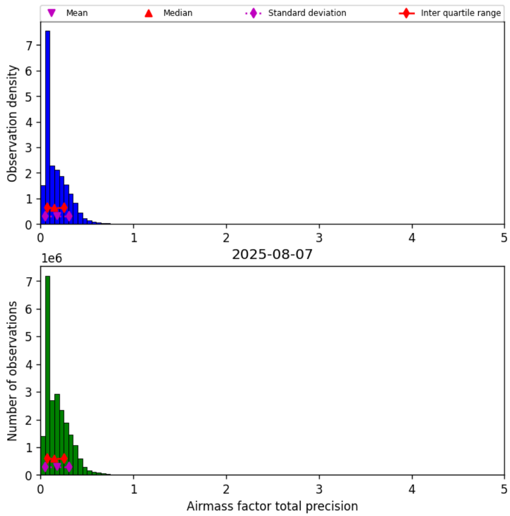
Figure 39: Histogram of “Airmass factor total precision” for 2025-08-07 to 2025-08-07
