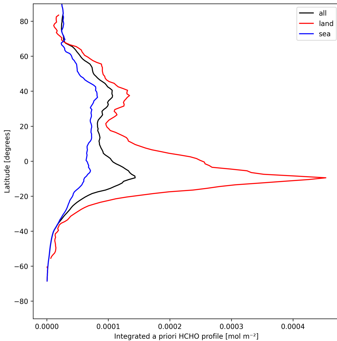
Figure 27: Zonal average of “Integrated a priori HCHO profile” for 2025-08-07 to 2025-08-07.
