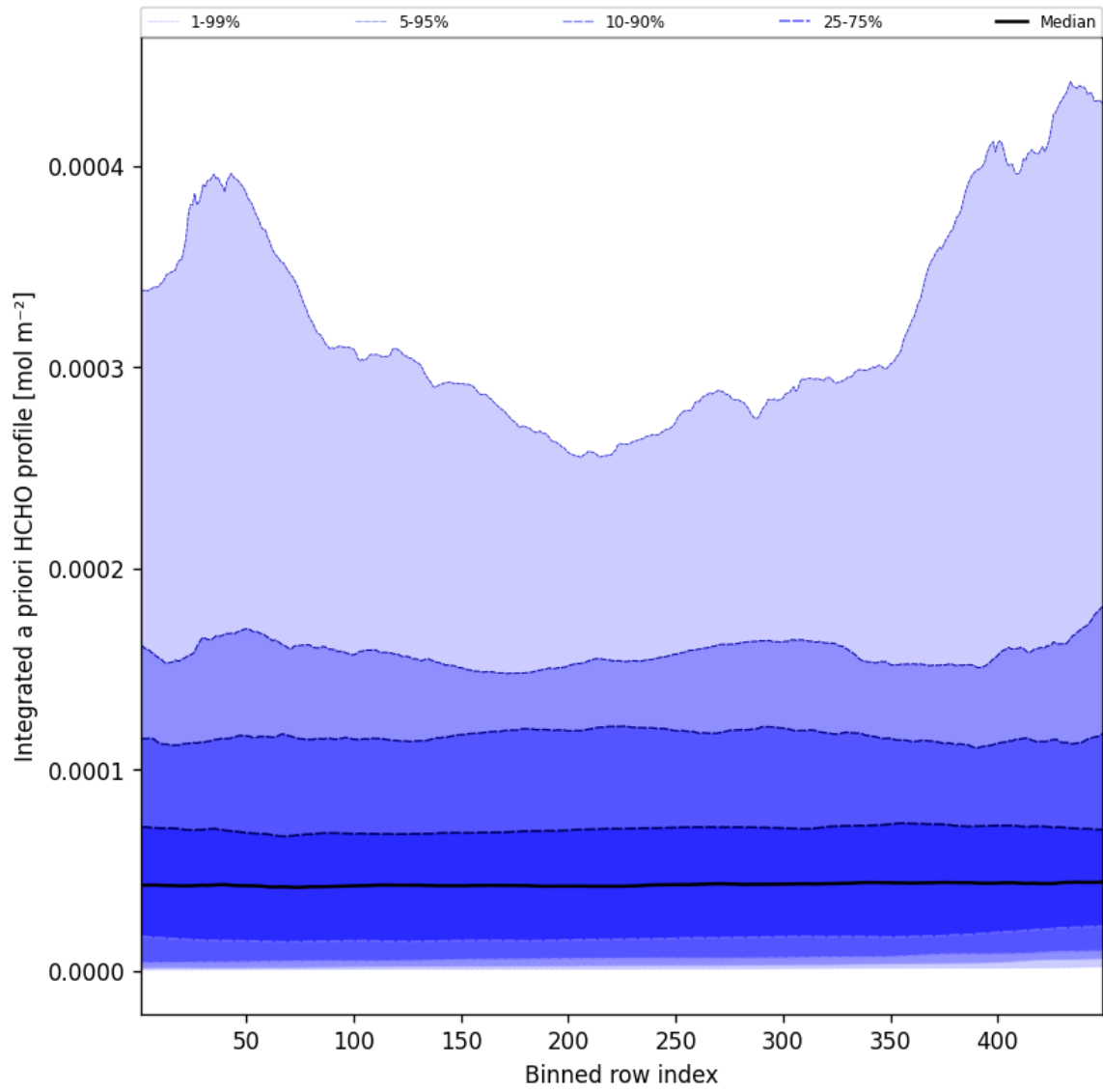
Figure 55: Along track statistics of “Integrated a priori HCHO profile” for 2025-08-07 to 2025-08-07
