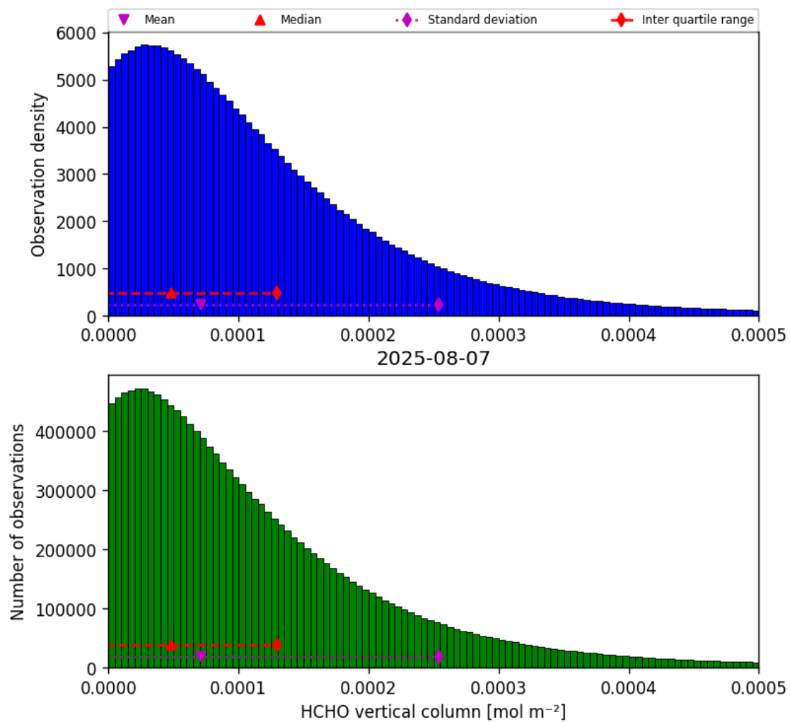
Figure 33: Histogram of “HCHO vertical column” for 2025-08-07 to 2025-08-07
