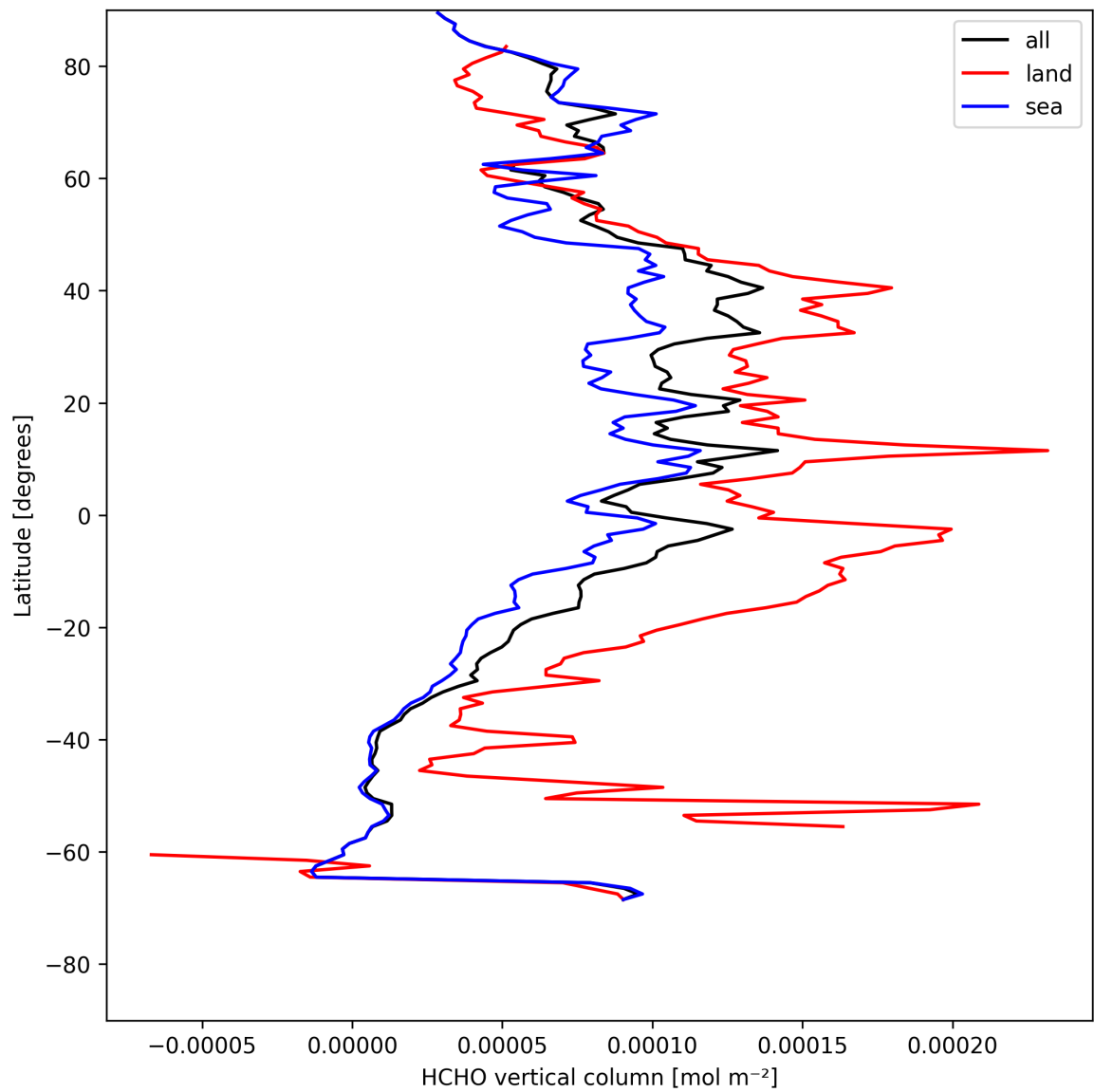
Figure 19: Zonal average of “HCHO vertical column” for 2025-08-07 to 2025-08-07.
