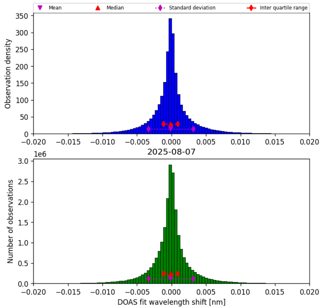
Figure 42: Histogram of “DOAS fit wavelength shift” for 2025-08-07 to 2025-08-07
