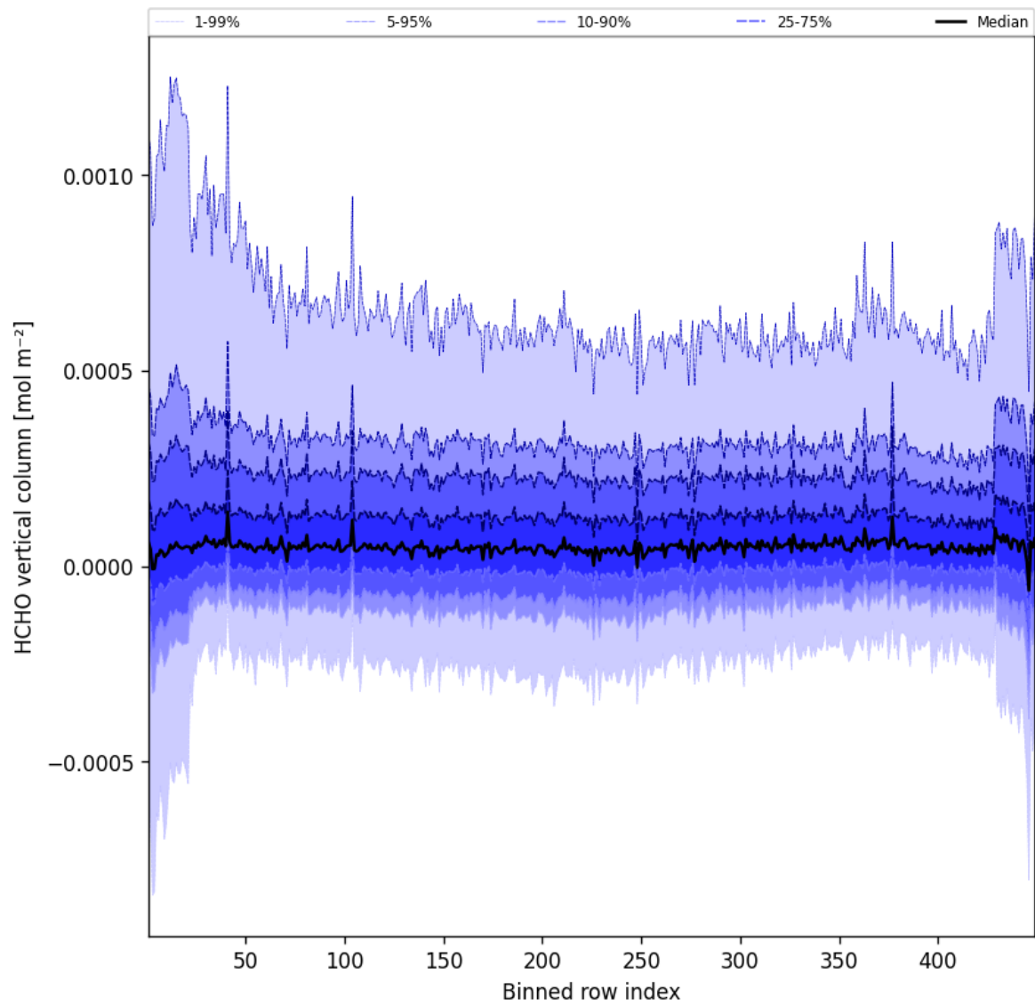
Figure 47: Along track statistics of “HCHO vertical column” for 2025-08-07 to 2025-08-07
