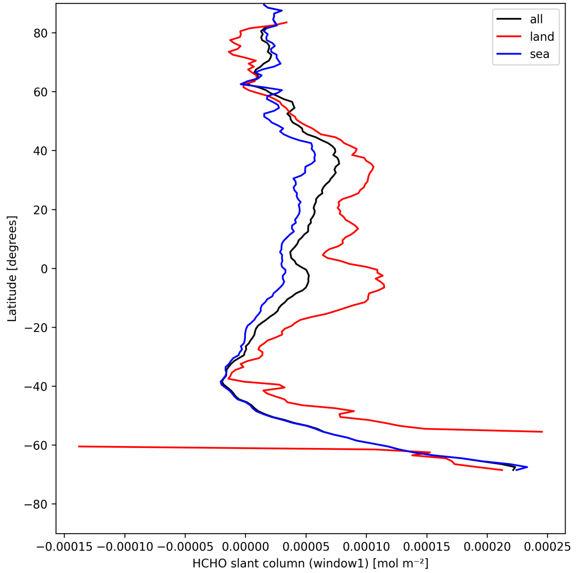
Figure 22: Zonal average of “HCHO slant column (window1)” for 2025-08-07 to 2025-08-07.
