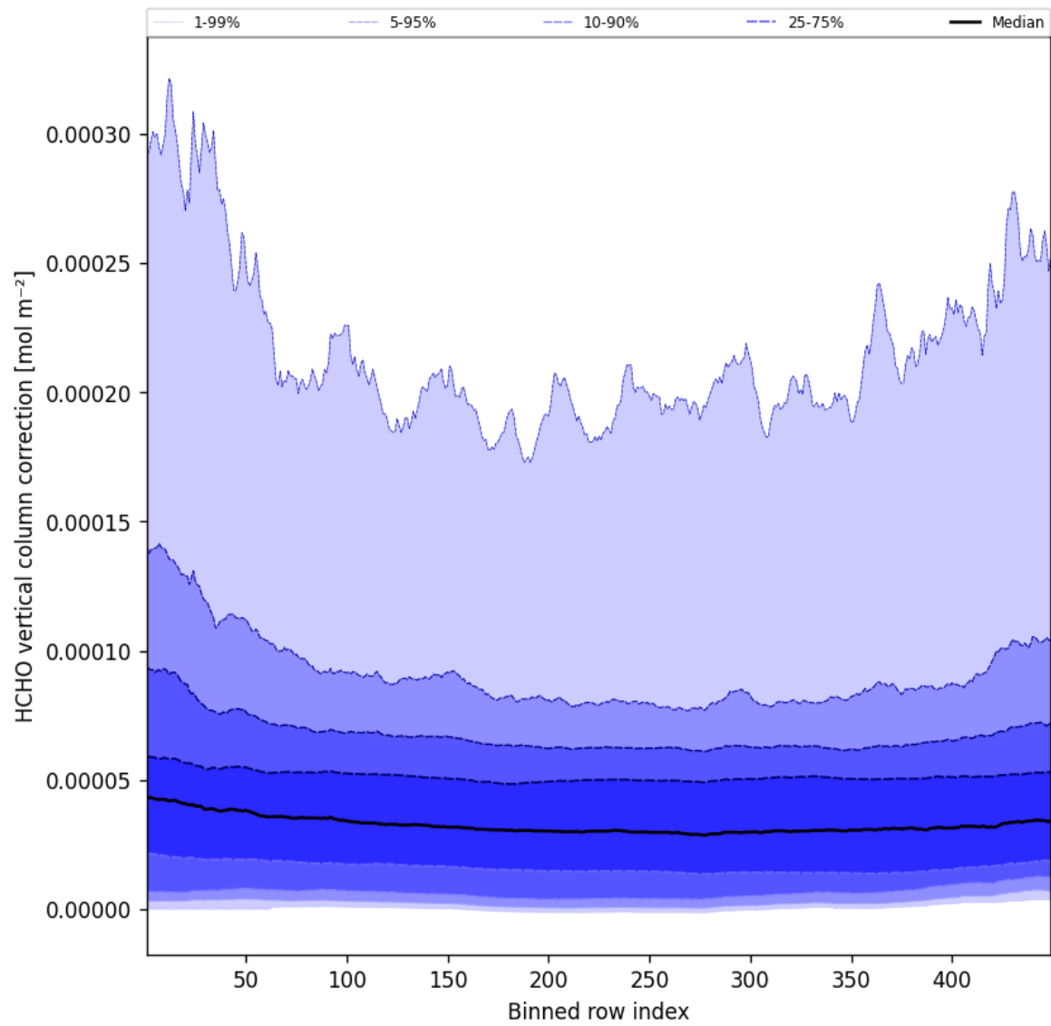
Figure 49: Along track statistics of “HCHO vertical column correction” for 2025-08-07 to 2025-08-07
