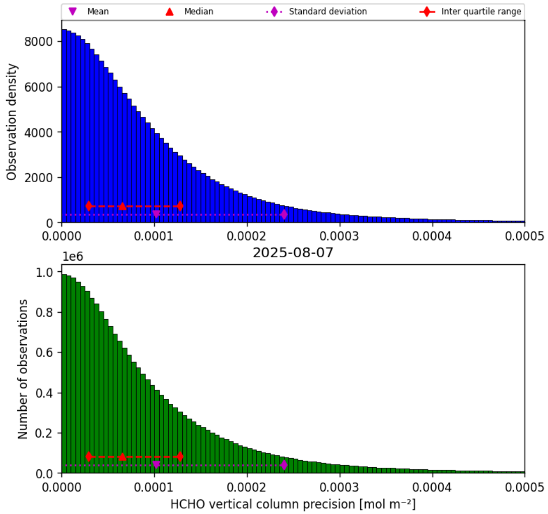
Figure 34: Histogram of “HCHO vertical column precision” for 2025-08-07 to 2025-08-07
