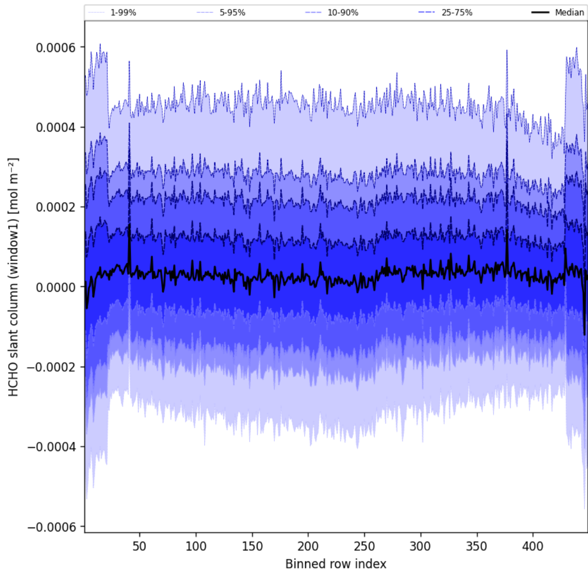
Figure 50: Along track statistics of “HCHO slant column (window1)” for 2025-08-07 to 2025-08-07
