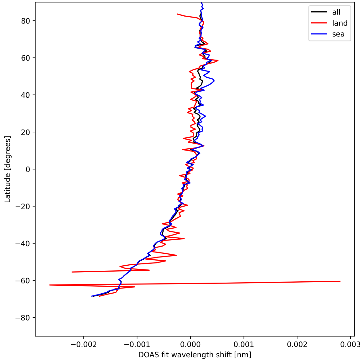
Figure 28: Zonal average of “DOAS fit wavelength shift” for 2025-08-07 to 2025-08-07.
