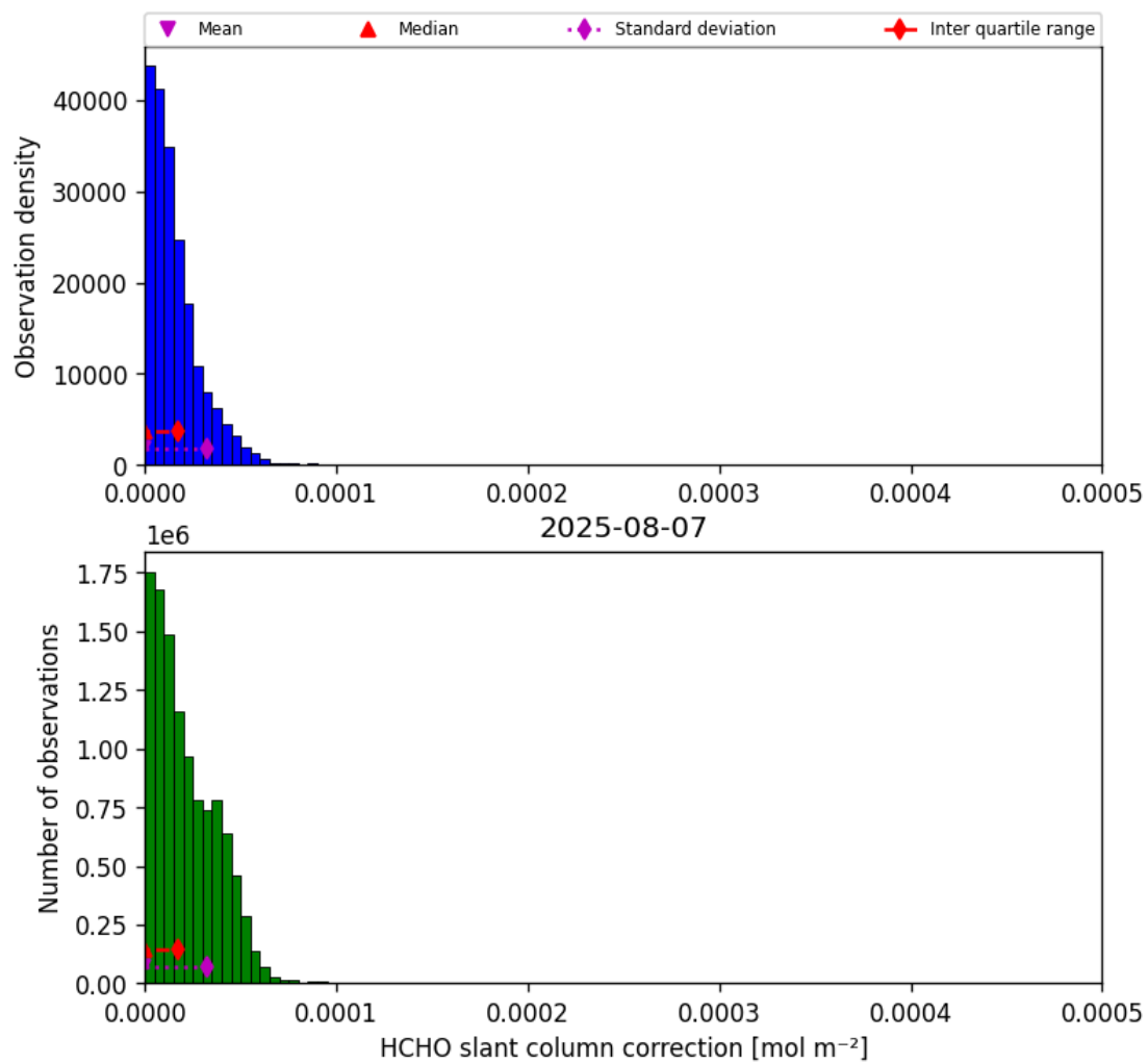
Figure 45: Histogram of “HCHO slant column correction” for 2025-08-07 to 2025-08-07
