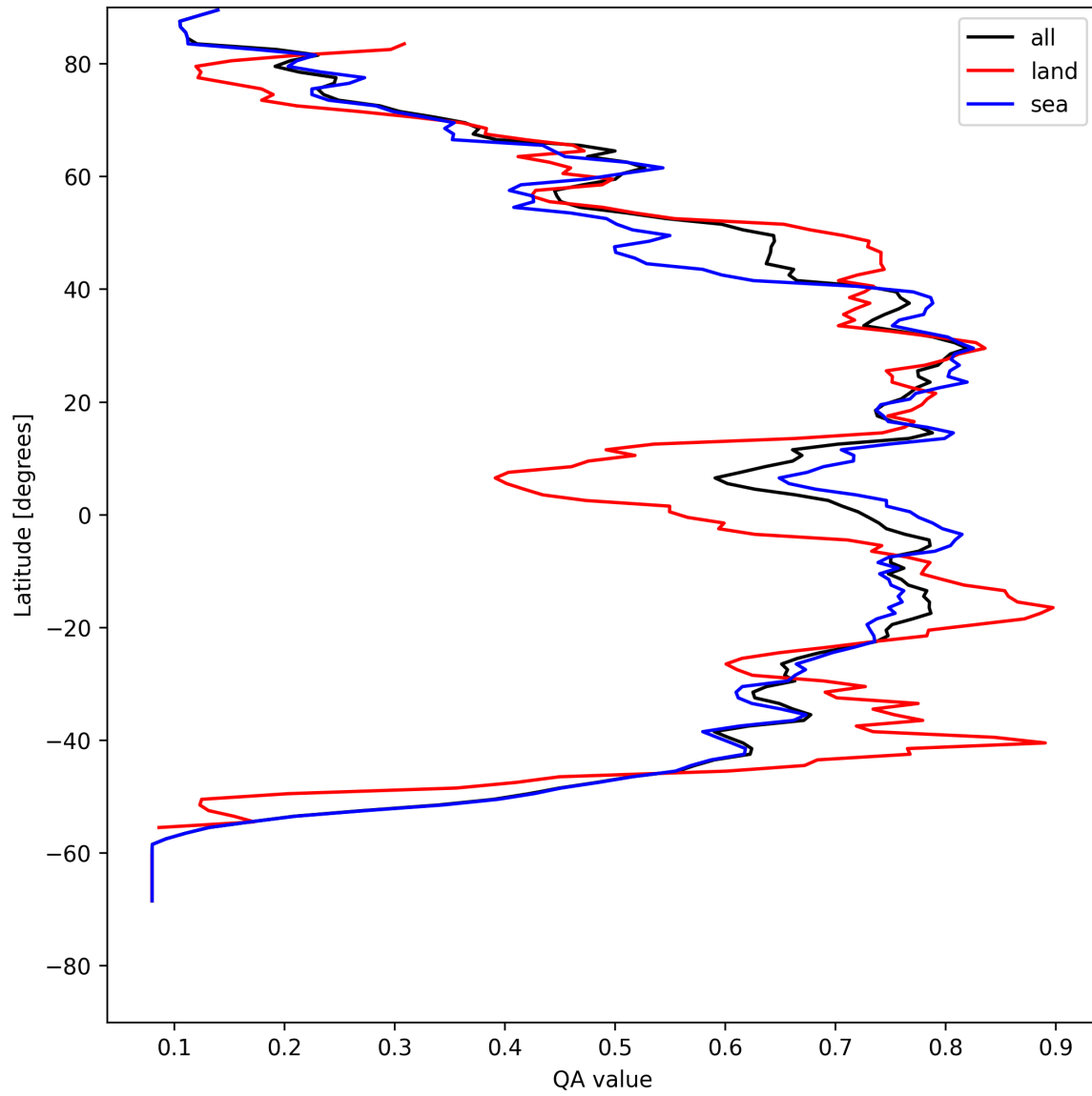
Figure 18: Zonal average of “QA value” for 2025-08-07 to 2025-08-07.
