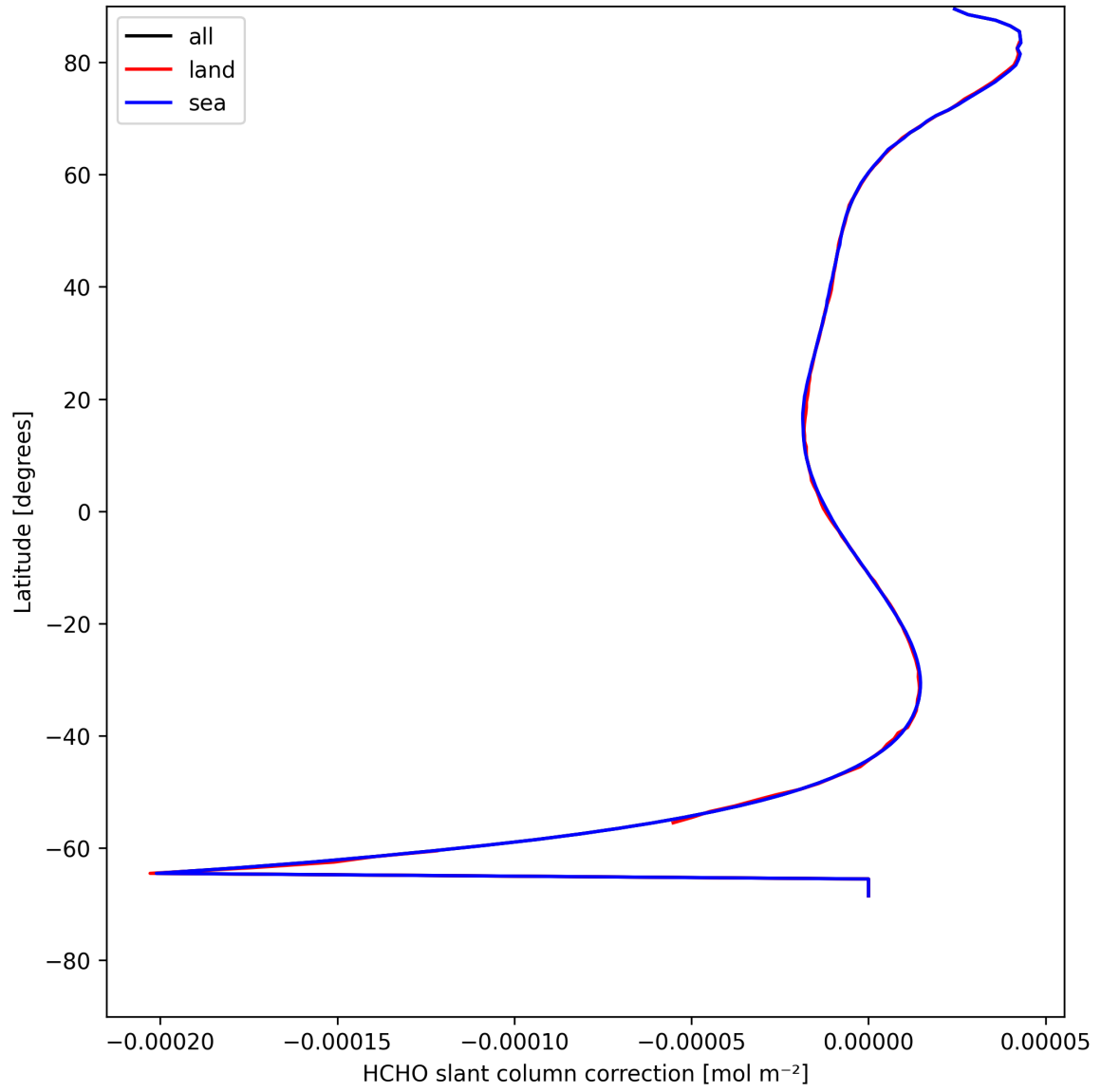
Figure 31: Zonal average of “HCHO slant column correction” for 2025-08-07 to 2025-08-07.
