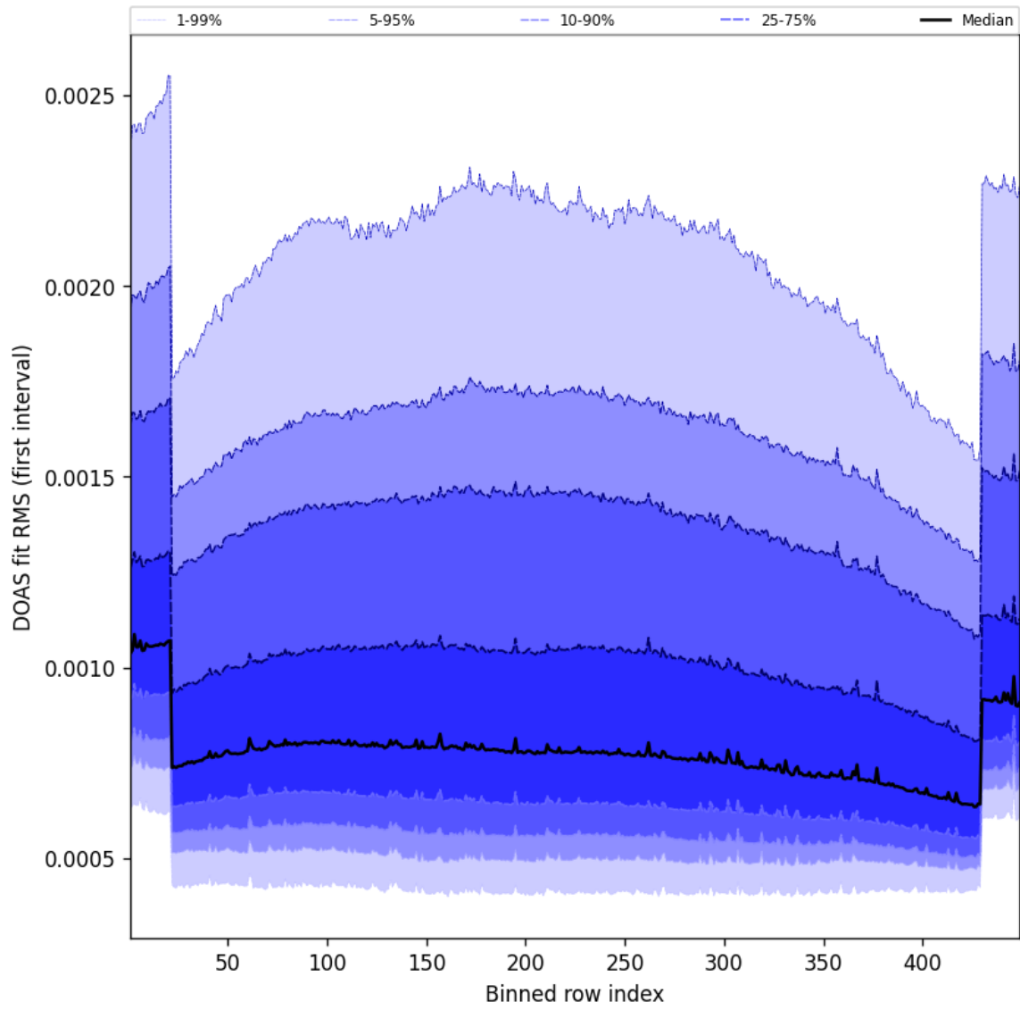
Figure 58: Along track statistics of “DOAS fit RMS (first interval)” for 2025-08-07 to 2025-08-07
