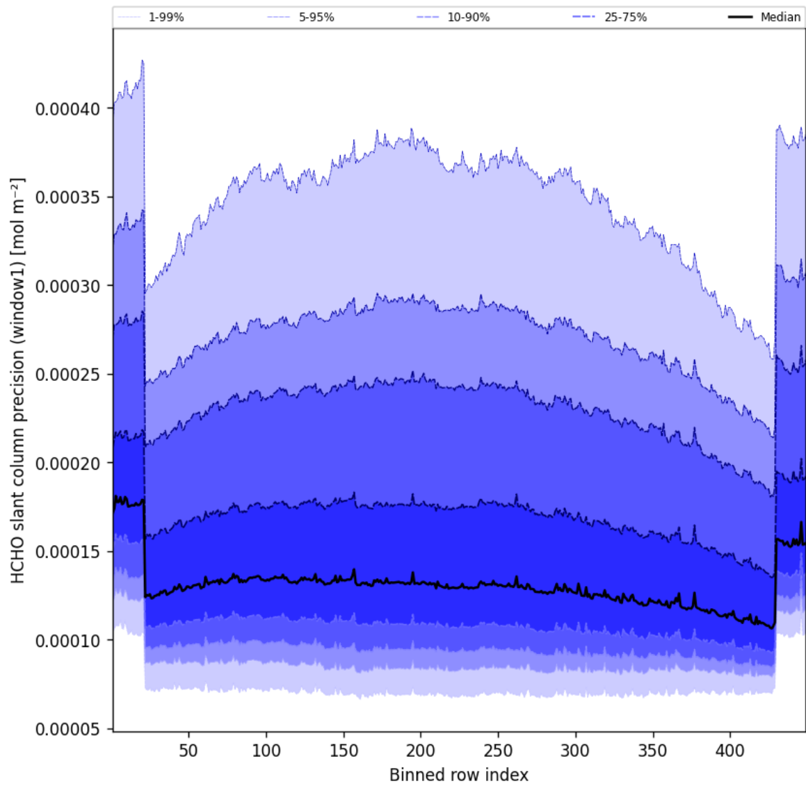
Figure 51: Along track statistics of “HCHO slant column precision (window1)” for 2025-08-07 to 2025-08-07
