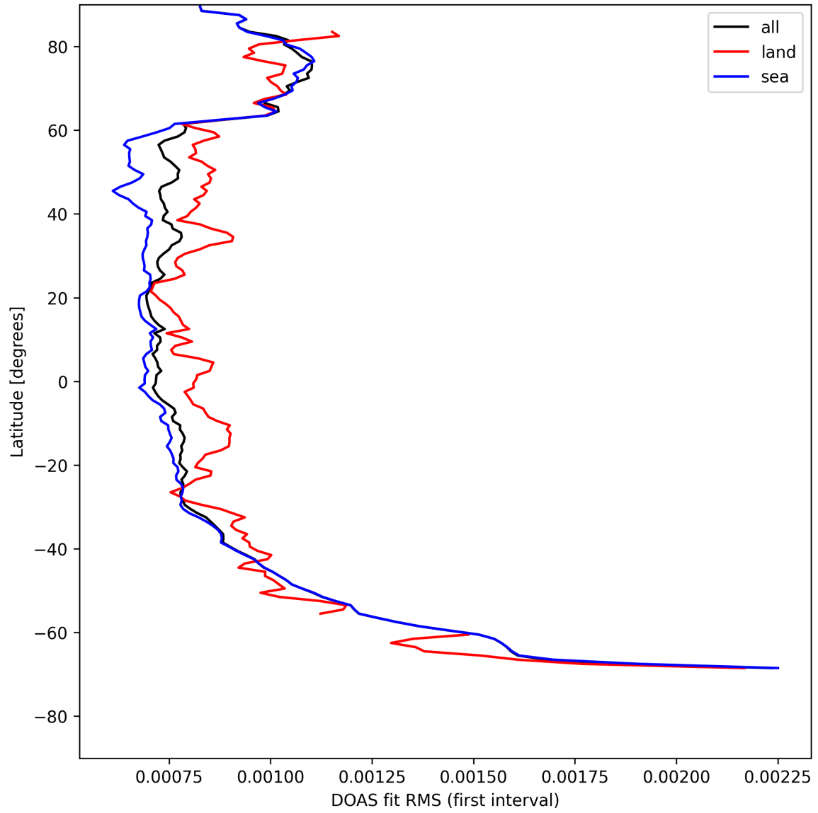
Figure 30: Zonal average of “DOAS fit RMS (first interval)” for 2025-08-07 to 2025-08-07.
