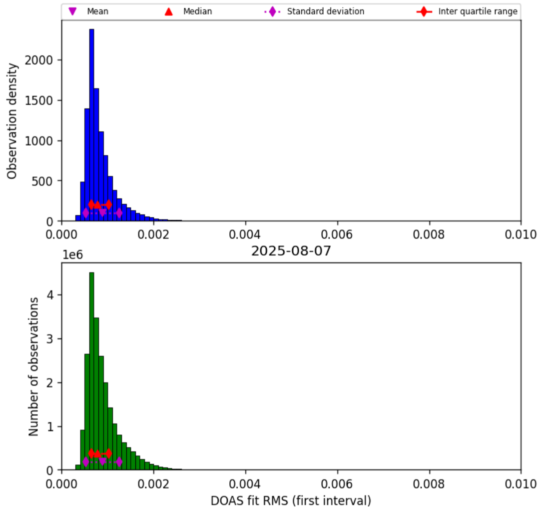
Figure 44: Histogram of “DOAS fit RMS (first interval)” for 2025-08-07 to 2025-08-07
