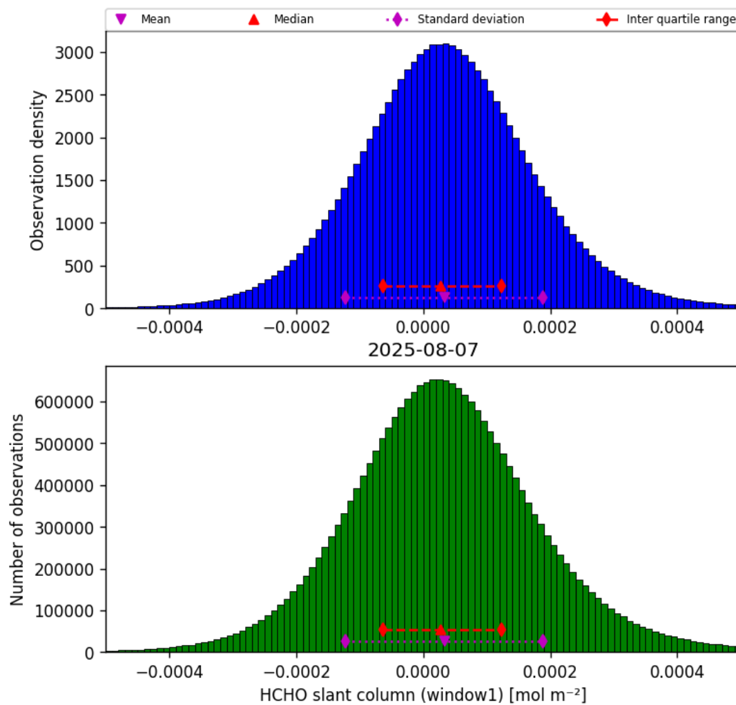
Figure 36: Histogram of “HCHO slant column (window1)” for 2025-08-07 to 2025-08-07
