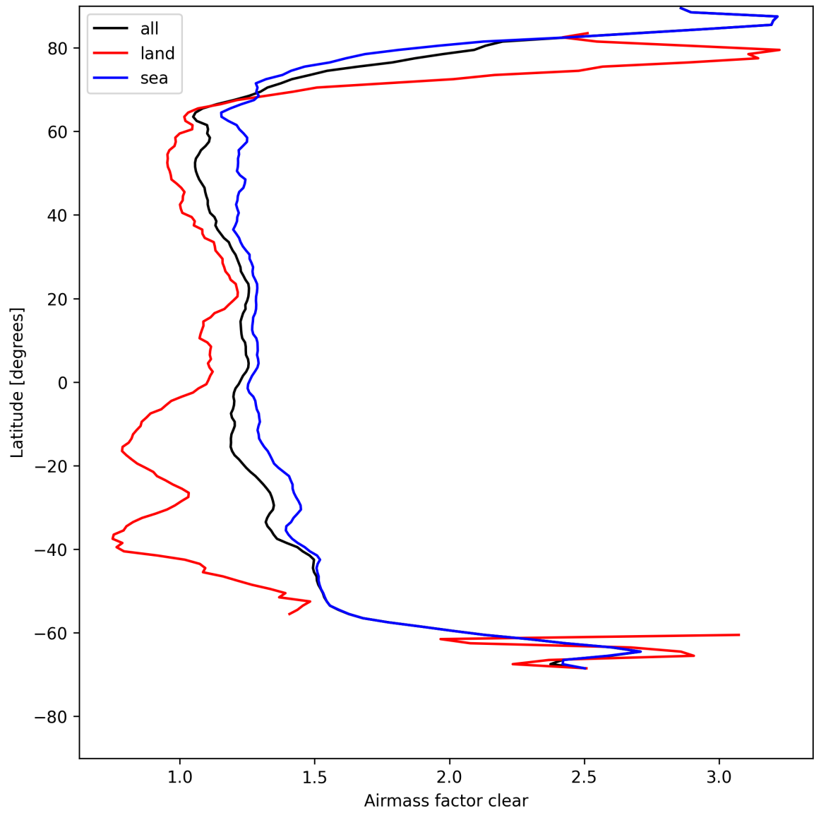
Figure 26: Zonal average of “Airmass factor clear” for 2025-08-07 to 2025-08-07.
