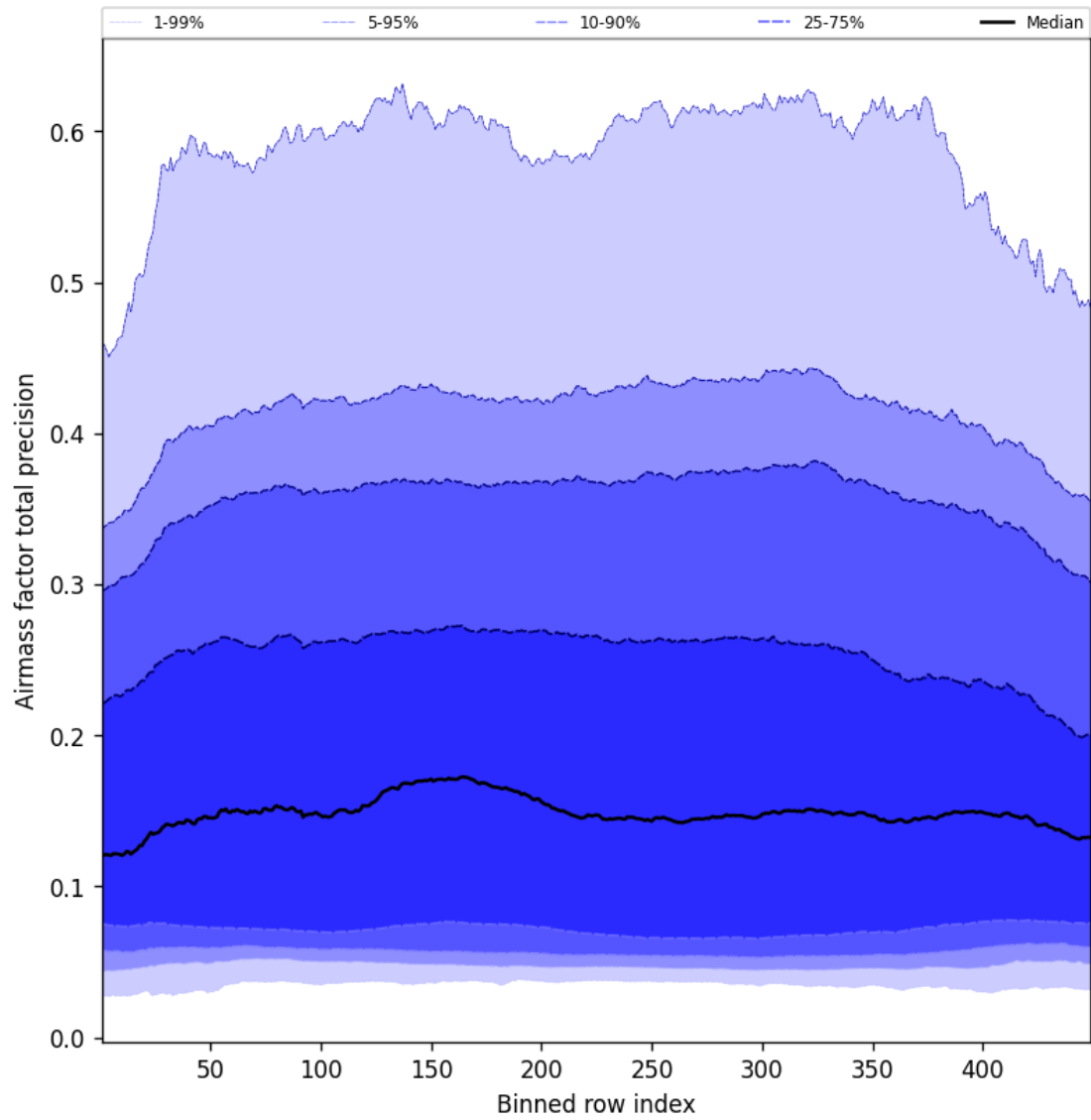
Figure 53: Along track statistics of “Airmass factor total precision” for 2025-08-07 to 2025-08-07
