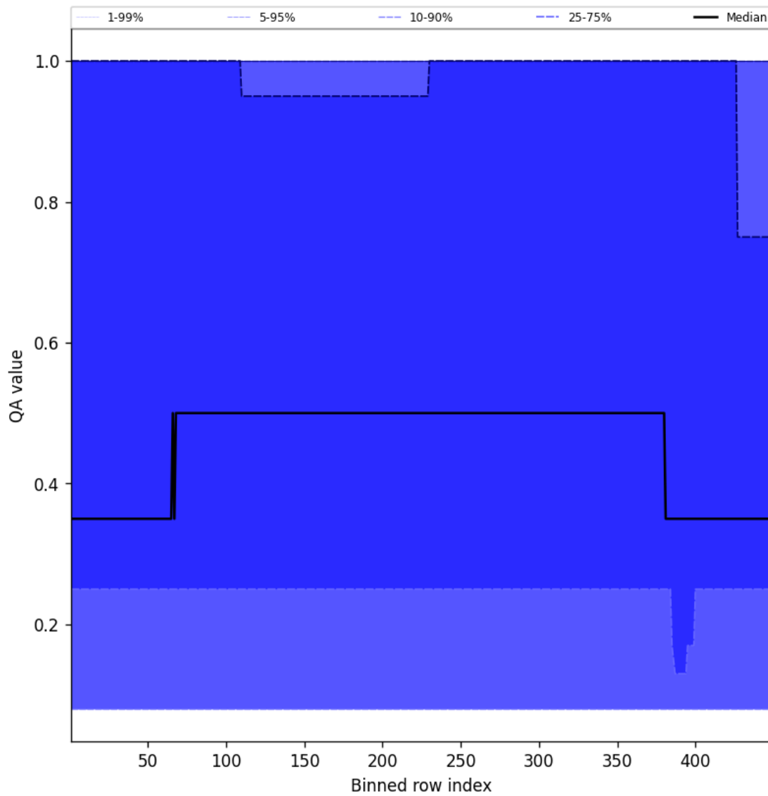
Figure 46: Along track statistics of “QA value” for 2025-08-07 to 2025-08-07
