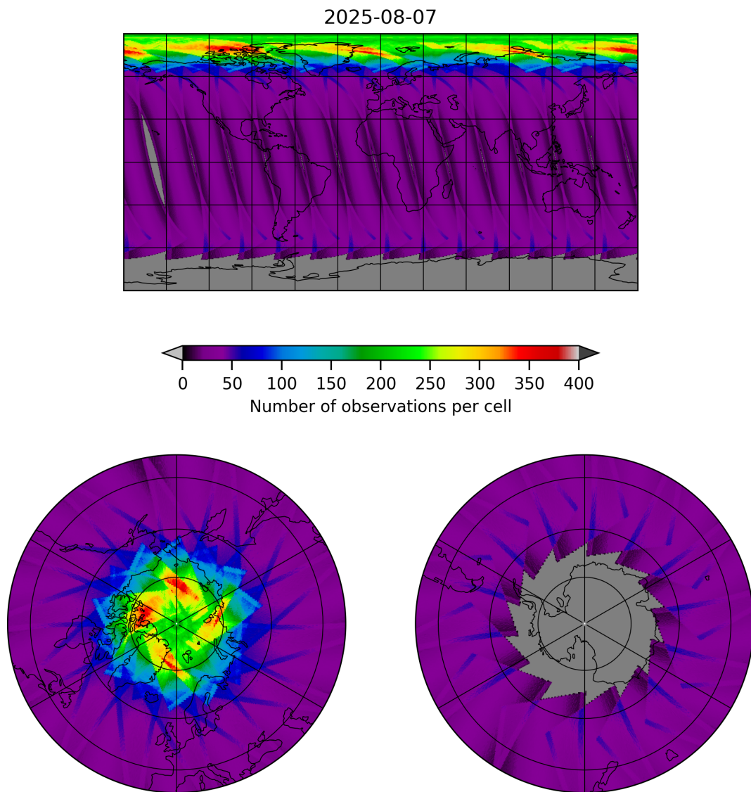
Figure 17: Map of the number of observations for 2025-08-07 to 2025-08-07
