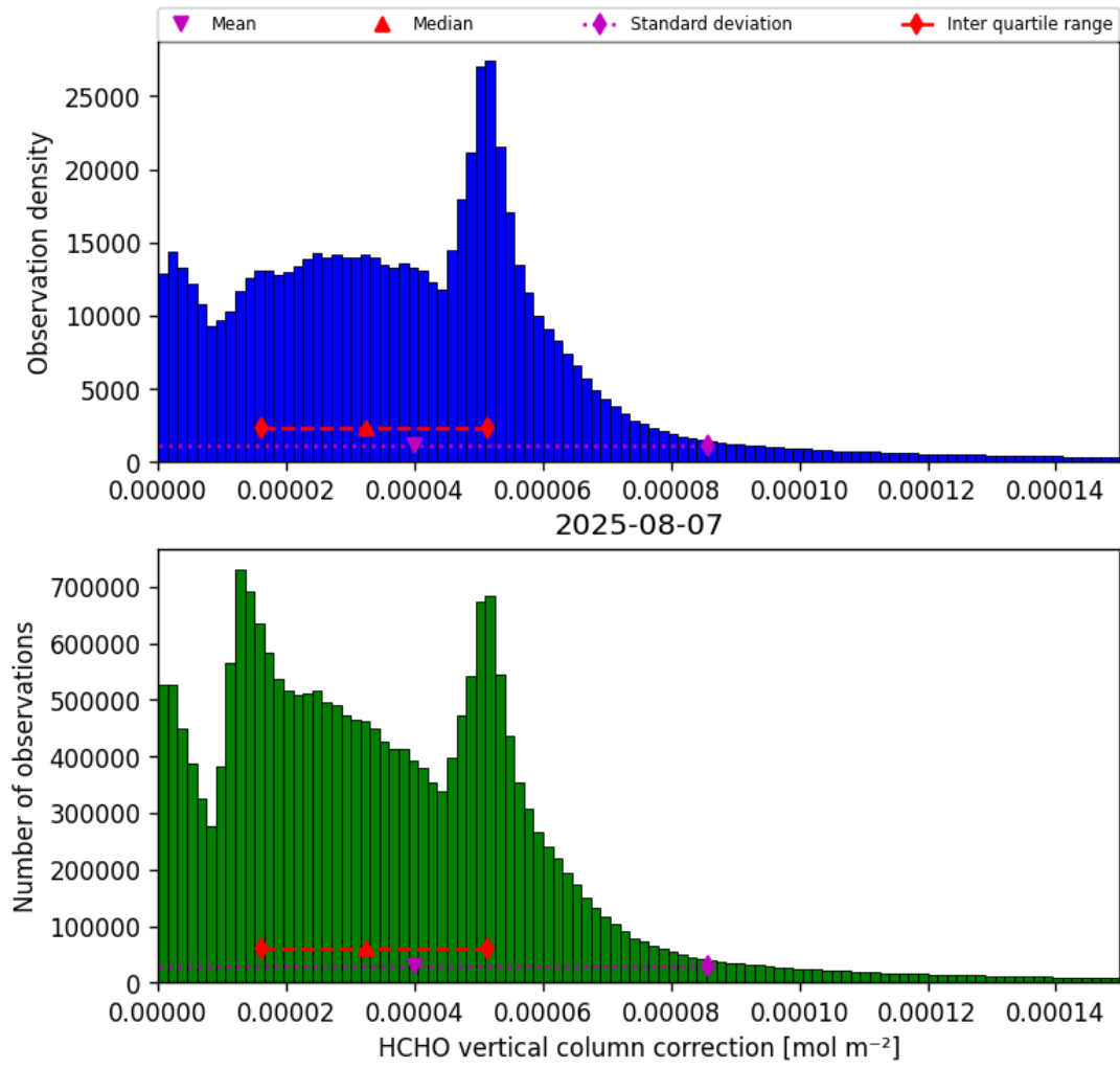
Figure 35: Histogram of “HCHO vertical column correction” for 2025-08-07 to 2025-08-07
