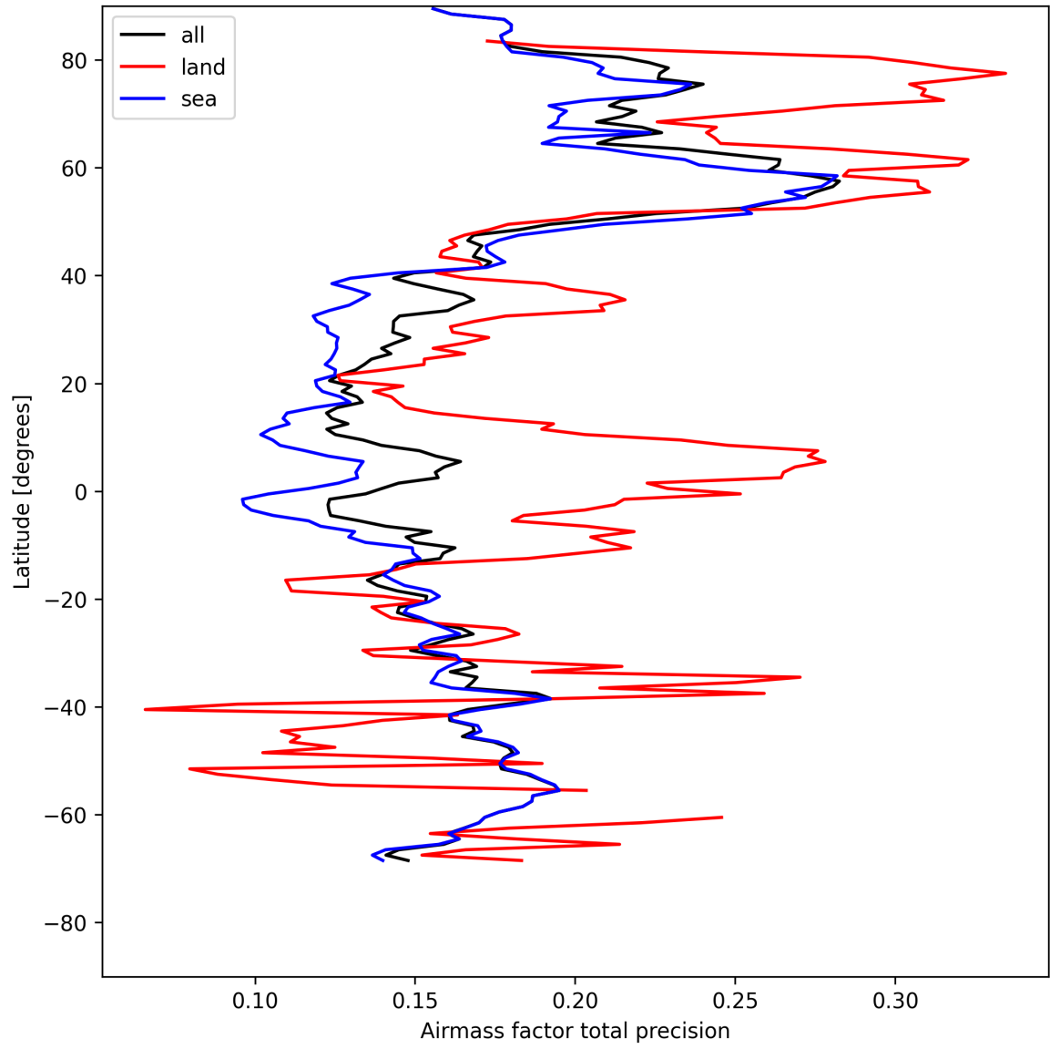
Figure 25: Zonal average of “Airmass factor total precision” for 2025-08-07 to 2025-08-07.
