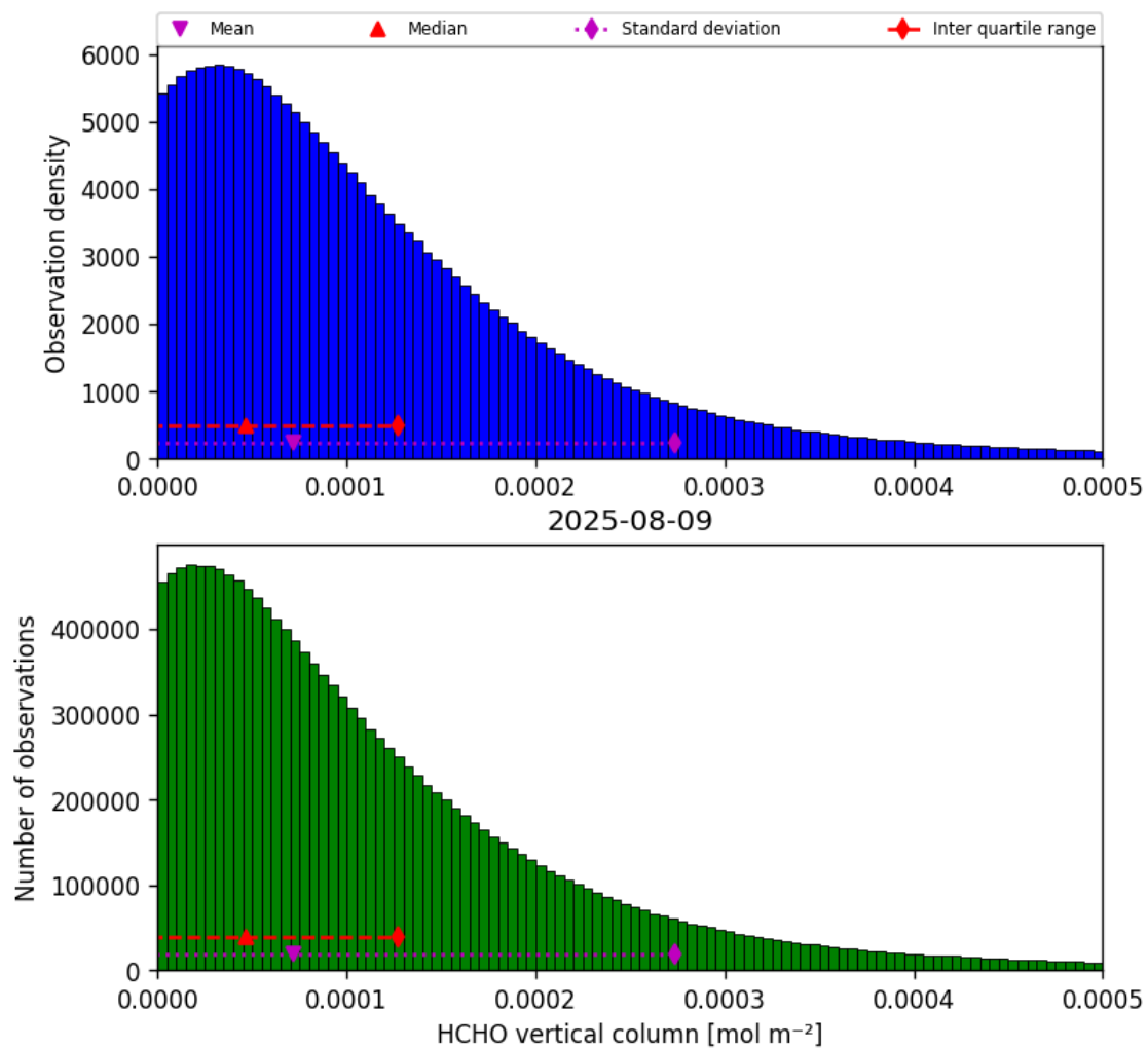
Figure 33: Histogram of “HCHO vertical column” for 2025-08-09 to 2025-08-10
