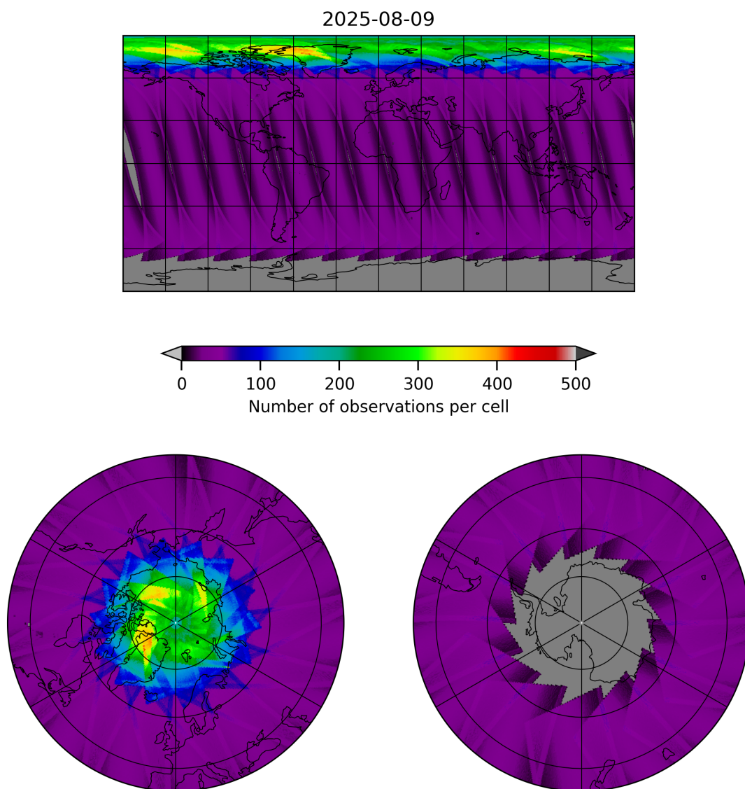
Figure 17: Map of the number of observations for 2025-08-09 to 2025-08-10
