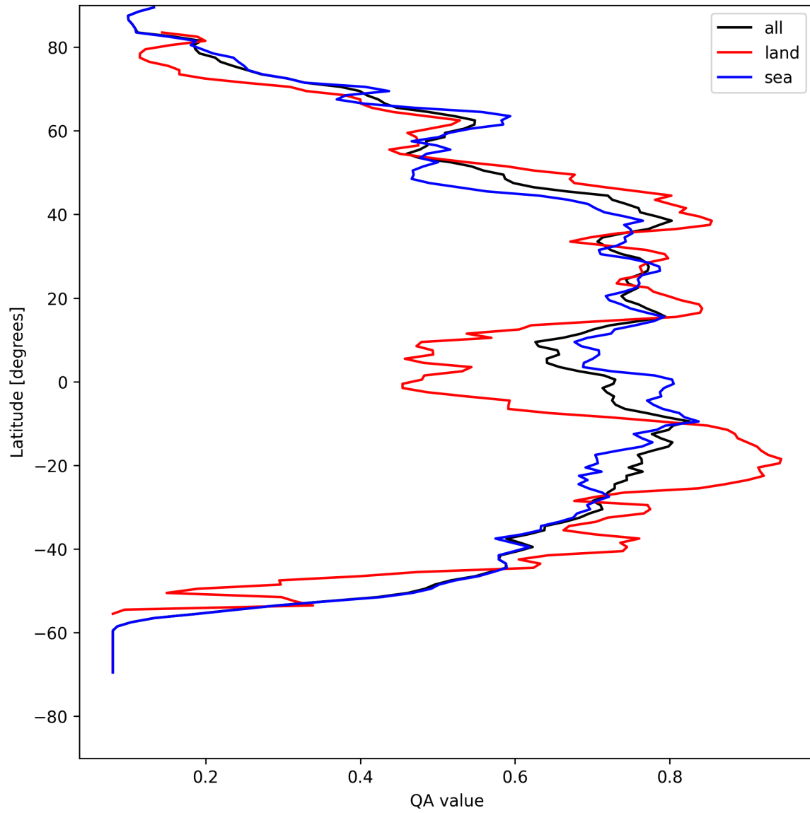
Figure 18: Zonal average of “QA value” for 2025-08-09 to 2025-08-10.
