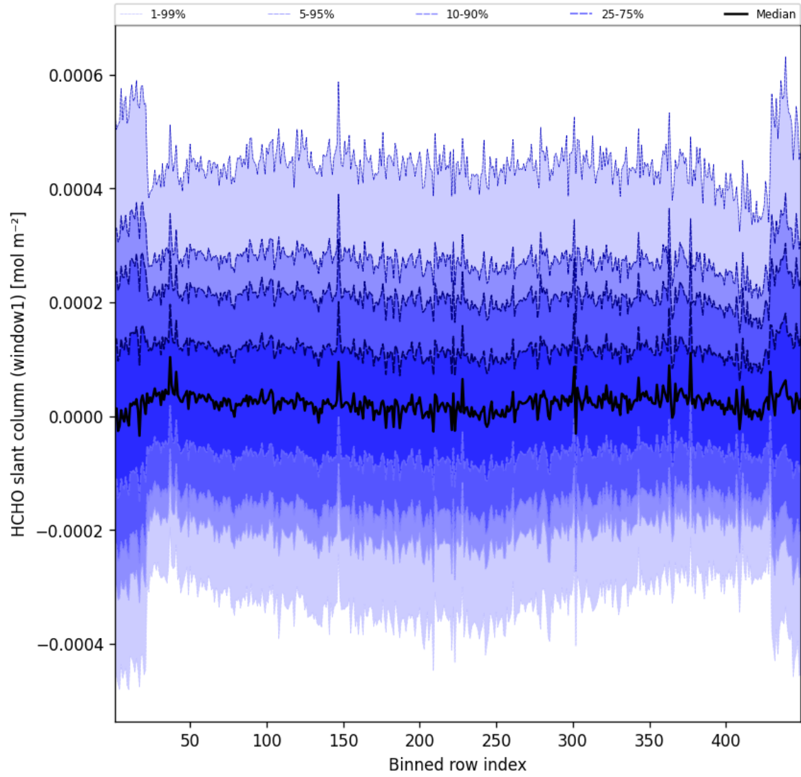
Figure 50: Along track statistics of “HCHO slant column (window1)” for 2025-08-09 to 2025-08-10
