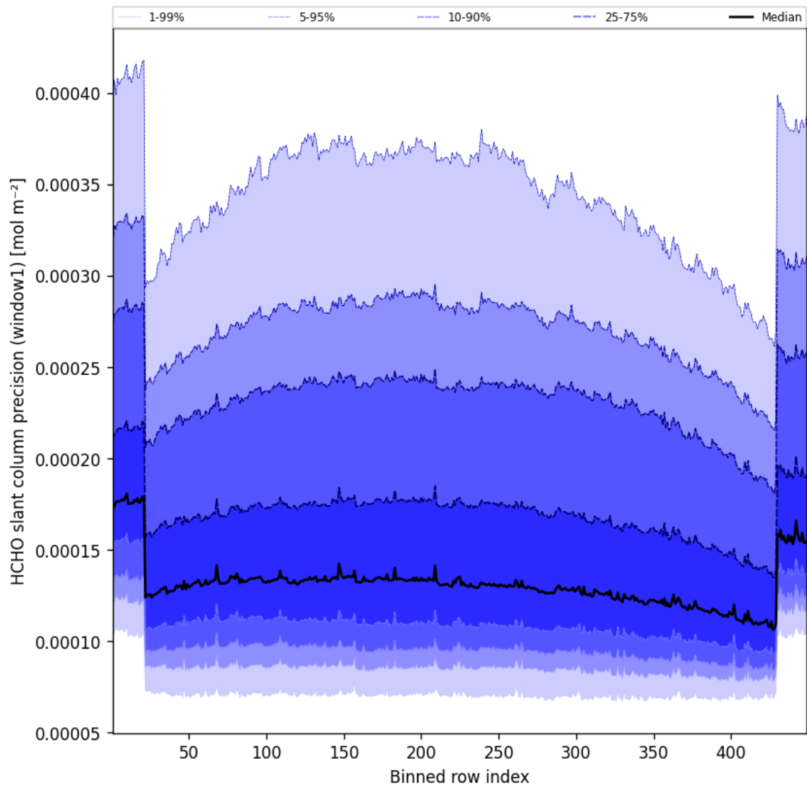
Figure 51: Along track statistics of “HCHO slant column precision (window1)” for 2025-08-09 to 2025-08-10
