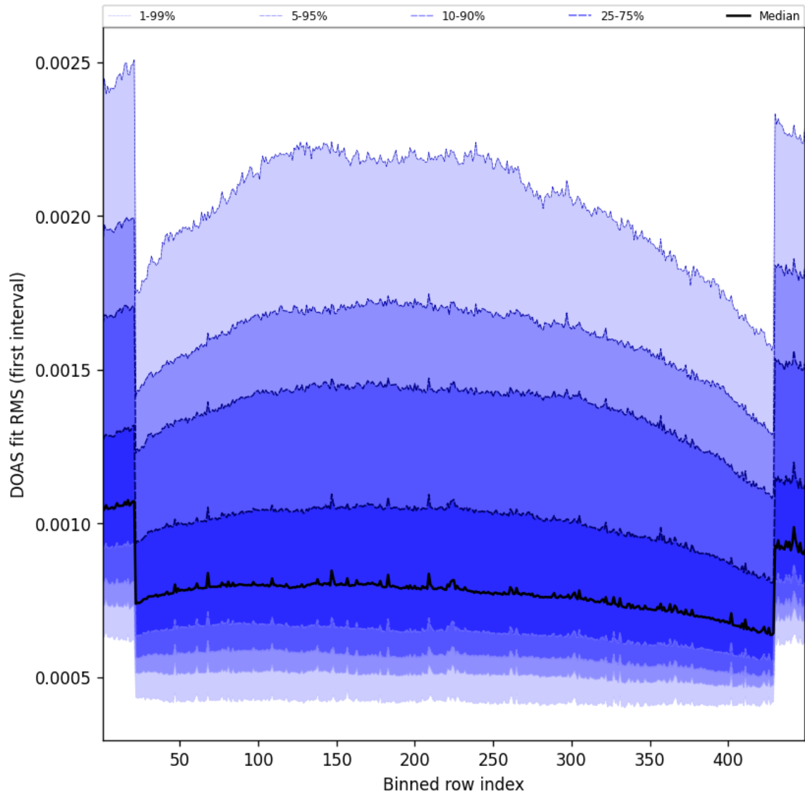
Figure 58: Along track statistics of “DOAS fit RMS (first interval)” for 2025-08-09 to 2025-08-10
