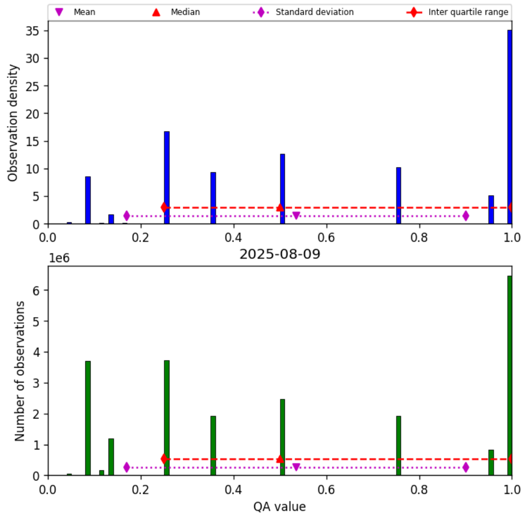
Figure 32: Histogram of “QA value” for 2025-08-09 to 2025-08-10
