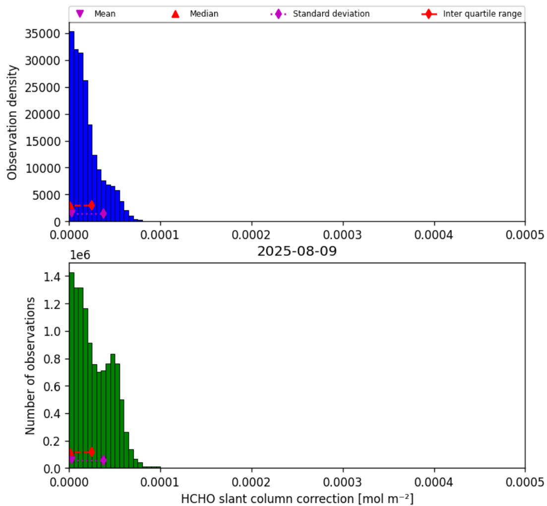
Figure 45: Histogram of “HCHO slant column correction” for 2025-08-09 to 2025-08-10
