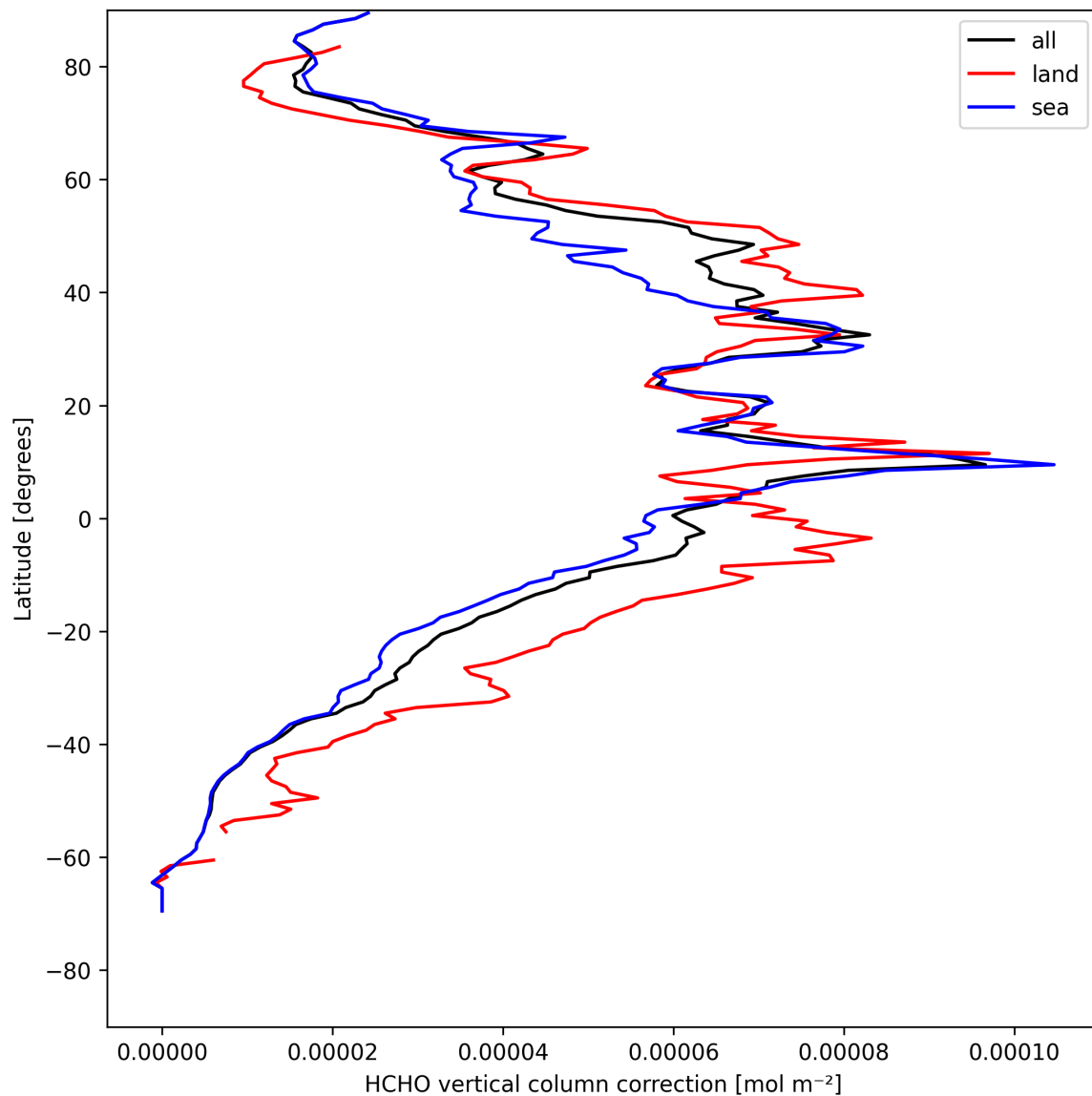
Figure 21: Zonal average of “HCHO vertical column correction” for 2025-08-09 to 2025-08-10.
