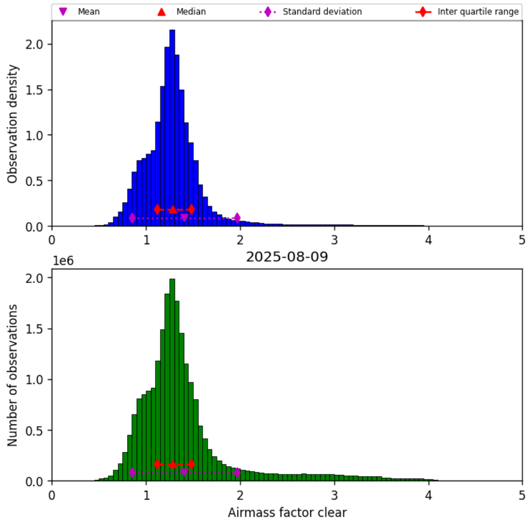
Figure 40: Histogram of “Airmass factor clear” for 2025-08-09 to 2025-08-10
