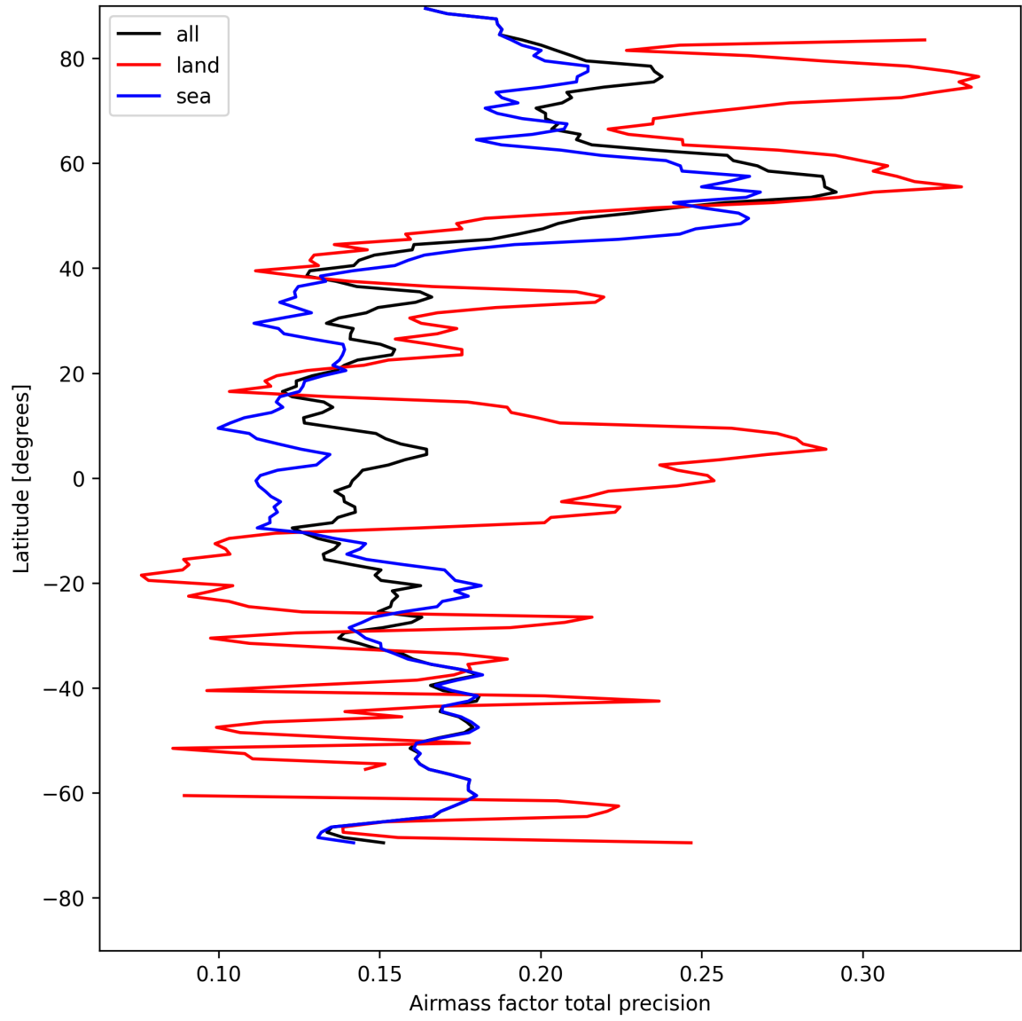
Figure 25: Zonal average of “Airmass factor total precision” for 2025-08-09 to 2025-08-10.
