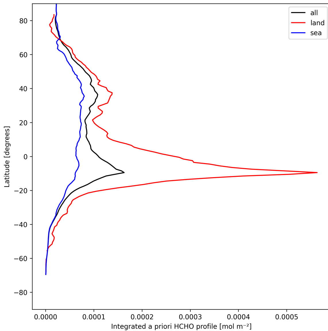
Figure 27: Zonal average of “Integrated a priori HCHO profile” for 2025-08-09 to 2025-08-10.
