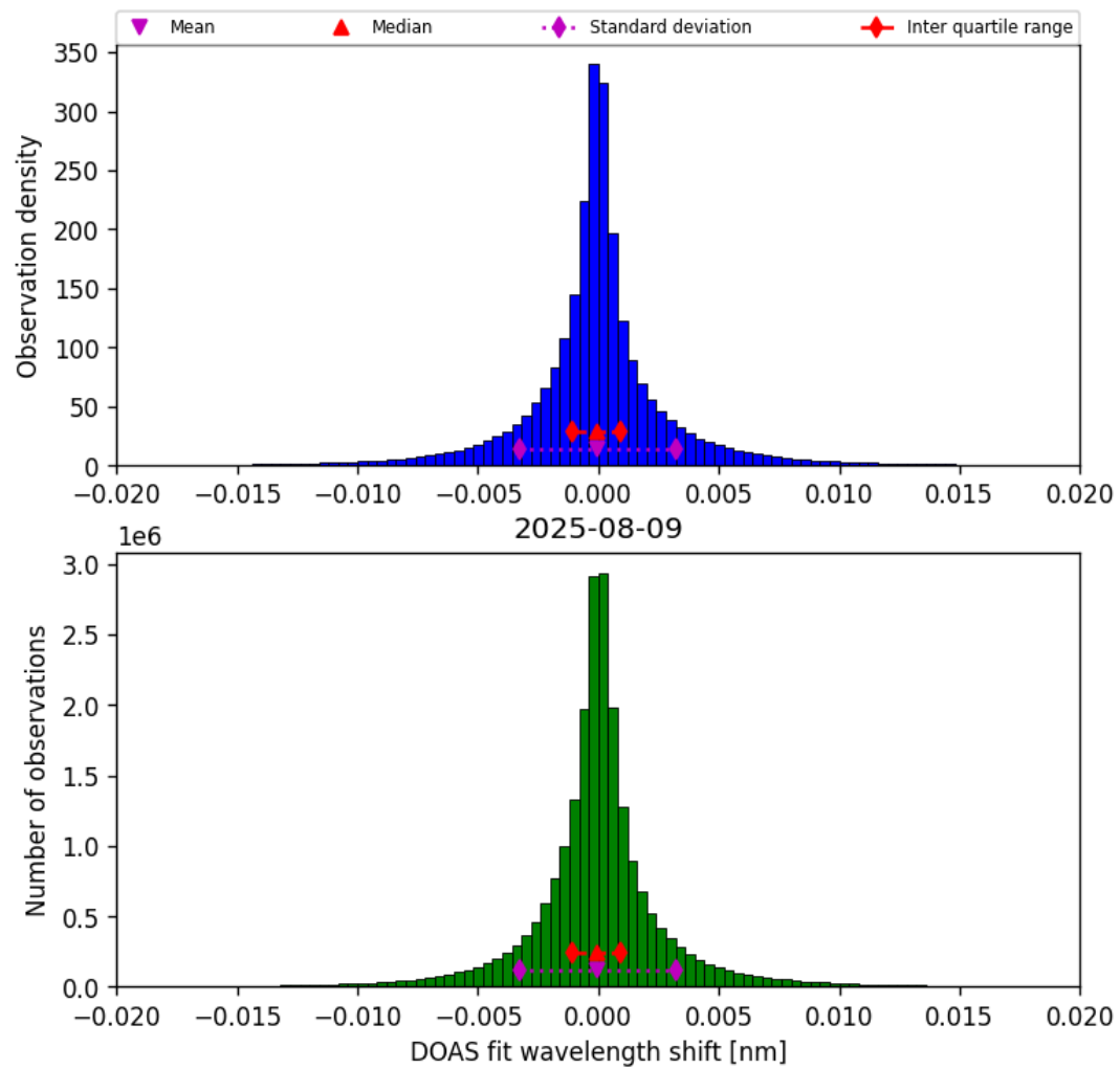
Figure 42: Histogram of “DOAS fit wavelength shift” for 2025-08-09 to 2025-08-10
