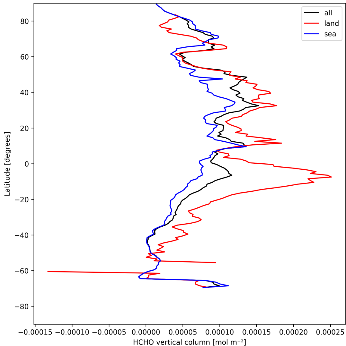
Figure 19: Zonal average of “HCHO vertical column” for 2025-08-09 to 2025-08-10.
