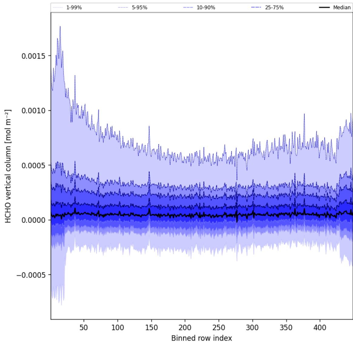
Figure 47: Along track statistics of “HCHO vertical column” for 2025-08-09 to 2025-08-10
