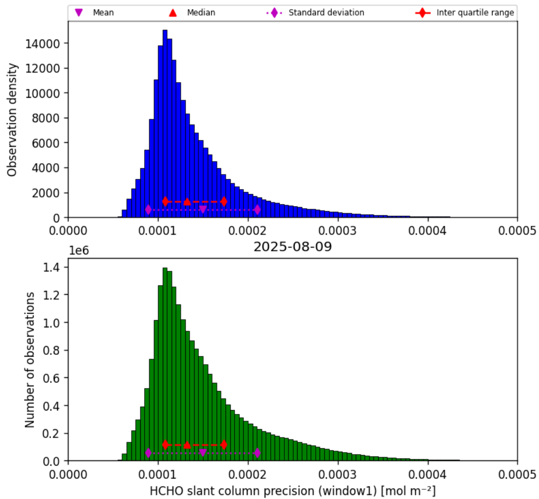
Figure 37: Histogram of “HCHO slant column precision (window1)” for 2025-08-09 to 2025-08-10
