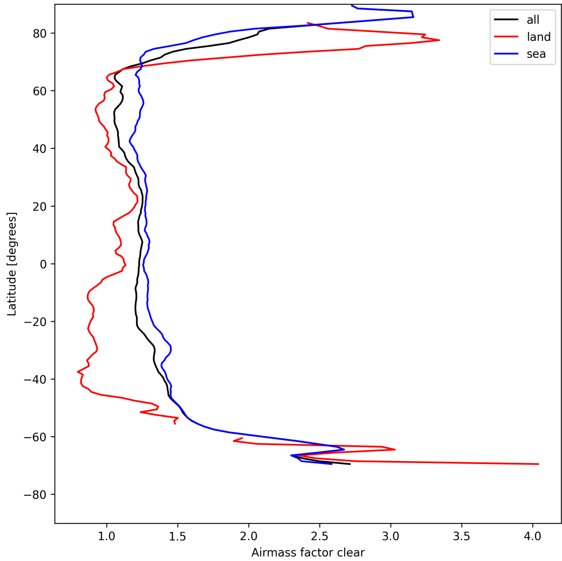
Figure 26: Zonal average of “Airmass factor clear” for 2025-08-09 to 2025-08-10.
