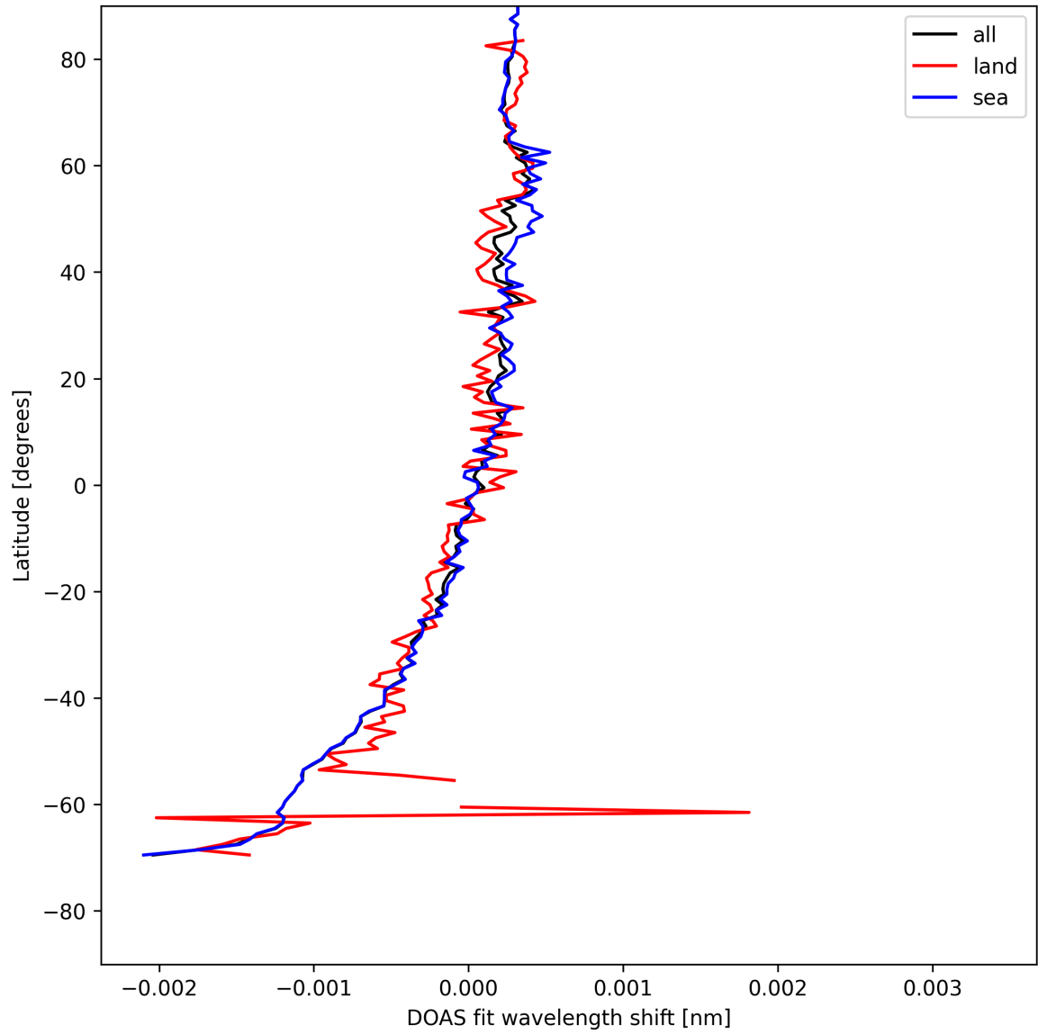
Figure 28: Zonal average of "DOAS fit wavelength shift" for 2025-08-09 to 2025-08-10.
