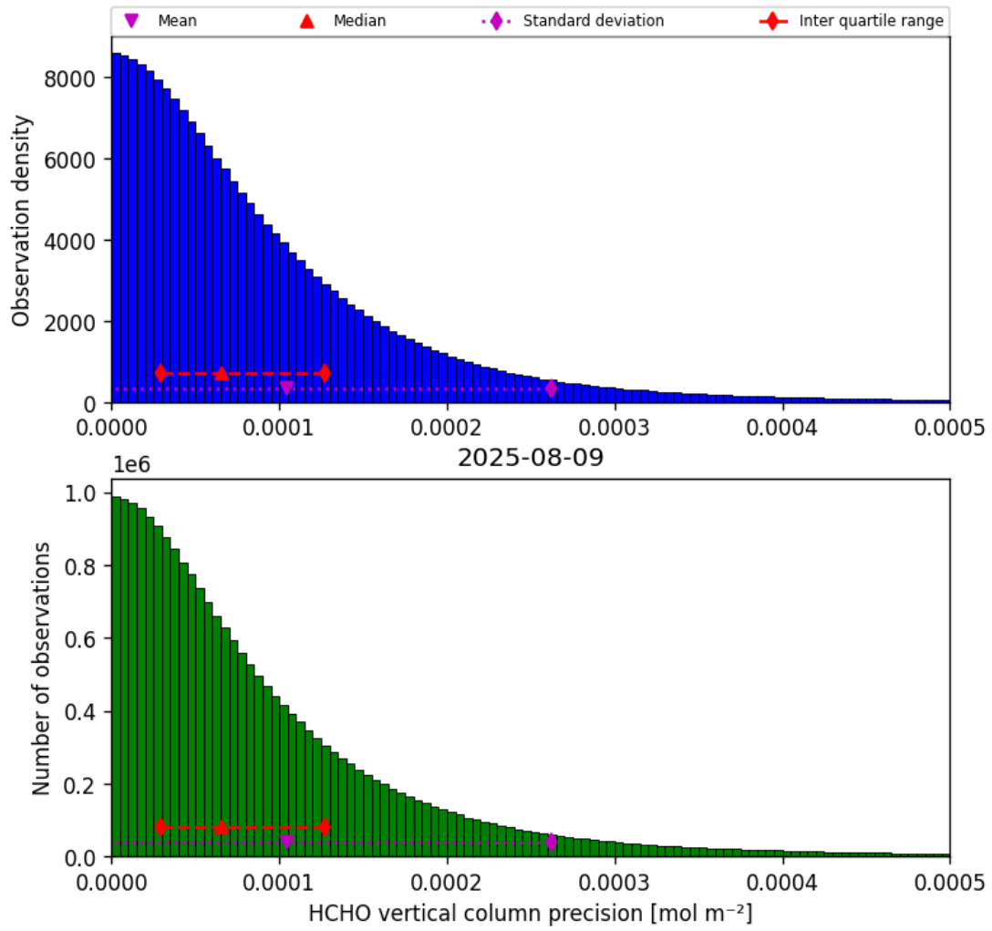
Figure 34: Histogram of “HCHO vertical column precision” for 2025-08-09 to 2025-08-10
