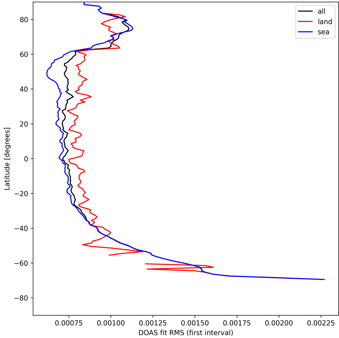
Figure 30: Zonal average of "DOAS fit RMS (first interval)" for 2025-08-09 to 2025-08-10.
