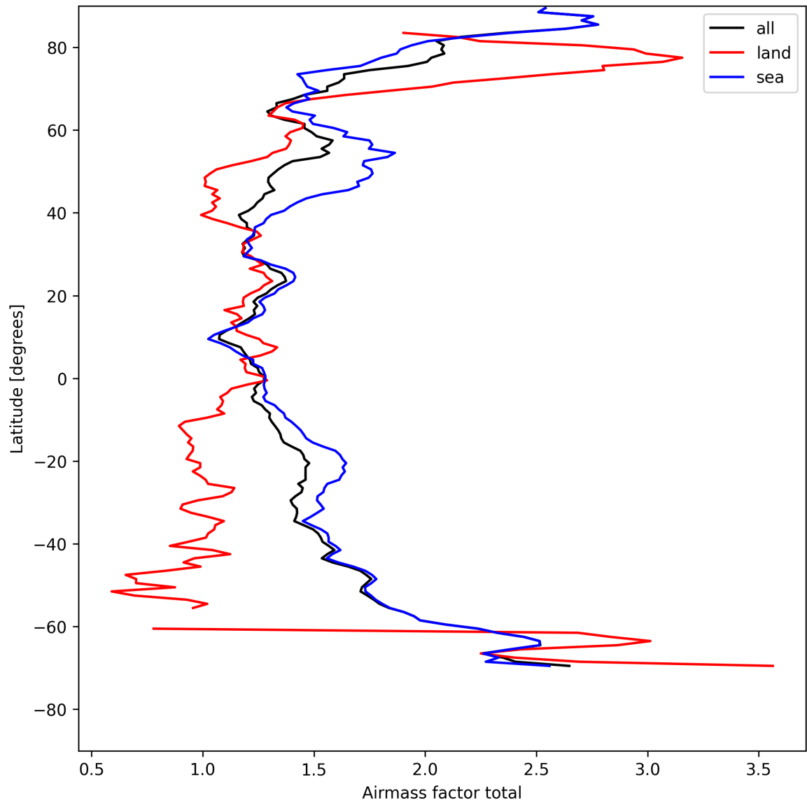
Figure 24: Zonal average of “Airmass factor total” for 2025-08-09 to 2025-08-10.
