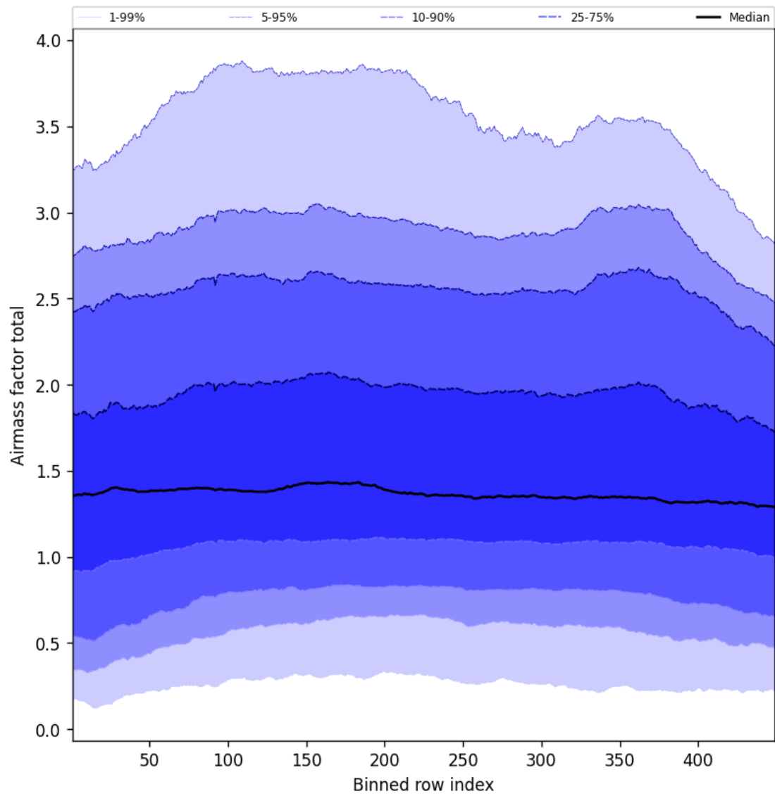
Figure 52: Along track statistics of “Airmass factor total” for 2025-08-09 to 2025-08-10
