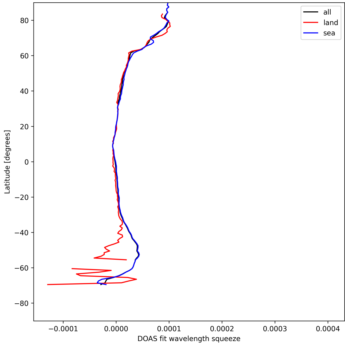
Figure 29: Zonal average of “DOAS fit wavelength squeeze” for 2025-08-09 to 2025-08-10.
