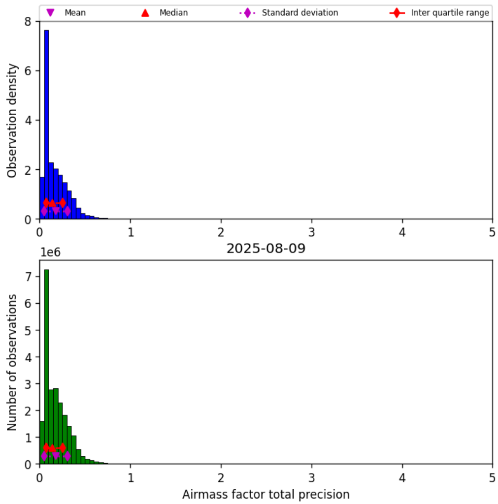
Figure 39: Histogram of “Airmass factor total precision” for 2025-08-09 to 2025-08-10
