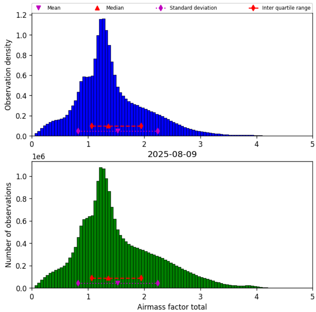
Figure 38: Histogram of “Airmass factor total” for 2025-08-09 to 2025-08-10
