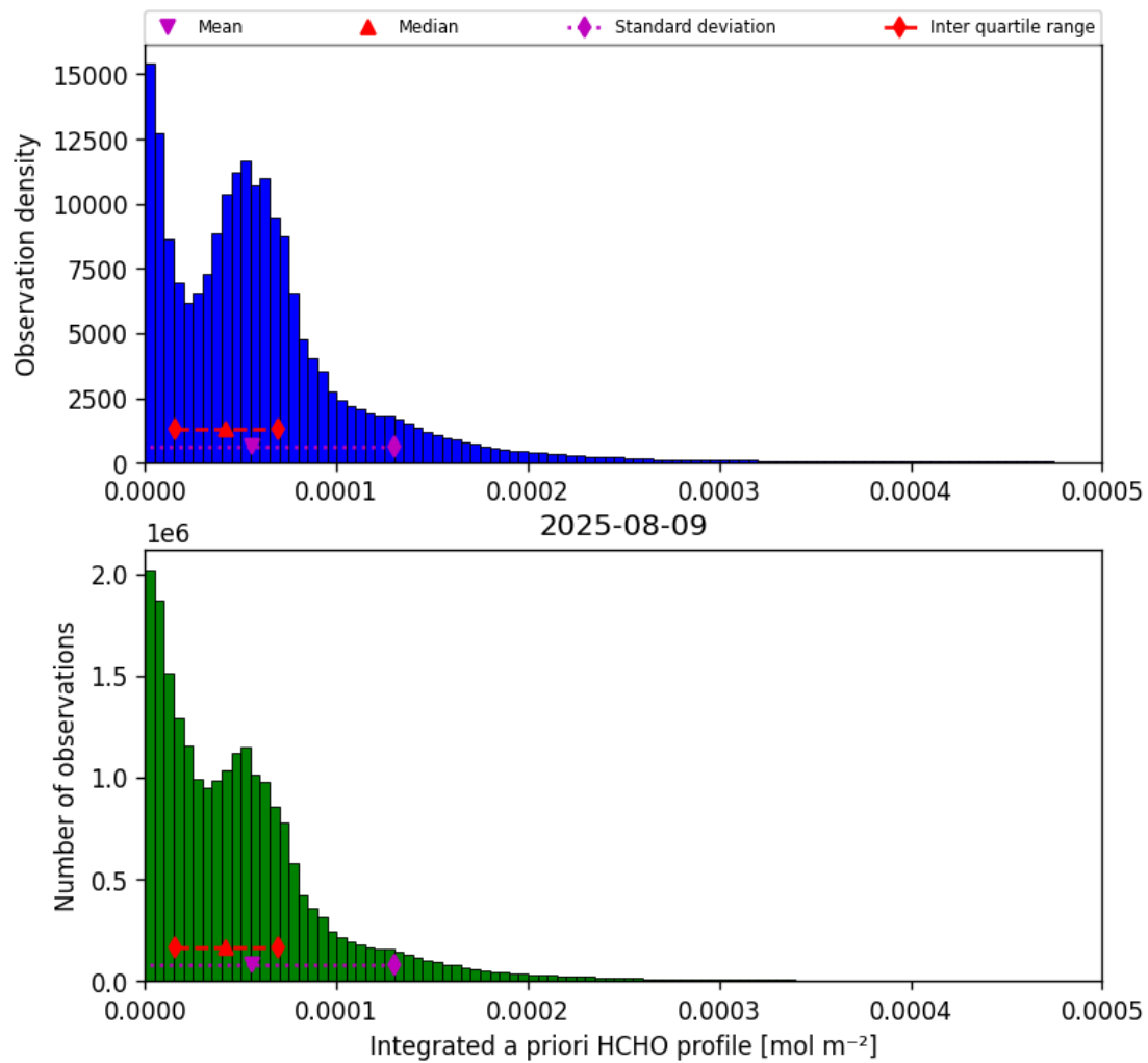
Figure 41: Histogram of “Integrated a priori HCHO profile” for 2025-08-09 to 2025-08-10
