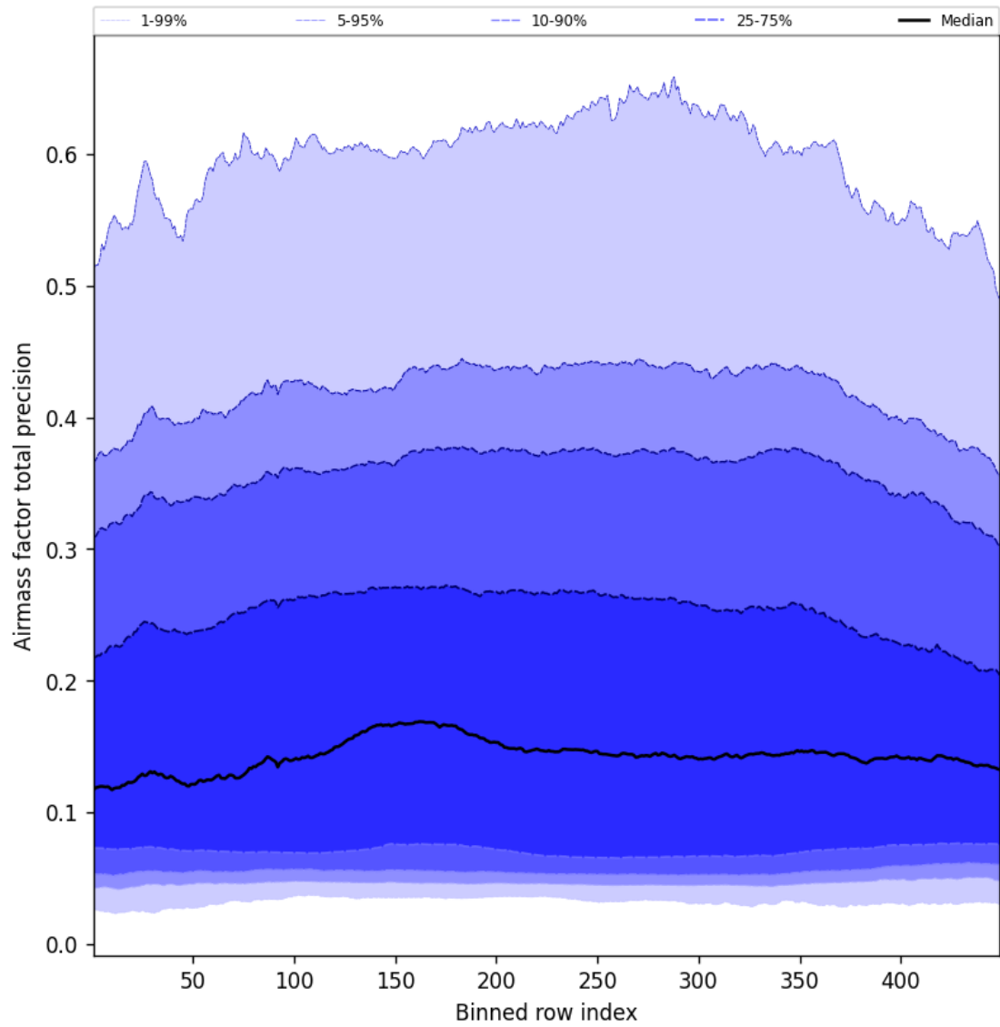
Figure 53: Along track statistics of “Airmass factor total precision” for 2025-08-09 to 2025-08-10
