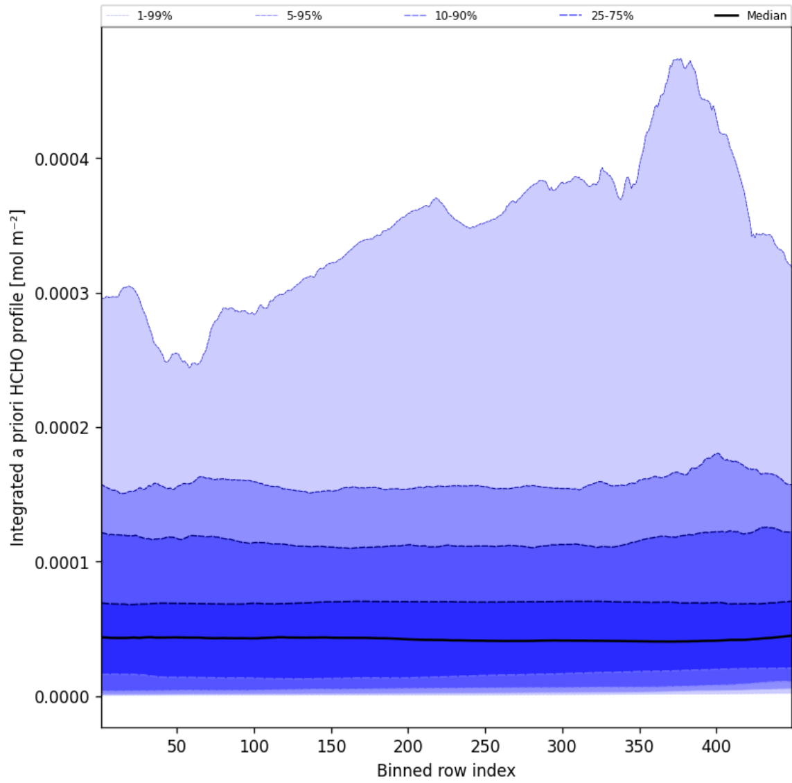
Figure 55: Along track statistics of “Integrated a priori HCHO profile” for 2025-08-09 to 2025-08-10
