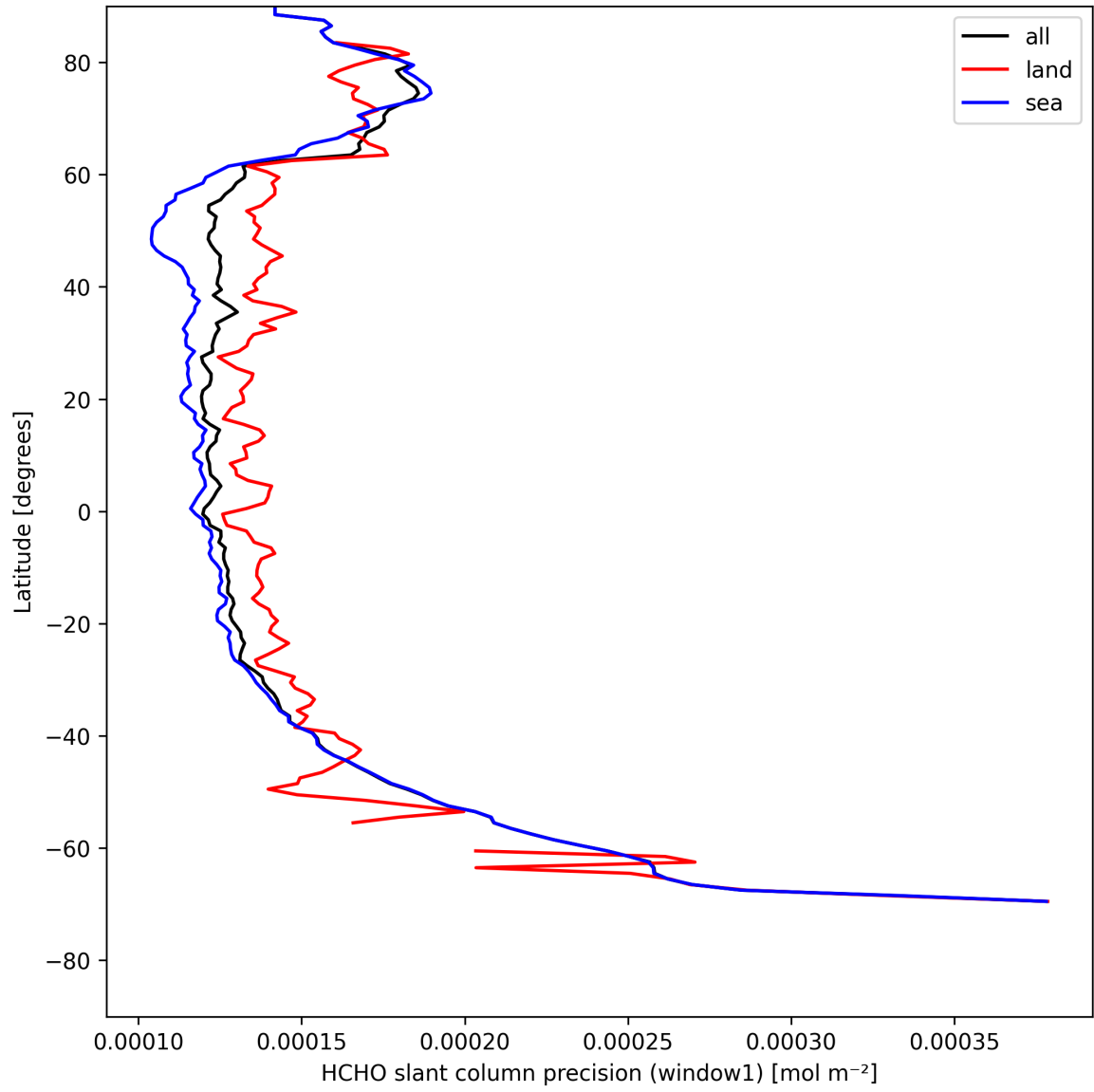
Figure 23: Zonal average of “HCHO slant column precision (window1)” for 2025-08-09 to 2025-08-10.
