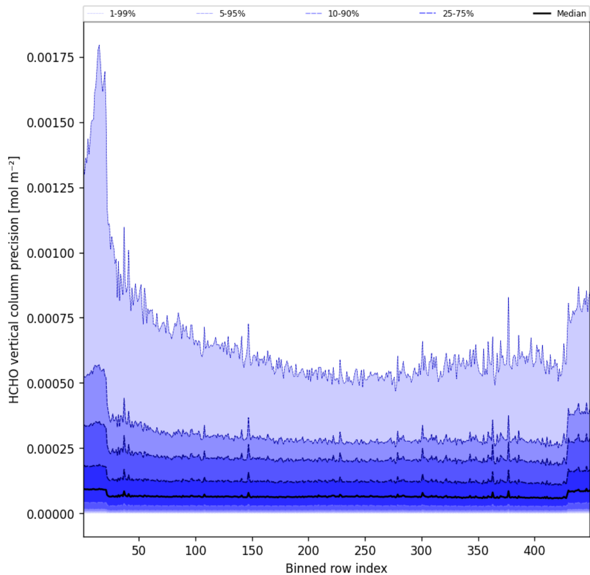
Figure 48: Along track statistics of “HCHO vertical column precision” for 2025-08-09 to 2025-08-10
