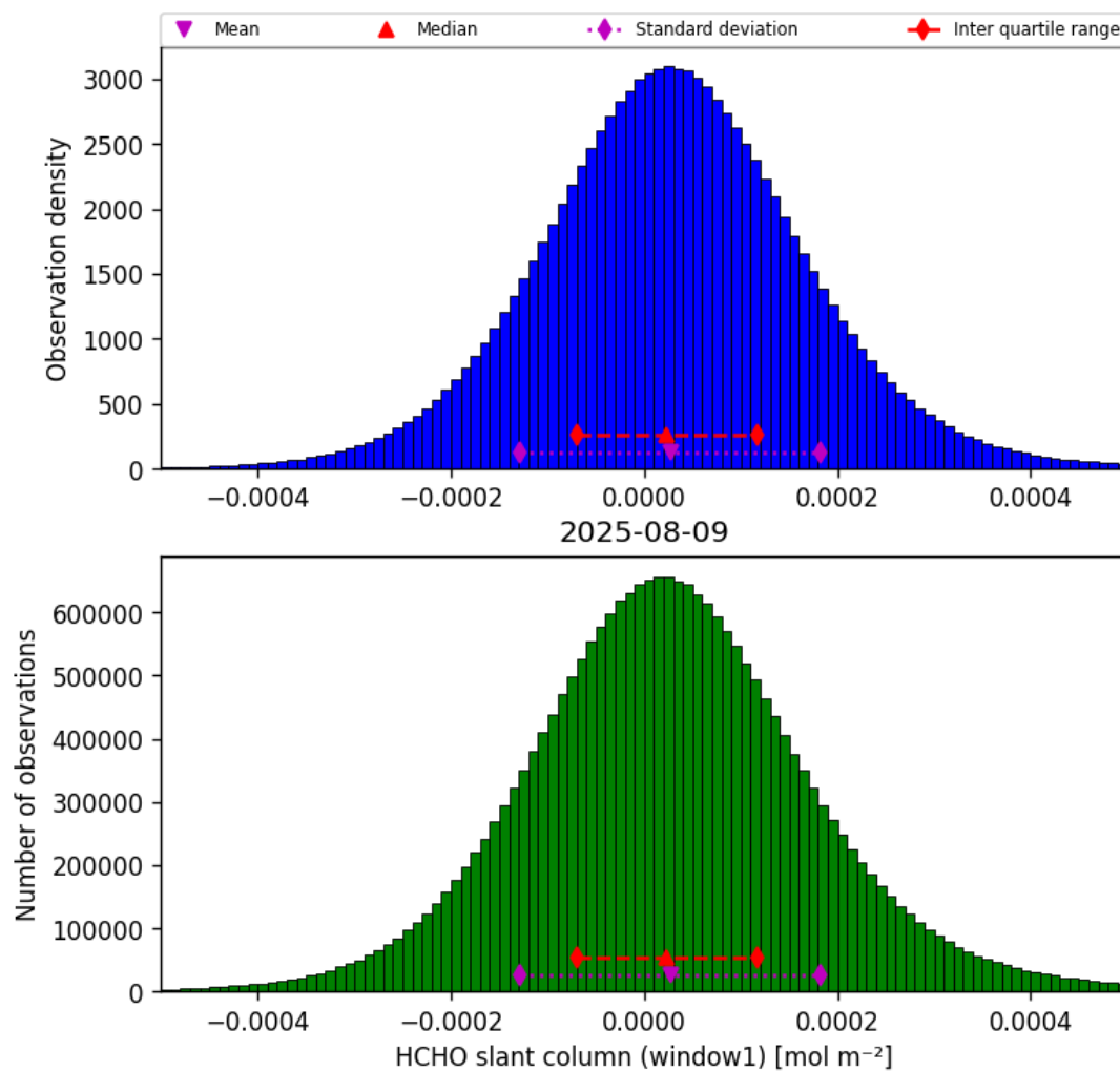
Figure 36: Histogram of “HCHO slant column (window1)” for 2025-08-09 to 2025-08-10
