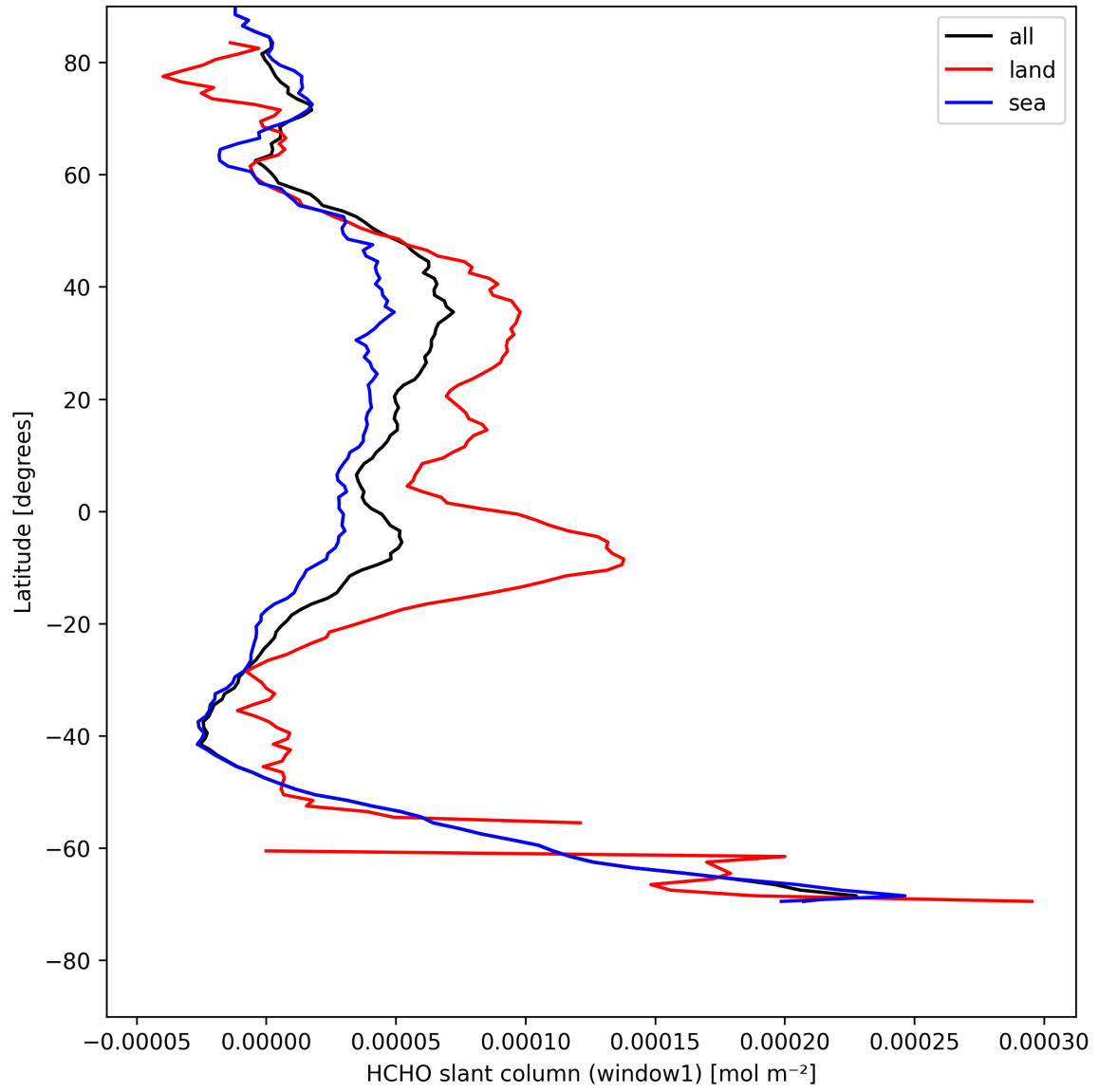
Figure 22: Zonal average of “HCHO slant column (window1)” for 2025-08-09 to 2025-08-10.
