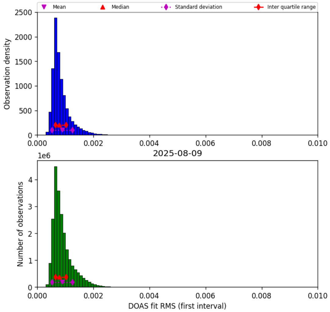
Figure 44: Histogram of “DOAS fit RMS (first interval)” for 2025-08-09 to 2025-08-10
