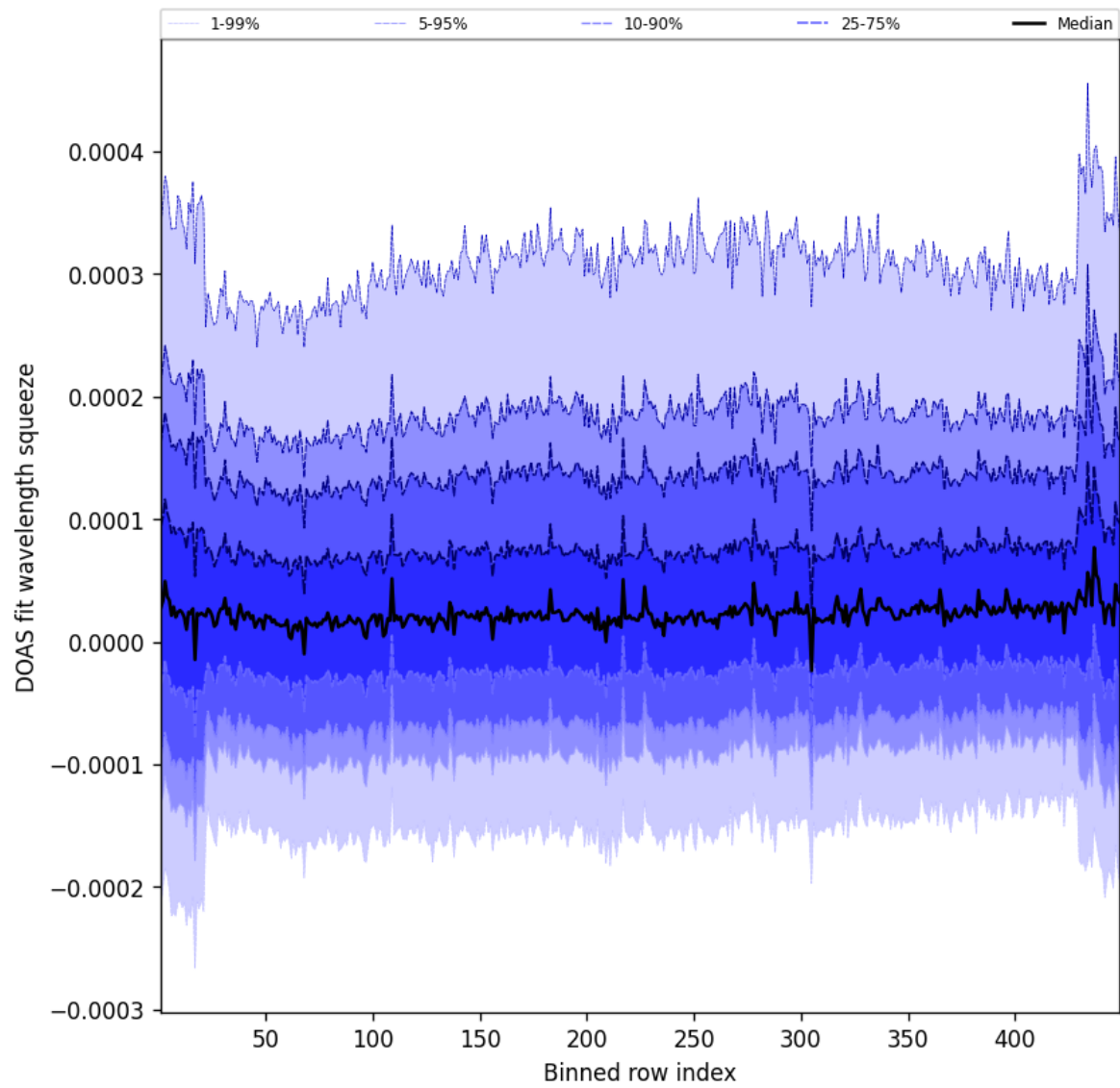
Figure 57: Along track statistics of “DOAS fit wavelength squeeze” for 2025-08-09 to 2025-08-10
