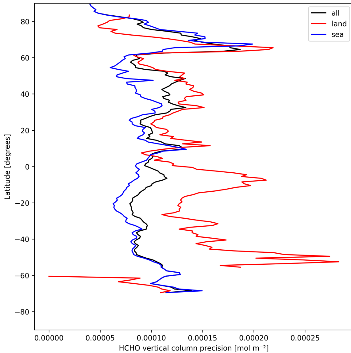
Figure 20: Zonal average of “HCHO vertical column precision” for 2025-08-09 to 2025-08-10.
