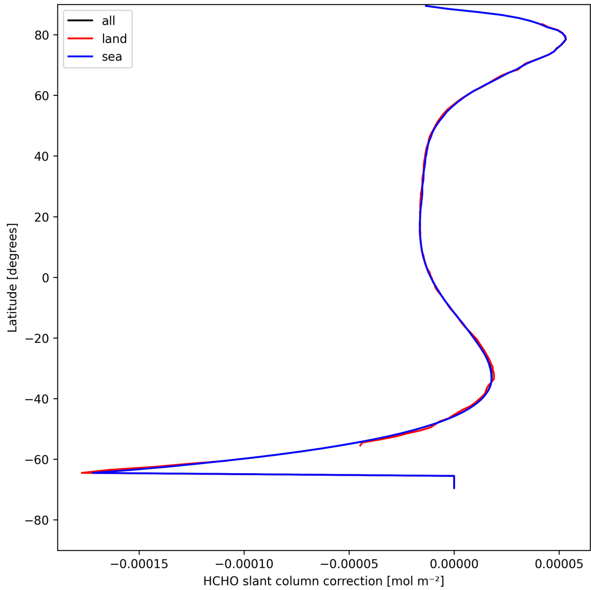
Figure 31: Zonal average of “HCHO slant column correction” for 2025-08-09 to 2025-08-10.
