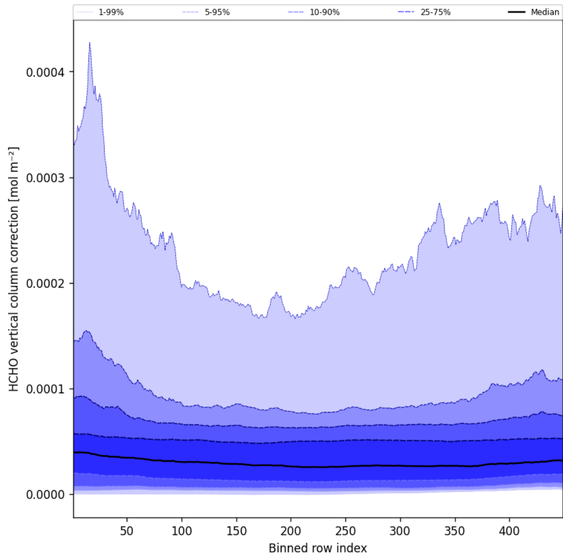
Figure 49: Along track statistics of “HCHO vertical column correction” for 2025-08-09 to 2025-08-10
