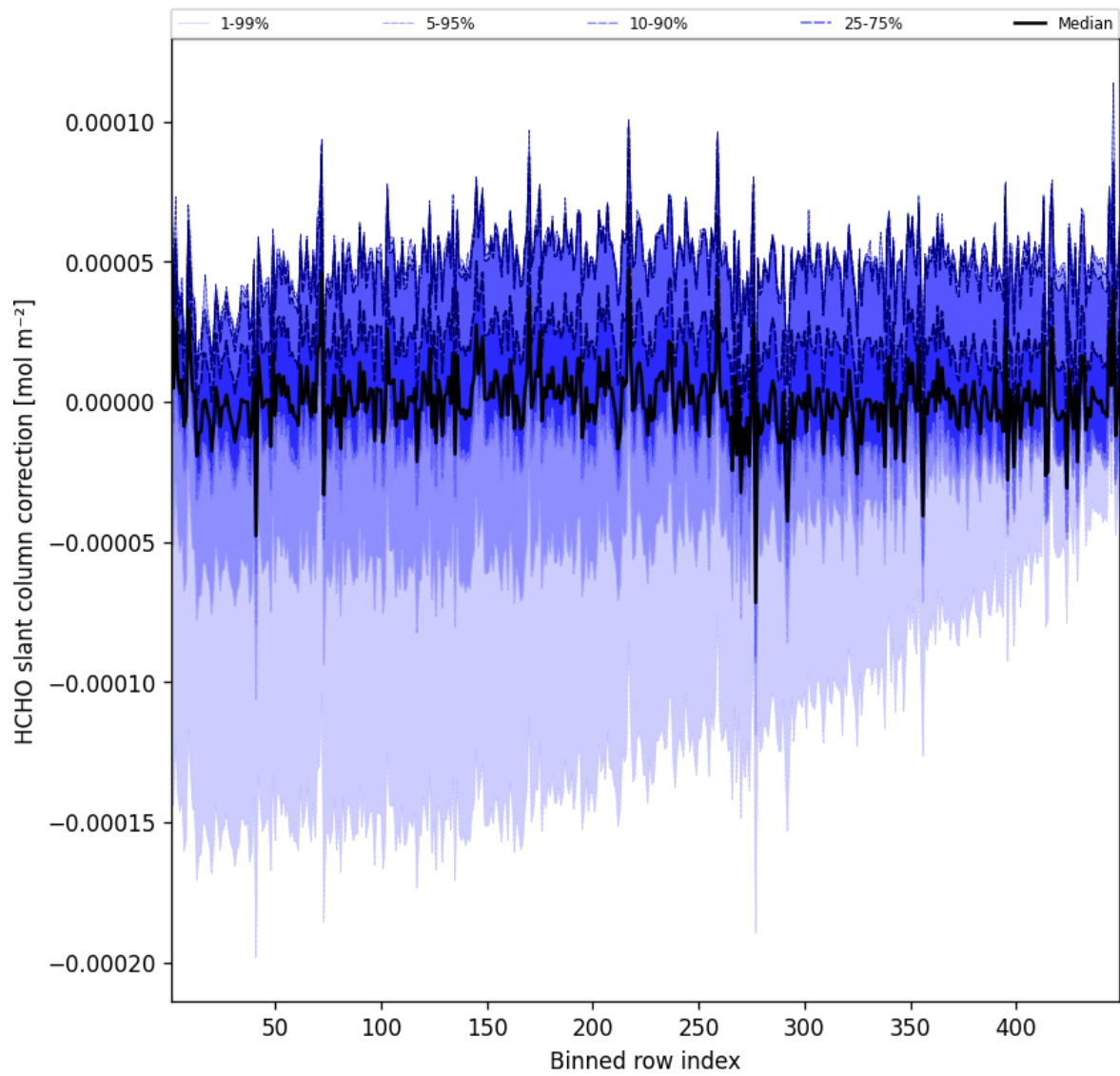
Figure 59: Along track statistics of “HCHO slant column correction” for 2025-08-09 to 2025-08-10
