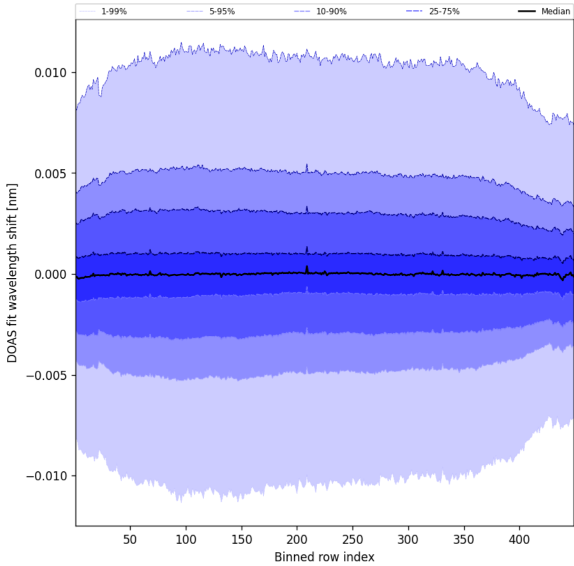
Figure 56: Along track statistics of “DOAS fit wavelength shift” for 2025-08-09 to 2025-08-10
