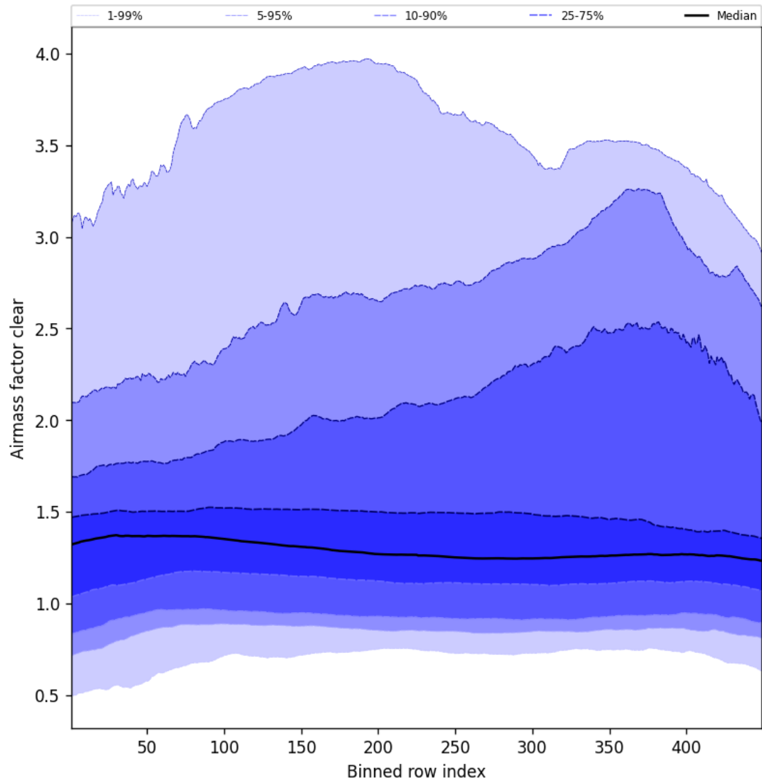
Figure 54: Along track statistics of “Airmass factor clear” for 2025-08-09 to 2025-08-10
