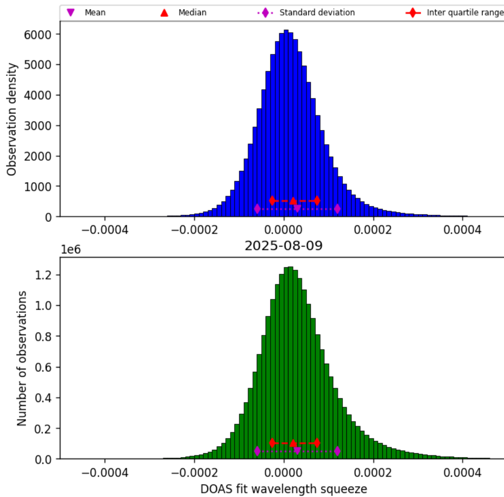
Figure 43: Histogram of “DOAS fit wavelength squeeze” for 2025-08-09 to 2025-08-10
