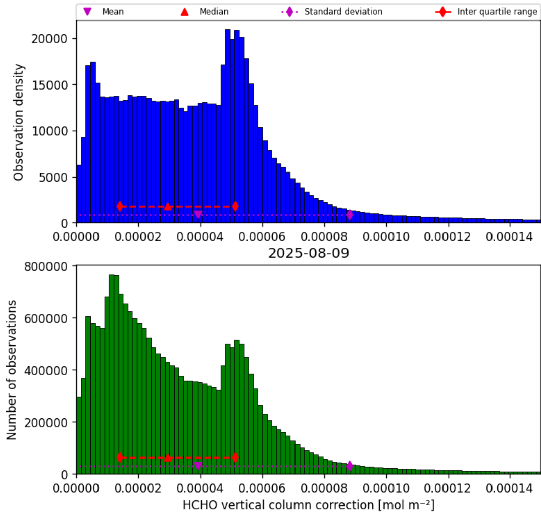
Figure 35: Histogram of “HCHO vertical column correction” for 2025-08-09 to 2025-08-10
