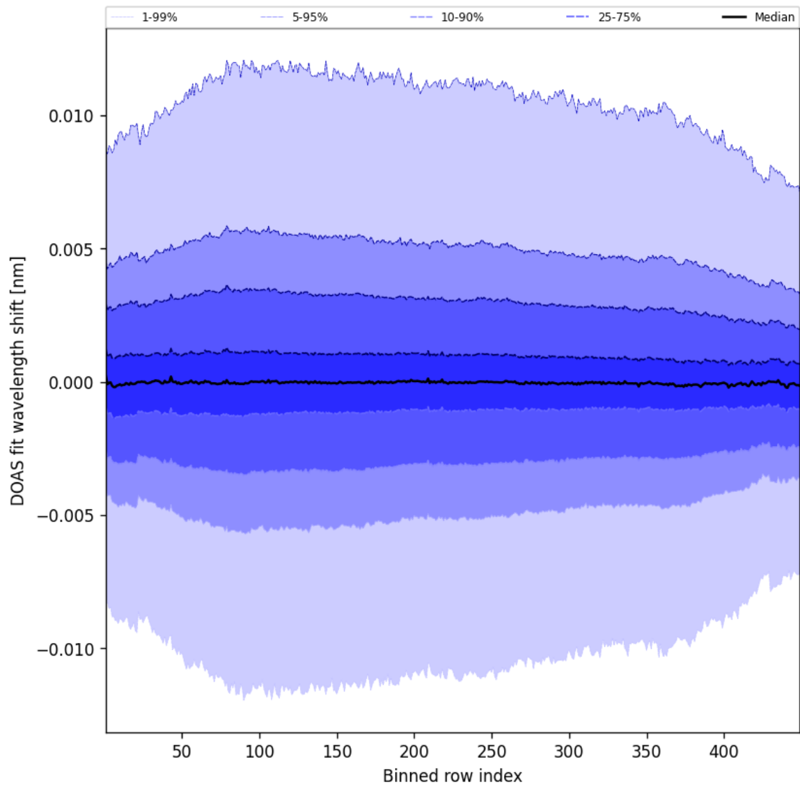
Figure 56: Along track statistics of “DOAS fit wavelength shift” for 2025-08-12 to 2025-08-12
