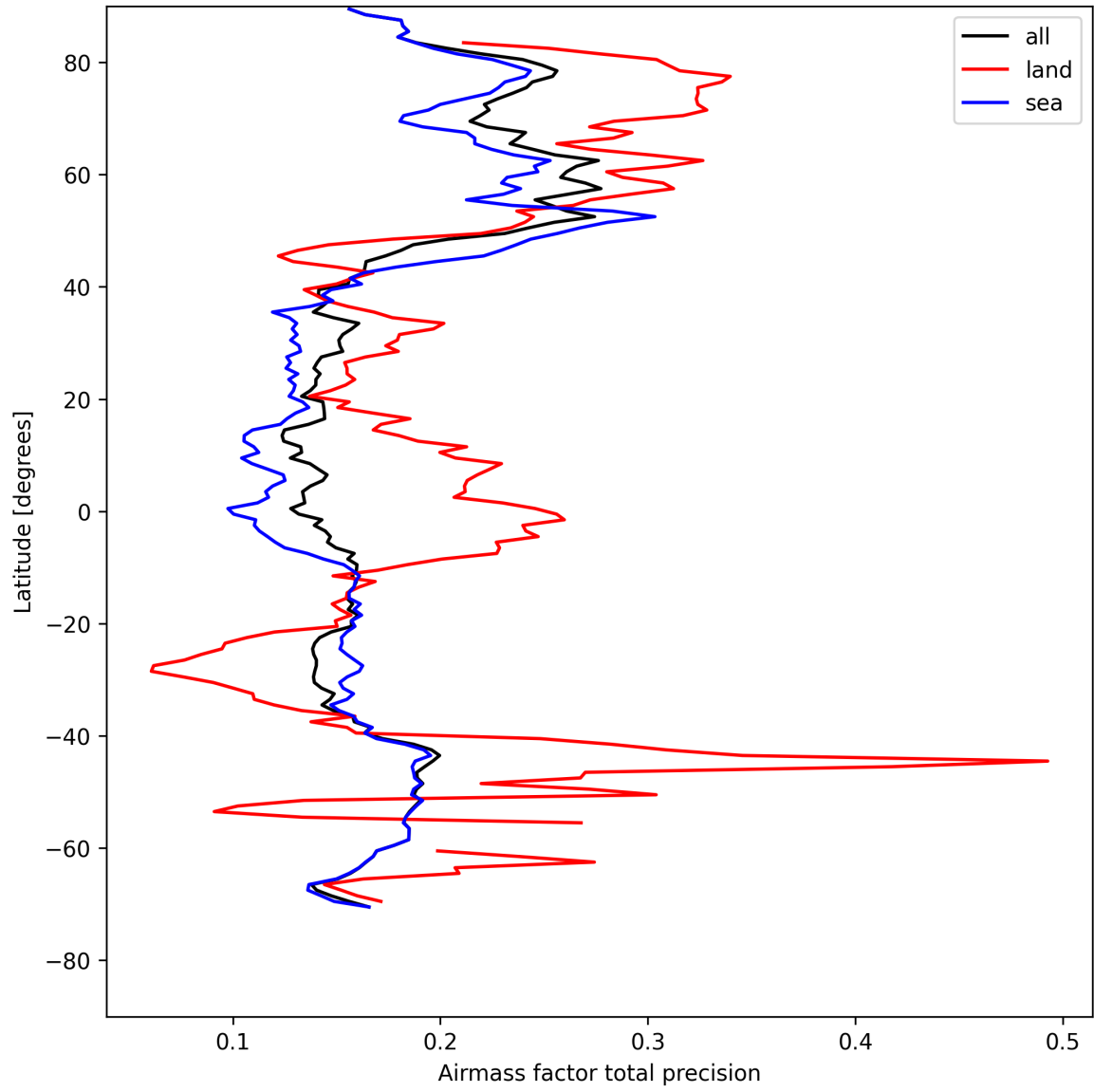
Figure 25: Zonal average of “Airmass factor total precision” for 2025-08-12 to 2025-08-12.
