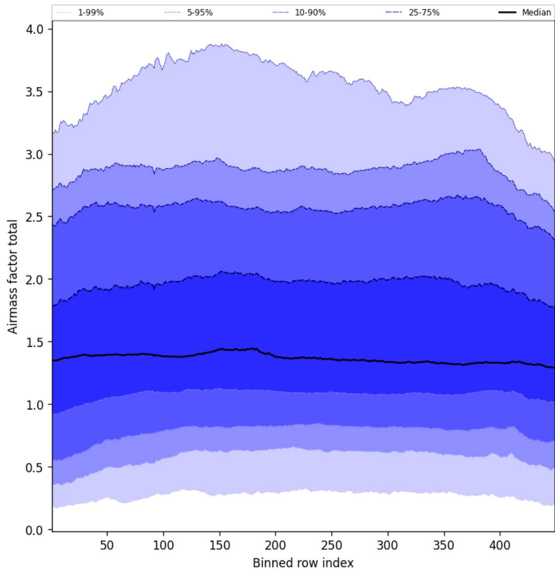
Figure 52: Along track statistics of “Airmass factor total” for 2025-08-12 to 2025-08-12
