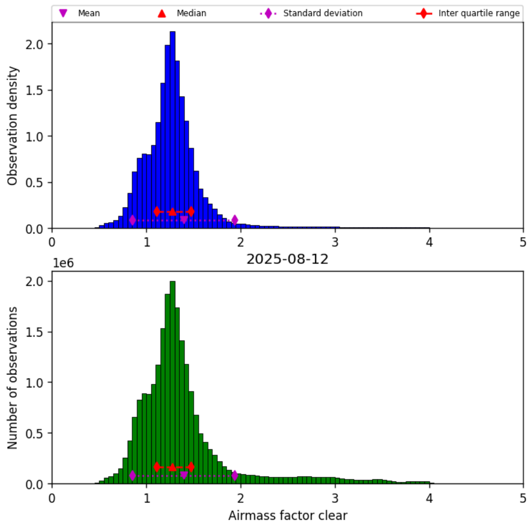
Figure 40: Histogram of “Airmass factor clear” for 2025-08-12 to 2025-08-12
