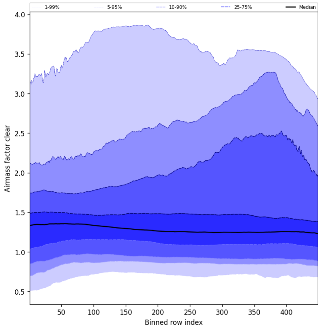
Figure 54: Along track statistics of “Airmass factor clear” for 2025-08-12 to 2025-08-12
