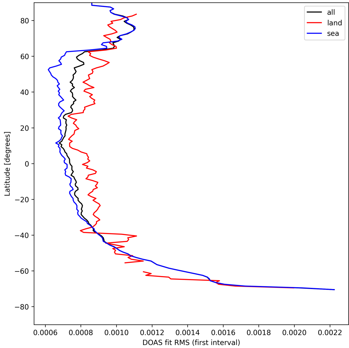
Figure 30: Zonal average of "DOAS fit RMS (first interval)" for 2025-08-12 to 2025-08-12.
