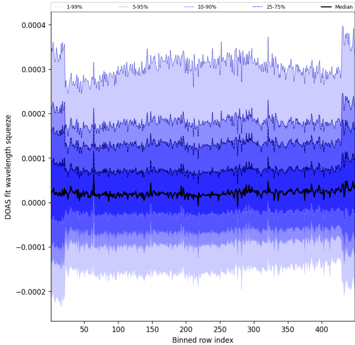
Figure 57: Along track statistics of “DOAS fit wavelength squeeze” for 2025-08-12 to 2025-08-12
