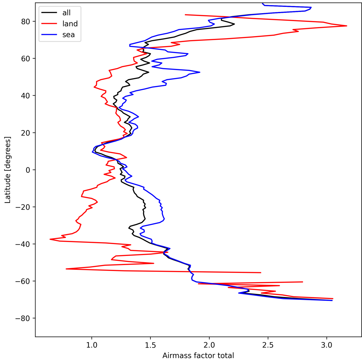
Figure 24: Zonal average of “Airmass factor total” for 2025-08-12 to 2025-08-12.
