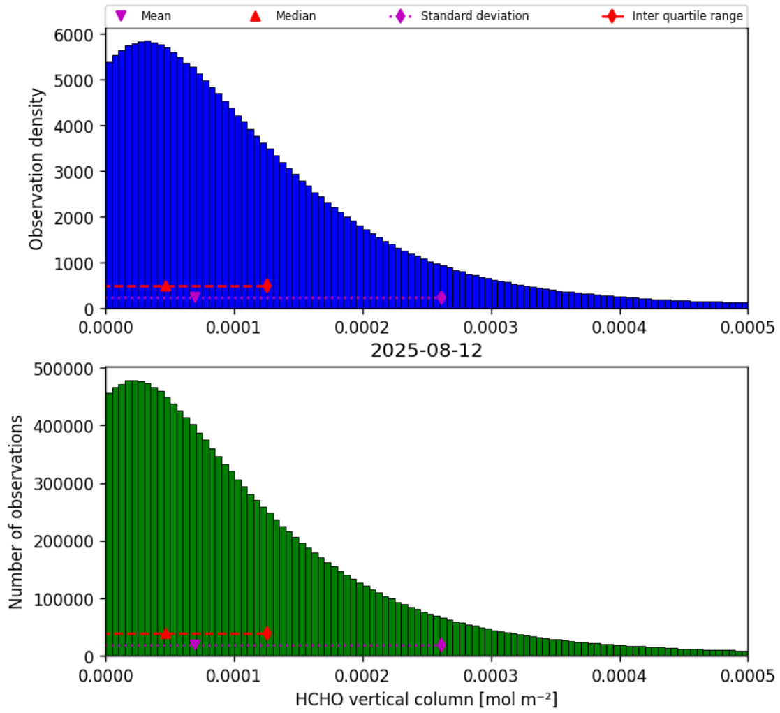
Figure 33: Histogram of “HCHO vertical column” for 2025-08-12 to 2025-08-12
