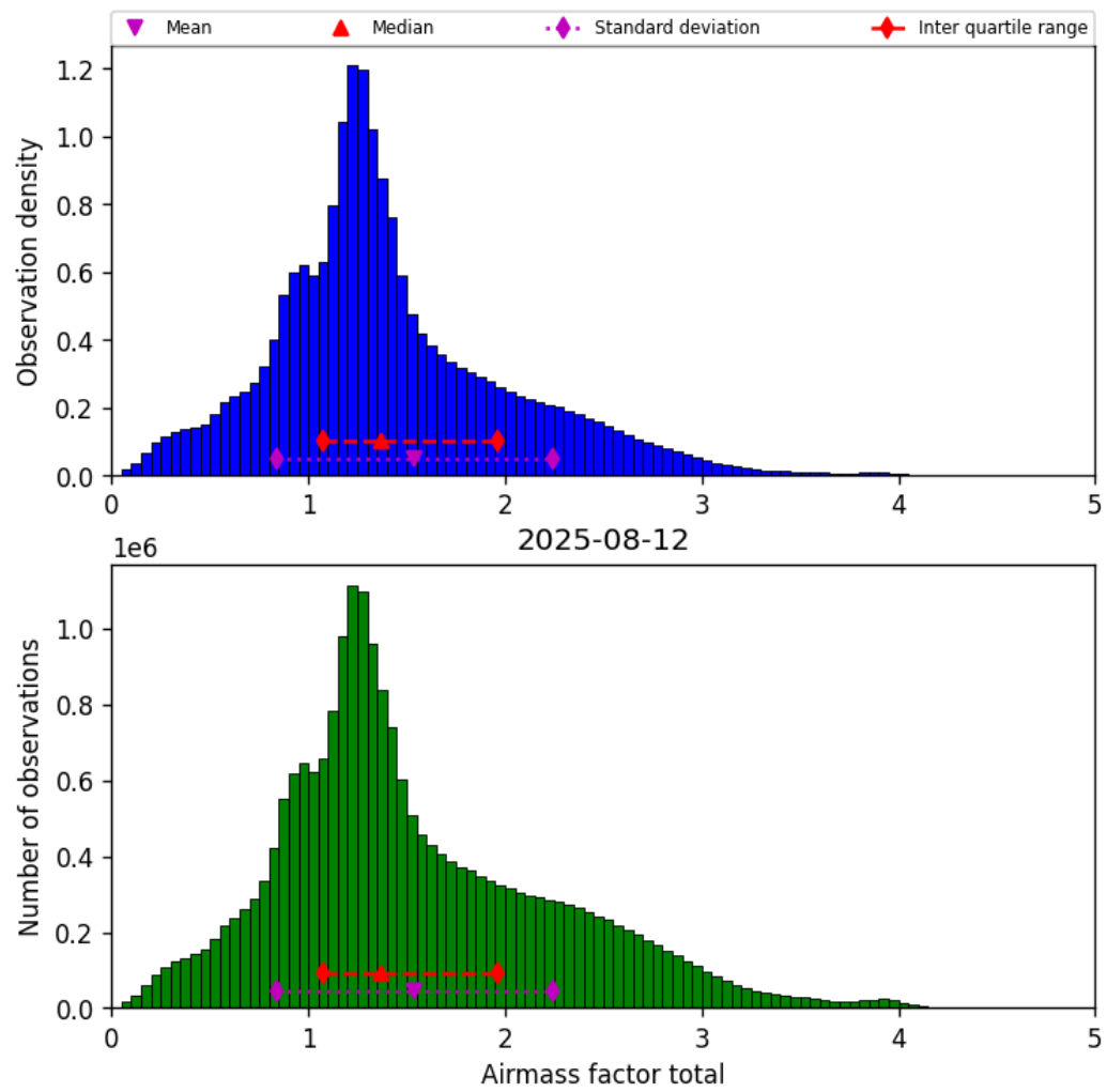
Figure 38: Histogram of “Airmass factor total” for 2025-08-12 to 2025-08-12
