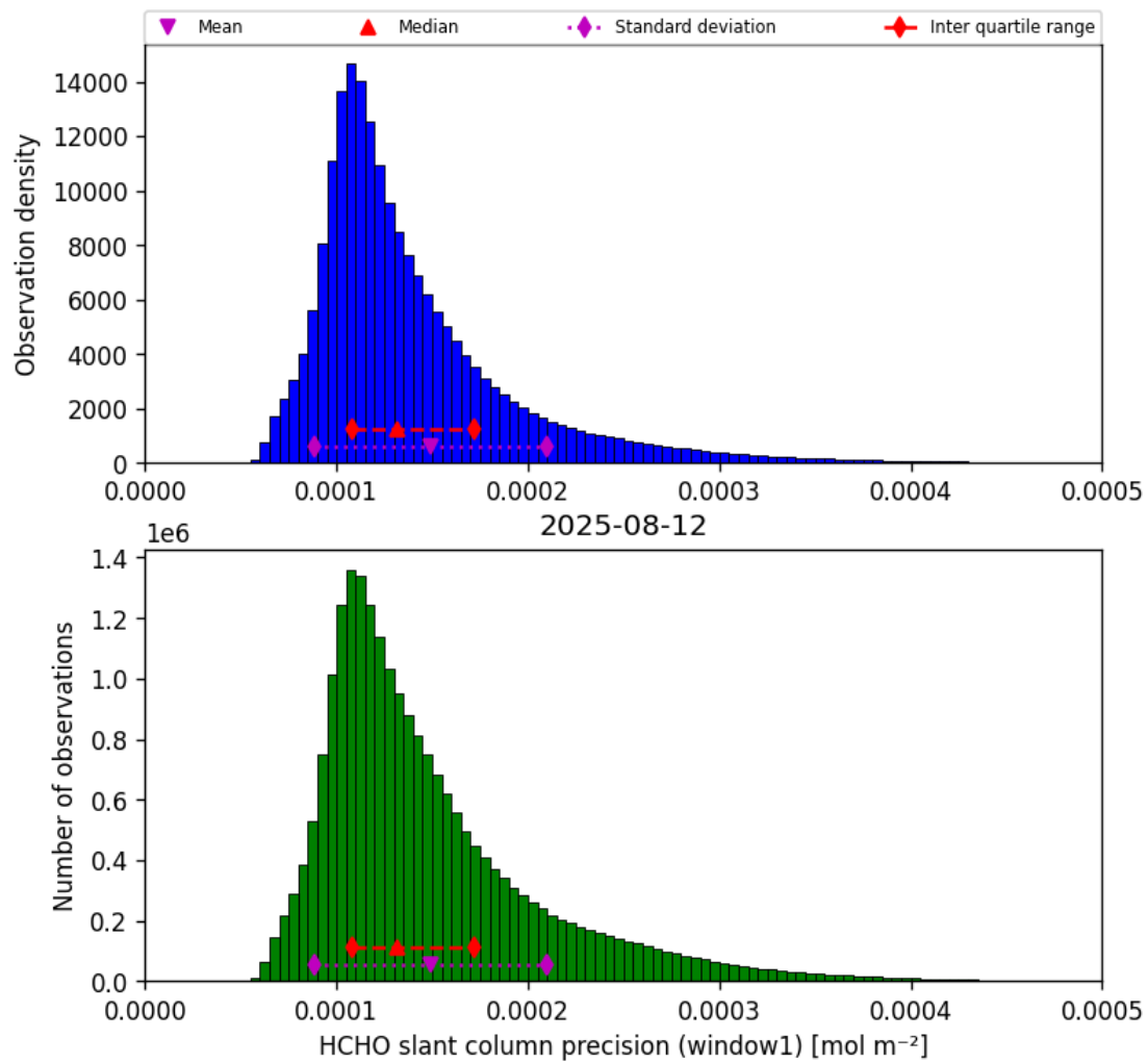
Figure 37: Histogram of “HCHO slant column precision (window1)” for 2025-08-12 to 2025-08-12
