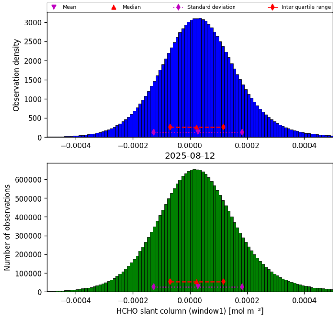
Figure 36: Histogram of “HCHO slant column (window1)” for 2025-08-12 to 2025-08-12
