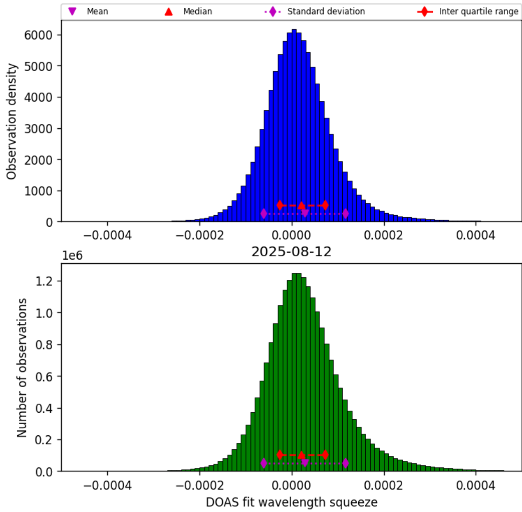
Figure 43: Histogram of “DOAS fit wavelength squeeze” for 2025-08-12 to 2025-08-12
