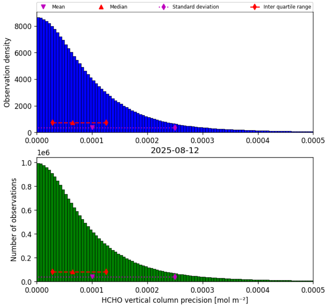
Figure 34: Histogram of “HCHO vertical column precision” for 2025-08-12 to 2025-08-12
