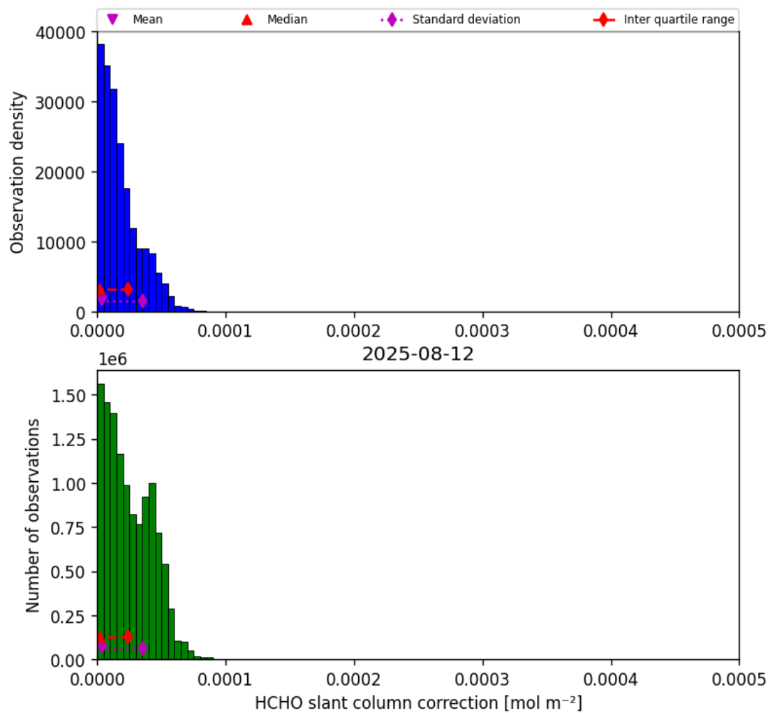
Figure 45: Histogram of “HCHO slant column correction” for 2025-08-12 to 2025-08-12
