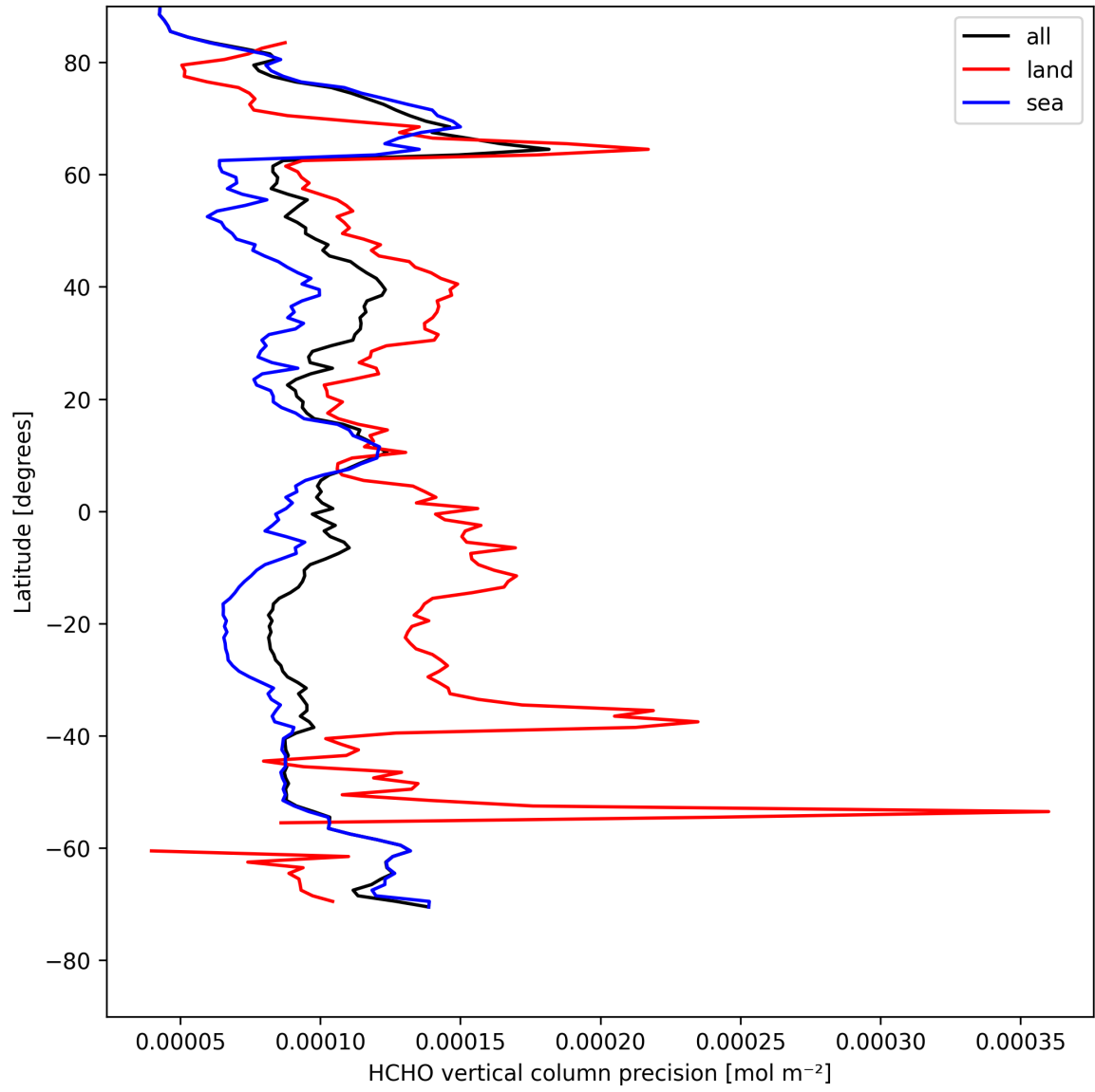
Figure 20: Zonal average of "HCHO vertical column precision" for 2025-08-12 to 2025-08-12.
