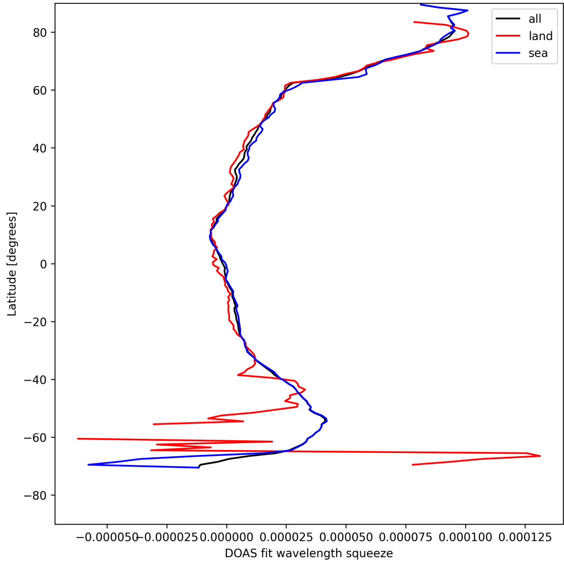
Figure 29: Zonal average of “DOAS fit wavelength squeeze” for 2025-08-12 to 2025-08-12.
