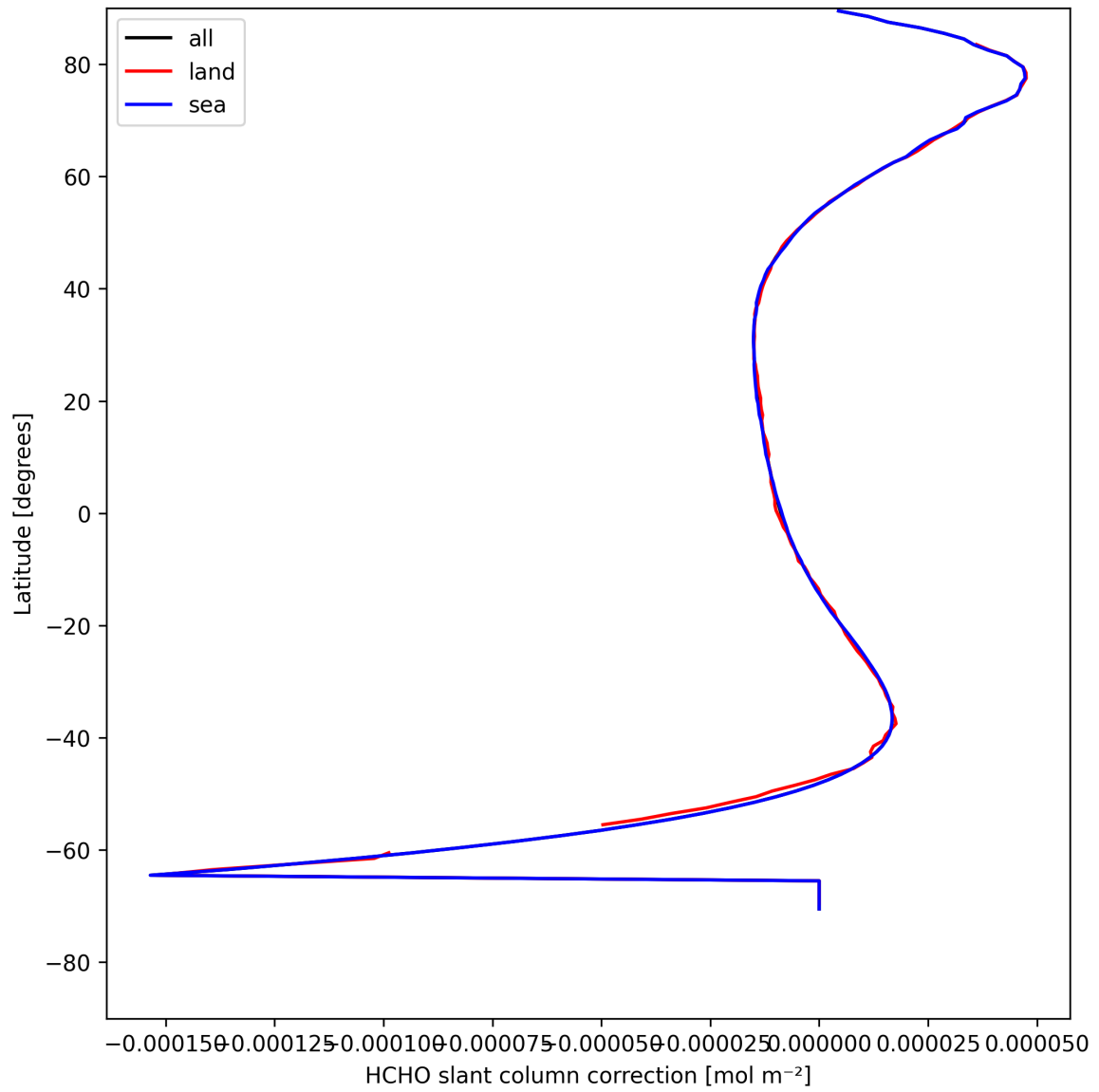
Figure 31: Zonal average of “HCHO slant column correction” for 2025-08-12 to 2025-08-12.
