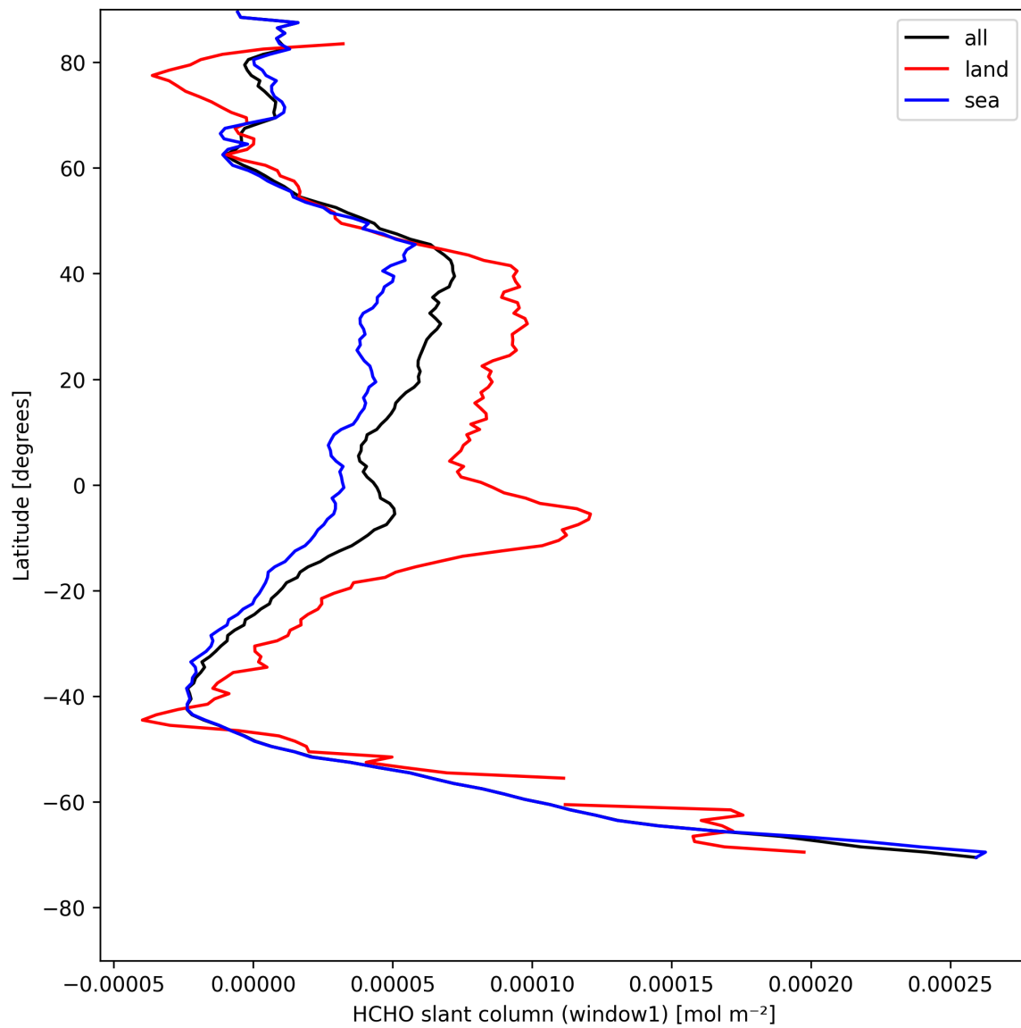
Figure 22: Zonal average of “HCHO slant column (window1)” for 2025-08-12 to 2025-08-12.
