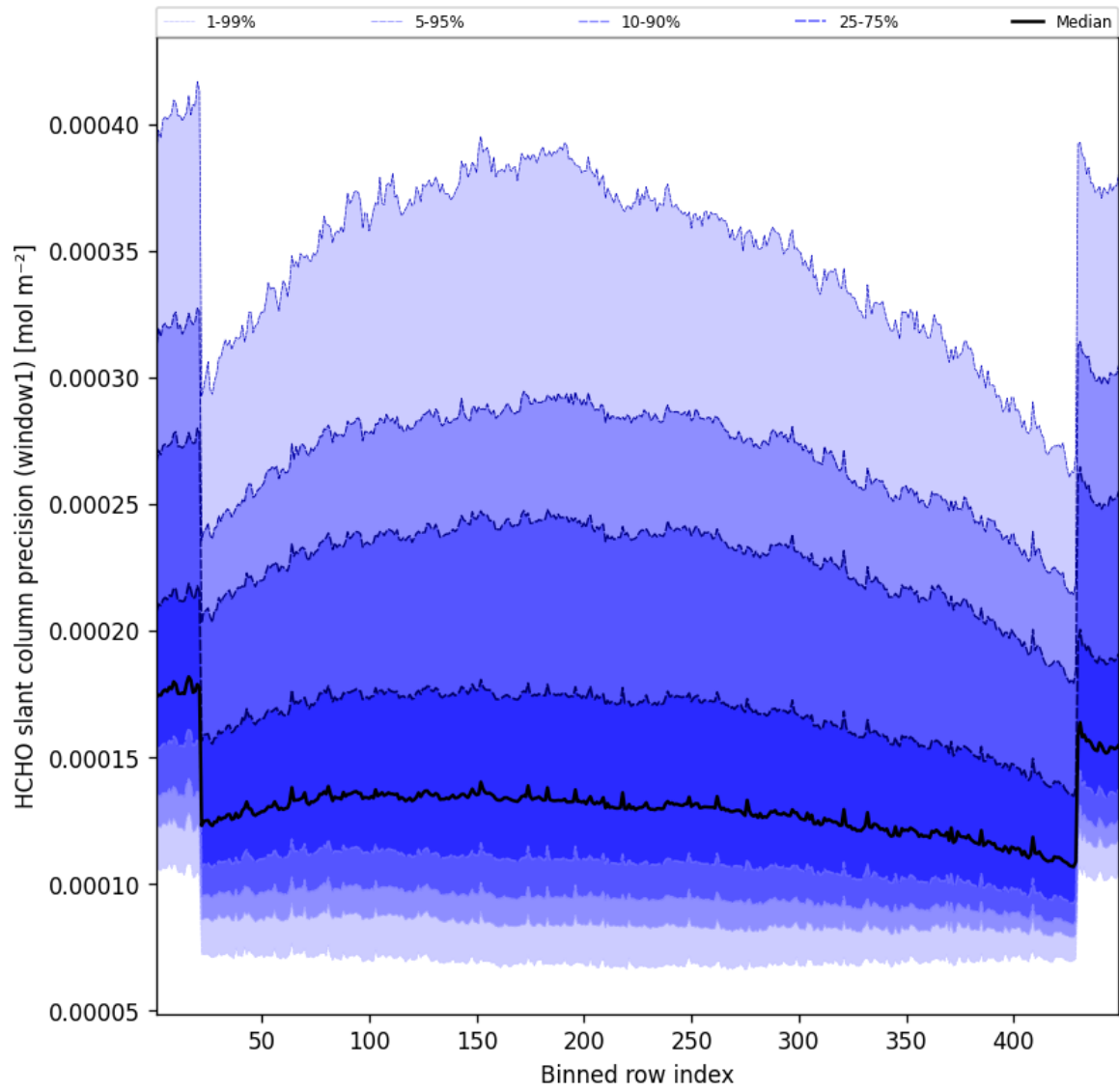
Figure 51: Along track statistics of “HCHO slant column precision (window1)” for 2025-08-12 to 2025-08-12
