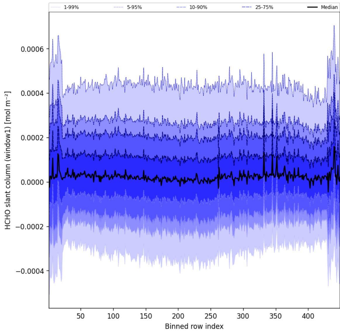
Figure 50: Along track statistics of “HCHO slant column (window1)” for 2025-08-12 to 2025-08-12
