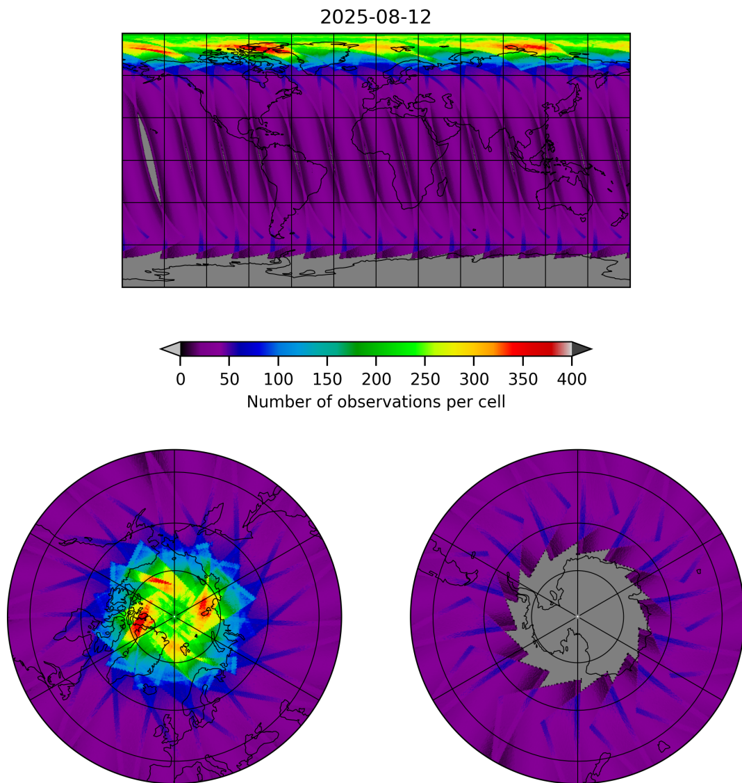
Figure 17: Map of the number of observations for 2025-08-12 to 2025-08-12
