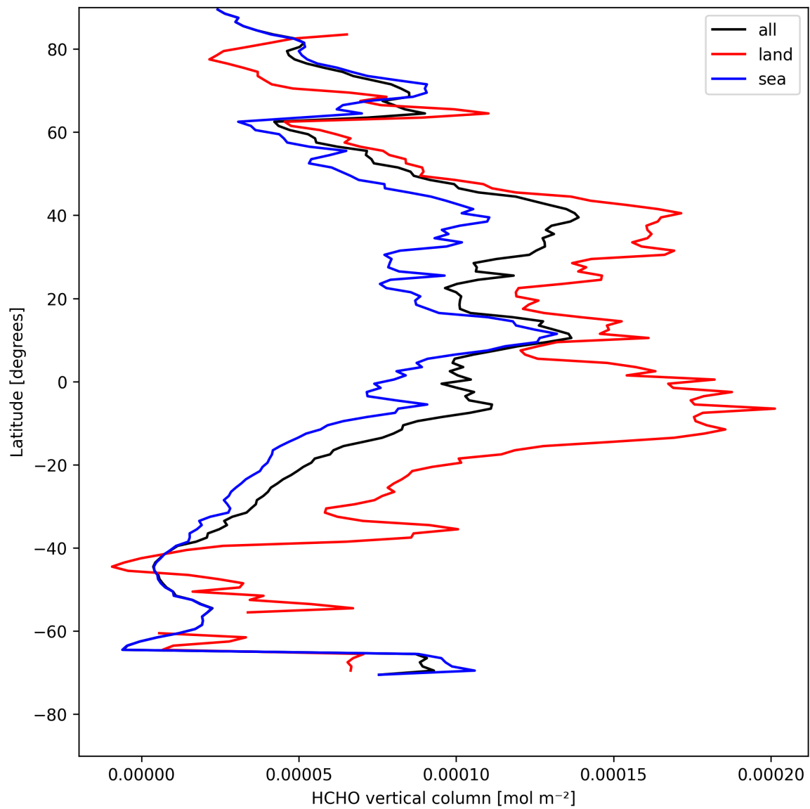
Figure 19: Zonal average of “HCHO vertical column” for 2025-08-12 to 2025-08-12.
