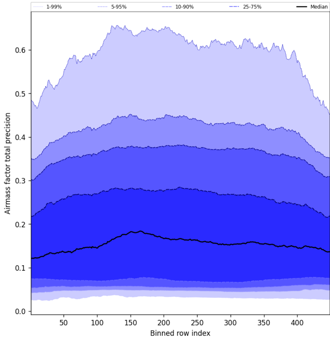
Figure 53: Along track statistics of “Airmass factor total precision” for 2025-08-12 to 2025-08-12
