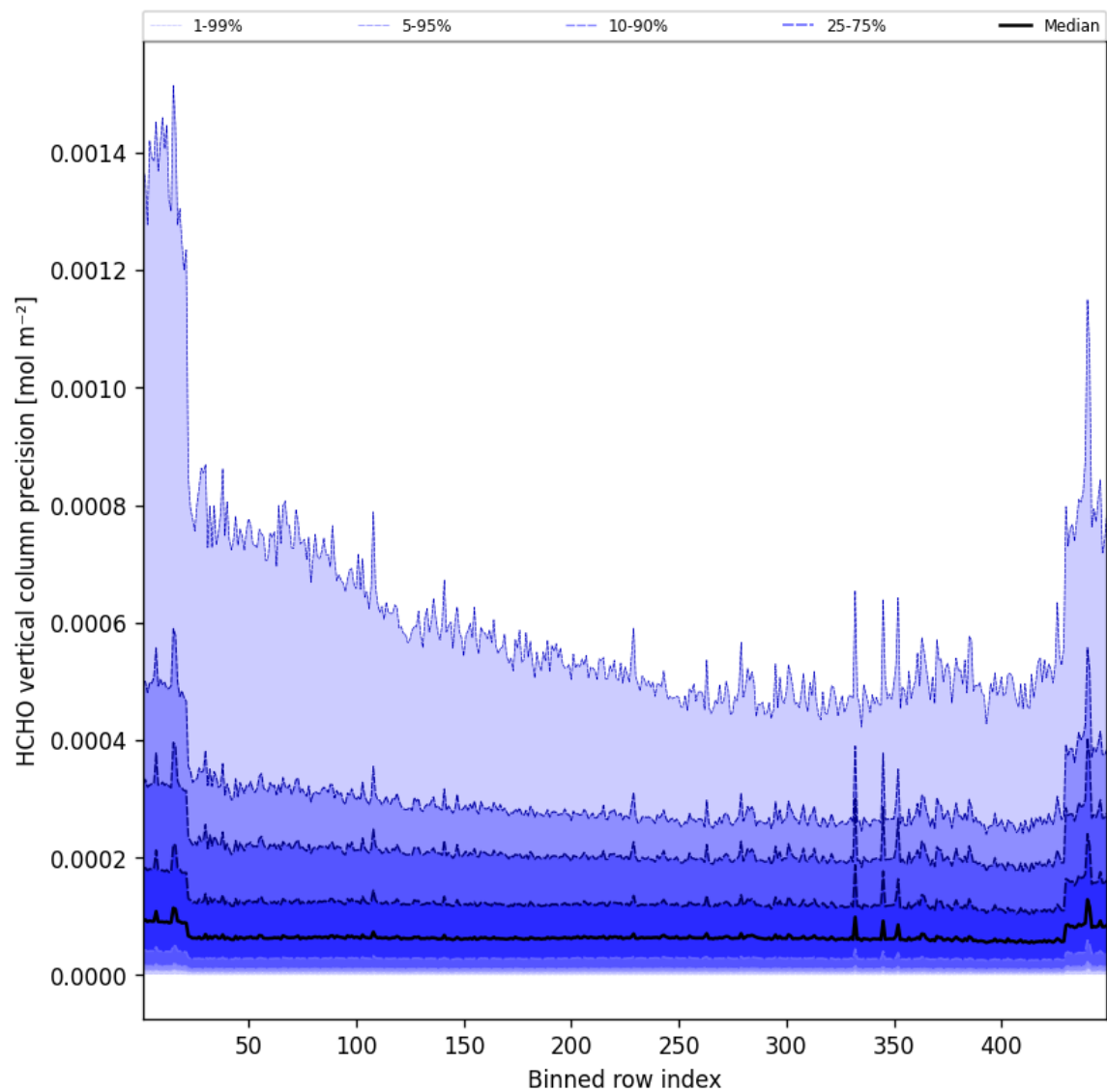
Figure 48: Along track statistics of “HCHO vertical column precision” for 2025-08-12 to 2025-08-12
