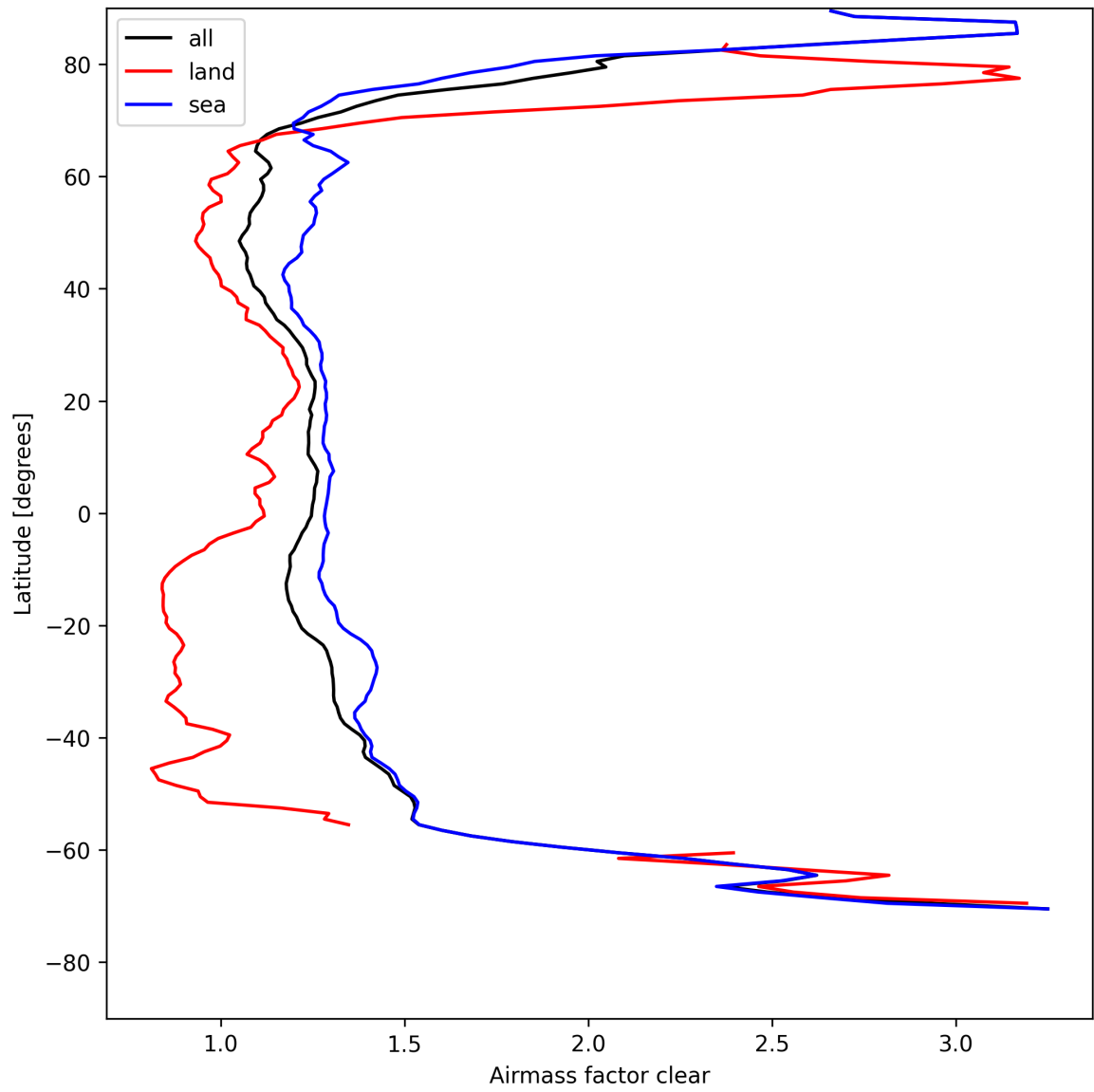
Figure 26: Zonal average of “Airmass factor clear” for 2025-08-12 to 2025-08-12.
