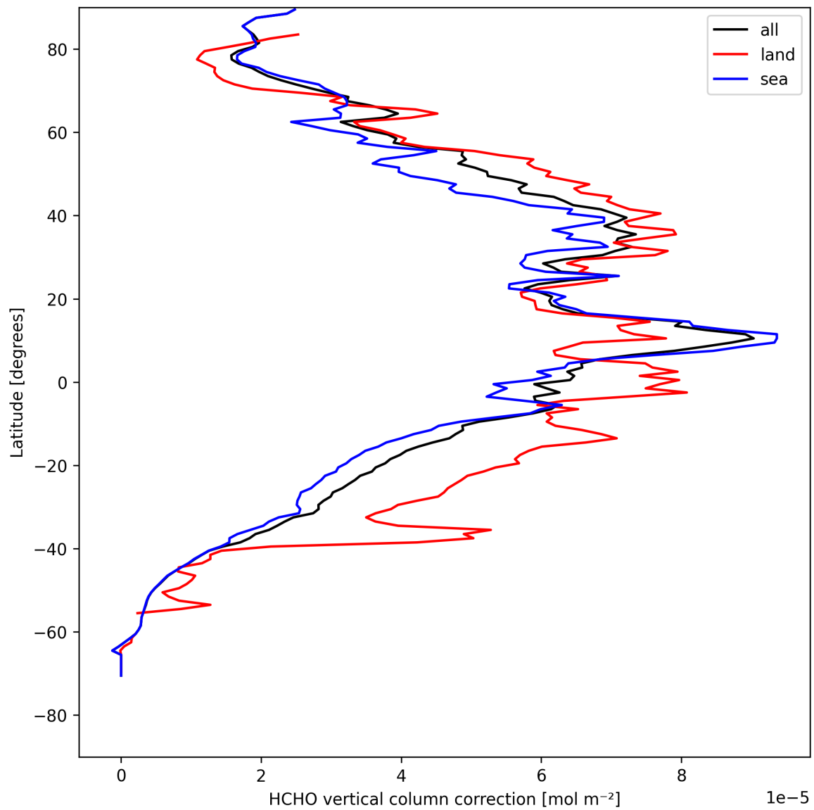
Figure 21: Zonal average of “HCHO vertical column correction” for 2025-08-12 to 2025-08-12.
