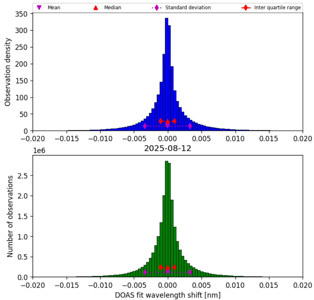
Figure 42: Histogram of “DOAS fit wavelength shift” for 2025-08-12 to 2025-08-12
