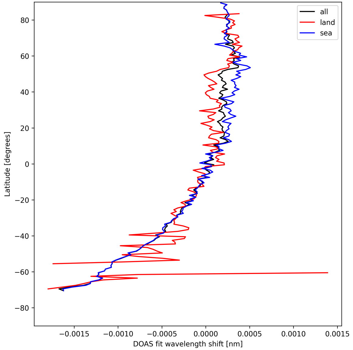
Figure 28: Zonal average of “DOAS fit wavelength shift” for 2025-08-12 to 2025-08-12.
