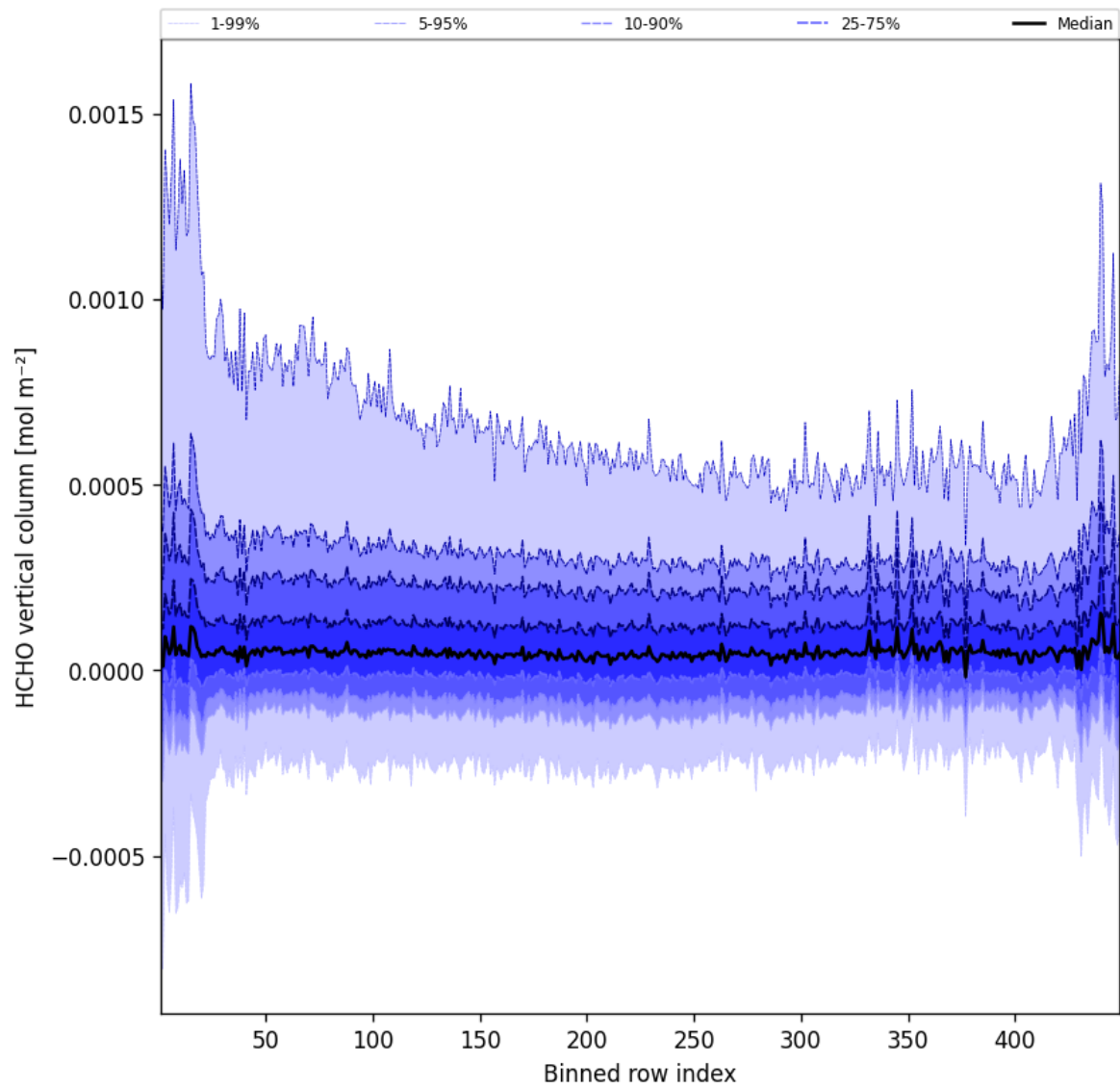
Figure 47: Along track statistics of “HCHO vertical column” for 2025-08-12 to 2025-08-12
