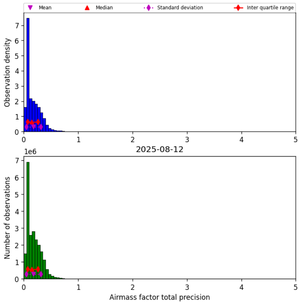
Figure 39: Histogram of “Airmass factor total precision” for 2025-08-12 to 2025-08-12
