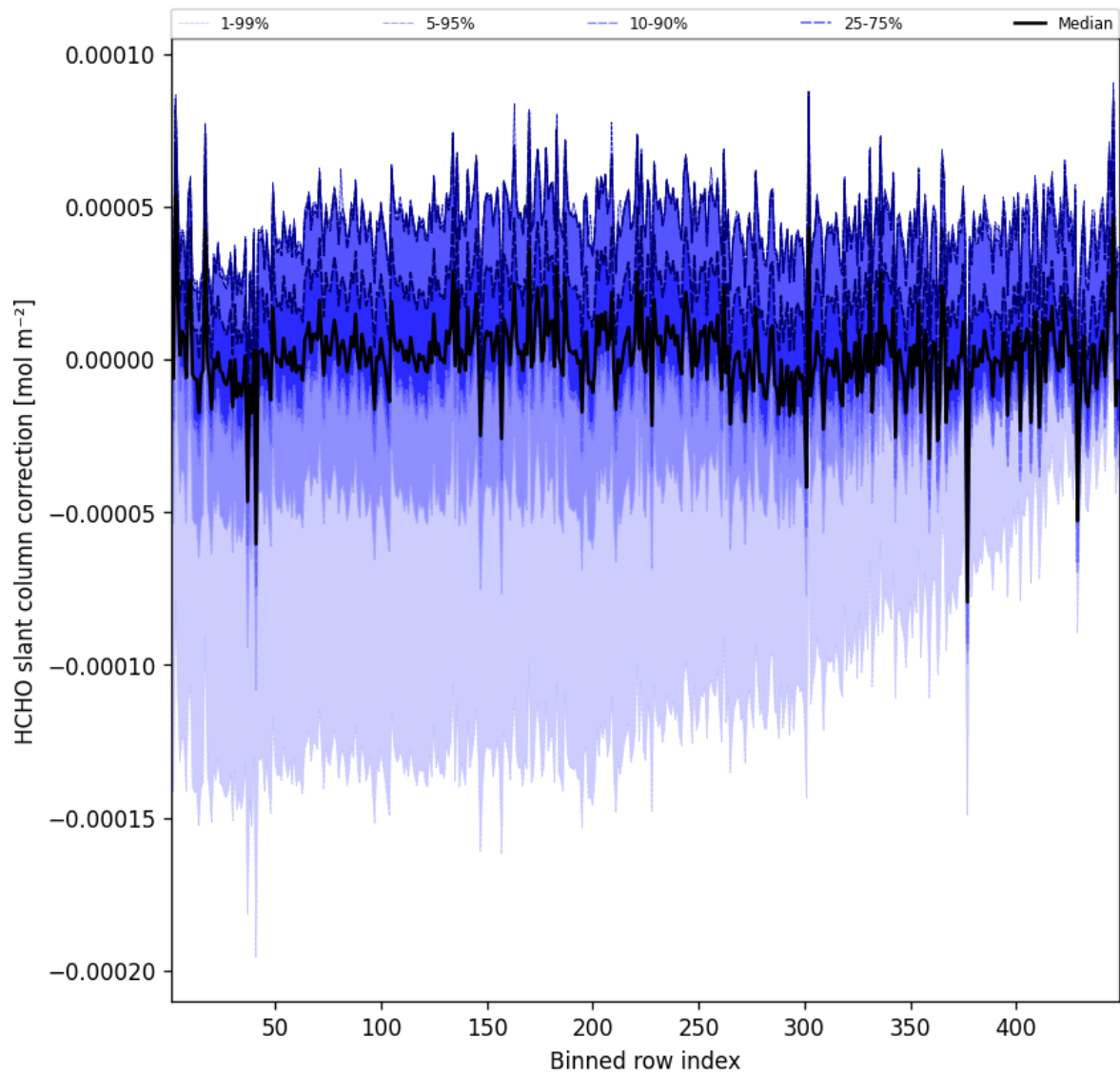
Figure 59: Along track statistics of “HCHO slant column correction” for 2025-08-12 to 2025-08-12
