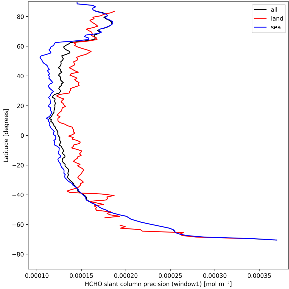
Figure 23: Zonal average of "HCHO slant column precision (window1)" for 2025-08-12 to 2025-08-12.
