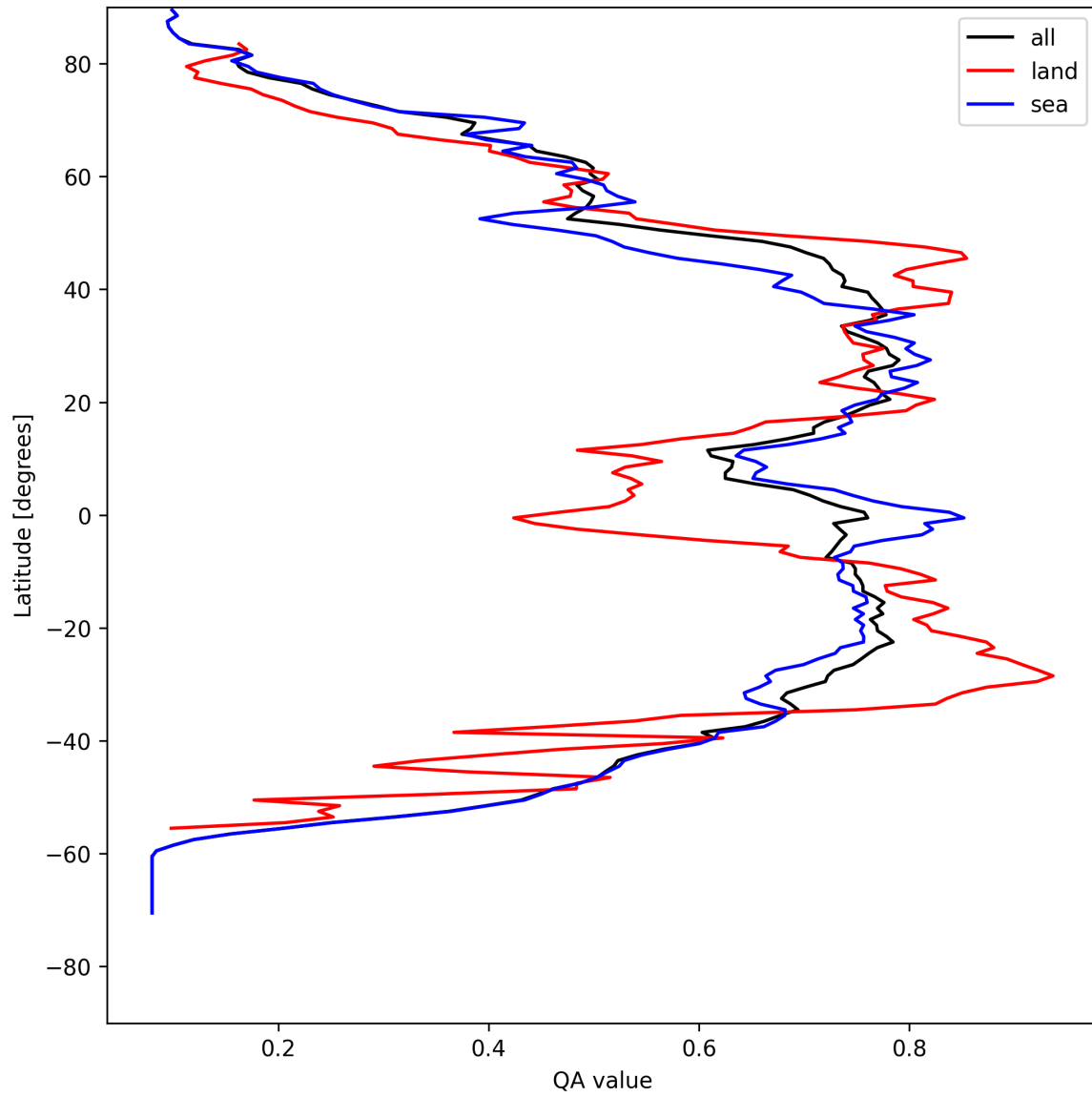
Figure 18: Zonal average of “QA value” for 2025-08-12 to 2025-08-12.
