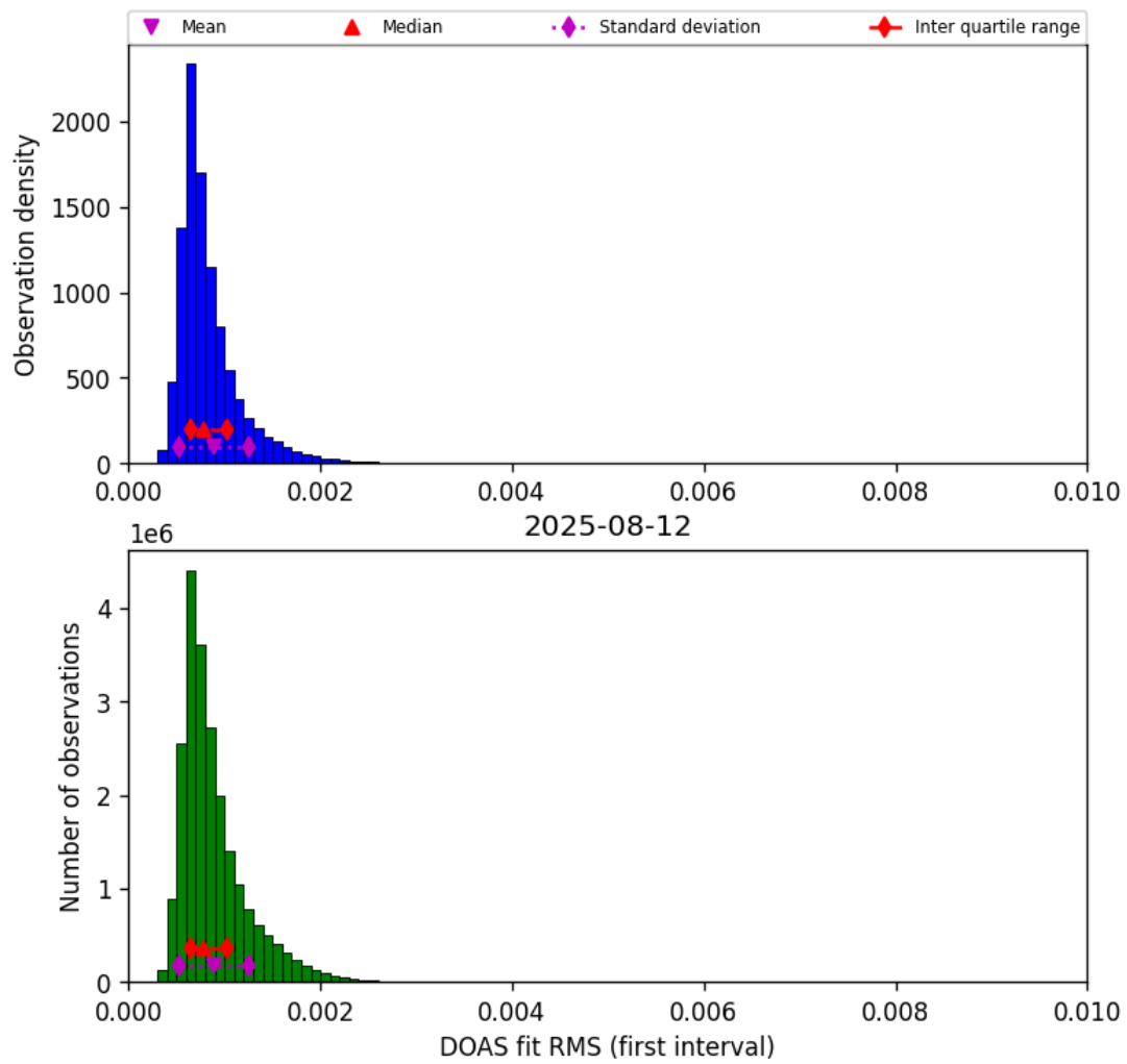
Figure 44: Histogram of “DOAS fit RMS (first interval)” for 2025-08-12 to 2025-08-12
