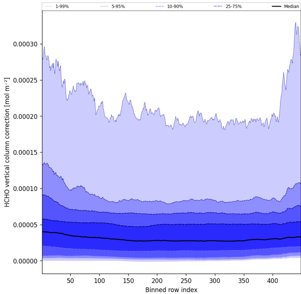
Figure 49: Along track statistics of “HCHO vertical column correction” for 2025-08-12 to 2025-08-12
