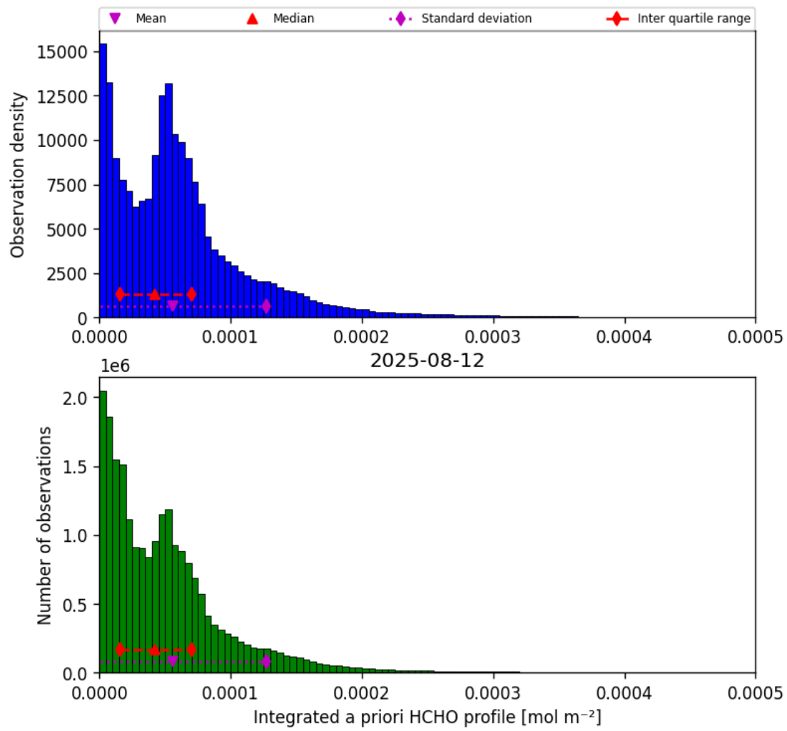
Figure 41: Histogram of “Integrated a priori HCHO profile” for 2025-08-12 to 2025-08-12
