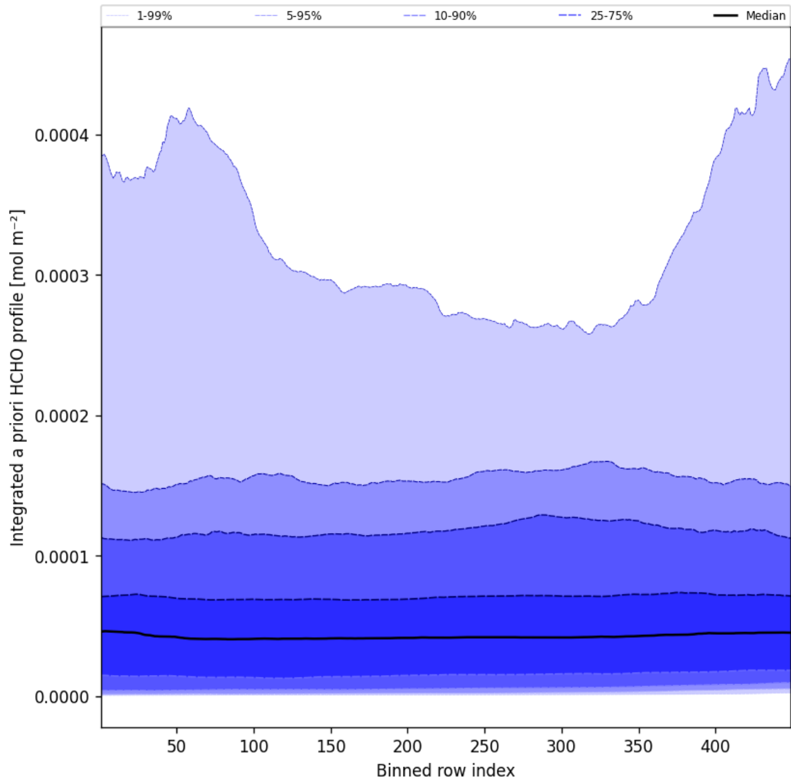
Figure 55: Along track statistics of “Integrated a priori HCHO profile” for 2025-08-12 to 2025-08-12
