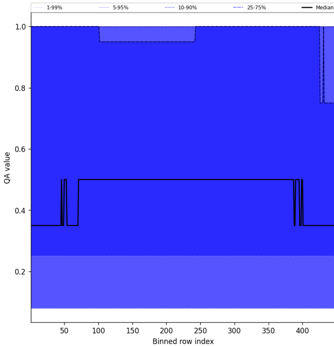
Figure 46: Along track statistics of “QA value” for 2025-08-12 to 2025-08-12
