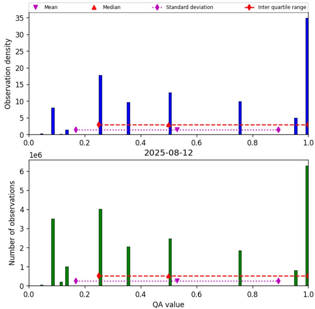
Figure 32: Histogram of “QA value” for 2025-08-12 to 2025-08-12
