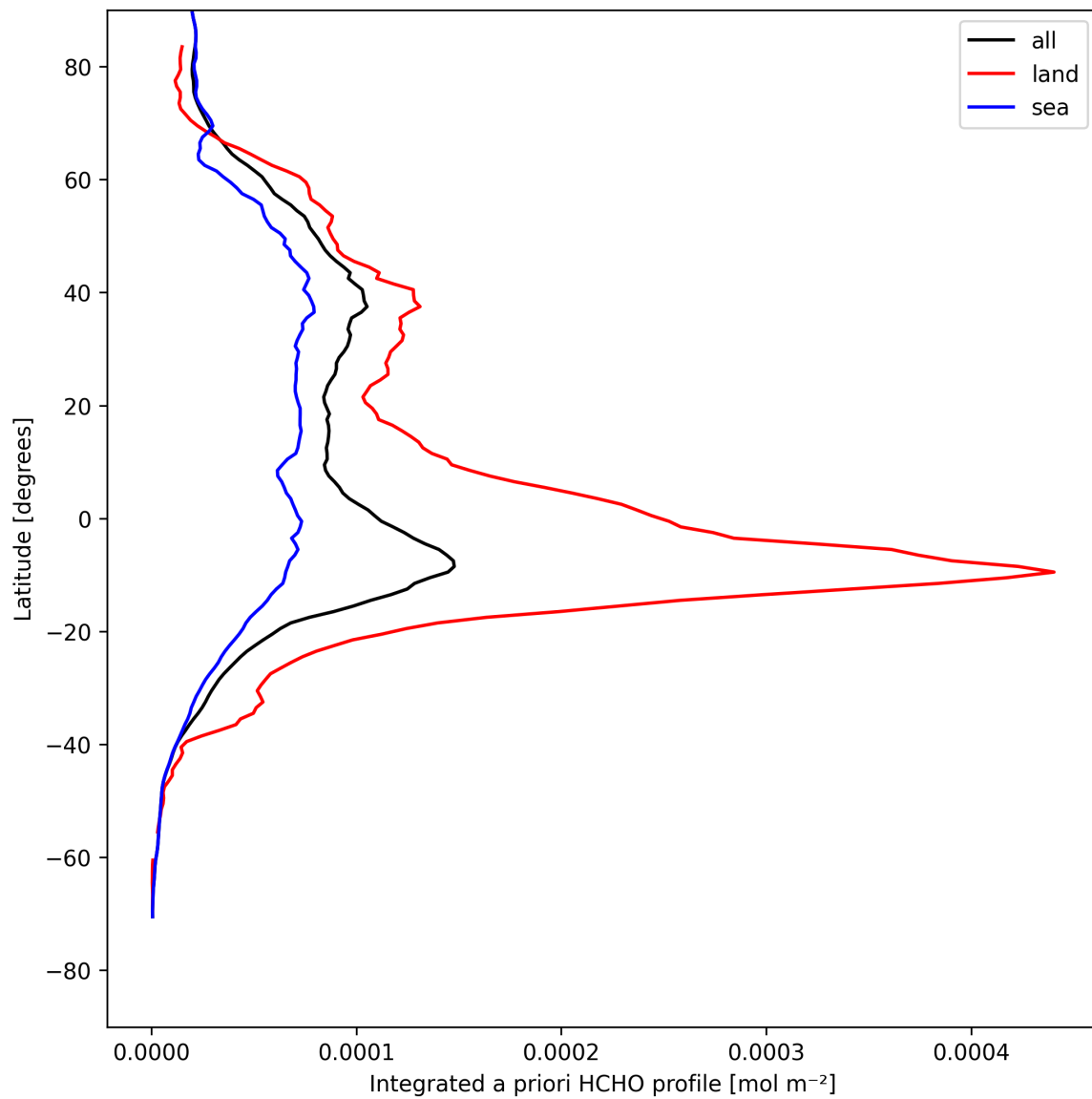
Figure 27: Zonal average of “Integrated a priori HCHO profile” for 2025-08-12 to 2025-08-12.
