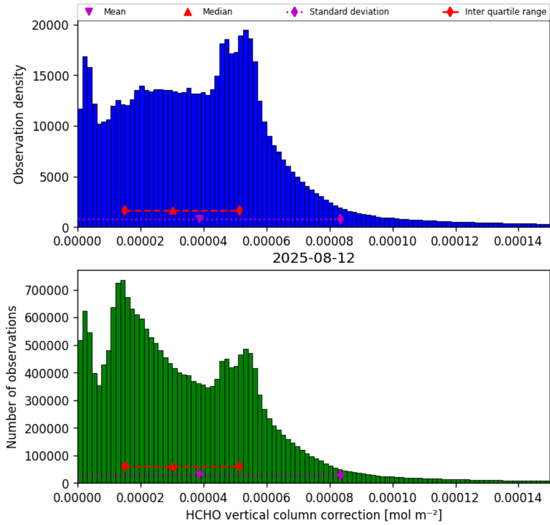
Figure 35: Histogram of “HCHO vertical column correction” for 2025-08-12 to 2025-08-12
