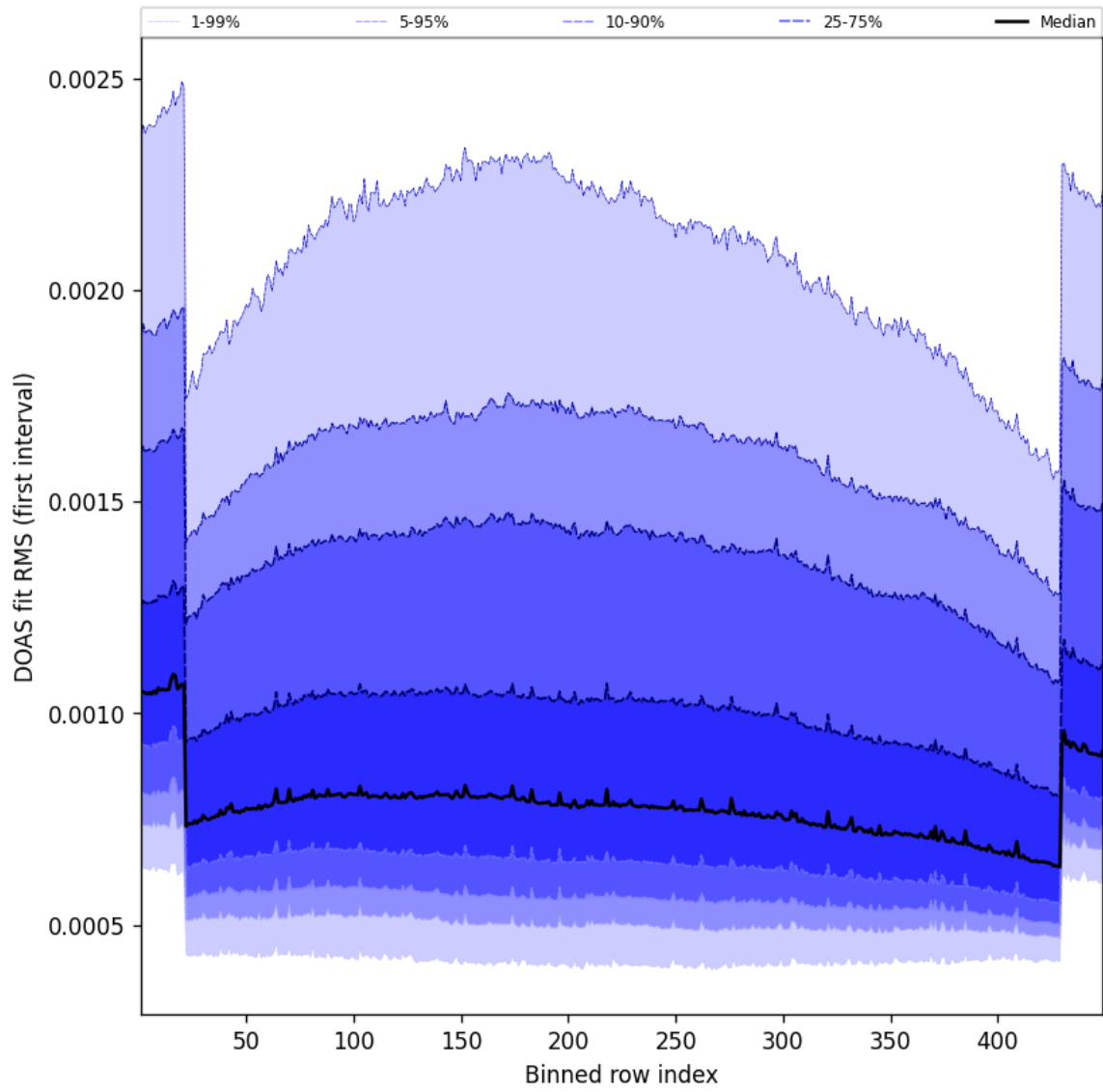
Figure 58: Along track statistics of “DOAS fit RMS (first interval)” for 2025-08-12 to 2025-08-12
