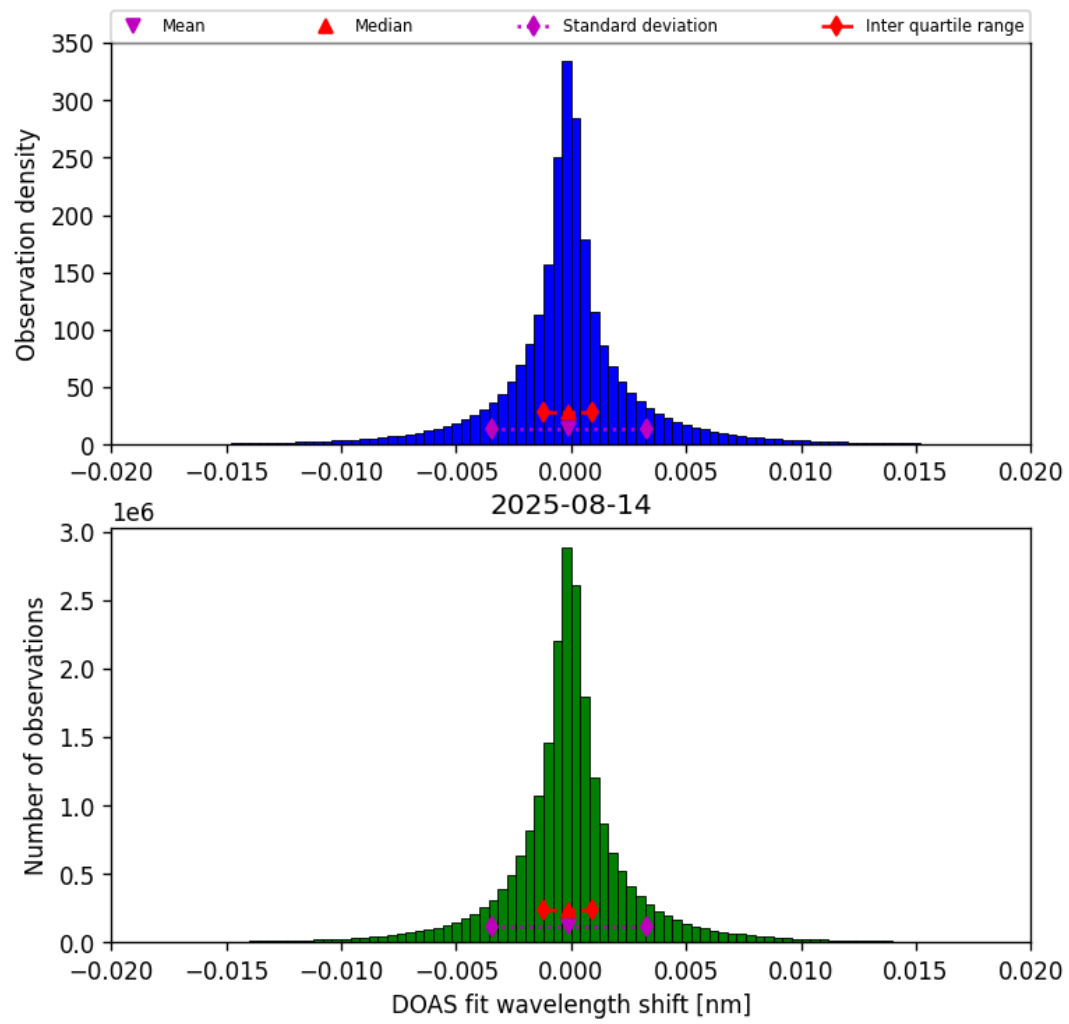
Figure 42: Histogram of “DOAS fit wavelength shift” for 2025-08-14 to 2025-08-15
