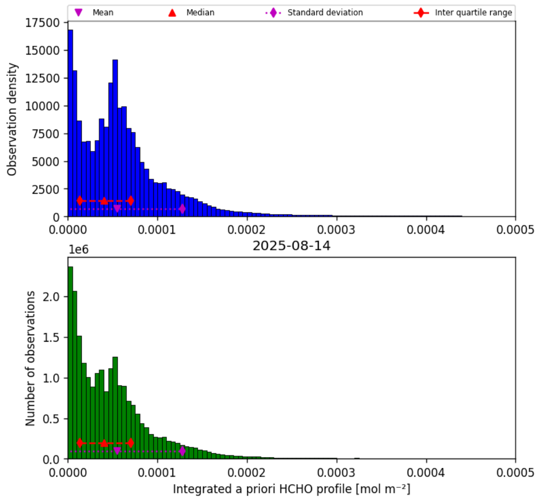
Figure 41: Histogram of “Integrated a priori HCHO profile” for 2025-08-14 to 2025-08-15
