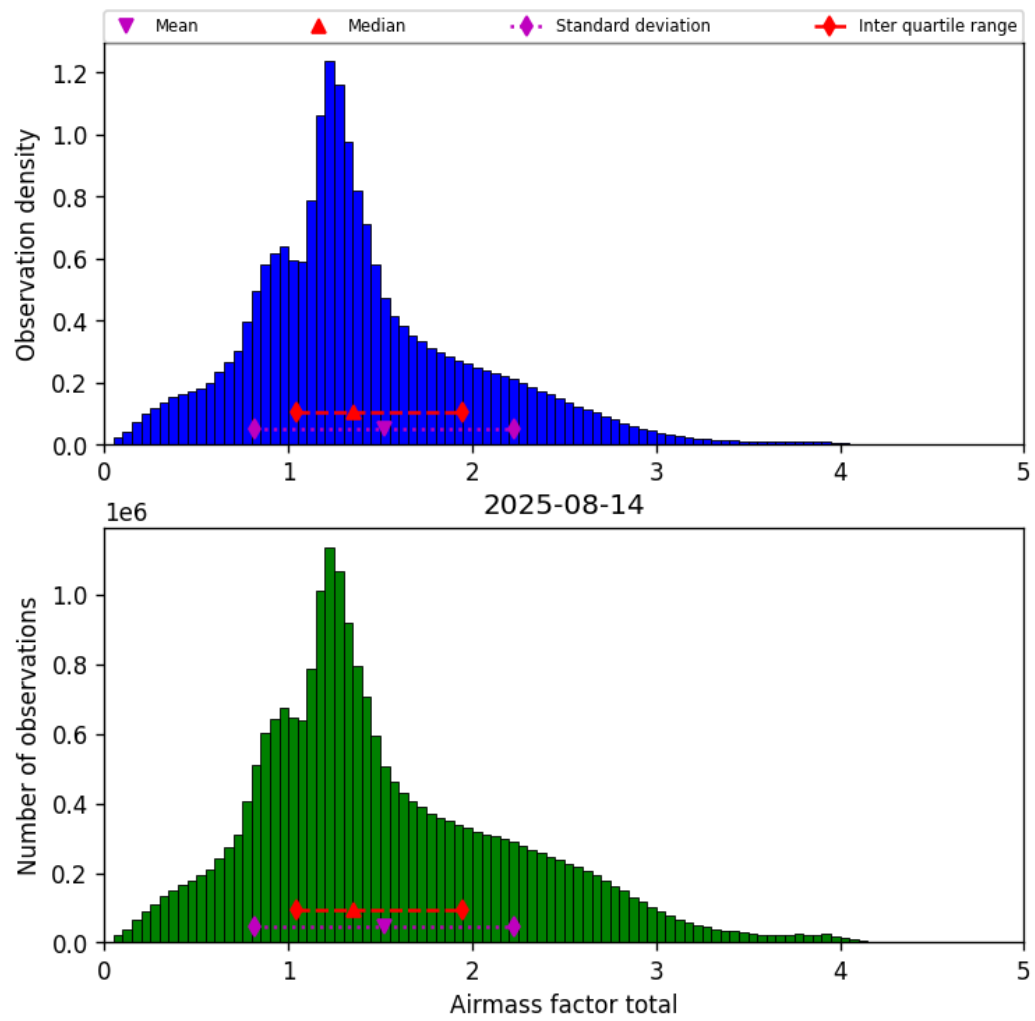
Figure 38: Histogram of “Airmass factor total” for 2025-08-14 to 2025-08-15
