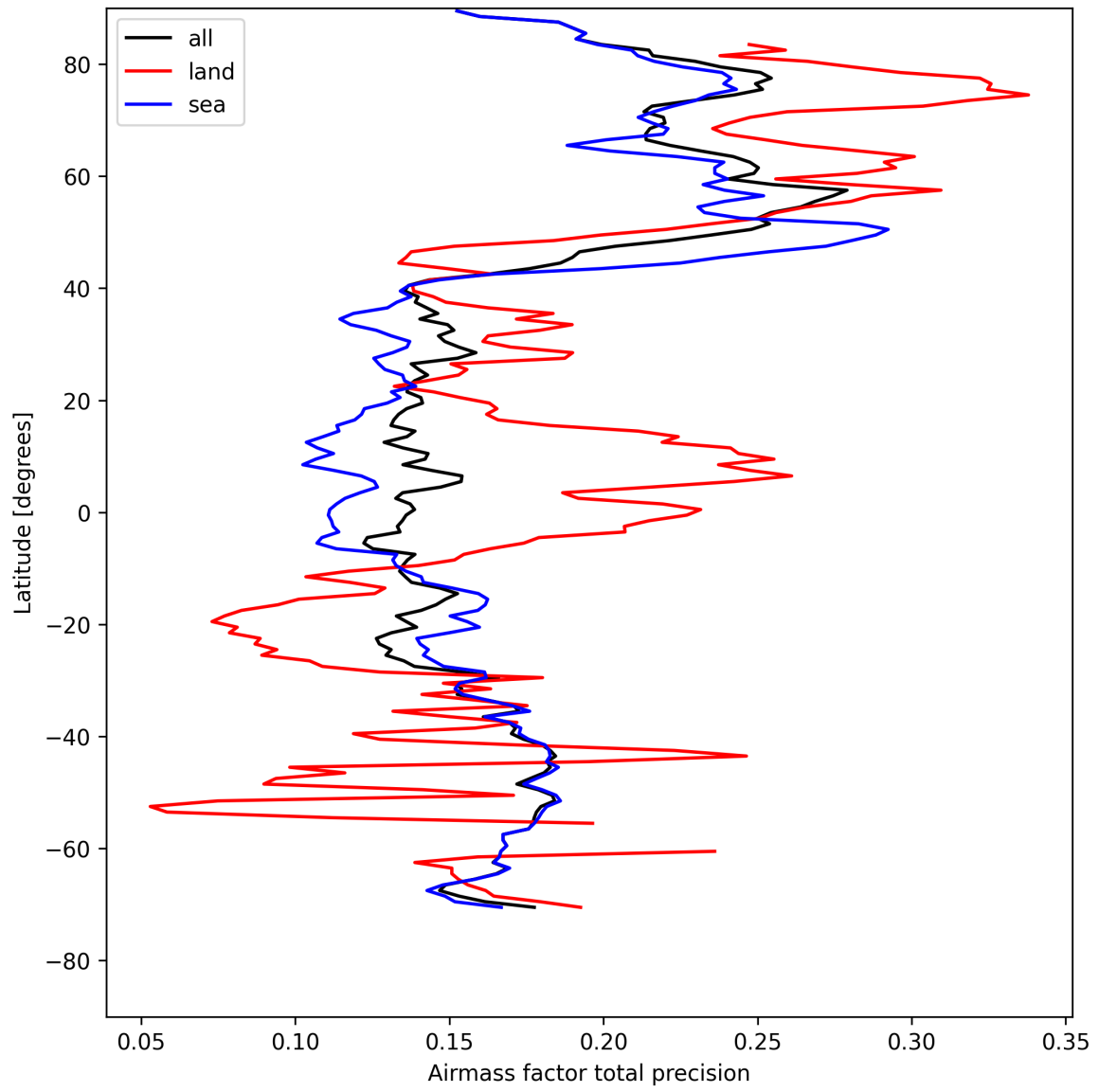
Figure 25: Zonal average of “Airmass factor total precision” for 2025-08-14 to 2025-08-15.
