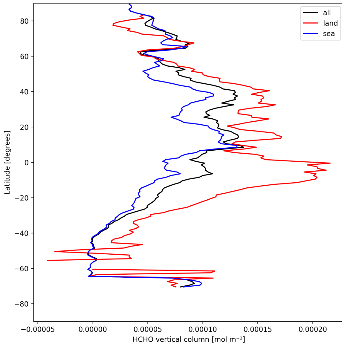
Figure 19: Zonal average of “HCHO vertical column” for 2025-08-14 to 2025-08-15.
