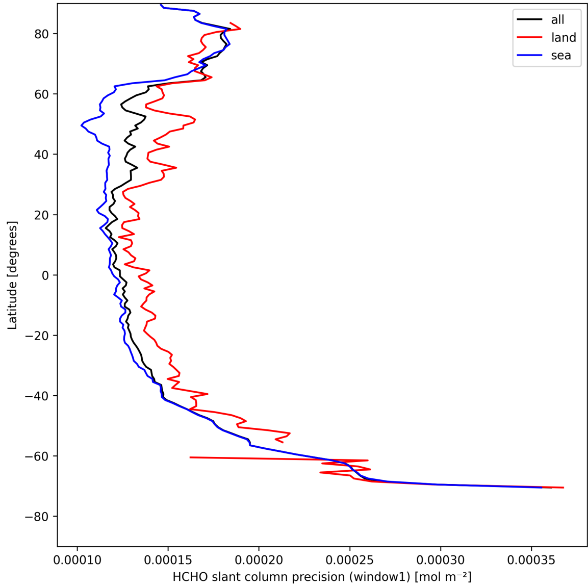
Figure 23: Zonal average of "HCHO slant column precision (window1)" for 2025-08-14 to 2025-08-15.
