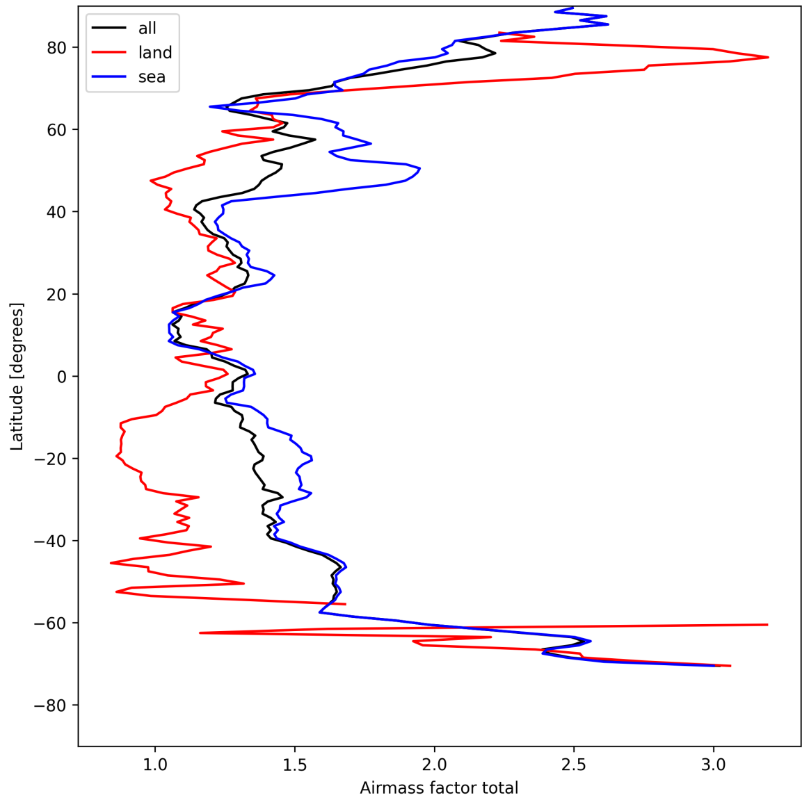
Figure 24: Zonal average of “Airmass factor total” for 2025-08-14 to 2025-08-15.
