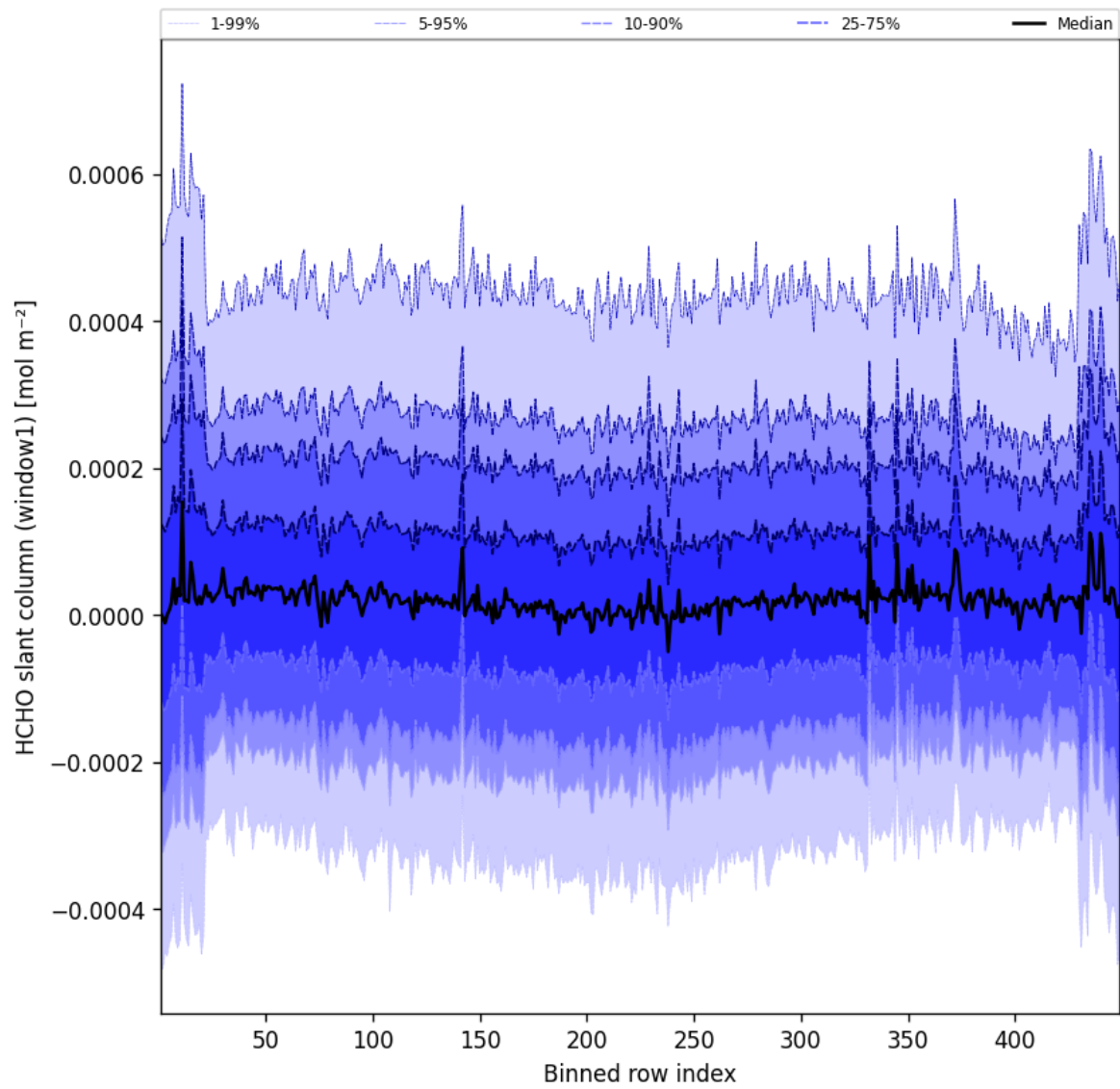
Figure 50: Along track statistics of “HCHO slant column (window1)” for 2025-08-14 to 2025-08-15
