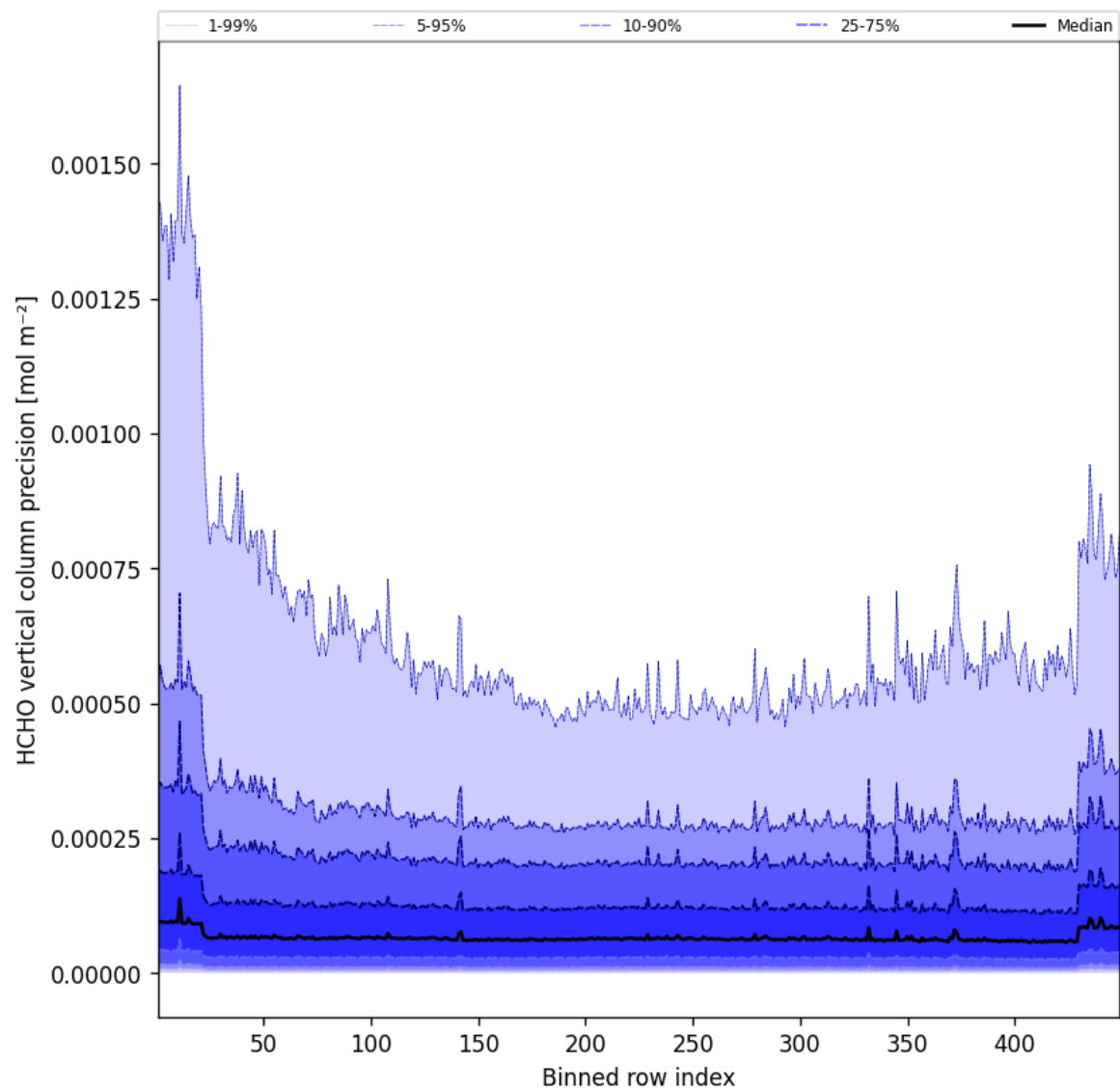
Figure 48: Along track statistics of “HCHO vertical column precision” for 2025-08-14 to 2025-08-15
