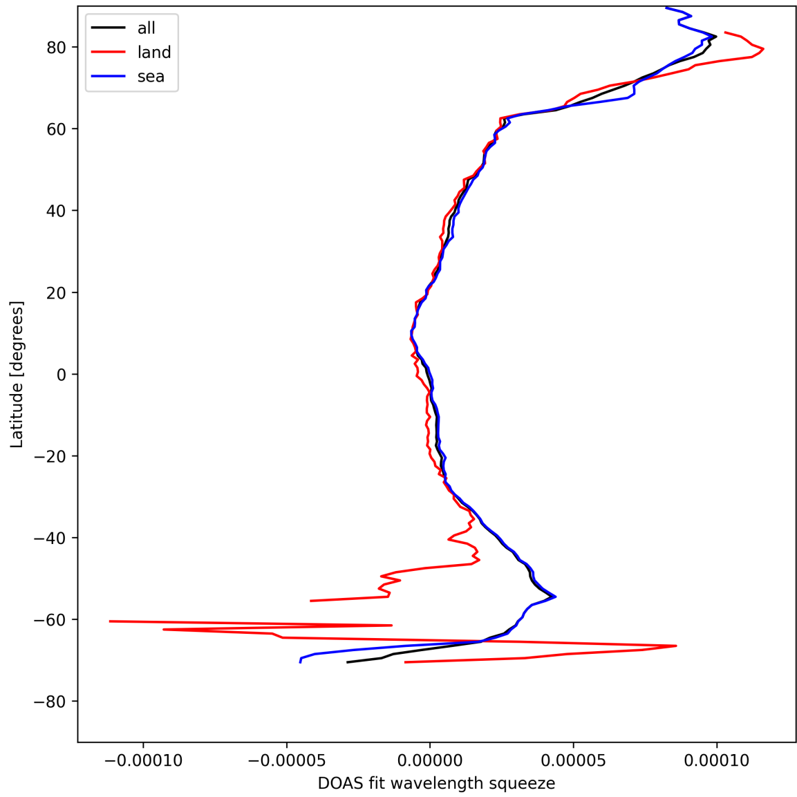
Figure 29: Zonal average of “DOAS fit wavelength squeeze” for 2025-08-14 to 2025-08-15.
