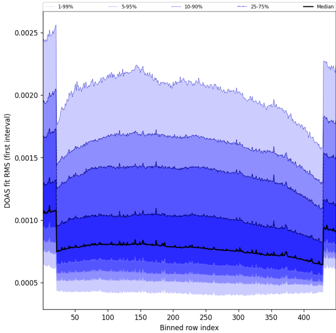
Figure 58: Along track statistics of “DOAS fit RMS (first interval)” for 2025-08-14 to 2025-08-15
