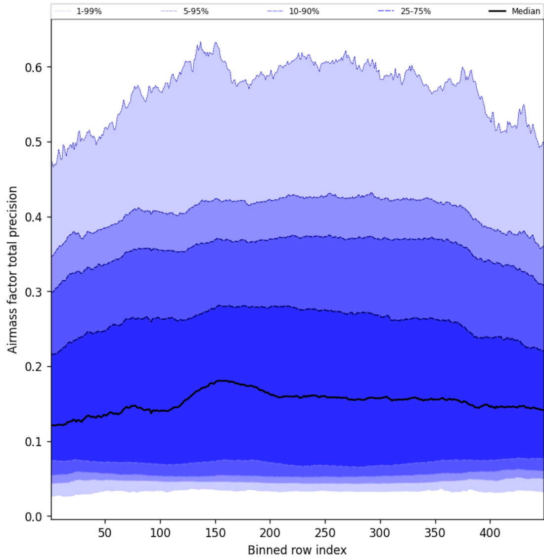
Figure 53: Along track statistics of “Airmass factor total precision” for 2025-08-14 to 2025-08-15
