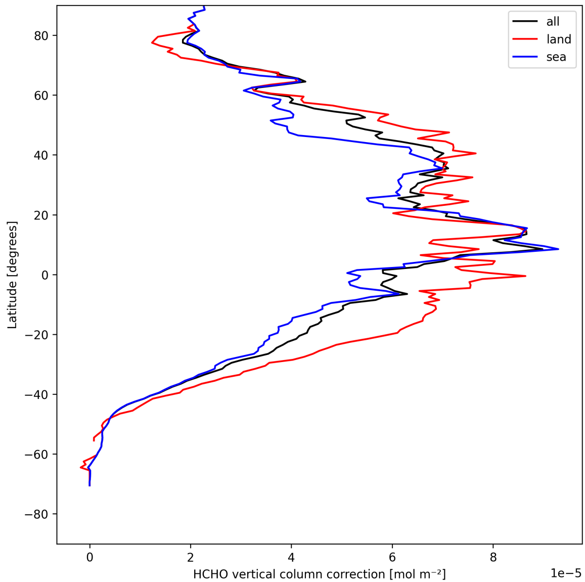
Figure 21: Zonal average of “HCHO vertical column correction” for 2025-08-14 to 2025-08-15.
