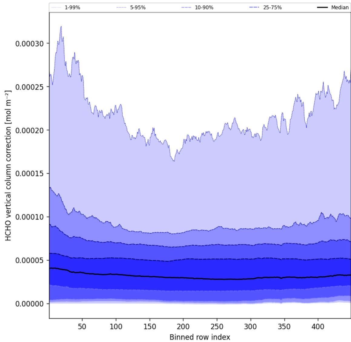
Figure 49: Along track statistics of “HCHO vertical column correction” for 2025-08-14 to 2025-08-15
