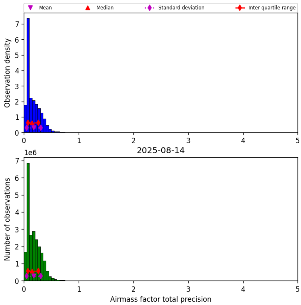
Figure 39: Histogram of “Airmass factor total precision” for 2025-08-14 to 2025-08-15
