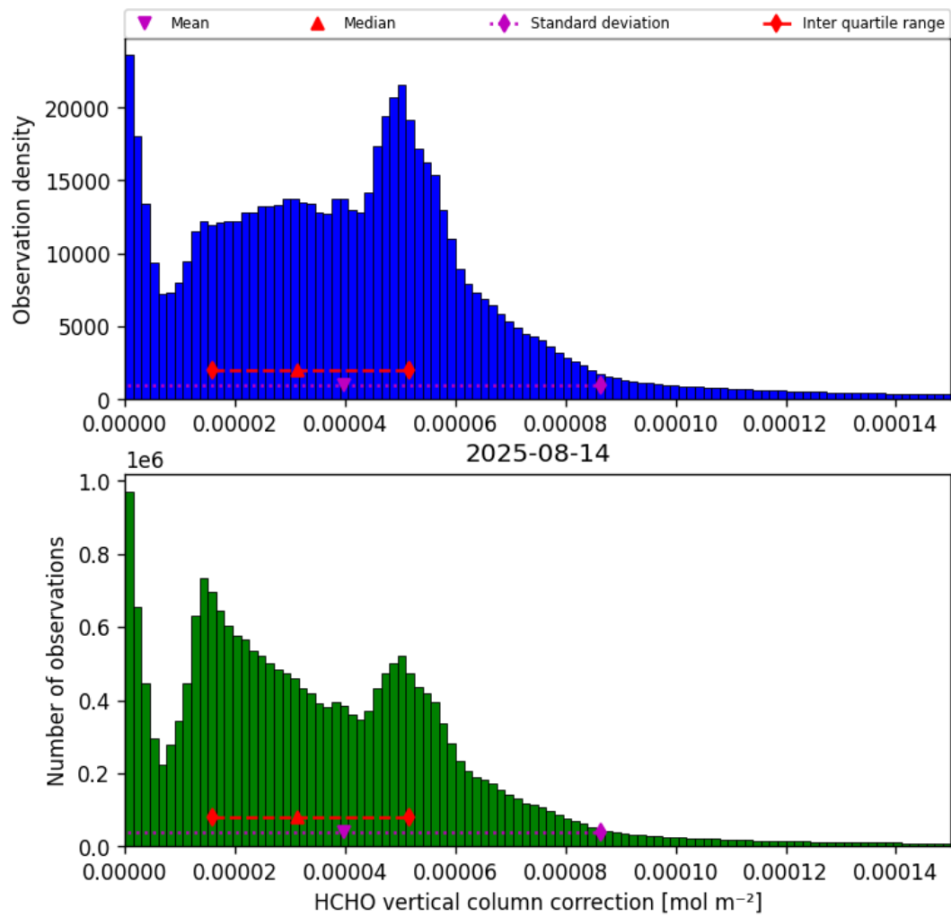
Figure 35: Histogram of “HCHO vertical column correction” for 2025-08-14 to 2025-08-15
