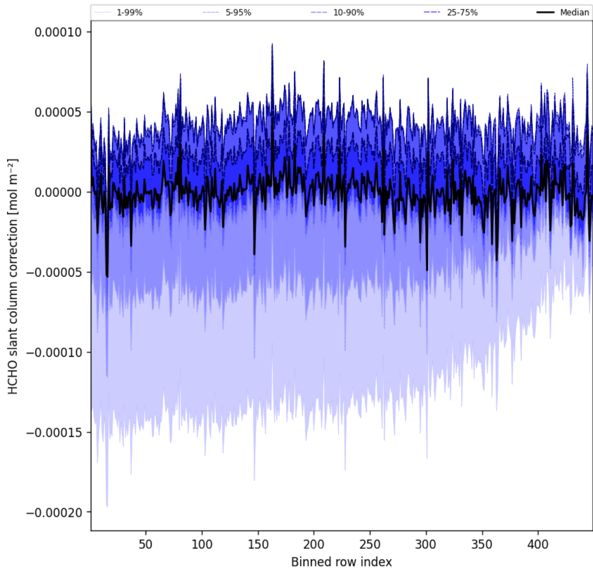
Figure 59: Along track statistics of “HCHO slant column correction” for 2025-08-14 to 2025-08-15
