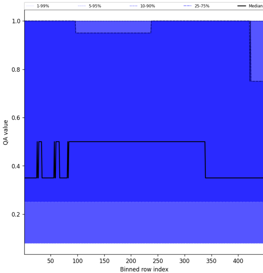
Figure 46: Along track statistics of “QA value” for 2025-08-14 to 2025-08-15
