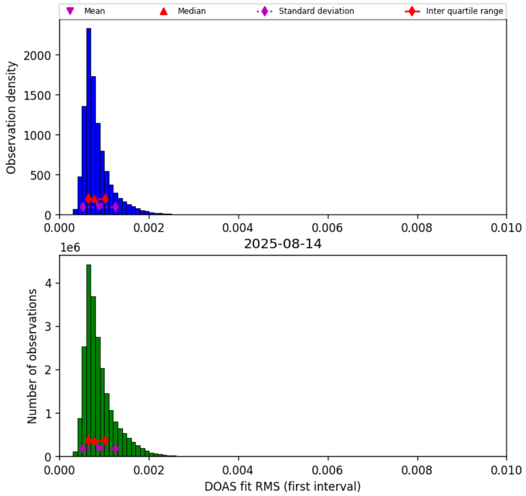
Figure 44: Histogram of “DOAS fit RMS (first interval)” for 2025-08-14 to 2025-08-15
