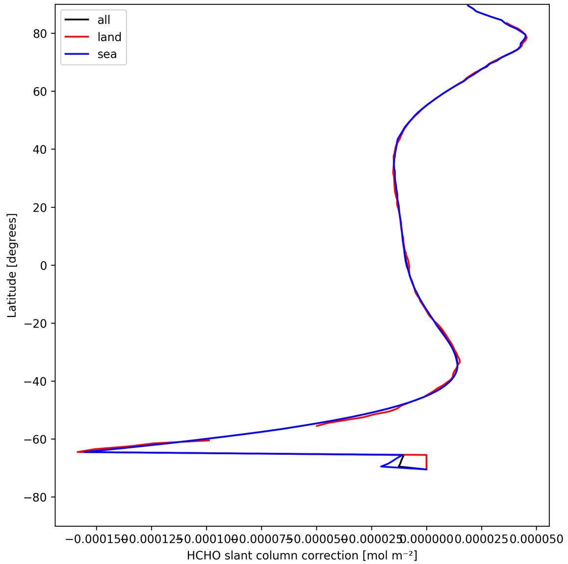
Figure 31: Zonal average of “HCHO slant column correction” for 2025-08-14 to 2025-08-15.
