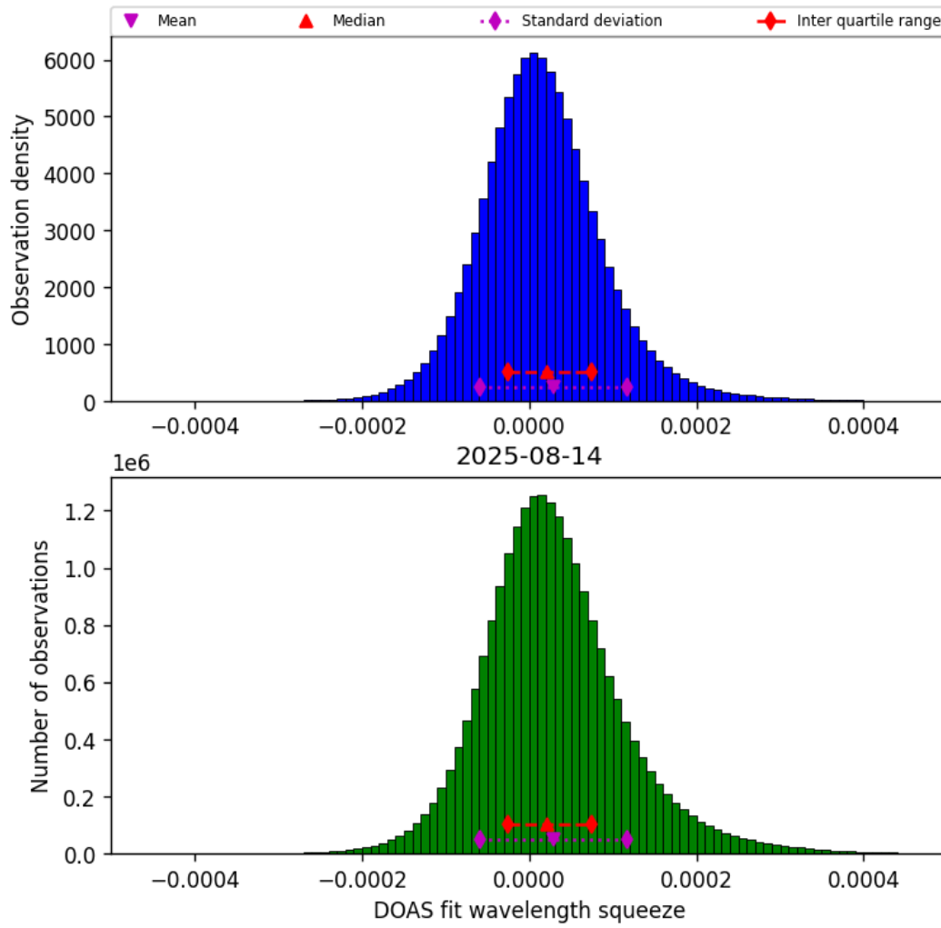
Figure 43: Histogram of “DOAS fit wavelength squeeze” for 2025-08-14 to 2025-08-15
