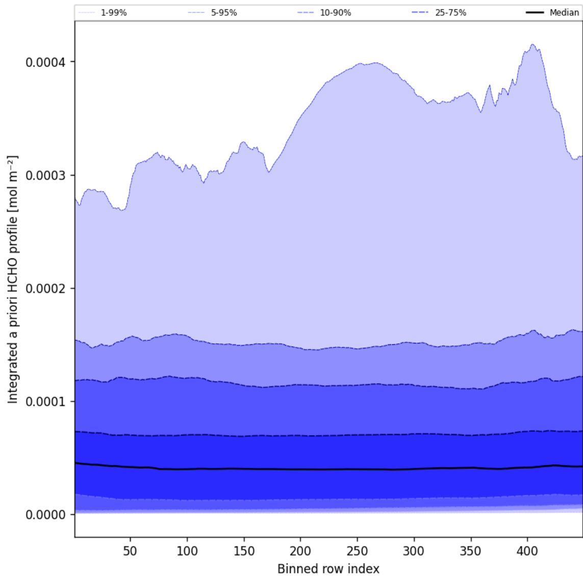
Figure 55: Along track statistics of “Integrated a priori HCHO profile” for 2025-08-14 to 2025-08-15
