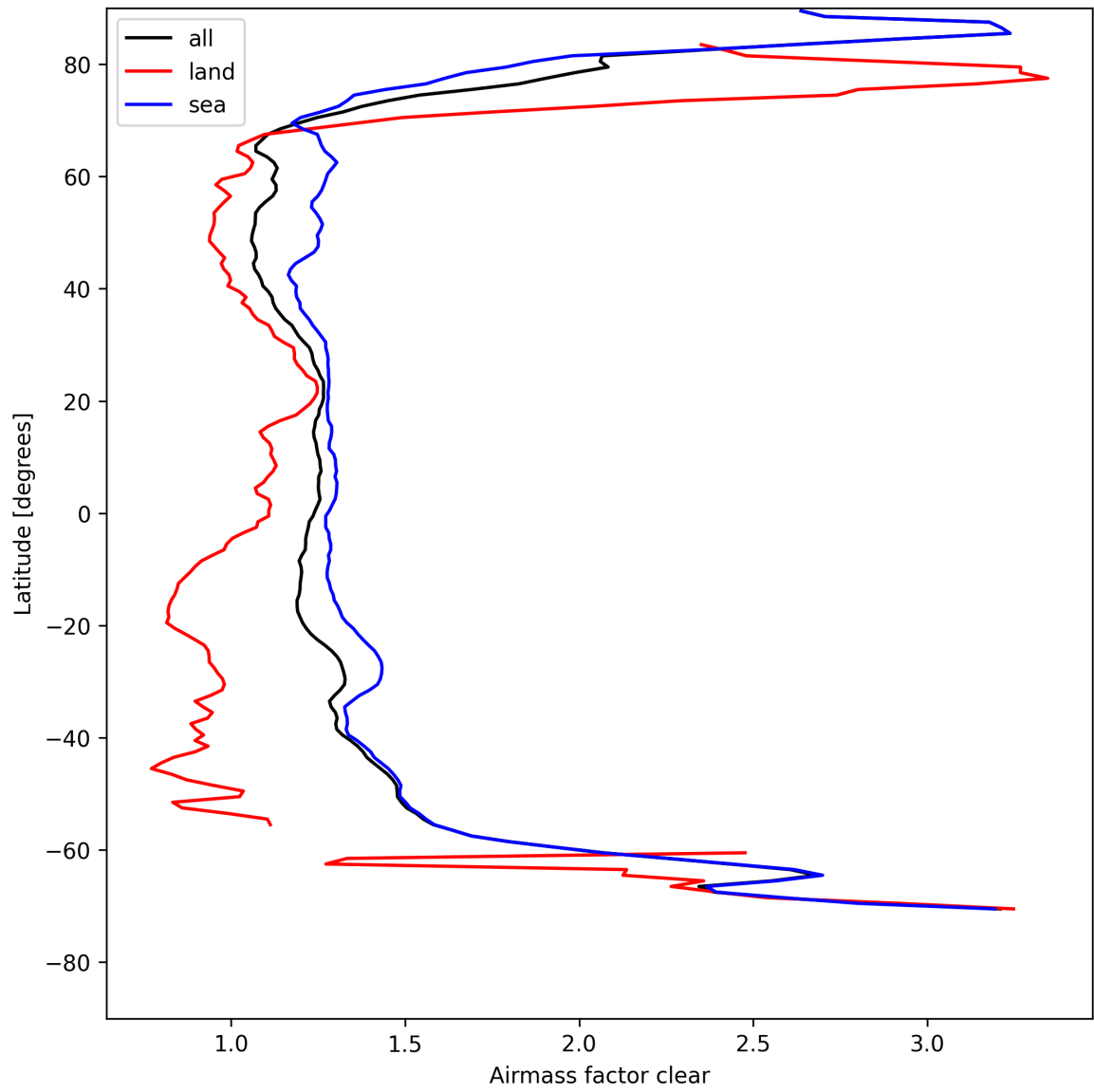
Figure 26: Zonal average of “Airmass factor clear” for 2025-08-14 to 2025-08-15.
