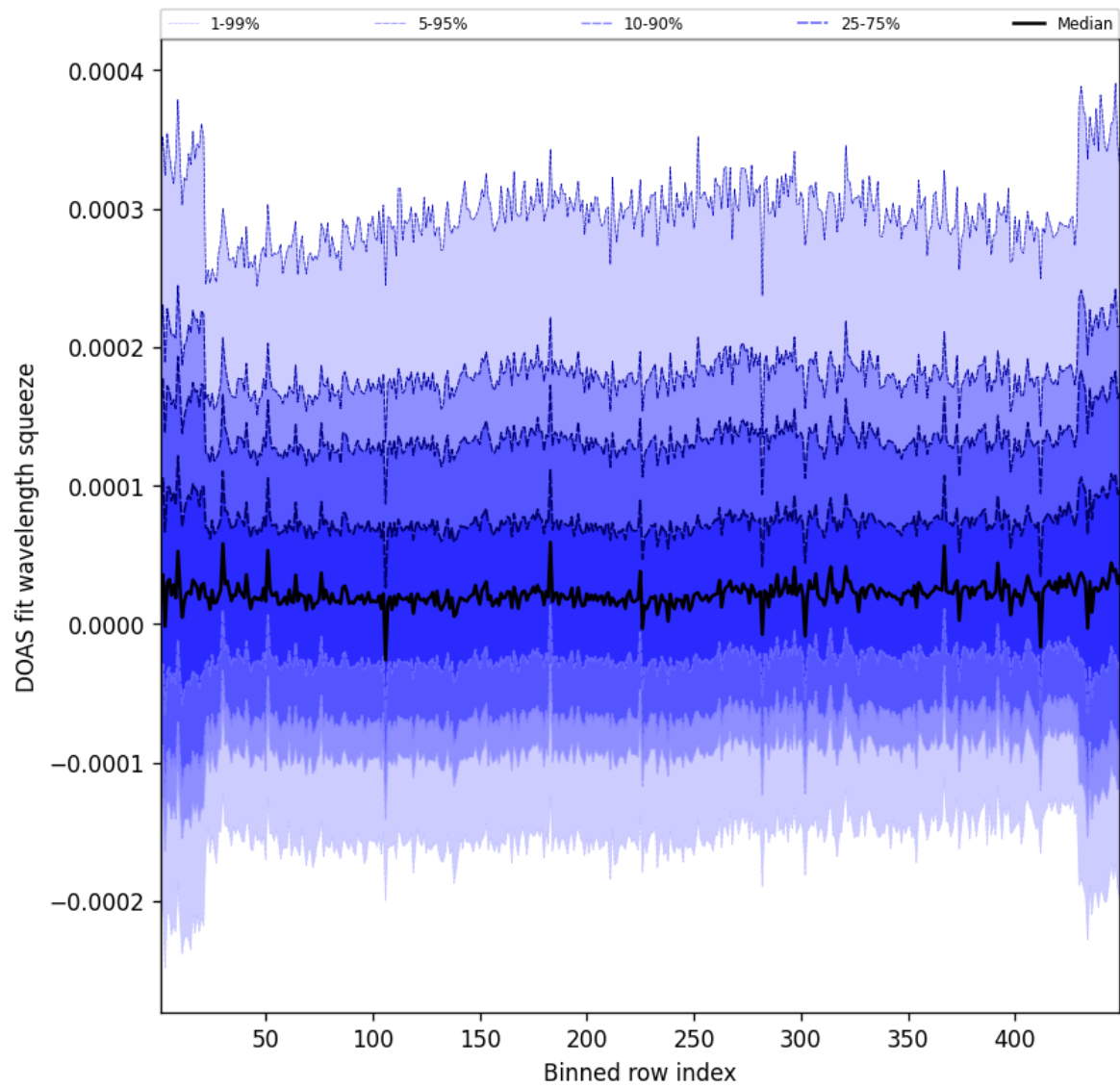
Figure 57: Along track statistics of “DOAS fit wavelength squeeze” for 2025-08-14 to 2025-08-15
