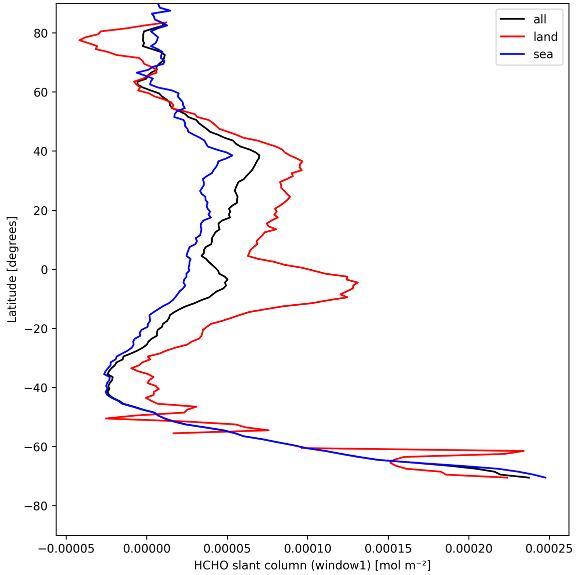
Figure 22: Zonal average of “HCHO slant column (window1)” for 2025-08-14 to 2025-08-15.
