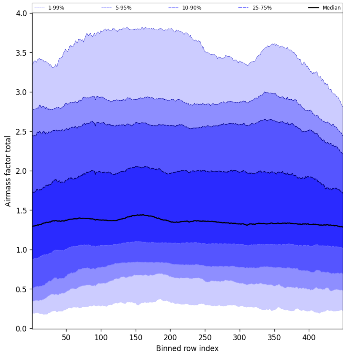
Figure 52: Along track statistics of “Airmass factor total” for 2025-08-14 to 2025-08-15
