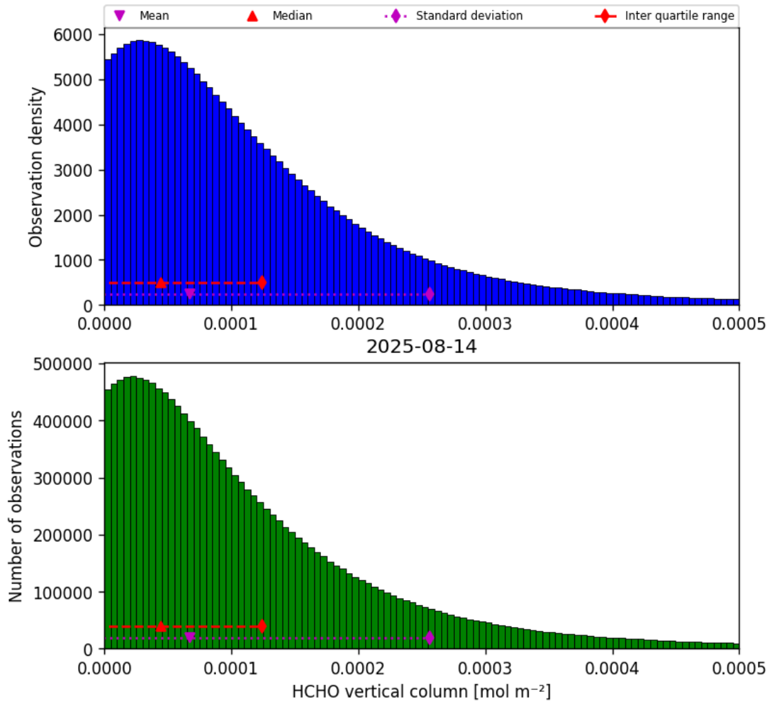
Figure 33: Histogram of “HCHO vertical column” for 2025-08-14 to 2025-08-15
