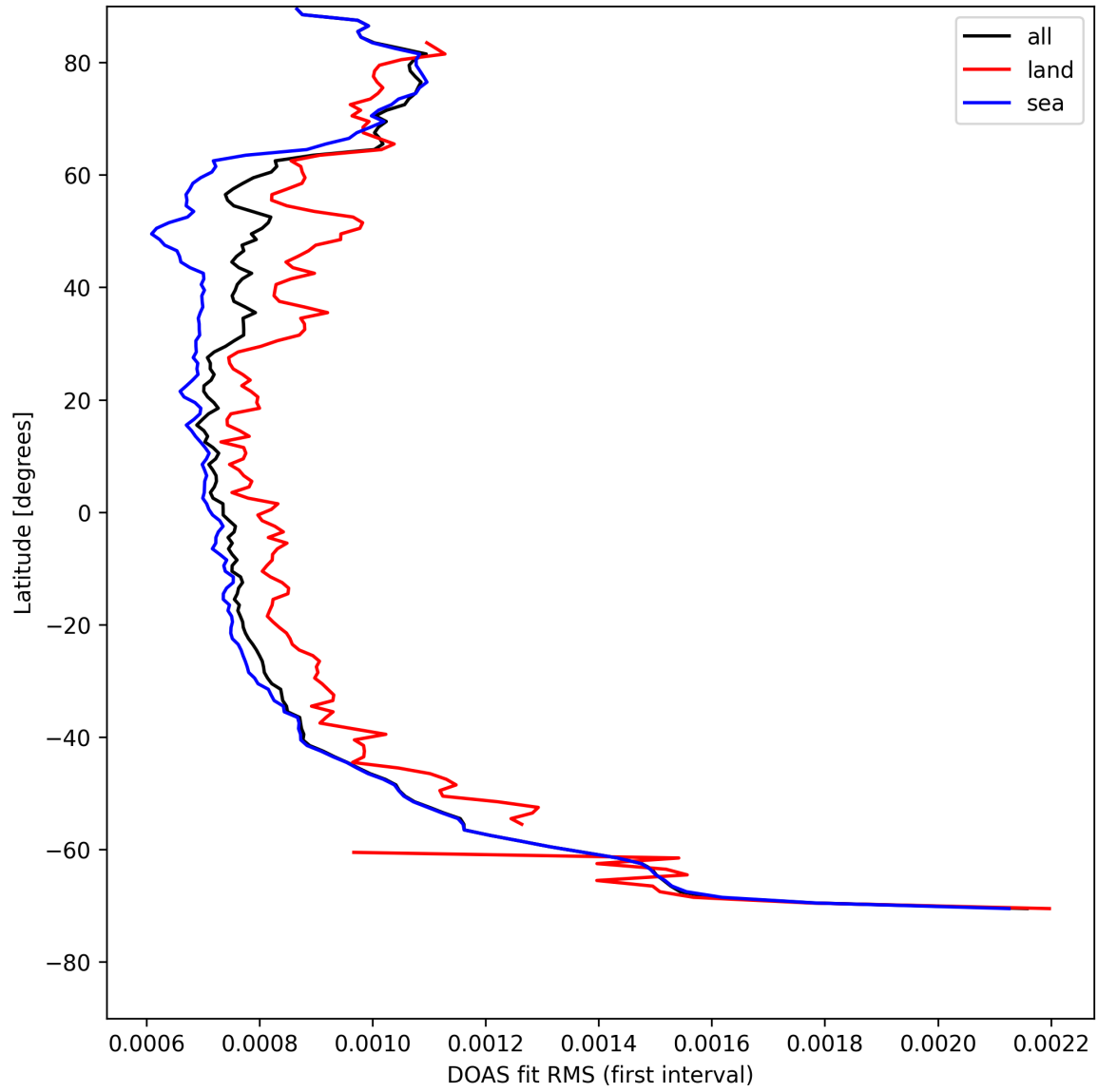
Figure 30: Zonal average of "DOAS fit RMS (first interval)" for 2025-08-14 to 2025-08-15.
