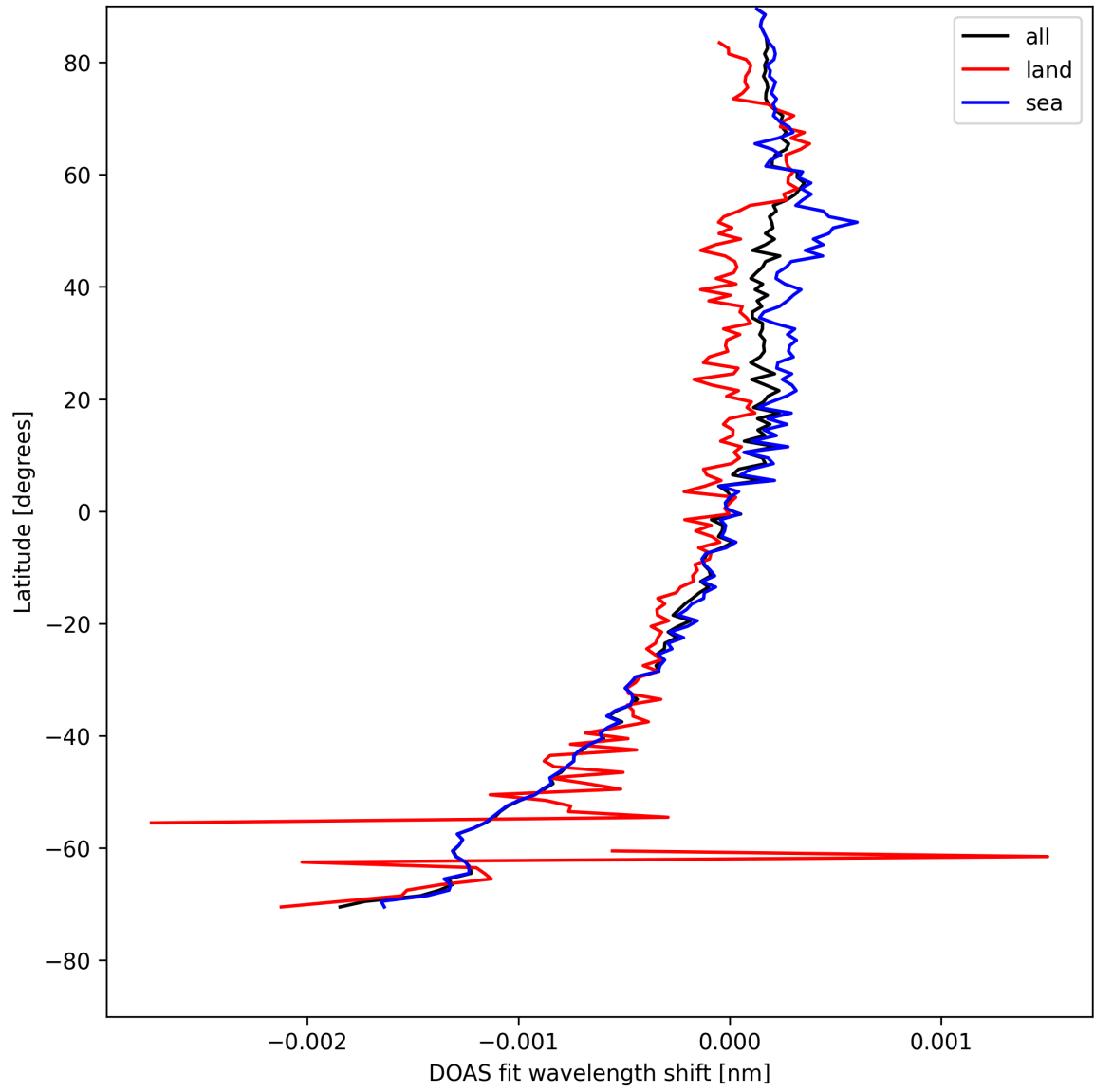
Figure 28: Zonal average of “DOAS fit wavelength shift” for 2025-08-14 to 2025-08-15.
