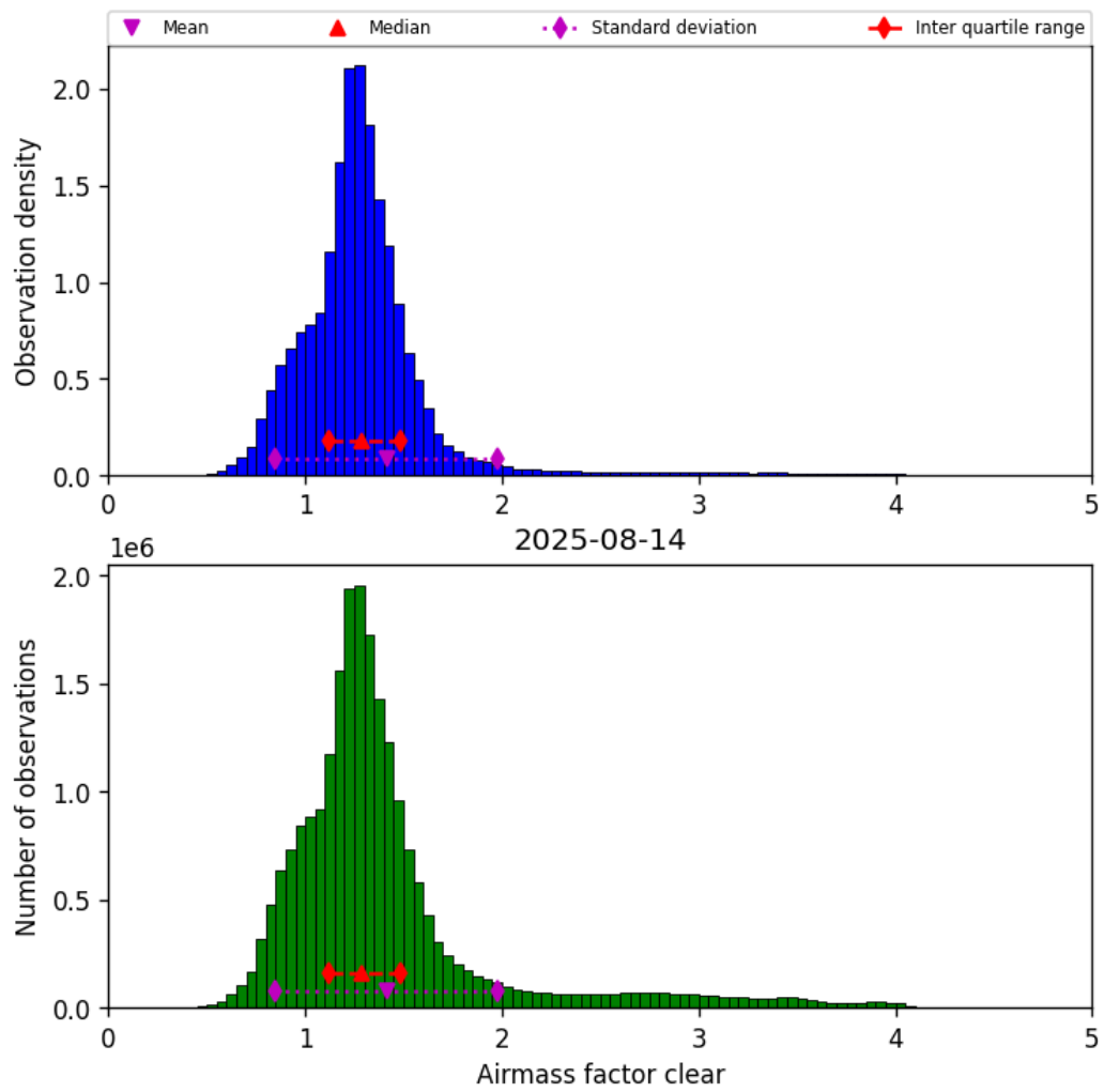
Figure 40: Histogram of “Airmass factor clear” for 2025-08-14 to 2025-08-15
