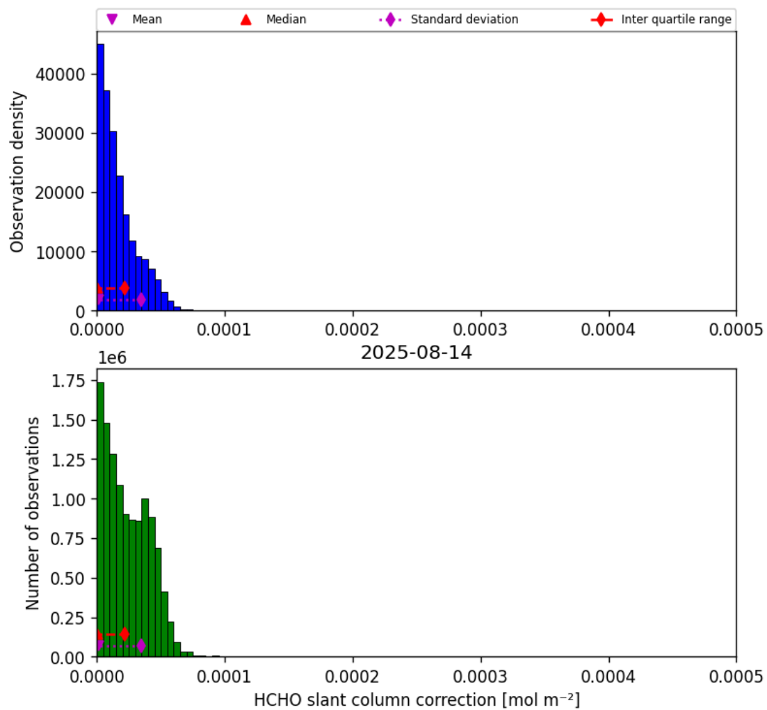
Figure 45: Histogram of “HCHO slant column correction” for 2025-08-14 to 2025-08-15
