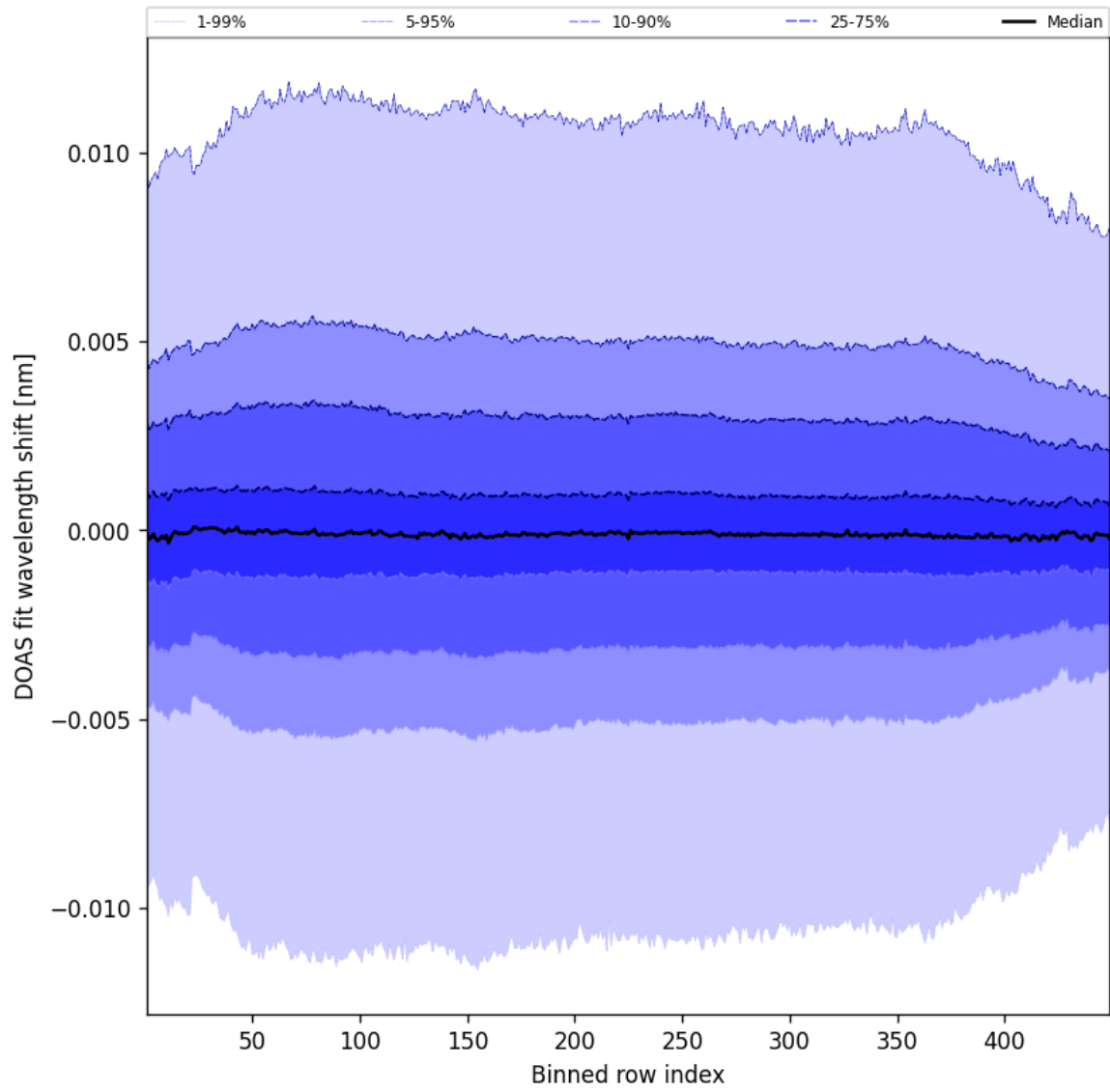
Figure 56: Along track statistics of “DOAS fit wavelength shift” for 2025-08-14 to 2025-08-15
