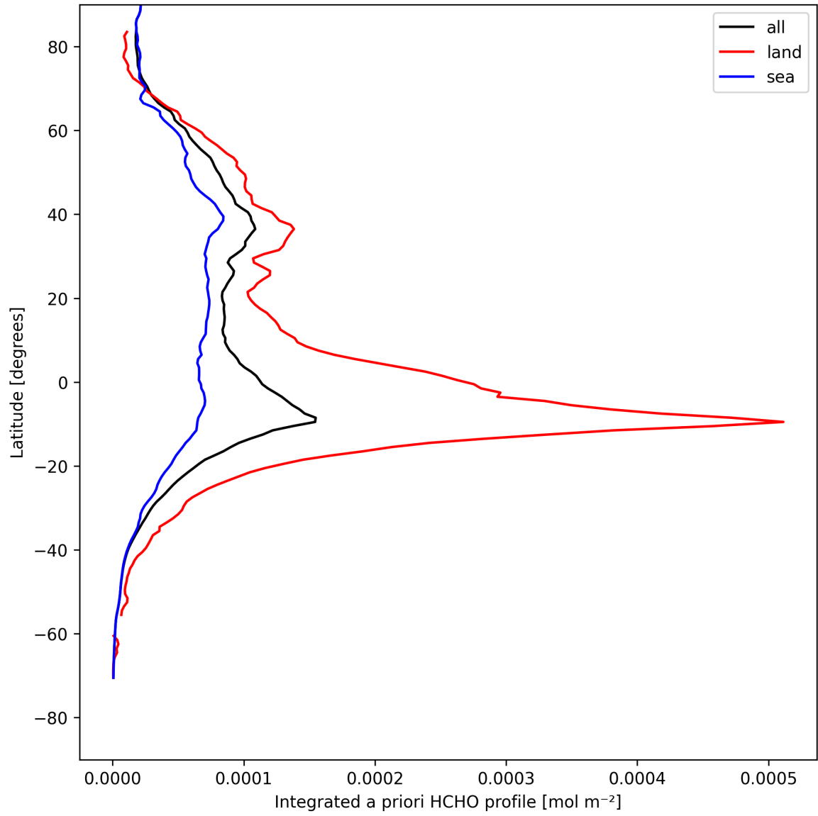
Figure 27: Zonal average of “Integrated a priori HCHO profile” for 2025-08-14 to 2025-08-15.
