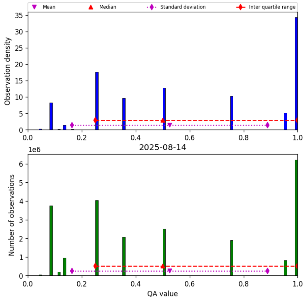
Figure 32: Histogram of “QA value” for 2025-08-14 to 2025-08-15
