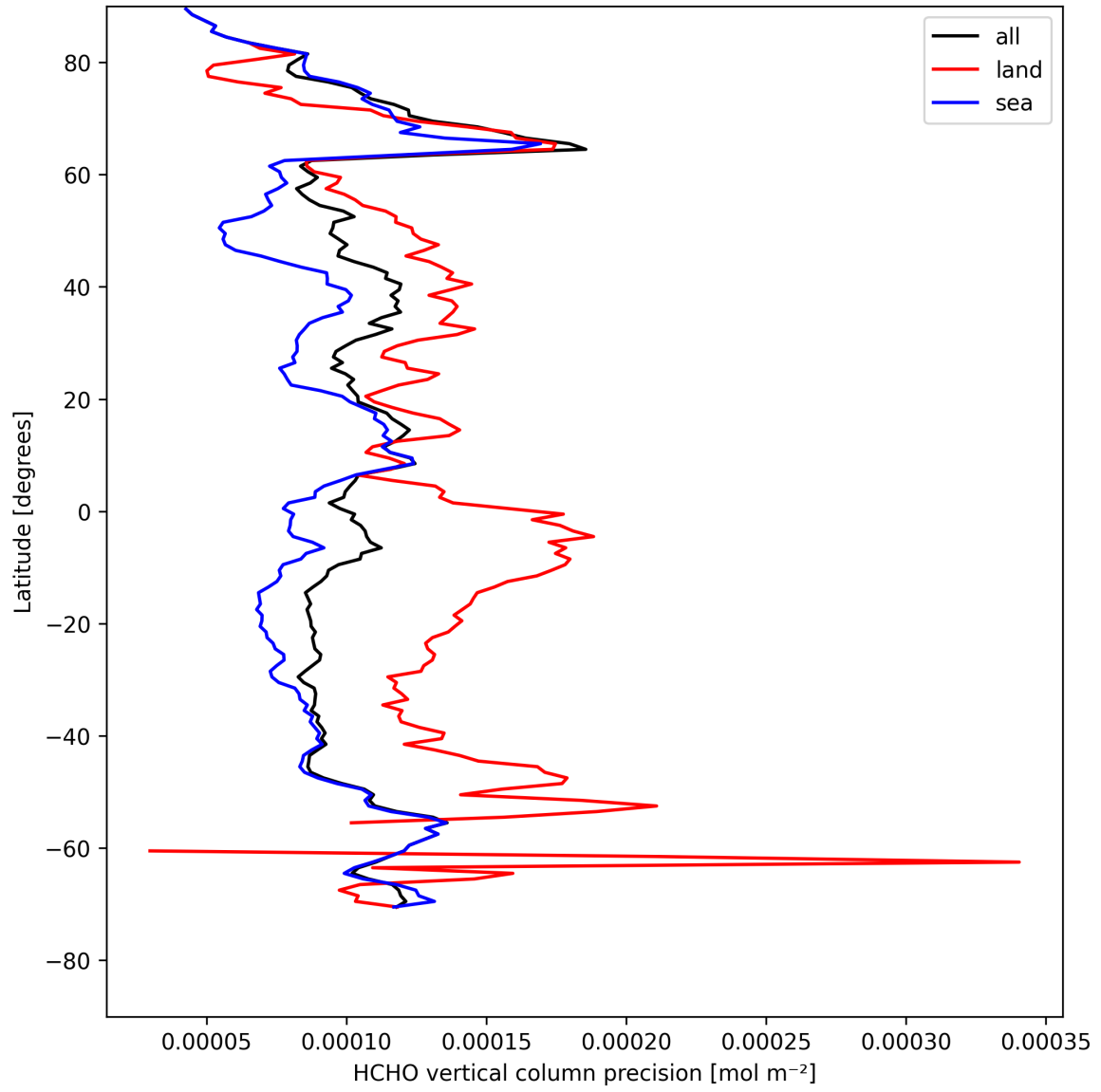
Figure 20: Zonal average of “HCHO vertical column precision” for 2025-08-14 to 2025-08-15.
