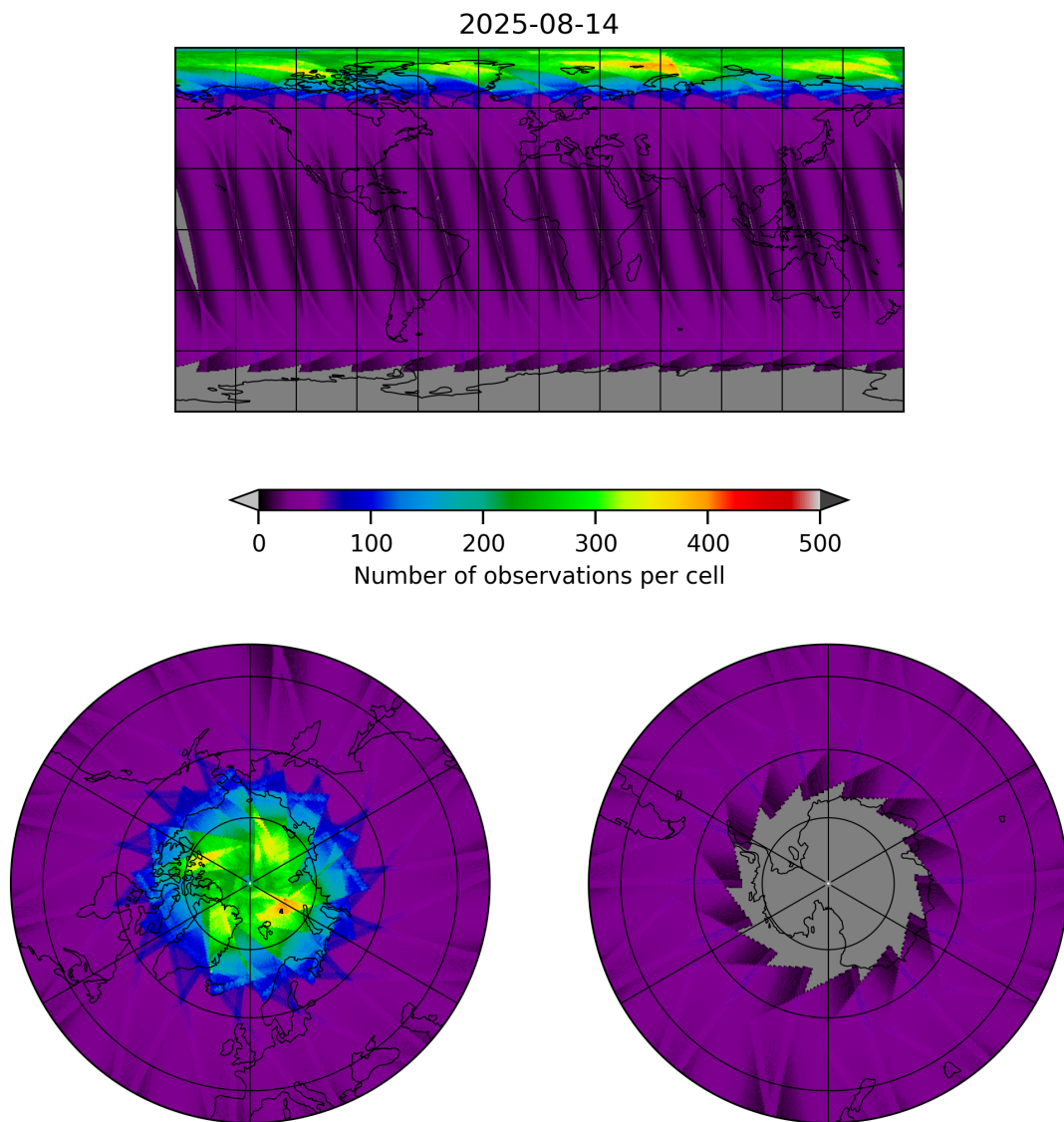
Figure 17: Map of the number of observations for 2025-08-14 to 2025-08-15
