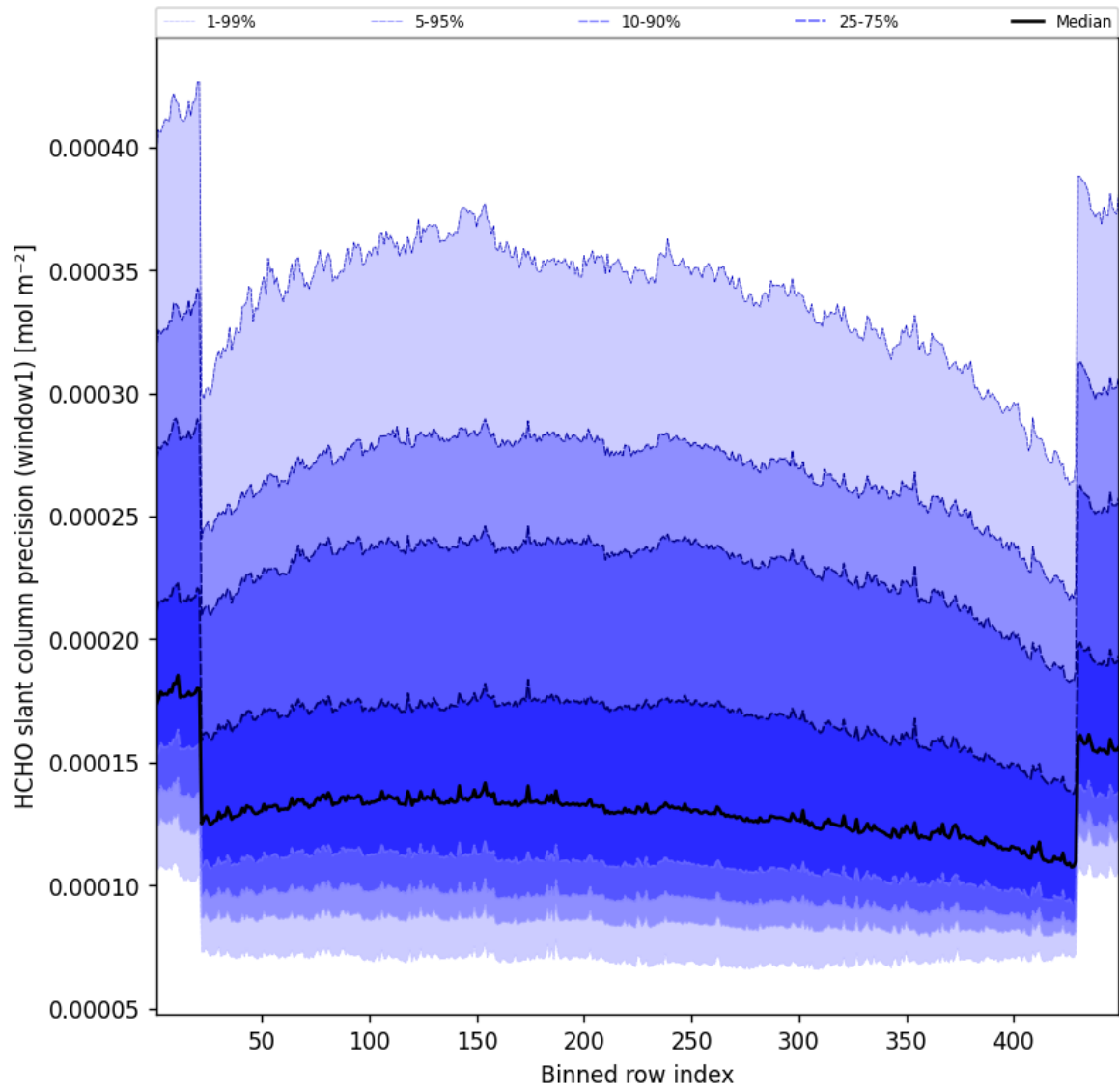
Figure 51: Along track statistics of “HCHO slant column precision (window1)” for 2025-08-14 to 2025-08-15
