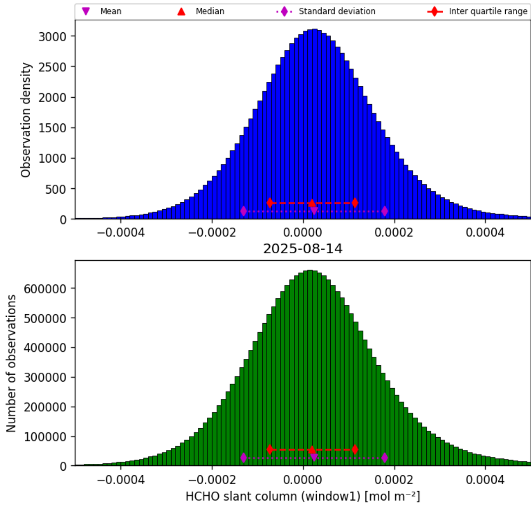
Figure 36: Histogram of “HCHO slant column (window1)” for 2025-08-14 to 2025-08-15
