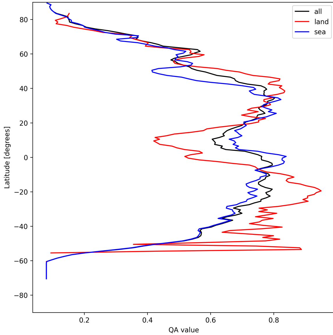
Figure 18: Zonal average of “QA value” for 2025-08-14 to 2025-08-15.
