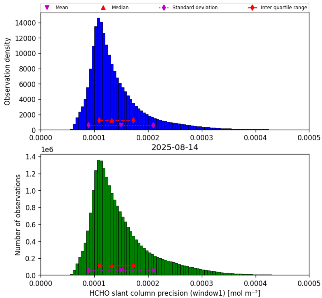
Figure 37: Histogram of “HCHO slant column precision (window1)” for 2025-08-14 to 2025-08-15
