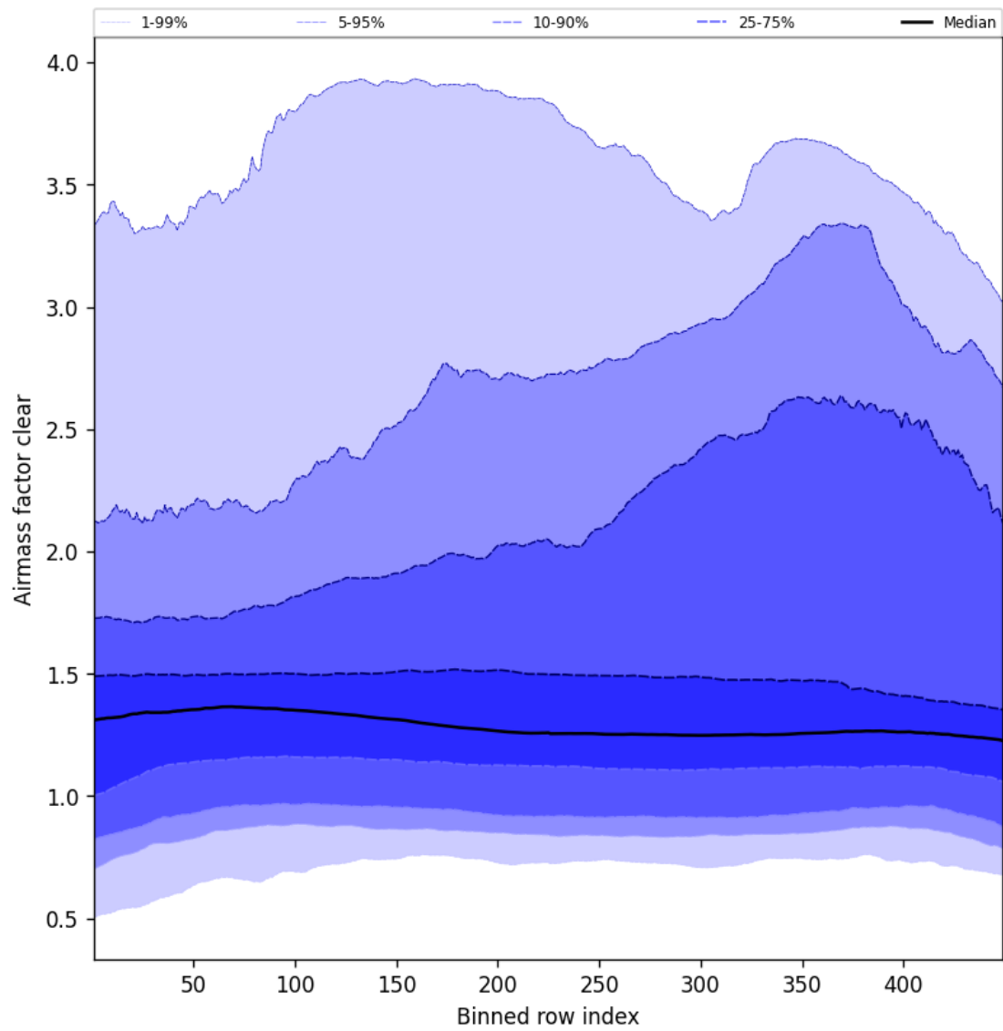
Figure 54: Along track statistics of “Airmass factor clear” for 2025-08-14 to 2025-08-15
