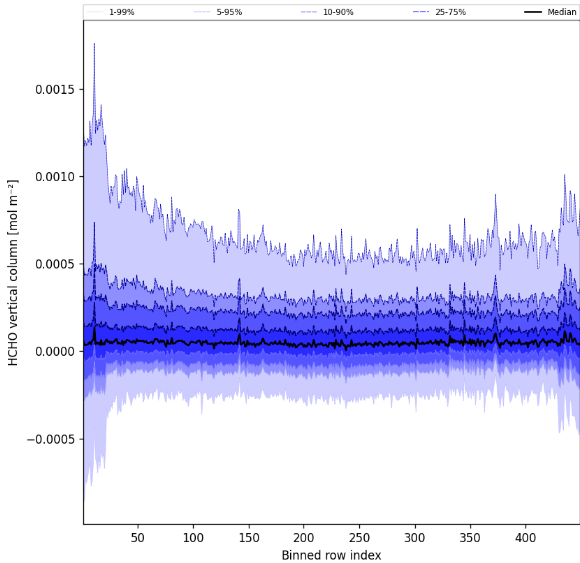
Figure 47: Along track statistics of “HCHO vertical column” for 2025-08-14 to 2025-08-15
