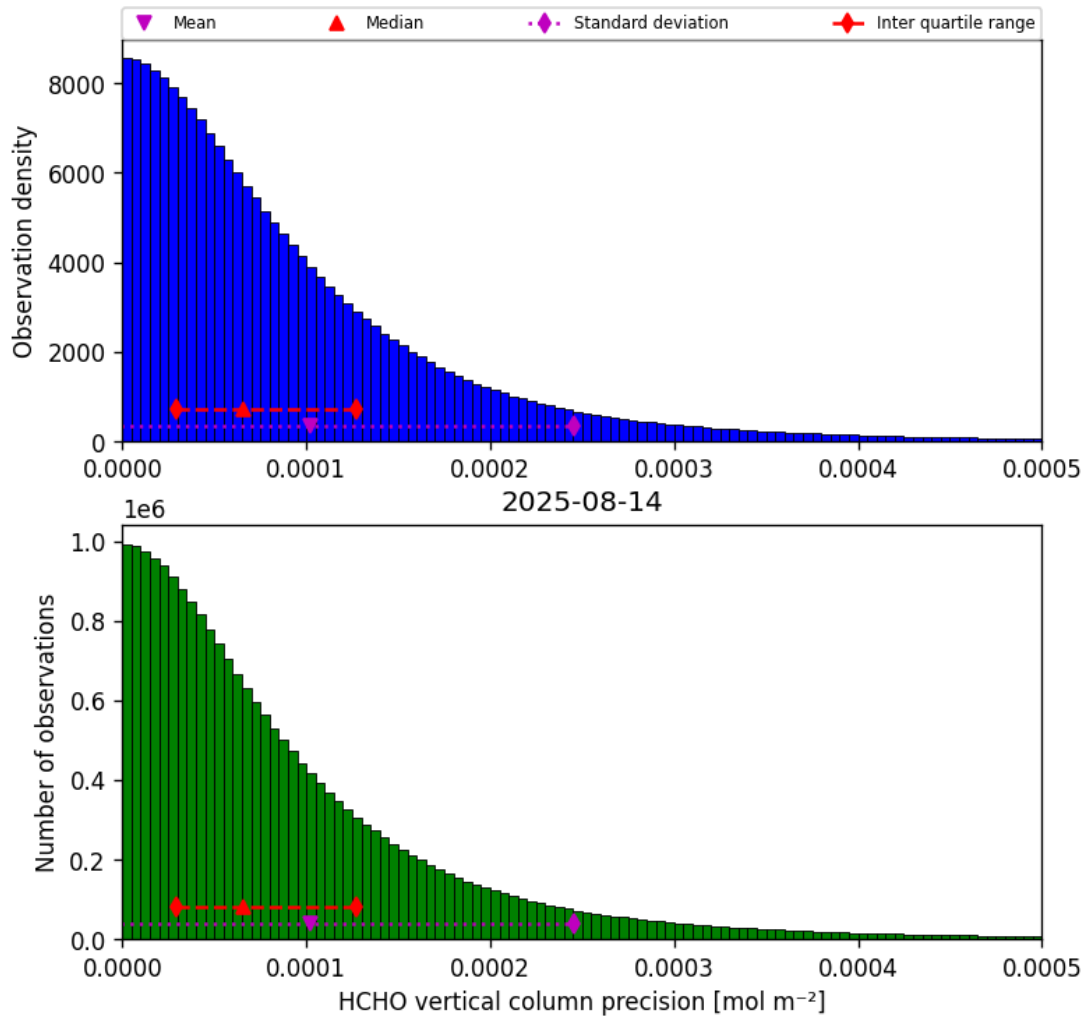
Figure 34: Histogram of “HCHO vertical column precision” for 2025-08-14 to 2025-08-15
