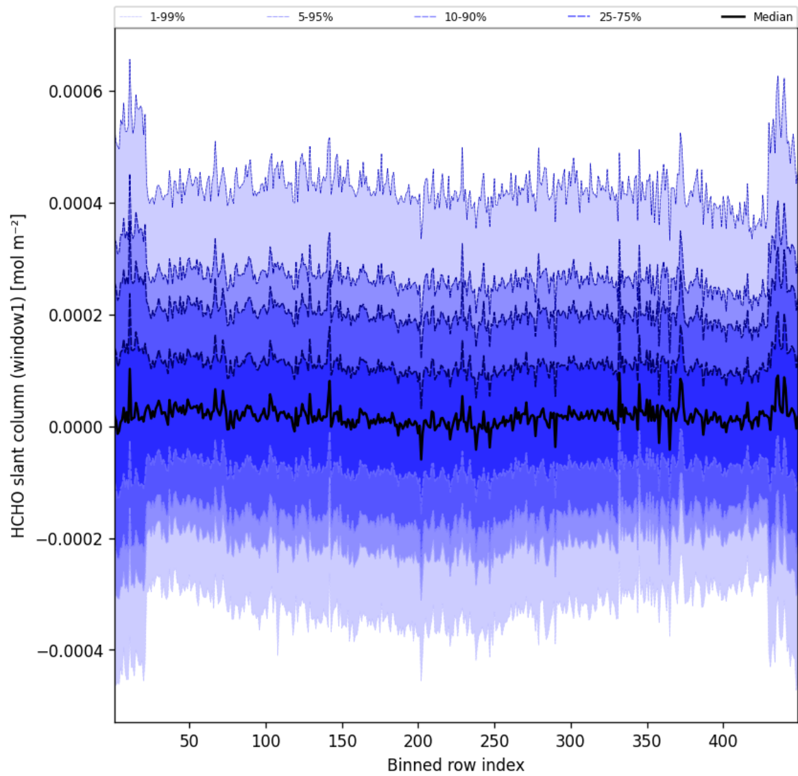
Figure 50: Along track statistics of "HCHO slant column (window1)" for 2025-08-15 to 2025-08-16
