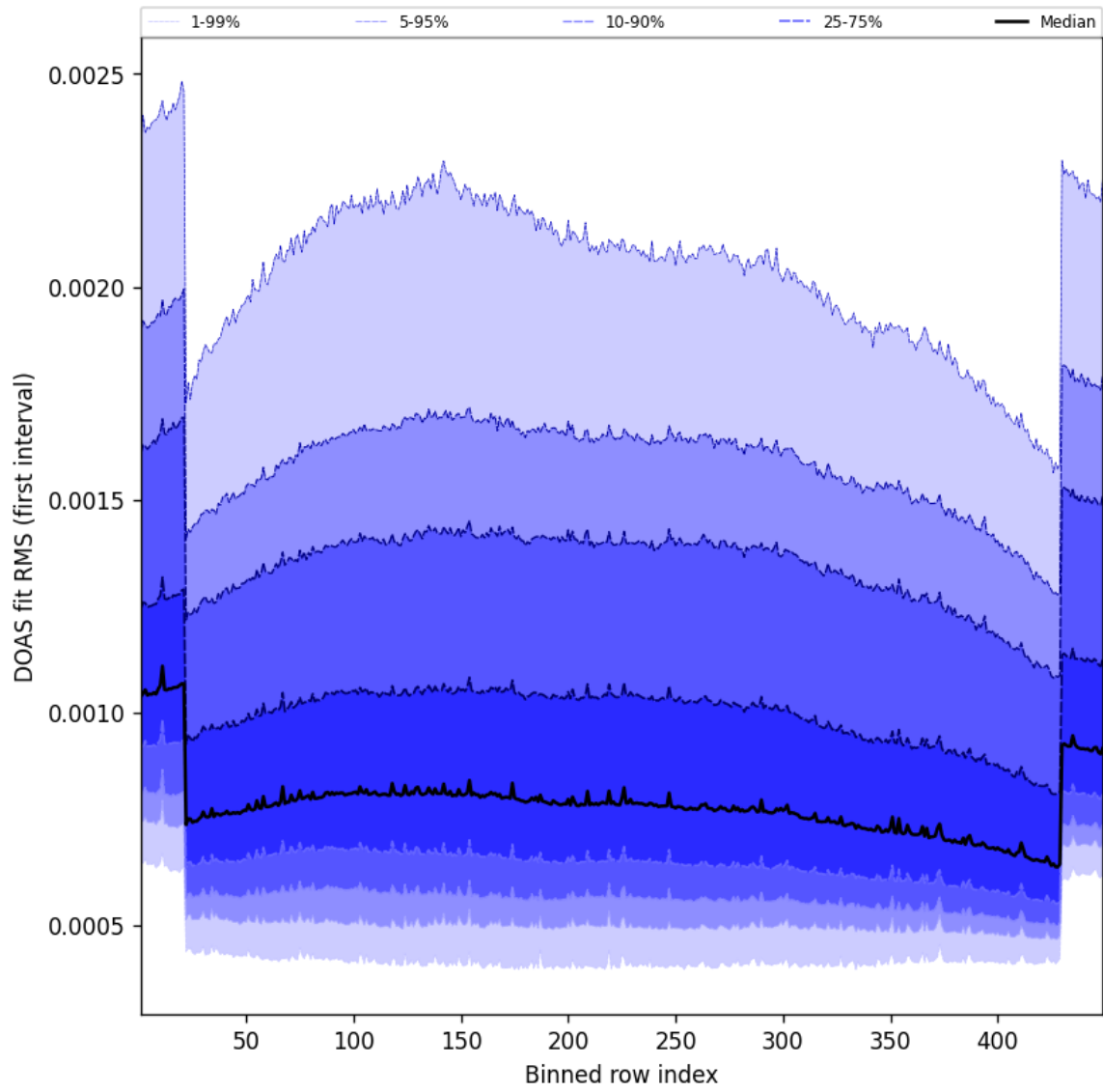
Figure 58: Along track statistics of “DOAS fit RMS (first interval)” for 2025-08-15 to 2025-08-16
