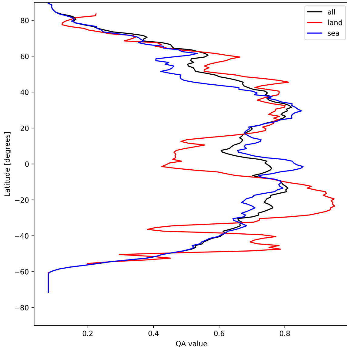
Figure 18: Zonal average of “QA value” for 2025-08-15 to 2025-08-16.
