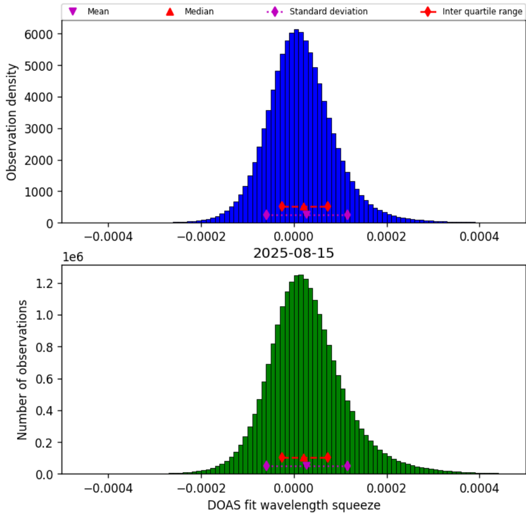
Figure 43: Histogram of “DOAS fit wavelength squeeze” for 2025-08-15 to 2025-08-16
