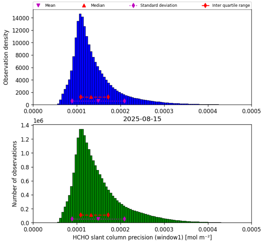
Figure 37: Histogram of “HCHO slant column precision (window1)” for 2025-08-15 to 2025-08-16
