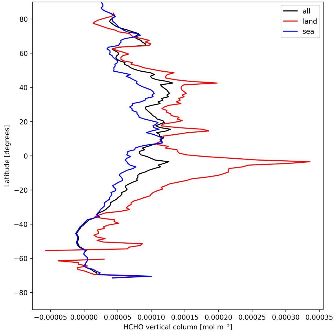
Figure 19: Zonal average of “HCHO vertical column” for 2025-08-15 to 2025-08-16.
