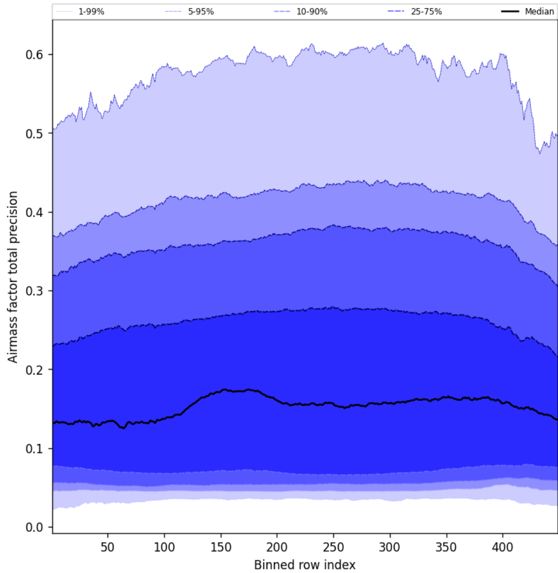
Figure 53: Along track statistics of “Airmass factor total precision” for 2025-08-15 to 2025-08-16
