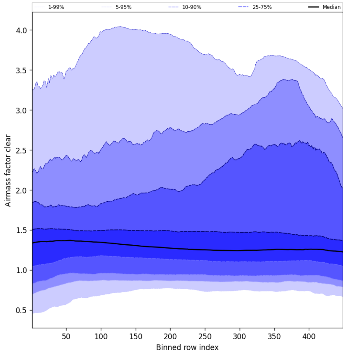
Figure 54: Along track statistics of “Airmass factor clear” for 2025-08-15 to 2025-08-16
