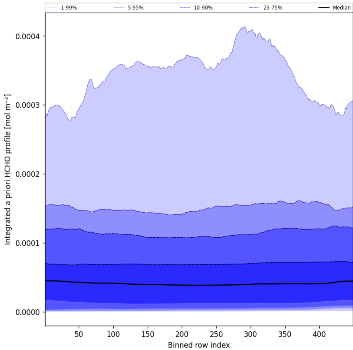
Figure 55: Along track statistics of "Integrated a priori HCHO profile" for 2025-08-15 to 2025-08-16
