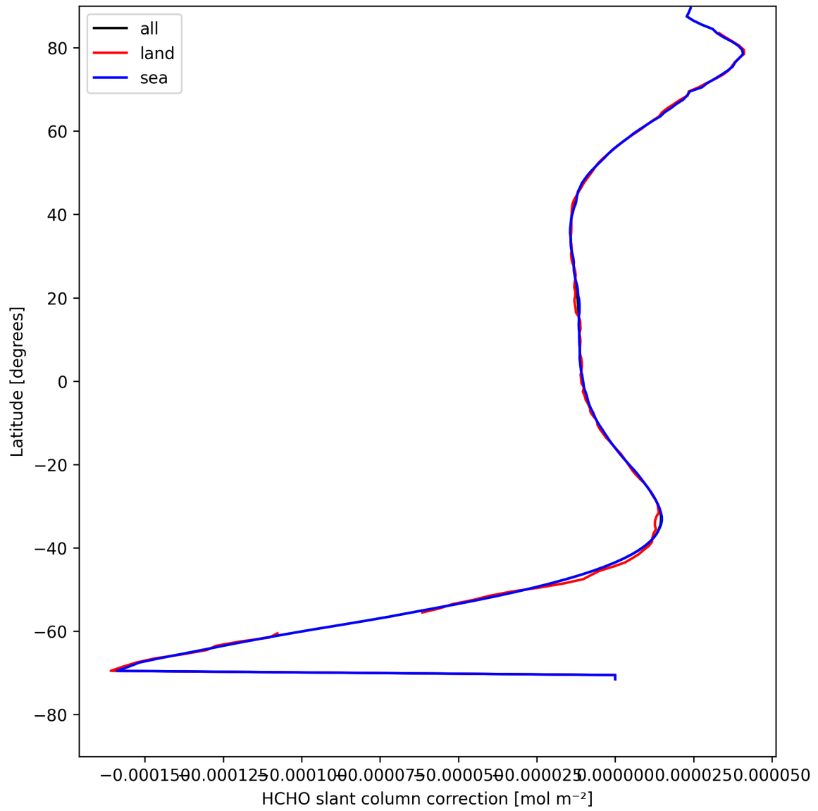
Figure 31: Zonal average of “HCHO slant column correction” for 2025-08-15 to 2025-08-16.
