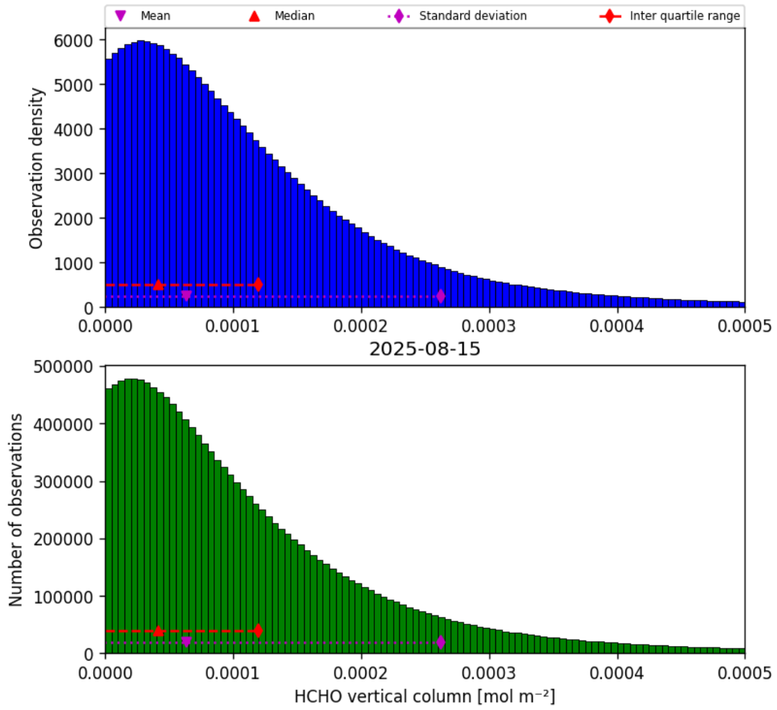
Figure 33: Histogram of “HCHO vertical column” for 2025-08-15 to 2025-08-16
