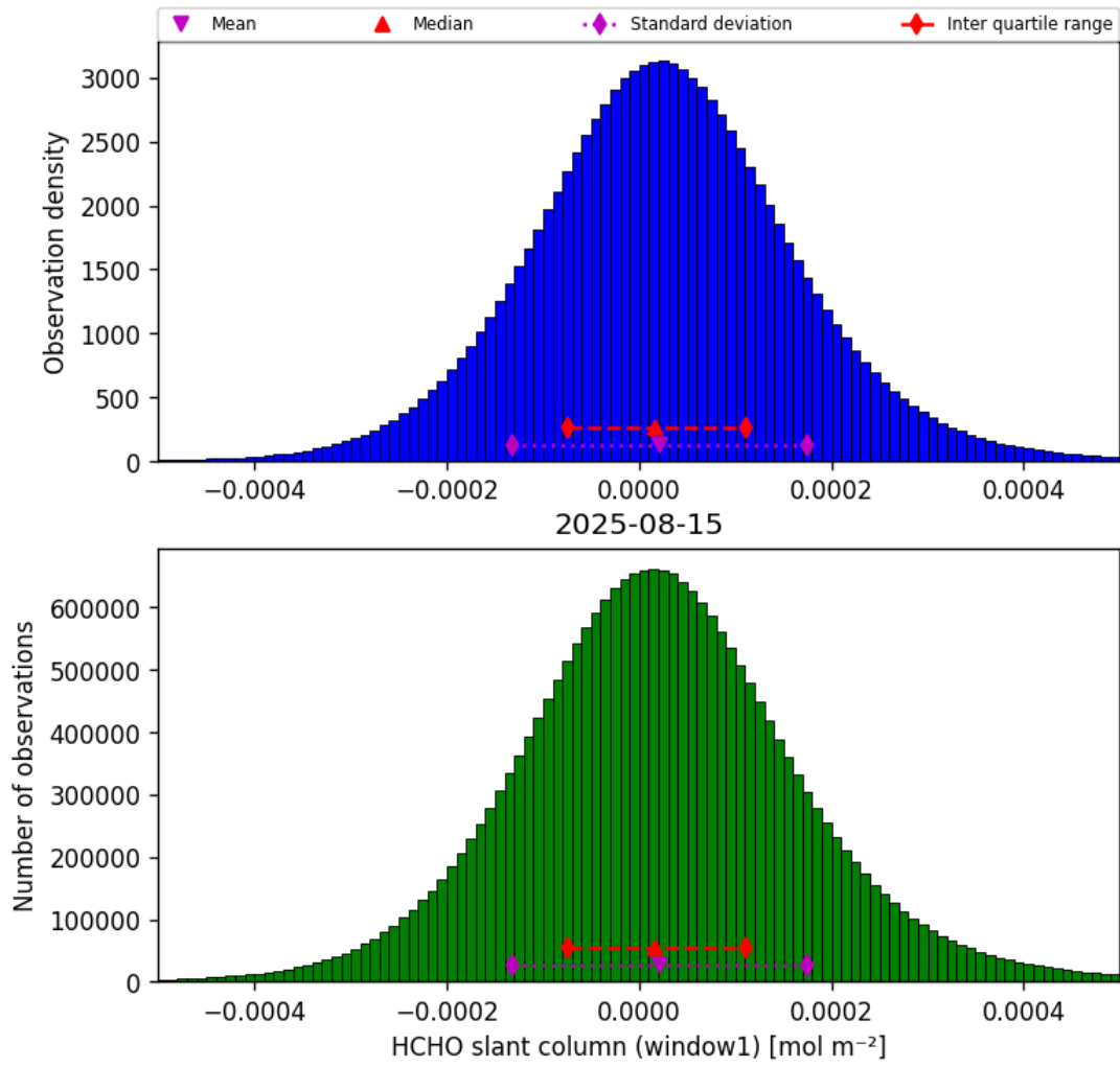
Figure 36: Histogram of “HCHO slant column (window1)” for 2025-08-15 to 2025-08-16
