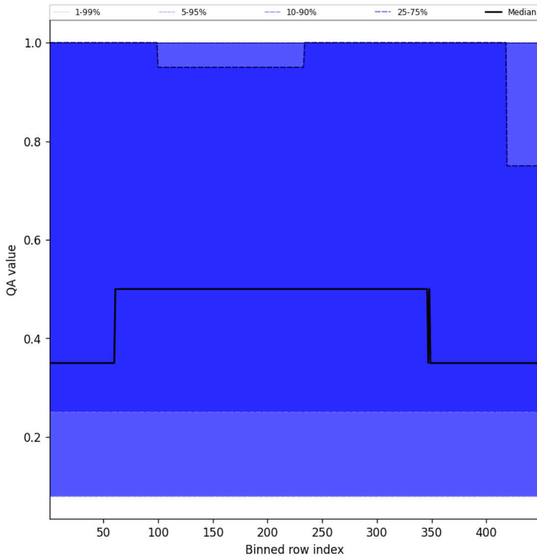
Figure 46: Along track statistics of “QA value” for 2025-08-15 to 2025-08-16
