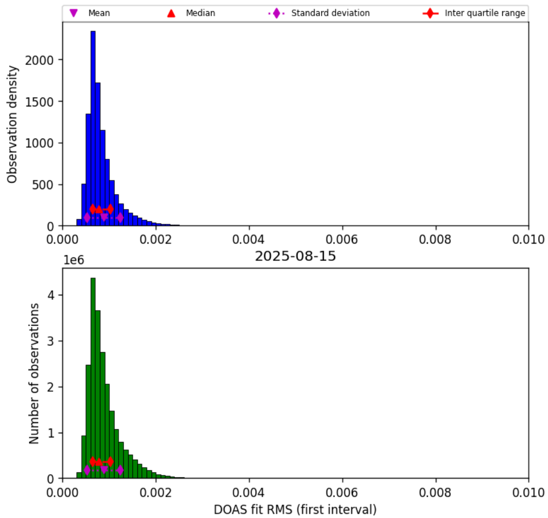
Figure 44: Histogram of “DOAS fit RMS (first interval)” for 2025-08-15 to 2025-08-16
