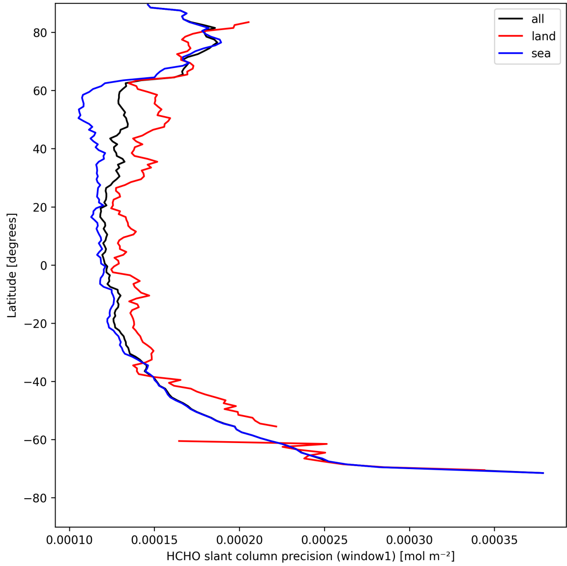
Figure 23: Zonal average of “HCHO slant column precision (window1)” for 2025-08-15 to 2025-08-16.
