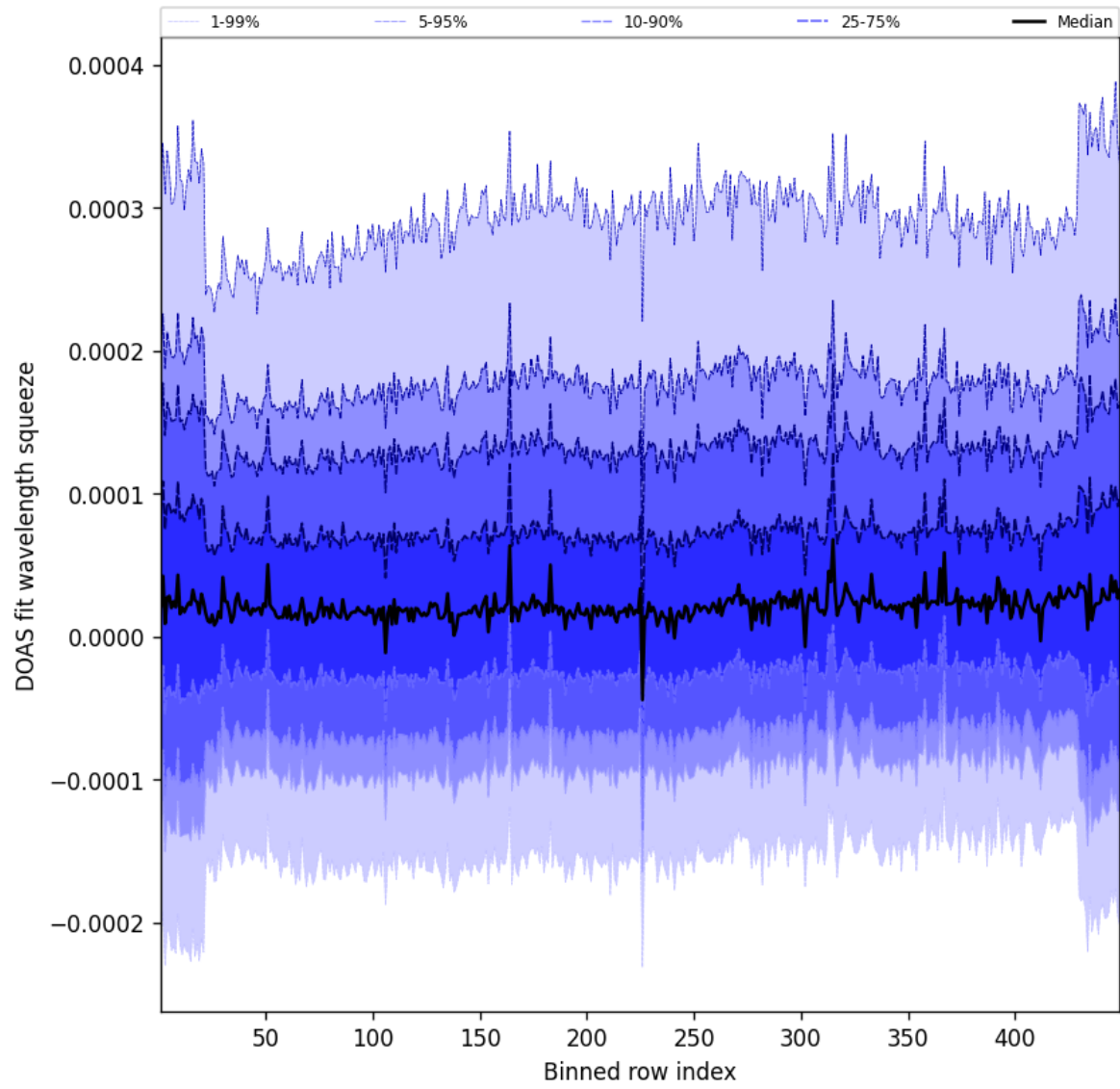
Figure 57: Along track statistics of “DOAS fit wavelength squeeze” for 2025-08-15 to 2025-08-16
