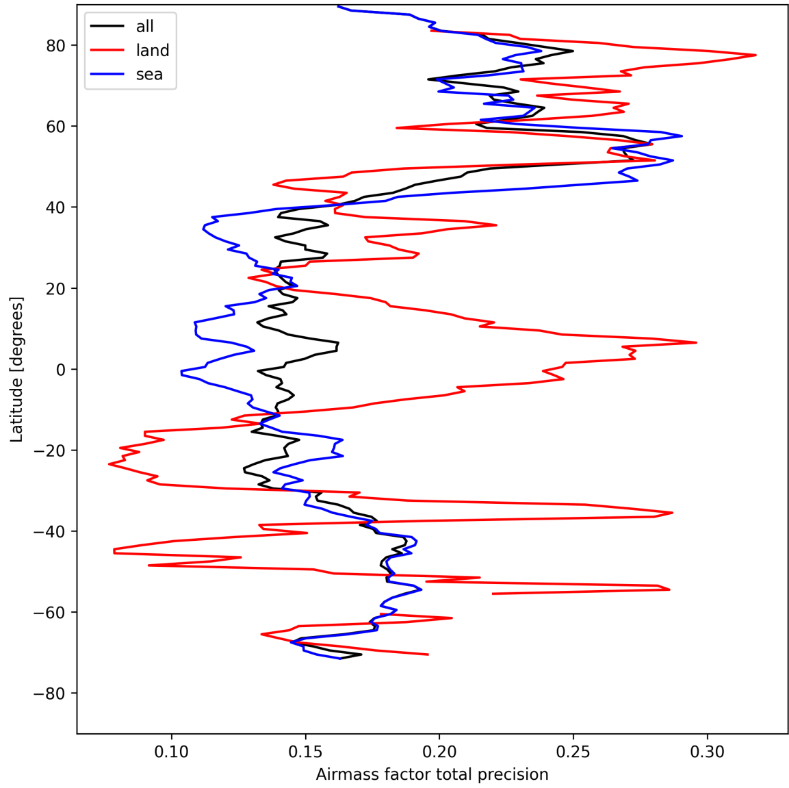
Figure 25: Zonal average of “Airmass factor total precision” for 2025-08-15 to 2025-08-16.
