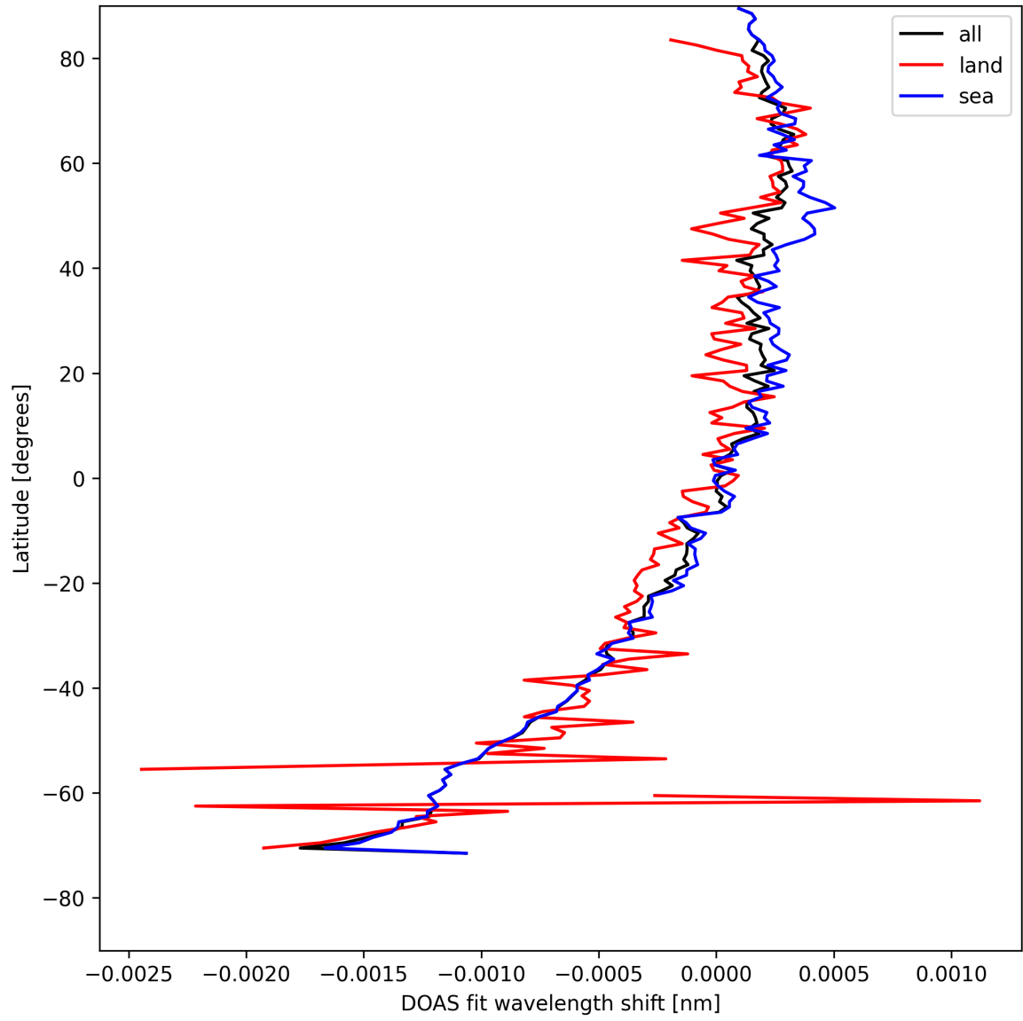
Figure 28: Zonal average of “DOAS fit wavelength shift” for 2025-08-15 to 2025-08-16.
