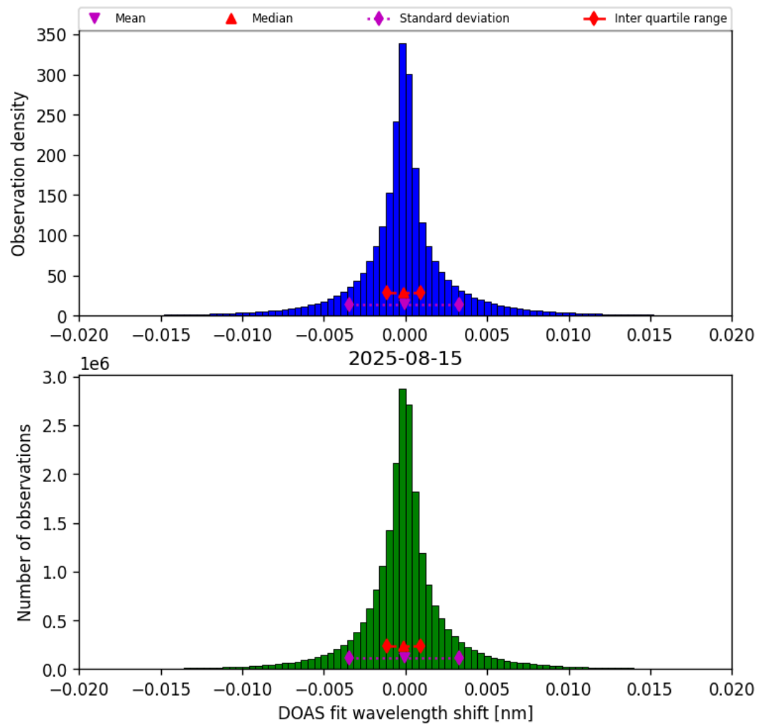
Figure 42: Histogram of “DOAS fit wavelength shift” for 2025-08-15 to 2025-08-16
