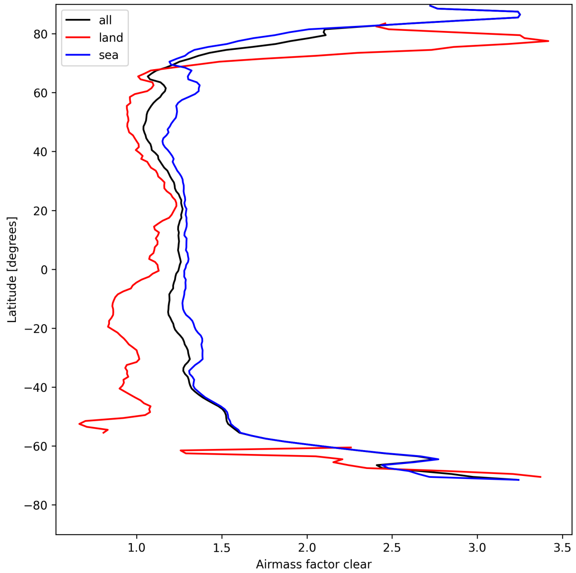
Figure 26: Zonal average of “Airmass factor clear” for 2025-08-15 to 2025-08-16.
