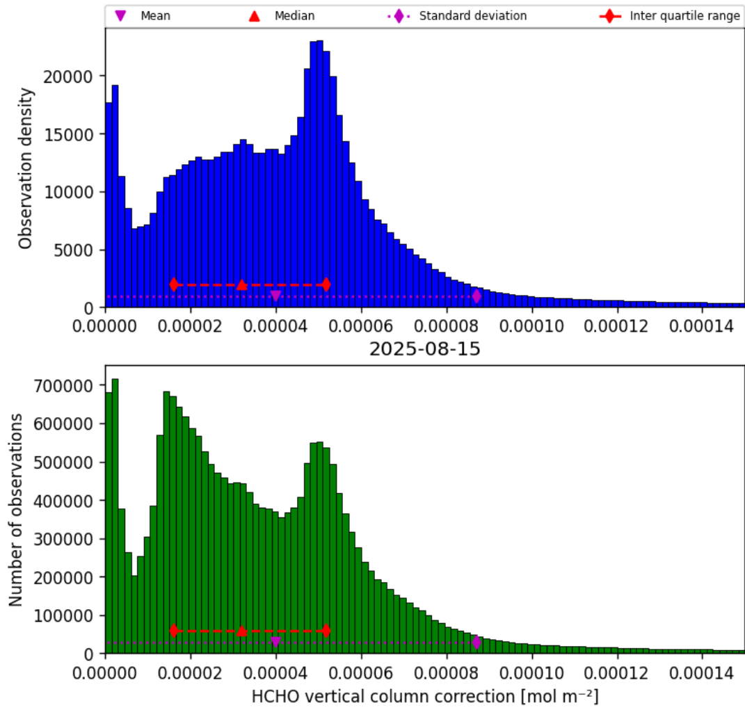
Figure 35: Histogram of “HCHO vertical column correction” for 2025-08-15 to 2025-08-16
