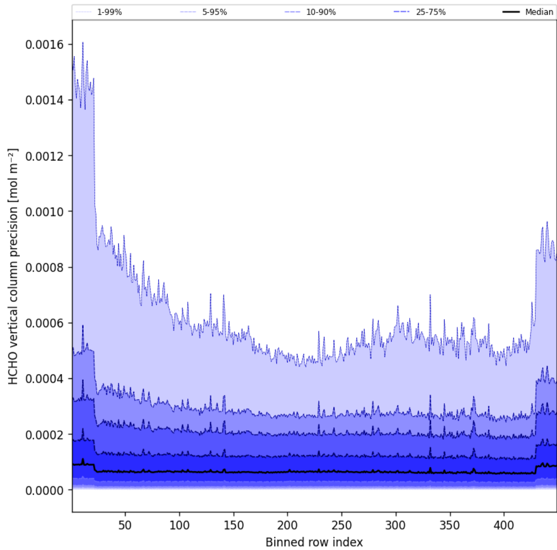
Figure 48: Along track statistics of “HCHO vertical column precision” for 2025-08-15 to 2025-08-16
