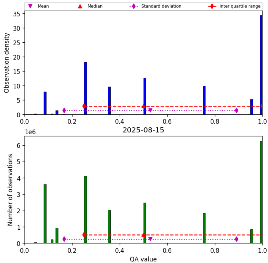
Figure 32: Histogram of “QA value” for 2025-08-15 to 2025-08-16
