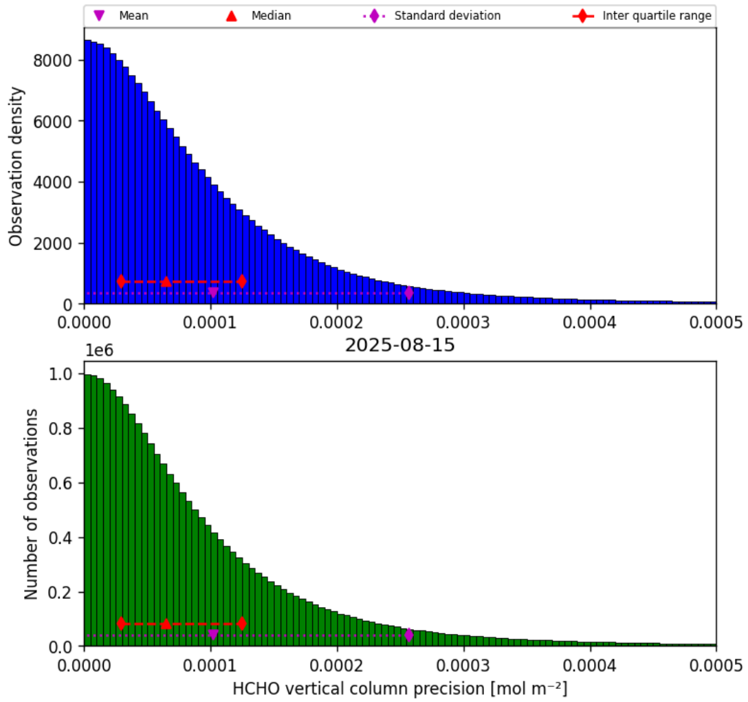
Figure 34: Histogram of “HCHO vertical column precision” for 2025-08-15 to 2025-08-16
