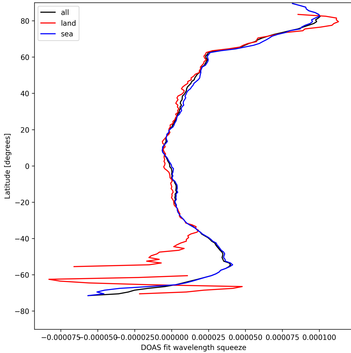
Figure 29: Zonal average of “DOAS fit wavelength squeeze” for 2025-08-15 to 2025-08-16.
