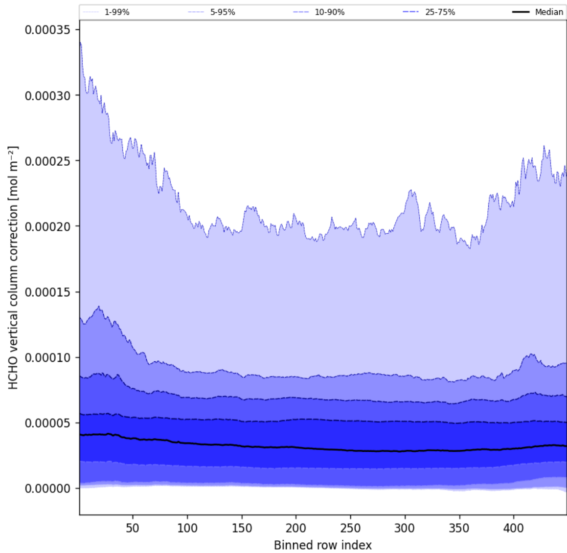
Figure 49: Along track statistics of “HCHO vertical column correction” for 2025-08-15 to 2025-08-16
