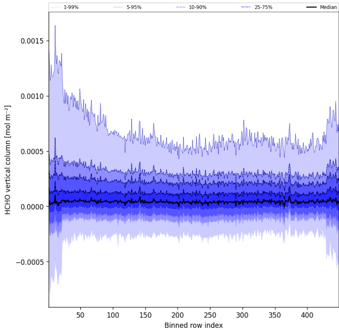
Figure 47: Along track statistics of “HCHO vertical column” for 2025-08-15 to 2025-08-16
