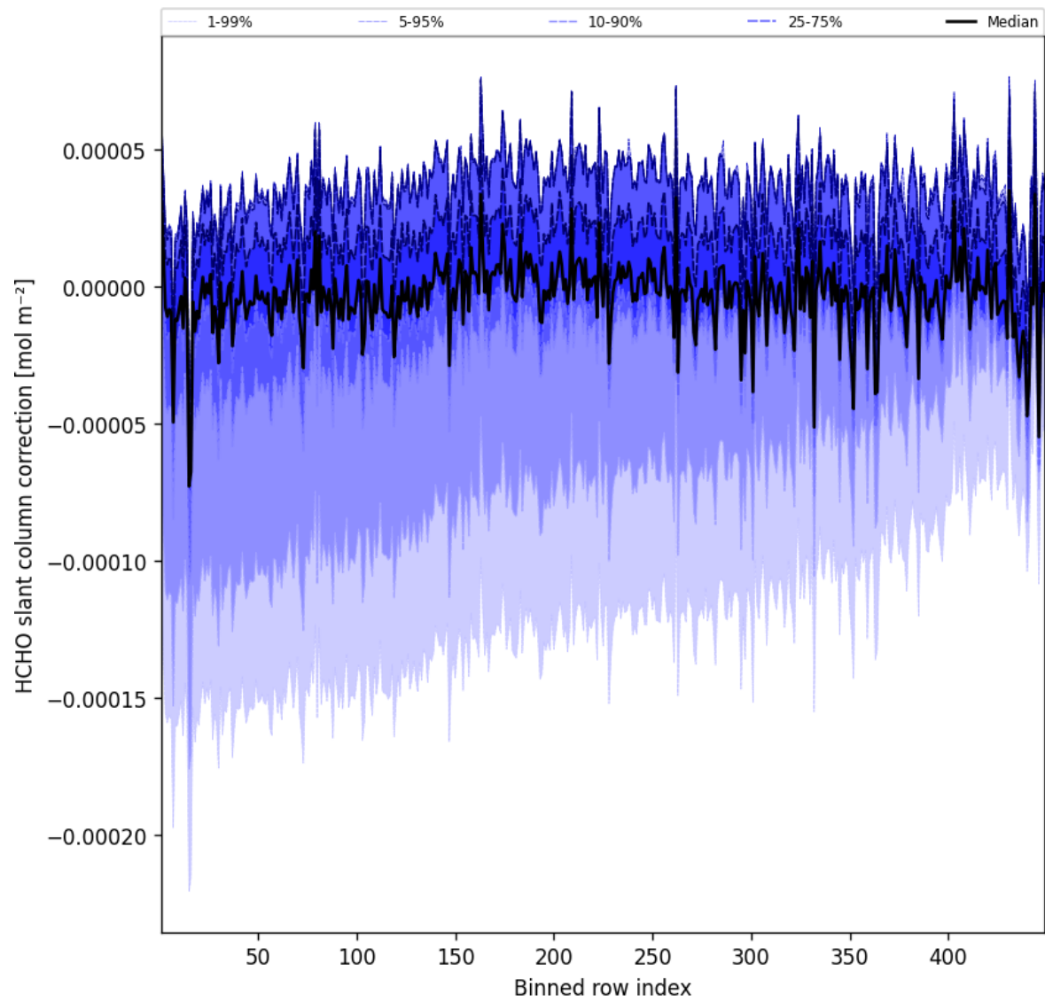
Figure 59: Along track statistics of “HCHO slant column correction” for 2025-08-15 to 2025-08-16
