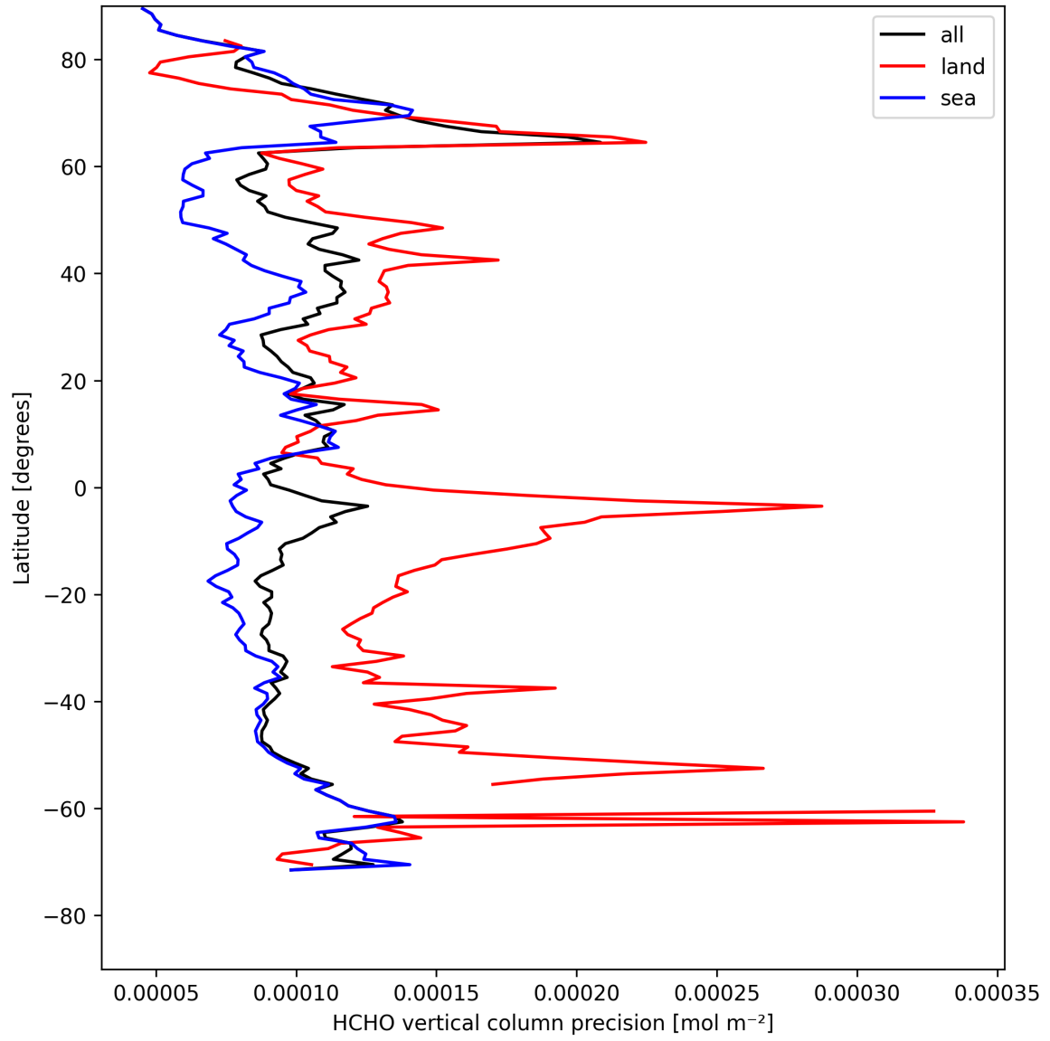
Figure 20: Zonal average of “HCHO vertical column precision” for 2025-08-15 to 2025-08-16.
