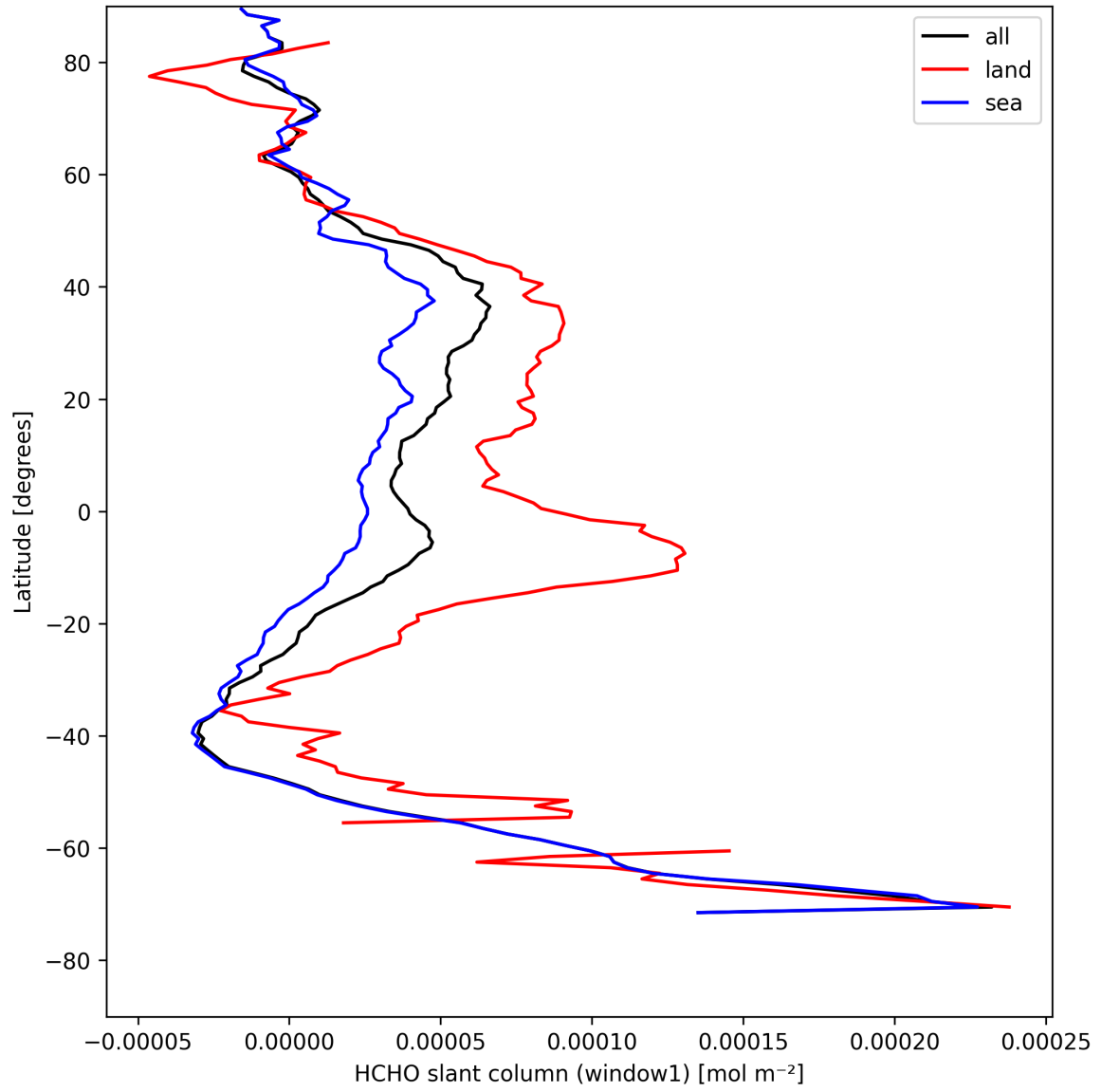
Figure 22: Zonal average of “HCHO slant column (window1)” for 2025-08-15 to 2025-08-16.
