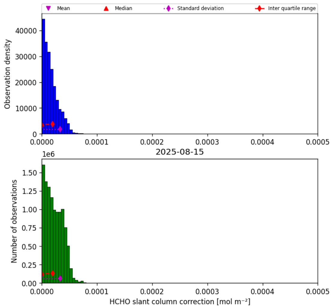
Figure 45: Histogram of “HCHO slant column correction” for 2025-08-15 to 2025-08-16
