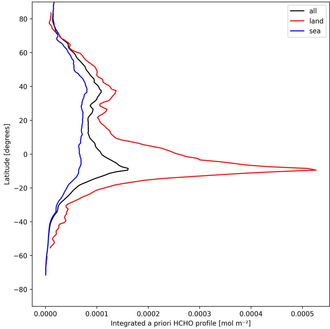
Figure 27: Zonal average of “Integrated a priori HCHO profile” for 2025-08-15 to 2025-08-16.
