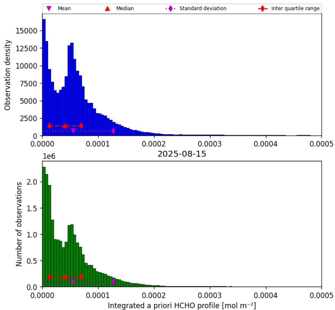
Figure 41: Histogram of “Integrated a priori HCHO profile” for 2025-08-15 to 2025-08-16
