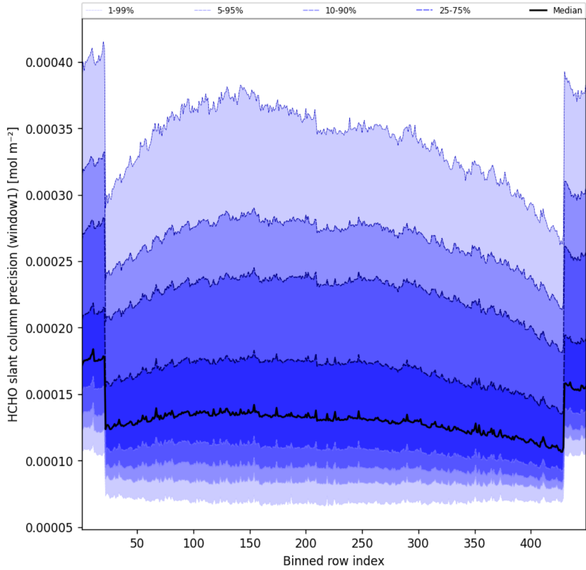
Figure 51: Along track statistics of “HCHO slant column precision (window1)” for 2025-08-15 to 2025-08-16
