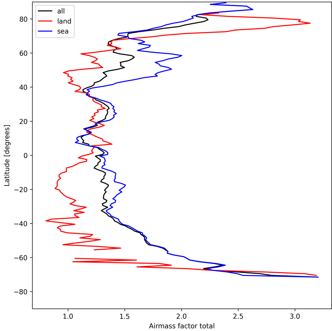
Figure 24: Zonal average of “Airmass factor total” for 2025-08-15 to 2025-08-16.
