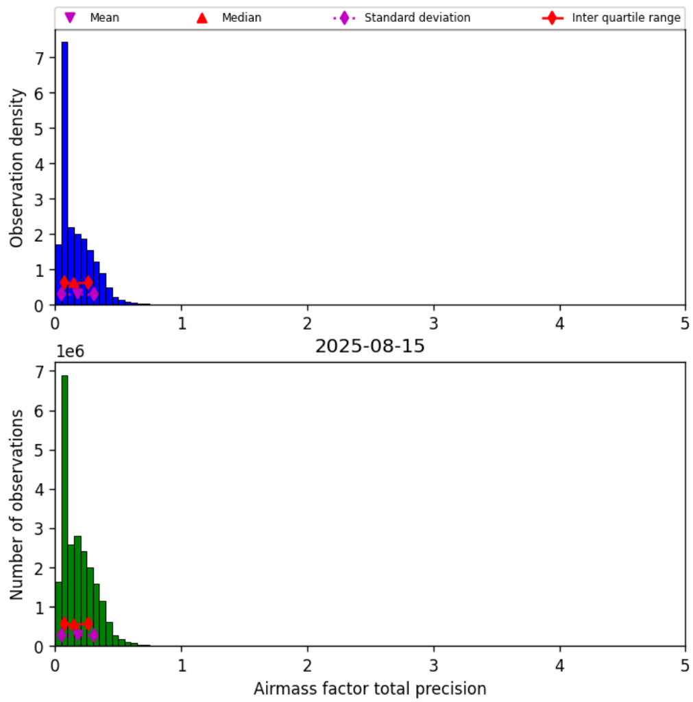
Figure 39: Histogram of “Airmass factor total precision” for 2025-08-15 to 2025-08-16
