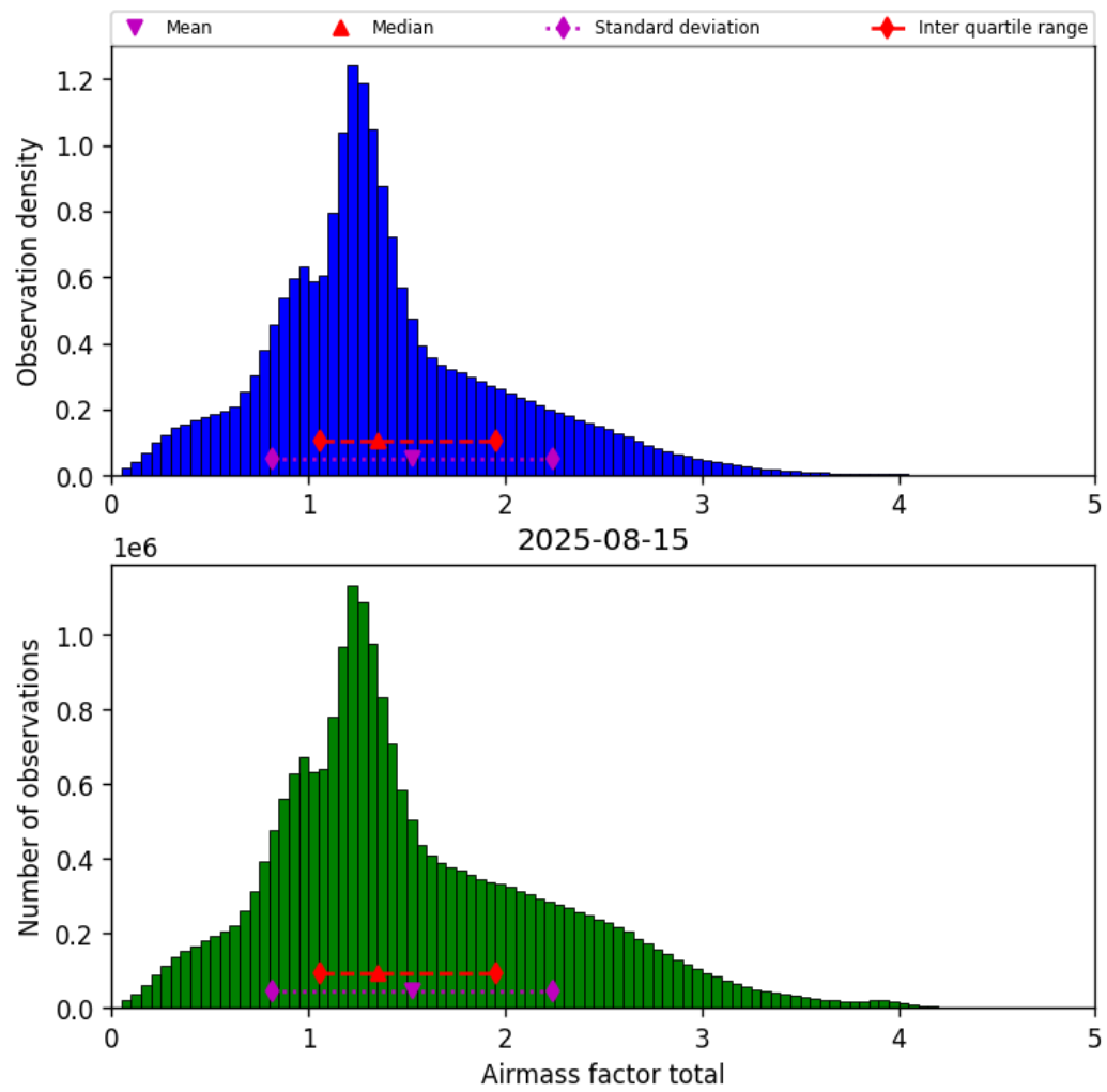
Figure 38: Histogram of “Airmass factor total” for 2025-08-15 to 2025-08-16
