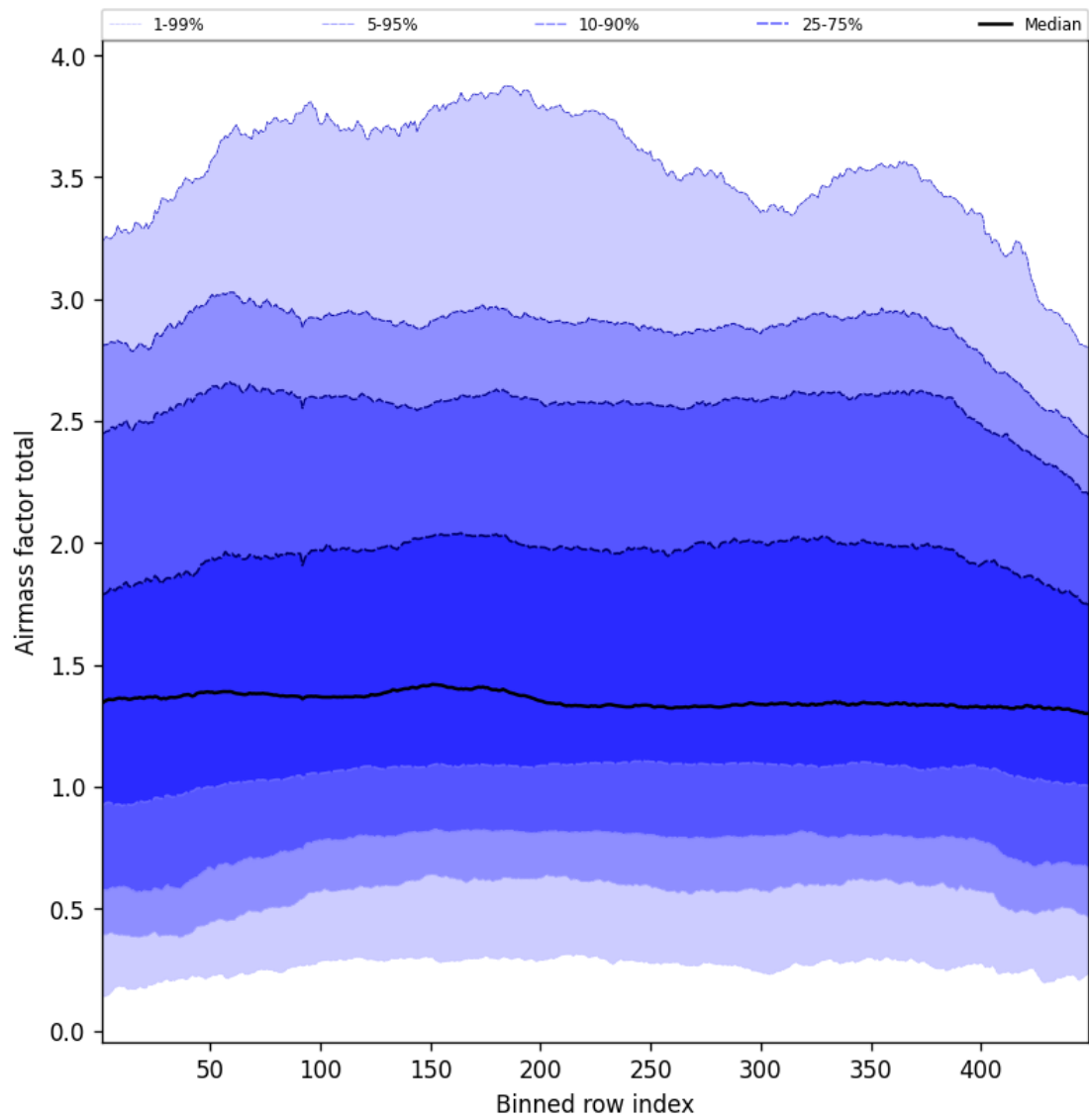
Figure 52: Along track statistics of “Airmass factor total” for 2025-08-15 to 2025-08-16
