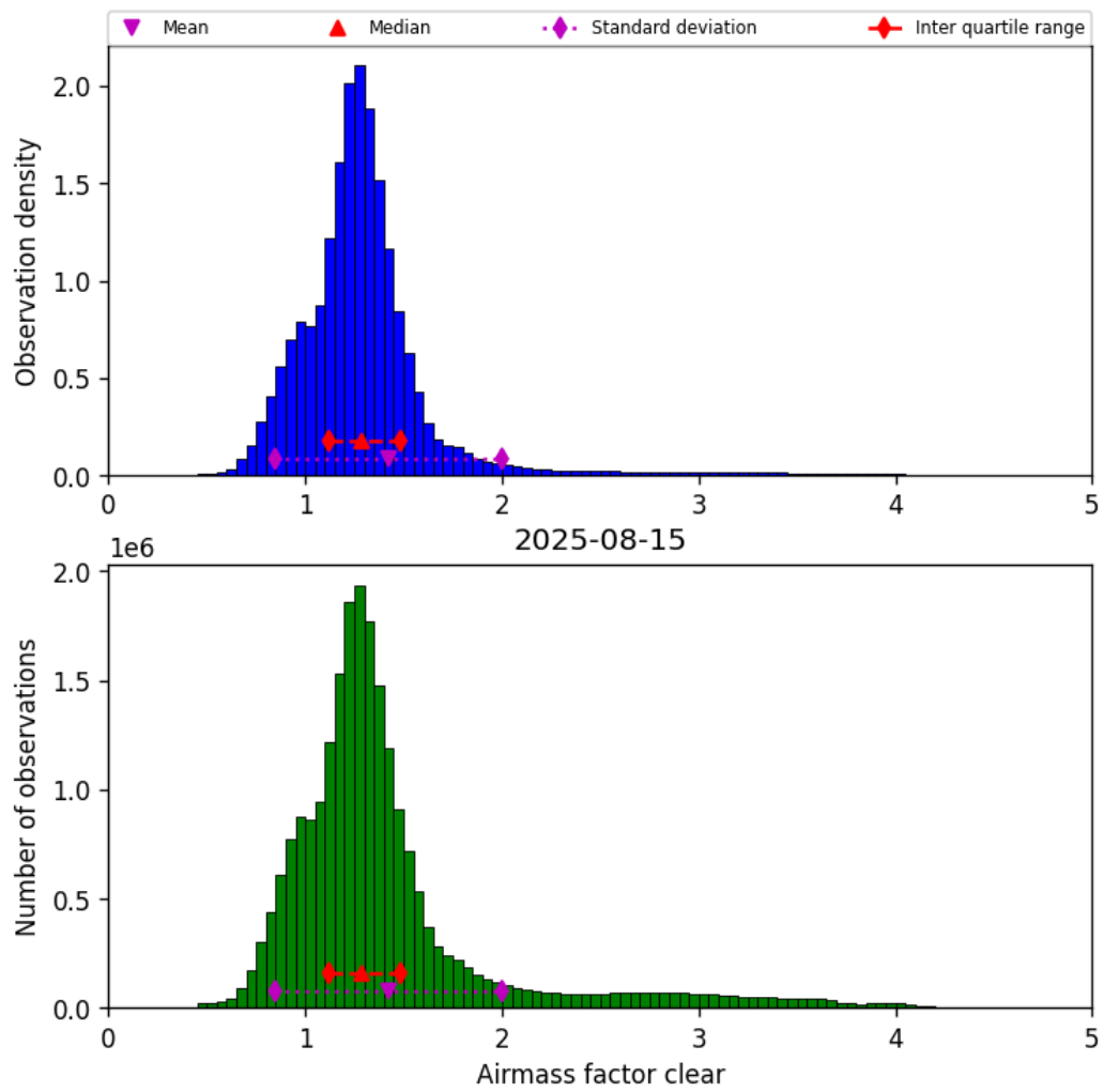
Figure 40: Histogram of “Airmass factor clear” for 2025-08-15 to 2025-08-16
