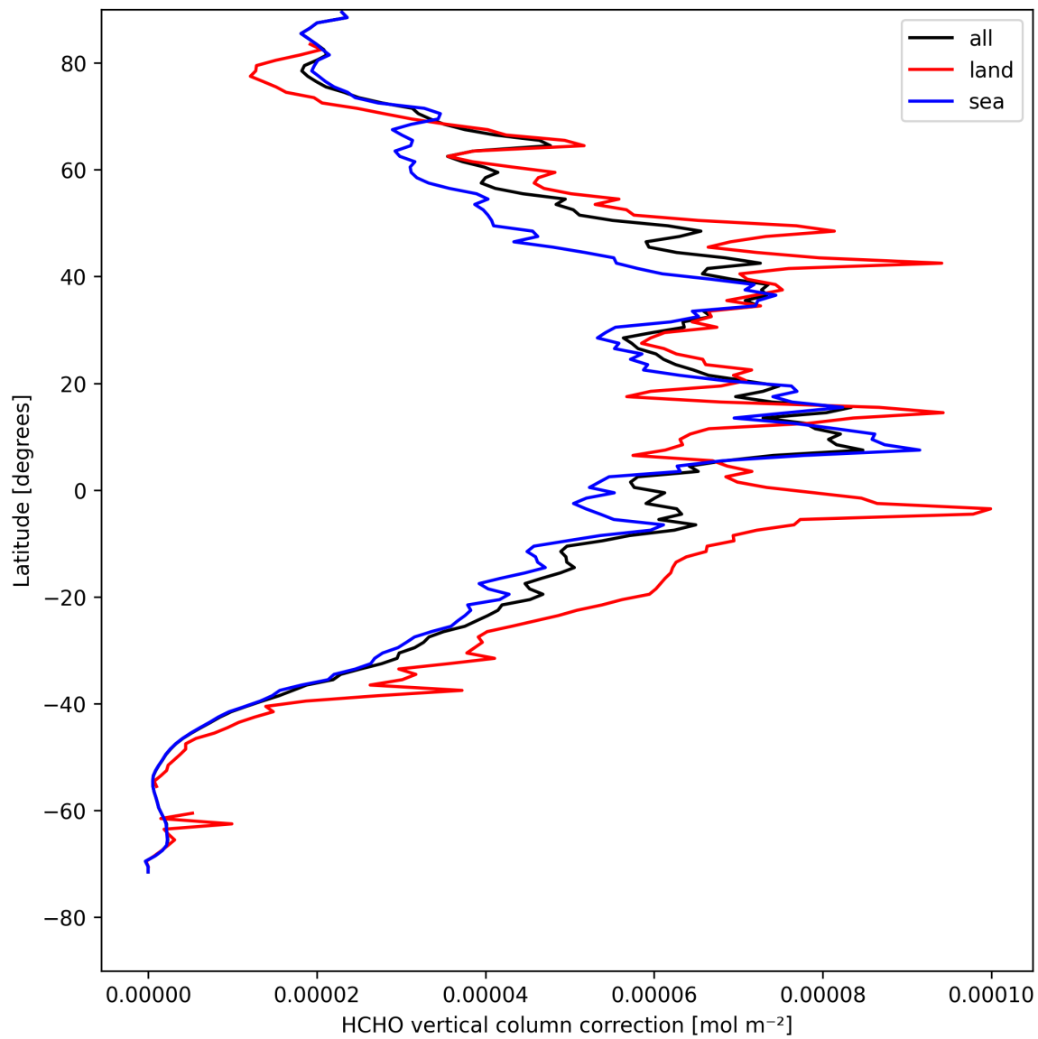
Figure 21: Zonal average of “HCHO vertical column correction” for 2025-08-15 to 2025-08-16.
