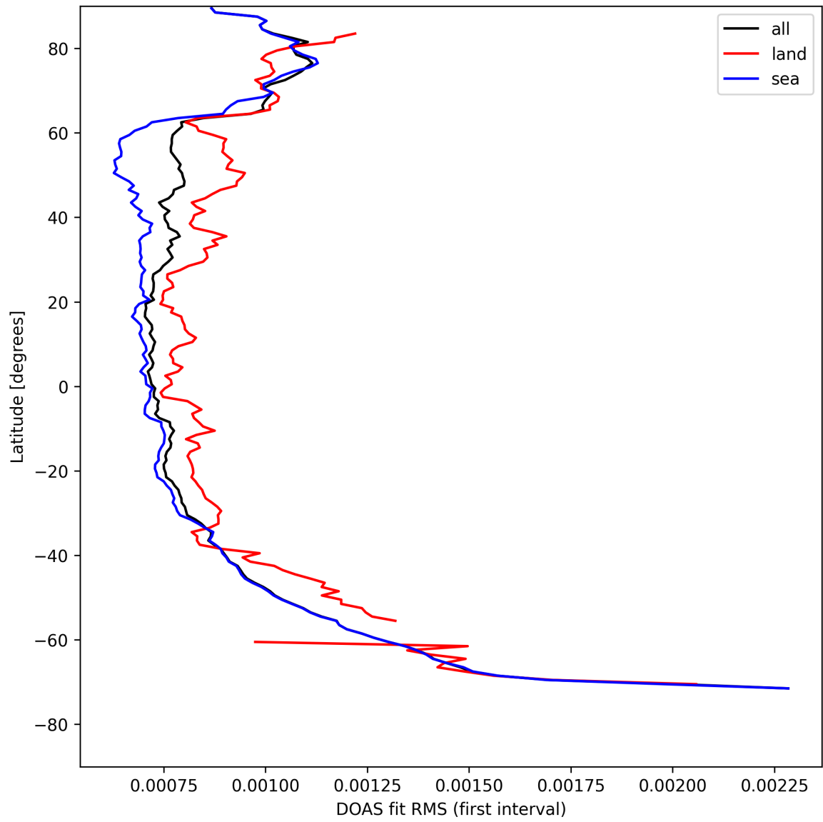
Figure 30: Zonal average of “DOAS fit RMS (first interval)” for 2025-08-15 to 2025-08-16.
