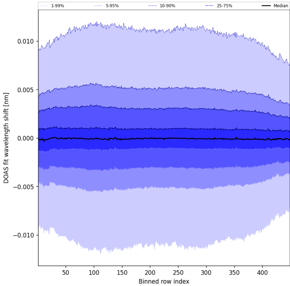
Figure 56: Along track statistics of “DOAS fit wavelength shift” for 2025-08-15 to 2025-08-16
