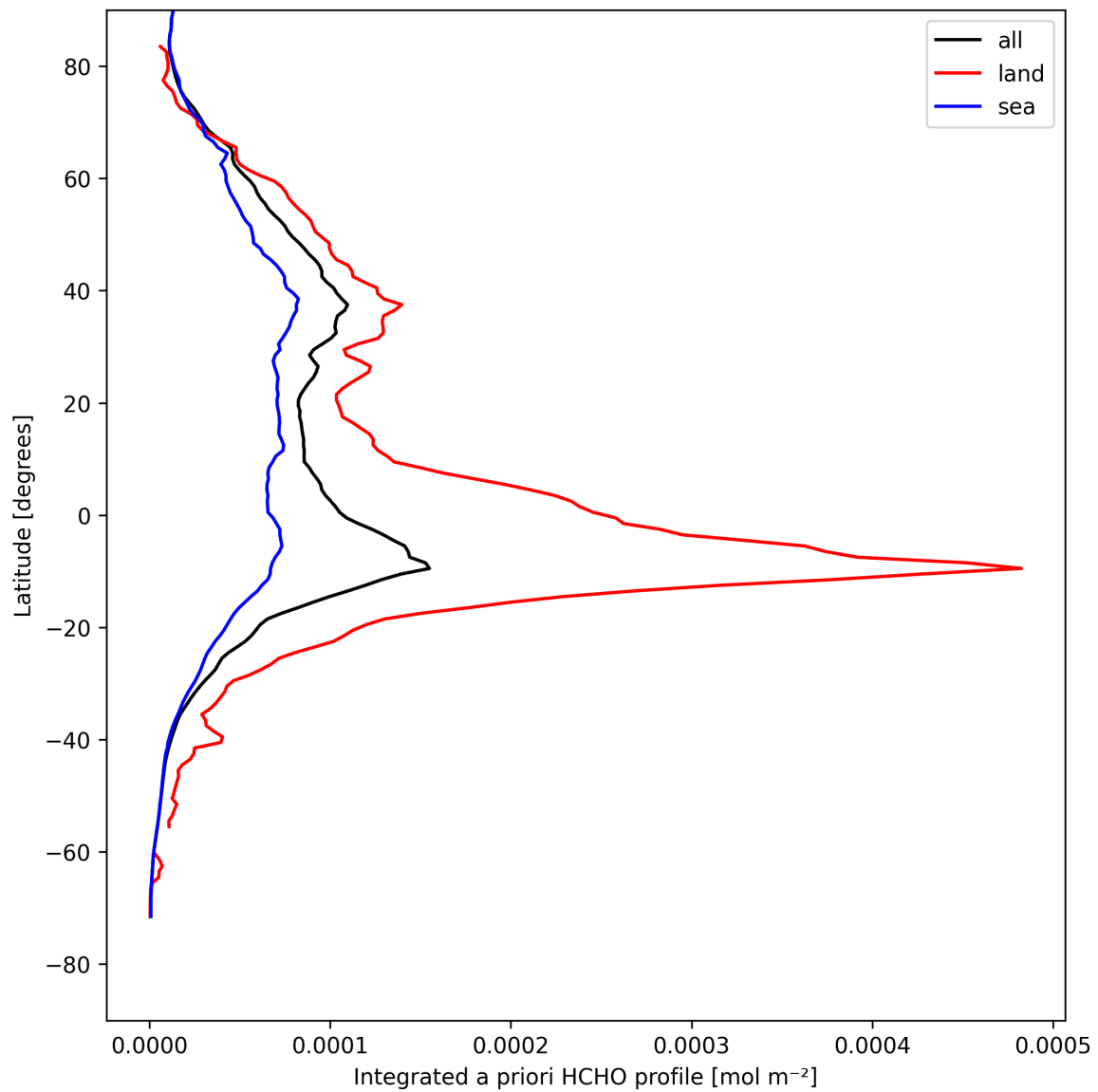
Figure 27: Zonal average of “Integrated a priori HCHO profile” for 2025-08-16 to 2025-08-17.
