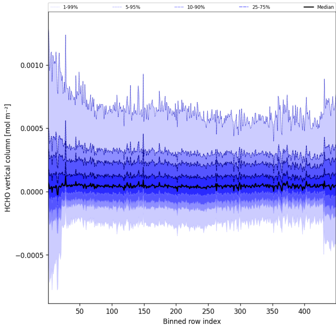
Figure 47: Along track statistics of “HCHO vertical column” for 2025-08-16 to 2025-08-17
