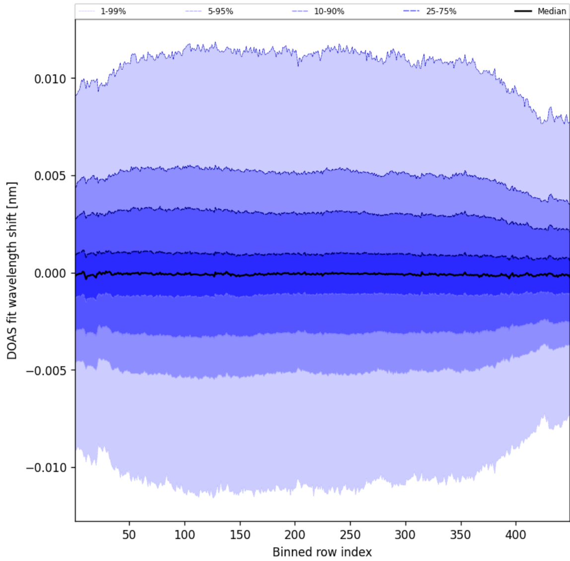
Figure 56: Along track statistics of “DOAS fit wavelength shift” for 2025-08-16 to 2025-08-17
