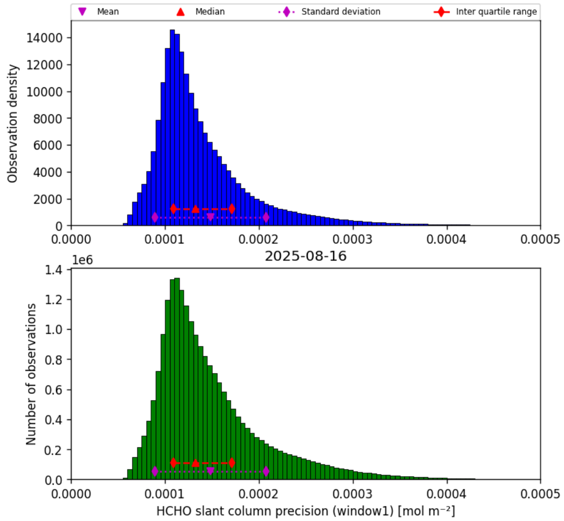
Figure 37: Histogram of “HCHO slant column precision (window1)” for 2025-08-16 to 2025-08-17
