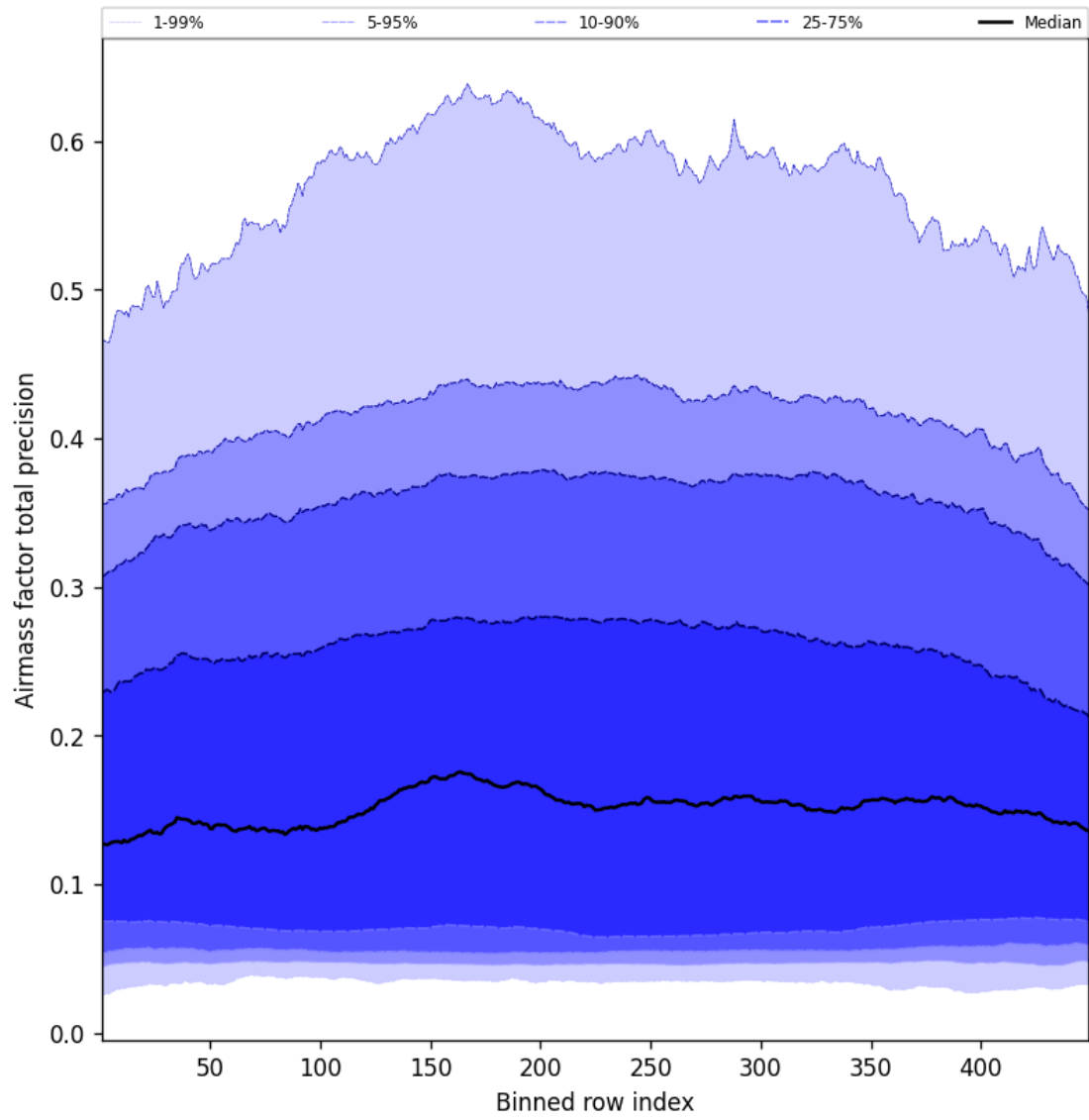
Figure 53: Along track statistics of “Airmass factor total precision” for 2025-08-16 to 2025-08-17
