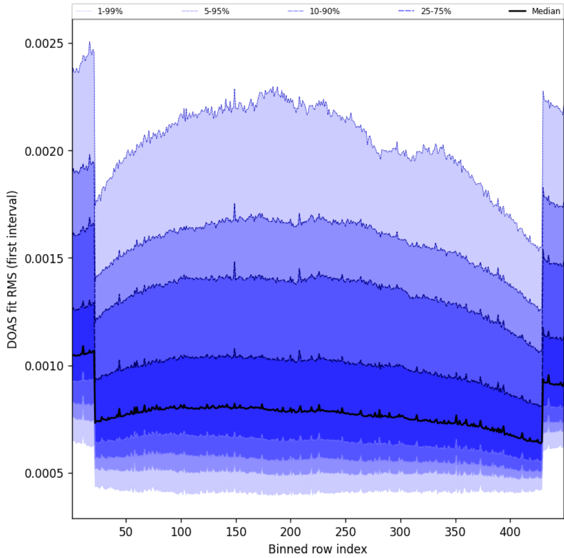
Figure 58: Along track statistics of “DOAS fit RMS (first interval)” for 2025-08-16 to 2025-08-17
