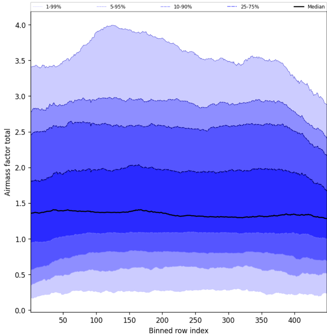
Figure 52: Along track statistics of “Airmass factor total” for 2025-08-16 to 2025-08-17
