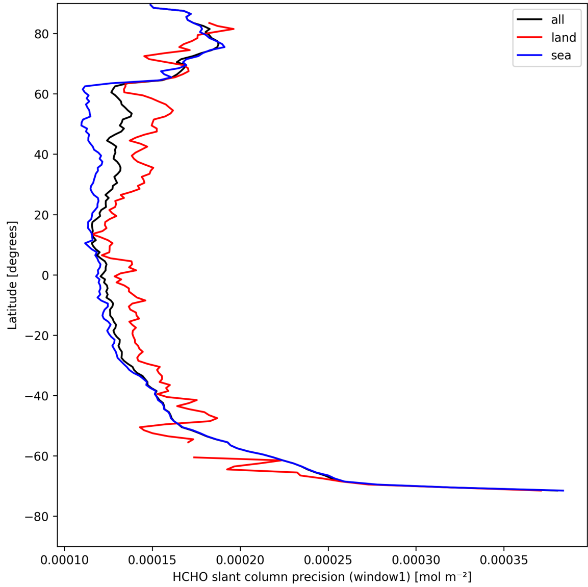
Figure 23: Zonal average of “HCHO slant column precision (window1)” for 2025-08-16 to 2025-08-17.
