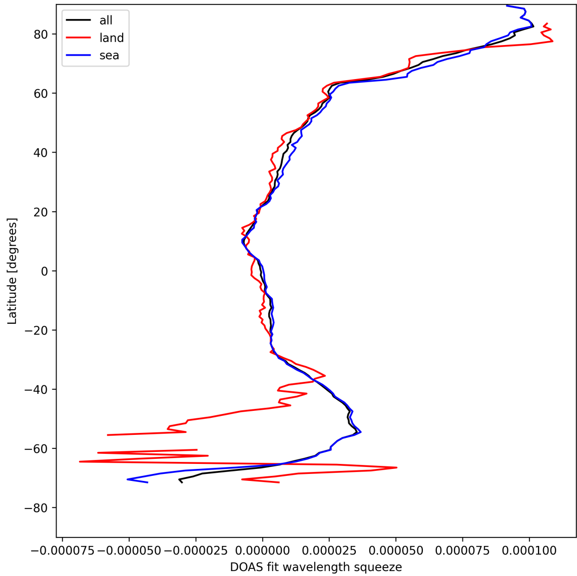
Figure 29: Zonal average of “DOAS fit wavelength squeeze” for 2025-08-16 to 2025-08-17.
