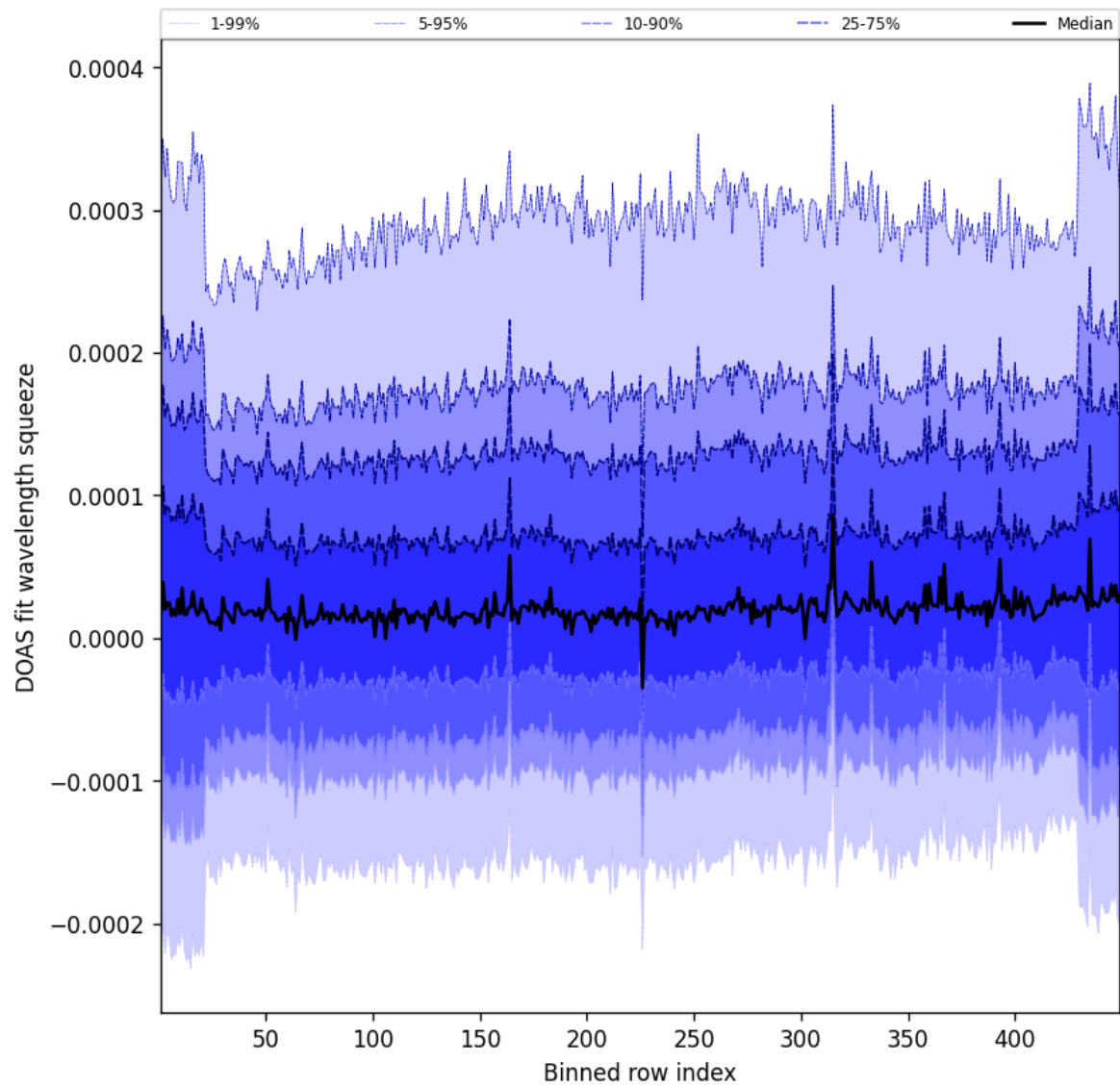
Figure 57: Along track statistics of “DOAS fit wavelength squeeze” for 2025-08-16 to 2025-08-17
