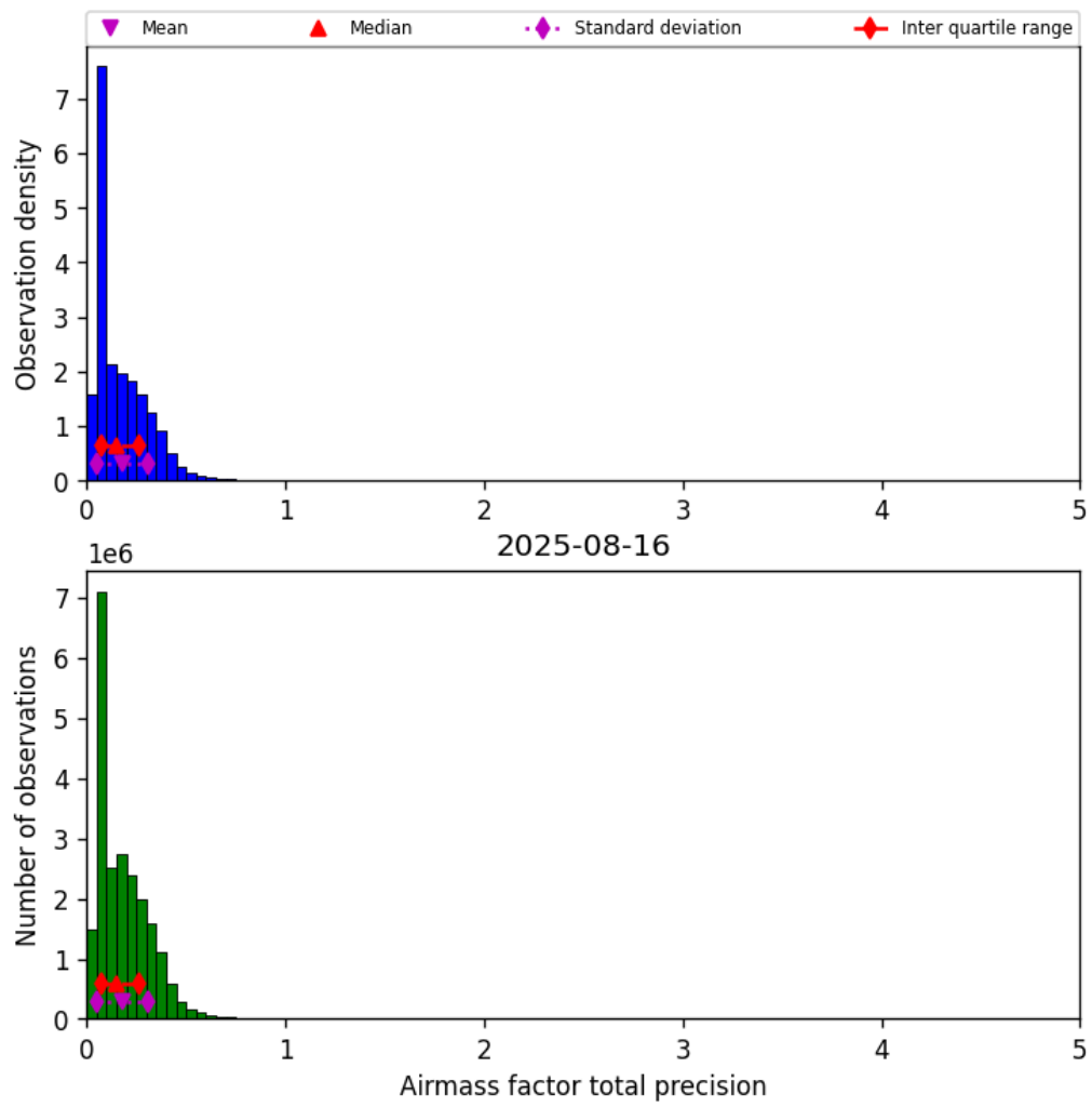
Figure 39: Histogram of “Airmass factor total precision” for 2025-08-16 to 2025-08-17
