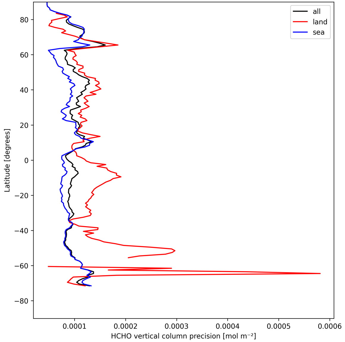
Figure 20: Zonal average of “HCHO vertical column precision” for 2025-08-16 to 2025-08-17.
