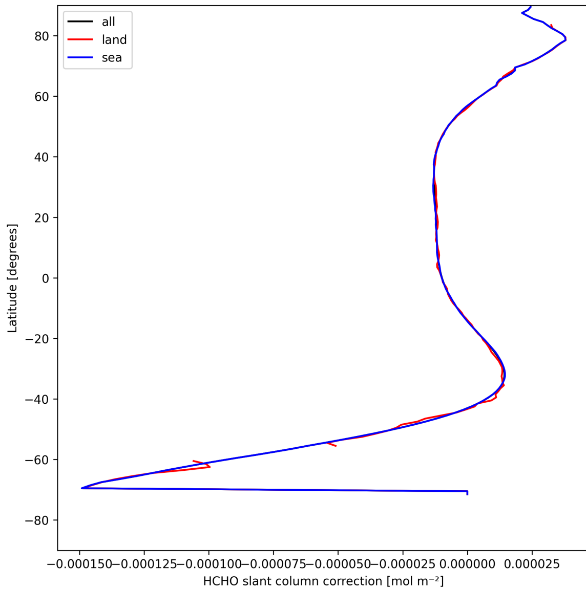
Figure 31: Zonal average of “HCHO slant column correction” for 2025-08-16 to 2025-08-17.
