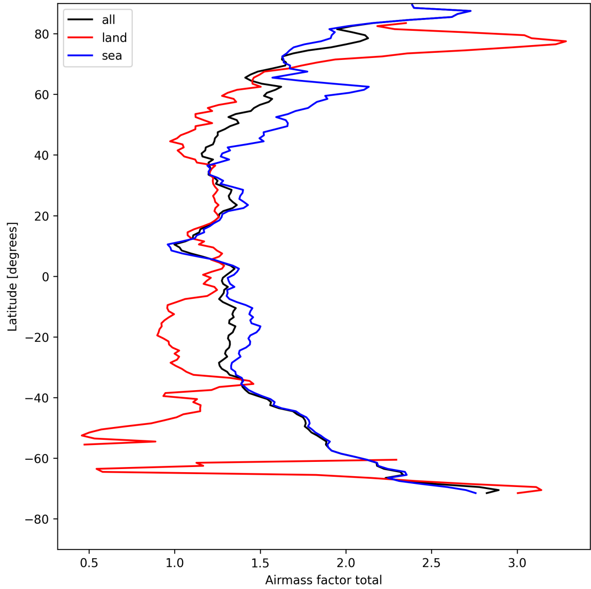
Figure 24: Zonal average of “Airmass factor total” for 2025-08-16 to 2025-08-17.
