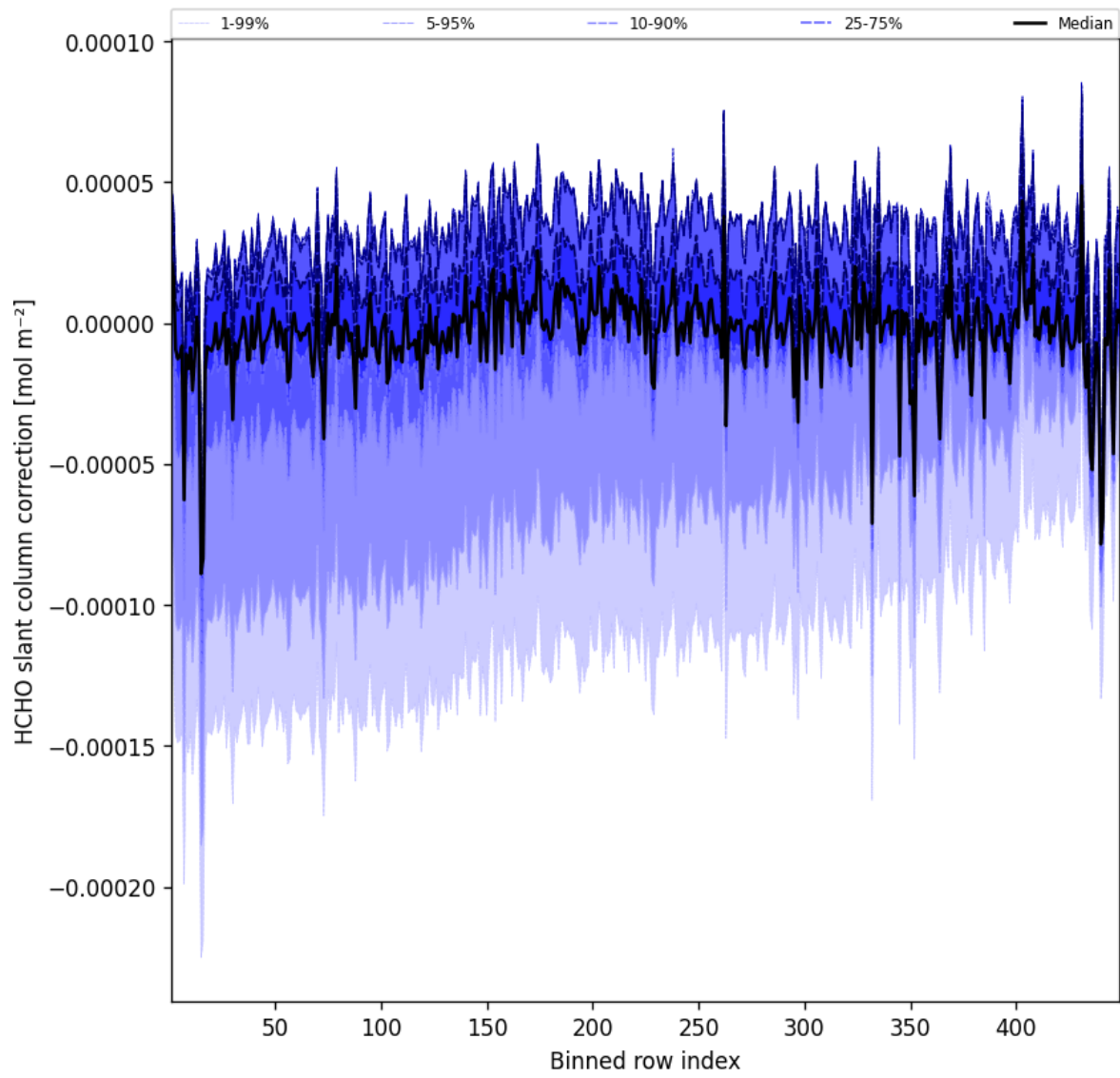
Figure 59: Along track statistics of “HCHO slant column correction” for 2025-08-16 to 2025-08-17
