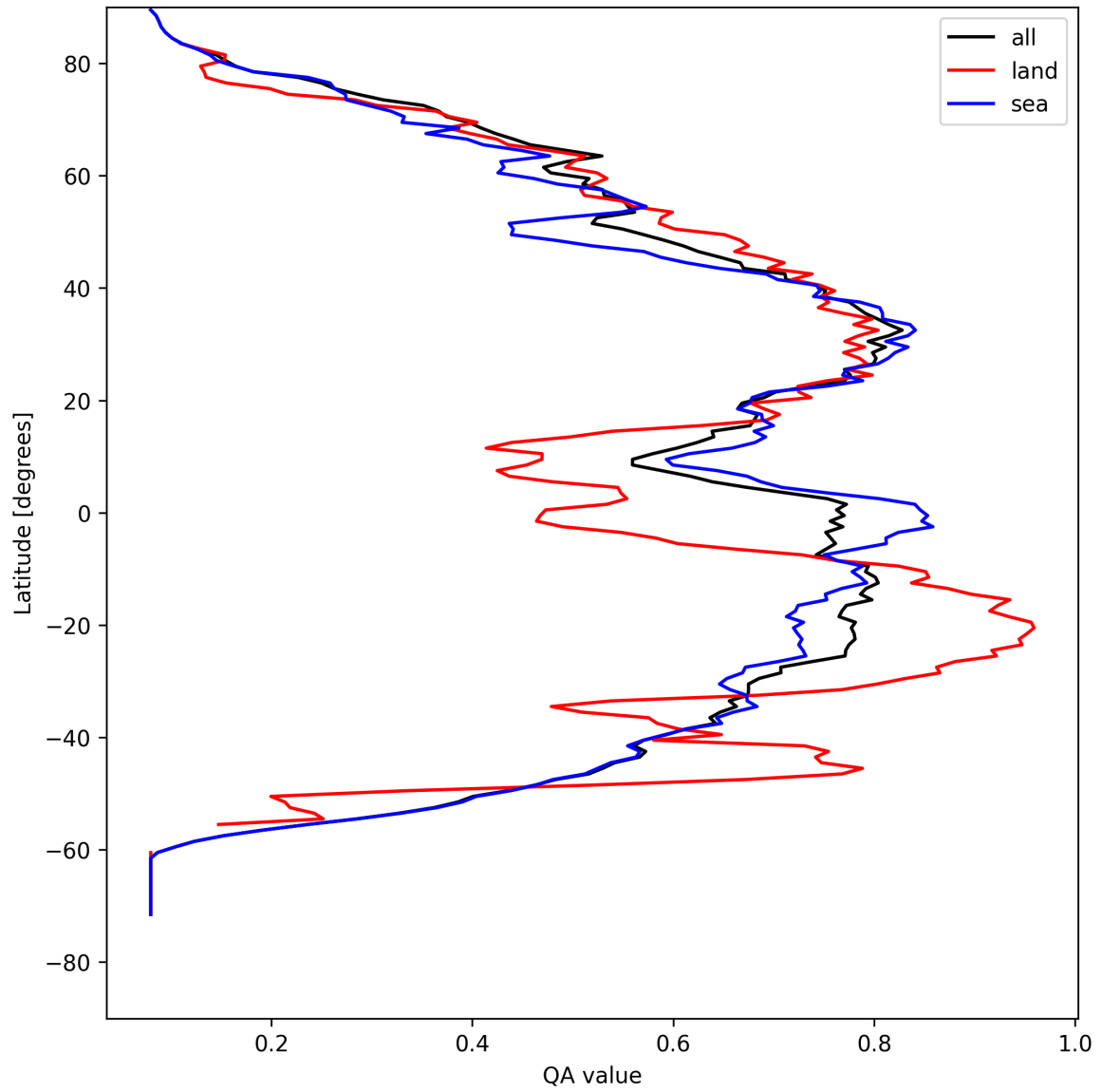
Figure 18: Zonal average of “QA value” for 2025-08-16 to 2025-08-17.
