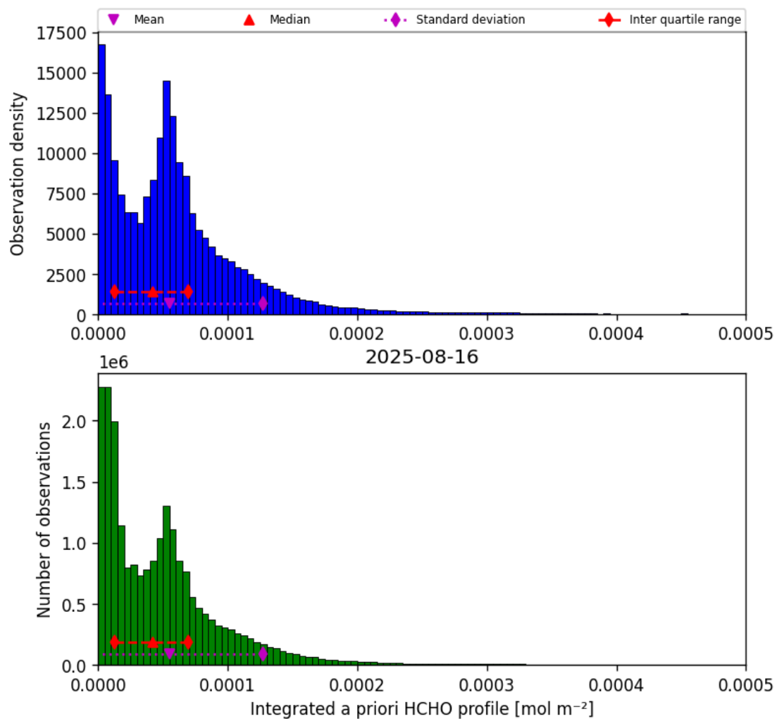
Figure 41: Histogram of “Integrated a priori HCHO profile” for 2025-08-16 to 2025-08-17
