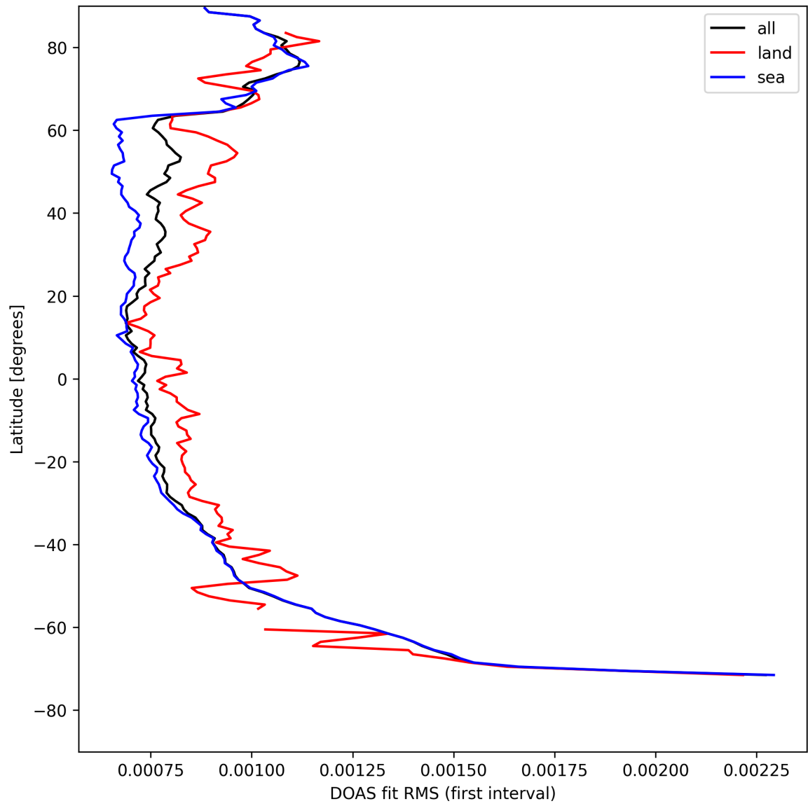
Figure 30: Zonal average of "DOAS fit RMS (first interval)" for 2025-08-16 to 2025-08-17.
