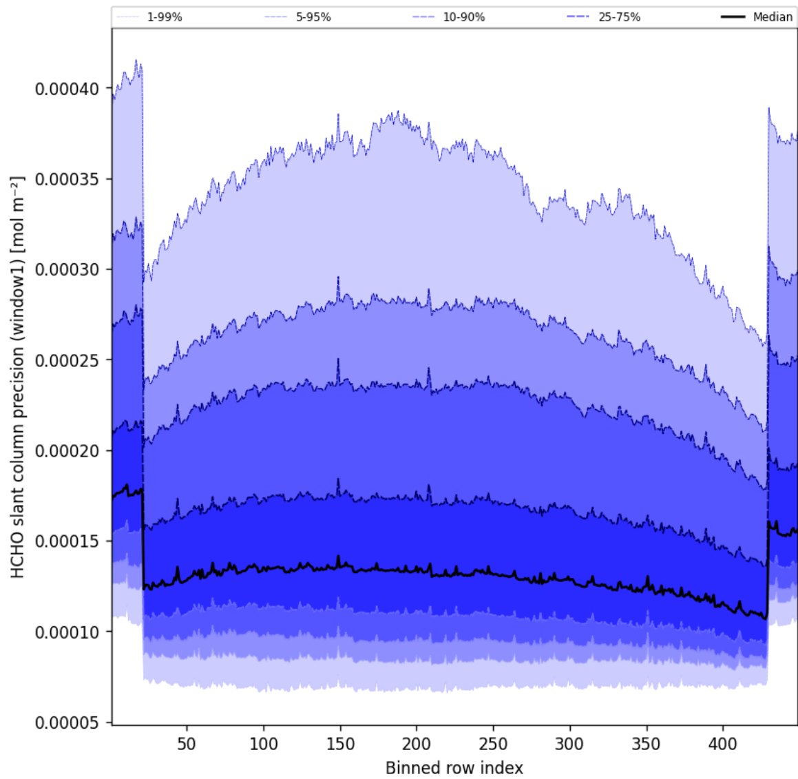
Figure 51: Along track statistics of “HCHO slant column precision (window1)” for 2025-08-16 to 2025-08-17
