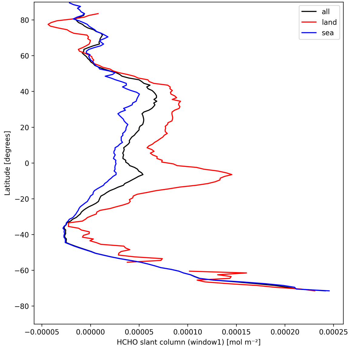
Figure 22: Zonal average of “HCHO slant column (window1)” for 2025-08-16 to 2025-08-17.
