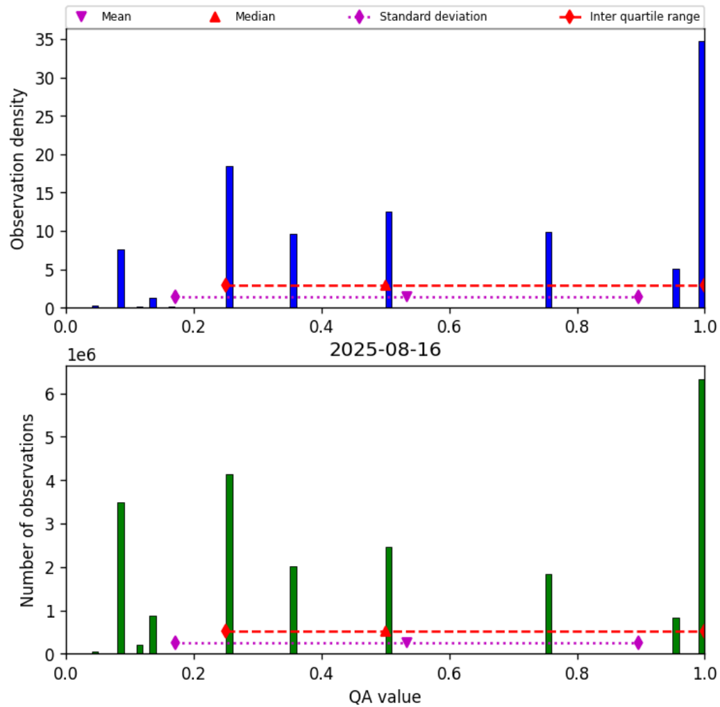
Figure 32: Histogram of “QA value” for 2025-08-16 to 2025-08-17
