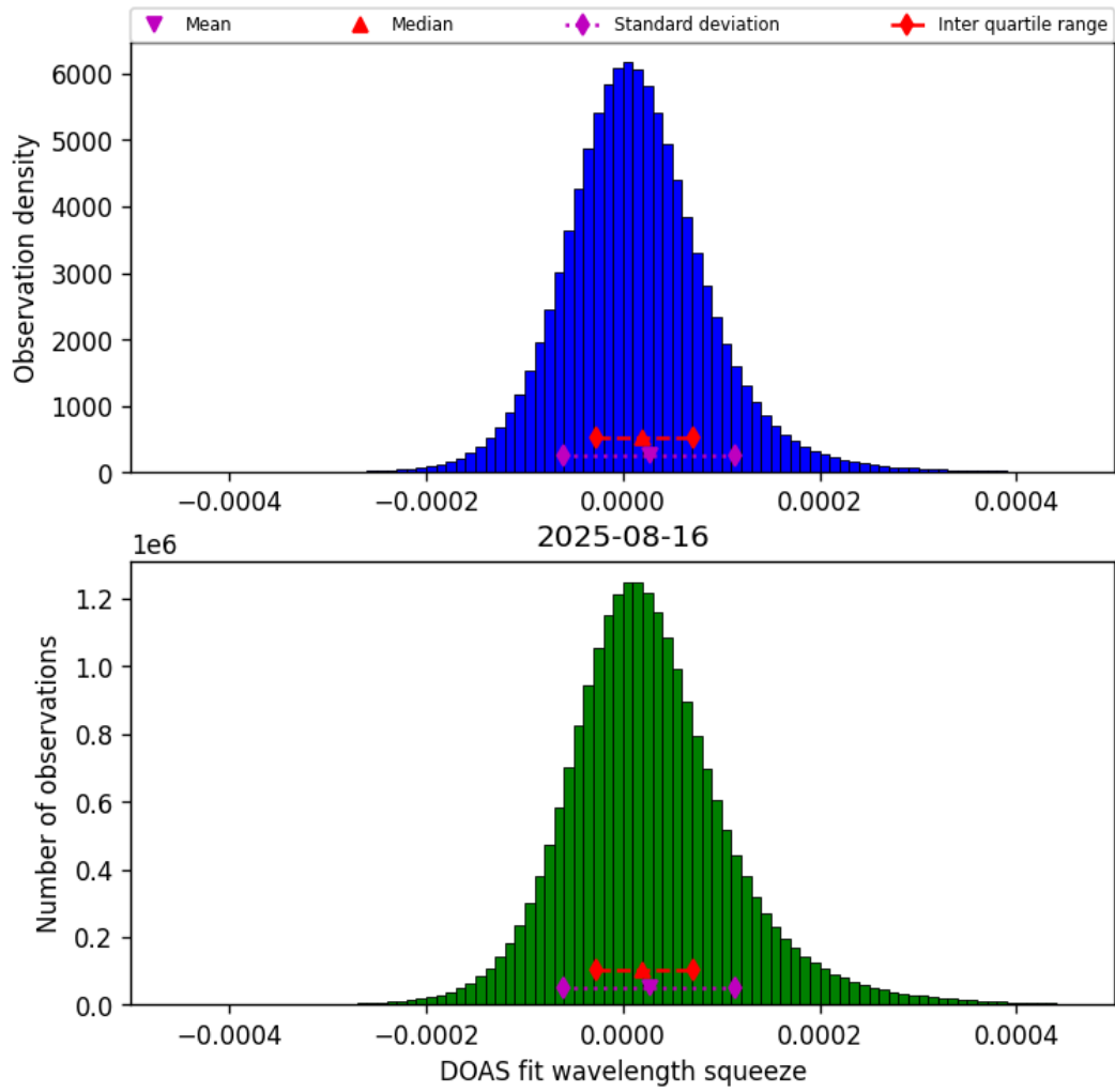
Figure 43: Histogram of “DOAS fit wavelength squeeze” for 2025-08-16 to 2025-08-17
