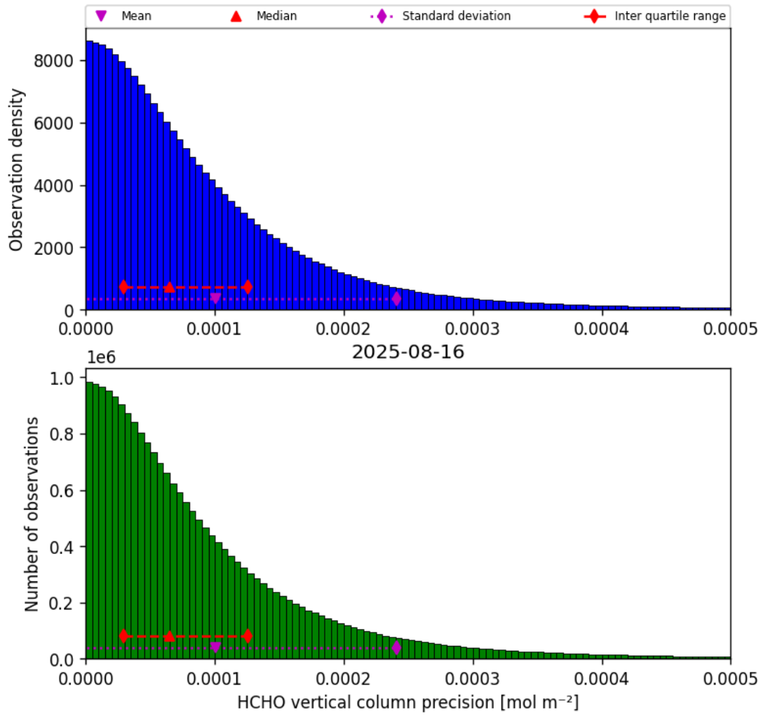
Figure 34: Histogram of “HCHO vertical column precision” for 2025-08-16 to 2025-08-17
