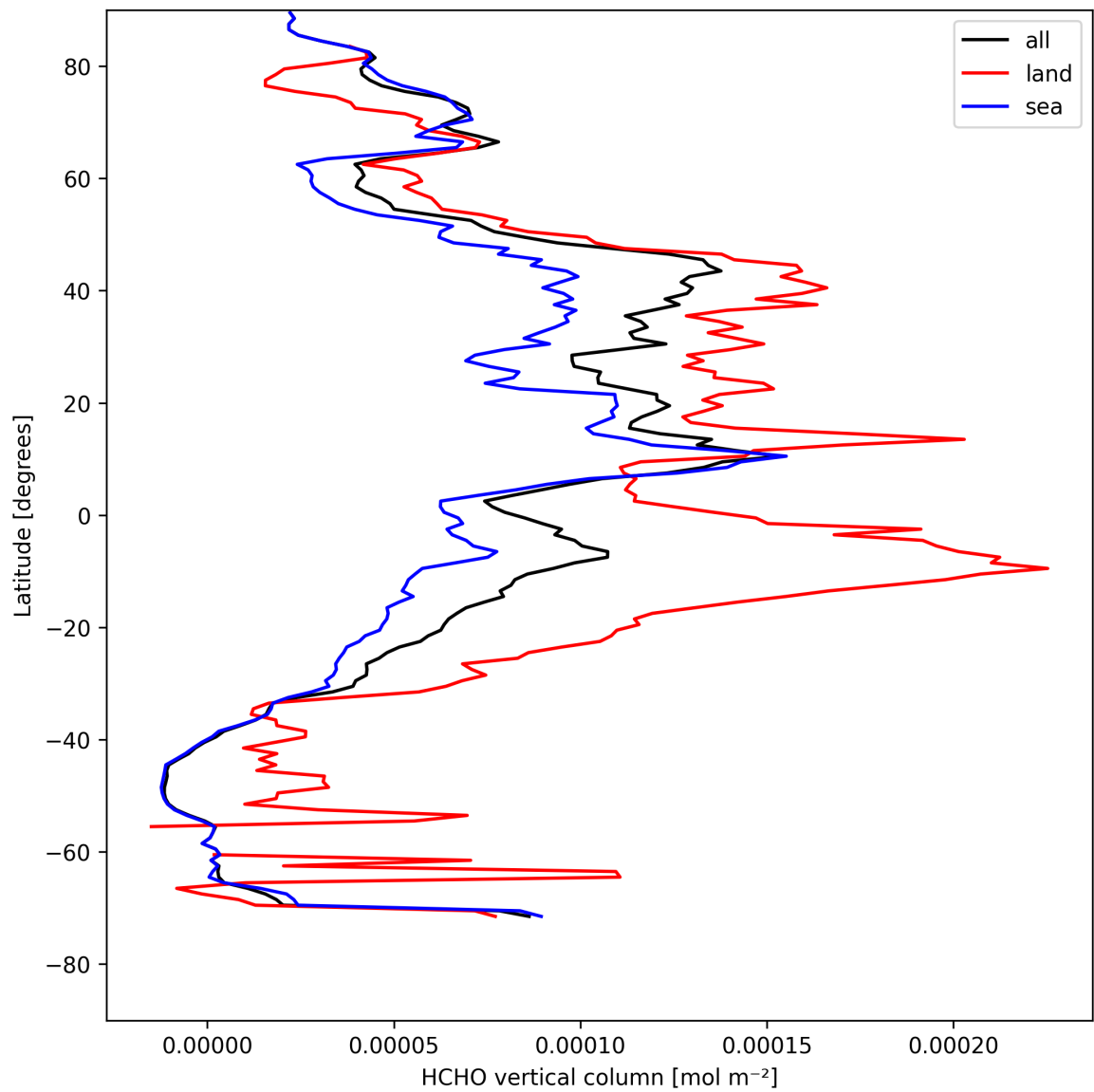
Figure 19: Zonal average of “HCHO vertical column” for 2025-08-16 to 2025-08-17.
