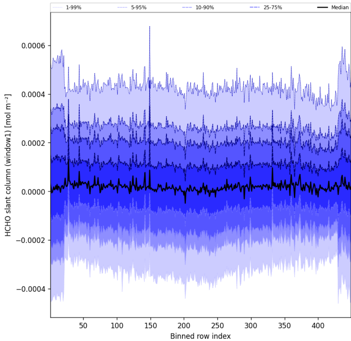
Figure 50: Along track statistics of “HCHO slant column (window1)” for 2025-08-16 to 2025-08-17
