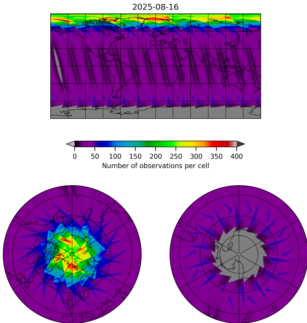
Figure 17: Map of the number of observations for 2025-08-16 to 2025-08-17
