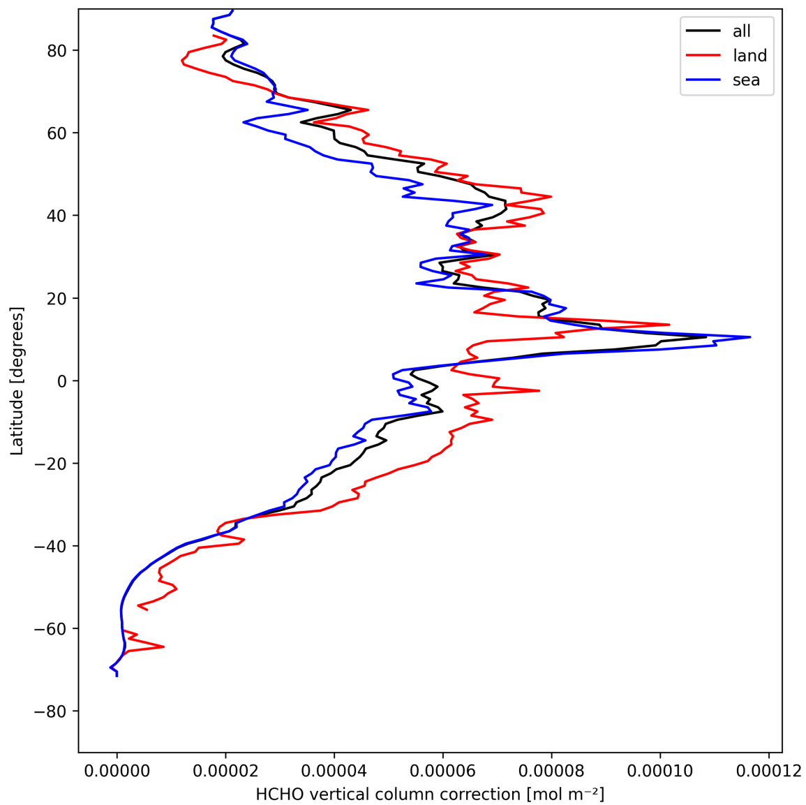
Figure 21: Zonal average of “HCHO vertical column correction” for 2025-08-16 to 2025-08-17.
