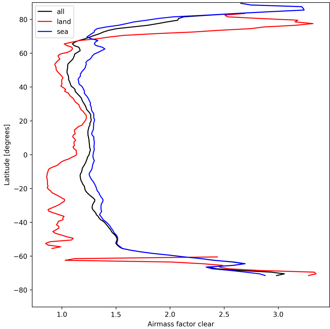
Figure 26: Zonal average of “Airmass factor clear” for 2025-08-16 to 2025-08-17.
