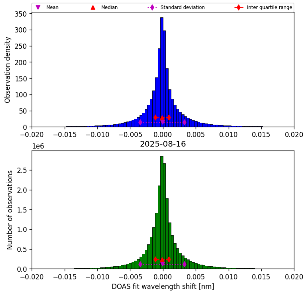
Figure 42: Histogram of “DOAS fit wavelength shift” for 2025-08-16 to 2025-08-17
