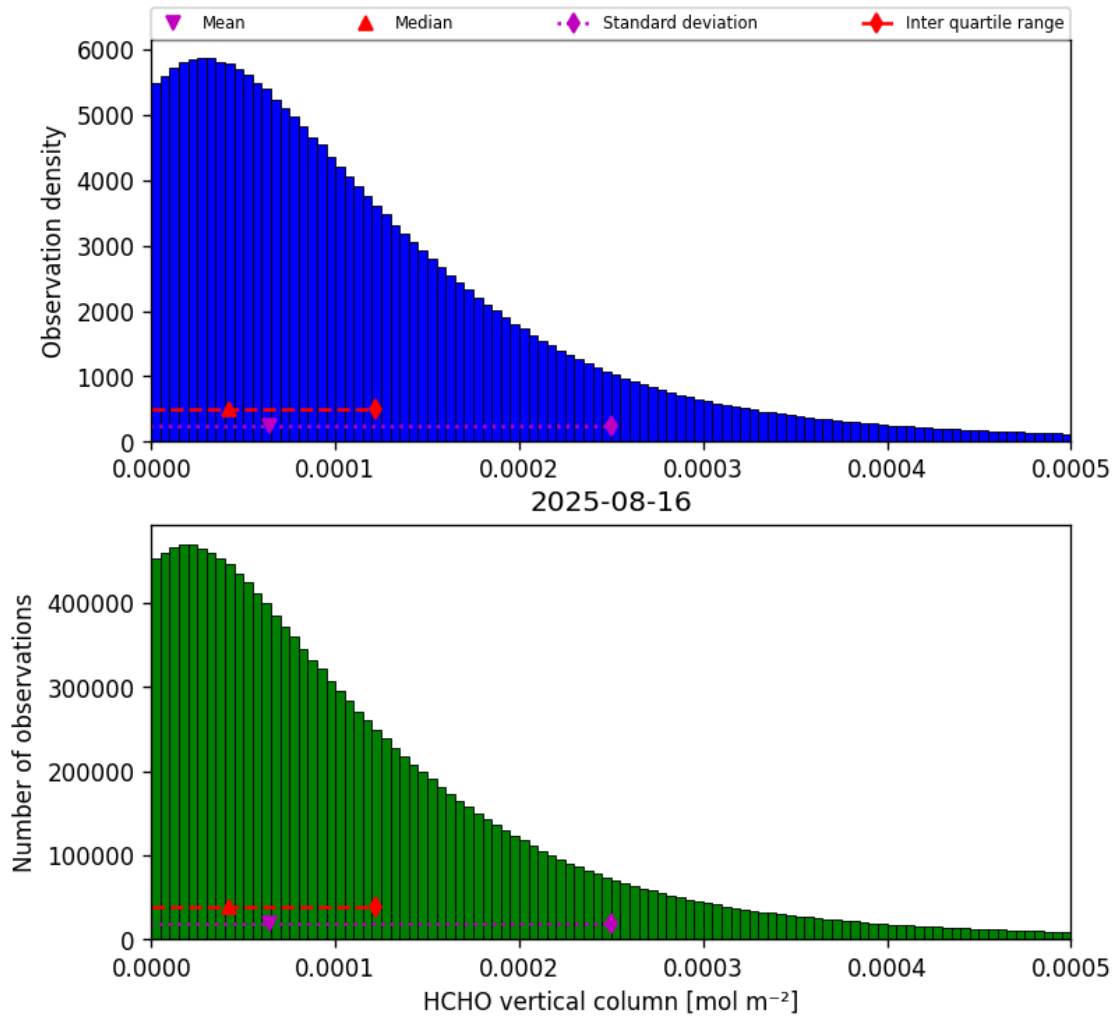
Figure 33: Histogram of “HCHO vertical column” for 2025-08-16 to 2025-08-17
