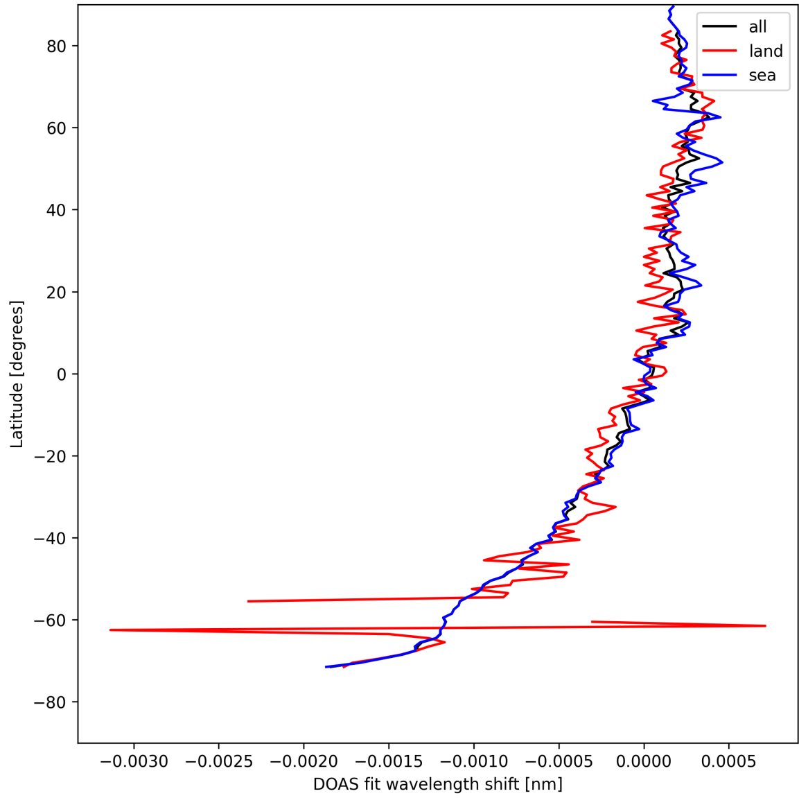
Figure 28: Zonal average of “DOAS fit wavelength shift” for 2025-08-16 to 2025-08-17.
