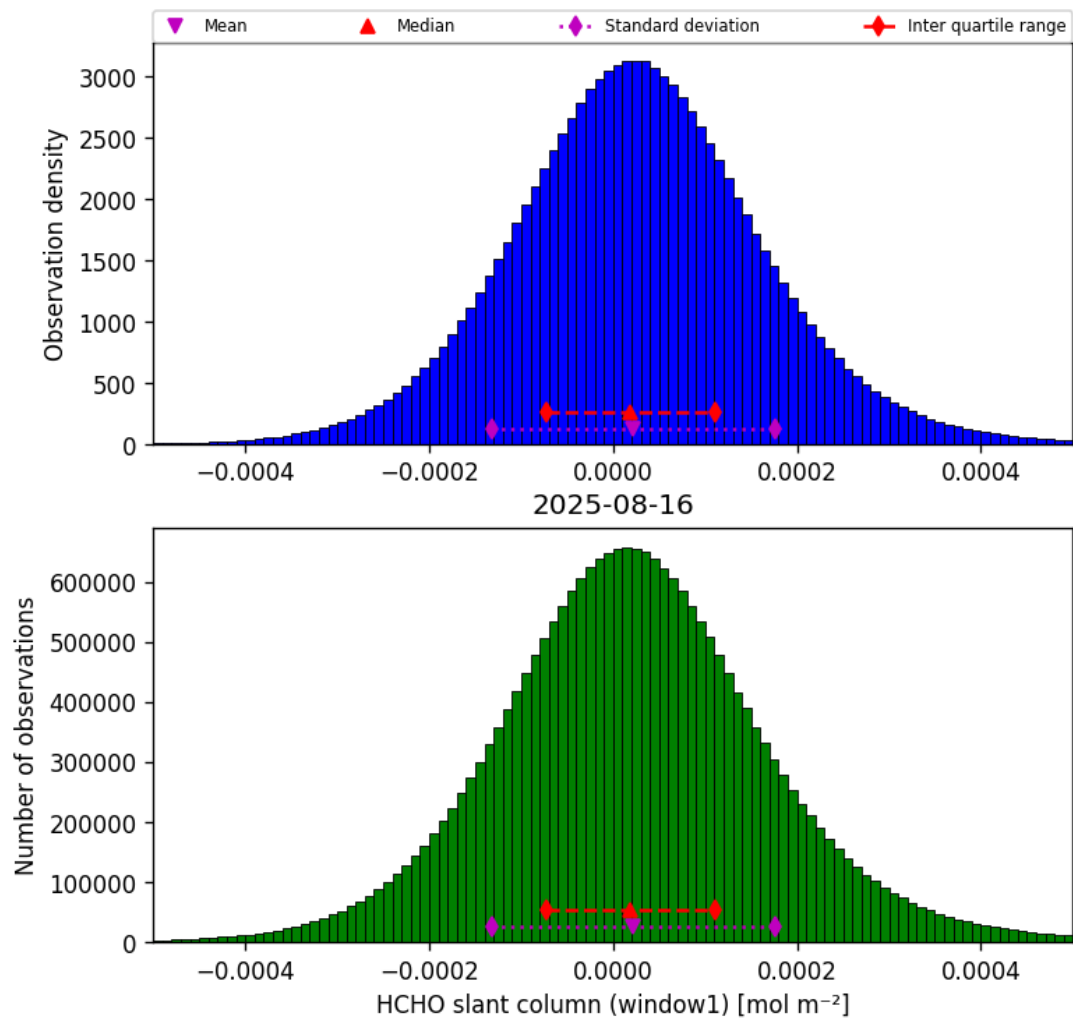
Figure 36: Histogram of “HCHO slant column (window1)” for 2025-08-16 to 2025-08-17
