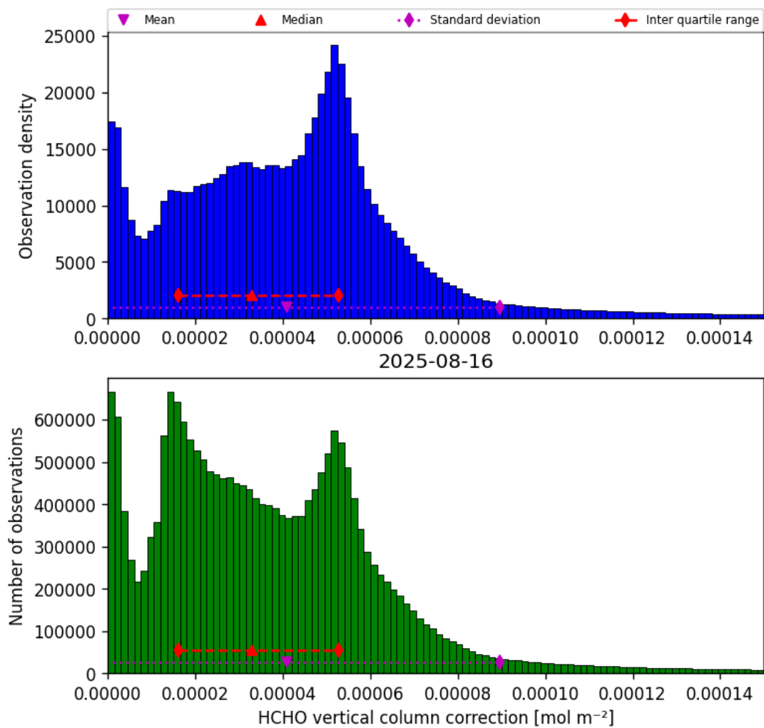
Figure 35: Histogram of “HCHO vertical column correction” for 2025-08-16 to 2025-08-17
