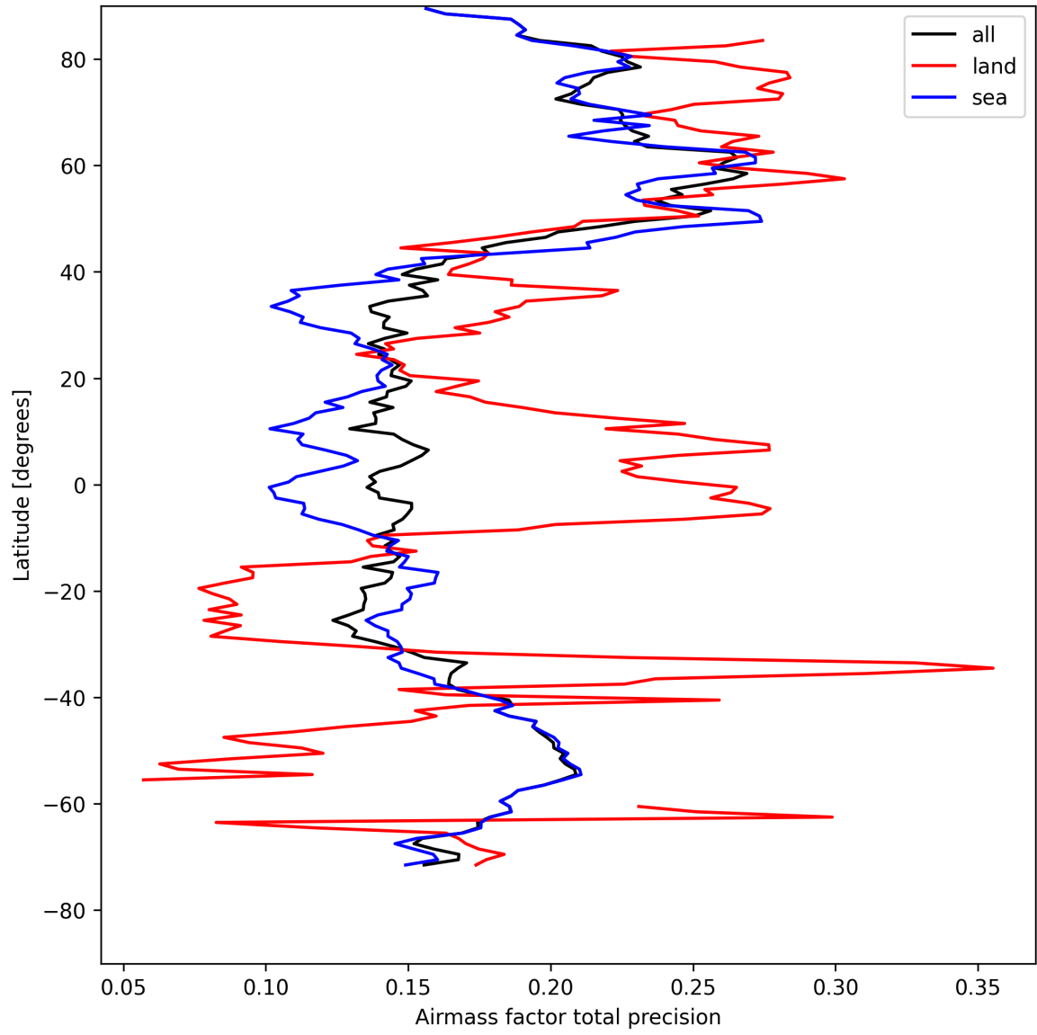
Figure 25: Zonal average of “Airmass factor total precision” for 2025-08-16 to 2025-08-17.
