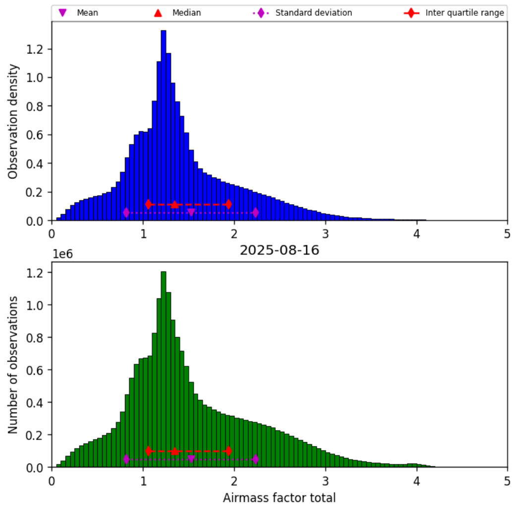
Figure 38: Histogram of “Airmass factor total” for 2025-08-16 to 2025-08-17
