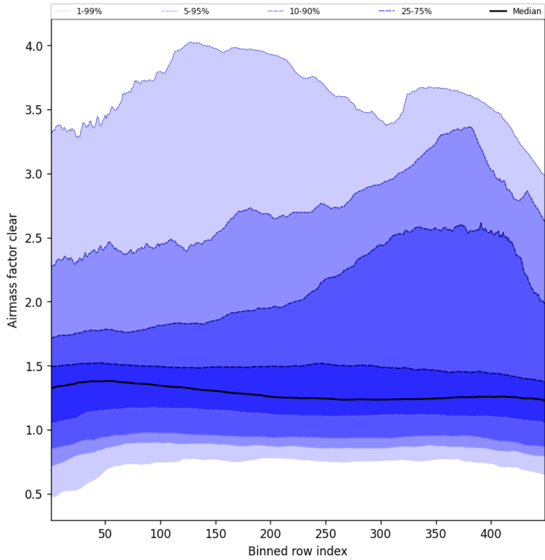
Figure 54: Along track statistics of “Airmass factor clear” for 2025-08-16 to 2025-08-17
