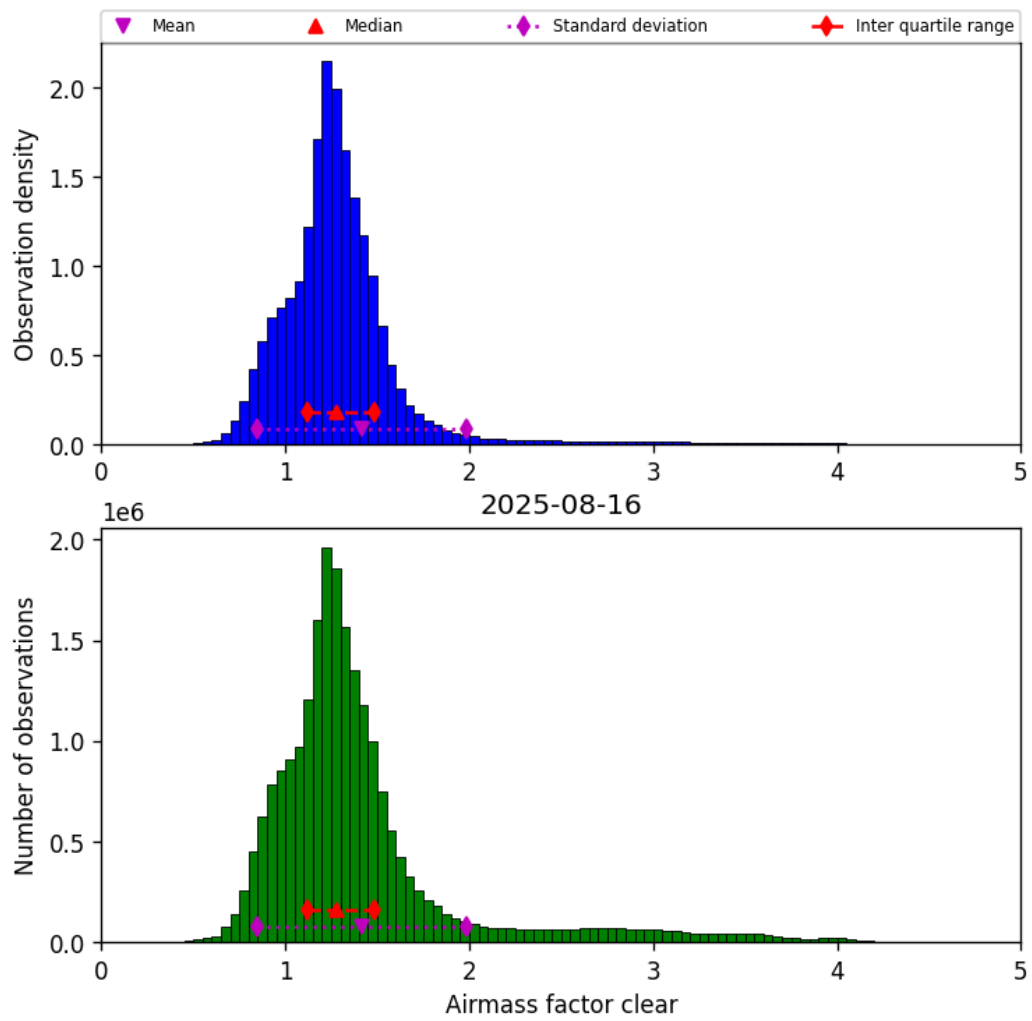
Figure 40: Histogram of “Airmass factor clear” for 2025-08-16 to 2025-08-17
