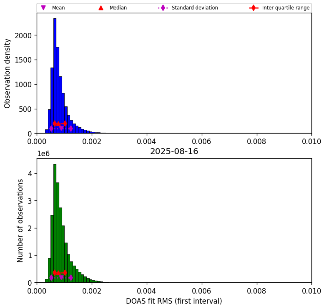
Figure 44: Histogram of “DOAS fit RMS (first interval)” for 2025-08-16 to 2025-08-17
