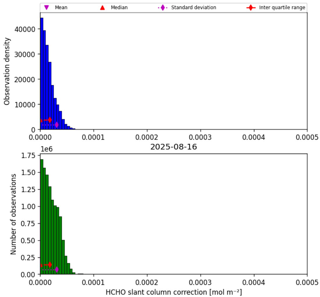
Figure 45: Histogram of “HCHO slant column correction” for 2025-08-16 to 2025-08-17
