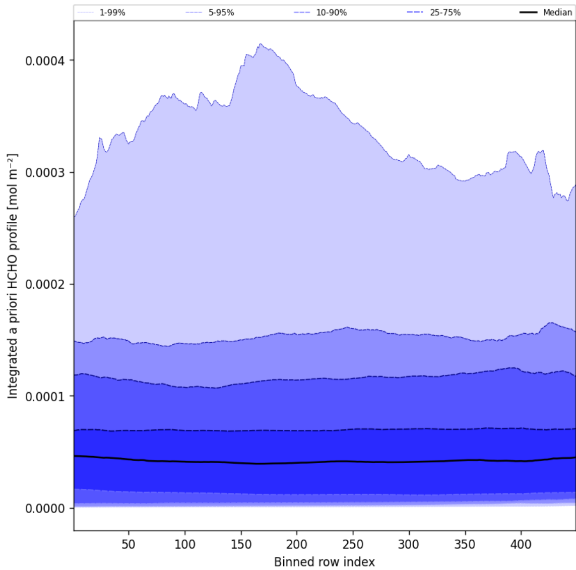
Figure 55: Along track statistics of "Integrated a priori HCHO profile" for 2025-08-16 to 2025-08-17
