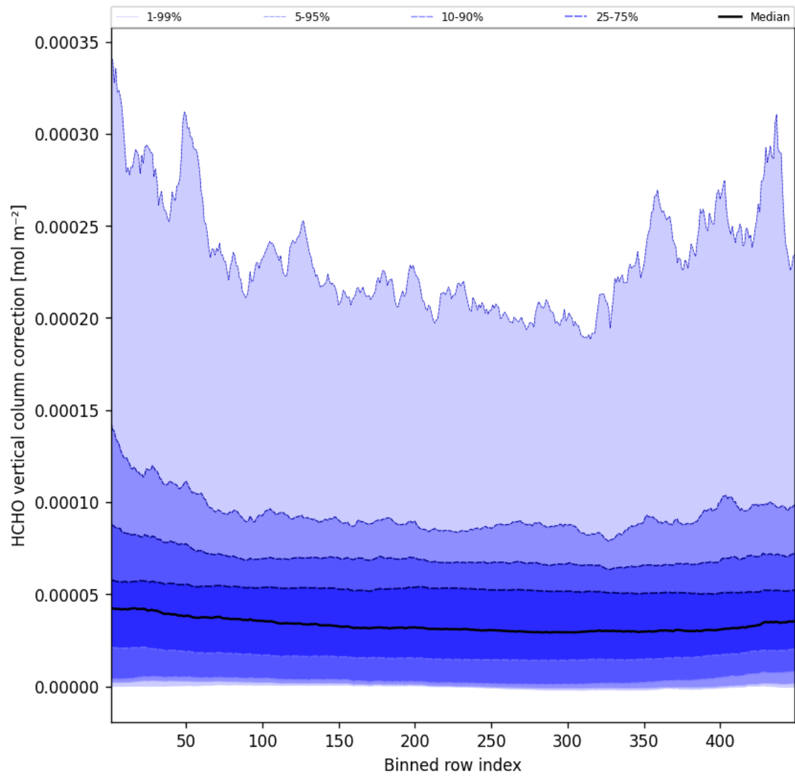
Figure 49: Along track statistics of “HCHO vertical column correction” for 2025-08-16 to 2025-08-17
