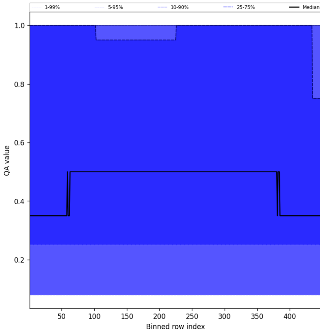
Figure 46: Along track statistics of “QA value” for 2025-08-16 to 2025-08-17
