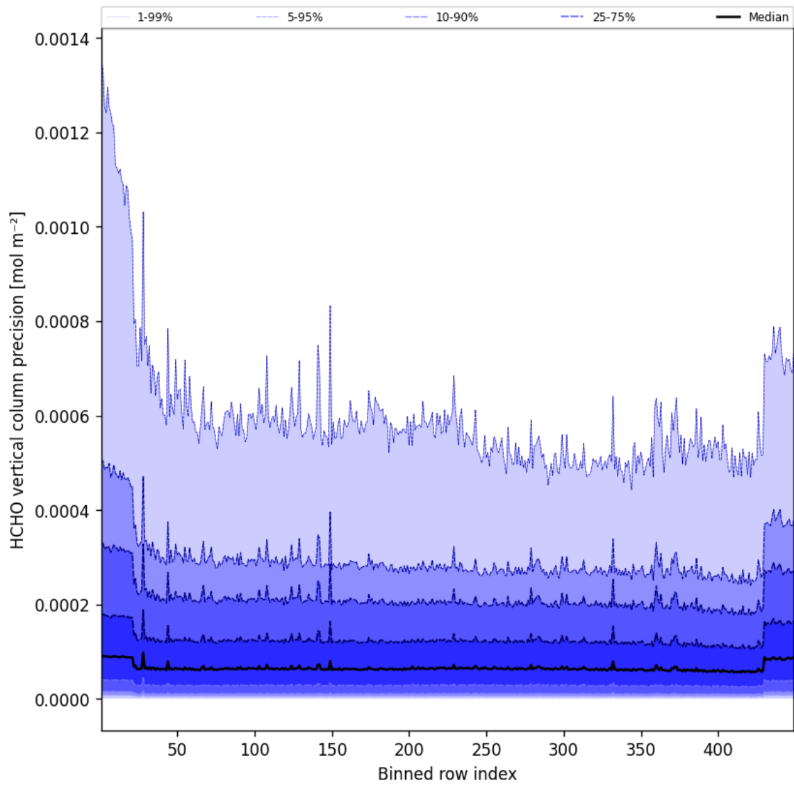
Figure 48: Along track statistics of “HCHO vertical column precision” for 2025-08-16 to 2025-08-17
