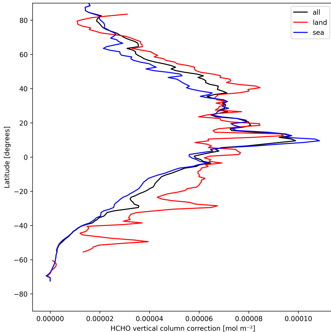
Figure 21: Zonal average of “HCHO vertical column correction” for 2025-08-18 to 2025-08-19.
