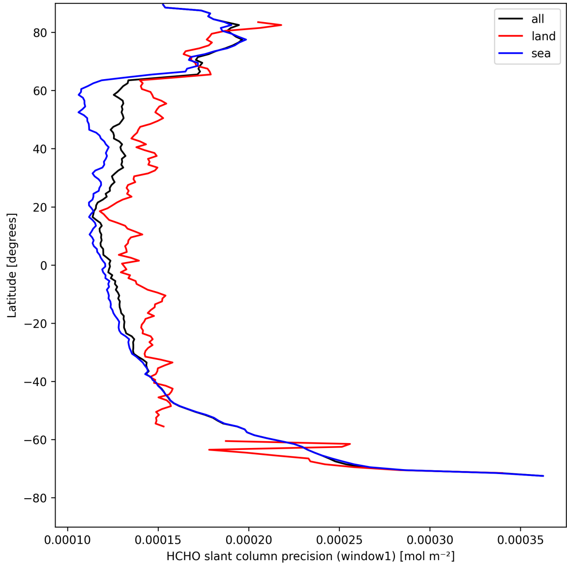
Figure 23: Zonal average of “HCHO slant column precision (window1)” for 2025-08-18 to 2025-08-19.
