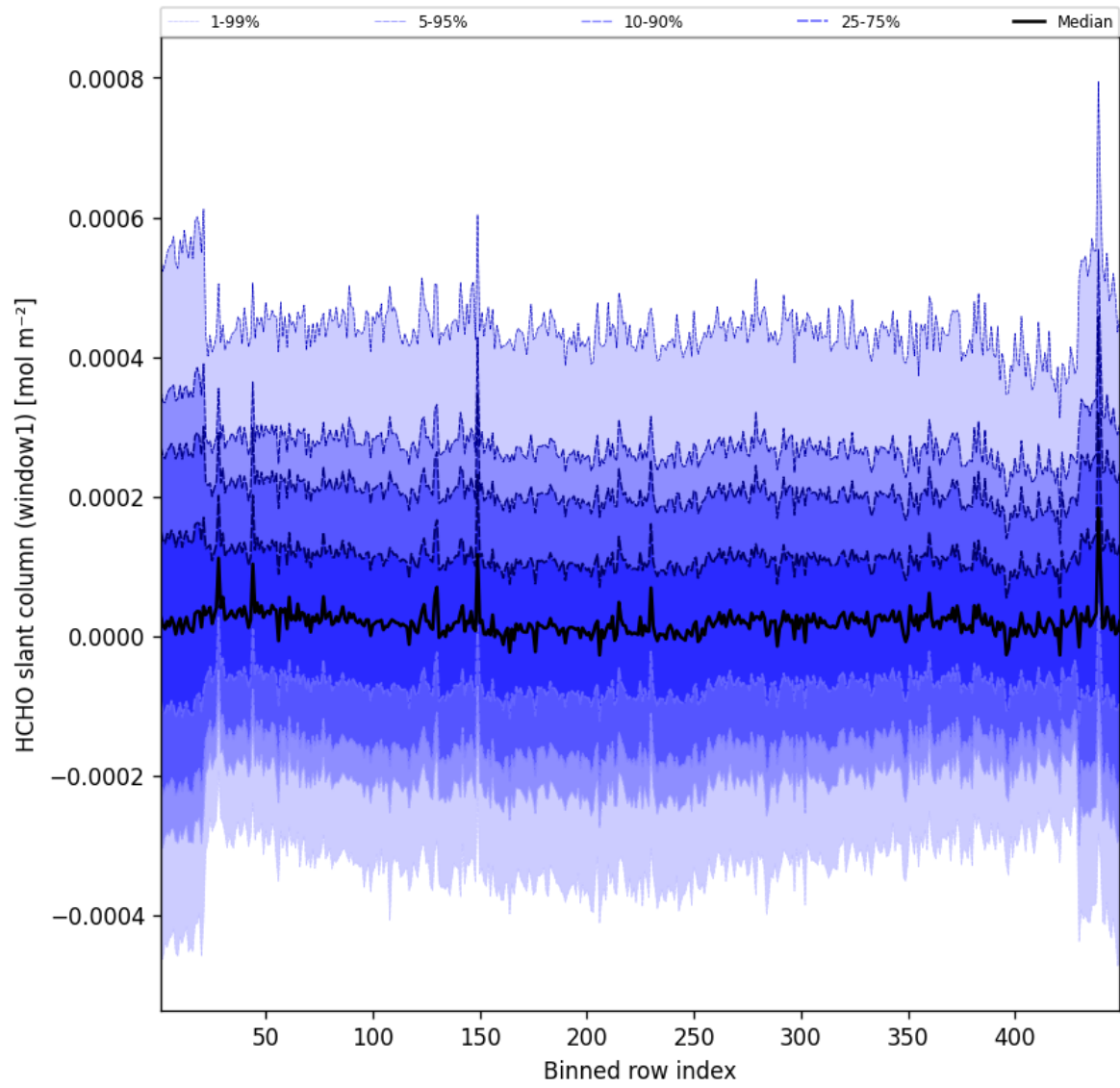
Figure 50: Along track statistics of “HCHO slant column (window1)” for 2025-08-18 to 2025-08-19
