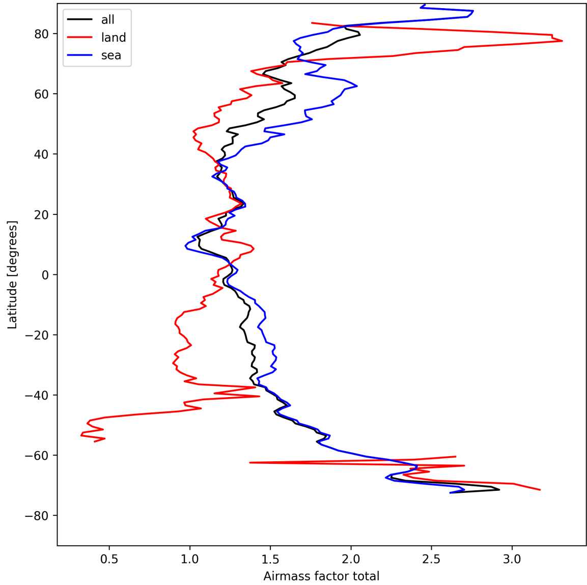
Figure 24: Zonal average of “Airmass factor total” for 2025-08-18 to 2025-08-19.
