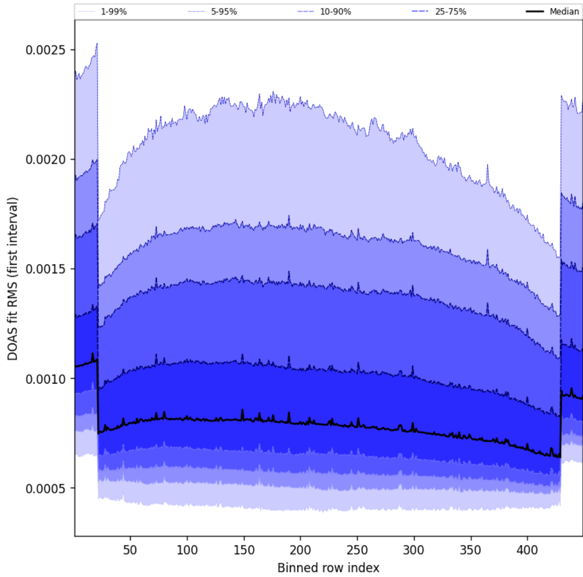
Figure 58: Along track statistics of “DOAS fit RMS (first interval)” for 2025-08-18 to 2025-08-19
