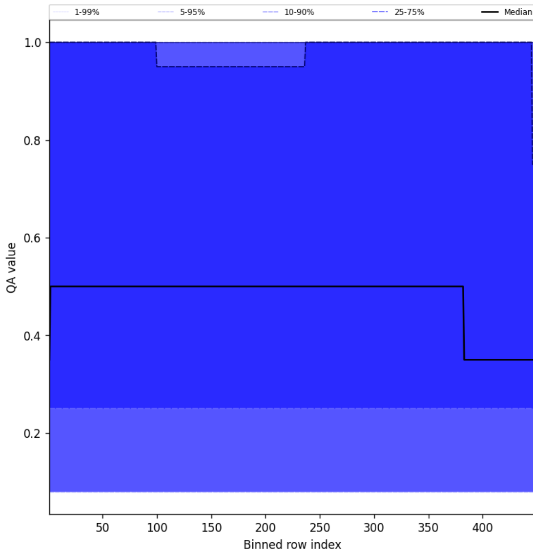
Figure 46: Along track statistics of “QA value” for 2025-08-18 to 2025-08-19
