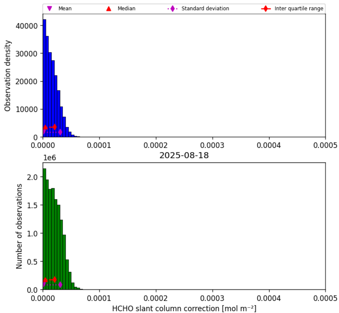
Figure 45: Histogram of “HCHO slant column correction” for 2025-08-18 to 2025-08-19
