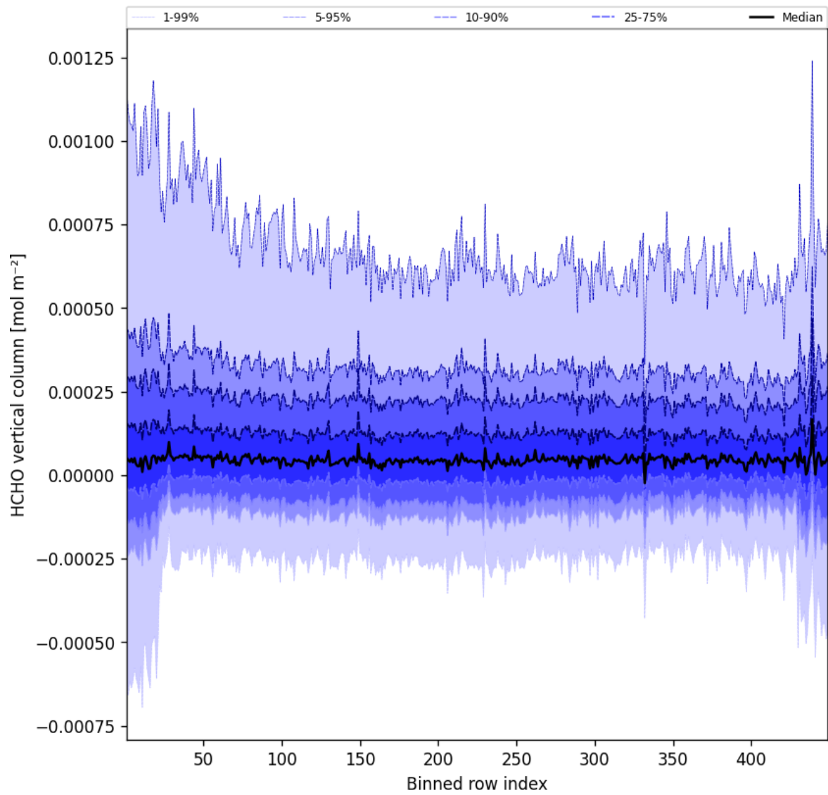
Figure 47: Along track statistics of “HCHO vertical column” for 2025-08-18 to 2025-08-19
