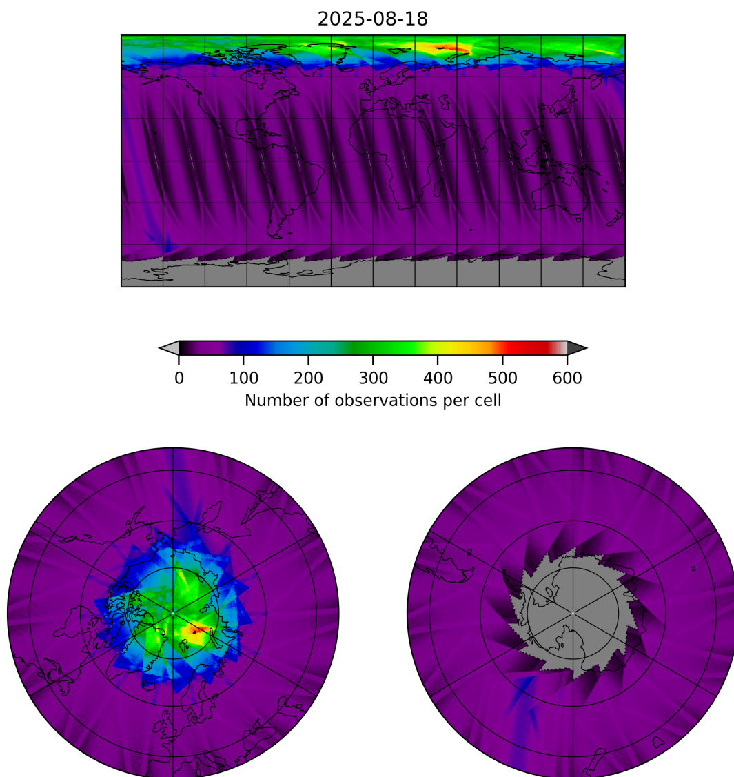
Figure 17: Map of the number of observations for 2025-08-18 to 2025-08-19
