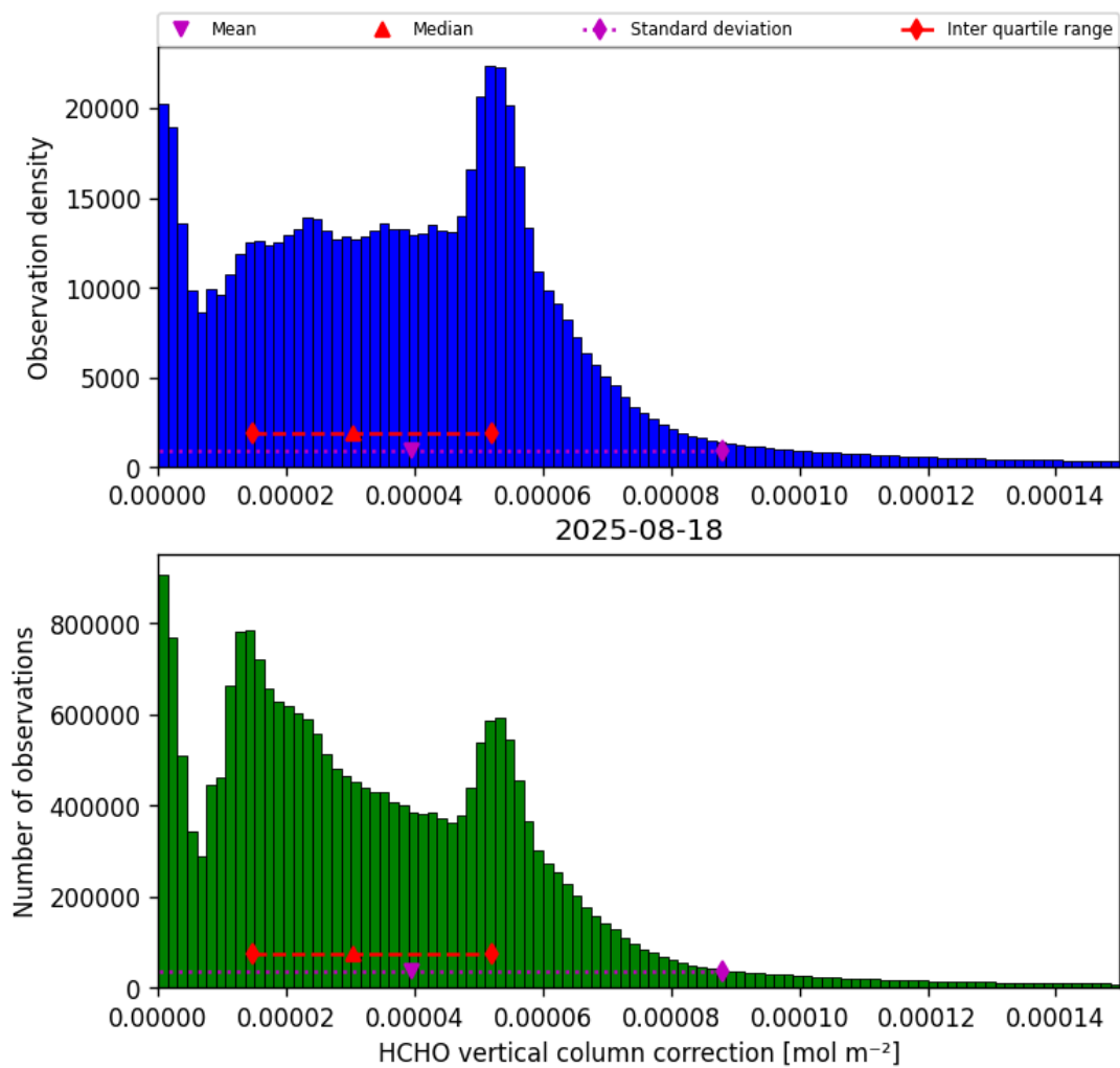
Figure 35: Histogram of “HCHO vertical column correction” for 2025-08-18 to 2025-08-19
