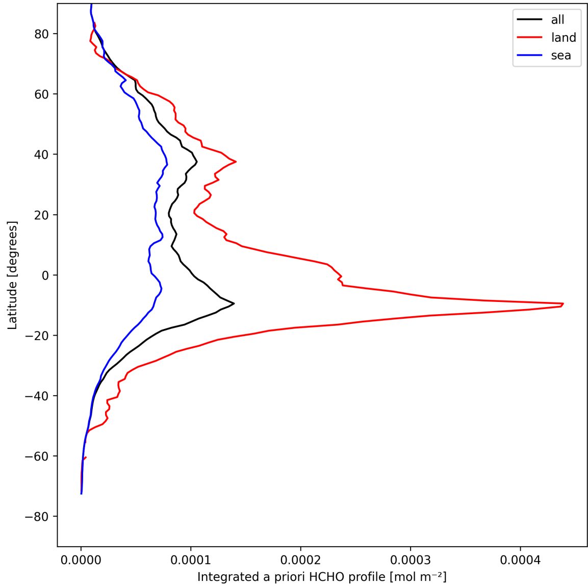
Figure 27: Zonal average of “Integrated a priori HCHO profile” for 2025-08-18 to 2025-08-19.
