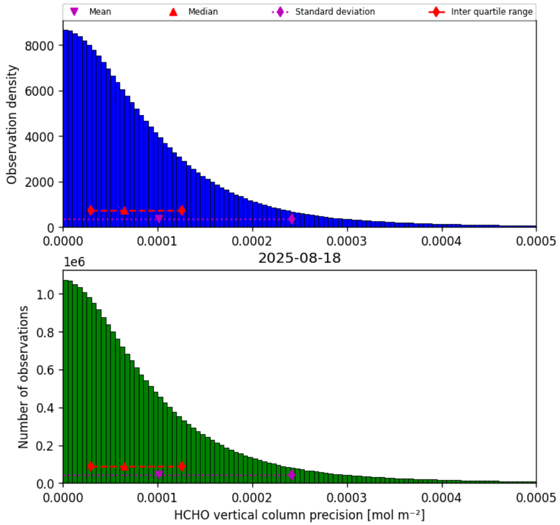
Figure 34: Histogram of “HCHO vertical column precision” for 2025-08-18 to 2025-08-19
