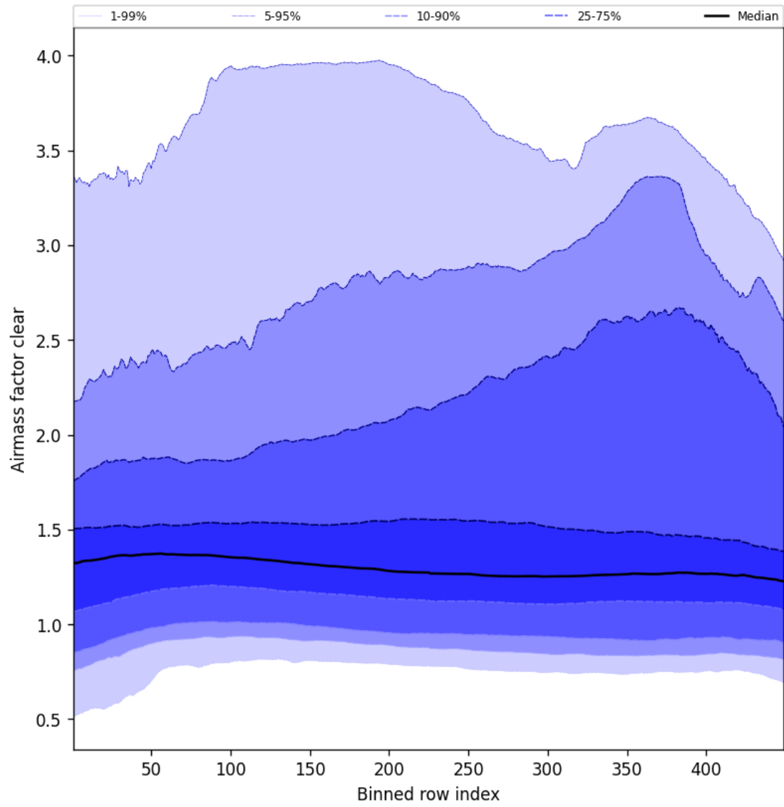
Figure 54: Along track statistics of “Airmass factor clear” for 2025-08-18 to 2025-08-19
