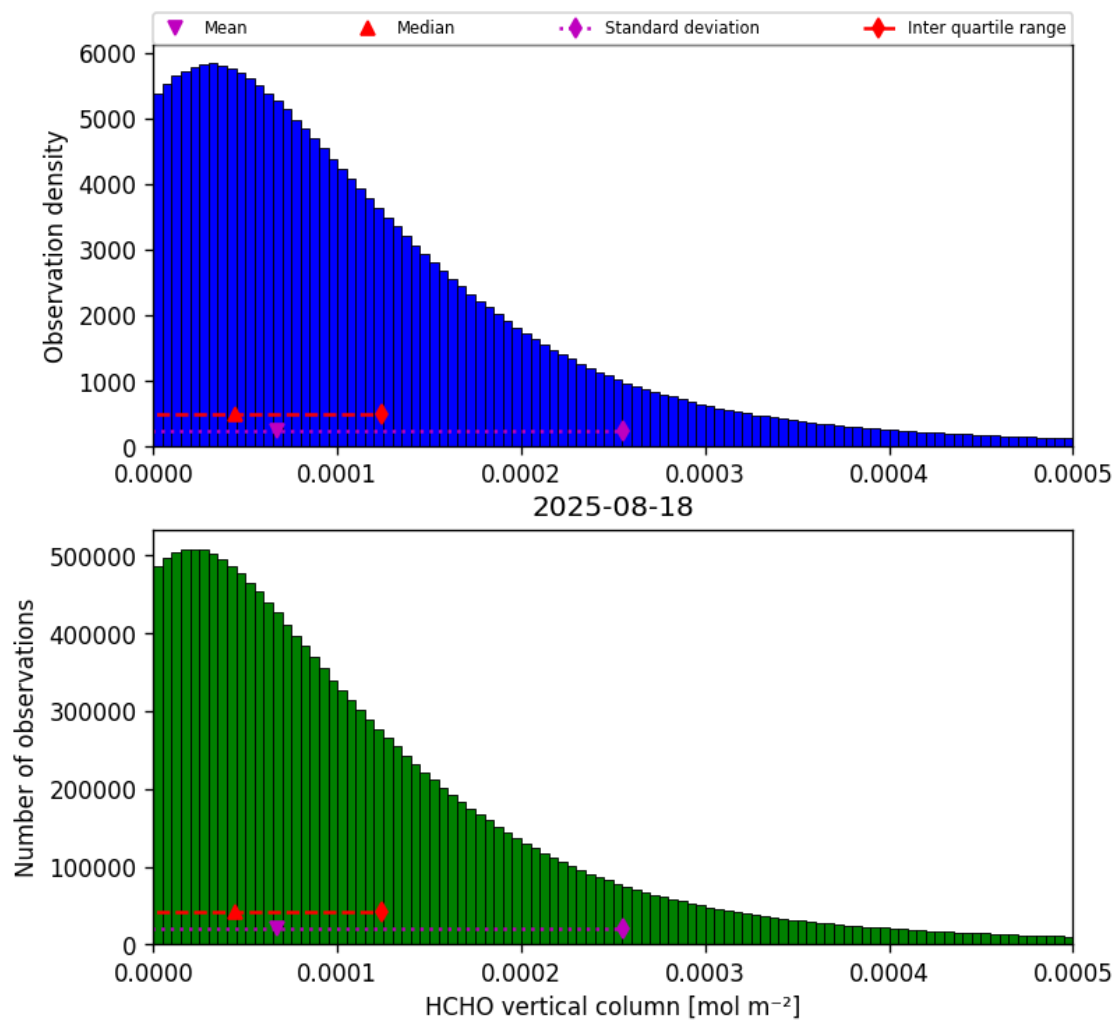
Figure 33: Histogram of “HCHO vertical column” for 2025-08-18 to 2025-08-19
