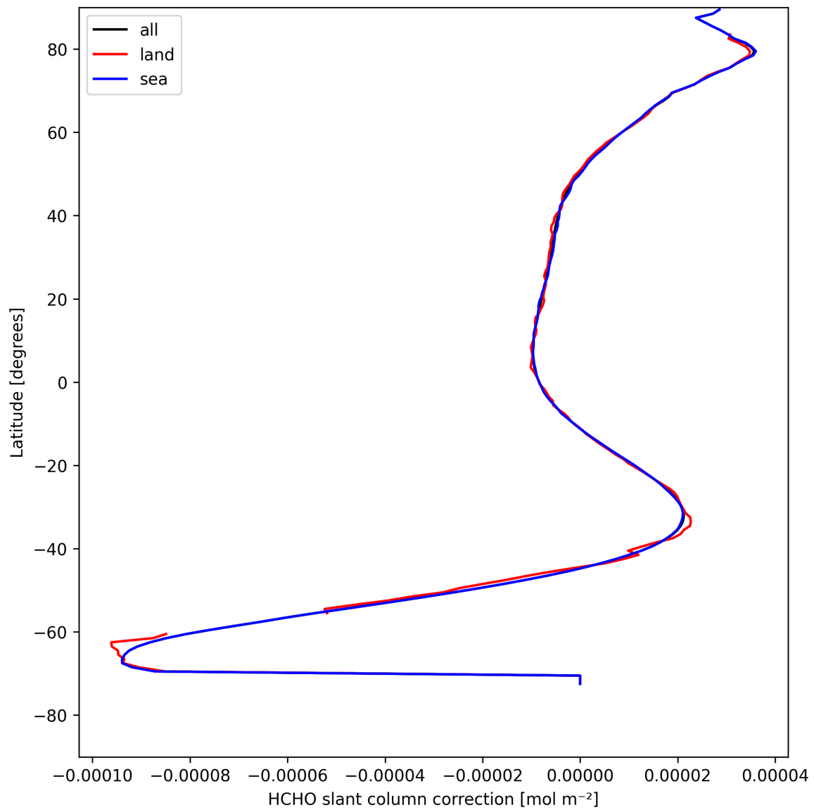
Figure 31: Zonal average of “HCHO slant column correction” for 2025-08-18 to 2025-08-19.
