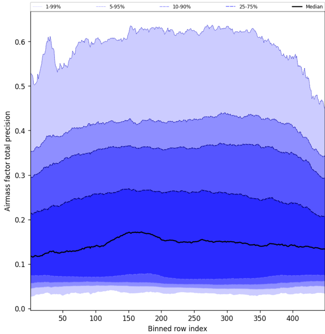
Figure 53: Along track statistics of “Airmass factor total precision” for 2025-08-18 to 2025-08-19
