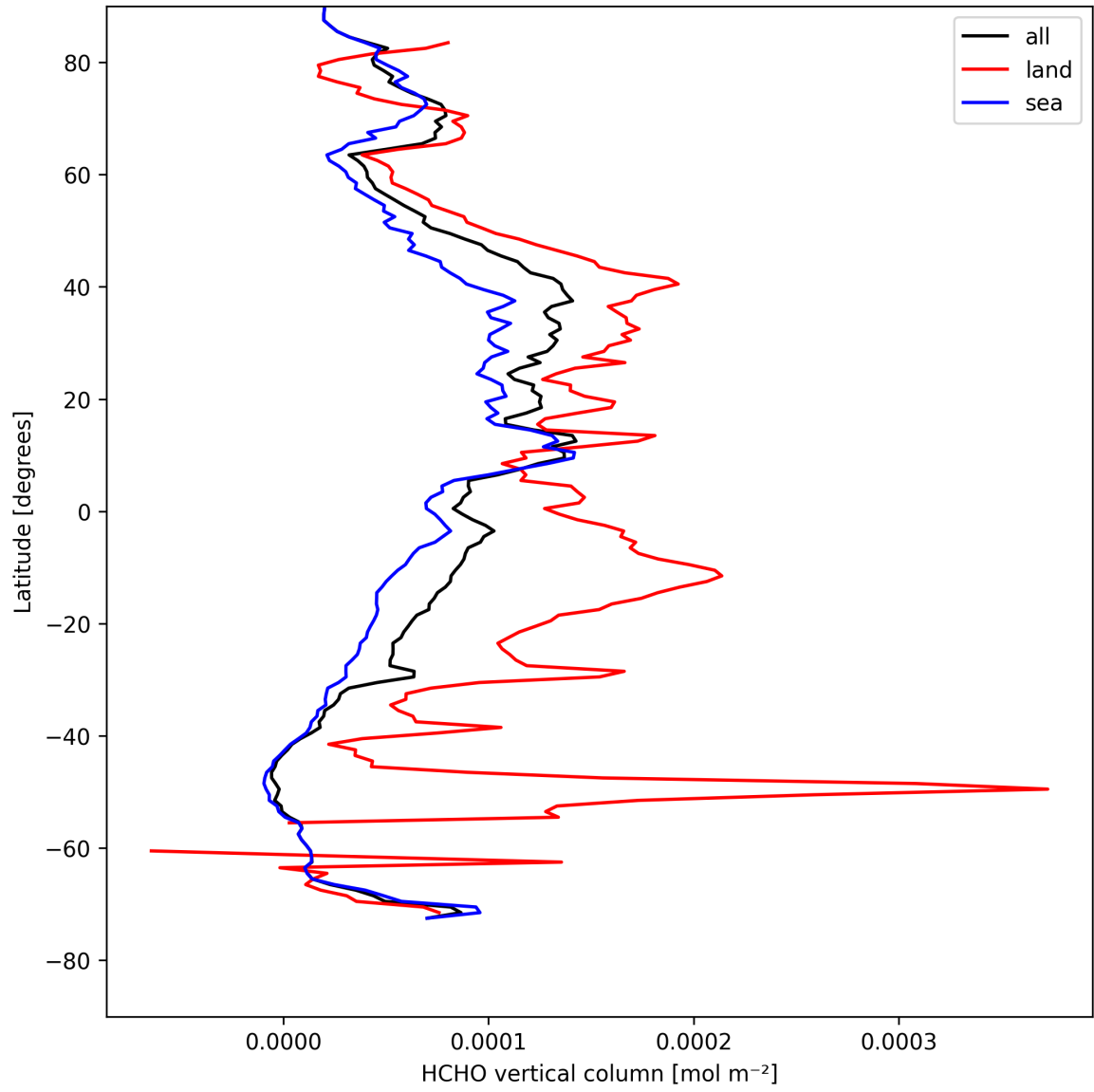
Figure 19: Zonal average of “HCHO vertical column” for 2025-08-18 to 2025-08-19.
