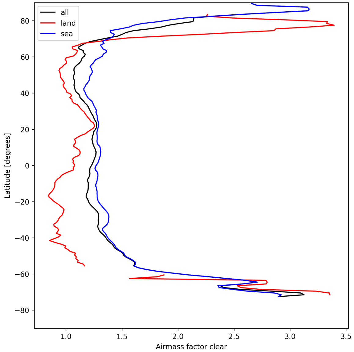
Figure 26: Zonal average of “Airmass factor clear” for 2025-08-18 to 2025-08-19.
