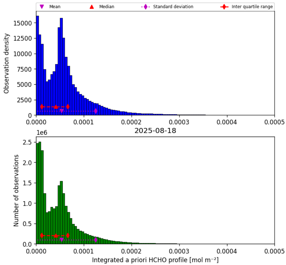
Figure 41: Histogram of “Integrated a priori HCHO profile” for 2025-08-18 to 2025-08-19
