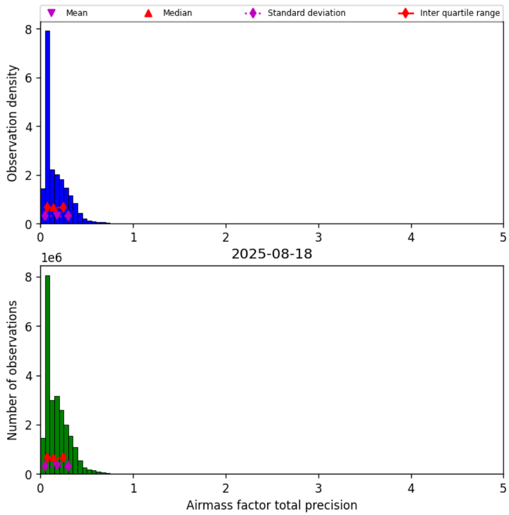
Figure 39: Histogram of “Airmass factor total precision” for 2025-08-18 to 2025-08-19
