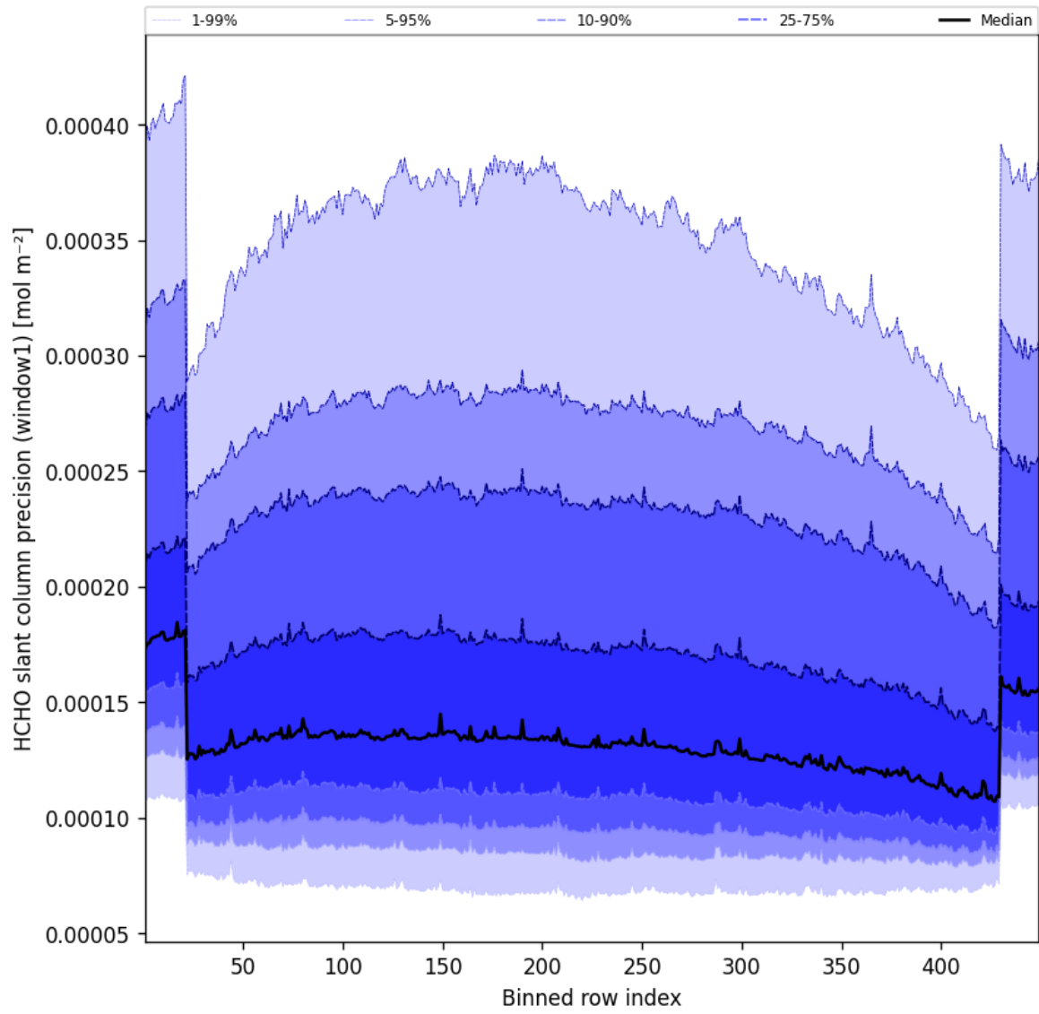
Figure 51: Along track statistics of “HCHO slant column precision (window1)” for 2025-08-18 to 2025-08-19
