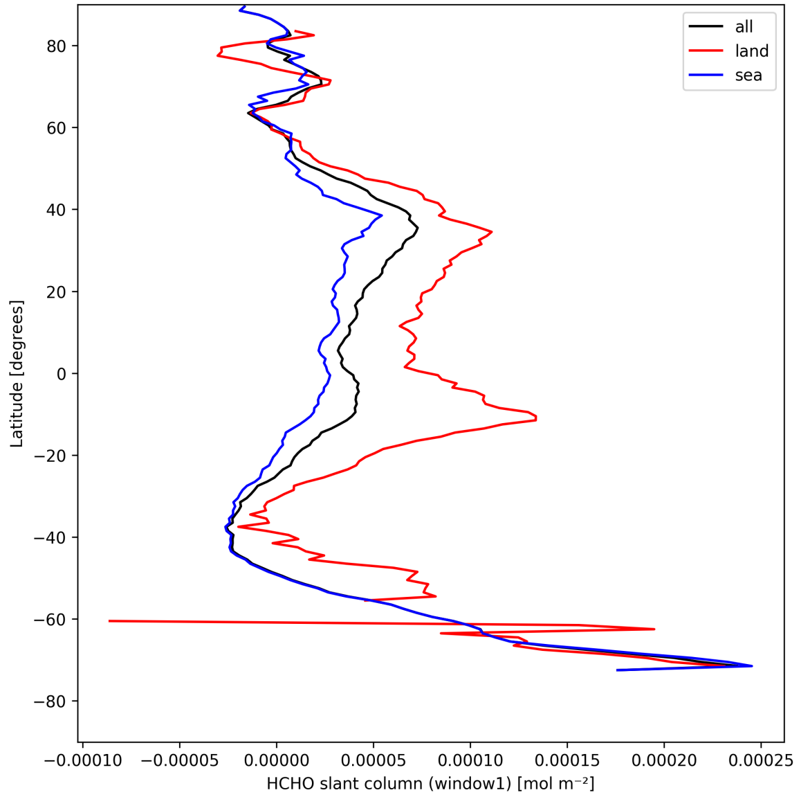
Figure 22: Zonal average of “HCHO slant column (window1)” for 2025-08-18 to 2025-08-19.
