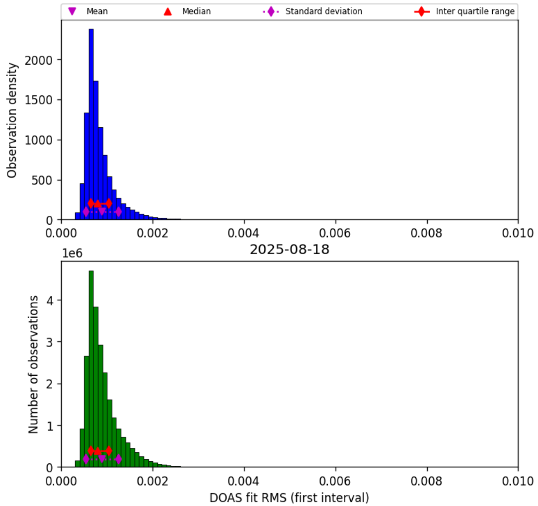
Figure 44: Histogram of “DOAS fit RMS (first interval)” for 2025-08-18 to 2025-08-19
