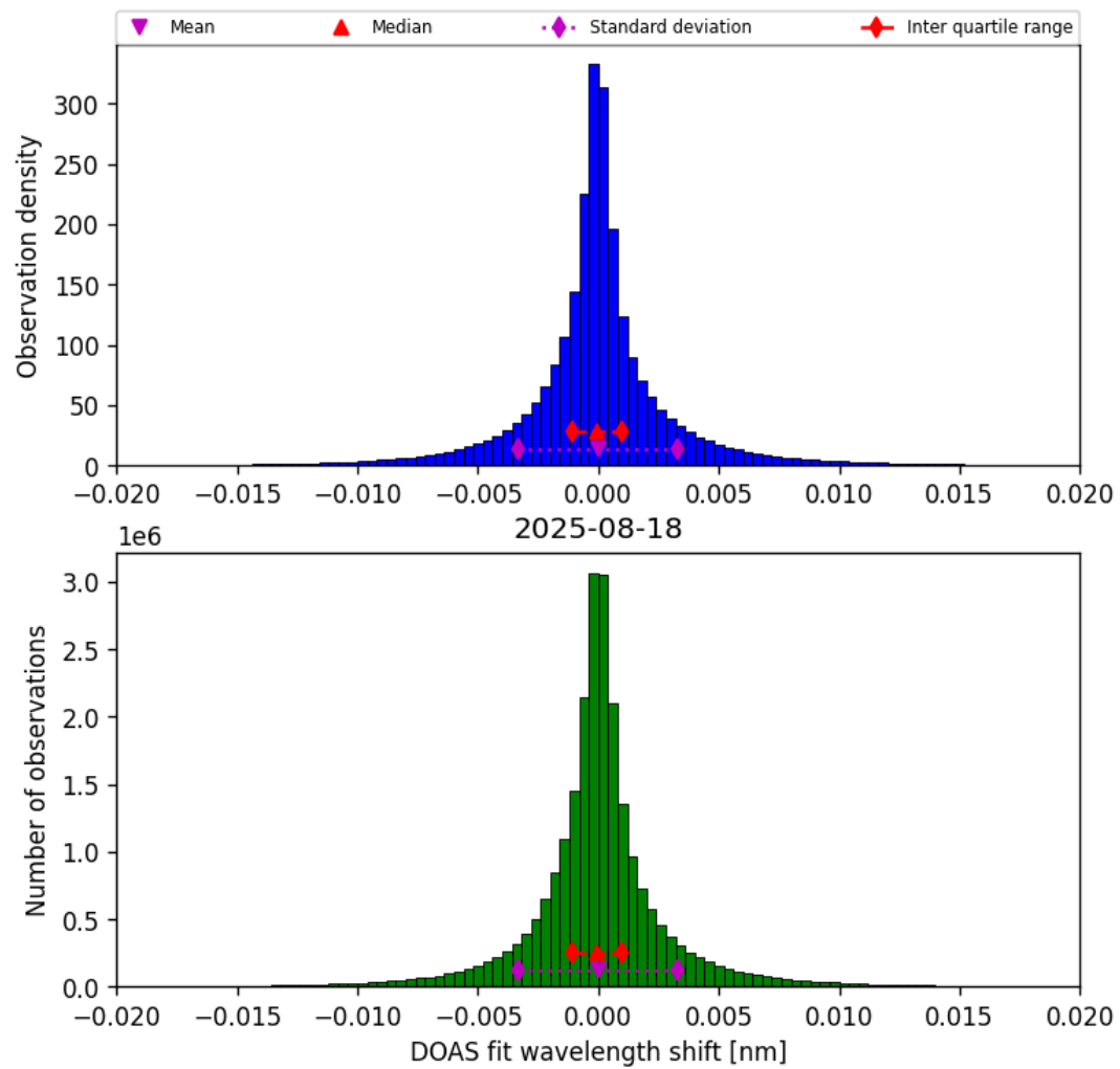
Figure 42: Histogram of “DOAS fit wavelength shift” for 2025-08-18 to 2025-08-19
