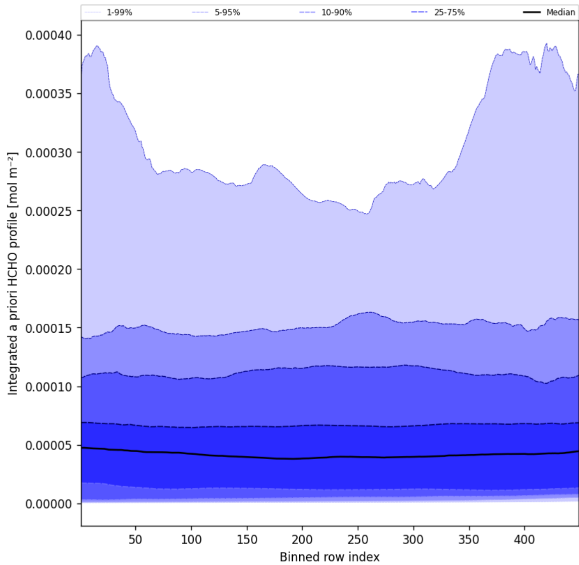
Figure 55: Along track statistics of “Integrated a priori HCHO profile” for 2025-08-18 to 2025-08-19
