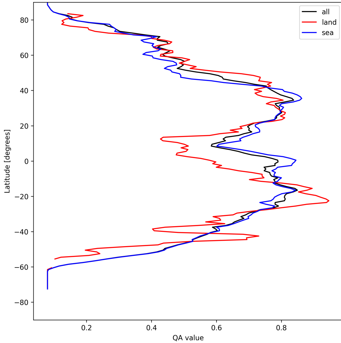
Figure 18: Zonal average of “QA value” for 2025-08-18 to 2025-08-19.
