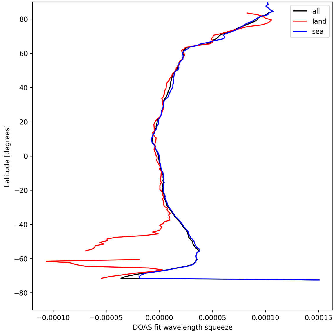
Figure 29: Zonal average of “DOAS fit wavelength squeeze” for 2025-08-18 to 2025-08-19.
