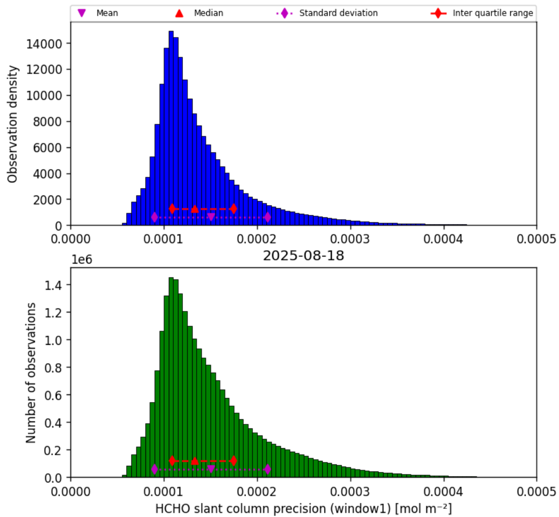
Figure 37: Histogram of “HCHO slant column precision (window1)” for 2025-08-18 to 2025-08-19
