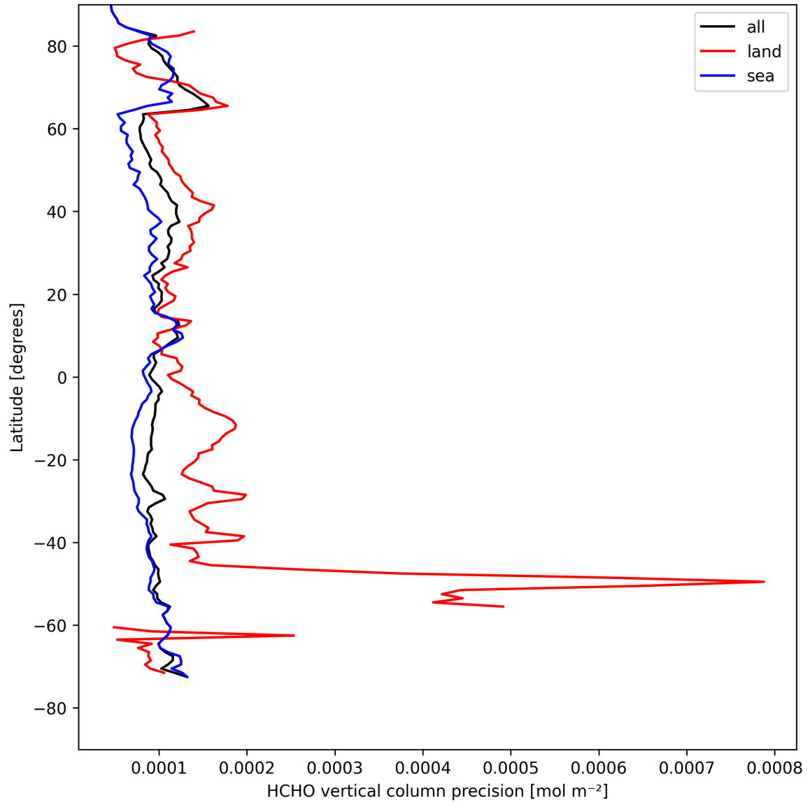
Figure 20: Zonal average of “HCHO vertical column precision” for 2025-08-18 to 2025-08-19.
