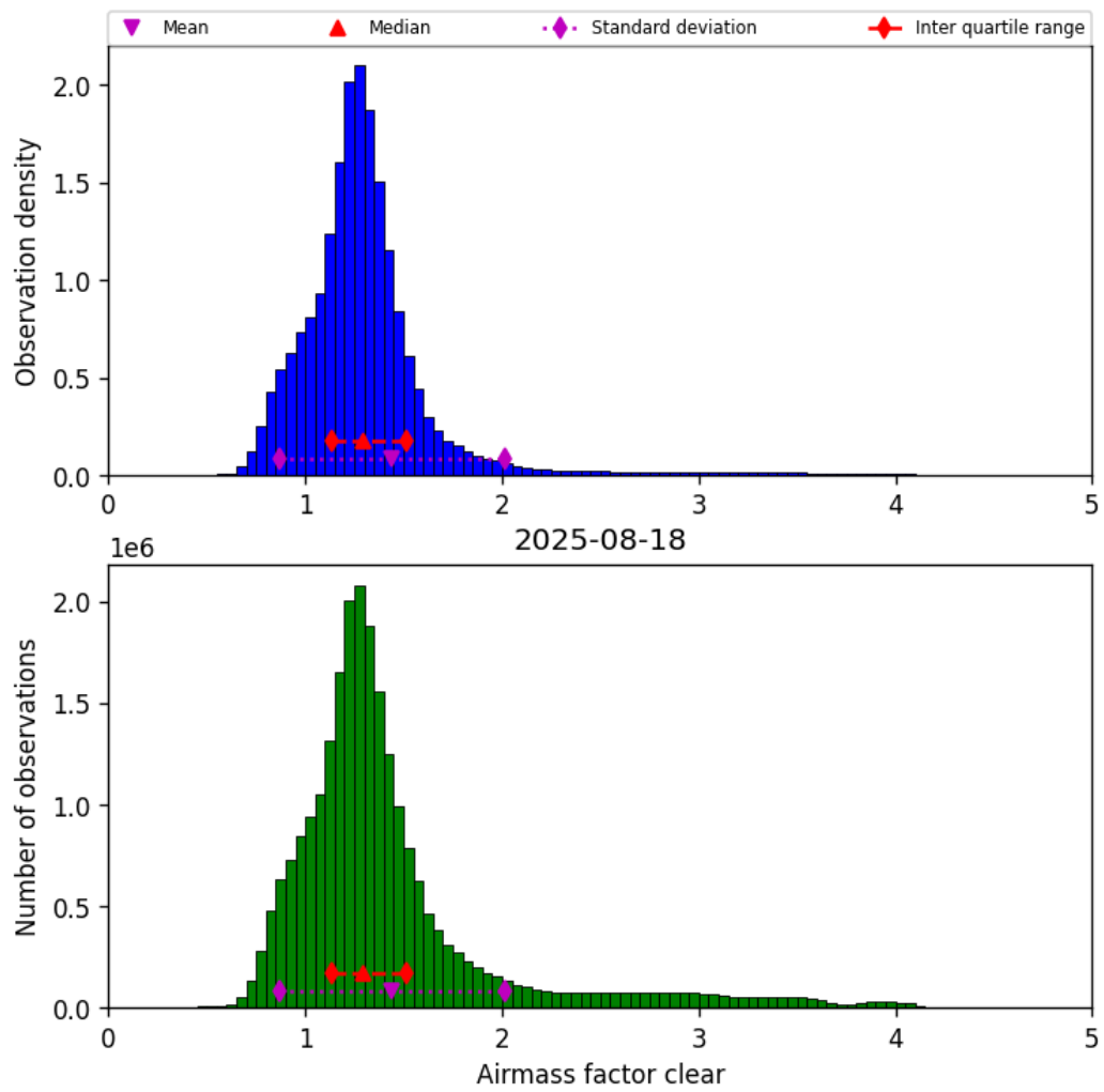
Figure 40: Histogram of “Airmass factor clear” for 2025-08-18 to 2025-08-19
