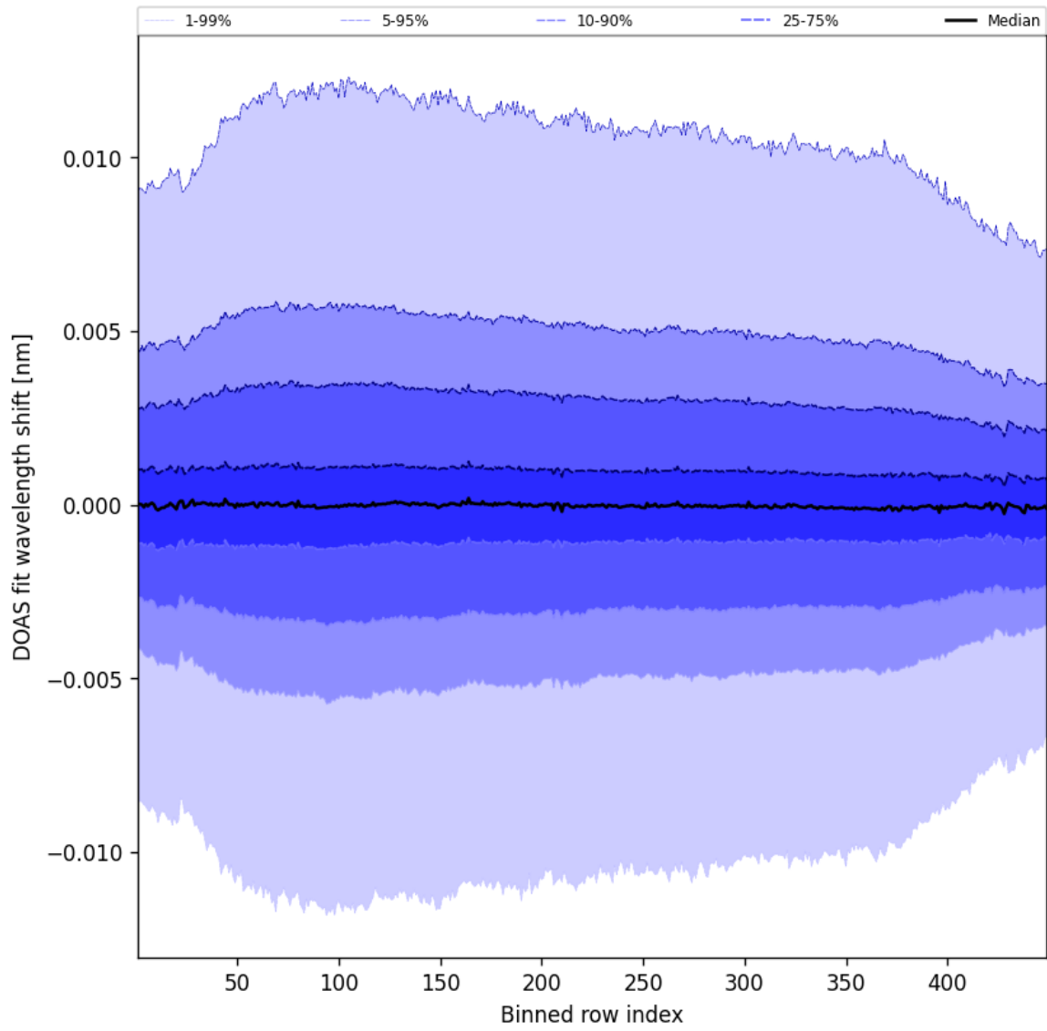
Figure 56: Along track statistics of “DOAS fit wavelength shift” for 2025-08-18 to 2025-08-19
