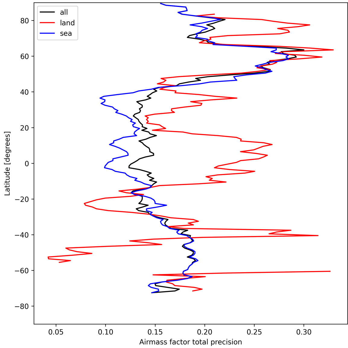
Figure 25: Zonal average of “Airmass factor total precision” for 2025-08-18 to 2025-08-19.
