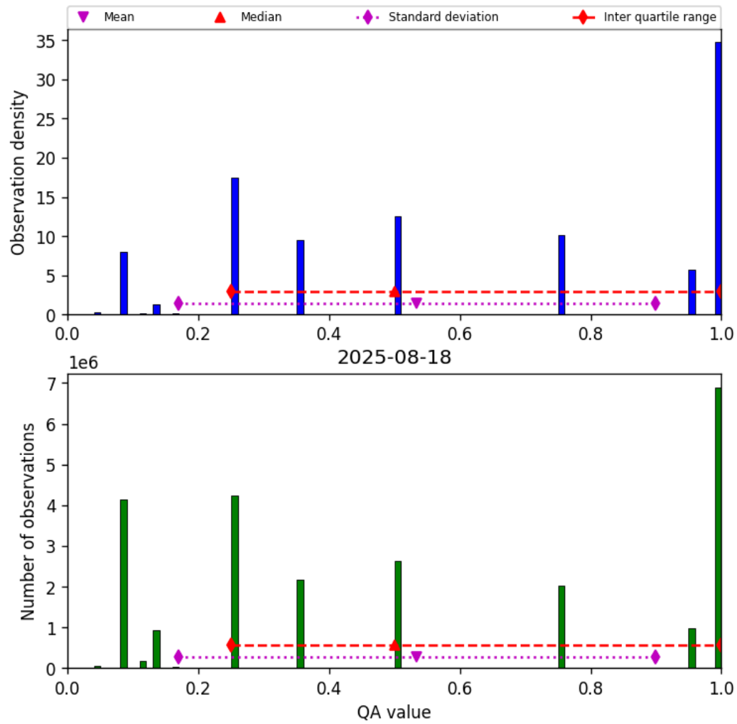
Figure 32: Histogram of “QA value” for 2025-08-18 to 2025-08-19
