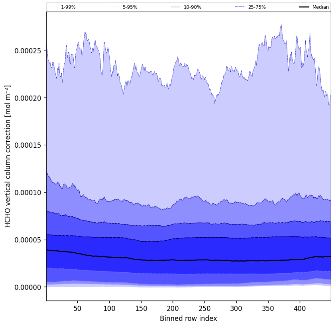
Figure 49: Along track statistics of “HCHO vertical column correction” for 2025-08-18 to 2025-08-19
