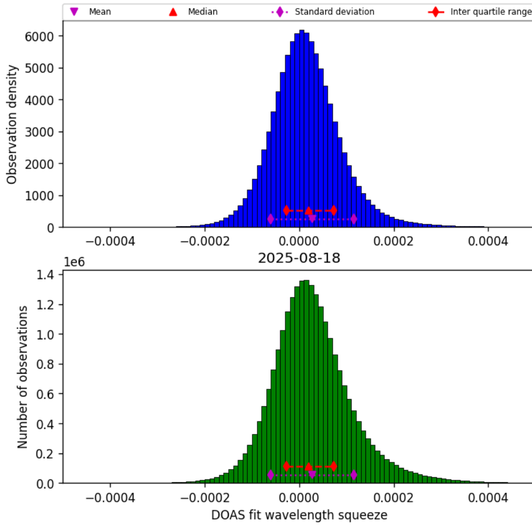
Figure 43: Histogram of “DOAS fit wavelength squeeze” for 2025-08-18 to 2025-08-19
