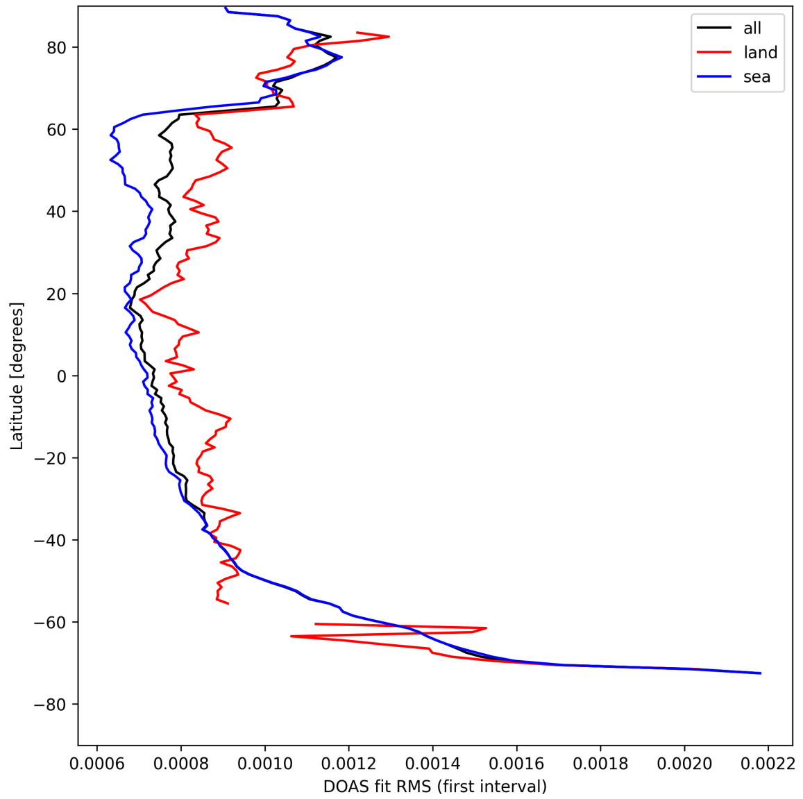
Figure 30: Zonal average of “DOAS fit RMS (first interval)” for 2025-08-18 to 2025-08-19.
