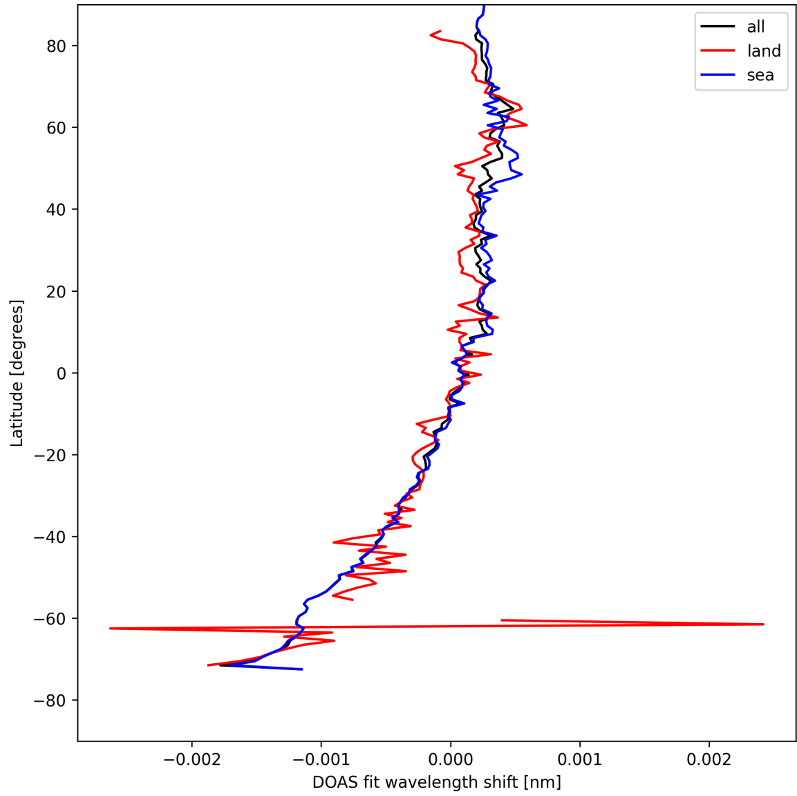
Figure 28: Zonal average of “DOAS fit wavelength shift” for 2025-08-18 to 2025-08-19.
