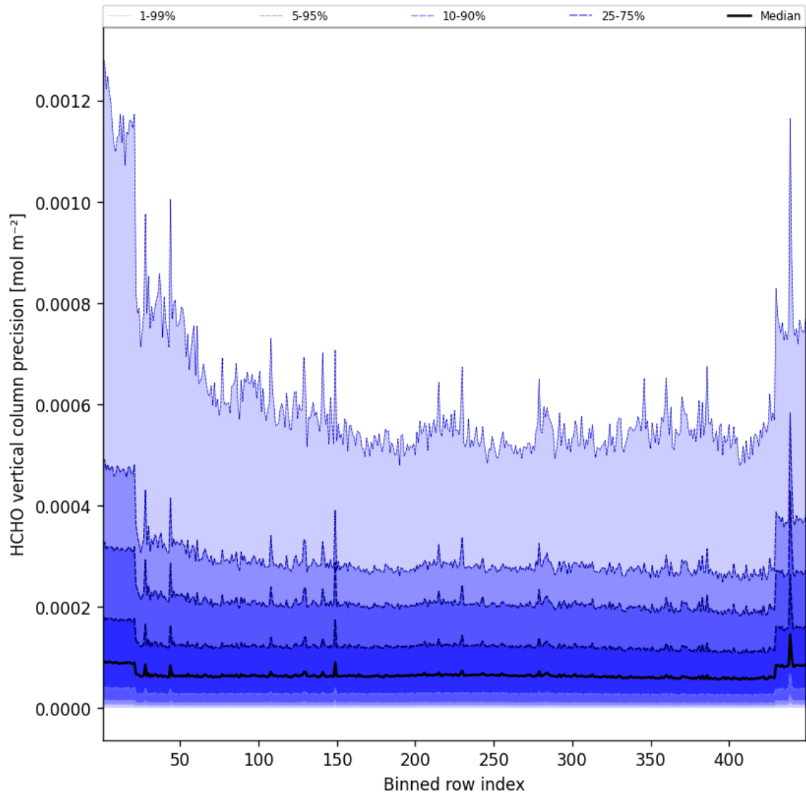
Figure 48: Along track statistics of “HCHO vertical column precision” for 2025-08-18 to 2025-08-19
