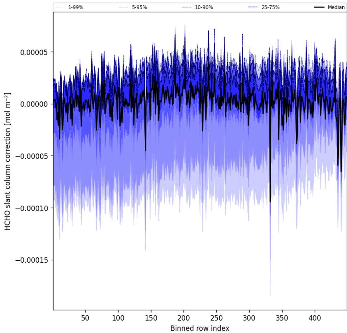
Figure 59: Along track statistics of “HCHO slant column correction” for 2025-08-18 to 2025-08-19
