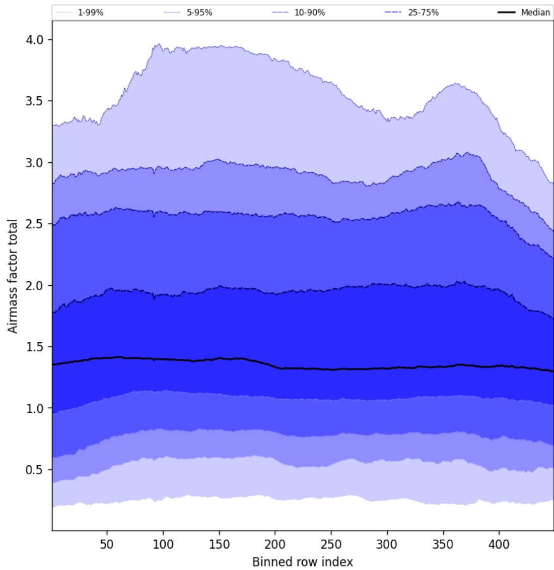
Figure 52: Along track statistics of “Airmass factor total” for 2025-08-18 to 2025-08-19
