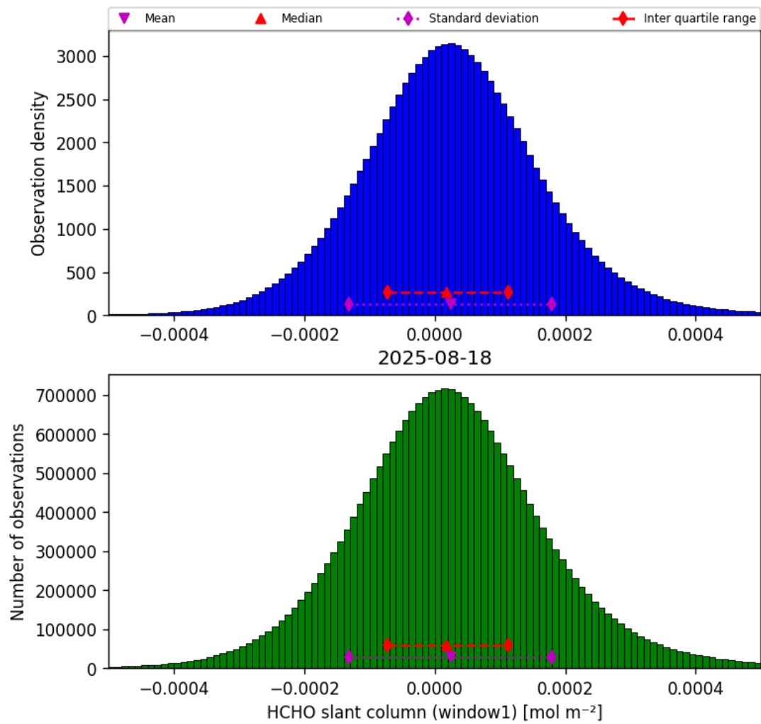
Figure 36: Histogram of “HCHO slant column (window1)” for 2025-08-18 to 2025-08-19
