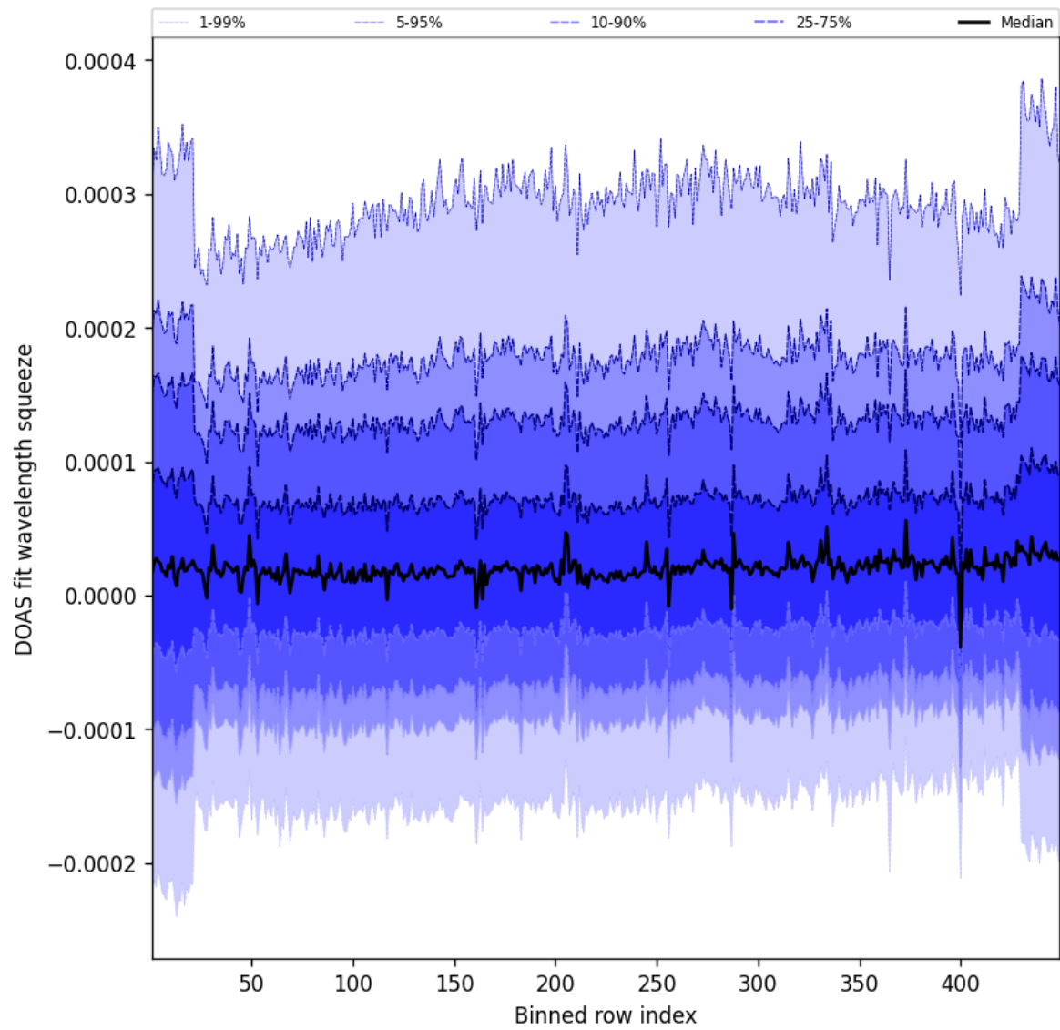
Figure 57: Along track statistics of “DOAS fit wavelength squeeze” for 2025-08-18 to 2025-08-19
