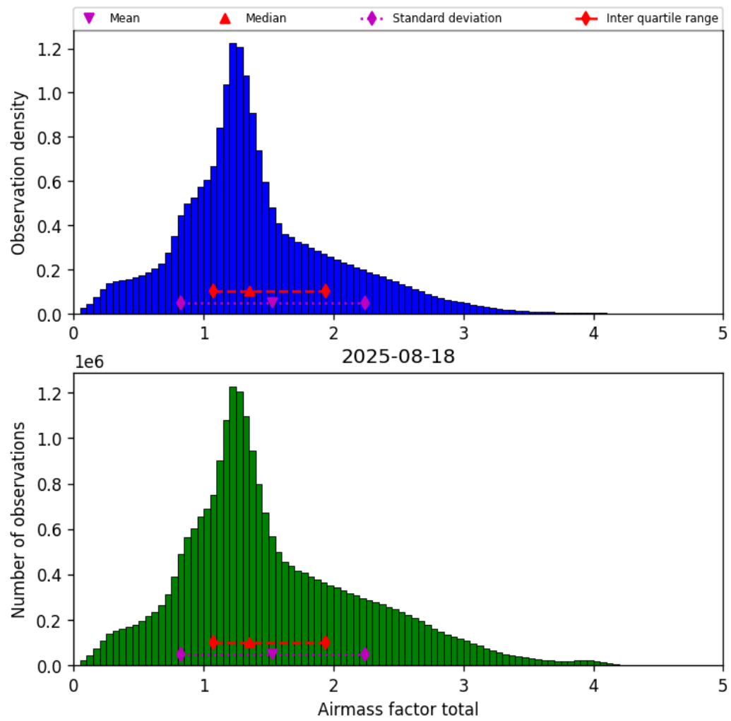
Figure 38: Histogram of “Airmass factor total” for 2025-08-18 to 2025-08-19
