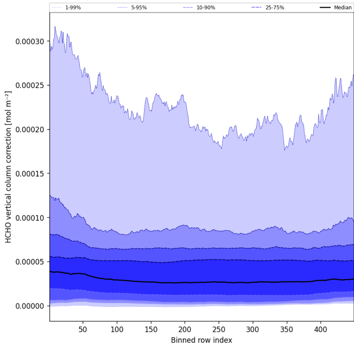
Figure 49: Along track statistics of “HCHO vertical column correction” for 2025-08-20 to 2025-08-21
