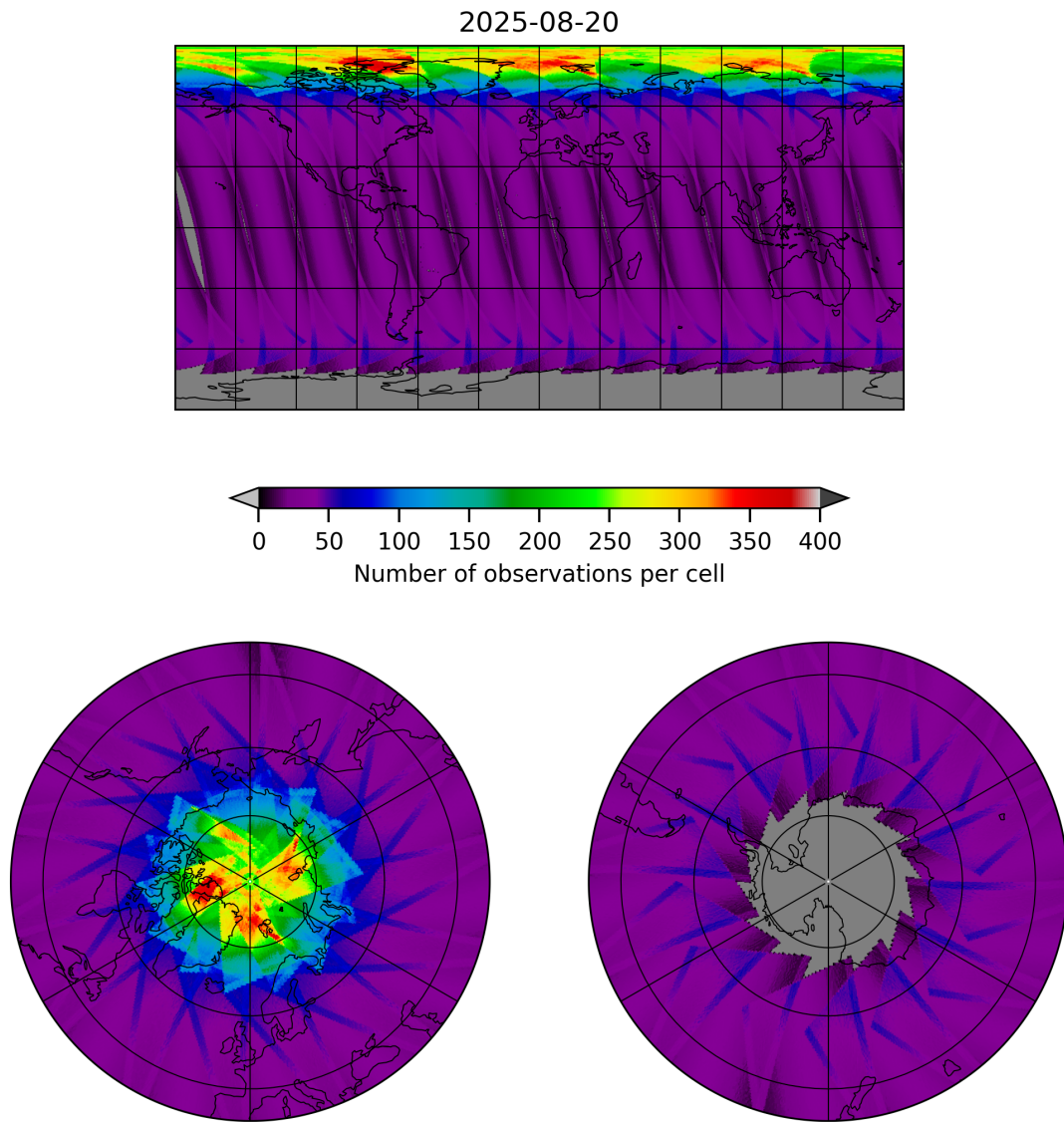
Figure 17: Map of the number of observations for 2025-08-20 to 2025-08-21
