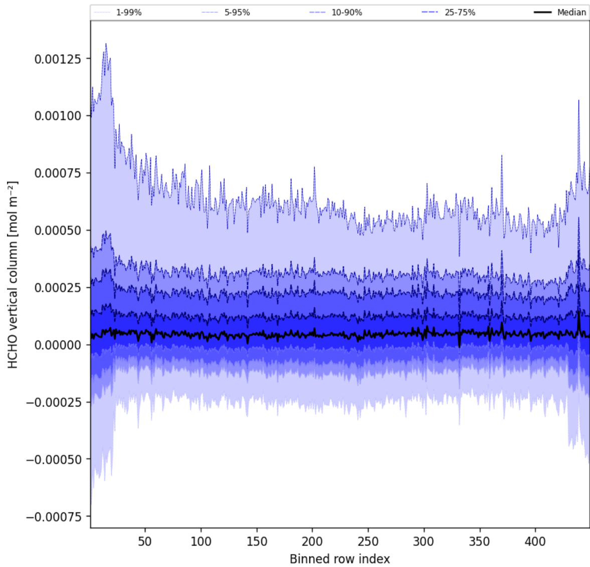
Figure 47: Along track statistics of “HCHO vertical column” for 2025-08-20 to 2025-08-21
