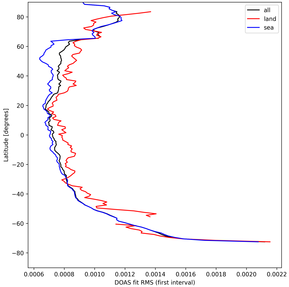
Figure 30: Zonal average of “DOAS fit RMS (first interval)” for 2025-08-20 to 2025-08-21.
