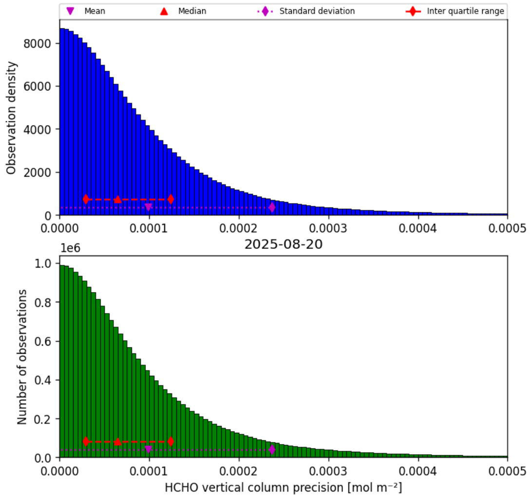
Figure 34: Histogram of “HCHO vertical column precision” for 2025-08-20 to 2025-08-21
