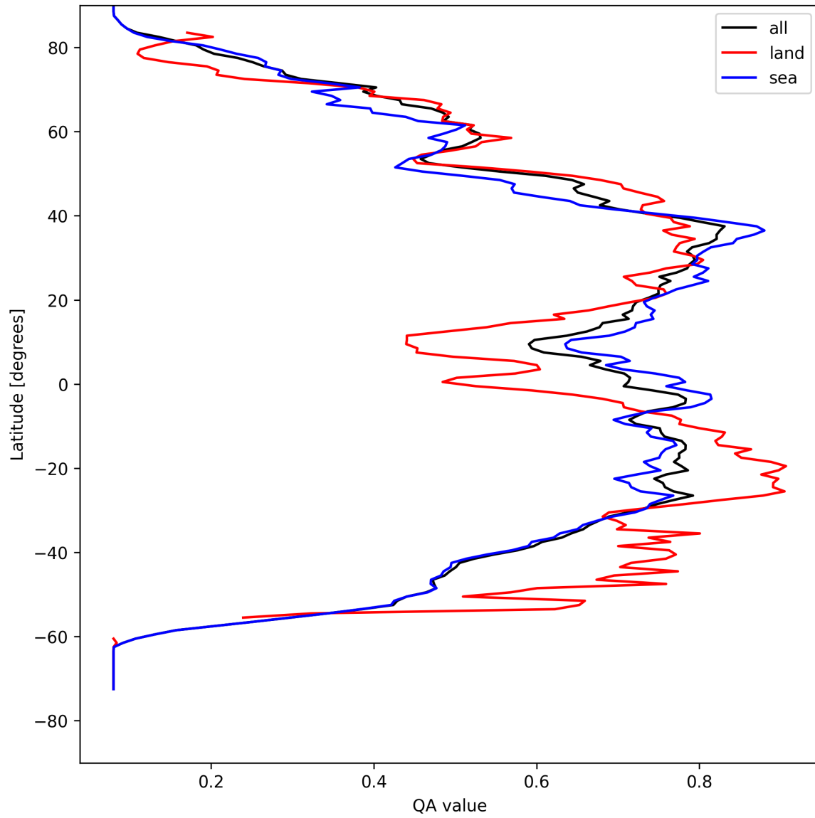
Figure 18: Zonal average of “QA value” for 2025-08-20 to 2025-08-21.
