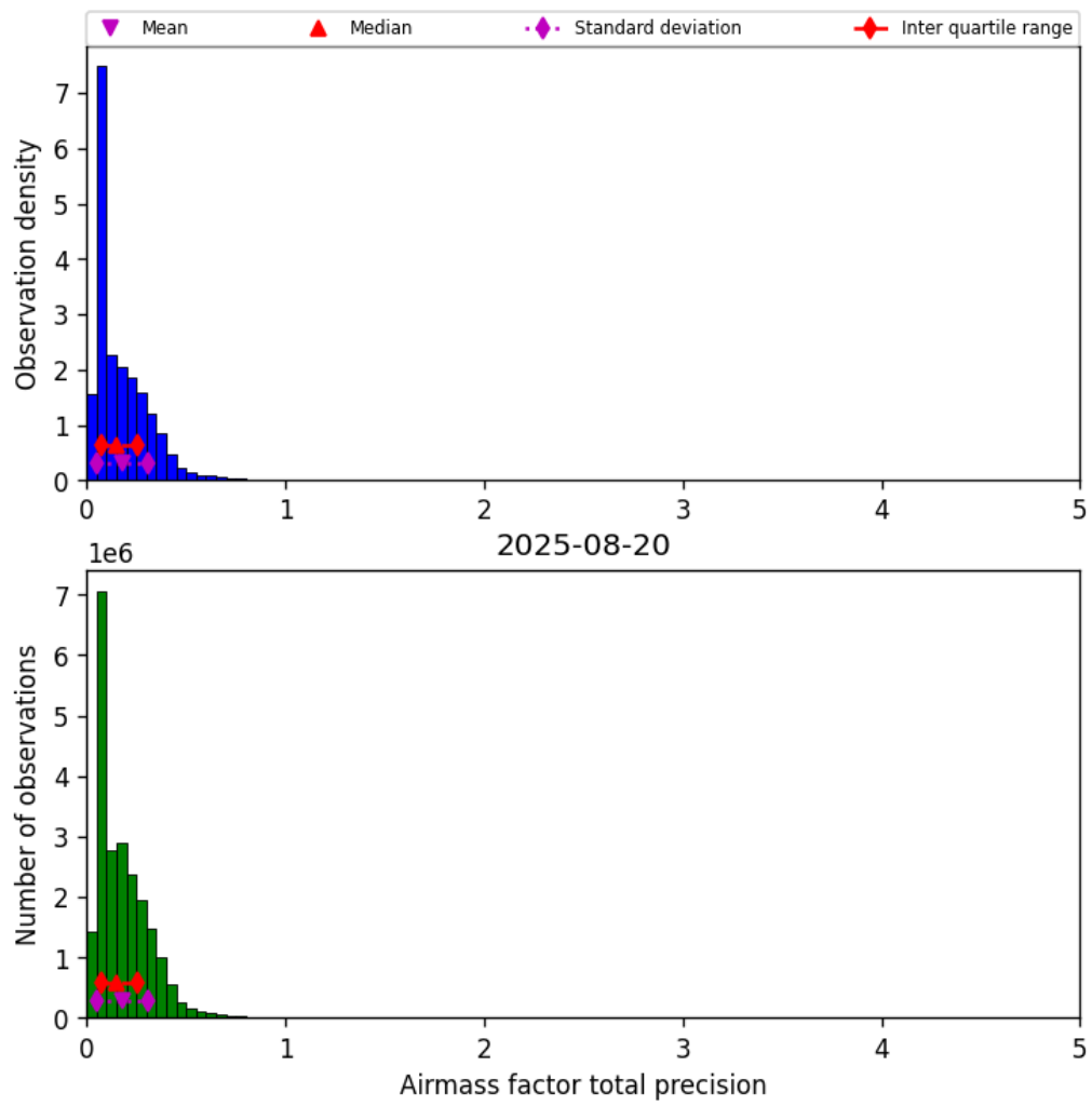
Figure 39: Histogram of “Airmass factor total precision” for 2025-08-20 to 2025-08-21
