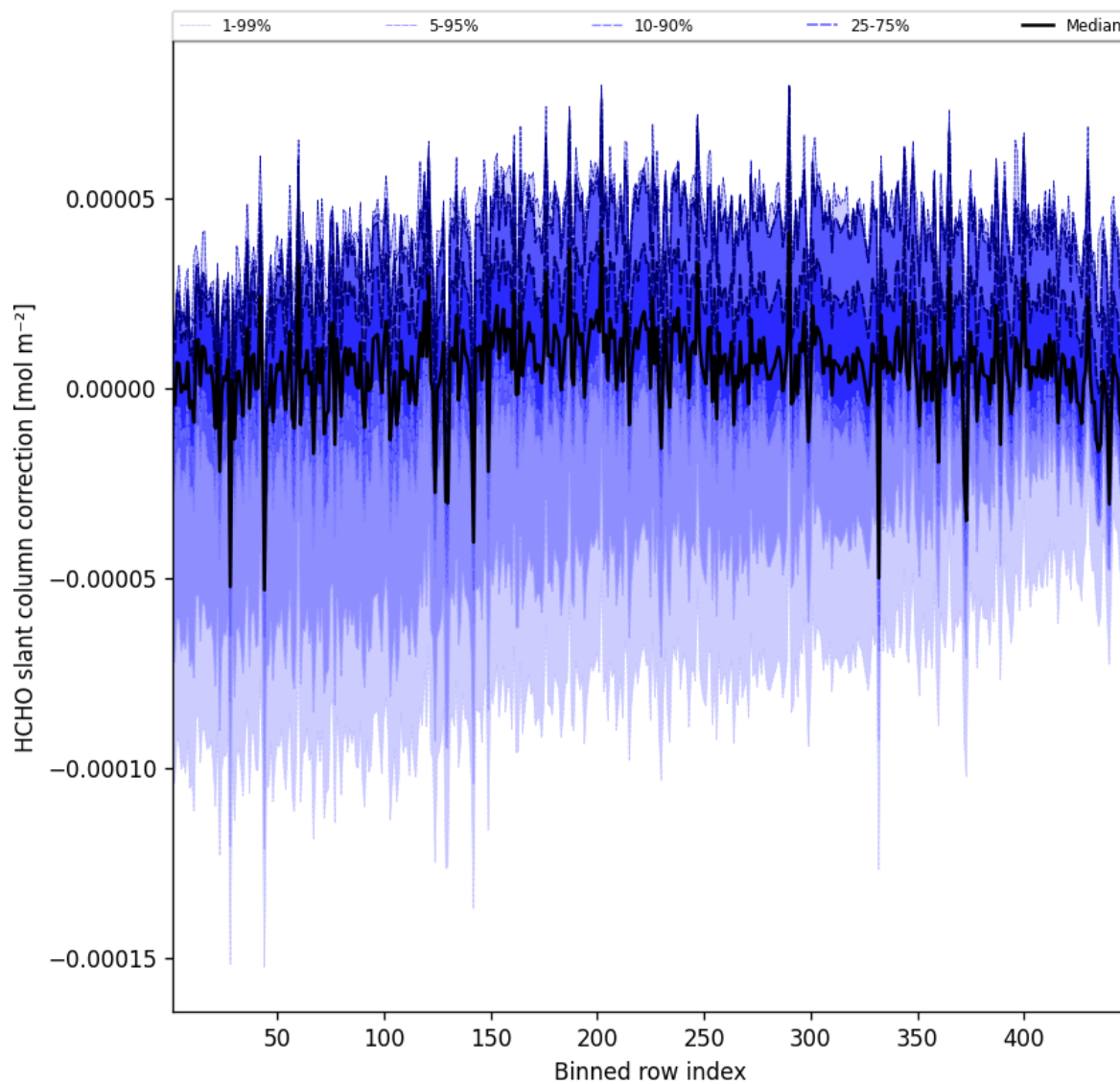
Figure 59: Along track statistics of “HCHO slant column correction” for 2025-08-20 to 2025-08-21
