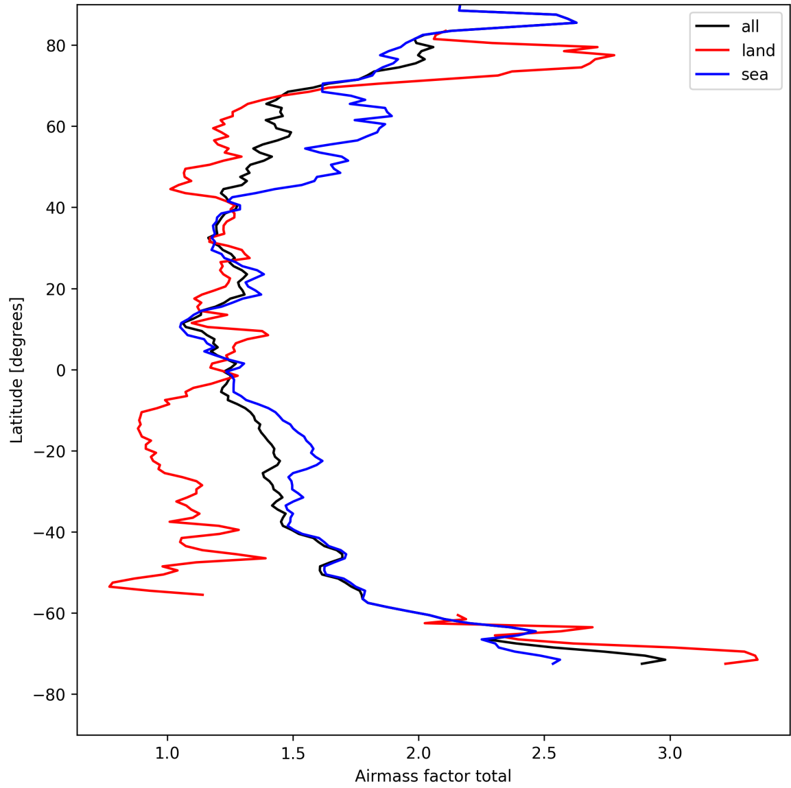
Figure 24: Zonal average of “Airmass factor total” for 2025-08-20 to 2025-08-21.
