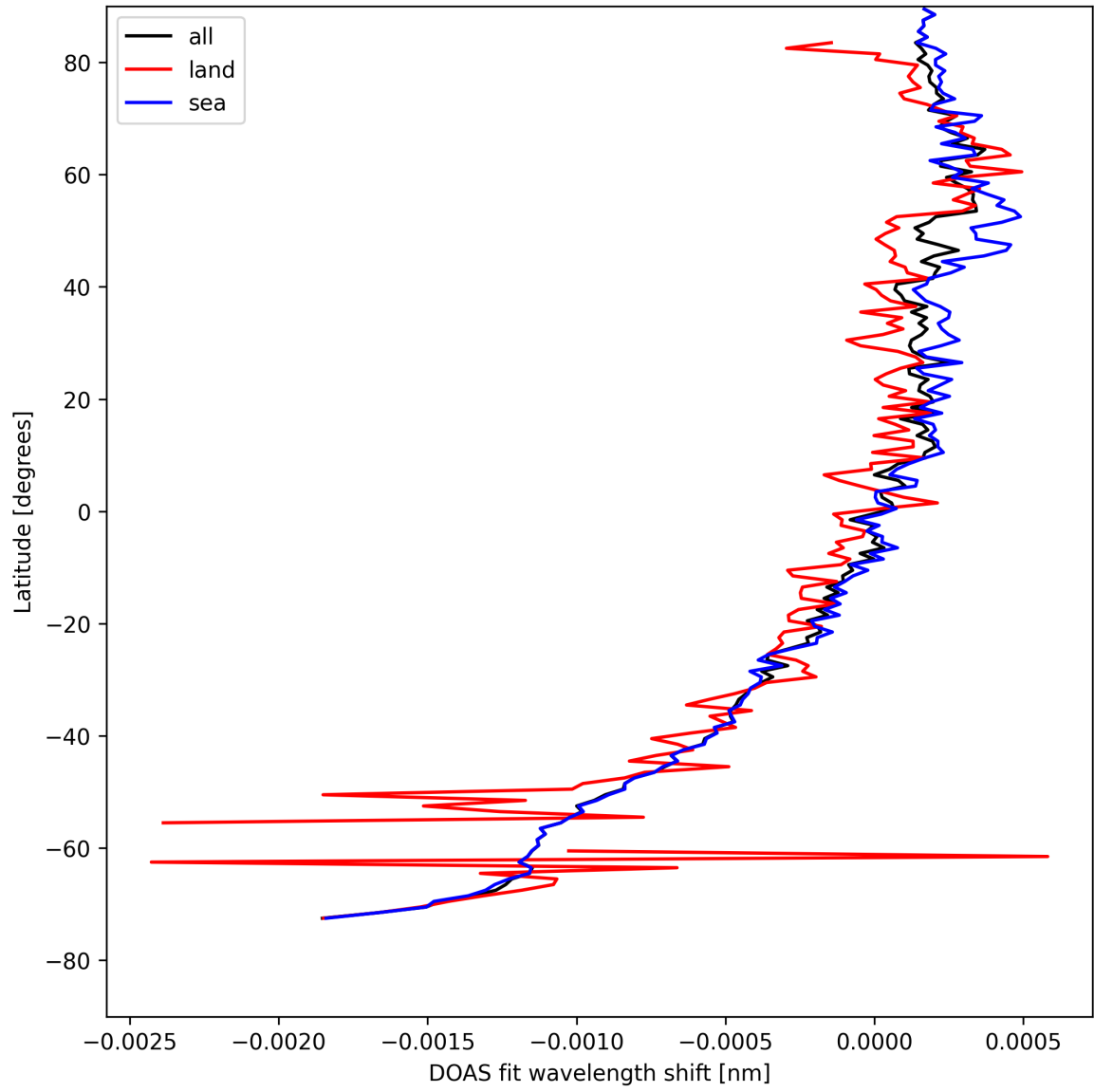
Figure 28: Zonal average of “DOAS fit wavelength shift” for 2025-08-20 to 2025-08-21.
