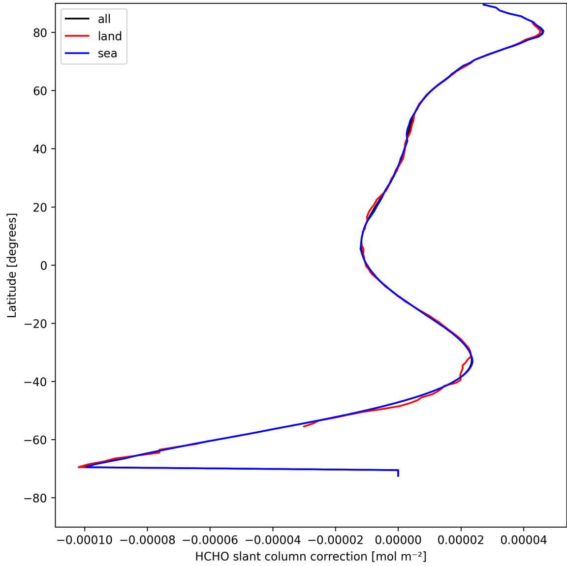
Figure 31: Zonal average of “HCHO slant column correction” for 2025-08-20 to 2025-08-21.
