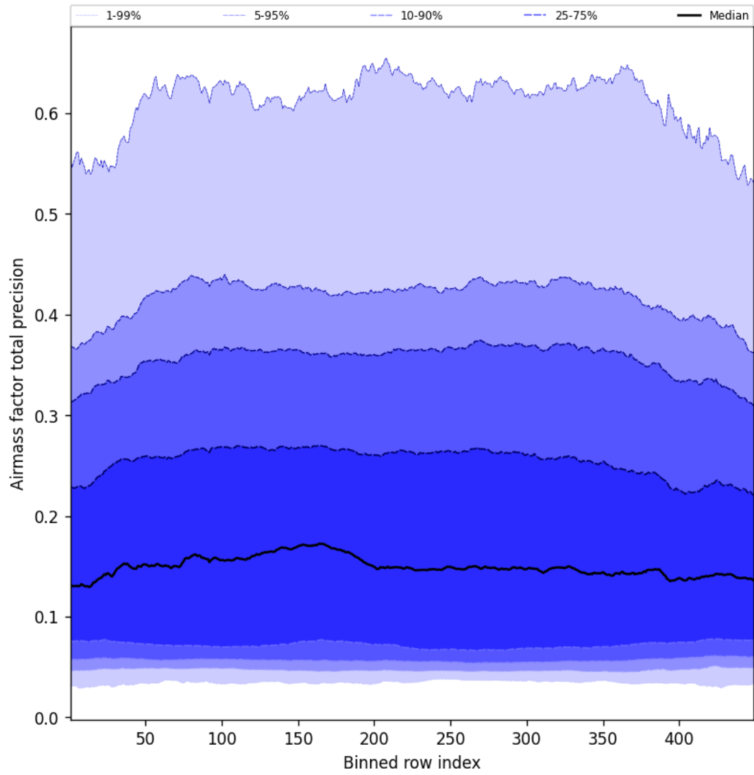
Figure 53: Along track statistics of “Airmass factor total precision” for 2025-08-20 to 2025-08-21
