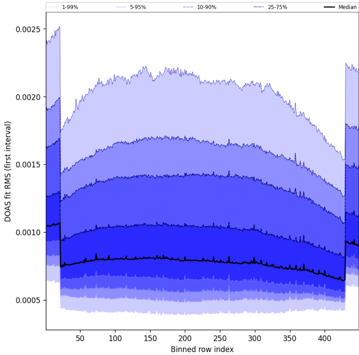
Figure 58: Along track statistics of “DOAS fit RMS (first interval)” for 2025-08-20 to 2025-08-21
