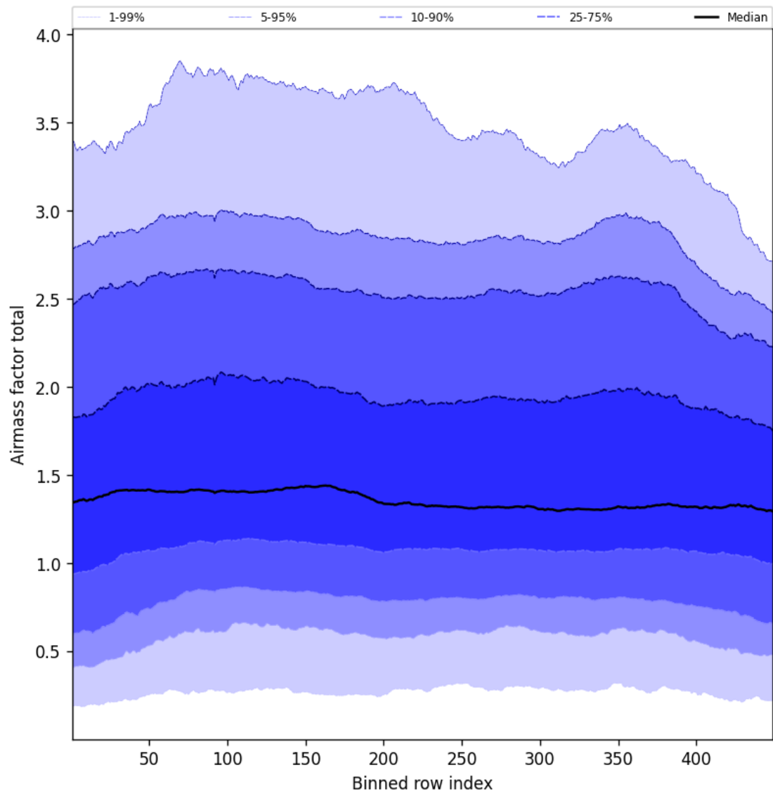
Figure 52: Along track statistics of “Airmass factor total” for 2025-08-20 to 2025-08-21
