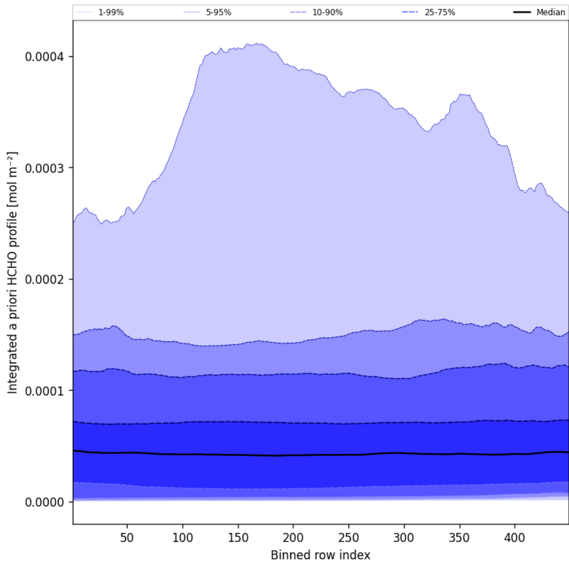
Figure 55: Along track statistics of “Integrated a priori HCHO profile” for 2025-08-20 to 2025-08-21
