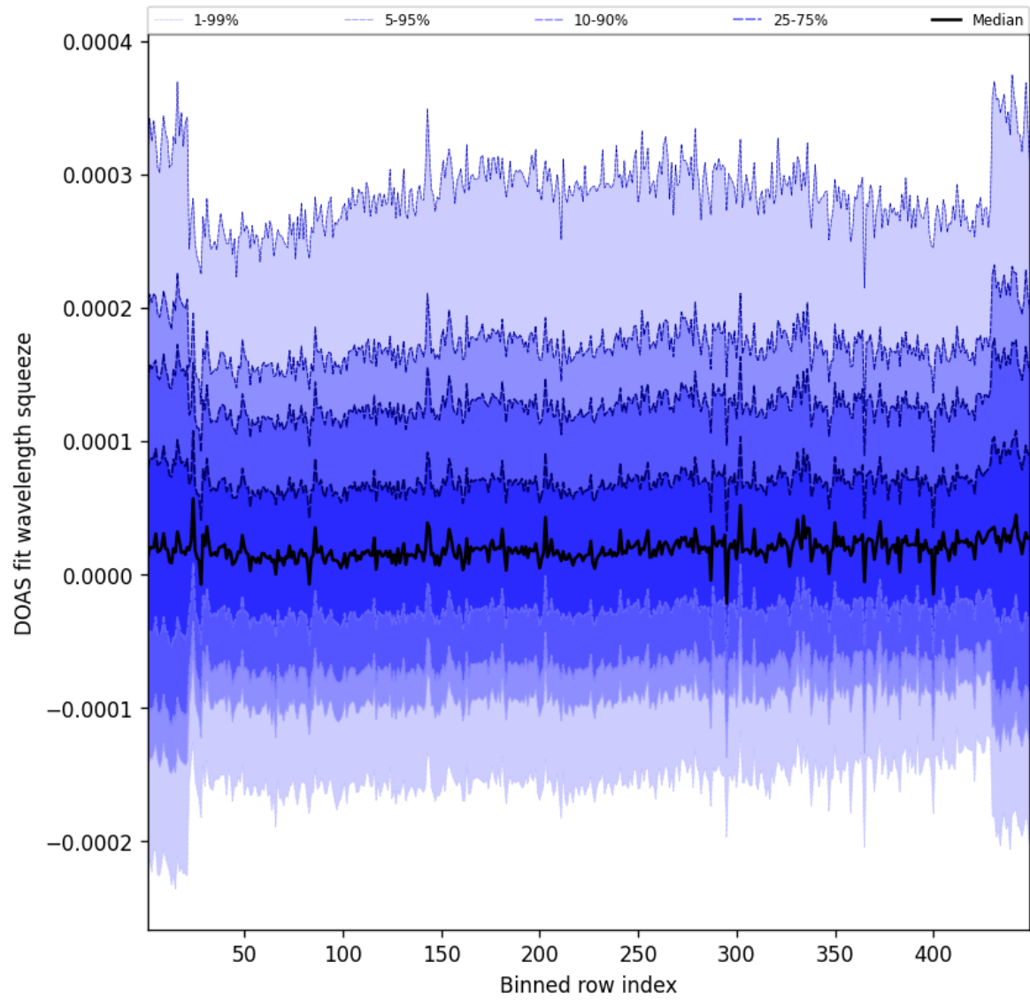
Figure 57: Along track statistics of “DOAS fit wavelength squeeze” for 2025-08-20 to 2025-08-21
