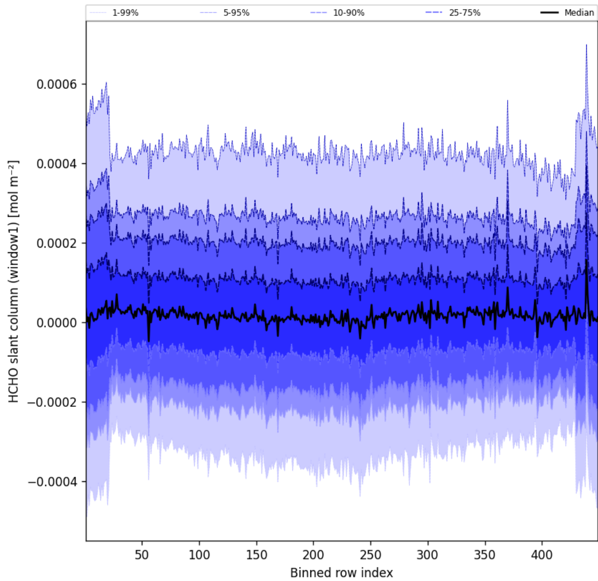
Figure 50: Along track statistics of “HCHO slant column (window1)” for 2025-08-20 to 2025-08-21
