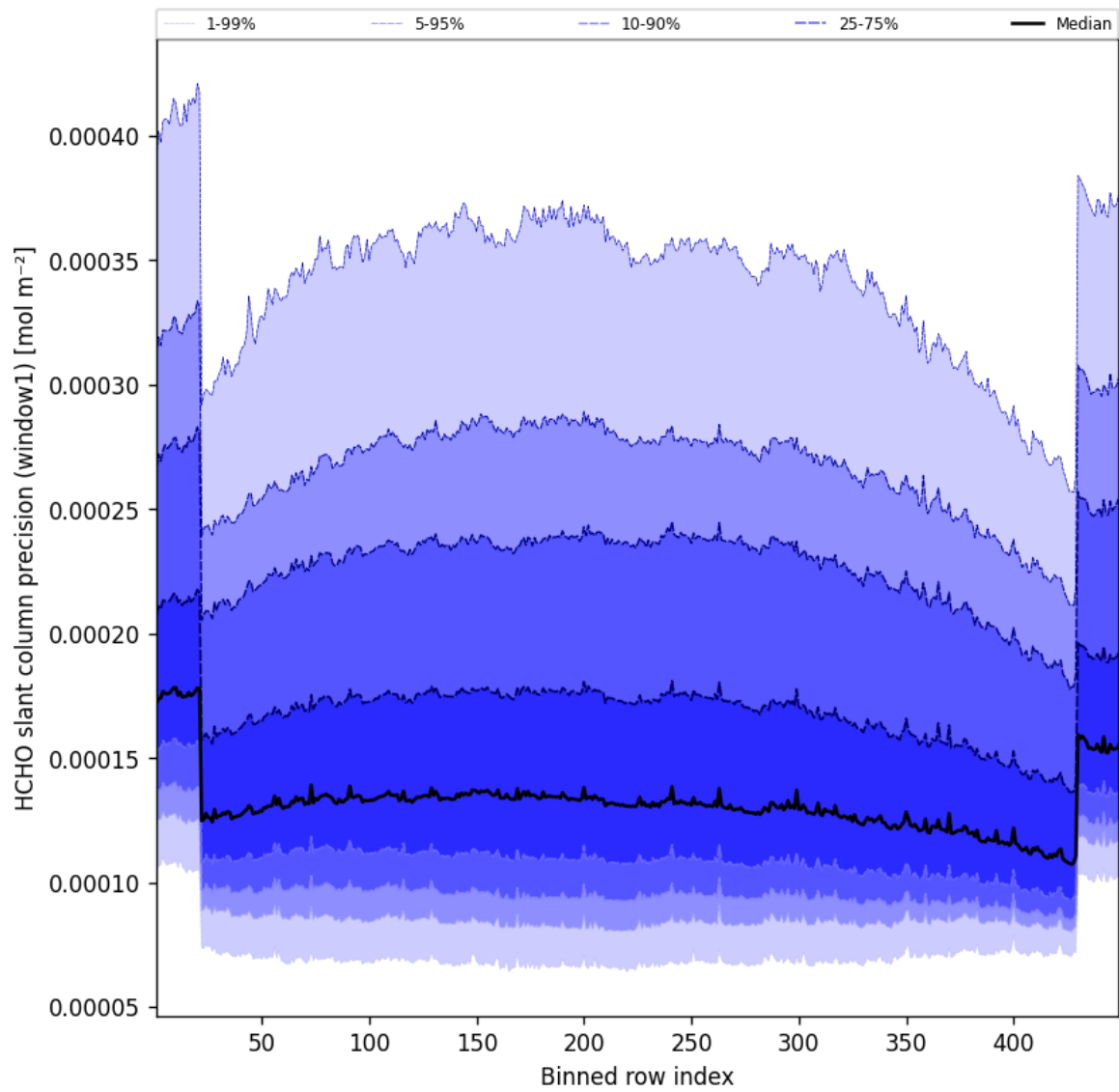
Figure 51: Along track statistics of “HCHO slant column precision (window1)” for 2025-08-20 to 2025-08-21
