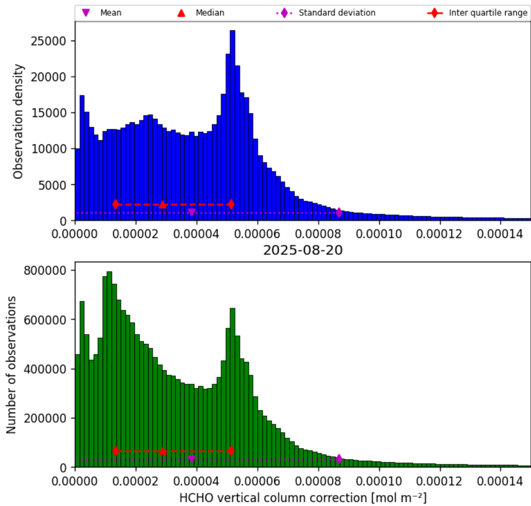
Figure 35: Histogram of “HCHO vertical column correction” for 2025-08-20 to 2025-08-21
