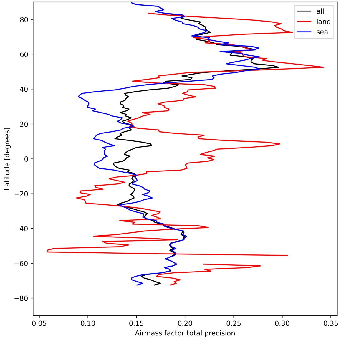
Figure 25: Zonal average of “Airmass factor total precision” for 2025-08-20 to 2025-08-21.
