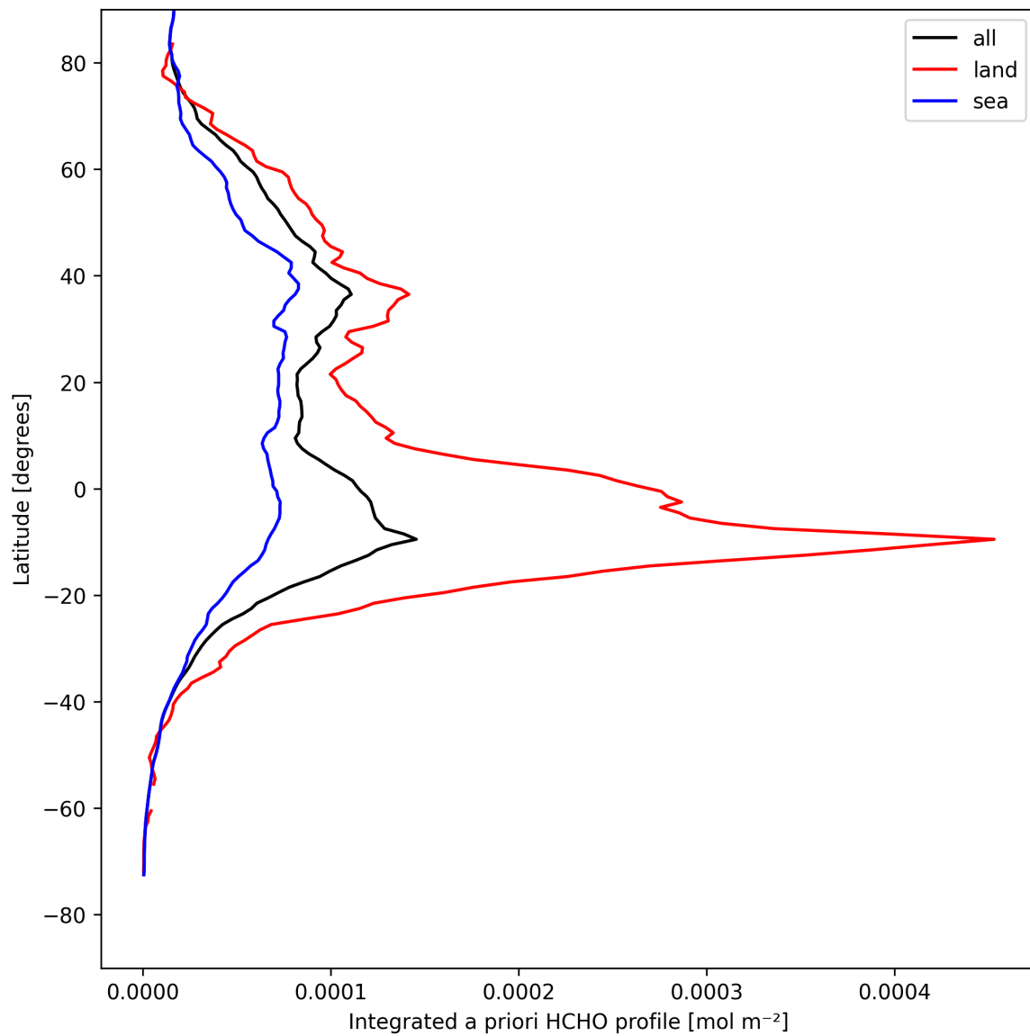
Figure 27: Zonal average of “Integrated a priori HCHO profile” for 2025-08-20 to 2025-08-21.
