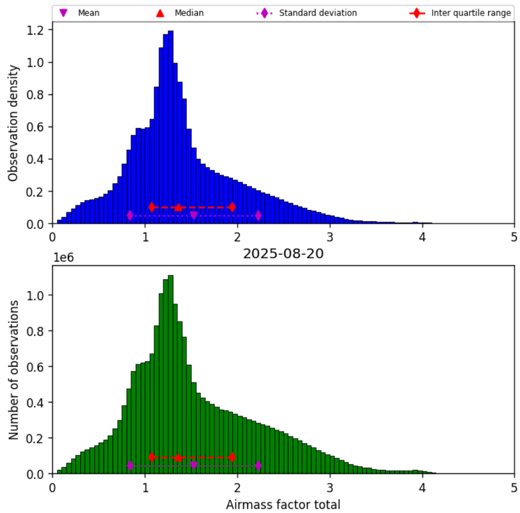
Figure 38: Histogram of “Airmass factor total” for 2025-08-20 to 2025-08-21
