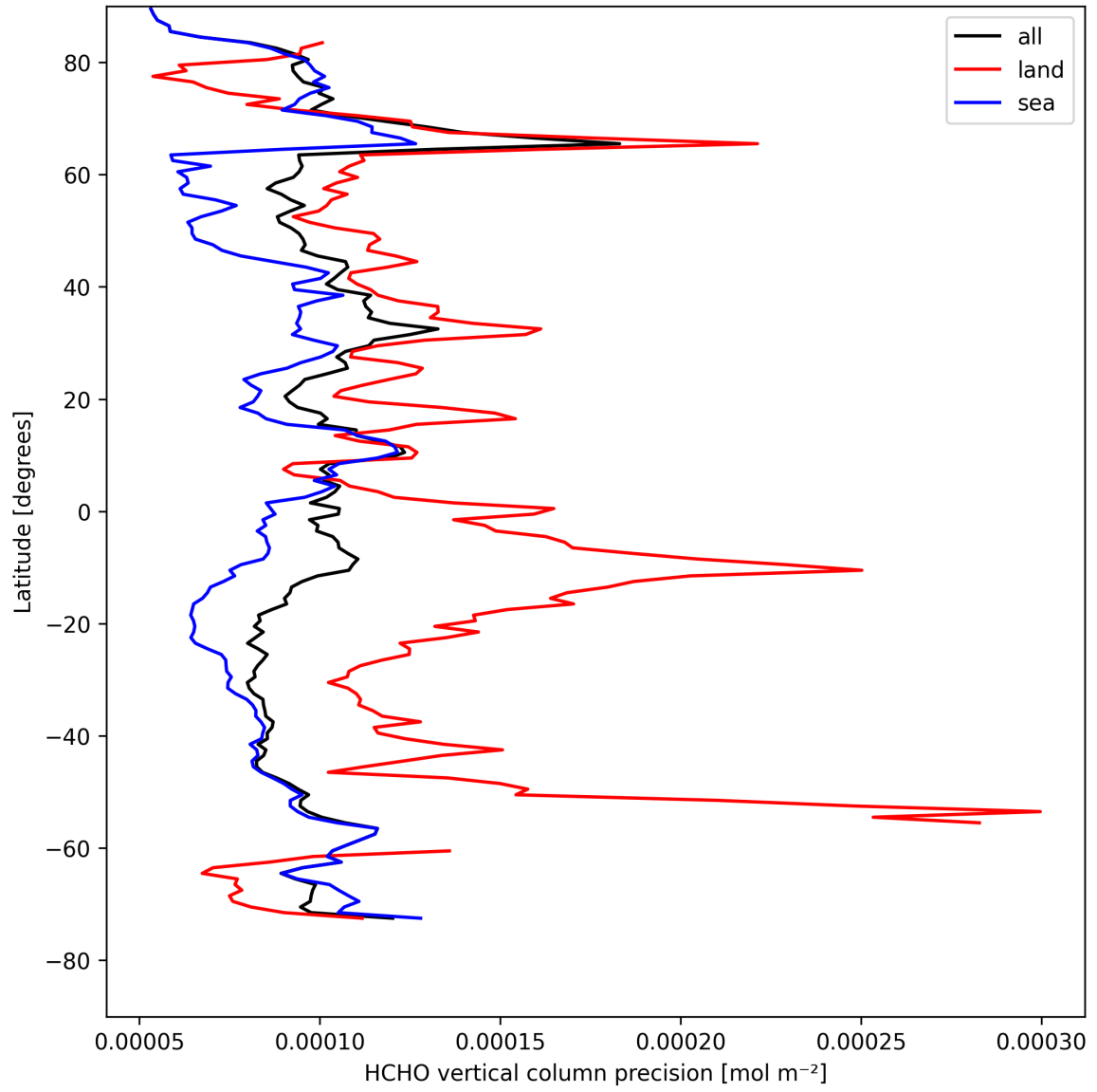
Figure 20: Zonal average of “HCHO vertical column precision” for 2025-08-20 to 2025-08-21.
