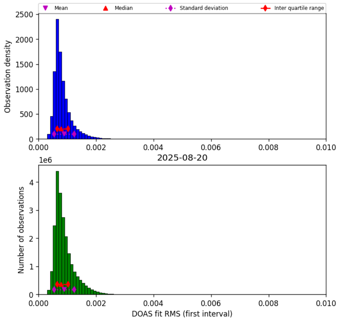
Figure 44: Histogram of “DOAS fit RMS (first interval)” for 2025-08-20 to 2025-08-21
