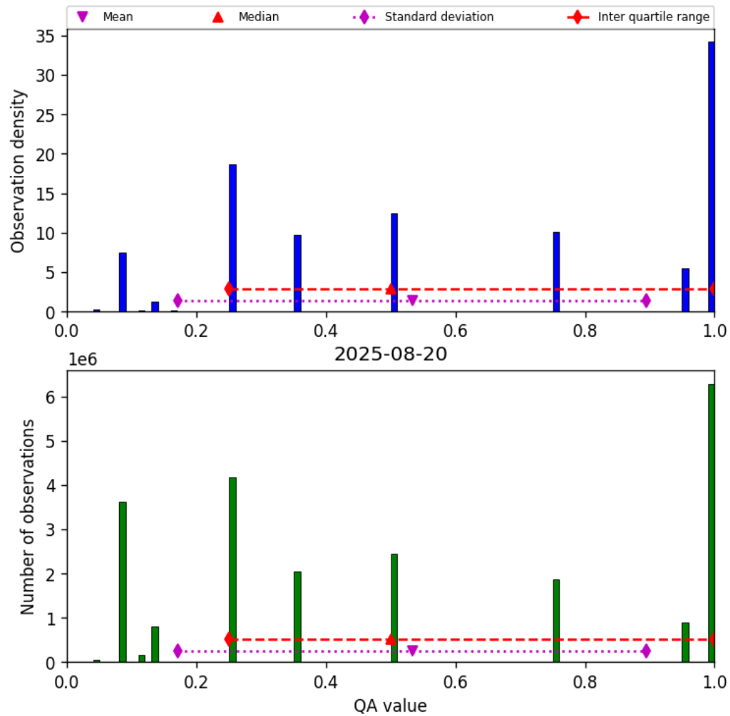
Figure 32: Histogram of “QA value” for 2025-08-20 to 2025-08-21
