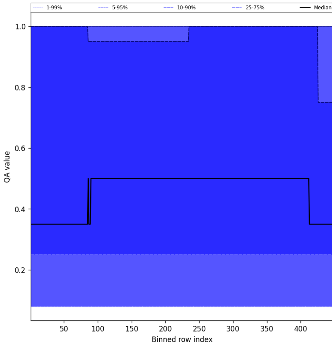
Figure 46: Along track statistics of “QA value” for 2025-08-20 to 2025-08-21
