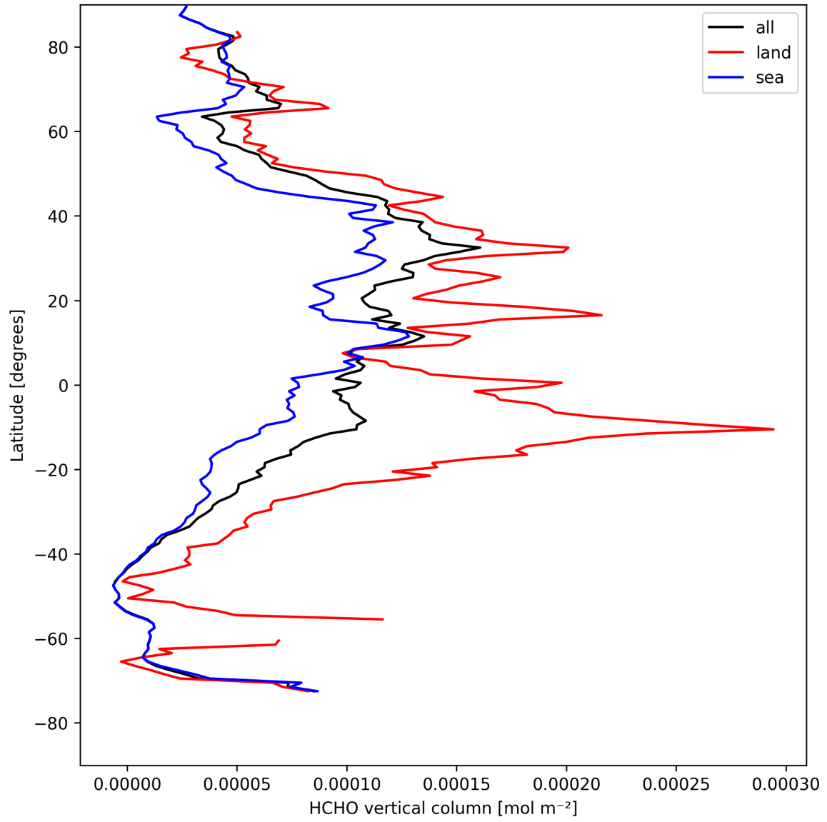
Figure 19: Zonal average of “HCHO vertical column” for 2025-08-20 to 2025-08-21.
