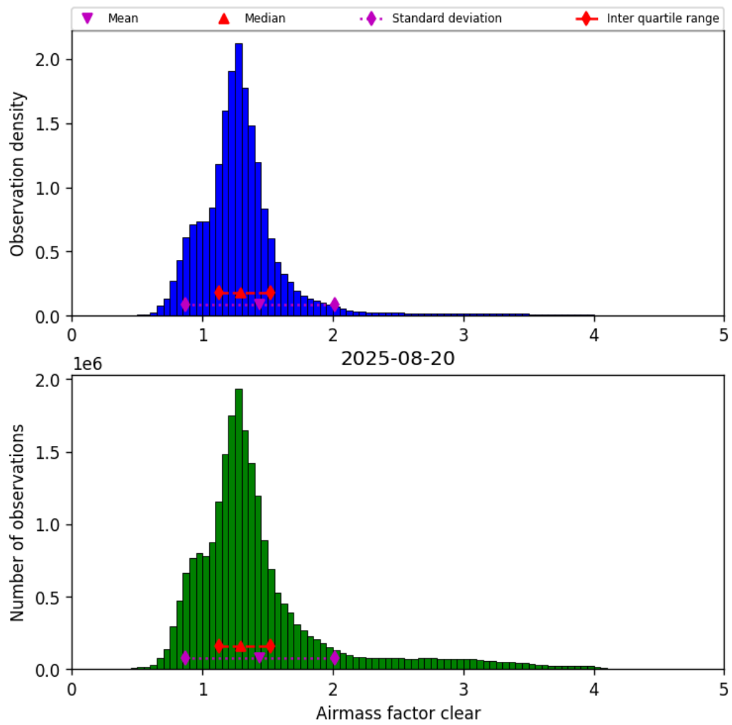
Figure 40: Histogram of “Airmass factor clear” for 2025-08-20 to 2025-08-21
