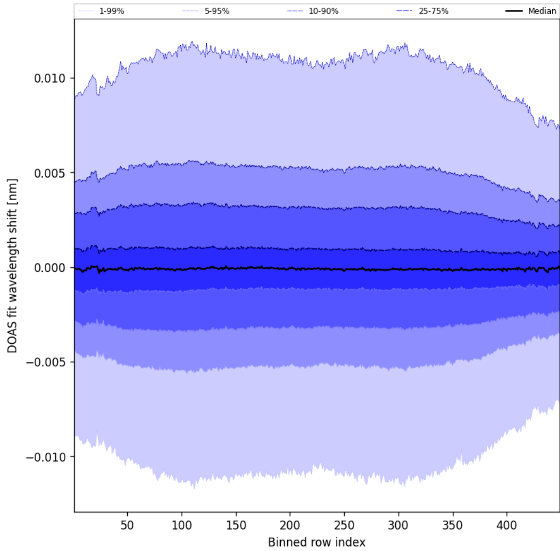
Figure 56: Along track statistics of “DOAS fit wavelength shift” for 2025-08-20 to 2025-08-21
