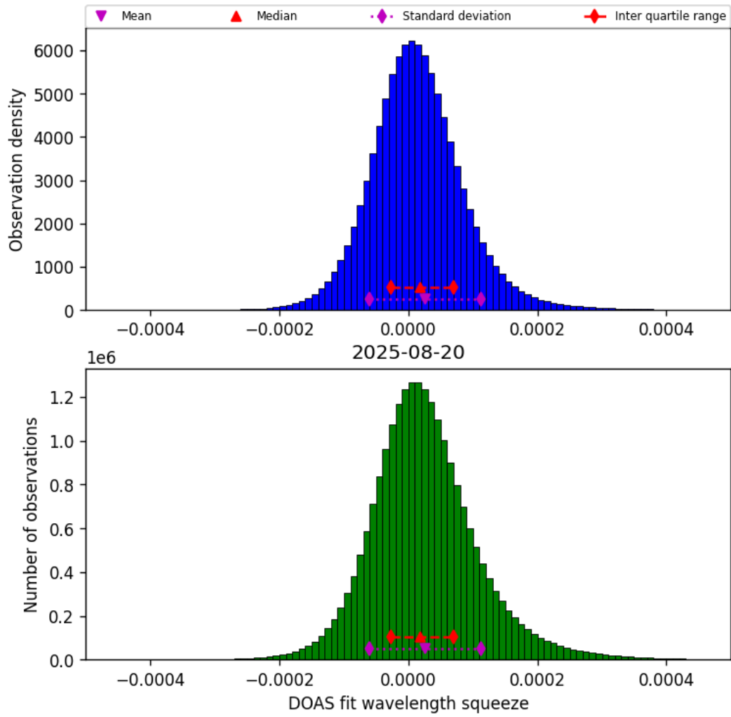
Figure 43: Histogram of “DOAS fit wavelength squeeze” for 2025-08-20 to 2025-08-21
