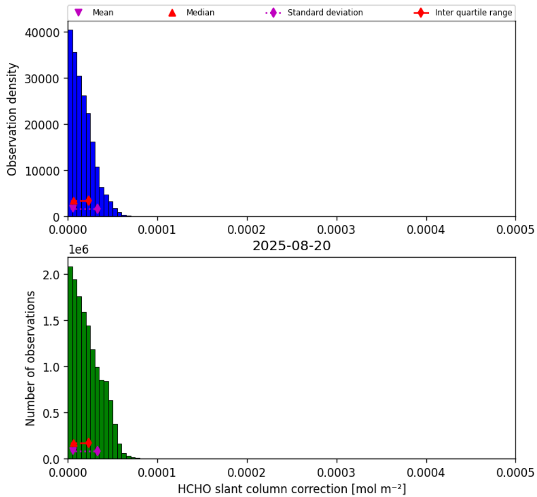
Figure 45: Histogram of “HCHO slant column correction” for 2025-08-20 to 2025-08-21
