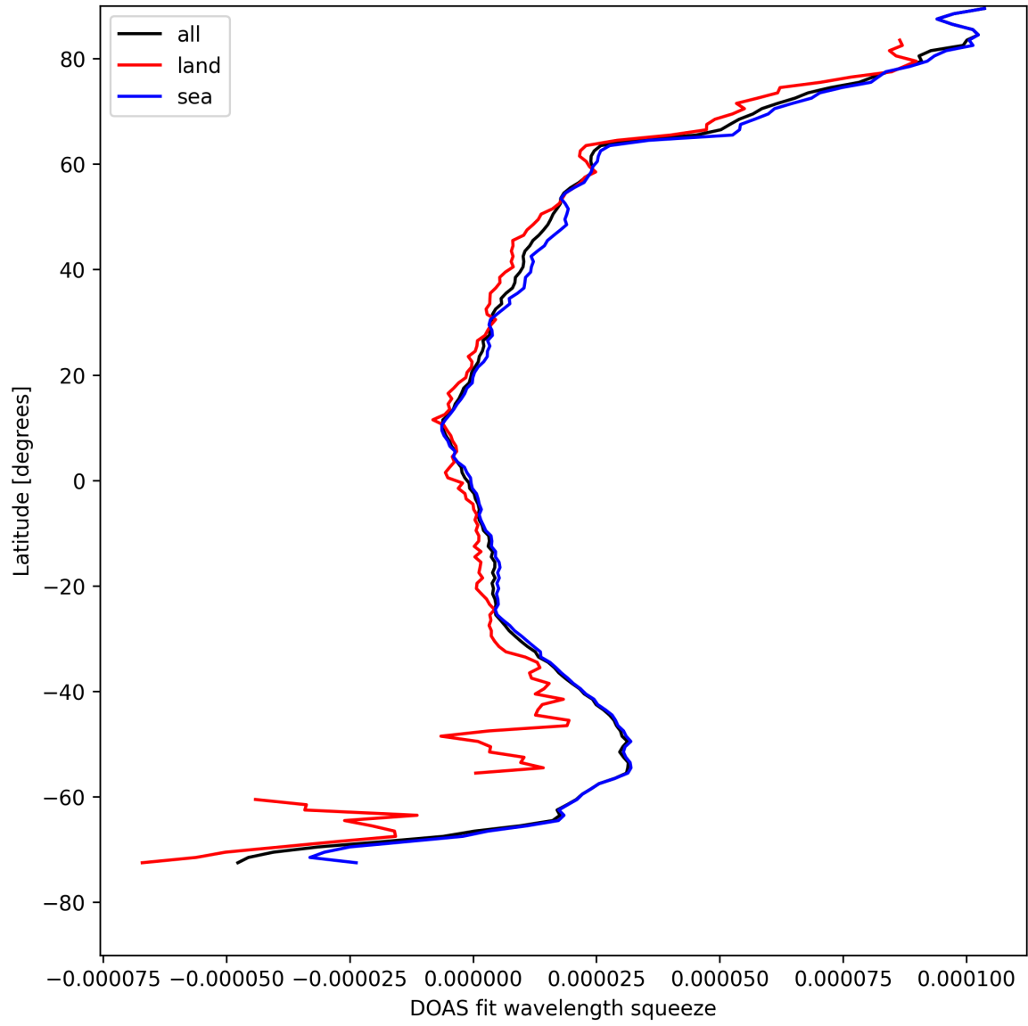
Figure 29: Zonal average of “DOAS fit wavelength squeeze” for 2025-08-20 to 2025-08-21.
