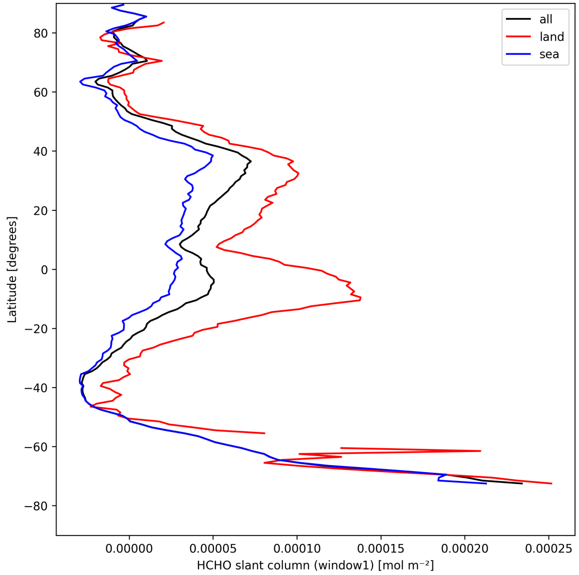
Figure 22: Zonal average of “HCHO slant column (window1)” for 2025-08-20 to 2025-08-21.
