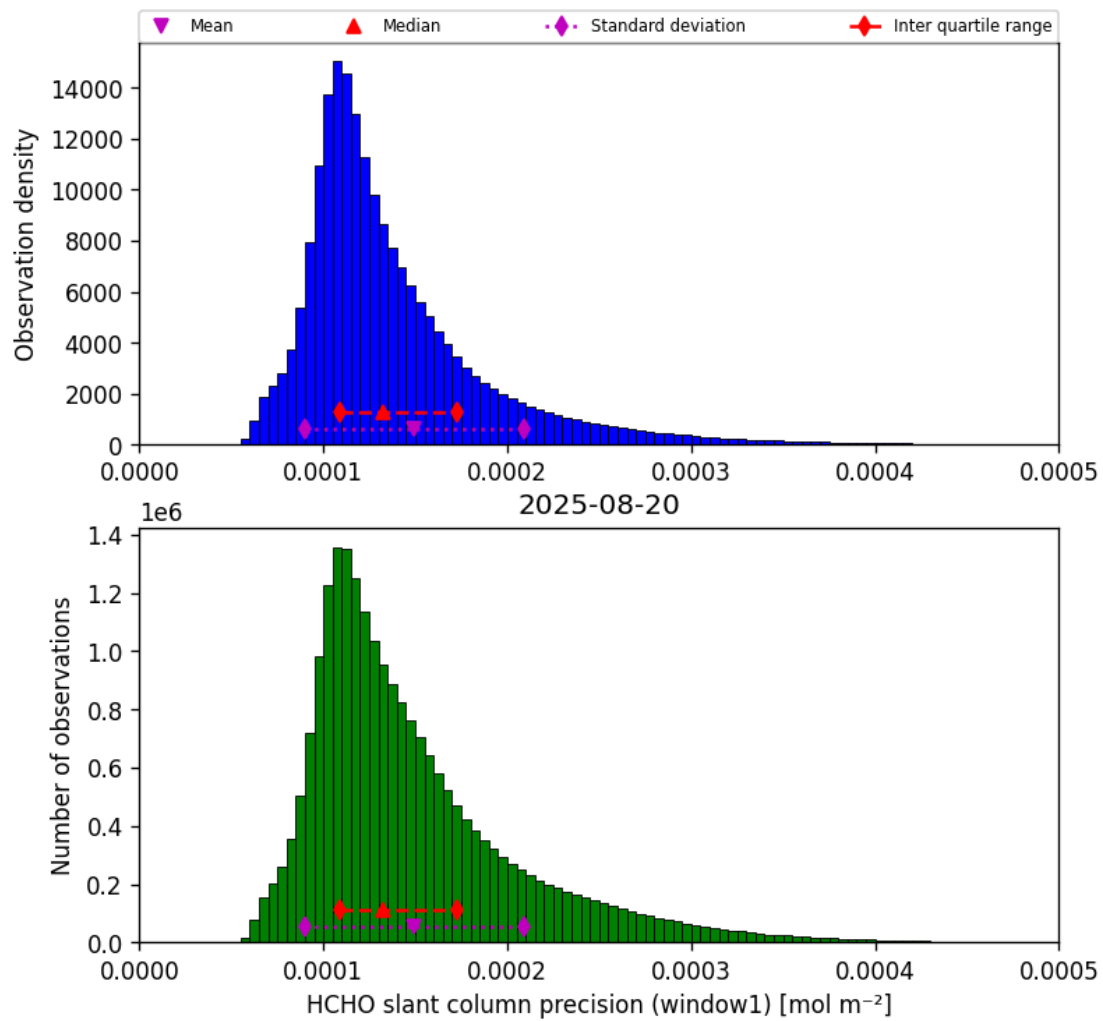
Figure 37: Histogram of “HCHO slant column precision (window1)” for 2025-08-20 to 2025-08-21
