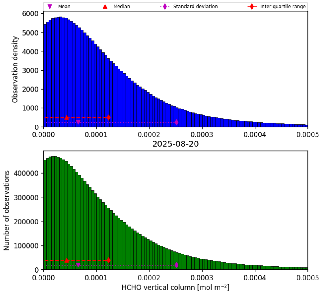
Figure 33: Histogram of “HCHO vertical column” for 2025-08-20 to 2025-08-21
