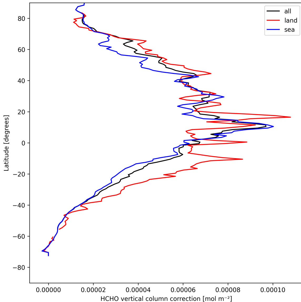
Figure 21: Zonal average of “HCHO vertical column correction” for 2025-08-20 to 2025-08-21.
