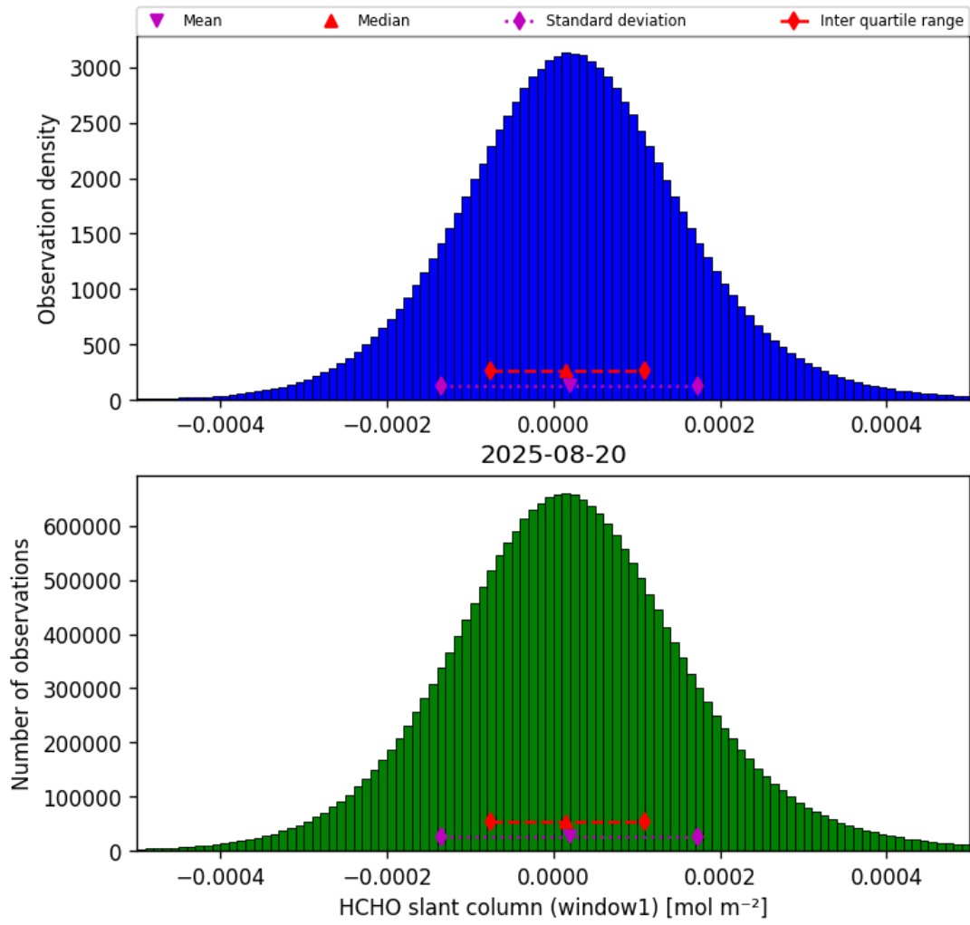
Figure 36: Histogram of “HCHO slant column (window1)” for 2025-08-20 to 2025-08-21
