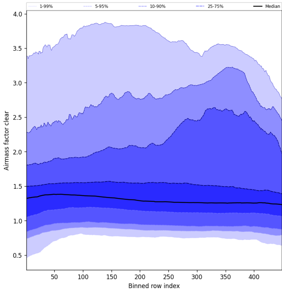
Figure 54: Along track statistics of “Airmass factor clear” for 2025-08-20 to 2025-08-21
