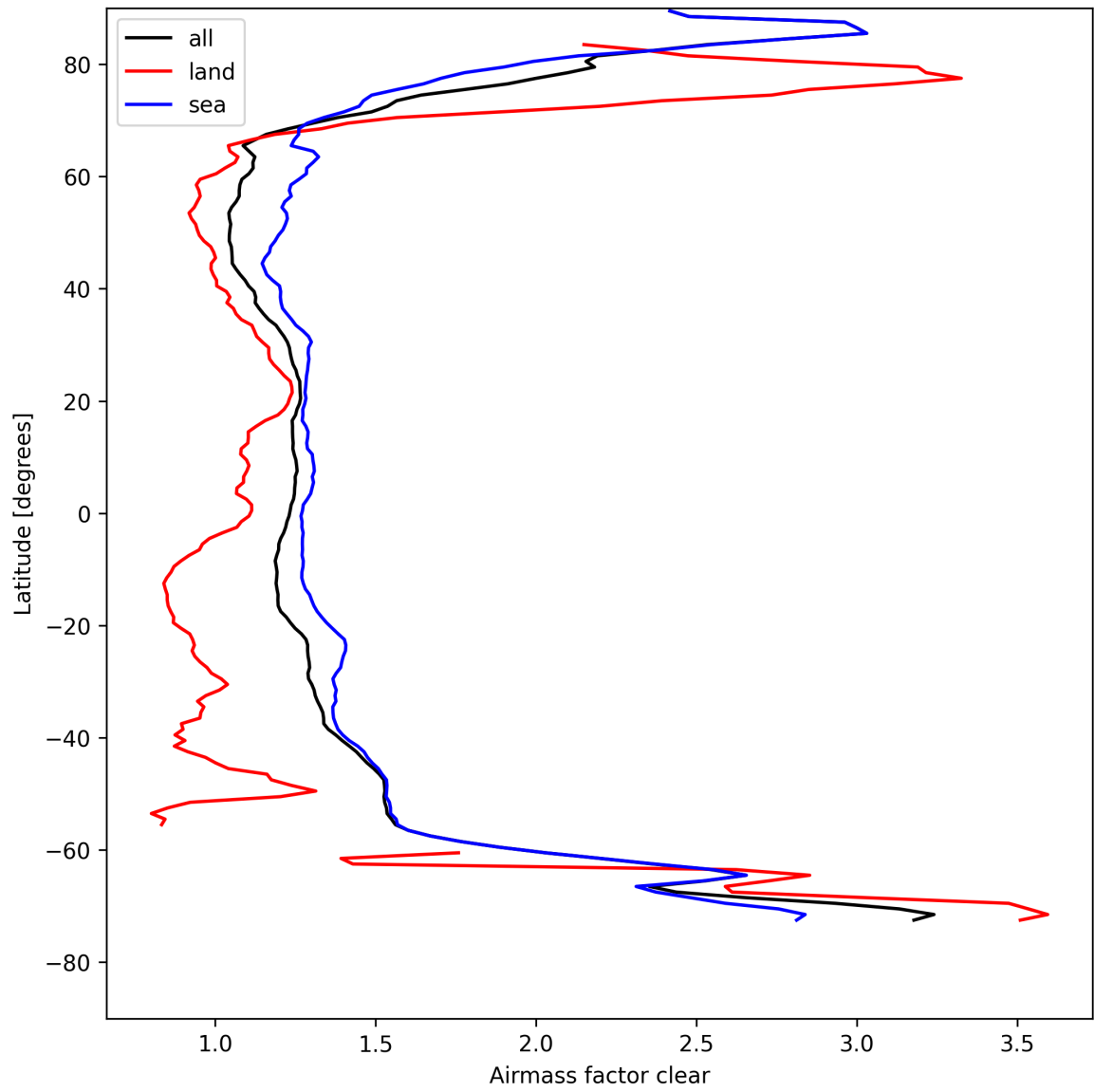
Figure 26: Zonal average of “Airmass factor clear” for 2025-08-20 to 2025-08-21.
