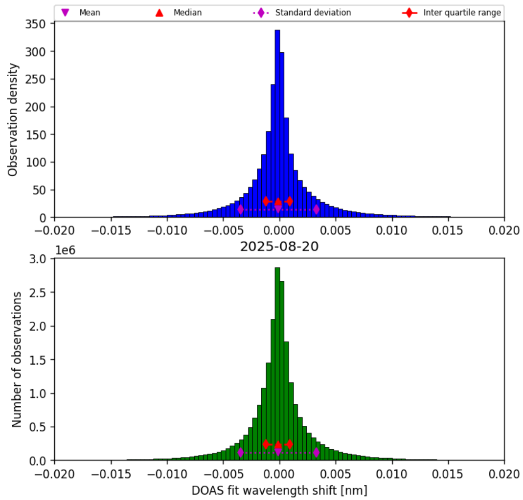
Figure 42: Histogram of “DOAS fit wavelength shift” for 2025-08-20 to 2025-08-21
