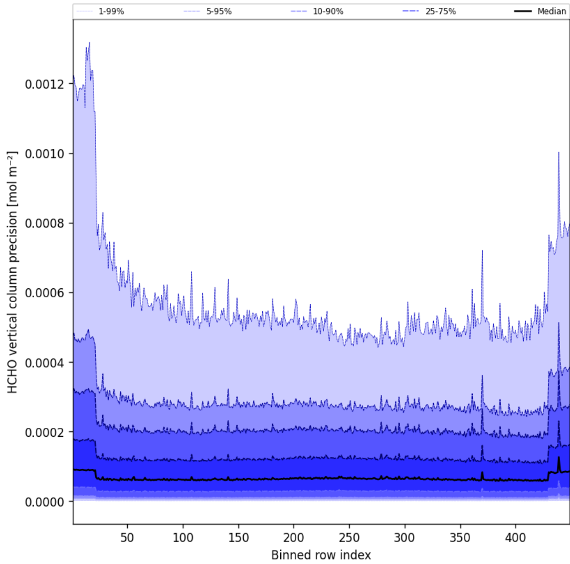
Figure 48: Along track statistics of “HCHO vertical column precision” for 2025-08-20 to 2025-08-21
