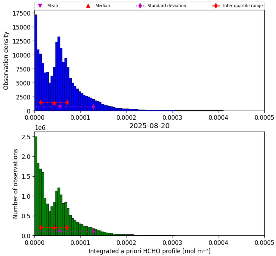
Figure 41: Histogram of “Integrated a priori HCHO profile” for 2025-08-20 to 2025-08-21
