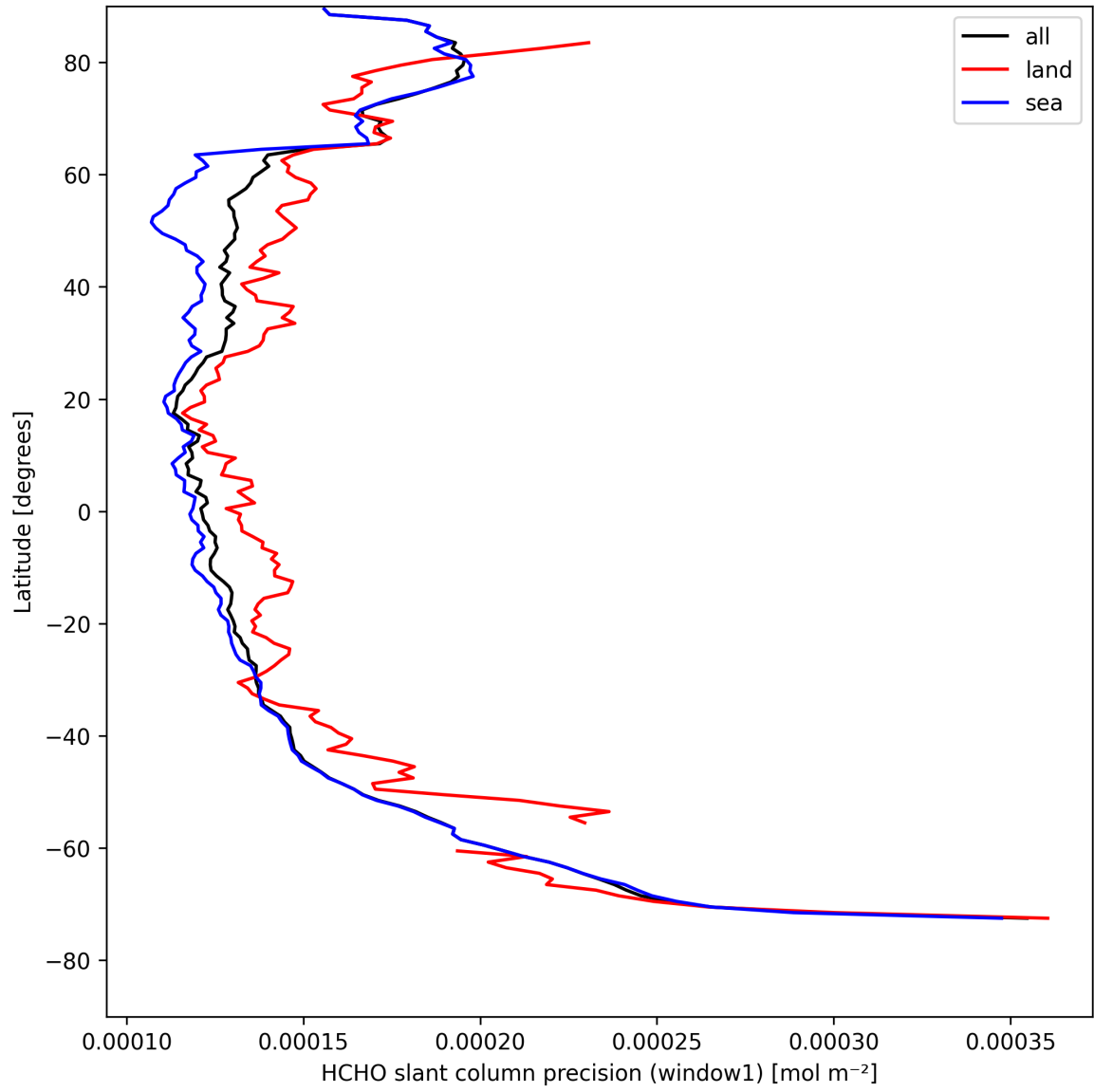
Figure 23: Zonal average of “HCHO slant column precision (window1)” for 2025-08-20 to 2025-08-21.
