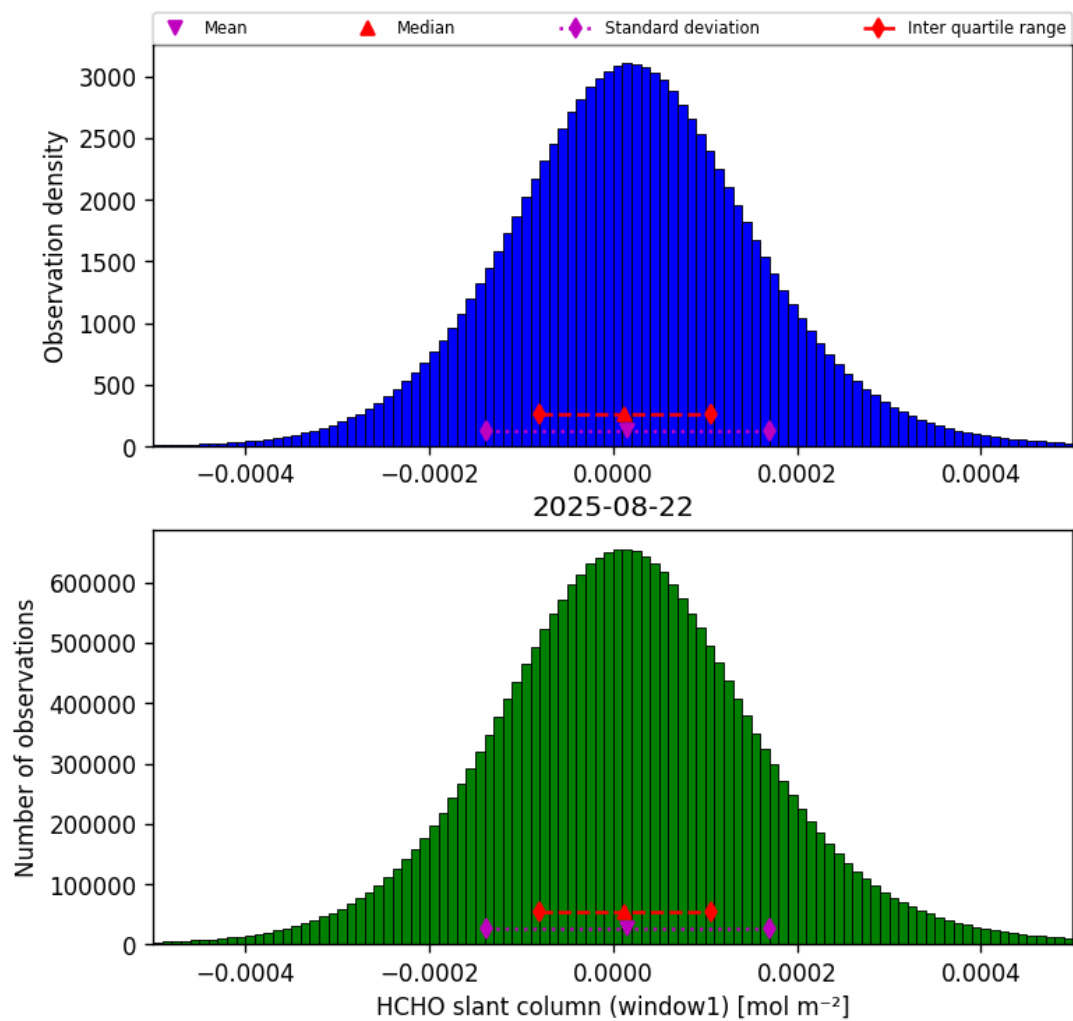
Figure 36: Histogram of “HCHO slant column (window1)” for 2025-08-22 to 2025-08-23
