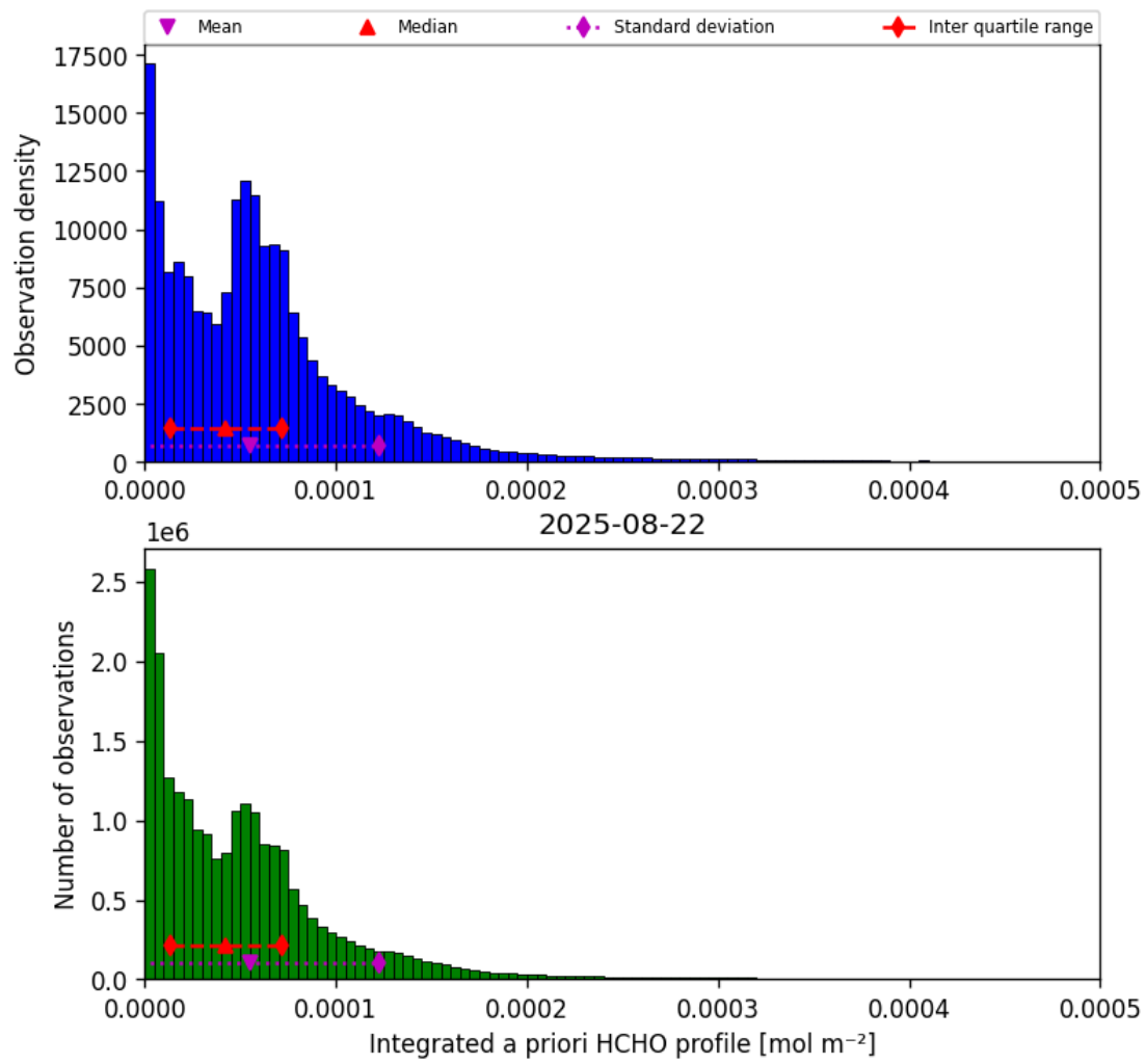
Figure 41: Histogram of “Integrated a priori HCHO profile” for 2025-08-22 to 2025-08-23
