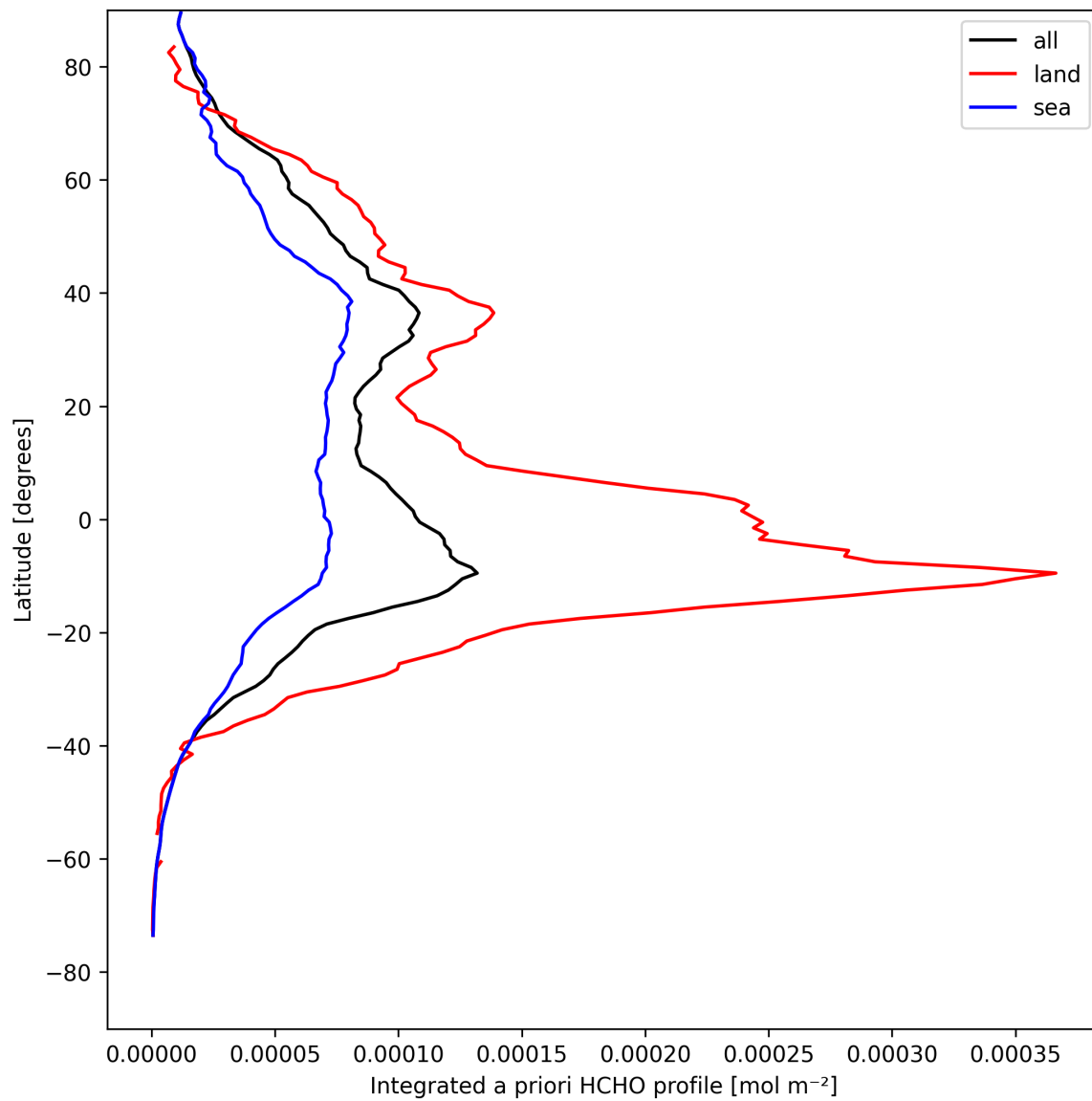
Figure 27: Zonal average of “Integrated a priori HCHO profile” for 2025-08-22 to 2025-08-23.
