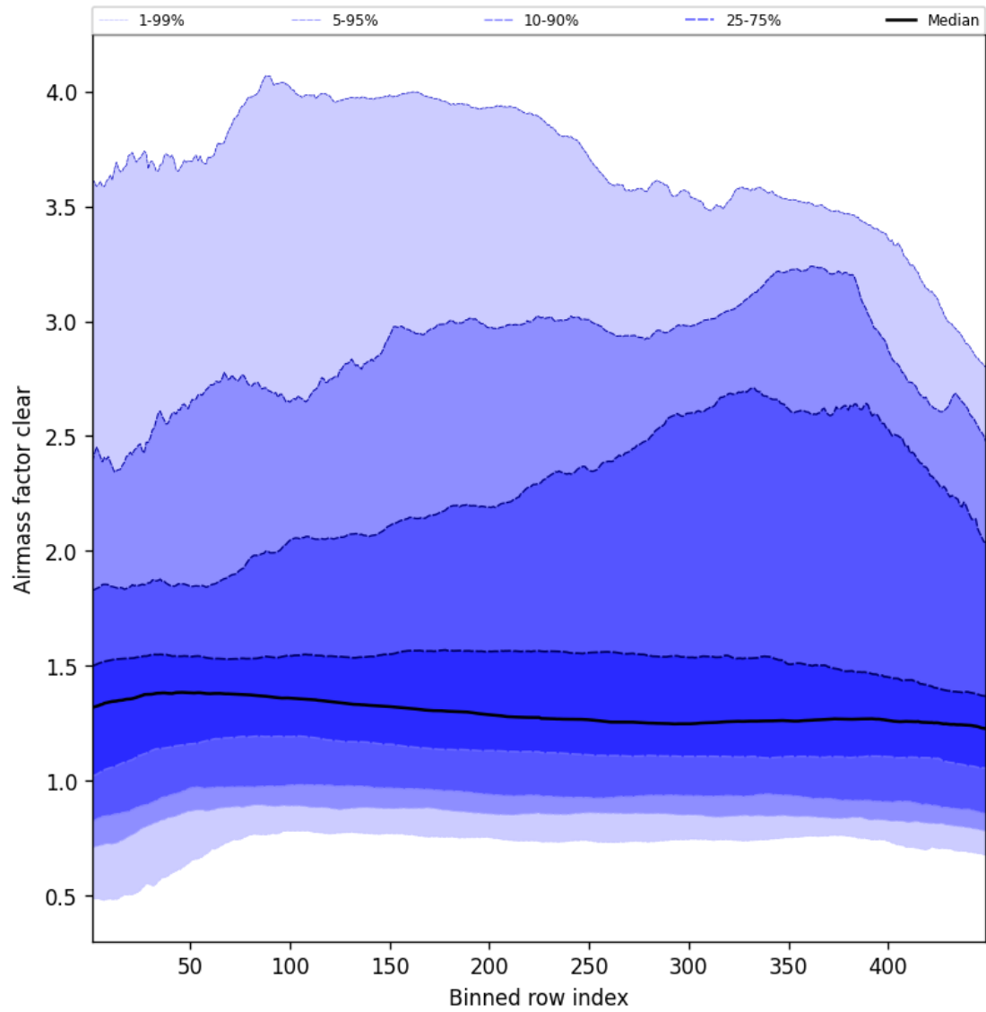
Figure 54: Along track statistics of “Airmass factor clear” for 2025-08-22 to 2025-08-23
