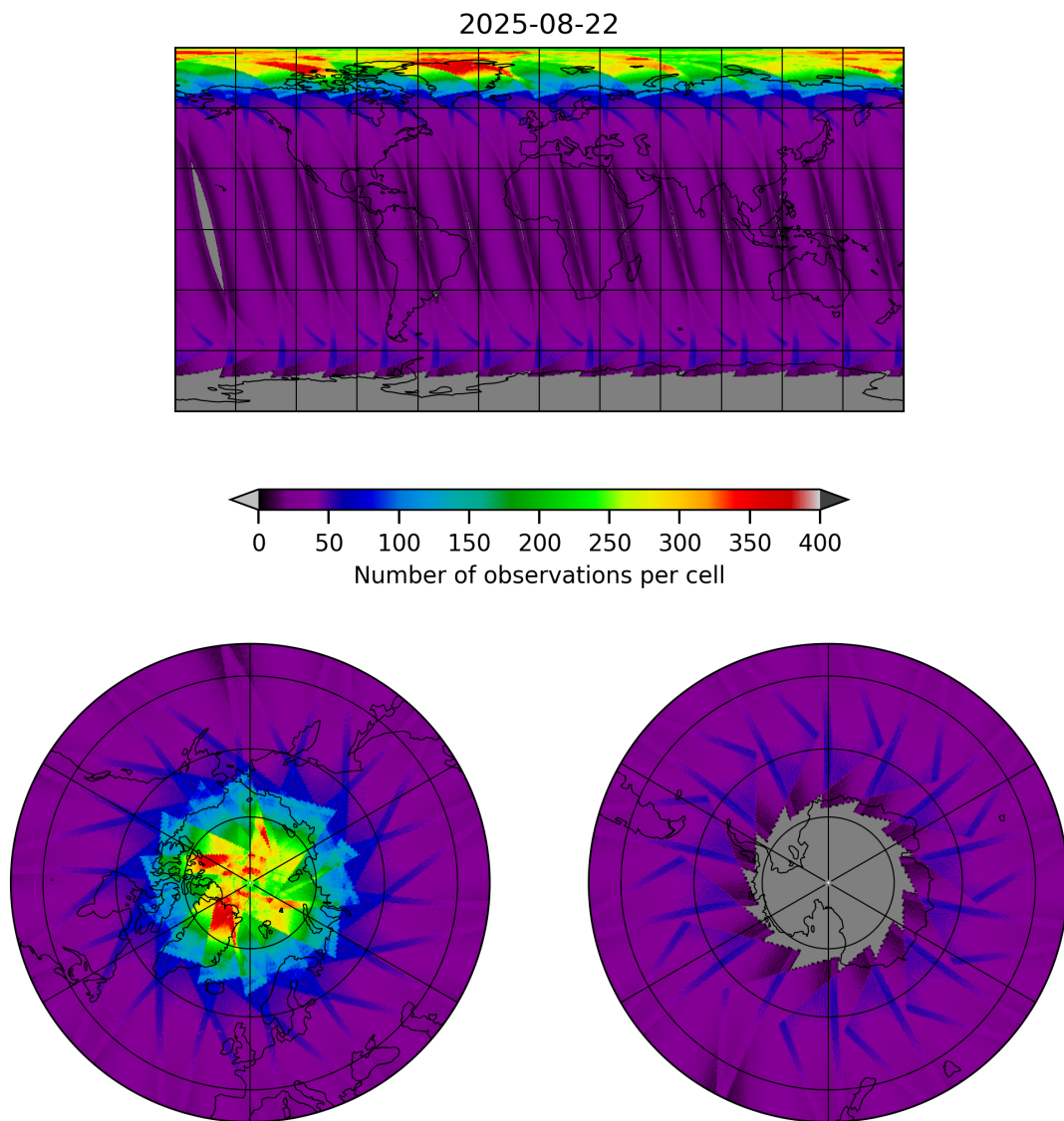
Figure 17: Map of the number of observations for 2025-08-22 to 2025-08-23
