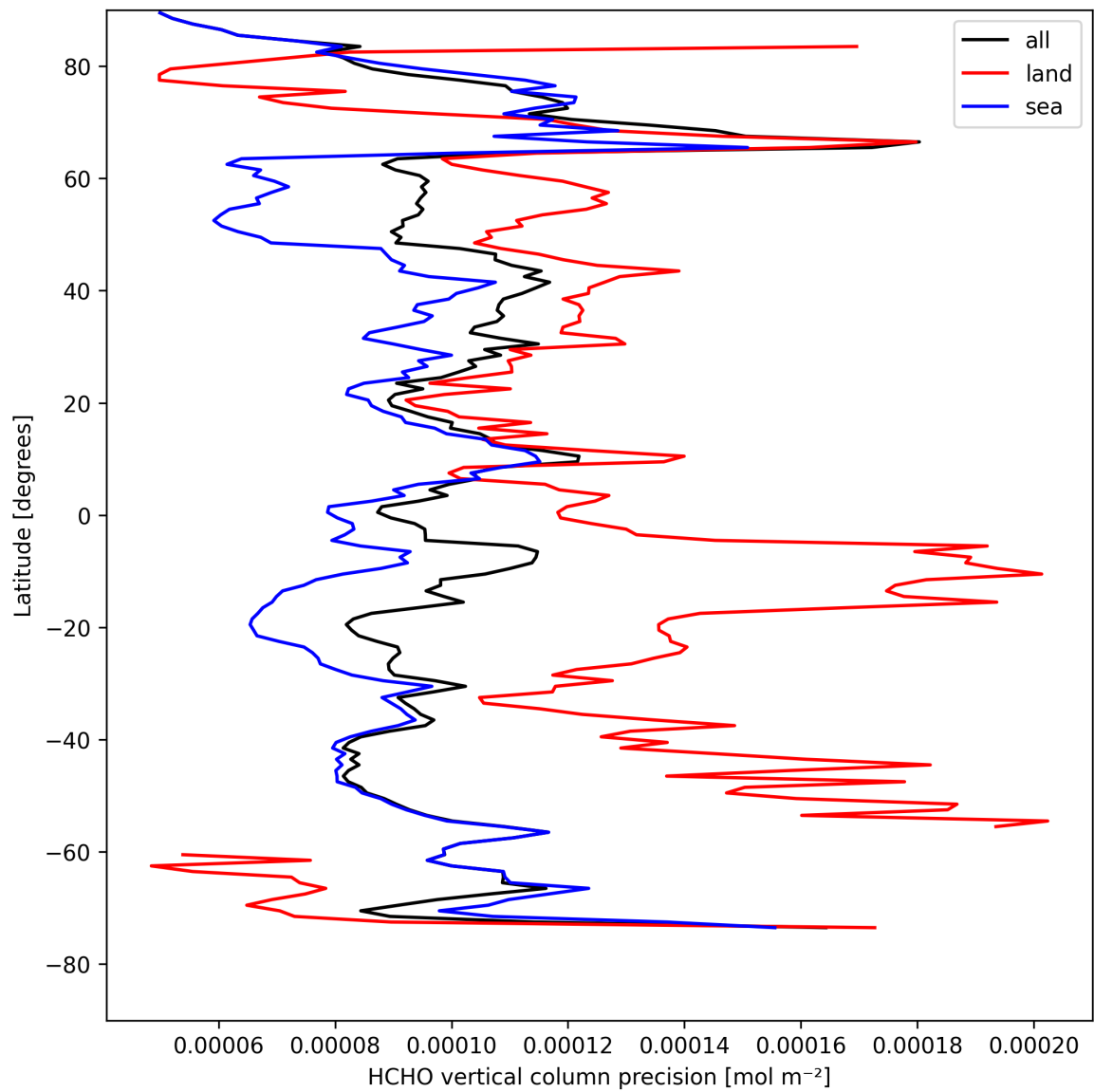
Figure 20: Zonal average of “HCHO vertical column precision” for 2025-08-22 to 2025-08-23.
