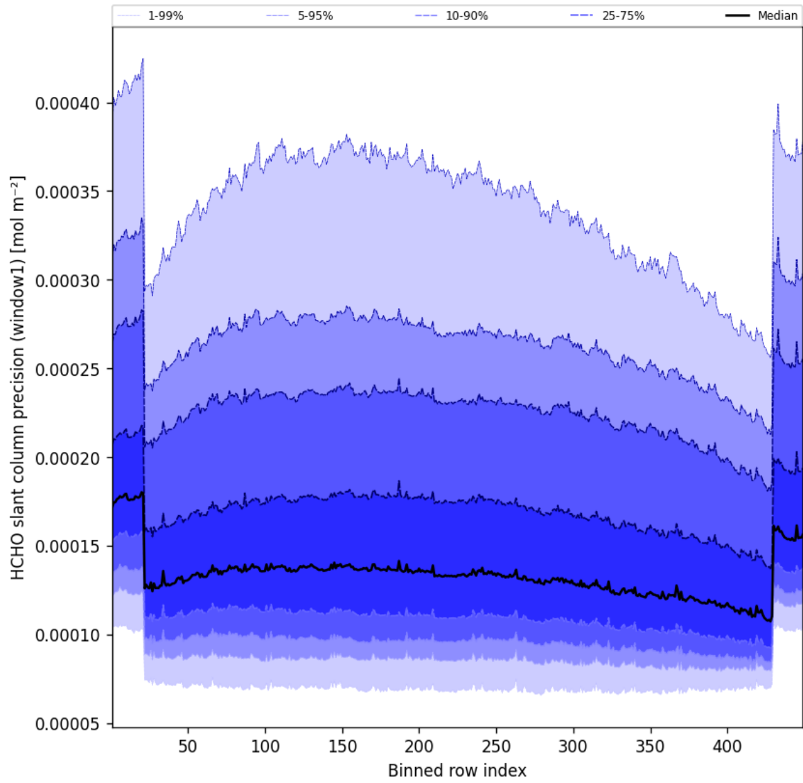
Figure 51: Along track statistics of “HCHO slant column precision (window1)” for 2025-08-22 to 2025-08-23
