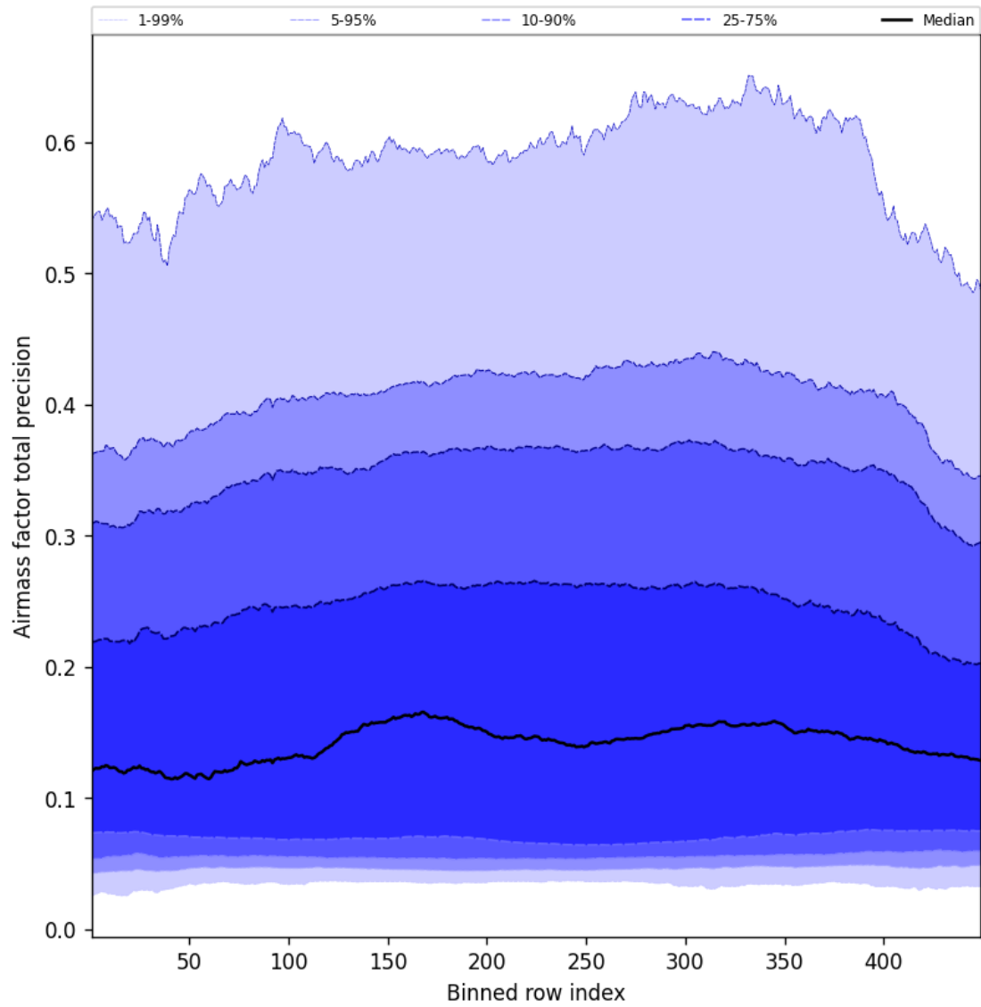
Figure 53: Along track statistics of “Airmass factor total precision” for 2025-08-22 to 2025-08-23
