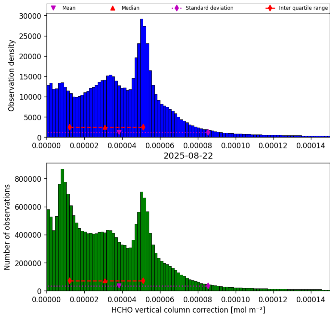
Figure 35: Histogram of “HCHO vertical column correction” for 2025-08-22 to 2025-08-23
