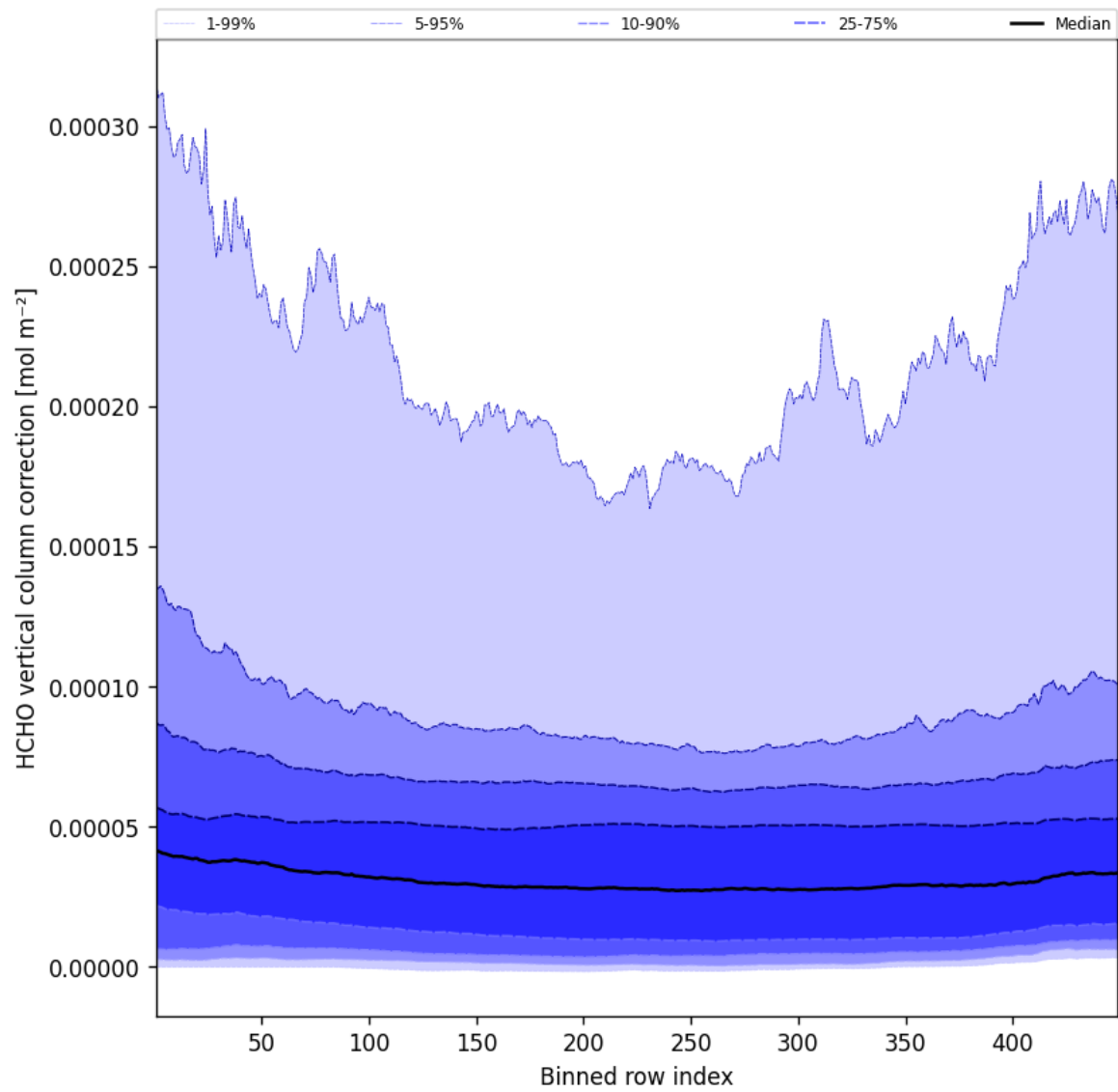
Figure 49: Along track statistics of “HCHO vertical column correction” for 2025-08-22 to 2025-08-23
