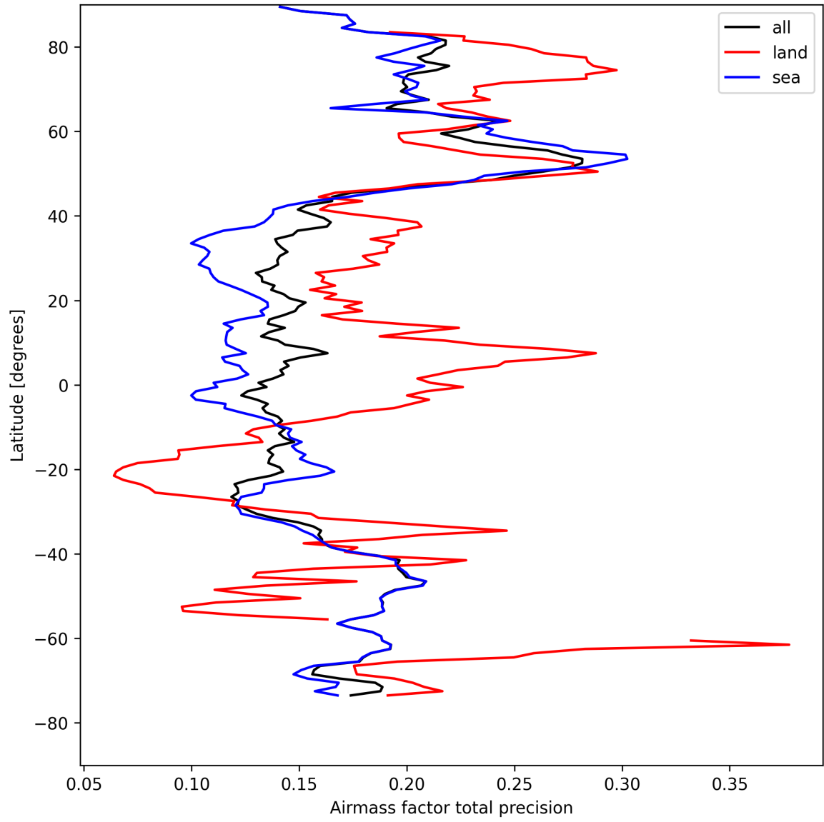
Figure 25: Zonal average of “Airmass factor total precision” for 2025-08-22 to 2025-08-23.
