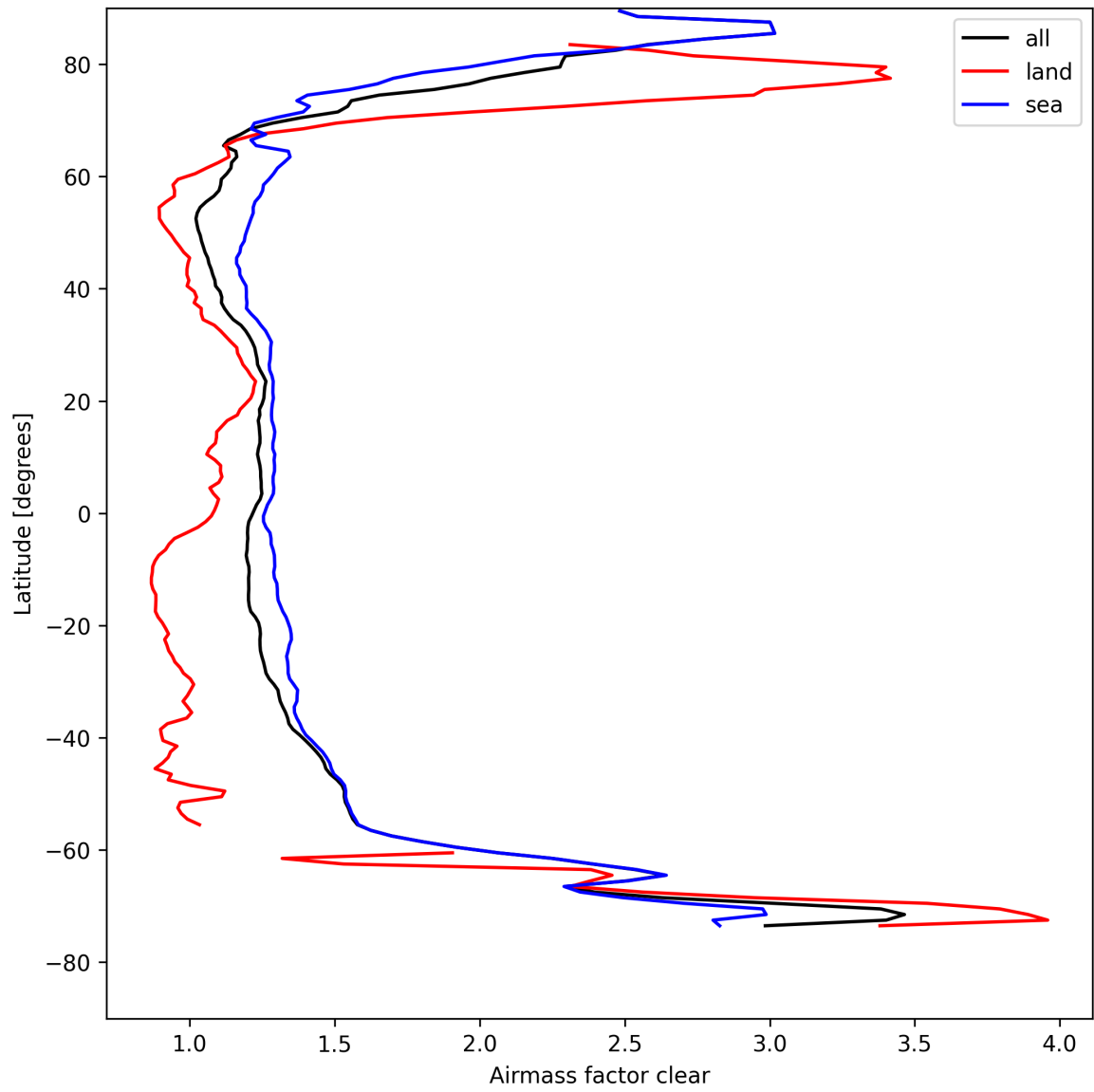
Figure 26: Zonal average of “Airmass factor clear” for 2025-08-22 to 2025-08-23.
