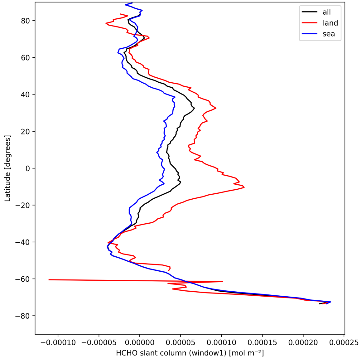
Figure 22: Zonal average of “HCHO slant column (window1)” for 2025-08-22 to 2025-08-23.
