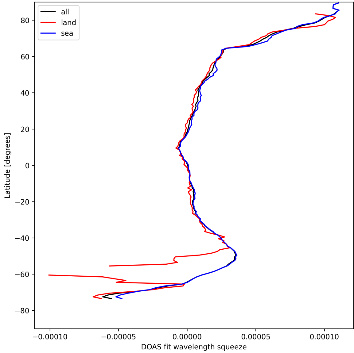
Figure 29: Zonal average of “DOAS fit wavelength squeeze” for 2025-08-22 to 2025-08-23.
