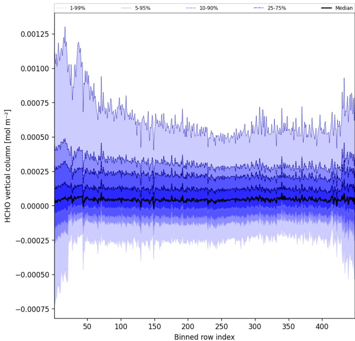
Figure 47: Along track statistics of “HCHO vertical column” for 2025-08-22 to 2025-08-23
