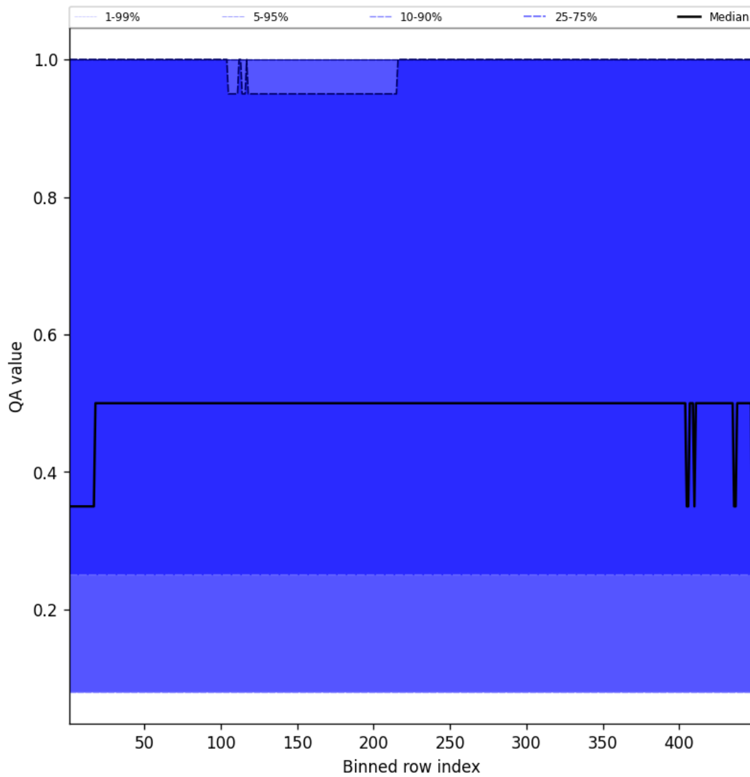
Figure 46: Along track statistics of “QA value” for 2025-08-22 to 2025-08-23
