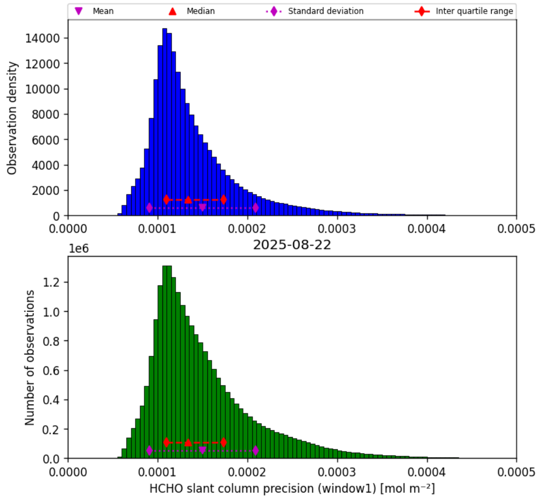
Figure 37: Histogram of “HCHO slant column precision (window1)” for 2025-08-22 to 2025-08-23
