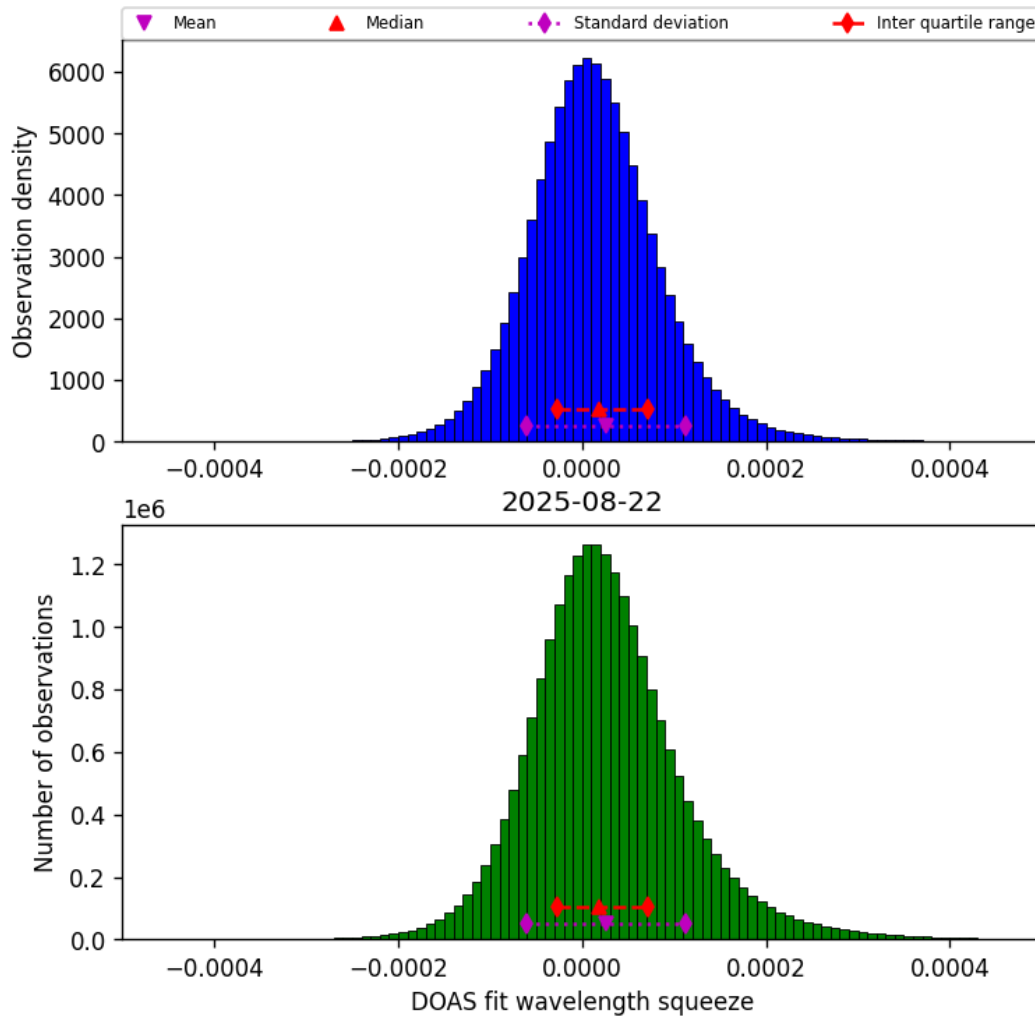
Figure 43: Histogram of “DOAS fit wavelength squeeze” for 2025-08-22 to 2025-08-23
