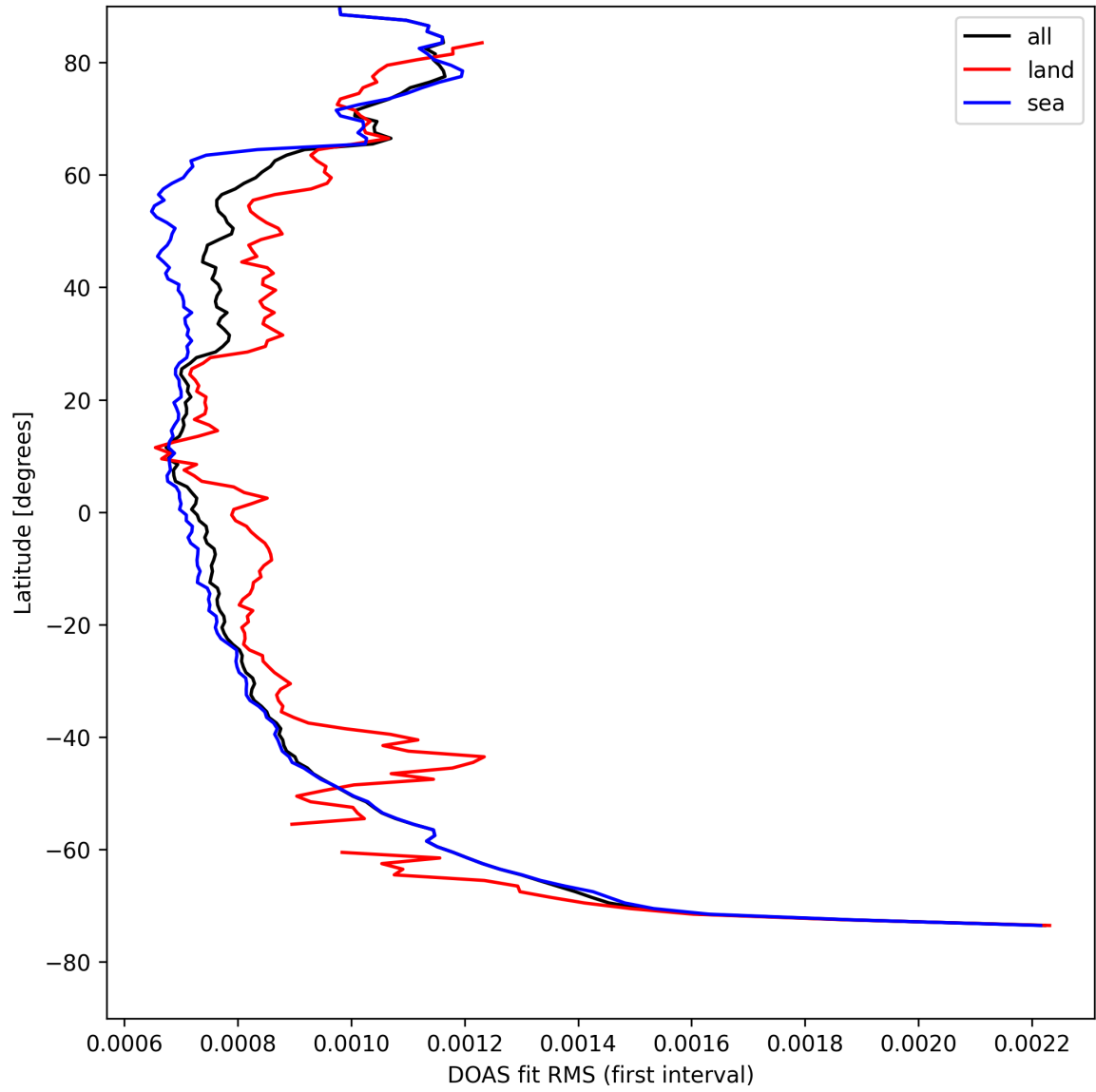
Figure 30: Zonal average of “DOAS fit RMS (first interval)” for 2025-08-22 to 2025-08-23.
