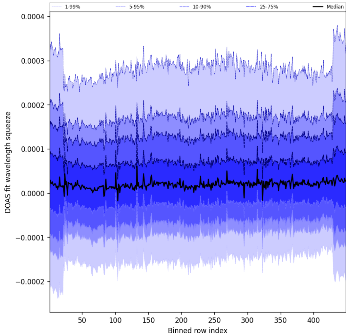
Figure 57: Along track statistics of “DOAS fit wavelength squeeze” for 2025-08-22 to 2025-08-23
