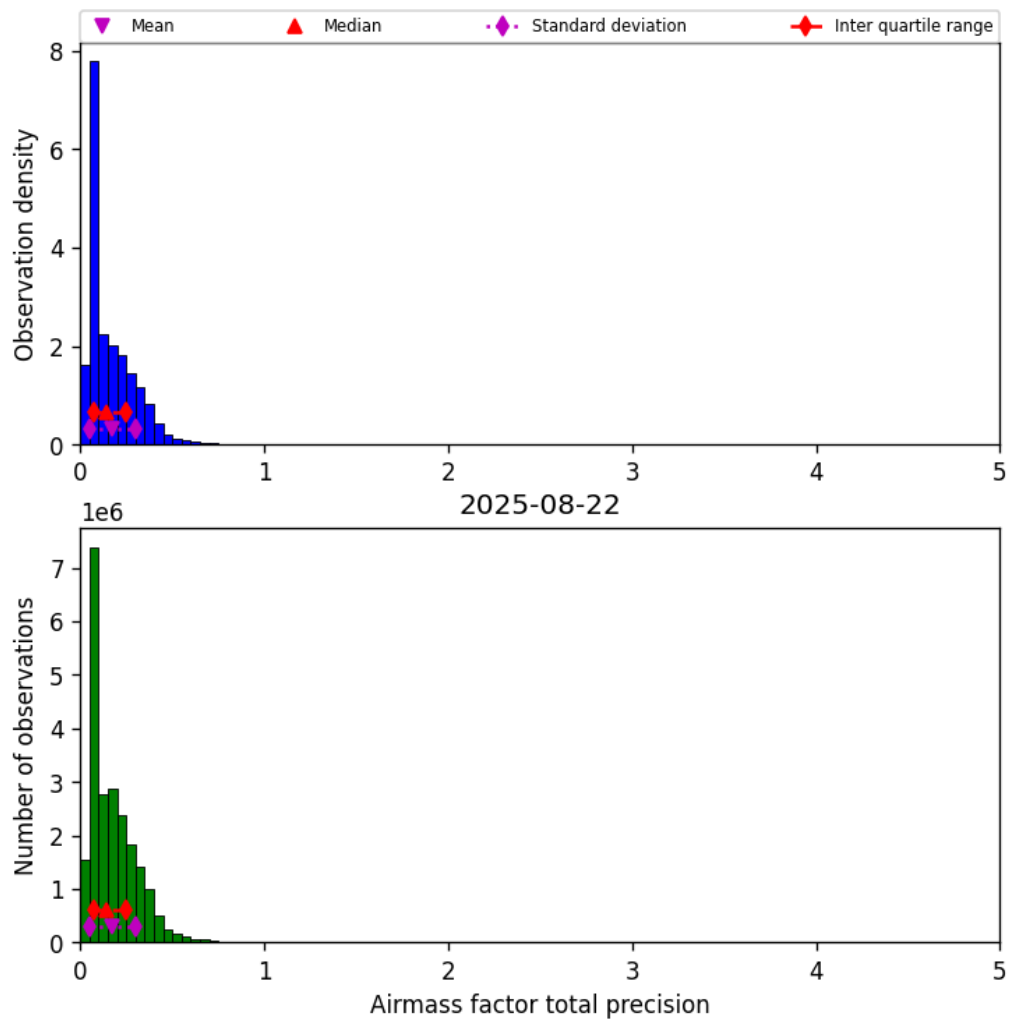
Figure 39: Histogram of “Airmass factor total precision” for 2025-08-22 to 2025-08-23
