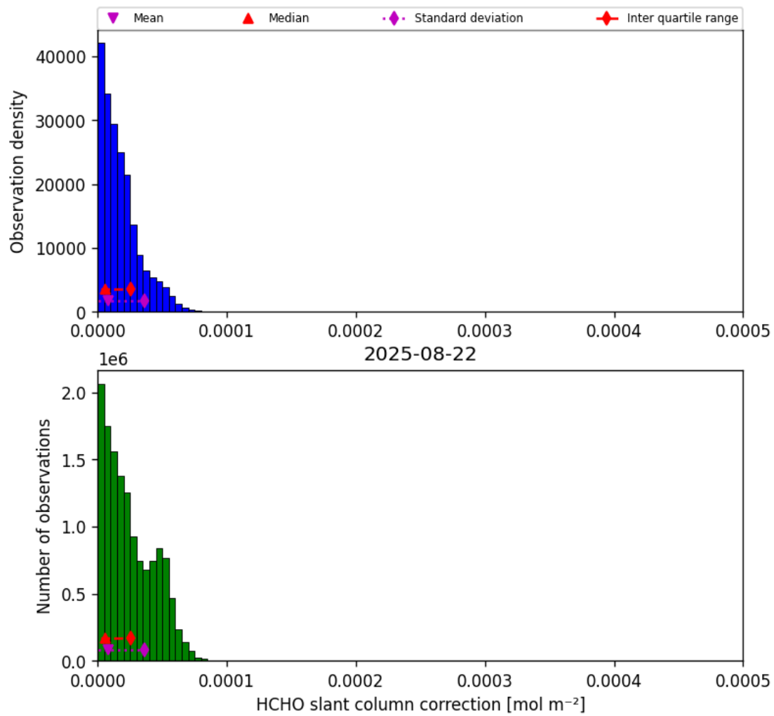
Figure 45: Histogram of “HCHO slant column correction” for 2025-08-22 to 2025-08-23
