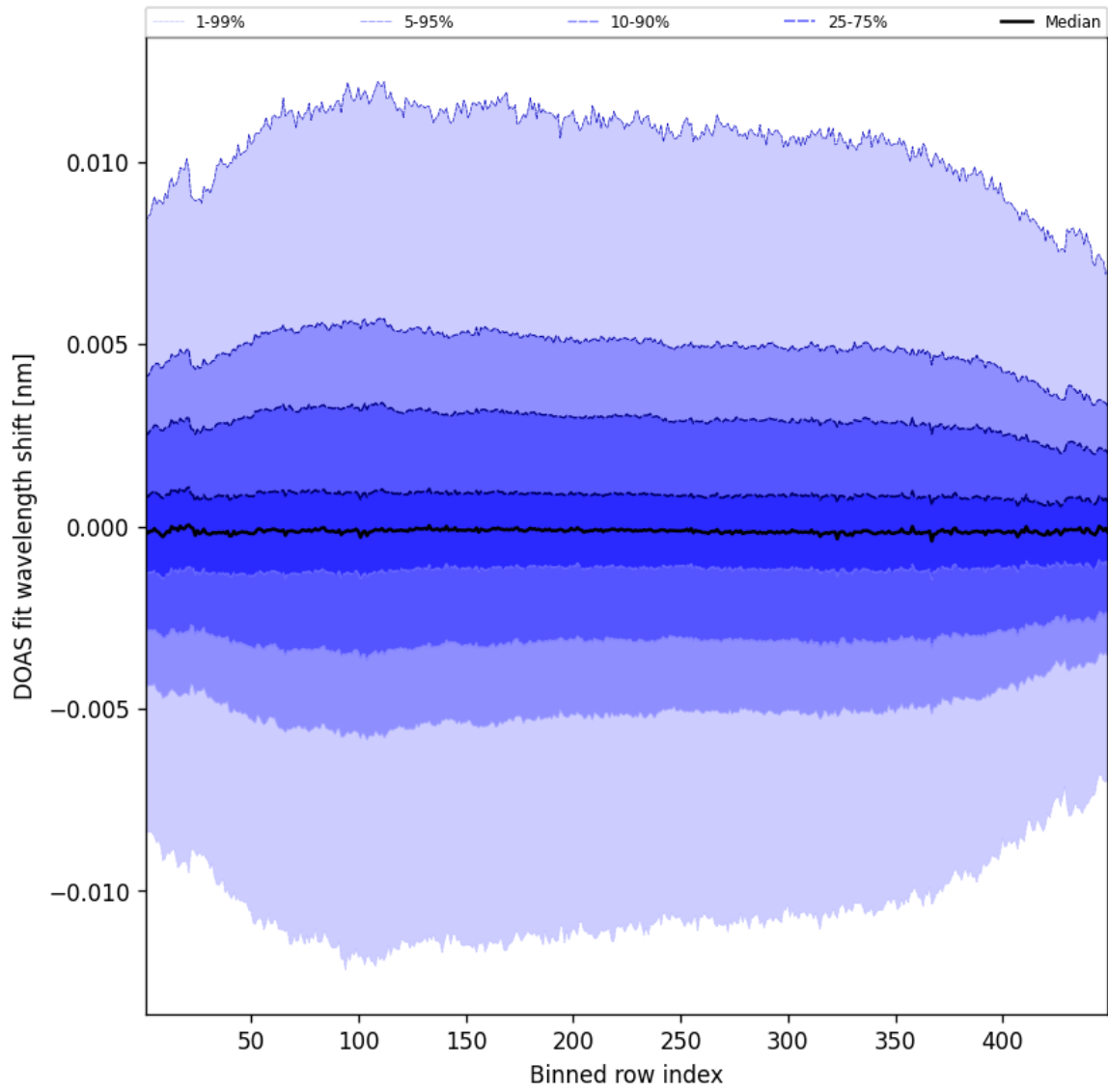
Figure 56: Along track statistics of “DOAS fit wavelength shift” for 2025-08-22 to 2025-08-23
