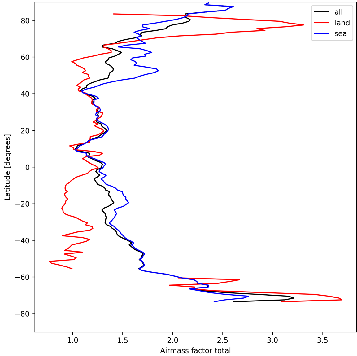
Figure 24: Zonal average of “Airmass factor total” for 2025-08-22 to 2025-08-23.
