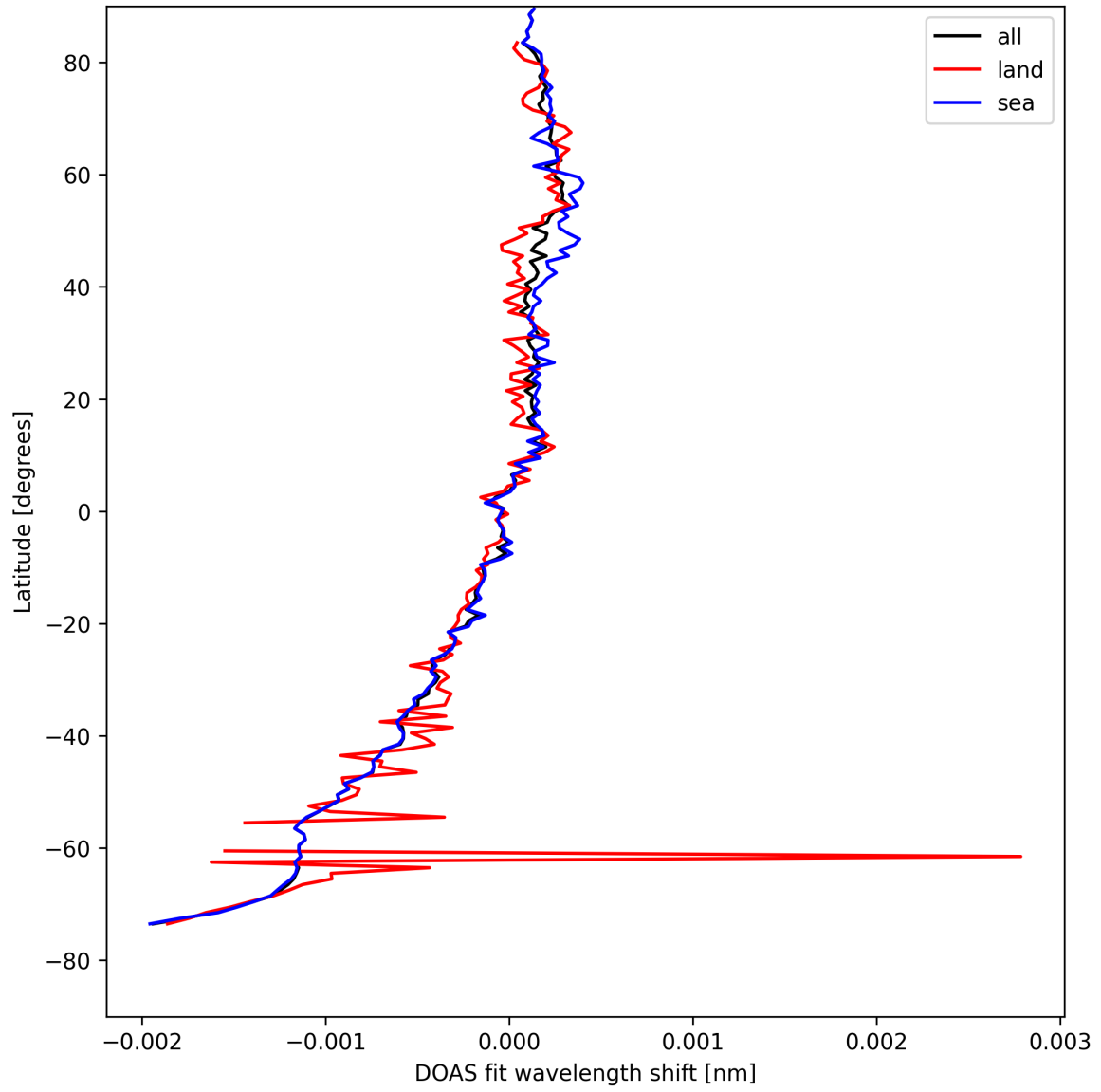
Figure 28: Zonal average of “DOAS fit wavelength shift” for 2025-08-22 to 2025-08-23.
