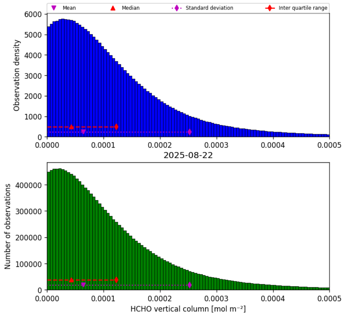
Figure 33: Histogram of “HCHO vertical column” for 2025-08-22 to 2025-08-23
