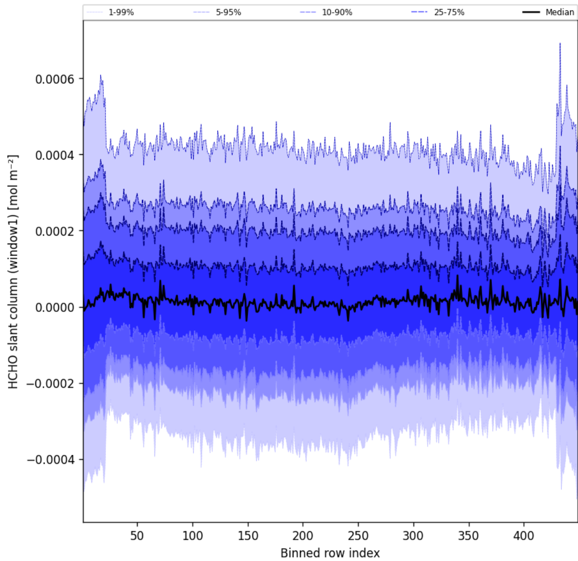
Figure 50: Along track statistics of “HCHO slant column (window1)” for 2025-08-22 to 2025-08-23
