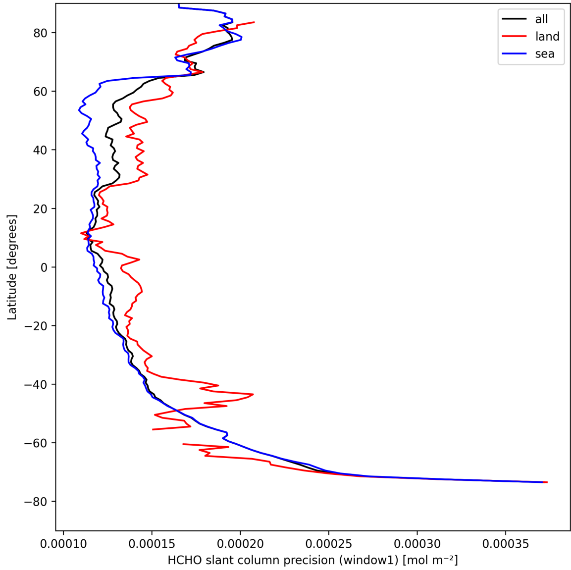
Figure 23: Zonal average of “HCHO slant column precision (window1)” for 2025-08-22 to 2025-08-23.
