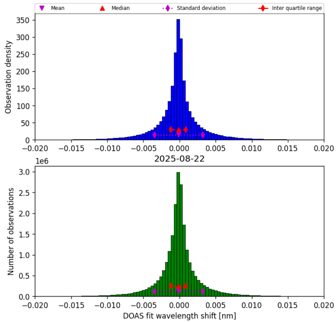
Figure 42: Histogram of “DOAS fit wavelength shift” for 2025-08-22 to 2025-08-23
