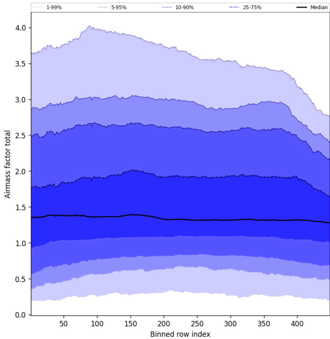
Figure 52: Along track statistics of “Airmass factor total” for 2025-08-22 to 2025-08-23
