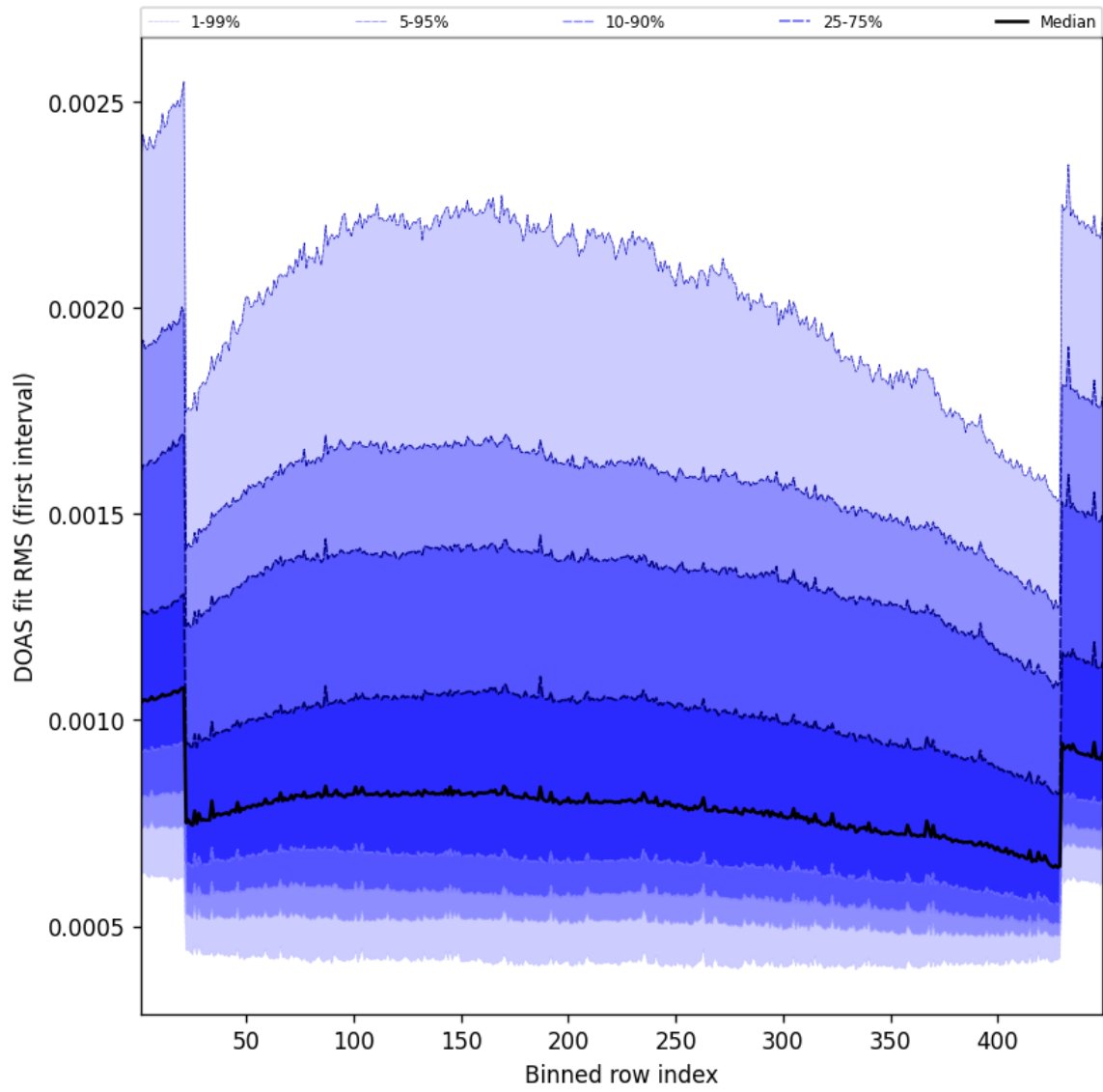
Figure 58: Along track statistics of “DOAS fit RMS (first interval)” for 2025-08-22 to 2025-08-23
