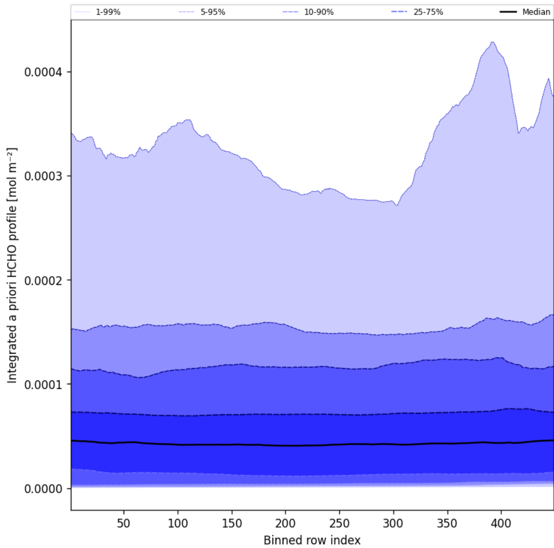
Figure 55: Along track statistics of “Integrated a priori HCHO profile” for 2025-08-22 to 2025-08-23
