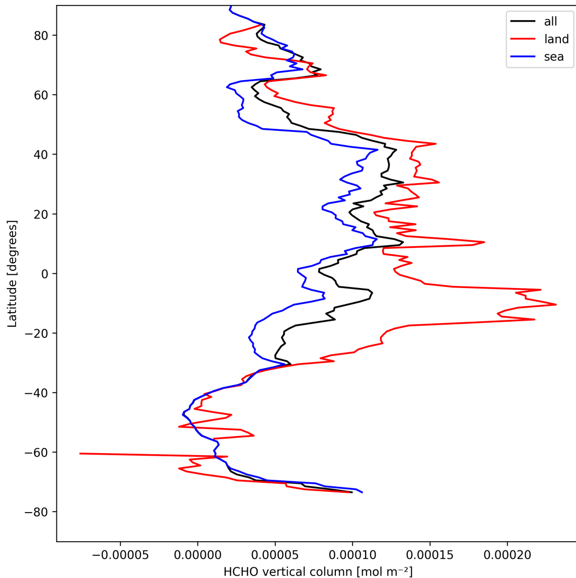
Figure 19: Zonal average of “HCHO vertical column” for 2025-08-22 to 2025-08-23.
