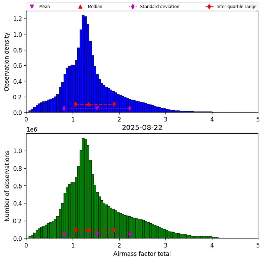
Figure 38: Histogram of “Airmass factor total” for 2025-08-22 to 2025-08-23
