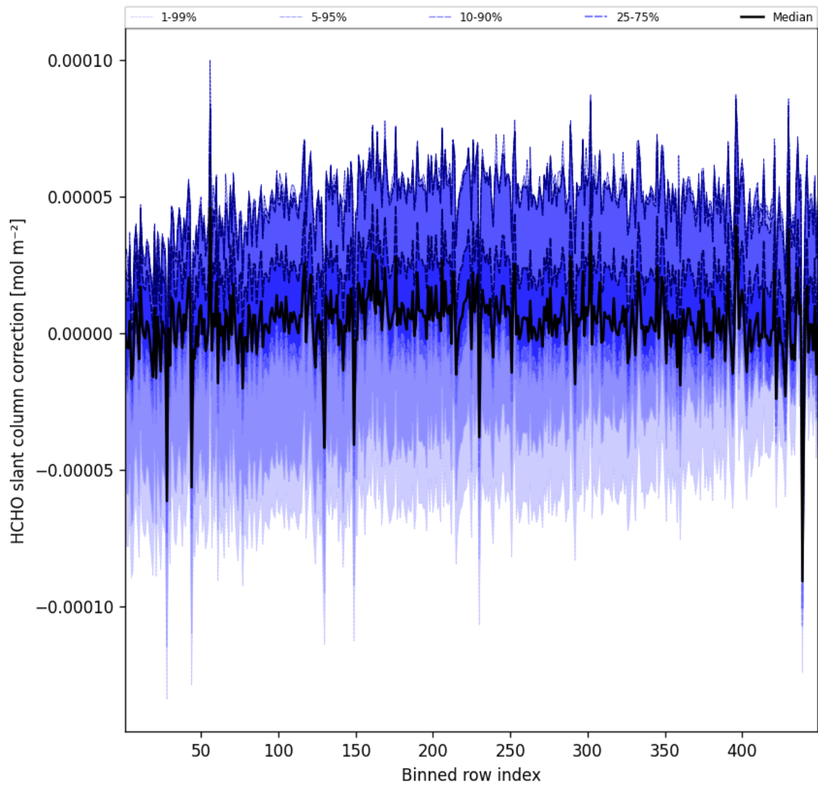
Figure 59: Along track statistics of “HCHO slant column correction” for 2025-08-22 to 2025-08-23
