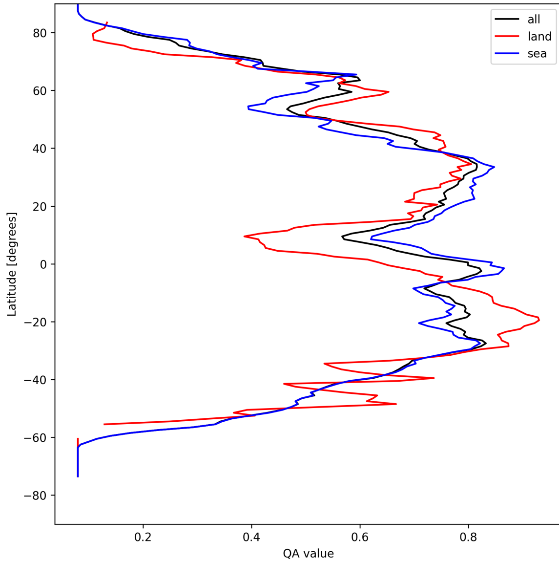
Figure 18: Zonal average of “QA value” for 2025-08-22 to 2025-08-23.
