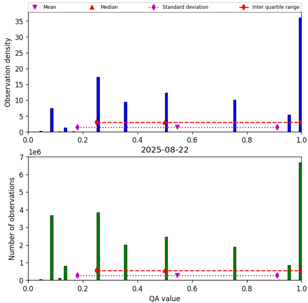
Figure 32: Histogram of “QA value” for 2025-08-22 to 2025-08-23
