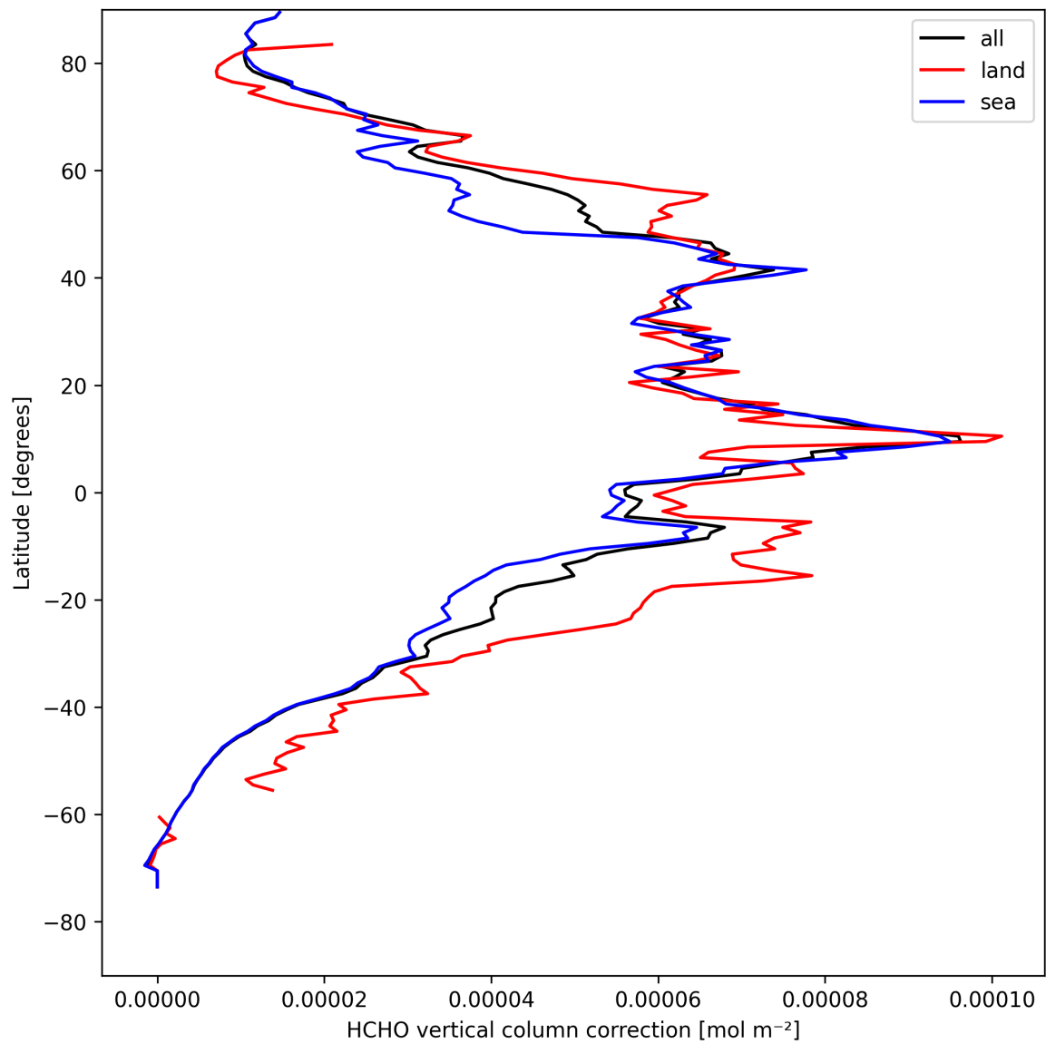
Figure 21: Zonal average of “HCHO vertical column correction” for 2025-08-22 to 2025-08-23.
