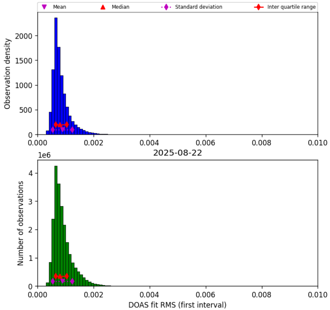
Figure 44: Histogram of “DOAS fit RMS (first interval)” for 2025-08-22 to 2025-08-23
