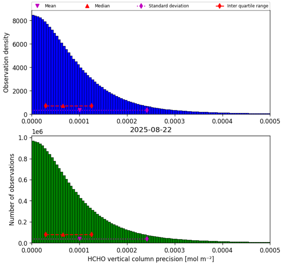
Figure 34: Histogram of “HCHO vertical column precision” for 2025-08-22 to 2025-08-23
