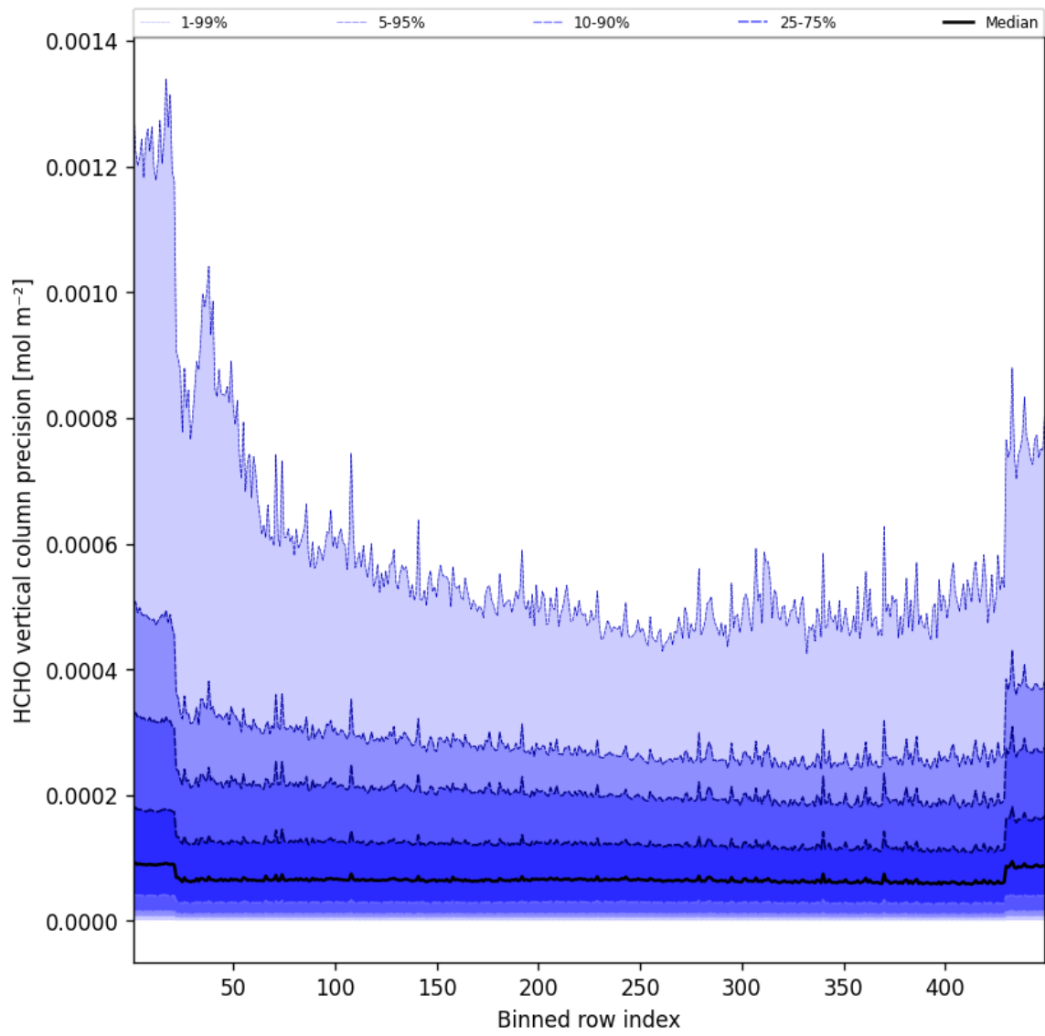
Figure 48: Along track statistics of “HCHO vertical column precision” for 2025-08-22 to 2025-08-23
