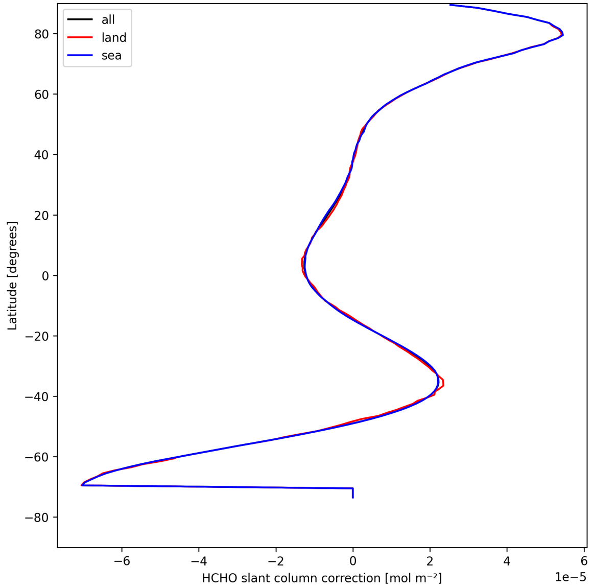
Figure 31: Zonal average of “HCHO slant column correction” for 2025-08-22 to 2025-08-23.
