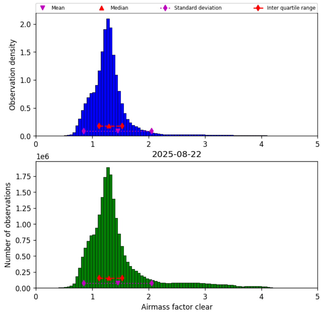
Figure 40: Histogram of “Airmass factor clear” for 2025-08-22 to 2025-08-23
