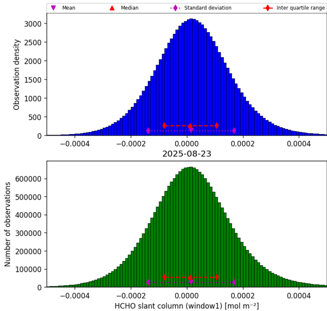
Figure 36: Histogram of “HCHO slant column (window1)” for 2025-08-23 to 2025-08-23
