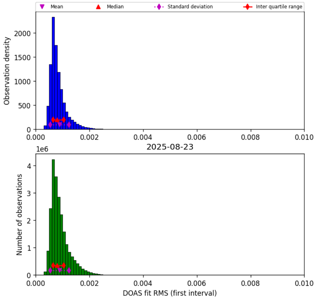
Figure 44: Histogram of “DOAS fit RMS (first interval)” for 2025-08-23 to 2025-08-23
