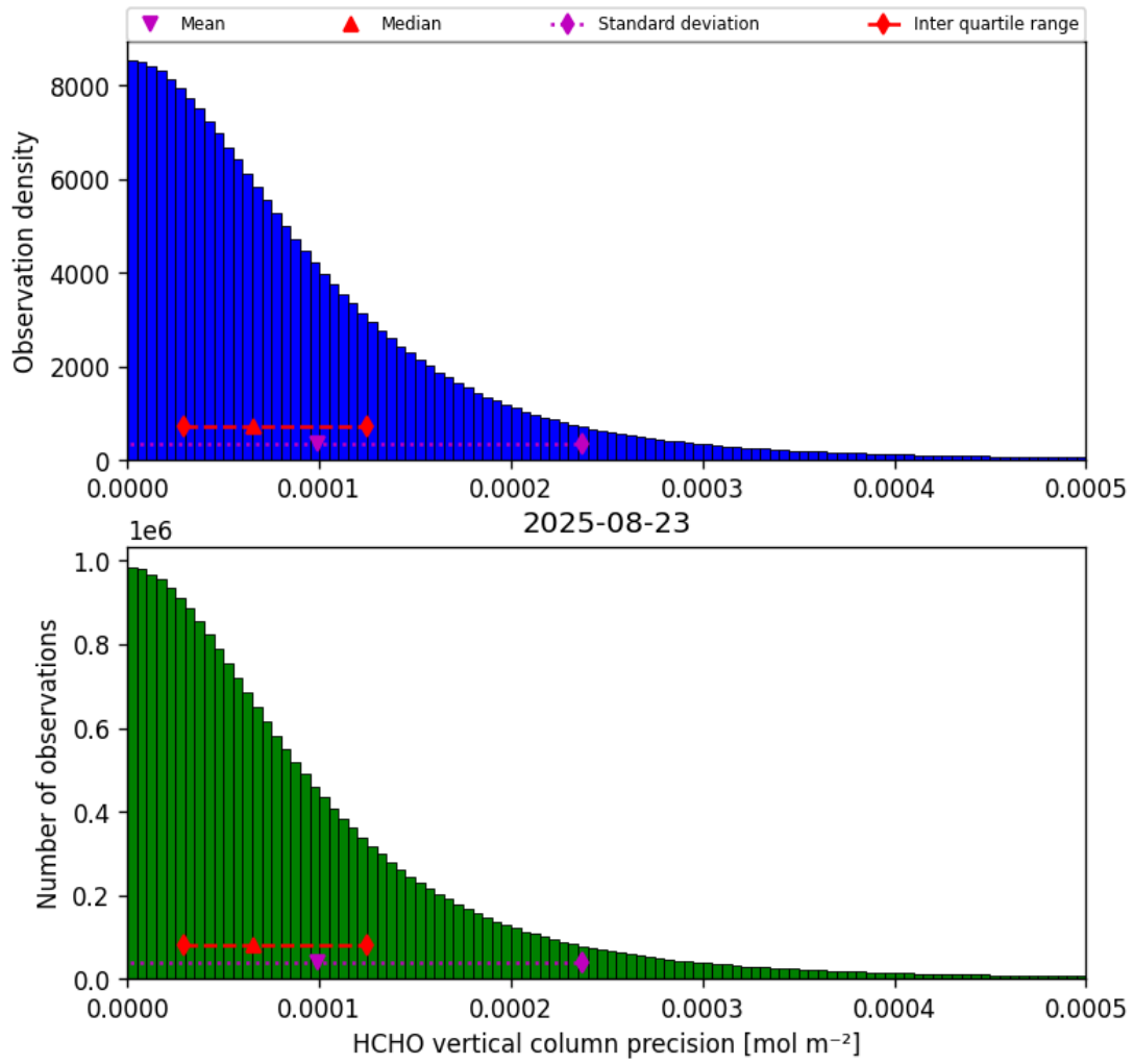
Figure 34: Histogram of “HCHO vertical column precision” for 2025-08-23 to 2025-08-23
