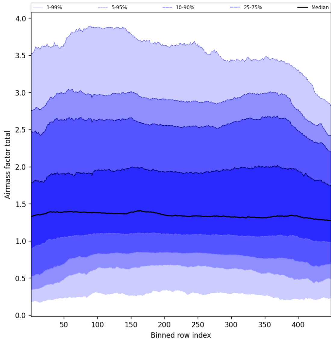
Figure 52: Along track statistics of “Airmass factor total” for 2025-08-23 to 2025-08-23
