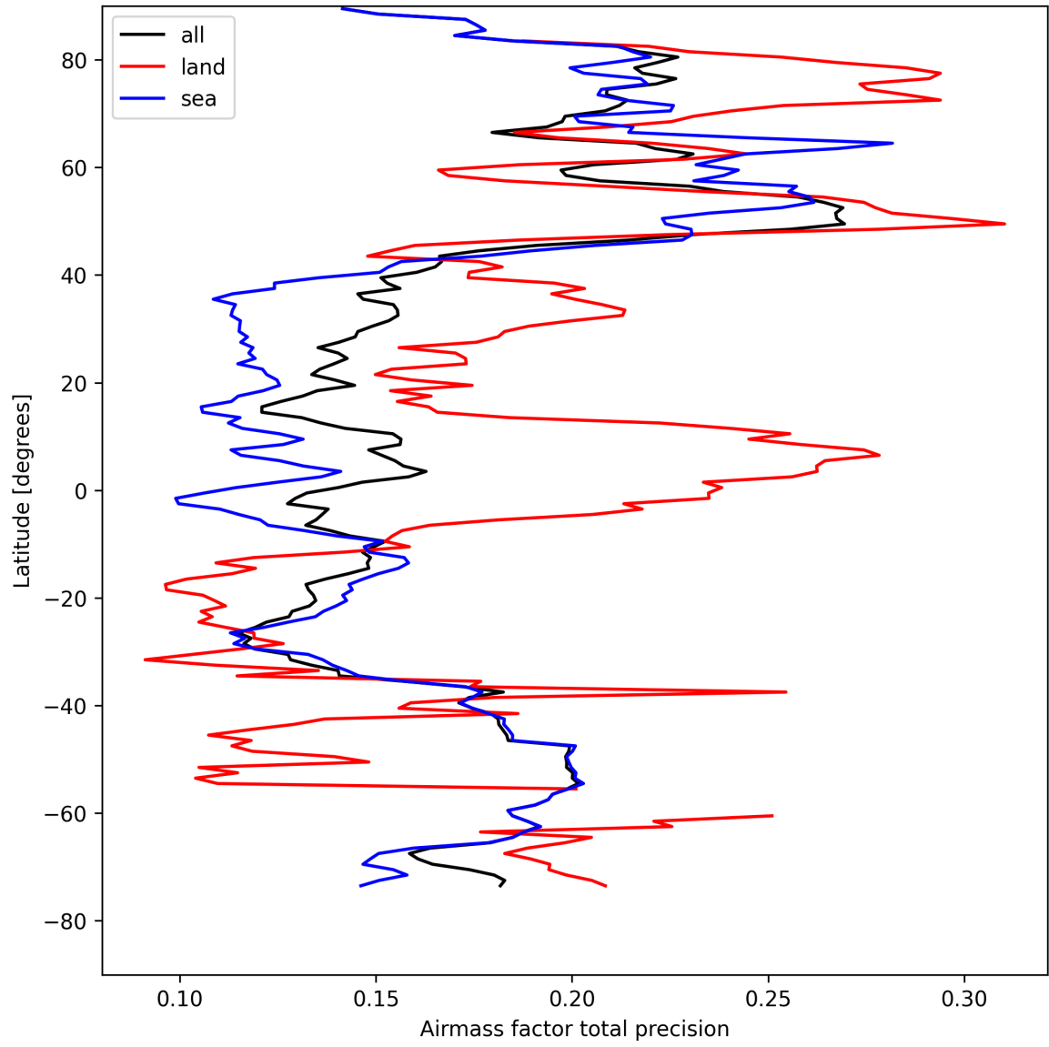
Figure 25: Zonal average of “Airmass factor total precision” for 2025-08-23 to 2025-08-23.
