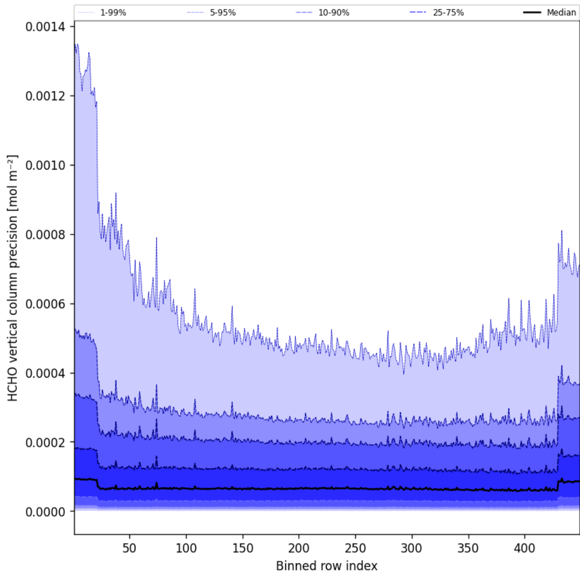
Figure 48: Along track statistics of “HCHO vertical column precision” for 2025-08-23 to 2025-08-23
