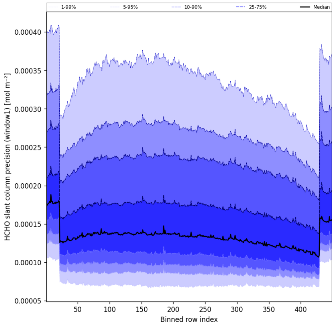
Figure 51: Along track statistics of “HCHO slant column precision (window1)” for 2025-08-23 to 2025-08-23
