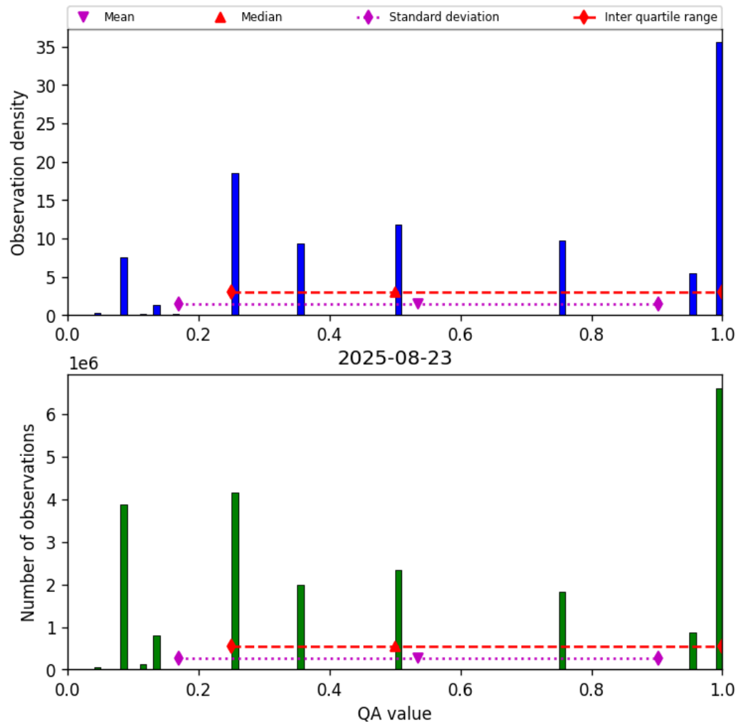
Figure 32: Histogram of “QA value” for 2025-08-23 to 2025-08-23
