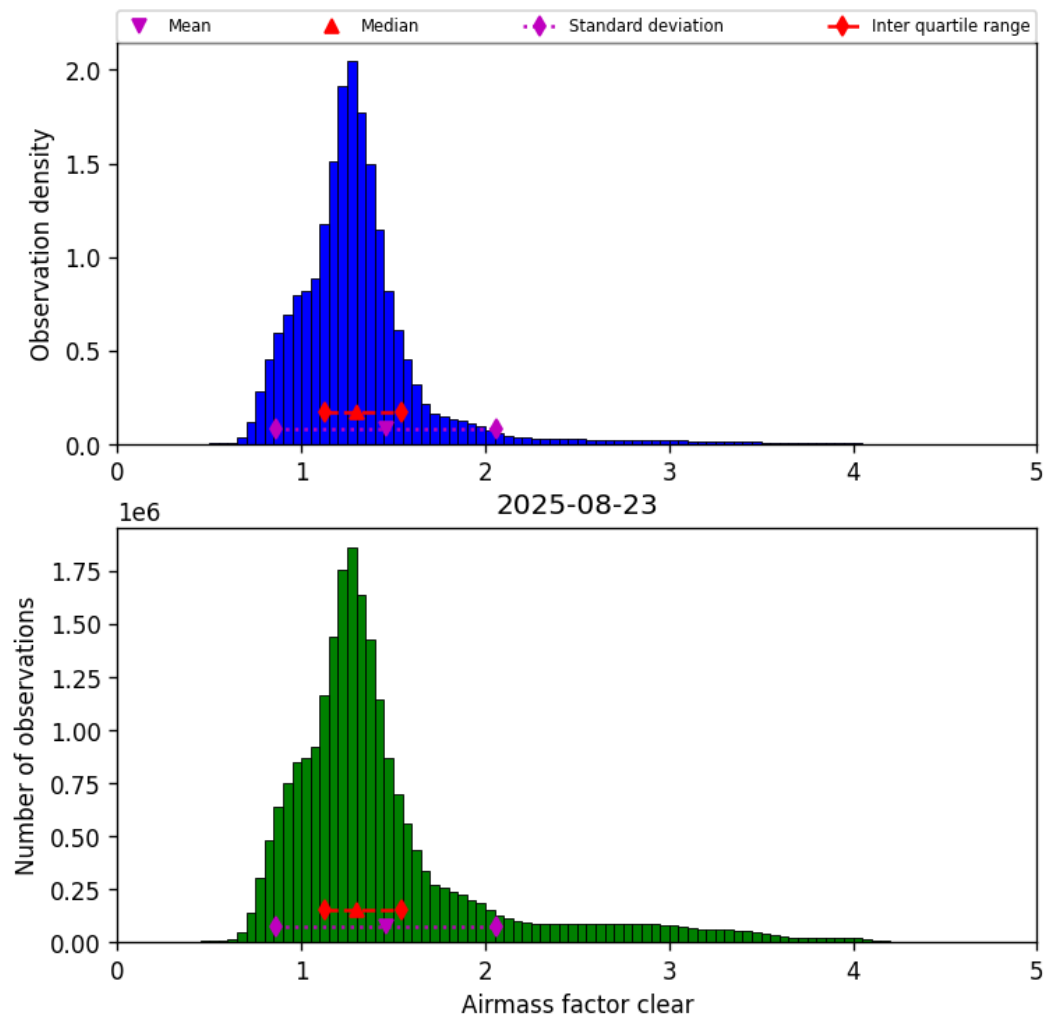
Figure 40: Histogram of “Airmass factor clear” for 2025-08-23 to 2025-08-23
