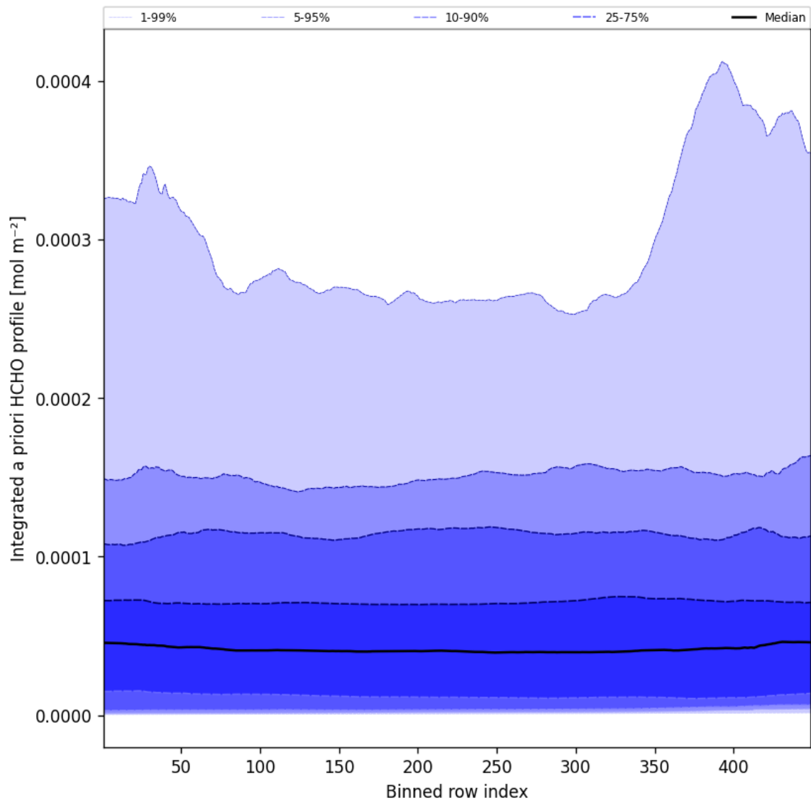
Figure 55: Along track statistics of “Integrated a priori HCHO profile” for 2025-08-23 to 2025-08-23
