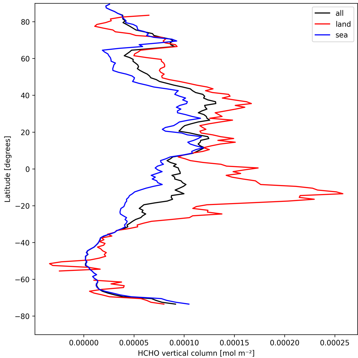
Figure 19: Zonal average of “HCHO vertical column” for 2025-08-23 to 2025-08-23.
