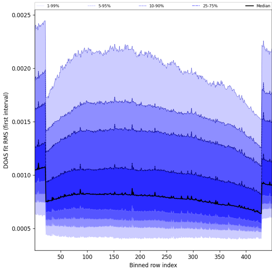
Figure 58: Along track statistics of “DOAS fit RMS (first interval)” for 2025-08-23 to 2025-08-23
