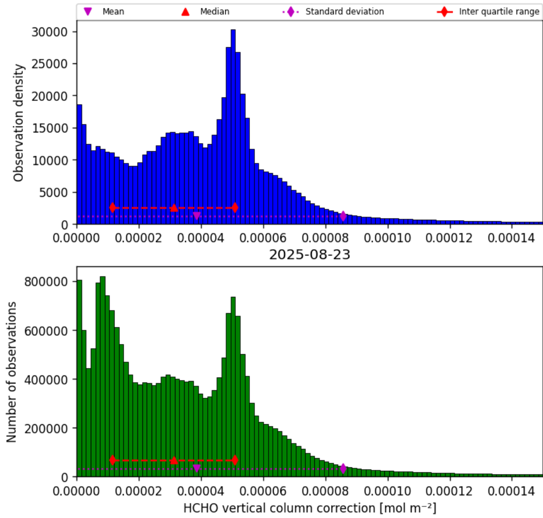
Figure 35: Histogram of “HCHO vertical column correction” for 2025-08-23 to 2025-08-23
