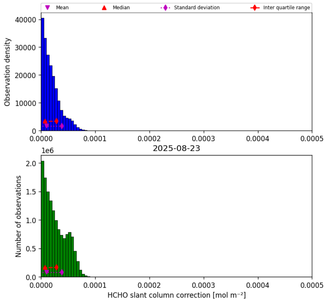
Figure 45: Histogram of “HCHO slant column correction” for 2025-08-23 to 2025-08-23
