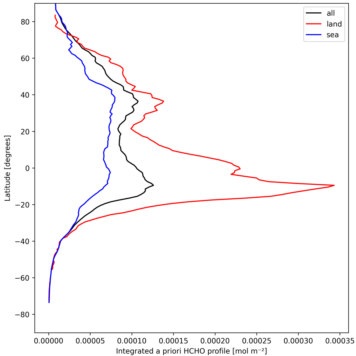
Figure 27: Zonal average of “Integrated a priori HCHO profile” for 2025-08-23 to 2025-08-23.
