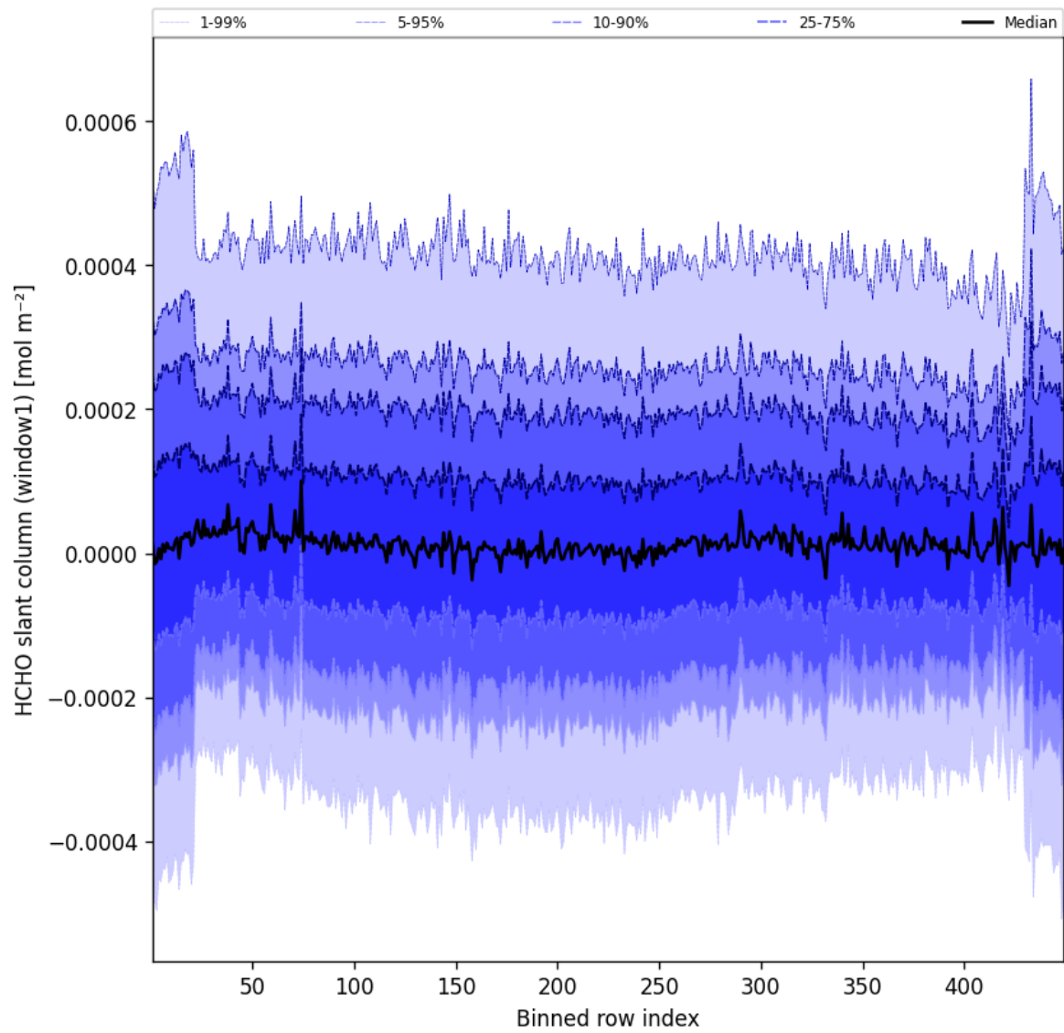
Figure 50: Along track statistics of “HCHO slant column (window1)” for 2025-08-23 to 2025-08-23
