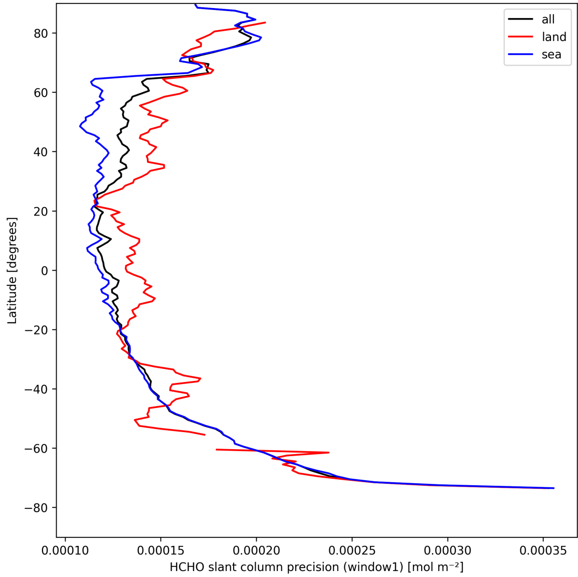
Figure 23: Zonal average of “HCHO slant column precision (window1)” for 2025-08-23 to 2025-08-23.
