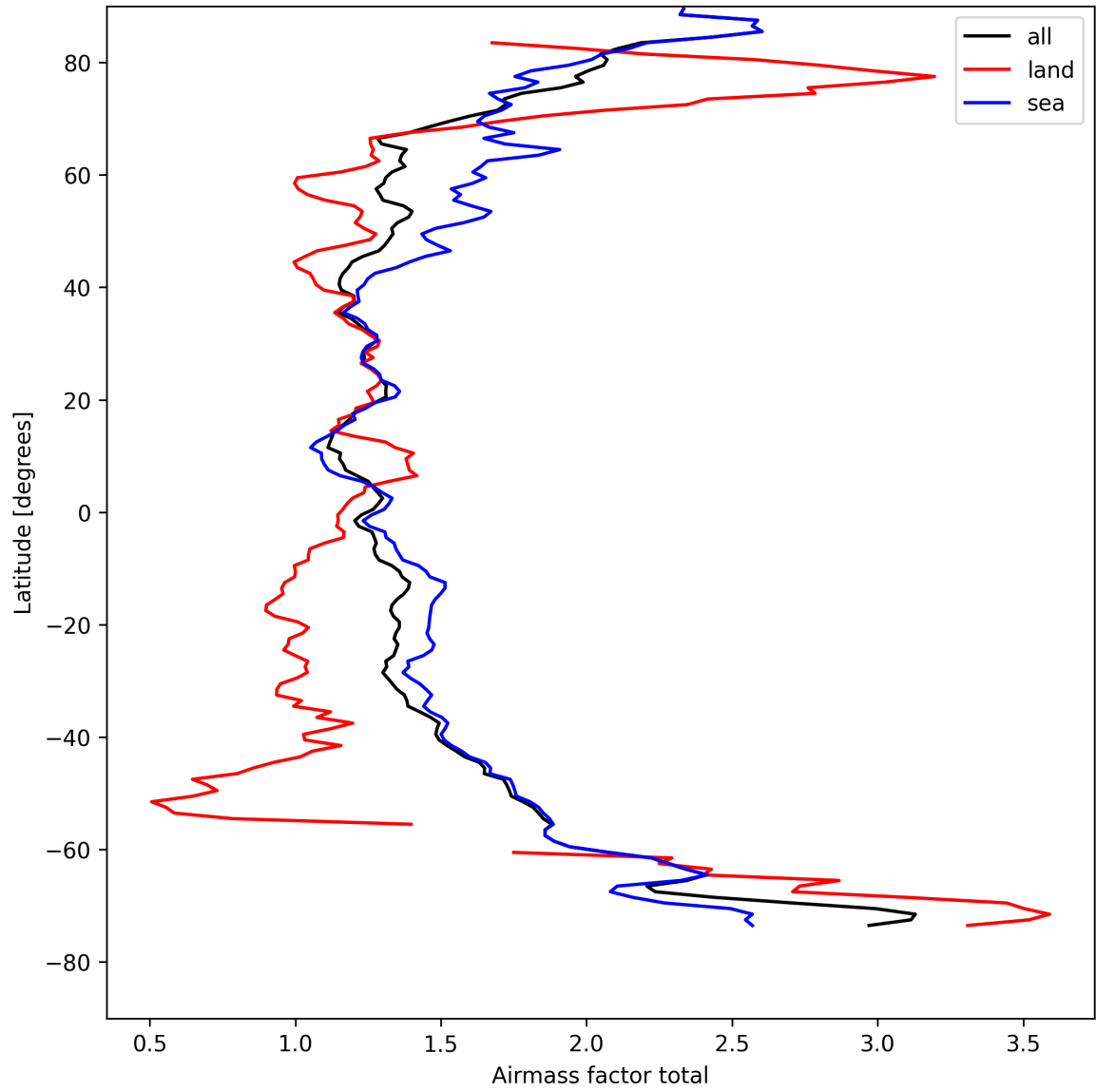
Figure 24: Zonal average of “Airmass factor total” for 2025-08-23 to 2025-08-23.
