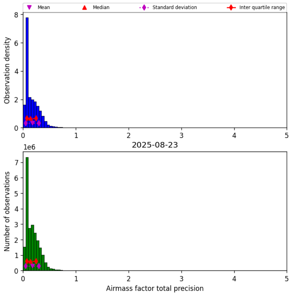
Figure 39: Histogram of “Airmass factor total precision” for 2025-08-23 to 2025-08-23
