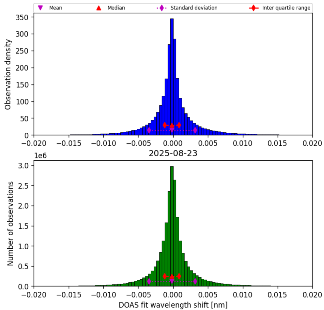
Figure 42: Histogram of “DOAS fit wavelength shift” for 2025-08-23 to 2025-08-23
