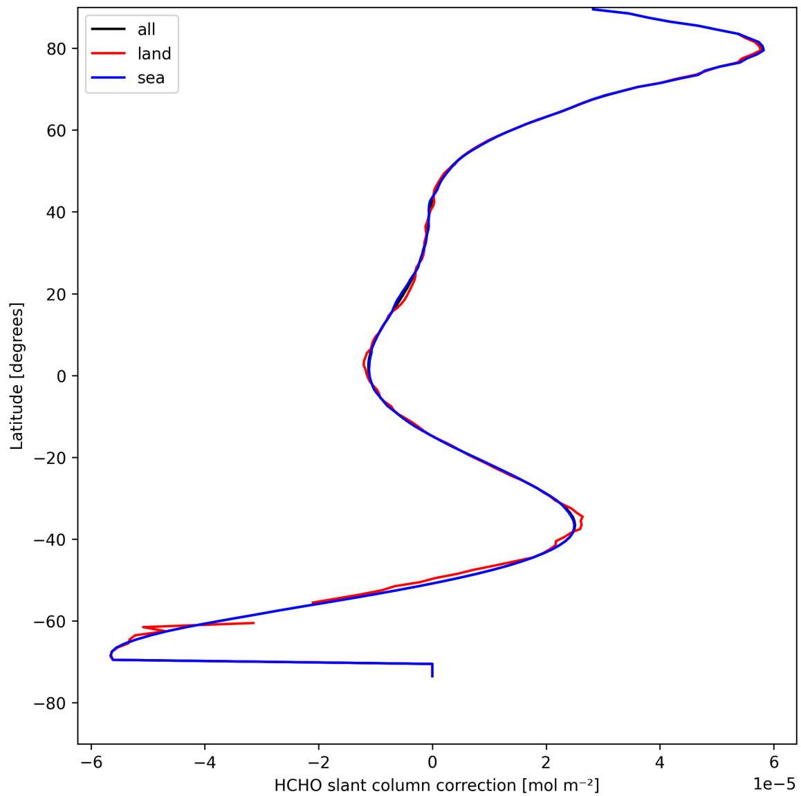
Figure 31: Zonal average of “HCHO slant column correction” for 2025-08-23 to 2025-08-23.
