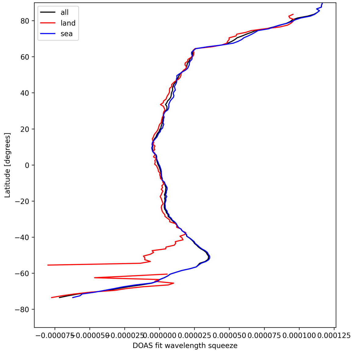
Figure 29: Zonal average of “DOAS fit wavelength squeeze” for 2025-08-23 to 2025-08-23.
