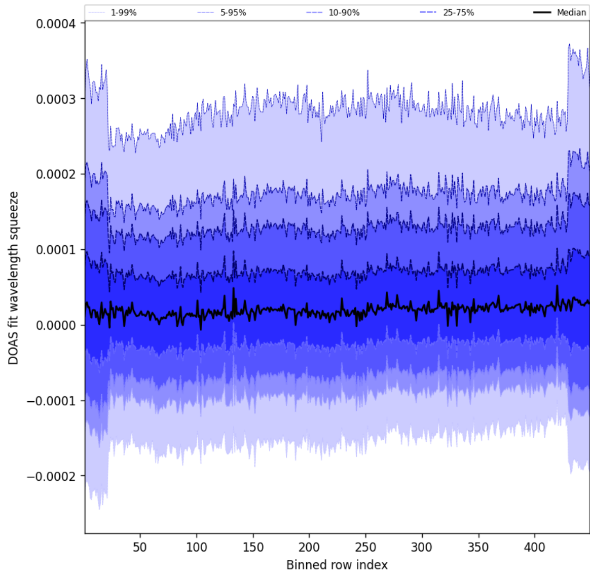
Figure 57: Along track statistics of “DOAS fit wavelength squeeze” for 2025-08-23 to 2025-08-23
