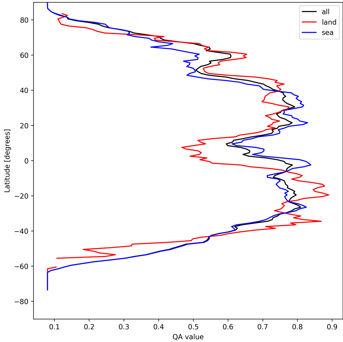
Figure 18: Zonal average of “QA value” for 2025-08-23 to 2025-08-23.
