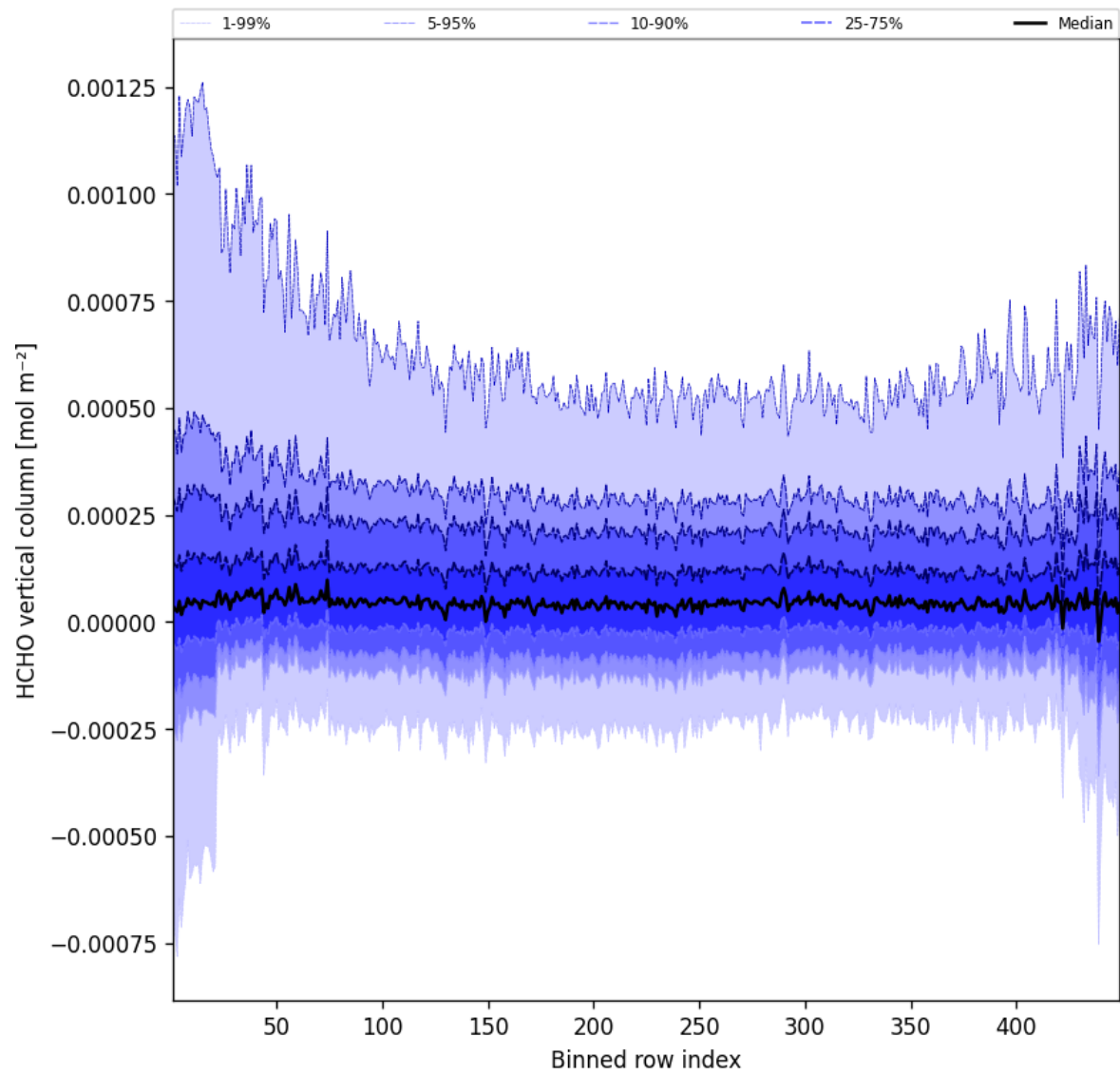
Figure 47: Along track statistics of “HCHO vertical column” for 2025-08-23 to 2025-08-23
