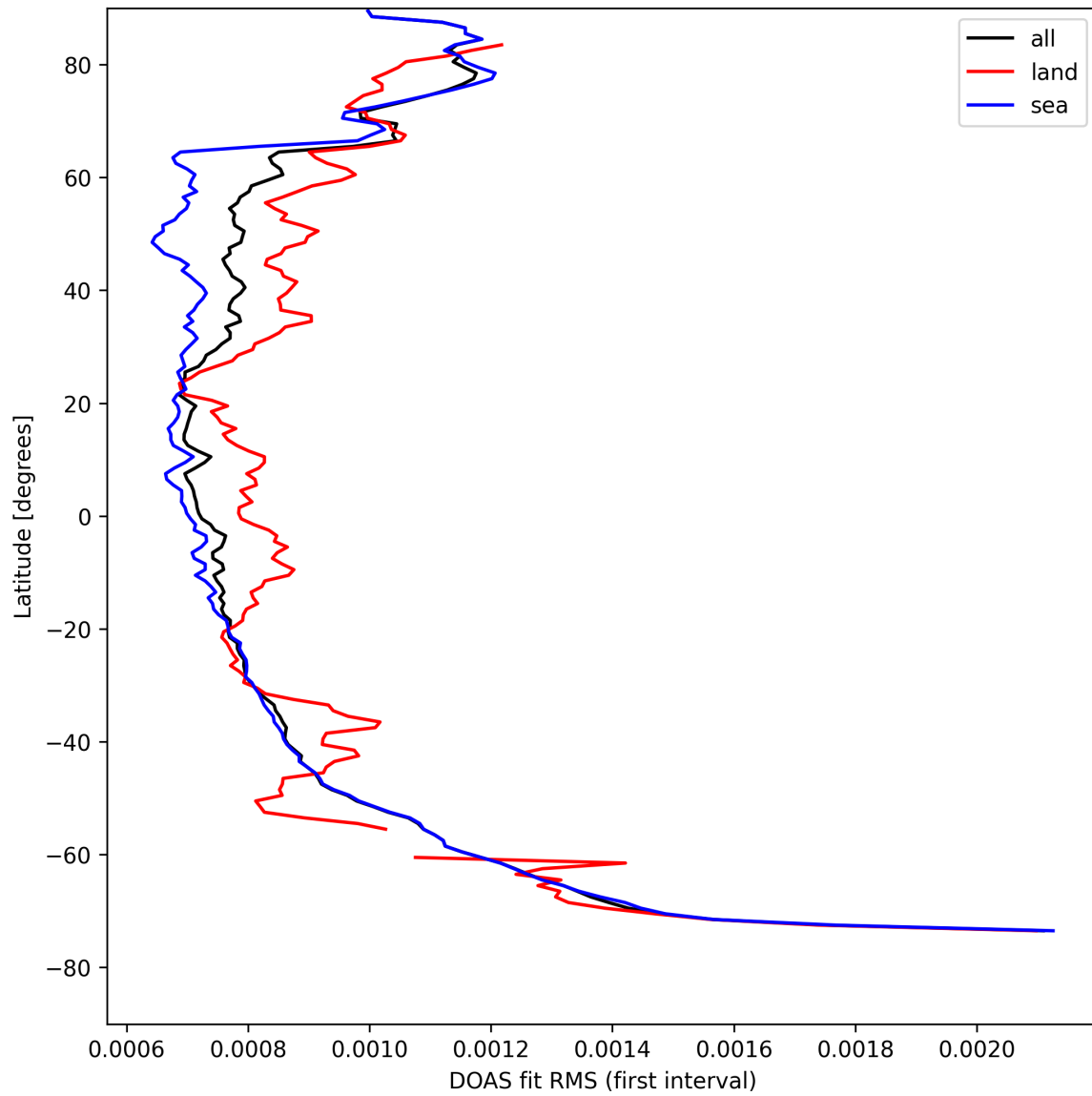
Figure 30: Zonal average of “DOAS fit RMS (first interval)” for 2025-08-23 to 2025-08-23.
