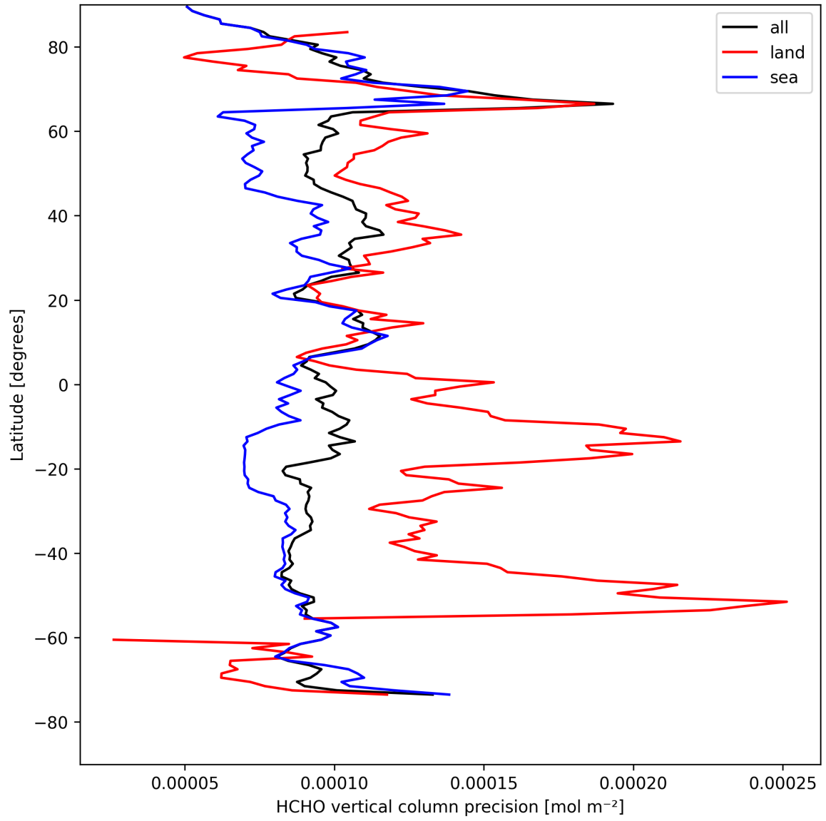
Figure 20: Zonal average of “HCHO vertical column precision” for 2025-08-23 to 2025-08-23.
