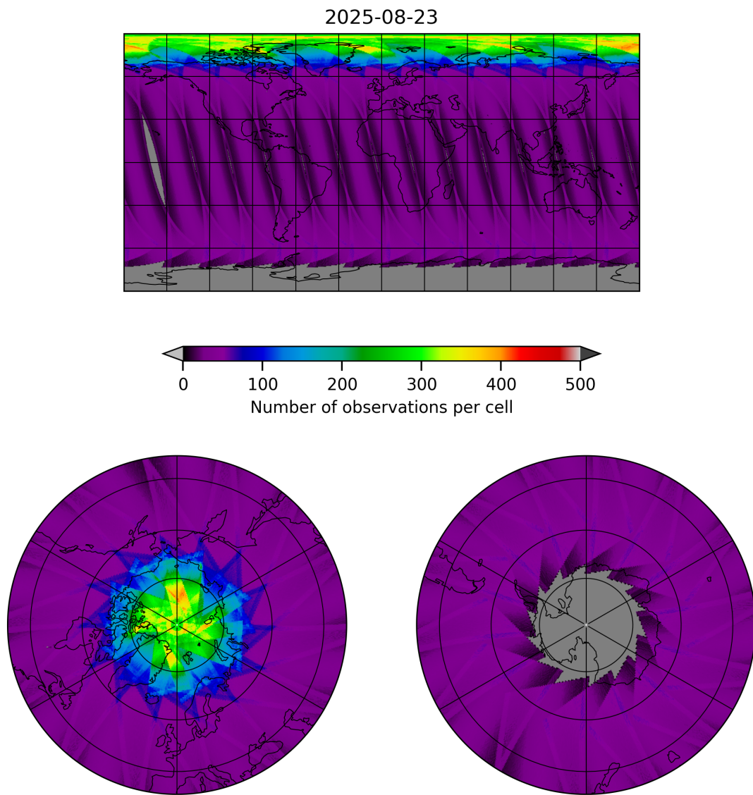
Figure 17: Map of the number of observations for 2025-08-23 to 2025-08-23
