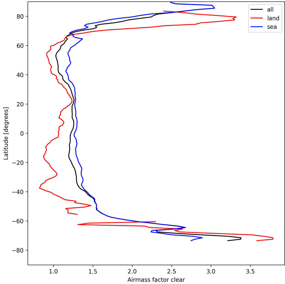
Figure 26: Zonal average of “Airmass factor clear” for 2025-08-23 to 2025-08-23.
