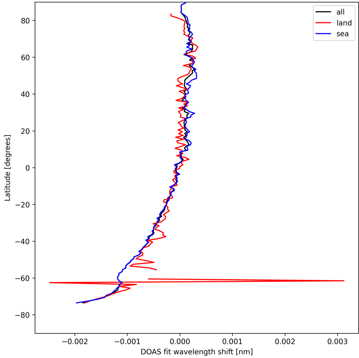
Figure 28: Zonal average of “DOAS fit wavelength shift” for 2025-08-23 to 2025-08-23.
