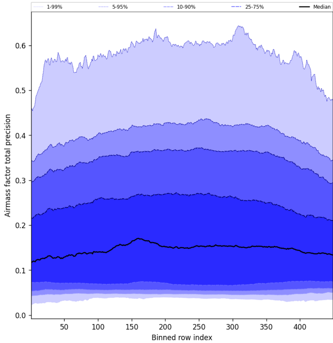
Figure 53: Along track statistics of “Airmass factor total precision” for 2025-08-23 to 2025-08-23
