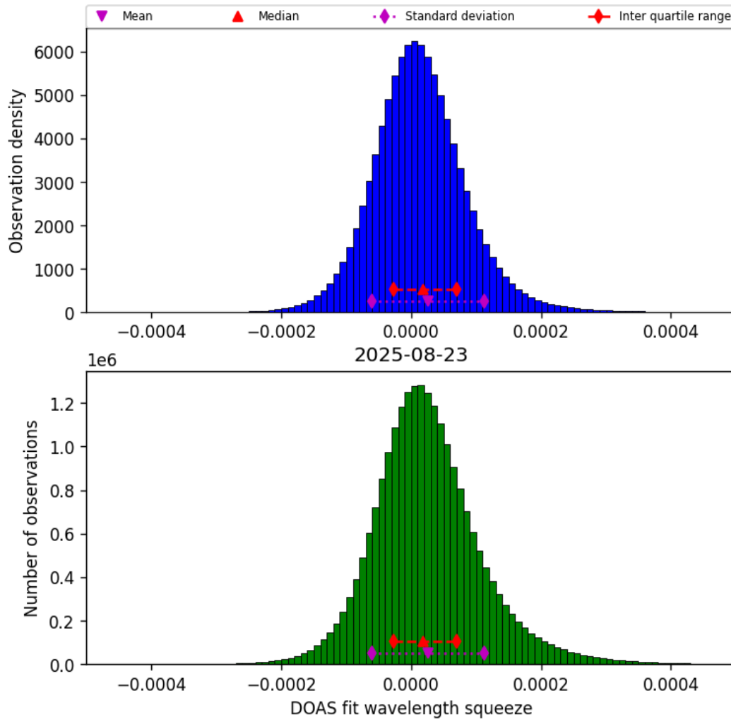
Figure 43: Histogram of “DOAS fit wavelength squeeze” for 2025-08-23 to 2025-08-23
