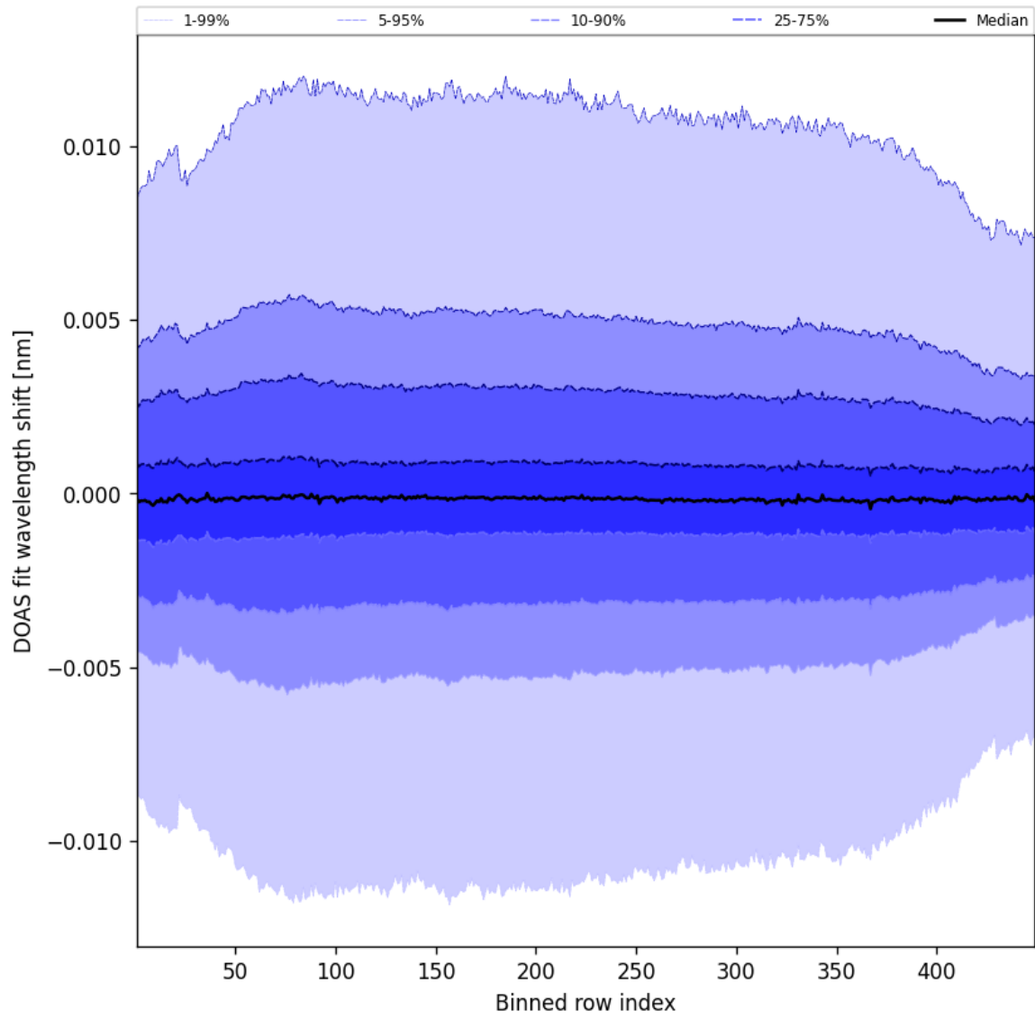
Figure 56: Along track statistics of “DOAS fit wavelength shift” for 2025-08-23 to 2025-08-23
