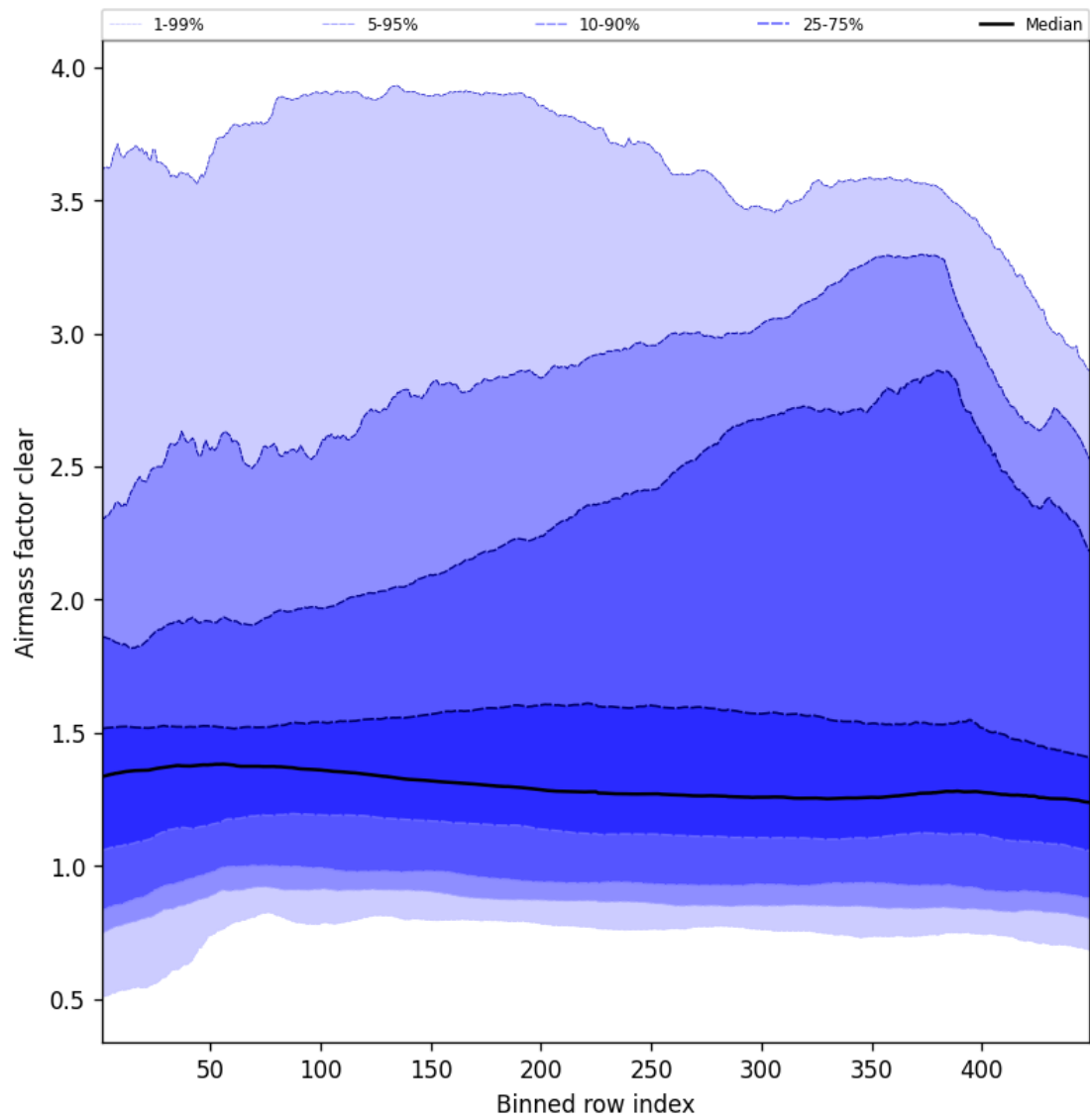
Figure 54: Along track statistics of “Airmass factor clear” for 2025-08-23 to 2025-08-23
