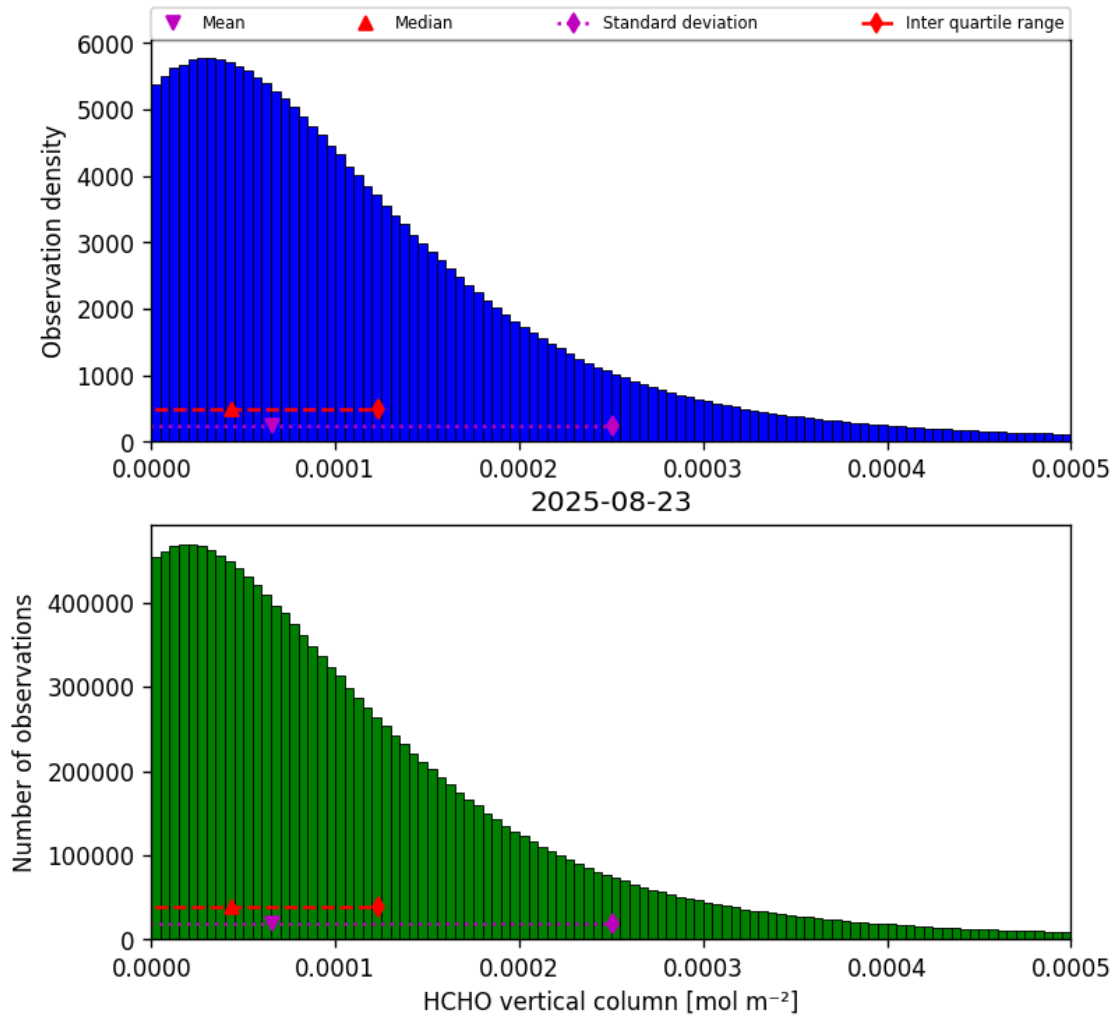
Figure 33: Histogram of “HCHO vertical column” for 2025-08-23 to 2025-08-23
