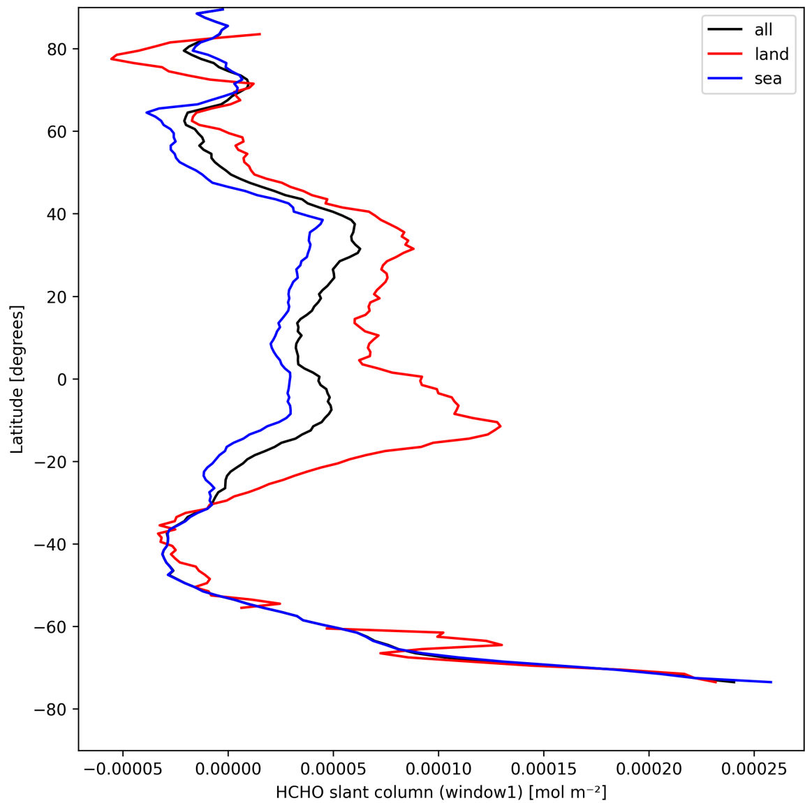
Figure 22: Zonal average of “HCHO slant column (window1)” for 2025-08-23 to 2025-08-23.
