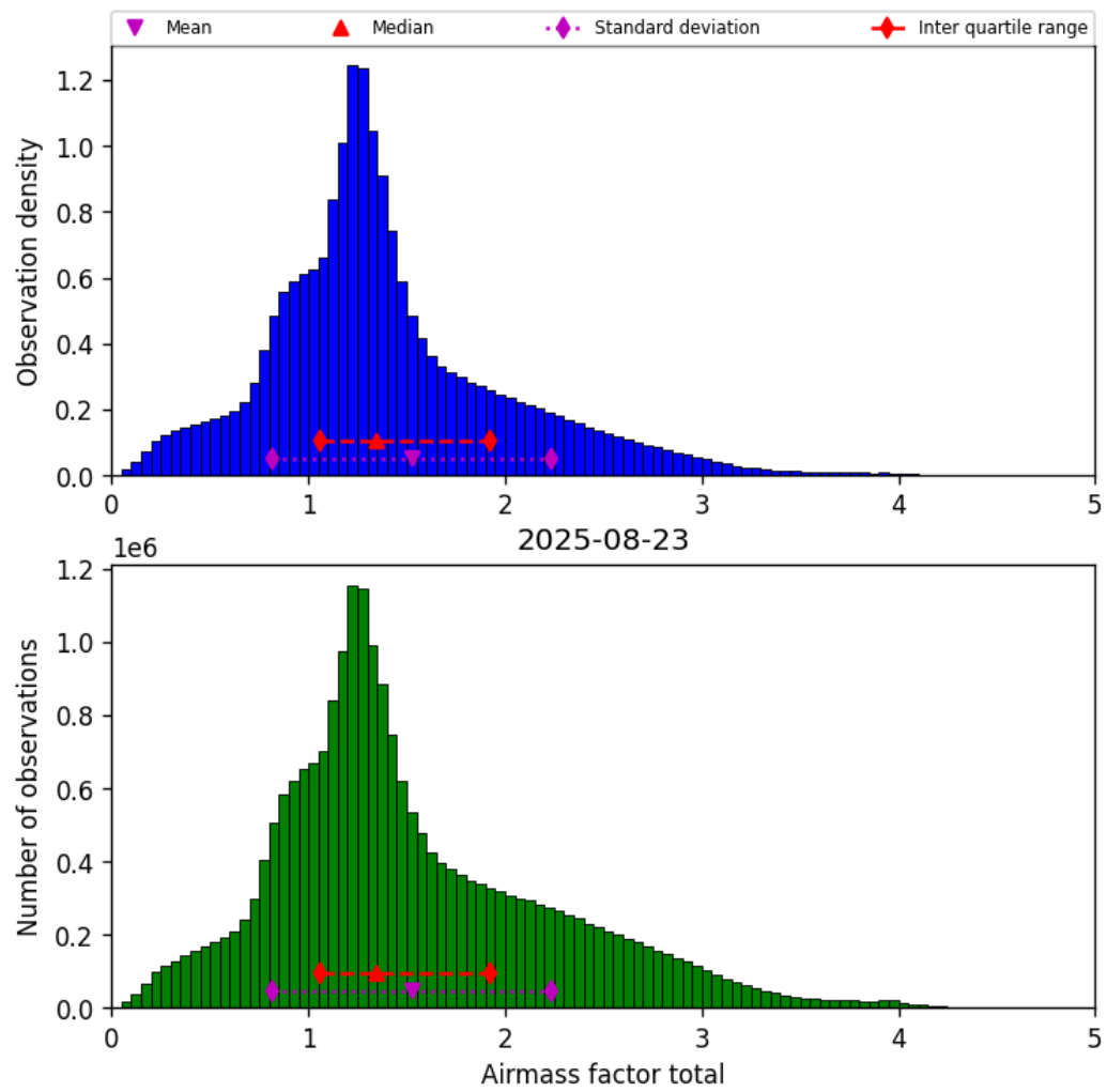
Figure 38: Histogram of “Airmass factor total” for 2025-08-23 to 2025-08-23
