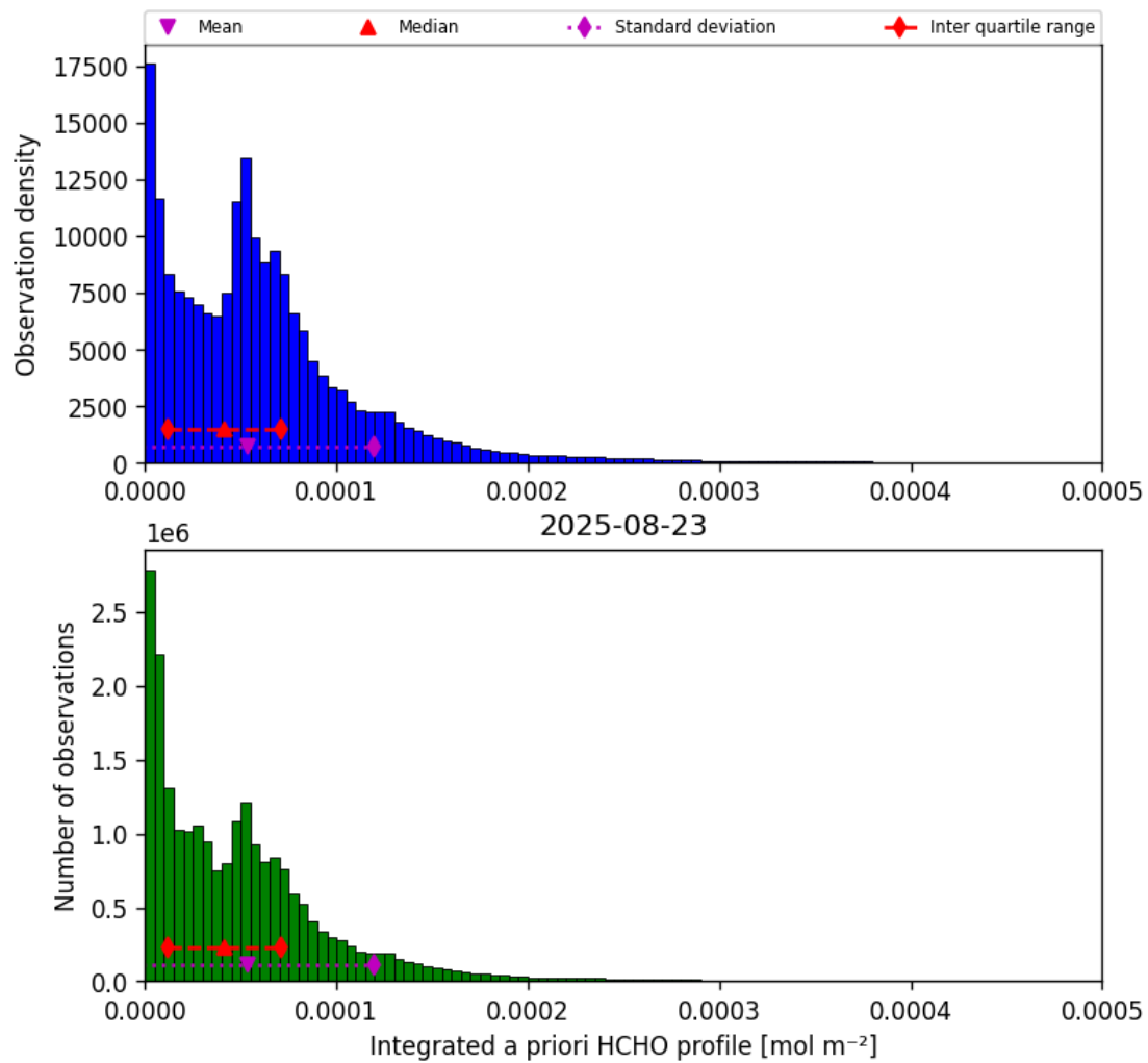
Figure 41: Histogram of “Integrated a priori HCHO profile” for 2025-08-23 to 2025-08-23
