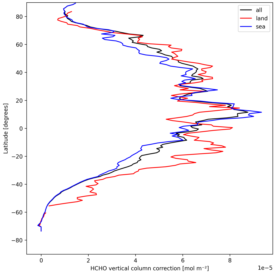
Figure 21: Zonal average of “HCHO vertical column correction” for 2025-08-23 to 2025-08-23.
