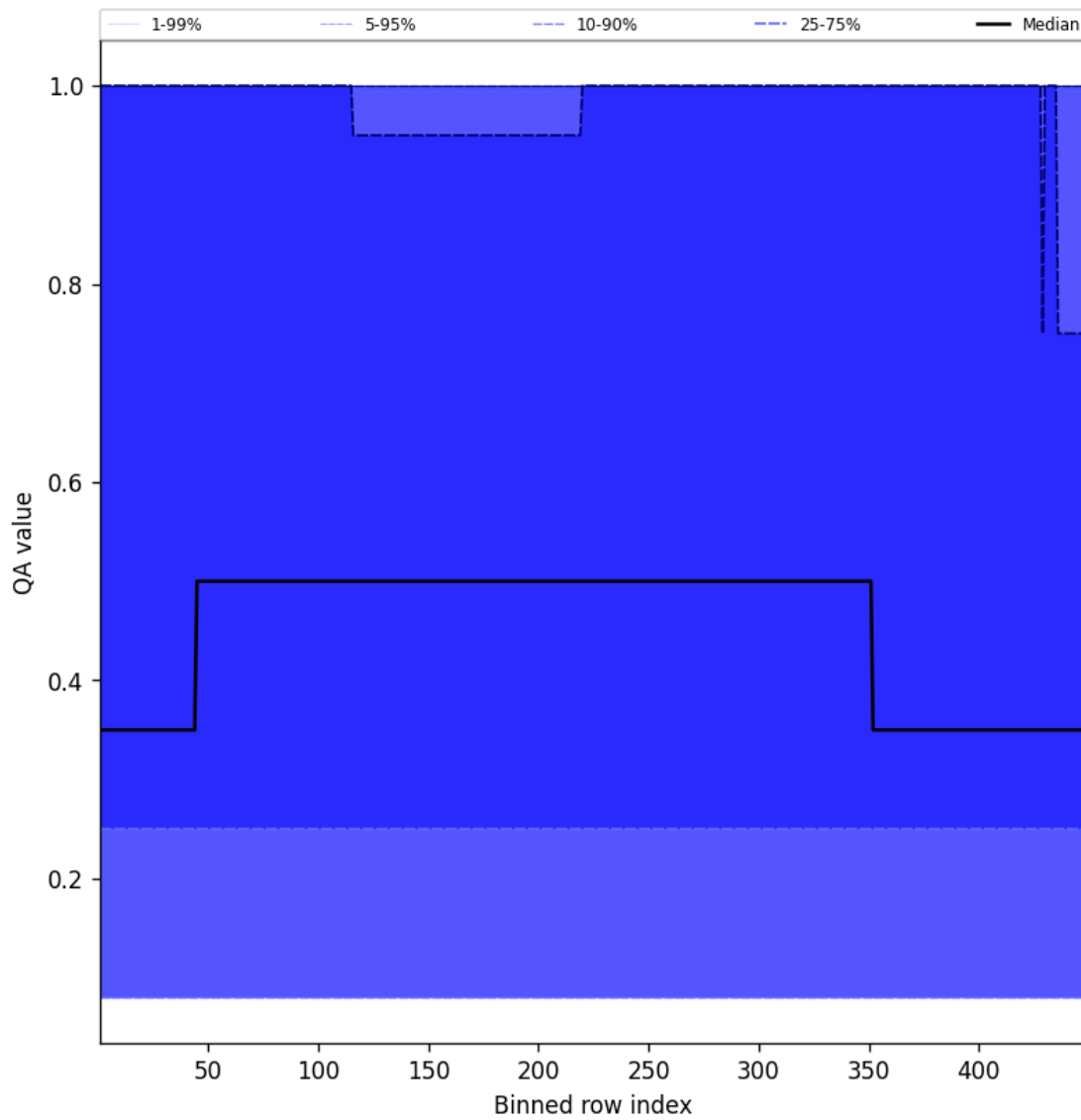
Figure 46: Along track statistics of “QA value” for 2025-08-23 to 2025-08-23
