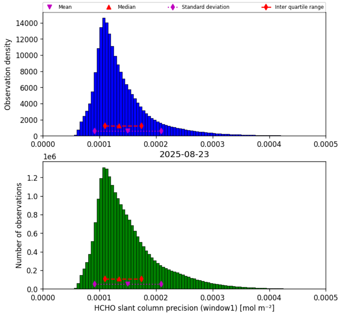
Figure 37: Histogram of “HCHO slant column precision (window1)” for 2025-08-23 to 2025-08-23
