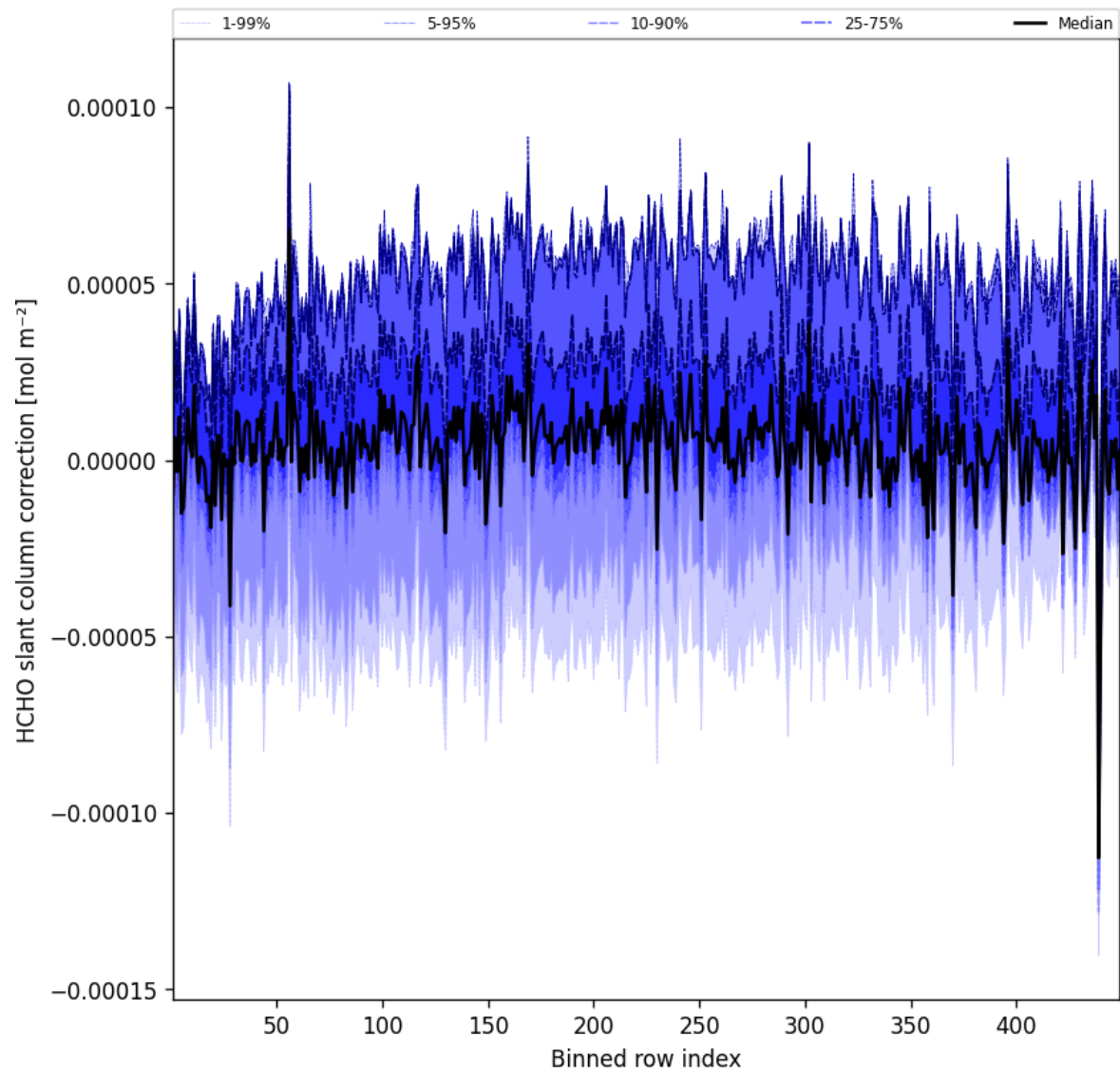
Figure 59: Along track statistics of “HCHO slant column correction” for 2025-08-23 to 2025-08-23
