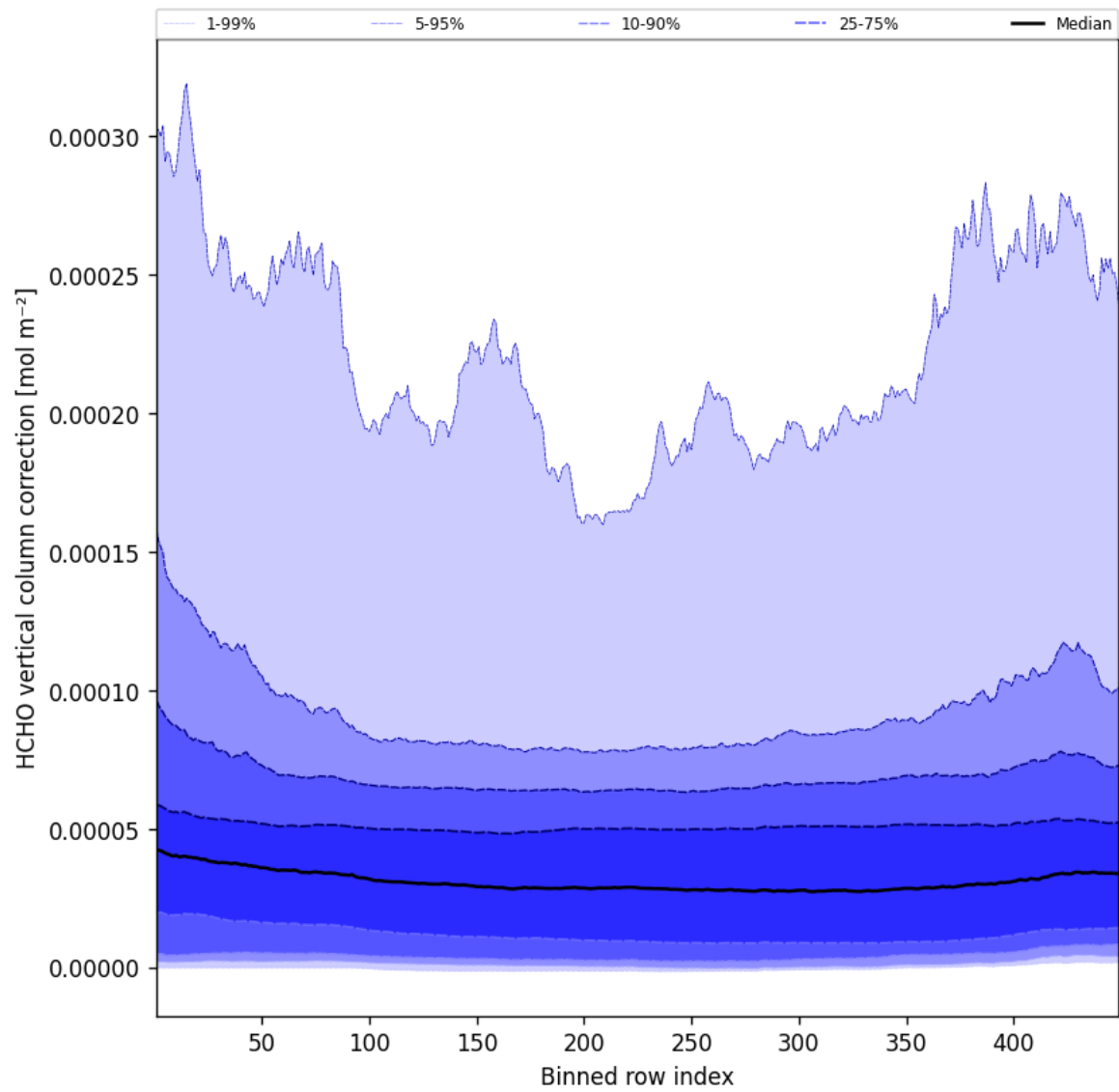
Figure 49: Along track statistics of “HCHO vertical column correction” for 2025-08-23 to 2025-08-23
