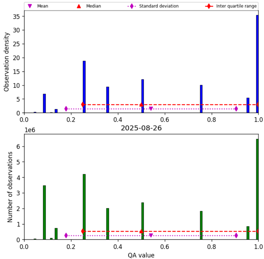
Figure 32: Histogram of “QA value” for 2025-08-26 to 2025-08-27
