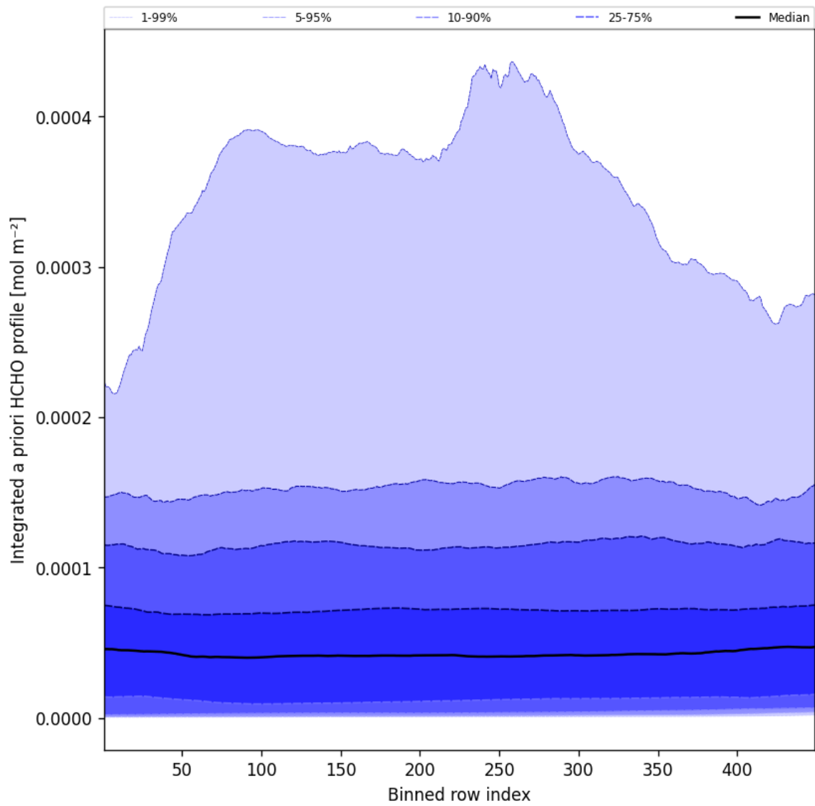
Figure 55: Along track statistics of “Integrated a priori HCHO profile” for 2025-08-26 to 2025-08-27
