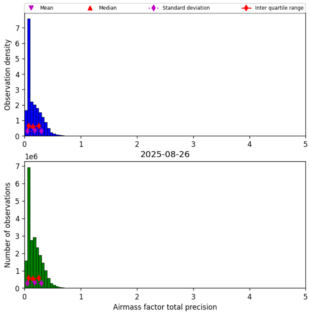
Figure 39: Histogram of “Airmass factor total precision” for 2025-08-26 to 2025-08-27
