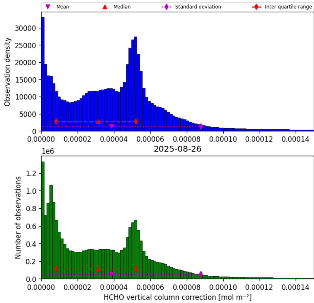
Figure 35: Histogram of “HCHO vertical column correction” for 2025-08-26 to 2025-08-27
