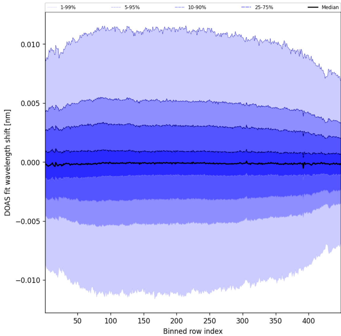
Figure 56: Along track statistics of “DOAS fit wavelength shift” for 2025-08-26 to 2025-08-27
