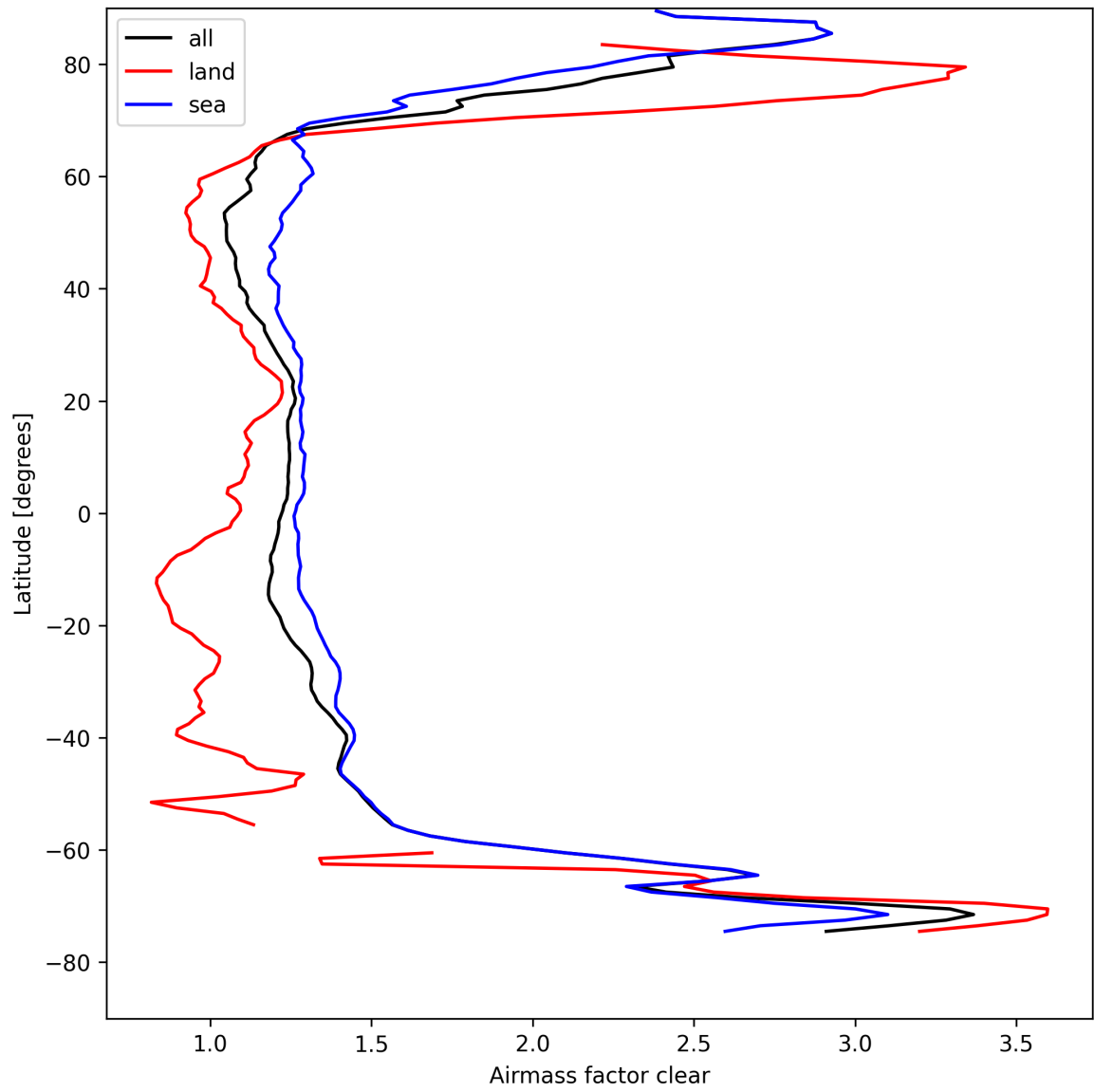
Figure 26: Zonal average of “Airmass factor clear” for 2025-08-26 to 2025-08-27.
