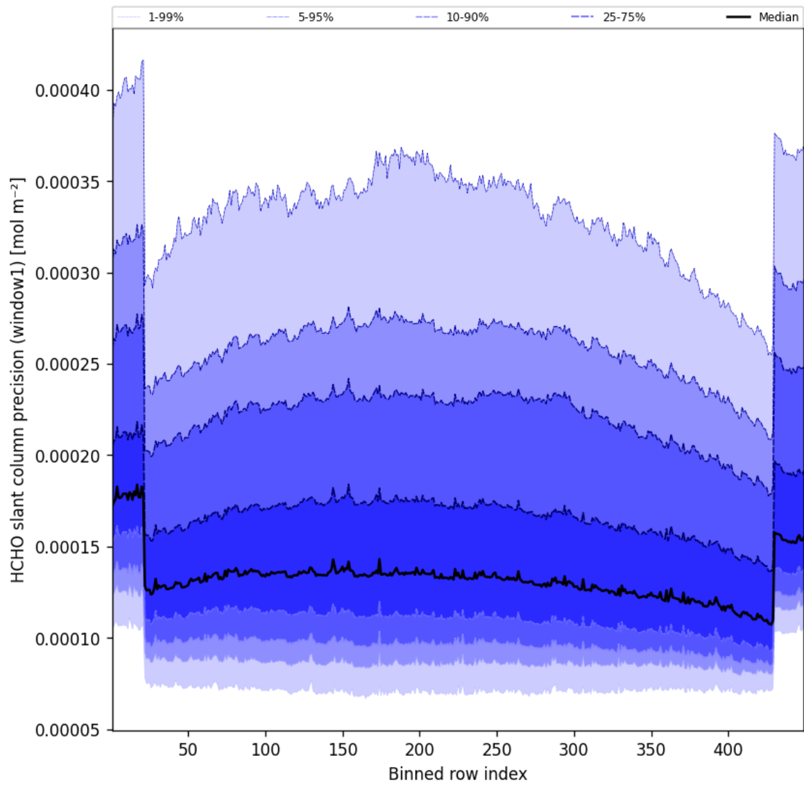
Figure 51: Along track statistics of “HCHO slant column precision (window1)” for 2025-08-26 to 2025-08-27
