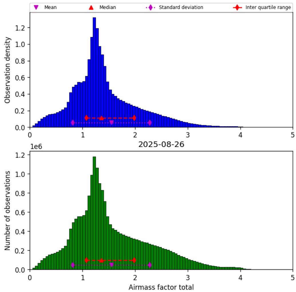
Figure 38: Histogram of “Airmass factor total” for 2025-08-26 to 2025-08-27
