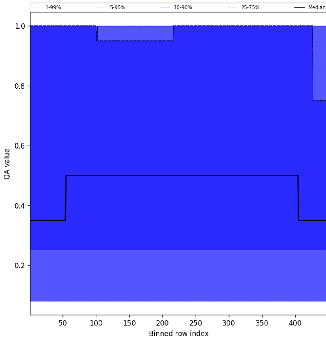
Figure 46: Along track statistics of “QA value” for 2025-08-26 to 2025-08-27
