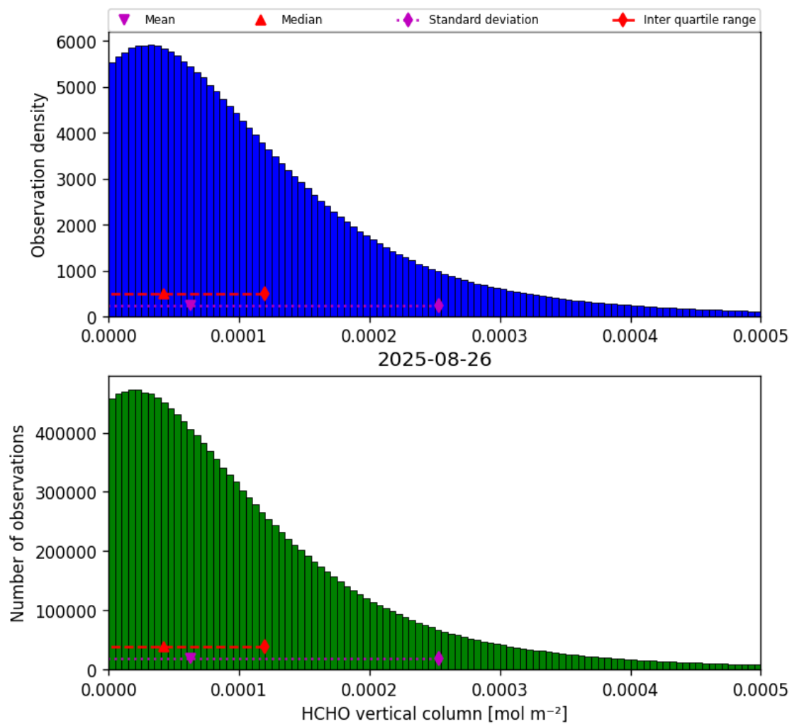
Figure 33: Histogram of “HCHO vertical column” for 2025-08-26 to 2025-08-27
