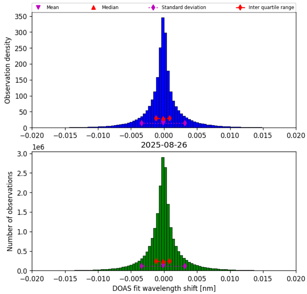
Figure 42: Histogram of “DOAS fit wavelength shift” for 2025-08-26 to 2025-08-27
