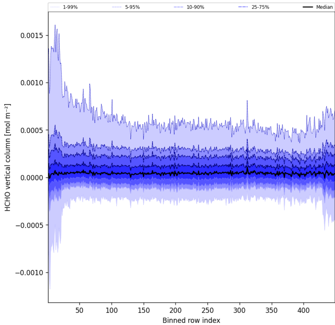
Figure 47: Along track statistics of “HCHO vertical column” for 2025-08-26 to 2025-08-27
