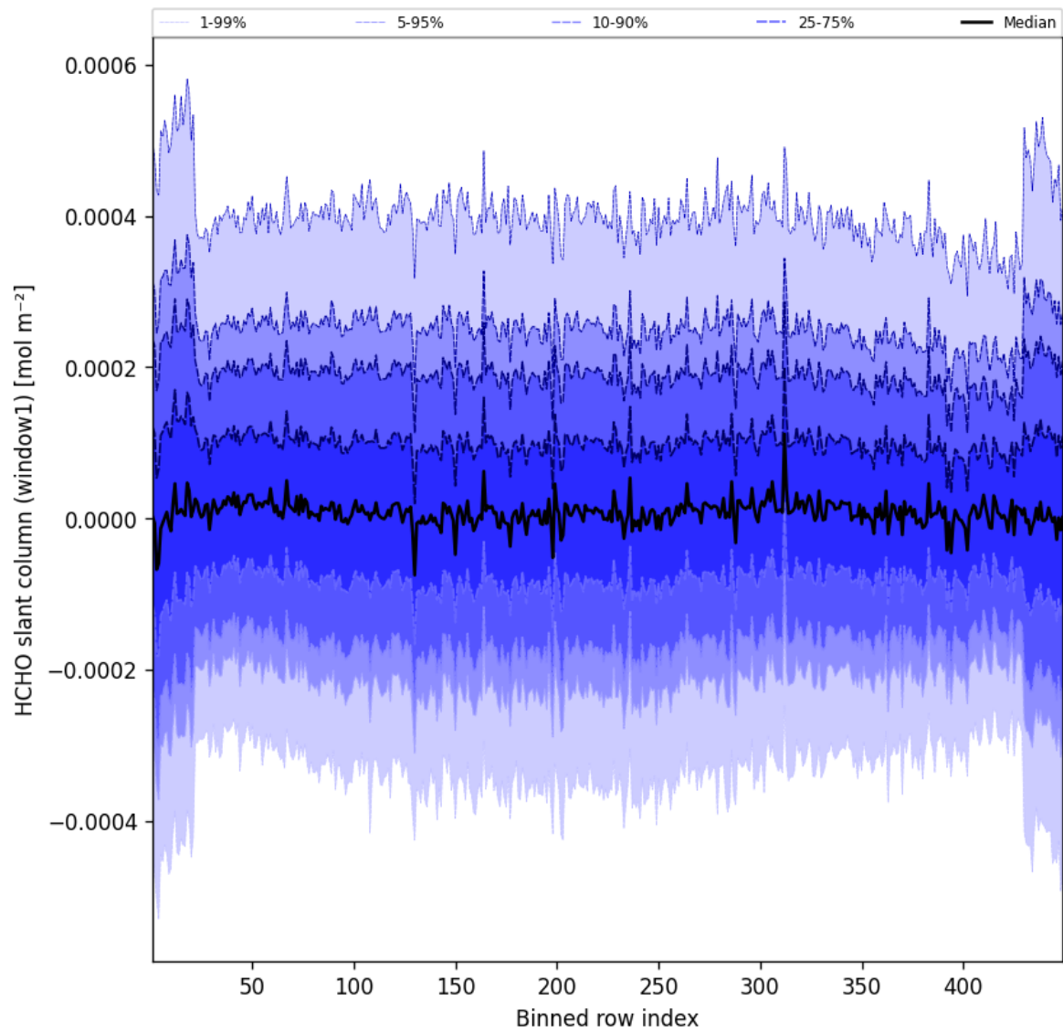
Figure 50: Along track statistics of “HCHO slant column (window1)” for 2025-08-26 to 2025-08-27
