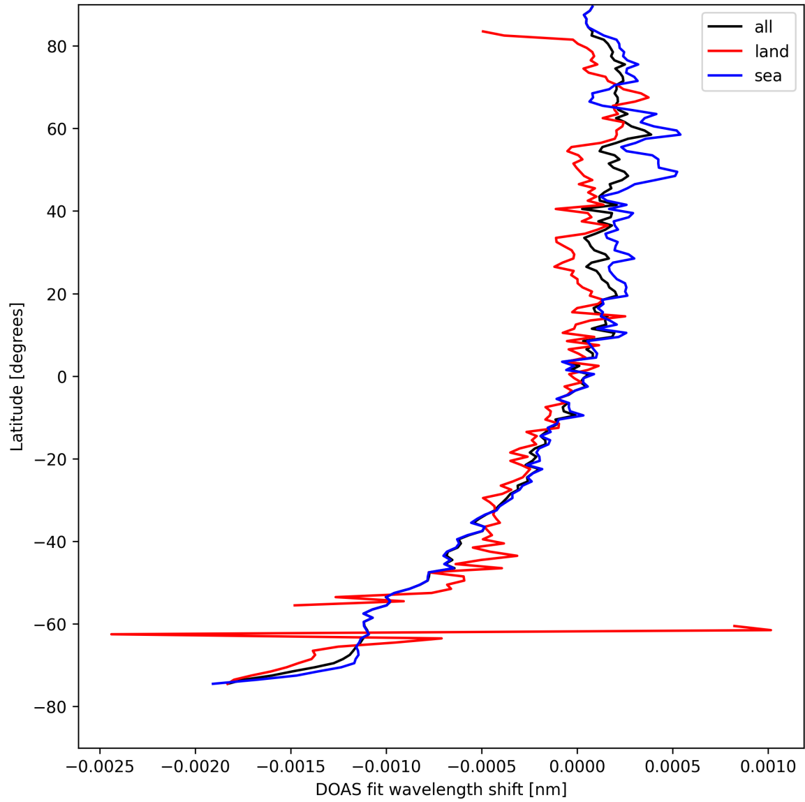
Figure 28: Zonal average of "DOAS fit wavelength shift" for 2025-08-26 to 2025-08-27.
