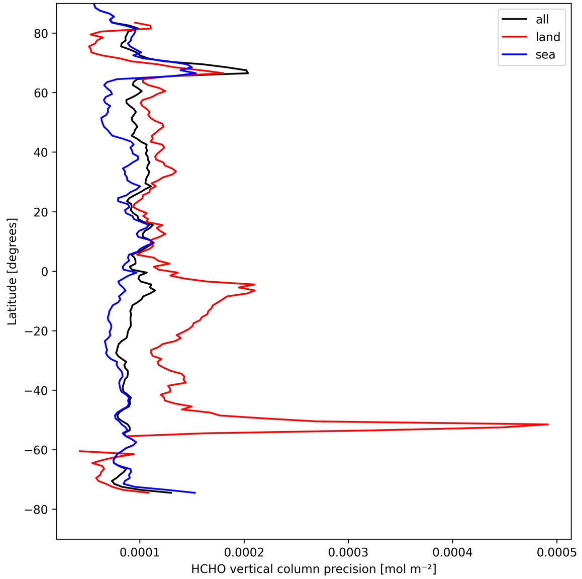
Figure 20: Zonal average of “HCHO vertical column precision” for 2025-08-26 to 2025-08-27.
