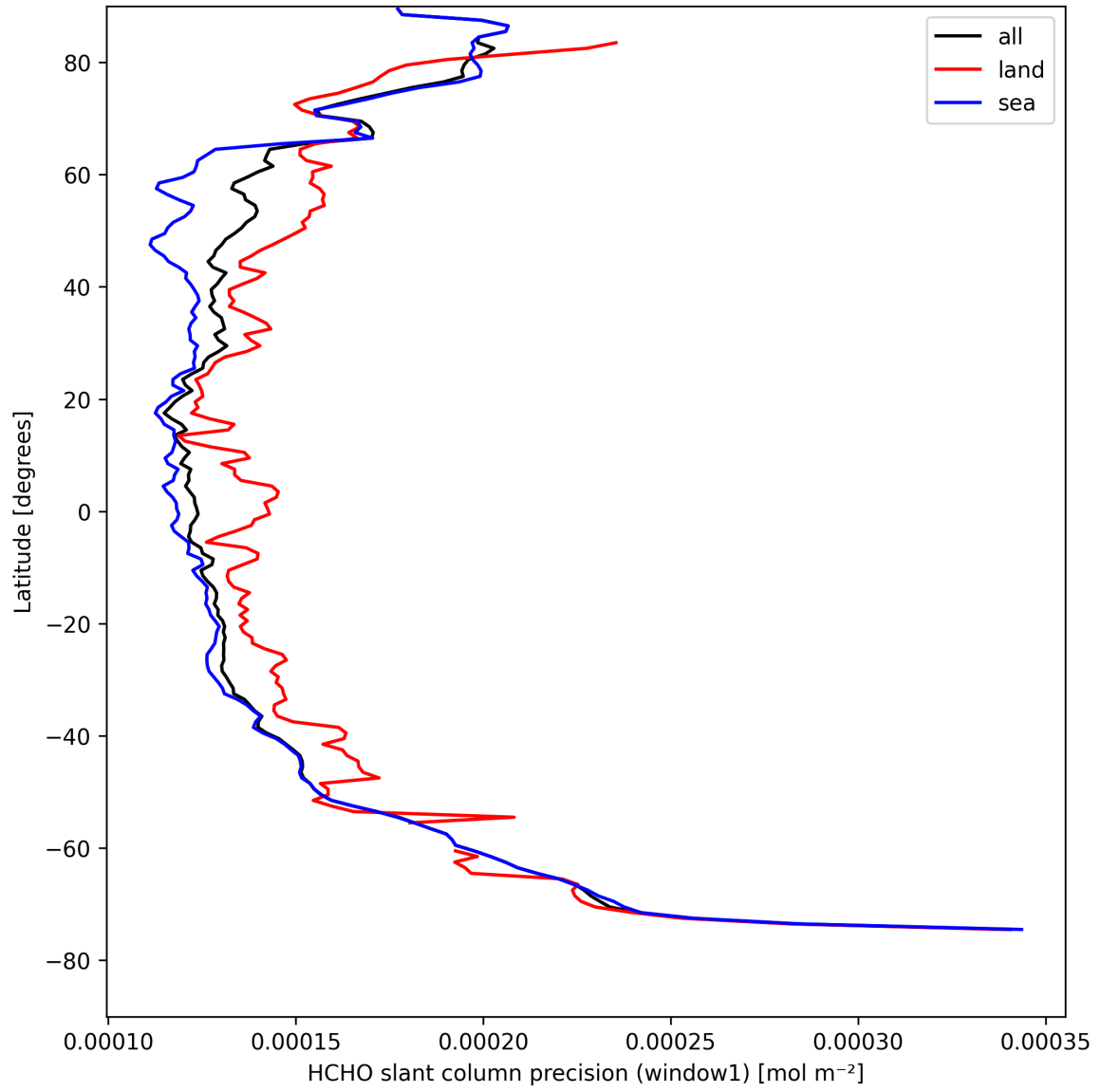
Figure 23: Zonal average of “HCHO slant column precision (window1)” for 2025-08-26 to 2025-08-27.
