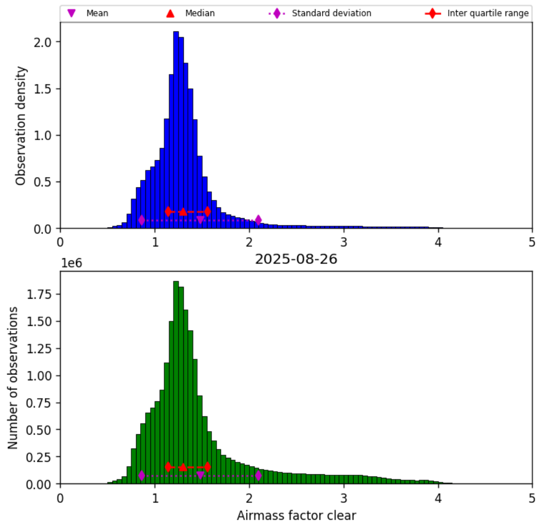
Figure 40: Histogram of “Airmass factor clear” for 2025-08-26 to 2025-08-27
