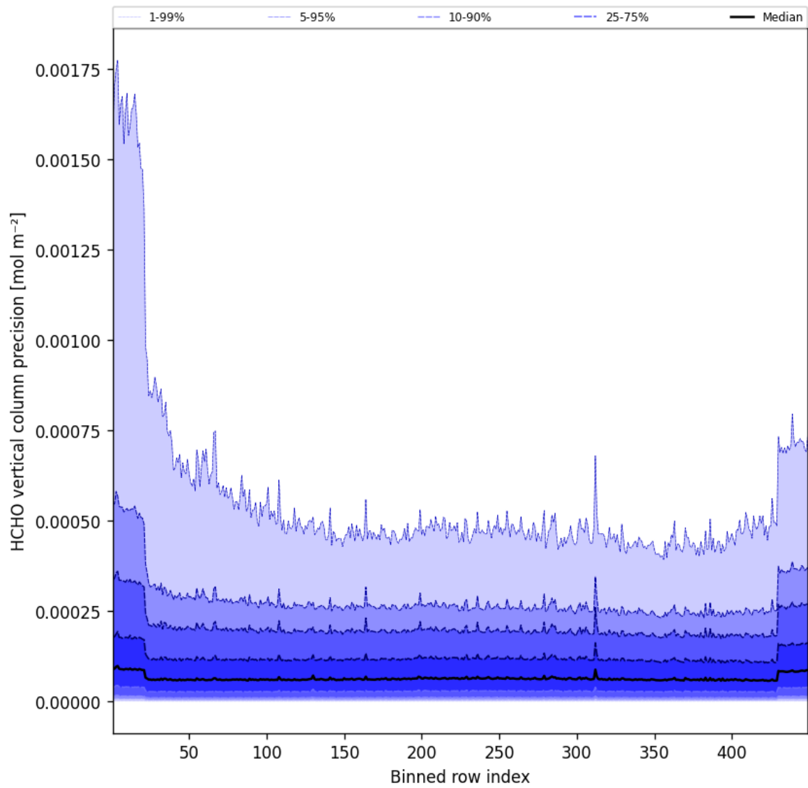
Figure 48: Along track statistics of “HCHO vertical column precision” for 2025-08-26 to 2025-08-27
