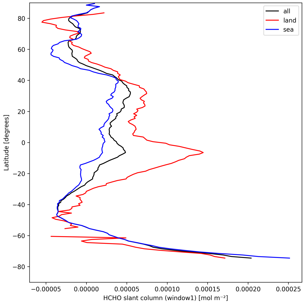
Figure 22: Zonal average of “HCHO slant column (window1)” for 2025-08-26 to 2025-08-27.
