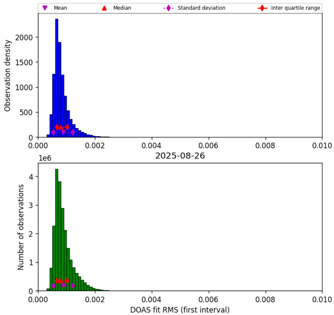
Figure 44: Histogram of “DOAS fit RMS (first interval)” for 2025-08-26 to 2025-08-27
