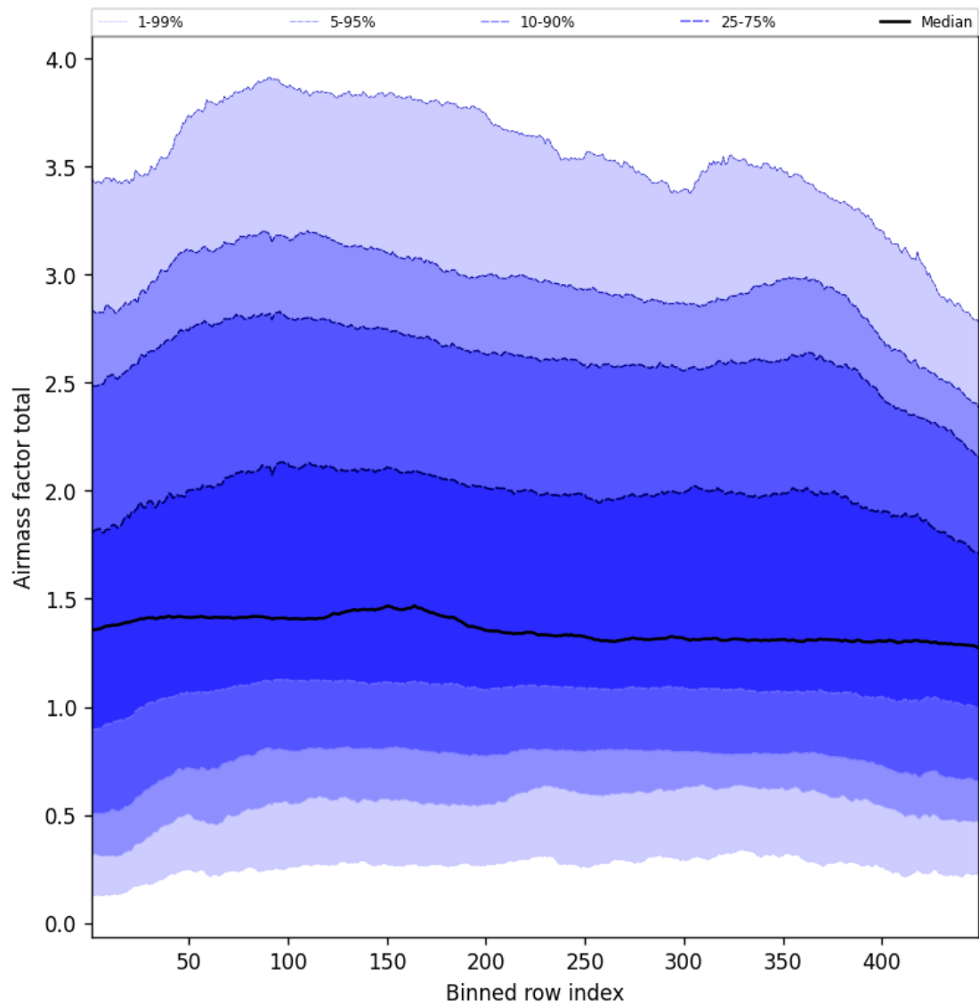
Figure 52: Along track statistics of “Airmass factor total” for 2025-08-26 to 2025-08-27
