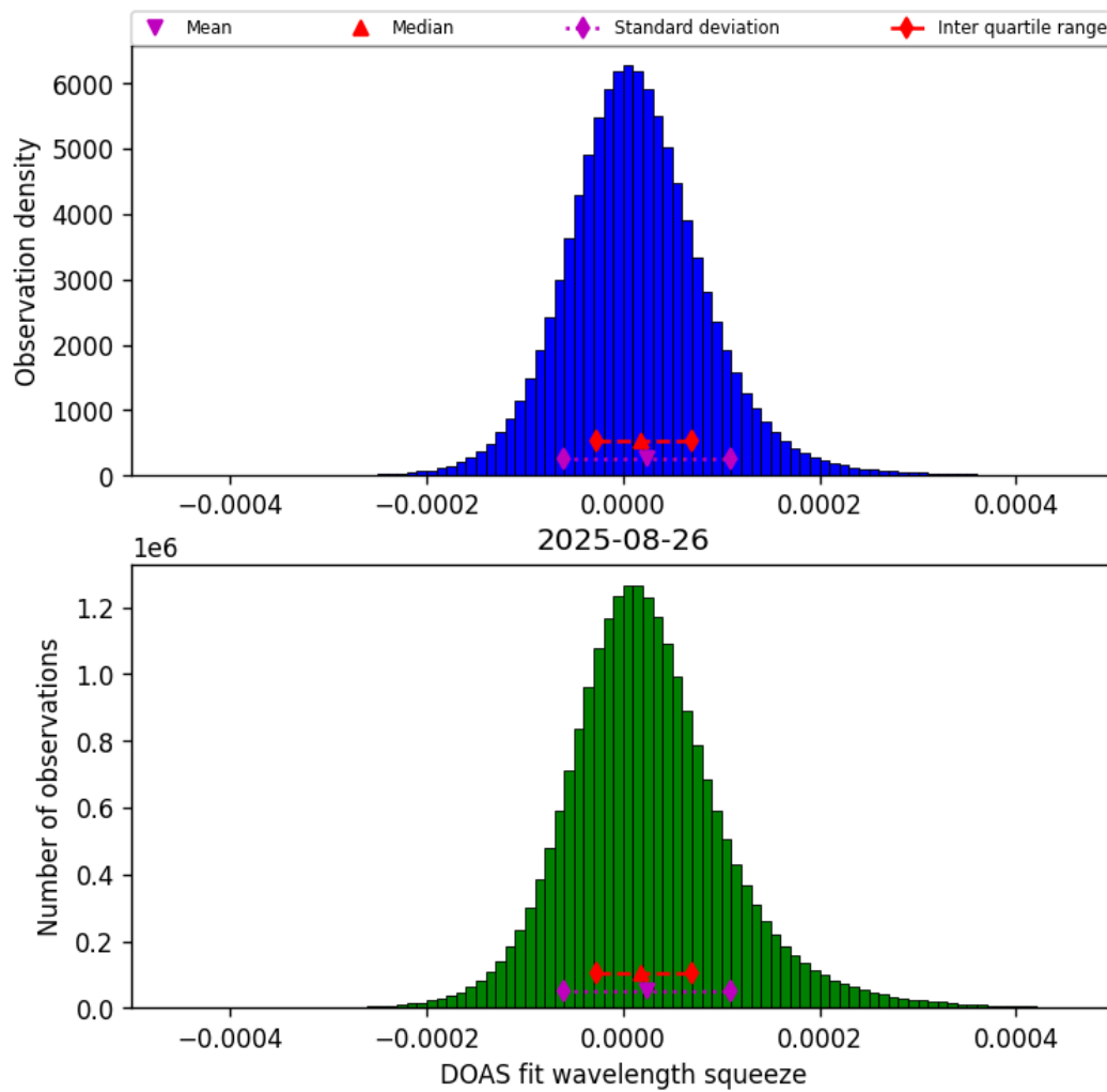
Figure 43: Histogram of “DOAS fit wavelength squeeze” for 2025-08-26 to 2025-08-27
