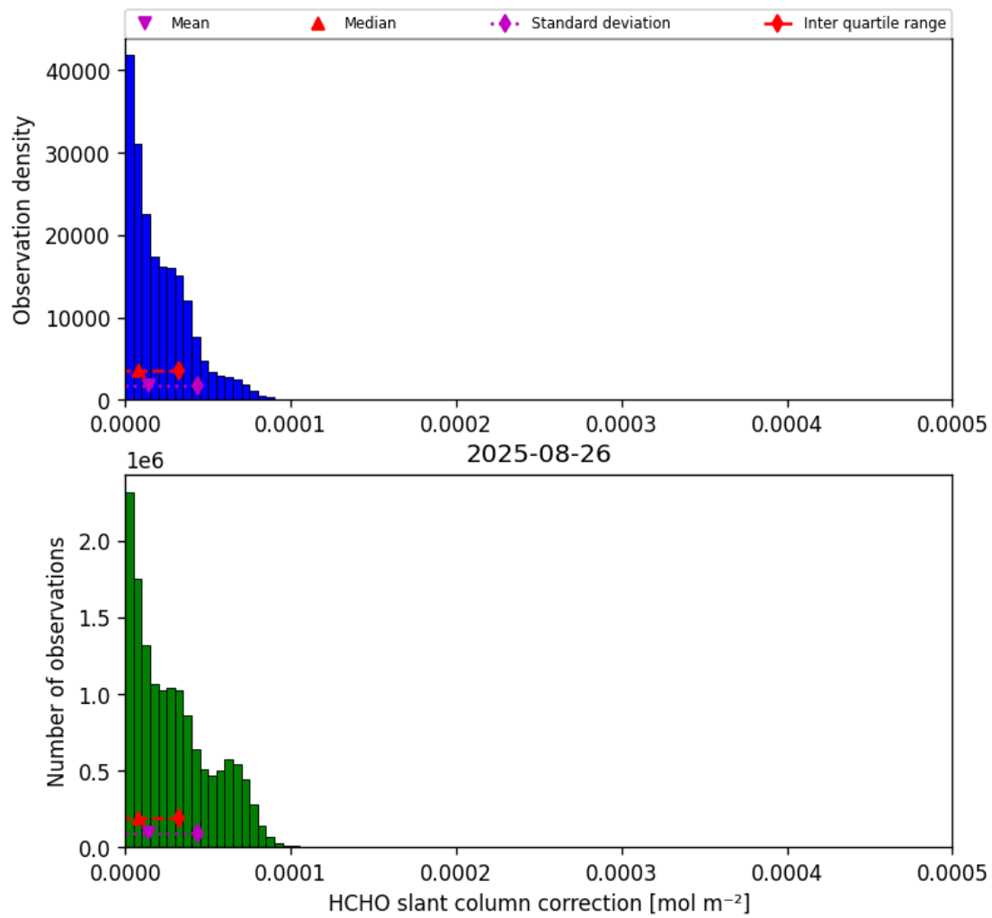
Figure 45: Histogram of “HCHO slant column correction” for 2025-08-26 to 2025-08-27
