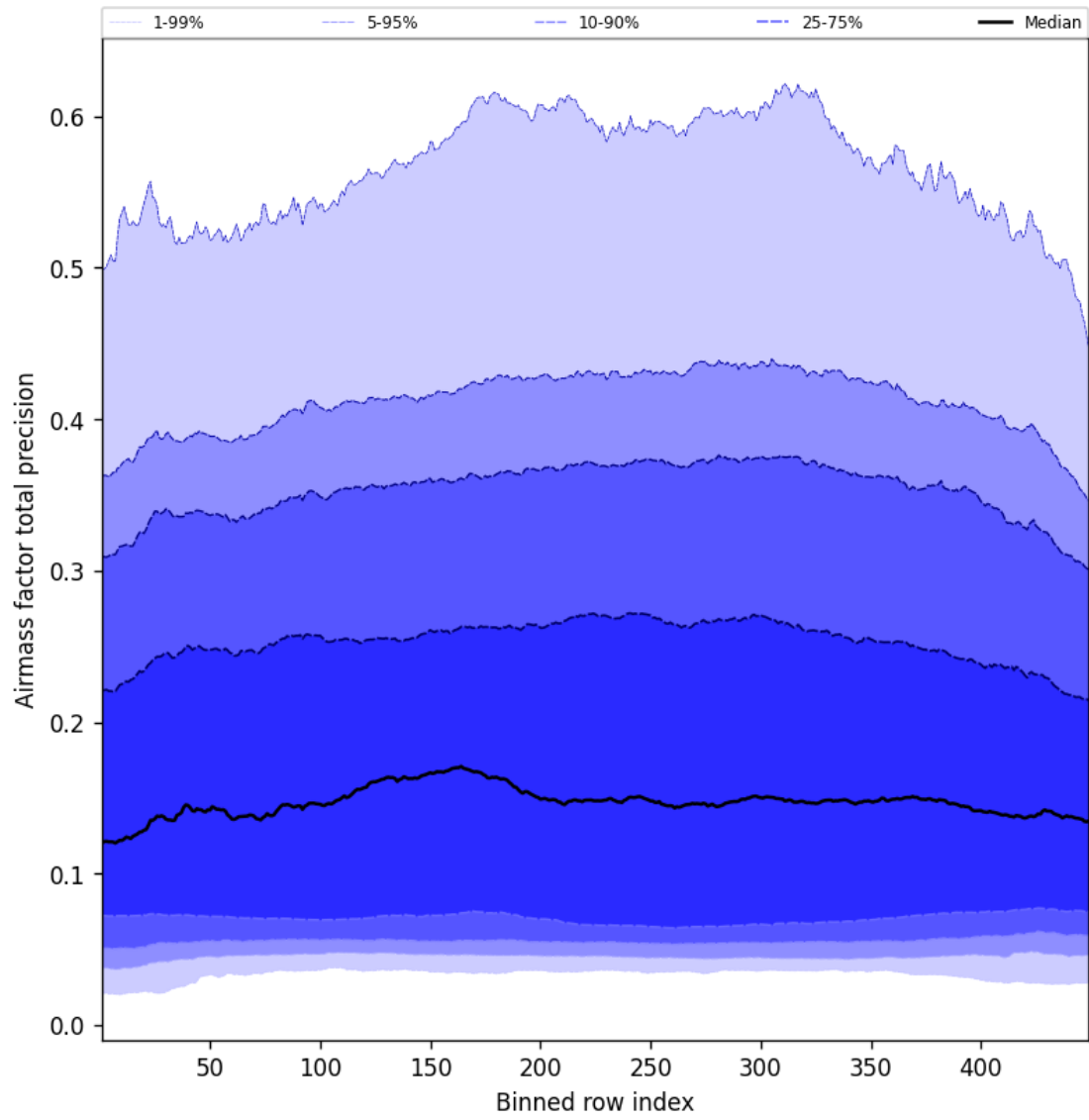
Figure 53: Along track statistics of “Airmass factor total precision” for 2025-08-26 to 2025-08-27
