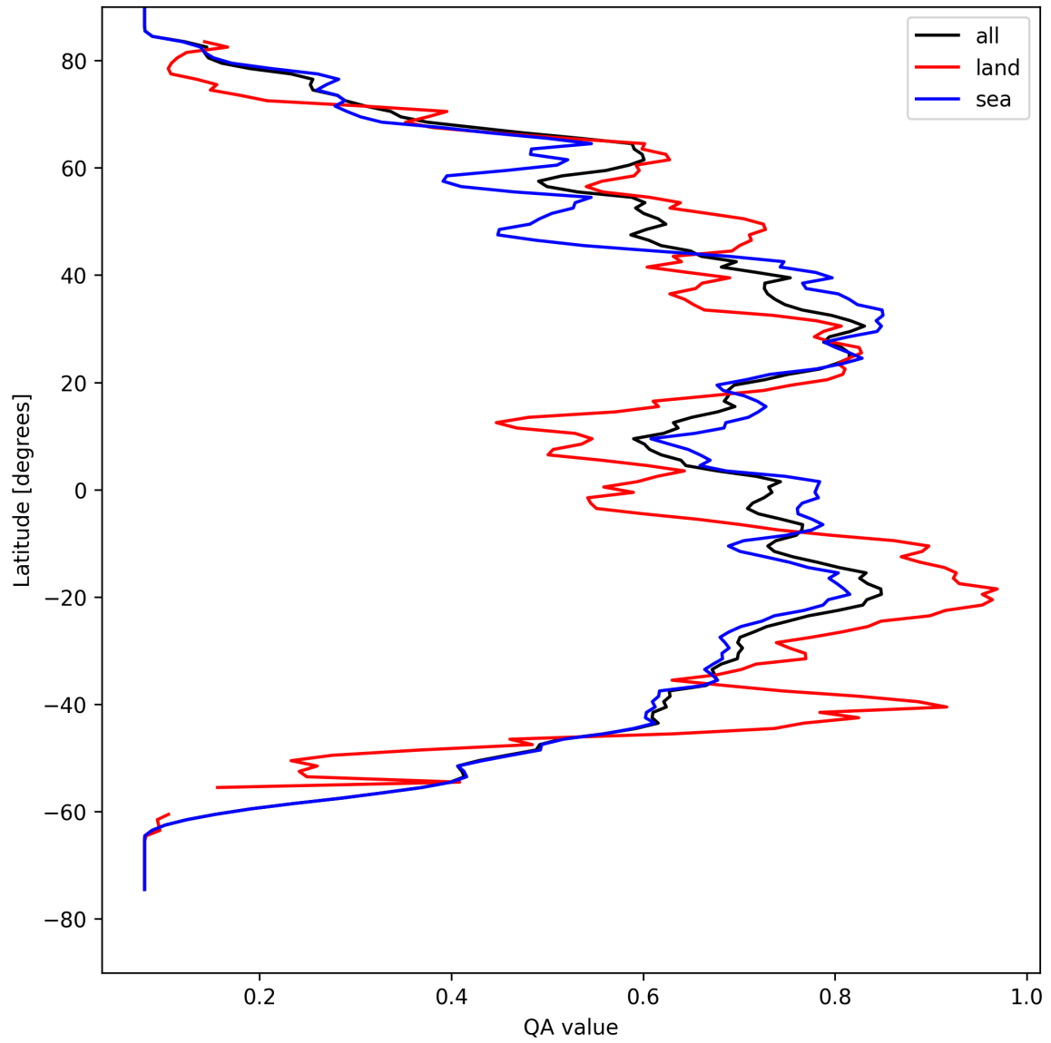
Figure 18: Zonal average of “QA value” for 2025-08-26 to 2025-08-27.
