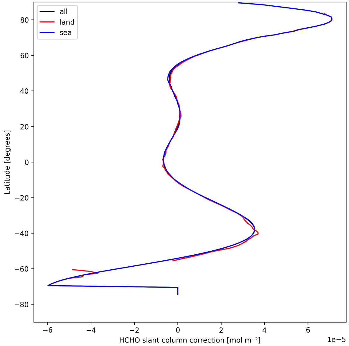
Figure 31: Zonal average of “HCHO slant column correction” for 2025-08-26 to 2025-08-27.
