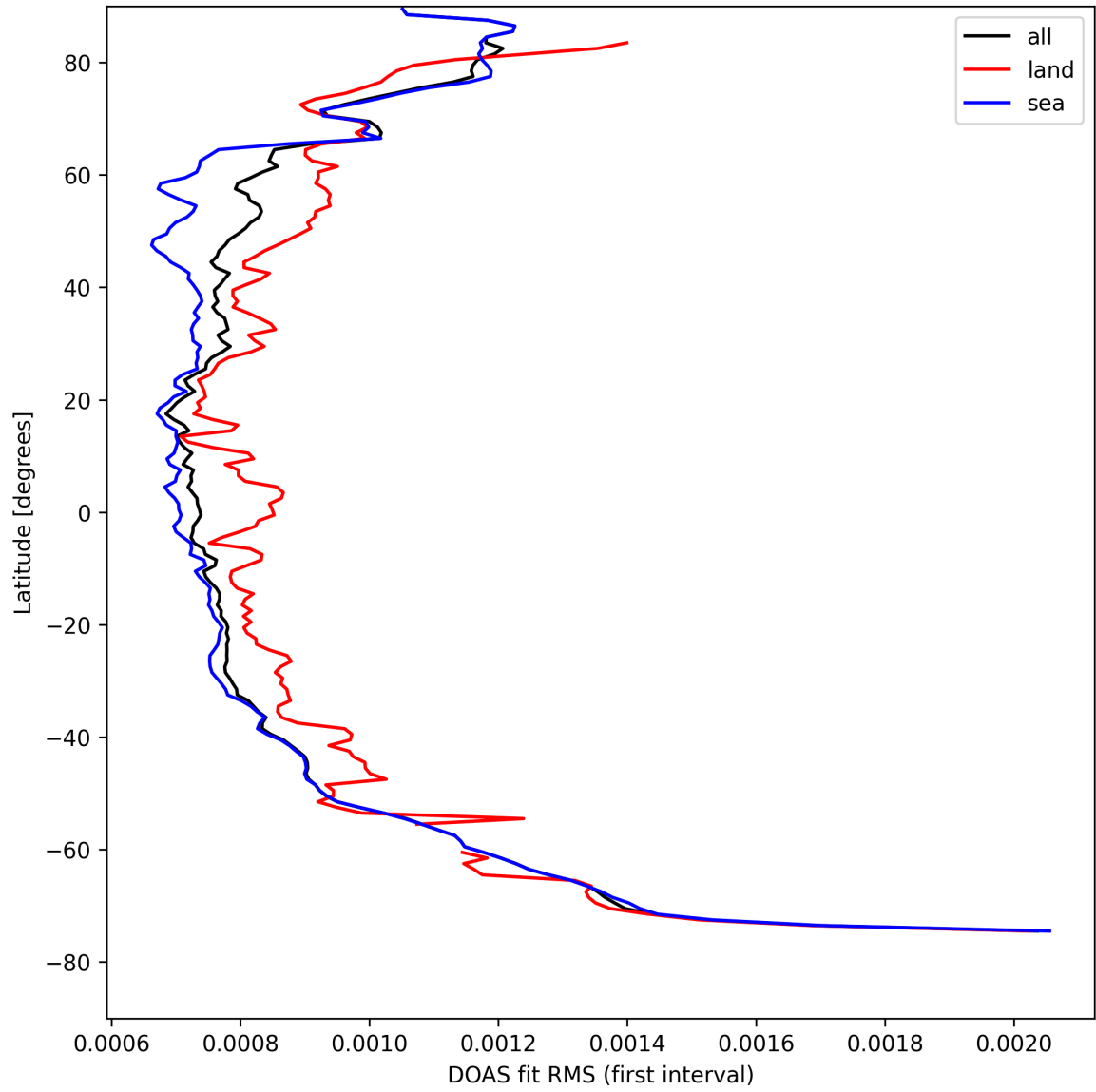
Figure 30: Zonal average of “DOAS fit RMS (first interval)” for 2025-08-26 to 2025-08-27.
