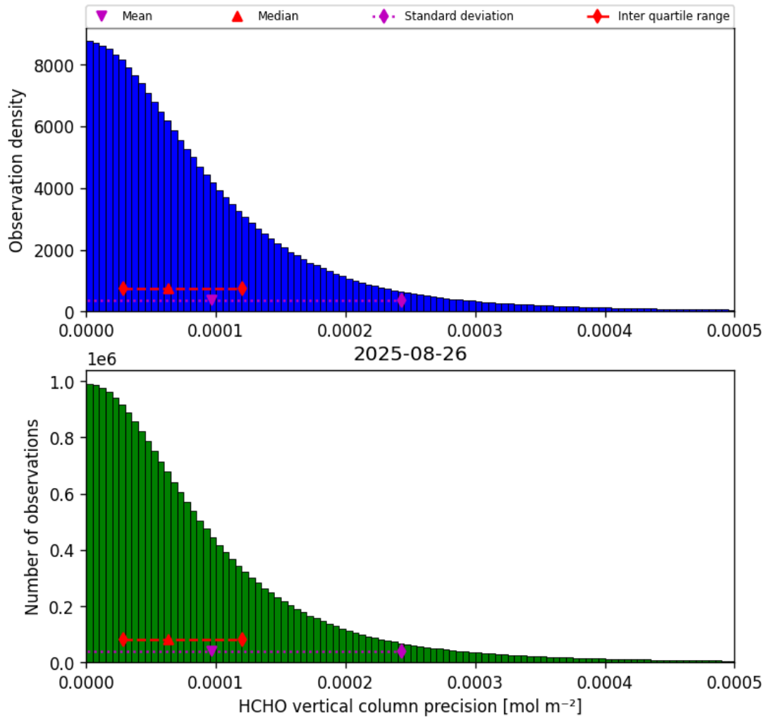
Figure 34: Histogram of “HCHO vertical column precision” for 2025-08-26 to 2025-08-27
