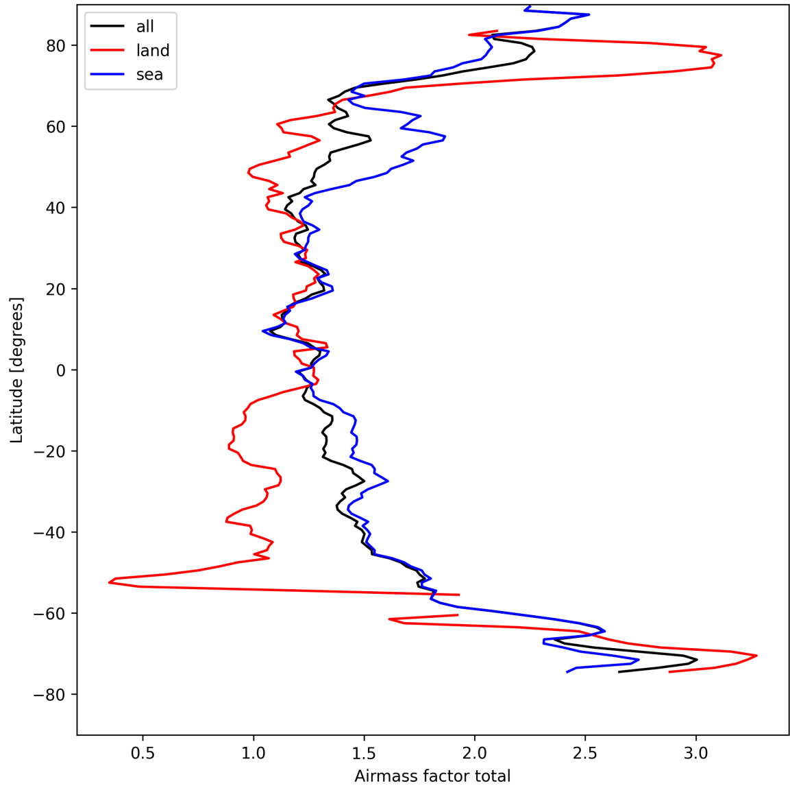
Figure 24: Zonal average of “Airmass factor total” for 2025-08-26 to 2025-08-27.
