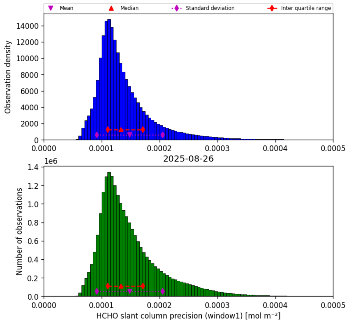
Figure 37: Histogram of “HCHO slant column precision (window1)” for 2025-08-26 to 2025-08-27
