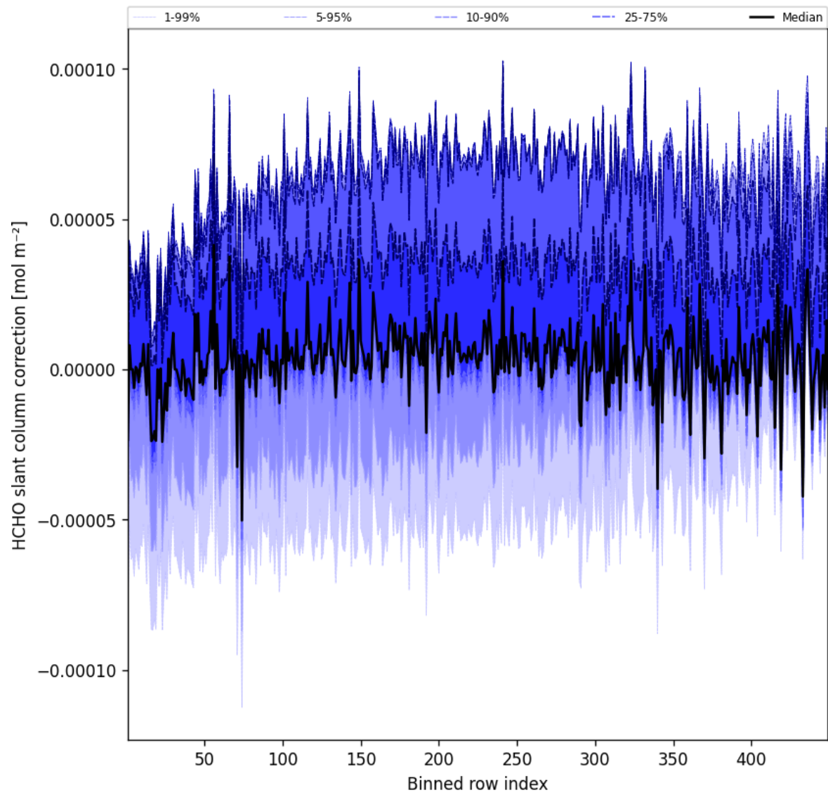
Figure 59: Along track statistics of “HCHO slant column correction” for 2025-08-26 to 2025-08-27
