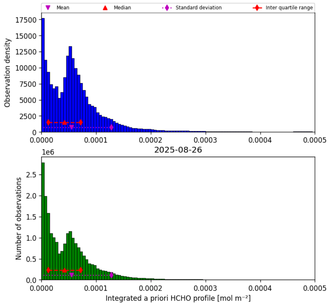
Figure 41: Histogram of “Integrated a priori HCHO profile” for 2025-08-26 to 2025-08-27
