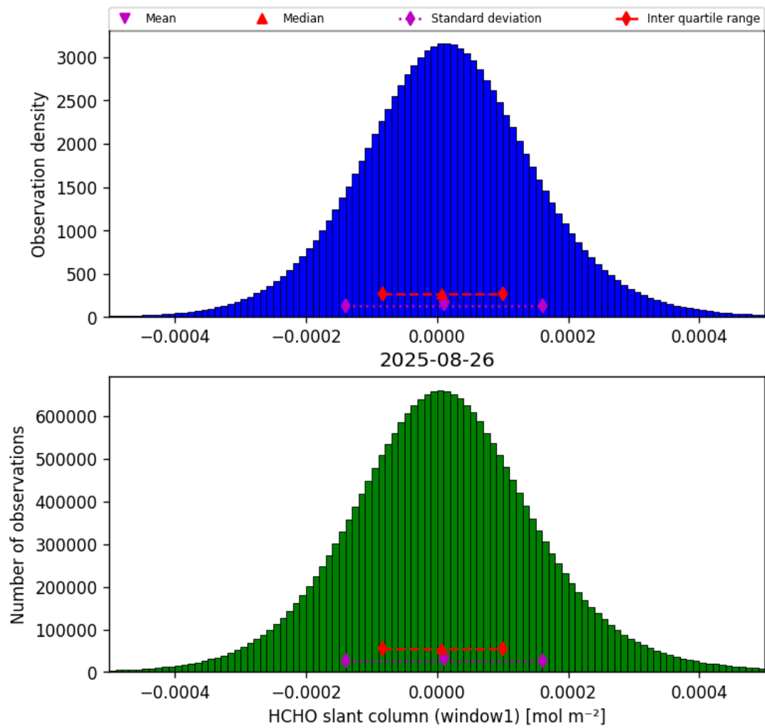
Figure 36: Histogram of “HCHO slant column (window1)” for 2025-08-26 to 2025-08-27
