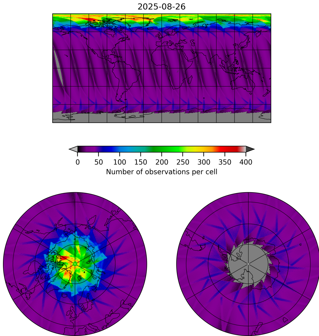
Figure 17: Map of the number of observations for 2025-08-26 to 2025-08-27
