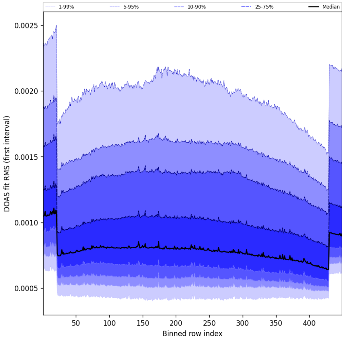
Figure 58: Along track statistics of “DOAS fit RMS (first interval)” for 2025-08-26 to 2025-08-27
