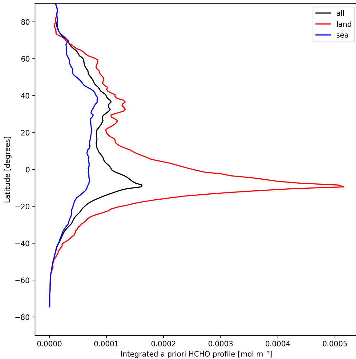
Figure 27: Zonal average of “Integrated a priori HCHO profile” for 2025-08-26 to 2025-08-27.
