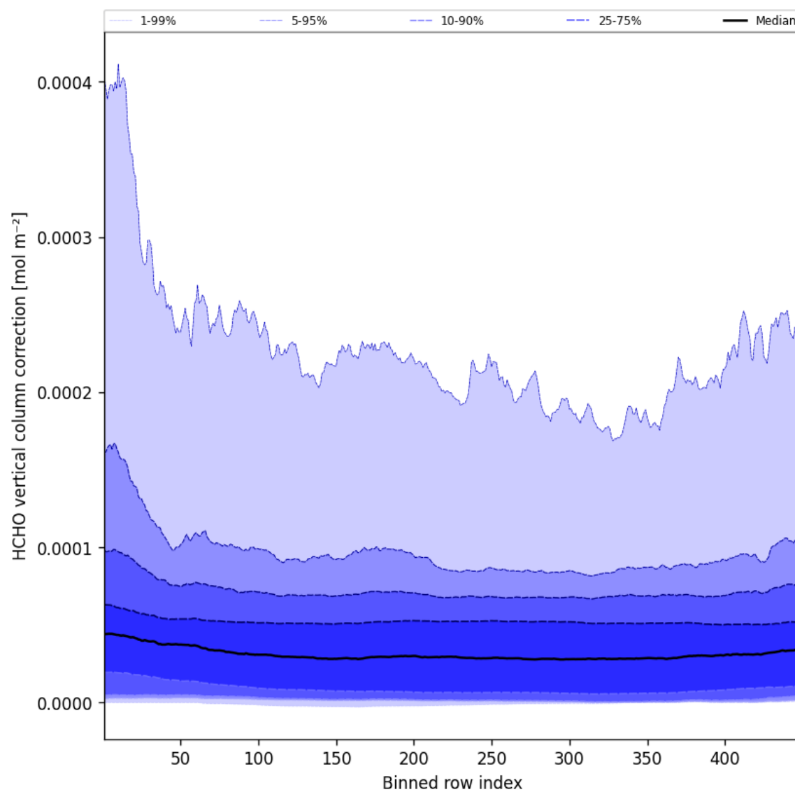
Figure 49: Along track statistics of “HCHO vertical column correction” for 2025-08-26 to 2025-08-27
