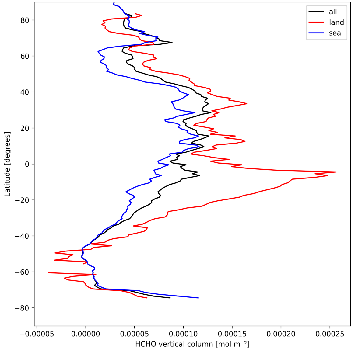
Figure 19: Zonal average of “HCHO vertical column” for 2025-08-26 to 2025-08-27.
