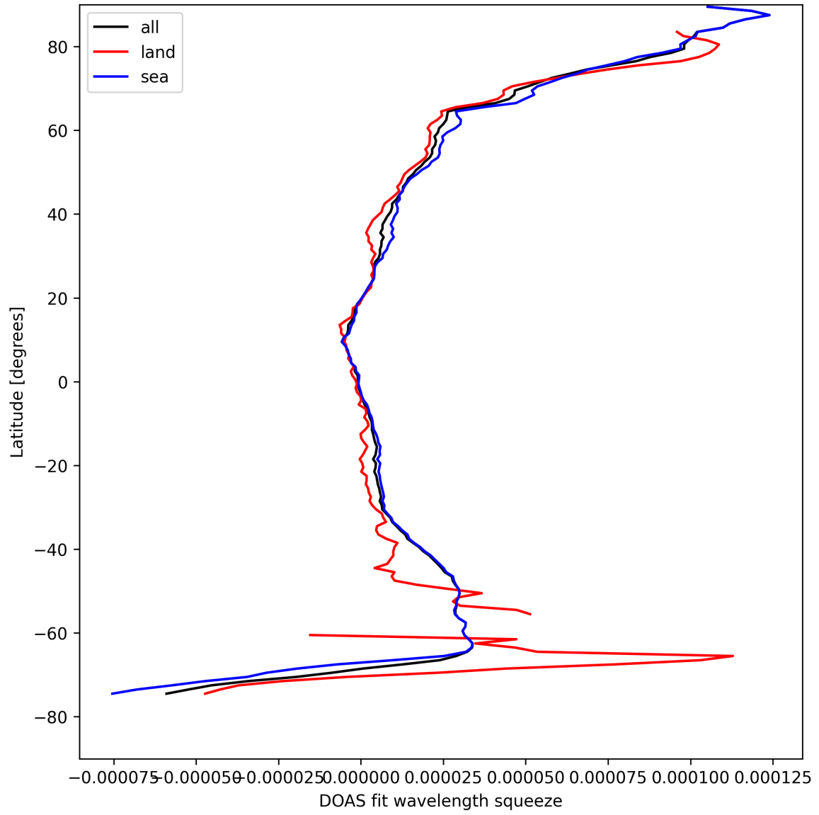
Figure 29: Zonal average of “DOAS fit wavelength squeeze” for 2025-08-26 to 2025-08-27.
