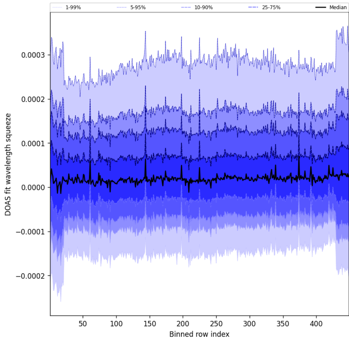
Figure 57: Along track statistics of “DOAS fit wavelength squeeze” for 2025-08-26 to 2025-08-27
