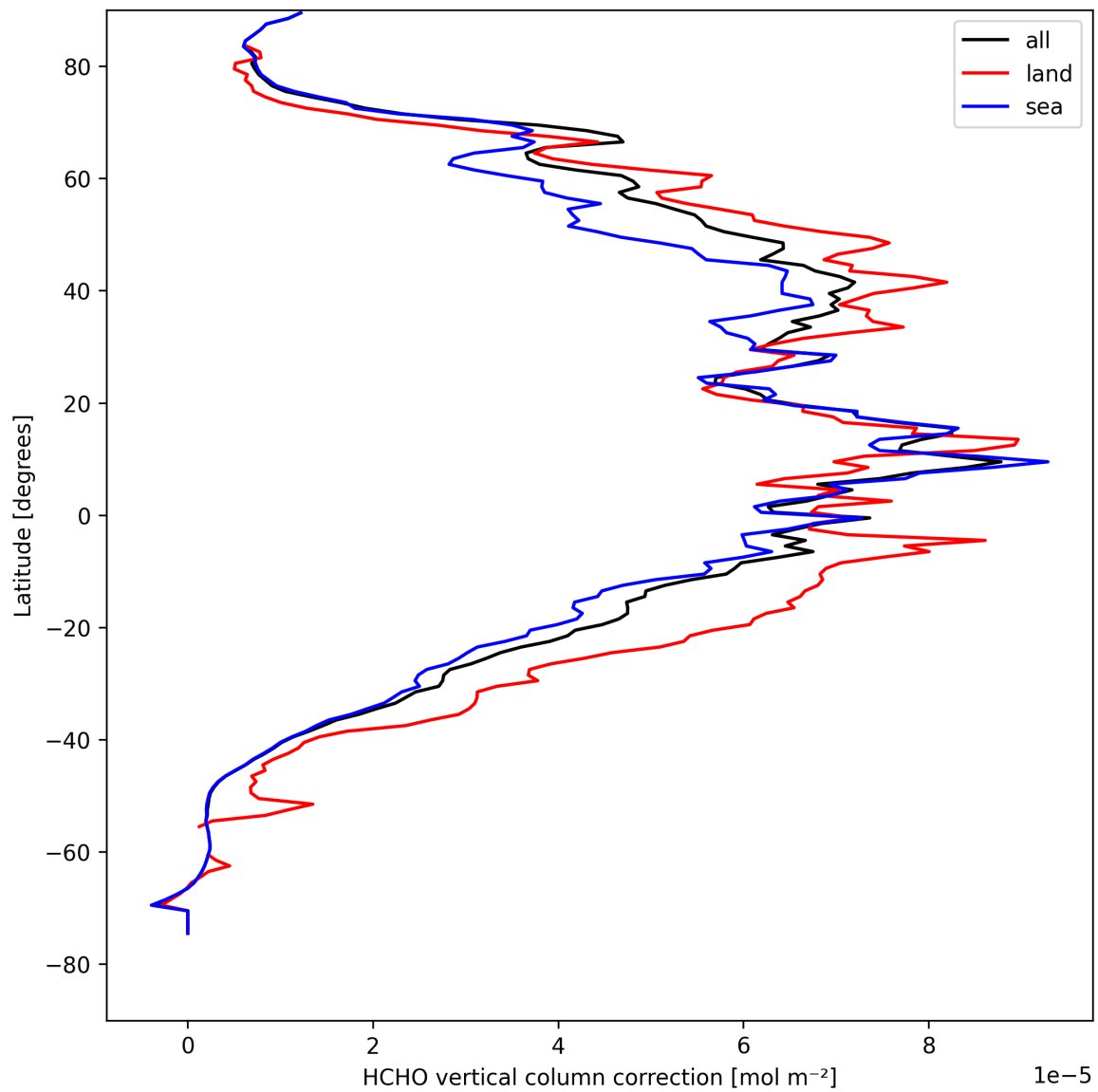
Figure 21: Zonal average of “HCHO vertical column correction” for 2025-08-26 to 2025-08-27.
