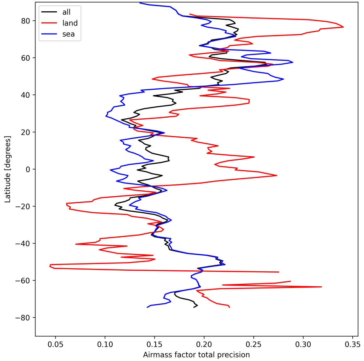
Figure 25: Zonal average of “Airmass factor total precision” for 2025-08-26 to 2025-08-27.
