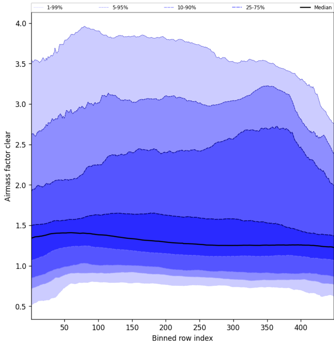
Figure 54: Along track statistics of “Airmass factor clear” for 2025-08-26 to 2025-08-27
