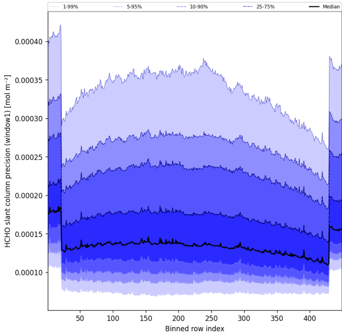
Figure 51: Along track statistics of “HCHO slant column precision (window1)” for 2025-08-27 to 2025-08-28
