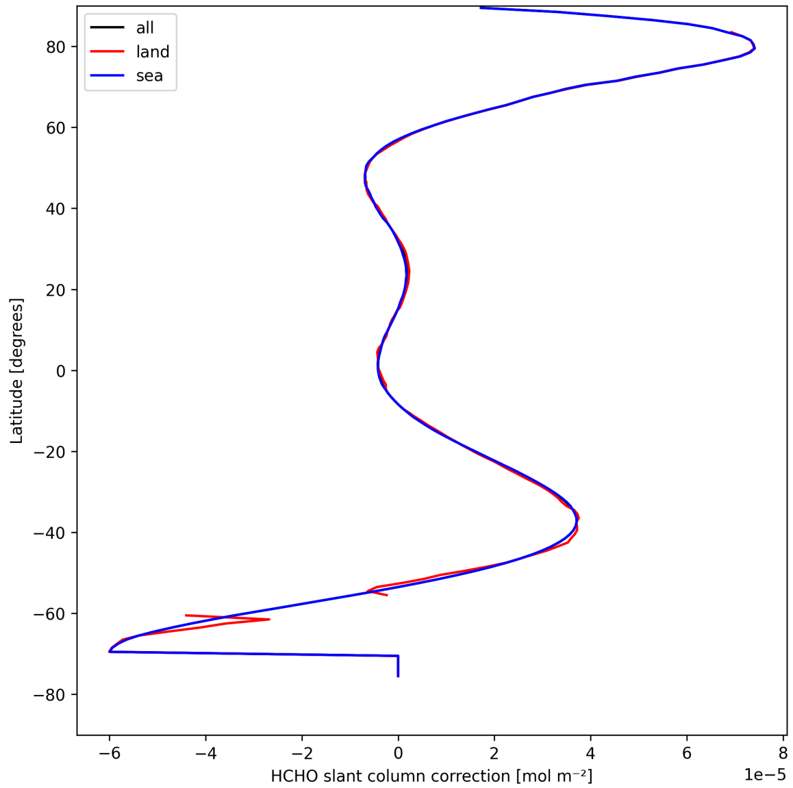
Figure 31: Zonal average of "HCHO slant column correction" for 2025-08-27 to 2025-08-28.
