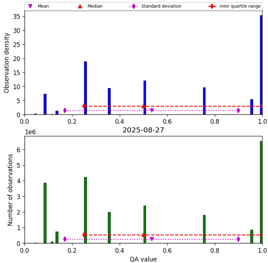
Figure 32: Histogram of “QA value” for 2025-08-27 to 2025-08-28
