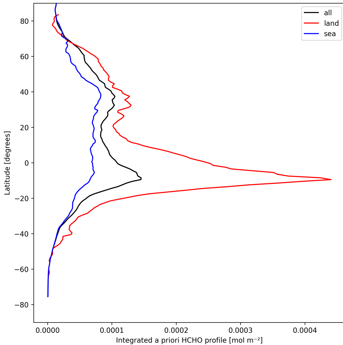
Figure 27: Zonal average of “Integrated a priori HCHO profile” for 2025-08-27 to 2025-08-28.
