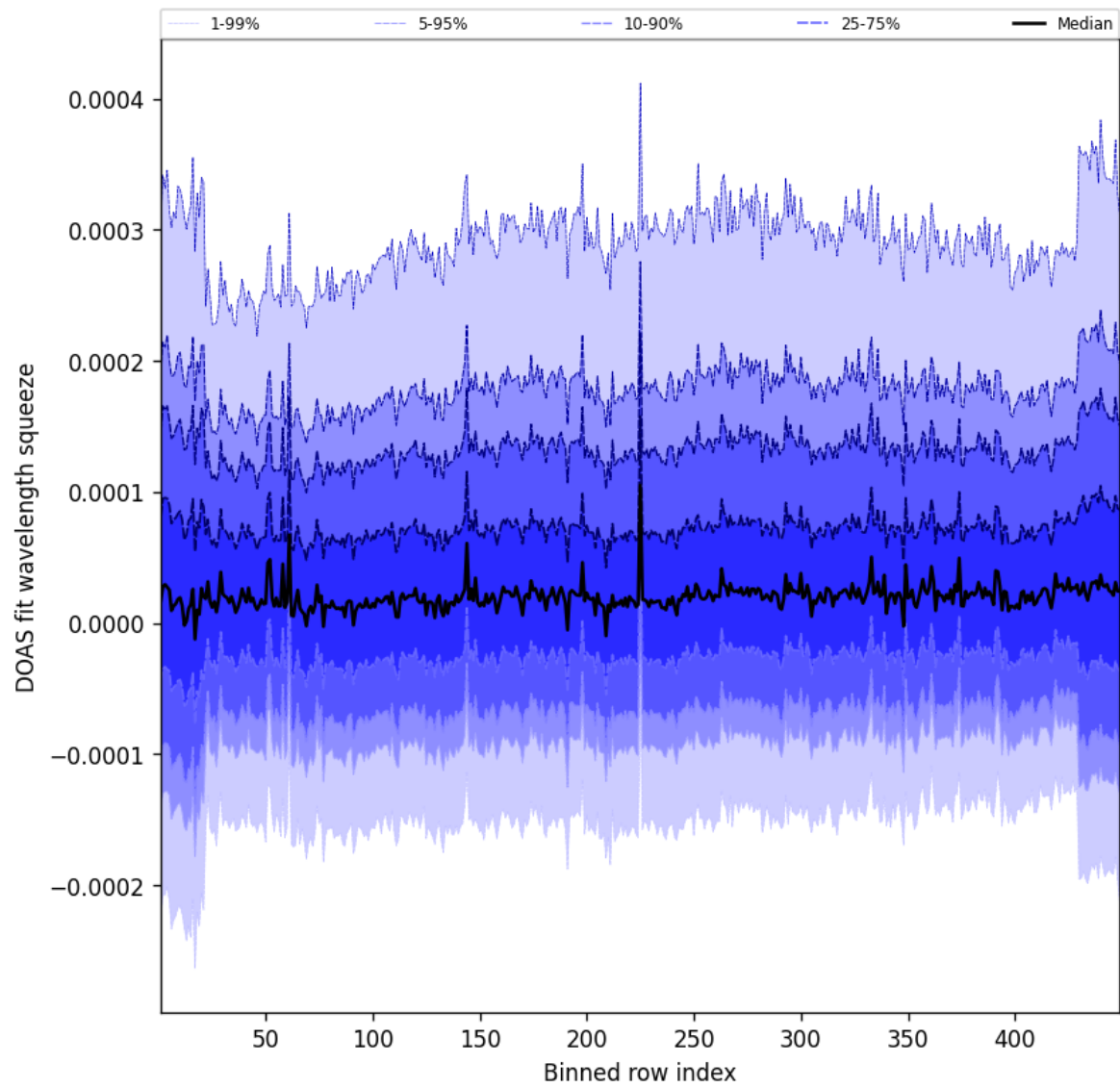
Figure 57: Along track statistics of “DOAS fit wavelength squeeze” for 2025-08-27 to 2025-08-28
