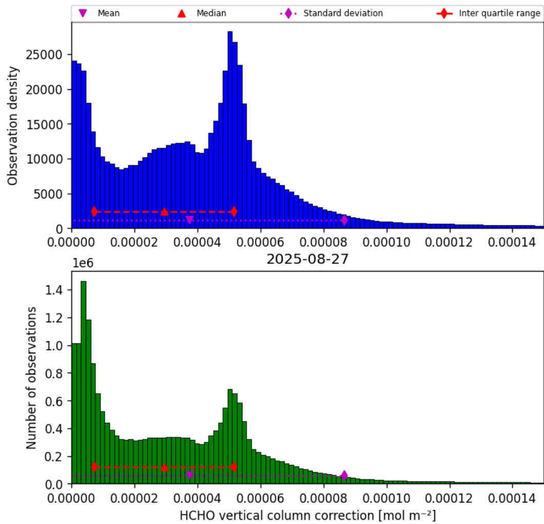
Figure 35: Histogram of “HCHO vertical column correction” for 2025-08-27 to 2025-08-28
