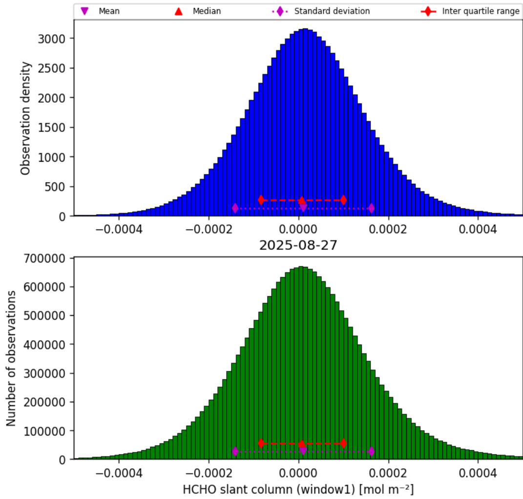
Figure 36: Histogram of “HCHO slant column (window1)” for 2025-08-27 to 2025-08-28
