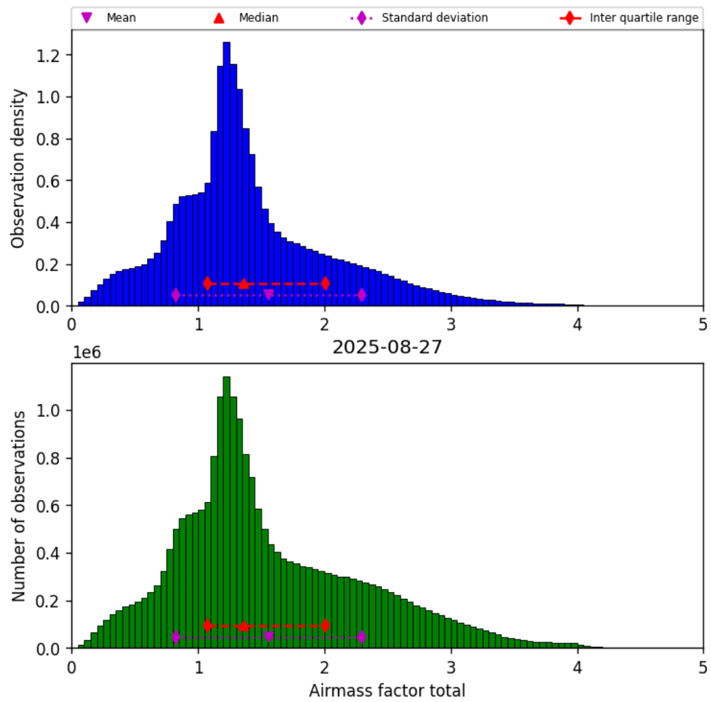
Figure 38: Histogram of “Airmass factor total” for 2025-08-27 to 2025-08-28
