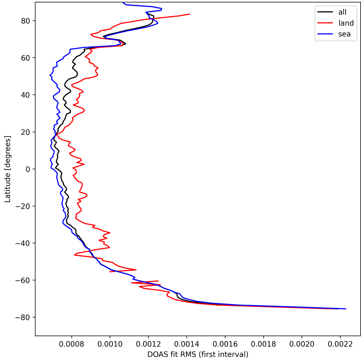
Figure 30: Zonal average of “DOAS fit RMS (first interval)” for 2025-08-27 to 2025-08-28.
