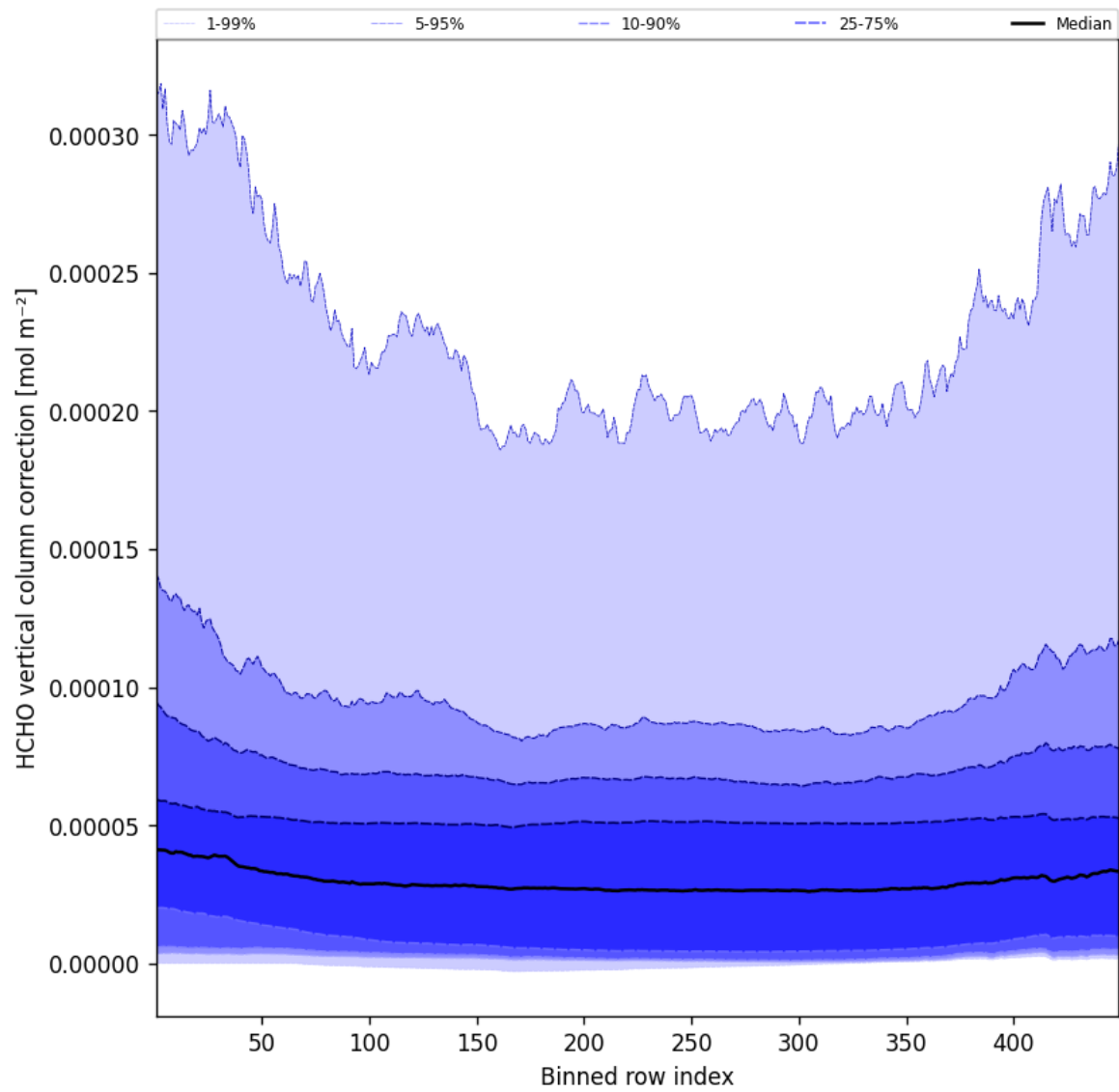
Figure 49: Along track statistics of “HCHO vertical column correction” for 2025-08-27 to 2025-08-28
