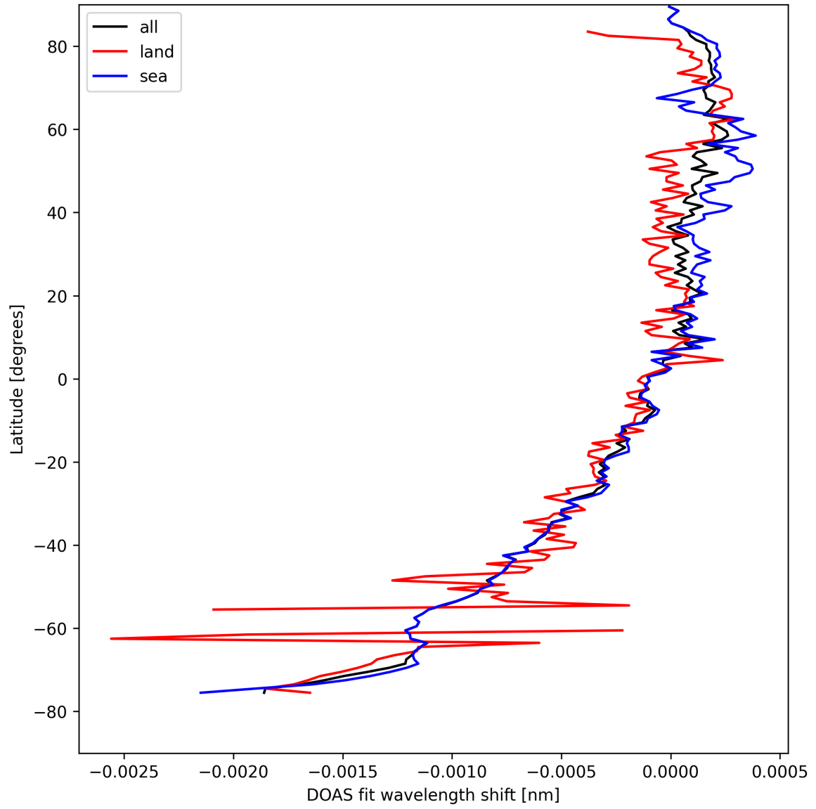
Figure 28: Zonal average of “DOAS fit wavelength shift” for 2025-08-27 to 2025-08-28.
