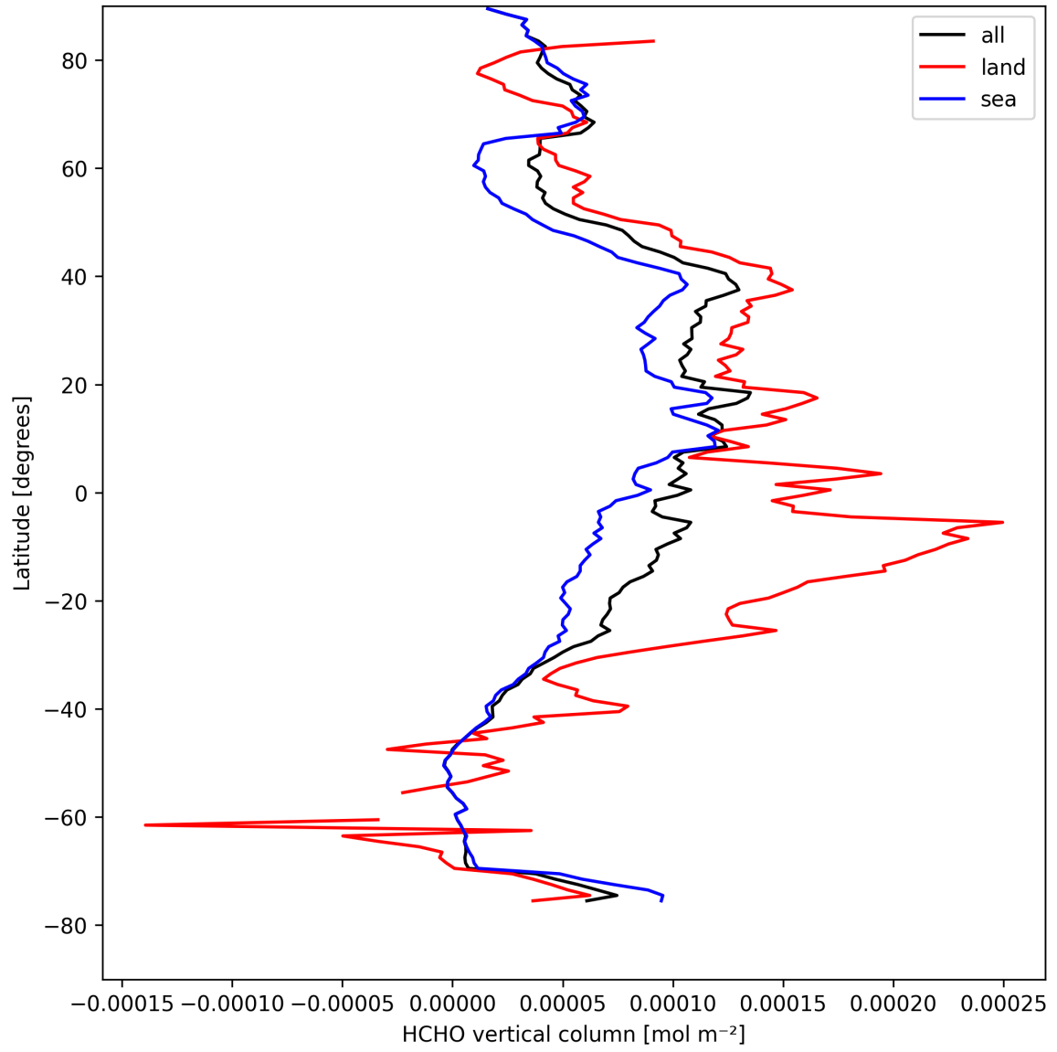
Figure 19: Zonal average of “HCHO vertical column” for 2025-08-27 to 2025-08-28.
