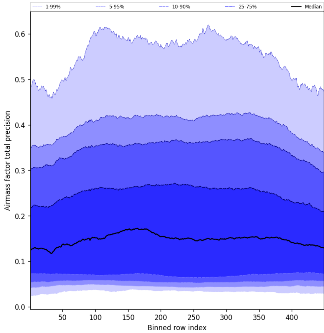
Figure 53: Along track statistics of “Airmass factor total precision” for 2025-08-27 to 2025-08-28
