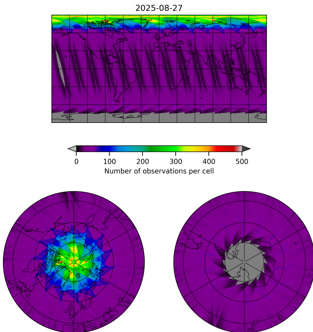
Figure 17: Map of the number of observations for 2025-08-27 to 2025-08-28
