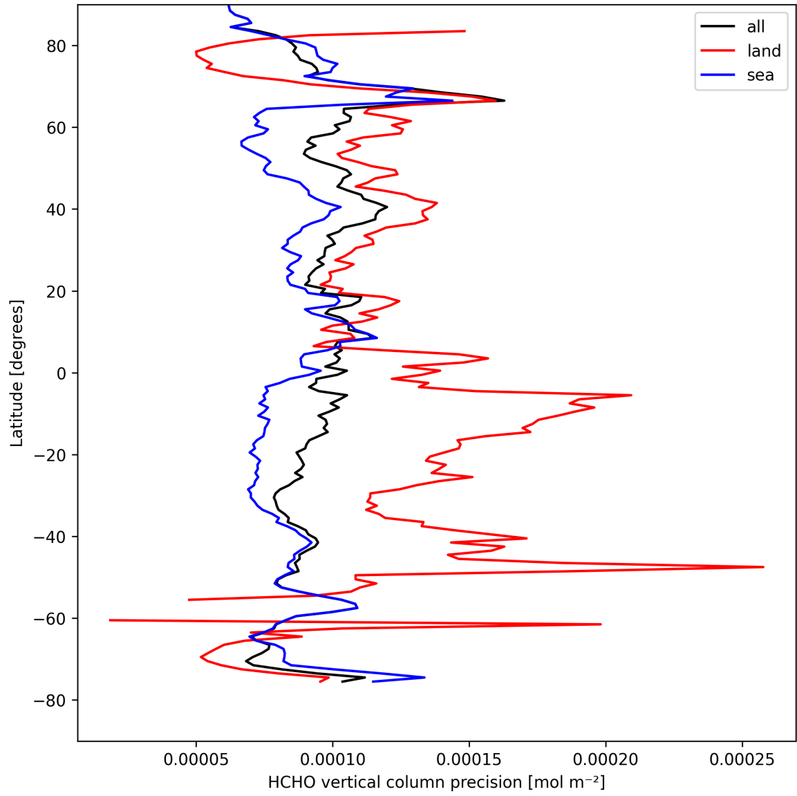
Figure 20: Zonal average of “HCHO vertical column precision” for 2025-08-27 to 2025-08-28.
