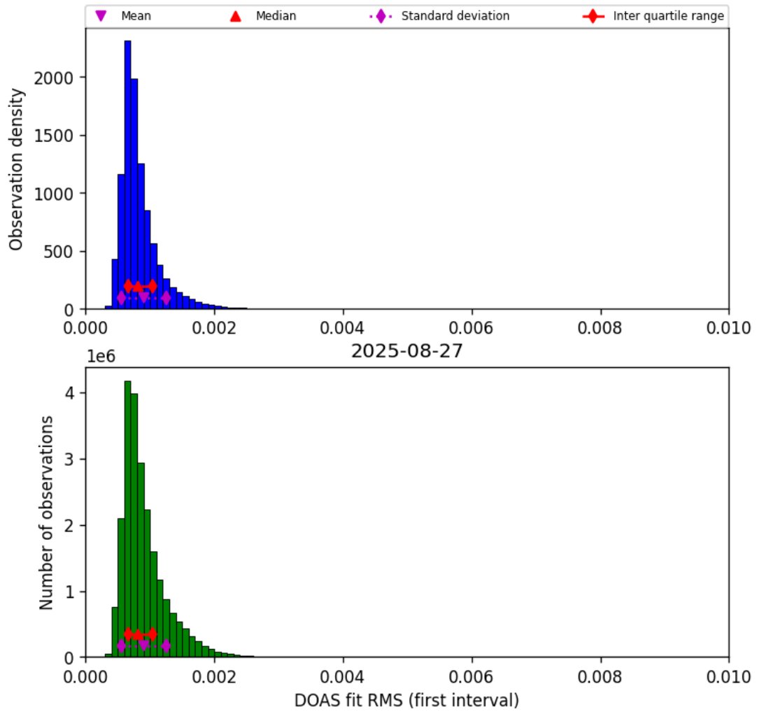
Figure 44: Histogram of “DOAS fit RMS (first interval)” for 2025-08-27 to 2025-08-28
