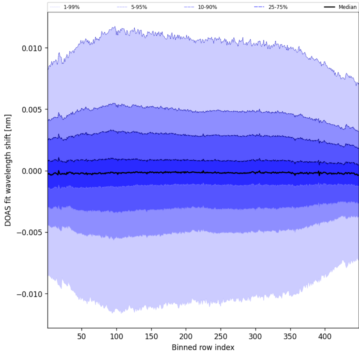
Figure 56: Along track statistics of “DOAS fit wavelength shift” for 2025-08-27 to 2025-08-28
