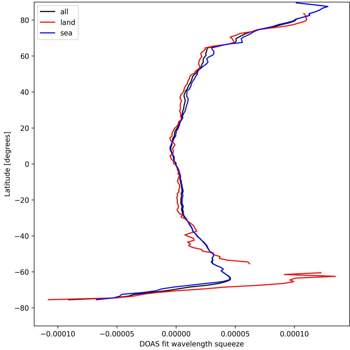
Figure 29: Zonal average of “DOAS fit wavelength squeeze” for 2025-08-27 to 2025-08-28.
