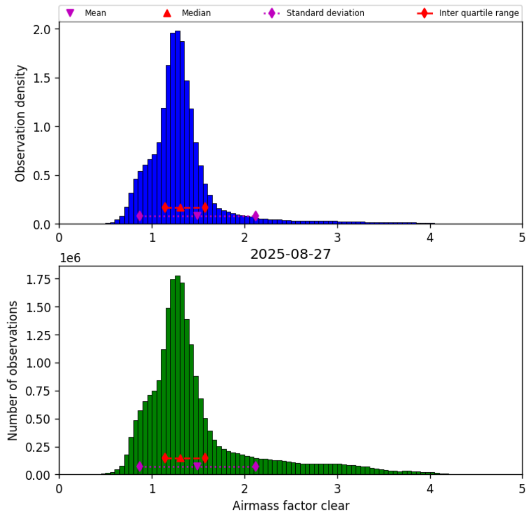
Figure 40: Histogram of “Airmass factor clear” for 2025-08-27 to 2025-08-28
