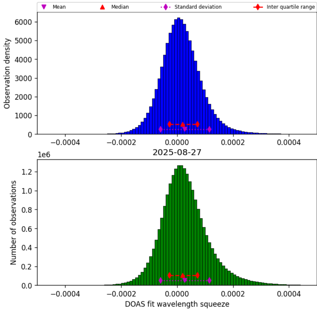
Figure 43: Histogram of “DOAS fit wavelength squeeze” for 2025-08-27 to 2025-08-28
