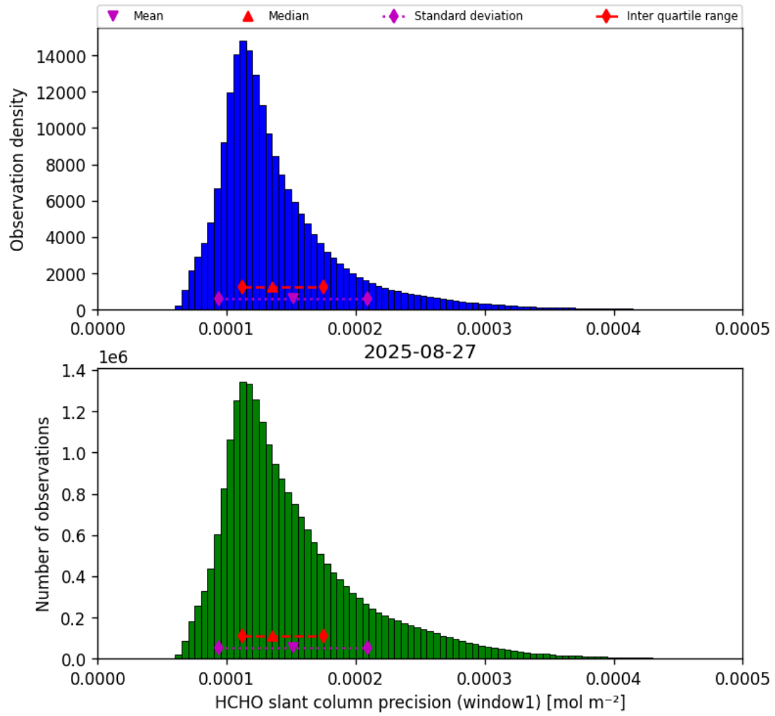
Figure 37: Histogram of “HCHO slant column precision (window1)” for 2025-08-27 to 2025-08-28
