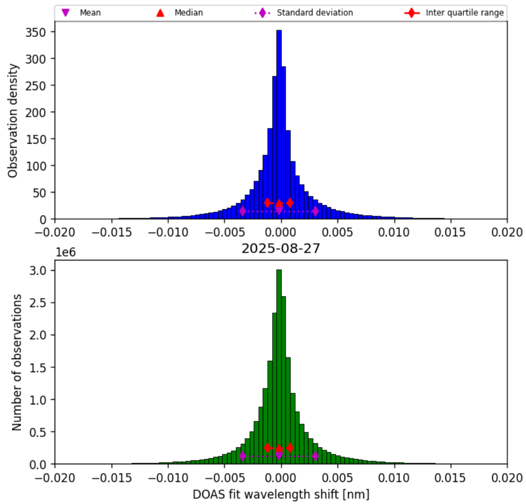
Figure 42: Histogram of “DOAS fit wavelength shift” for 2025-08-27 to 2025-08-28
