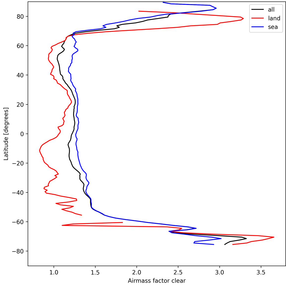
Figure 26: Zonal average of “Airmass factor clear” for 2025-08-27 to 2025-08-28.
