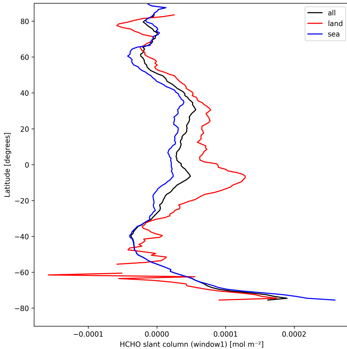
Figure 22: Zonal average of “HCHO slant column (window1)” for 2025-08-27 to 2025-08-28.
