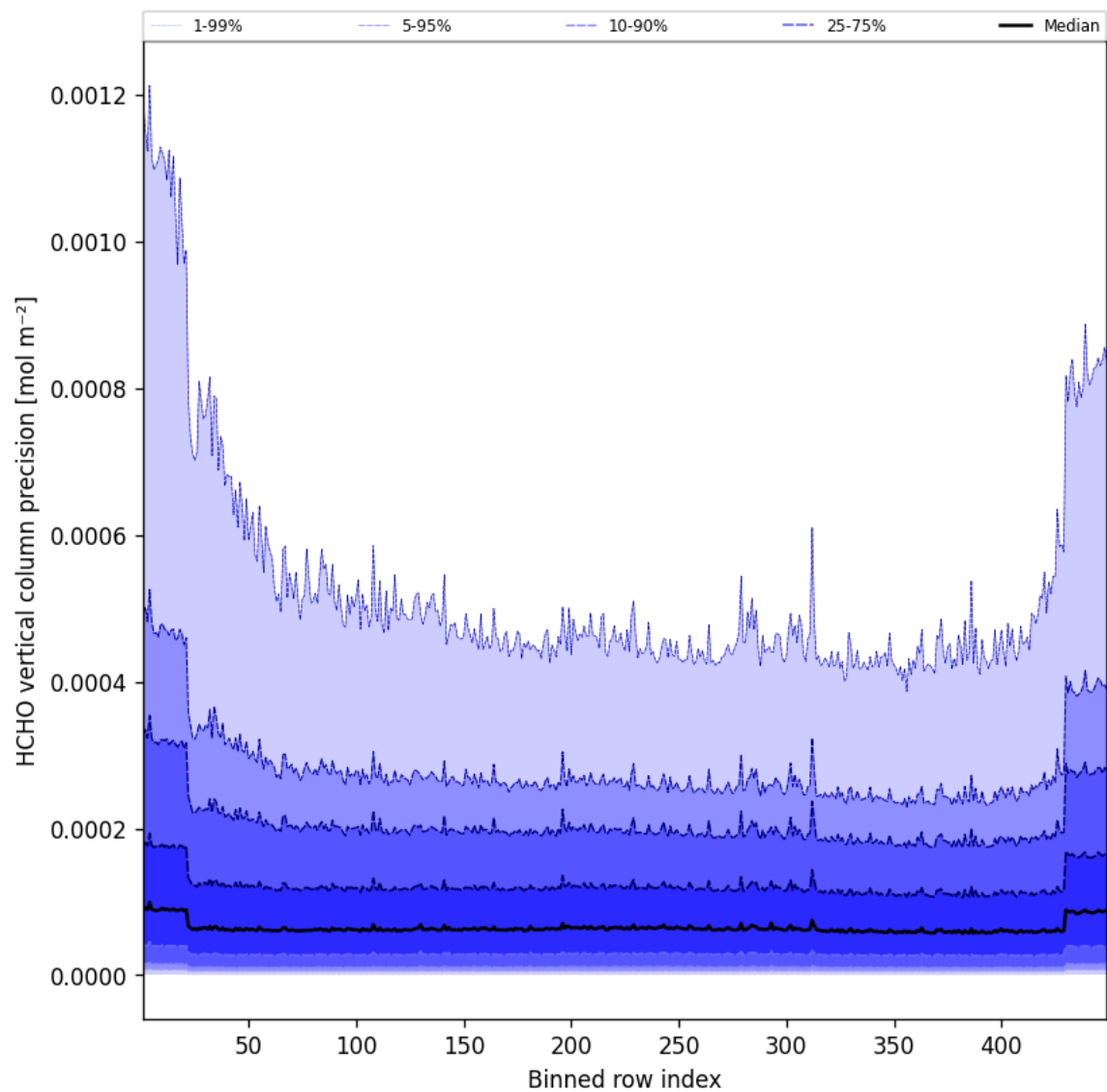
Figure 48: Along track statistics of “HCHO vertical column precision” for 2025-08-27 to 2025-08-28
