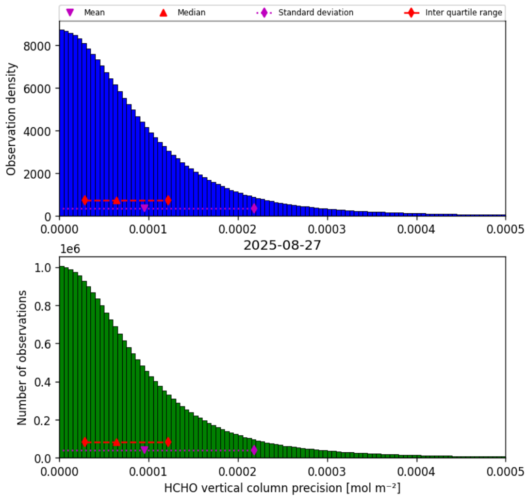
Figure 34: Histogram of “HCHO vertical column precision” for 2025-08-27 to 2025-08-28
