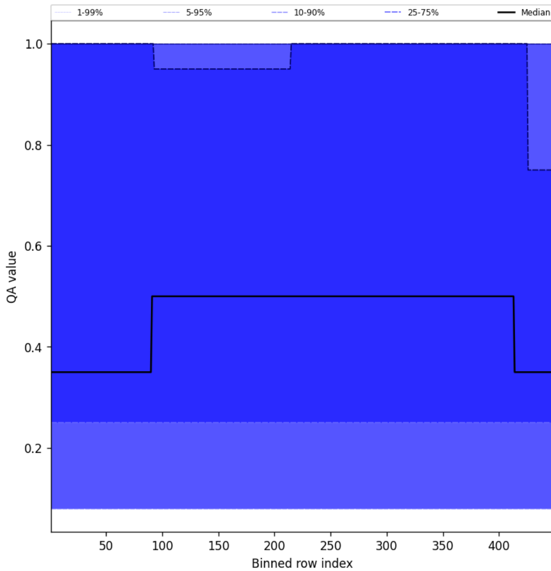
Figure 46: Along track statistics of “QA value” for 2025-08-27 to 2025-08-28
