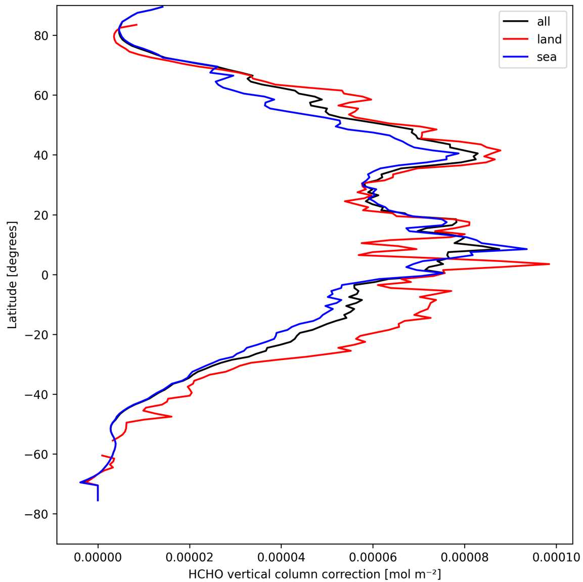
Figure 21: Zonal average of “HCHO vertical column correction” for 2025-08-27 to 2025-08-28.
