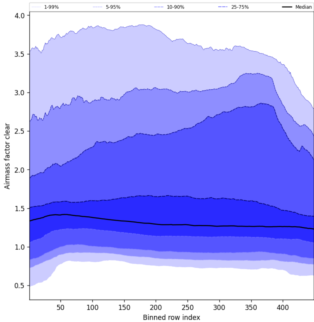
Figure 54: Along track statistics of “Airmass factor clear” for 2025-08-27 to 2025-08-28
