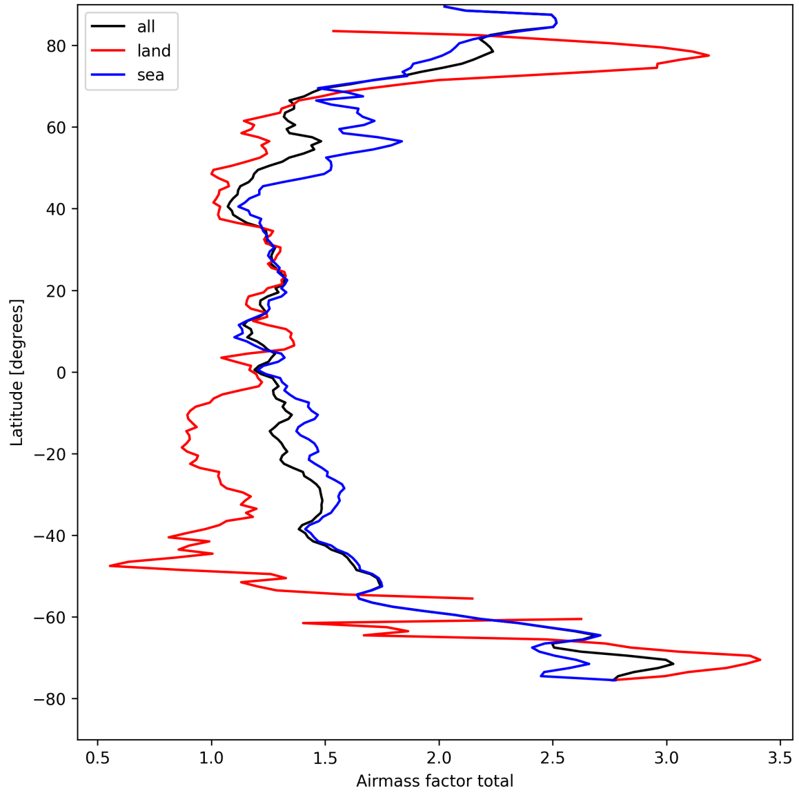
Figure 24: Zonal average of “Airmass factor total” for 2025-08-27 to 2025-08-28.
