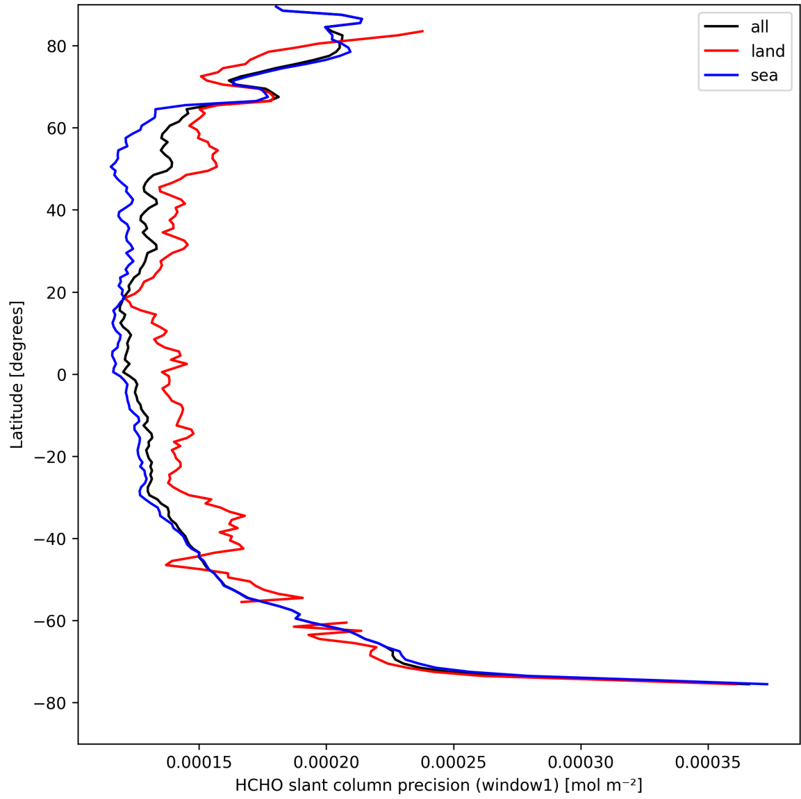
Figure 23: Zonal average of “HCHO slant column precision (window1)” for 2025-08-27 to 2025-08-28.
