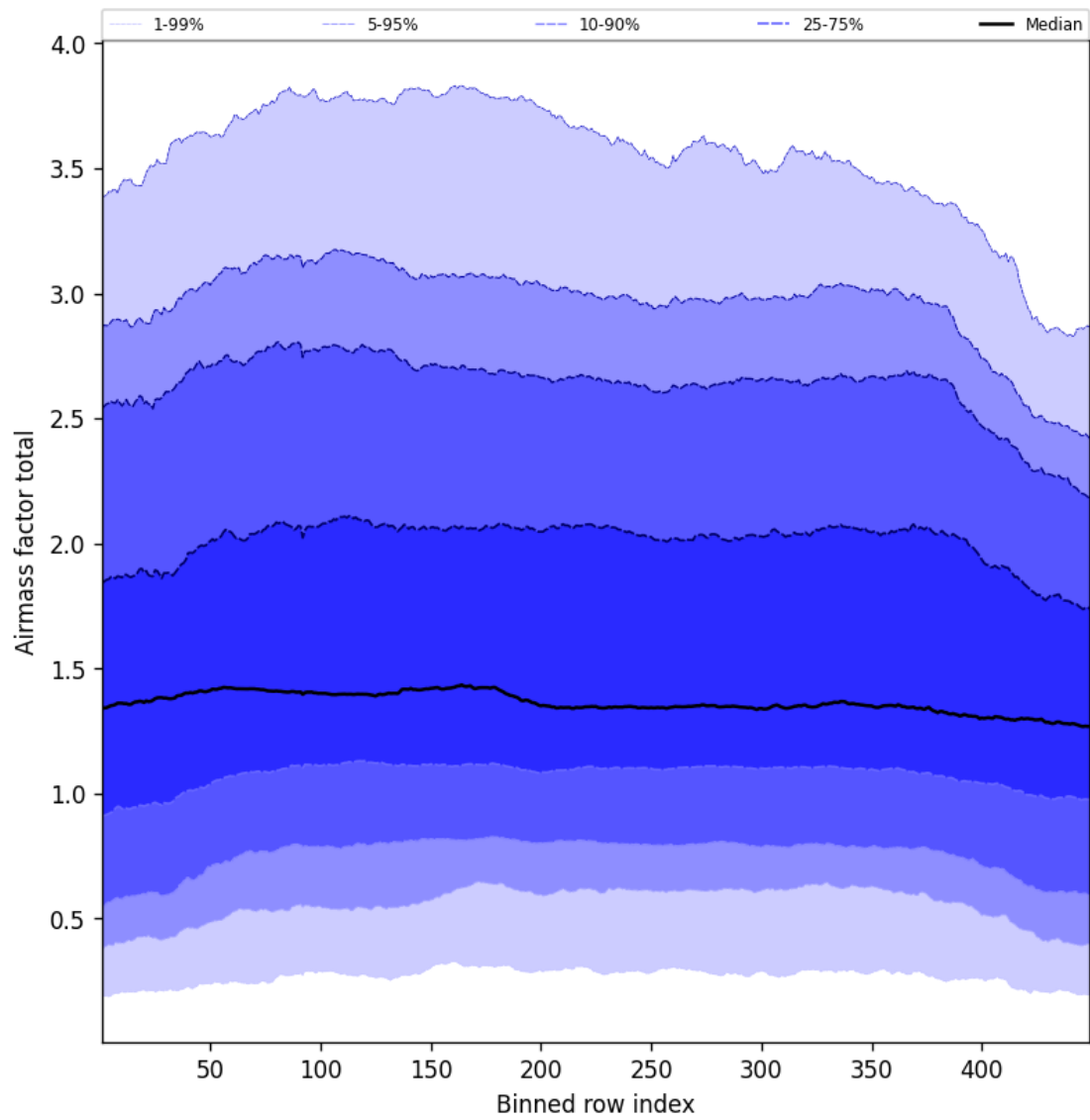
Figure 52: Along track statistics of “Airmass factor total” for 2025-08-27 to 2025-08-28
