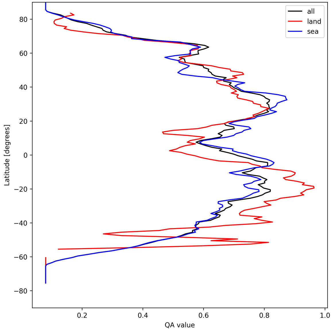
Figure 18: Zonal average of “QA value” for 2025-08-27 to 2025-08-28.
