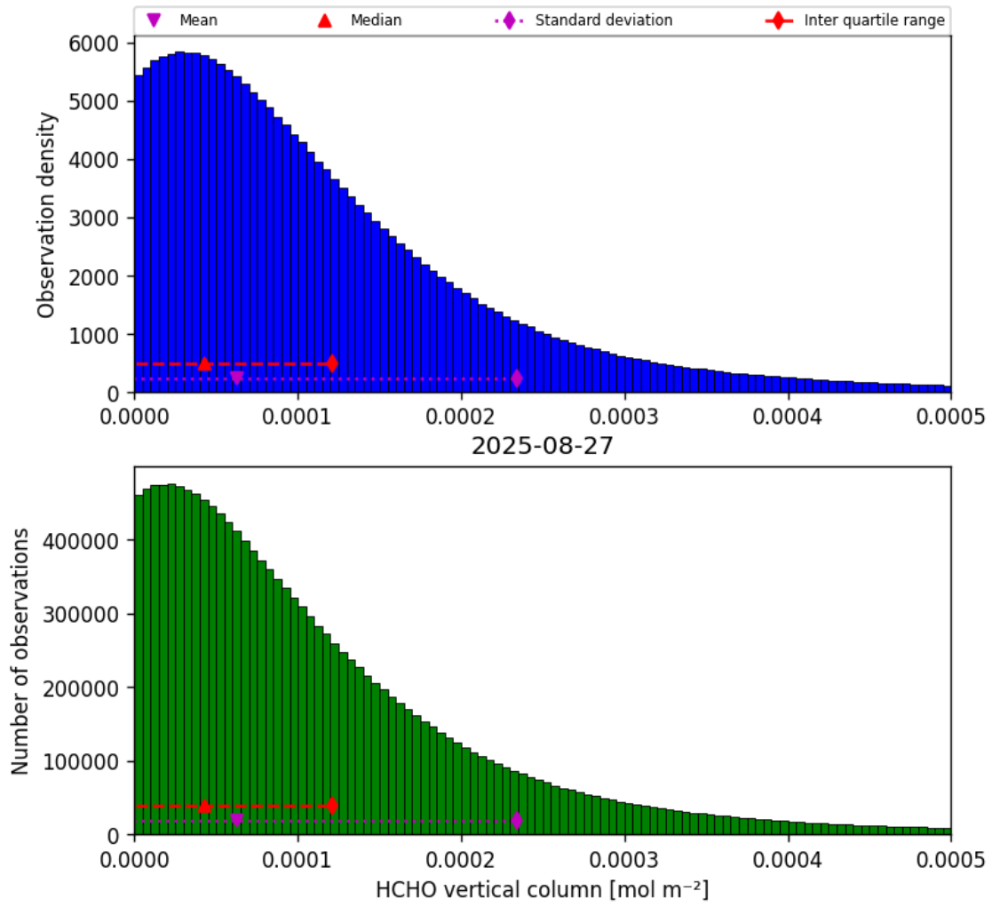
Figure 33: Histogram of “HCHO vertical column” for 2025-08-27 to 2025-08-28
