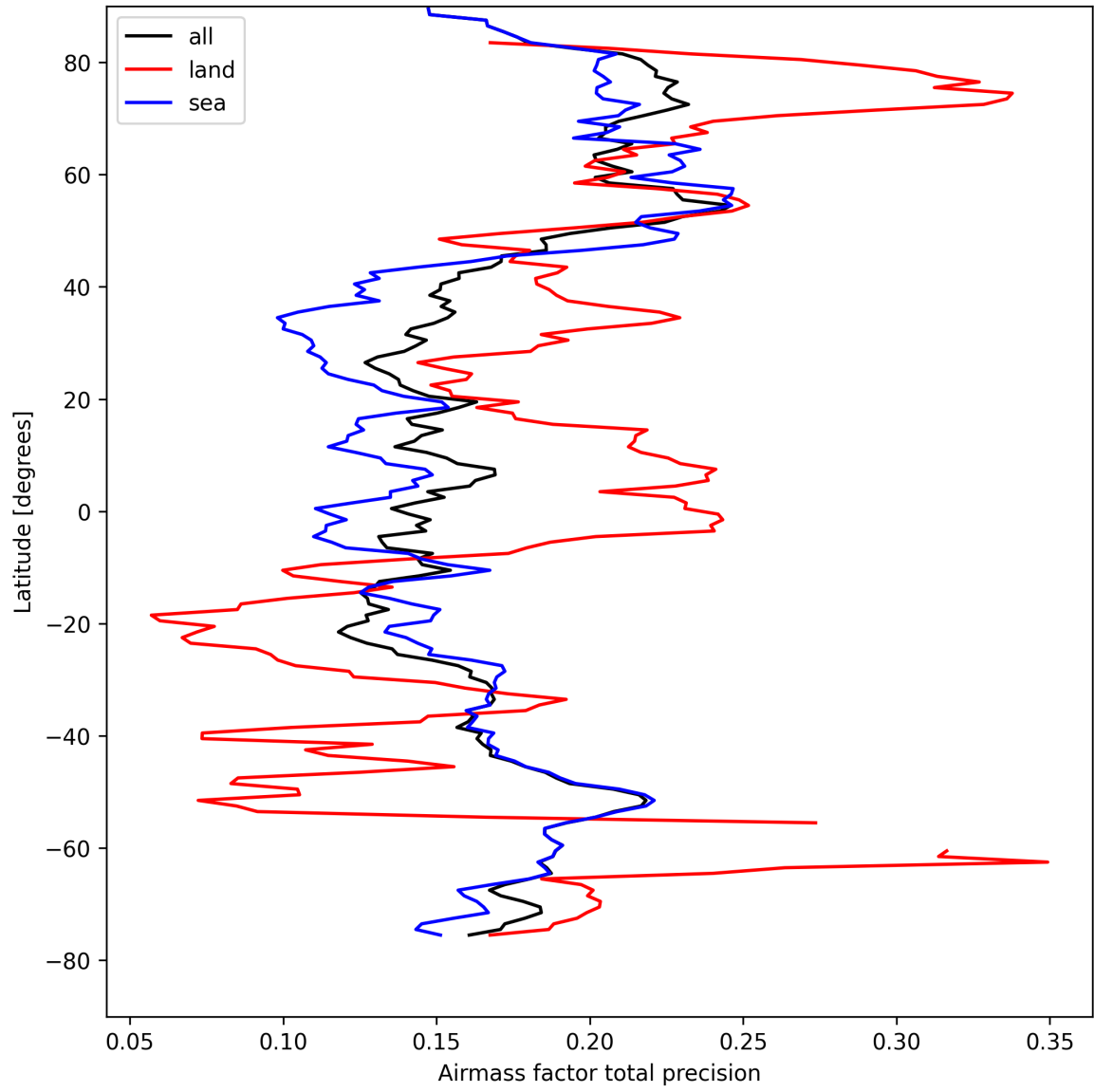
Figure 25: Zonal average of “Airmass factor total precision” for 2025-08-27 to 2025-08-28.
