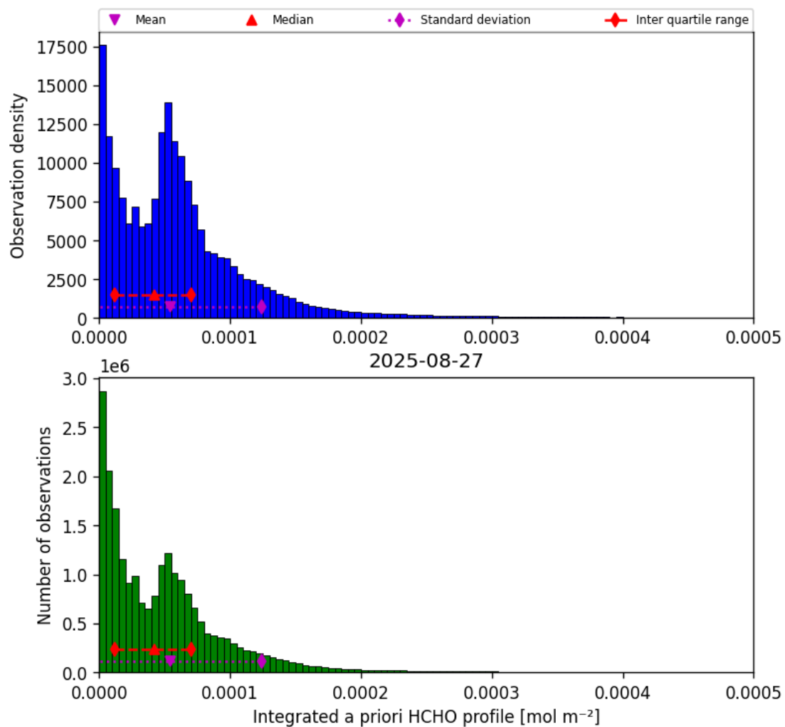
Figure 41: Histogram of “Integrated a priori HCHO profile” for 2025-08-27 to 2025-08-28
