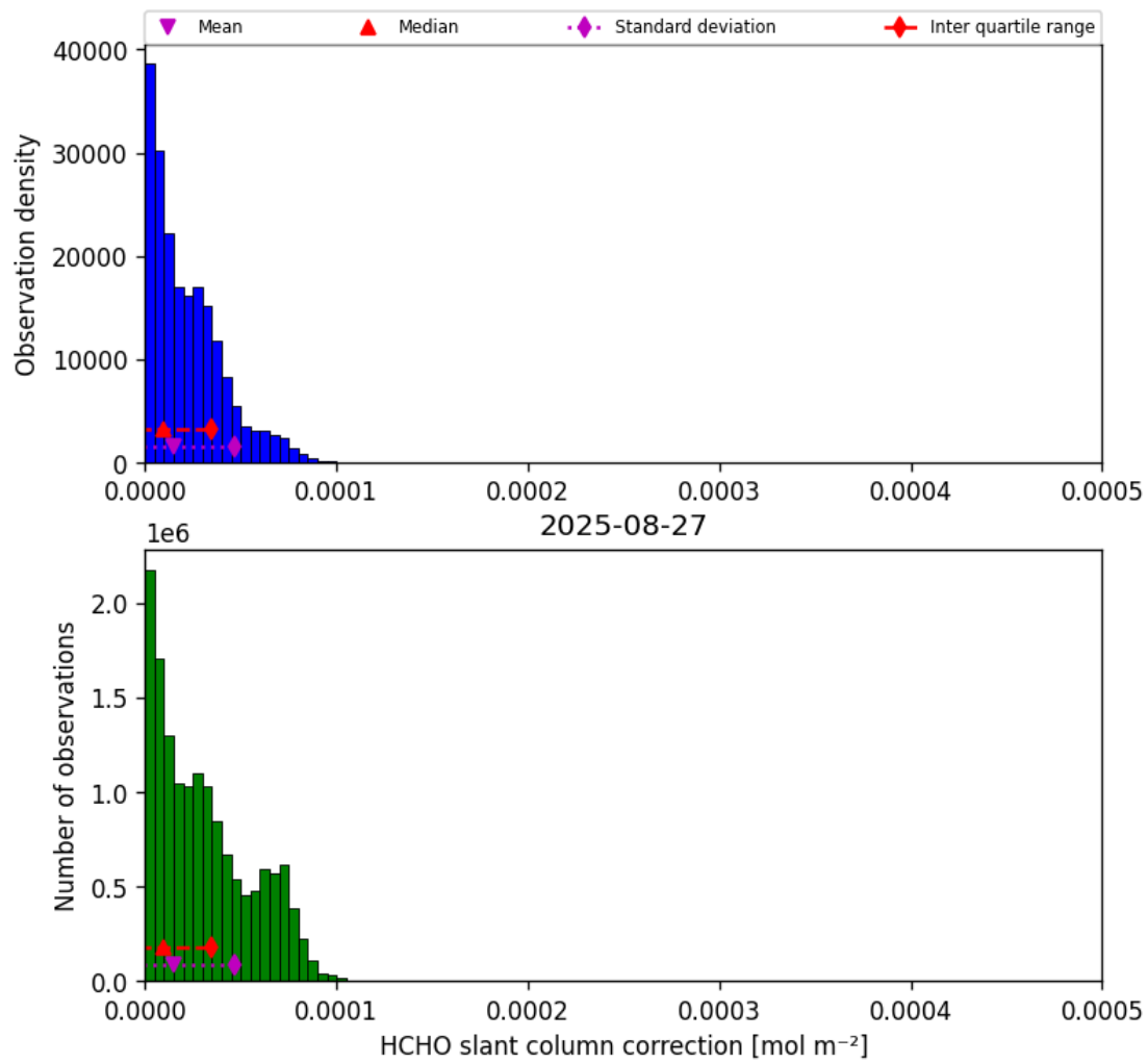
Figure 45: Histogram of “HCHO slant column correction” for 2025-08-27 to 2025-08-28
