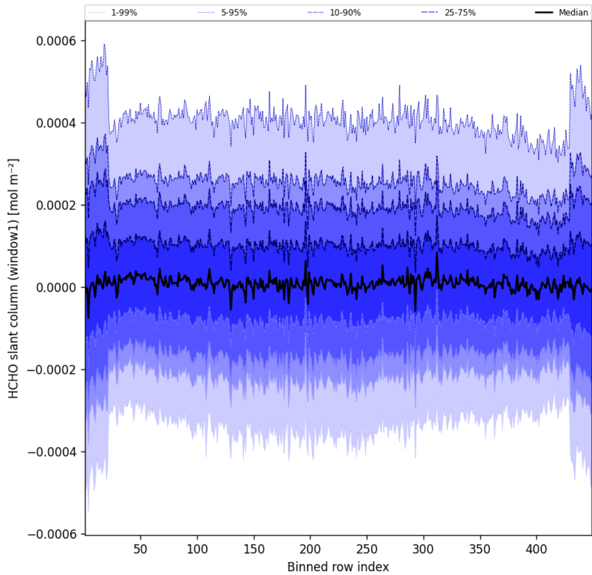
Figure 50: Along track statistics of “HCHO slant column (window1)” for 2025-08-27 to 2025-08-28
