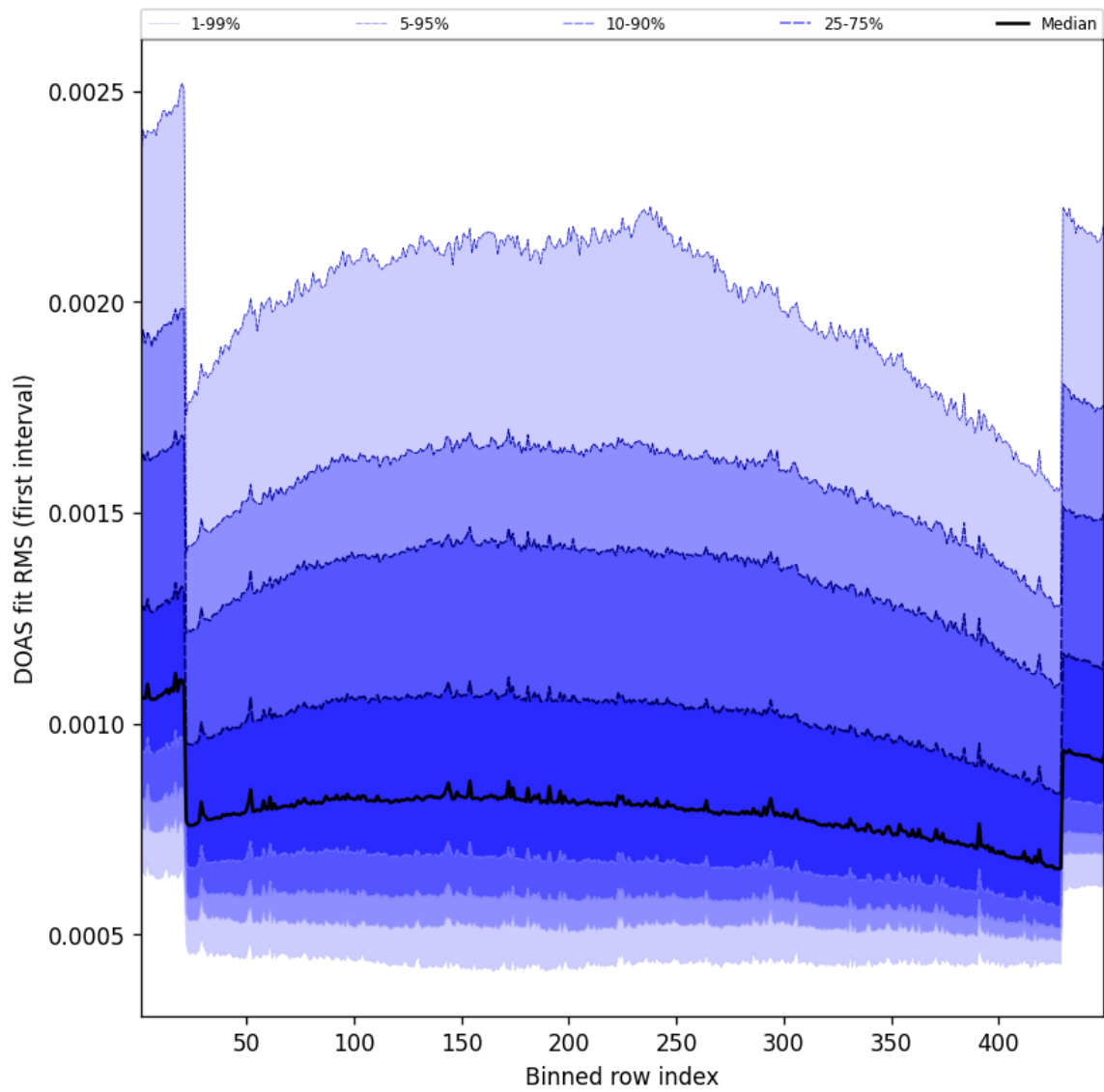
Figure 58: Along track statistics of “DOAS fit RMS (first interval)” for 2025-08-27 to 2025-08-28
