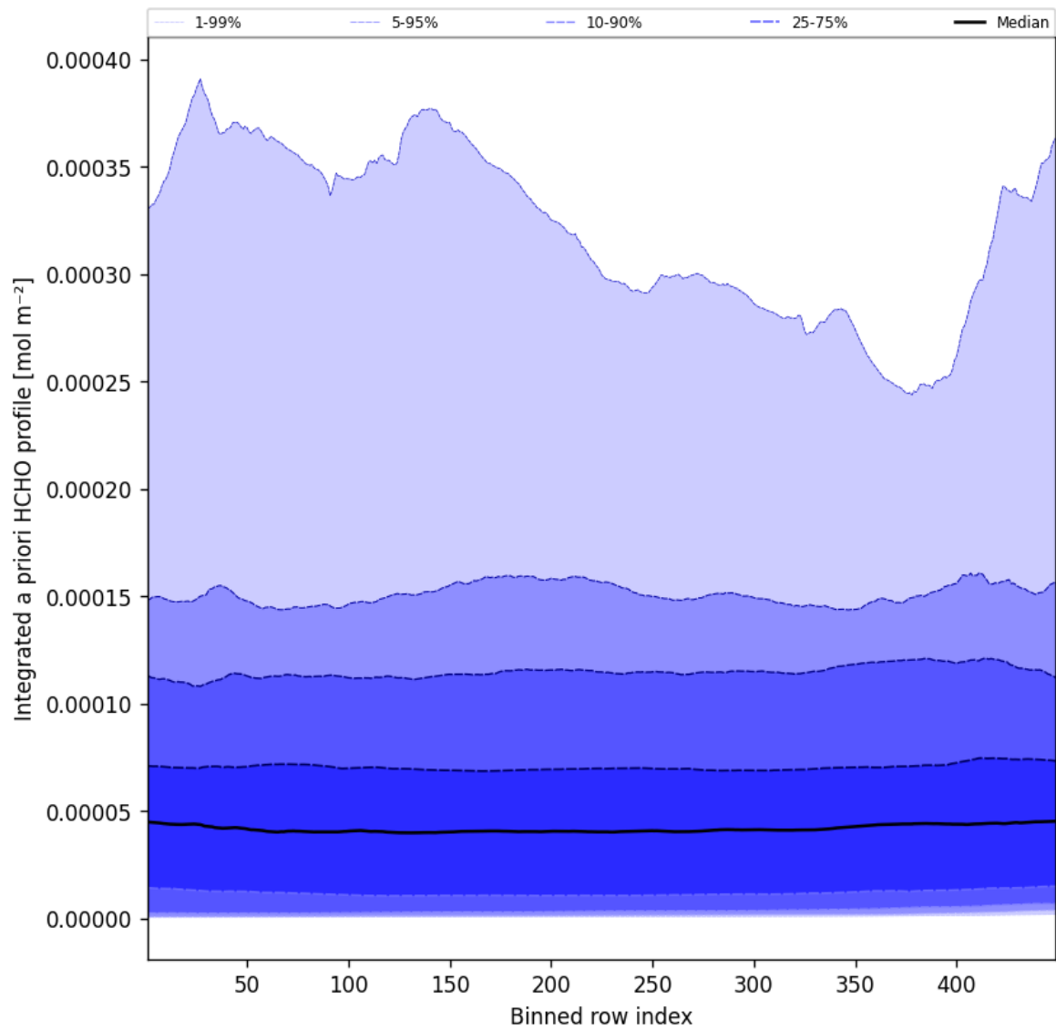
Figure 55: Along track statistics of “Integrated a priori HCHO profile” for 2025-08-27 to 2025-08-28
