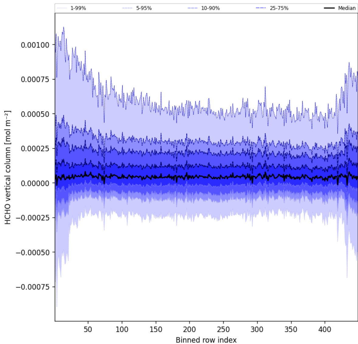
Figure 47: Along track statistics of “HCHO vertical column” for 2025-08-27 to 2025-08-28
