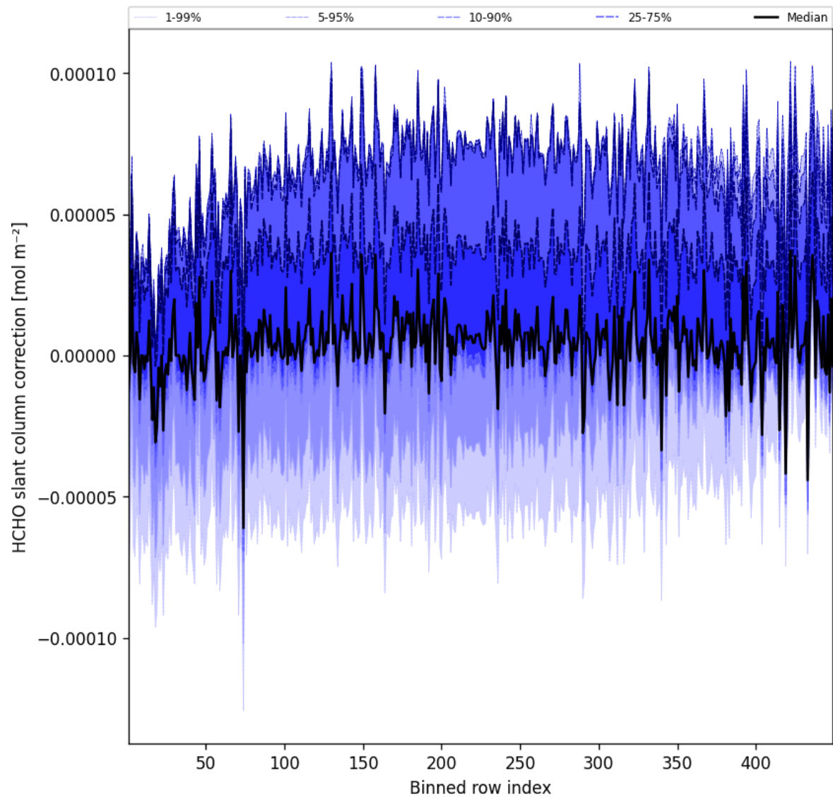
Figure 59: Along track statistics of “HCHO slant column correction” for 2025-08-27 to 2025-08-28
