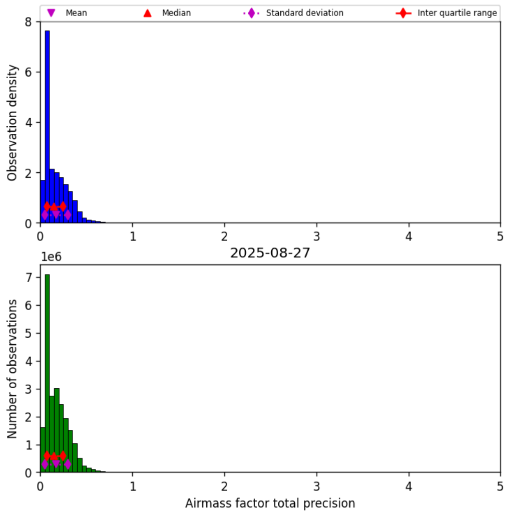
Figure 39: Histogram of “Airmass factor total precision” for 2025-08-27 to 2025-08-28
