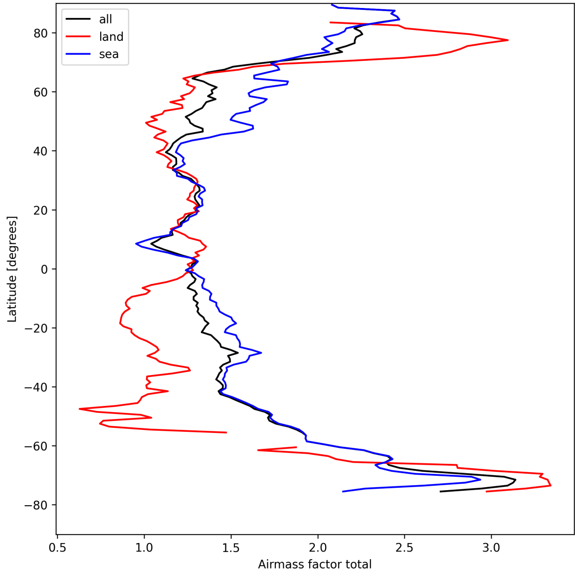
Figure 24: Zonal average of “Airmass factor total” for 2025-08-28 to 2025-08-28.
