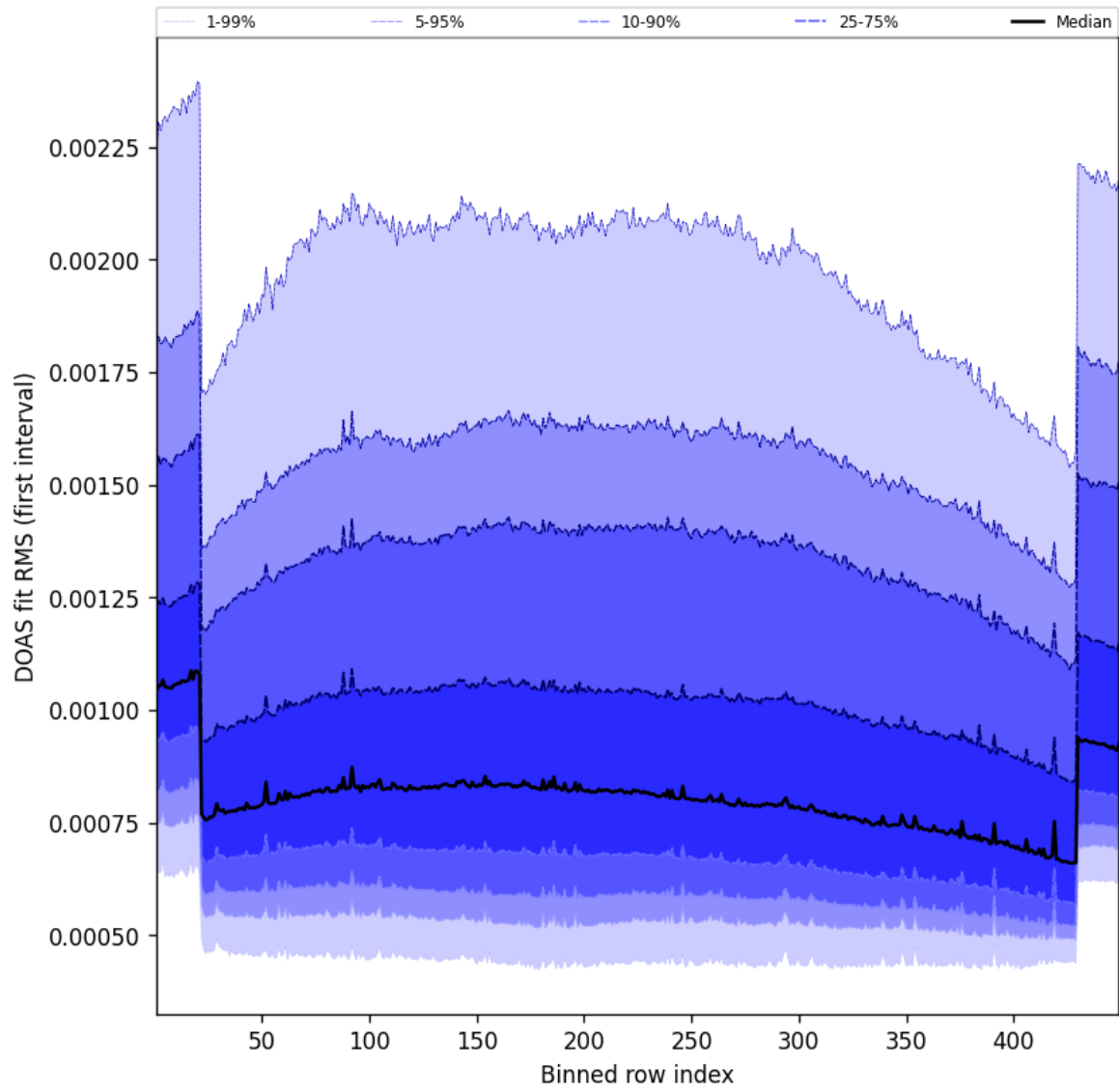
Figure 58: Along track statistics of “DOAS fit RMS (first interval)” for 2025-08-28 to 2025-08-28
