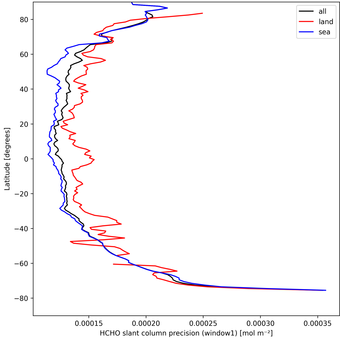
Figure 23: Zonal average of “HCHO slant column precision (window1)” for 2025-08-28 to 2025-08-28.
