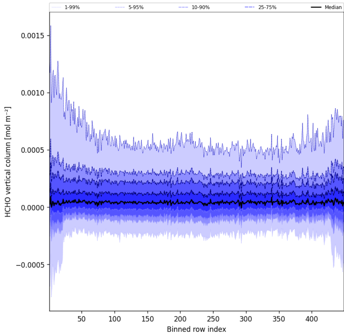
Figure 47: Along track statistics of “HCHO vertical column” for 2025-08-28 to 2025-08-28
