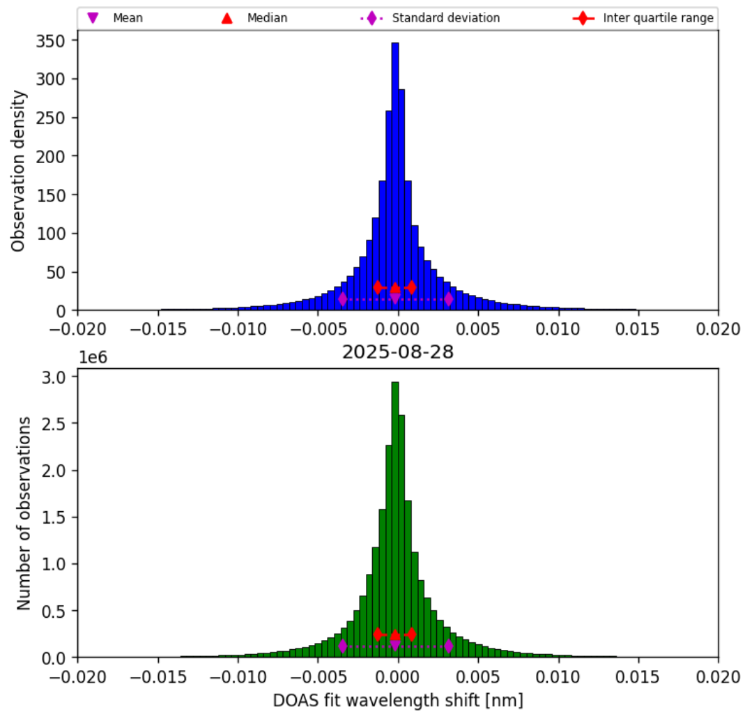
Figure 42: Histogram of “DOAS fit wavelength shift” for 2025-08-28 to 2025-08-28
