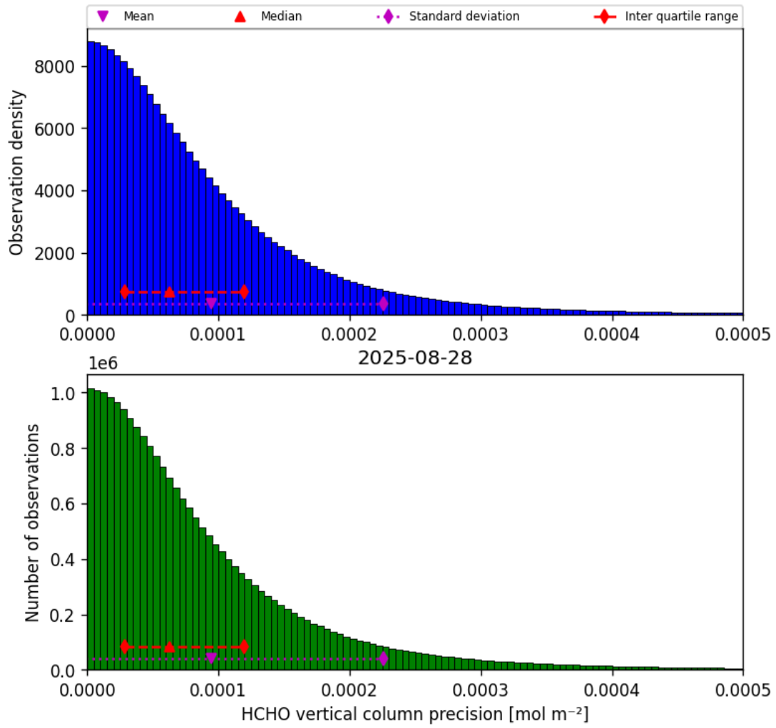
Figure 34: Histogram of “HCHO vertical column precision” for 2025-08-28 to 2025-08-28
