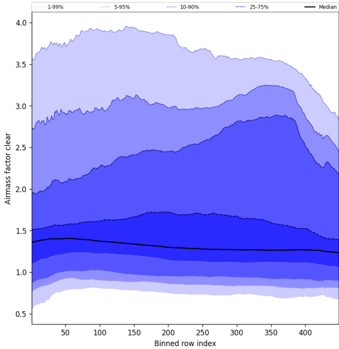
Figure 54: Along track statistics of “Airmass factor clear” for 2025-08-28 to 2025-08-28
