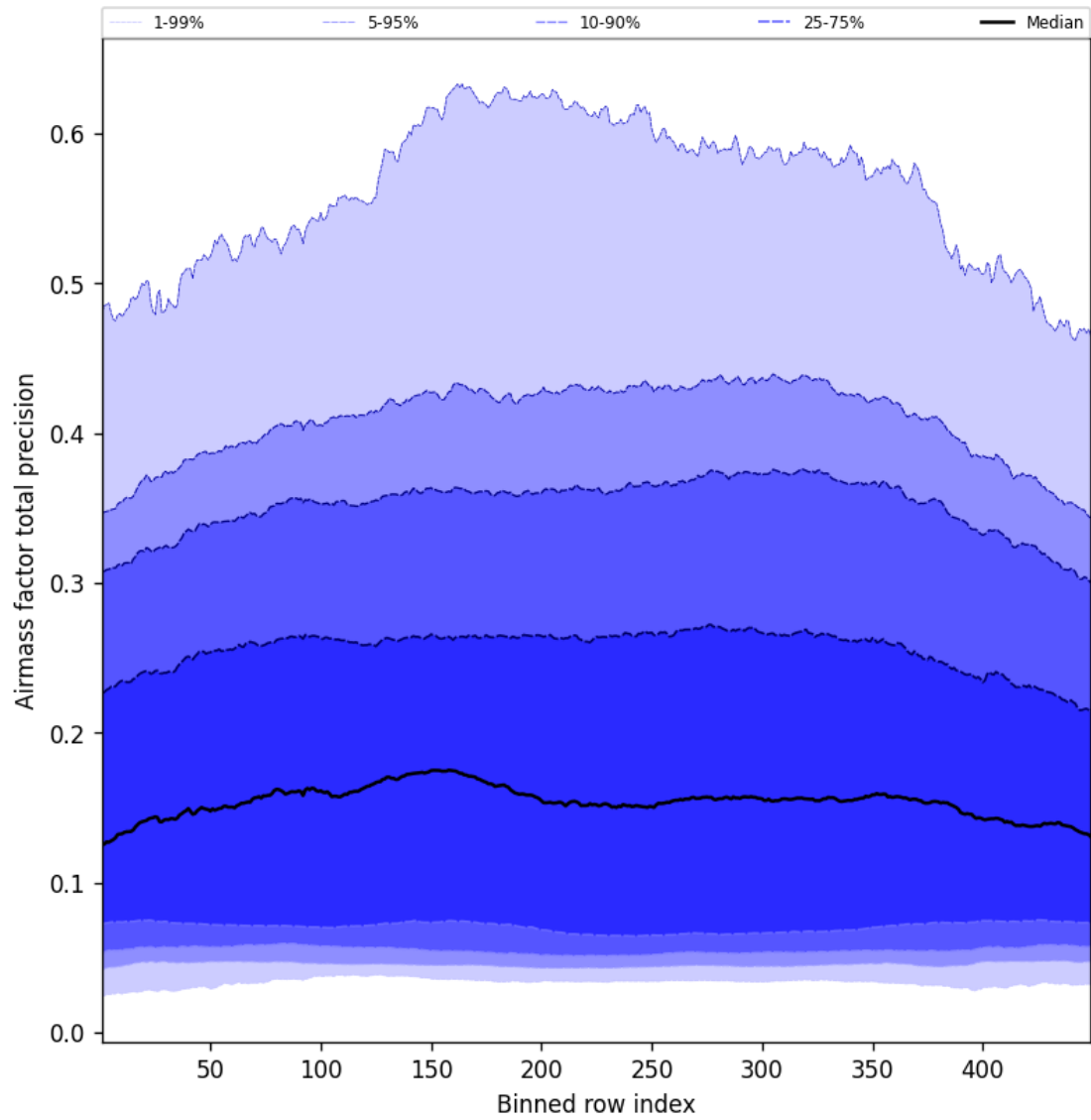
Figure 53: Along track statistics of “Airmass factor total precision” for 2025-08-28 to 2025-08-28
