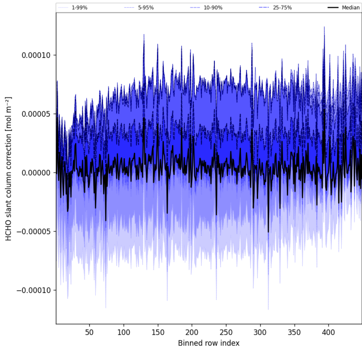
Figure 59: Along track statistics of “HCHO slant column correction” for 2025-08-28 to 2025-08-28
