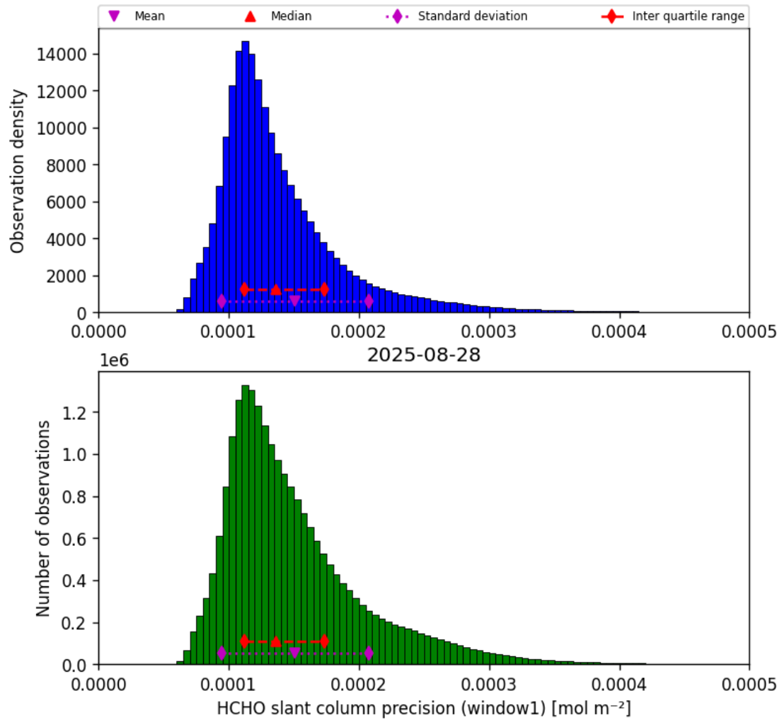
Figure 37: Histogram of “HCHO slant column precision (window1)” for 2025-08-28 to 2025-08-28
