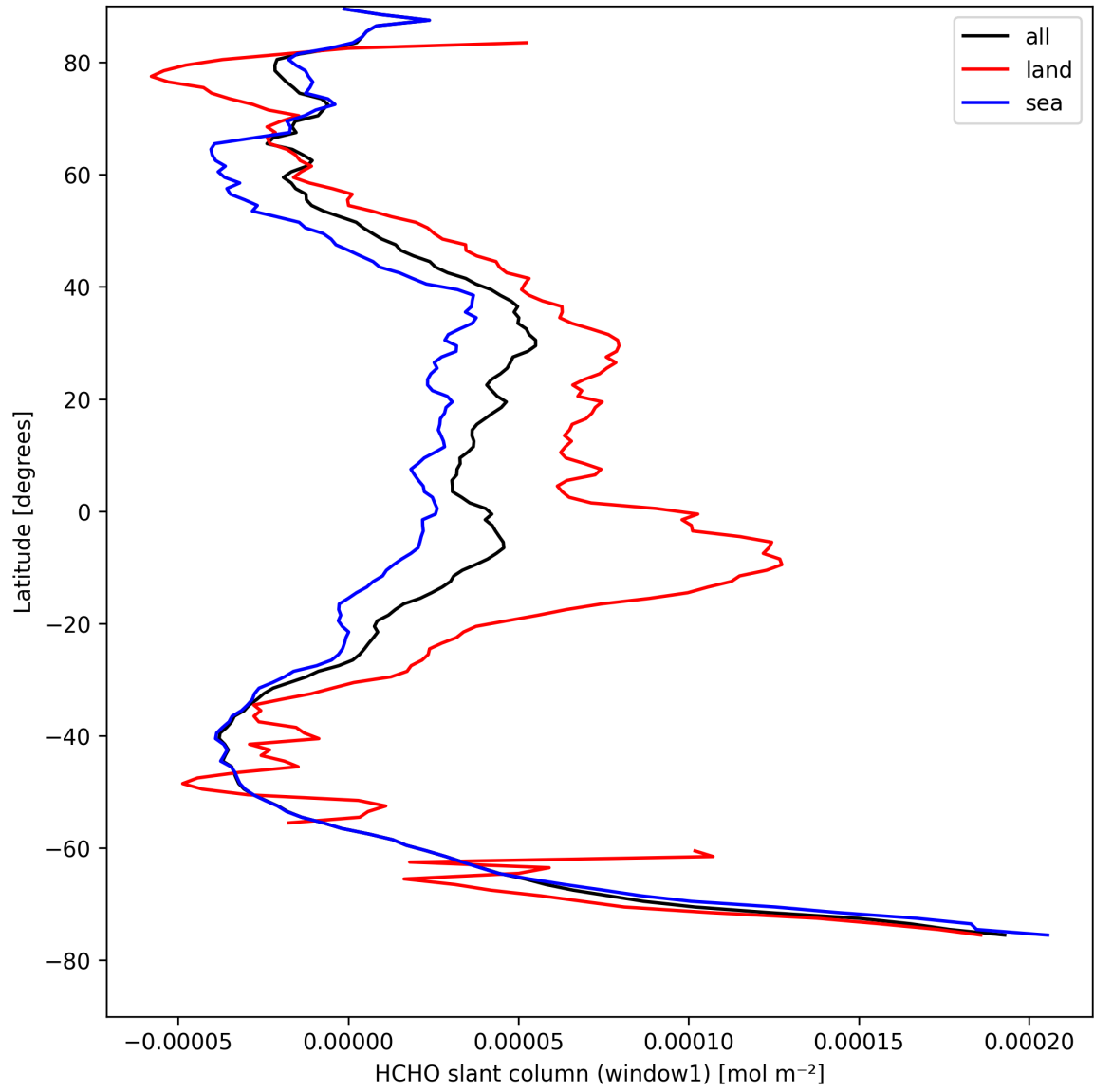
Figure 22: Zonal average of “HCHO slant column (window1)” for 2025-08-28 to 2025-08-28.
