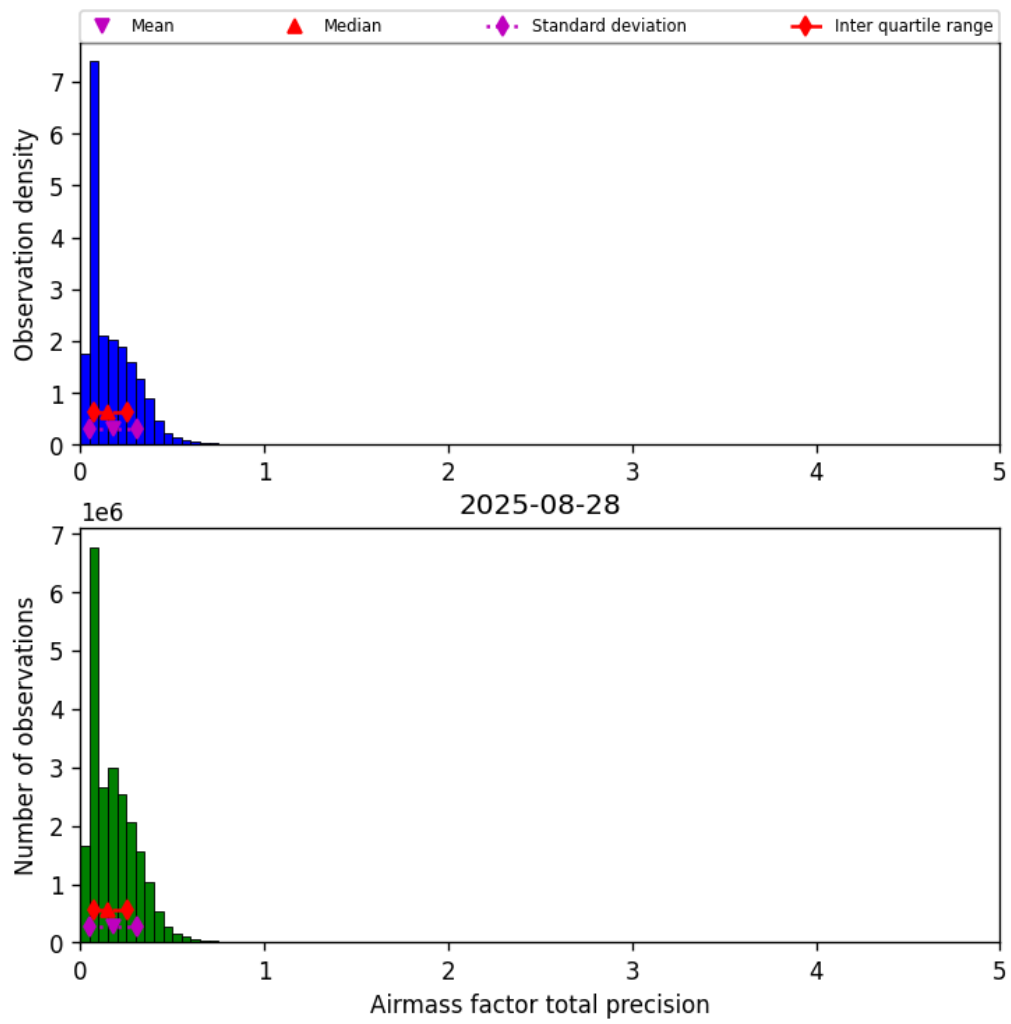
Figure 39: Histogram of “Airmass factor total precision” for 2025-08-28 to 2025-08-28
