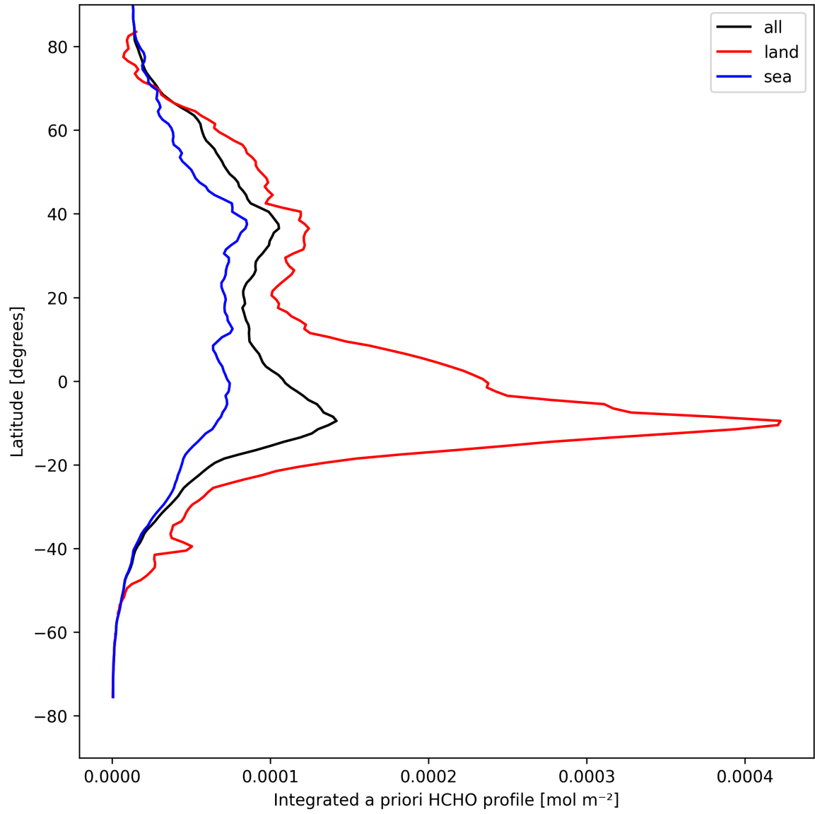
Figure 27: Zonal average of “Integrated a priori HCHO profile” for 2025-08-28 to 2025-08-28.
