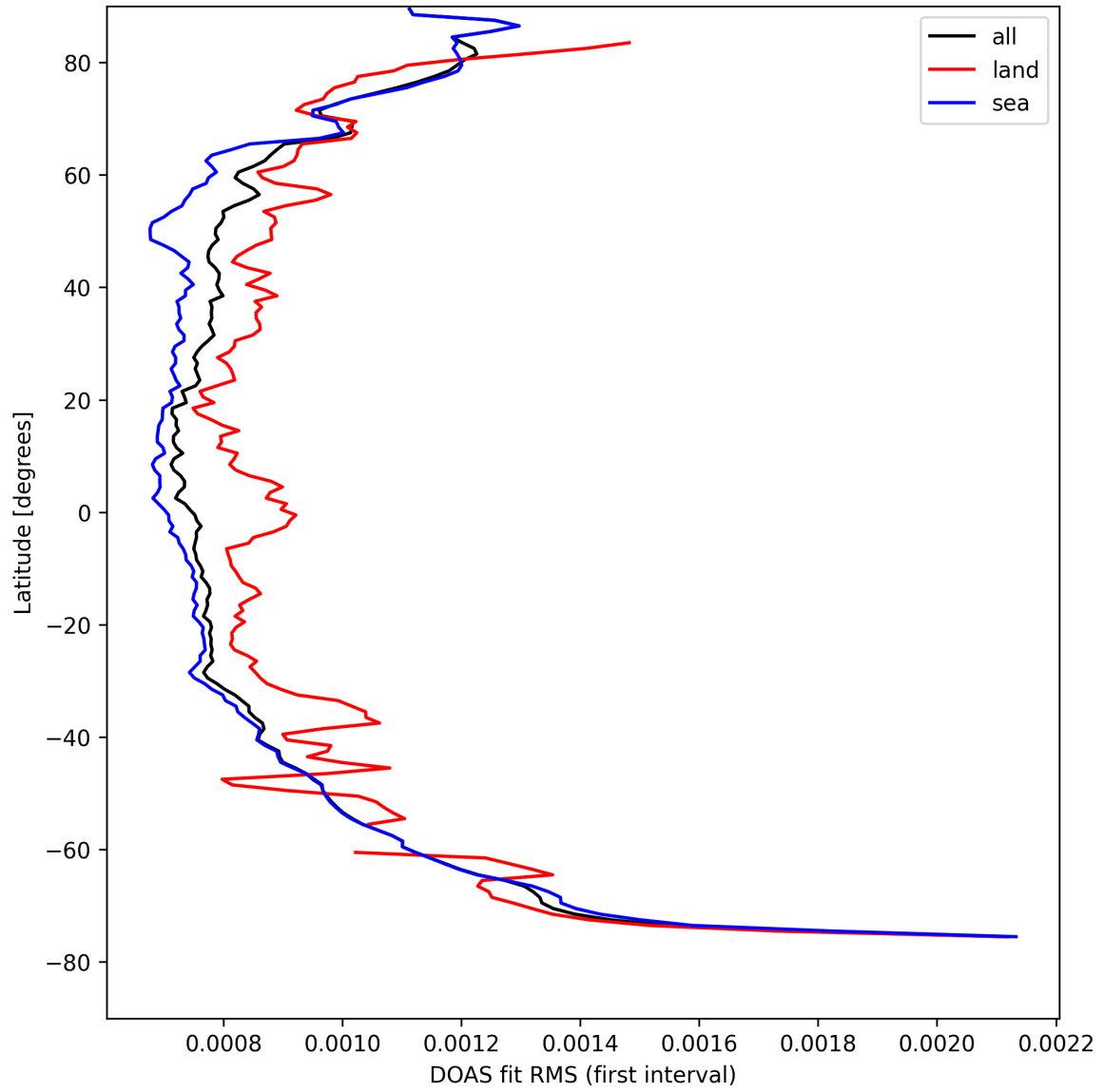
Figure 30: Zonal average of "DOAS fit RMS (first interval)" for 2025-08-28 to 2025-08-28.
