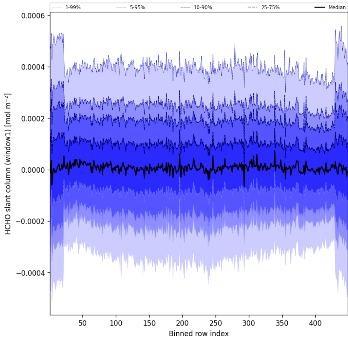
Figure 50: Along track statistics of “HCHO slant column (window1)” for 2025-08-28 to 2025-08-28
