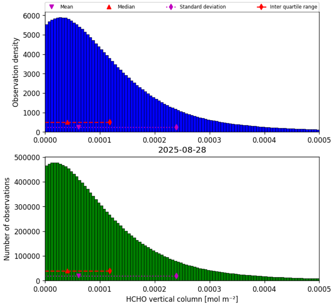
Figure 33: Histogram of “HCHO vertical column” for 2025-08-28 to 2025-08-28
