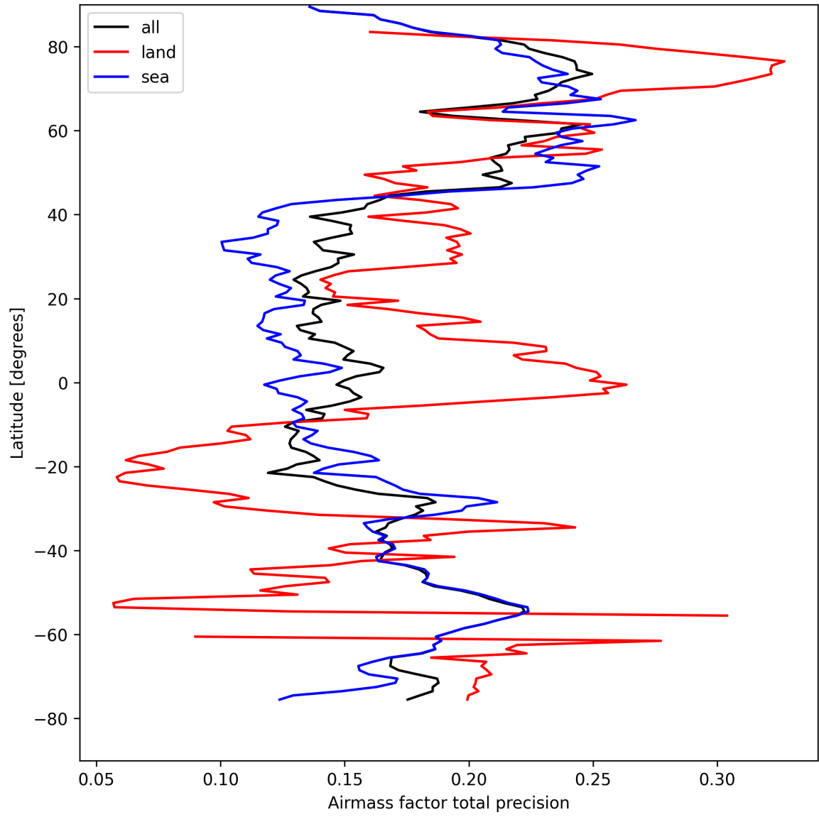
Figure 25: Zonal average of “Airmass factor total precision” for 2025-08-28 to 2025-08-28.
