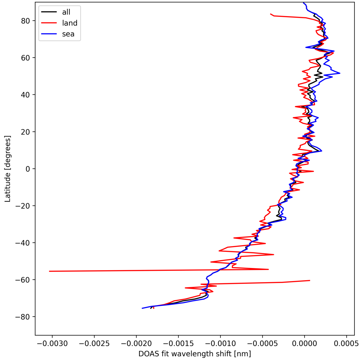
Figure 28: Zonal average of “DOAS fit wavelength shift” for 2025-08-28 to 2025-08-28.
