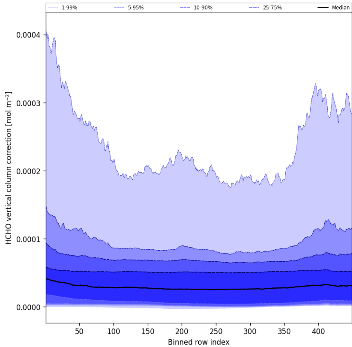
Figure 49: Along track statistics of “HCHO vertical column correction” for 2025-08-28 to 2025-08-28
