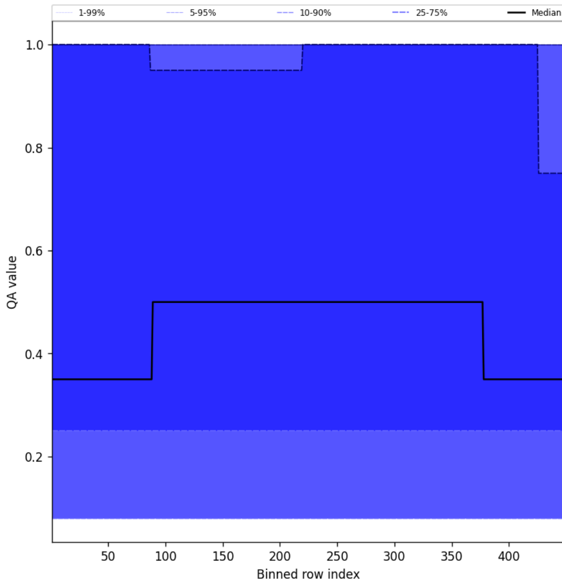
Figure 46: Along track statistics of “QA value” for 2025-08-28 to 2025-08-28
