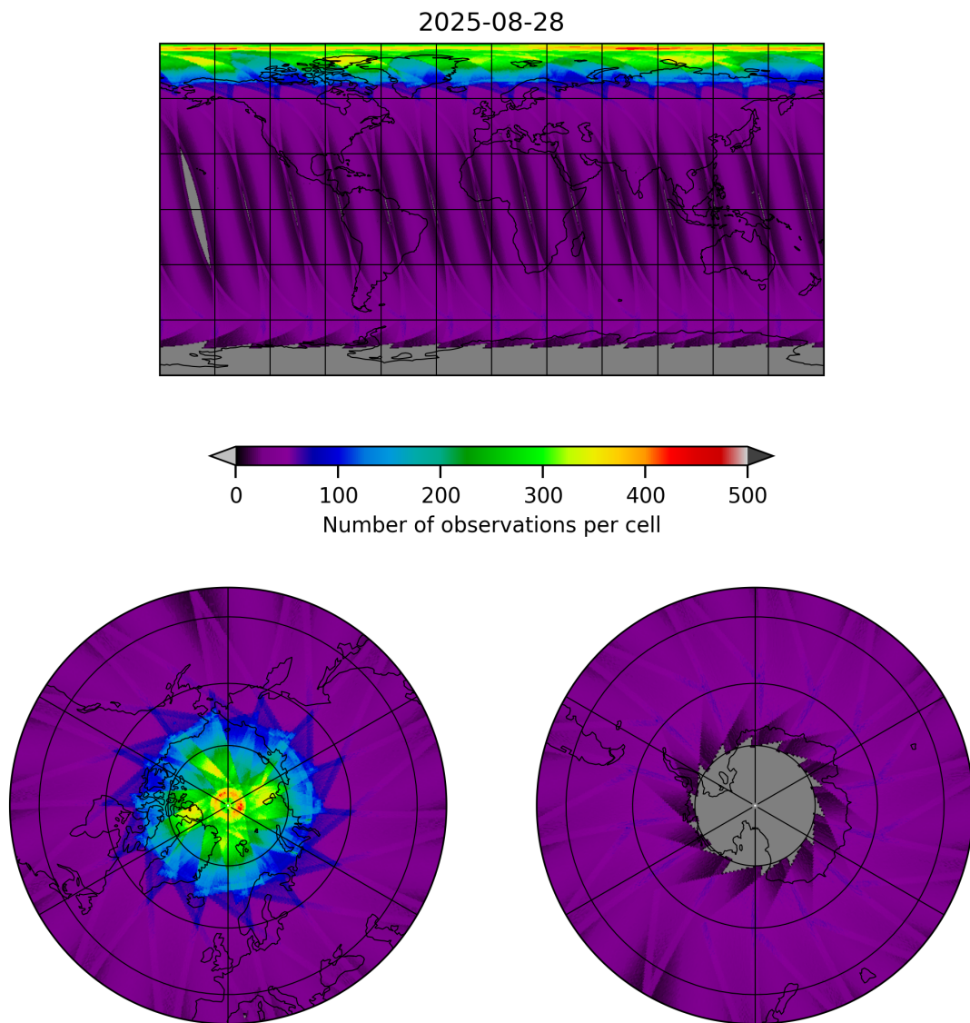
Figure 17: Map of the number of observations for 2025-08-28 to 2025-08-28
