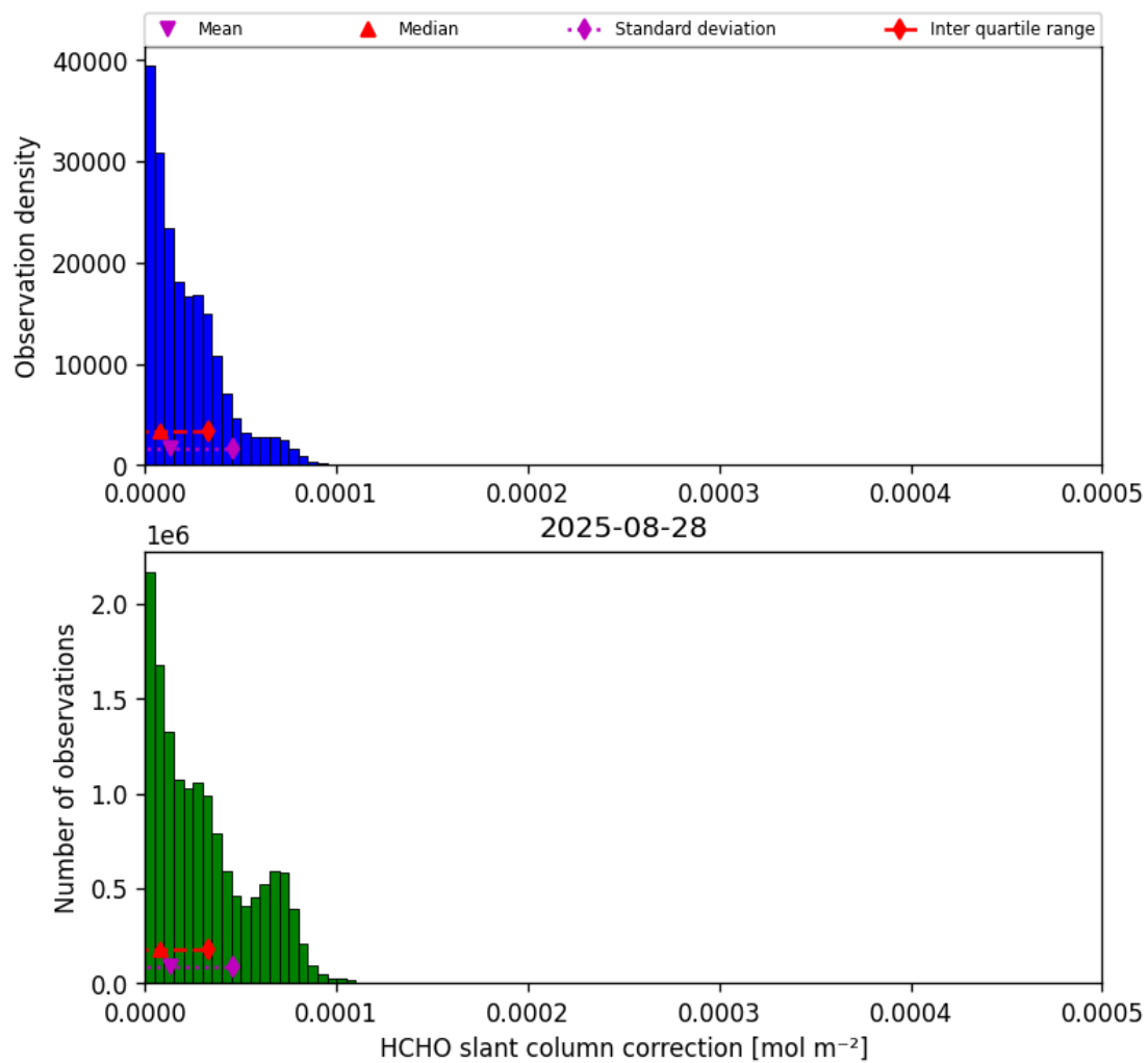
Figure 45: Histogram of “HCHO slant column correction” for 2025-08-28 to 2025-08-28
