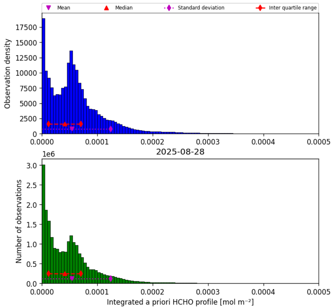
Figure 41: Histogram of “Integrated a priori HCHO profile” for 2025-08-28 to 2025-08-28
