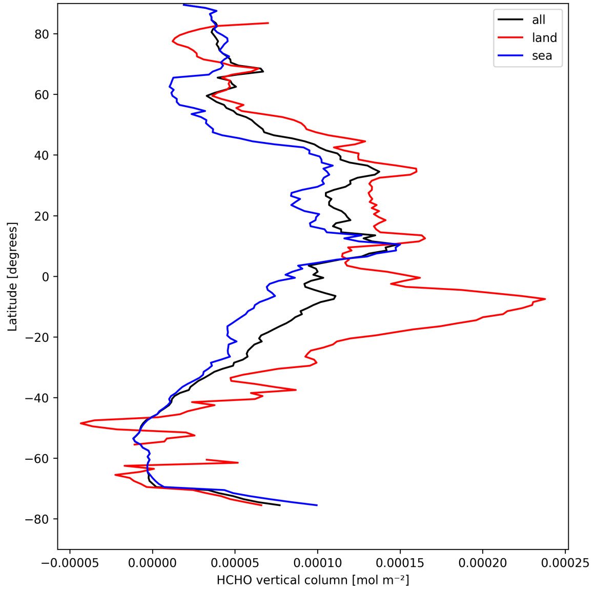
Figure 19: Zonal average of “HCHO vertical column” for 2025-08-28 to 2025-08-28.
