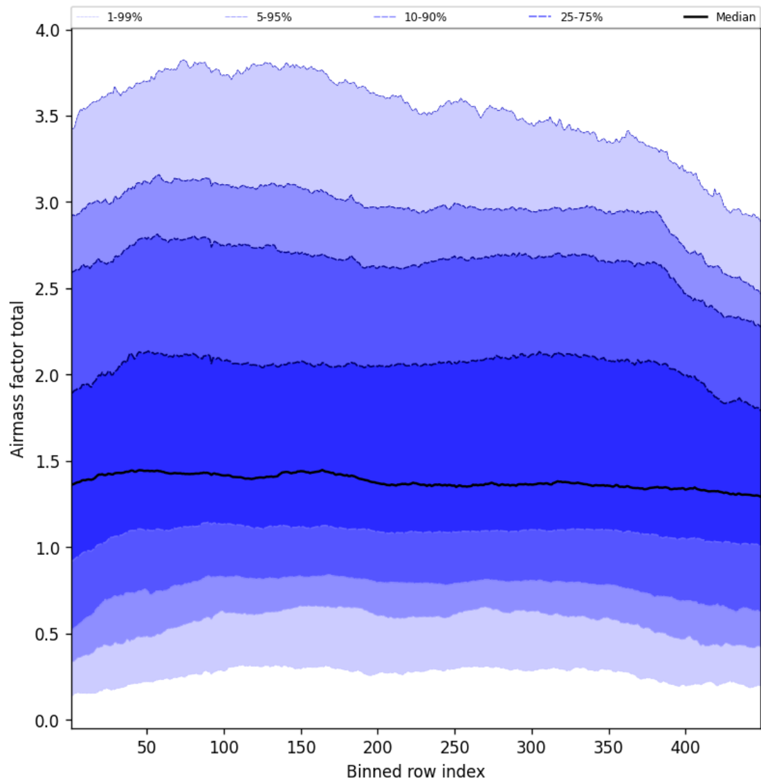
Figure 52: Along track statistics of “Airmass factor total” for 2025-08-28 to 2025-08-28
