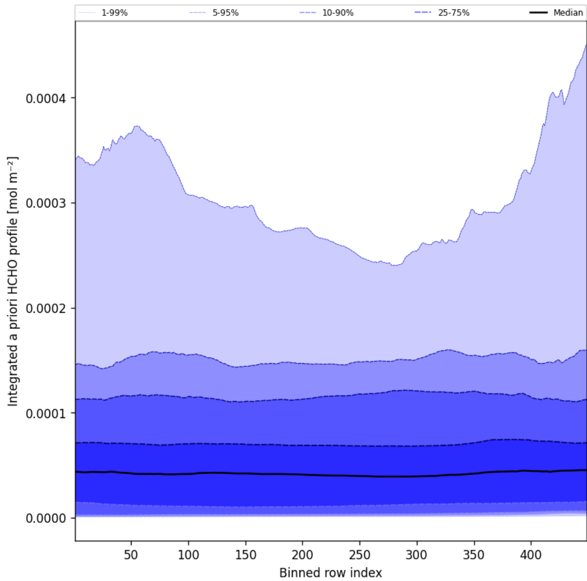
Figure 55: Along track statistics of “Integrated a priori HCHO profile” for 2025-08-28 to 2025-08-28
