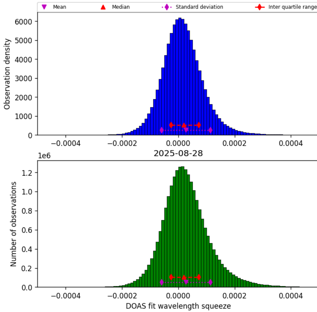
Figure 43: Histogram of “DOAS fit wavelength squeeze” for 2025-08-28 to 2025-08-28
