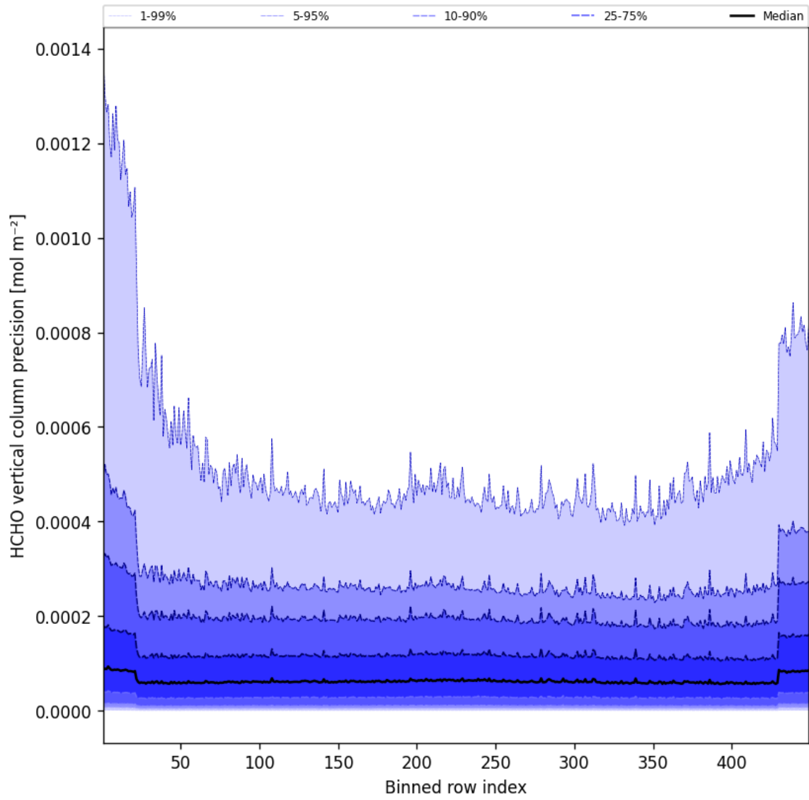
Figure 48: Along track statistics of “HCHO vertical column precision” for 2025-08-28 to 2025-08-28
