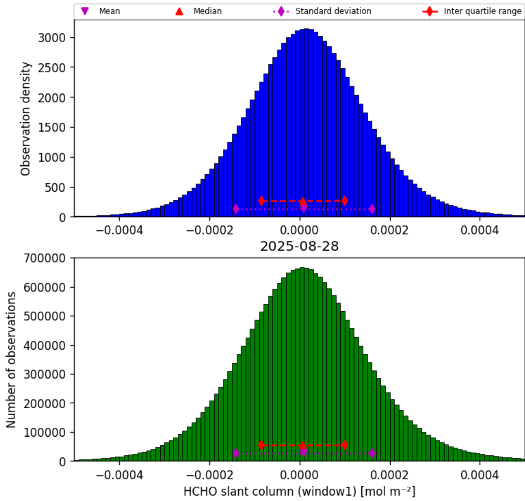
Figure 36: Histogram of “HCHO slant column (window1)” for 2025-08-28 to 2025-08-28
