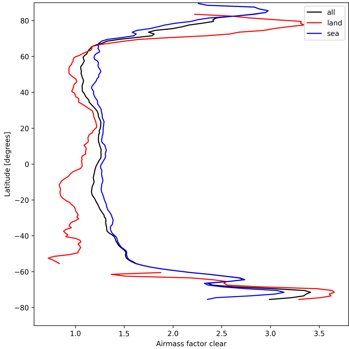
Figure 26: Zonal average of “Airmass factor clear” for 2025-08-28 to 2025-08-28.
