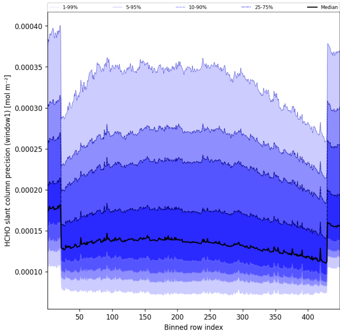
Figure 51: Along track statistics of “HCHO slant column precision (window1)” for 2025-08-28 to 2025-08-28
