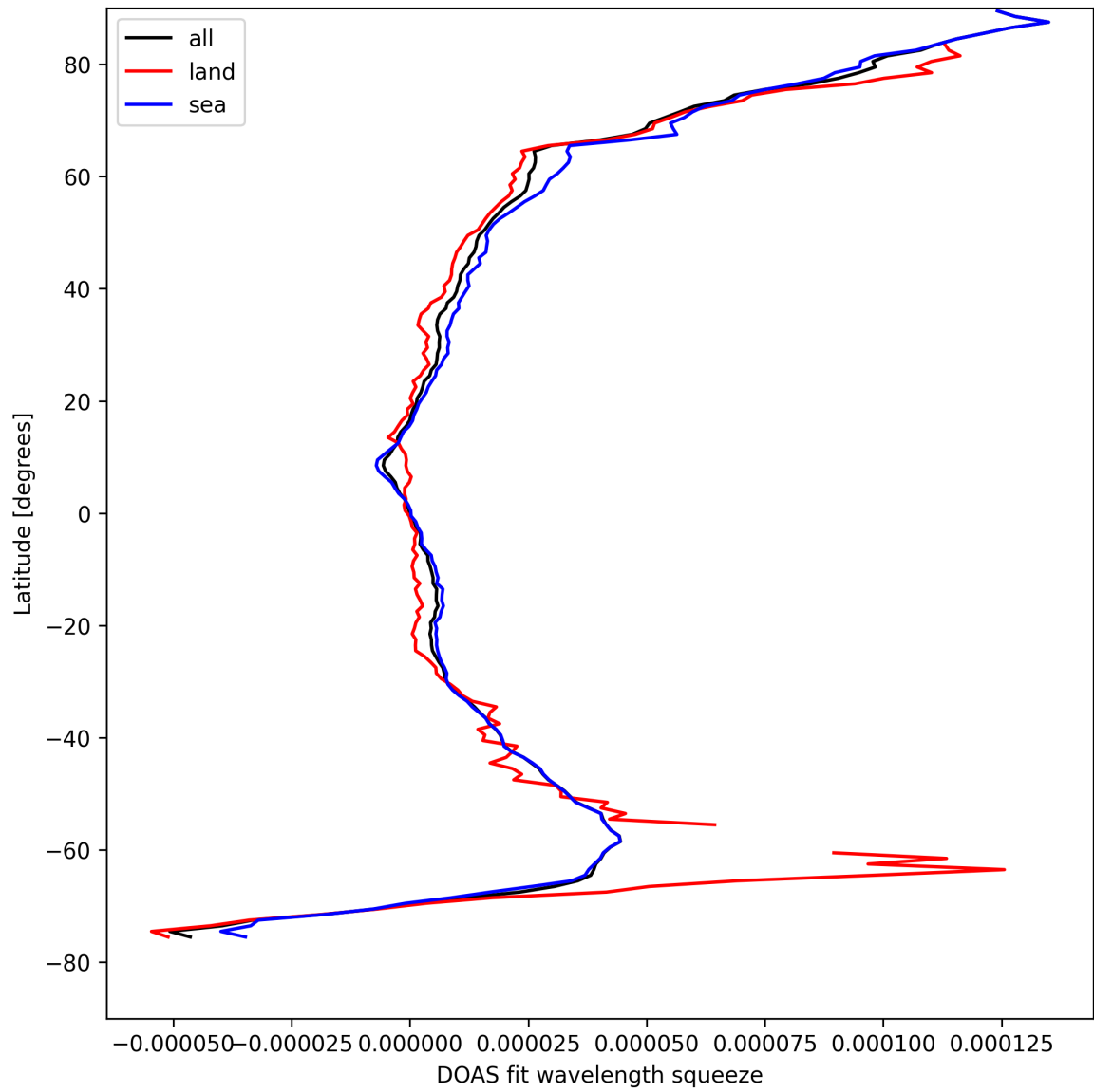
Figure 29: Zonal average of “DOAS fit wavelength squeeze” for 2025-08-28 to 2025-08-28.
