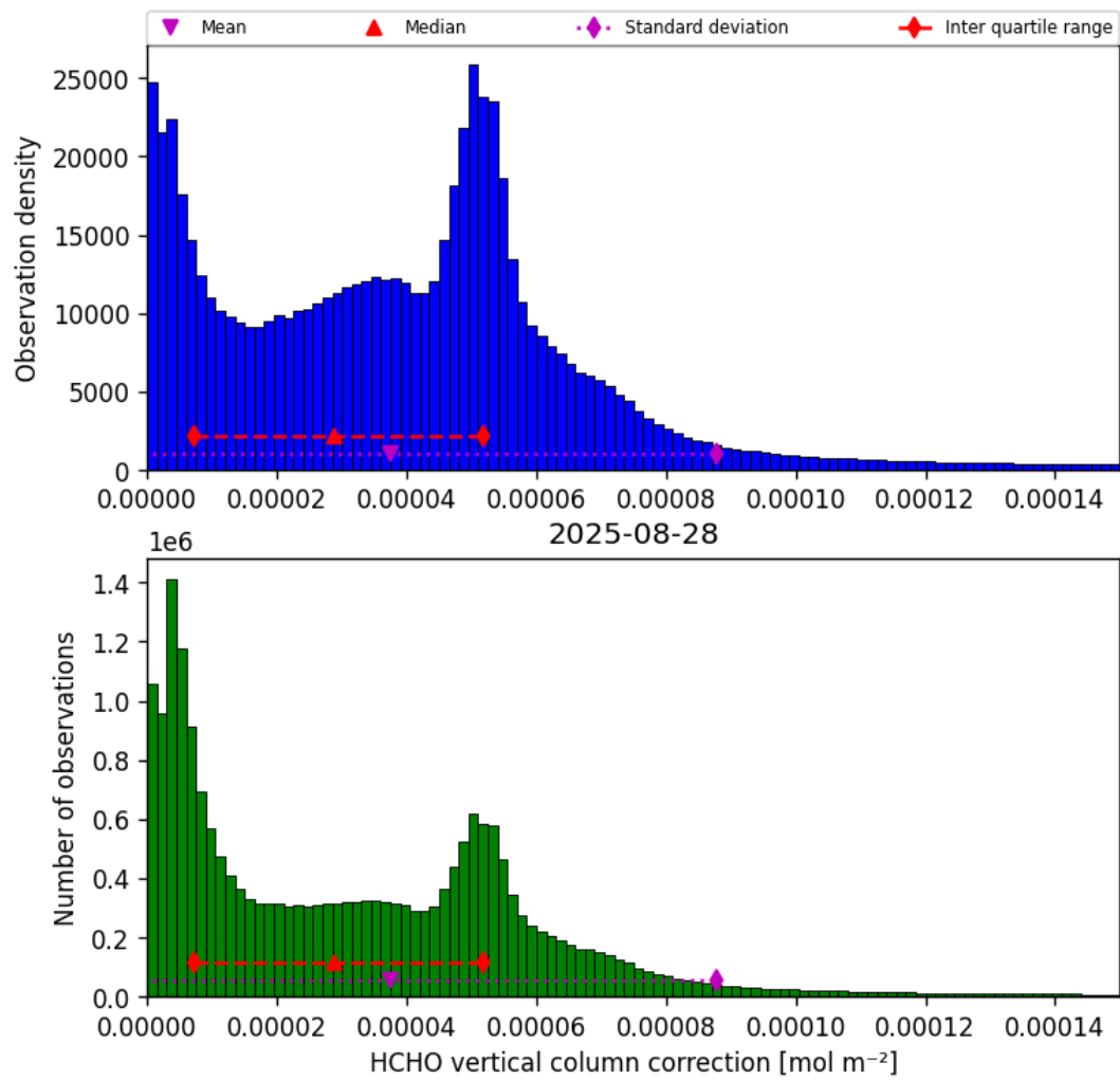
Figure 35: Histogram of “HCHO vertical column correction” for 2025-08-28 to 2025-08-28
