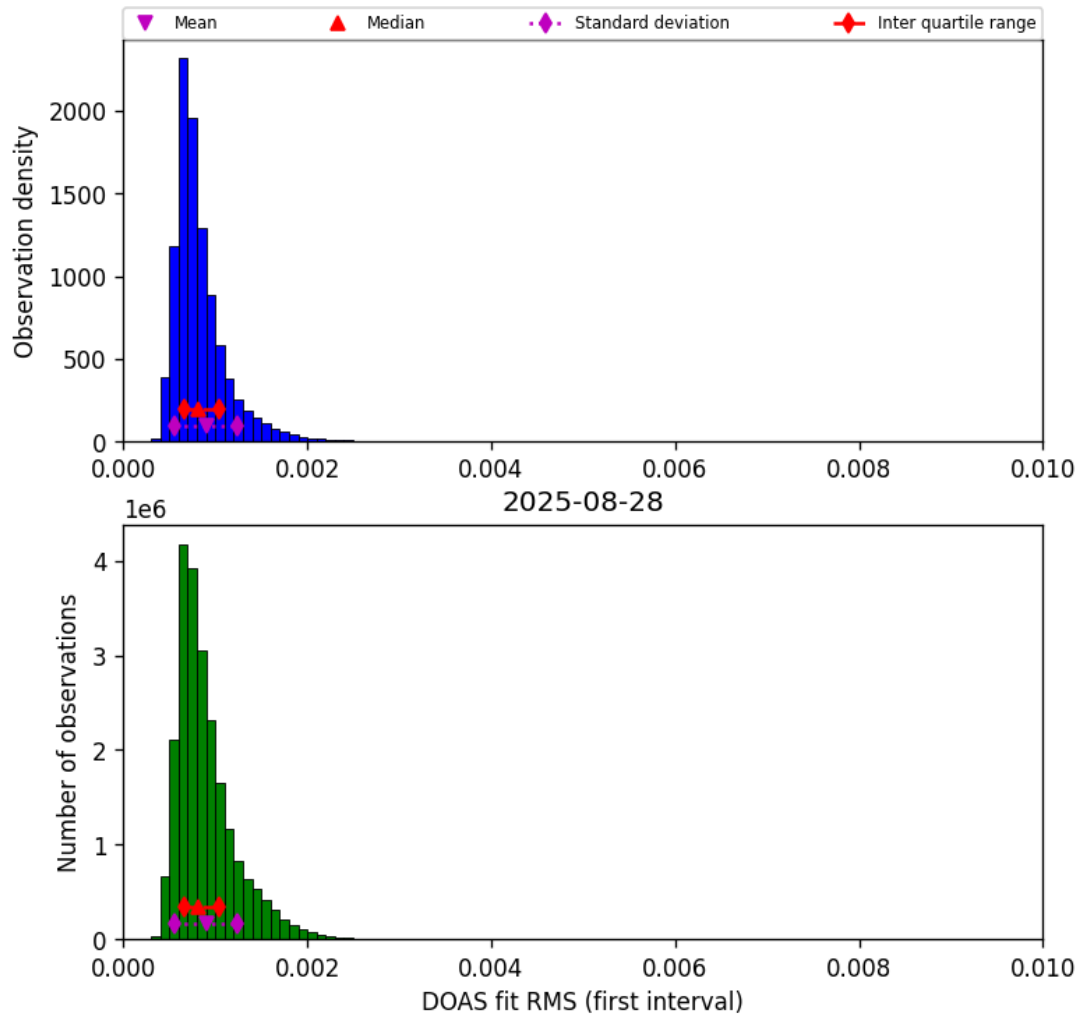
Figure 44: Histogram of “DOAS fit RMS (first interval)” for 2025-08-28 to 2025-08-28
