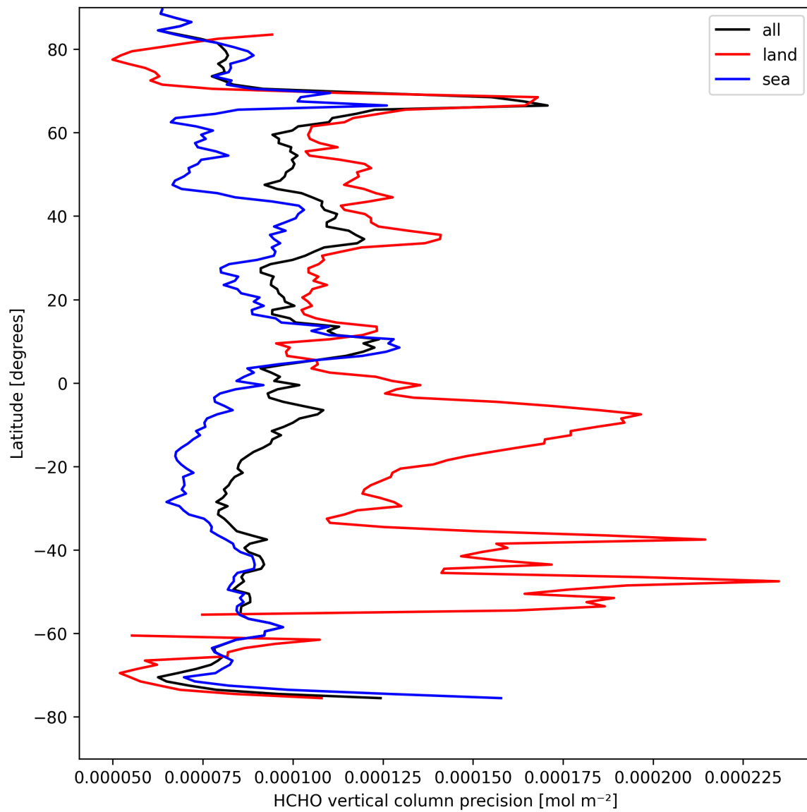
Figure 20: Zonal average of “HCHO vertical column precision” for 2025-08-28 to 2025-08-28.
