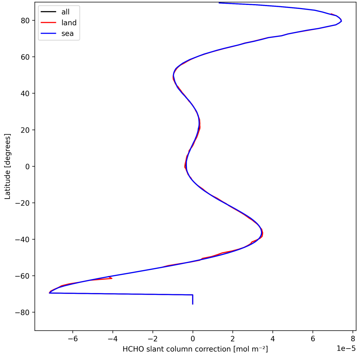
Figure 31: Zonal average of “HCHO slant column correction” for 2025-08-28 to 2025-08-28.
