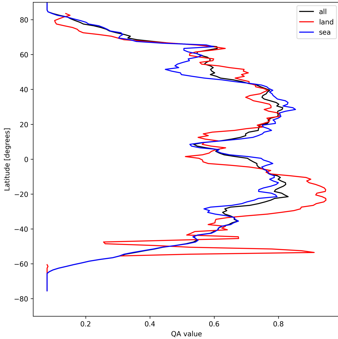
Figure 18: Zonal average of “QA value” for 2025-08-28 to 2025-08-28.
