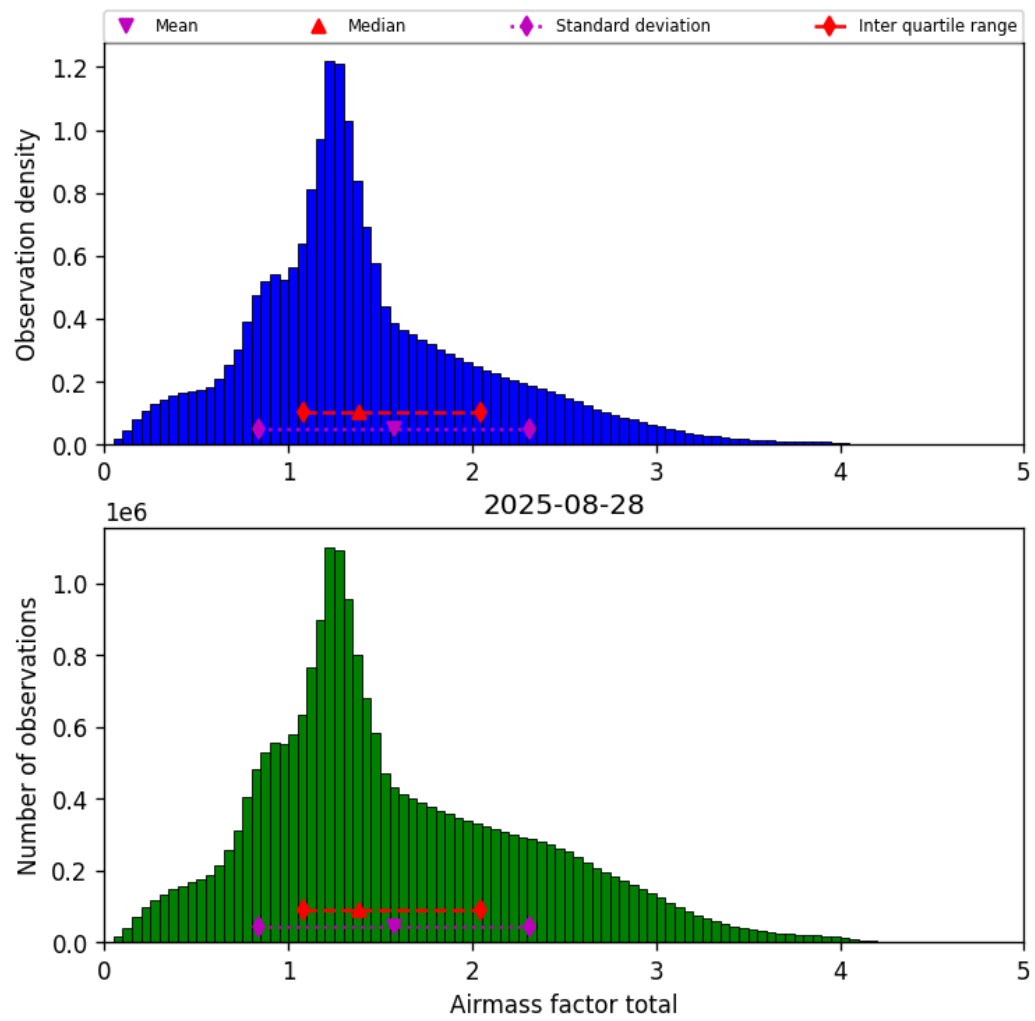
Figure 38: Histogram of “Airmass factor total” for 2025-08-28 to 2025-08-28
