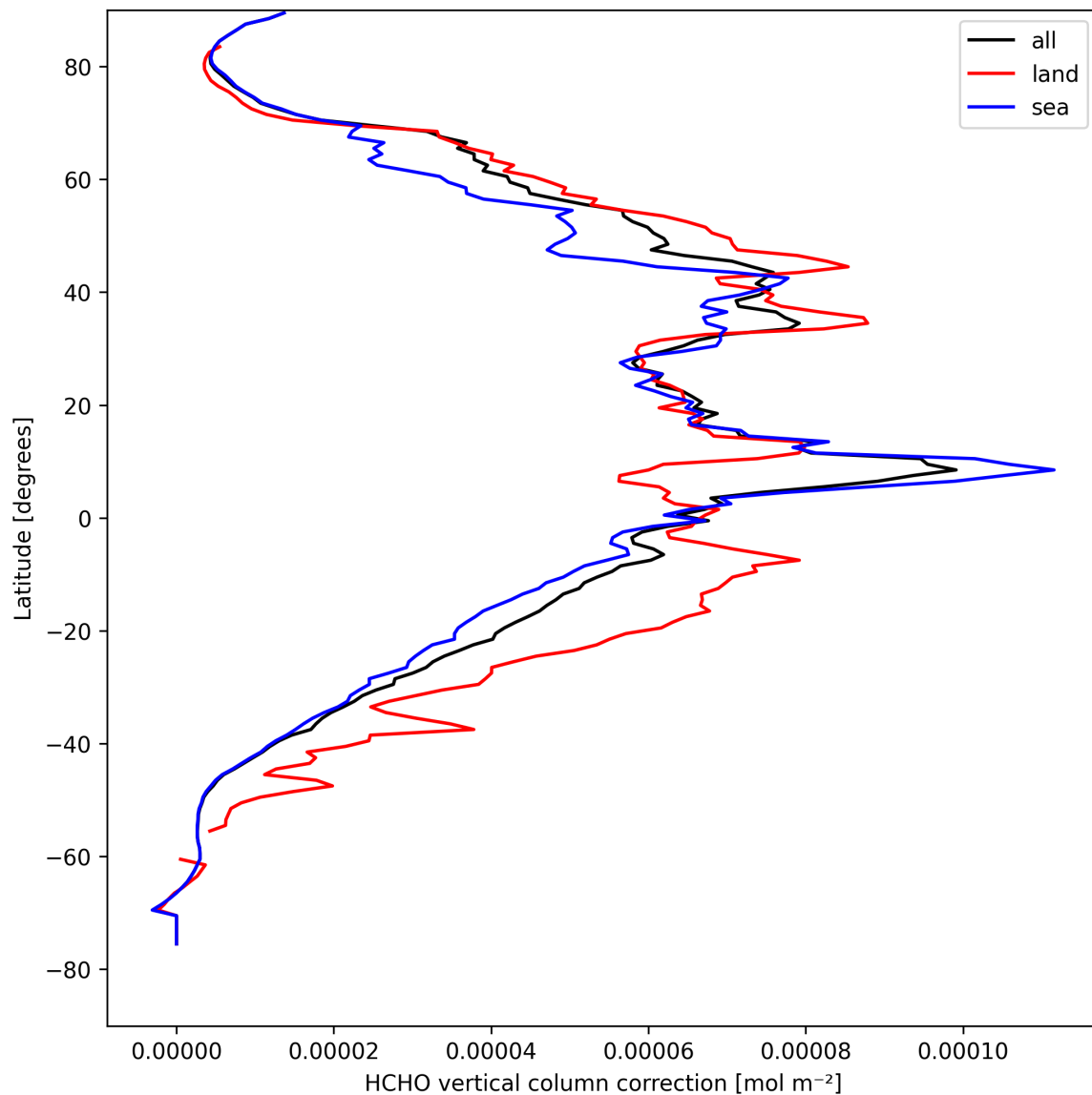
Figure 21: Zonal average of “HCHO vertical column correction” for 2025-08-28 to 2025-08-28.
