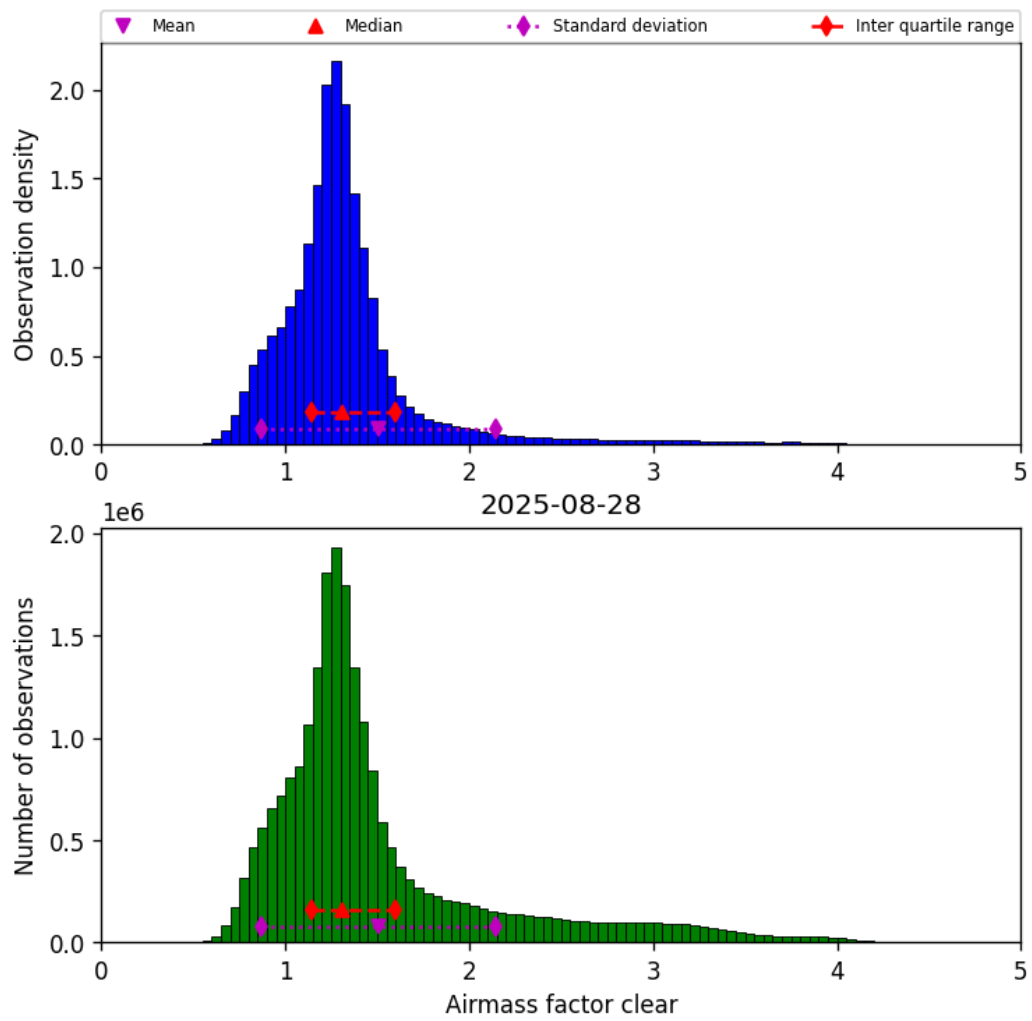
Figure 40: Histogram of “Airmass factor clear” for 2025-08-28 to 2025-08-28
