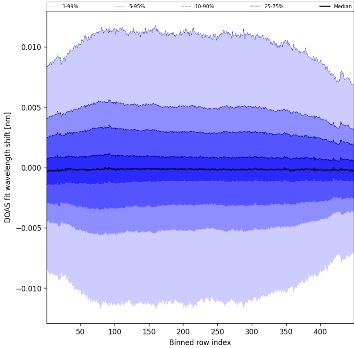
Figure 56: Along track statistics of “DOAS fit wavelength shift” for 2025-08-28 to 2025-08-28
