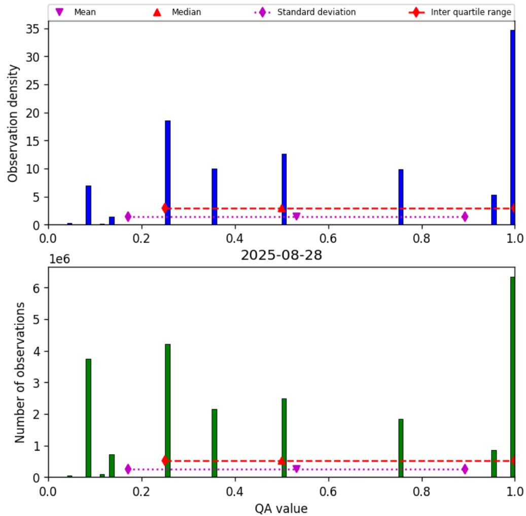
Figure 32: Histogram of “QA value” for 2025-08-28 to 2025-08-28
