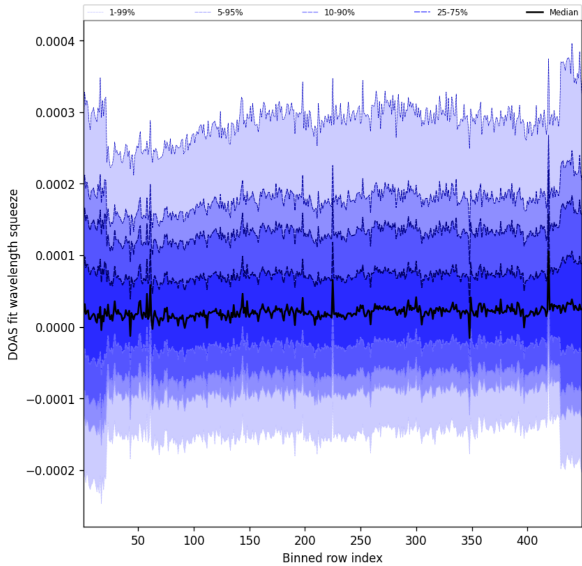
Figure 57: Along track statistics of “DOAS fit wavelength squeeze” for 2025-08-28 to 2025-08-28
