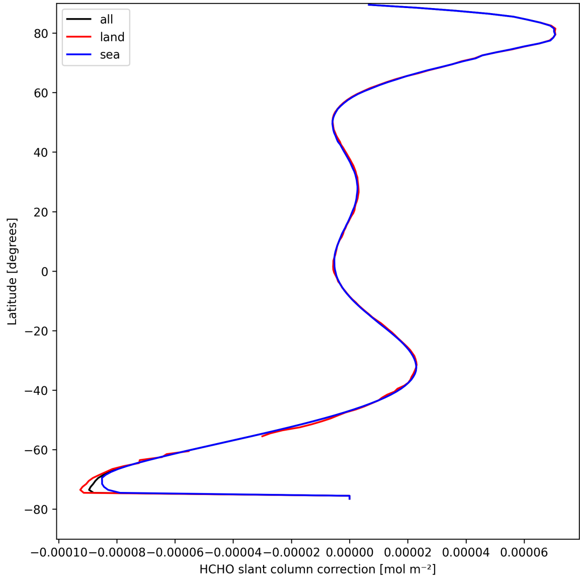
Figure 31: Zonal average of "HCHO slant column correction" for 2025-08-31 to 2025-09-01.
