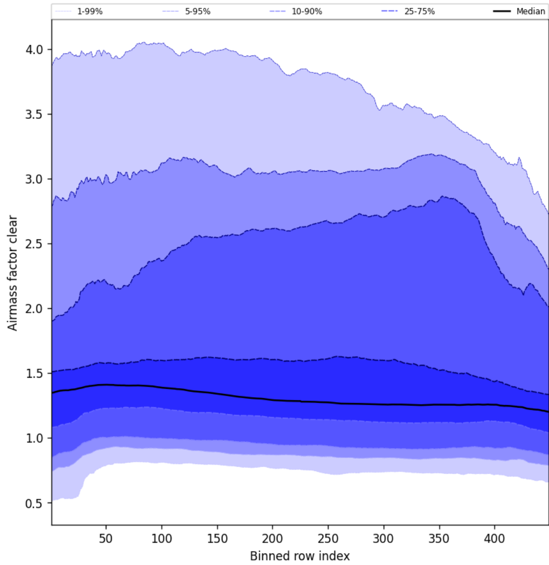
Figure 54: Along track statistics of “Airmass factor clear” for 2025-08-31 to 2025-09-01
