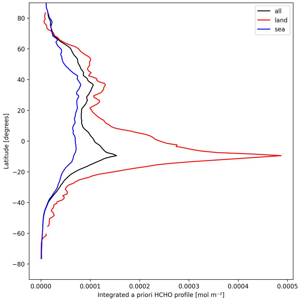
Figure 27: Zonal average of “Integrated a priori HCHO profile” for 2025-08-31 to 2025-09-01.
