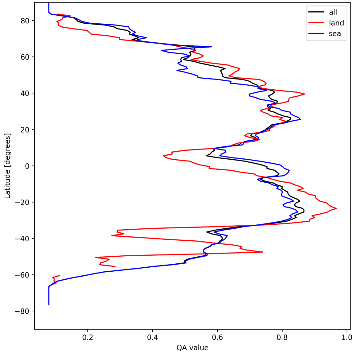
Figure 18: Zonal average of “QA value” for 2025-08-31 to 2025-09-01.
