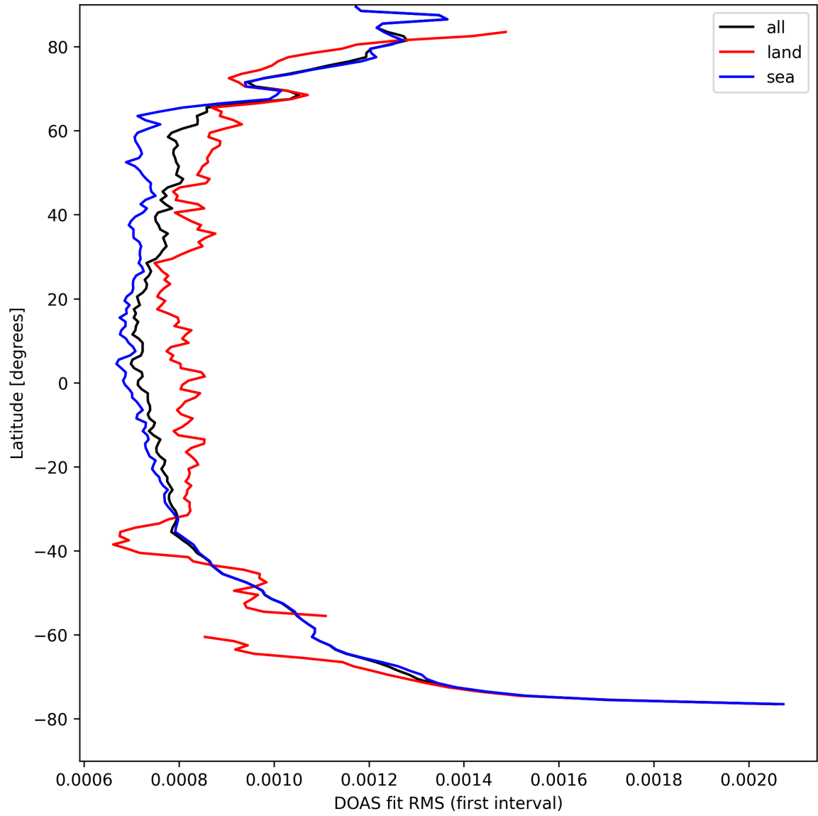
Figure 30: Zonal average of “DOAS fit RMS (first interval)” for 2025-08-31 to 2025-09-01.
