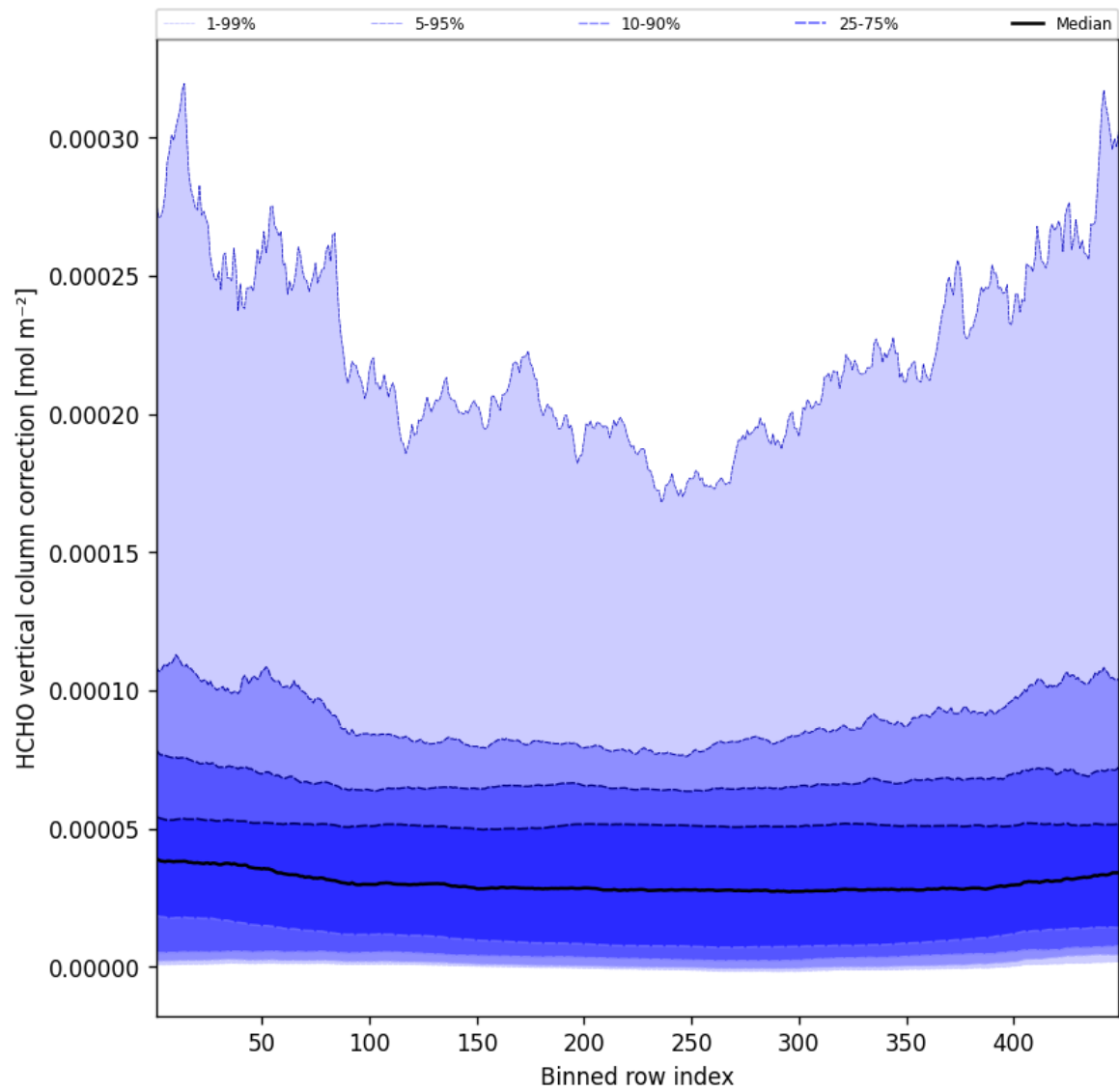
Figure 49: Along track statistics of “HCHO vertical column correction” for 2025-08-31 to 2025-09-01
