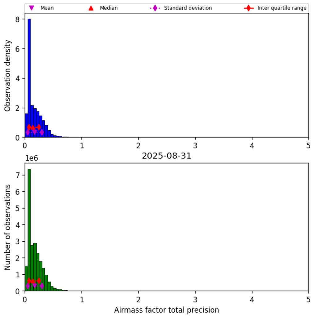
Figure 39: Histogram of “Airmass factor total precision” for 2025-08-31 to 2025-09-01
