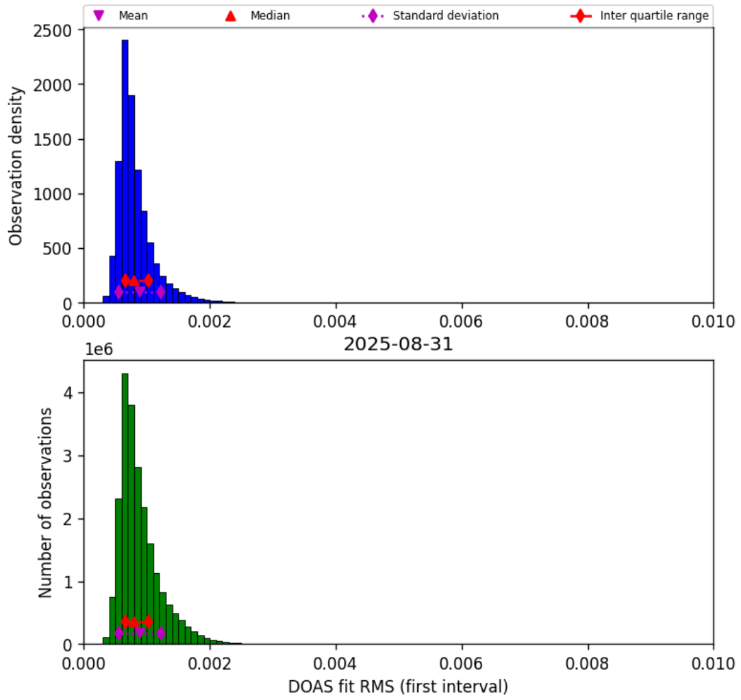
Figure 44: Histogram of “DOAS fit RMS (first interval)” for 2025-08-31 to 2025-09-01
