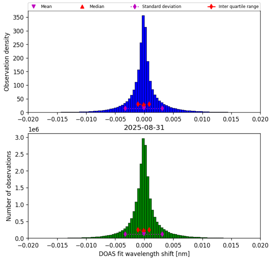
Figure 42: Histogram of “DOAS fit wavelength shift” for 2025-08-31 to 2025-09-01
