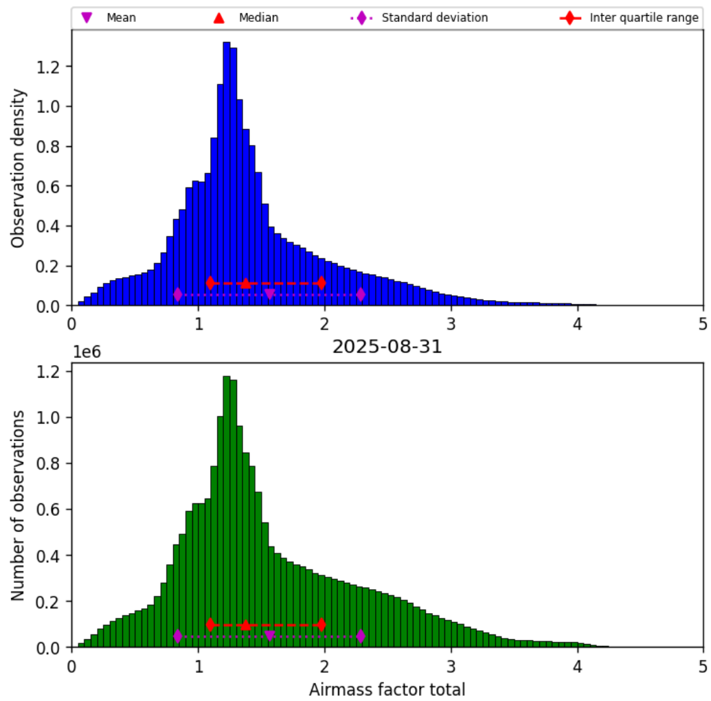
Figure 38: Histogram of “Airmass factor total” for 2025-08-31 to 2025-09-01
