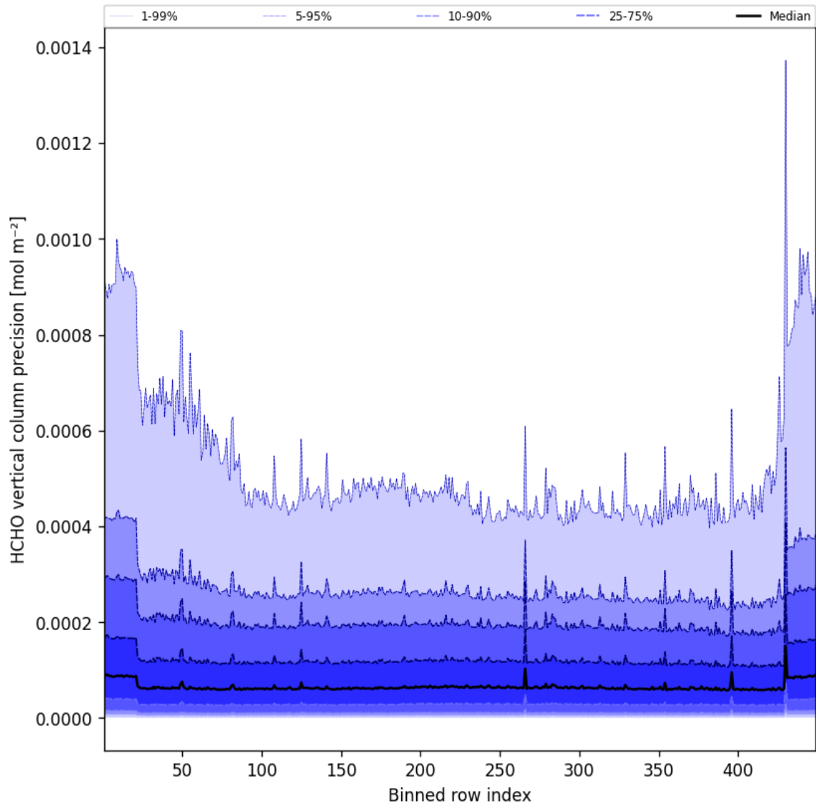
Figure 48: Along track statistics of “HCHO vertical column precision” for 2025-08-31 to 2025-09-01
