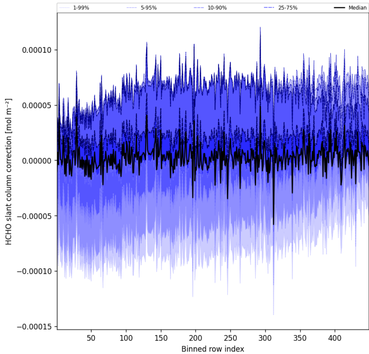
Figure 59: Along track statistics of “HCHO slant column correction” for 2025-08-31 to 2025-09-01
