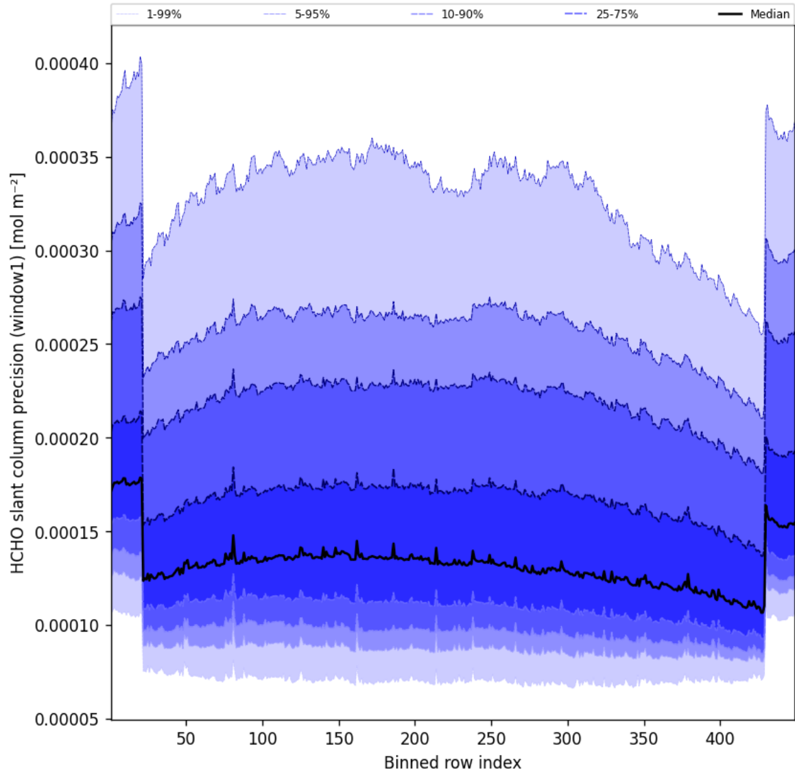
Figure 51: Along track statistics of “HCHO slant column precision (window1)” for 2025-08-31 to 2025-09-01
