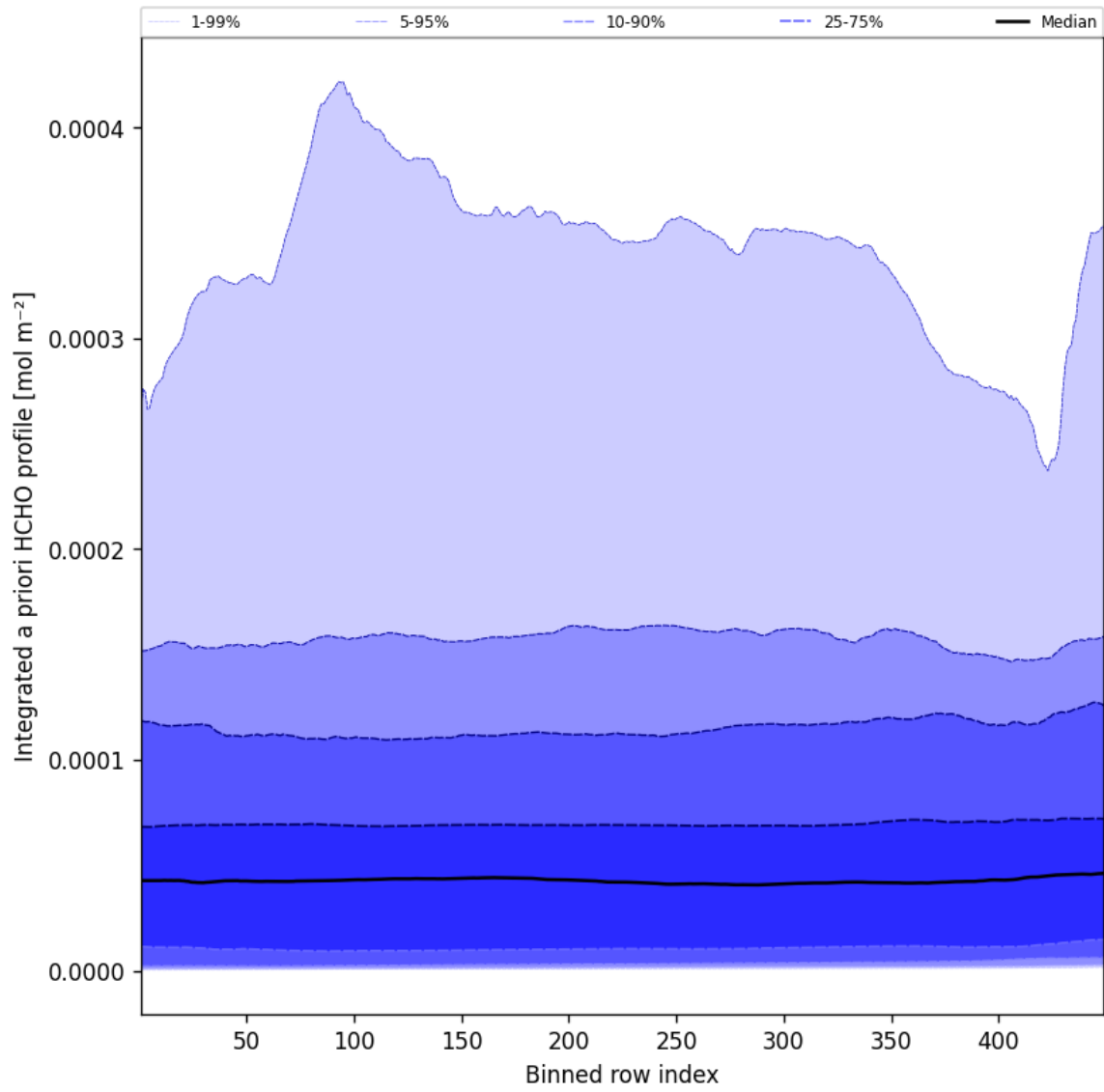
Figure 55: Along track statistics of “Integrated a priori HCHO profile” for 2025-08-31 to 2025-09-01
