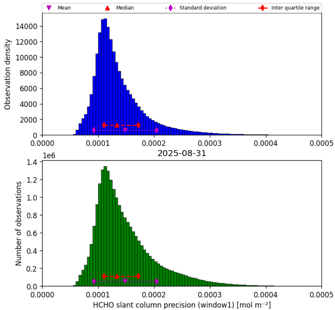
Figure 37: Histogram of “HCHO slant column precision (window1)” for 2025-08-31 to 2025-09-01
