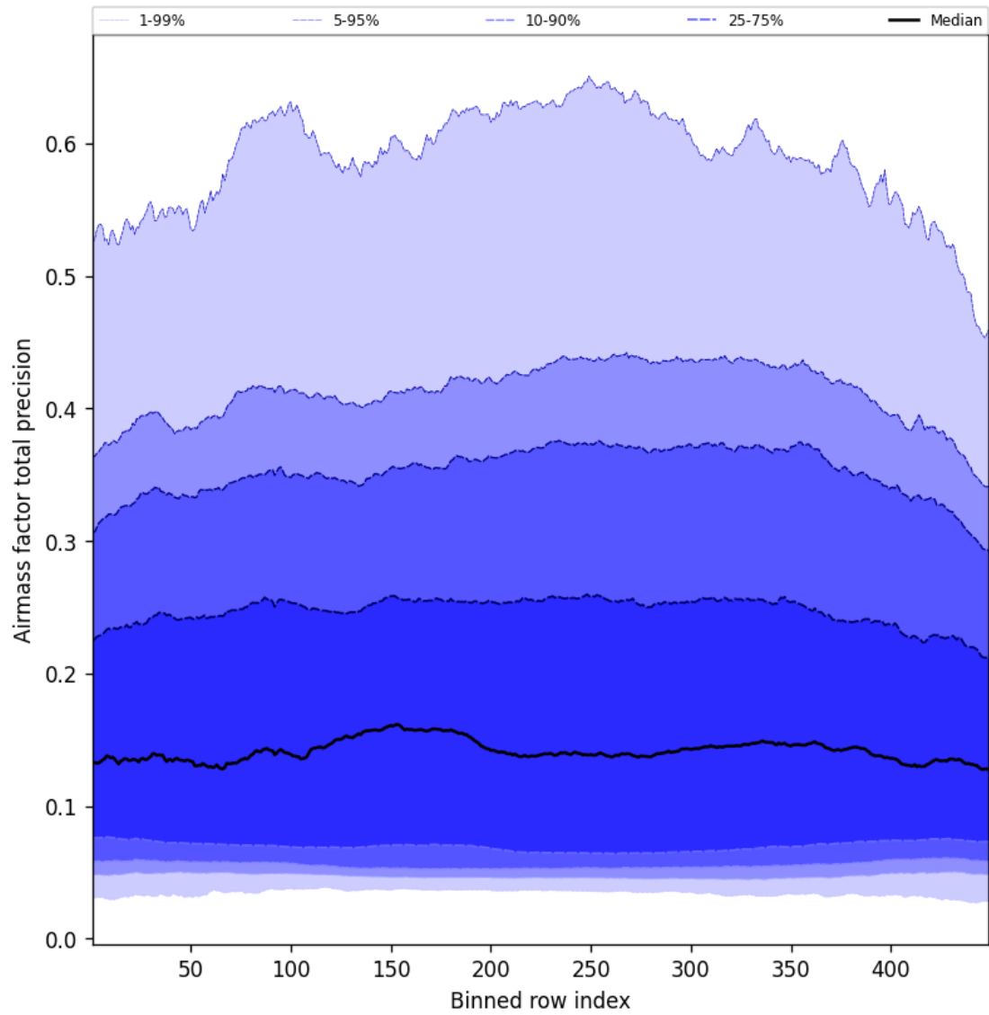
Figure 53: Along track statistics of “Airmass factor total precision” for 2025-08-31 to 2025-09-01
