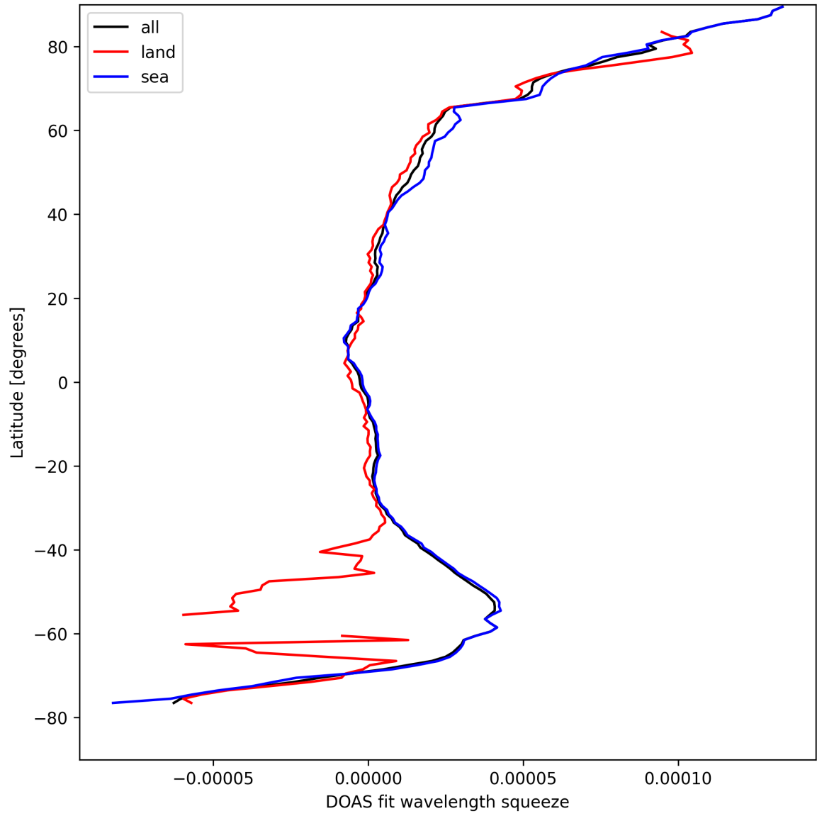
Figure 29: Zonal average of "DOAS fit wavelength squeeze" for 2025-08-31 to 2025-09-01.
