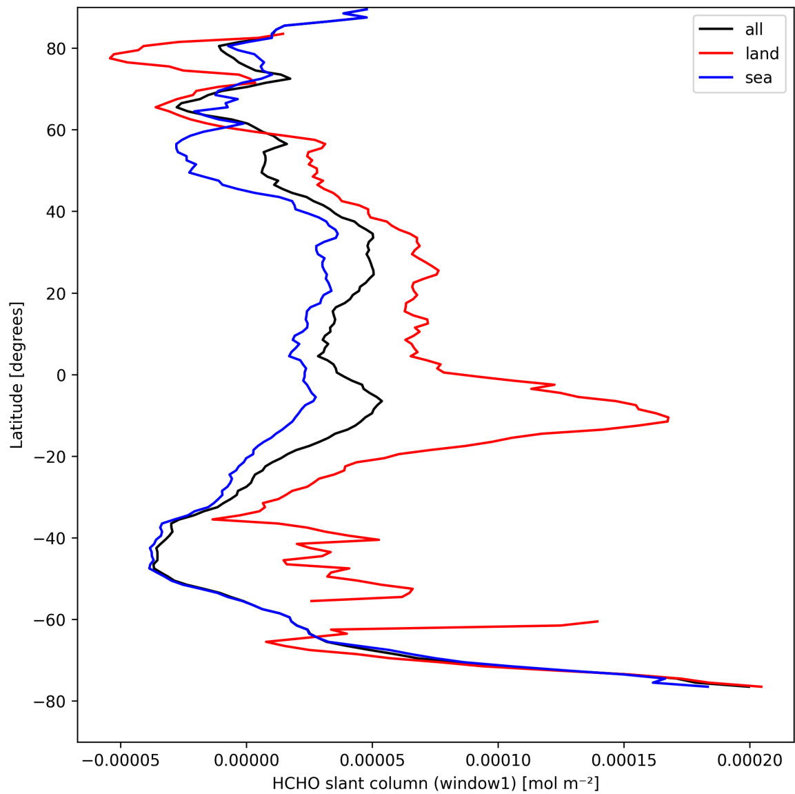
Figure 22: Zonal average of “HCHO slant column (window1)” for 2025-08-31 to 2025-09-01.
