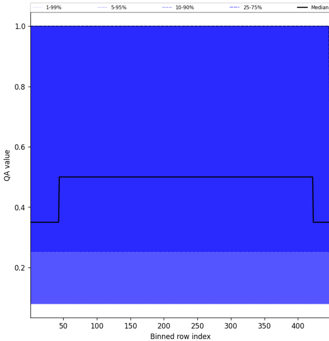
Figure 46: Along track statistics of “QA value” for 2025-08-31 to 2025-09-01
