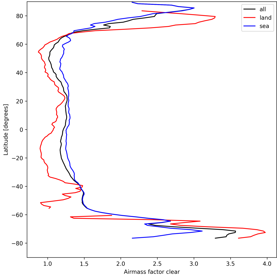
Figure 26: Zonal average of “Airmass factor clear” for 2025-08-31 to 2025-09-01.
