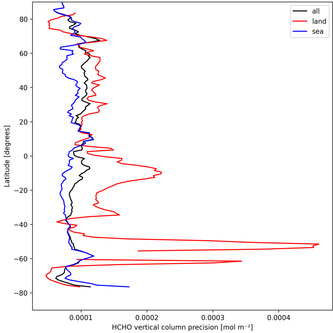
Figure 20: Zonal average of “HCHO vertical column precision” for 2025-08-31 to 2025-09-01.
