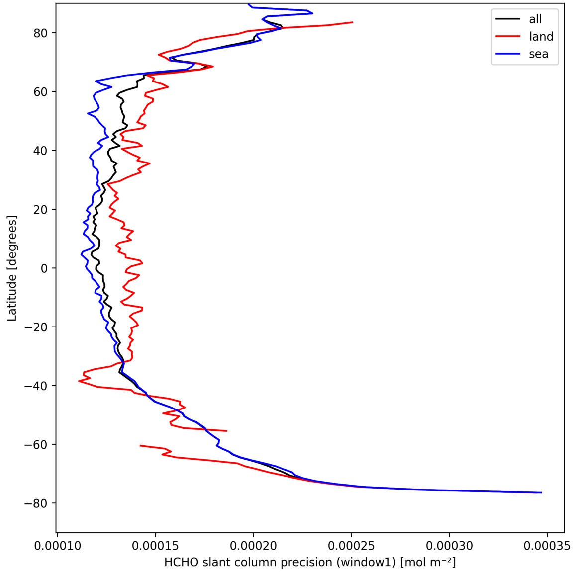
Figure 23: Zonal average of “HCHO slant column precision (window1)” for 2025-08-31 to 2025-09-01.
