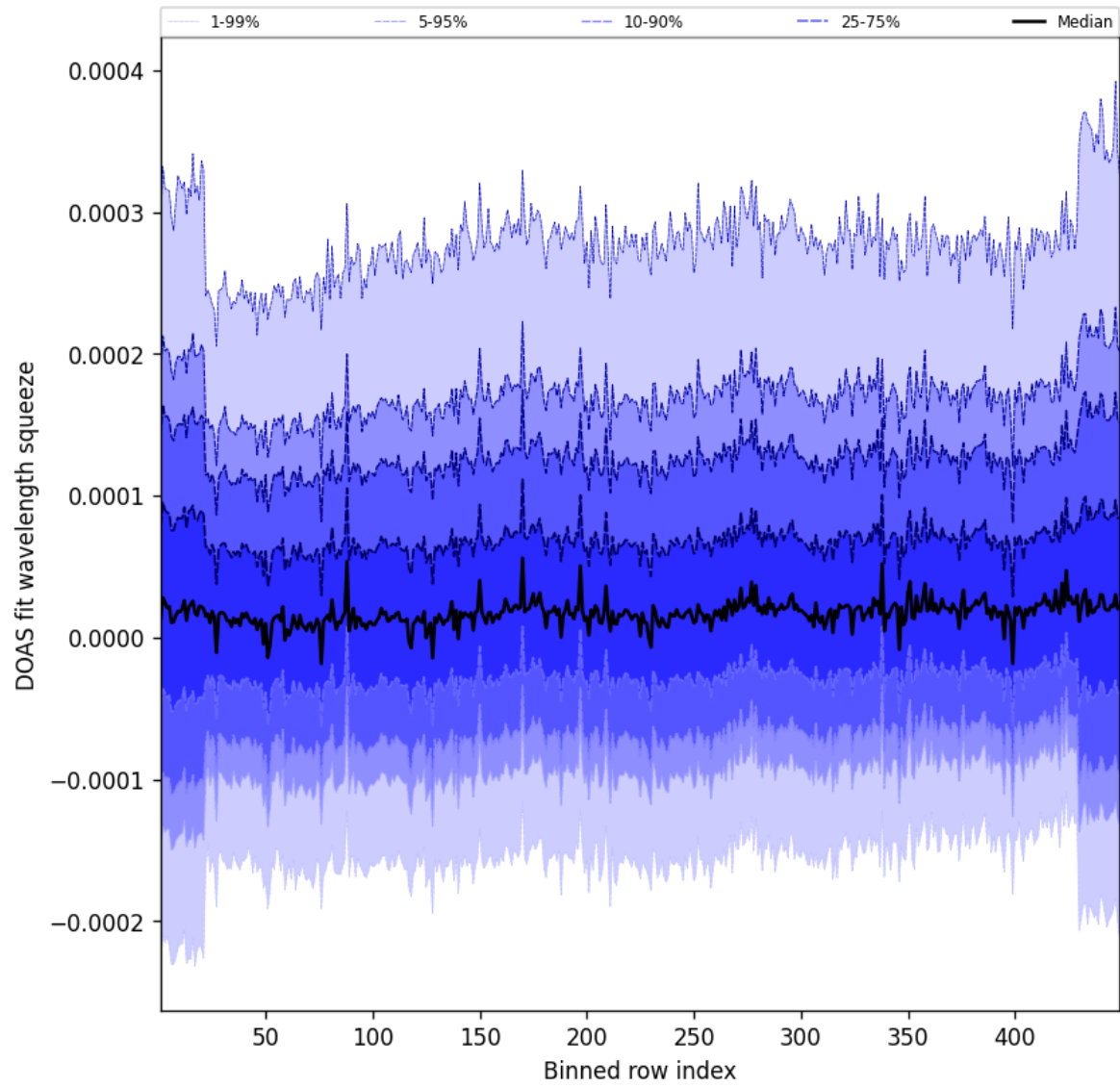
Figure 57: Along track statistics of “DOAS fit wavelength squeeze” for 2025-08-31 to 2025-09-01
