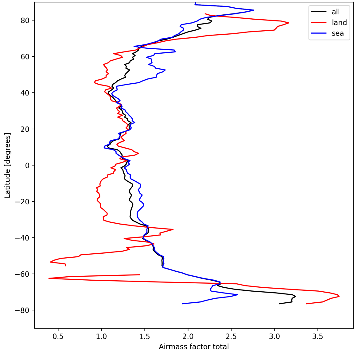
Figure 24: Zonal average of “Airmass factor total” for 2025-08-31 to 2025-09-01.
