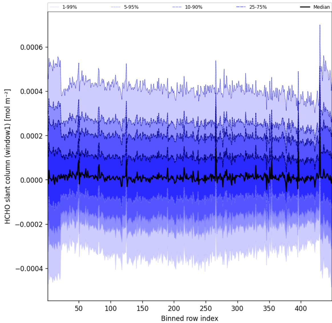
Figure 50: Along track statistics of “HCHO slant column (window1)” for 2025-08-31 to 2025-09-01
