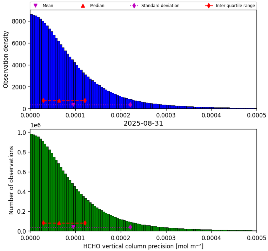
Figure 34: Histogram of “HCHO vertical column precision” for 2025-08-31 to 2025-09-01
