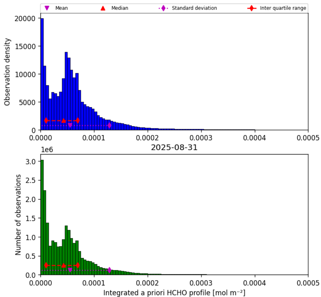
Figure 41: Histogram of “Integrated a priori HCHO profile” for 2025-08-31 to 2025-09-01
