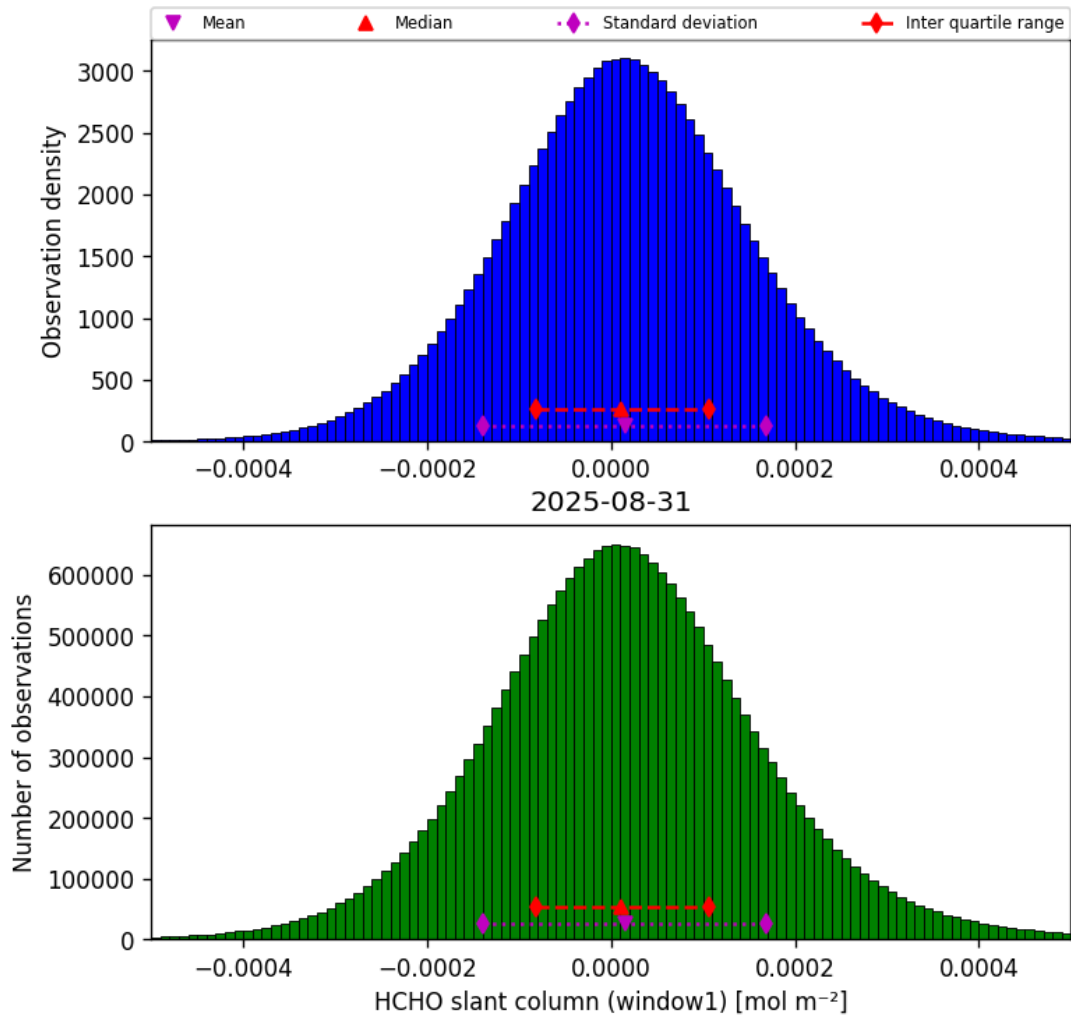
Figure 36: Histogram of “HCHO slant column (window1)” for 2025-08-31 to 2025-09-01
