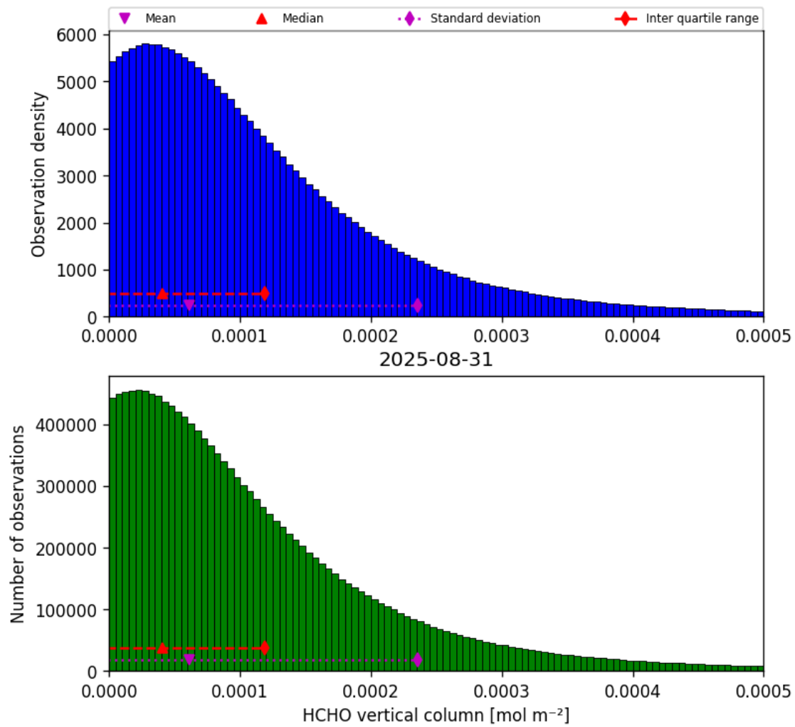
Figure 33: Histogram of “HCHO vertical column” for 2025-08-31 to 2025-09-01
