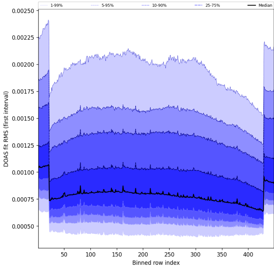
Figure 58: Along track statistics of “DOAS fit RMS (first interval)” for 2025-08-31 to 2025-09-01
