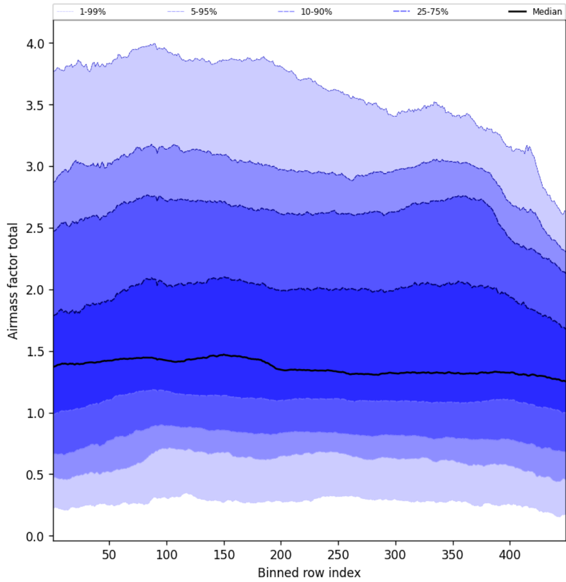
Figure 52: Along track statistics of “Airmass factor total” for 2025-08-31 to 2025-09-01
