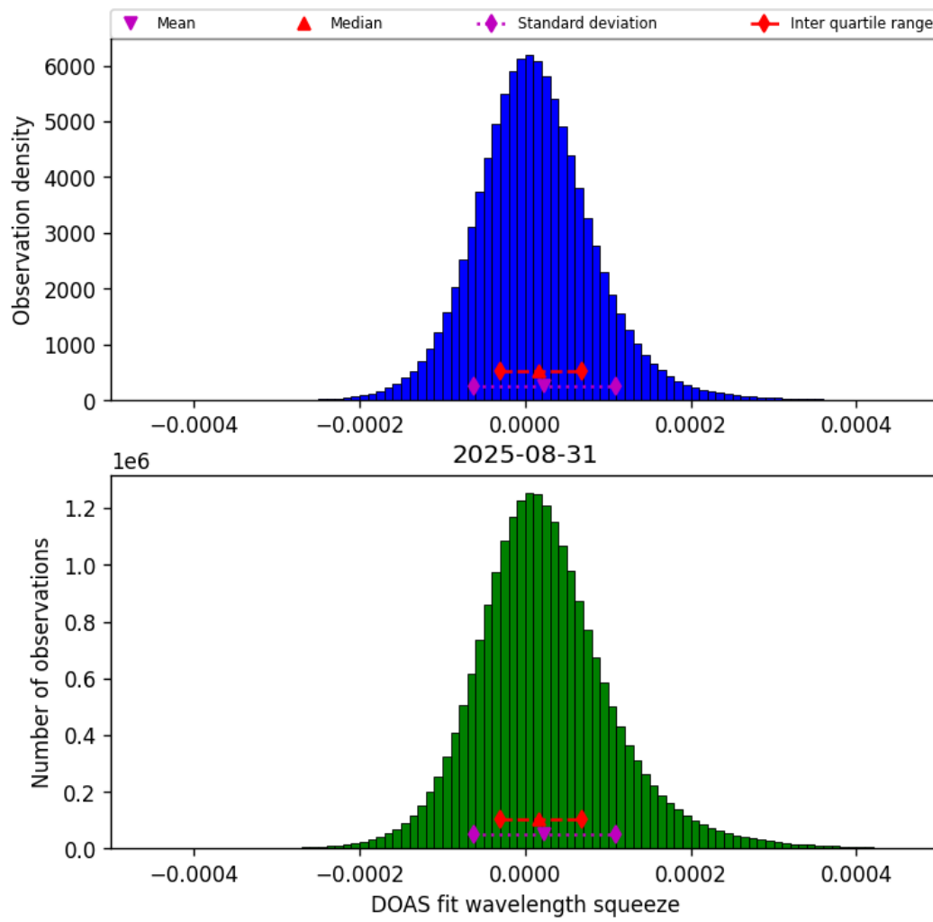
Figure 43: Histogram of “DOAS fit wavelength squeeze” for 2025-08-31 to 2025-09-01
