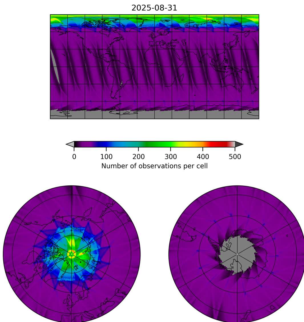
Figure 17: Map of the number of observations for 2025-08-31 to 2025-09-01
