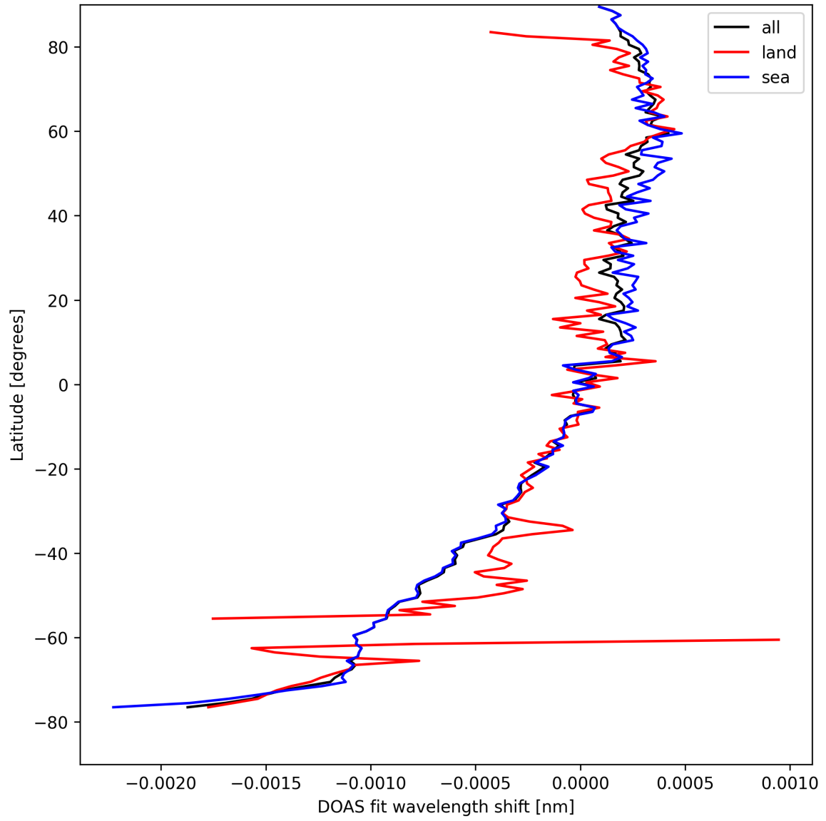
Figure 28: Zonal average of “DOAS fit wavelength shift” for 2025-08-31 to 2025-09-01.
