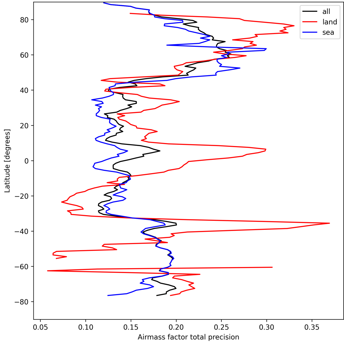
Figure 25: Zonal average of “Airmass factor total precision” for 2025-08-31 to 2025-09-01.
