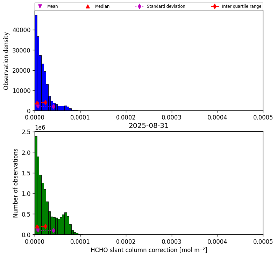
Figure 45: Histogram of “HCHO slant column correction” for 2025-08-31 to 2025-09-01
