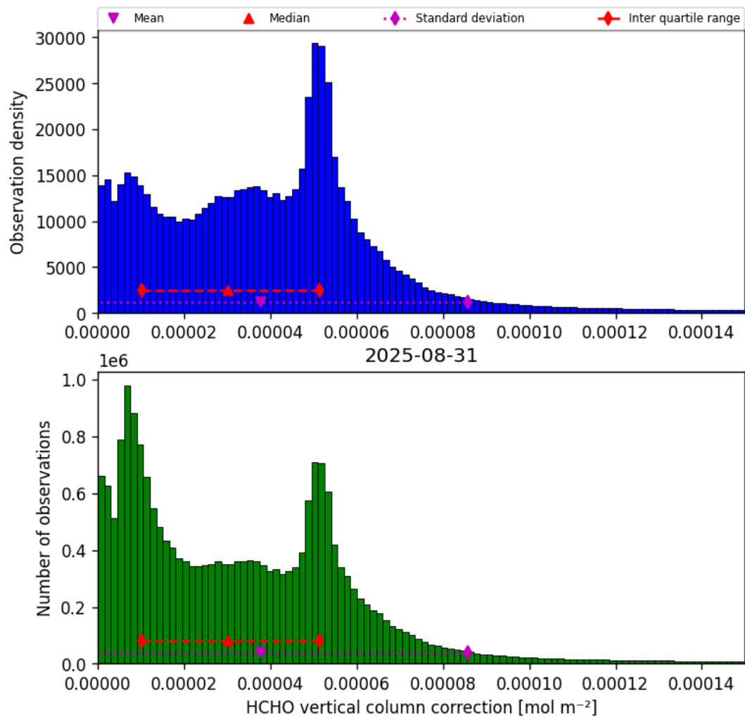
Figure 35: Histogram of “HCHO vertical column correction” for 2025-08-31 to 2025-09-01
