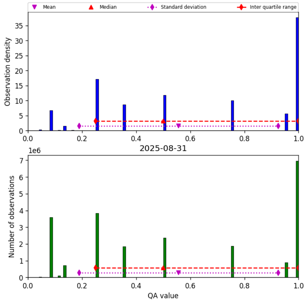
Figure 32: Histogram of “QA value” for 2025-08-31 to 2025-09-01
