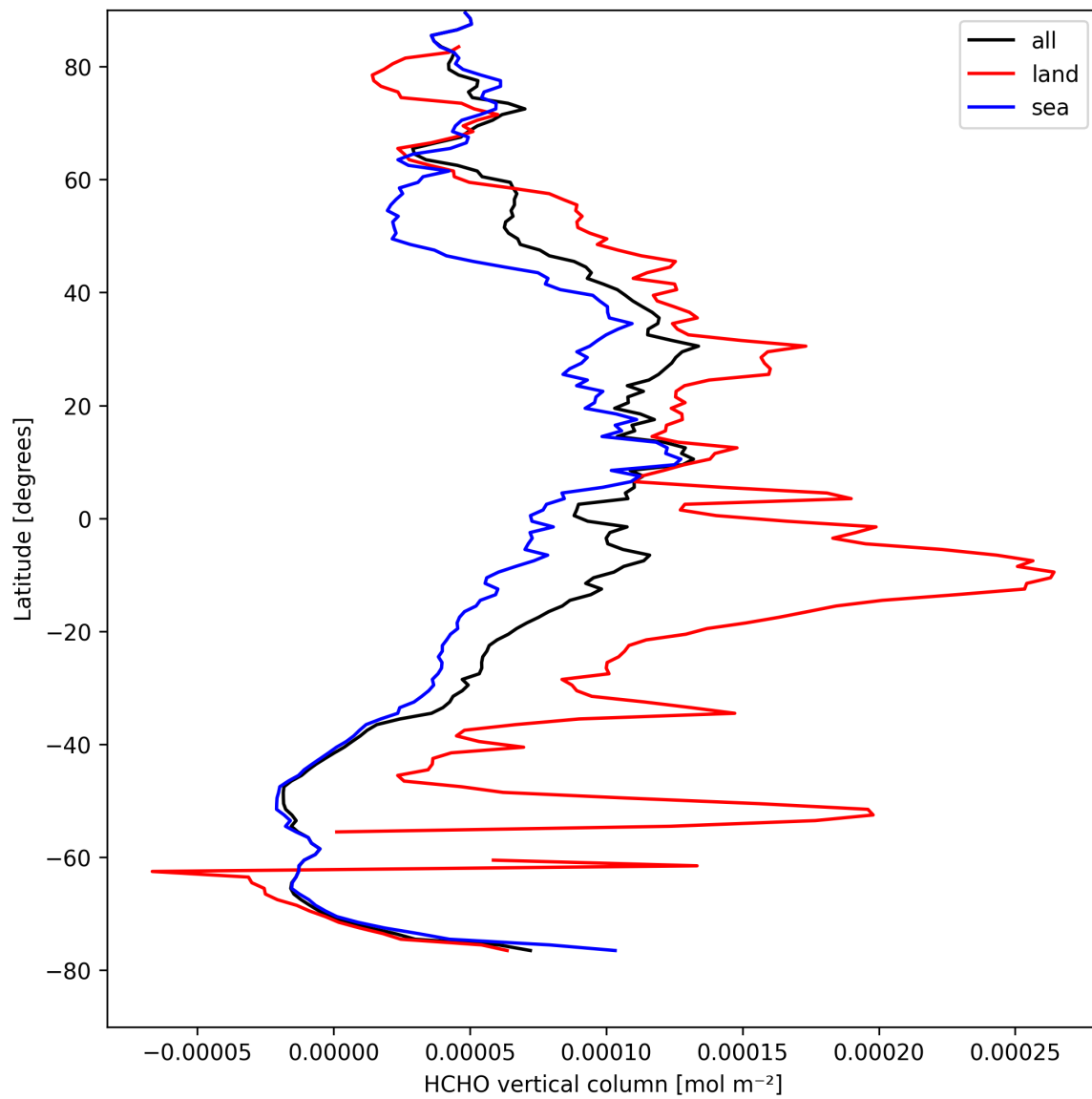
Figure 19: Zonal average of “HCHO vertical column” for 2025-08-31 to 2025-09-01.
