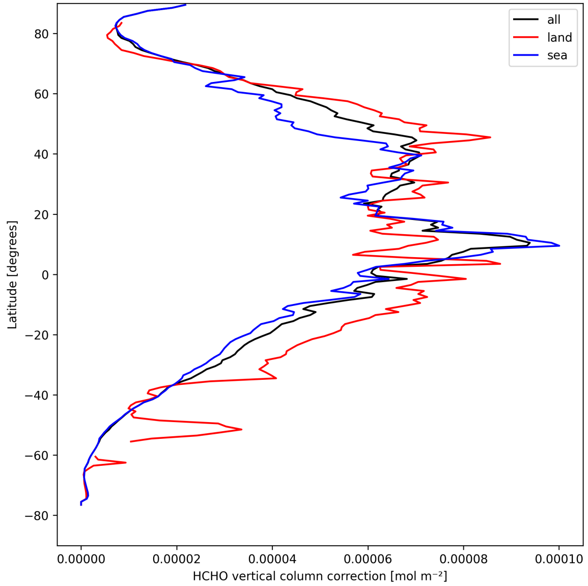
Figure 21: Zonal average of “HCHO vertical column correction” for 2025-08-31 to 2025-09-01.
