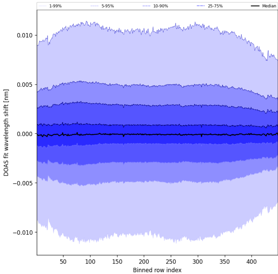
Figure 56: Along track statistics of “DOAS fit wavelength shift” for 2025-08-31 to 2025-09-01
