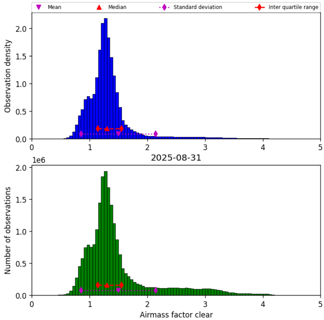
Figure 40: Histogram of “Airmass factor clear” for 2025-08-31 to 2025-09-01
