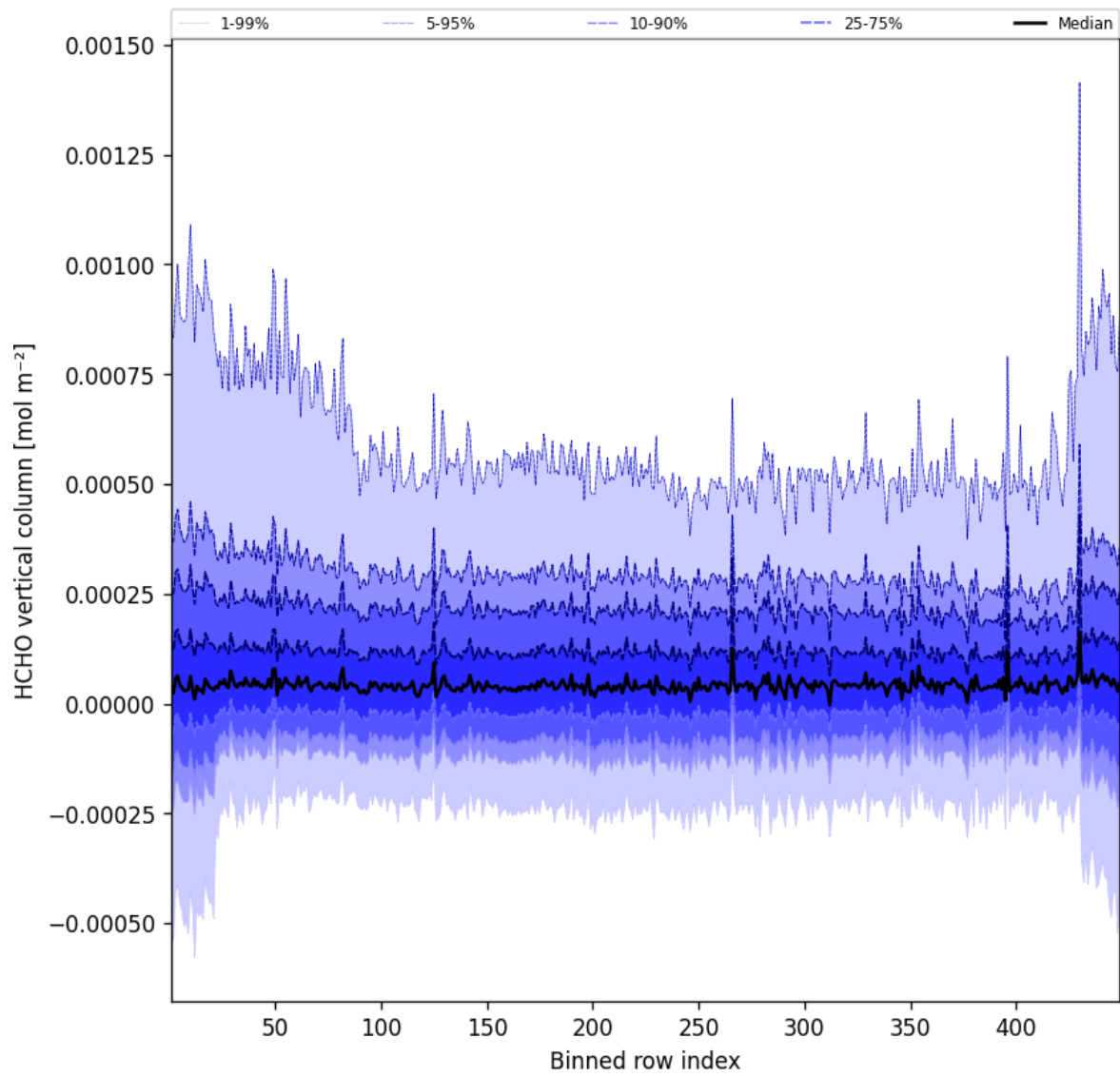
Figure 47: Along track statistics of “HCHO vertical column” for 2025-08-31 to 2025-09-01
