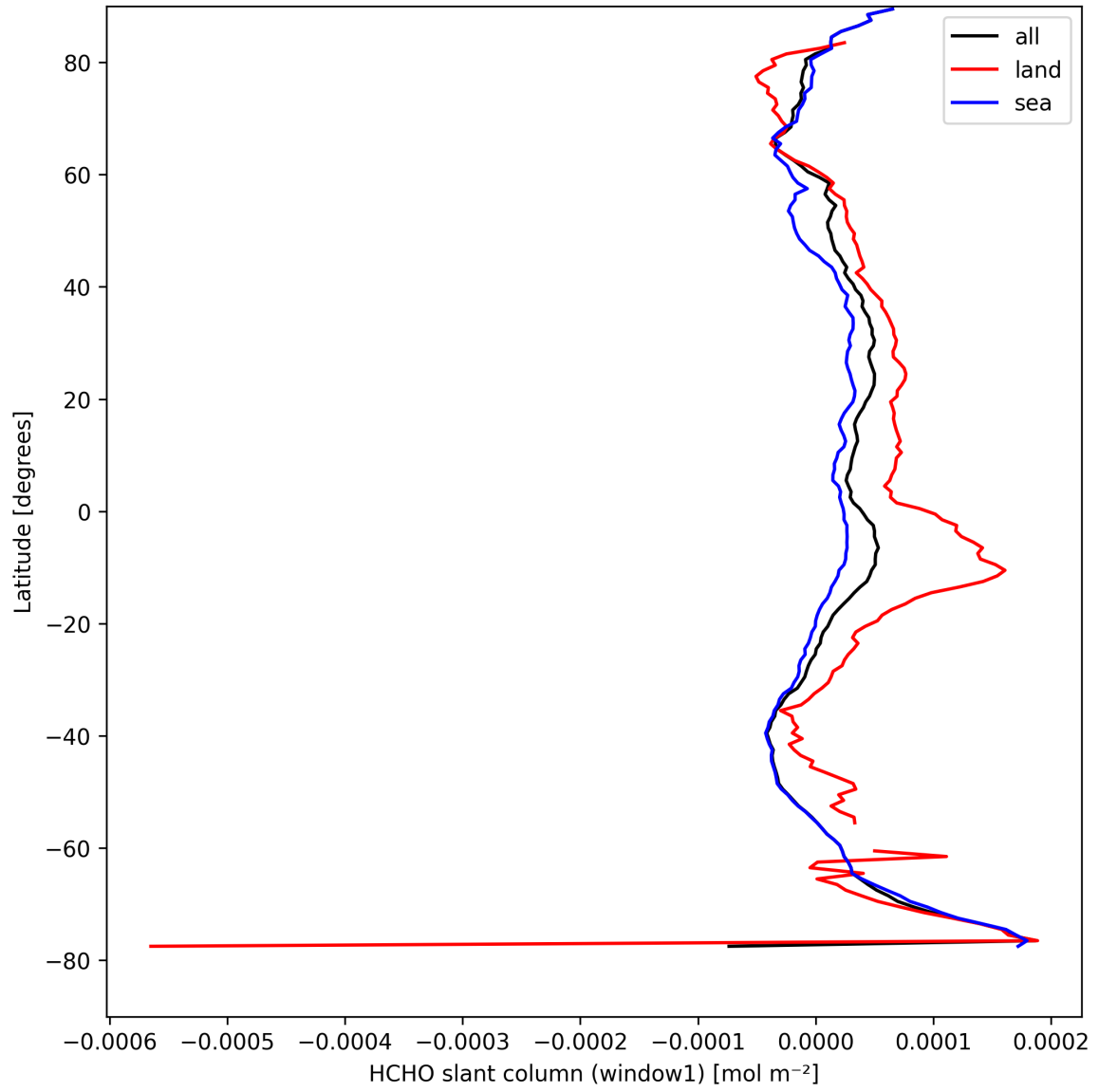
Figure 22: Zonal average of “HCHO slant column (window1)” for 2025-09-01 to 2025-09-02.
