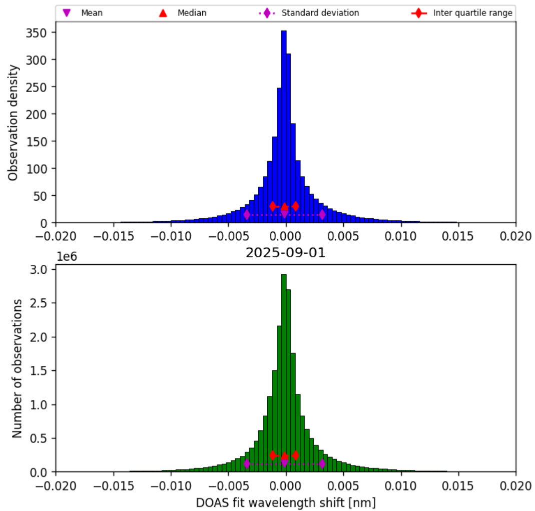
Figure 42: Histogram of “DOAS fit wavelength shift” for 2025-09-01 to 2025-09-02
