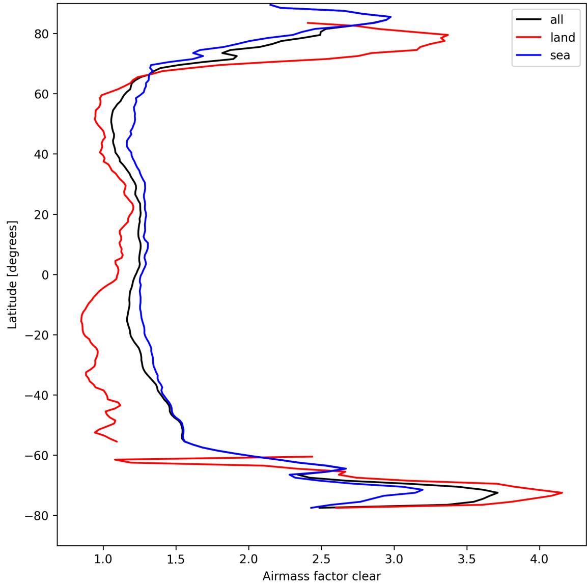
Figure 26: Zonal average of “Airmass factor clear” for 2025-09-01 to 2025-09-02.
