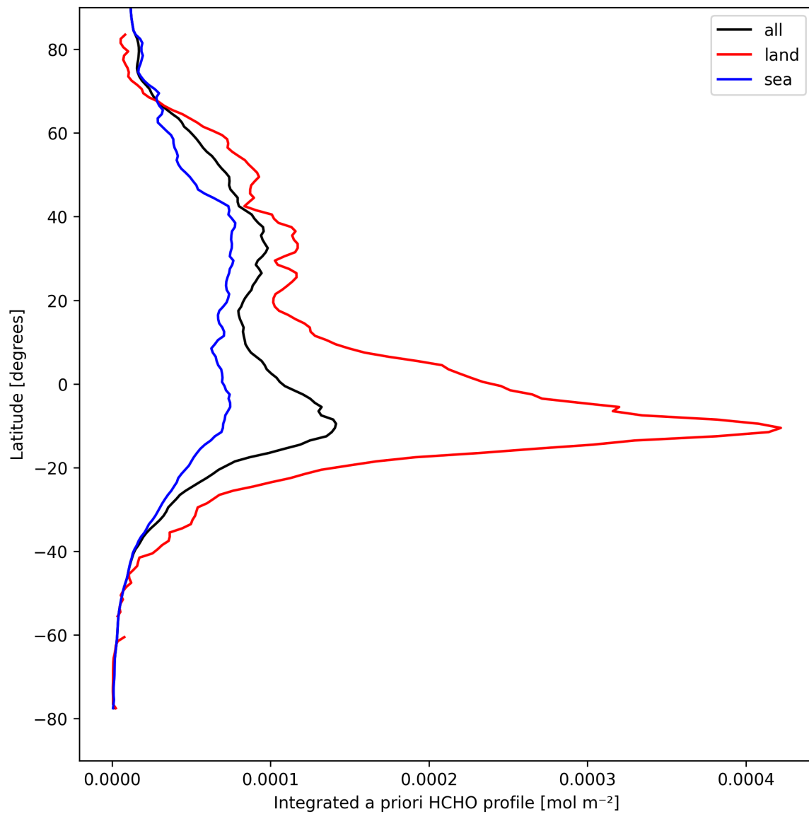
Figure 27: Zonal average of “Integrated a priori HCHO profile” for 2025-09-01 to 2025-09-02.
