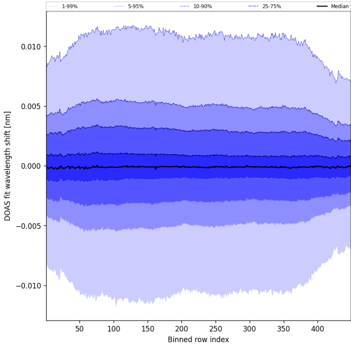
Figure 56: Along track statistics of “DOAS fit wavelength shift” for 2025-09-01 to 2025-09-02
