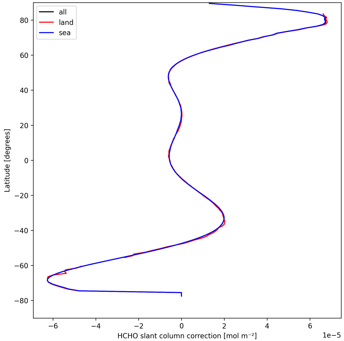
Figure 31: Zonal average of “HCHO slant column correction” for 2025-09-01 to 2025-09-02.
