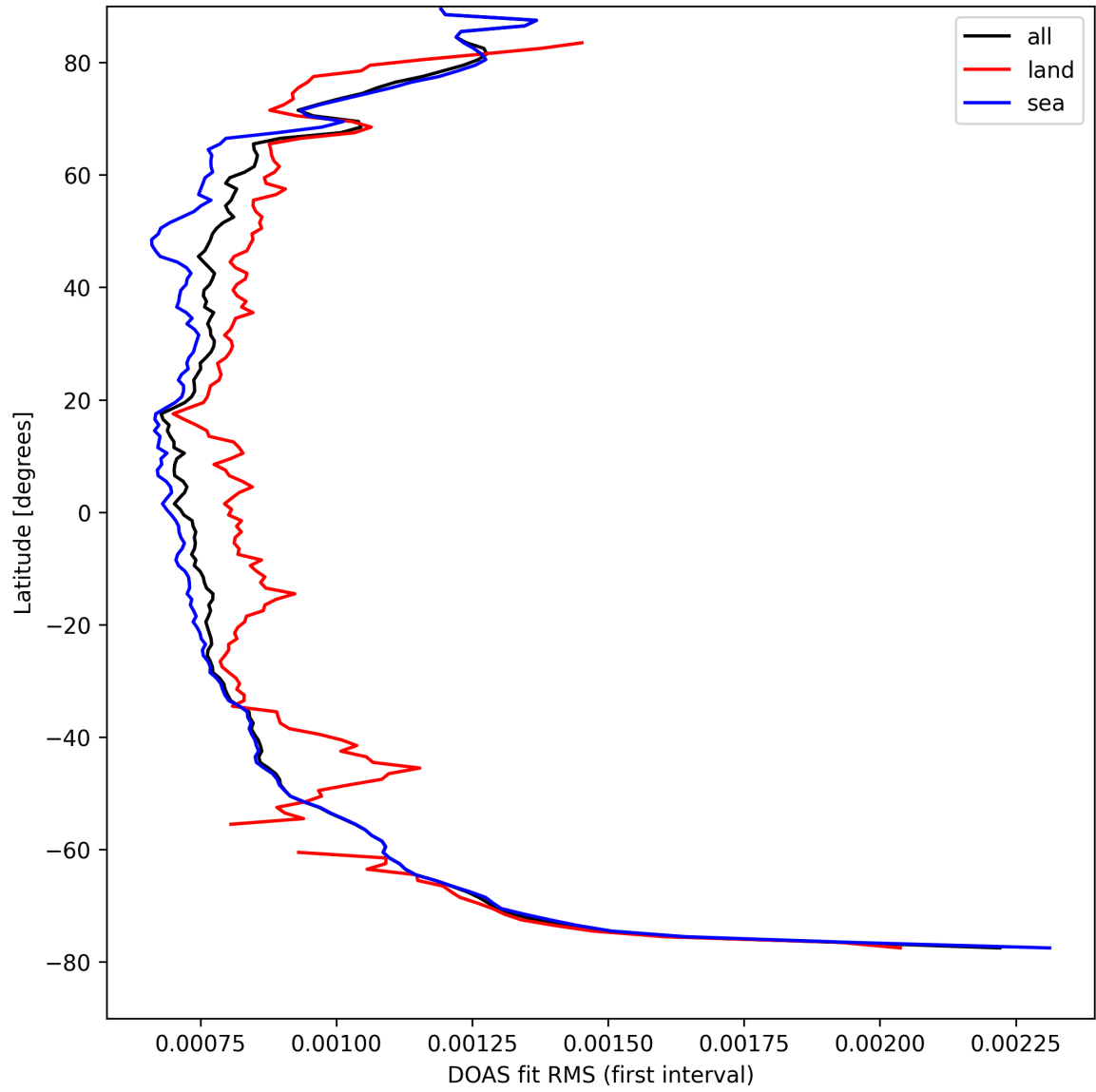
Figure 30: Zonal average of “DOAS fit RMS (first interval)” for 2025-09-01 to 2025-09-02.
