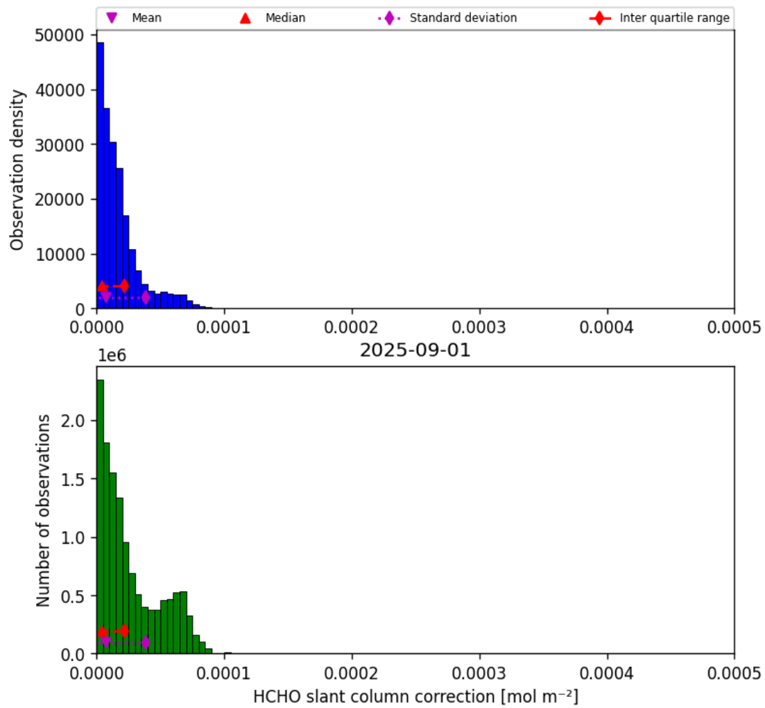
Figure 45: Histogram of “HCHO slant column correction” for 2025-09-01 to 2025-09-02
