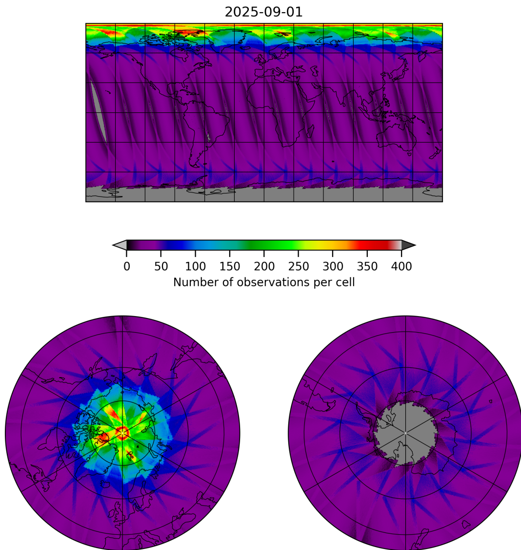
Figure 17: Map of the number of observations for 2025-09-01 to 2025-09-02
