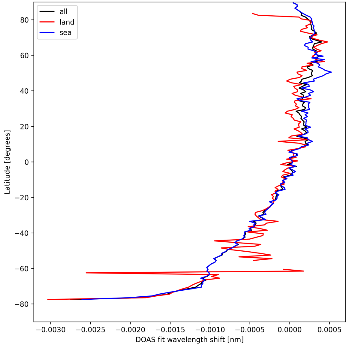
Figure 28: Zonal average of “DOAS fit wavelength shift” for 2025-09-01 to 2025-09-02.
