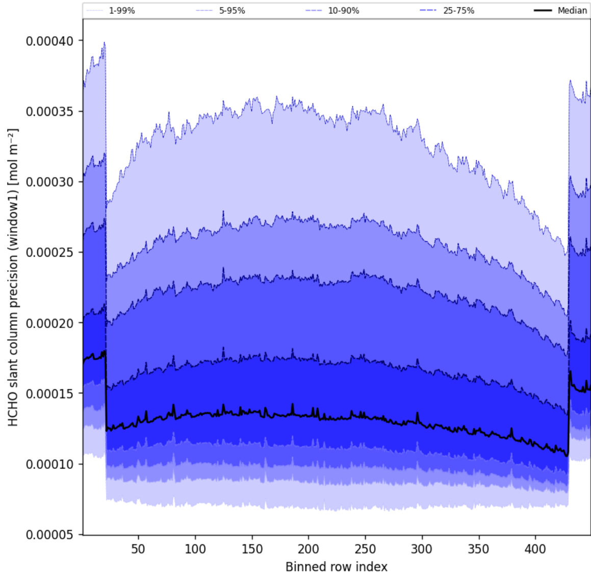
Figure 51: Along track statistics of "HCHO slant column precision (window1)" for 2025-09-01 to 2025-09-02
