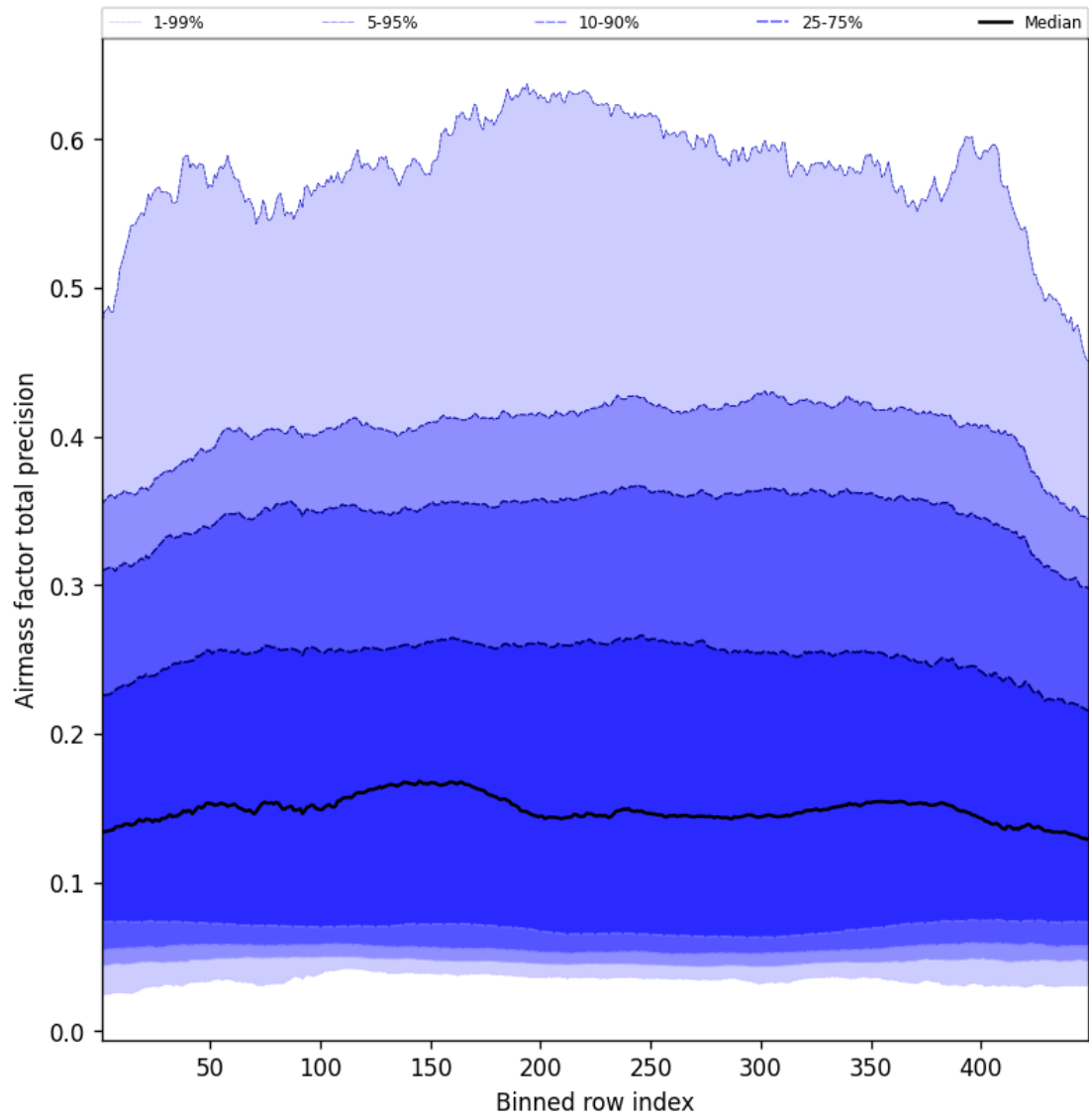
Figure 53: Along track statistics of “Airmass factor total precision” for 2025-09-01 to 2025-09-02
