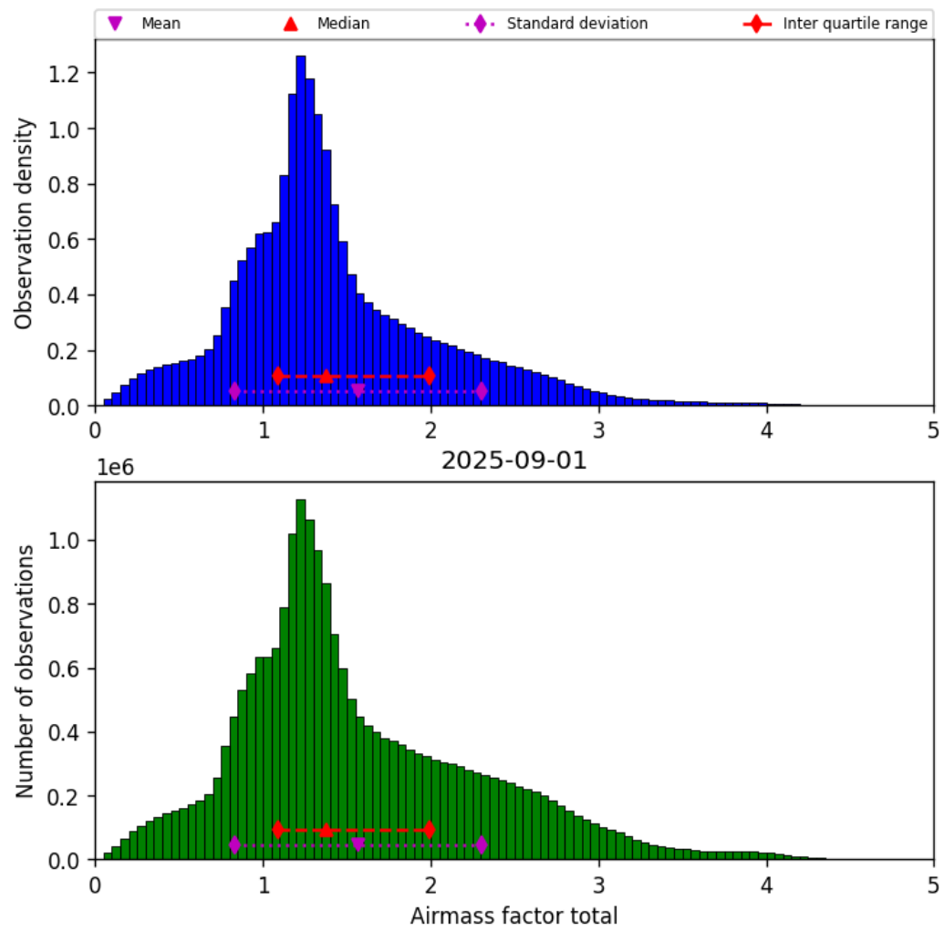
Figure 38: Histogram of “Airmass factor total” for 2025-09-01 to 2025-09-02
