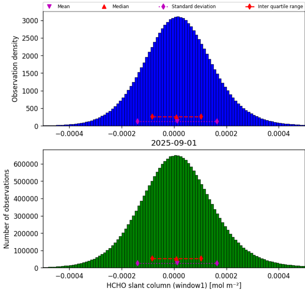
Figure 36: Histogram of “HCHO slant column (window1)” for 2025-09-01 to 2025-09-02
