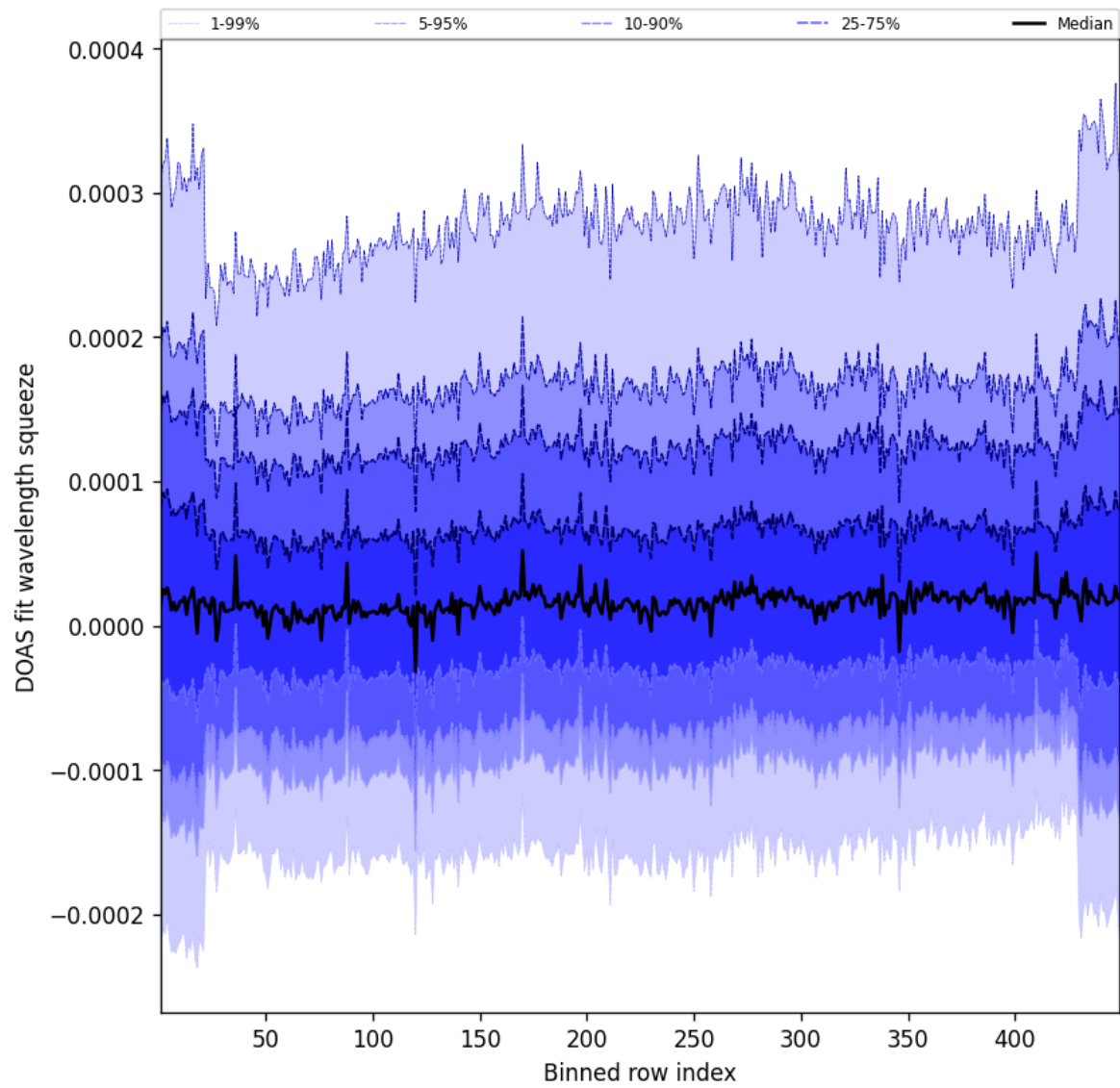
Figure 57: Along track statistics of “DOAS fit wavelength squeeze” for 2025-09-01 to 2025-09-02
