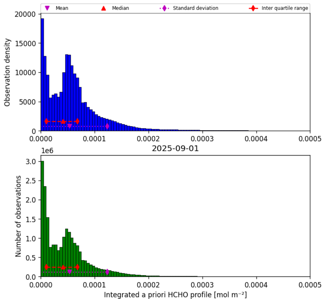
Figure 41: Histogram of “Integrated a priori HCHO profile” for 2025-09-01 to 2025-09-02
