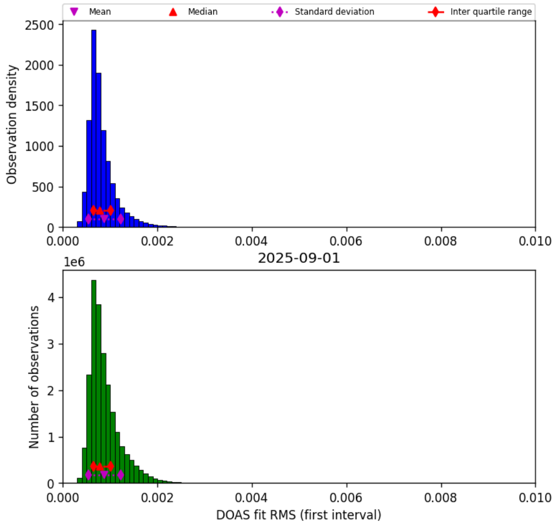
Figure 44: Histogram of “DOAS fit RMS (first interval)” for 2025-09-01 to 2025-09-02
