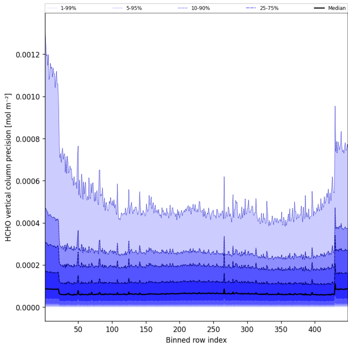
Figure 48: Along track statistics of “HCHO vertical column precision” for 2025-09-01 to 2025-09-02
