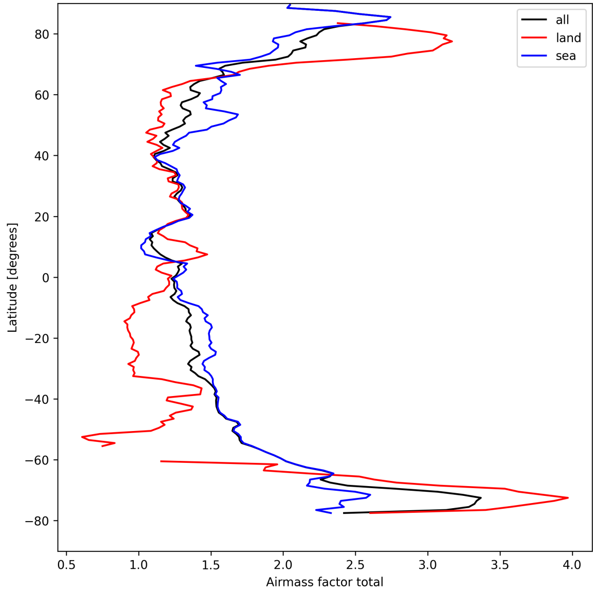
Figure 24: Zonal average of “Airmass factor total” for 2025-09-01 to 2025-09-02.
