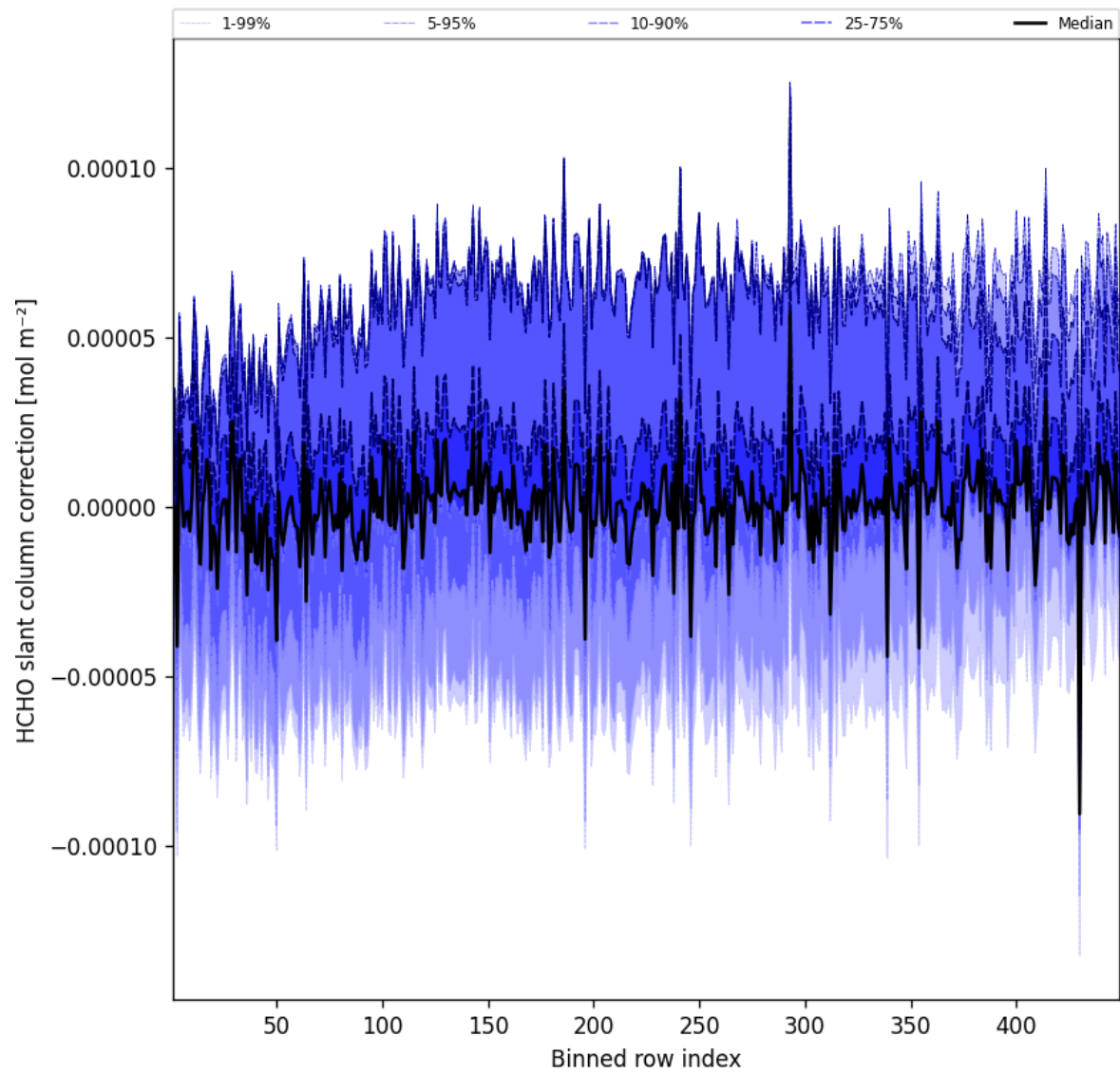
Figure 59: Along track statistics of “HCHO slant column correction” for 2025-09-01 to 2025-09-02
