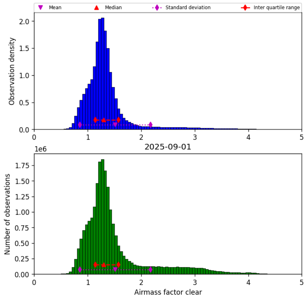
Figure 40: Histogram of “Airmass factor clear” for 2025-09-01 to 2025-09-02
