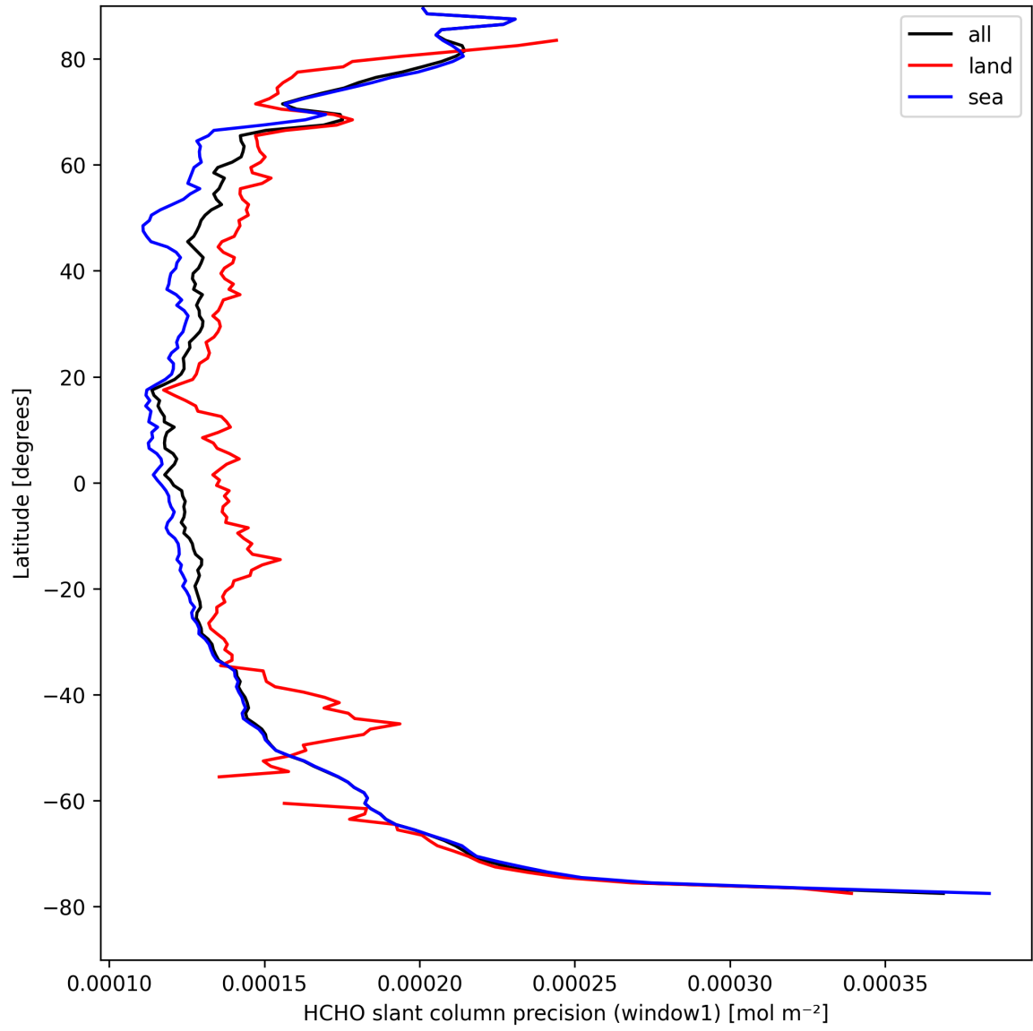
Figure 23: Zonal average of "HCHO slant column precision (window1)" for 2025-09-01 to 2025-09-02.
