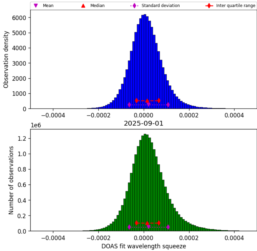
Figure 43: Histogram of “DOAS fit wavelength squeeze” for 2025-09-01 to 2025-09-02
