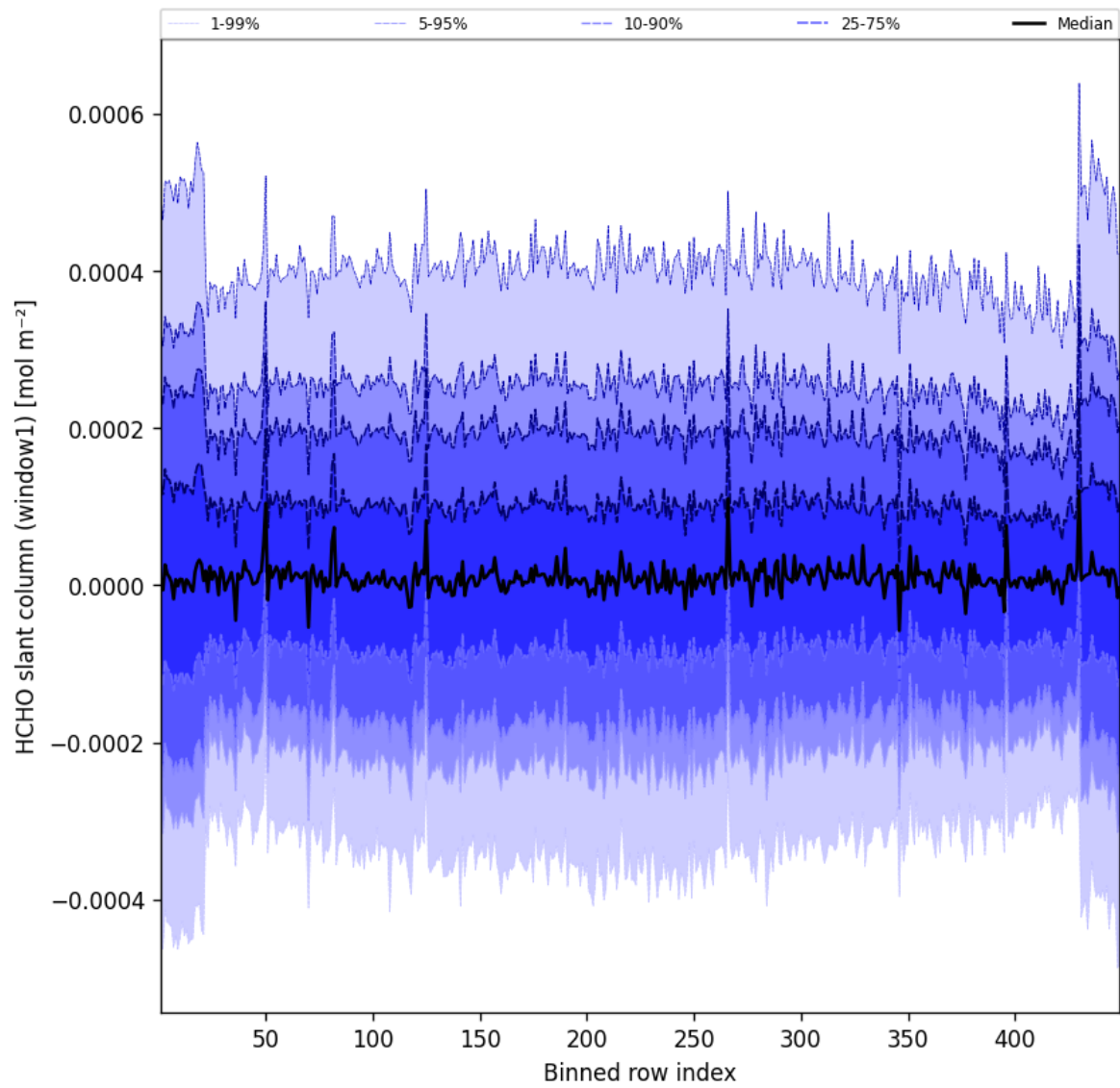
Figure 50: Along track statistics of “HCHO slant column (window1)” for 2025-09-01 to 2025-09-02
