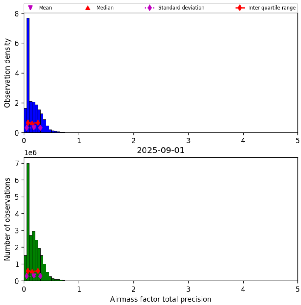
Figure 39: Histogram of “Airmass factor total precision” for 2025-09-01 to 2025-09-02
