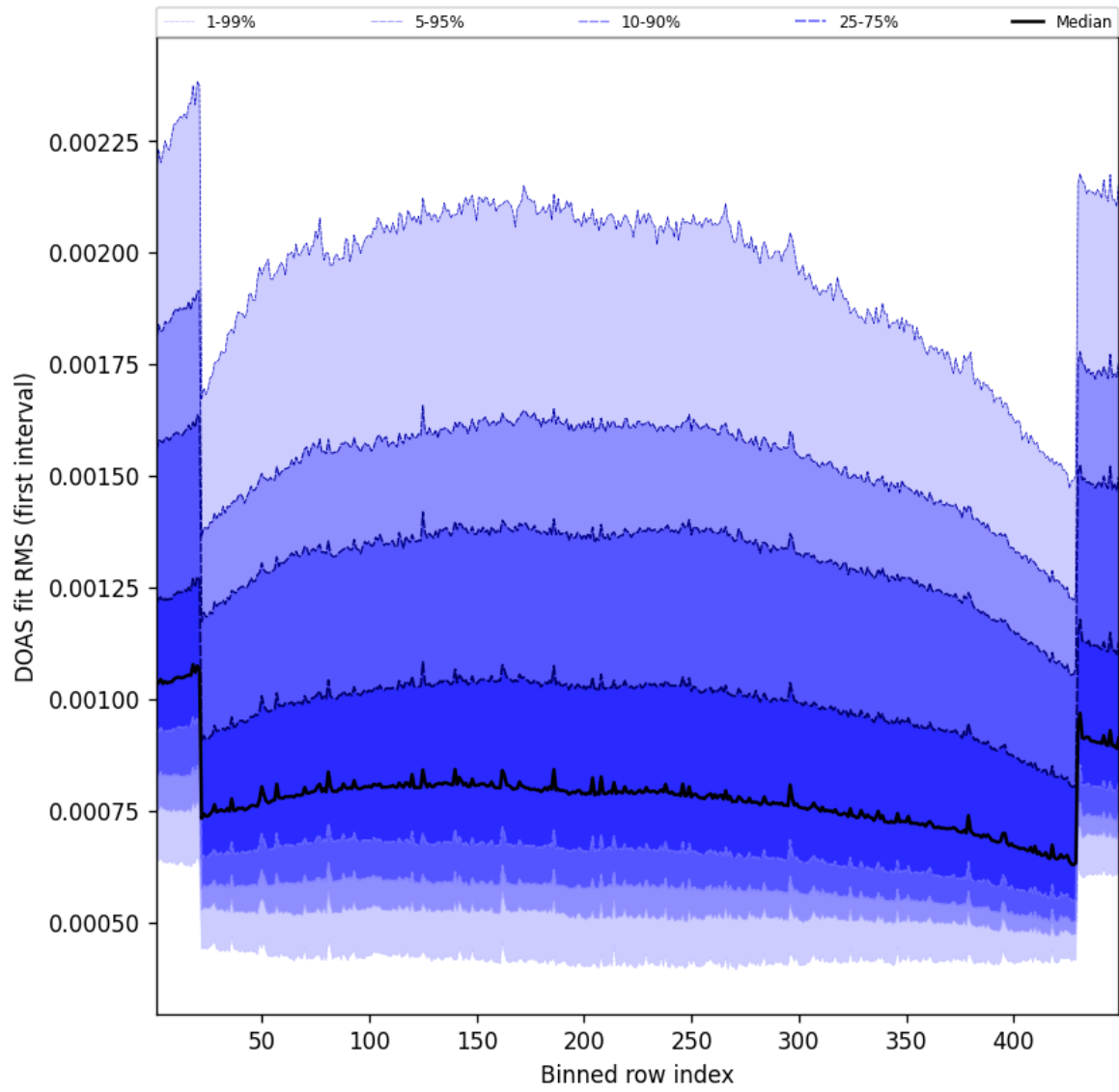
Figure 58: Along track statistics of “DOAS fit RMS (first interval)” for 2025-09-01 to 2025-09-02
