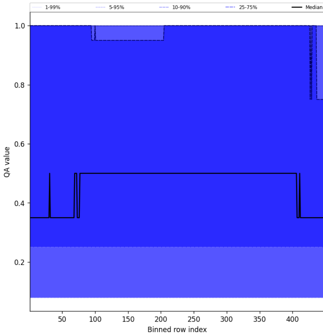
Figure 46: Along track statistics of “QA value” for 2025-09-01 to 2025-09-02
