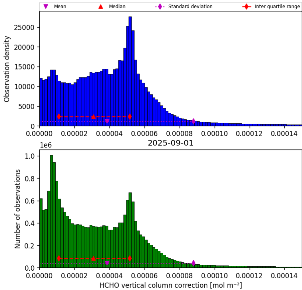
Figure 35: Histogram of “HCHO vertical column correction” for 2025-09-01 to 2025-09-02
