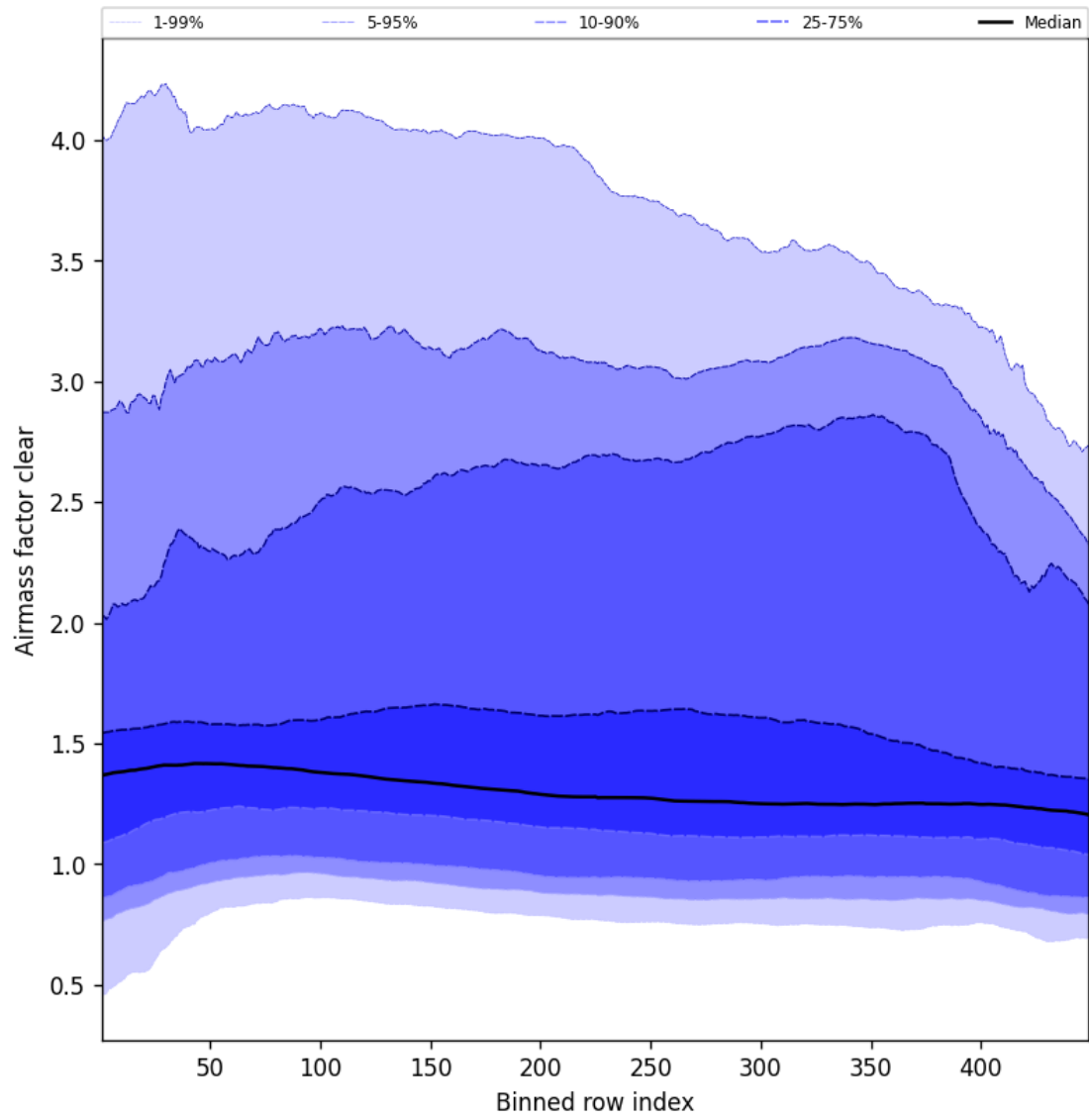
Figure 54: Along track statistics of “Airmass factor clear” for 2025-09-01 to 2025-09-02
