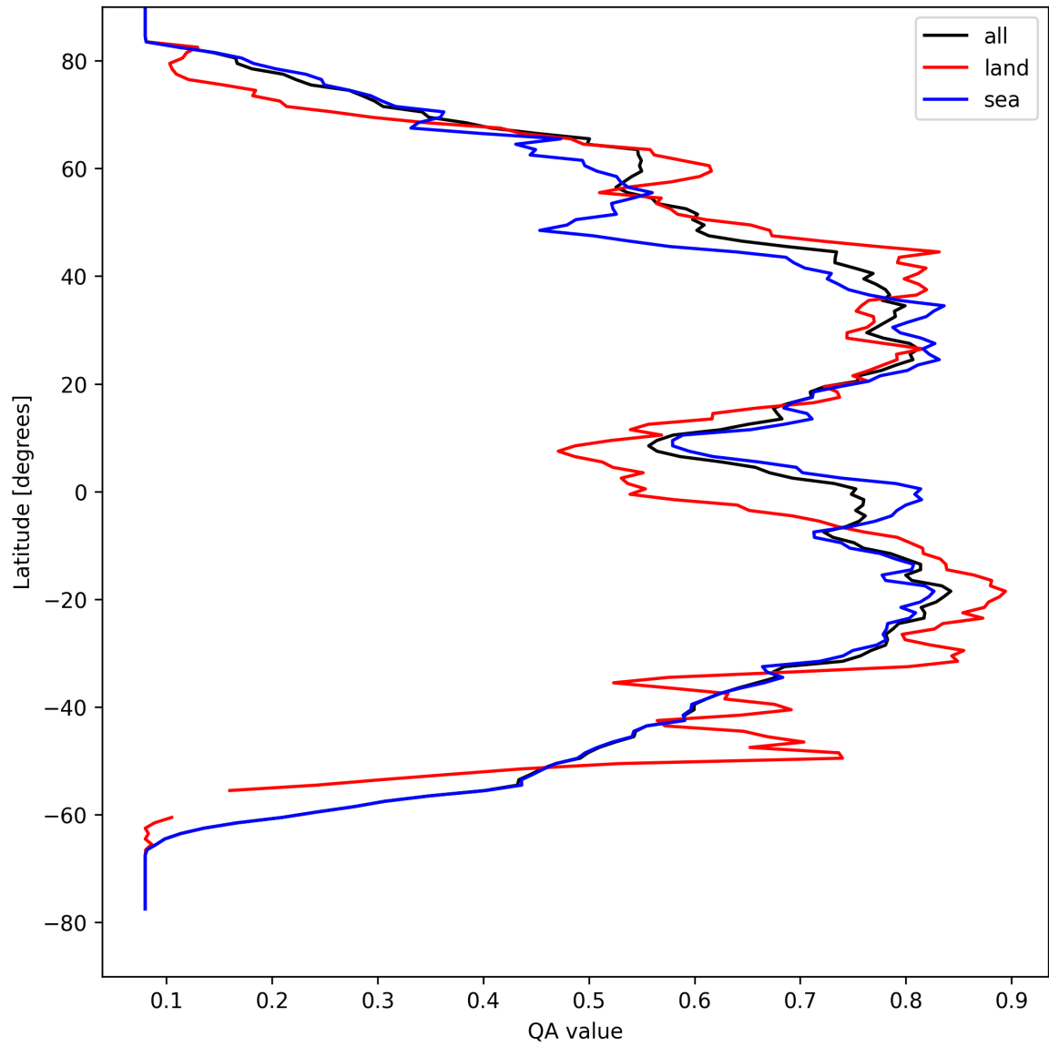
Figure 18: Zonal average of “QA value” for 2025-09-01 to 2025-09-02.
