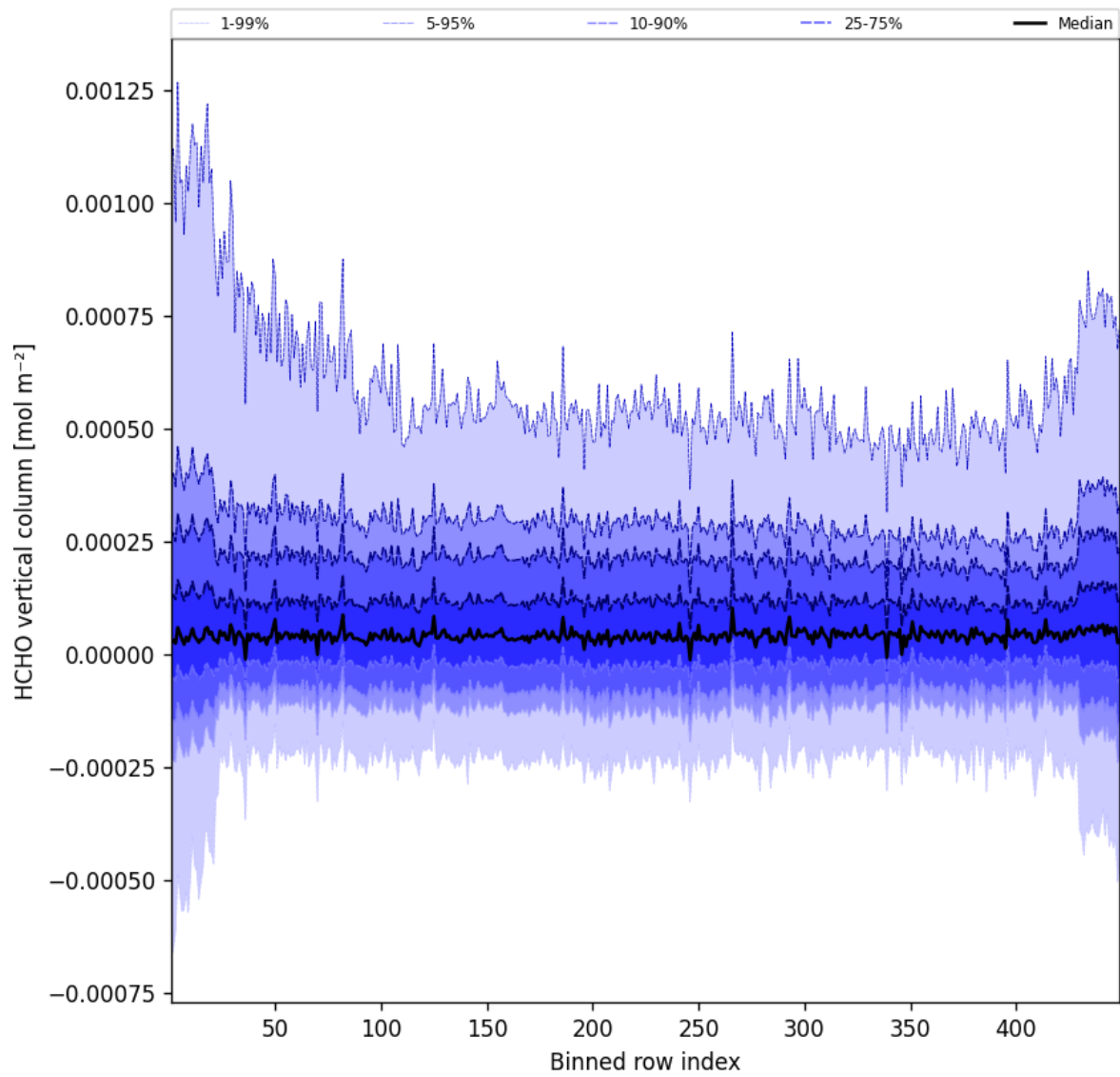
Figure 47: Along track statistics of “HCHO vertical column” for 2025-09-01 to 2025-09-02
