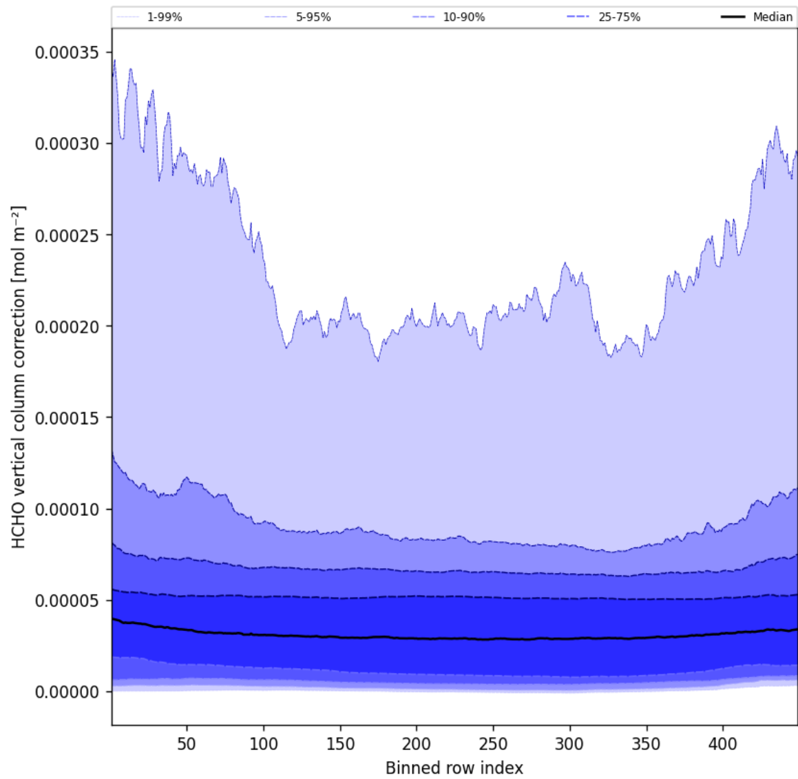
Figure 49: Along track statistics of “HCHO vertical column correction” for 2025-09-01 to 2025-09-02
