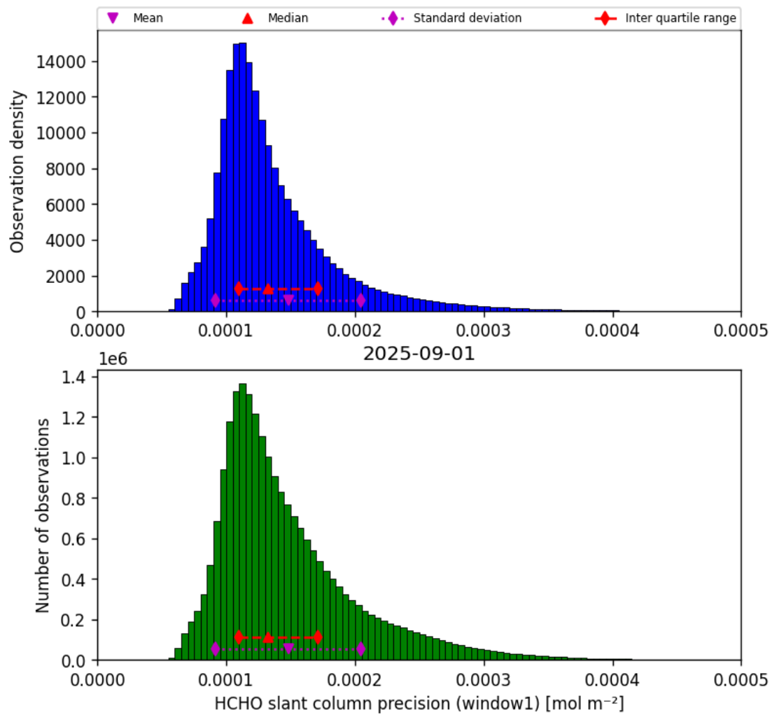
Figure 37: Histogram of “HCHO slant column precision (window1)” for 2025-09-01 to 2025-09-02
