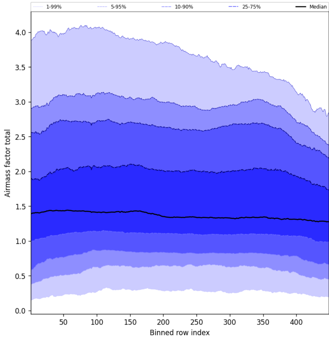
Figure 52: Along track statistics of “Airmass factor total” for 2025-09-01 to 2025-09-02
