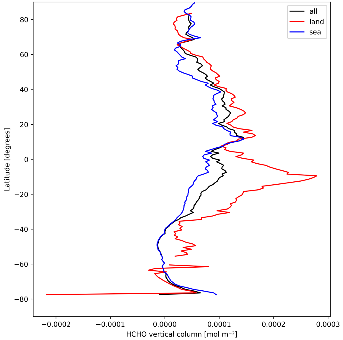
Figure 19: Zonal average of “HCHO vertical column” for 2025-09-01 to 2025-09-02.
