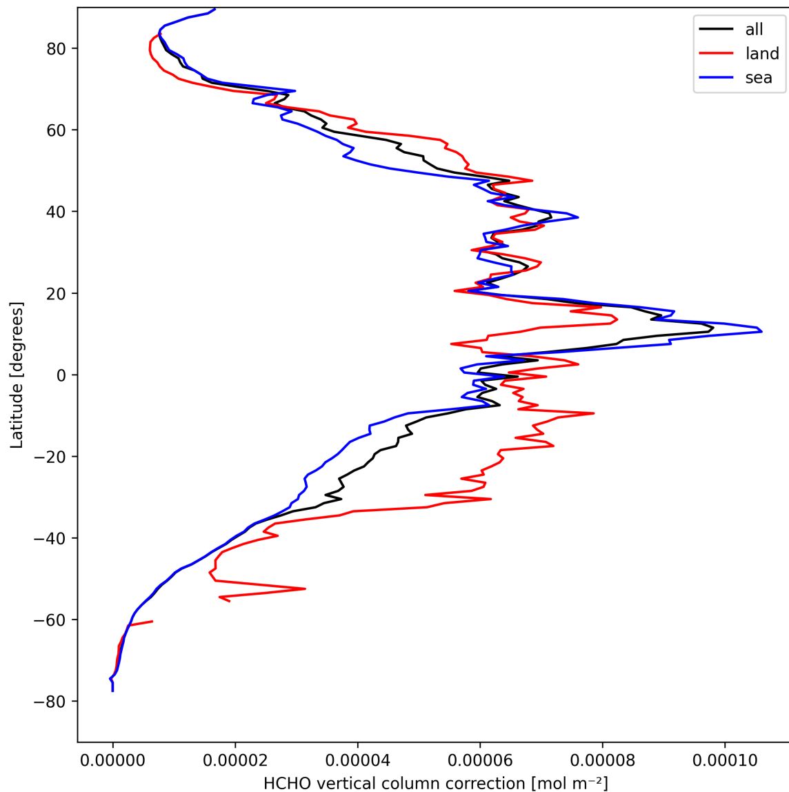
Figure 21: Zonal average of “HCHO vertical column correction” for 2025-09-01 to 2025-09-02.
