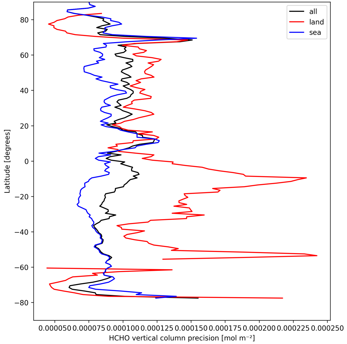
Figure 20: Zonal average of "HCHO vertical column precision" for 2025-09-01 to 2025-09-02.
