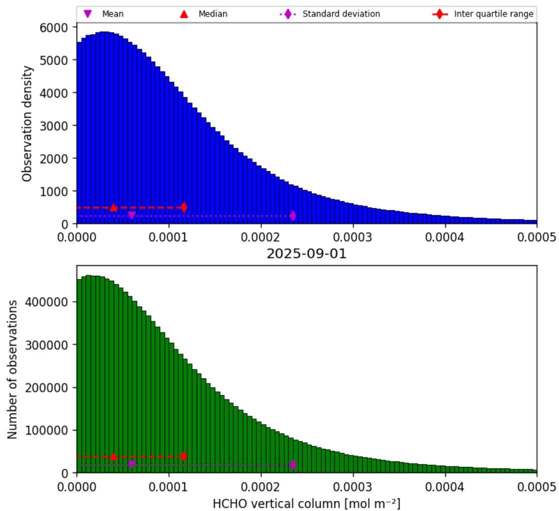
Figure 33: Histogram of “HCHO vertical column” for 2025-09-01 to 2025-09-02
