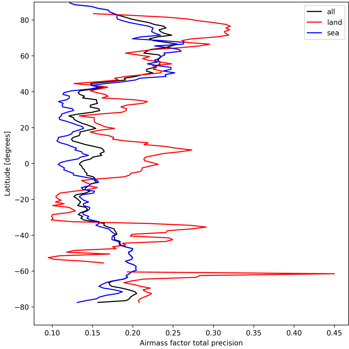
Figure 25: Zonal average of “Airmass factor total precision” for 2025-09-01 to 2025-09-02.
