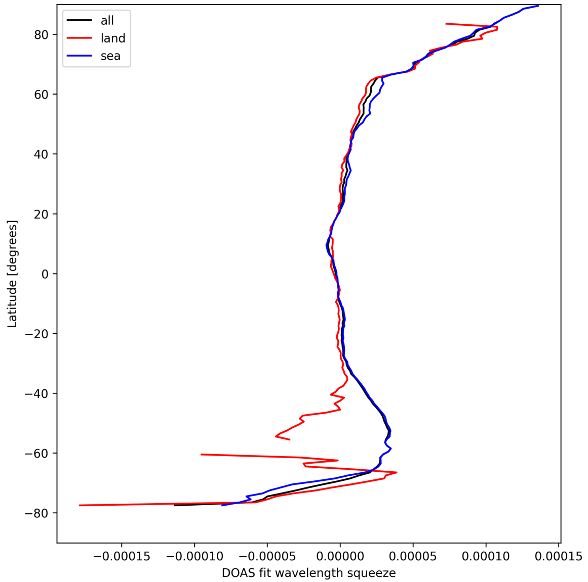
Figure 29: Zonal average of “DOAS fit wavelength squeeze” for 2025-09-01 to 2025-09-02.
