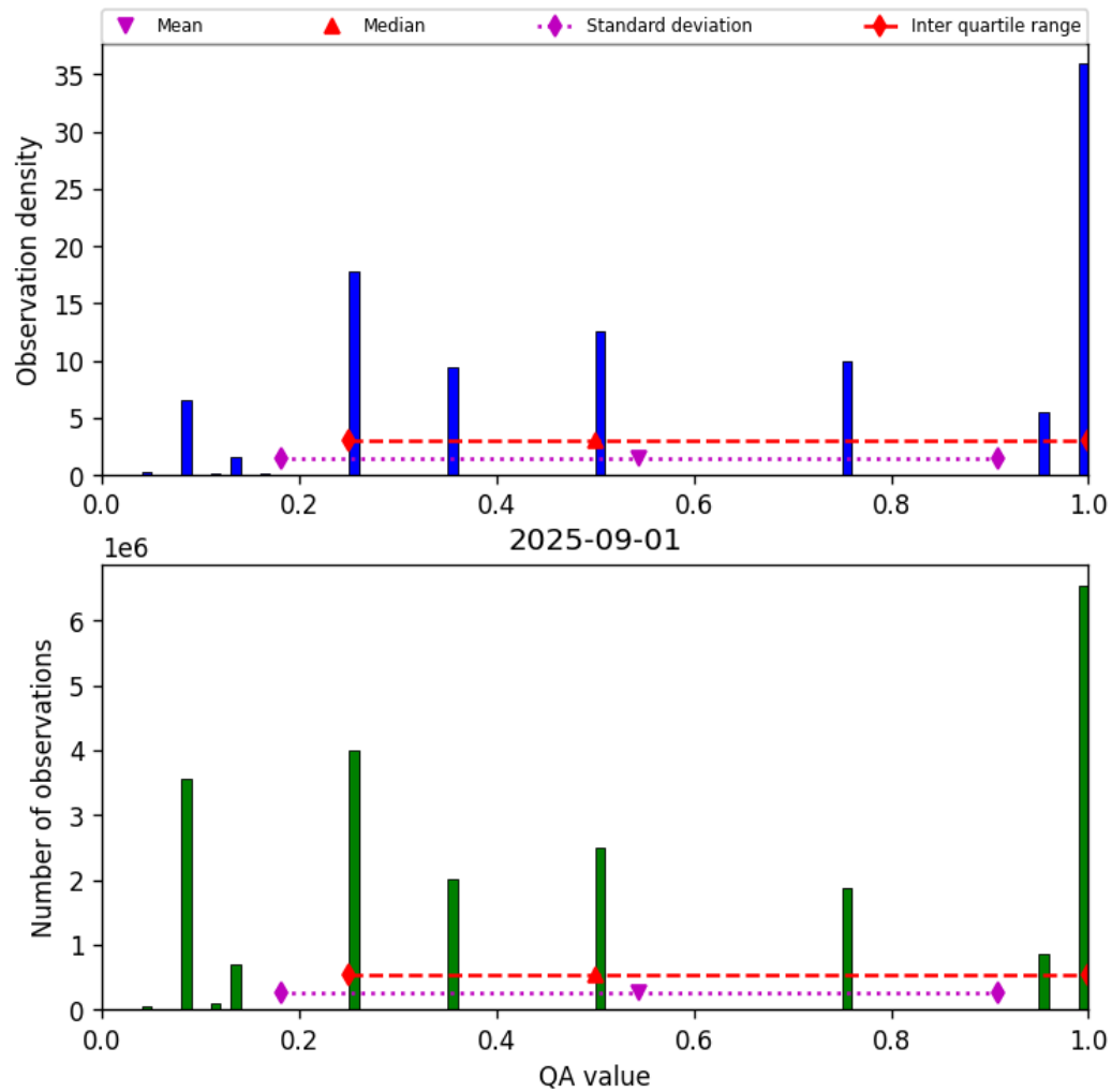
Figure 32: Histogram of “QA value” for 2025-09-01 to 2025-09-02
