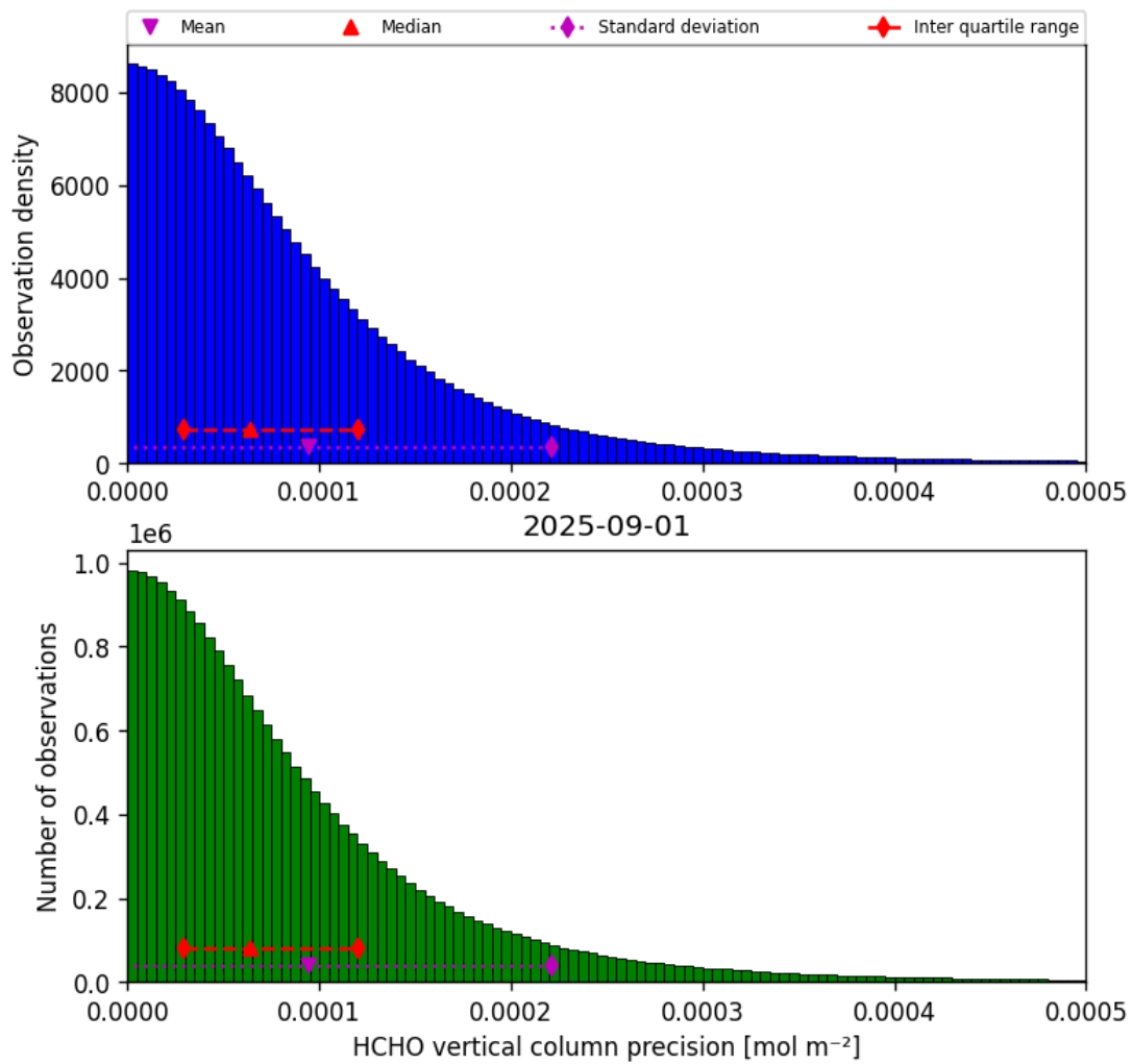
Figure 34: Histogram of “HCHO vertical column precision” for 2025-09-01 to 2025-09-02
