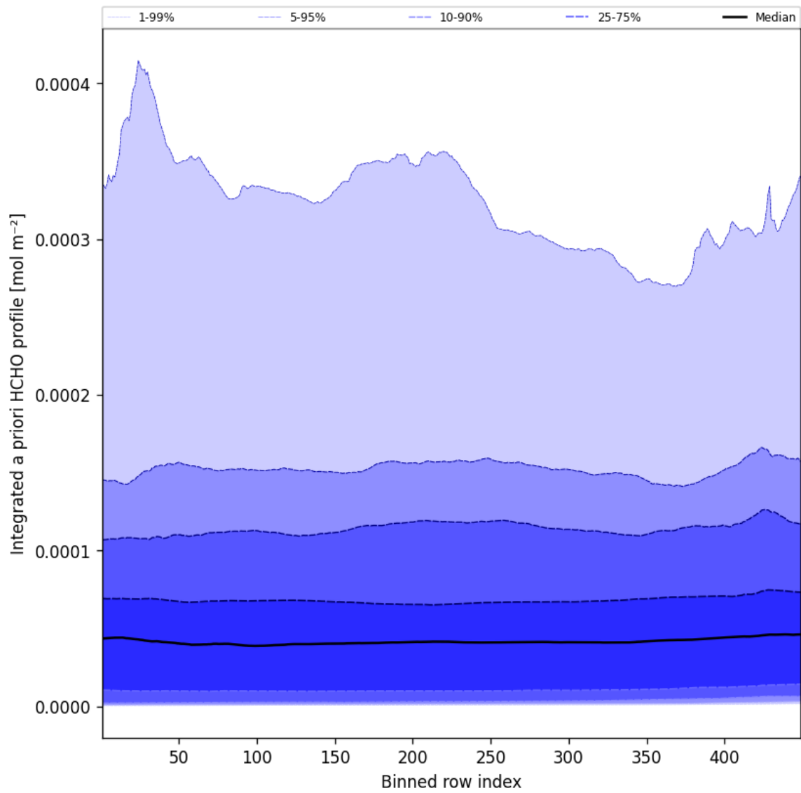
Figure 55: Along track statistics of “Integrated a priori HCHO profile” for 2025-09-01 to 2025-09-02
