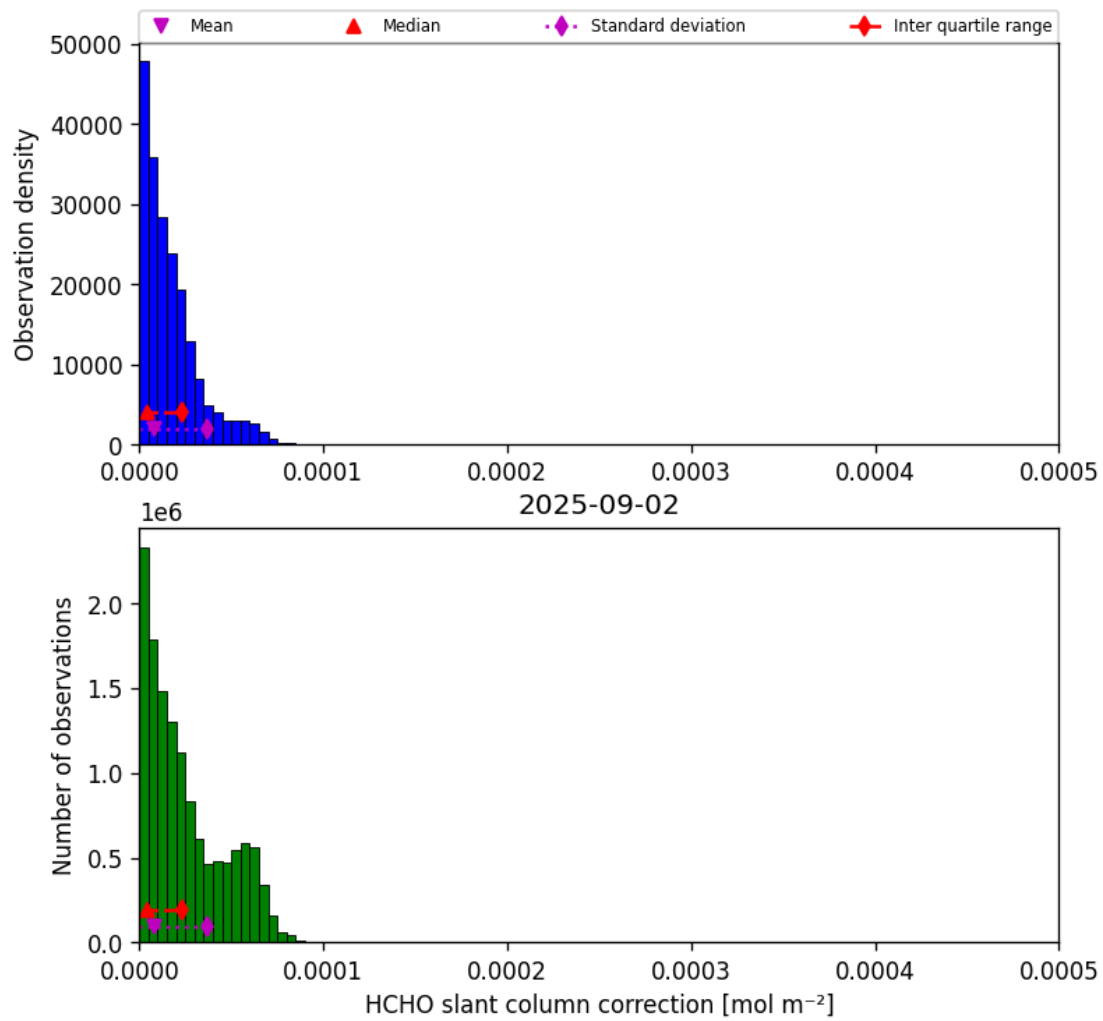
Figure 45: Histogram of “HCHO slant column correction” for 2025-09-02 to 2025-09-02
