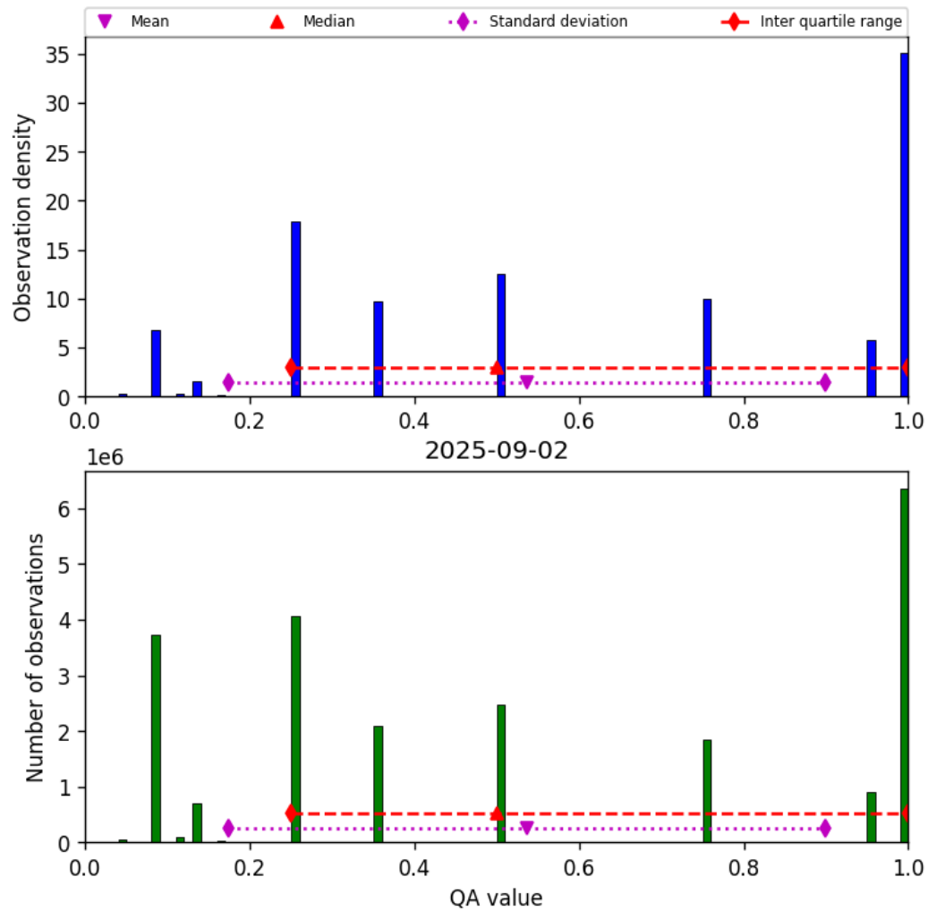
Figure 32: Histogram of “QA value” for 2025-09-02 to 2025-09-02
