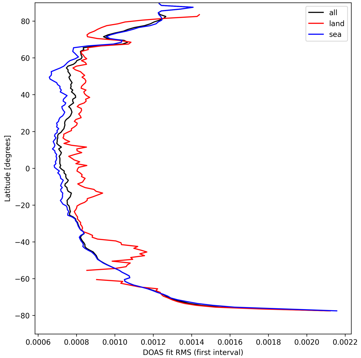
Figure 30: Zonal average of “DOAS fit RMS (first interval)” for 2025-09-02 to 2025-09-02.
