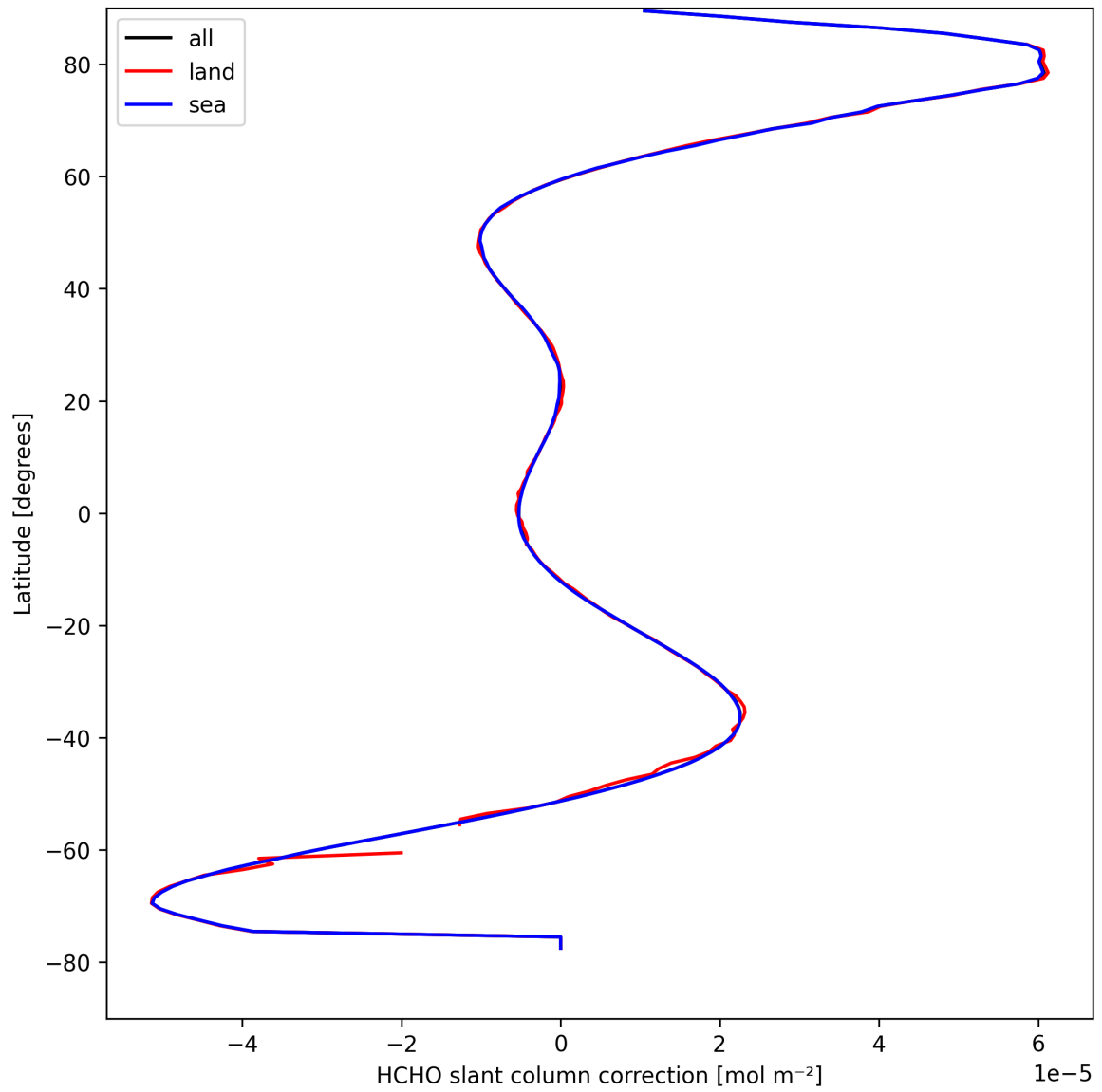
Figure 31: Zonal average of “HCHO slant column correction” for 2025-09-02 to 2025-09-02.
