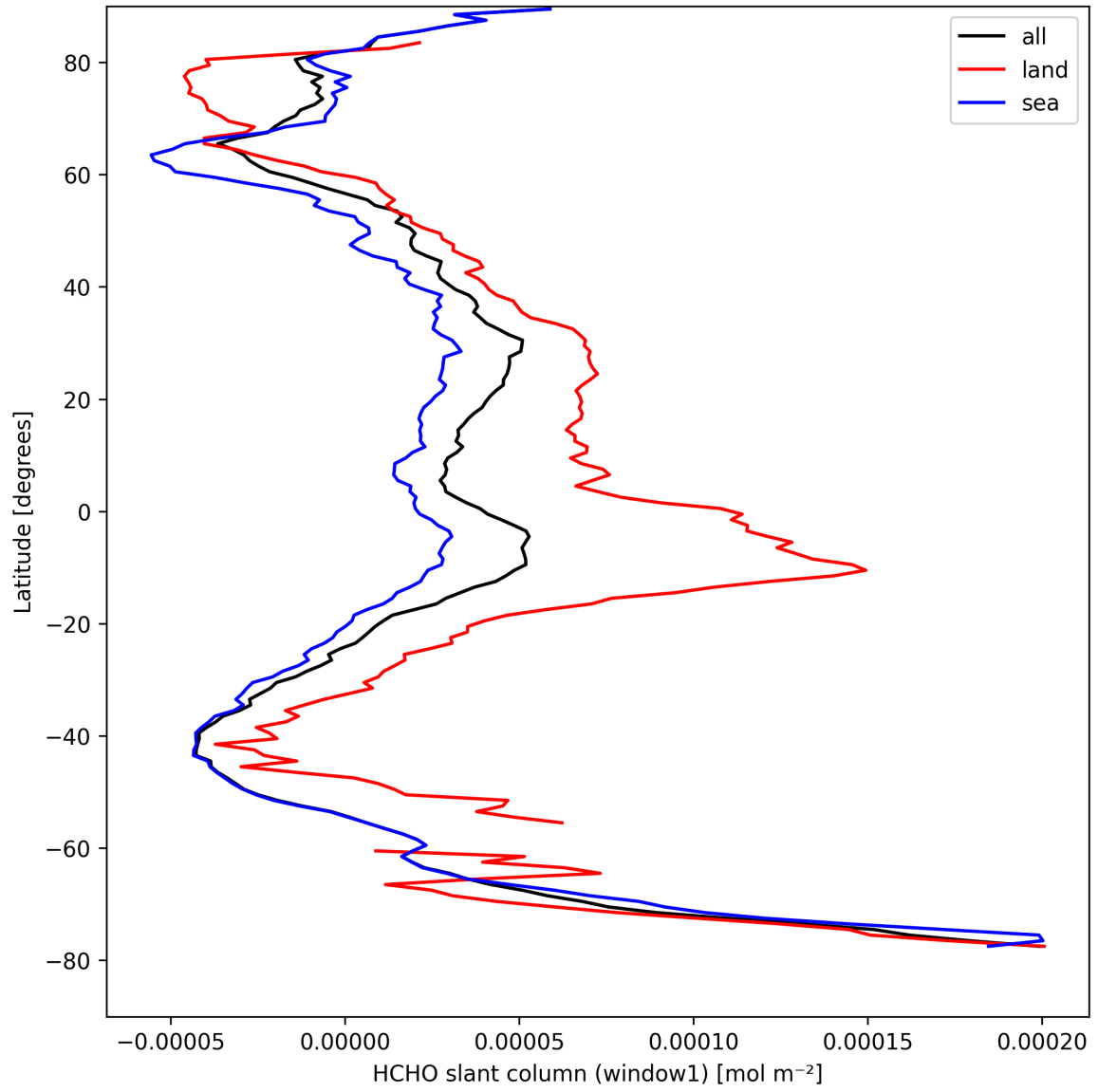
Figure 22: Zonal average of “HCHO slant column (window1)” for 2025-09-02 to 2025-09-02.
