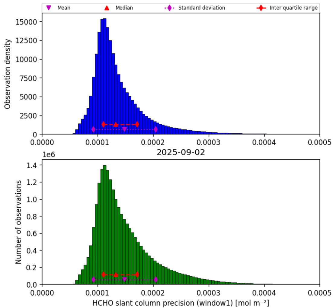
Figure 37: Histogram of “HCHO slant column precision (window1)” for 2025-09-02 to 2025-09-02
