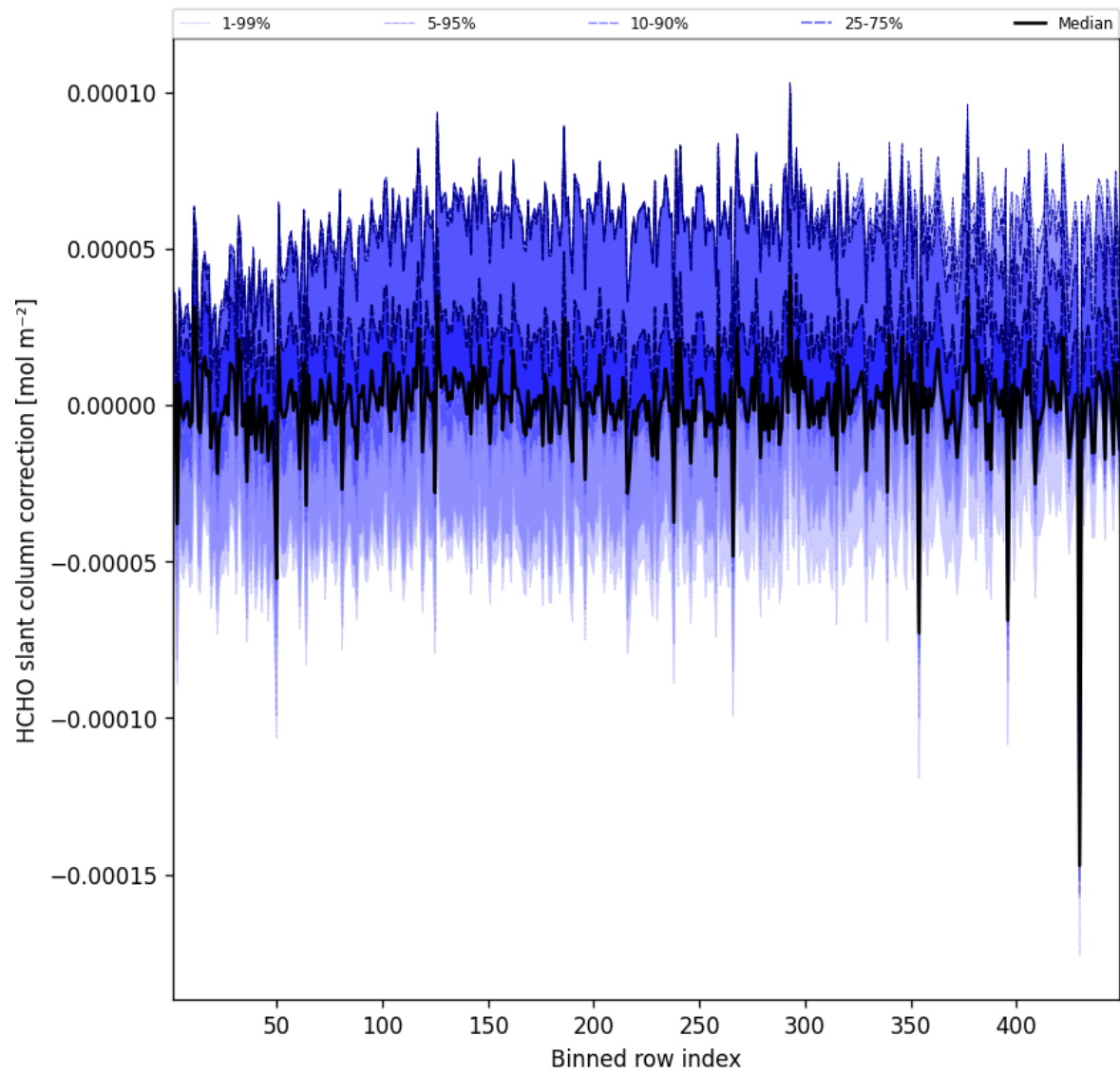
Figure 59: Along track statistics of “HCHO slant column correction” for 2025-09-02 to 2025-09-02
