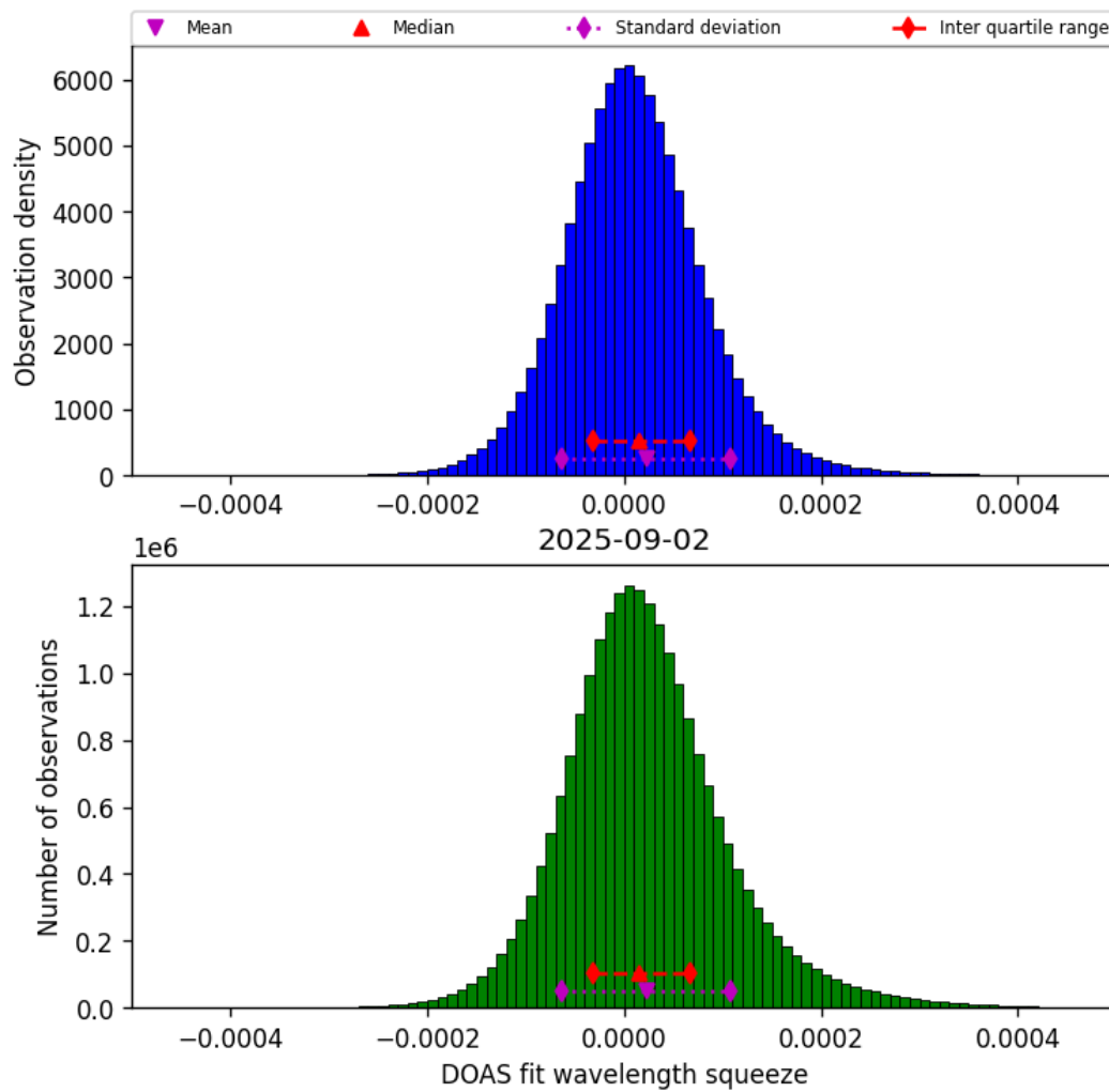
Figure 43: Histogram of “DOAS fit wavelength squeeze” for 2025-09-02 to 2025-09-02
