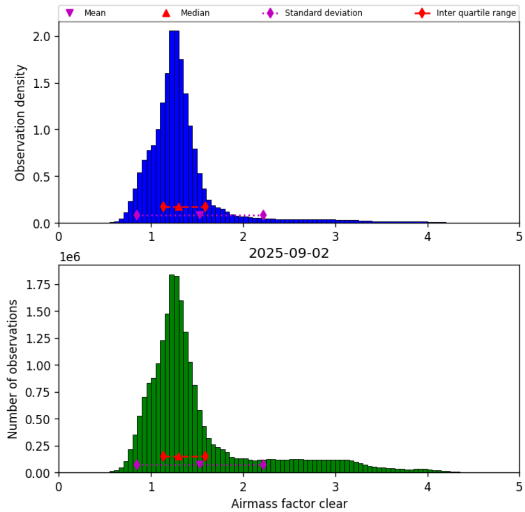
Figure 40: Histogram of “Airmass factor clear” for 2025-09-02 to 2025-09-02
