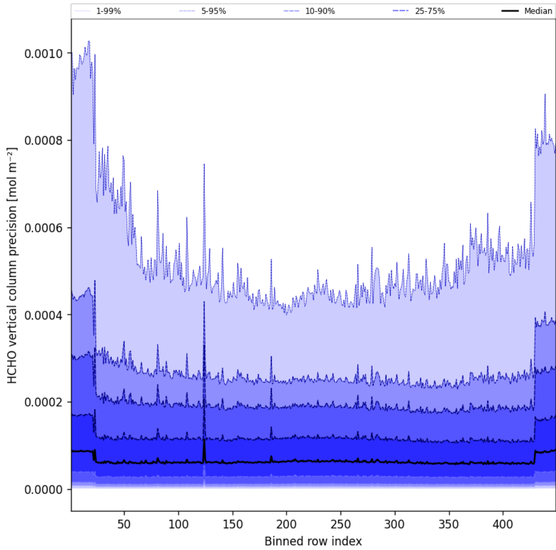
Figure 48: Along track statistics of “HCHO vertical column precision” for 2025-09-02 to 2025-09-02
