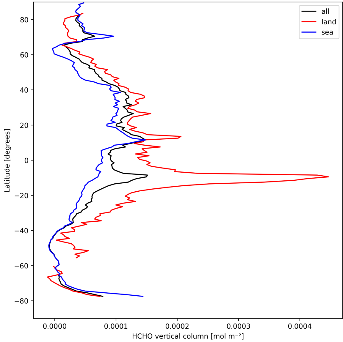
Figure 19: Zonal average of “HCHO vertical column” for 2025-09-02 to 2025-09-02.
