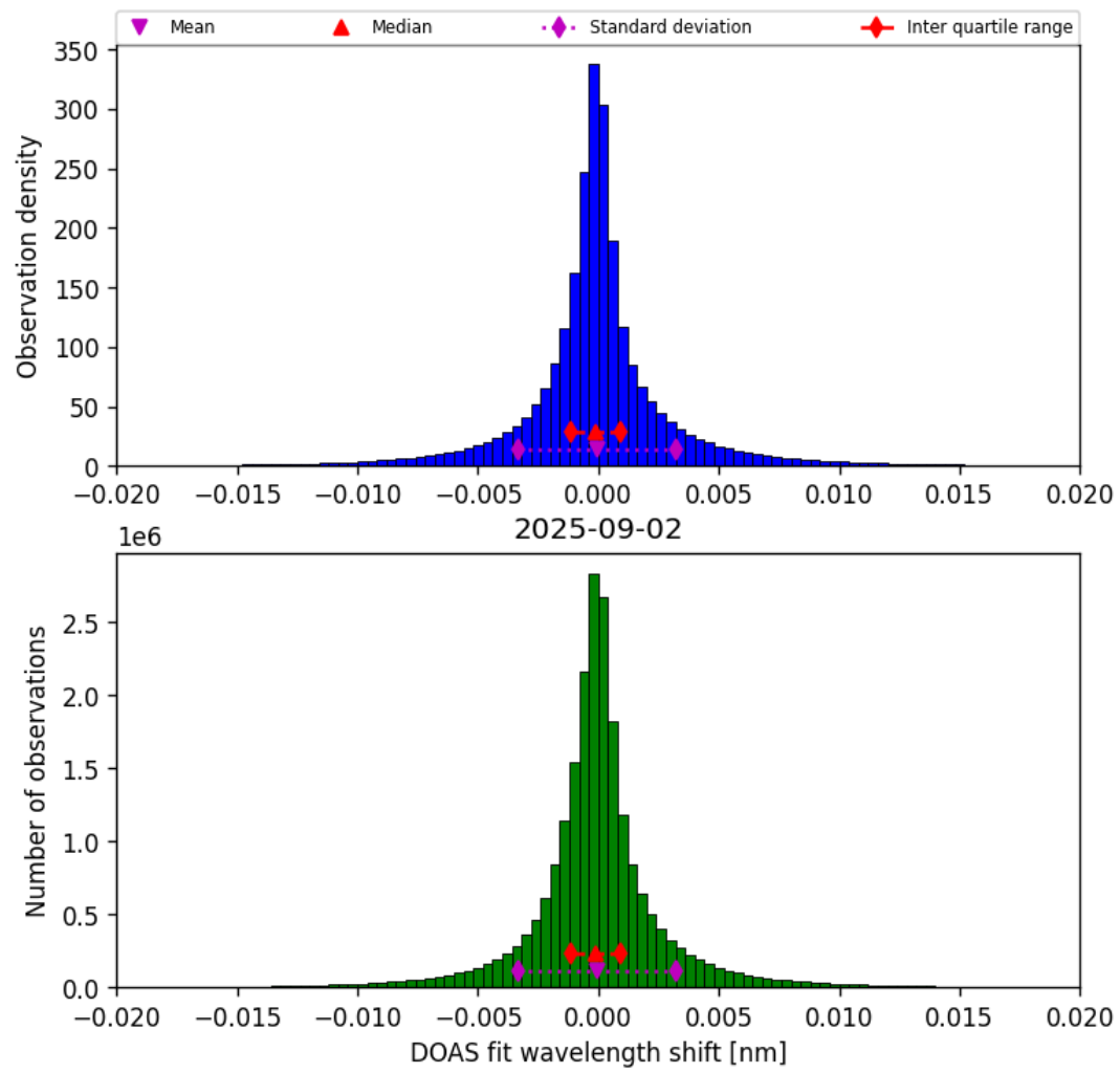
Figure 42: Histogram of “DOAS fit wavelength shift” for 2025-09-02 to 2025-09-02
