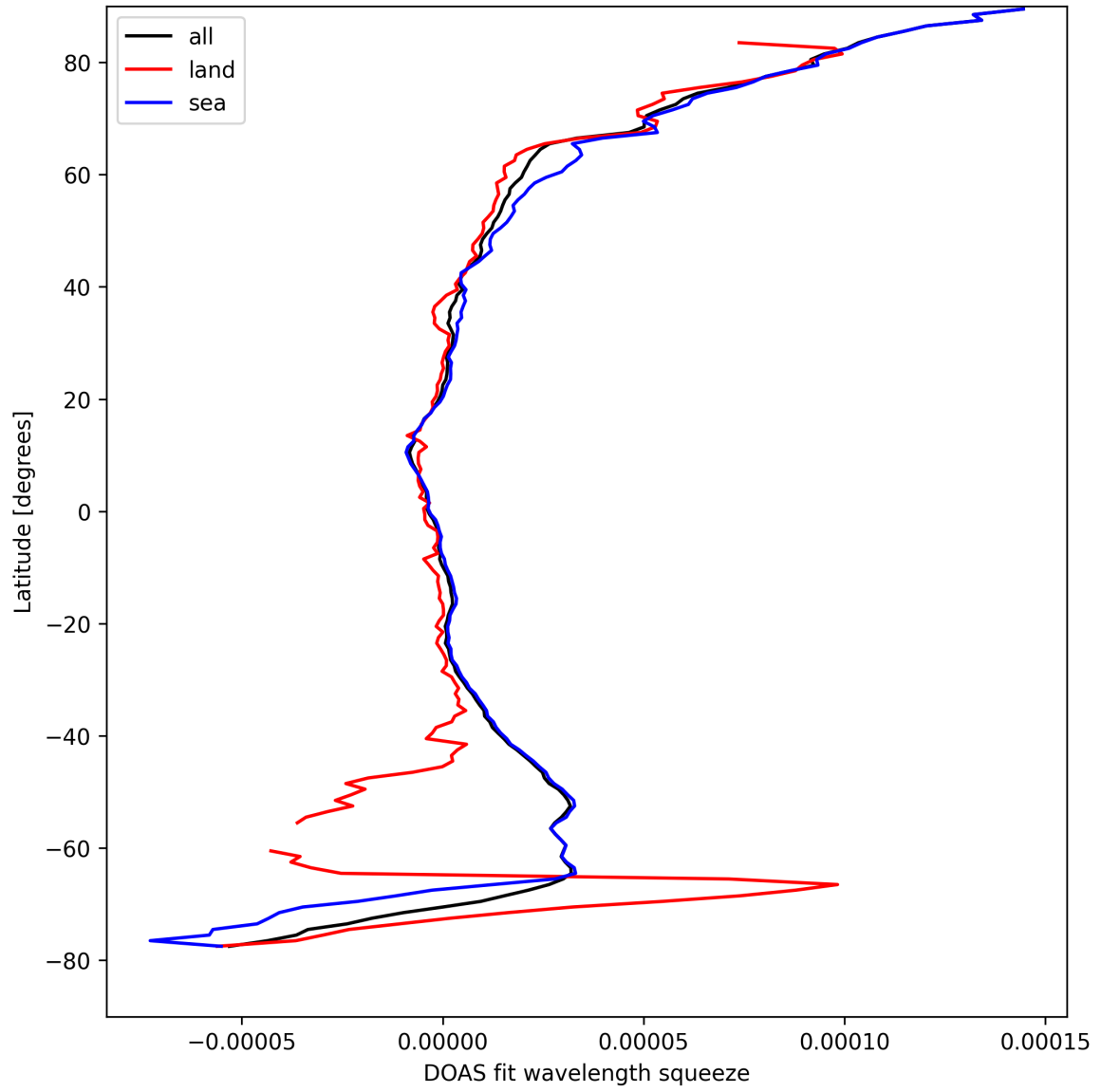
Figure 29: Zonal average of “DOAS fit wavelength squeeze” for 2025-09-02 to 2025-09-02.
