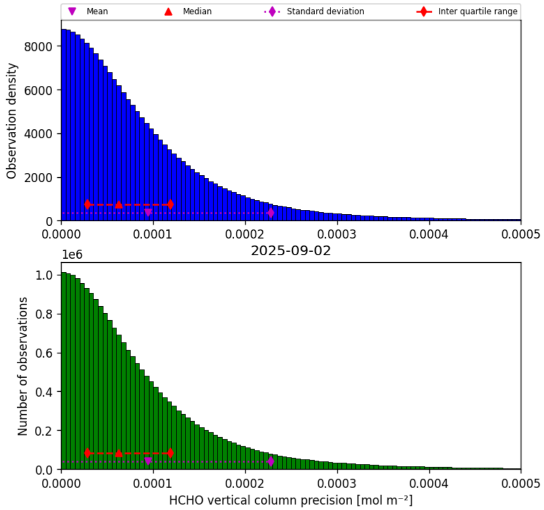
Figure 34: Histogram of “HCHO vertical column precision” for 2025-09-02 to 2025-09-02
