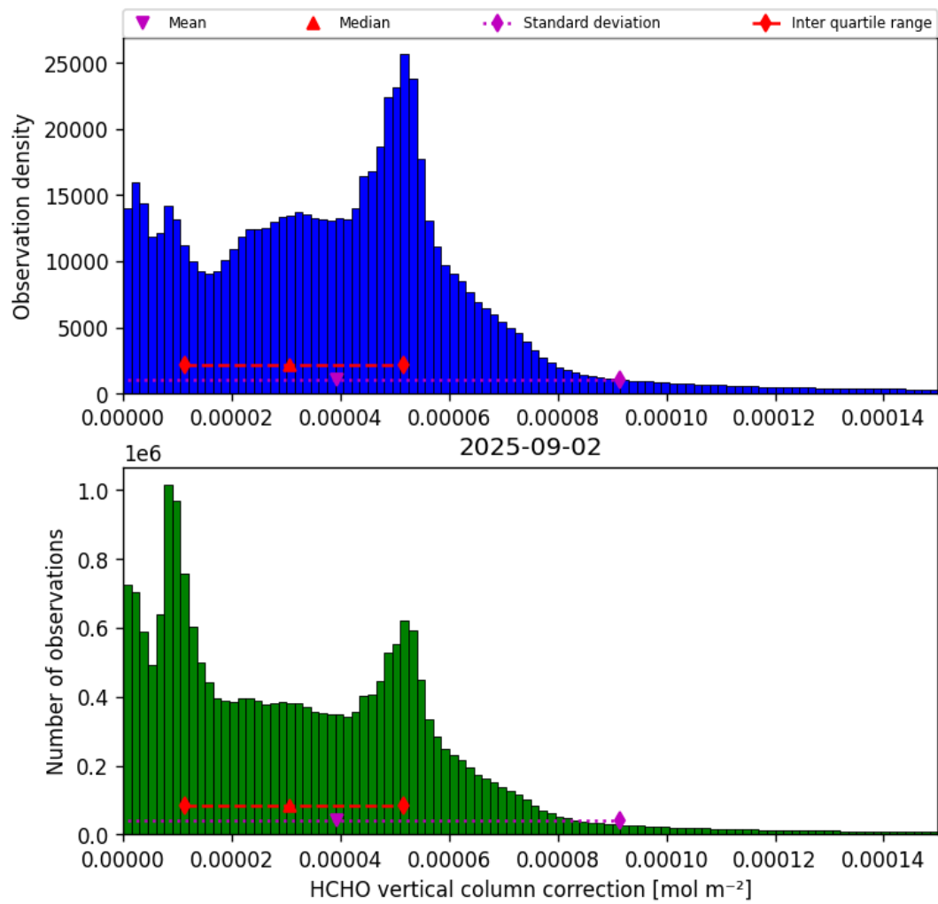
Figure 35: Histogram of “HCHO vertical column correction” for 2025-09-02 to 2025-09-02
