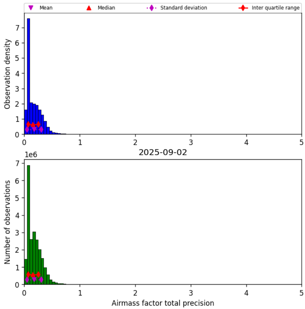
Figure 39: Histogram of “Airmass factor total precision” for 2025-09-02 to 2025-09-02
