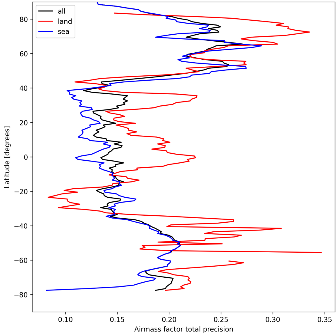
Figure 25: Zonal average of “Airmass factor total precision” for 2025-09-02 to 2025-09-02.
