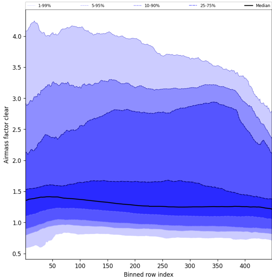
Figure 54: Along track statistics of “Airmass factor clear” for 2025-09-02 to 2025-09-02
