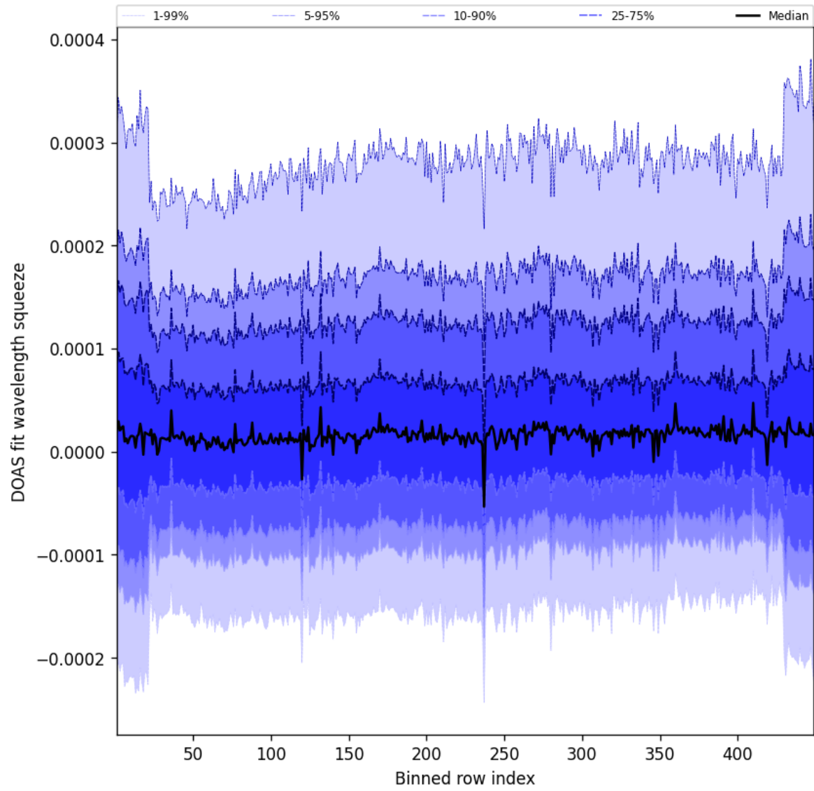
Figure 57: Along track statistics of “DOAS fit wavelength squeeze” for 2025-09-02 to 2025-09-02
