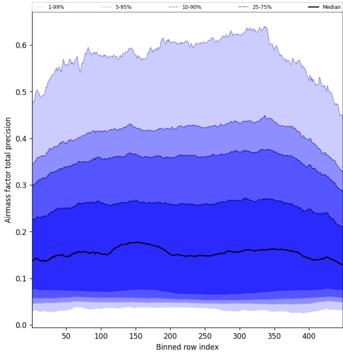
Figure 53: Along track statistics of “Airmass factor total precision” for 2025-09-02 to 2025-09-02
