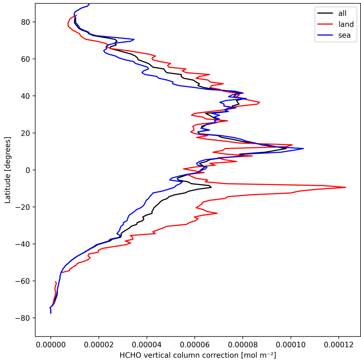
Figure 21: Zonal average of “HCHO vertical column correction” for 2025-09-02 to 2025-09-02.
