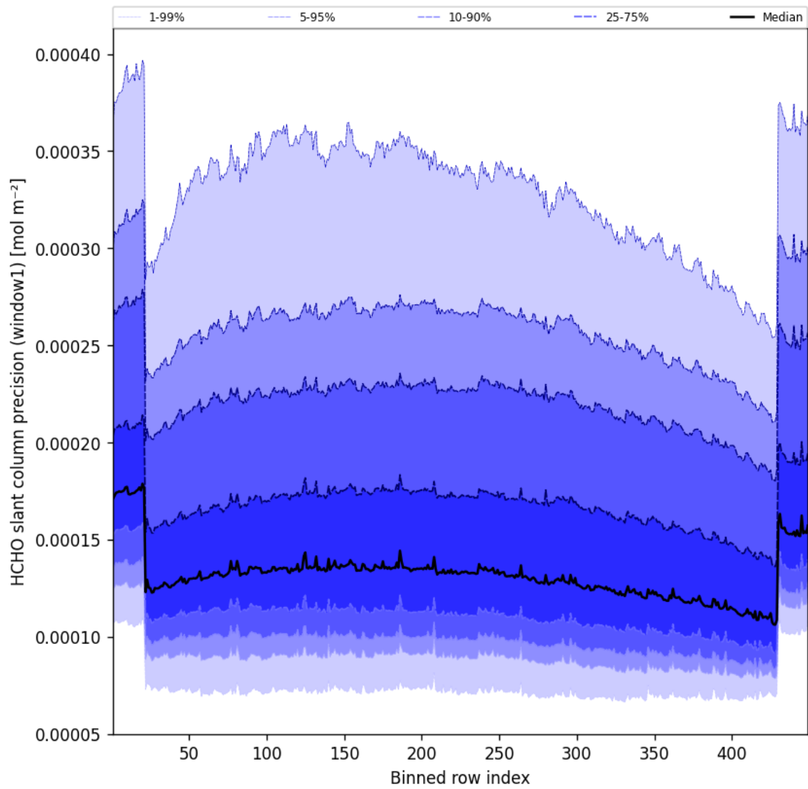
Figure 51: Along track statistics of “HCHO slant column precision (window1)” for 2025-09-02 to 2025-09-02
