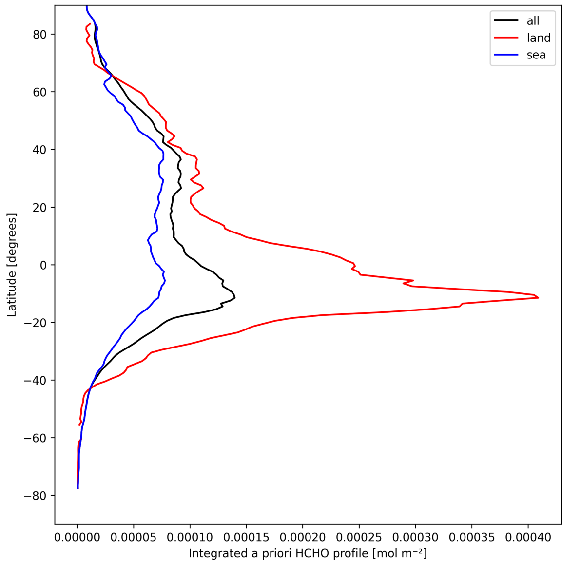
Figure 27: Zonal average of “Integrated a priori HCHO profile” for 2025-09-02 to 2025-09-02.
