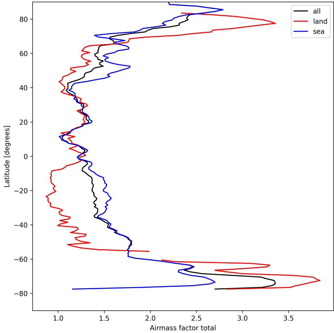
Figure 24: Zonal average of “Airmass factor total” for 2025-09-02 to 2025-09-02.
