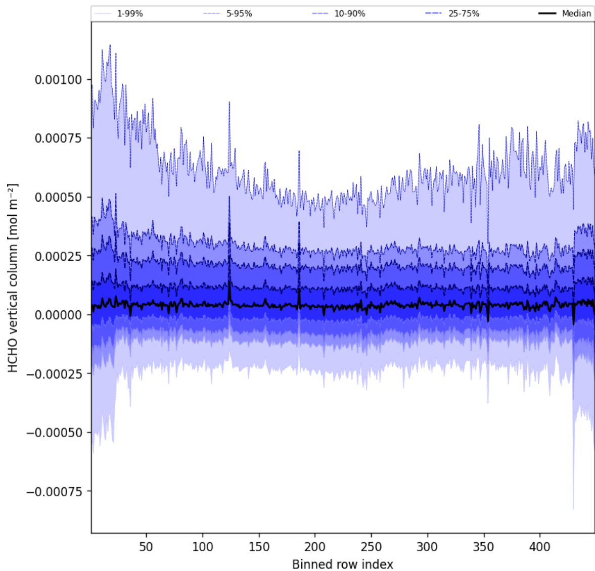
Figure 47: Along track statistics of “HCHO vertical column” for 2025-09-02 to 2025-09-02
