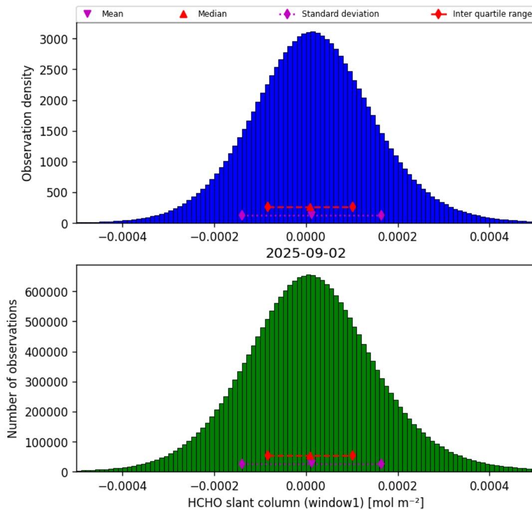
Figure 36: Histogram of “HCHO slant column (window1)” for 2025-09-02 to 2025-09-02
