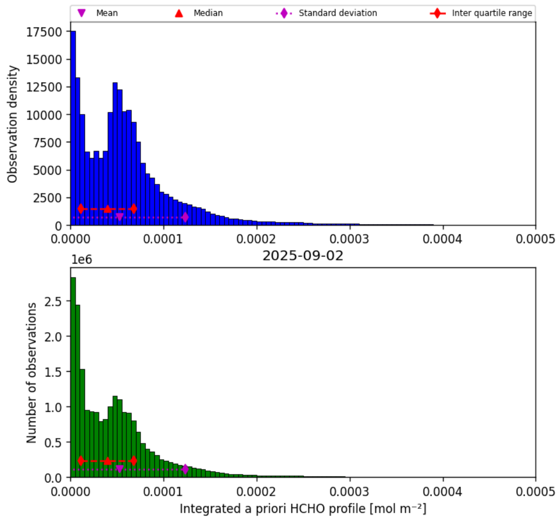
Figure 41: Histogram of “Integrated a priori HCHO profile” for 2025-09-02 to 2025-09-02
