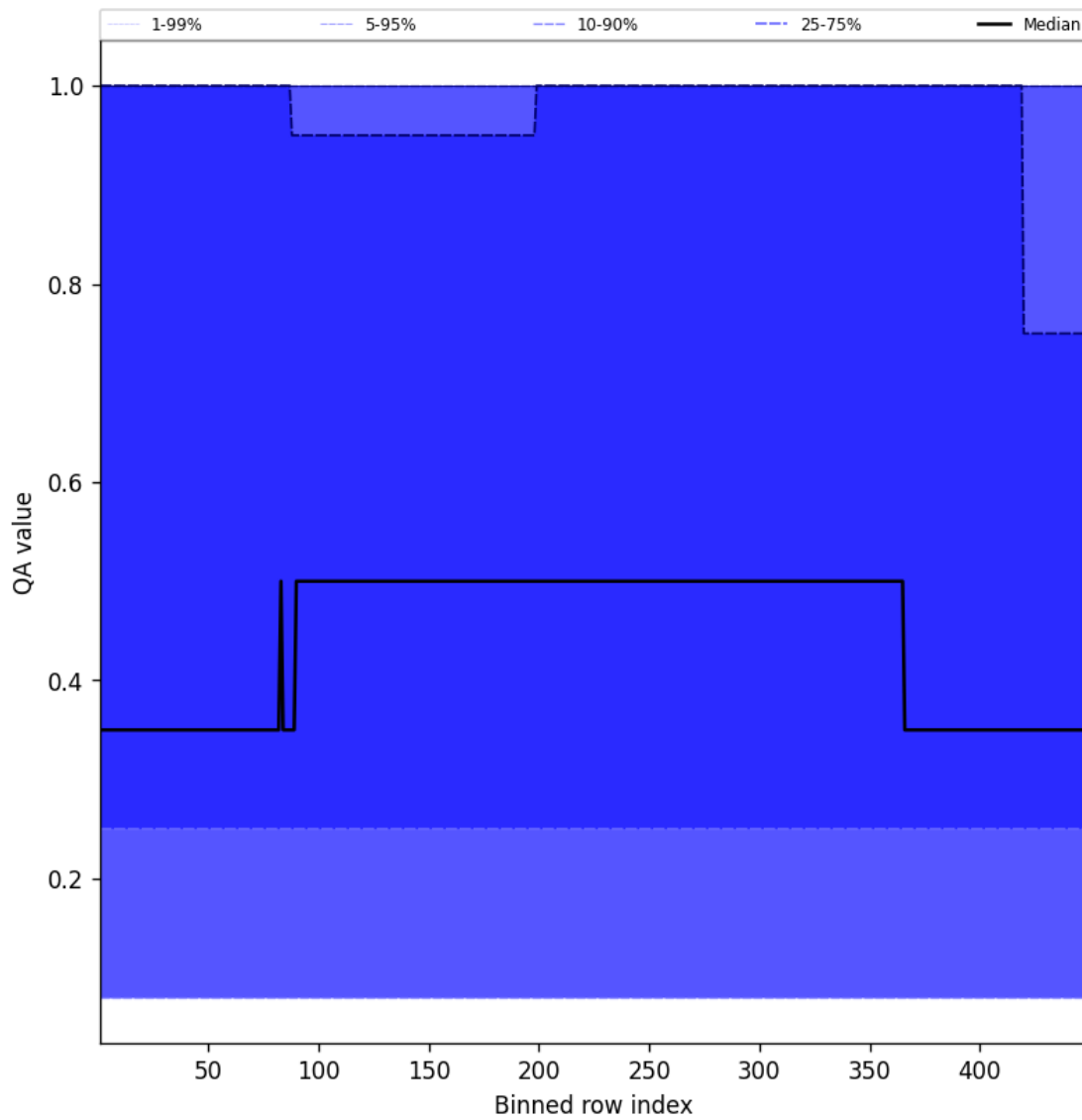
Figure 46: Along track statistics of “QA value” for 2025-09-02 to 2025-09-02
