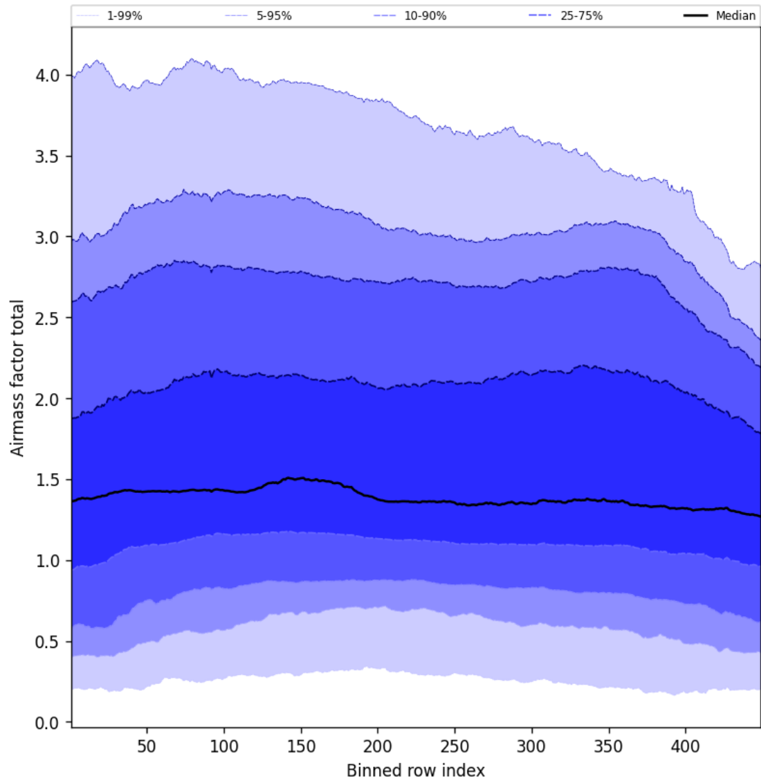
Figure 52: Along track statistics of “Airmass factor total” for 2025-09-02 to 2025-09-02
