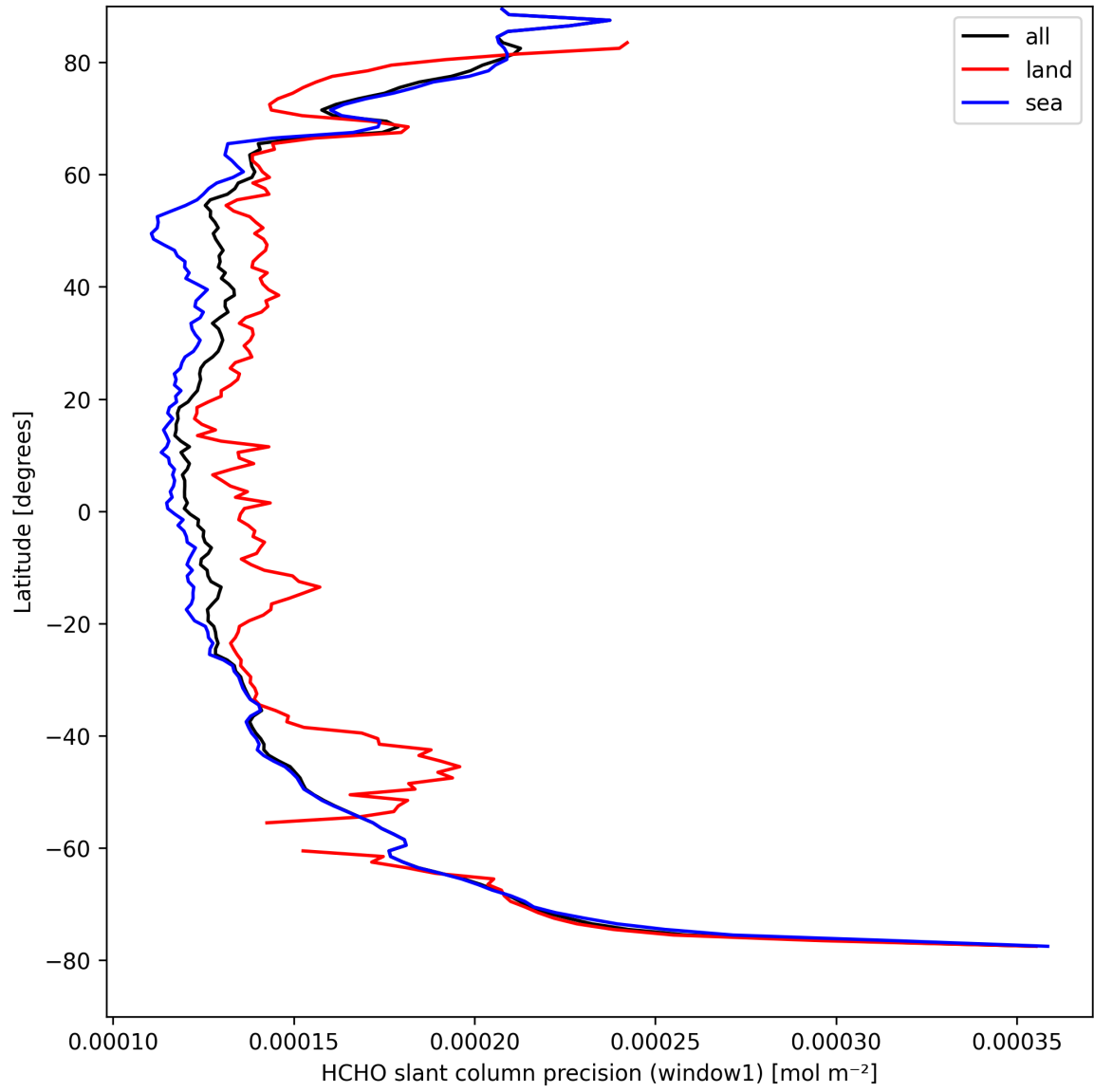
Figure 23: Zonal average of "HCHO slant column precision (window1)" for 2025-09-02 to 2025-09-02.
