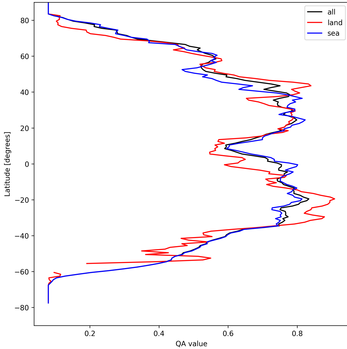
Figure 18: Zonal average of “QA value” for 2025-09-02 to 2025-09-02.
