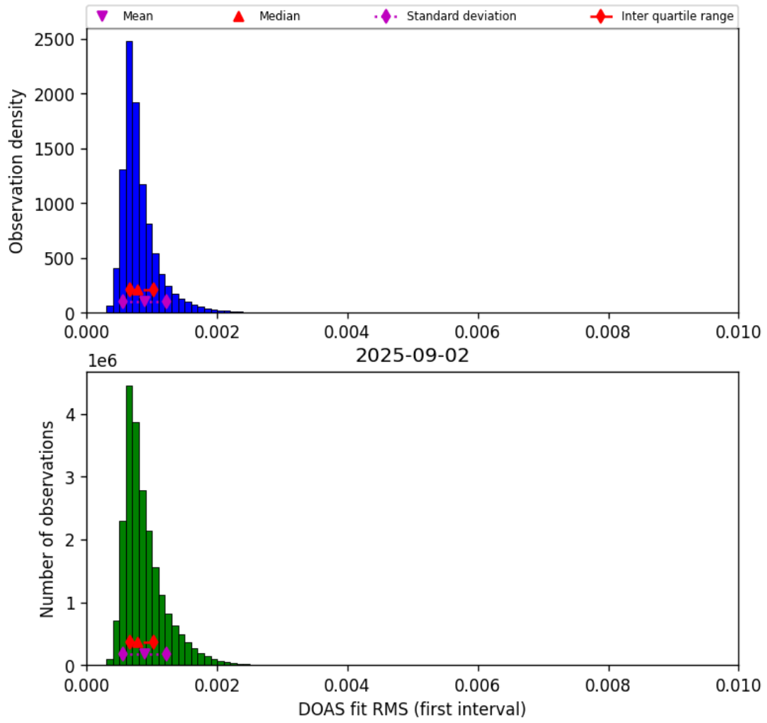
Figure 44: Histogram of “DOAS fit RMS (first interval)” for 2025-09-02 to 2025-09-02
