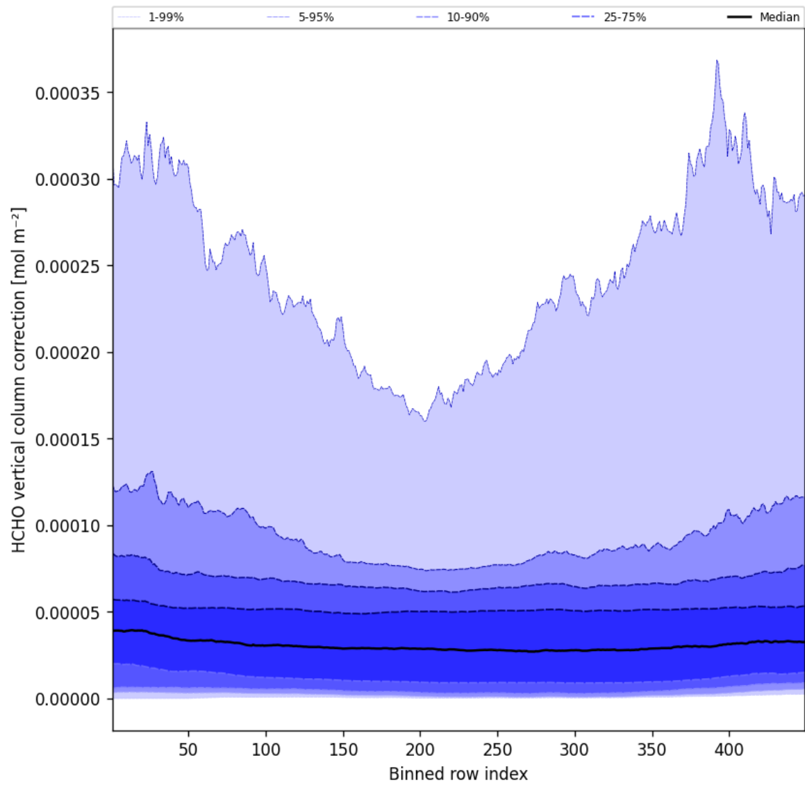
Figure 49: Along track statistics of “HCHO vertical column correction” for 2025-09-02 to 2025-09-02
