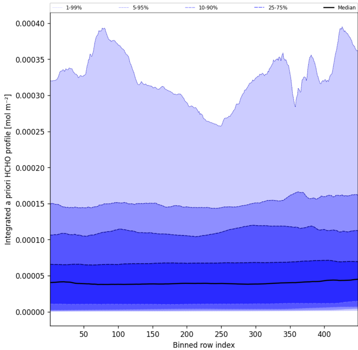
Figure 55: Along track statistics of “Integrated a priori HCHO profile” for 2025-09-02 to 2025-09-02
