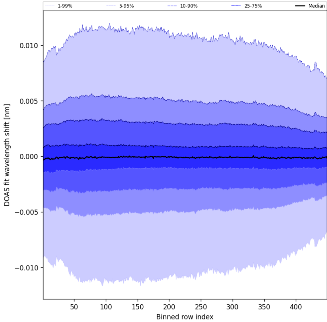
Figure 56: Along track statistics of “DOAS fit wavelength shift” for 2025-09-02 to 2025-09-02
