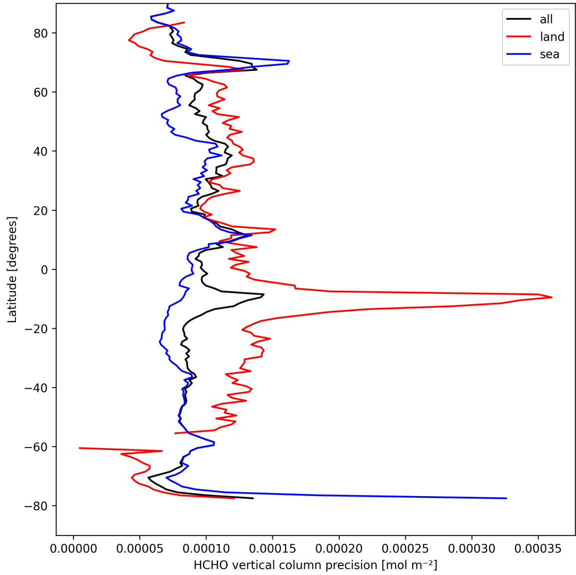
Figure 20: Zonal average of “HCHO vertical column precision” for 2025-09-02 to 2025-09-02.
