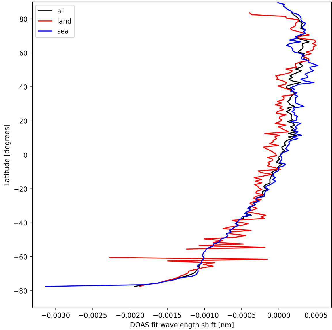
Figure 28: Zonal average of “DOAS fit wavelength shift” for 2025-09-02 to 2025-09-02.
