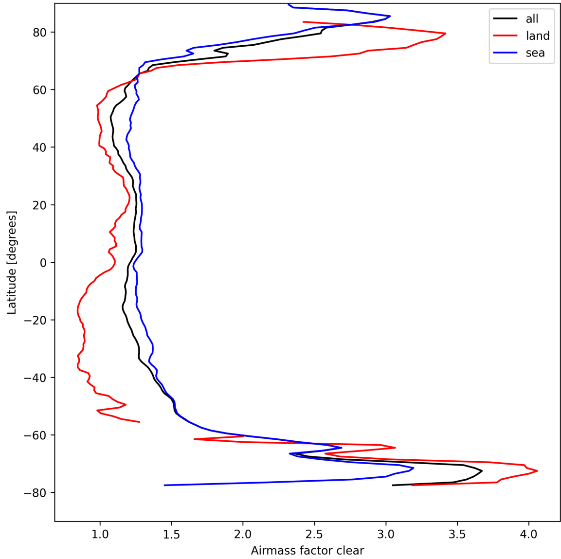
Figure 26: Zonal average of “Airmass factor clear” for 2025-09-02 to 2025-09-02.
