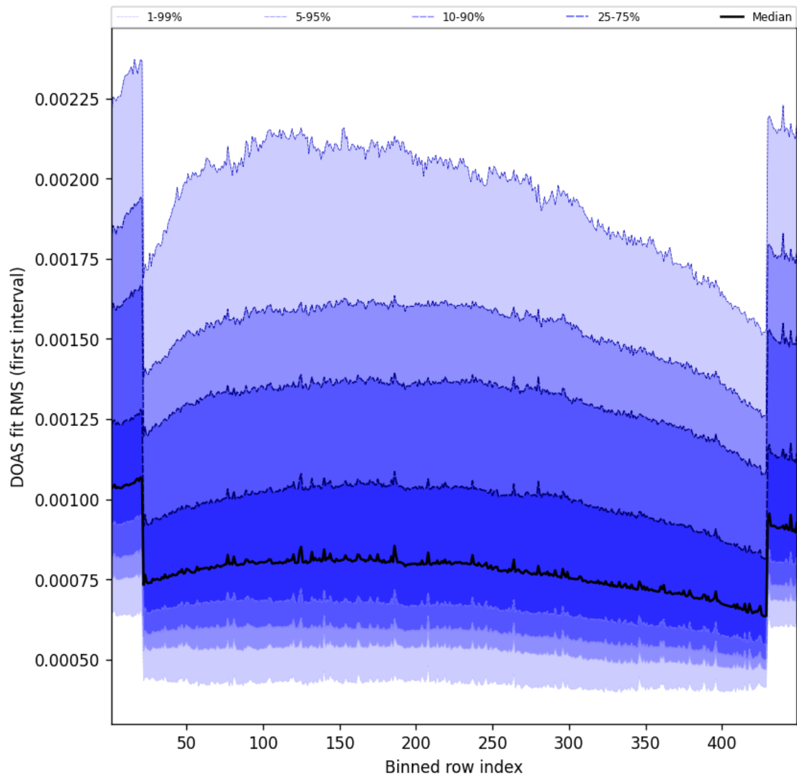
Figure 58: Along track statistics of “DOAS fit RMS (first interval)” for 2025-09-02 to 2025-09-02
