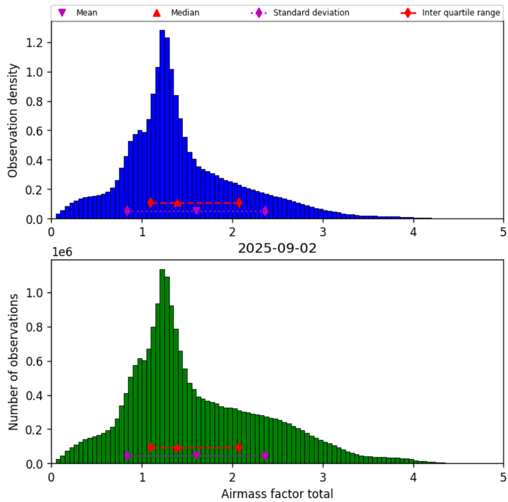
Figure 38: Histogram of “Airmass factor total” for 2025-09-02 to 2025-09-02
