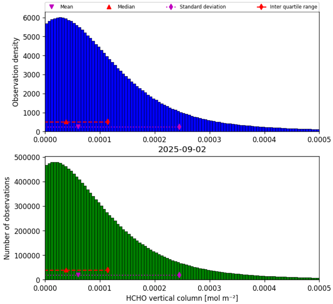
Figure 33: Histogram of “HCHO vertical column” for 2025-09-02 to 2025-09-02
