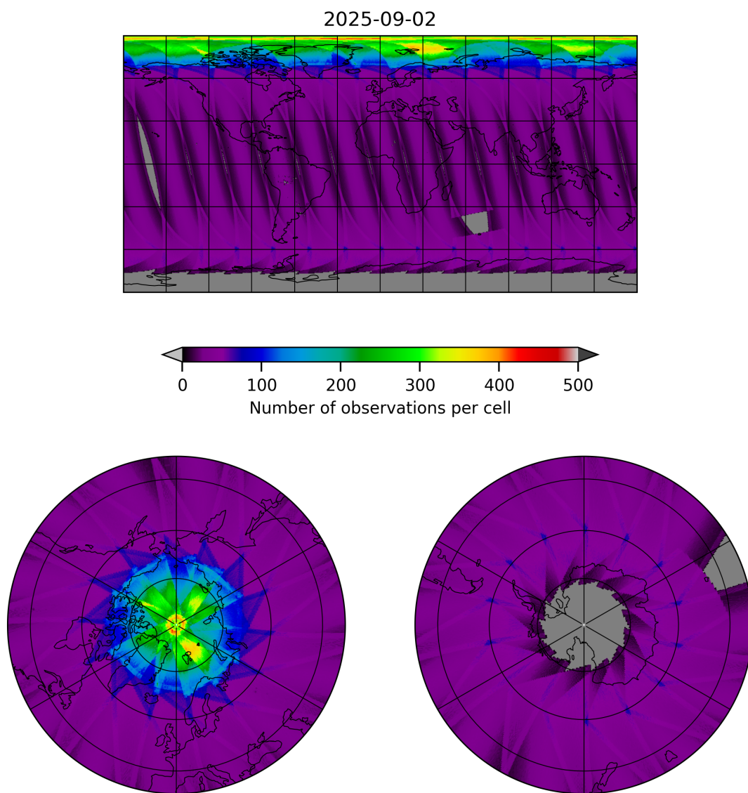
Figure 17: Map of the number of observations for 2025-09-02 to 2025-09-02
