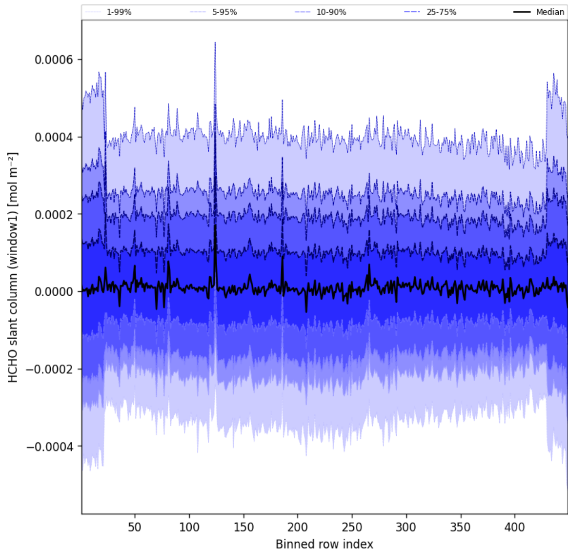
Figure 50: Along track statistics of “HCHO slant column (window1)” for 2025-09-02 to 2025-09-02
