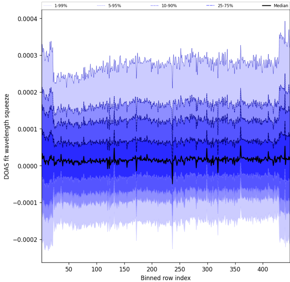
Figure 57: Along track statistics of “DOAS fit wavelength squeeze” for 2025-09-03 to 2025-09-04
