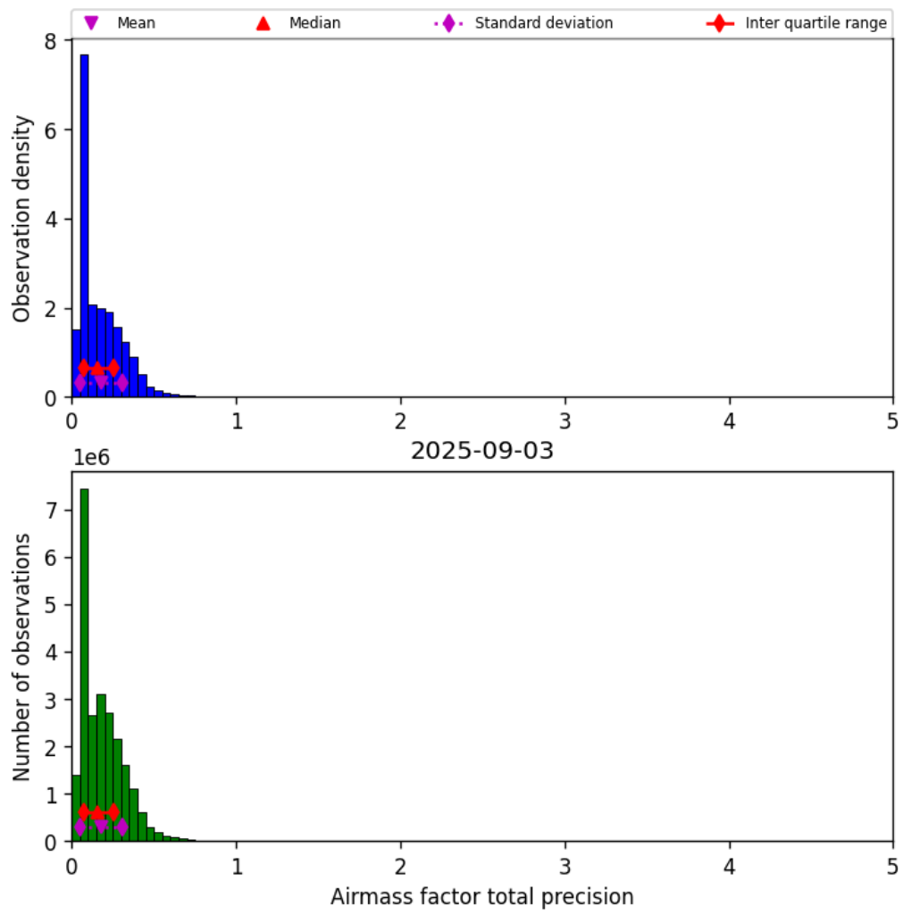
Figure 39: Histogram of “Airmass factor total precision” for 2025-09-03 to 2025-09-04
