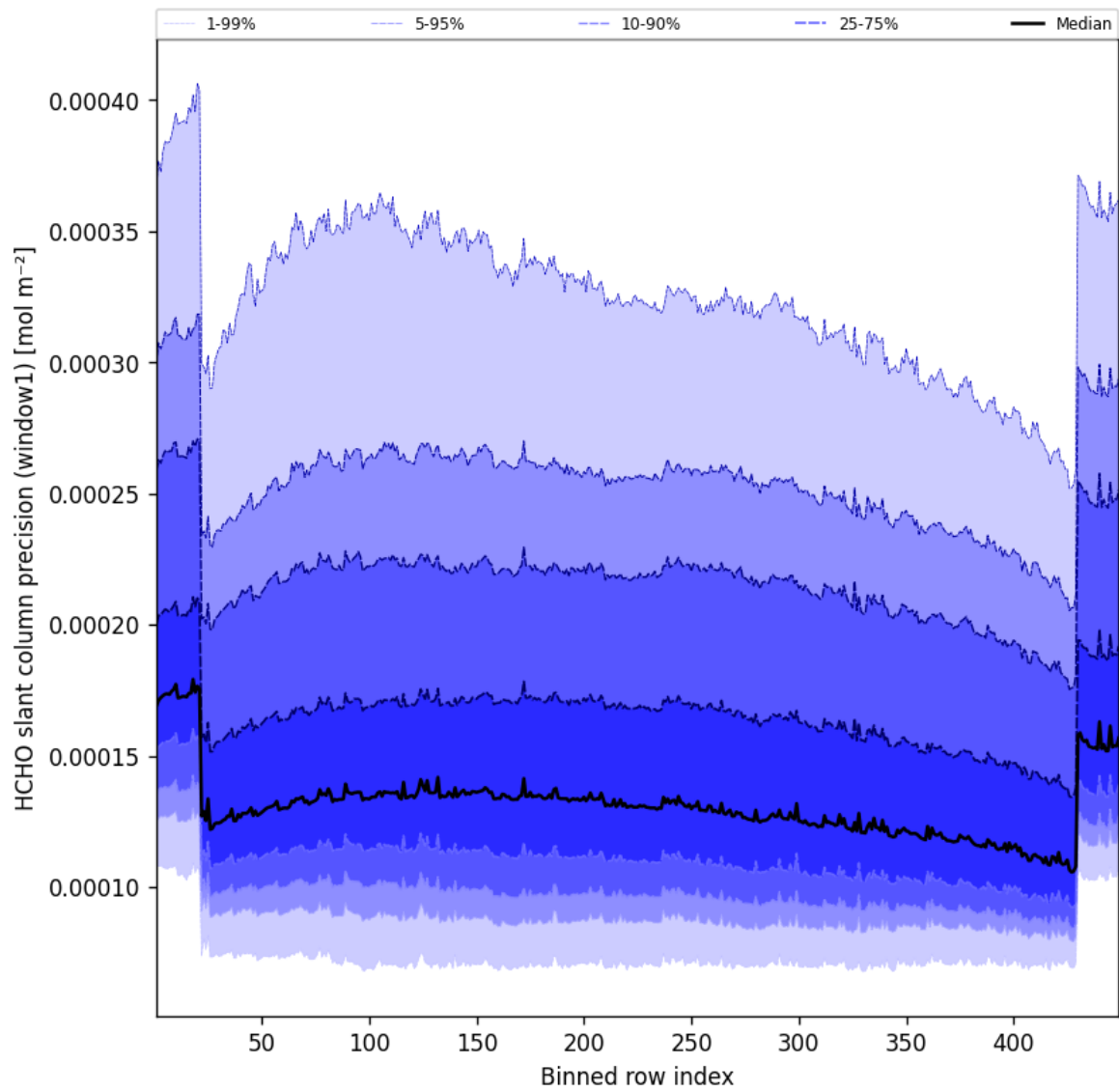
Figure 51: Along track statistics of “HCHO slant column precision (window1)” for 2025-09-03 to 2025-09-04
