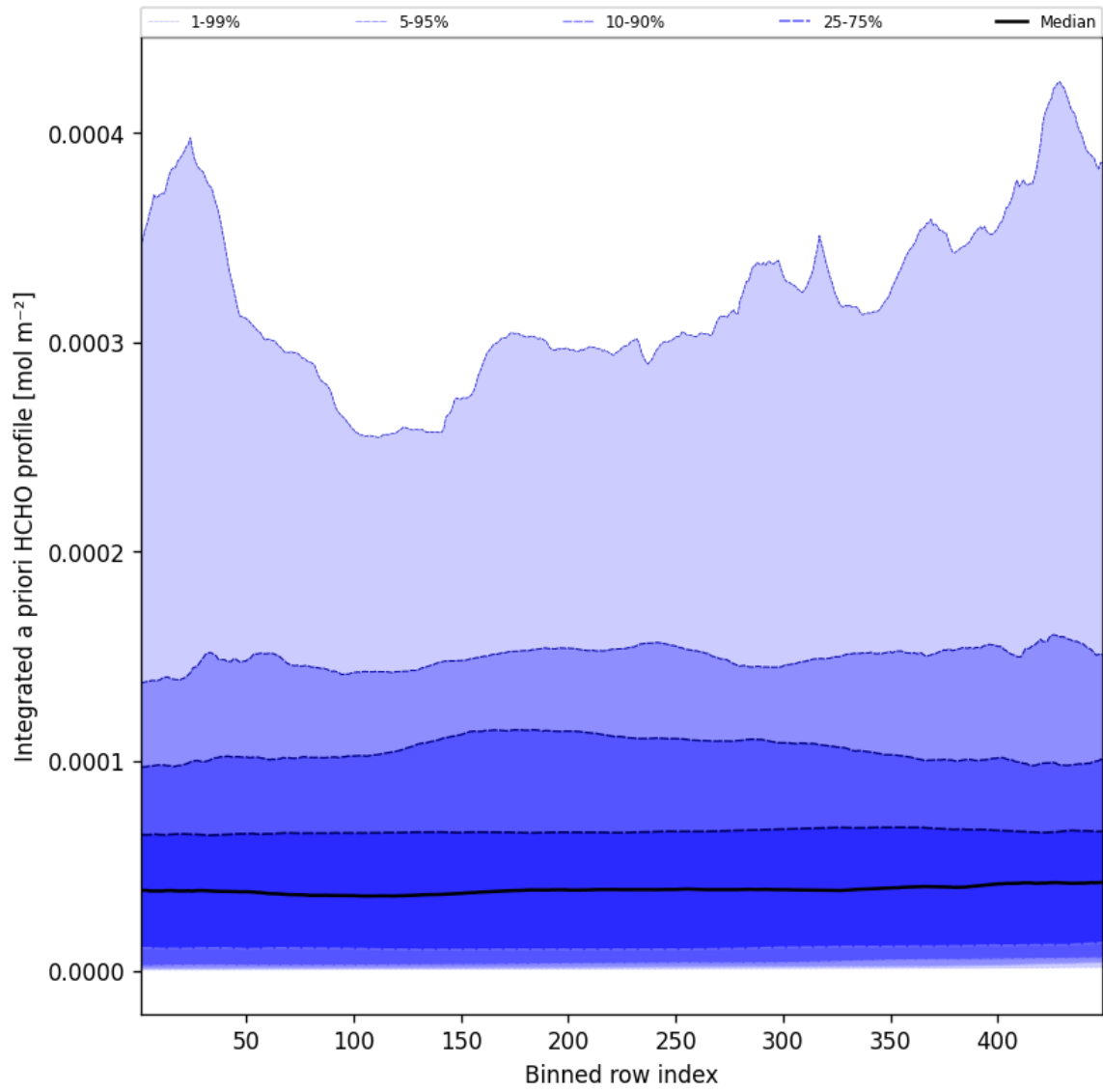
Figure 55: Along track statistics of "Integrated a priori HCHO profile" for 2025-09-03 to 2025-09-04
