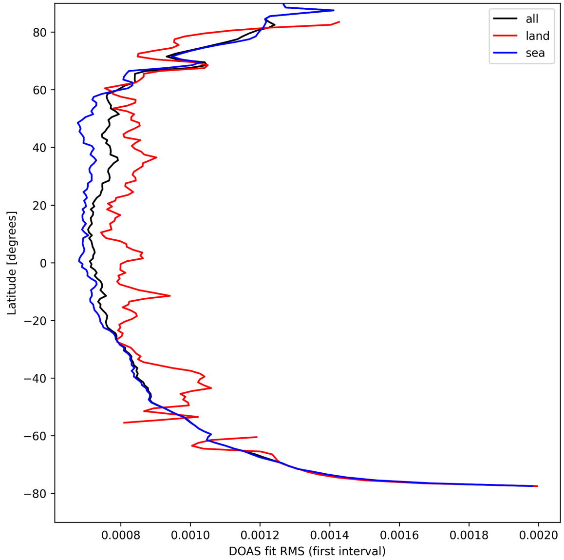
Figure 30: Zonal average of “DOAS fit RMS (first interval)” for 2025-09-03 to 2025-09-04.
