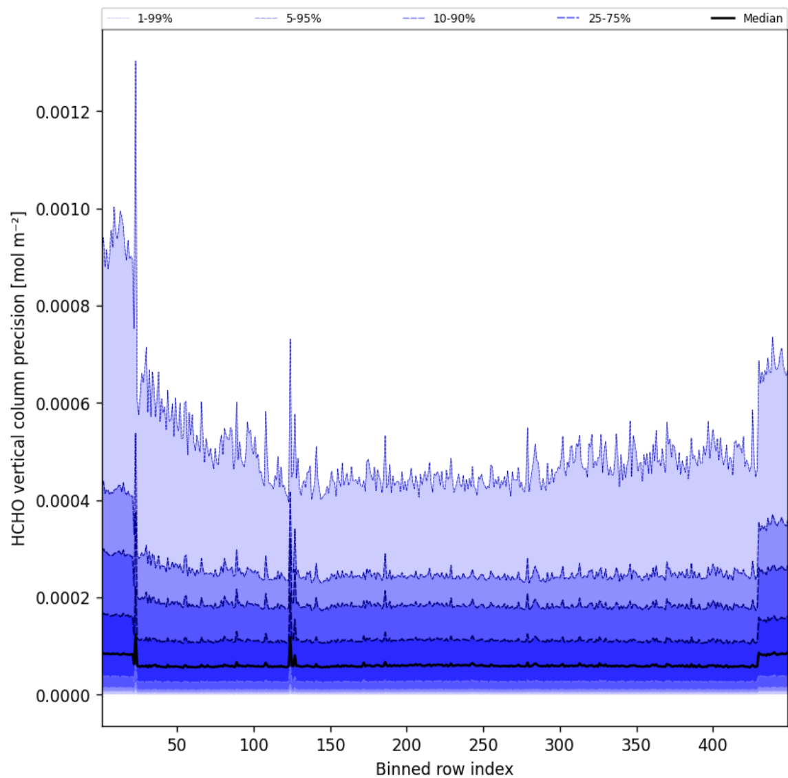
Figure 48: Along track statistics of “HCHO vertical column precision” for 2025-09-03 to 2025-09-04
