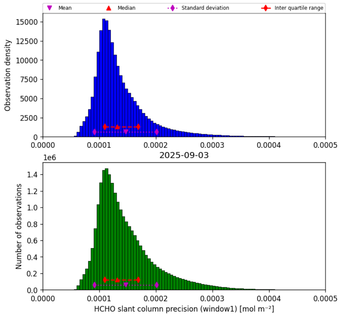
Figure 37: Histogram of “HCHO slant column precision (window1)” for 2025-09-03 to 2025-09-04
