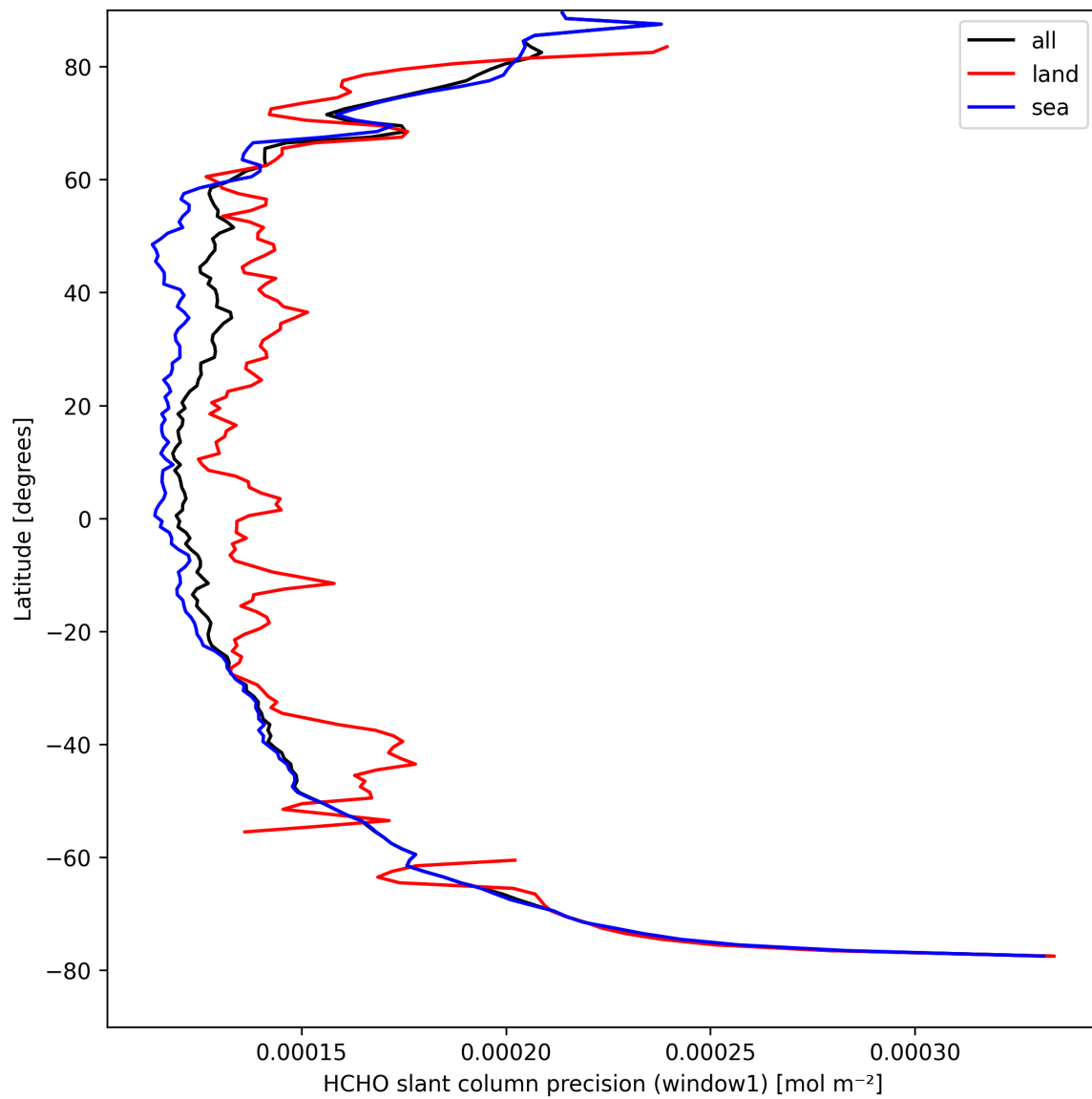
Figure 23: Zonal average of “HCHO slant column precision (window1)” for 2025-09-03 to 2025-09-04.
