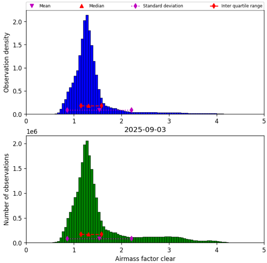
Figure 40: Histogram of “Airmass factor clear” for 2025-09-03 to 2025-09-04
