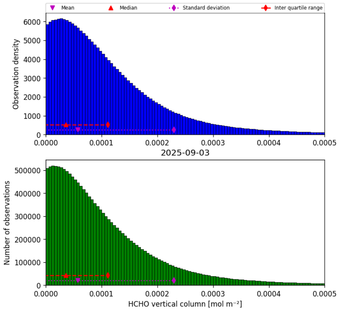
Figure 33: Histogram of “HCHO vertical column” for 2025-09-03 to 2025-09-04
