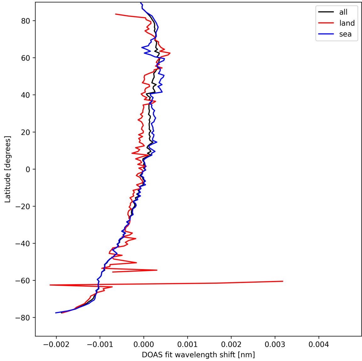
Figure 28: Zonal average of “DOAS fit wavelength shift” for 2025-09-03 to 2025-09-04.
