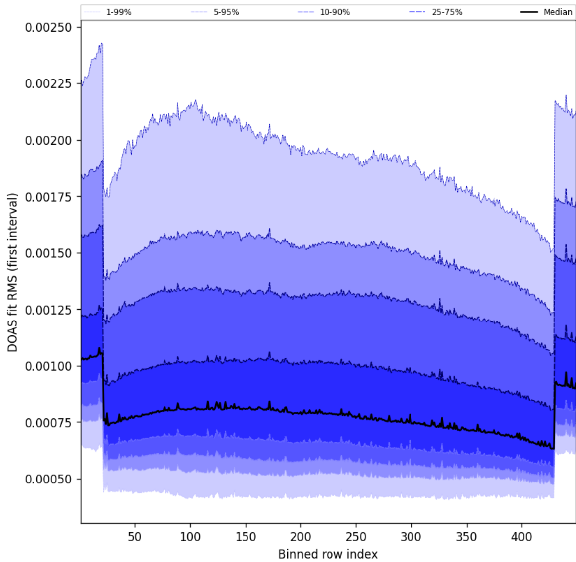
Figure 58: Along track statistics of “DOAS fit RMS (first interval)” for 2025-09-03 to 2025-09-04
