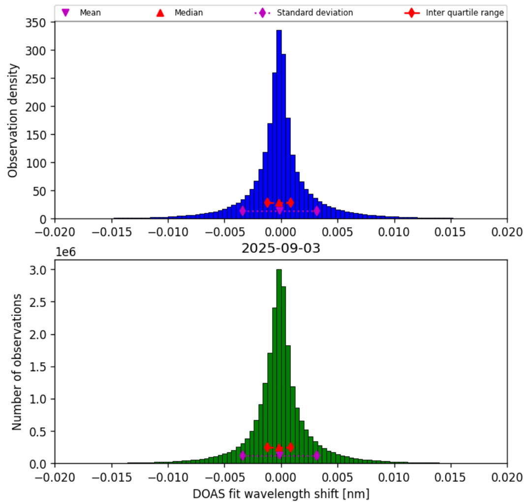
Figure 42: Histogram of “DOAS fit wavelength shift” for 2025-09-03 to 2025-09-04
