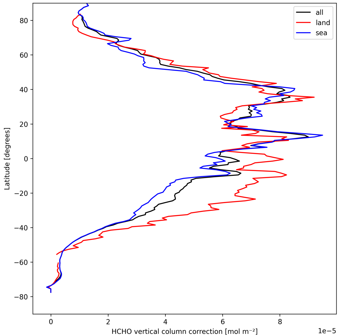
Figure 21: Zonal average of “HCHO vertical column correction” for 2025-09-03 to 2025-09-04.
