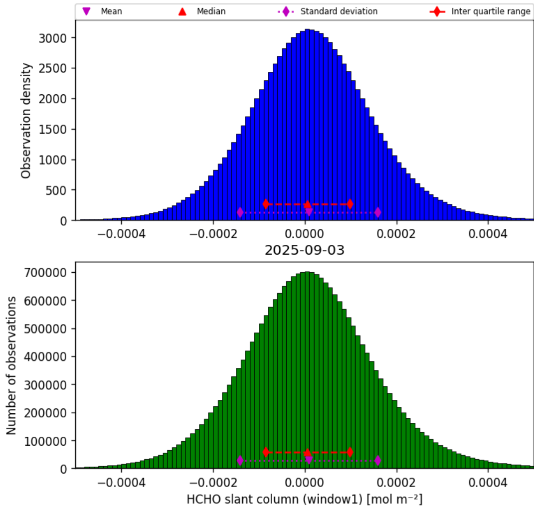
Figure 36: Histogram of “HCHO slant column (window1)” for 2025-09-03 to 2025-09-04
