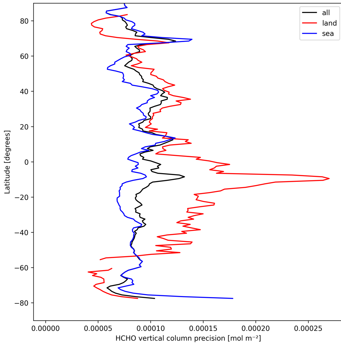
Figure 20: Zonal average of “HCHO vertical column precision” for 2025-09-03 to 2025-09-04.
