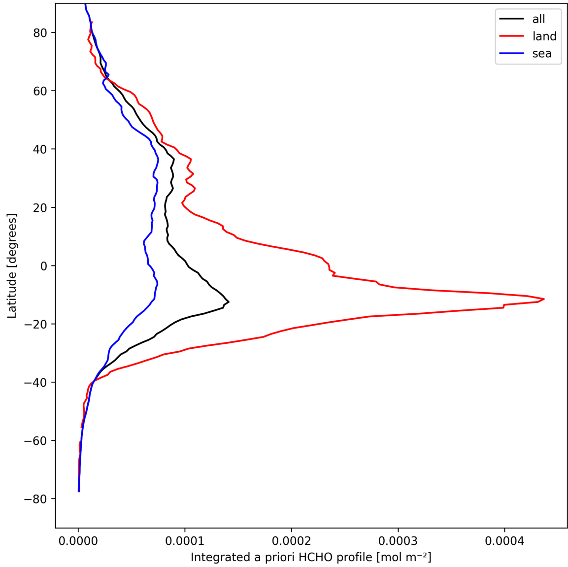
Figure 27: Zonal average of “Integrated a priori HCHO profile” for 2025-09-03 to 2025-09-04.
