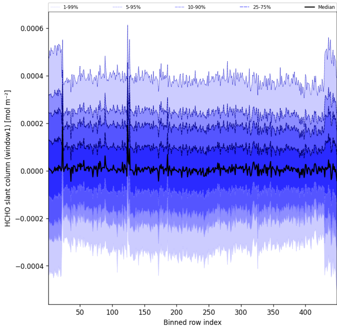
Figure 50: Along track statistics of “HCHO slant column (window1)” for 2025-09-03 to 2025-09-04
