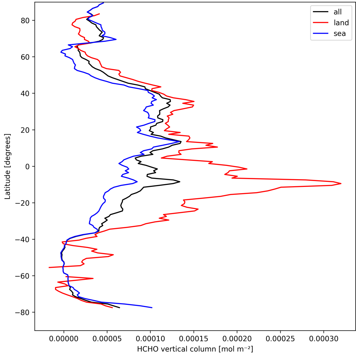
Figure 19: Zonal average of “HCHO vertical column” for 2025-09-03 to 2025-09-04.
