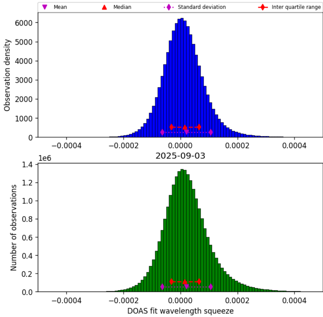
Figure 43: Histogram of “DOAS fit wavelength squeeze” for 2025-09-03 to 2025-09-04
