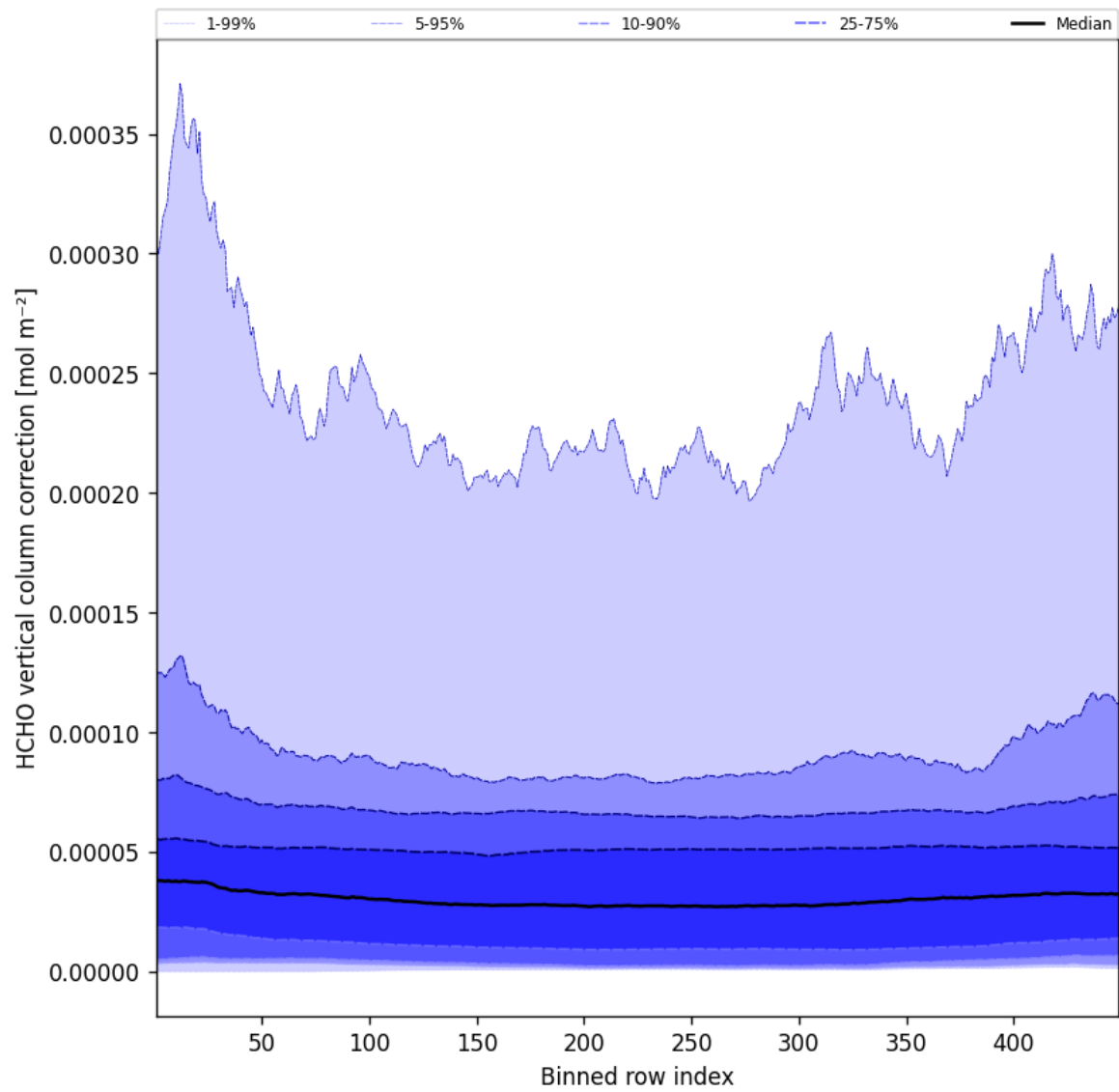
Figure 49: Along track statistics of “HCHO vertical column correction” for 2025-09-03 to 2025-09-04
