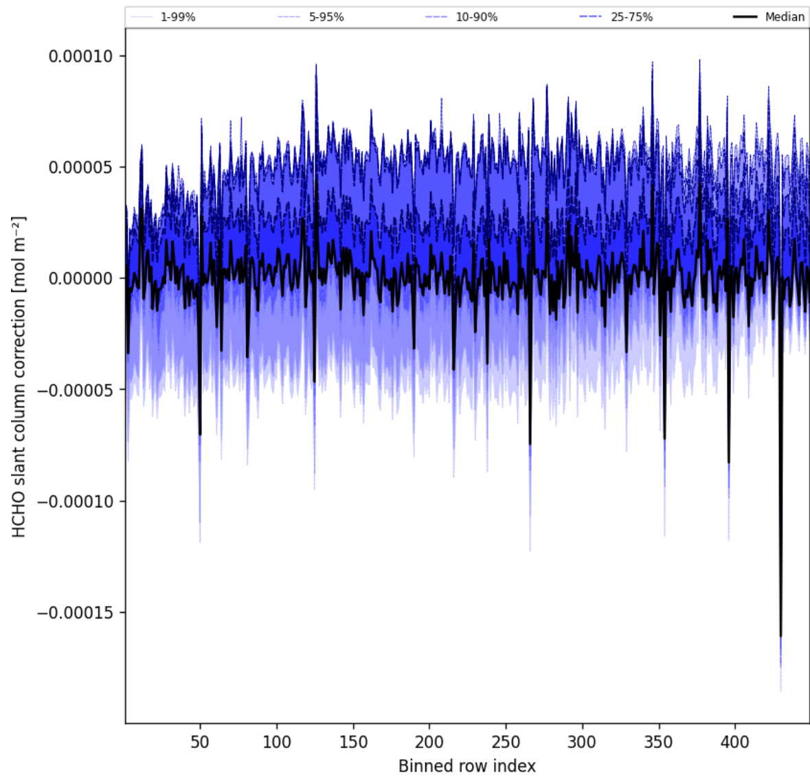
Figure 59: Along track statistics of “HCHO slant column correction” for 2025-09-03 to 2025-09-04
