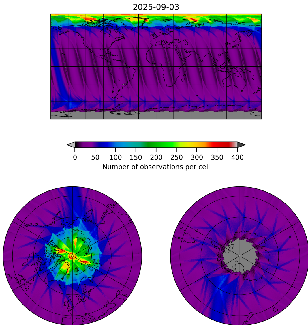
Figure 17: Map of the number of observations for 2025-09-03 to 2025-09-04
