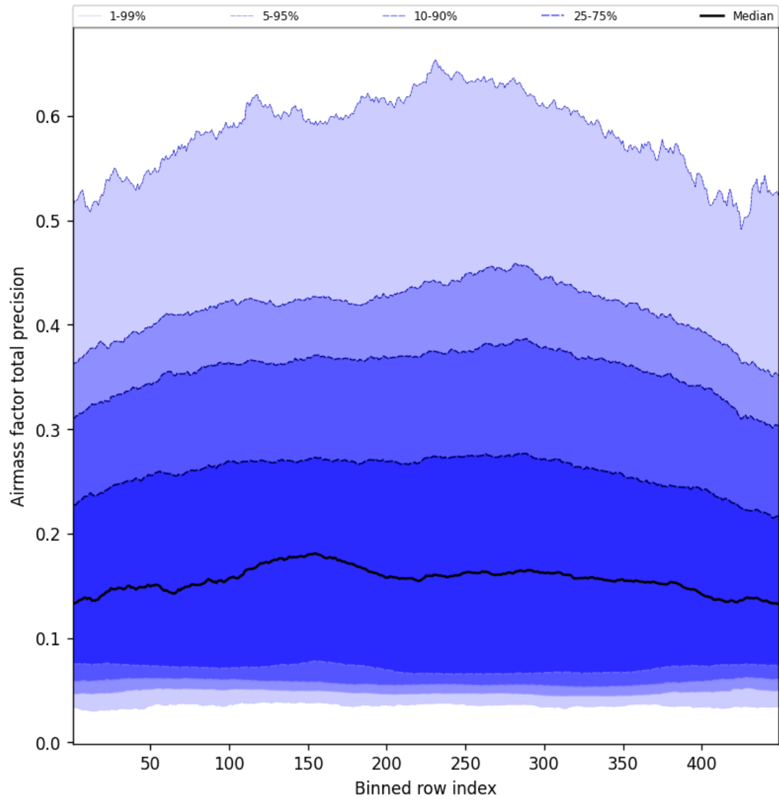
Figure 53: Along track statistics of “Airmass factor total precision” for 2025-09-03 to 2025-09-04
