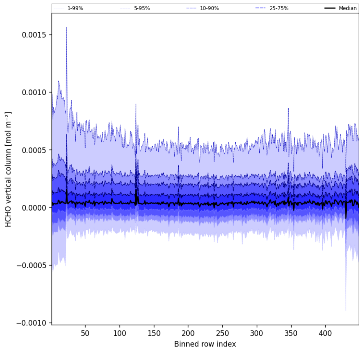
Figure 47: Along track statistics of “HCHO vertical column” for 2025-09-03 to 2025-09-04
