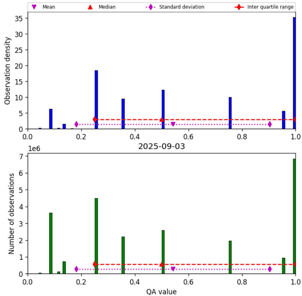
Figure 32: Histogram of “QA value” for 2025-09-03 to 2025-09-04
