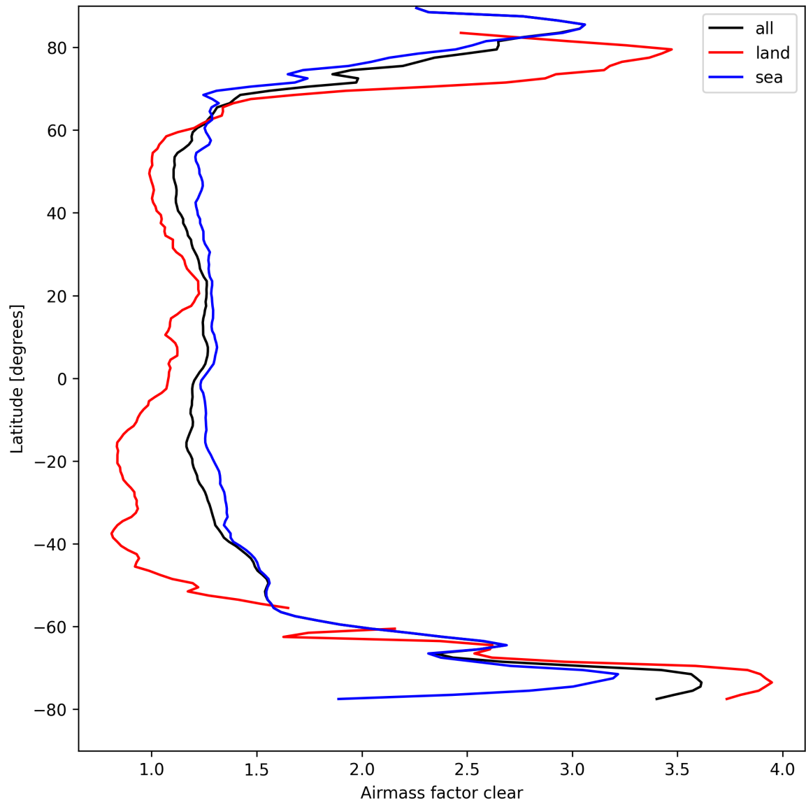
Figure 26: Zonal average of “Airmass factor clear” for 2025-09-03 to 2025-09-04.
