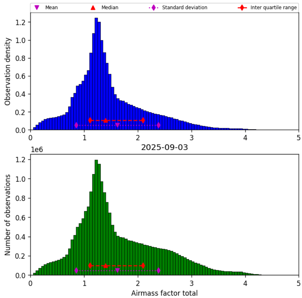
Figure 38: Histogram of “Airmass factor total” for 2025-09-03 to 2025-09-04
