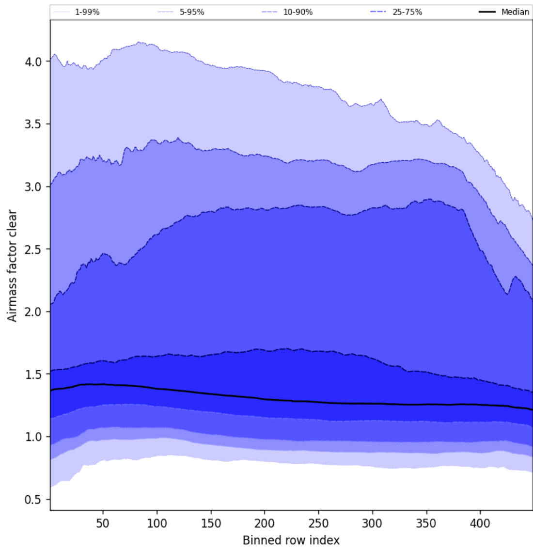
Figure 54: Along track statistics of “Airmass factor clear” for 2025-09-03 to 2025-09-04
