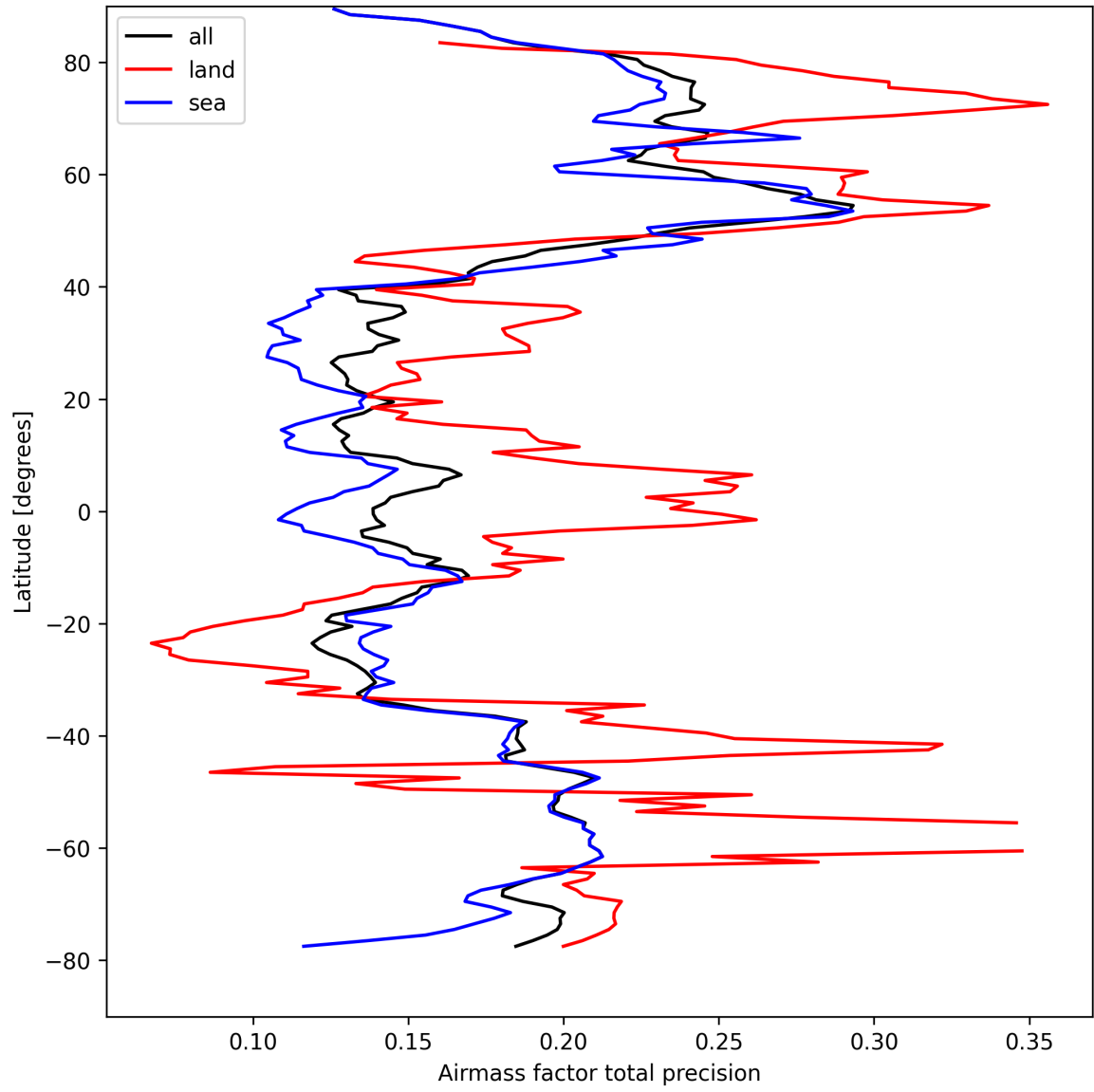
Figure 25: Zonal average of “Airmass factor total precision” for 2025-09-03 to 2025-09-04.
