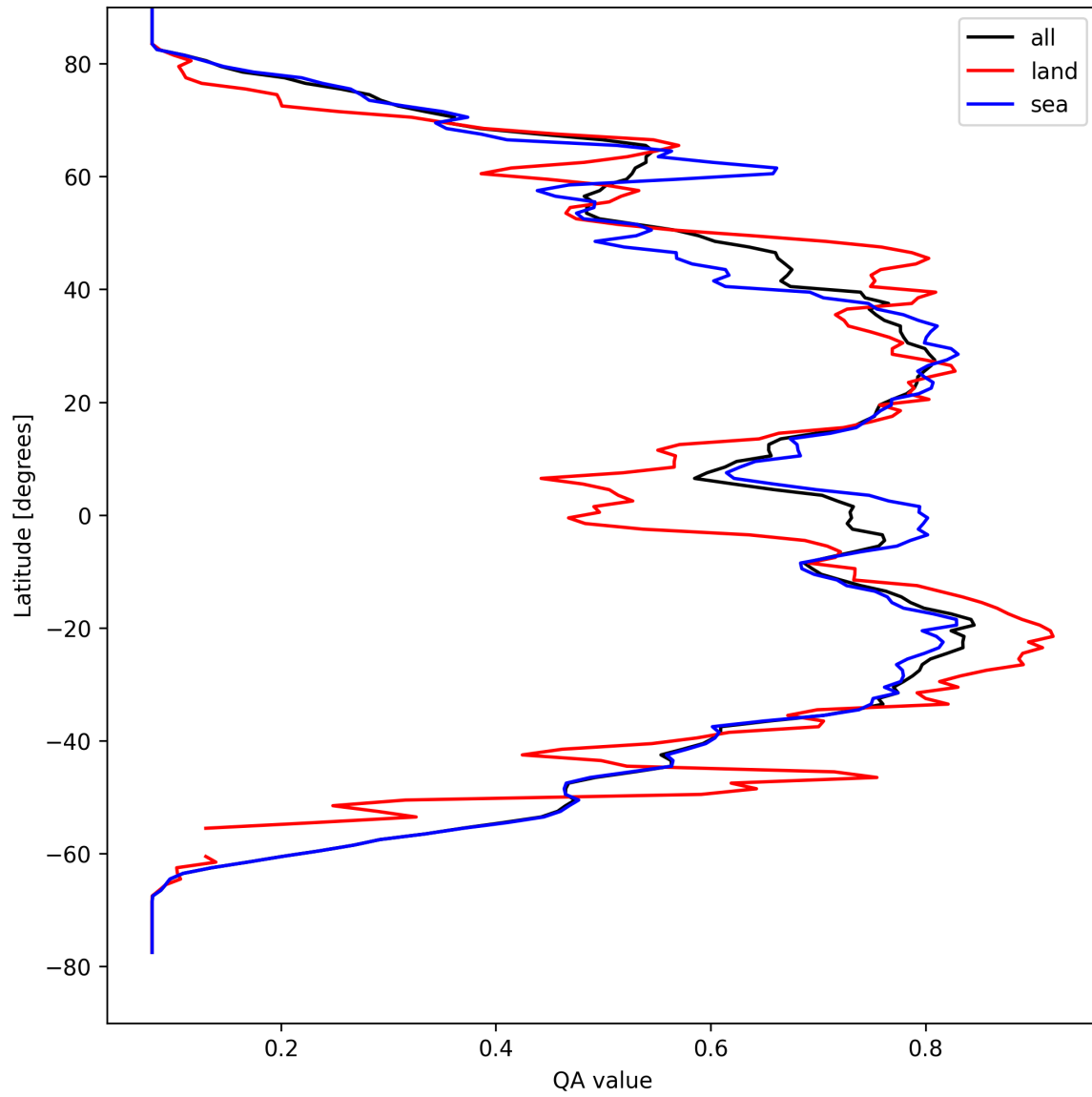
Figure 18: Zonal average of “QA value” for 2025-09-03 to 2025-09-04.
