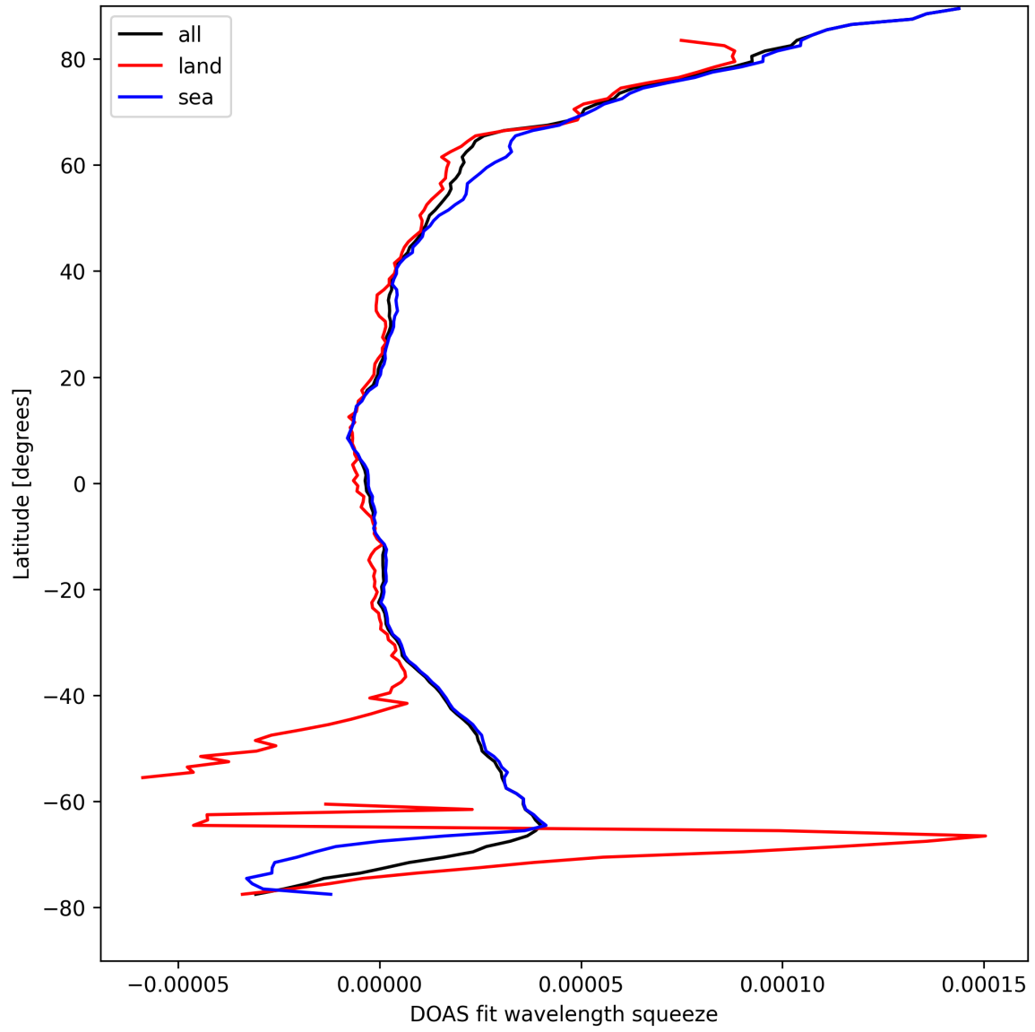
Figure 29: Zonal average of “DOAS fit wavelength squeeze” for 2025-09-03 to 2025-09-04.
