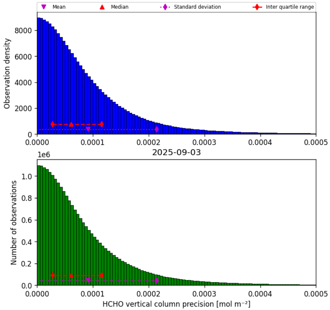
Figure 34: Histogram of “HCHO vertical column precision” for 2025-09-03 to 2025-09-04
