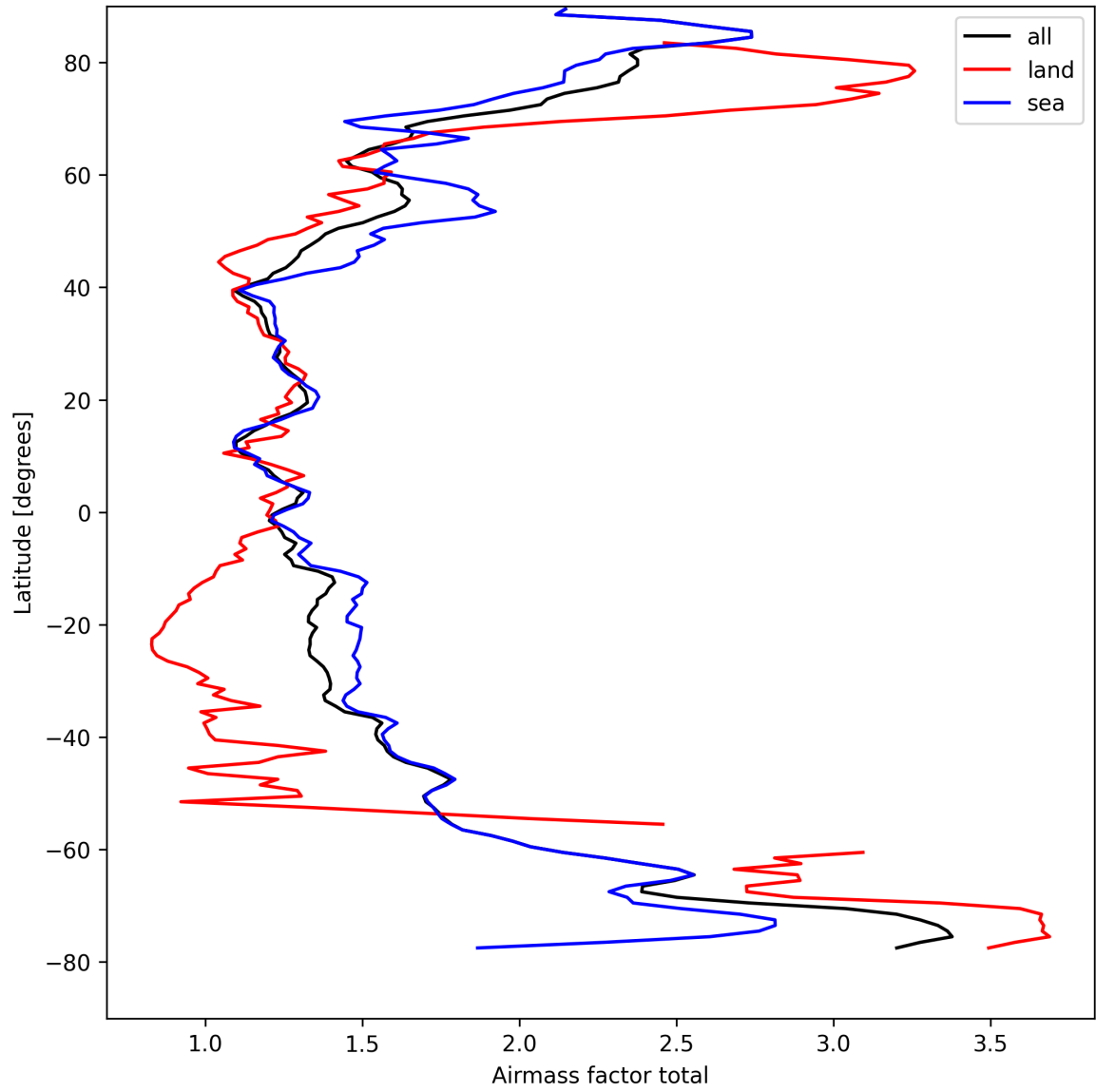
Figure 24: Zonal average of “Airmass factor total” for 2025-09-03 to 2025-09-04.
