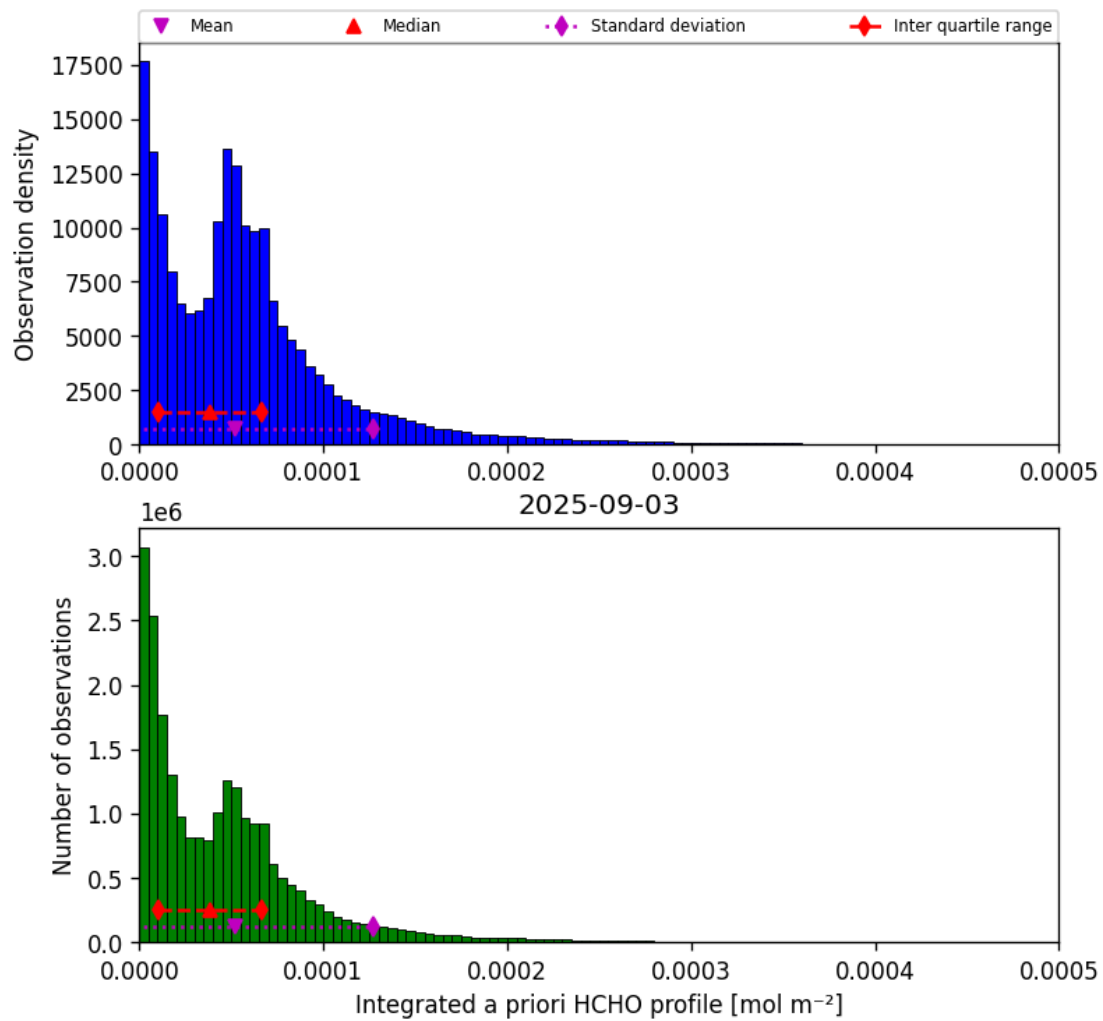
Figure 41: Histogram of “Integrated a priori HCHO profile” for 2025-09-03 to 2025-09-04
