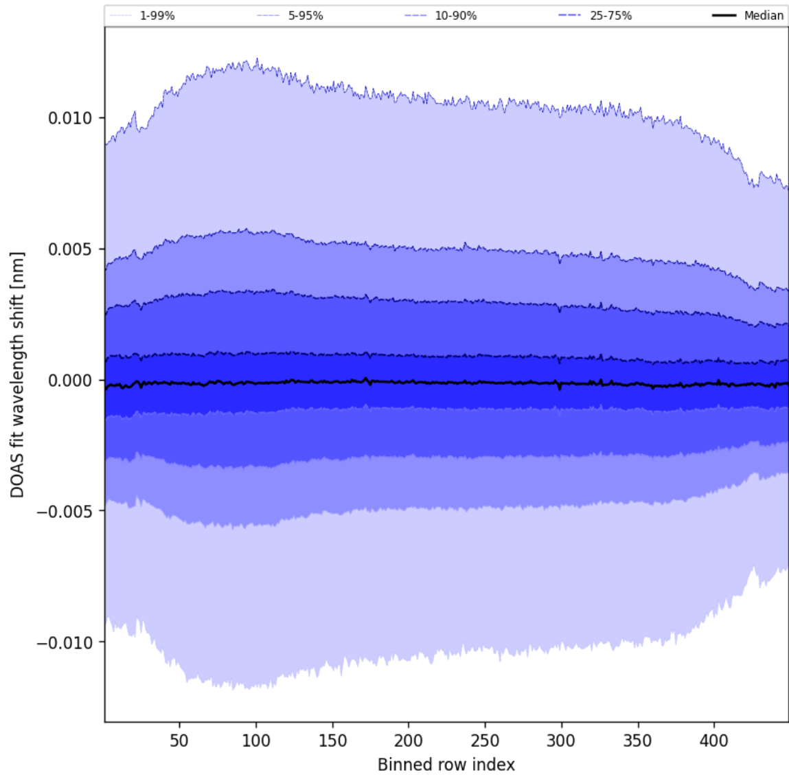
Figure 56: Along track statistics of “DOAS fit wavelength shift” for 2025-09-03 to 2025-09-04
