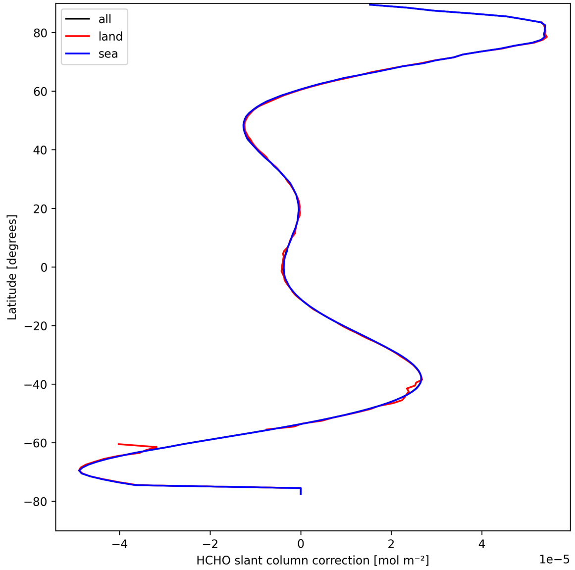
Figure 31: Zonal average of "HCHO slant column correction" for 2025-09-03 to 2025-09-04.
