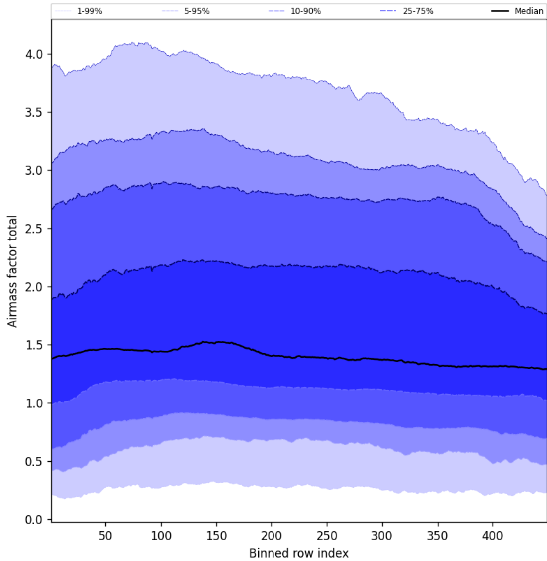
Figure 52: Along track statistics of “Airmass factor total” for 2025-09-03 to 2025-09-04
