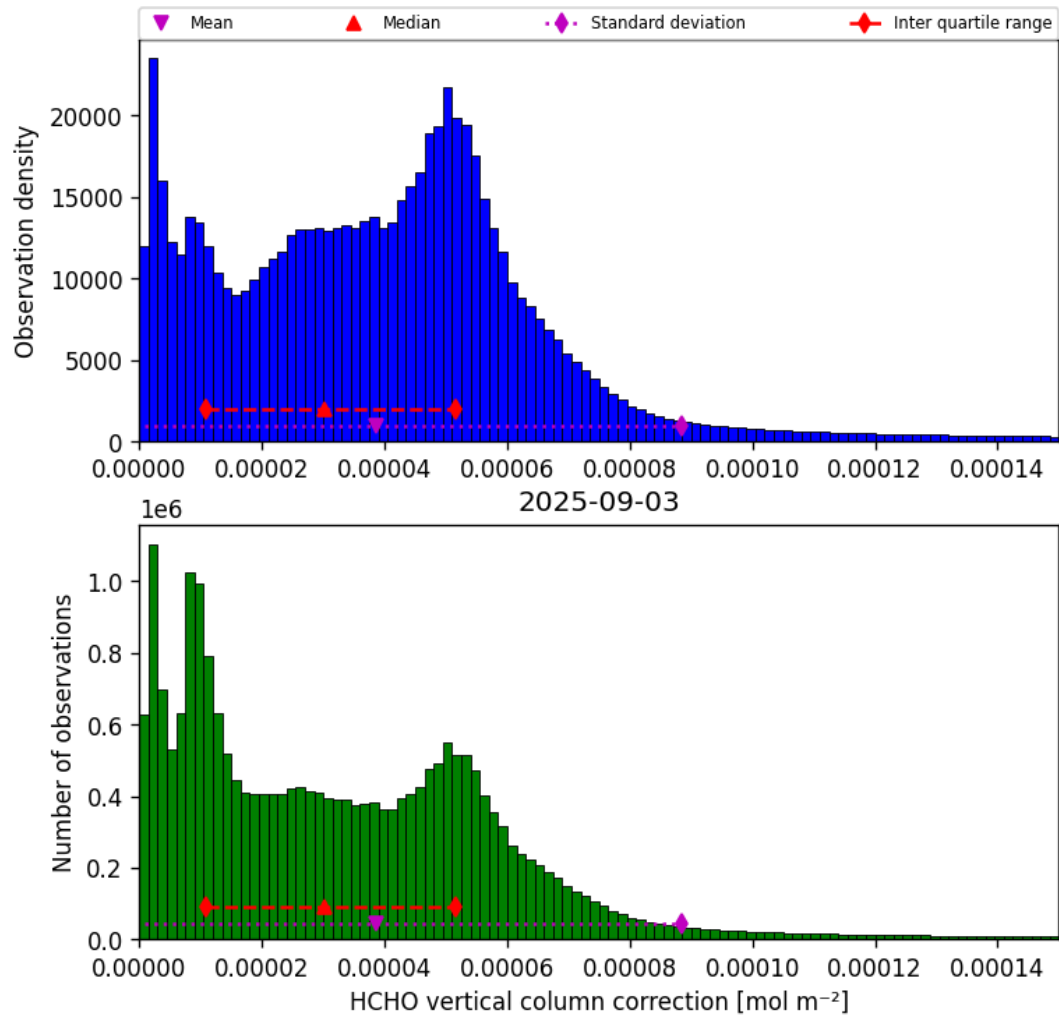
Figure 35: Histogram of “HCHO vertical column correction” for 2025-09-03 to 2025-09-04
