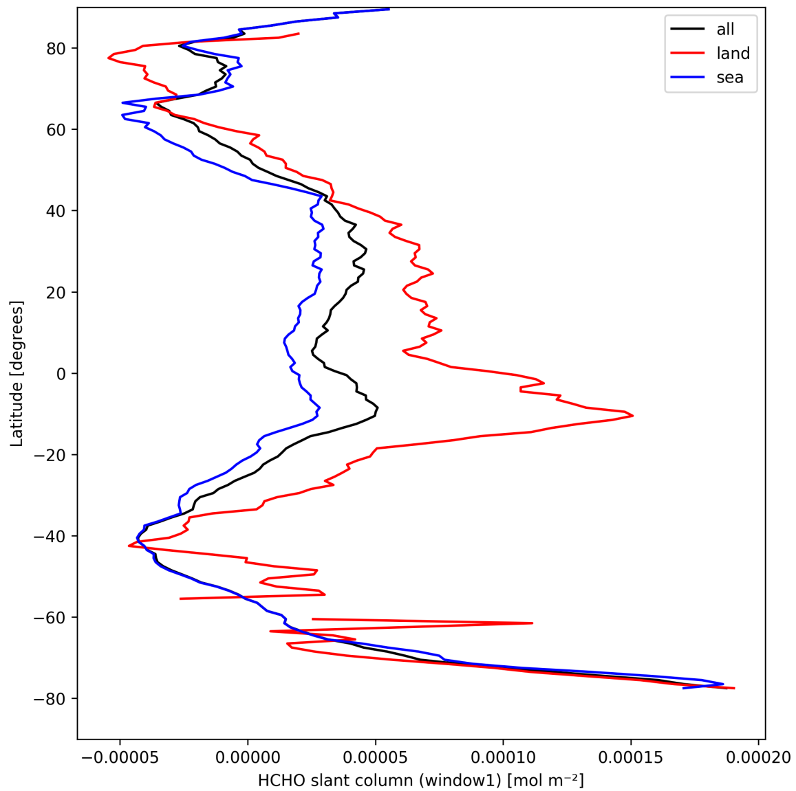
Figure 22: Zonal average of “HCHO slant column (window1)” for 2025-09-03 to 2025-09-04.
