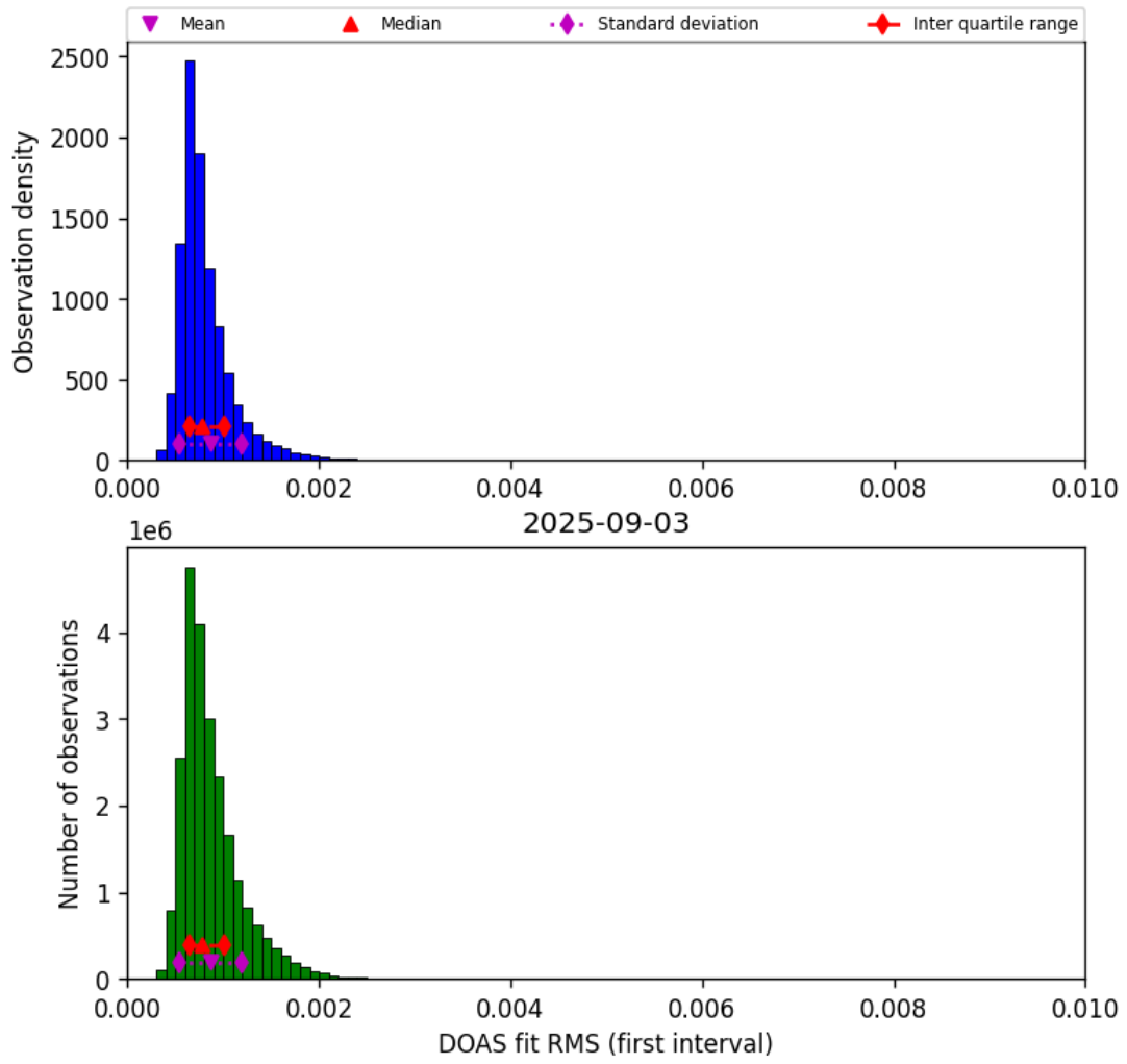
Figure 44: Histogram of “DOAS fit RMS (first interval)” for 2025-09-03 to 2025-09-04
