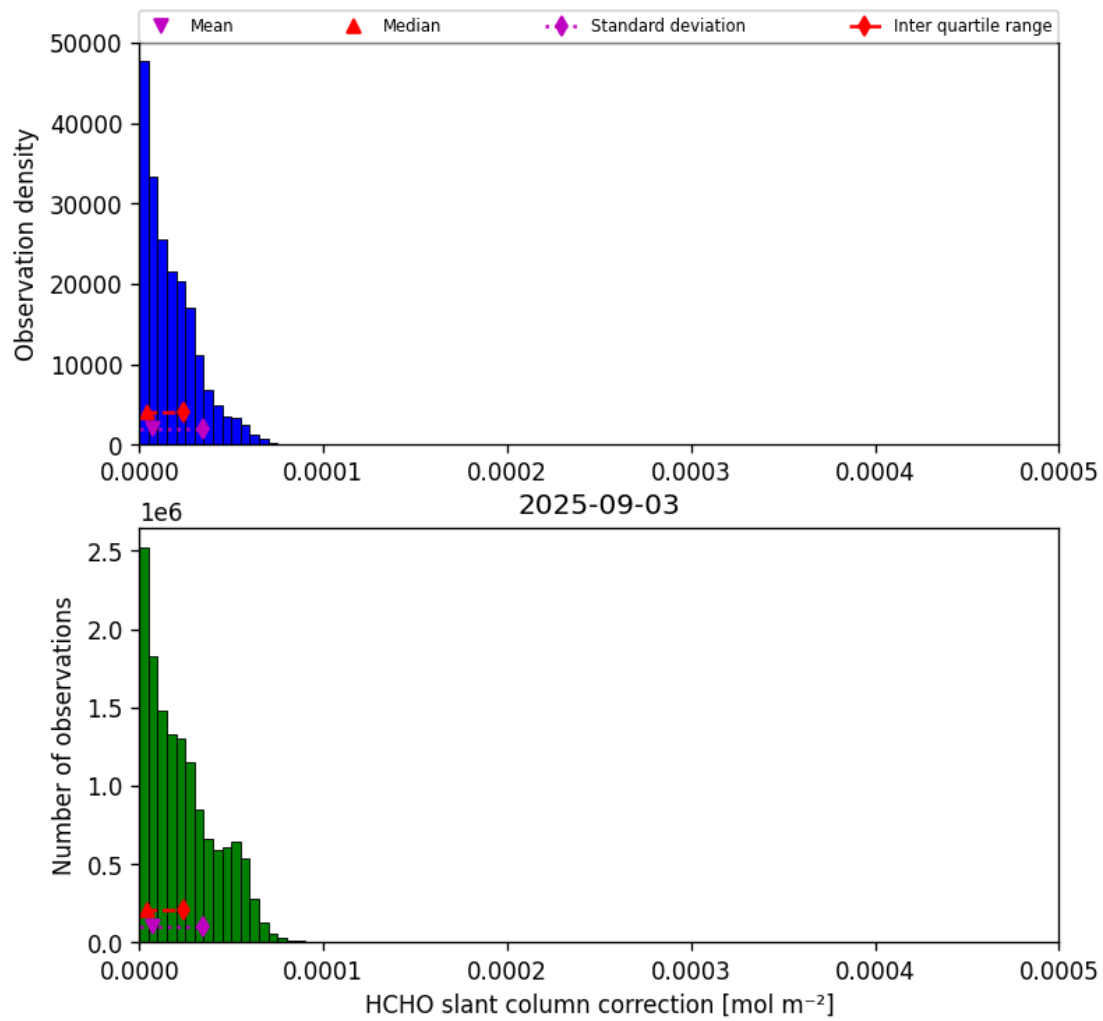
Figure 45: Histogram of “HCHO slant column correction” for 2025-09-03 to 2025-09-04
