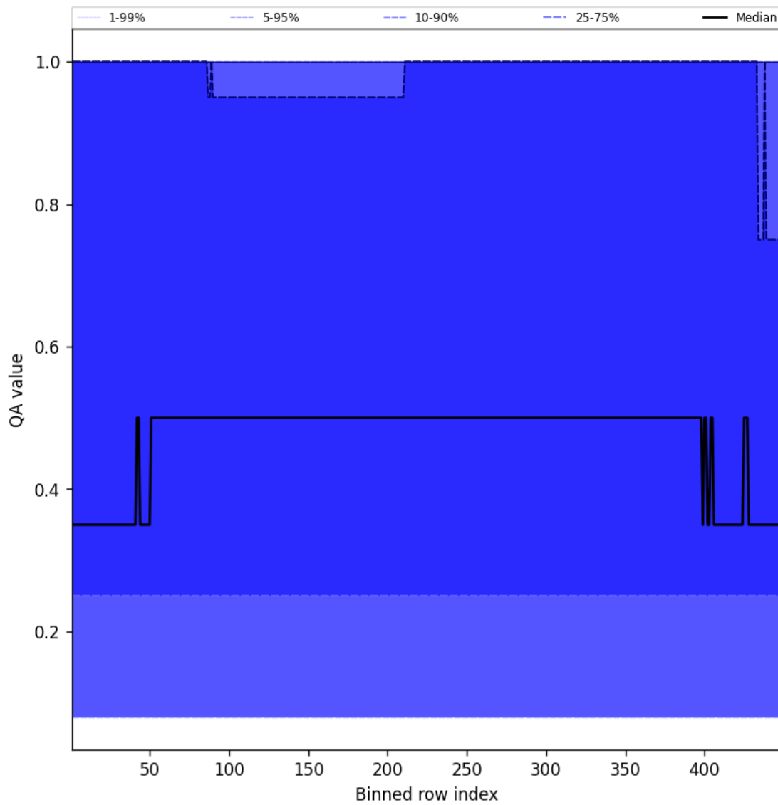
Figure 46: Along track statistics of “QA value” for 2025-09-03 to 2025-09-04
