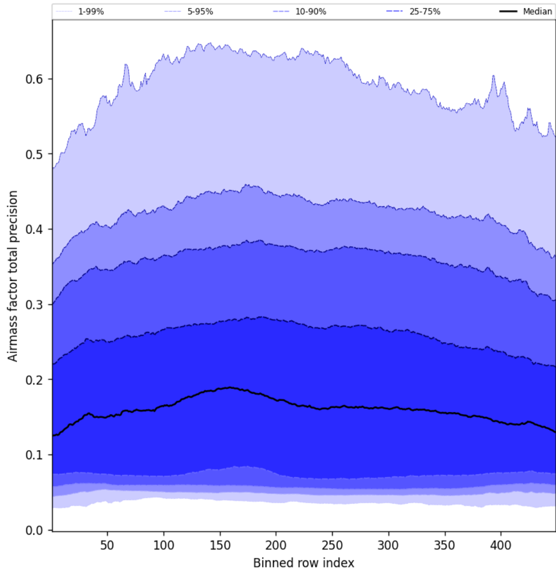
Figure 53: Along track statistics of “Airmass factor total precision” for 2025-09-04 to 2025-09-05
