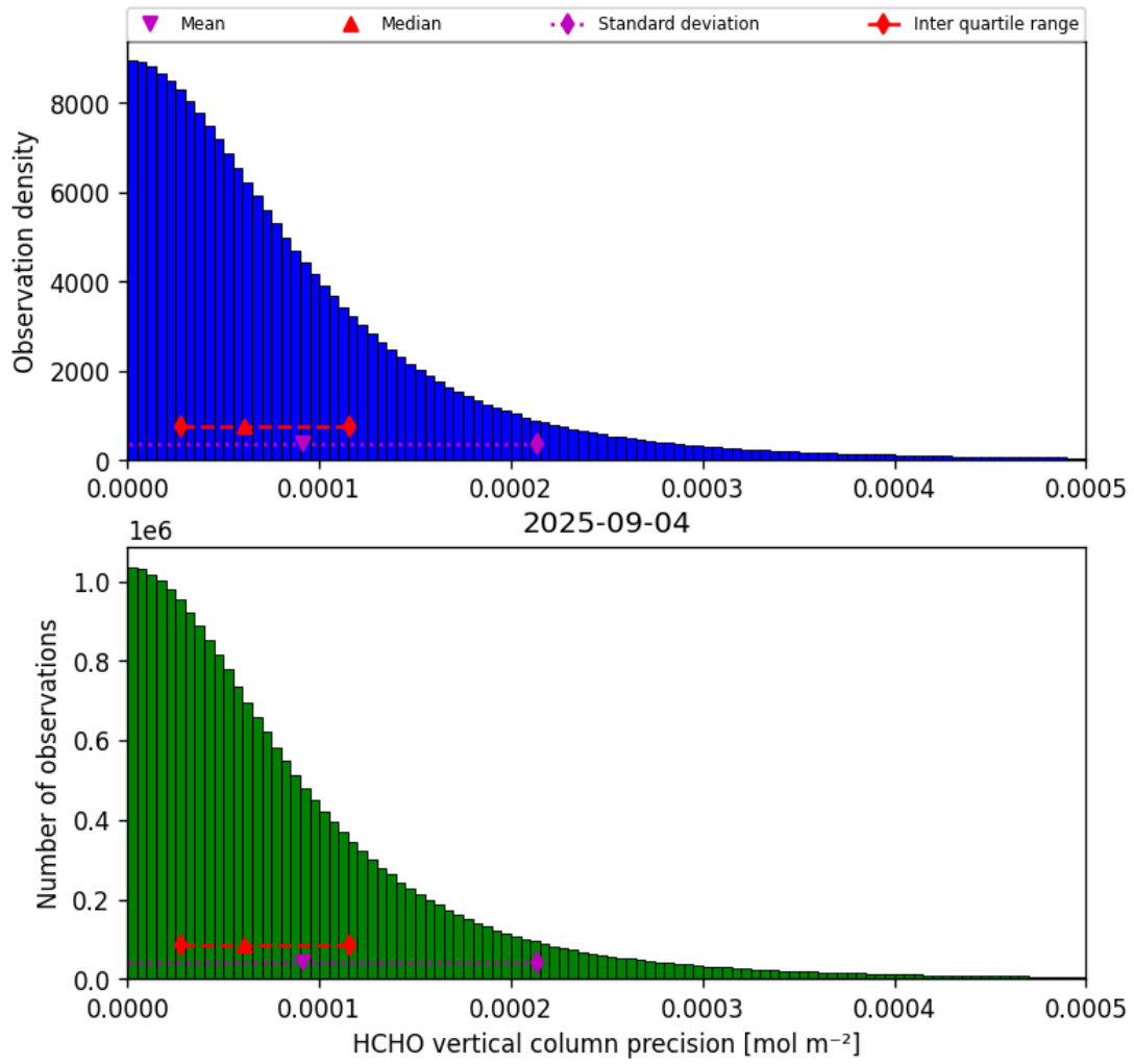
Figure 34: Histogram of “HCHO vertical column precision” for 2025-09-04 to 2025-09-05
