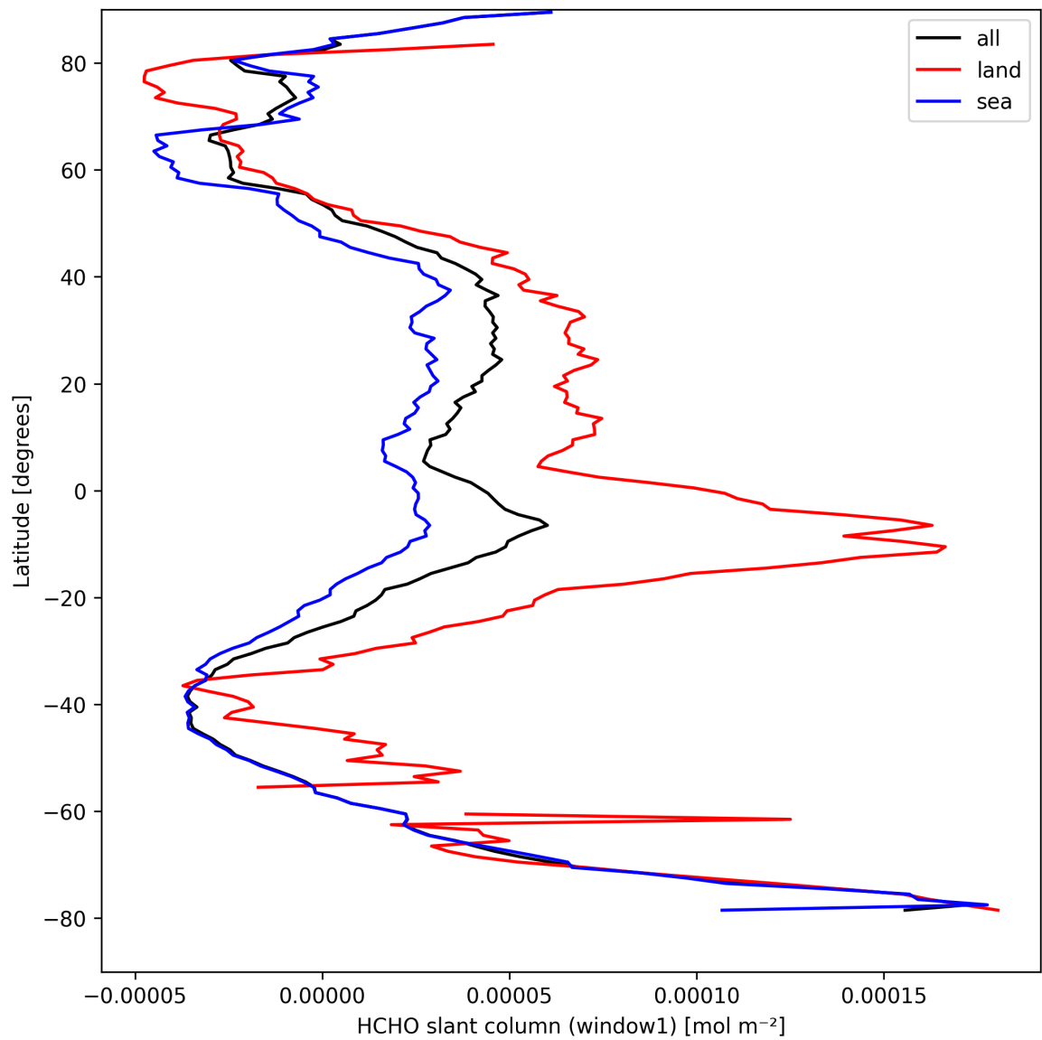
Figure 22: Zonal average of “HCHO slant column (window1)” for 2025-09-04 to 2025-09-05.
