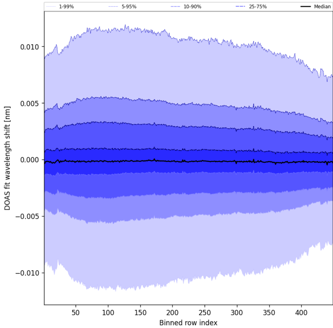
Figure 56: Along track statistics of “DOAS fit wavelength shift” for 2025-09-04 to 2025-09-05
