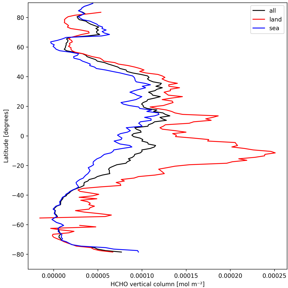
Figure 19: Zonal average of “HCHO vertical column” for 2025-09-04 to 2025-09-05.
