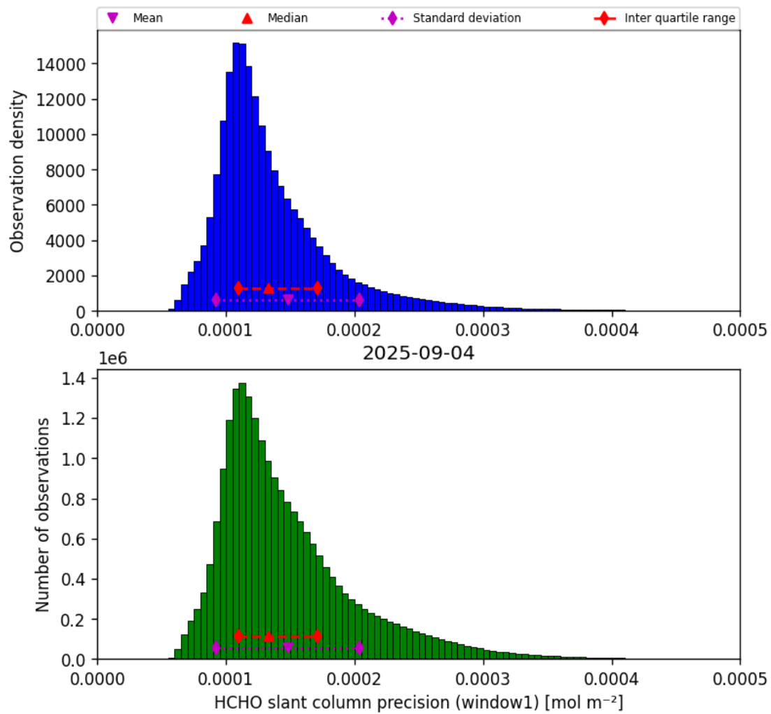
Figure 37: Histogram of “HCHO slant column precision (window1)” for 2025-09-04 to 2025-09-05
