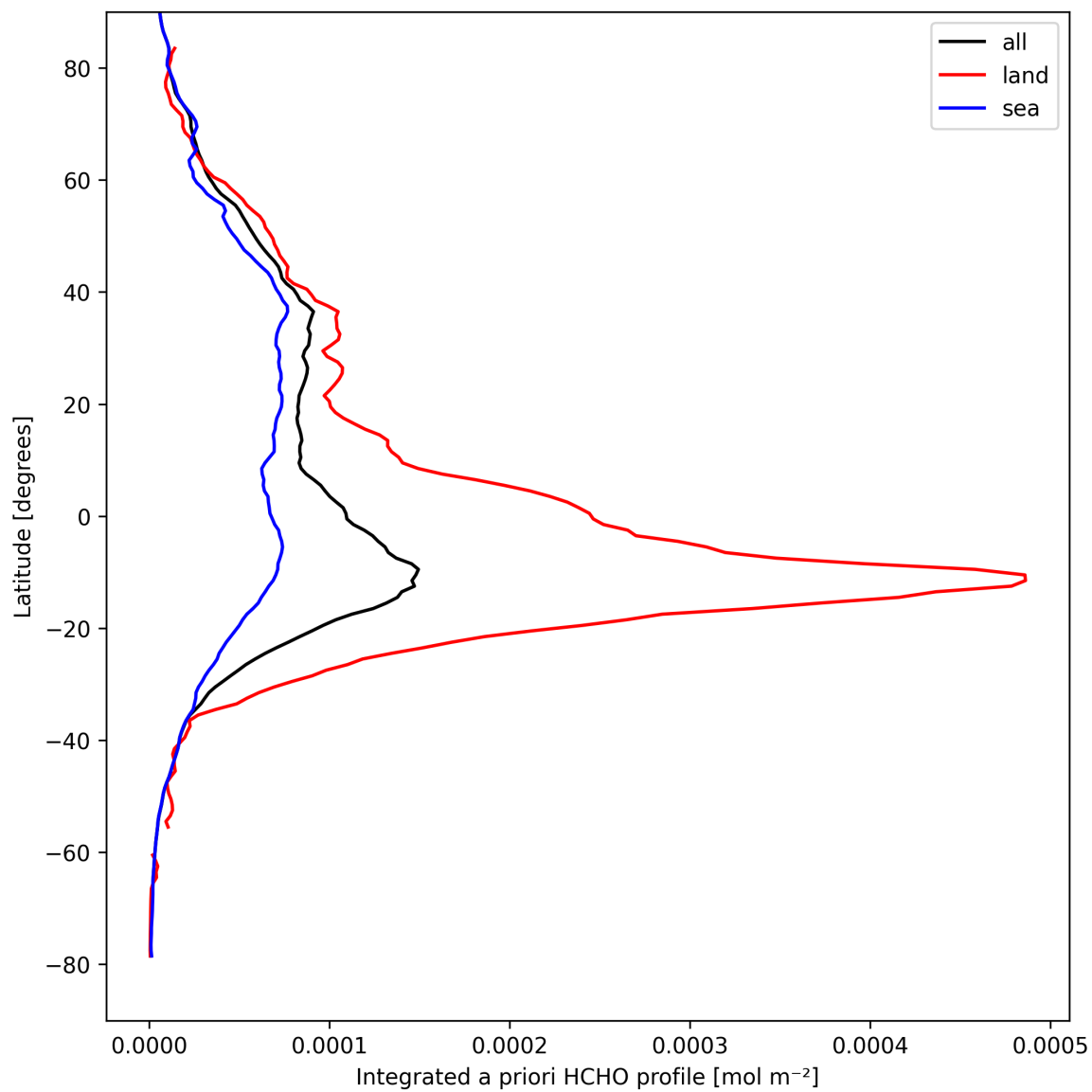
Figure 27: Zonal average of “Integrated a priori HCHO profile” for 2025-09-04 to 2025-09-05.
