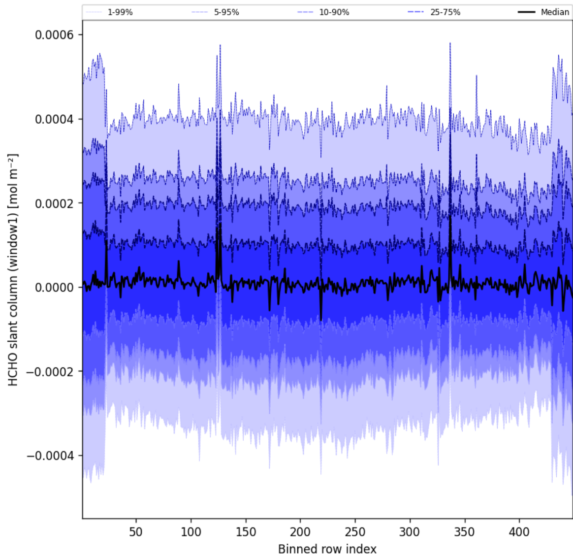
Figure 50: Along track statistics of “HCHO slant column (window1)” for 2025-09-04 to 2025-09-05
