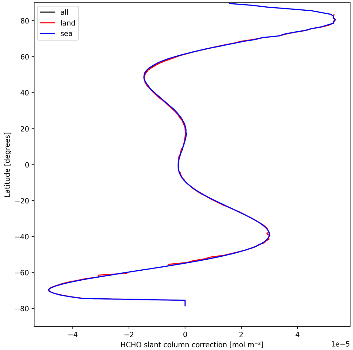
Figure 31: Zonal average of “HCHO slant column correction” for 2025-09-04 to 2025-09-05.
