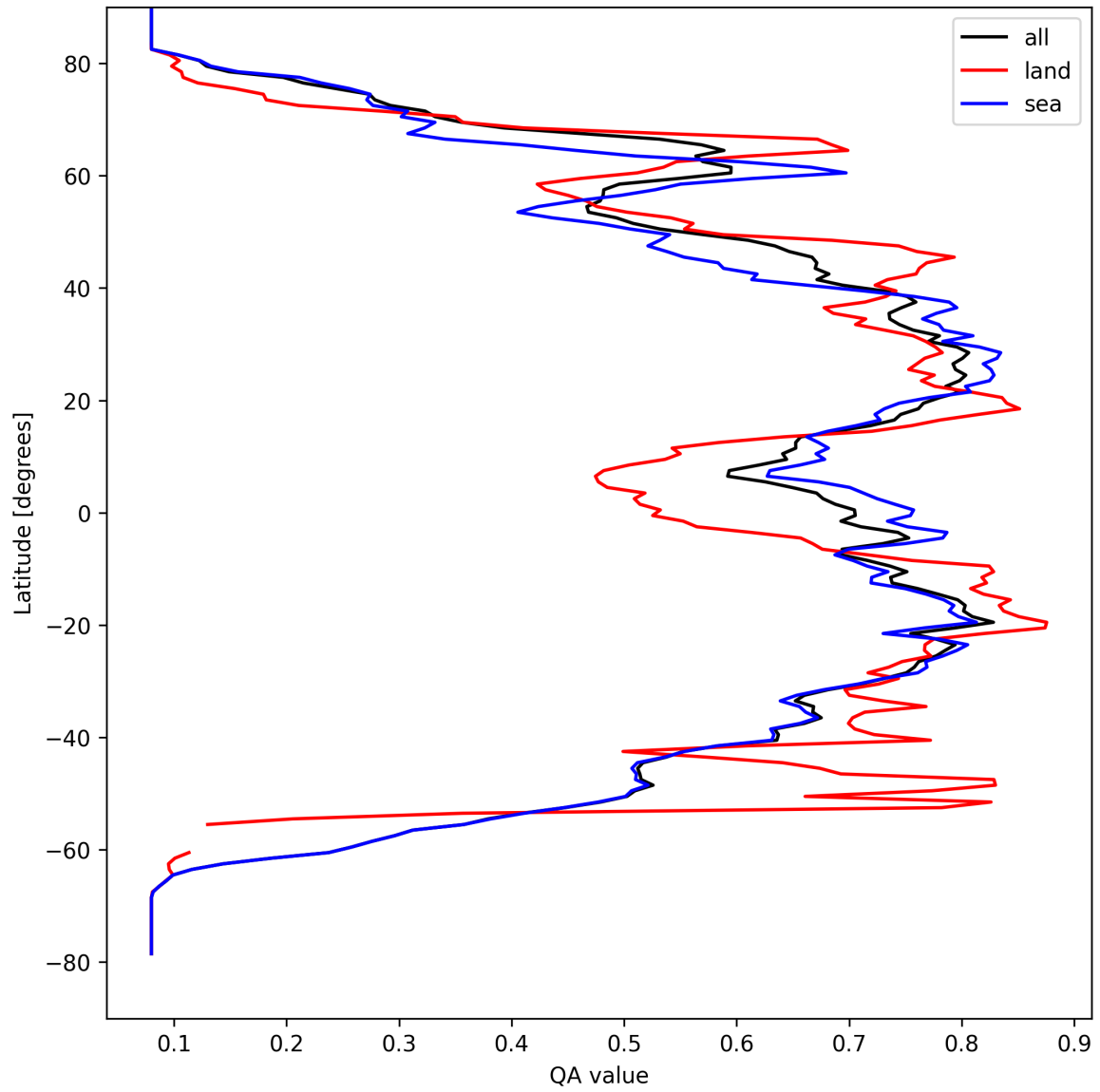
Figure 18: Zonal average of “QA value” for 2025-09-04 to 2025-09-05.
