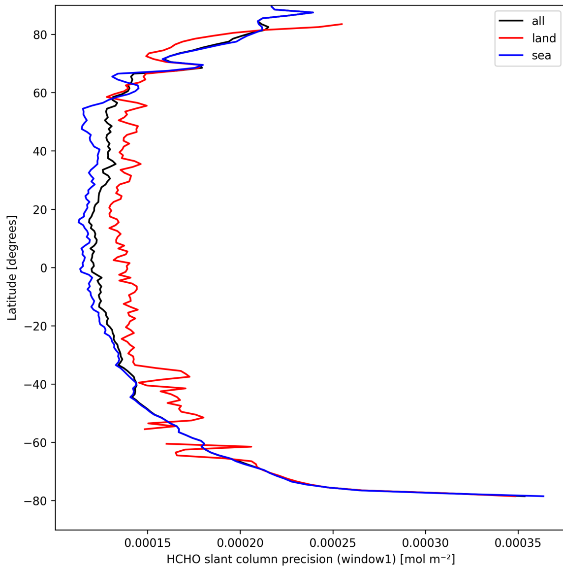
Figure 23: Zonal average of “HCHO slant column precision (window1)” for 2025-09-04 to 2025-09-05.
