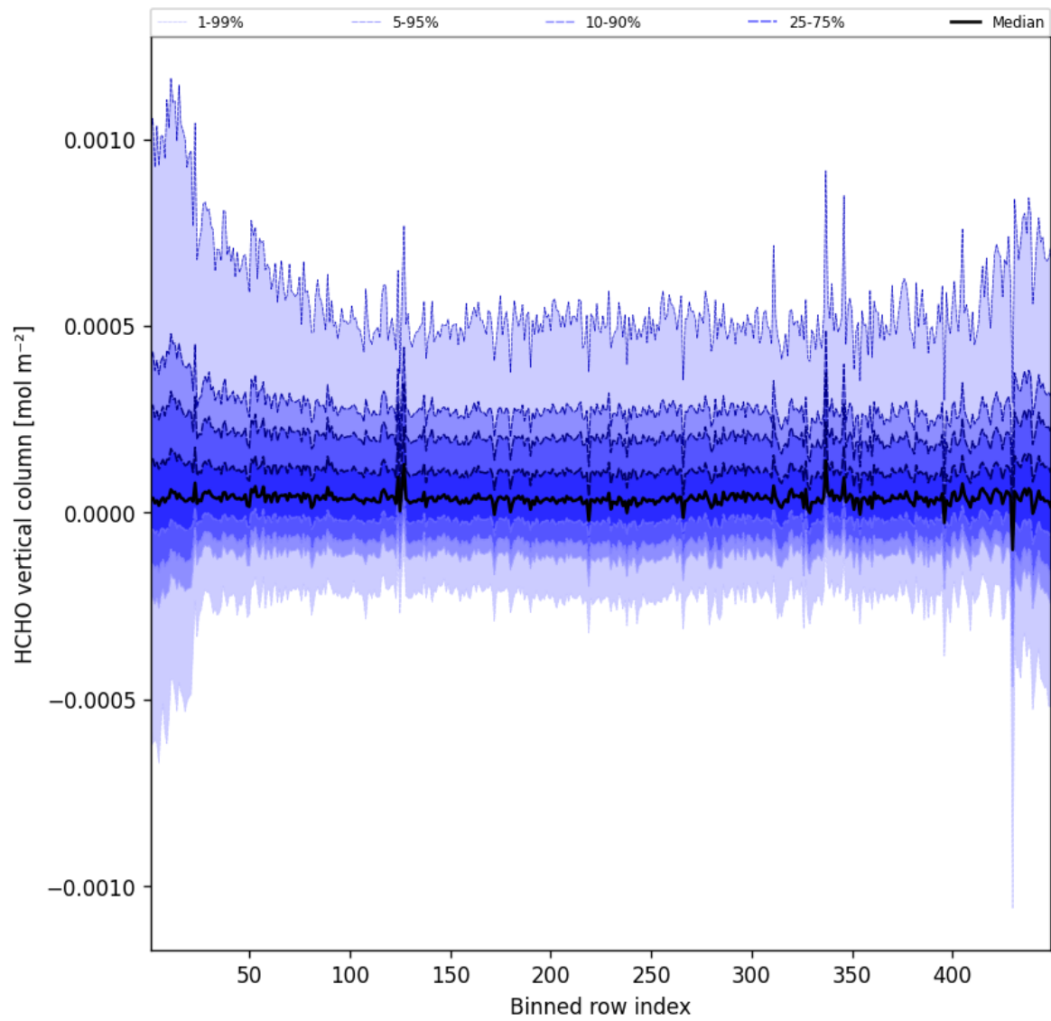
Figure 47: Along track statistics of “HCHO vertical column” for 2025-09-04 to 2025-09-05
