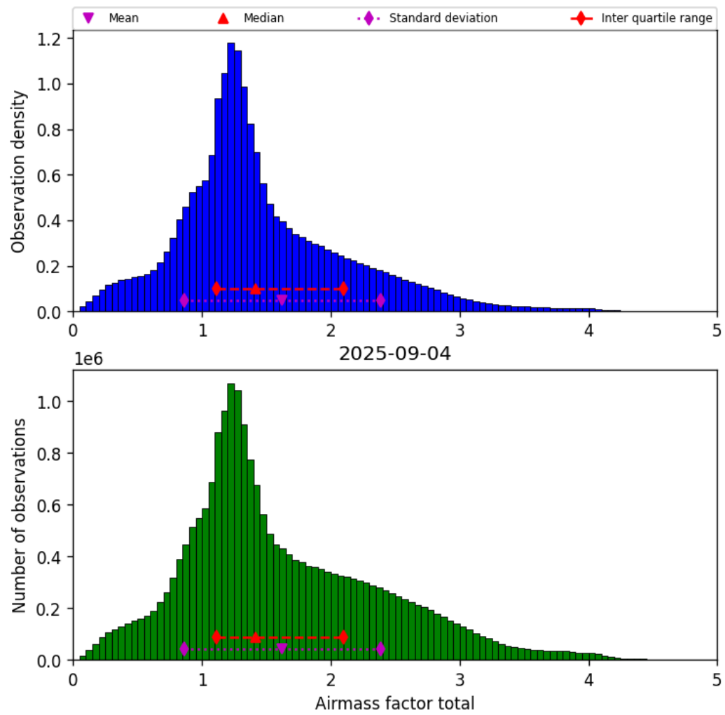
Figure 38: Histogram of “Airmass factor total” for 2025-09-04 to 2025-09-05
