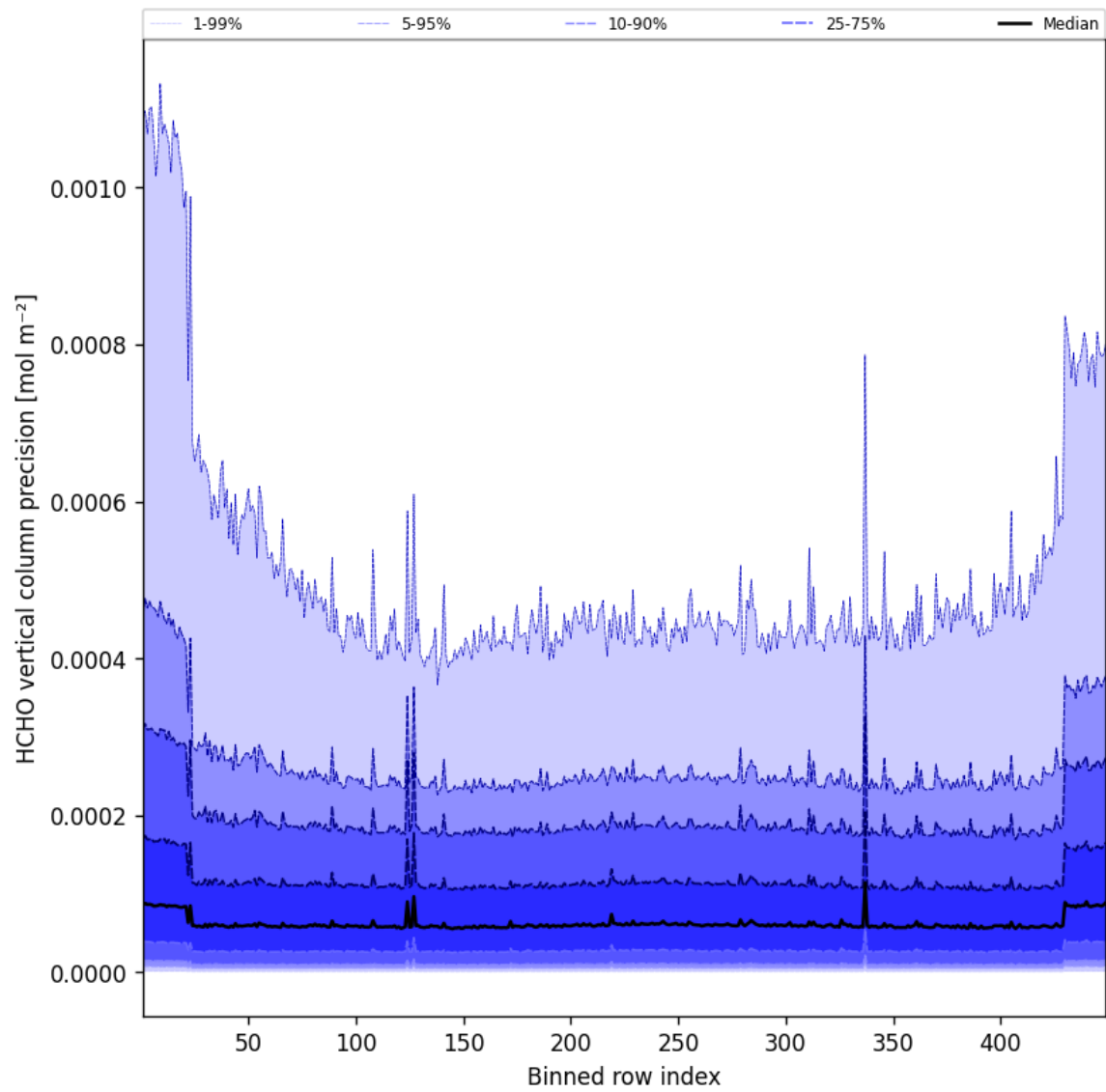
Figure 48: Along track statistics of “HCHO vertical column precision” for 2025-09-04 to 2025-09-05
