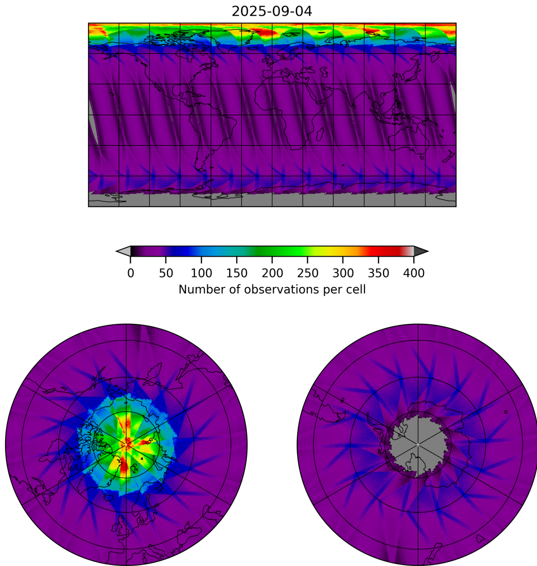
Figure 17: Map of the number of observations for 2025-09-04 to 2025-09-05
