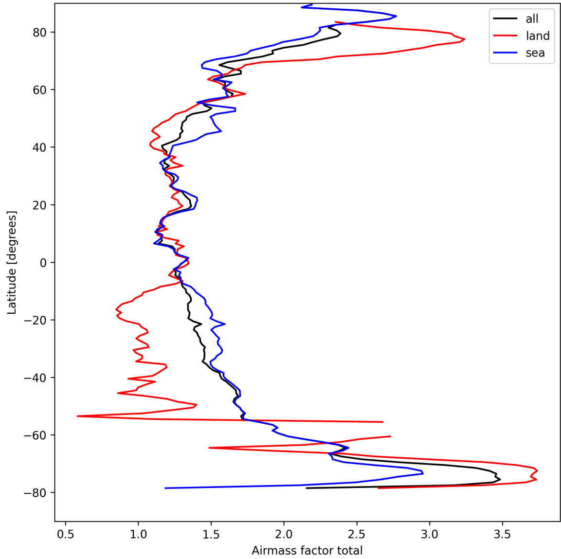
Figure 24: Zonal average of “Airmass factor total” for 2025-09-04 to 2025-09-05.
