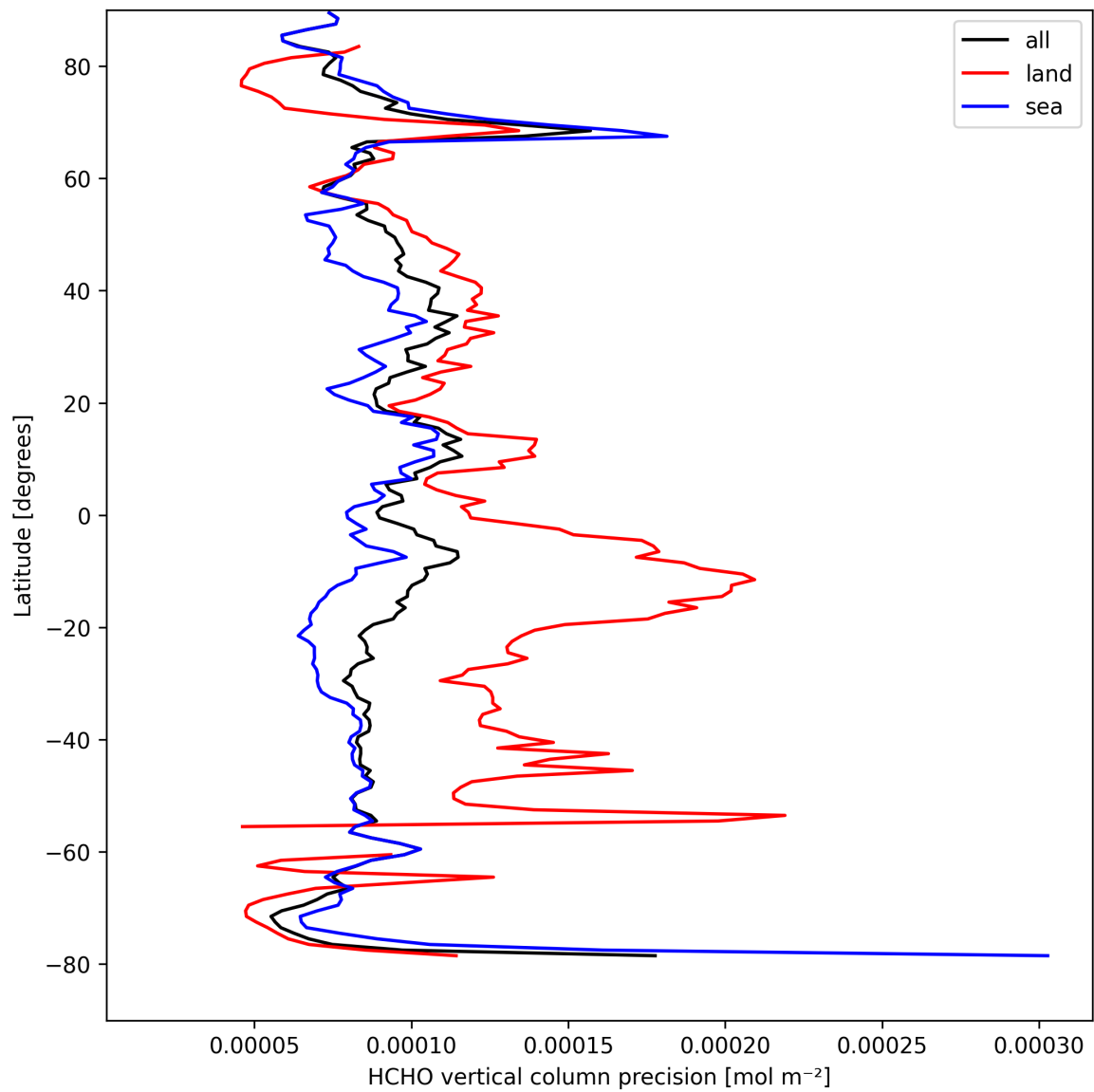
Figure 20: Zonal average of “HCHO vertical column precision” for 2025-09-04 to 2025-09-05.
