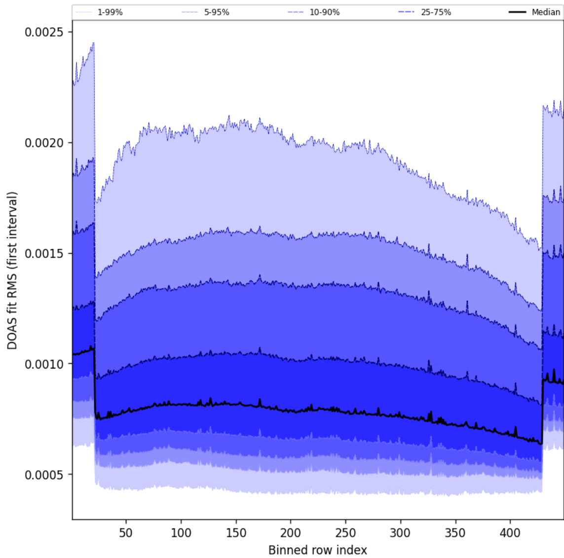
Figure 58: Along track statistics of “DOAS fit RMS (first interval)” for 2025-09-04 to 2025-09-05
