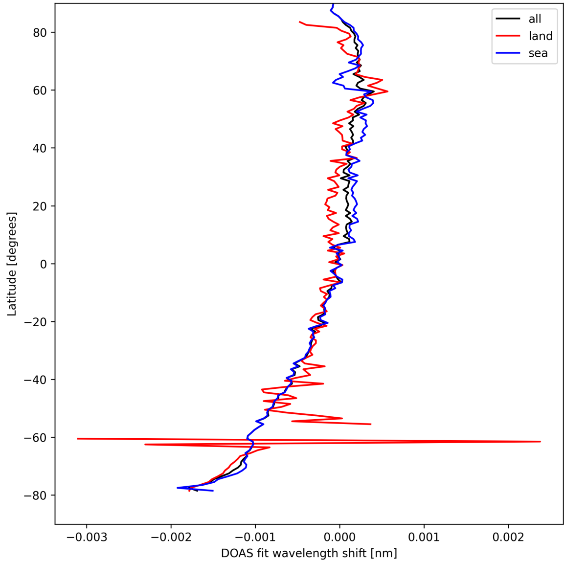
Figure 28: Zonal average of “DOAS fit wavelength shift” for 2025-09-04 to 2025-09-05.
