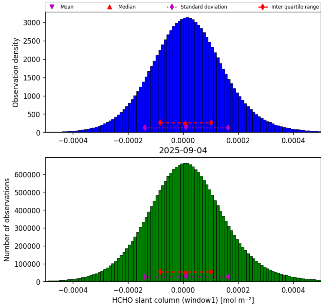
Figure 36: Histogram of “HCHO slant column (window1)” for 2025-09-04 to 2025-09-05
