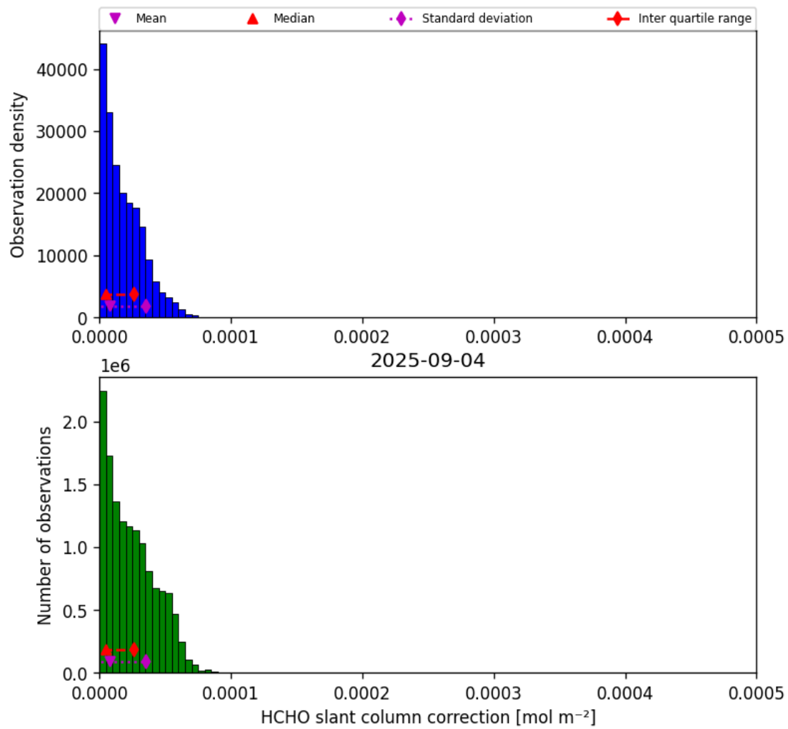
Figure 45: Histogram of “HCHO slant column correction” for 2025-09-04 to 2025-09-05
