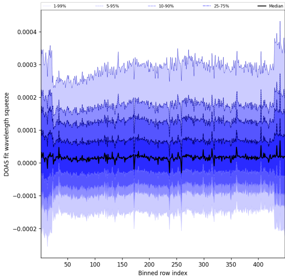
Figure 57: Along track statistics of “DOAS fit wavelength squeeze” for 2025-09-04 to 2025-09-05
