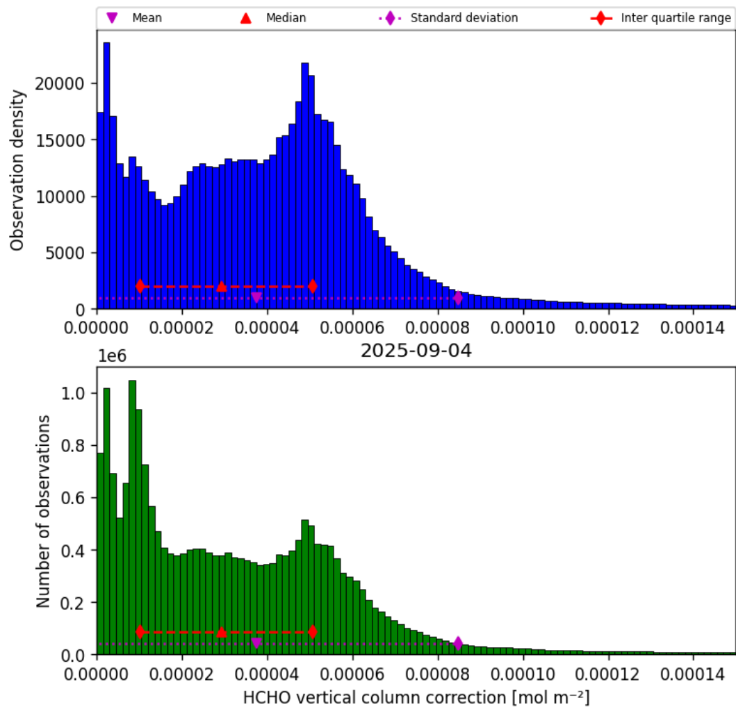
Figure 35: Histogram of “HCHO vertical column correction” for 2025-09-04 to 2025-09-05
