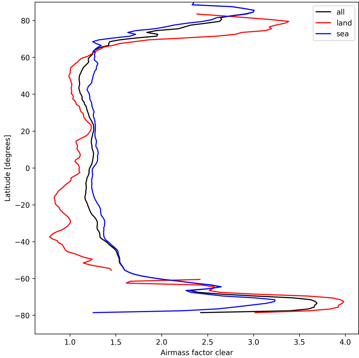
Figure 26: Zonal average of “Airmass factor clear” for 2025-09-04 to 2025-09-05.
