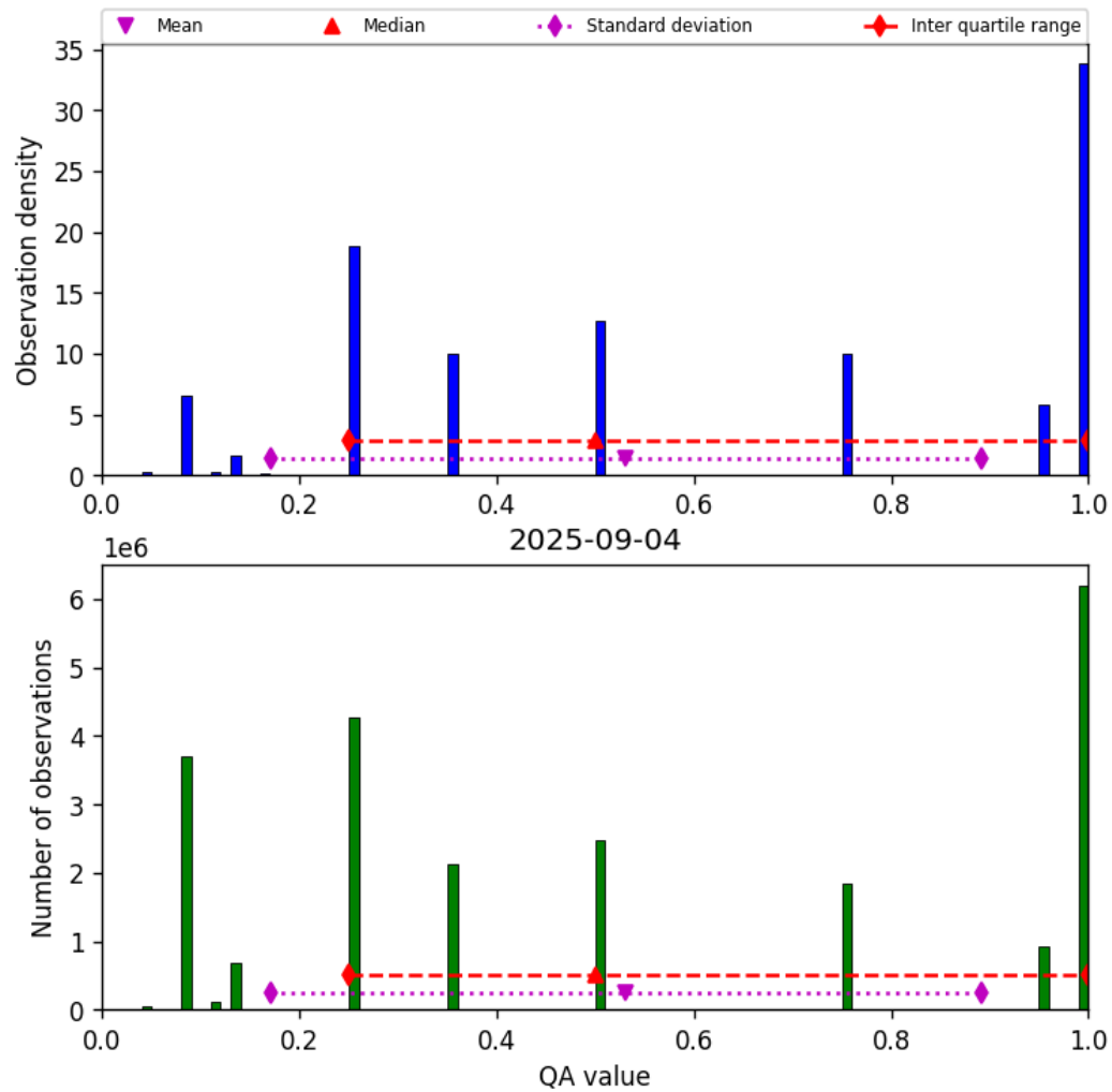
Figure 32: Histogram of “QA value” for 2025-09-04 to 2025-09-05
