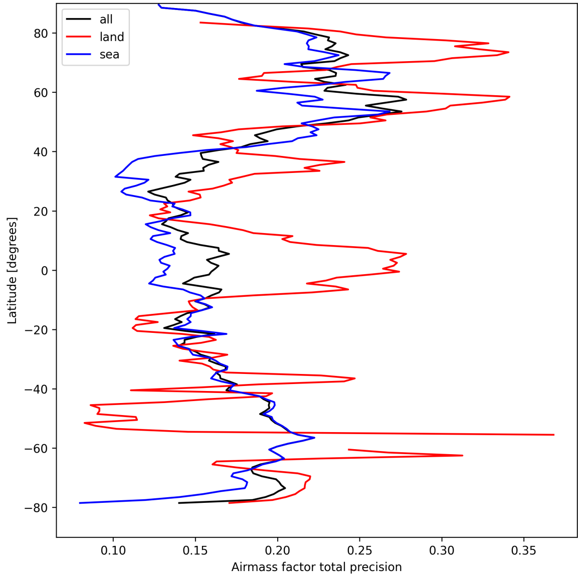
Figure 25: Zonal average of “Airmass factor total precision” for 2025-09-04 to 2025-09-05.
