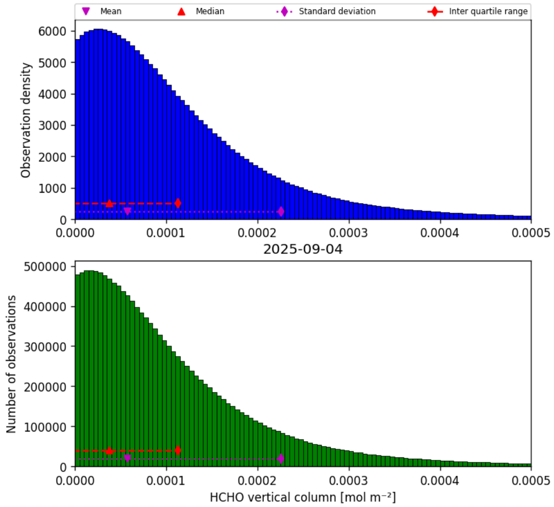
Figure 33: Histogram of “HCHO vertical column” for 2025-09-04 to 2025-09-05
