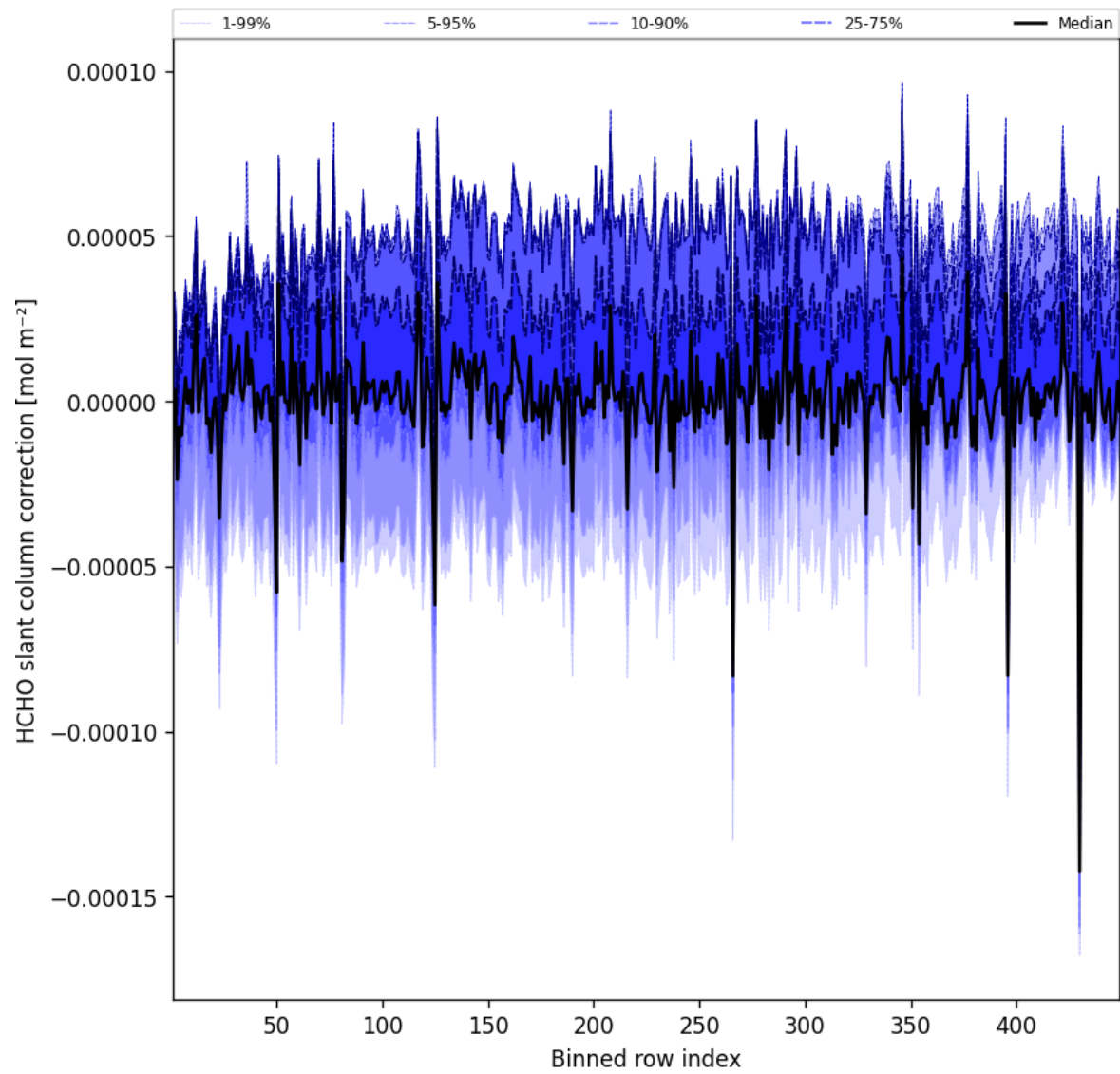
Figure 59: Along track statistics of “HCHO slant column correction” for 2025-09-04 to 2025-09-05
