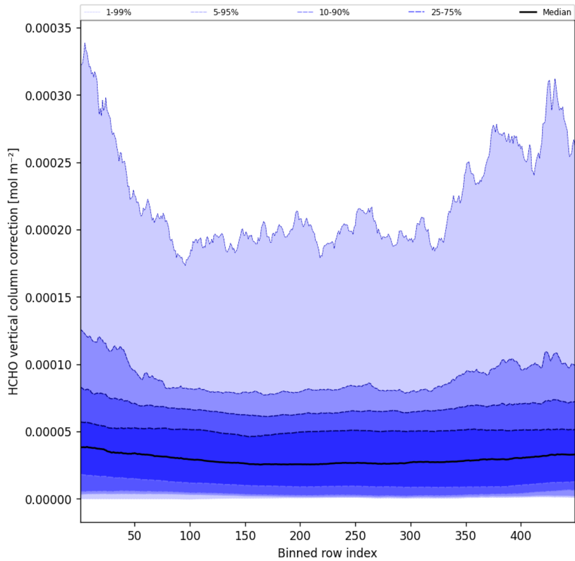
Figure 49: Along track statistics of “HCHO vertical column correction” for 2025-09-04 to 2025-09-05
