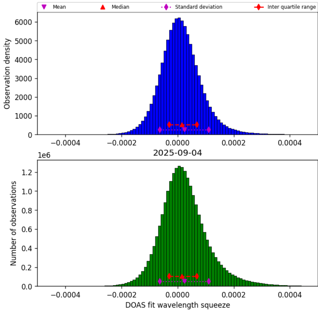
Figure 43: Histogram of “DOAS fit wavelength squeeze” for 2025-09-04 to 2025-09-05
