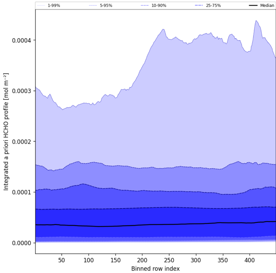
Figure 55: Along track statistics of “Integrated a priori HCHO profile” for 2025-09-04 to 2025-09-05
