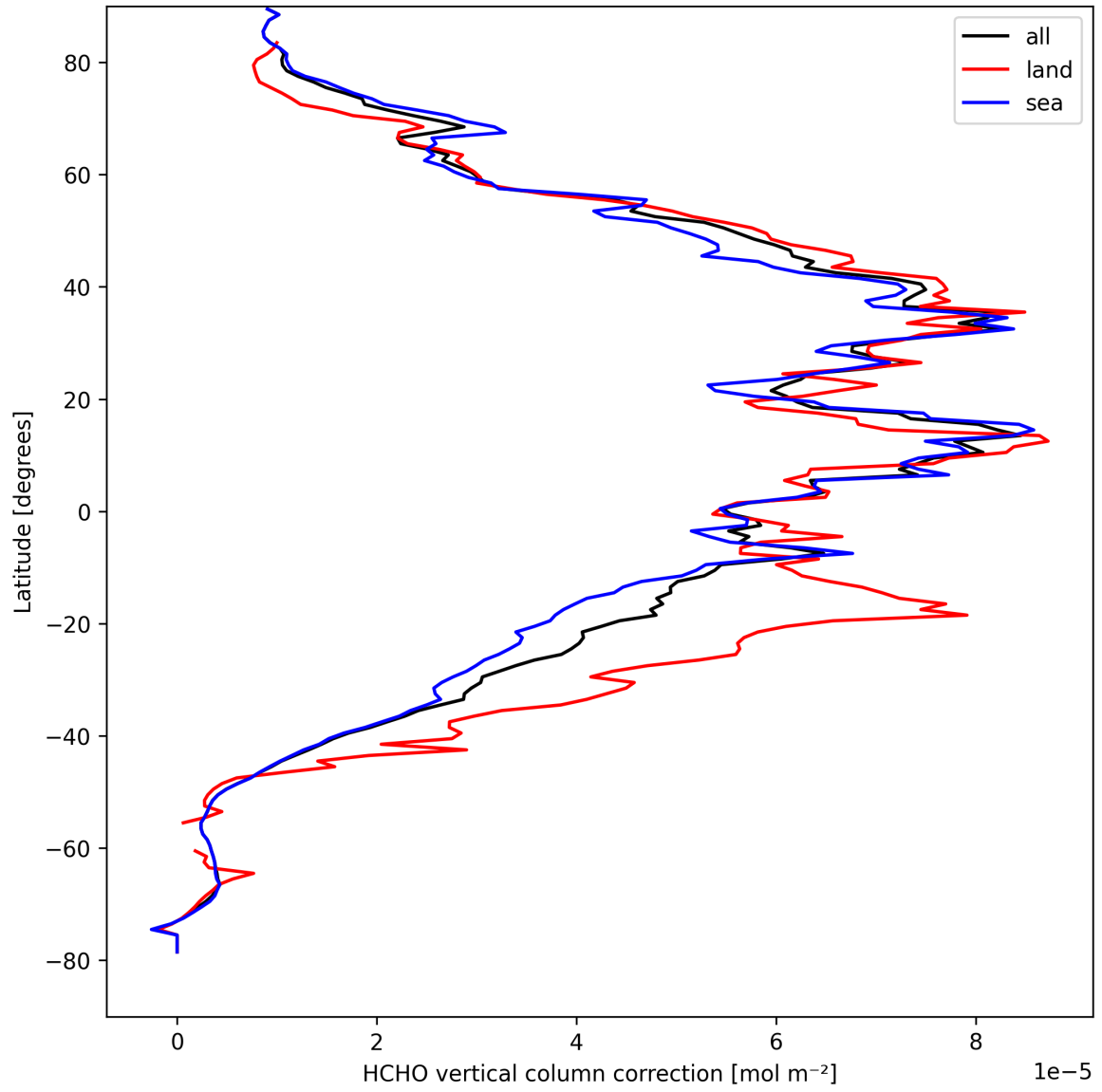
Figure 21: Zonal average of “HCHO vertical column correction” for 2025-09-04 to 2025-09-05.
