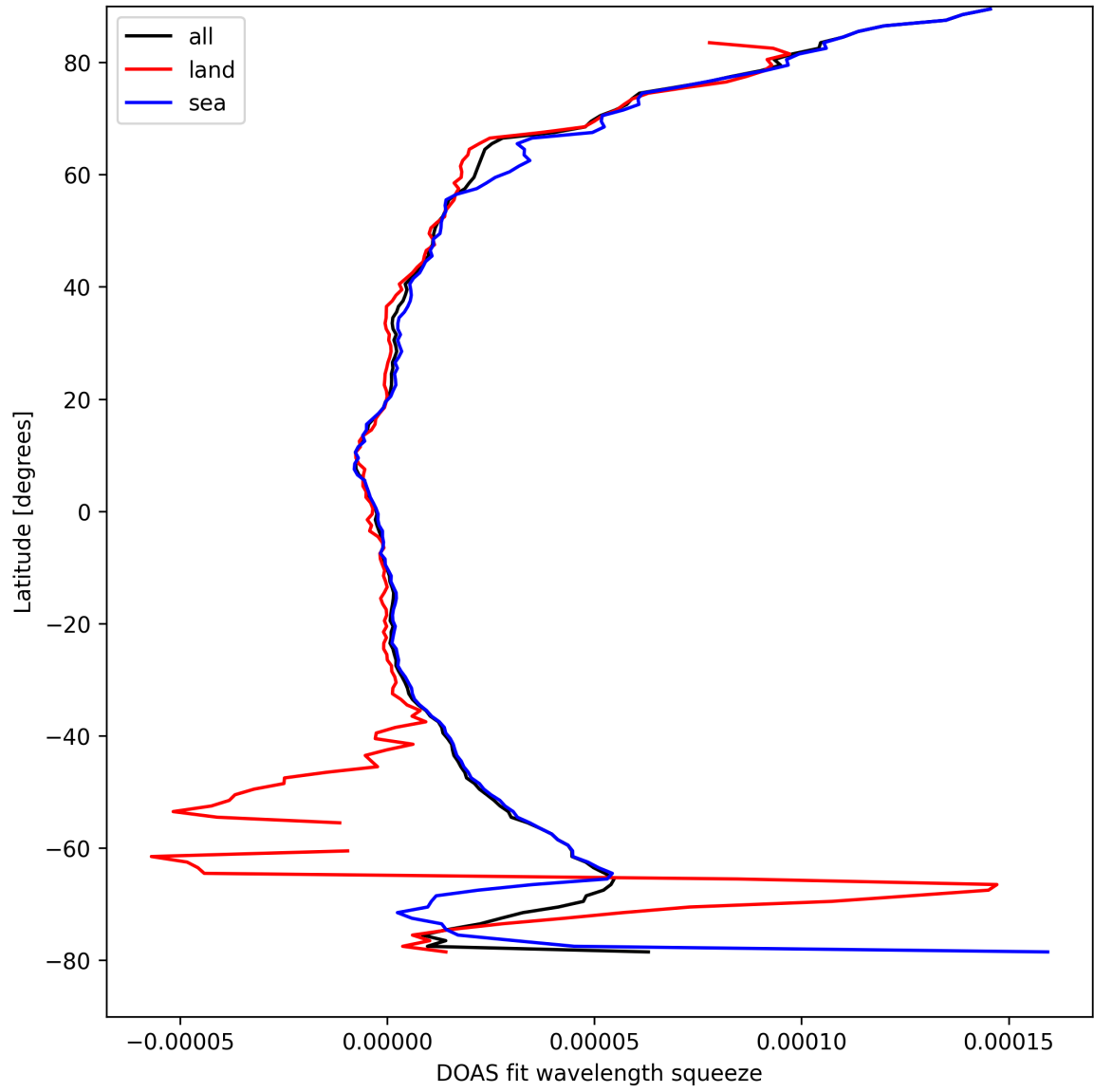
Figure 29: Zonal average of “DOAS fit wavelength squeeze” for 2025-09-04 to 2025-09-05.
