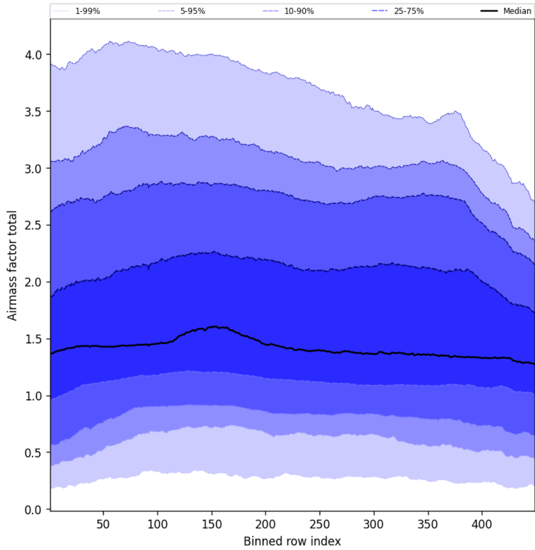
Figure 52: Along track statistics of “Airmass factor total” for 2025-09-04 to 2025-09-05
