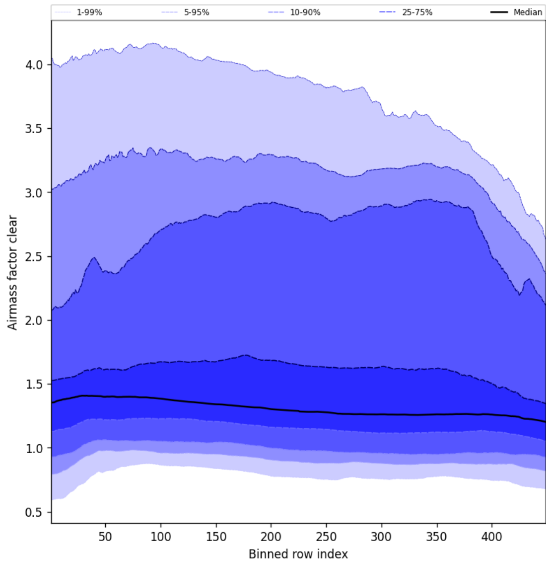
Figure 54: Along track statistics of “Airmass factor clear” for 2025-09-04 to 2025-09-05
