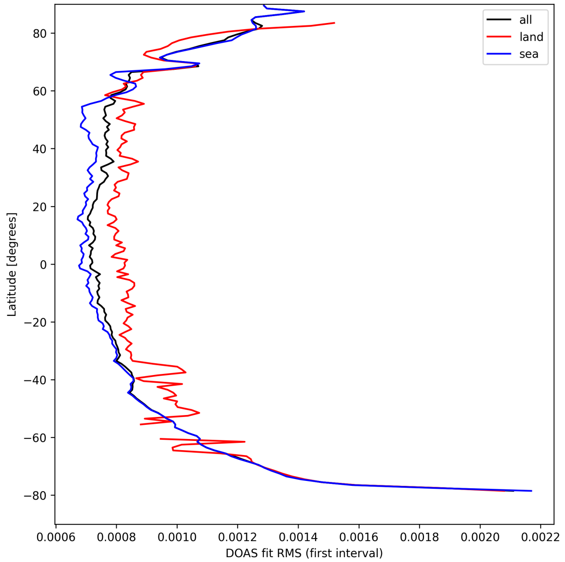
Figure 30: Zonal average of “DOAS fit RMS (first interval)” for 2025-09-04 to 2025-09-05.
