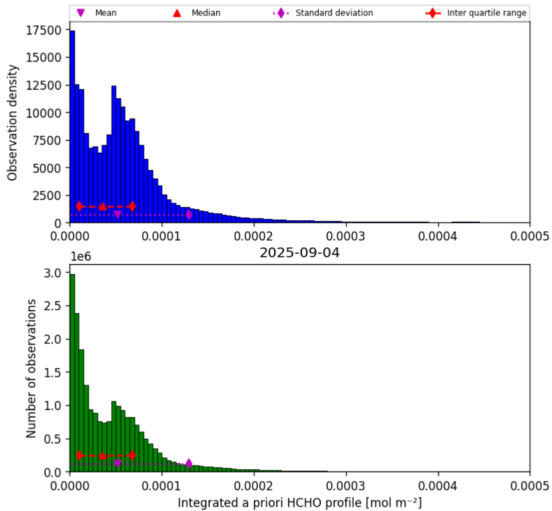
Figure 41: Histogram of “Integrated a priori HCHO profile” for 2025-09-04 to 2025-09-05
