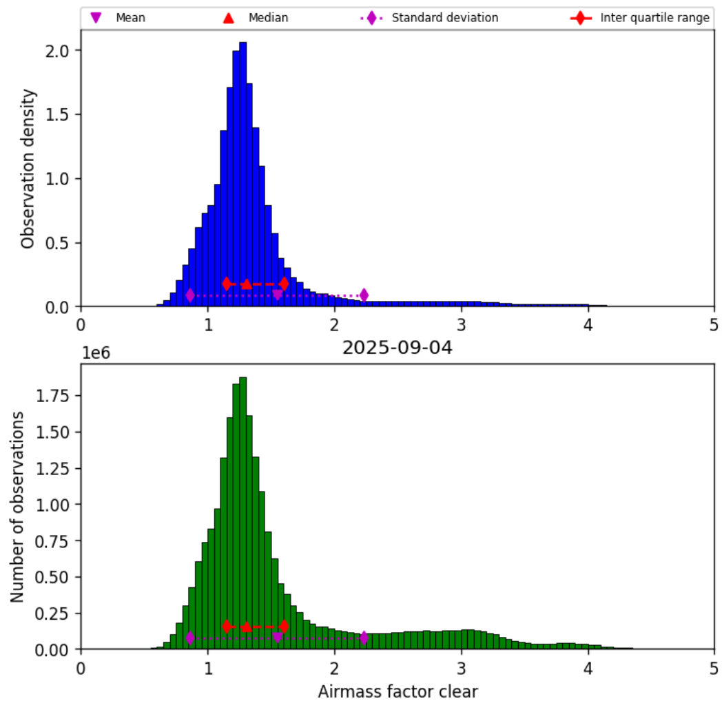
Figure 40: Histogram of “Airmass factor clear” for 2025-09-04 to 2025-09-05
