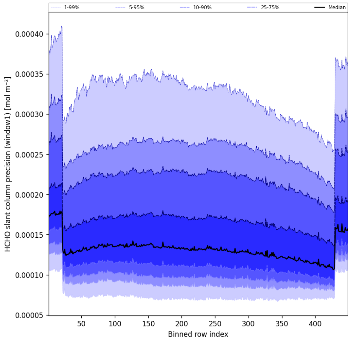
Figure 51: Along track statistics of “HCHO slant column precision (window1)” for 2025-09-04 to 2025-09-05
