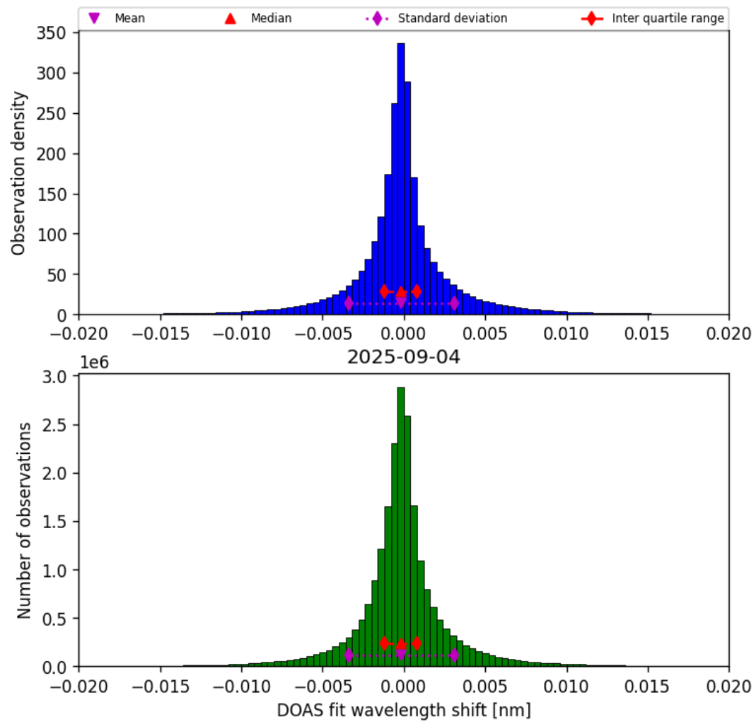
Figure 42: Histogram of “DOAS fit wavelength shift” for 2025-09-04 to 2025-09-05
