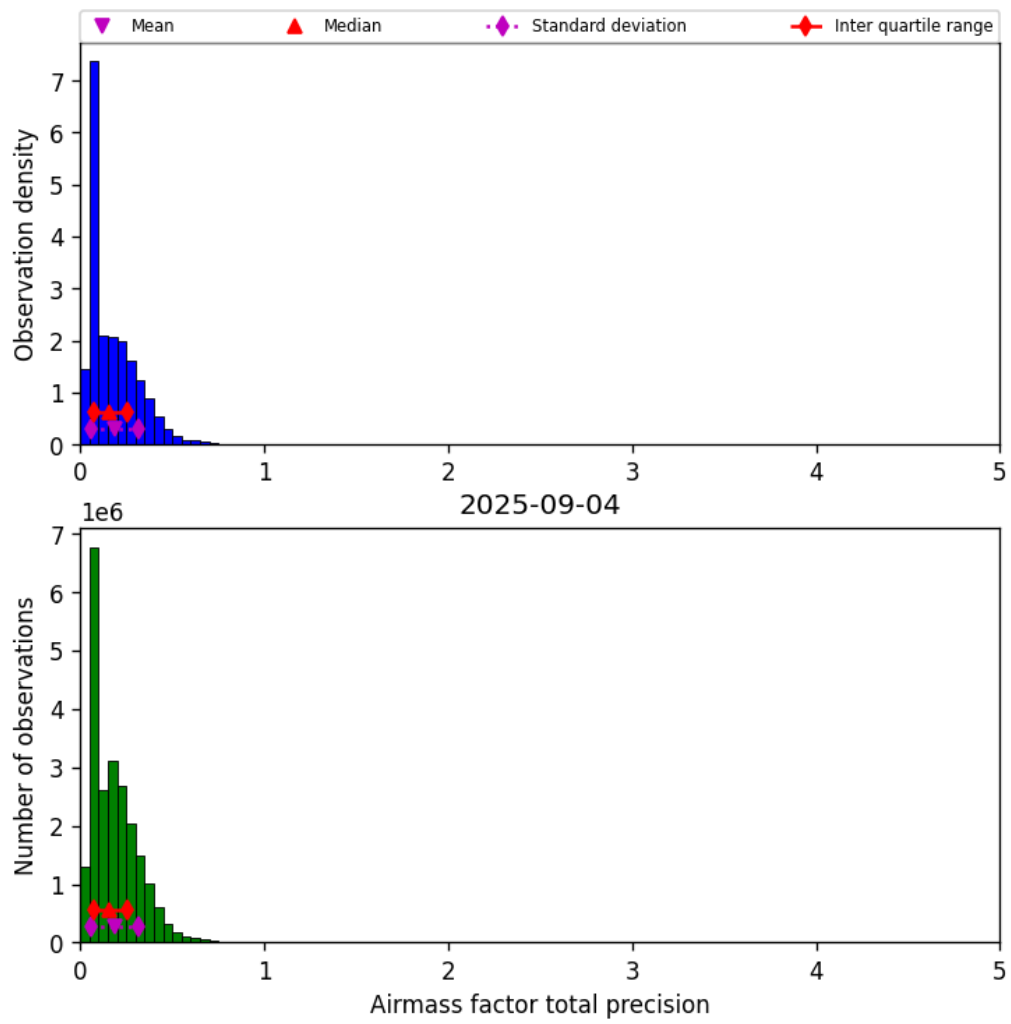
Figure 39: Histogram of “Airmass factor total precision” for 2025-09-04 to 2025-09-05
