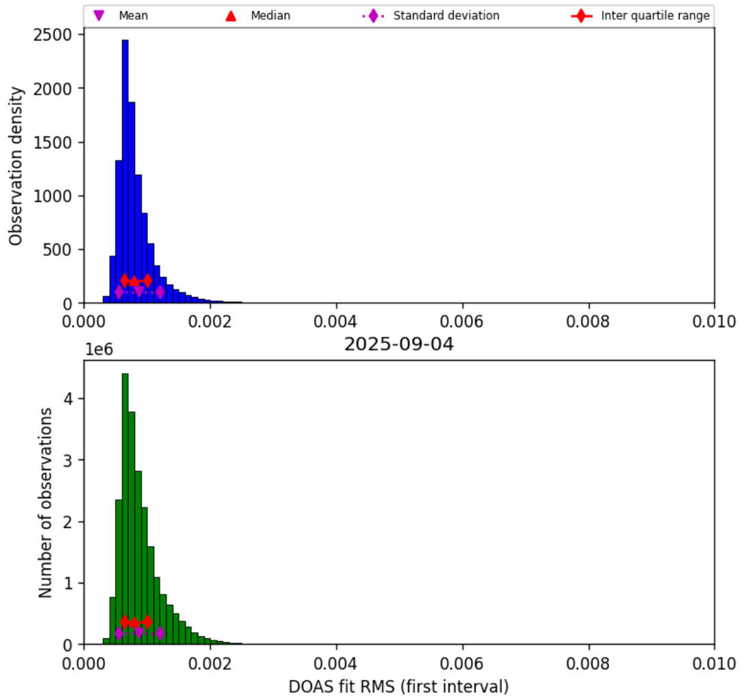
Figure 44: Histogram of “DOAS fit RMS (first interval)” for 2025-09-04 to 2025-09-05
