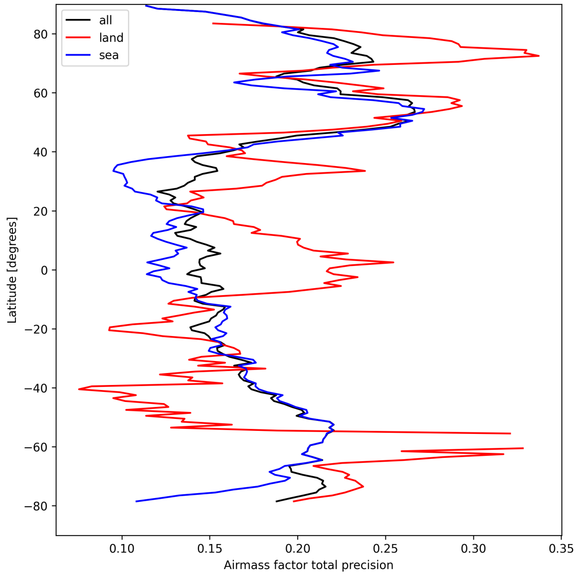
Figure 25: Zonal average of “Airmass factor total precision” for 2025-09-05 to 2025-09-06.
