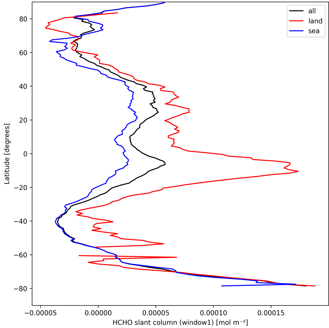
Figure 22: Zonal average of “HCHO slant column (window1)” for 2025-09-05 to 2025-09-06.
