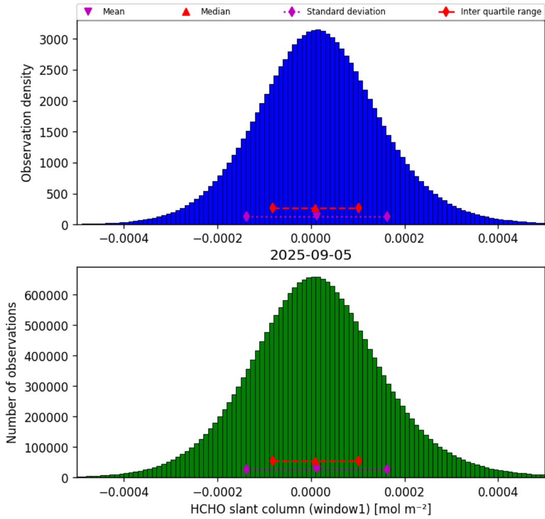
Figure 36: Histogram of “HCHO slant column (window1)” for 2025-09-05 to 2025-09-06
