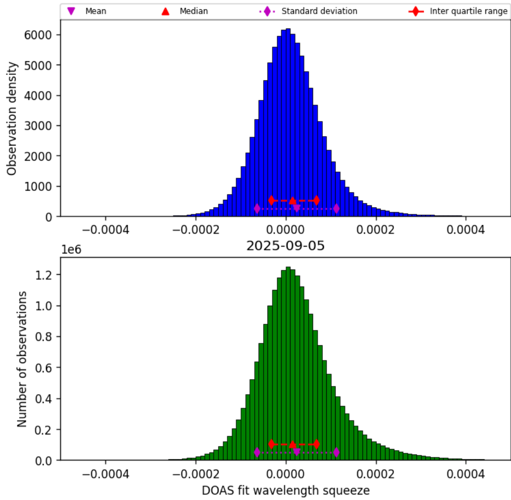
Figure 43: Histogram of “DOAS fit wavelength squeeze” for 2025-09-05 to 2025-09-06
