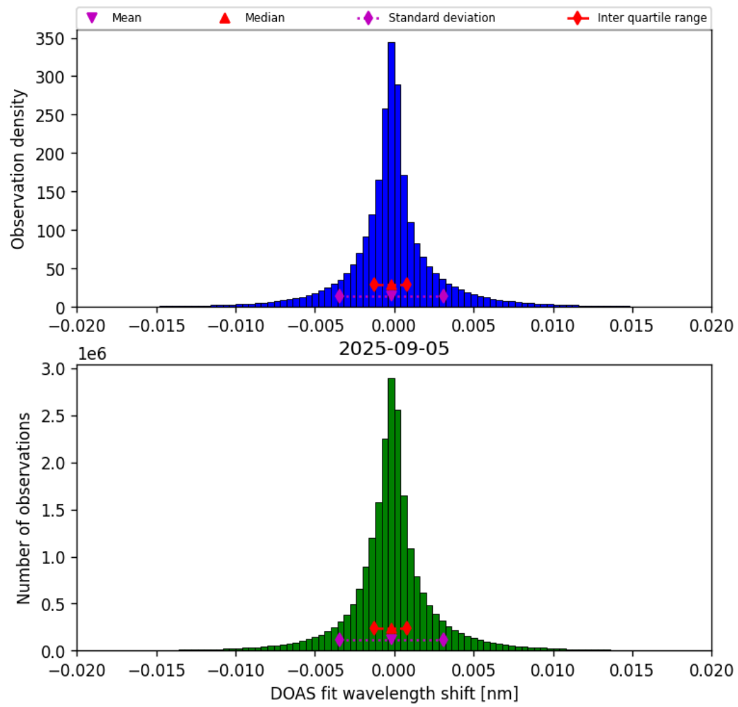
Figure 42: Histogram of “DOAS fit wavelength shift” for 2025-09-05 to 2025-09-06
