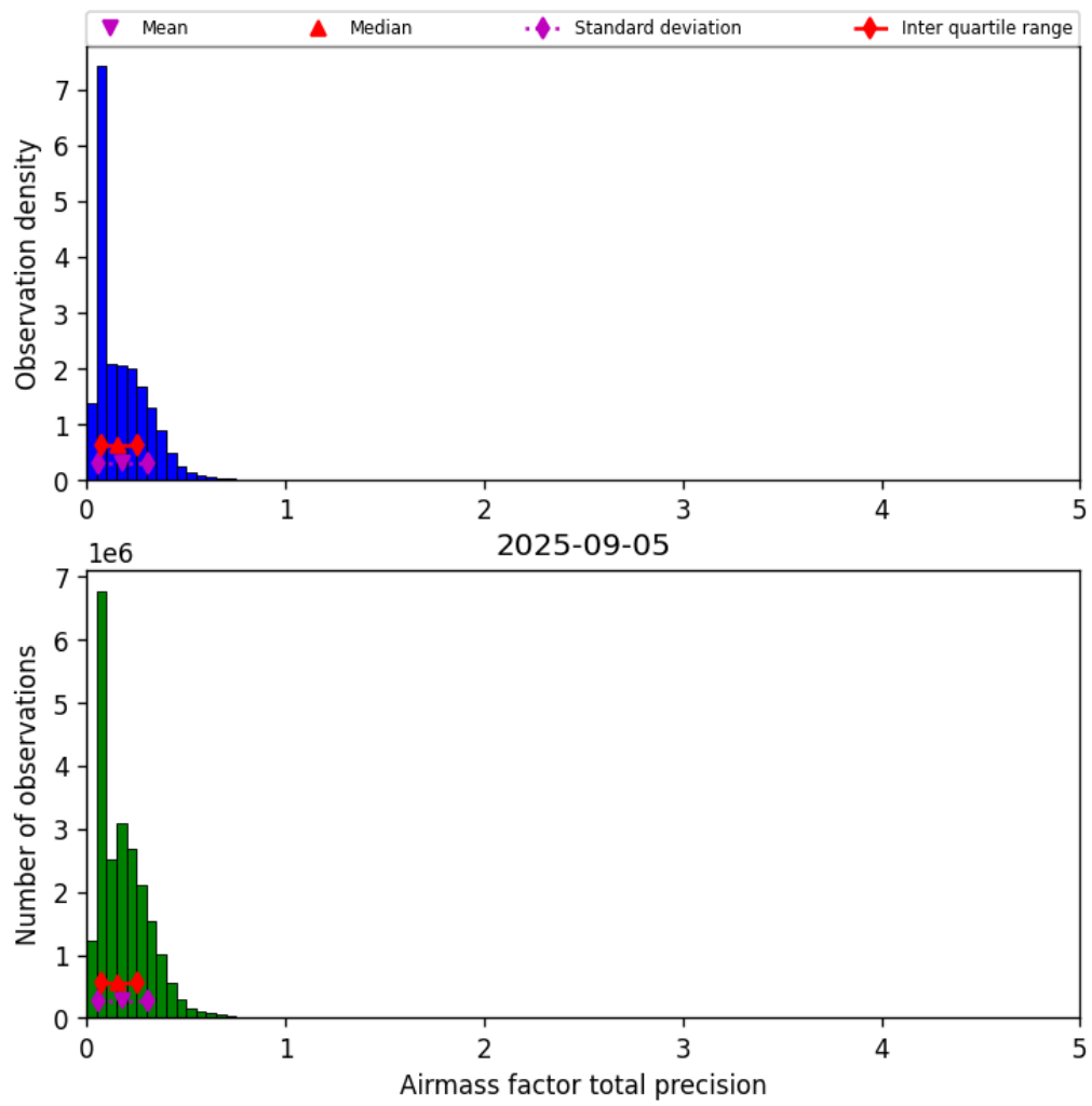
Figure 39: Histogram of “Airmass factor total precision” for 2025-09-05 to 2025-09-06
