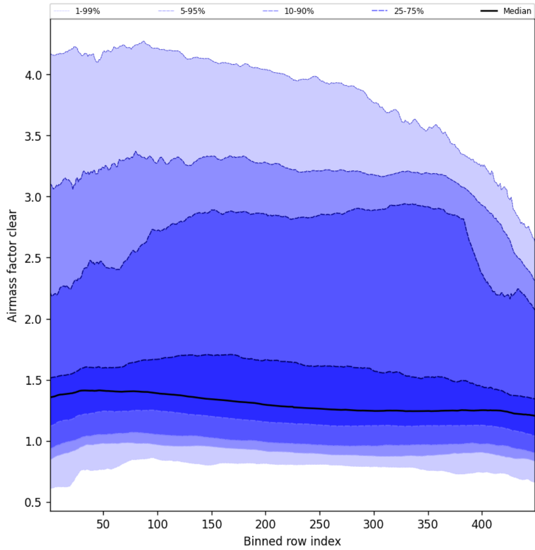
Figure 54: Along track statistics of “Airmass factor clear” for 2025-09-05 to 2025-09-06
