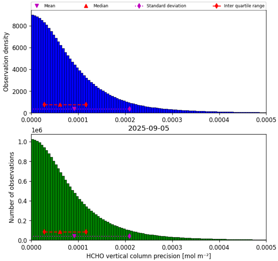
Figure 34: Histogram of “HCHO vertical column precision” for 2025-09-05 to 2025-09-06
