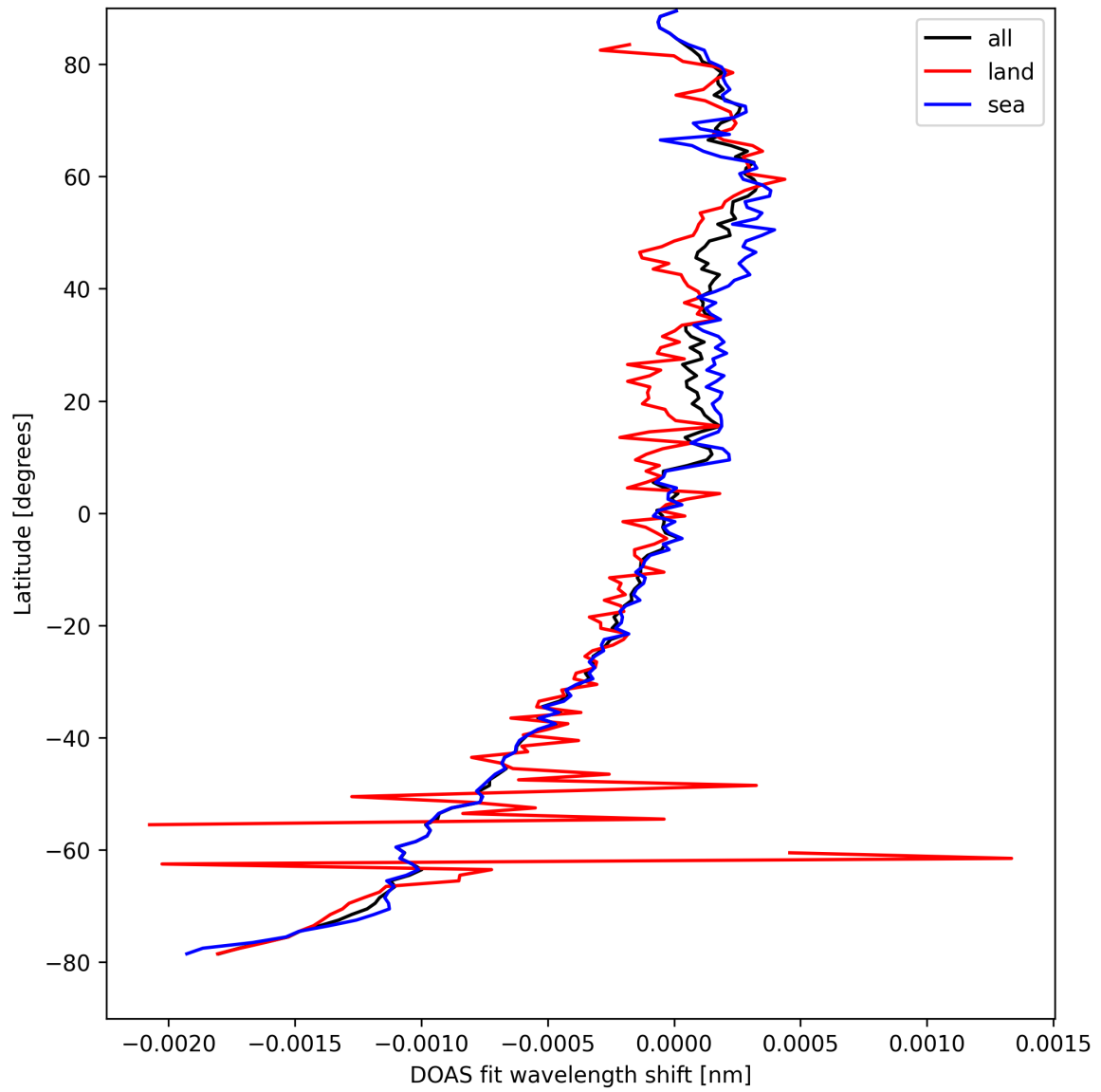
Figure 28: Zonal average of “DOAS fit wavelength shift” for 2025-09-05 to 2025-09-06.
