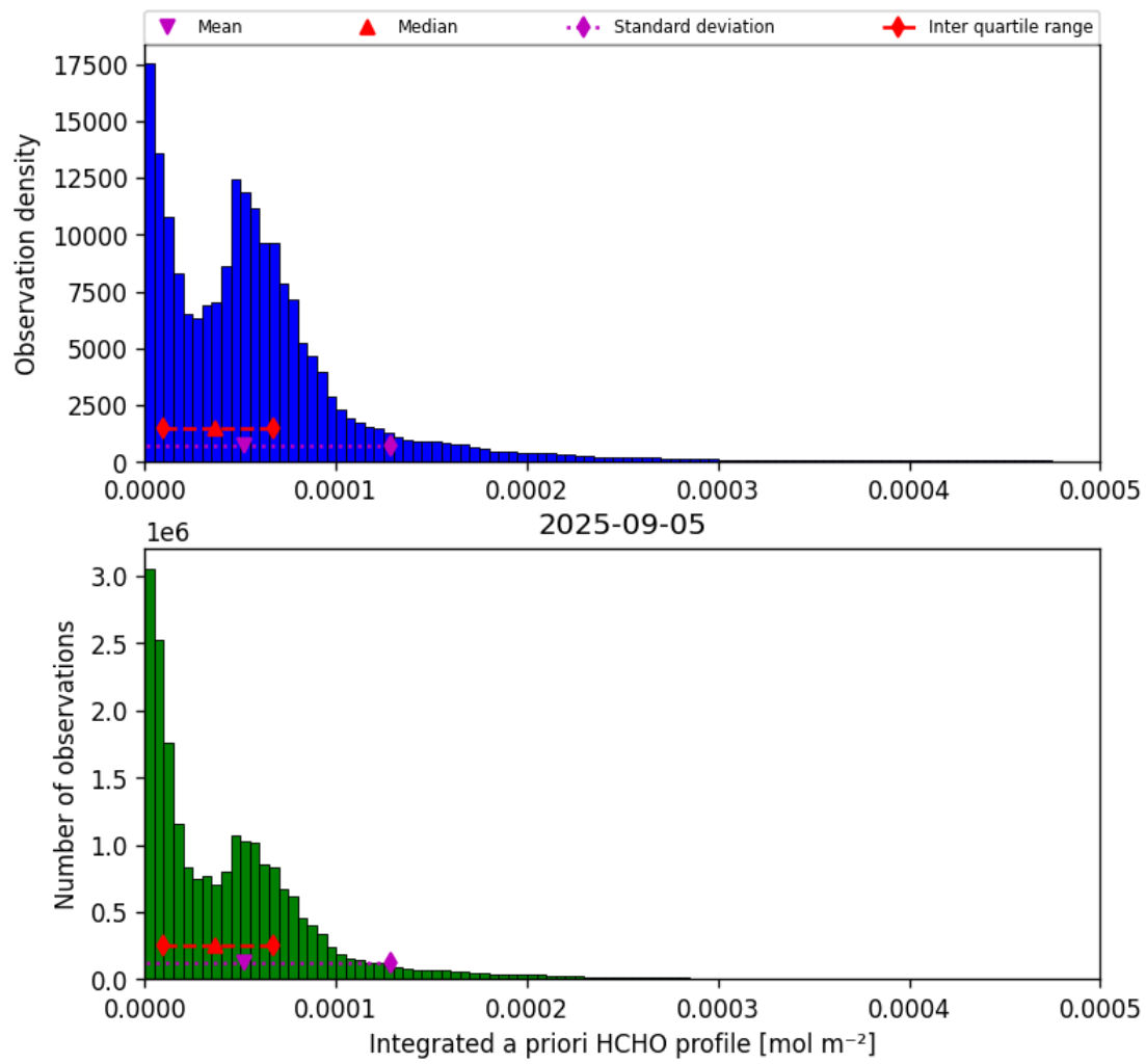
Figure 41: Histogram of “Integrated a priori HCHO profile” for 2025-09-05 to 2025-09-06
