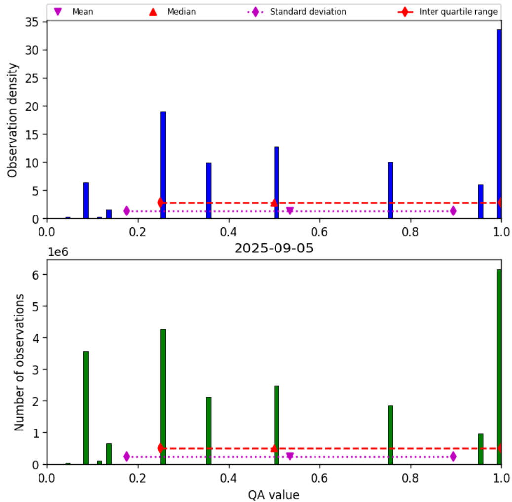
Figure 32: Histogram of “QA value” for 2025-09-05 to 2025-09-06
