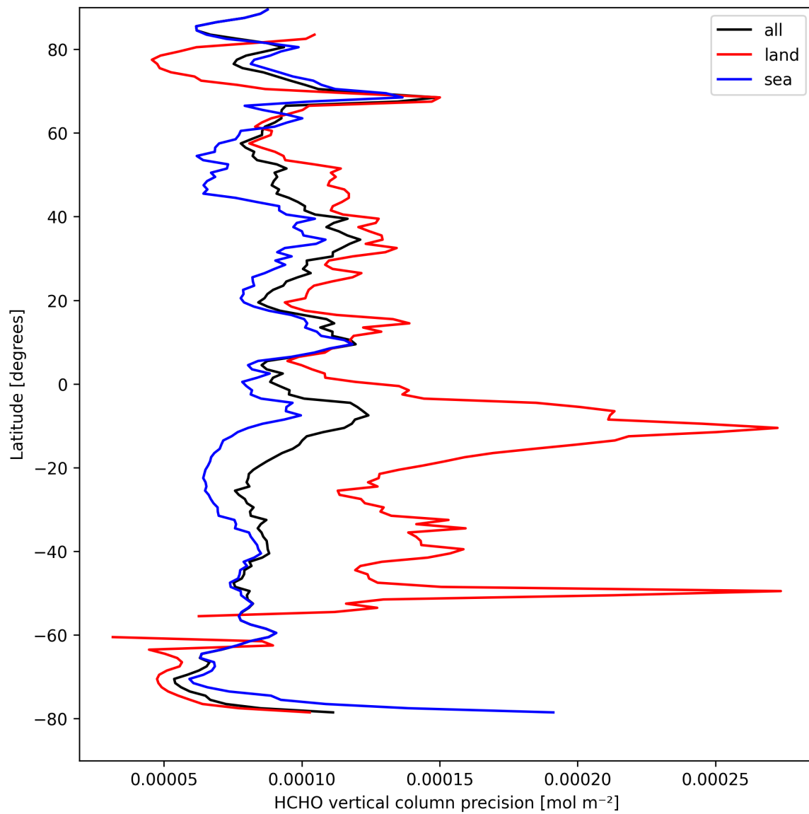
Figure 20: Zonal average of “HCHO vertical column precision” for 2025-09-05 to 2025-09-06.
