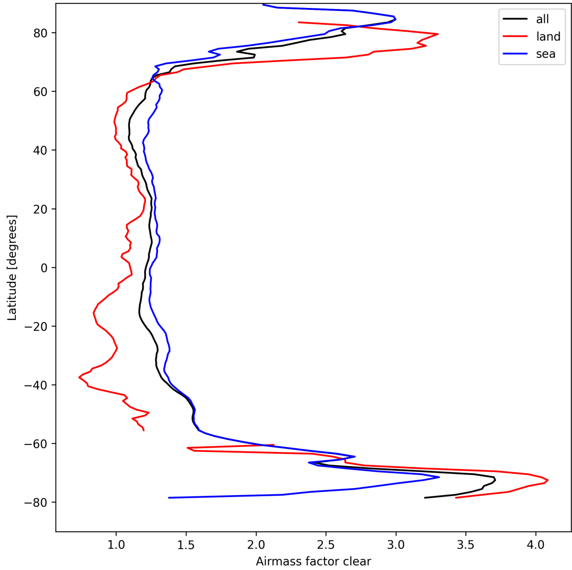
Figure 26: Zonal average of “Airmass factor clear” for 2025-09-05 to 2025-09-06.
