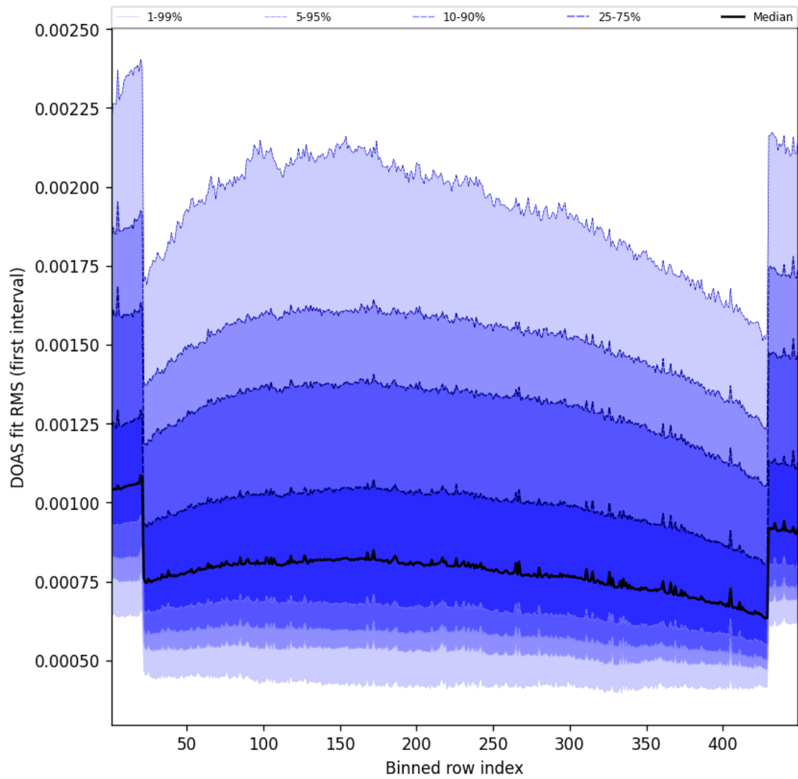
Figure 58: Along track statistics of “DOAS fit RMS (first interval)” for 2025-09-05 to 2025-09-06
