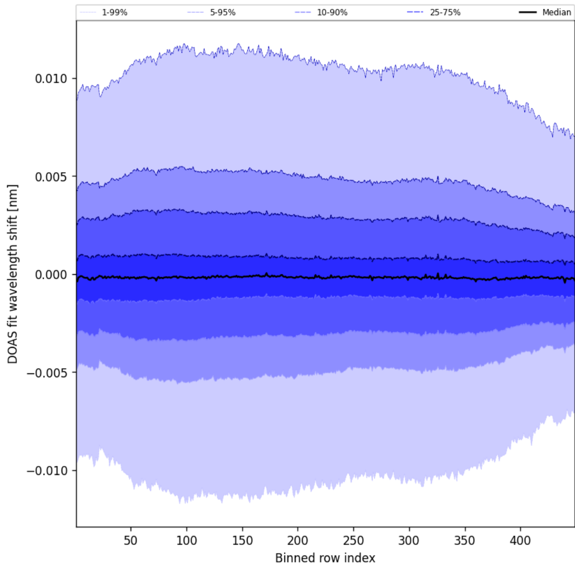
Figure 56: Along track statistics of “DOAS fit wavelength shift” for 2025-09-05 to 2025-09-06
