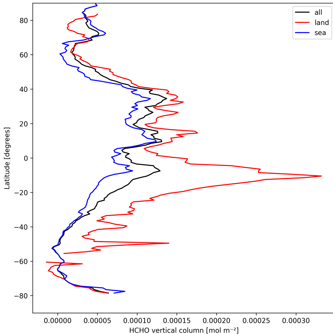
Figure 19: Zonal average of “HCHO vertical column” for 2025-09-05 to 2025-09-06.
