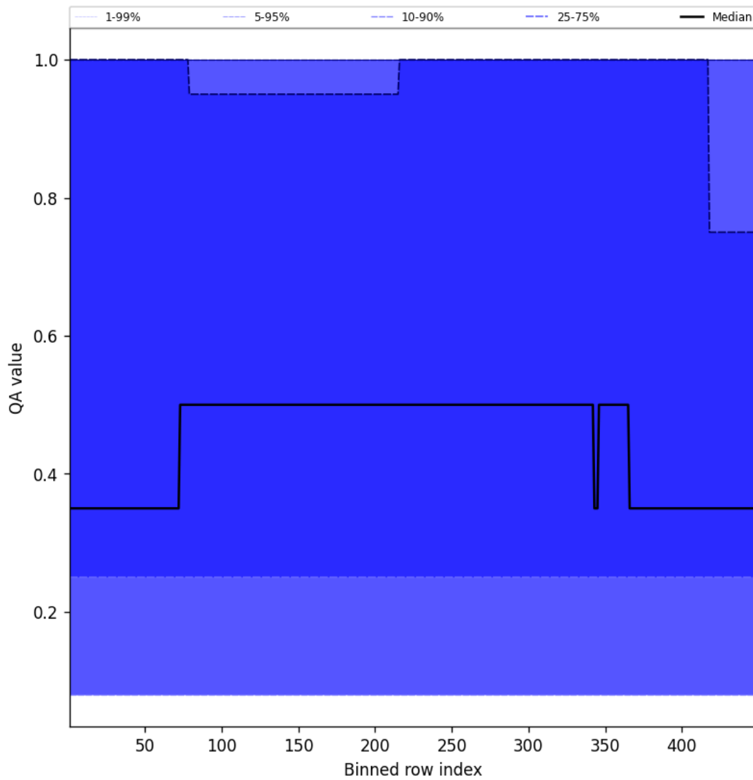
Figure 46: Along track statistics of “QA value” for 2025-09-05 to 2025-09-06
