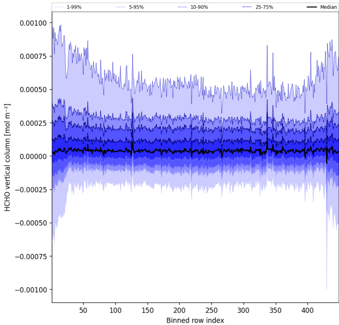
Figure 47: Along track statistics of “HCHO vertical column” for 2025-09-05 to 2025-09-06
