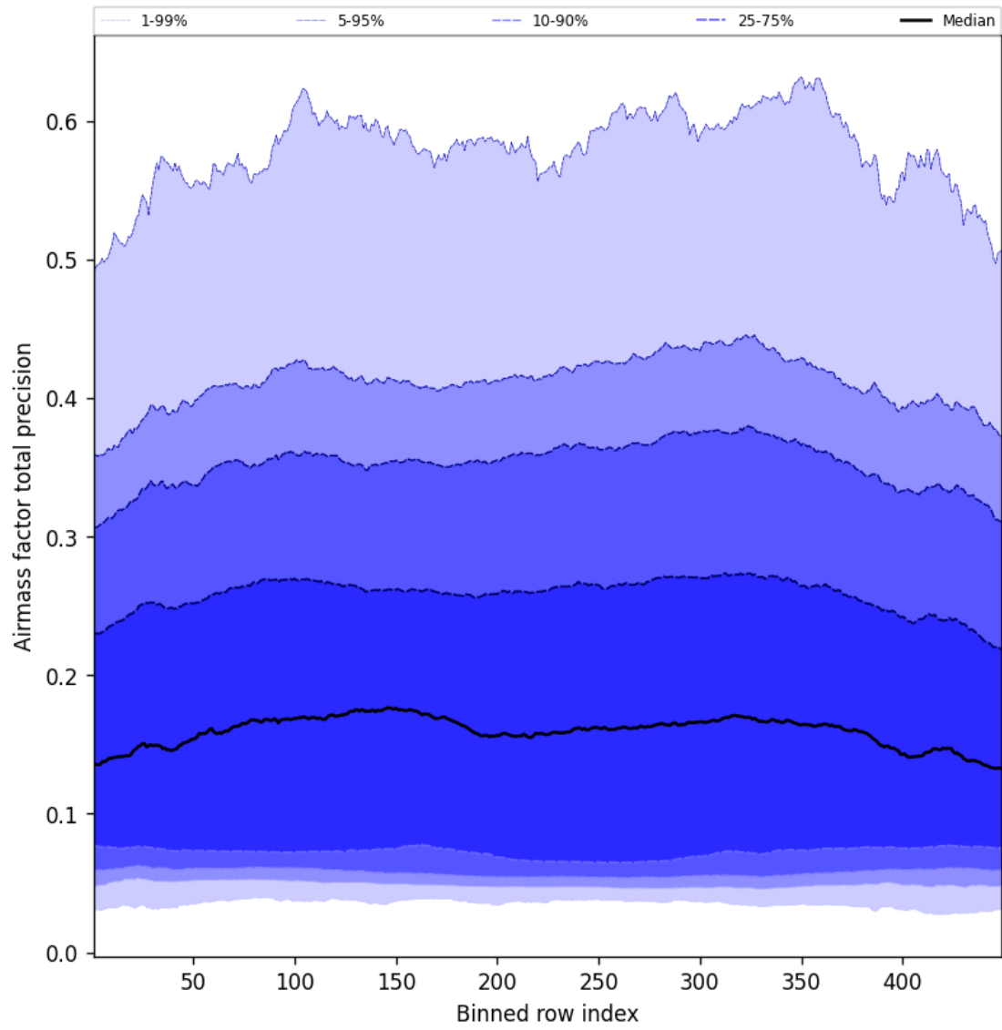
Figure 53: Along track statistics of “Airmass factor total precision” for 2025-09-05 to 2025-09-06
