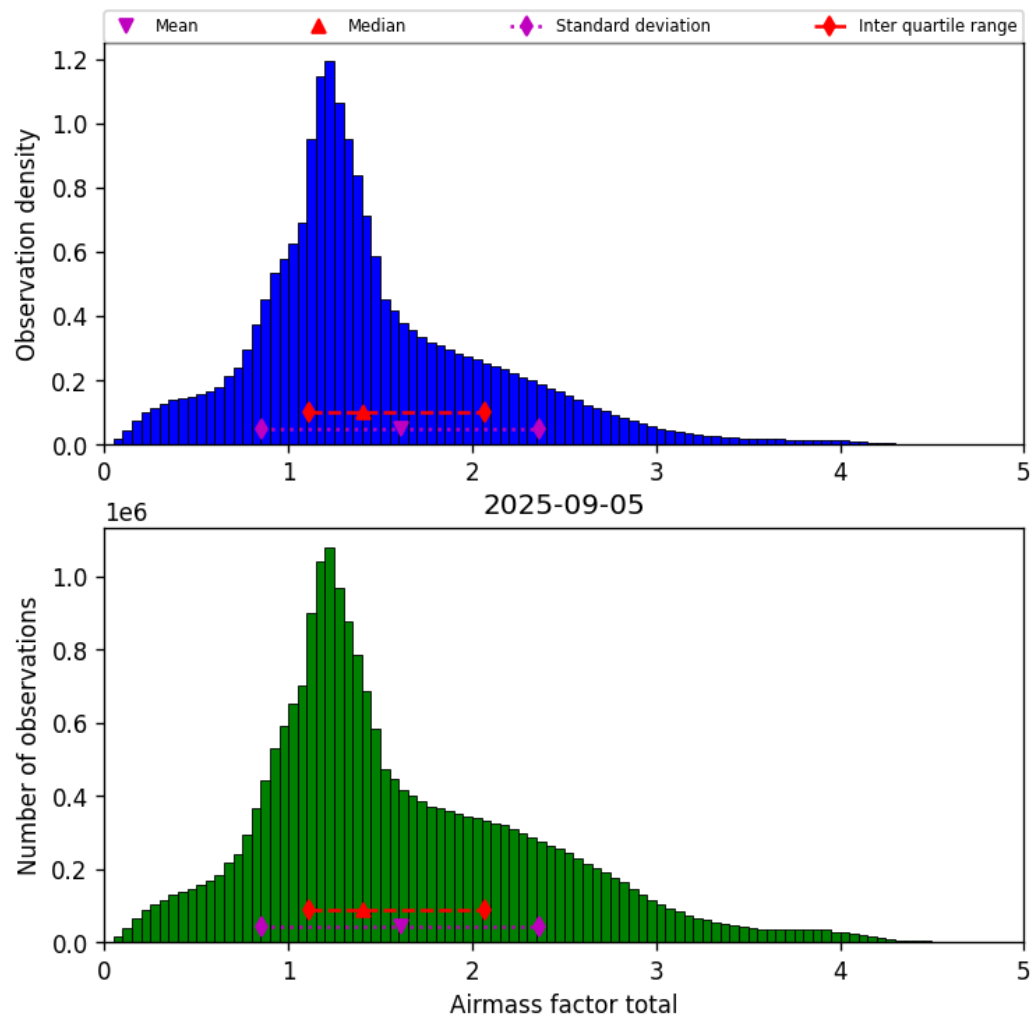
Figure 38: Histogram of “Airmass factor total” for 2025-09-05 to 2025-09-06
