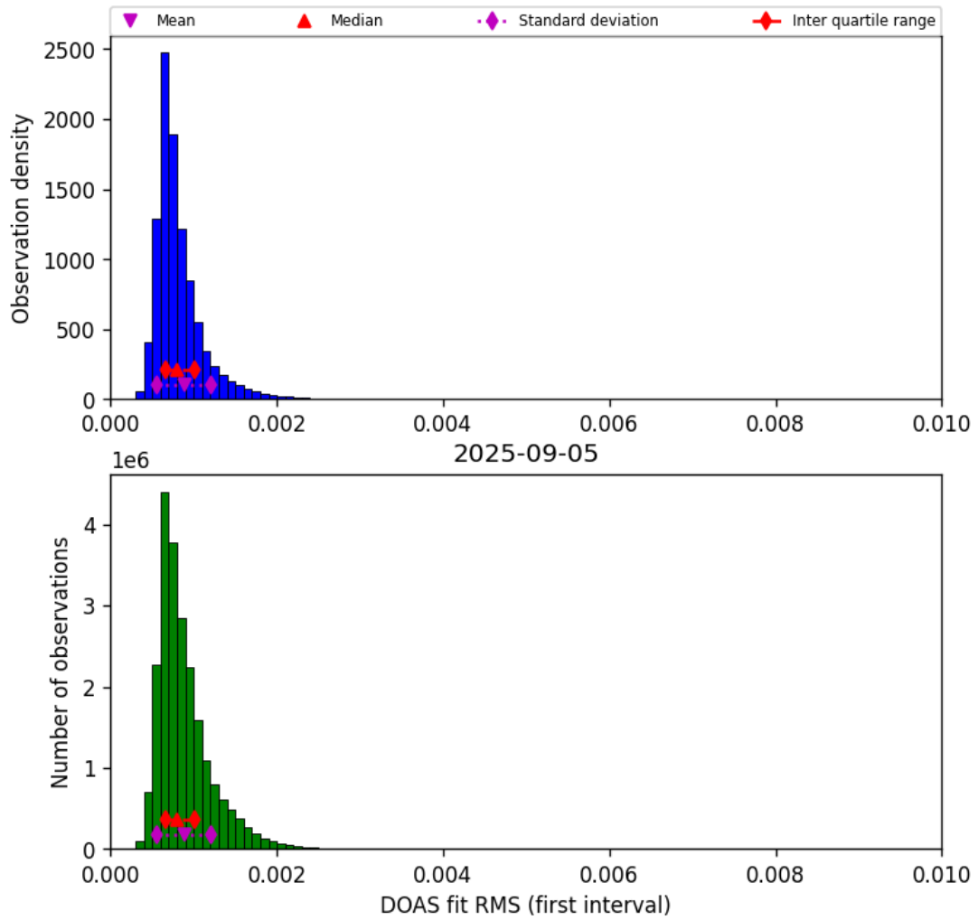
Figure 44: Histogram of “DOAS fit RMS (first interval)” for 2025-09-05 to 2025-09-06
