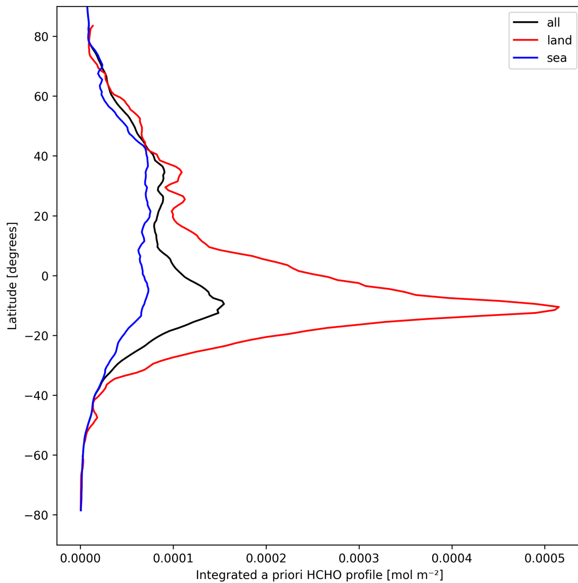
Figure 27: Zonal average of “Integrated a priori HCHO profile” for 2025-09-05 to 2025-09-06.
