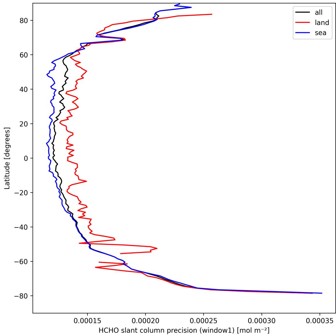
Figure 23: Zonal average of “HCHO slant column precision (window1)” for 2025-09-05 to 2025-09-06.
