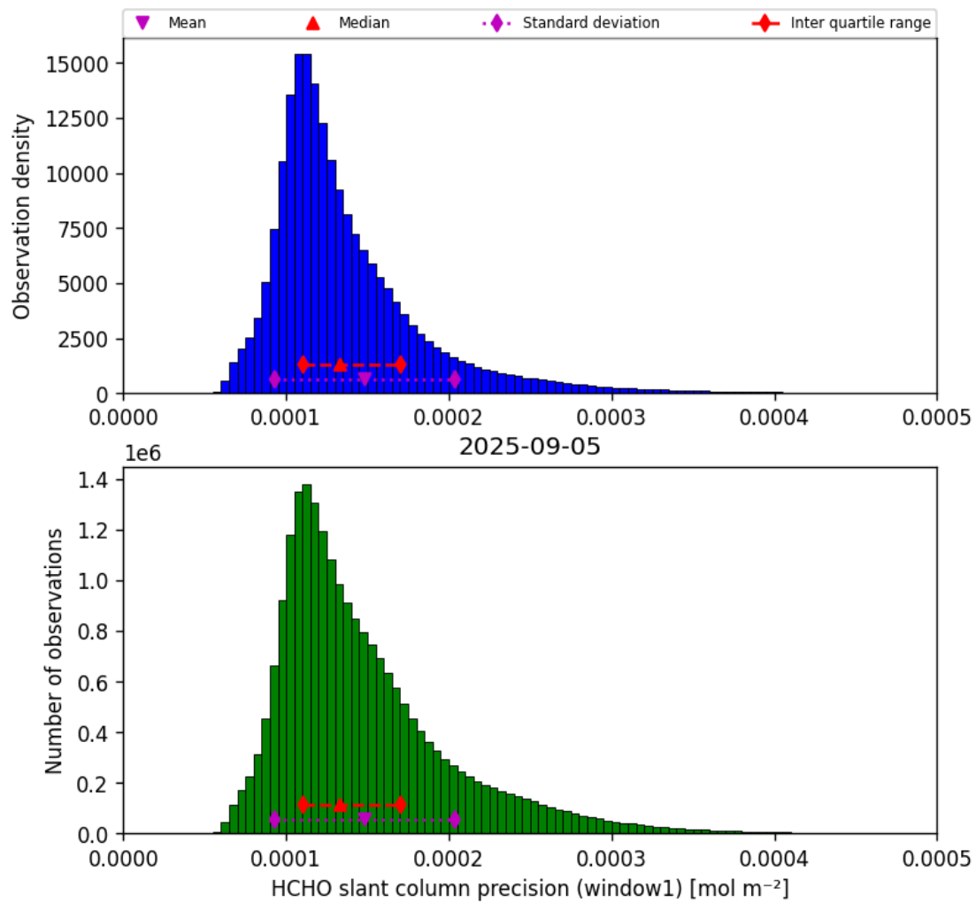
Figure 37: Histogram of “HCHO slant column precision (window1)” for 2025-09-05 to 2025-09-06
