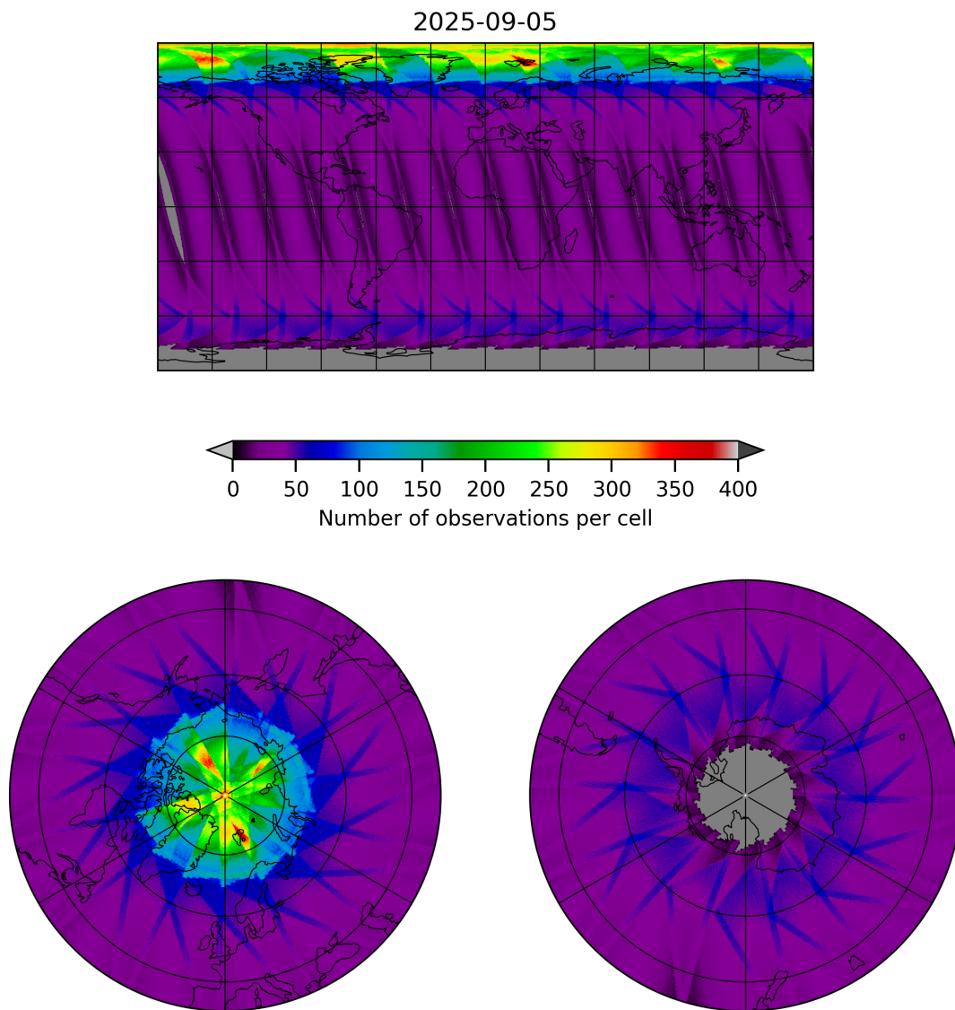
Figure 17: Map of the number of observations for 2025-09-05 to 2025-09-06
