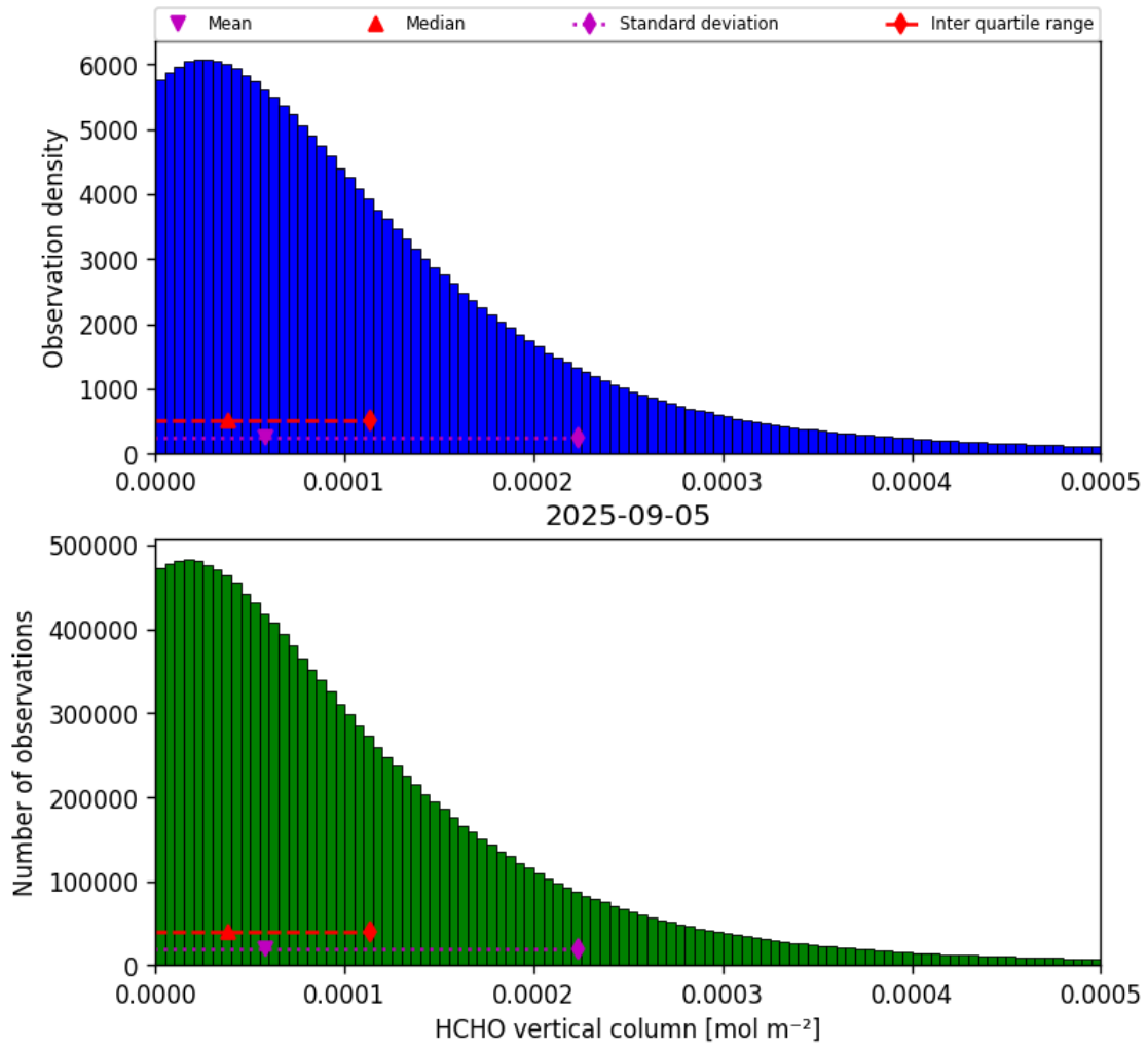
Figure 33: Histogram of “HCHO vertical column” for 2025-09-05 to 2025-09-06
