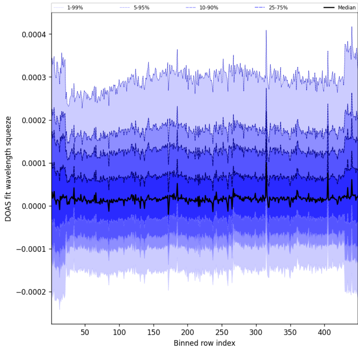
Figure 57: Along track statistics of “DOAS fit wavelength squeeze” for 2025-09-05 to 2025-09-06
