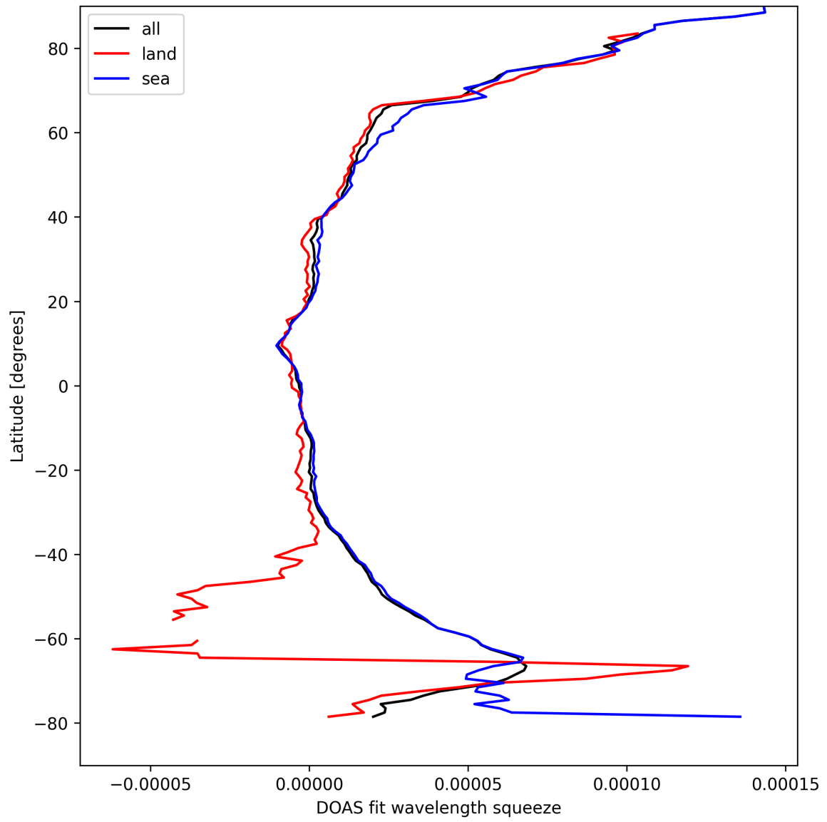
Figure 29: Zonal average of “DOAS fit wavelength squeeze” for 2025-09-05 to 2025-09-06.
