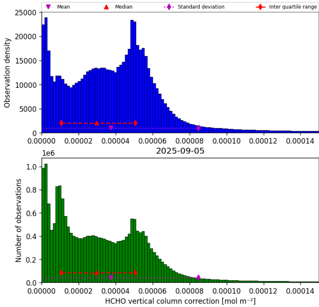
Figure 35: Histogram of “HCHO vertical column correction” for 2025-09-05 to 2025-09-06
