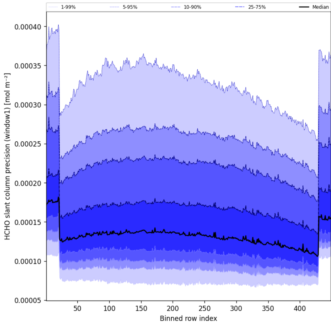
Figure 51: Along track statistics of “HCHO slant column precision (window1)” for 2025-09-05 to 2025-09-06
