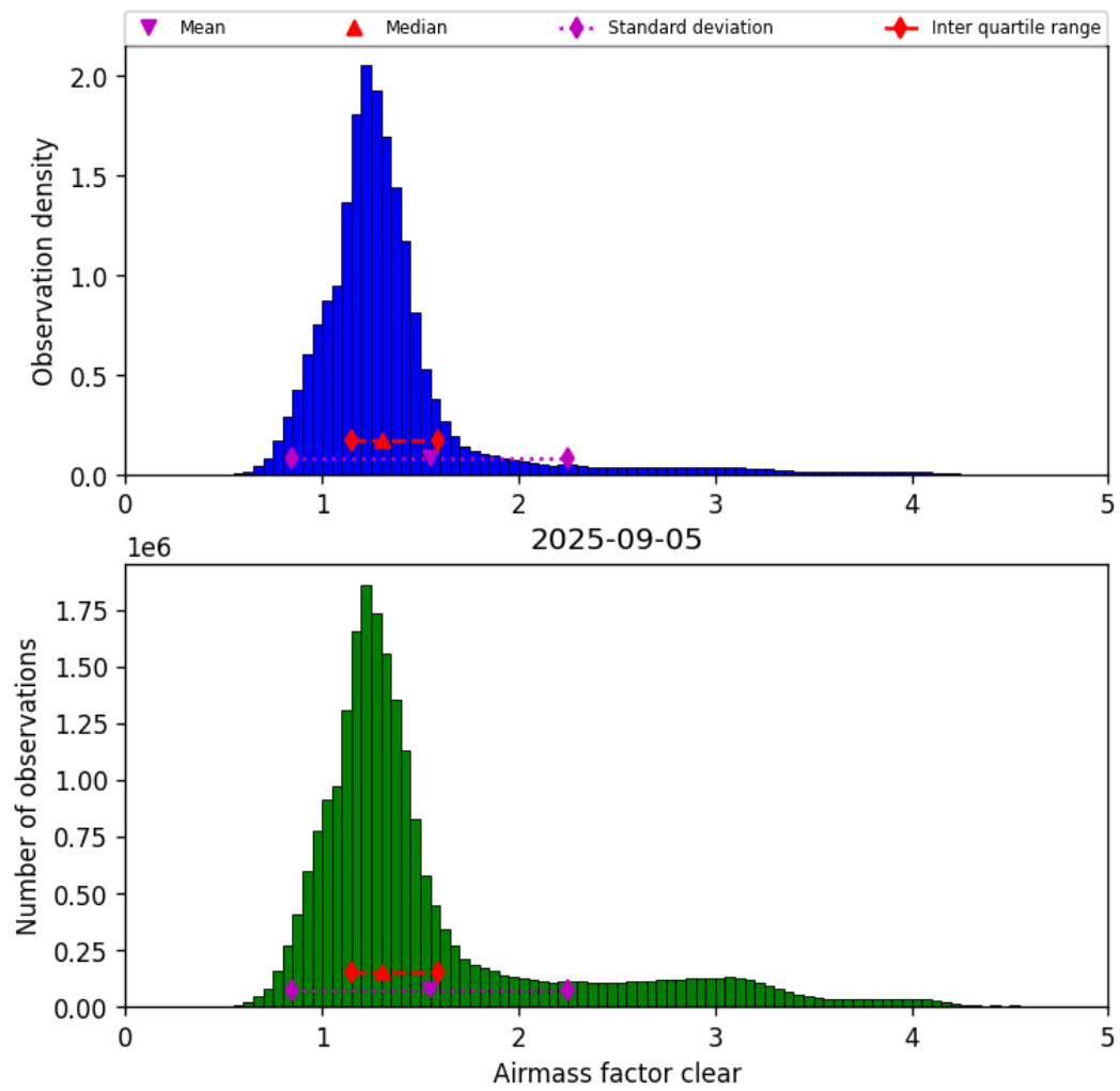
Figure 40: Histogram of “Airmass factor clear” for 2025-09-05 to 2025-09-06
