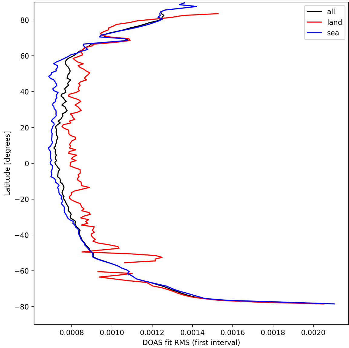
Figure 30: Zonal average of "DOAS fit RMS (first interval)" for 2025-09-05 to 2025-09-06.
