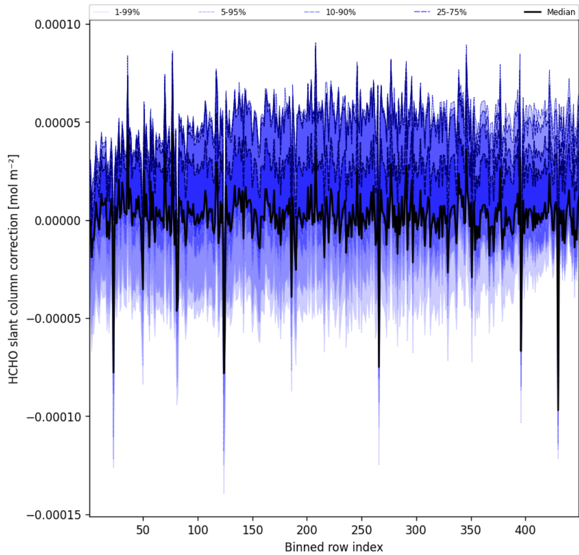
Figure 59: Along track statistics of “HCHO slant column correction” for 2025-09-05 to 2025-09-06
