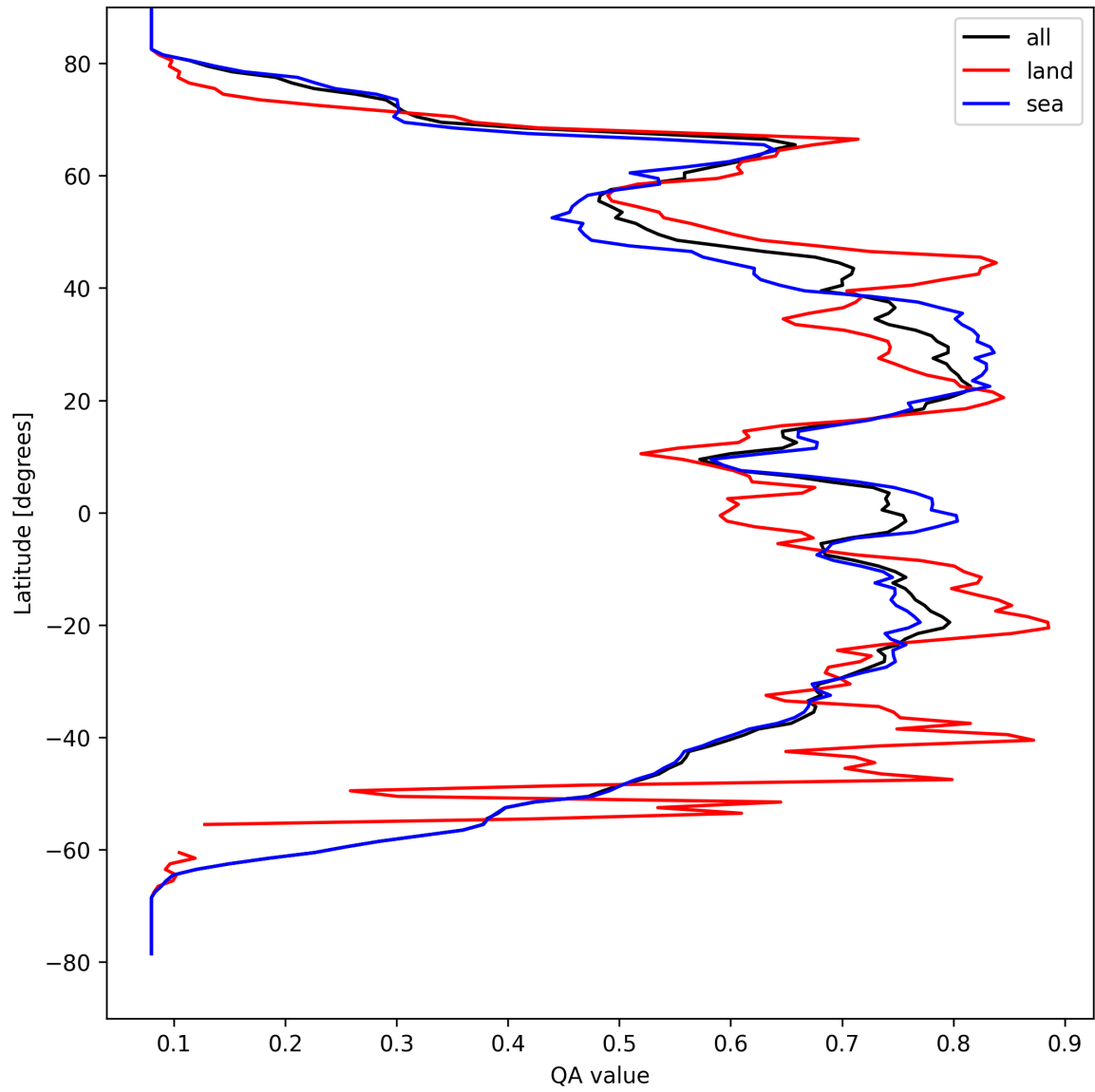
Figure 18: Zonal average of “QA value” for 2025-09-05 to 2025-09-06.
