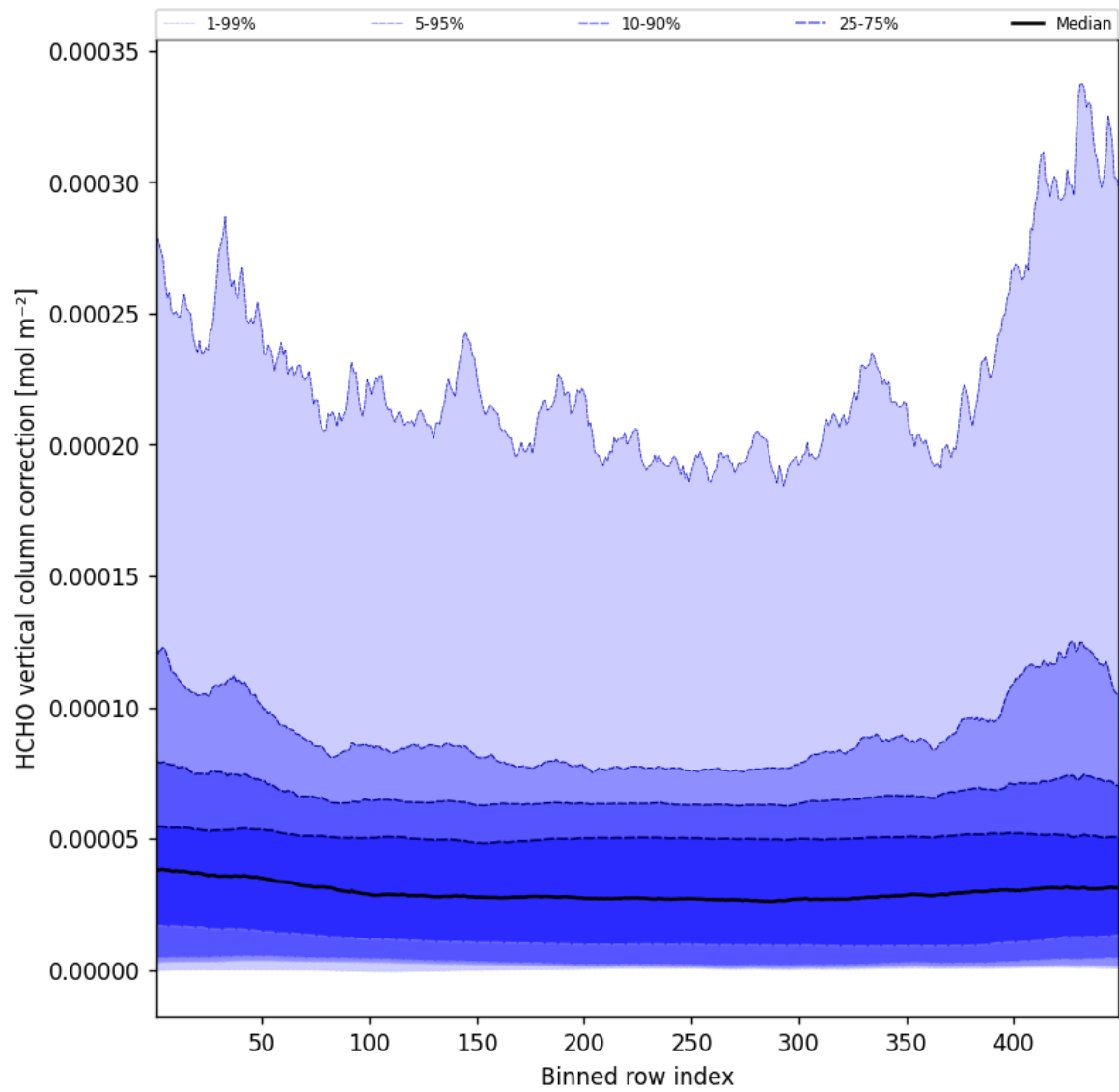
Figure 49: Along track statistics of “HCHO vertical column correction” for 2025-09-05 to 2025-09-06
