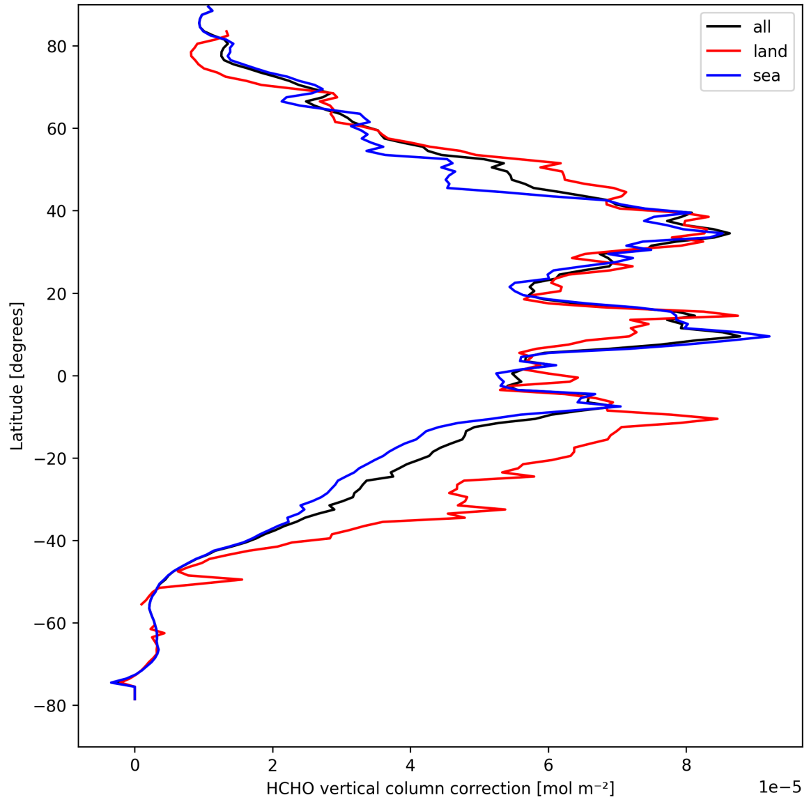
Figure 21: Zonal average of “HCHO vertical column correction” for 2025-09-05 to 2025-09-06.
