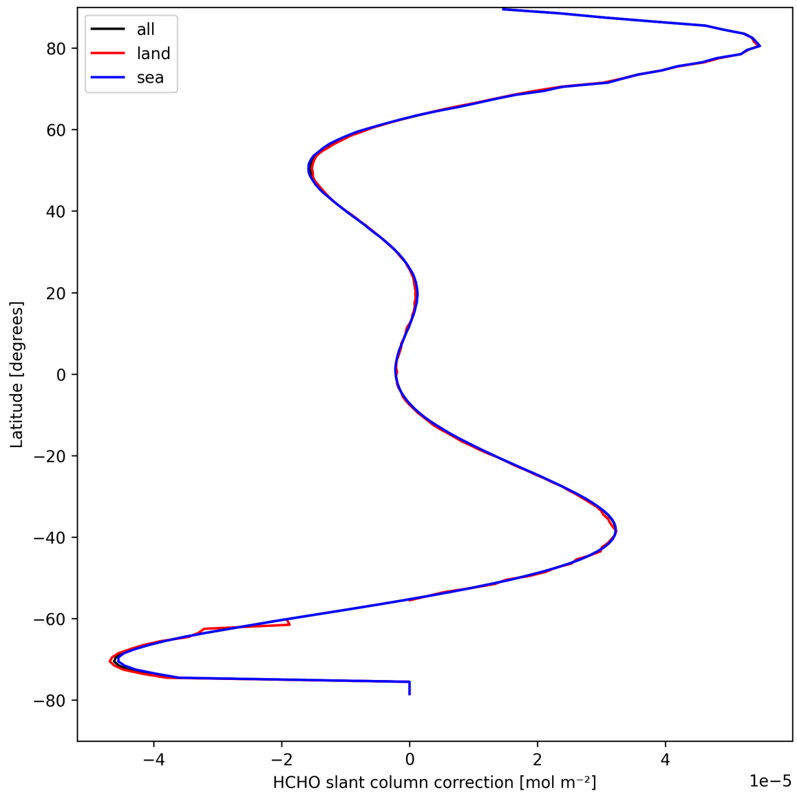
Figure 31: Zonal average of “HCHO slant column correction” for 2025-09-05 to 2025-09-06.
