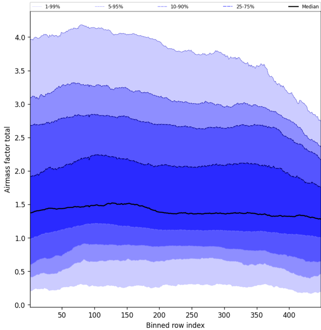
Figure 52: Along track statistics of “Airmass factor total” for 2025-09-05 to 2025-09-06
