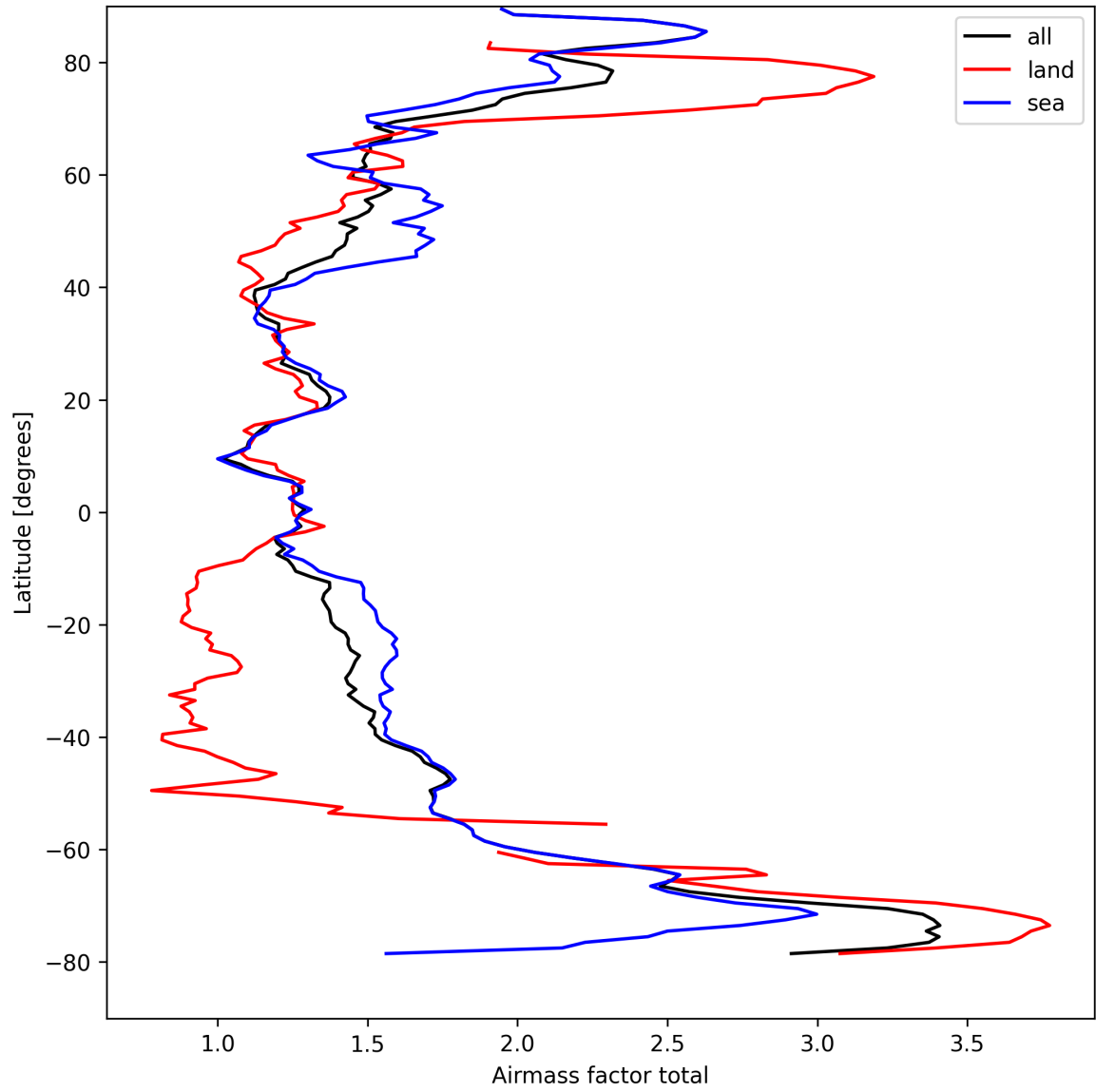
Figure 24: Zonal average of “Airmass factor total” for 2025-09-05 to 2025-09-06.
