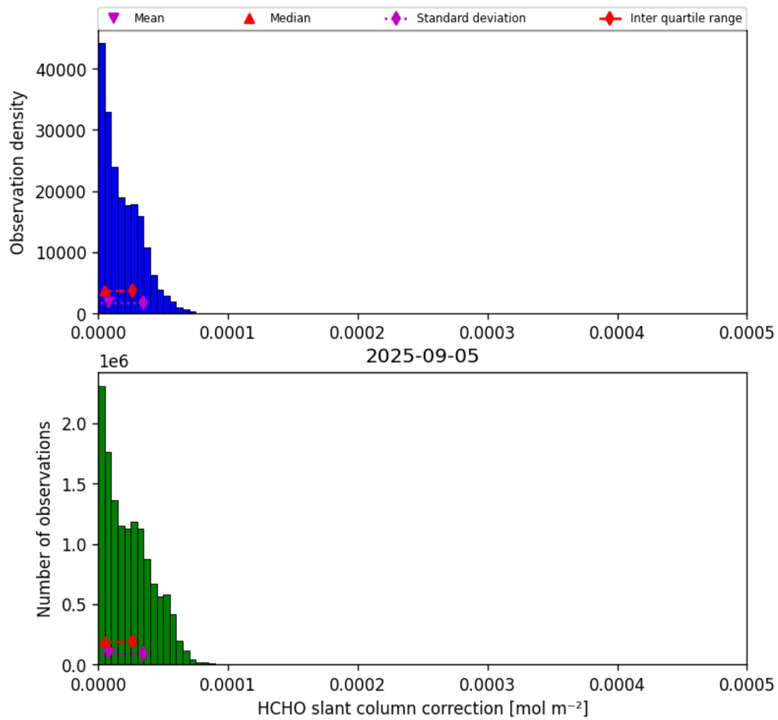
Figure 45: Histogram of “HCHO slant column correction” for 2025-09-05 to 2025-09-06
