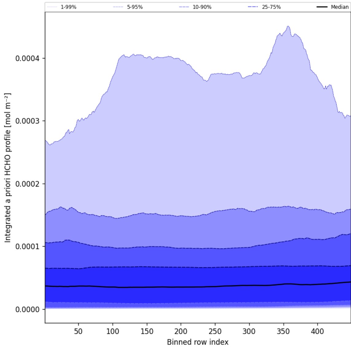
Figure 55: Along track statistics of “Integrated a priori HCHO profile” for 2025-09-05 to 2025-09-06
