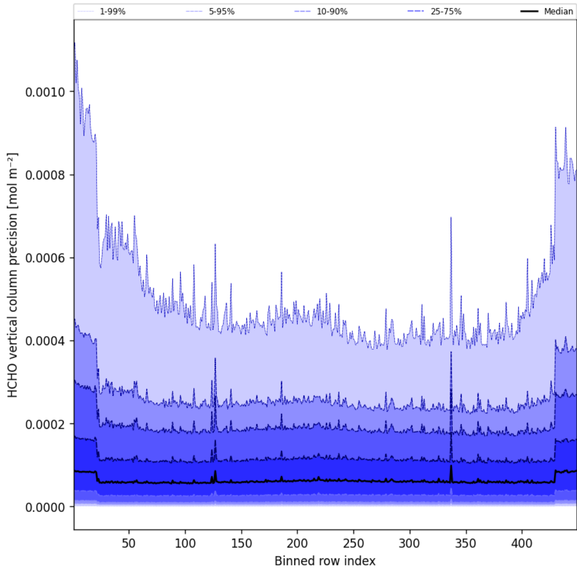
Figure 48: Along track statistics of “HCHO vertical column precision” for 2025-09-05 to 2025-09-06
