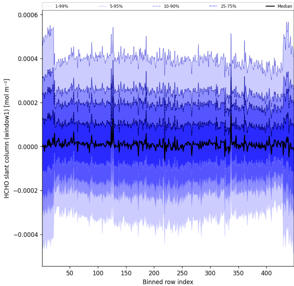
Figure 50: Along track statistics of “HCHO slant column (window1)” for 2025-09-05 to 2025-09-06
