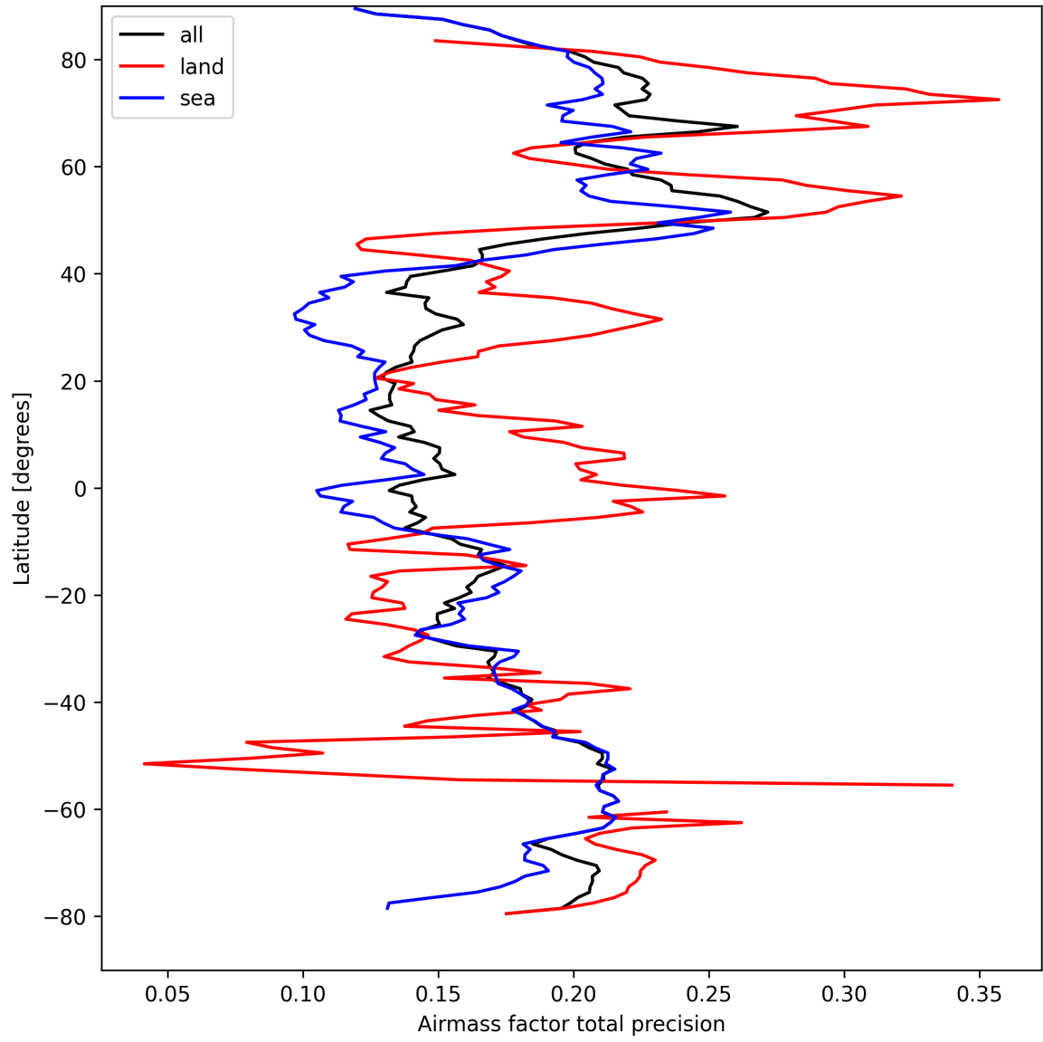
Figure 25: Zonal average of “Airmass factor total precision” for 2025-09-07 to 2025-09-07.
