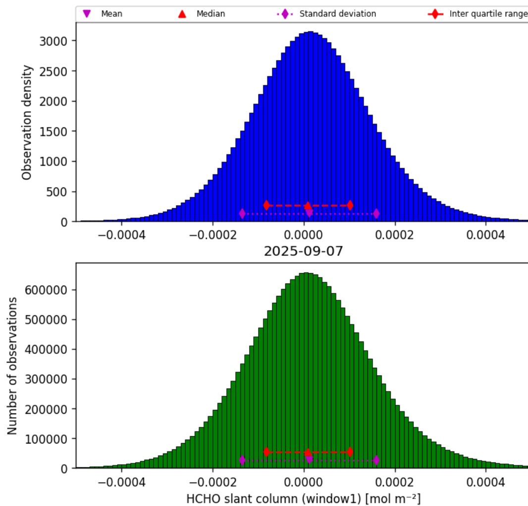
Figure 36: Histogram of “HCHO slant column (window1)” for 2025-09-07 to 2025-09-07
