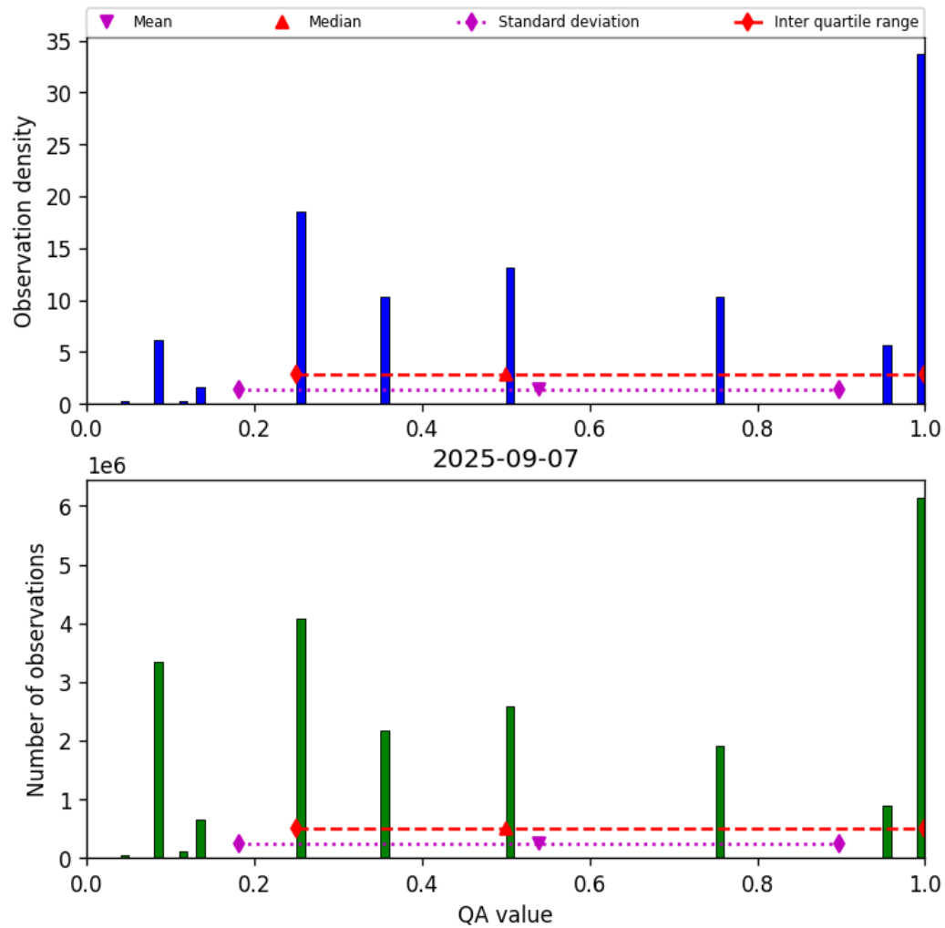
Figure 32: Histogram of “QA value” for 2025-09-07 to 2025-09-07
