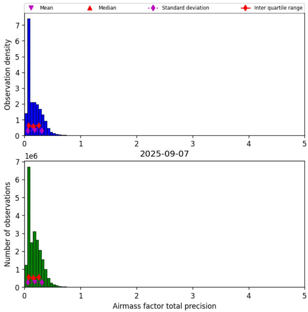
Figure 39: Histogram of “Airmass factor total precision” for 2025-09-07 to 2025-09-07
