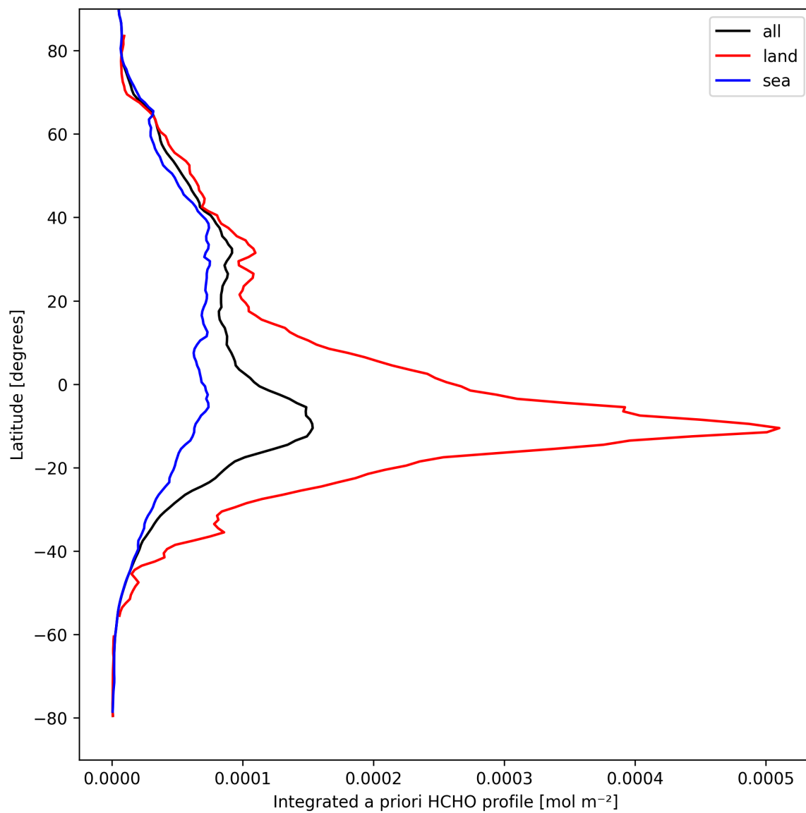
Figure 27: Zonal average of “Integrated a priori HCHO profile” for 2025-09-07 to 2025-09-07.
