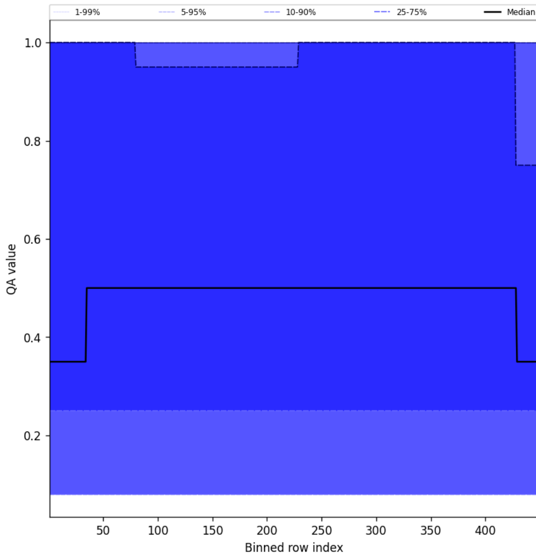
Figure 46: Along track statistics of “QA value” for 2025-09-07 to 2025-09-07
