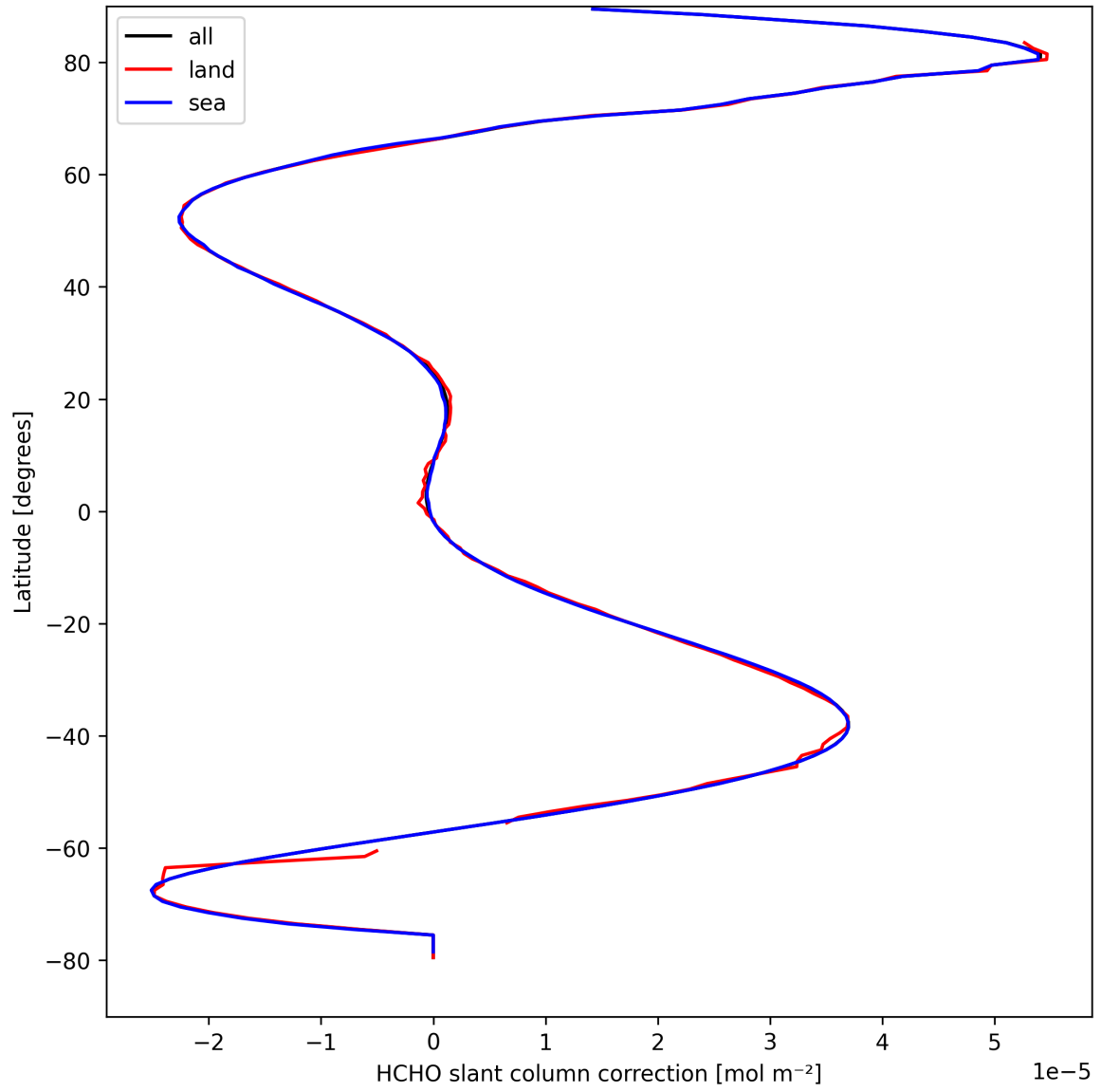
Figure 31: Zonal average of “HCHO slant column correction” for 2025-09-07 to 2025-09-07.
