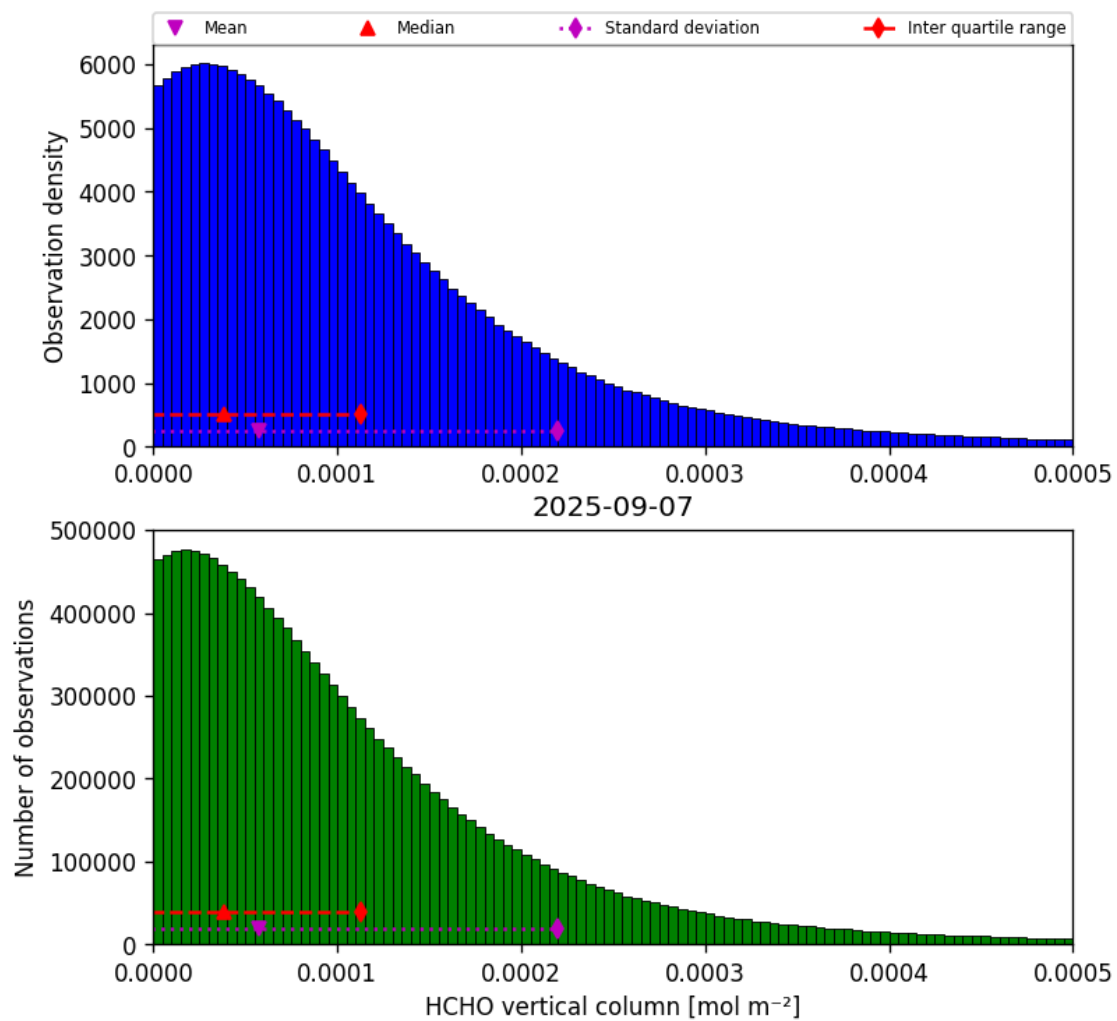
Figure 33: Histogram of “HCHO vertical column” for 2025-09-07 to 2025-09-07
