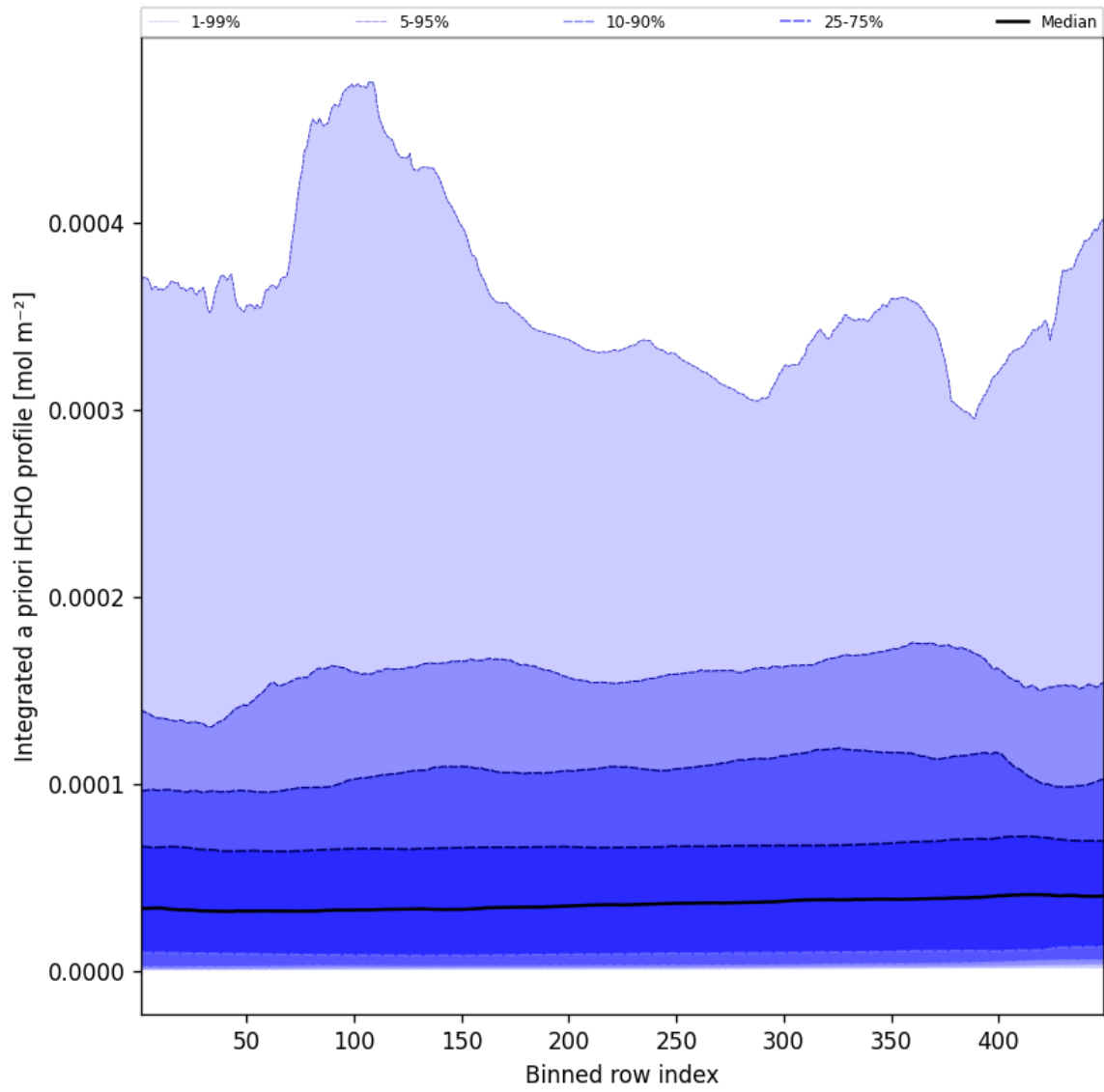
Figure 55: Along track statistics of “Integrated a priori HCHO profile” for 2025-09-07 to 2025-09-07
