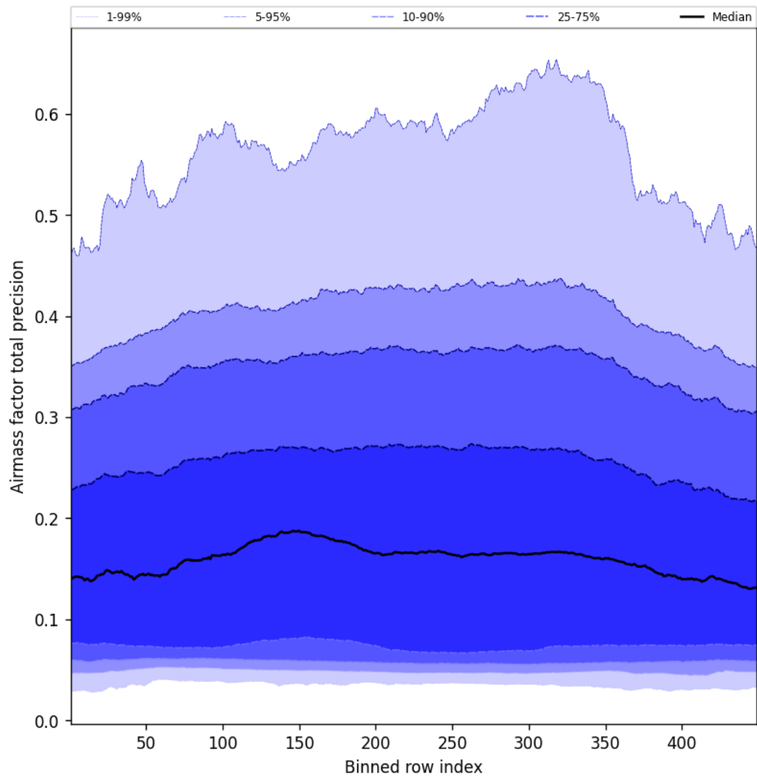
Figure 53: Along track statistics of “Airmass factor total precision” for 2025-09-07 to 2025-09-07
