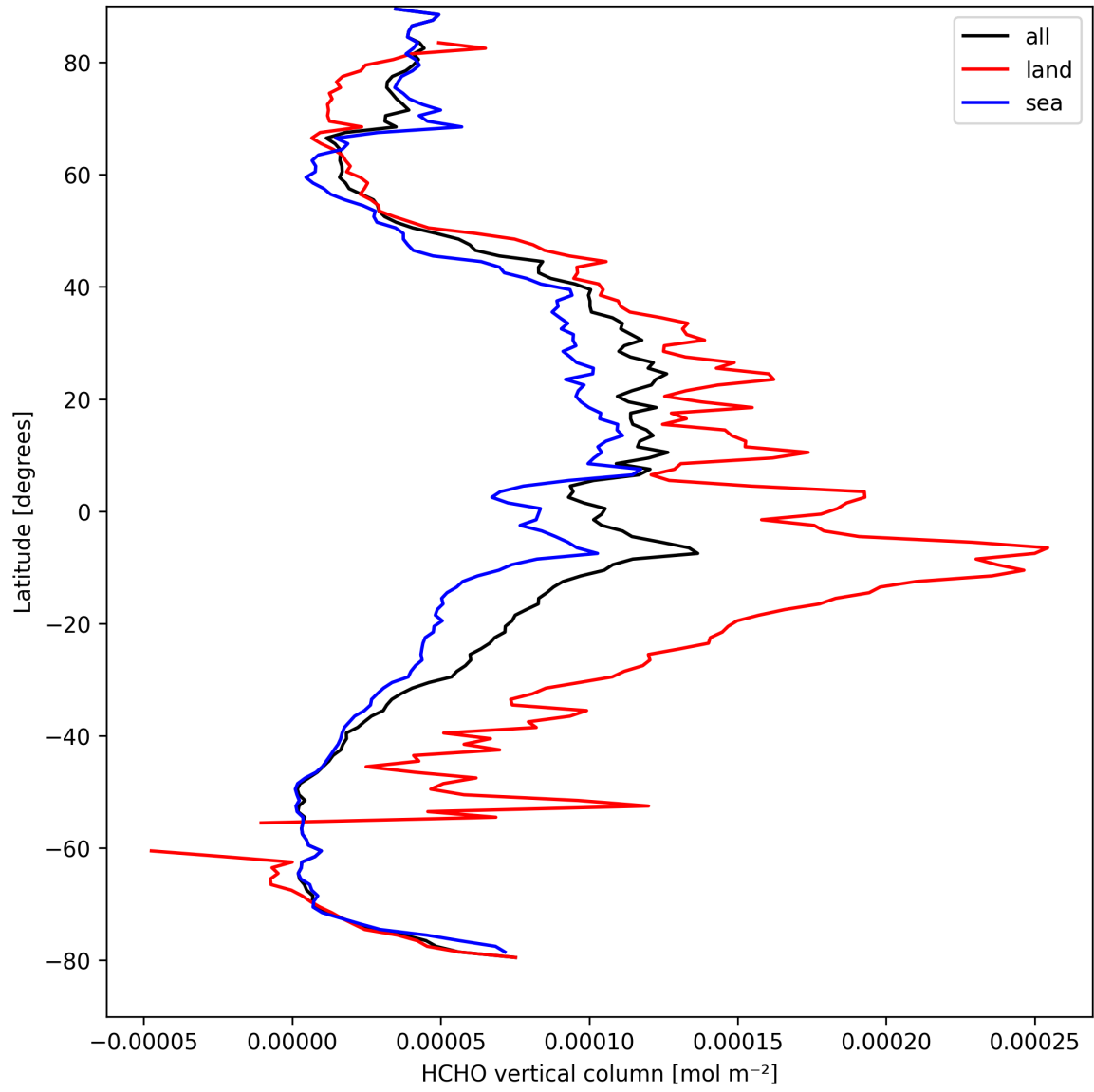
Figure 19: Zonal average of “HCHO vertical column” for 2025-09-07 to 2025-09-07.
