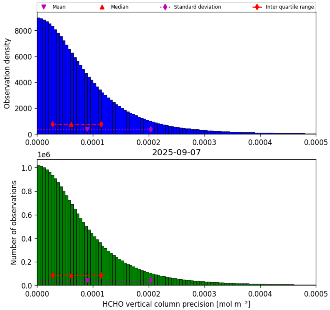
Figure 34: Histogram of “HCHO vertical column precision” for 2025-09-07 to 2025-09-07
