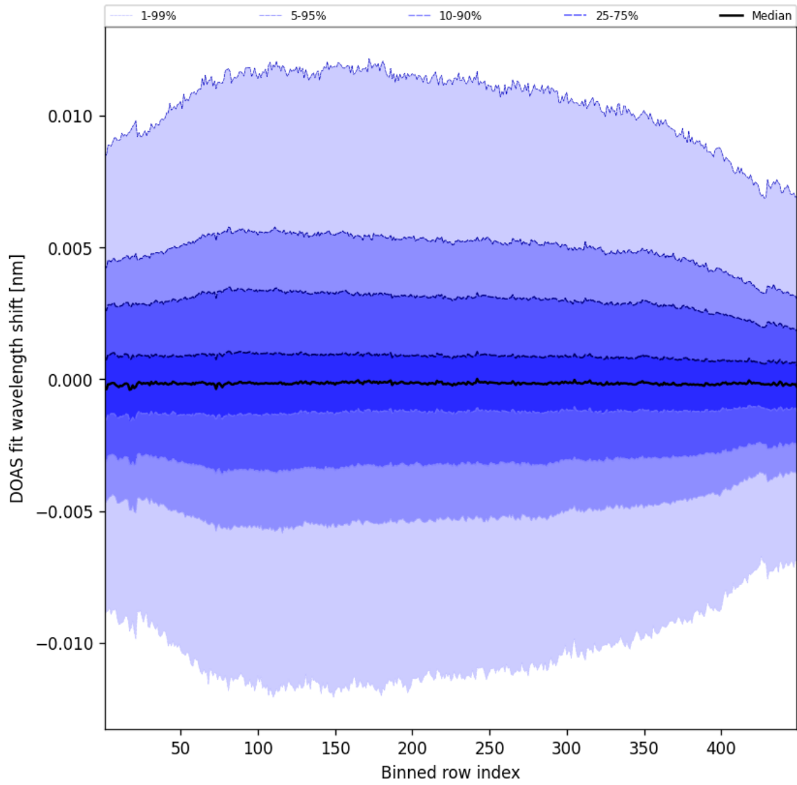
Figure 56: Along track statistics of “DOAS fit wavelength shift” for 2025-09-07 to 2025-09-07
