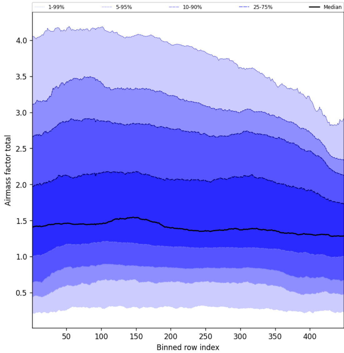
Figure 52: Along track statistics of “Airmass factor total” for 2025-09-07 to 2025-09-07
