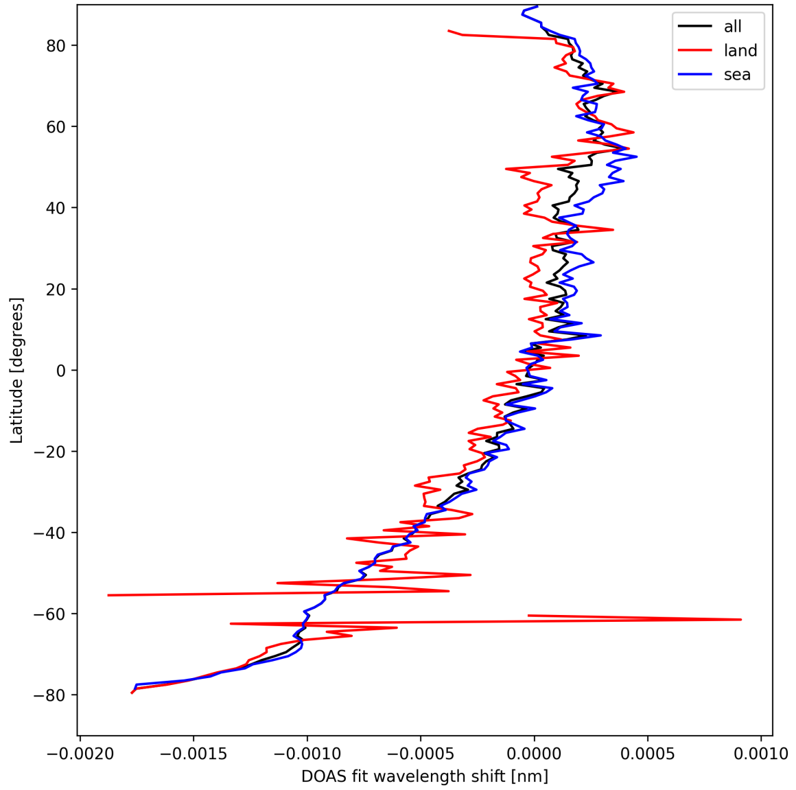
Figure 28: Zonal average of “DOAS fit wavelength shift” for 2025-09-07 to 2025-09-07.
