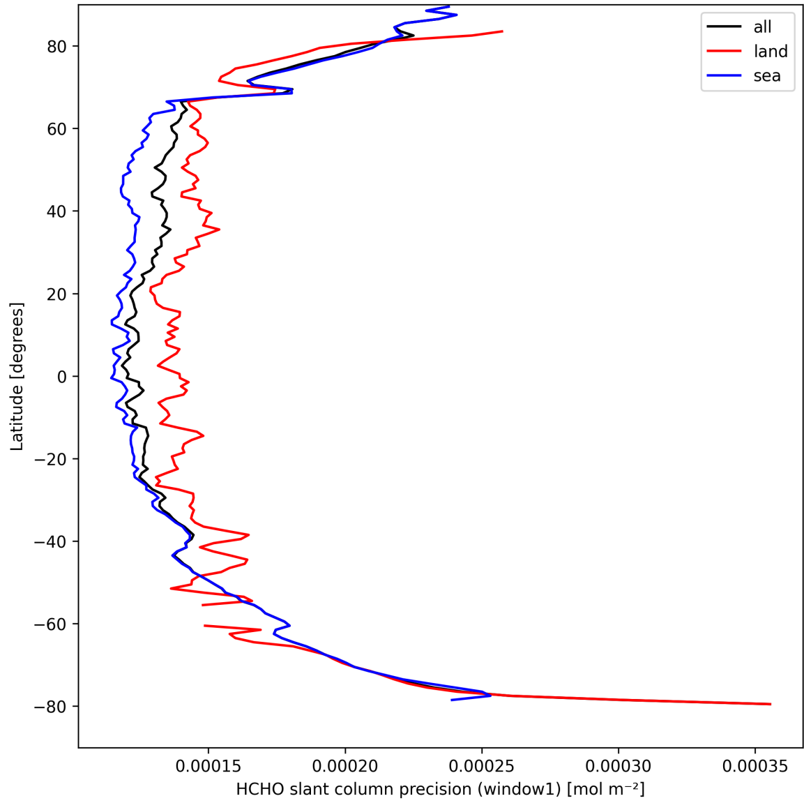
Figure 23: Zonal average of “HCHO slant column precision (window1)” for 2025-09-07 to 2025-09-07.
