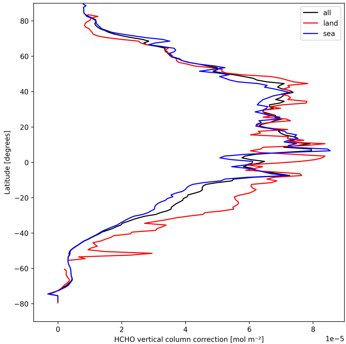
Figure 21: Zonal average of “HCHO vertical column correction” for 2025-09-07 to 2025-09-07.
