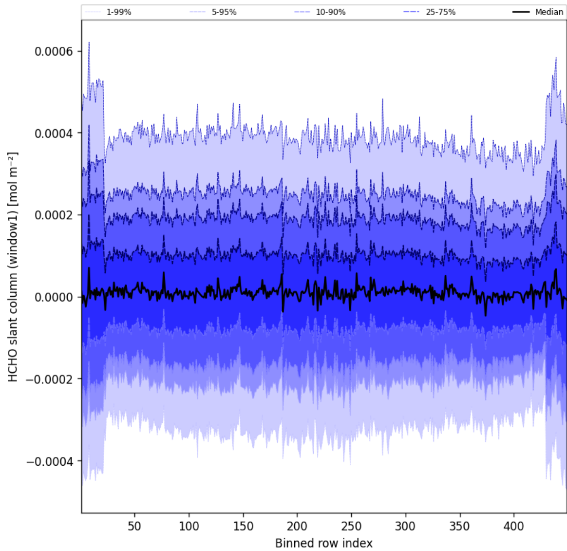
Figure 50: Along track statistics of “HCHO slant column (window1)” for 2025-09-07 to 2025-09-07
