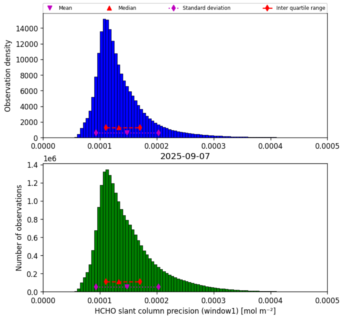
Figure 37: Histogram of “HCHO slant column precision (window1)” for 2025-09-07 to 2025-09-07
