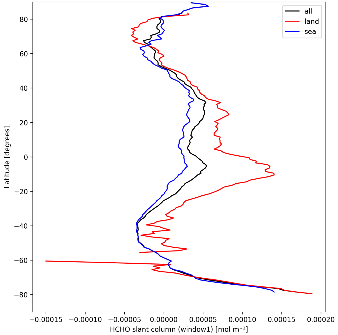
Figure 22: Zonal average of “HCHO slant column (window1)” for 2025-09-07 to 2025-09-07.
