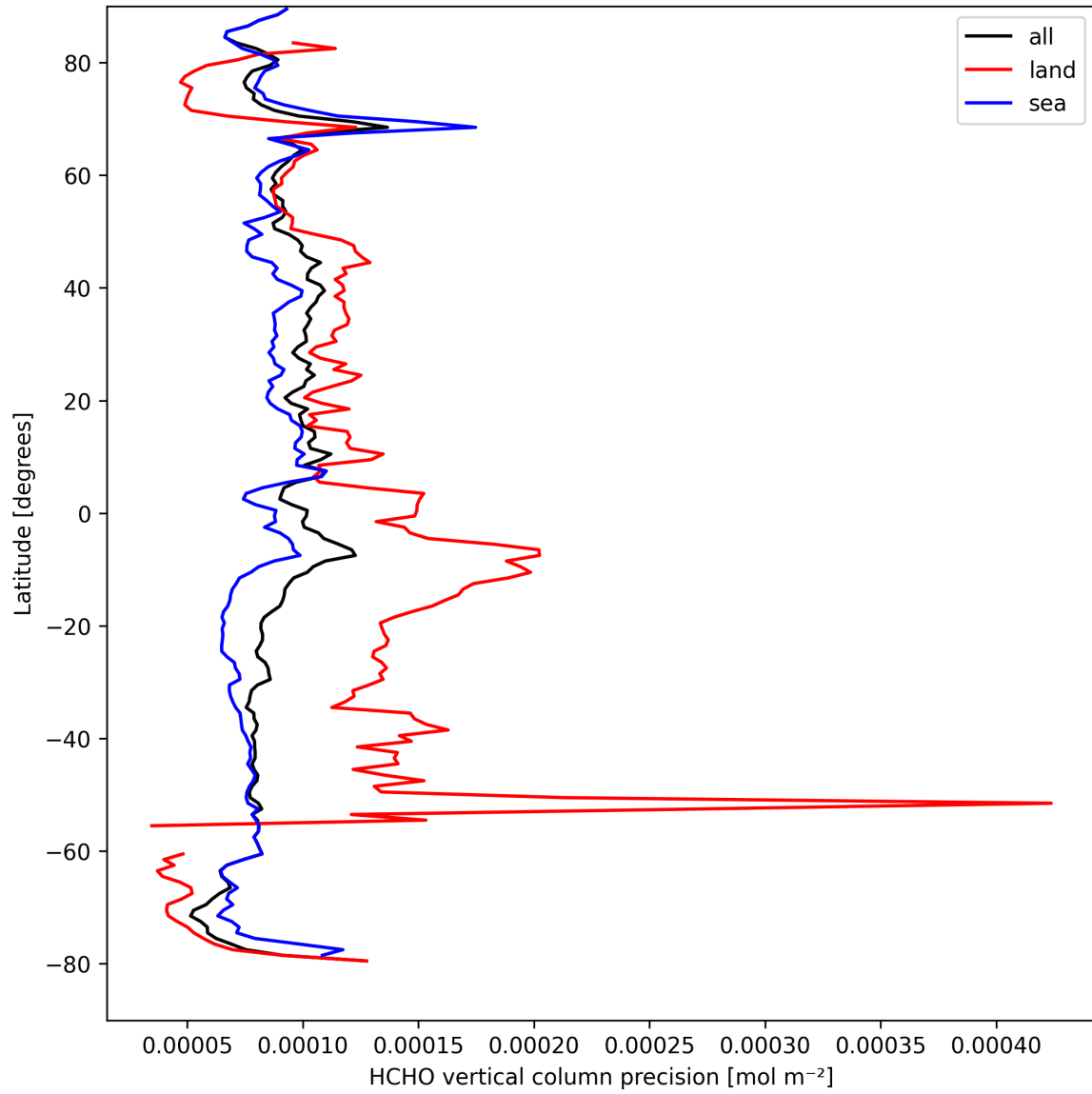
Figure 20: Zonal average of “HCHO vertical column precision” for 2025-09-07 to 2025-09-07.
