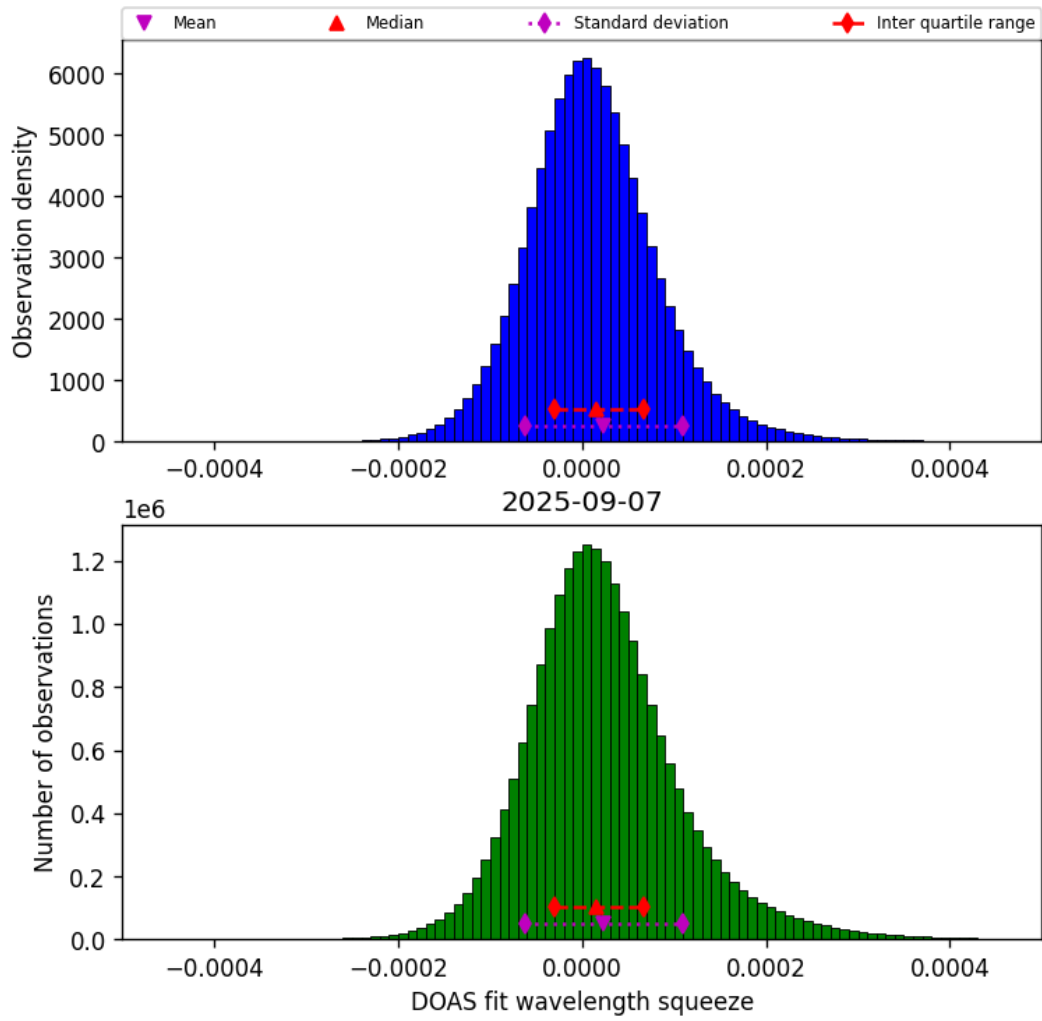
Figure 43: Histogram of “DOAS fit wavelength squeeze” for 2025-09-07 to 2025-09-07
