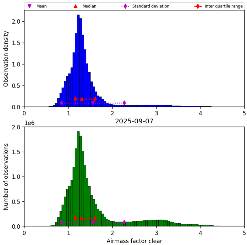
Figure 40: Histogram of “Airmass factor clear” for 2025-09-07 to 2025-09-07
