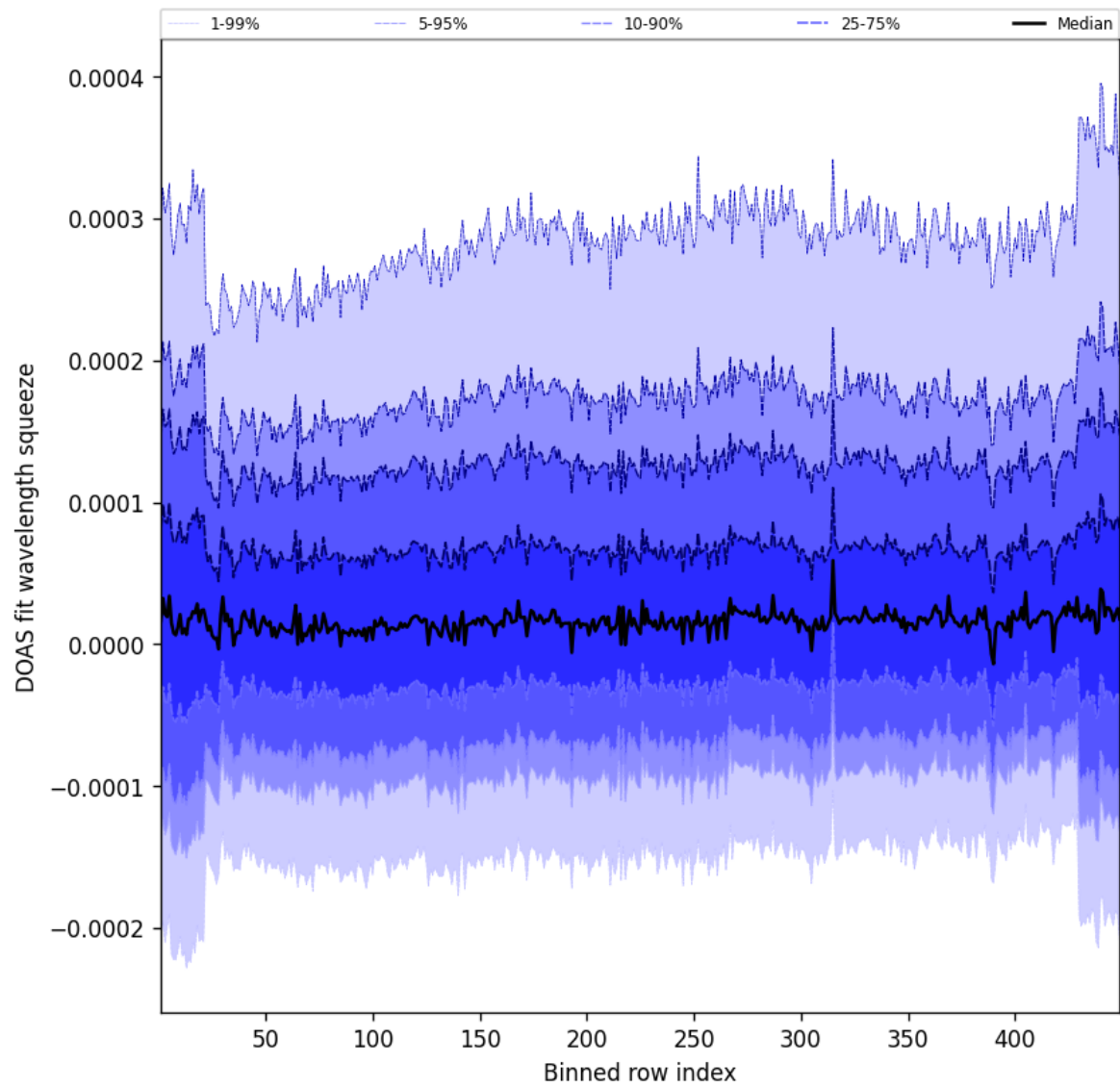
Figure 57: Along track statistics of “DOAS fit wavelength squeeze” for 2025-09-07 to 2025-09-07
