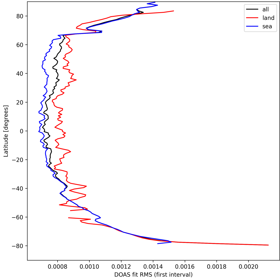
Figure 30: Zonal average of "DOAS fit RMS (first interval)" for 2025-09-07 to 2025-09-07.
