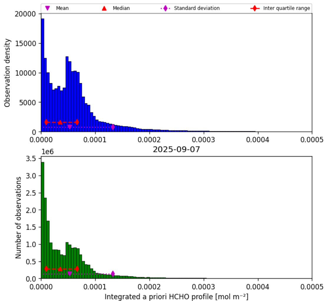
Figure 41: Histogram of “Integrated a priori HCHO profile” for 2025-09-07 to 2025-09-07
