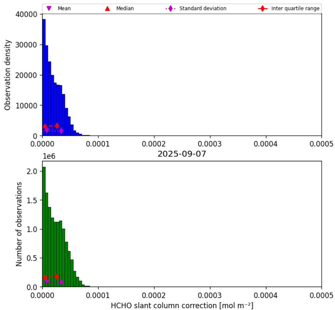
Figure 45: Histogram of “HCHO slant column correction” for 2025-09-07 to 2025-09-07
