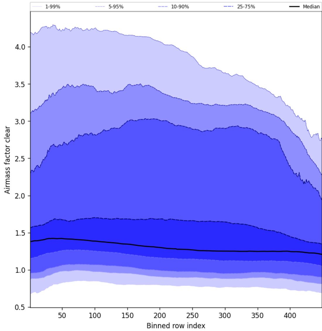
Figure 54: Along track statistics of “Airmass factor clear” for 2025-09-07 to 2025-09-07
