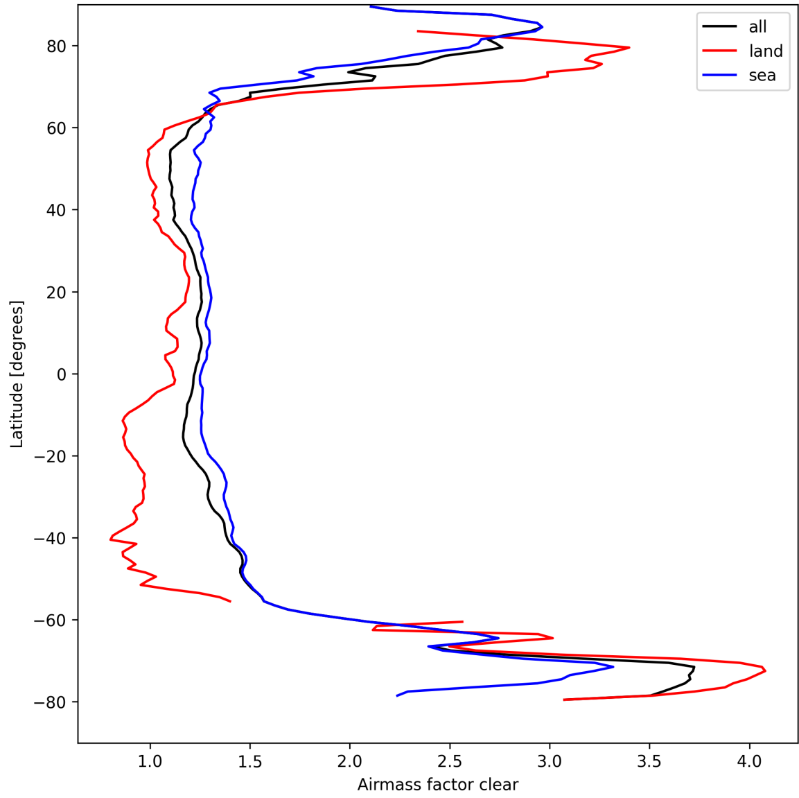
Figure 26: Zonal average of “Airmass factor clear” for 2025-09-07 to 2025-09-07.
