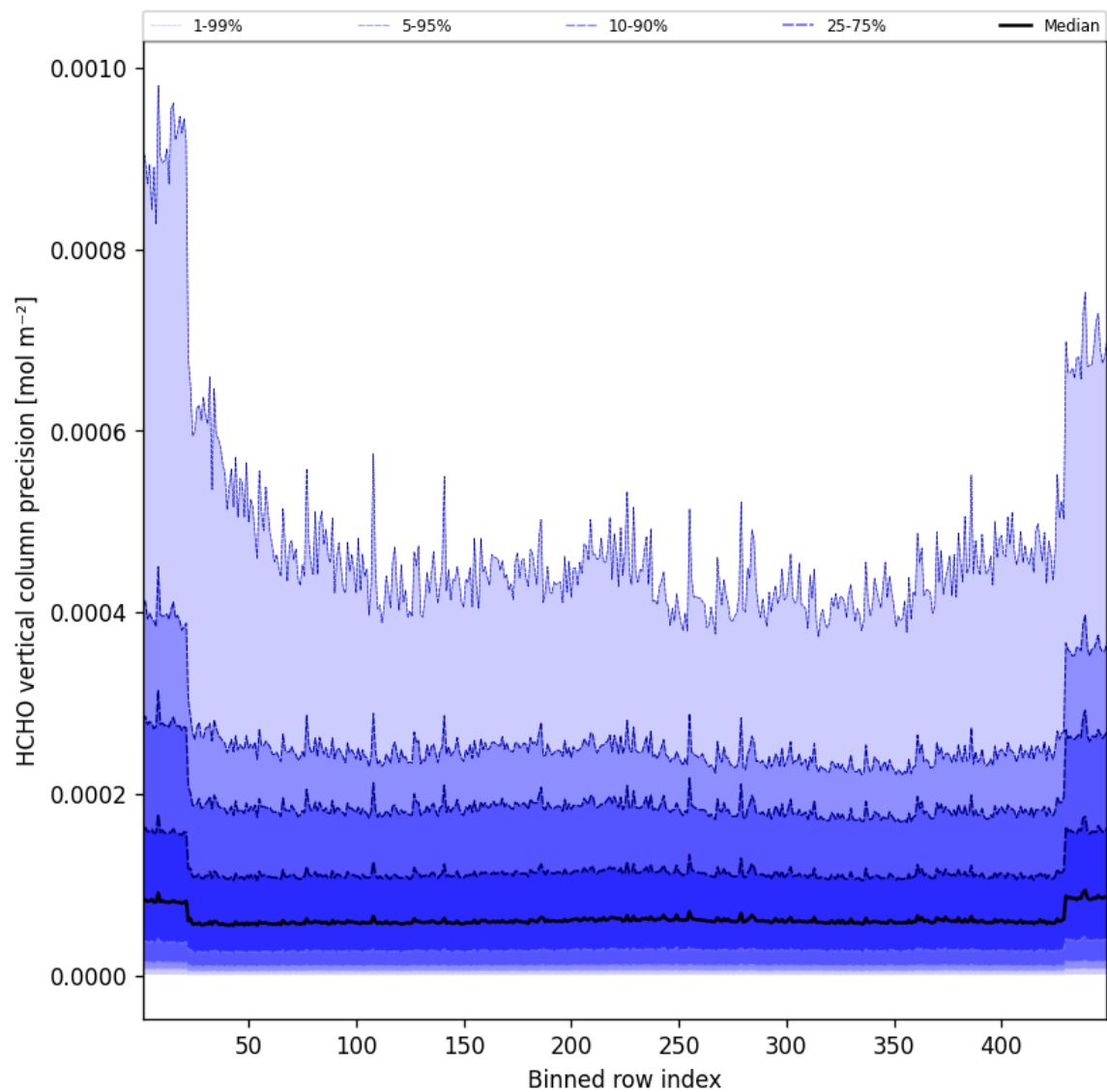
Figure 48: Along track statistics of “HCHO vertical column precision” for 2025-09-07 to 2025-09-07
