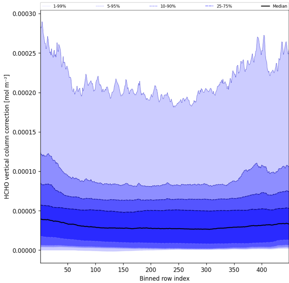
Figure 49: Along track statistics of “HCHO vertical column correction” for 2025-09-07 to 2025-09-07
