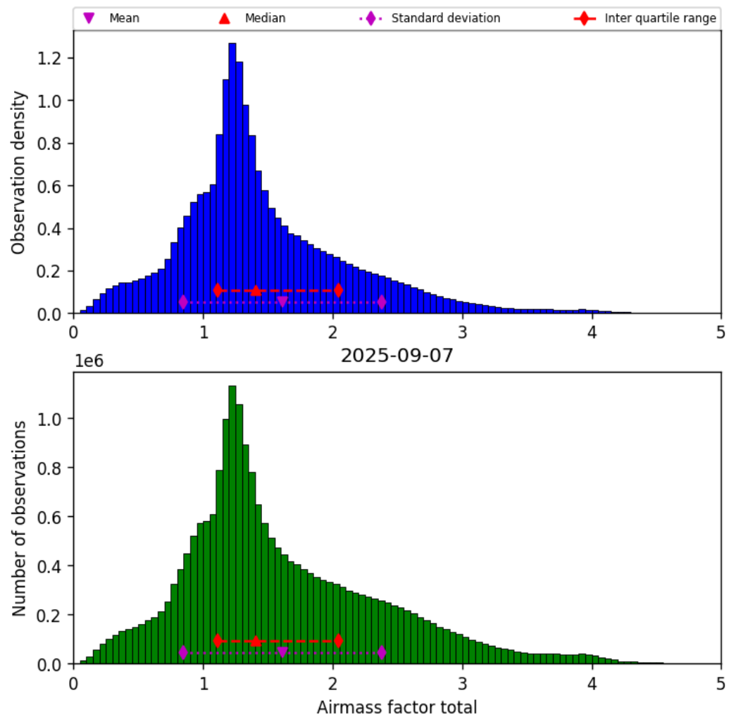
Figure 38: Histogram of “Airmass factor total” for 2025-09-07 to 2025-09-07
