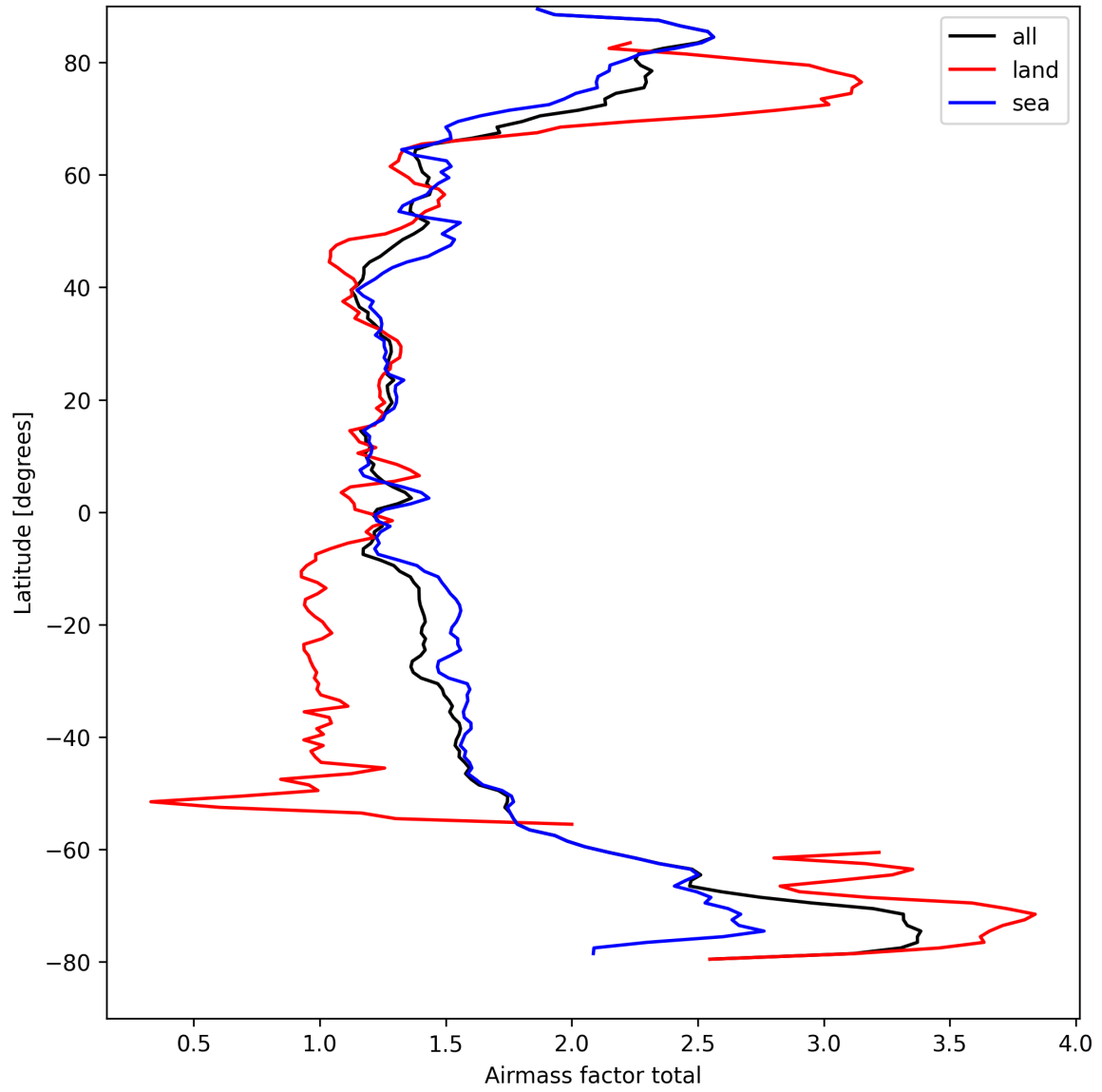
Figure 24: Zonal average of “Airmass factor total” for 2025-09-07 to 2025-09-07.
