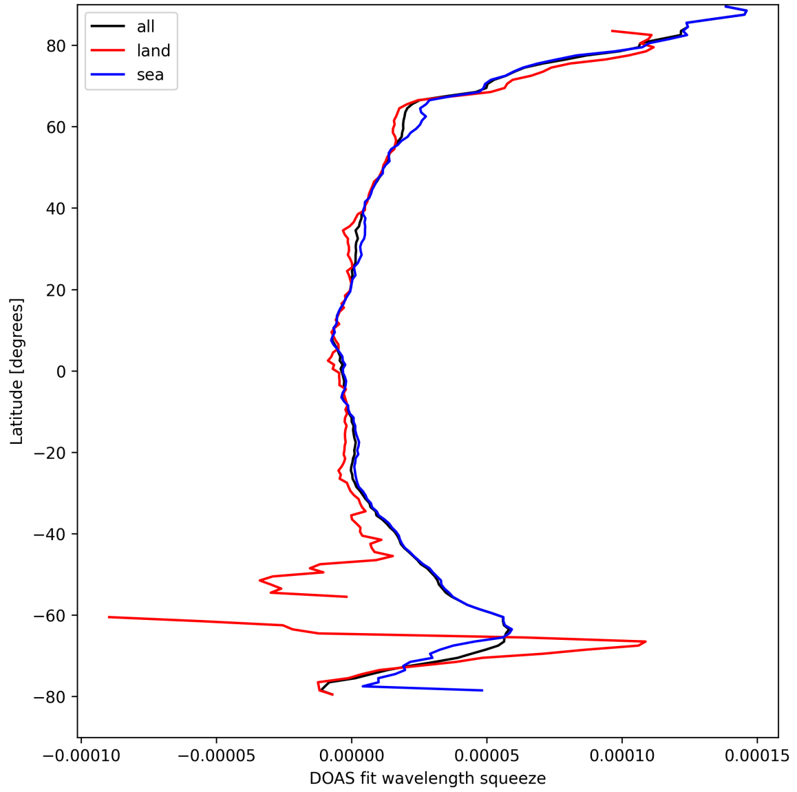
Figure 29: Zonal average of “DOAS fit wavelength squeeze” for 2025-09-07 to 2025-09-07.
