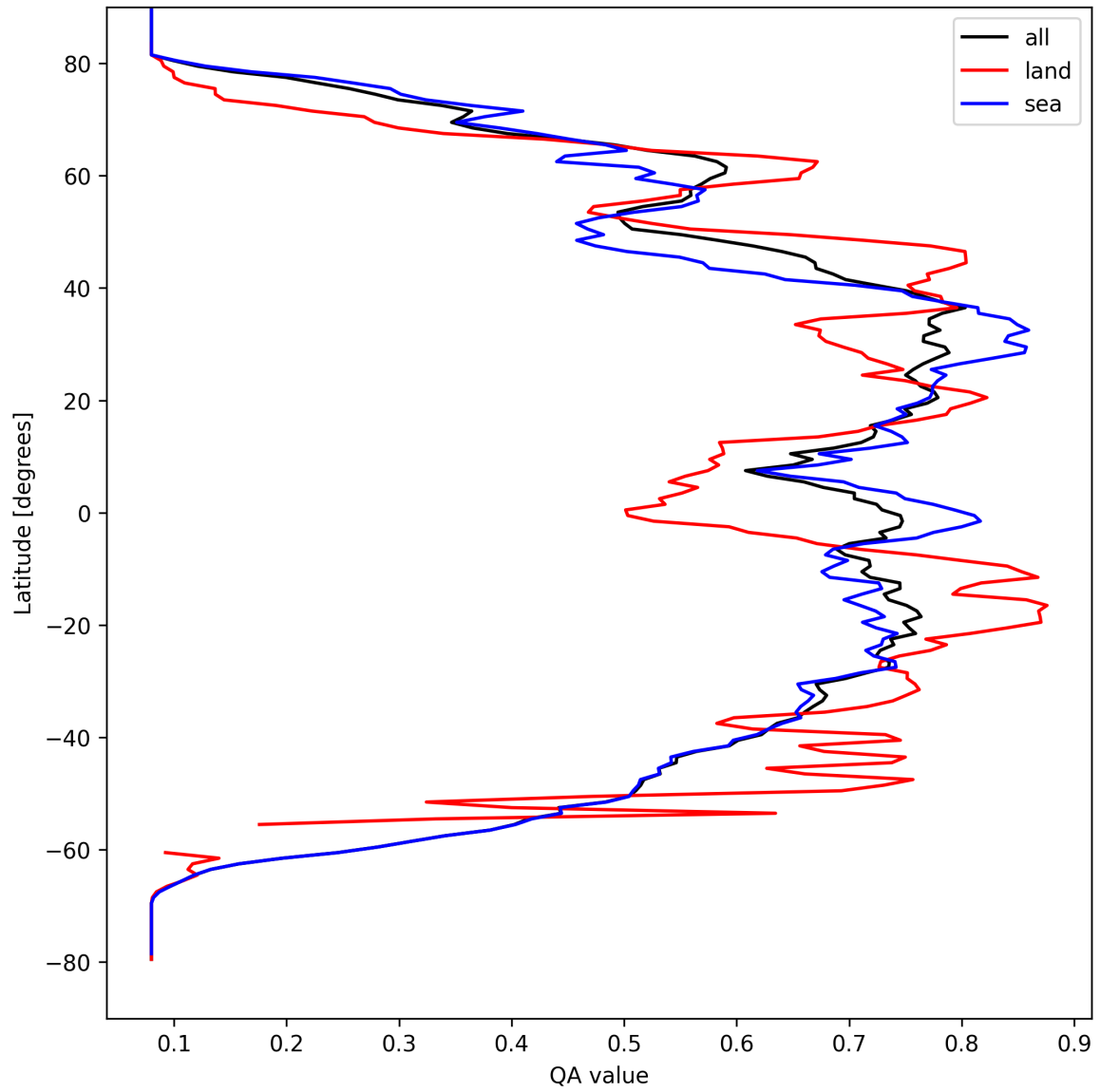
Figure 18: Zonal average of “QA value” for 2025-09-07 to 2025-09-07.
