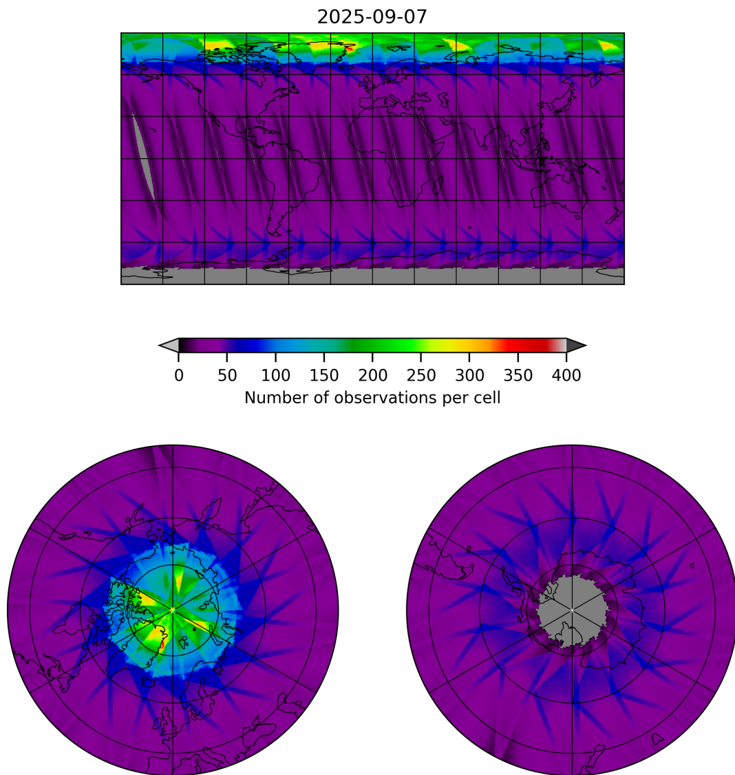
Figure 17: Map of the number of observations for 2025-09-07 to 2025-09-07
