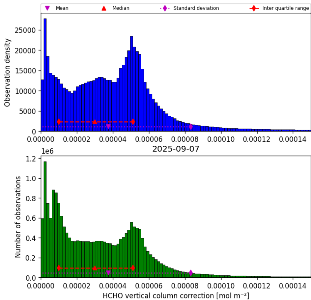
Figure 35: Histogram of “HCHO vertical column correction” for 2025-09-07 to 2025-09-07
