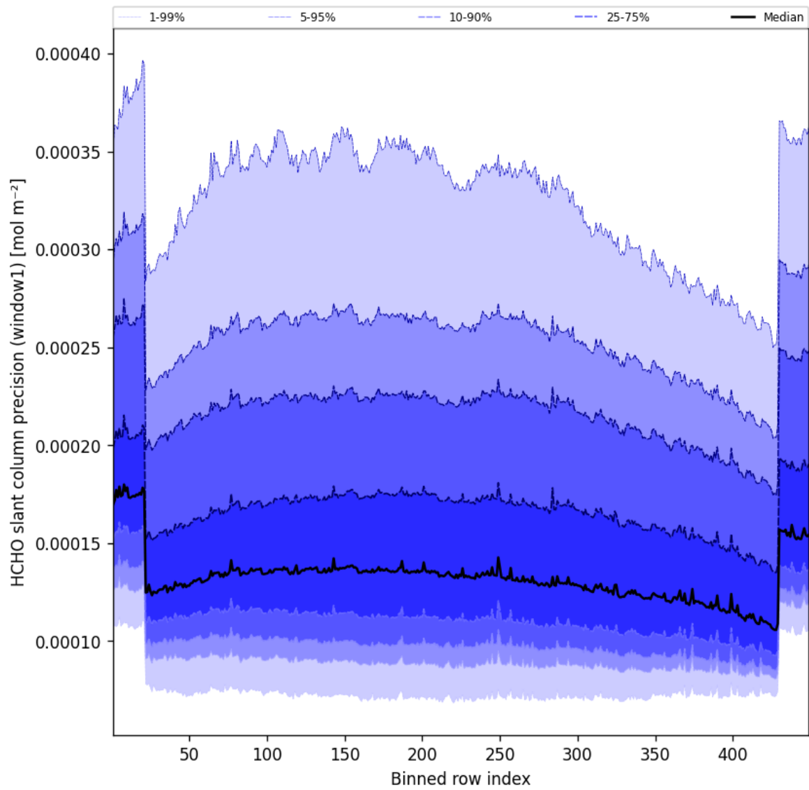
Figure 51: Along track statistics of “HCHO slant column precision (window1)” for 2025-09-07 to 2025-09-07
