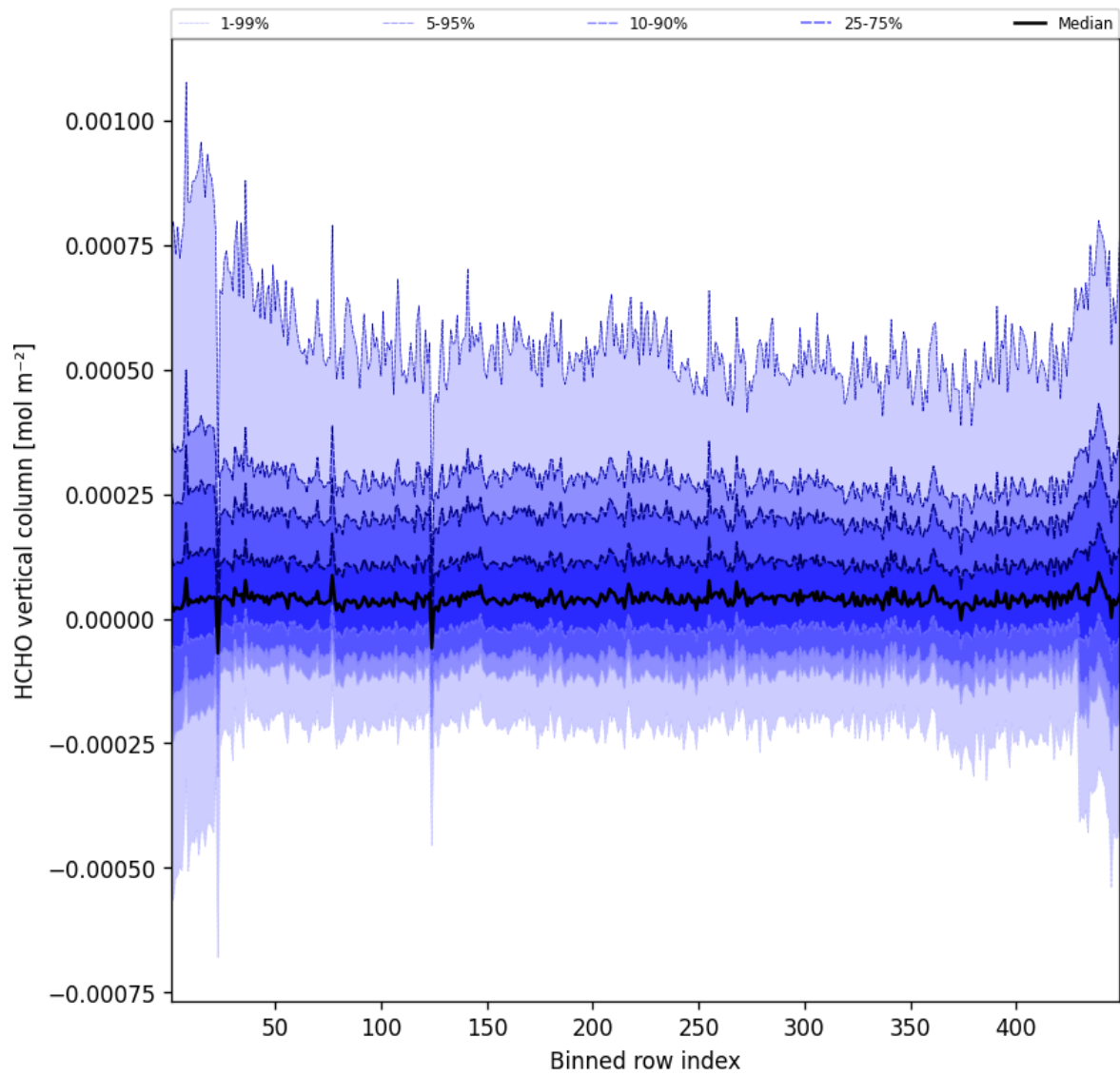
Figure 47: Along track statistics of “HCHO vertical column” for 2025-09-07 to 2025-09-07
