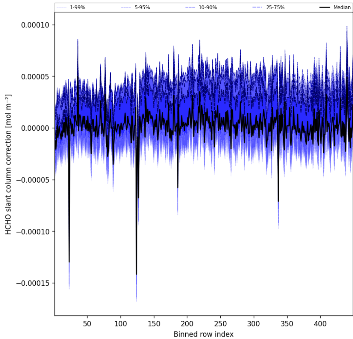
Figure 59: Along track statistics of “HCHO slant column correction” for 2025-09-07 to 2025-09-07
