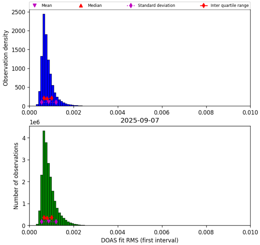
Figure 44: Histogram of “DOAS fit RMS (first interval)” for 2025-09-07 to 2025-09-07
