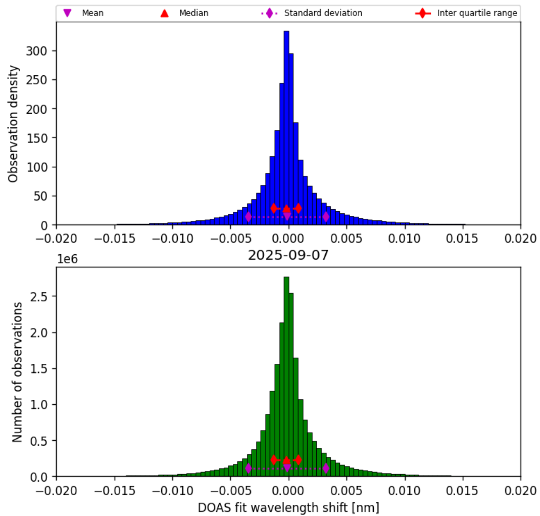
Figure 42: Histogram of “DOAS fit wavelength shift” for 2025-09-07 to 2025-09-07
