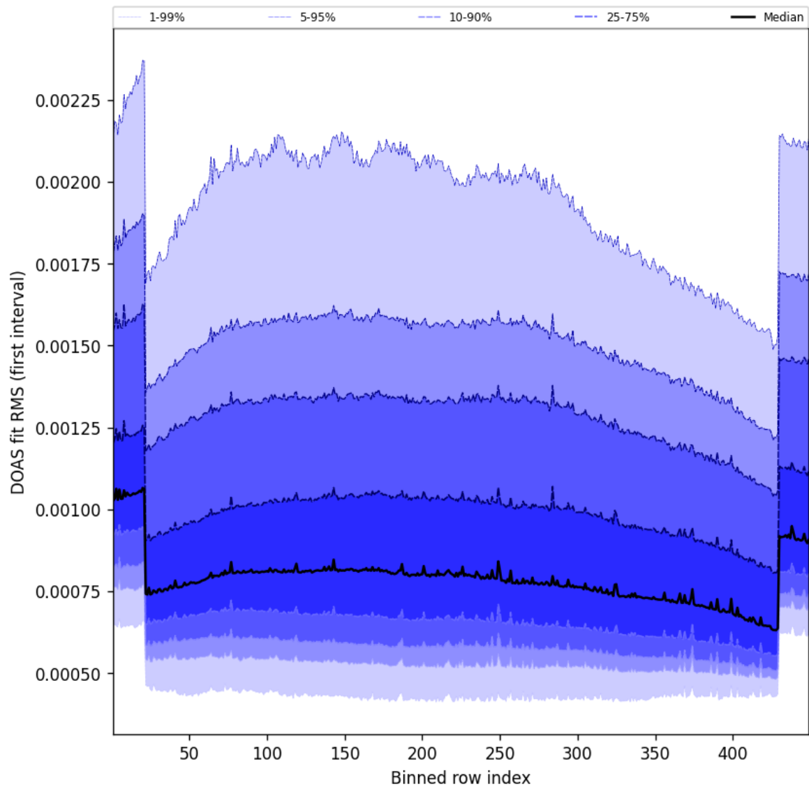
Figure 58: Along track statistics of “DOAS fit RMS (first interval)” for 2025-09-07 to 2025-09-07
