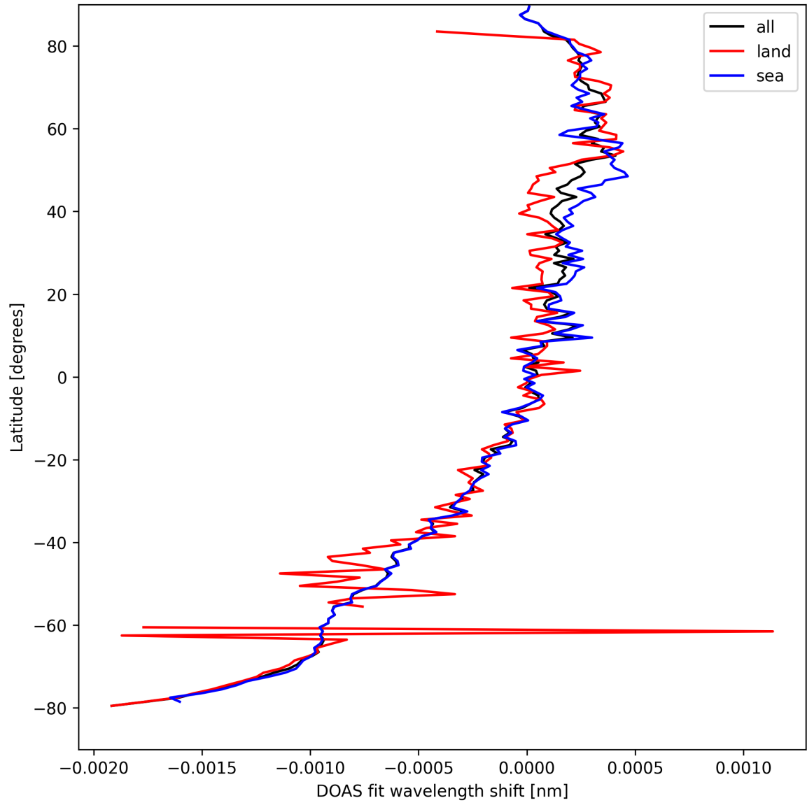
Figure 28: Zonal average of “DOAS fit wavelength shift” for 2025-09-08 to 2025-09-08.
