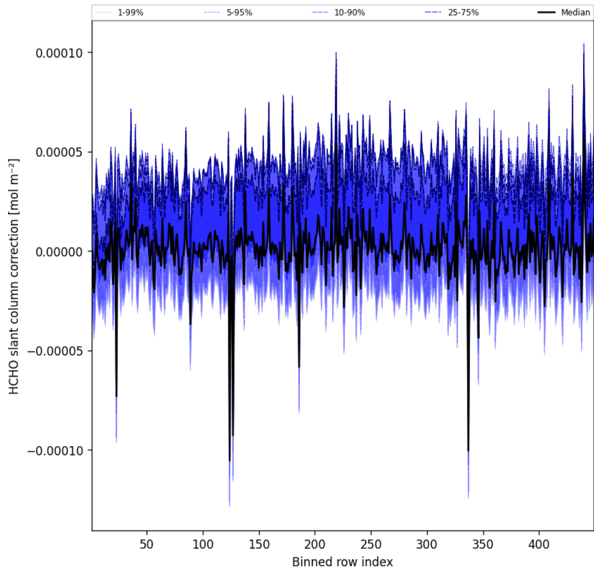
Figure 59: Along track statistics of “HCHO slant column correction” for 2025-09-08 to 2025-09-08
