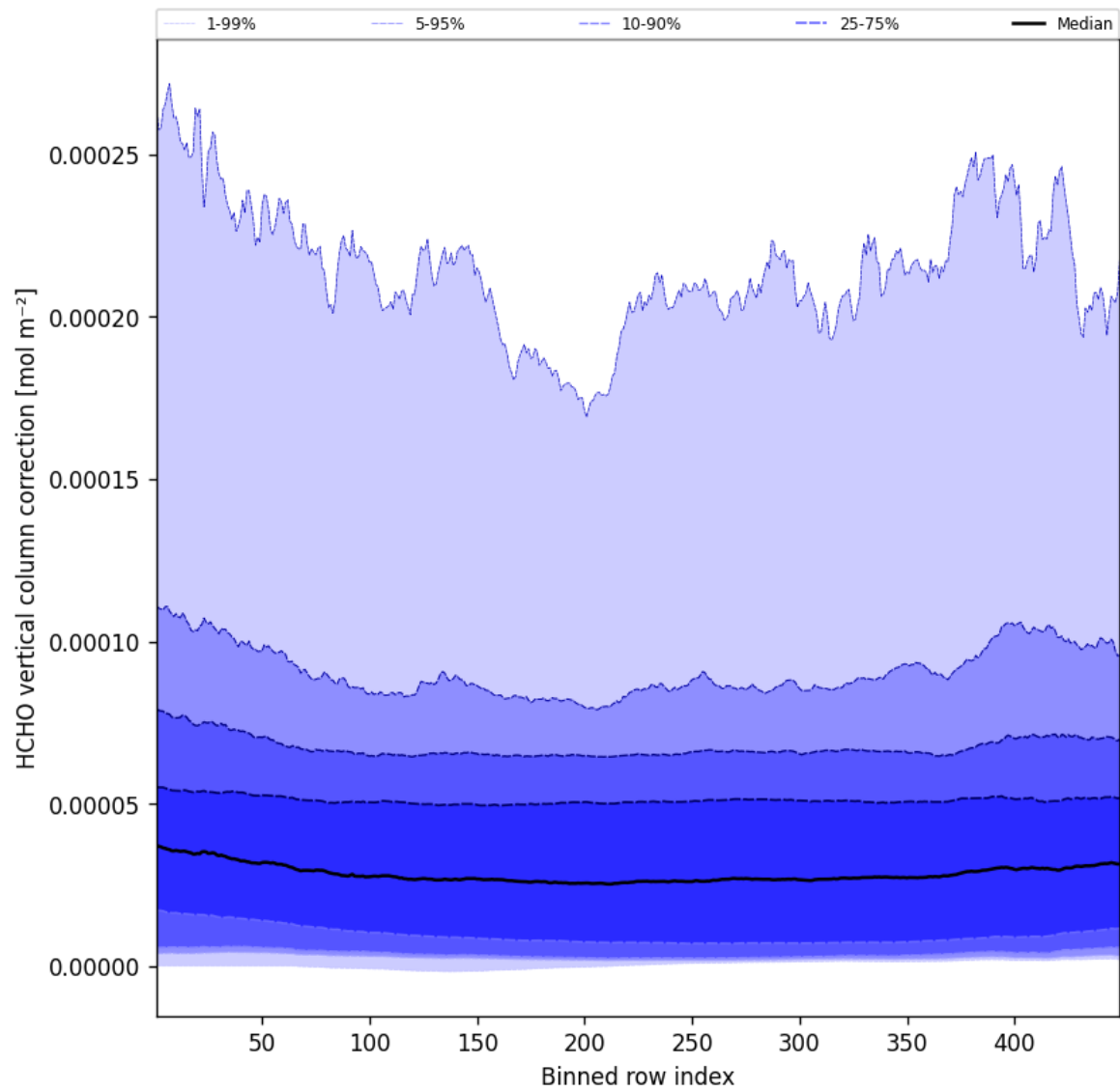
Figure 49: Along track statistics of “HCHO vertical column correction” for 2025-09-08 to 2025-09-08
