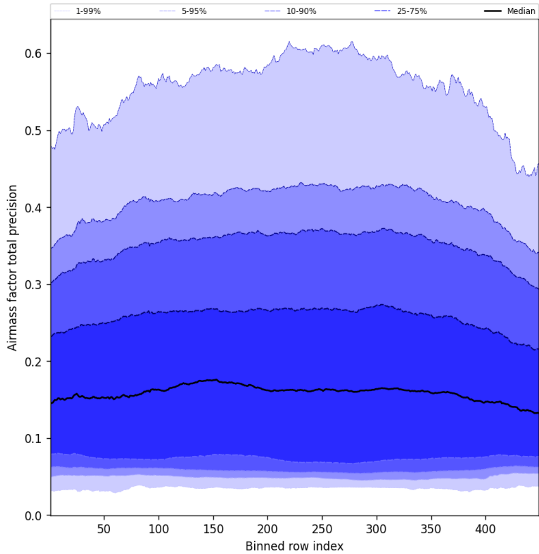
Figure 53: Along track statistics of “Airmass factor total precision” for 2025-09-08 to 2025-09-08
