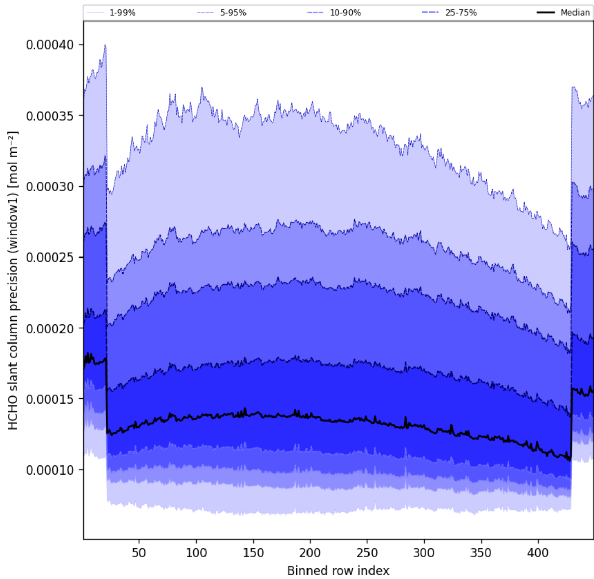
Figure 51: Along track statistics of “HCHO slant column precision (window1)” for 2025-09-08 to 2025-09-08
