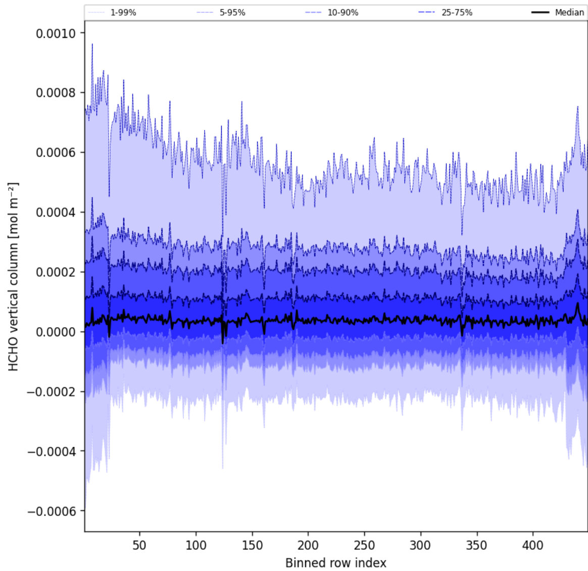
Figure 47: Along track statistics of “HCHO vertical column” for 2025-09-08 to 2025-09-08
