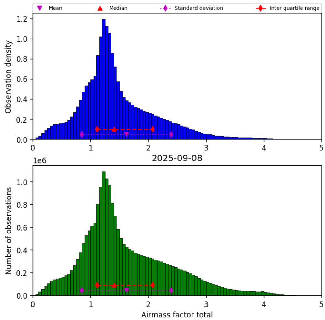
Figure 38: Histogram of “Airmass factor total” for 2025-09-08 to 2025-09-08
