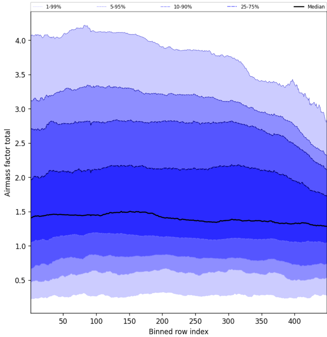
Figure 52: Along track statistics of “Airmass factor total” for 2025-09-08 to 2025-09-08
