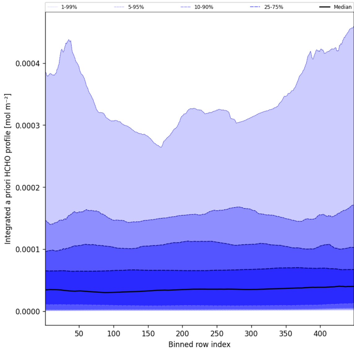
Figure 55: Along track statistics of "Integrated a priori HCHO profile" for 2025-09-08 to 2025-09-08
