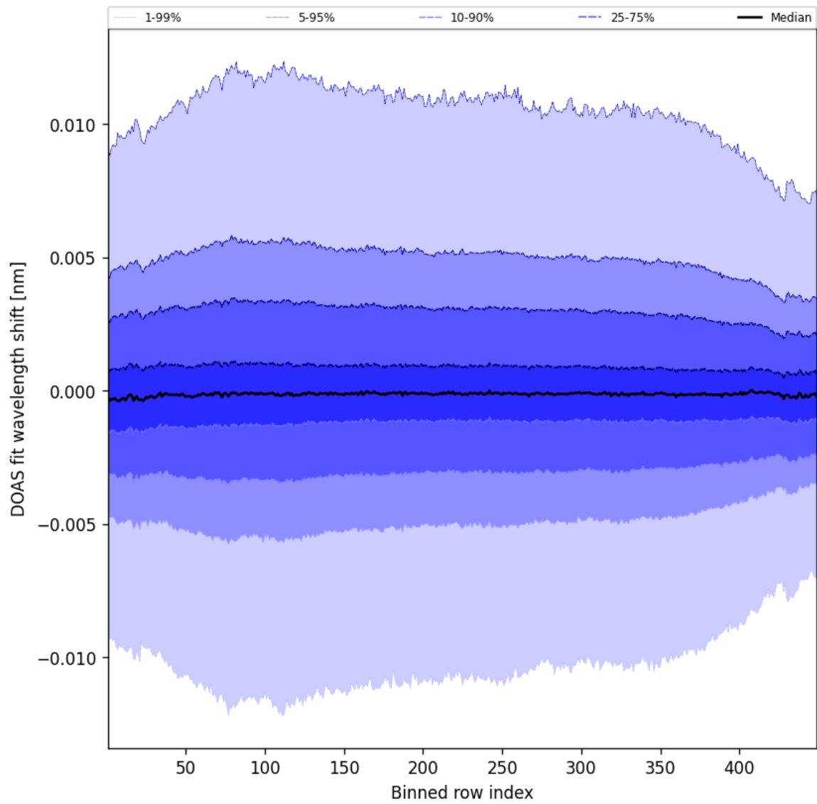
Figure 56: Along track statistics of “DOAS fit wavelength shift” for 2025-09-08 to 2025-09-08
