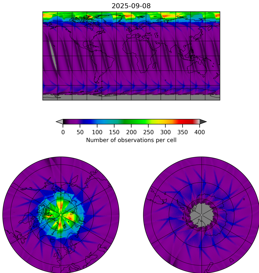
Figure 17: Map of the number of observations for 2025-09-08 to 2025-09-08
