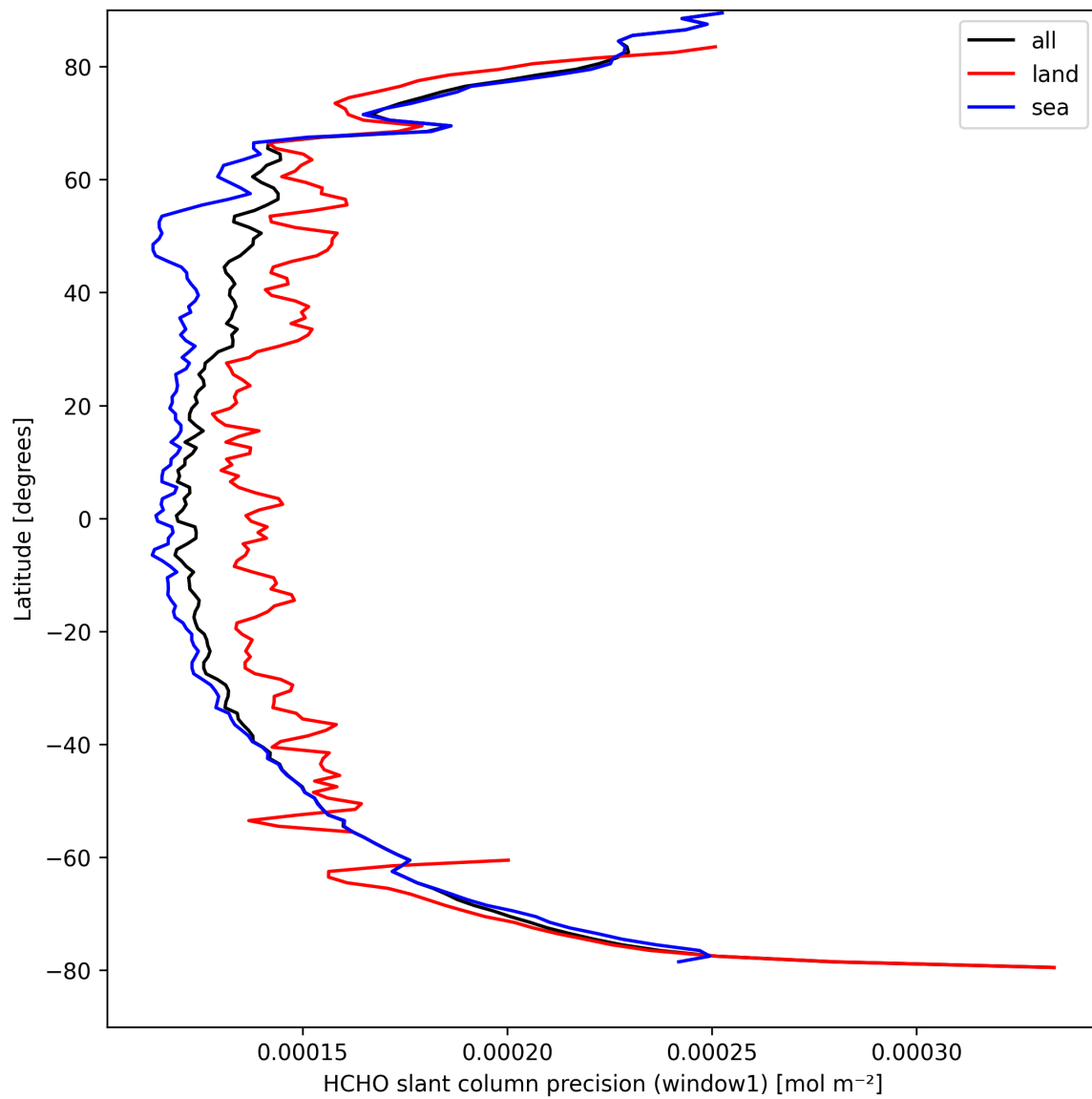
Figure 23: Zonal average of “HCHO slant column precision (window1)” for 2025-09-08 to 2025-09-08.
