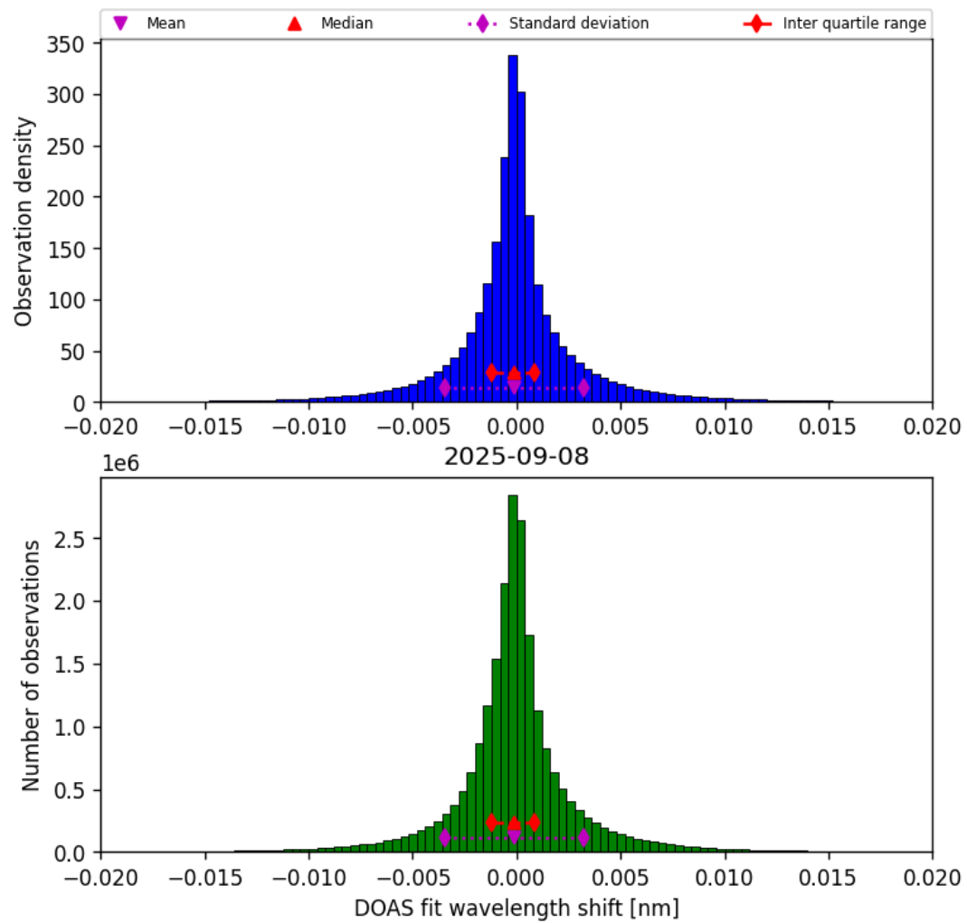
Figure 42: Histogram of “DOAS fit wavelength shift” for 2025-09-08 to 2025-09-08
