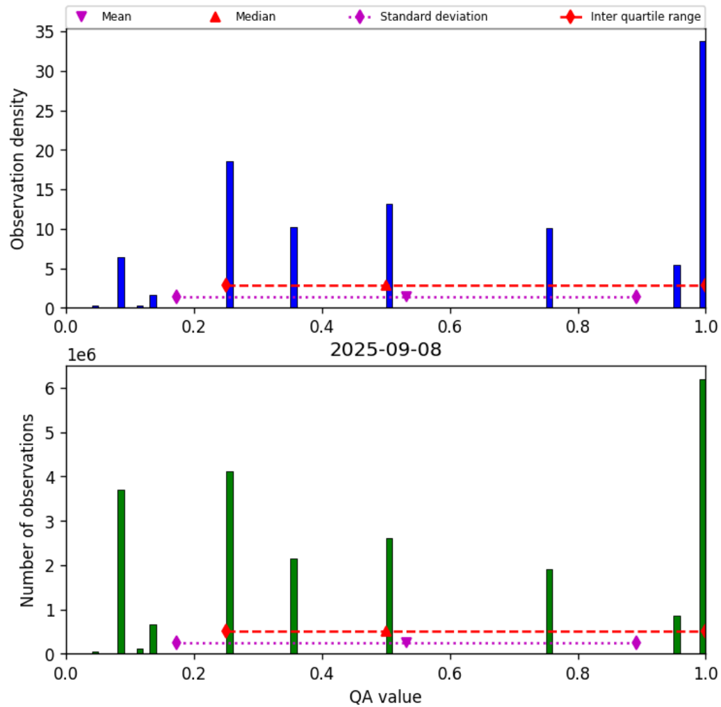
Figure 32: Histogram of “QA value” for 2025-09-08 to 2025-09-08
