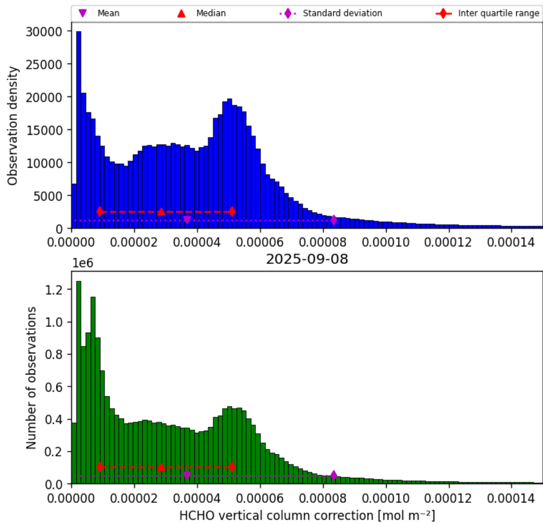
Figure 35: Histogram of “HCHO vertical column correction” for 2025-09-08 to 2025-09-08
