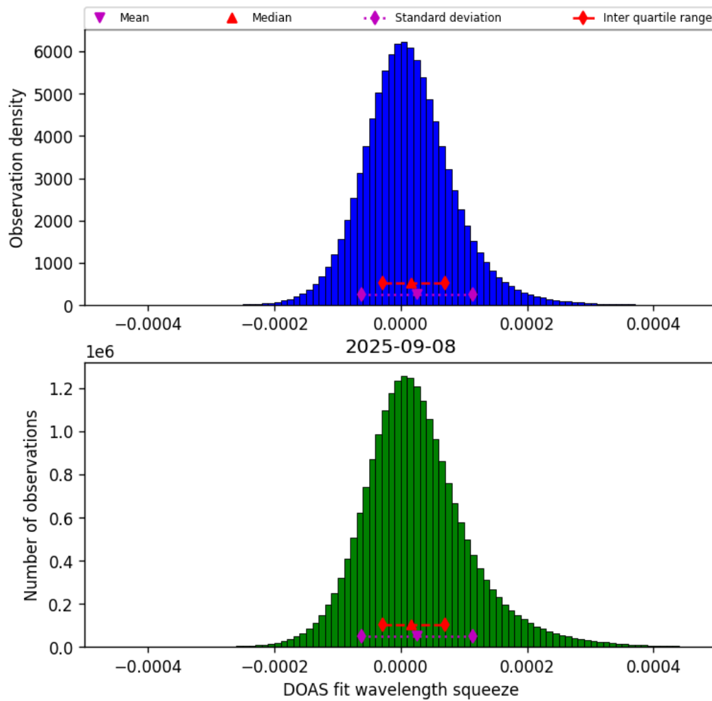
Figure 43: Histogram of “DOAS fit wavelength squeeze” for 2025-09-08 to 2025-09-08
