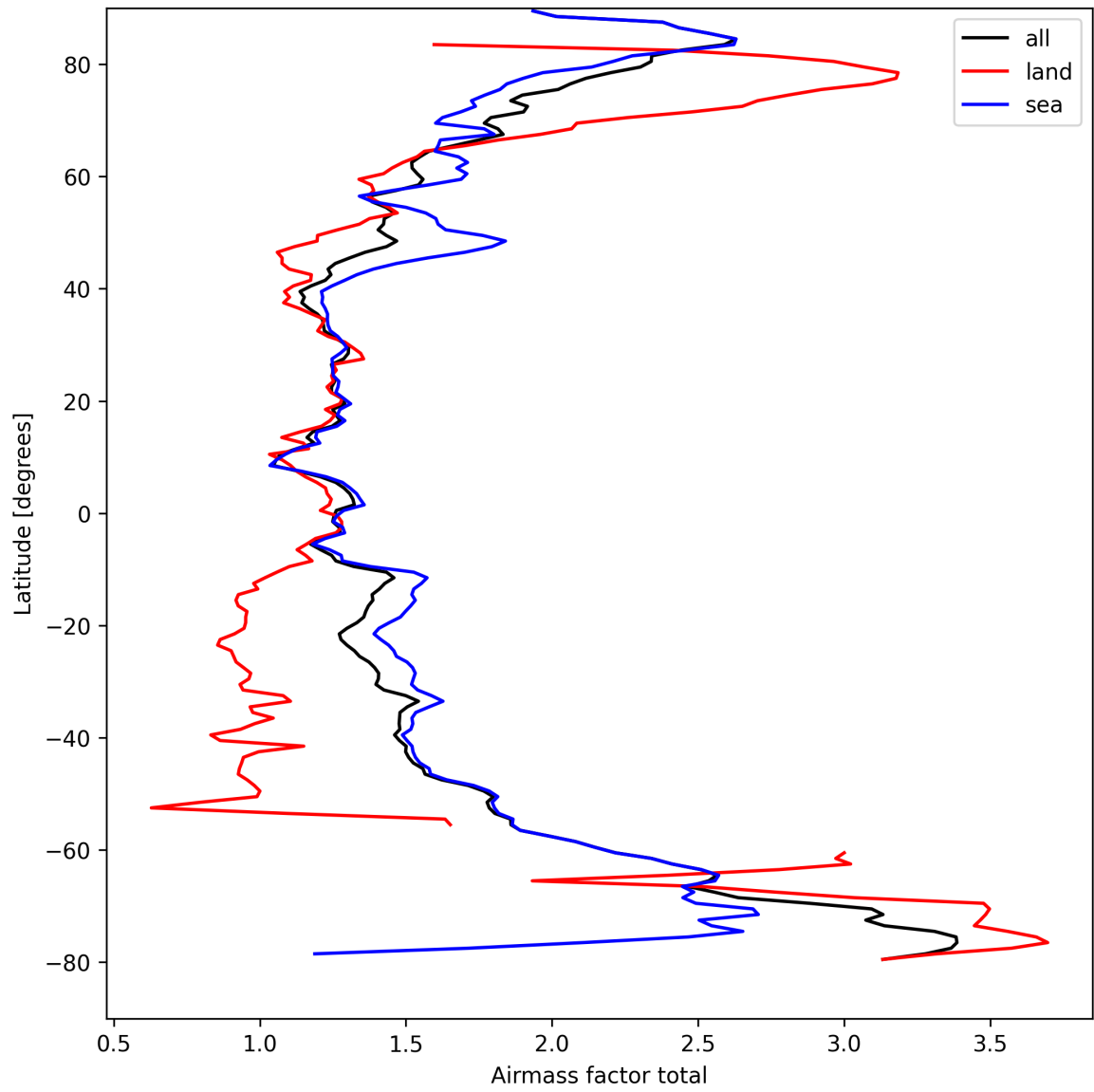
Figure 24: Zonal average of “Airmass factor total” for 2025-09-08 to 2025-09-08.
