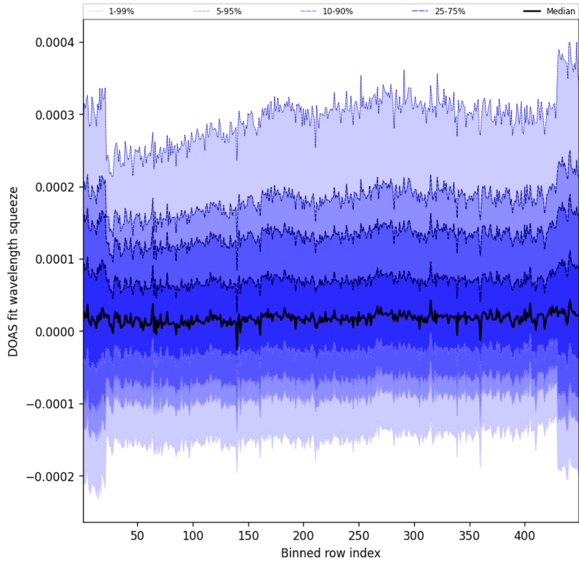
Figure 57: Along track statistics of “DOAS fit wavelength squeeze” for 2025-09-08 to 2025-09-08
