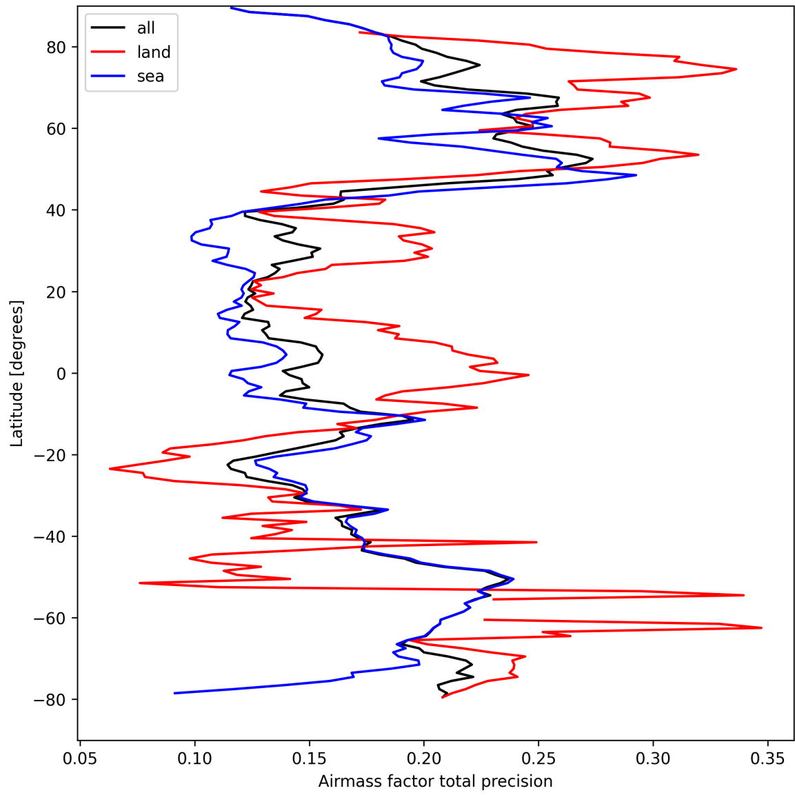
Figure 25: Zonal average of “Airmass factor total precision” for 2025-09-08 to 2025-09-08.
