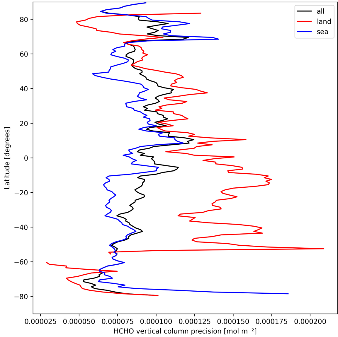
Figure 20: Zonal average of “HCHO vertical column precision” for 2025-09-08 to 2025-09-08.
