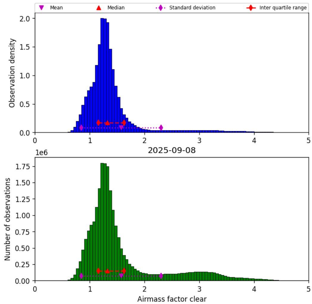
Figure 40: Histogram of “Airmass factor clear” for 2025-09-08 to 2025-09-08
