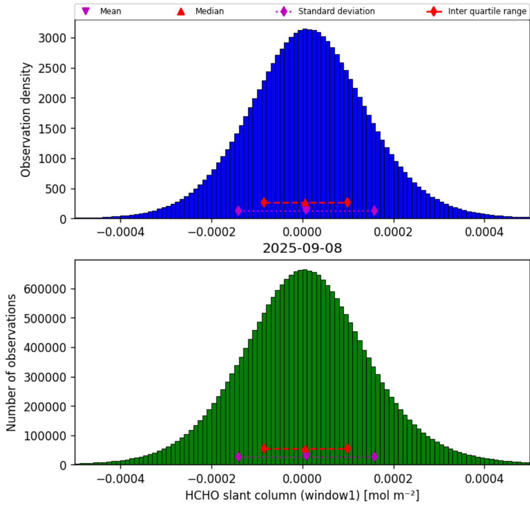
Figure 36: Histogram of “HCHO slant column (window1)” for 2025-09-08 to 2025-09-08
