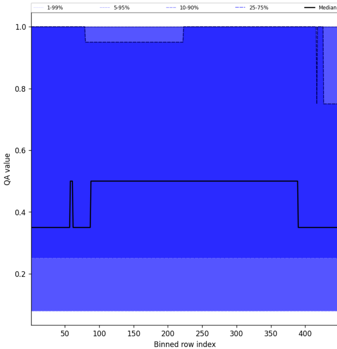
Figure 46: Along track statistics of “QA value” for 2025-09-08 to 2025-09-08
