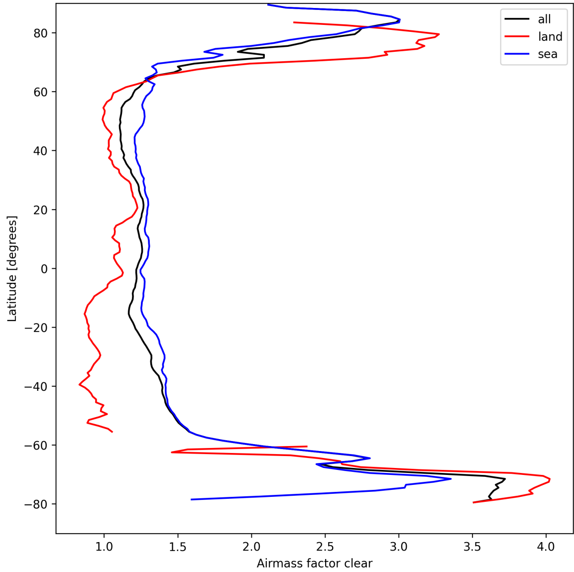
Figure 26: Zonal average of “Airmass factor clear” for 2025-09-08 to 2025-09-08.
