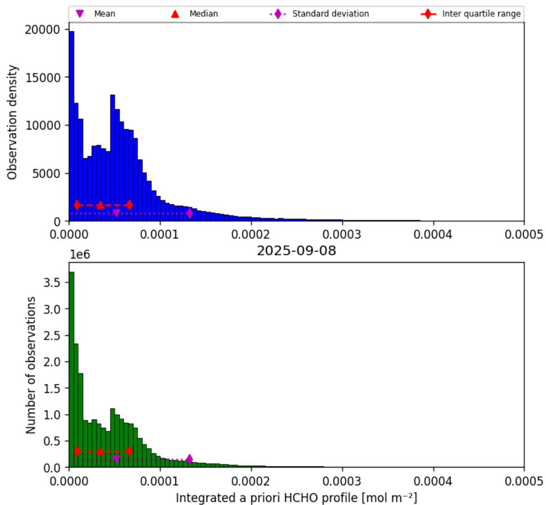
Figure 41: Histogram of “Integrated a priori HCHO profile” for 2025-09-08 to 2025-09-08
