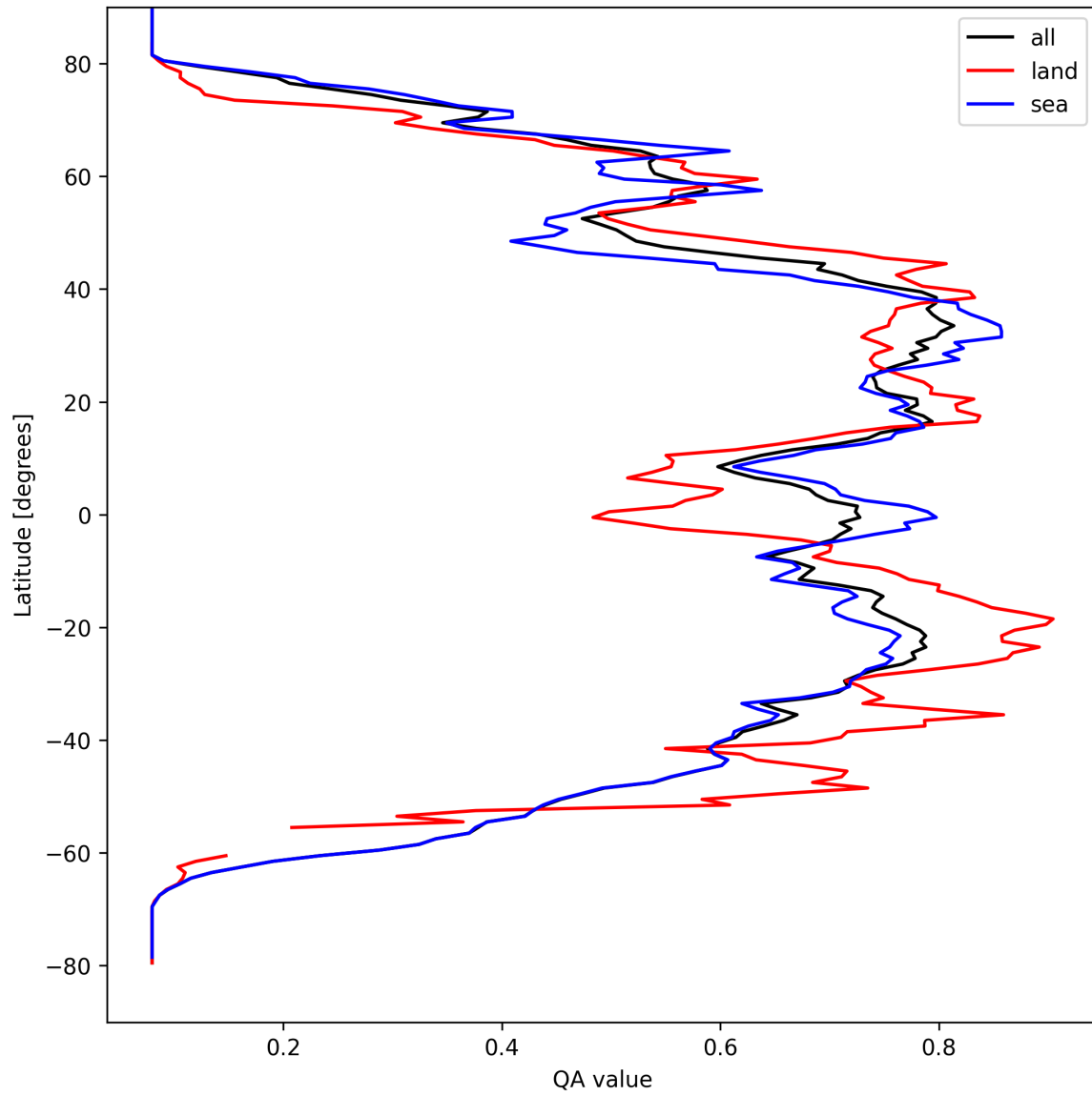
Figure 18: Zonal average of “QA value” for 2025-09-08 to 2025-09-08.
