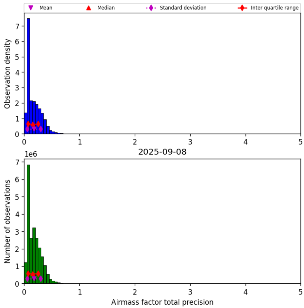
Figure 39: Histogram of “Airmass factor total precision” for 2025-09-08 to 2025-09-08
