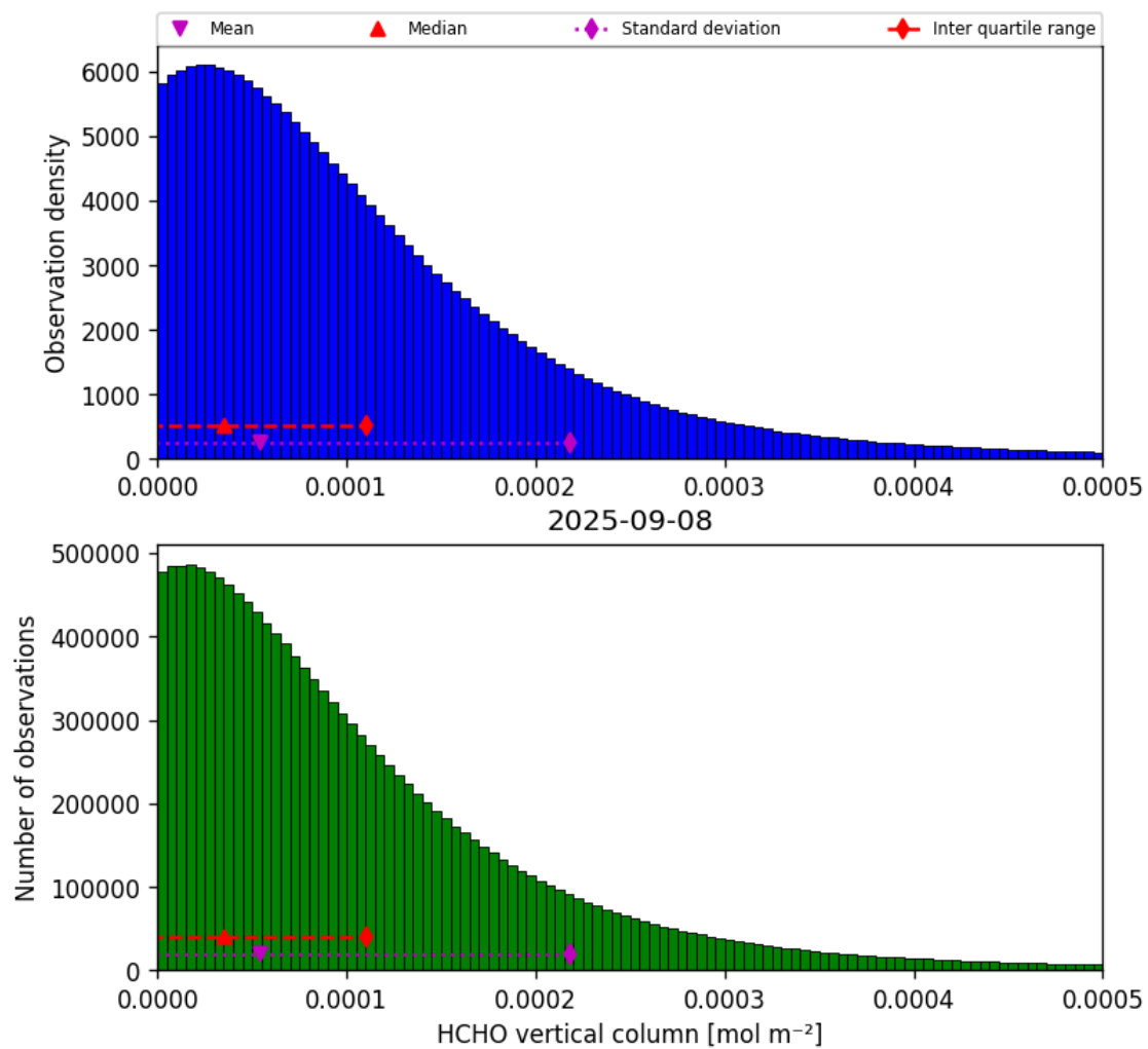
Figure 33: Histogram of “HCHO vertical column” for 2025-09-08 to 2025-09-08
