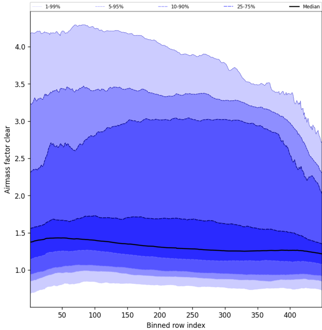
Figure 54: Along track statistics of “Airmass factor clear” for 2025-09-08 to 2025-09-08
