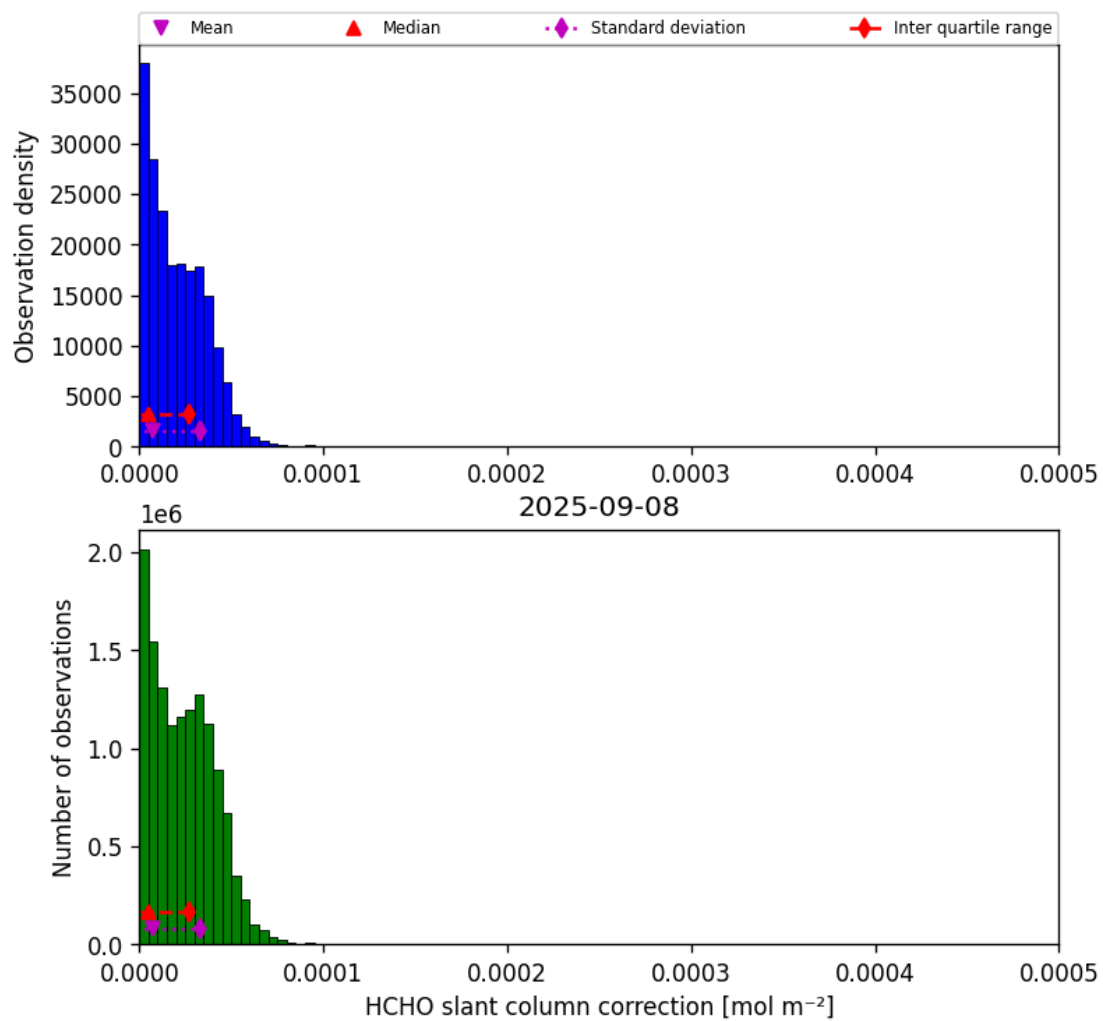
Figure 45: Histogram of “HCHO slant column correction” for 2025-09-08 to 2025-09-08
