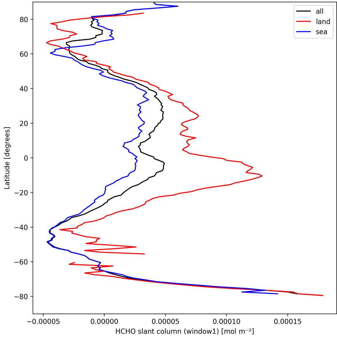
Figure 22: Zonal average of “HCHO slant column (window1)” for 2025-09-08 to 2025-09-08.
