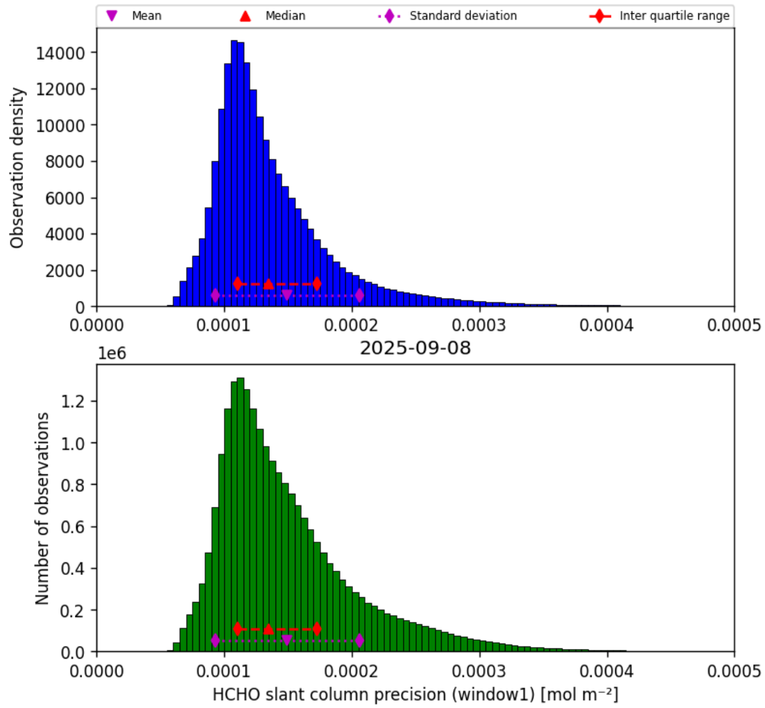
Figure 37: Histogram of “HCHO slant column precision (window1)” for 2025-09-08 to 2025-09-08
