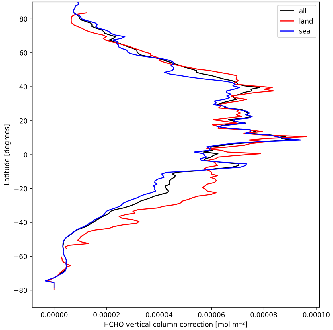
Figure 21: Zonal average of "HCHO vertical column correction" for 2025-09-08 to 2025-09-08.
