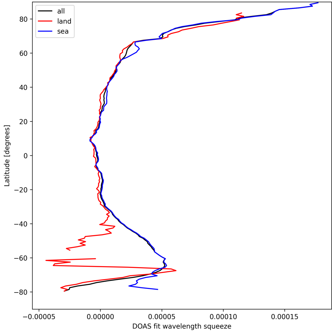
Figure 29: Zonal average of “DOAS fit wavelength squeeze” for 2025-09-08 to 2025-09-08.
