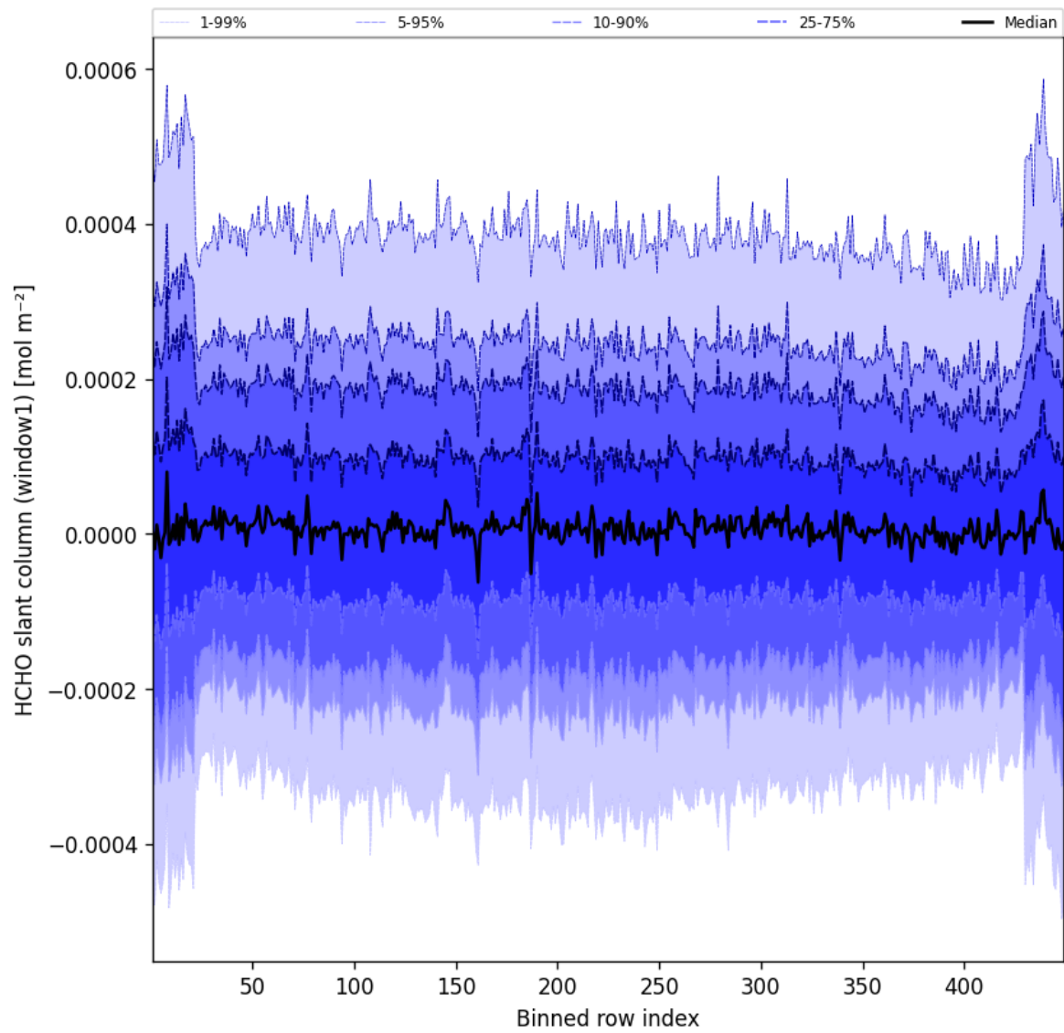
Figure 50: Along track statistics of “HCHO slant column (window1)” for 2025-09-08 to 2025-09-08
