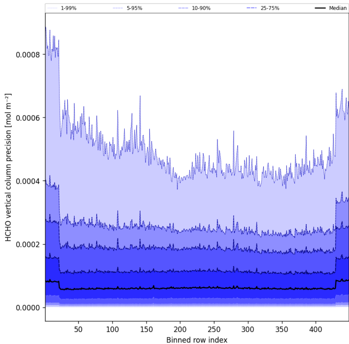
Figure 48: Along track statistics of “HCHO vertical column precision” for 2025-09-08 to 2025-09-08
