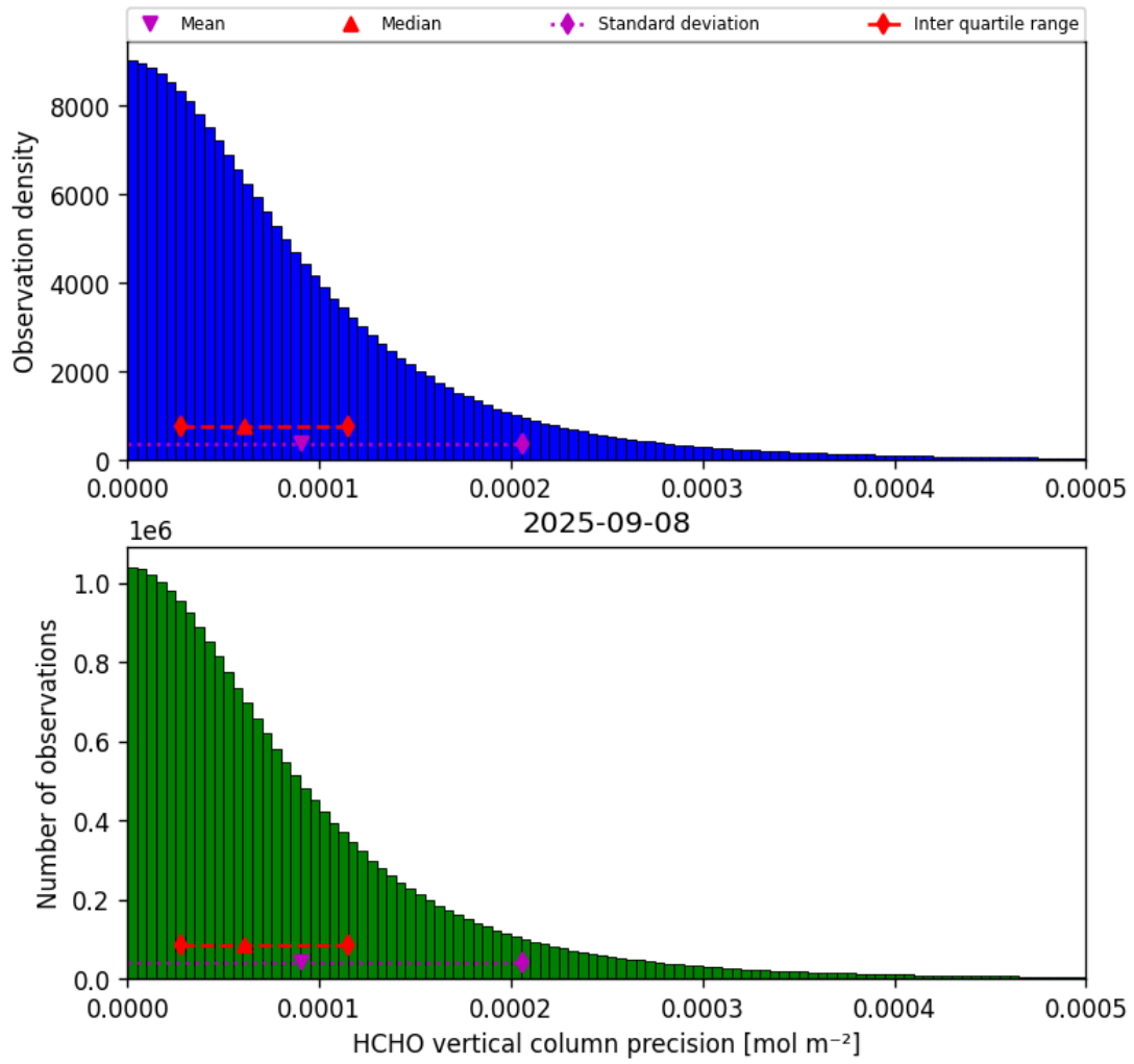
Figure 34: Histogram of “HCHO vertical column precision” for 2025-09-08 to 2025-09-08
