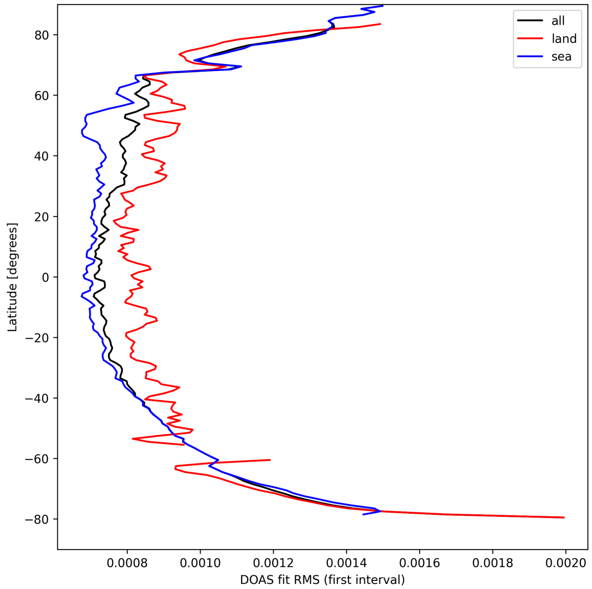
Figure 30: Zonal average of “DOAS fit RMS (first interval)” for 2025-09-08 to 2025-09-08.
