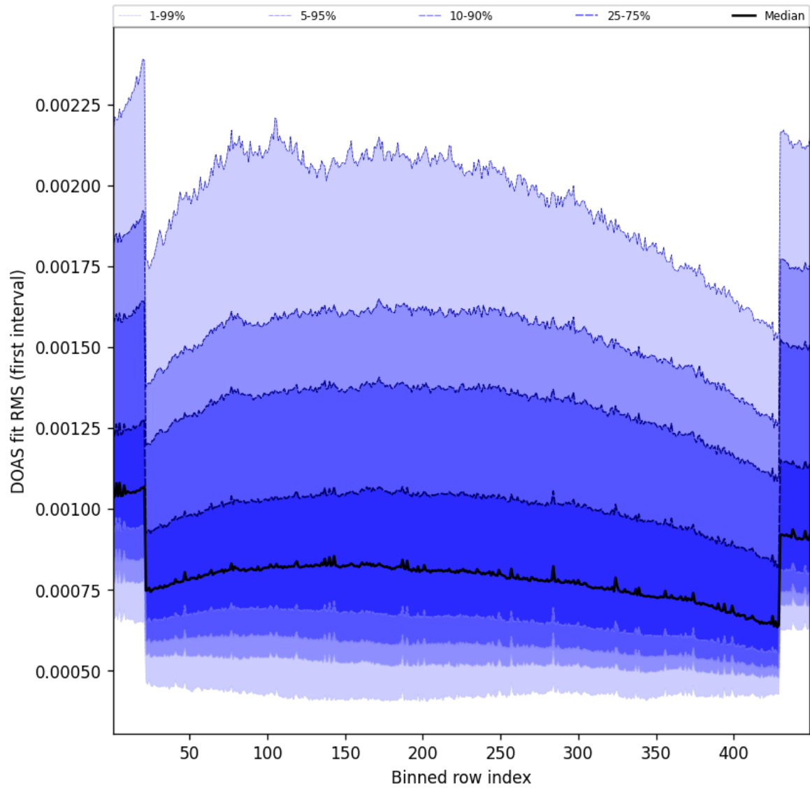
Figure 58: Along track statistics of “DOAS fit RMS (first interval)” for 2025-09-08 to 2025-09-08
