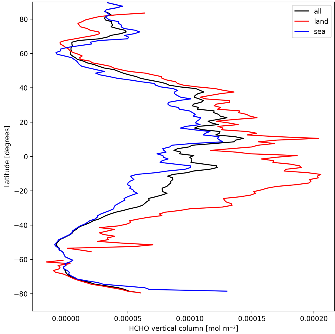
Figure 19: Zonal average of “HCHO vertical column” for 2025-09-08 to 2025-09-08.
