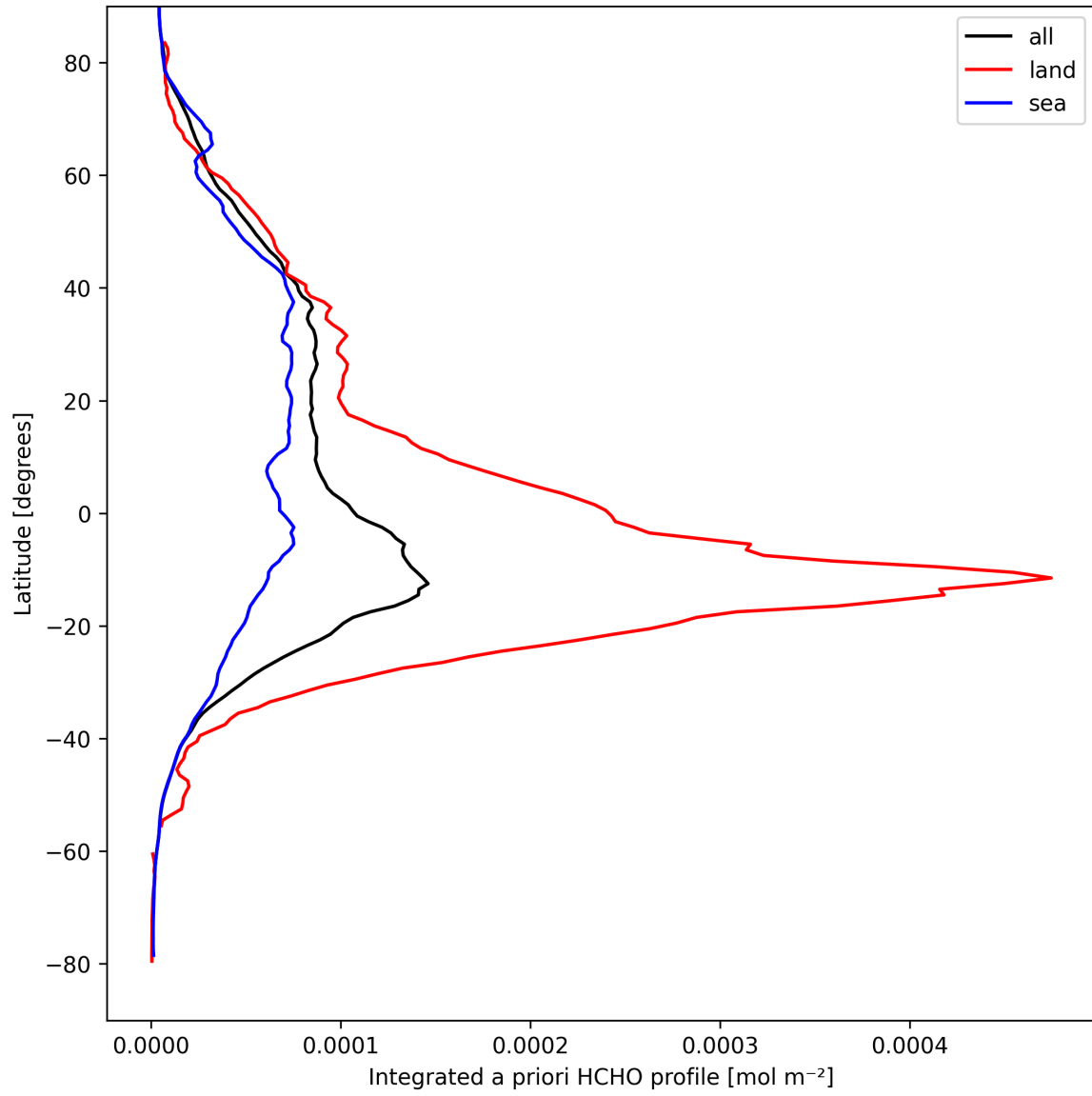
Figure 27: Zonal average of “Integrated a priori HCHO profile” for 2025-09-08 to 2025-09-08.
