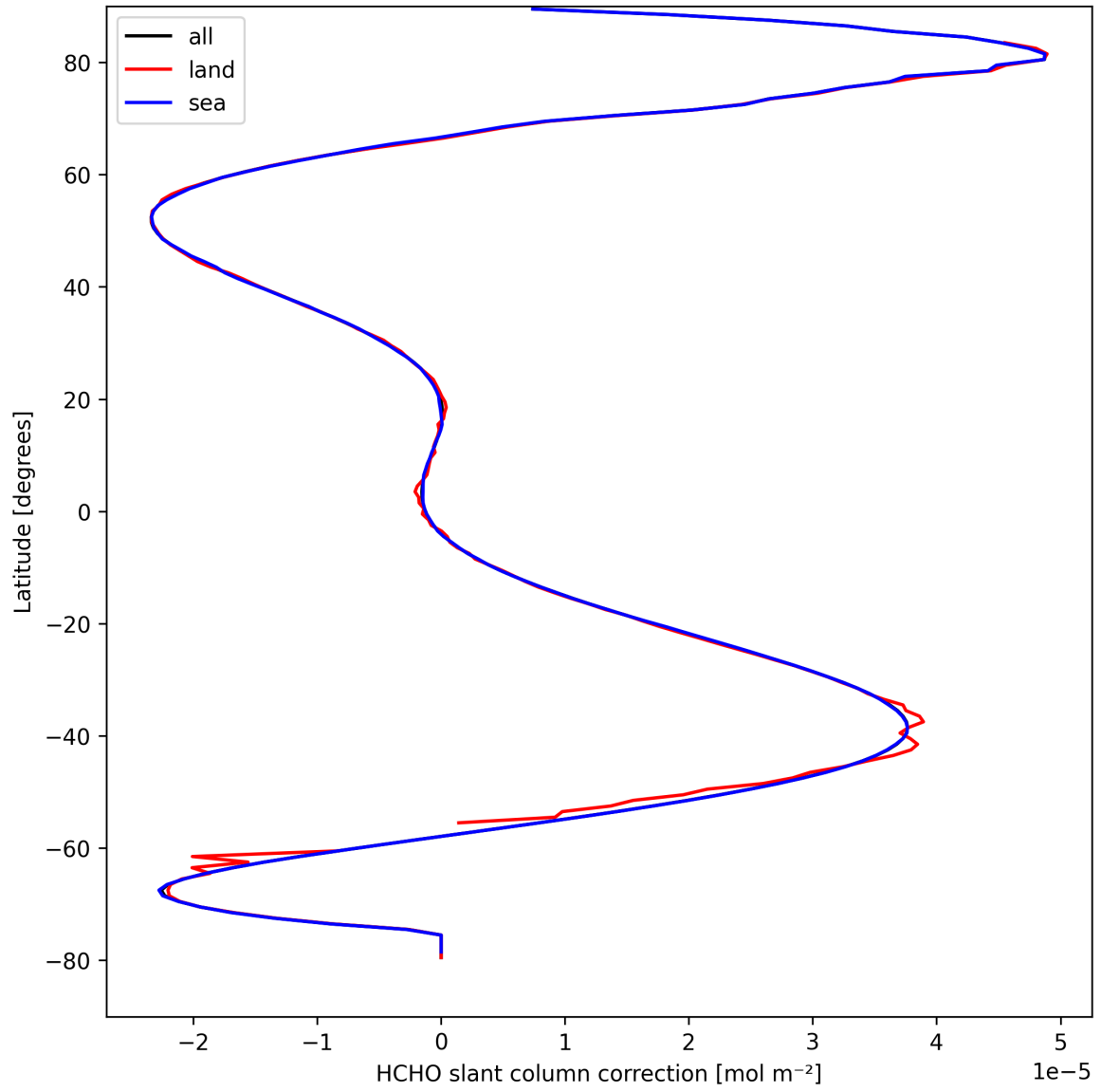
Figure 31: Zonal average of “HCHO slant column correction” for 2025-09-08 to 2025-09-08.
