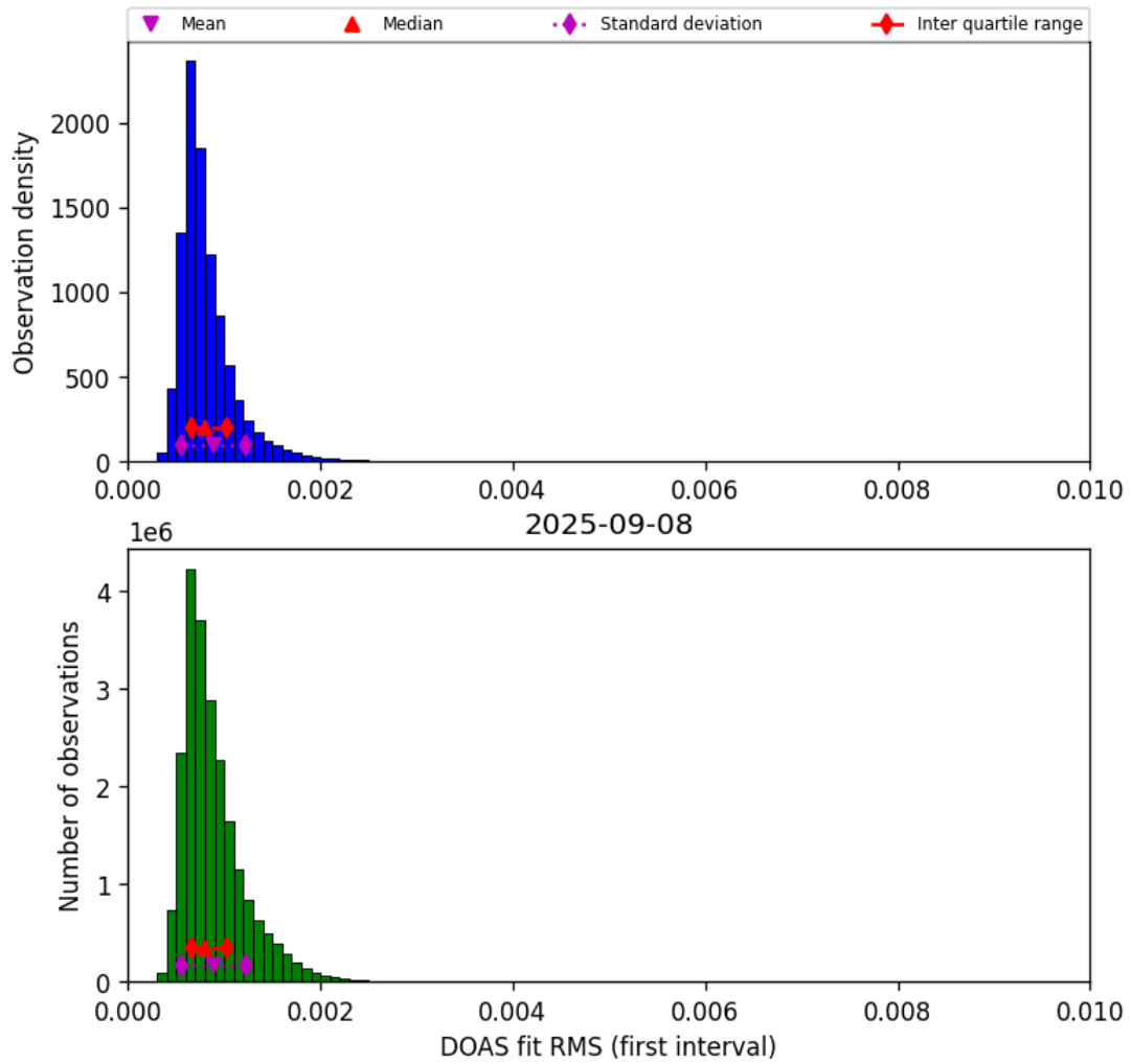
Figure 44: Histogram of “DOAS fit RMS (first interval)” for 2025-09-08 to 2025-09-08
