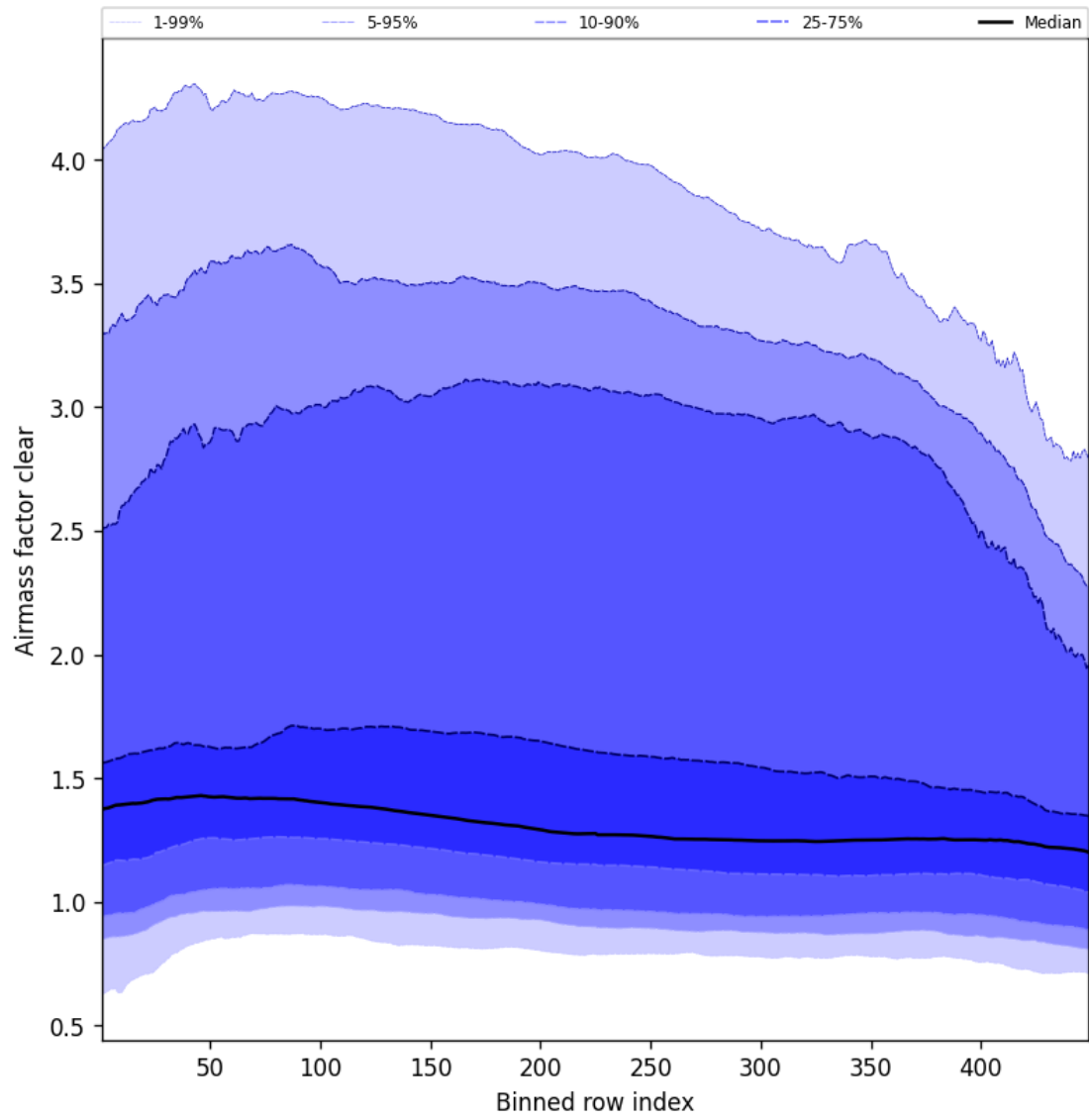
Figure 54: Along track statistics of “Airmass factor clear” for 2025-09-11 to 2025-09-12
