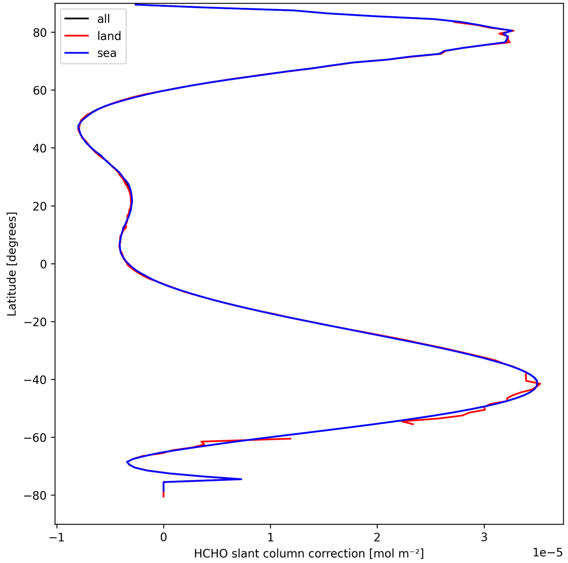
Figure 31: Zonal average of "HCHO slant column correction" for 2025-09-11 to 2025-09-12.
