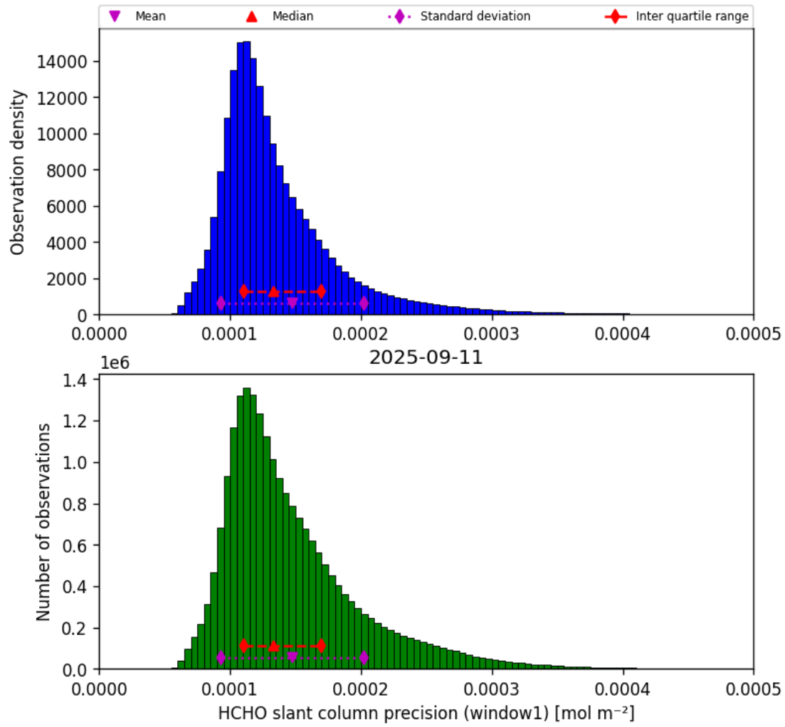
Figure 37: Histogram of “HCHO slant column precision (window1)” for 2025-09-11 to 2025-09-12
