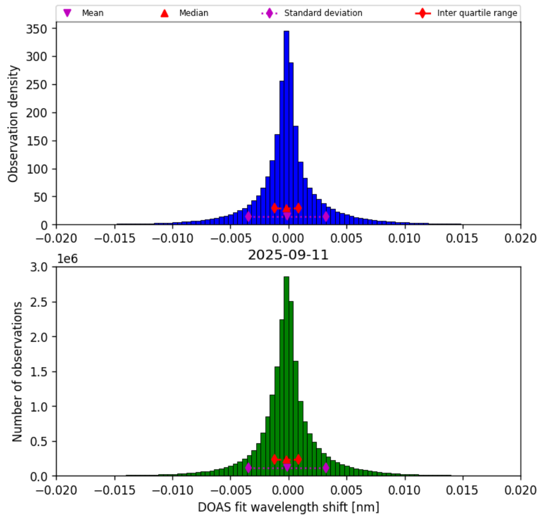
Figure 42: Histogram of “DOAS fit wavelength shift” for 2025-09-11 to 2025-09-12
