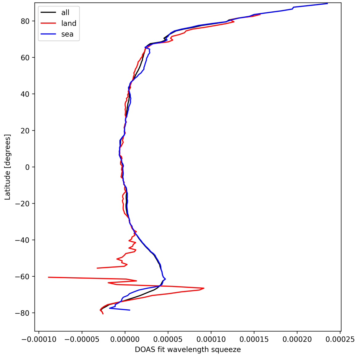
Figure 29: Zonal average of “DOAS fit wavelength squeeze” for 2025-09-11 to 2025-09-12.
