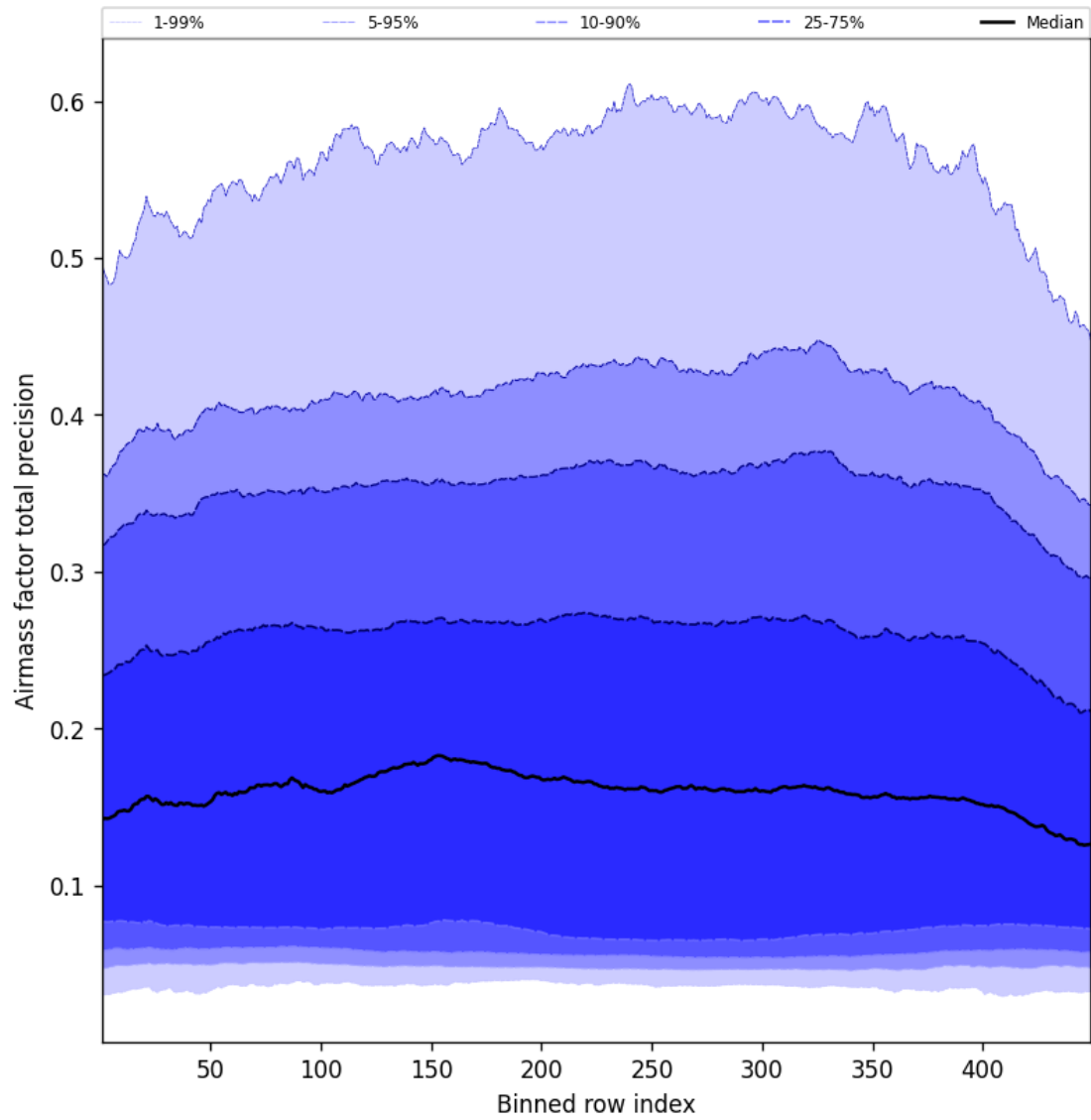
Figure 53: Along track statistics of “Airmass factor total precision” for 2025-09-11 to 2025-09-12
