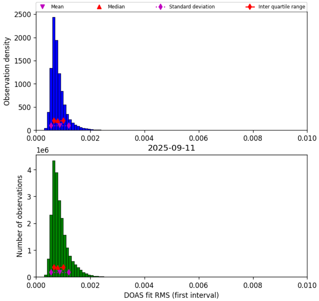
Figure 44: Histogram of “DOAS fit RMS (first interval)” for 2025-09-11 to 2025-09-12
