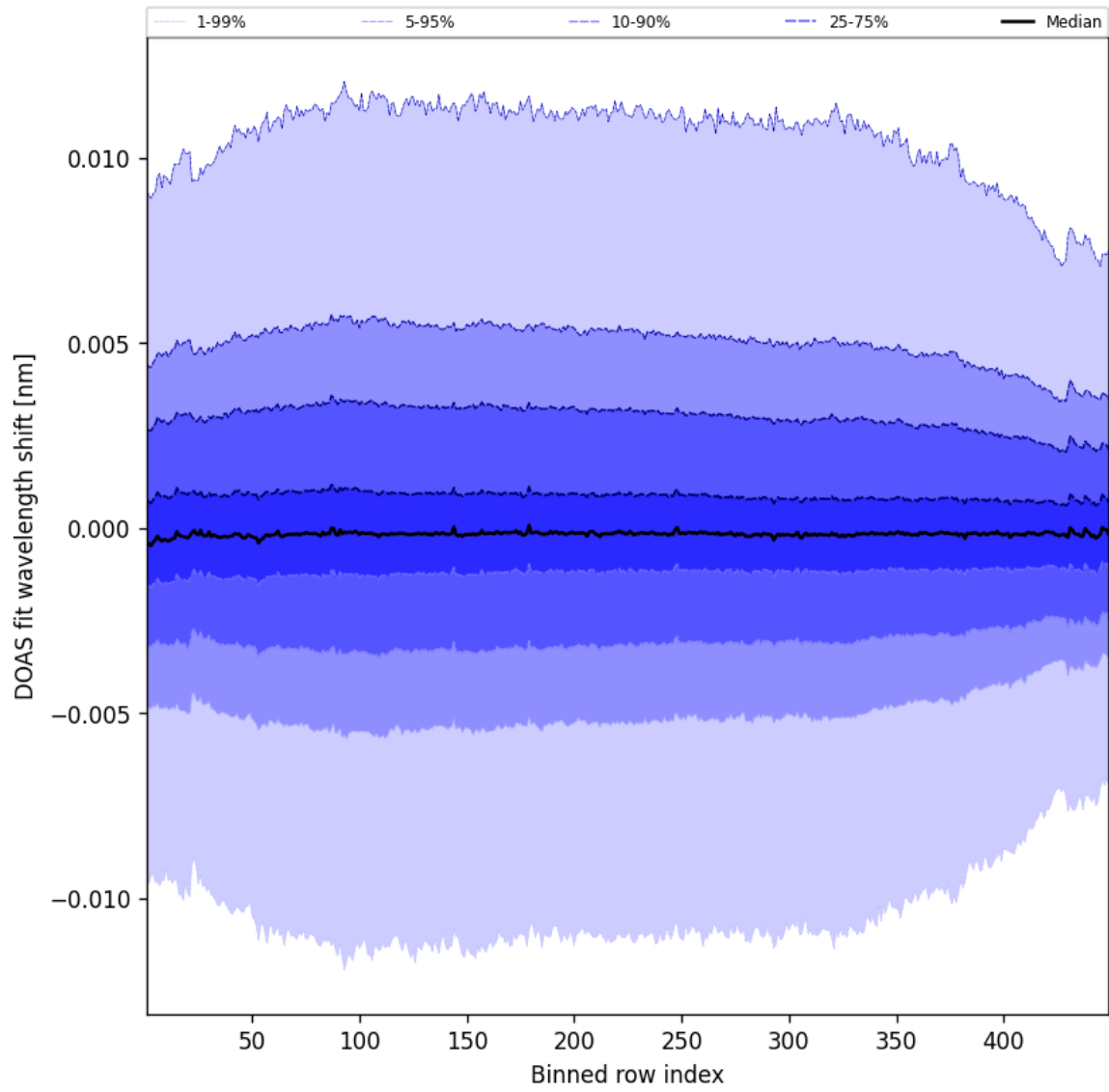
Figure 56: Along track statistics of “DOAS fit wavelength shift” for 2025-09-11 to 2025-09-12
