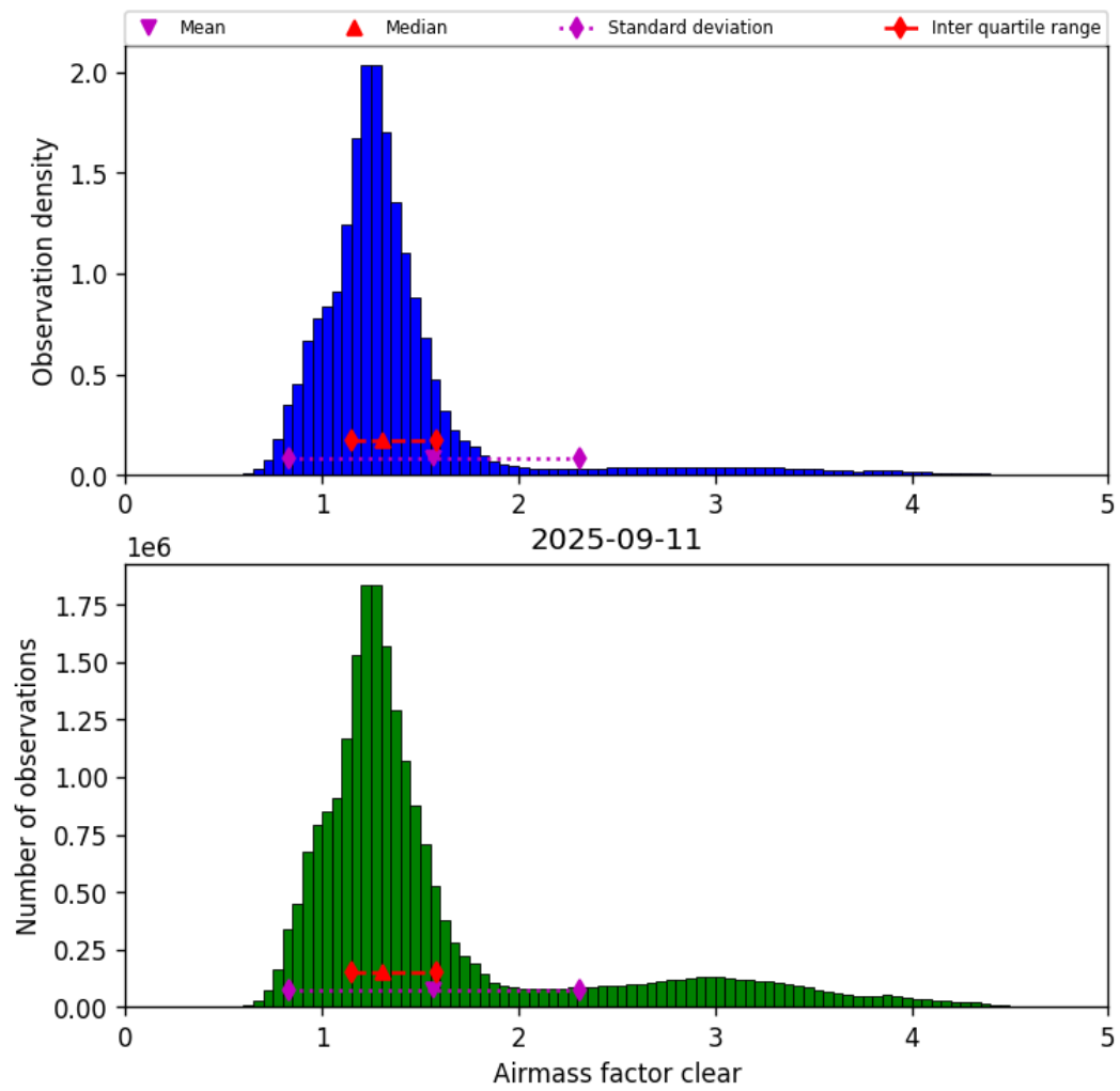
Figure 40: Histogram of “Airmass factor clear” for 2025-09-11 to 2025-09-12
