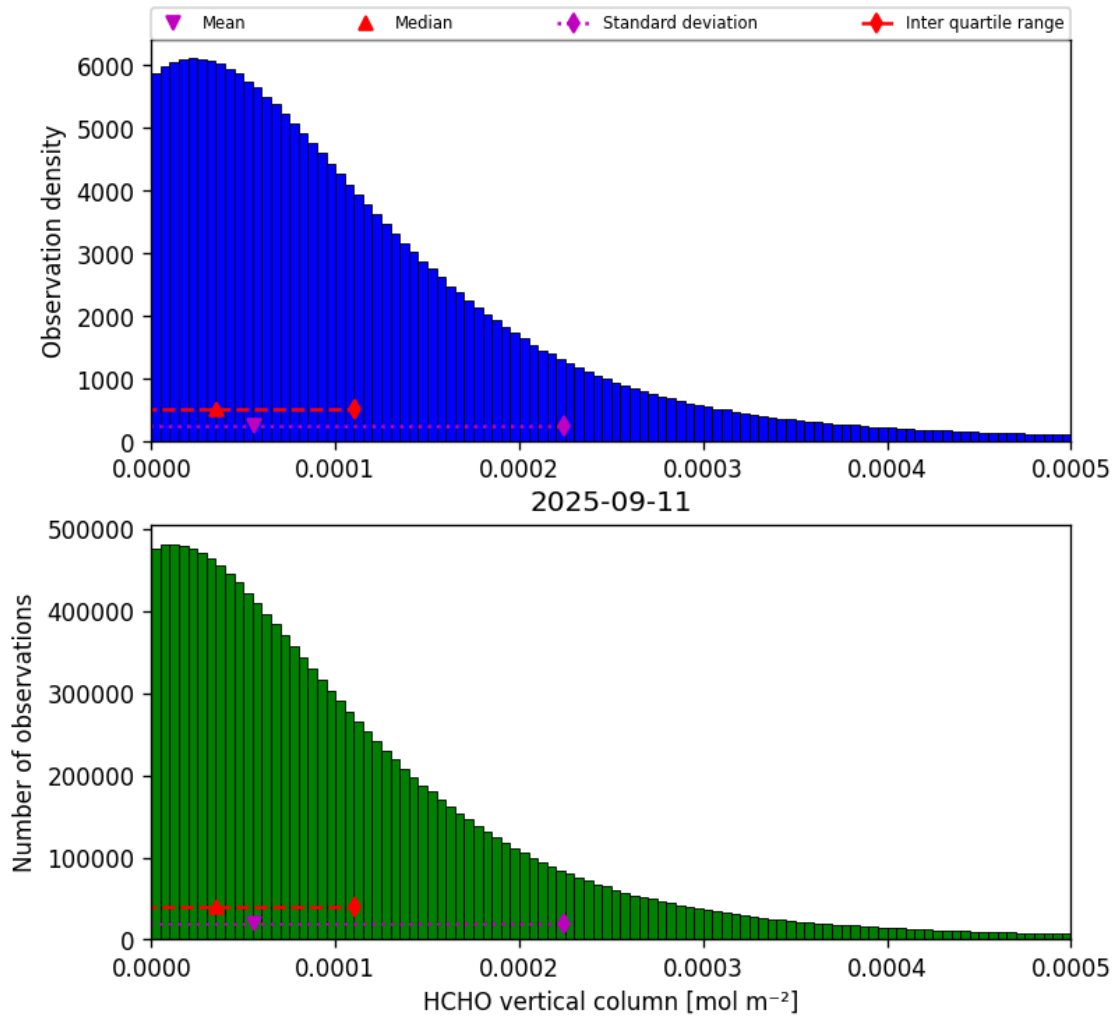
Figure 33: Histogram of “HCHO vertical column” for 2025-09-11 to 2025-09-12
