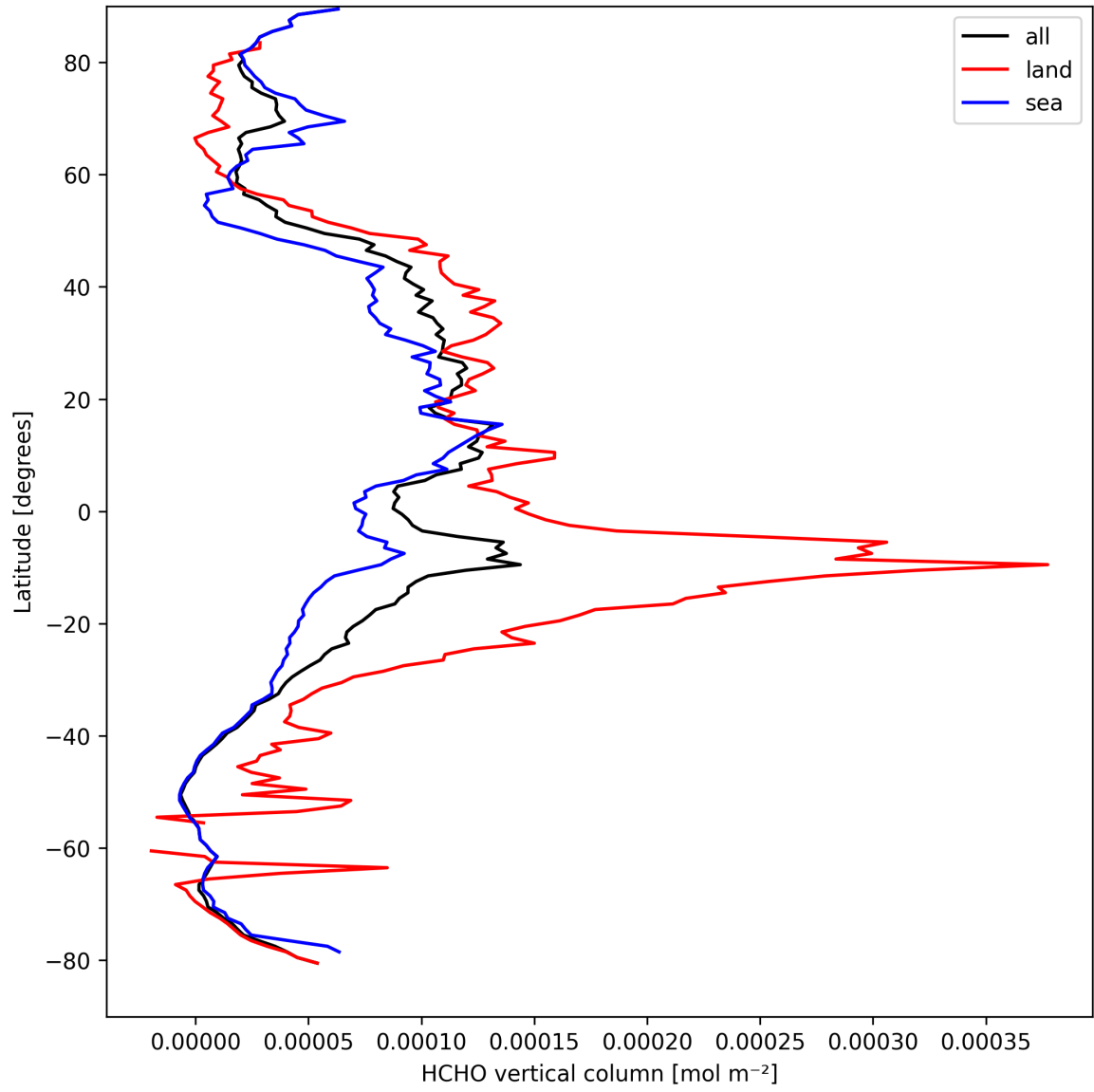
Figure 19: Zonal average of “HCHO vertical column” for 2025-09-11 to 2025-09-12.
