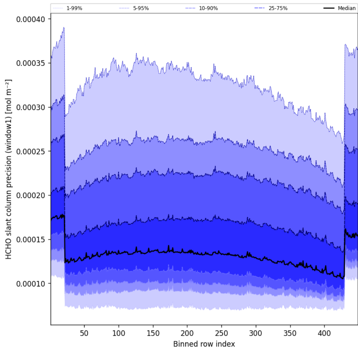
Figure 51: Along track statistics of “HCHO slant column precision (window1)” for 2025-09-11 to 2025-09-12
