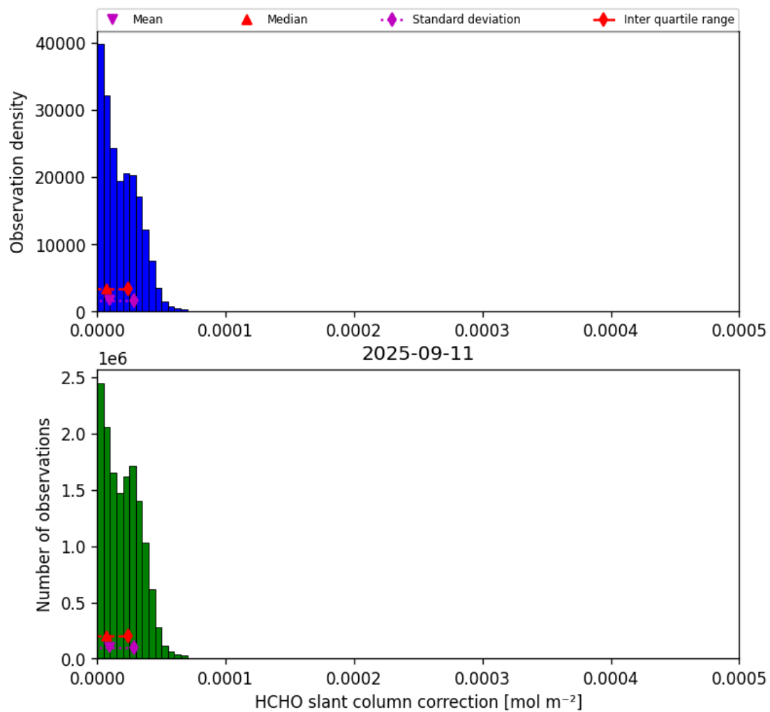
Figure 45: Histogram of “HCHO slant column correction” for 2025-09-11 to 2025-09-12
