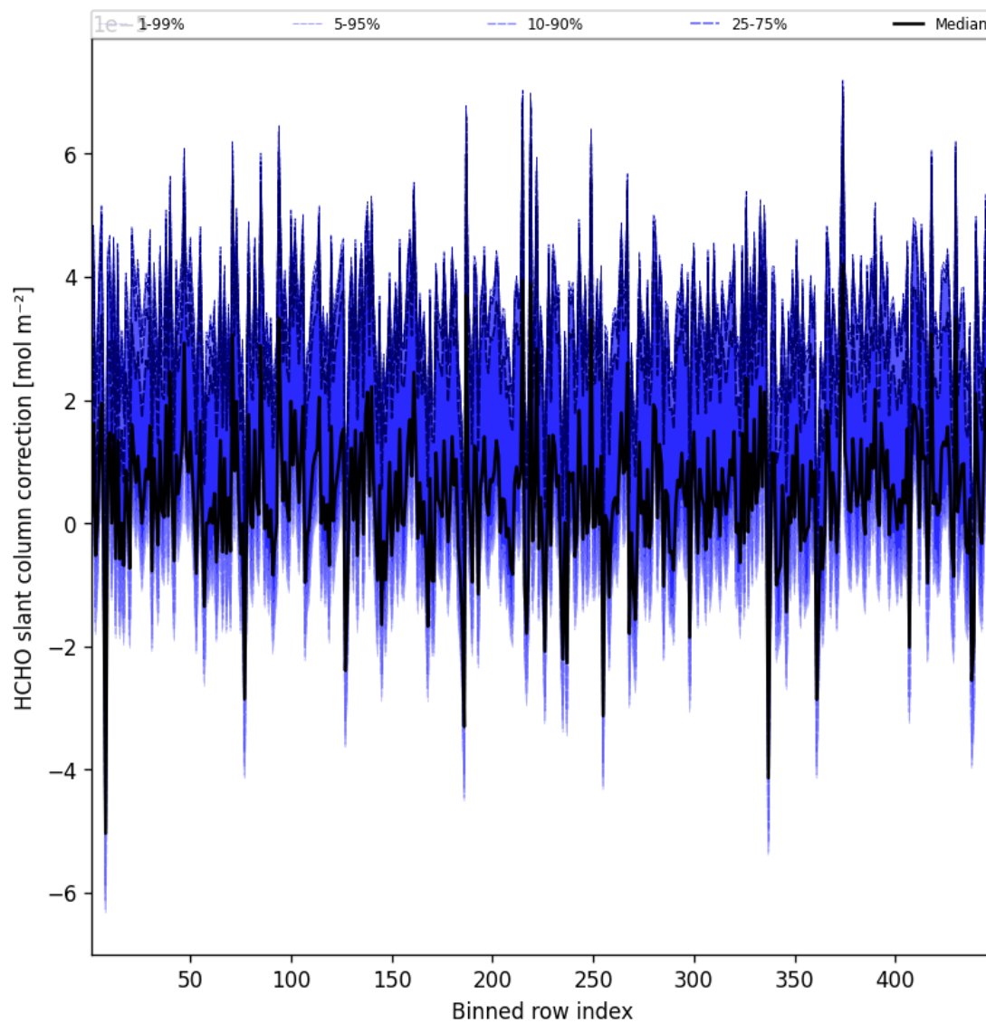
Figure 59: Along track statistics of “HCHO slant column correction” for 2025-09-11 to 2025-09-12
