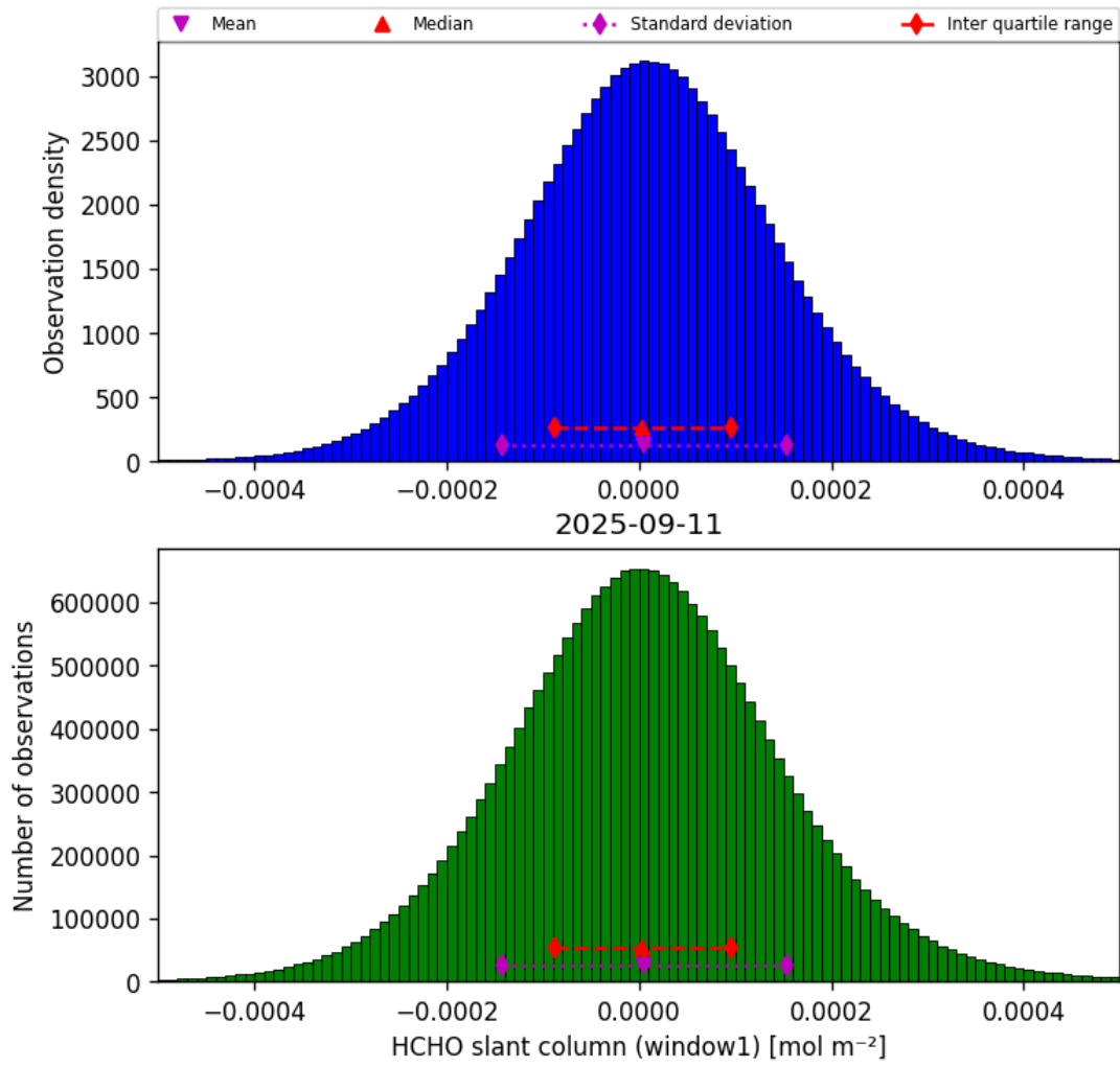
Figure 36: Histogram of “HCHO slant column (window1)” for 2025-09-11 to 2025-09-12
