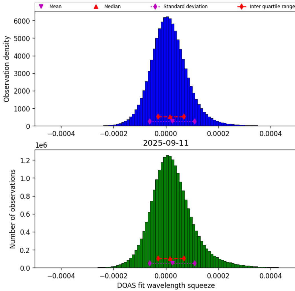
Figure 43: Histogram of “DOAS fit wavelength squeeze” for 2025-09-11 to 2025-09-12
