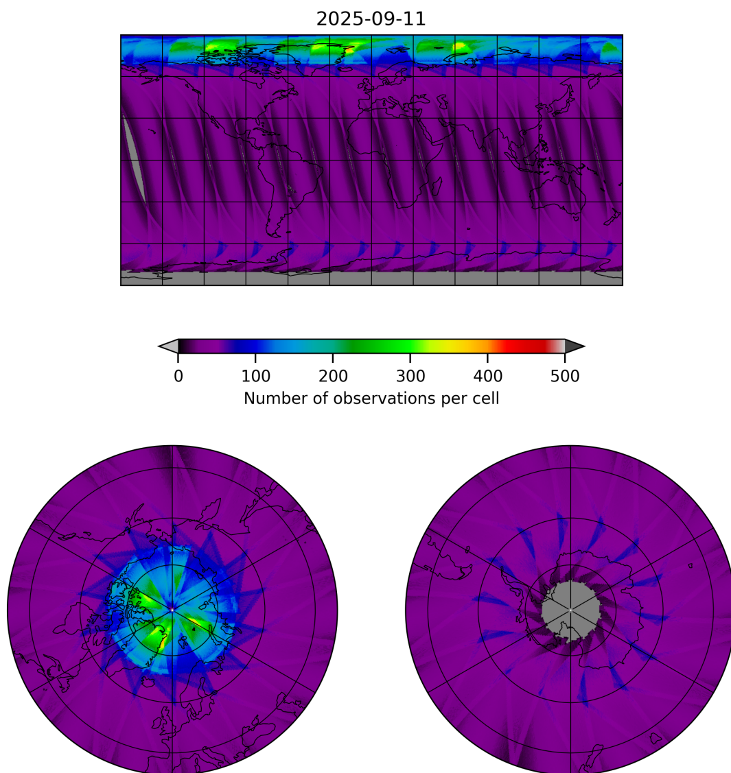
Figure 17: Map of the number of observations for 2025-09-11 to 2025-09-12
