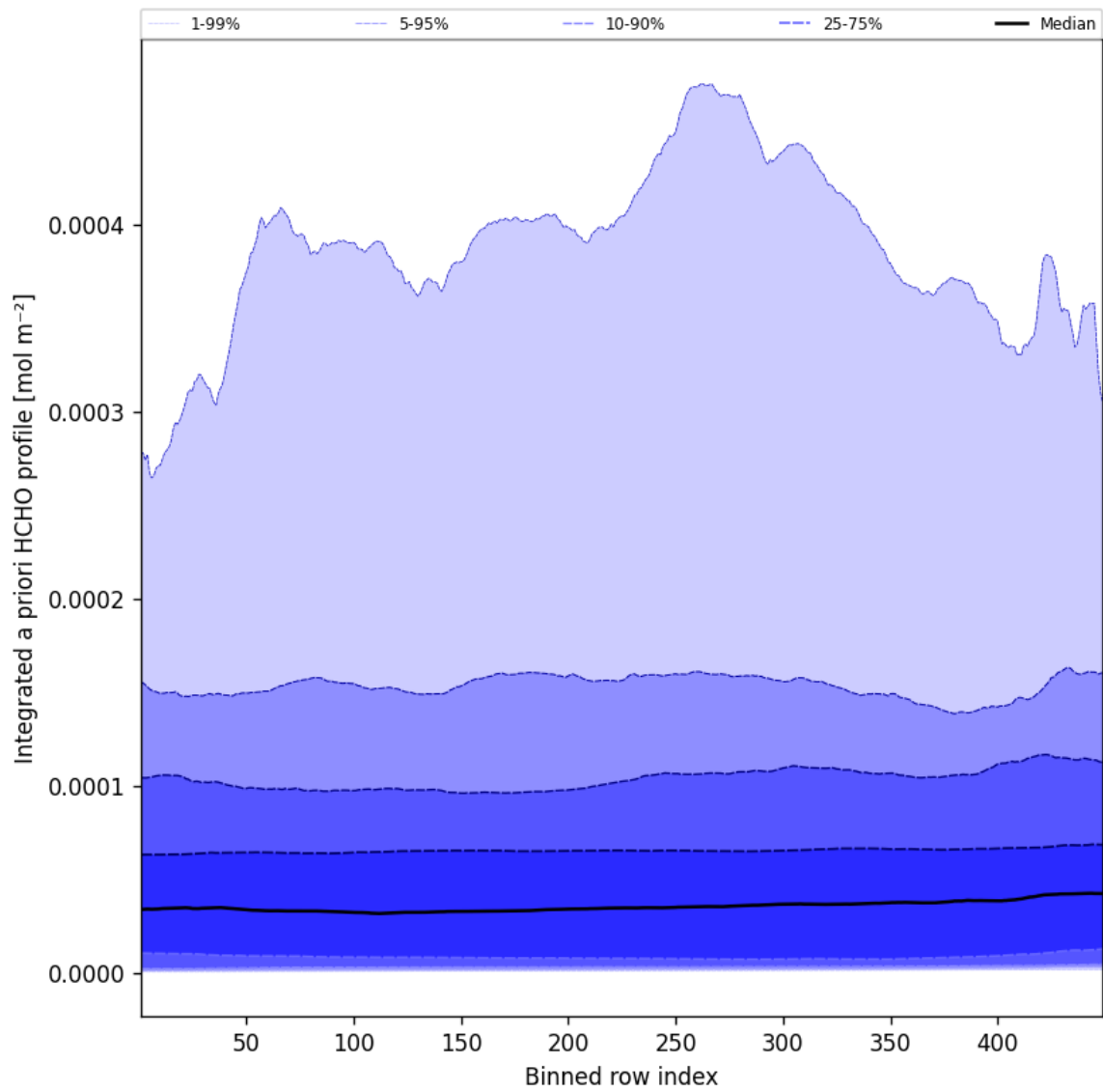
Figure 55: Along track statistics of “Integrated a priori HCHO profile” for 2025-09-11 to 2025-09-12
