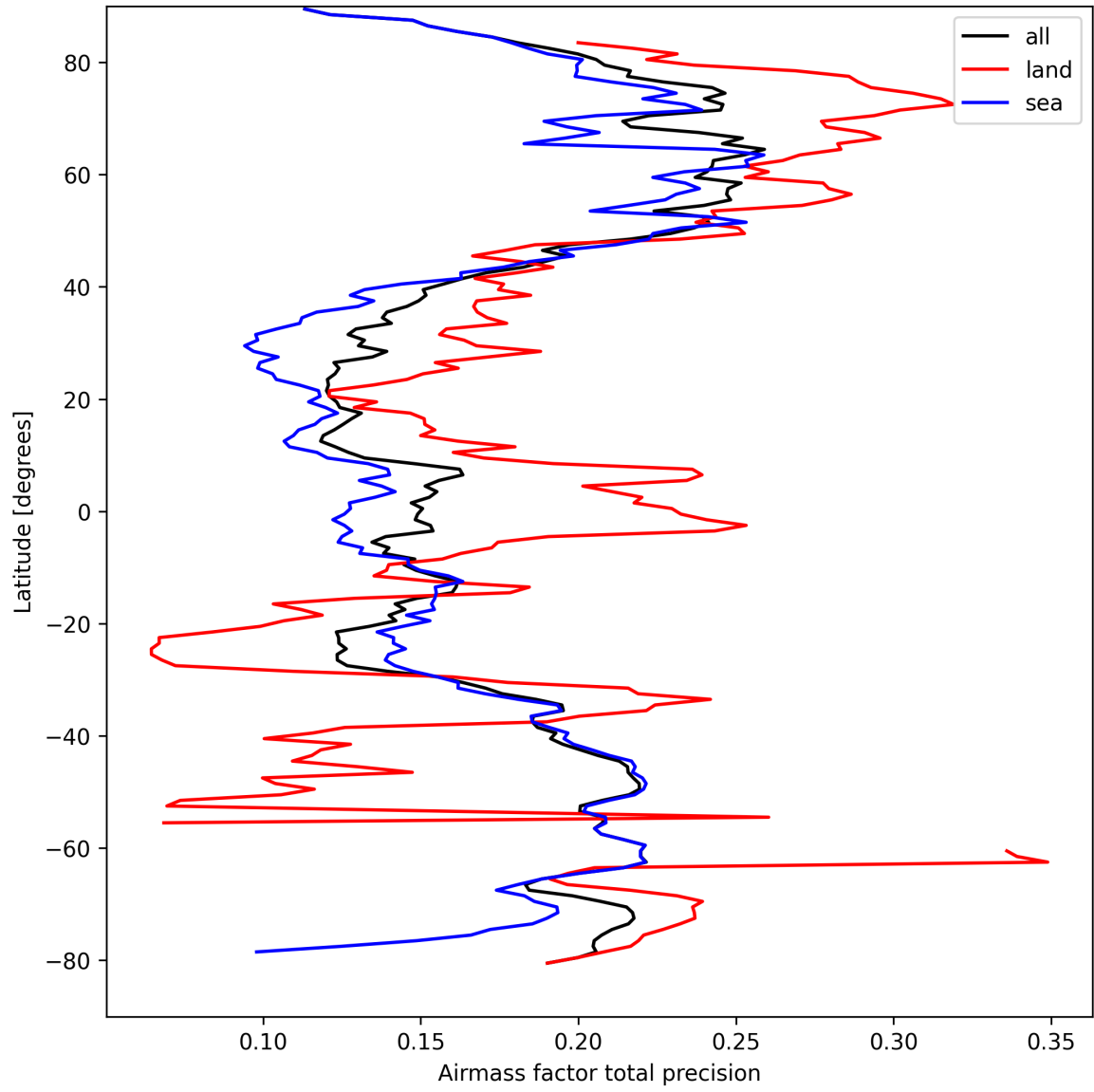
Figure 25: Zonal average of “Airmass factor total precision” for 2025-09-11 to 2025-09-12.
