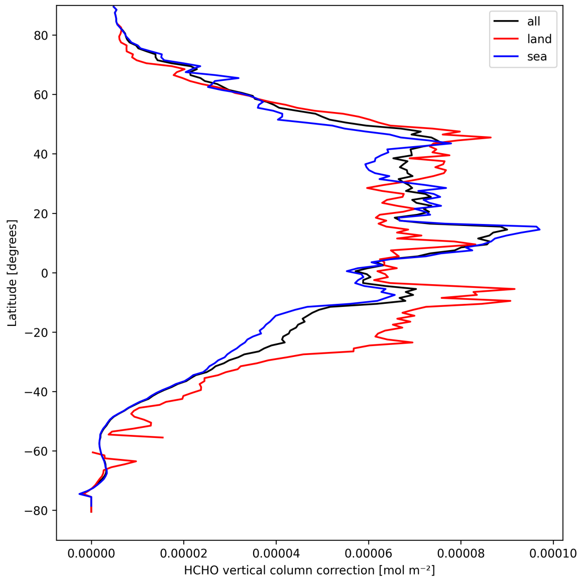
Figure 21: Zonal average of “HCHO vertical column correction” for 2025-09-11 to 2025-09-12.
