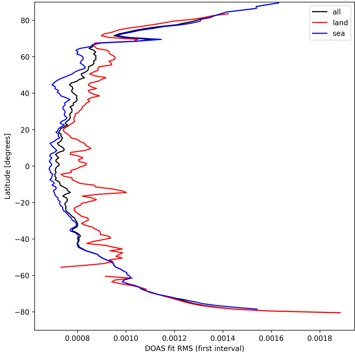
Figure 30: Zonal average of "DOAS fit RMS (first interval)" for 2025-09-11 to 2025-09-12.
