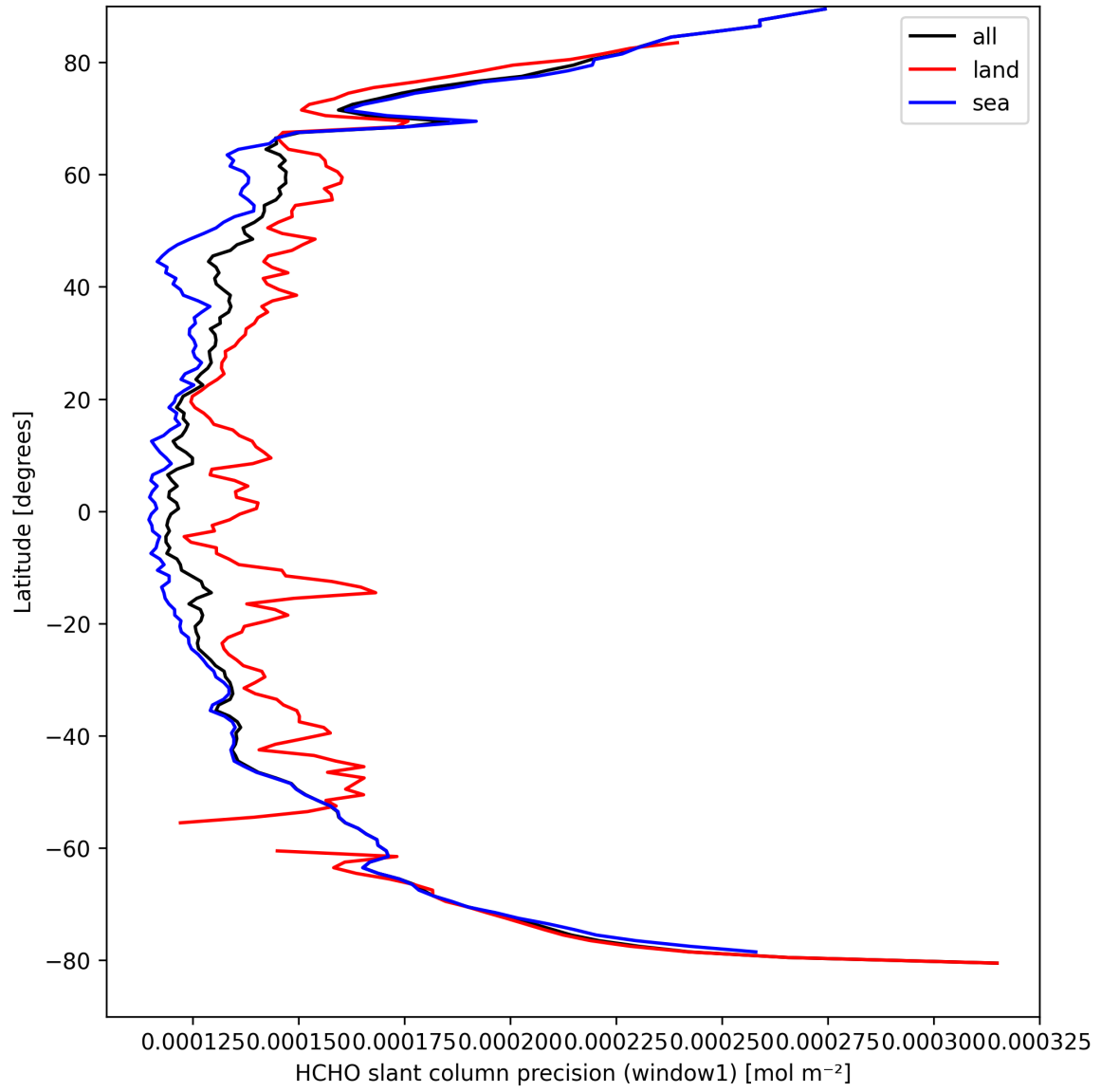
Figure 23: Zonal average of "HCHO slant column precision (window1)" for 2025-09-11 to 2025-09-12.
