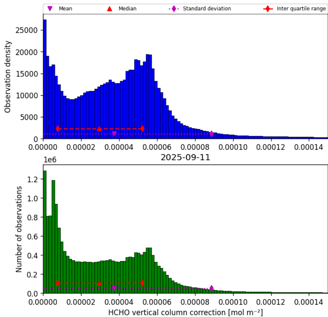
Figure 35: Histogram of “HCHO vertical column correction” for 2025-09-11 to 2025-09-12
