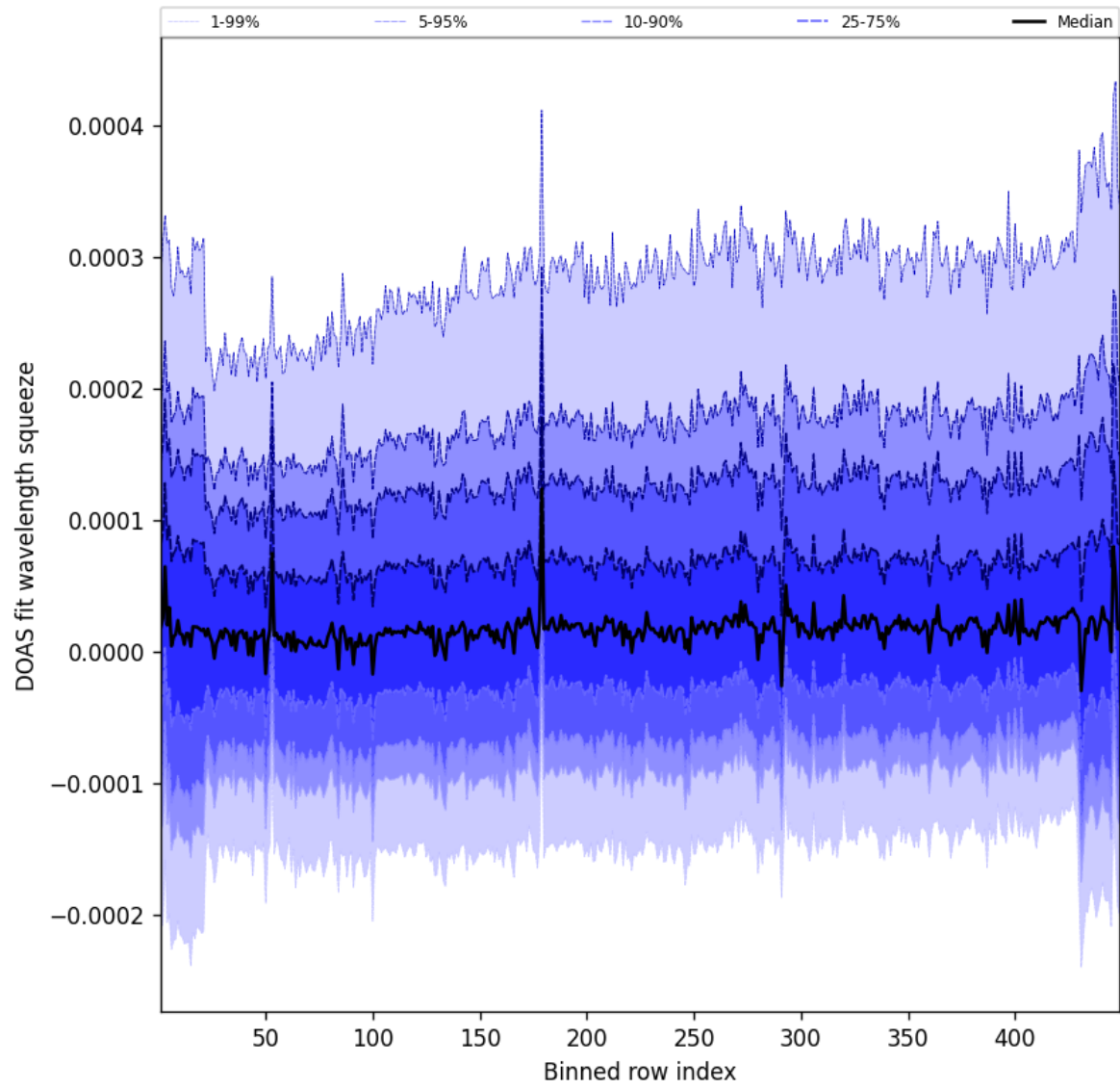
Figure 57: Along track statistics of “DOAS fit wavelength squeeze” for 2025-09-11 to 2025-09-12
