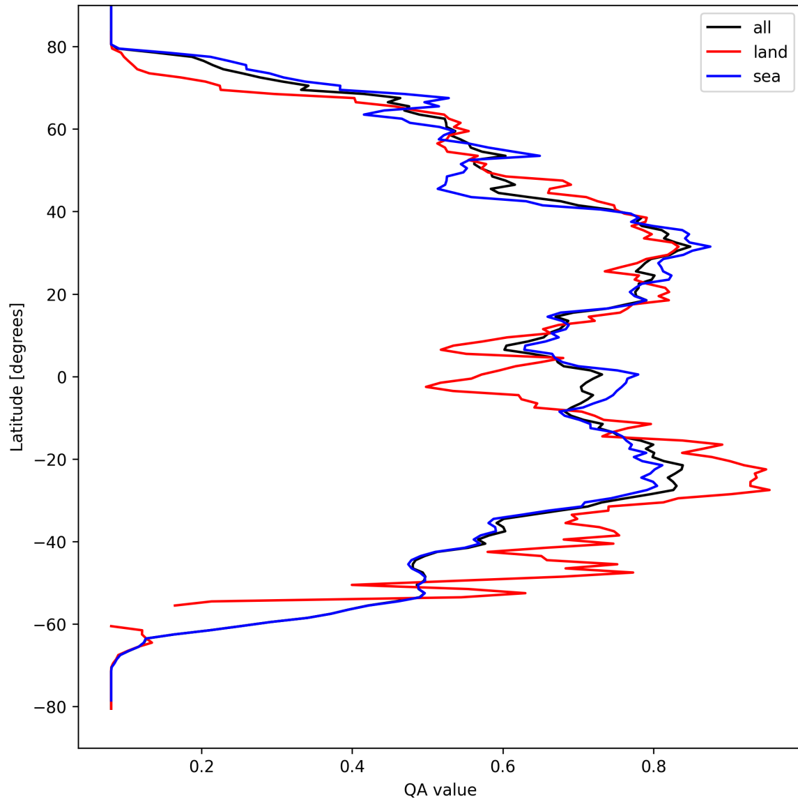
Figure 18: Zonal average of “QA value” for 2025-09-11 to 2025-09-12.
