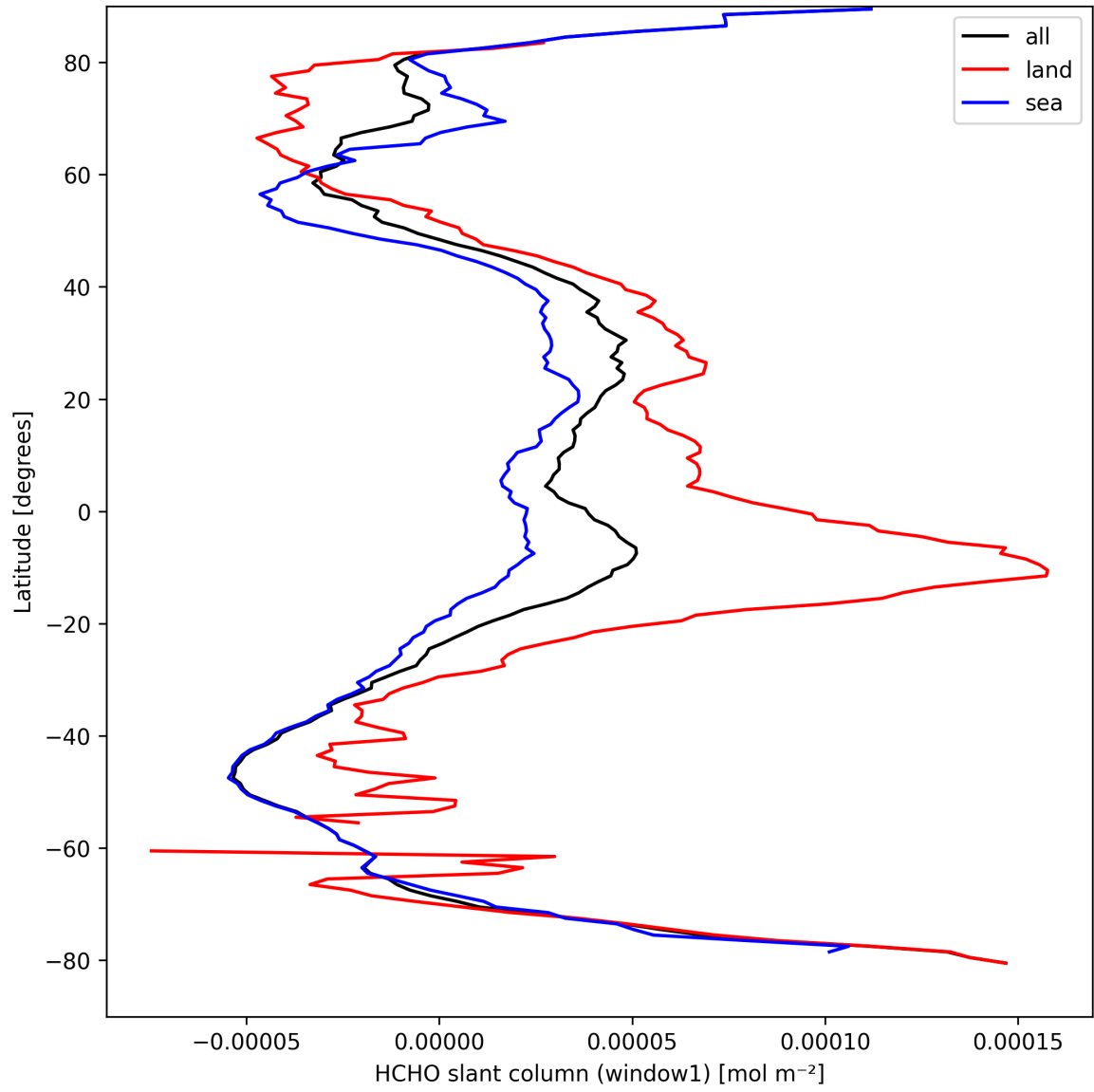
Figure 22: Zonal average of “HCHO slant column (window1)” for 2025-09-11 to 2025-09-12.
