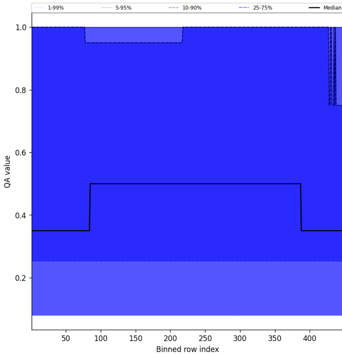
Figure 46: Along track statistics of “QA value” for 2025-09-11 to 2025-09-12
