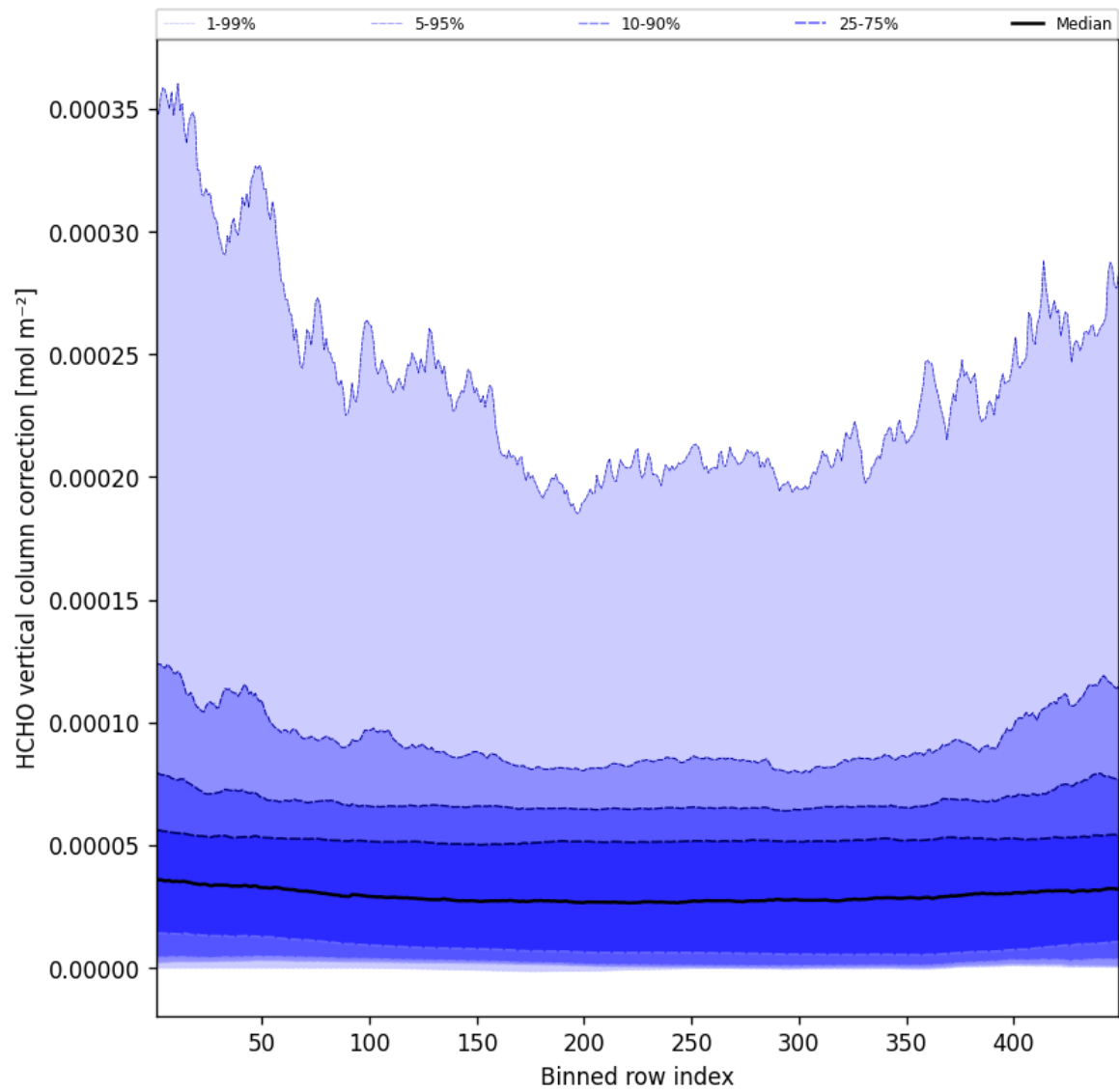
Figure 49: Along track statistics of "HCHO vertical column correction" for 2025-09-11 to 2025-09-12
