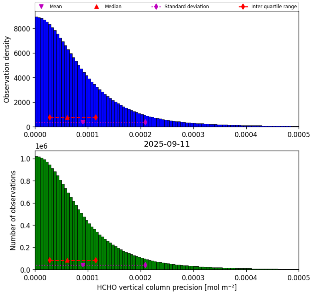
Figure 34: Histogram of “HCHO vertical column precision” for 2025-09-11 to 2025-09-12
