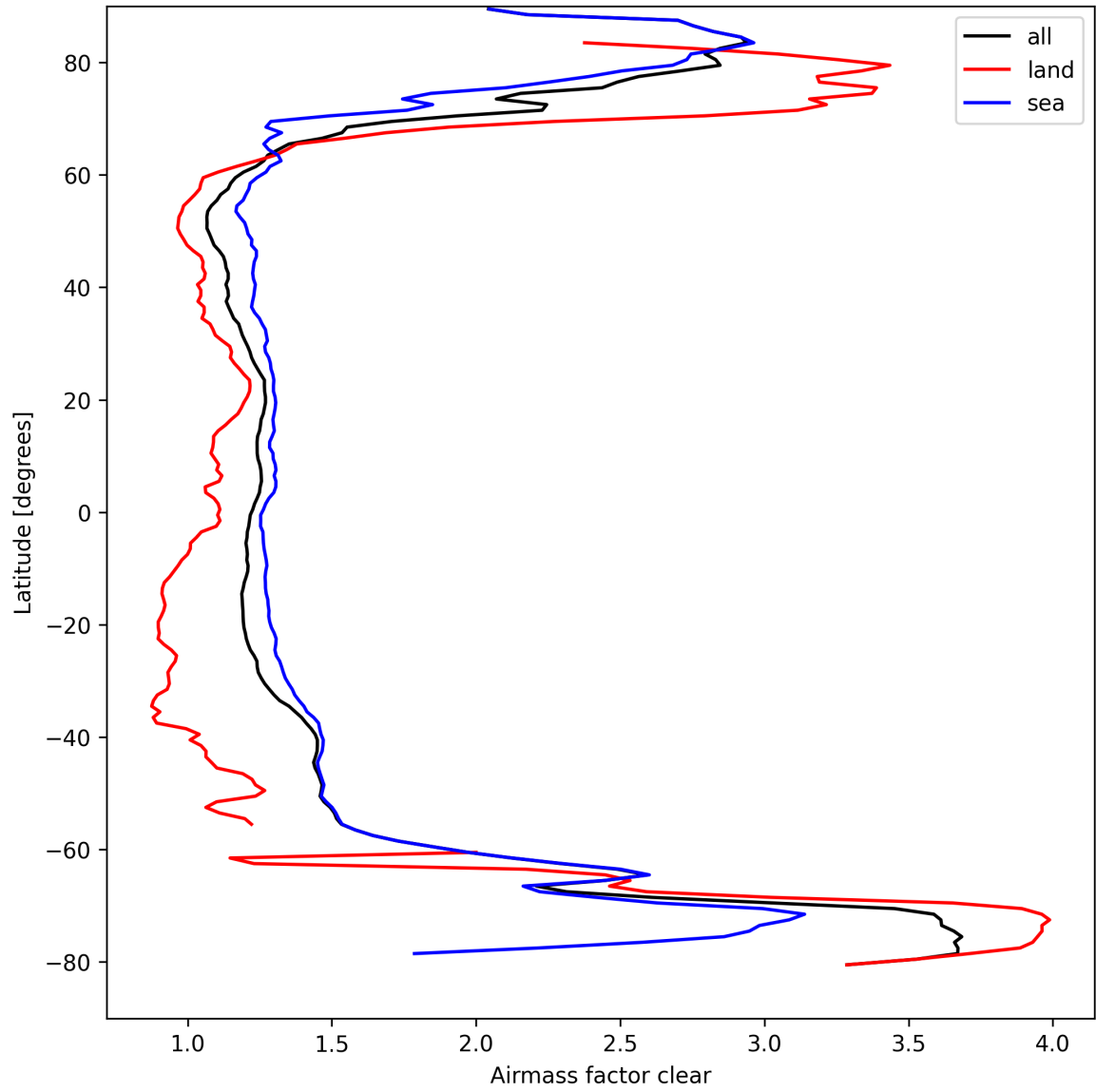
Figure 26: Zonal average of “Airmass factor clear” for 2025-09-11 to 2025-09-12.
