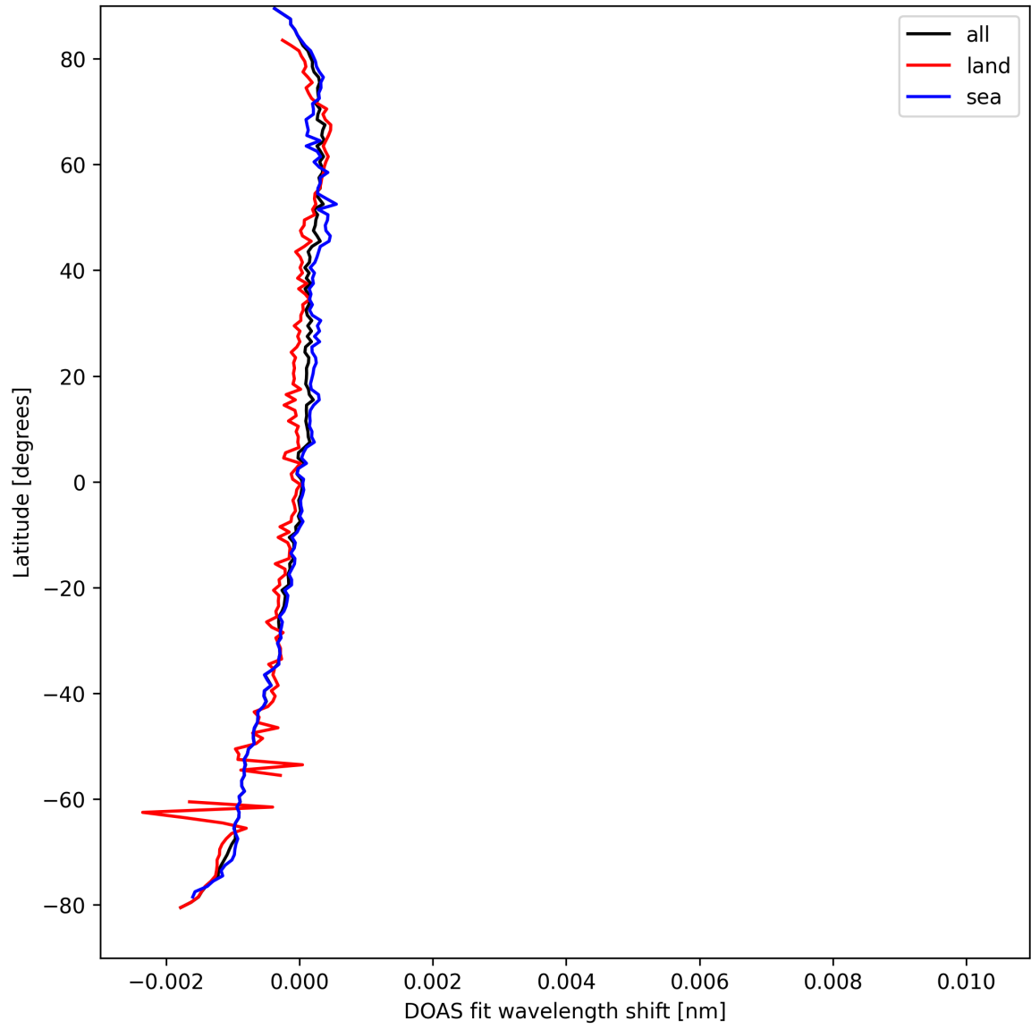
Figure 28: Zonal average of “DOAS fit wavelength shift” for 2025-09-11 to 2025-09-12.
