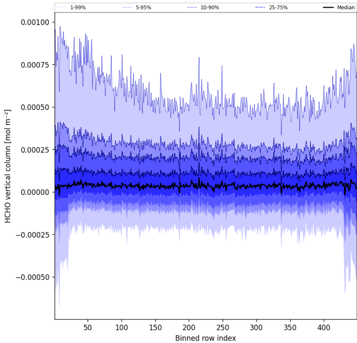
Figure 47: Along track statistics of “HCHO vertical column” for 2025-09-11 to 2025-09-12
