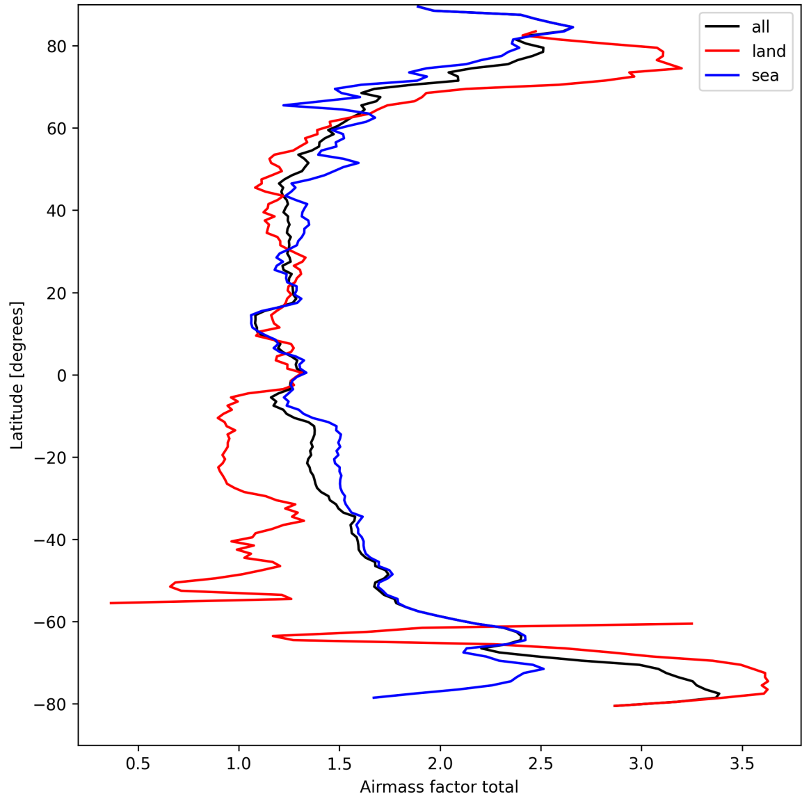
Figure 24: Zonal average of “Airmass factor total” for 2025-09-11 to 2025-09-12.
