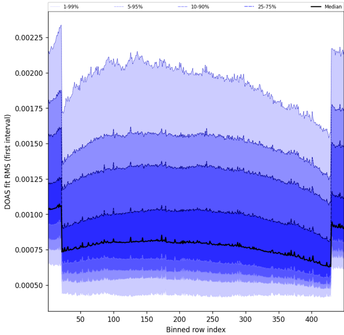
Figure 58: Along track statistics of “DOAS fit RMS (first interval)” for 2025-09-11 to 2025-09-12
