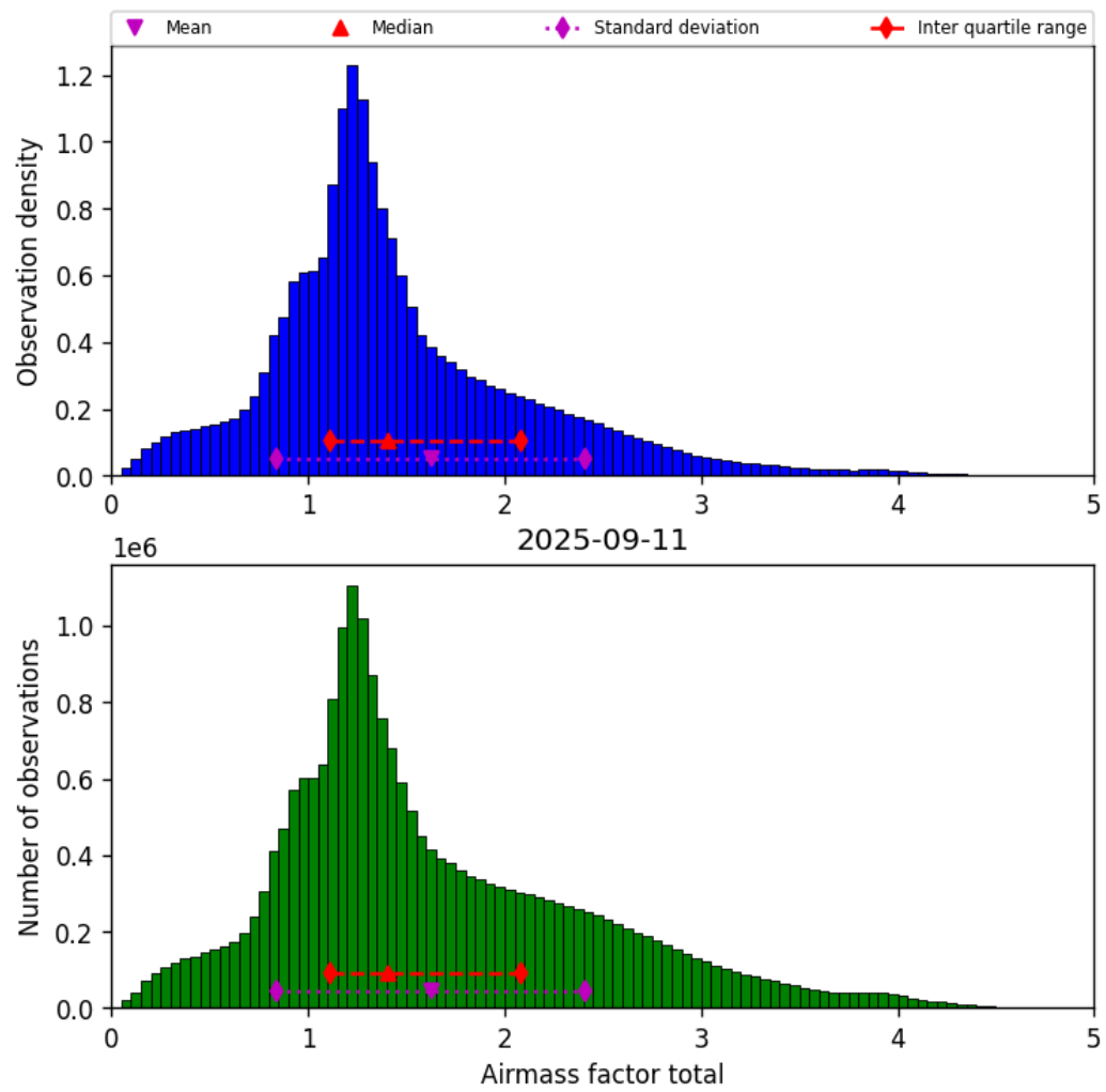
Figure 38: Histogram of “Airmass factor total” for 2025-09-11 to 2025-09-12
