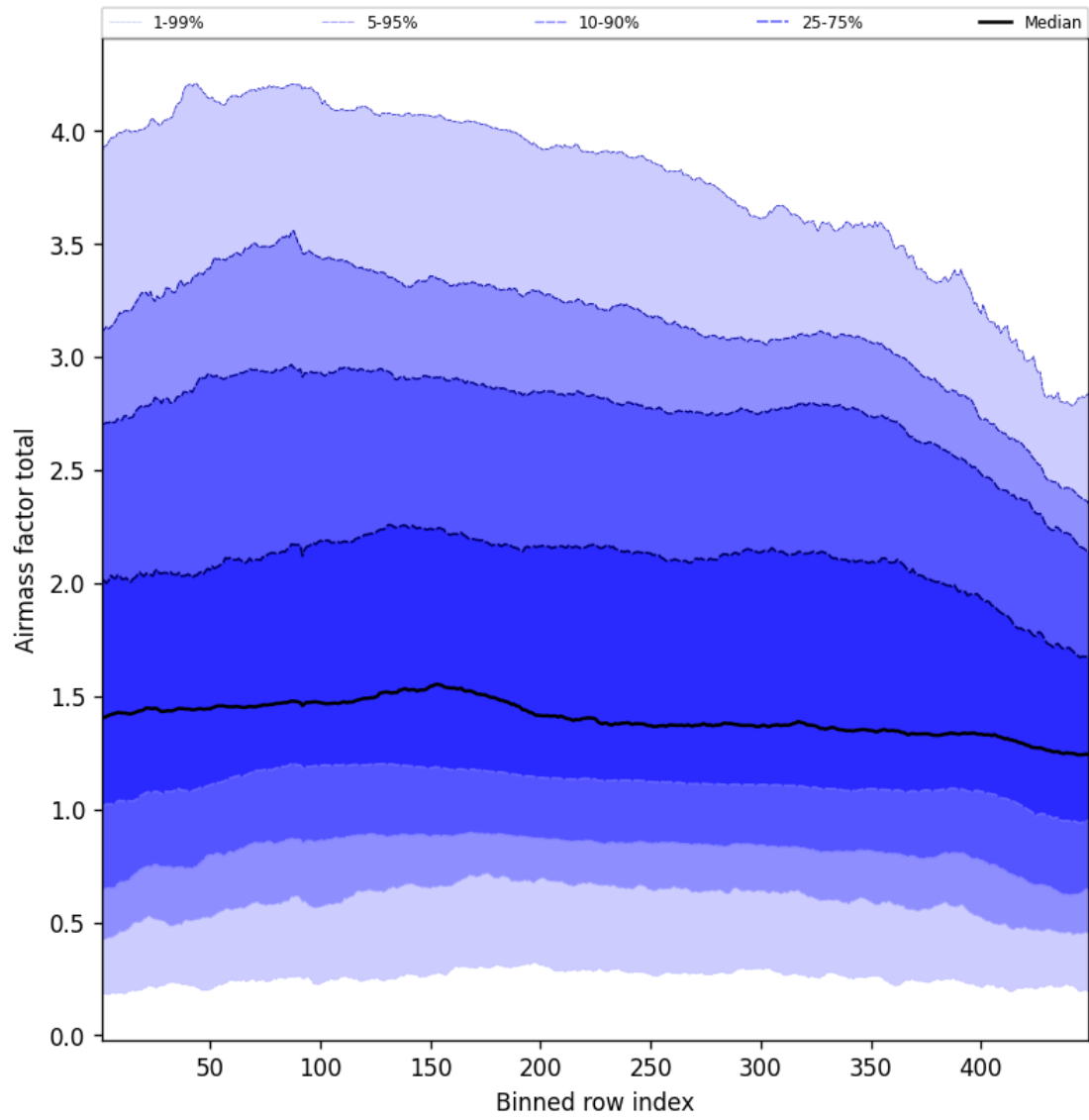
Figure 52: Along track statistics of “Airmass factor total” for 2025-09-11 to 2025-09-12
