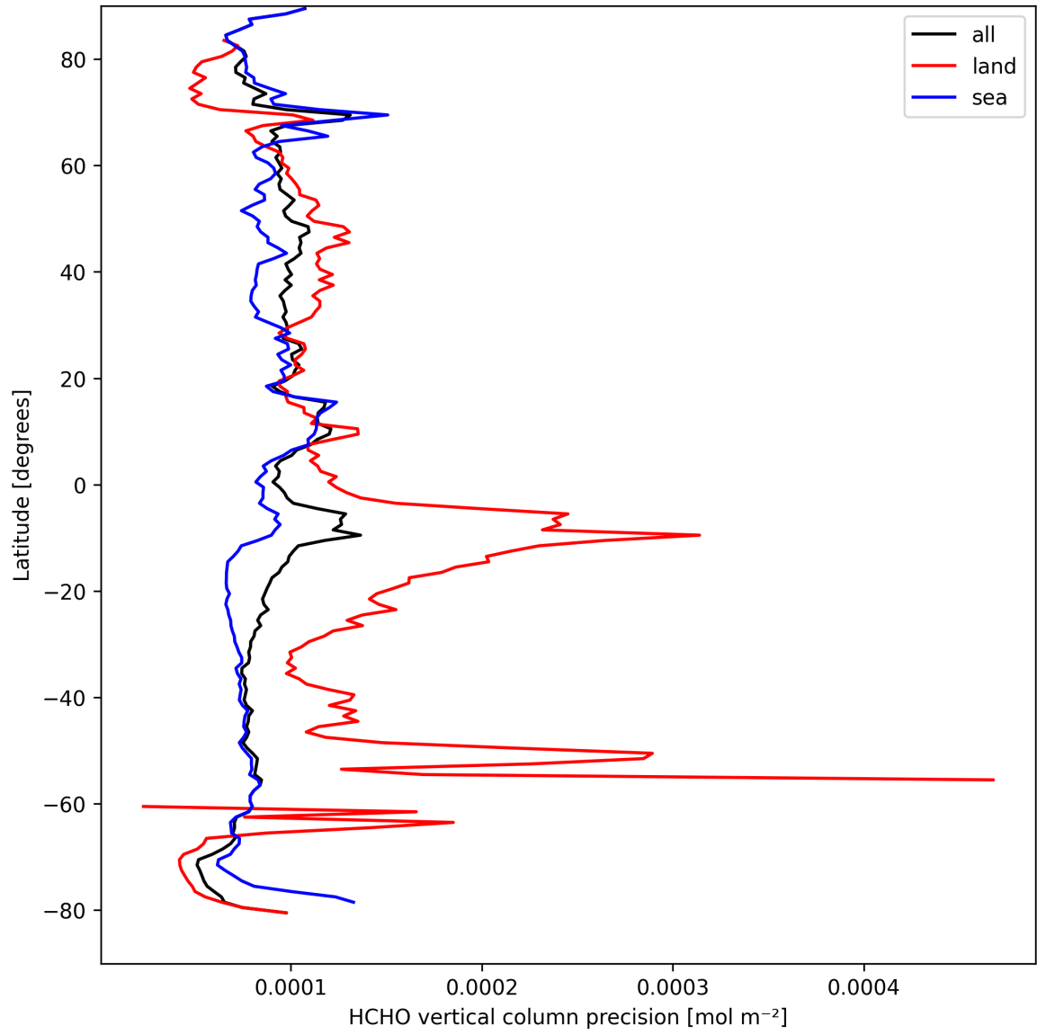
Figure 20: Zonal average of “HCHO vertical column precision” for 2025-09-11 to 2025-09-12.
