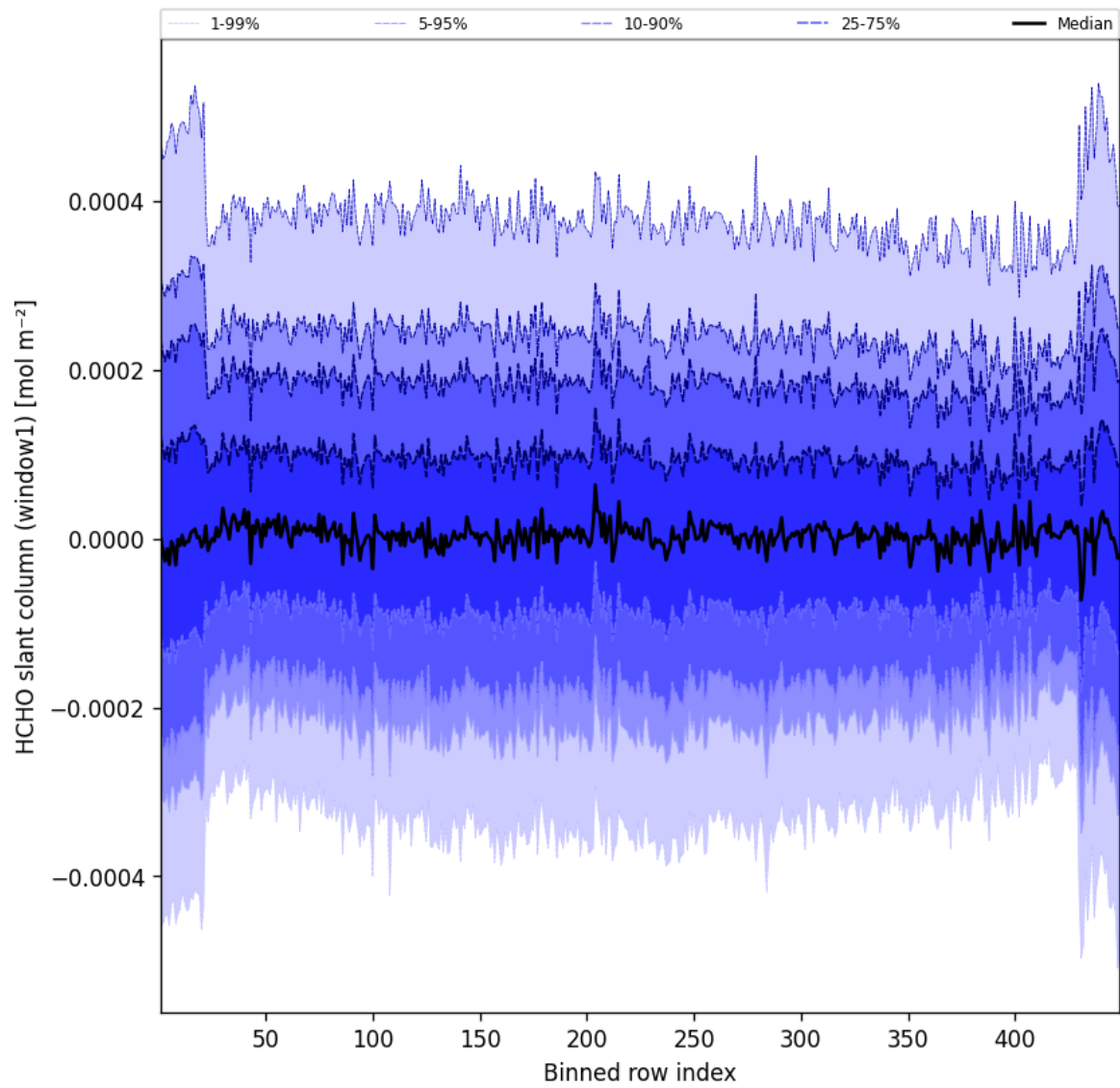
Figure 50: Along track statistics of “HCHO slant column (window1)” for 2025-09-11 to 2025-09-12
