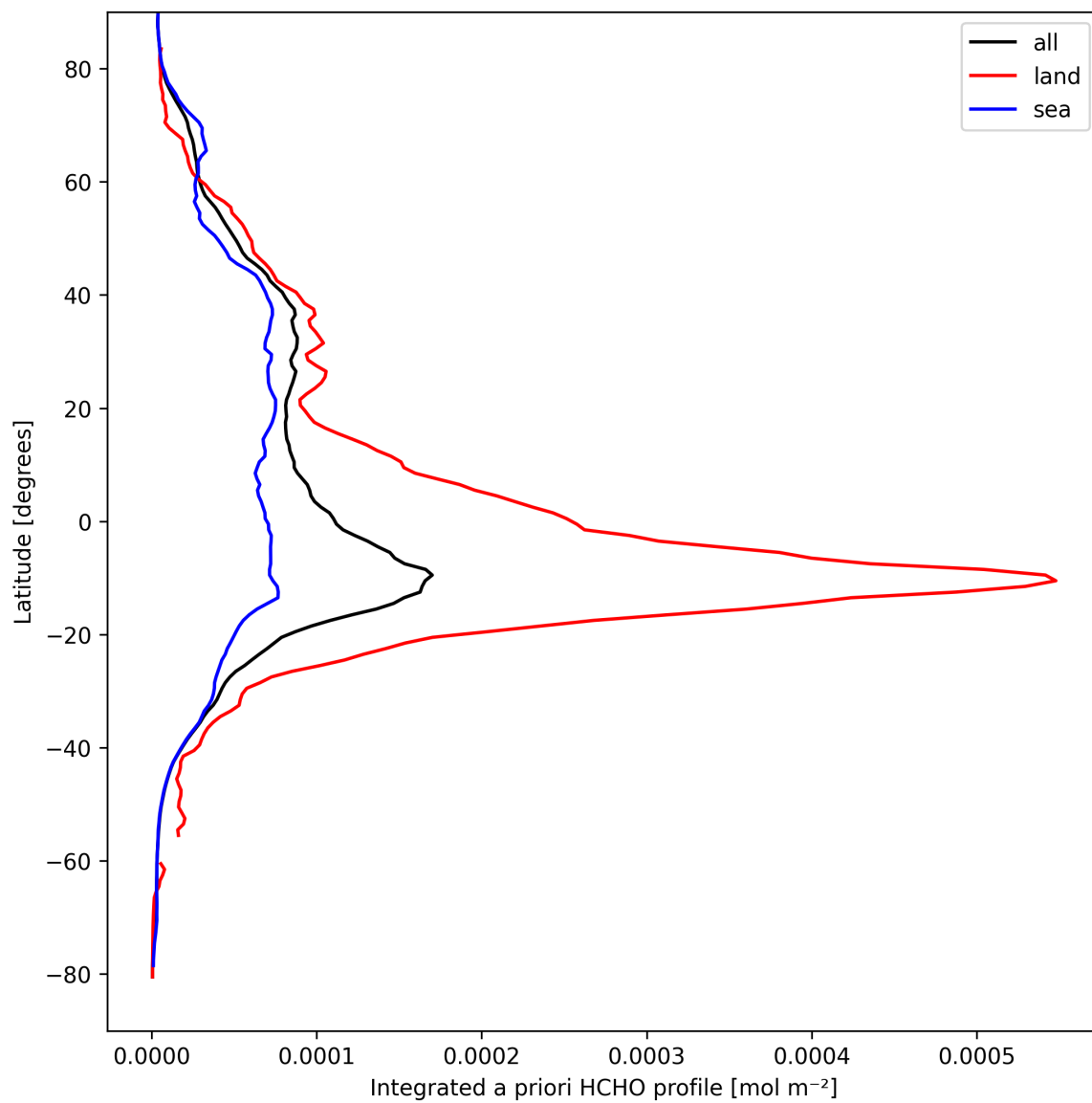
Figure 27: Zonal average of “Integrated a priori HCHO profile” for 2025-09-11 to 2025-09-12.
