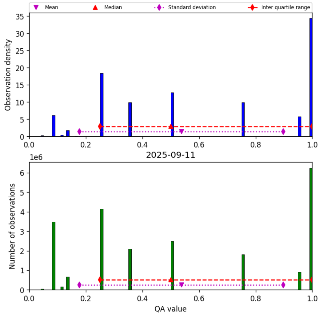
Figure 32: Histogram of “QA value” for 2025-09-11 to 2025-09-12
