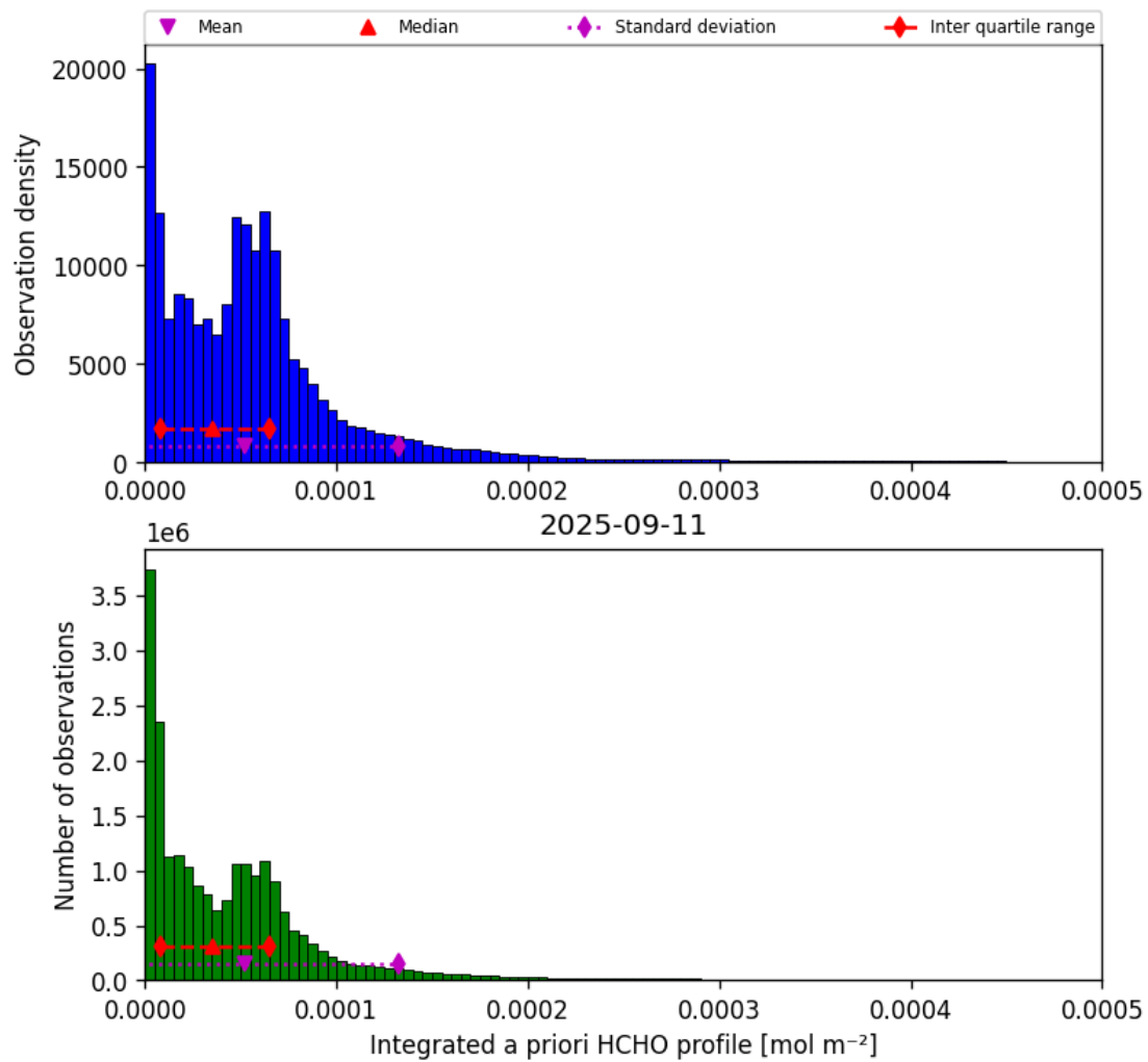
Figure 41: Histogram of “Integrated a priori HCHO profile” for 2025-09-11 to 2025-09-12
