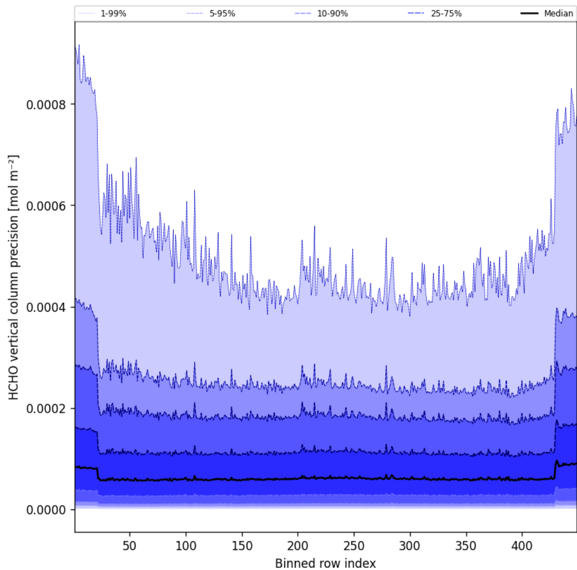
Figure 48: Along track statistics of “HCHO vertical column precision” for 2025-09-11 to 2025-09-12
