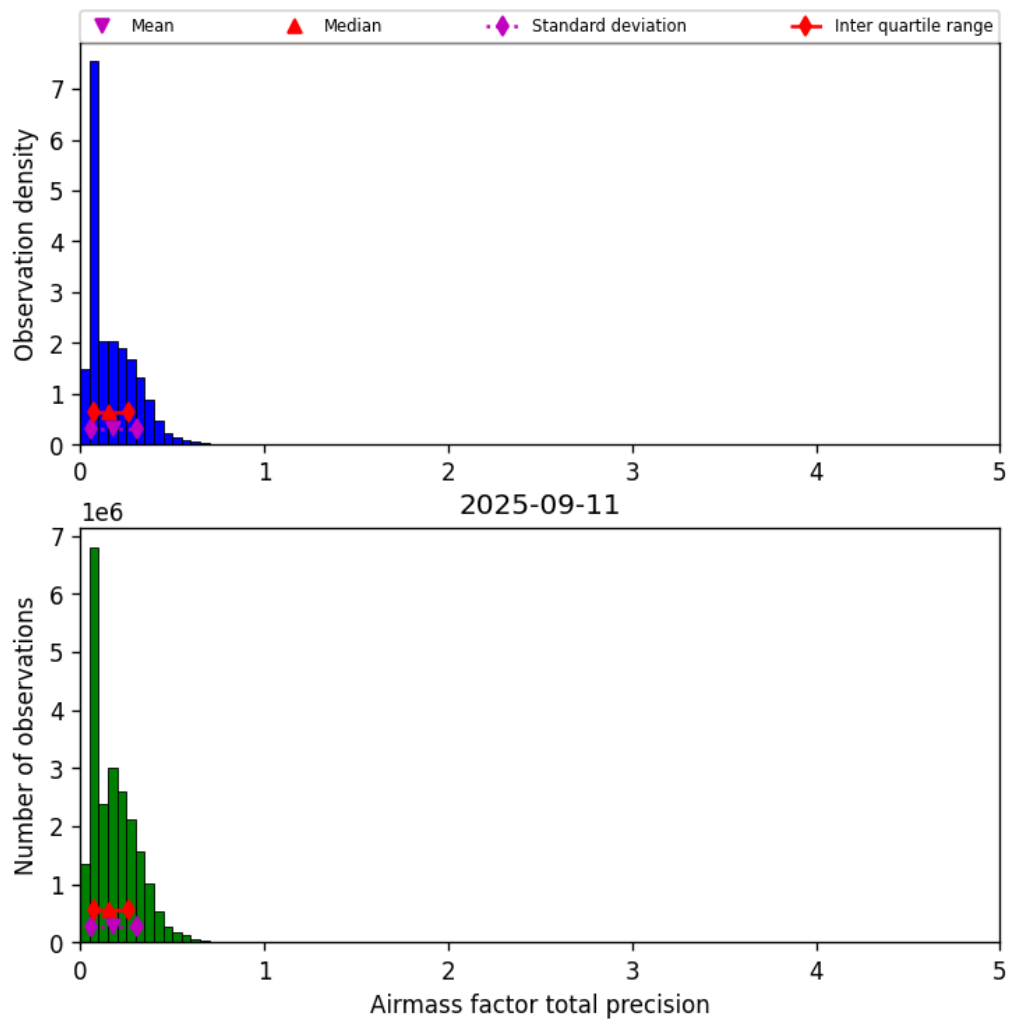
Figure 39: Histogram of “Airmass factor total precision” for 2025-09-11 to 2025-09-12
