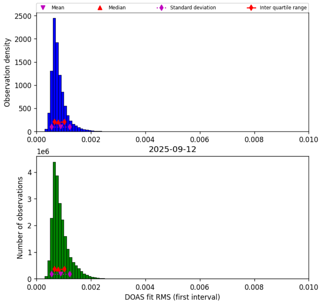
Figure 44: Histogram of “DOAS fit RMS (first interval)” for 2025-09-12 to 2025-09-13
