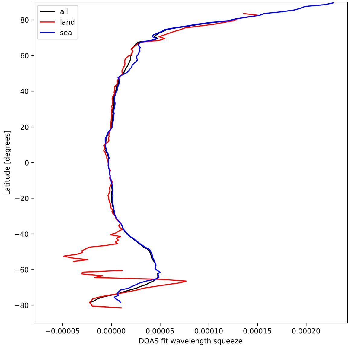
Figure 29: Zonal average of “DOAS fit wavelength squeeze” for 2025-09-12 to 2025-09-13.
