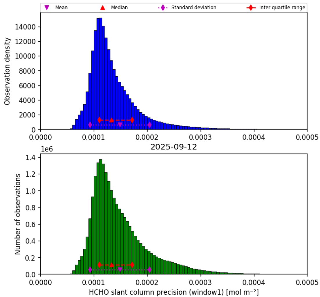
Figure 37: Histogram of “HCHO slant column precision (window1)” for 2025-09-12 to 2025-09-13
