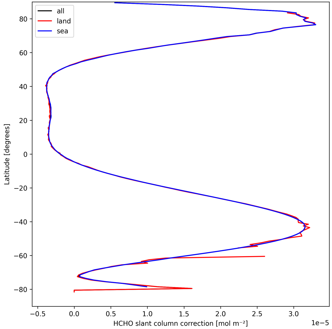
Figure 31: Zonal average of "HCHO slant column correction" for 2025-09-12 to 2025-09-13.
