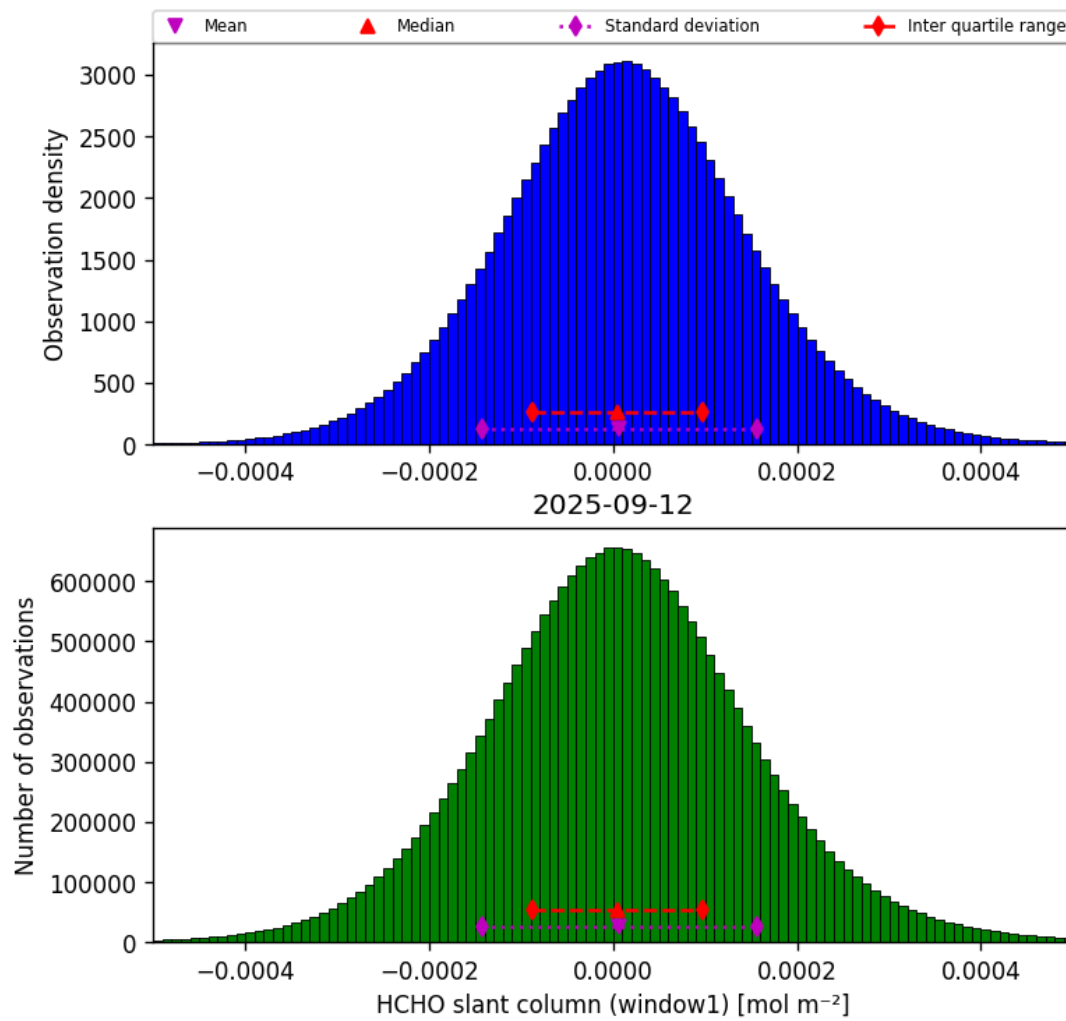
Figure 36: Histogram of “HCHO slant column (window1)” for 2025-09-12 to 2025-09-13
