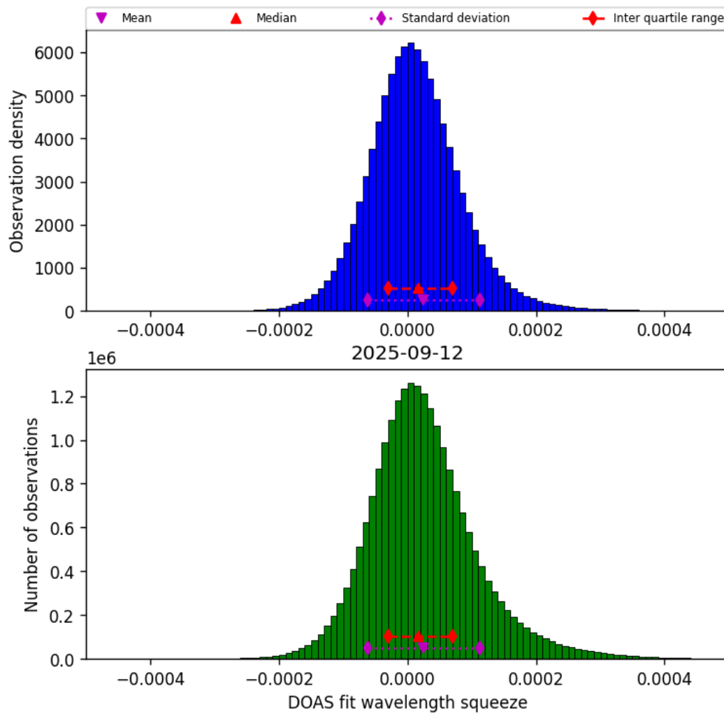
Figure 43: Histogram of “DOAS fit wavelength squeeze” for 2025-09-12 to 2025-09-13
