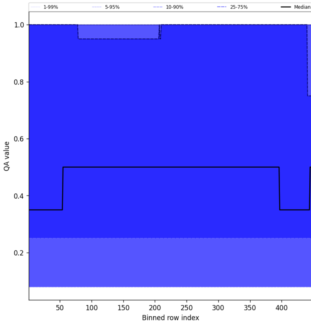
Figure 46: Along track statistics of “QA value” for 2025-09-12 to 2025-09-13
