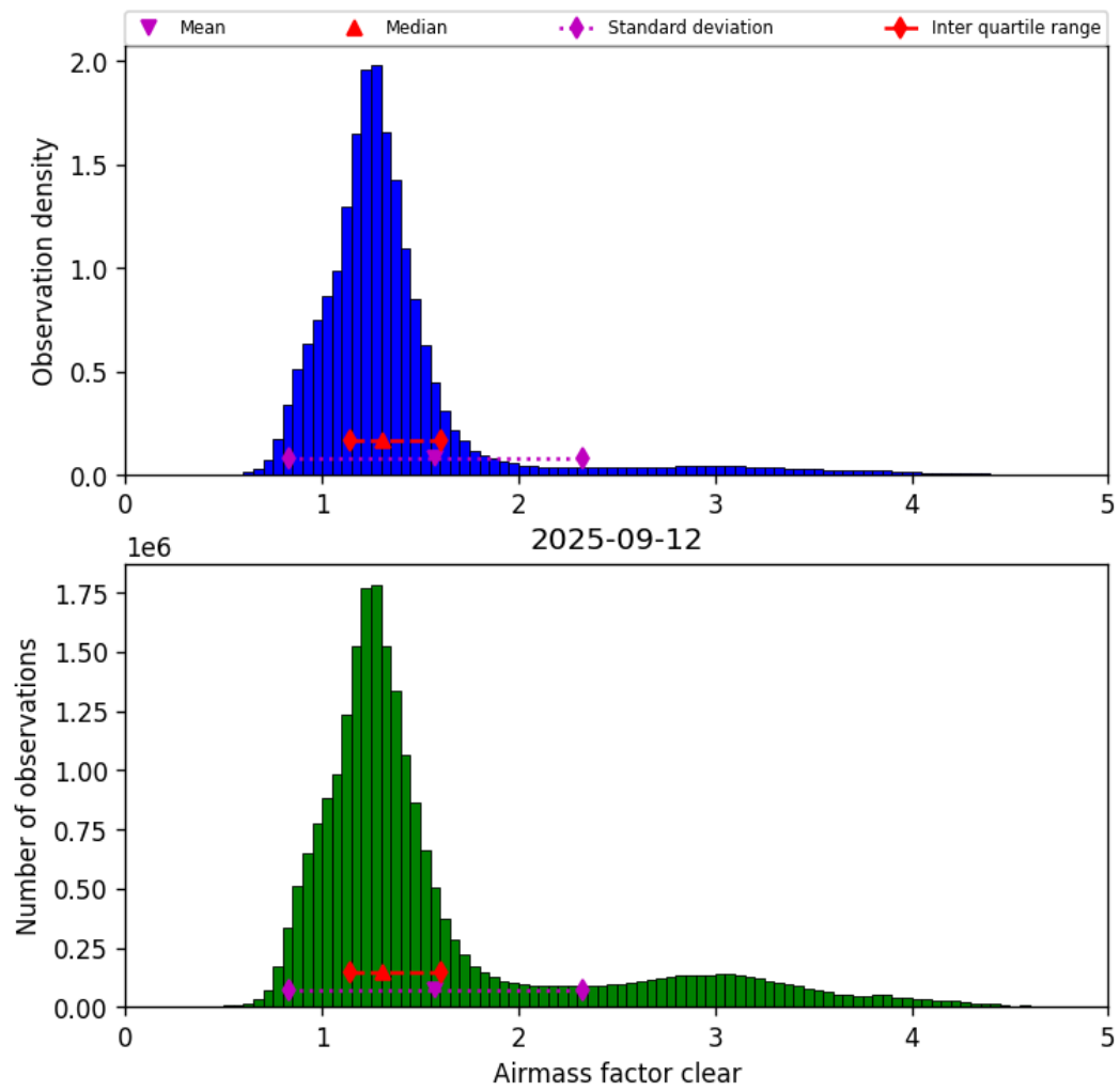
Figure 40: Histogram of “Airmass factor clear” for 2025-09-12 to 2025-09-13
