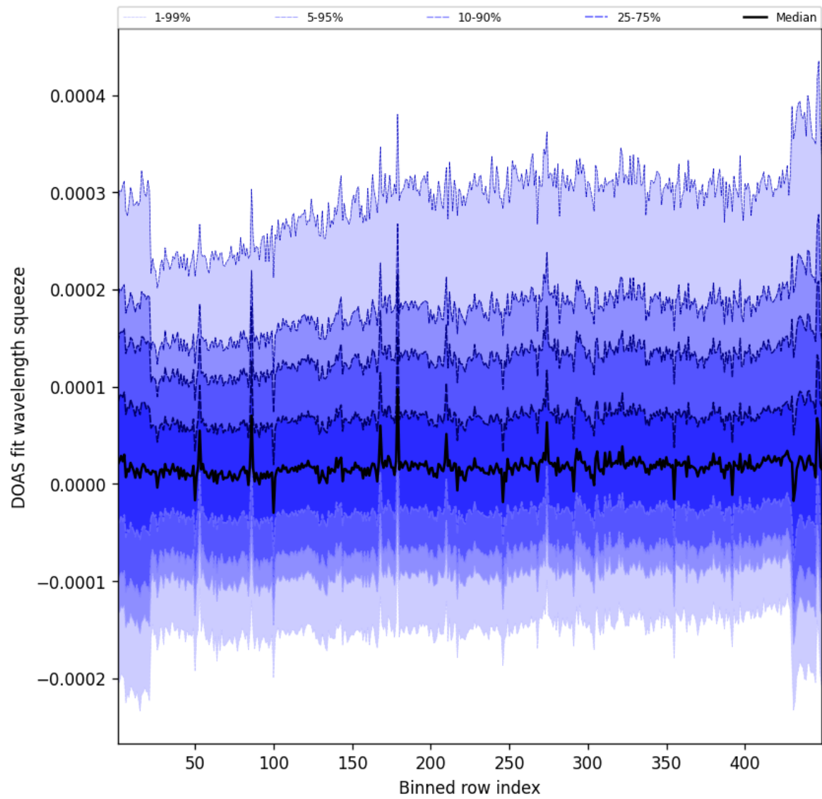
Figure 57: Along track statistics of “DOAS fit wavelength squeeze” for 2025-09-12 to 2025-09-13
