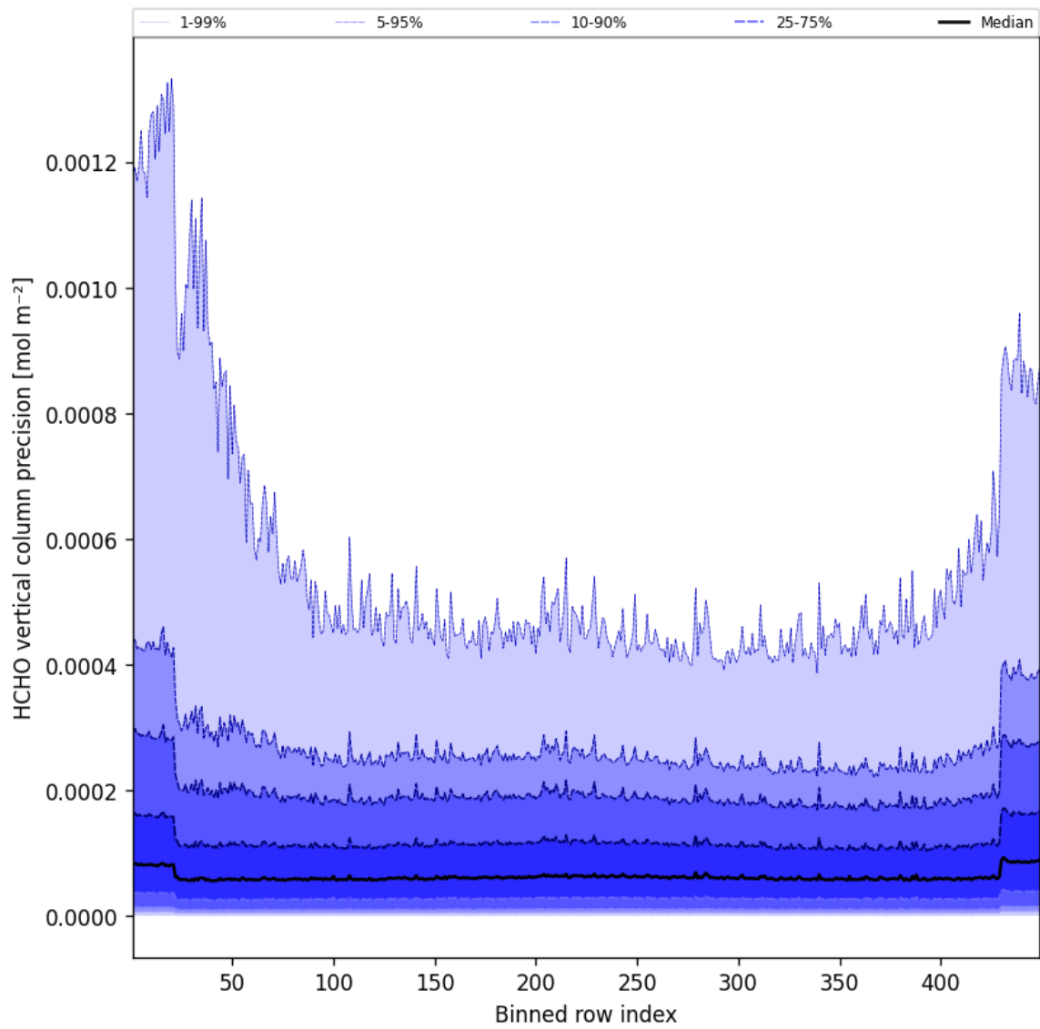
Figure 48: Along track statistics of “HCHO vertical column precision” for 2025-09-12 to 2025-09-13
