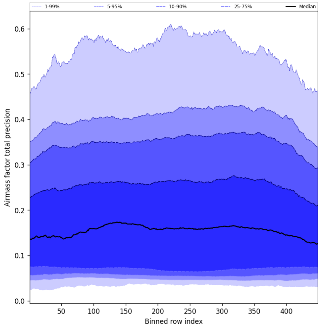
Figure 53: Along track statistics of “Airmass factor total precision” for 2025-09-12 to 2025-09-13
