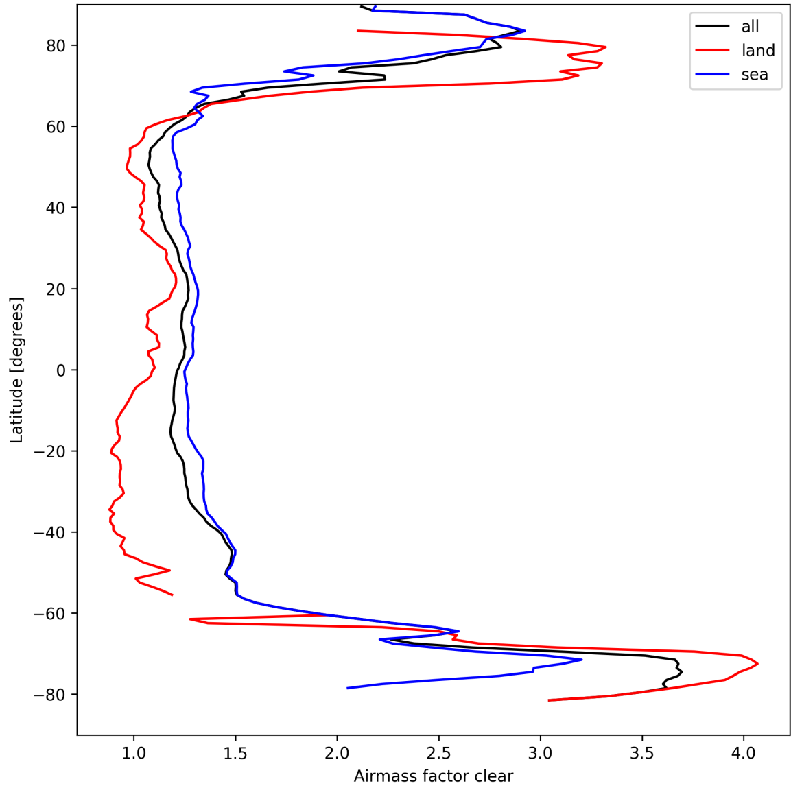
Figure 26: Zonal average of “Airmass factor clear” for 2025-09-12 to 2025-09-13.
