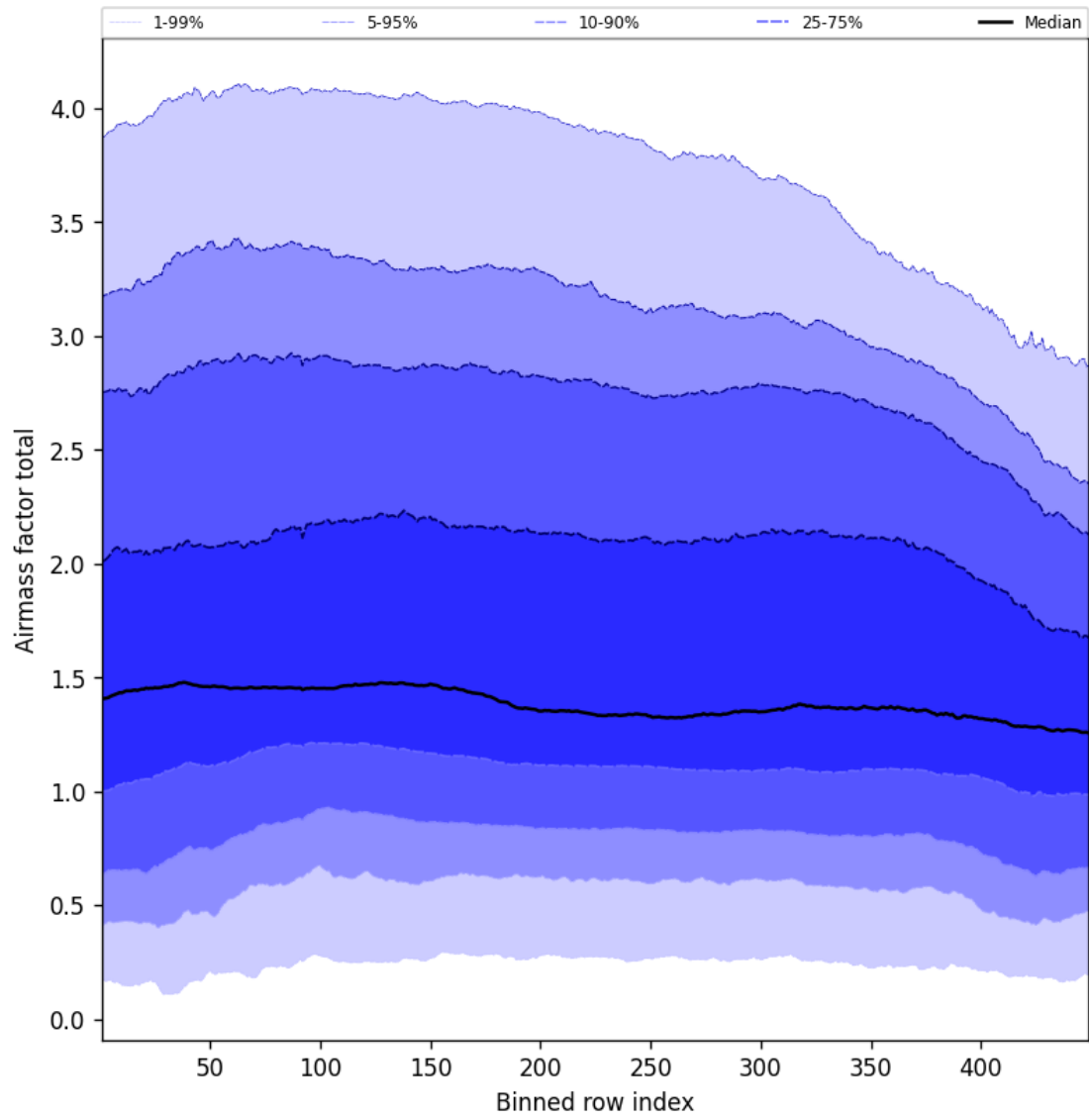
Figure 52: Along track statistics of “Airmass factor total” for 2025-09-12 to 2025-09-13
