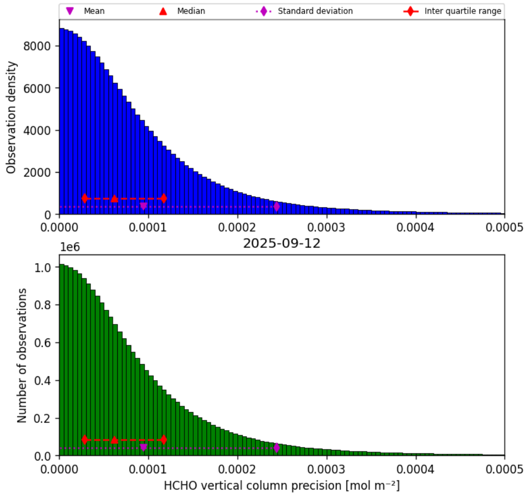
Figure 34: Histogram of “HCHO vertical column precision” for 2025-09-12 to 2025-09-13
