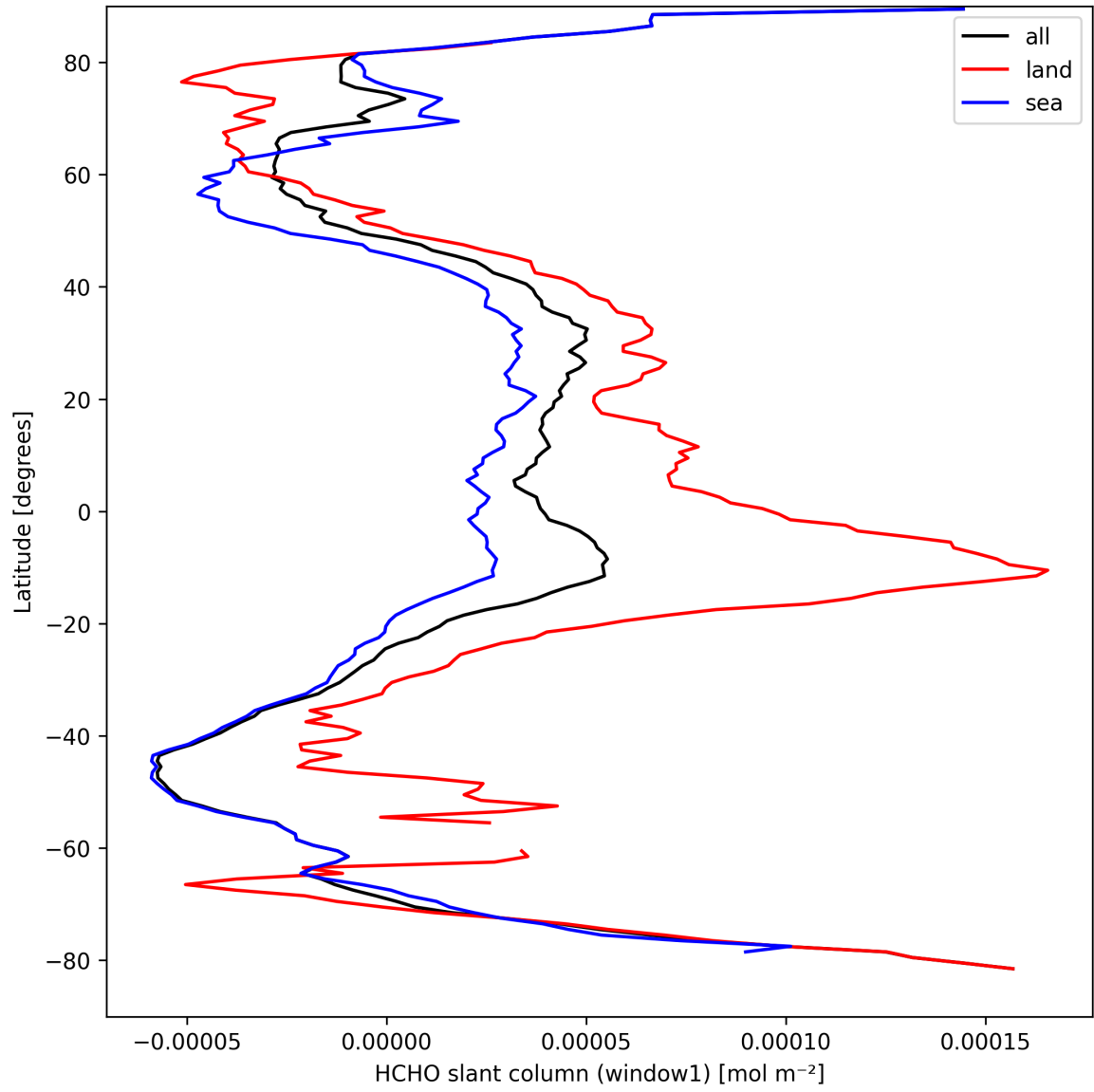
Figure 22: Zonal average of “HCHO slant column (window1)” for 2025-09-12 to 2025-09-13.
