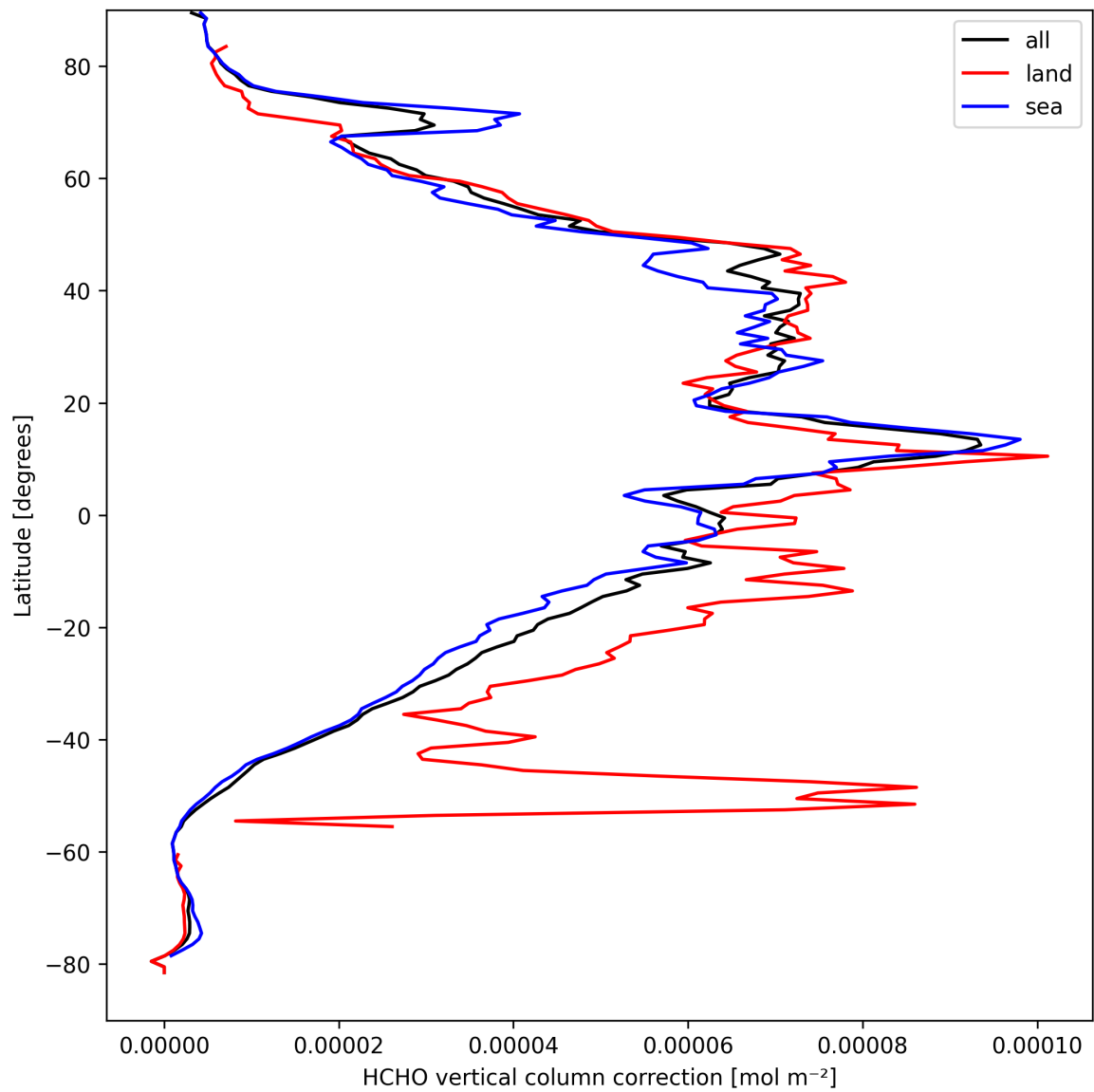
Figure 21: Zonal average of “HCHO vertical column correction” for 2025-09-12 to 2025-09-13.
