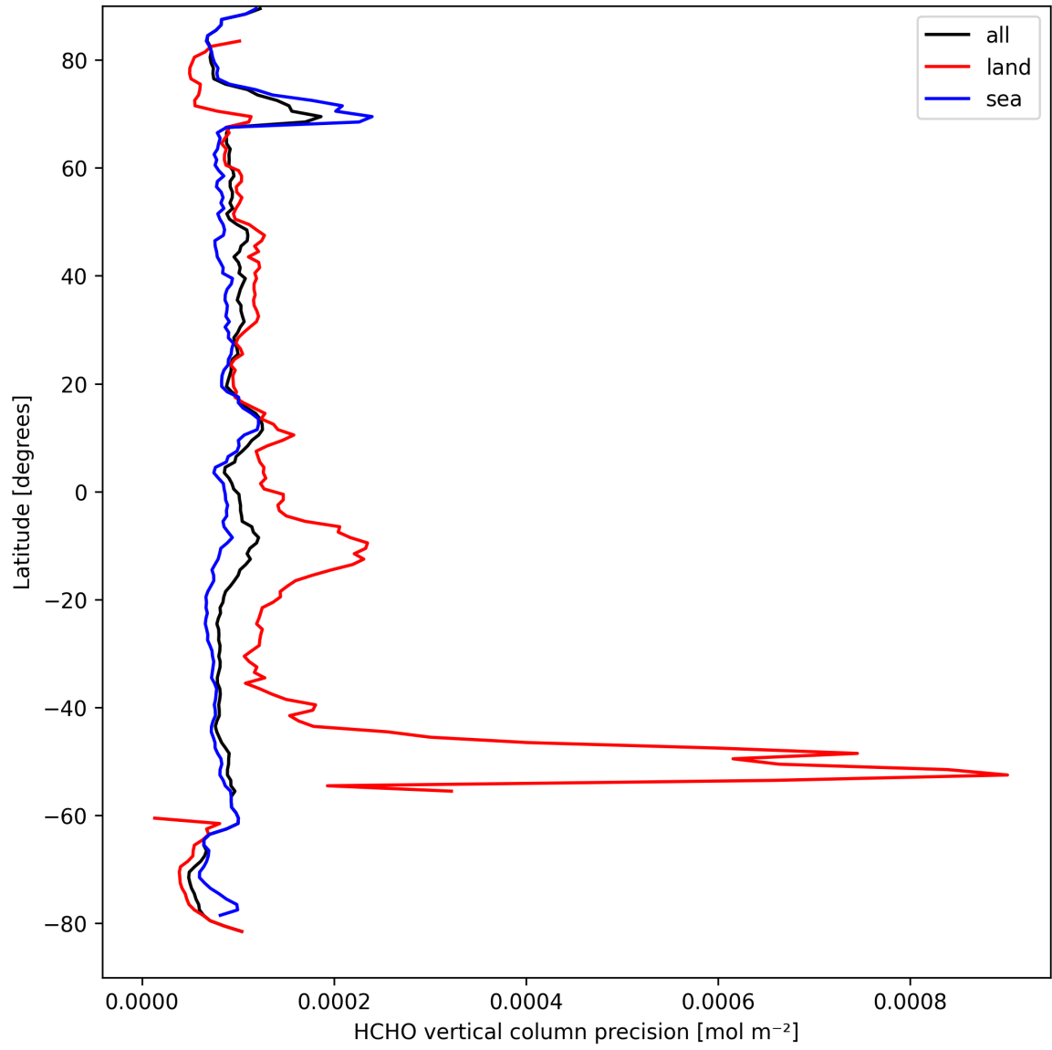
Figure 20: Zonal average of “HCHO vertical column precision” for 2025-09-12 to 2025-09-13.
