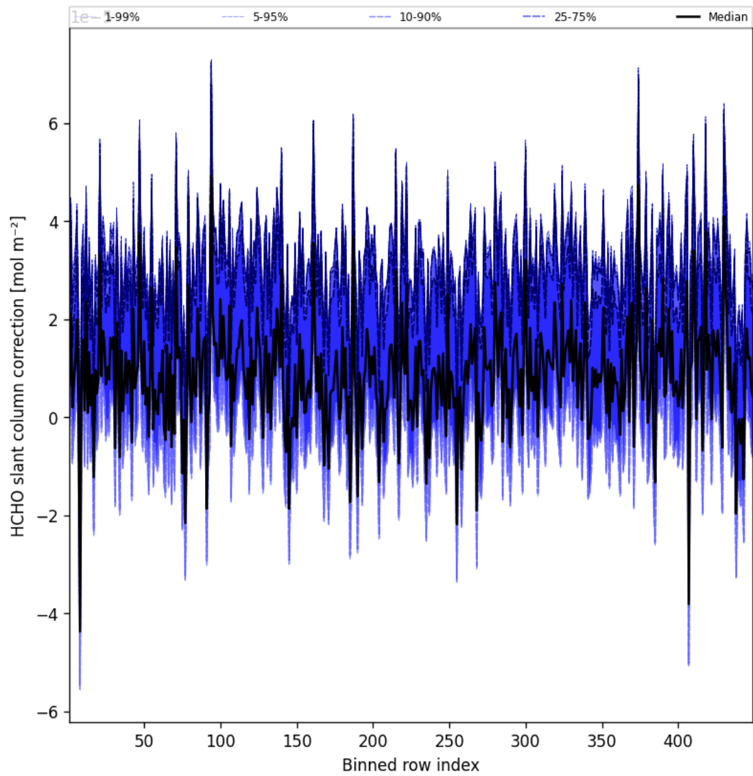
Figure 59: Along track statistics of “HCHO slant column correction” for 2025-09-12 to 2025-09-13
