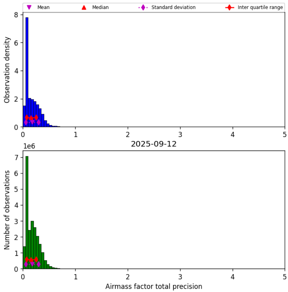
Figure 39: Histogram of “Airmass factor total precision” for 2025-09-12 to 2025-09-13
