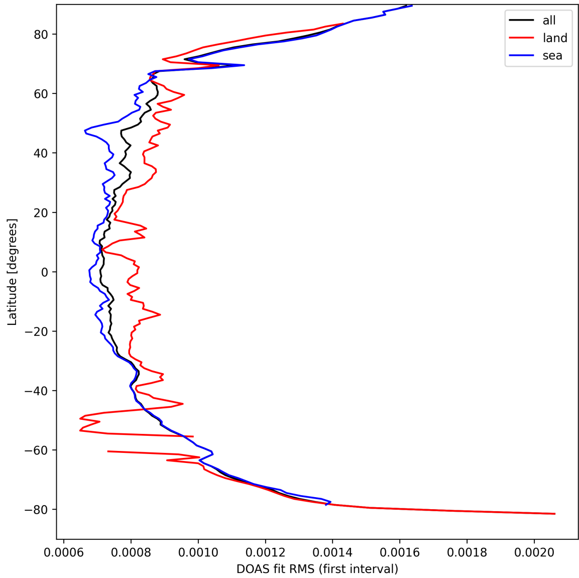
Figure 30: Zonal average of “DOAS fit RMS (first interval)” for 2025-09-12 to 2025-09-13.
