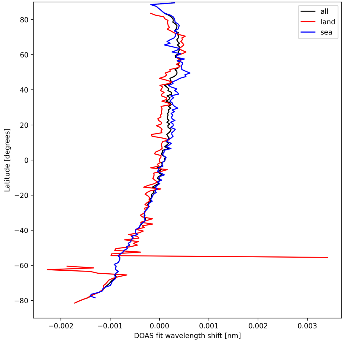
Figure 28: Zonal average of "DOAS fit wavelength shift" for 2025-09-12 to 2025-09-13.
