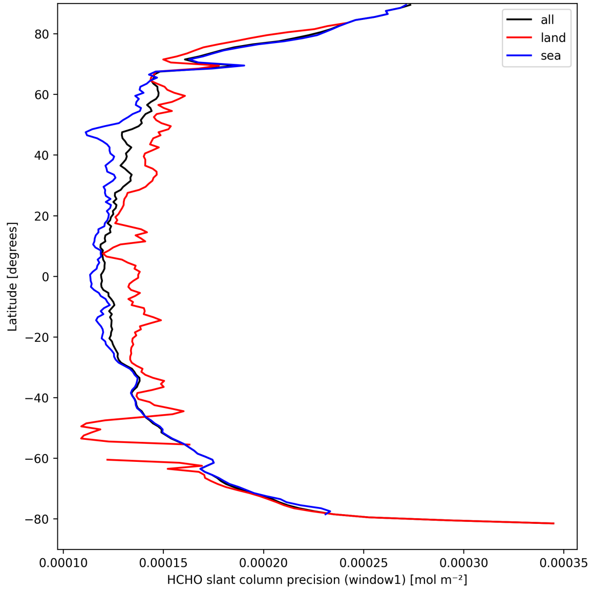
Figure 23: Zonal average of "HCHO slant column precision (window1)" for 2025-09-12 to 2025-09-13.
