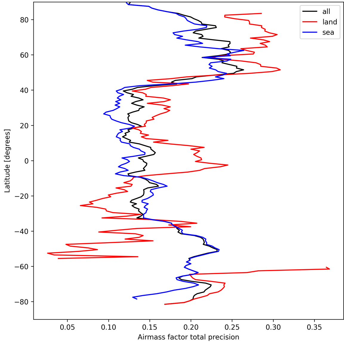
Figure 25: Zonal average of “Airmass factor total precision” for 2025-09-12 to 2025-09-13.
