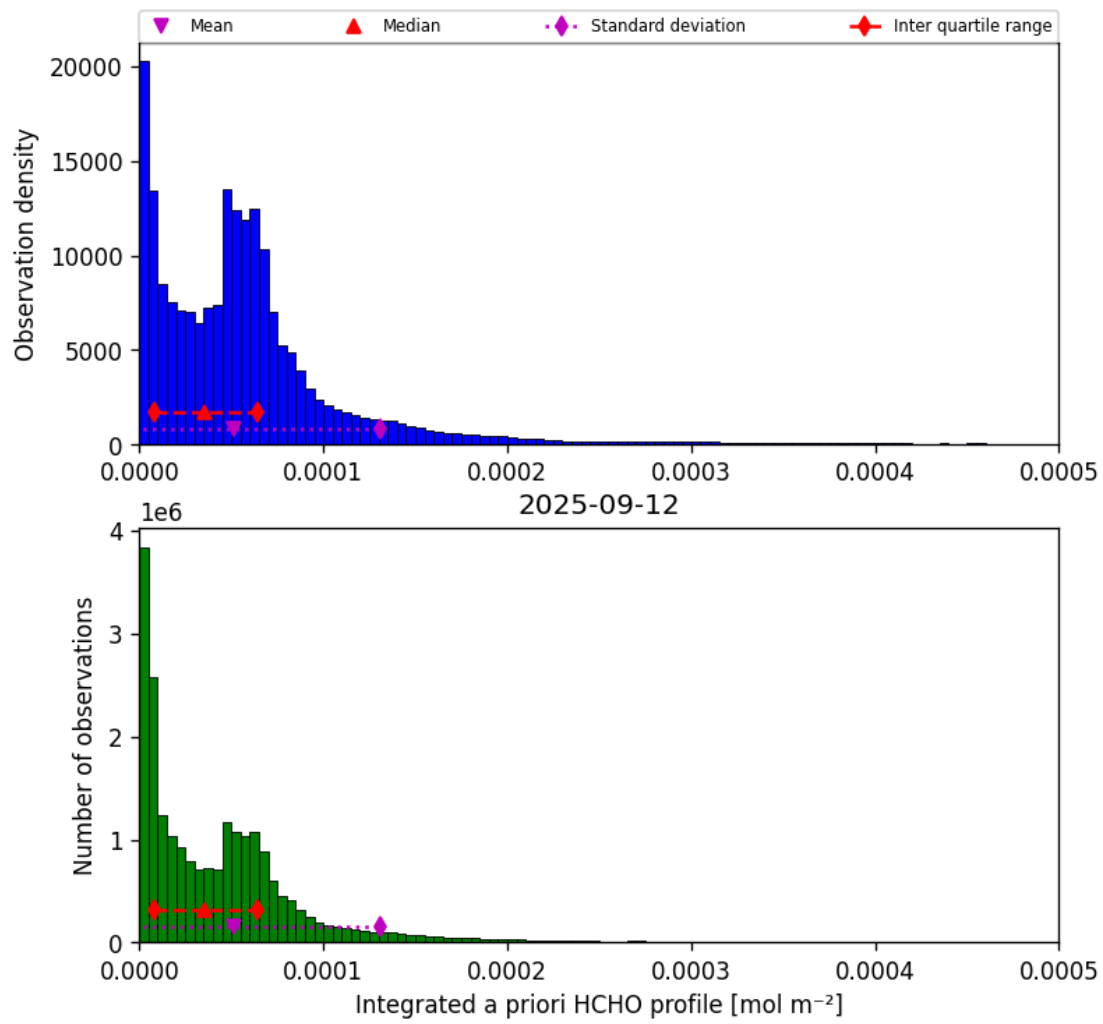
Figure 41: Histogram of “Integrated a priori HCHO profile” for 2025-09-12 to 2025-09-13
