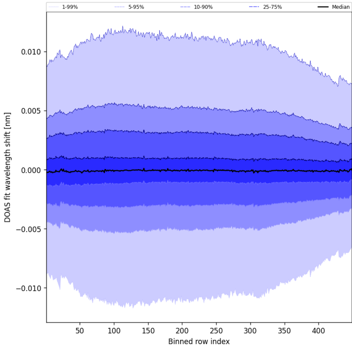
Figure 56: Along track statistics of “DOAS fit wavelength shift” for 2025-09-12 to 2025-09-13
