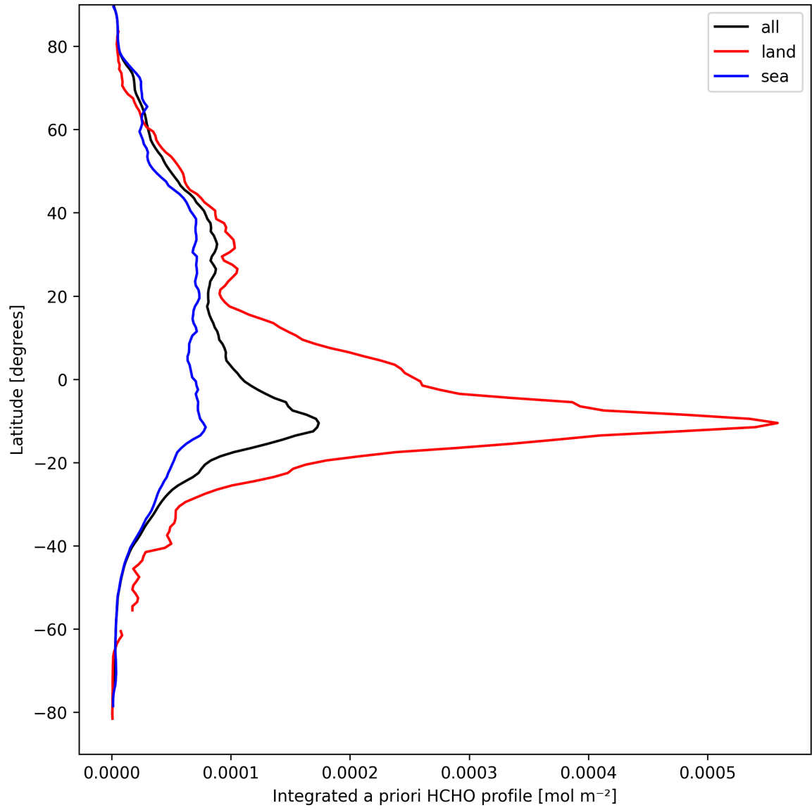
Figure 27: Zonal average of “Integrated a priori HCHO profile” for 2025-09-12 to 2025-09-13.
