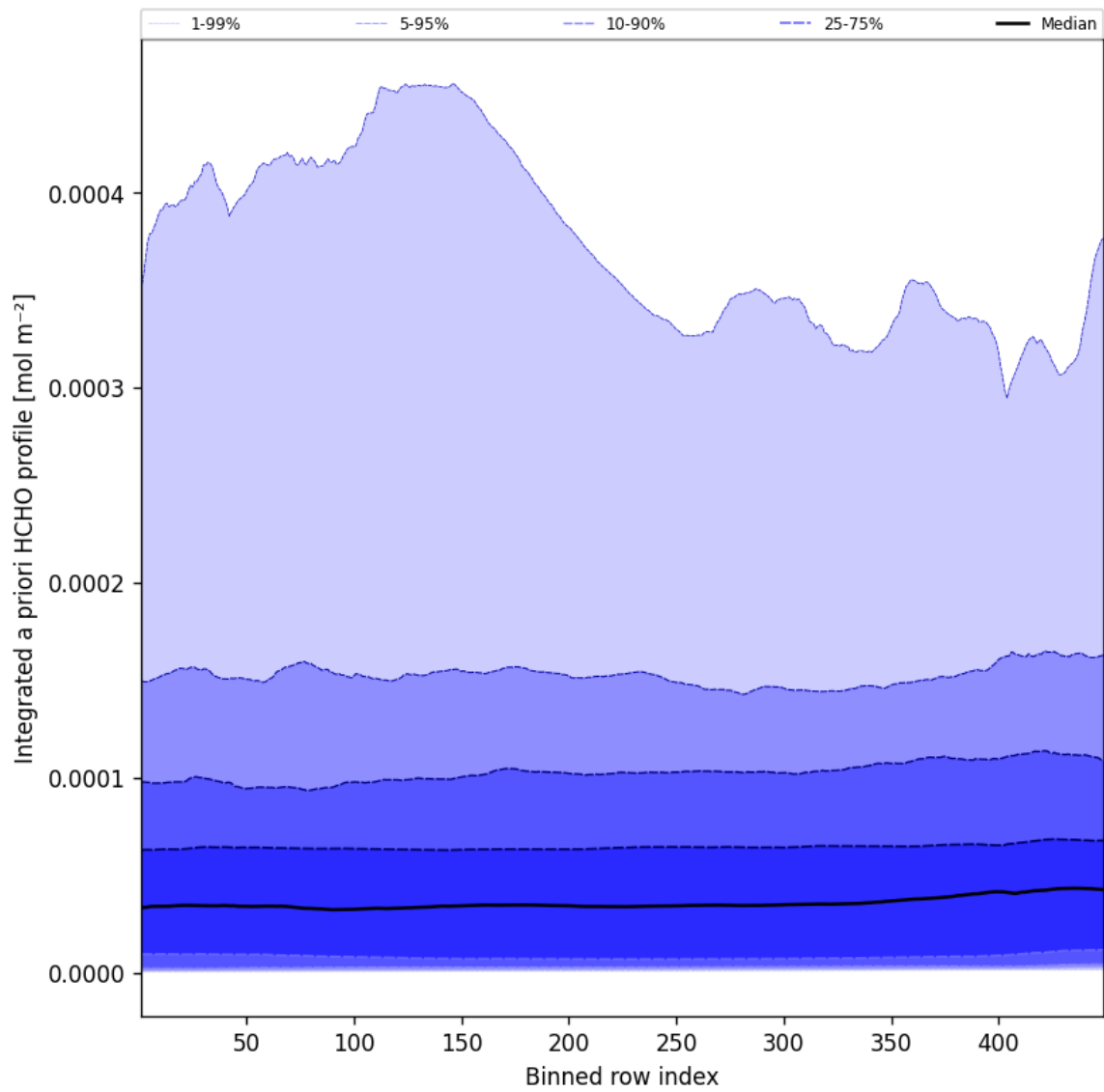
Figure 55: Along track statistics of “Integrated a priori HCHO profile” for 2025-09-12 to 2025-09-13
