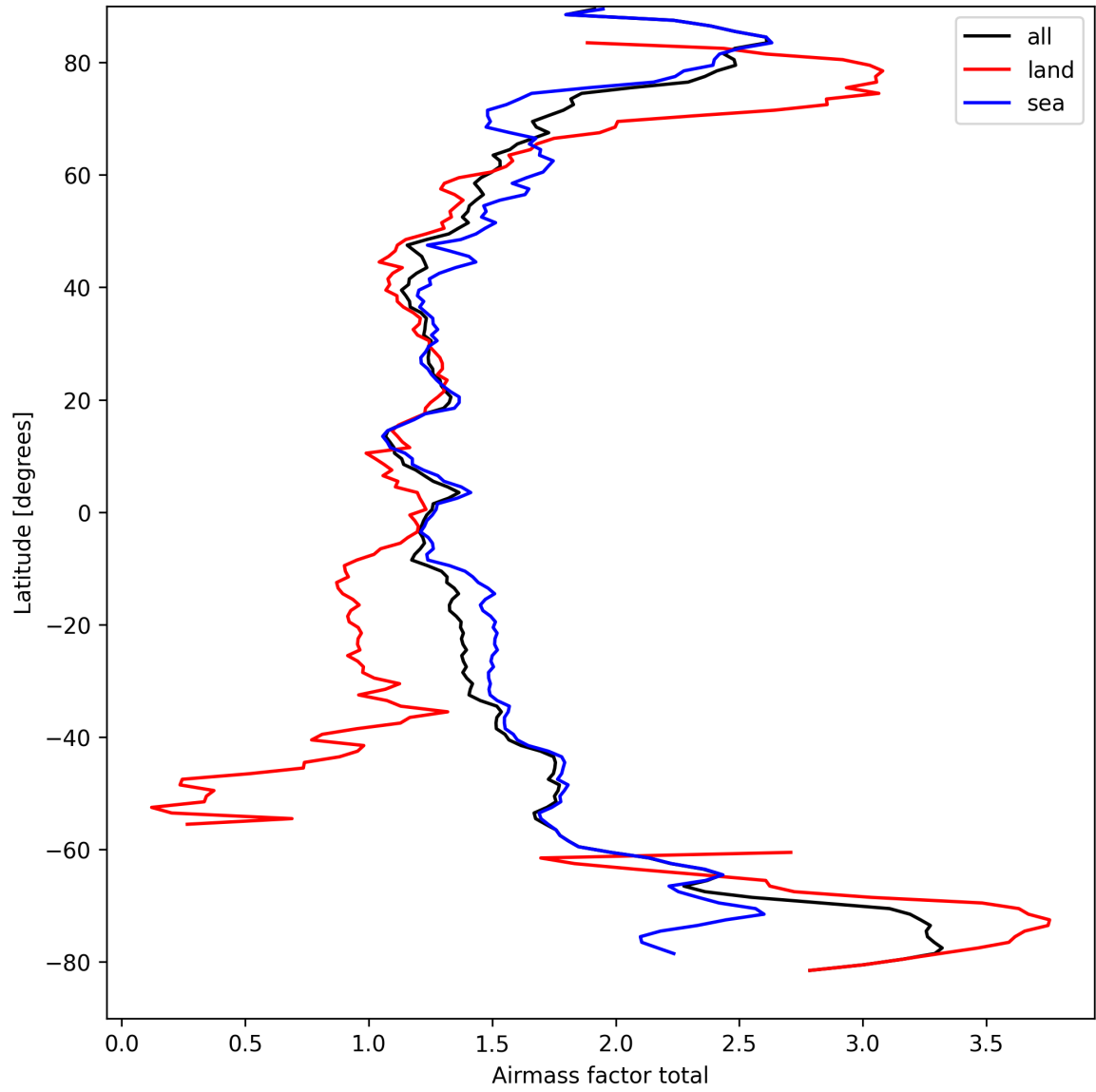
Figure 24: Zonal average of “Airmass factor total” for 2025-09-12 to 2025-09-13.
