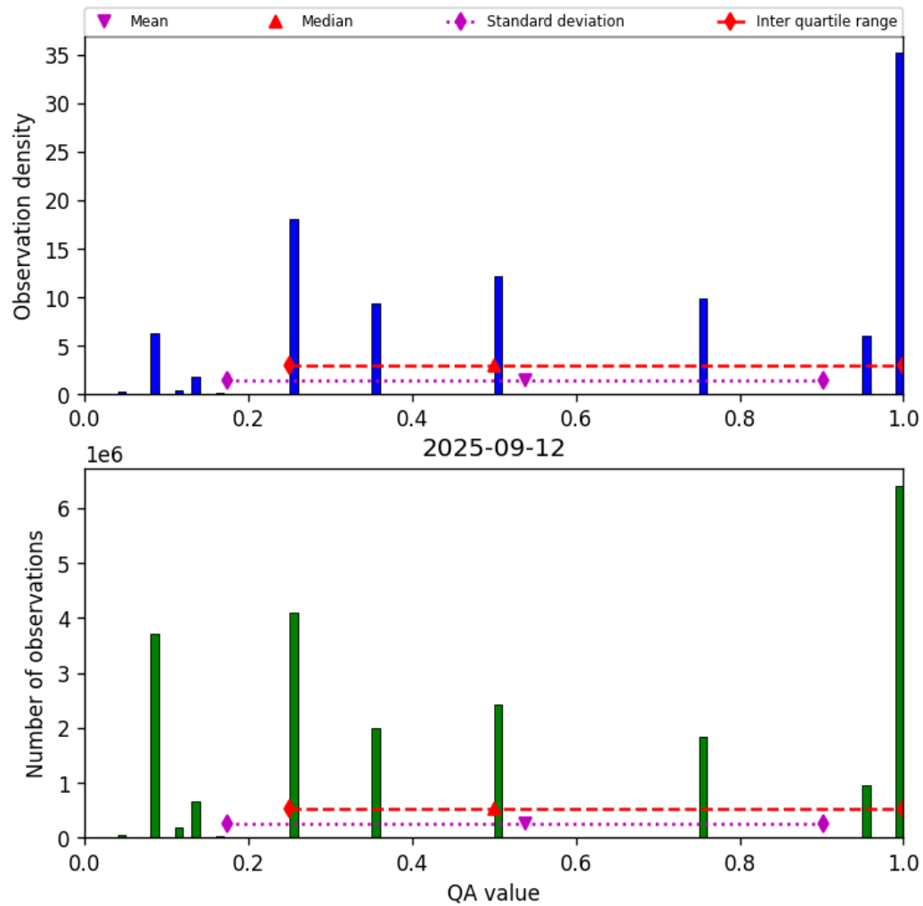
Figure 32: Histogram of “QA value” for 2025-09-12 to 2025-09-13
