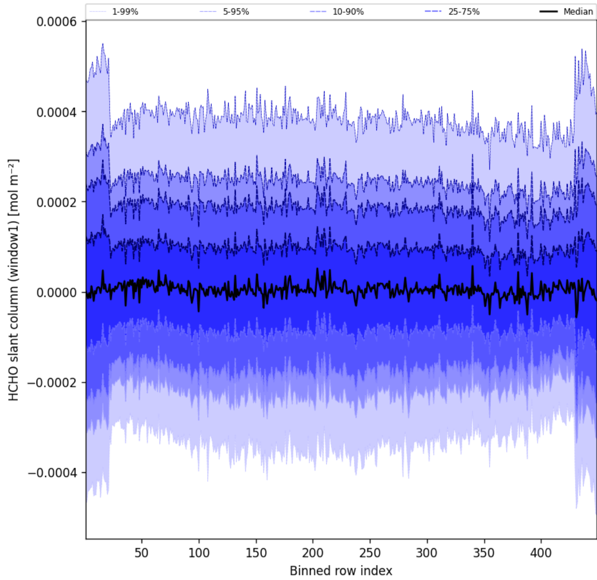
Figure 50: Along track statistics of “HCHO slant column (window1)” for 2025-09-12 to 2025-09-13
