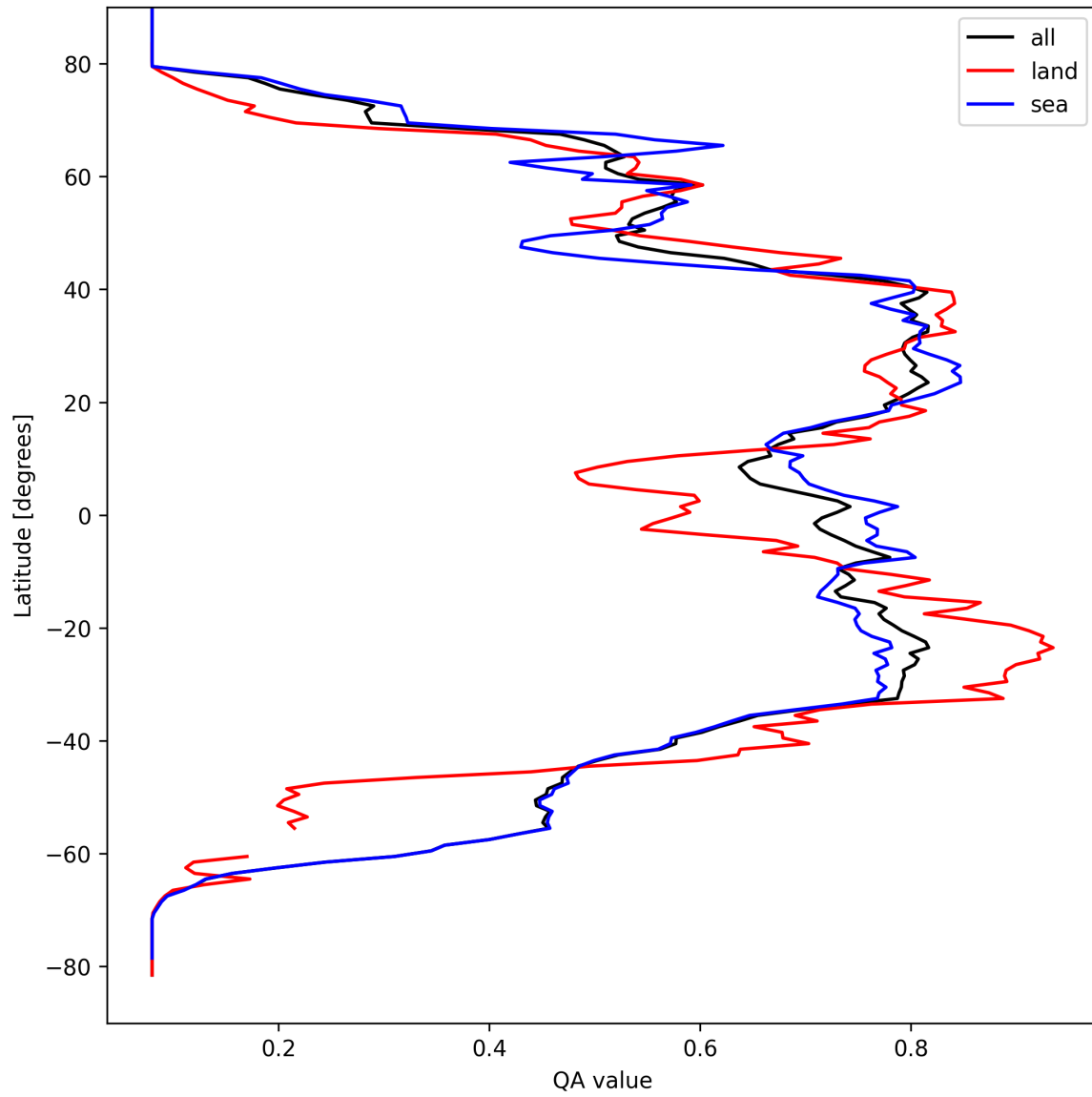
Figure 18: Zonal average of “QA value” for 2025-09-12 to 2025-09-13.
