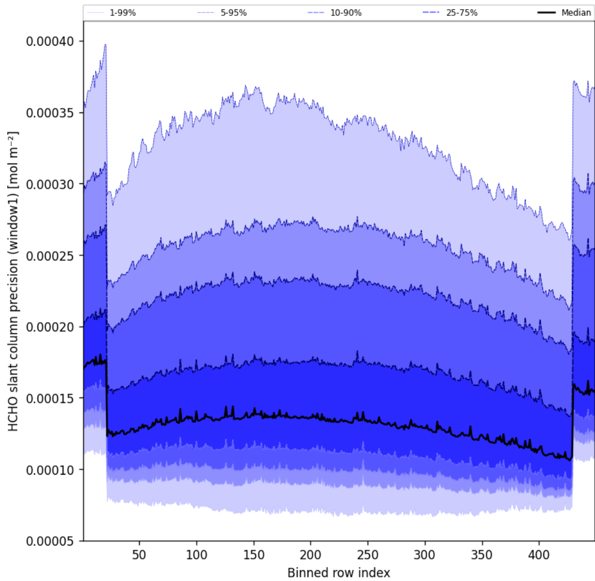
Figure 51: Along track statistics of “HCHO slant column precision (window1)” for 2025-09-12 to 2025-09-13
