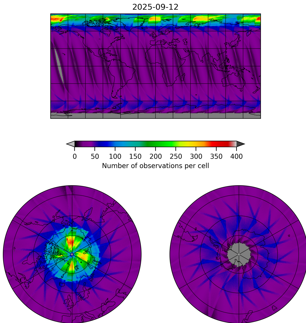
Figure 17: Map of the number of observations for 2025-09-12 to 2025-09-13
