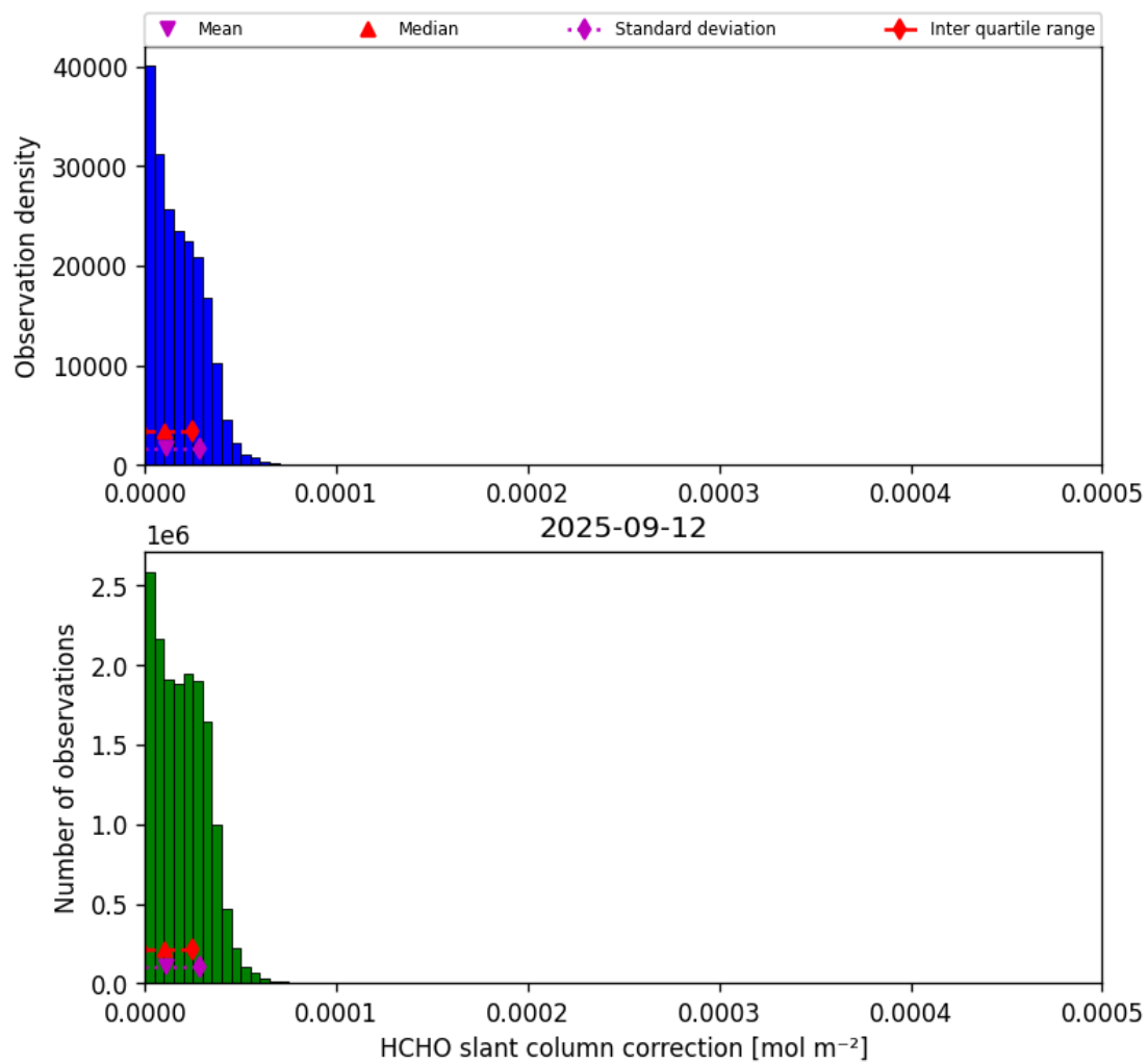
Figure 45: Histogram of “HCHO slant column correction” for 2025-09-12 to 2025-09-13
