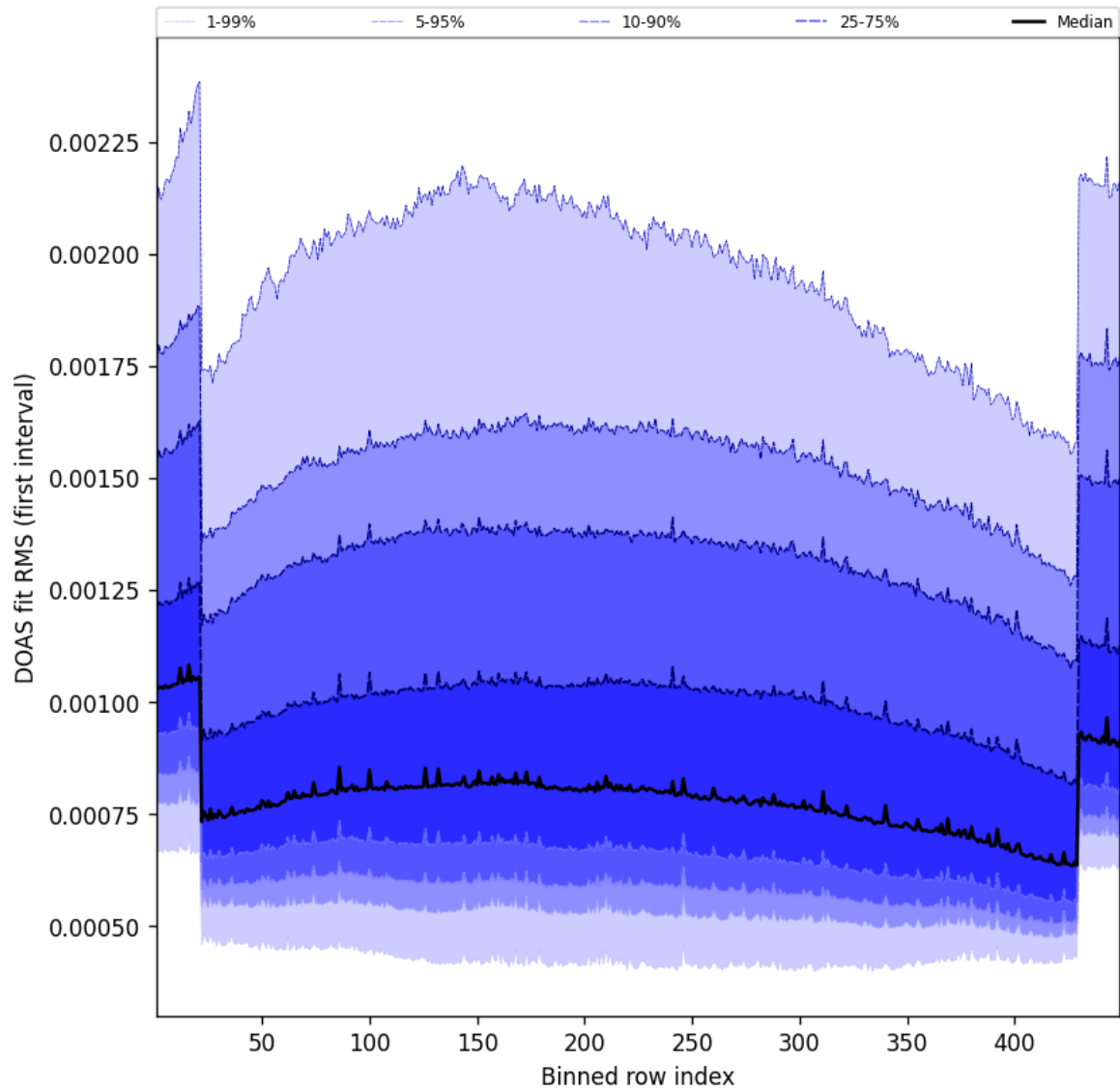
Figure 58: Along track statistics of “DOAS fit RMS (first interval)” for 2025-09-12 to 2025-09-13
