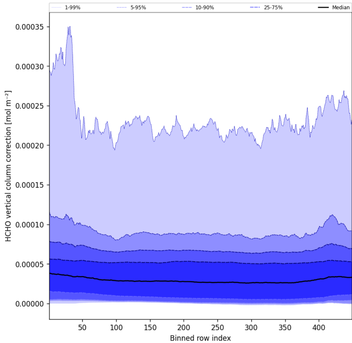
Figure 49: Along track statistics of “HCHO vertical column correction” for 2025-09-12 to 2025-09-13
