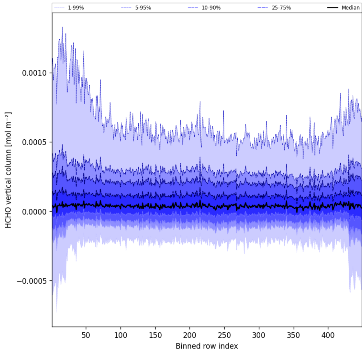
Figure 47: Along track statistics of “HCHO vertical column” for 2025-09-12 to 2025-09-13
