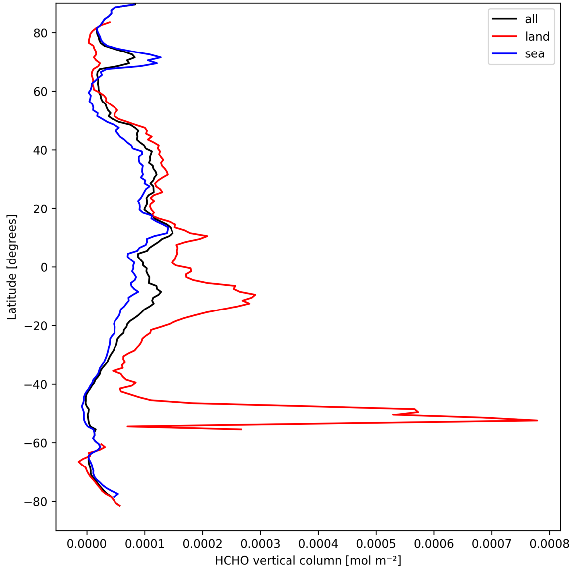
Figure 19: Zonal average of “HCHO vertical column” for 2025-09-12 to 2025-09-13.
