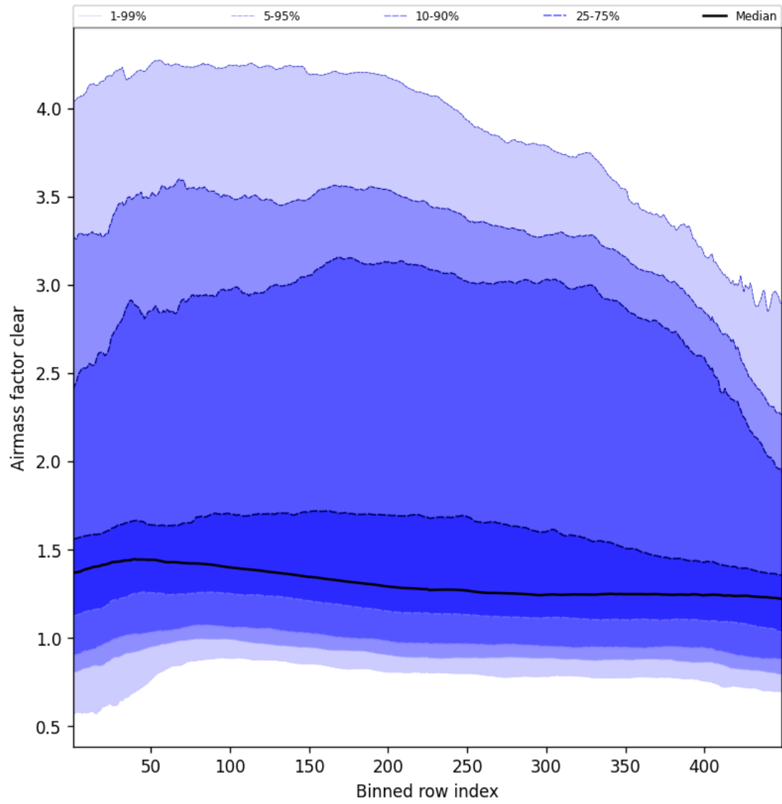
Figure 54: Along track statistics of “Air mass factor clear” for 2025-09-12 to 2025-09-13
