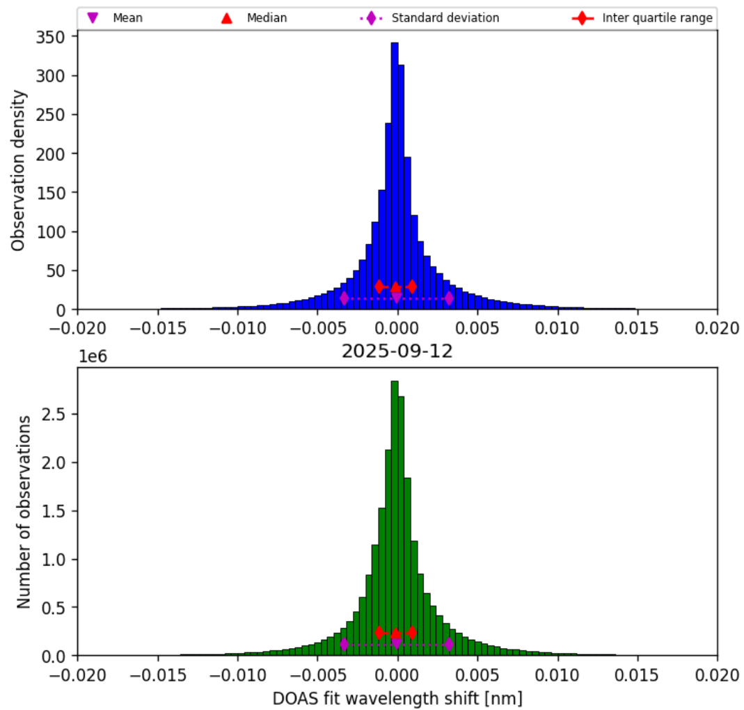
Figure 42: Histogram of “DOAS fit wavelength shift” for 2025-09-12 to 2025-09-13
