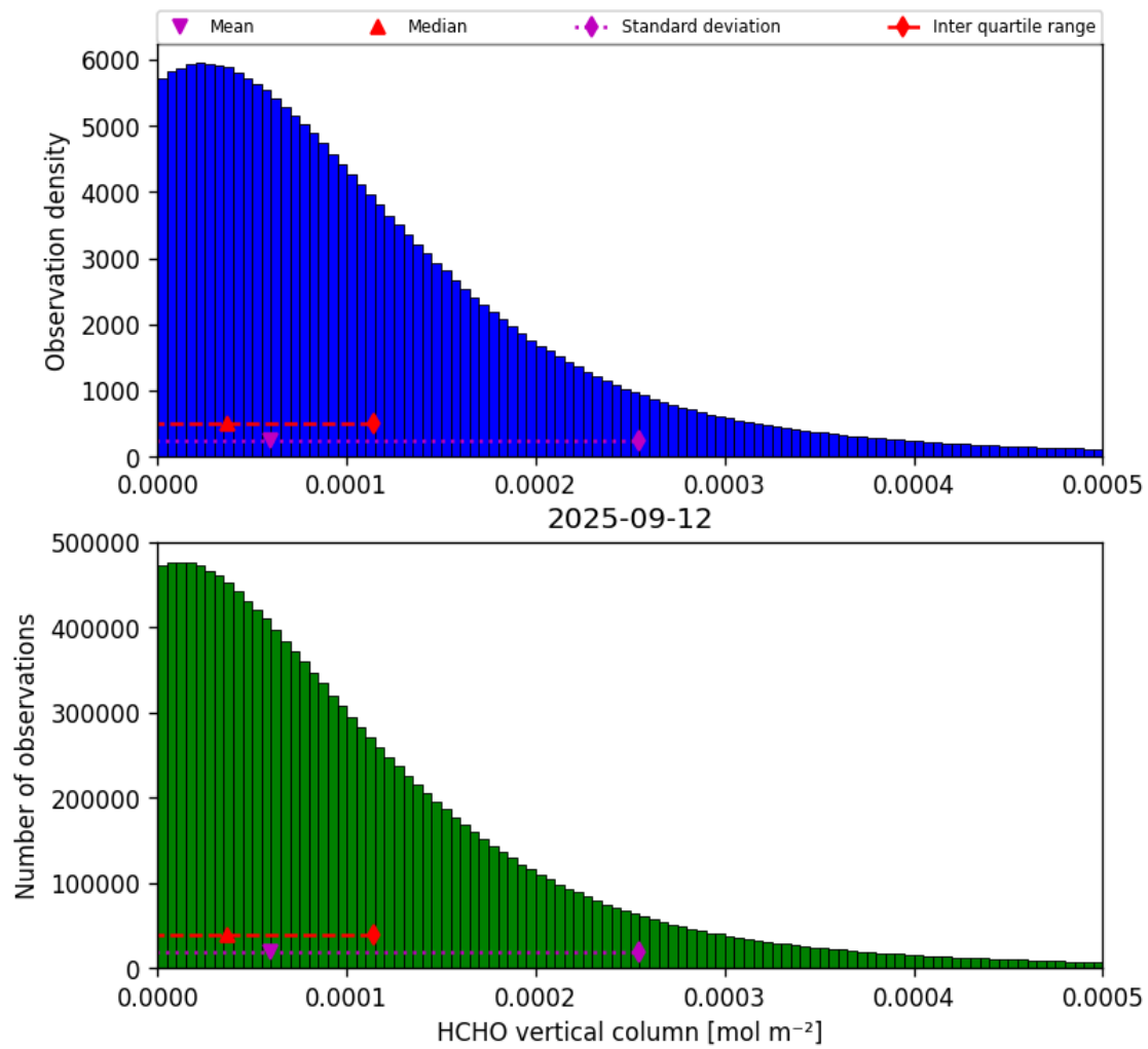
Figure 33: Histogram of “HCHO vertical column” for 2025-09-12 to 2025-09-13
