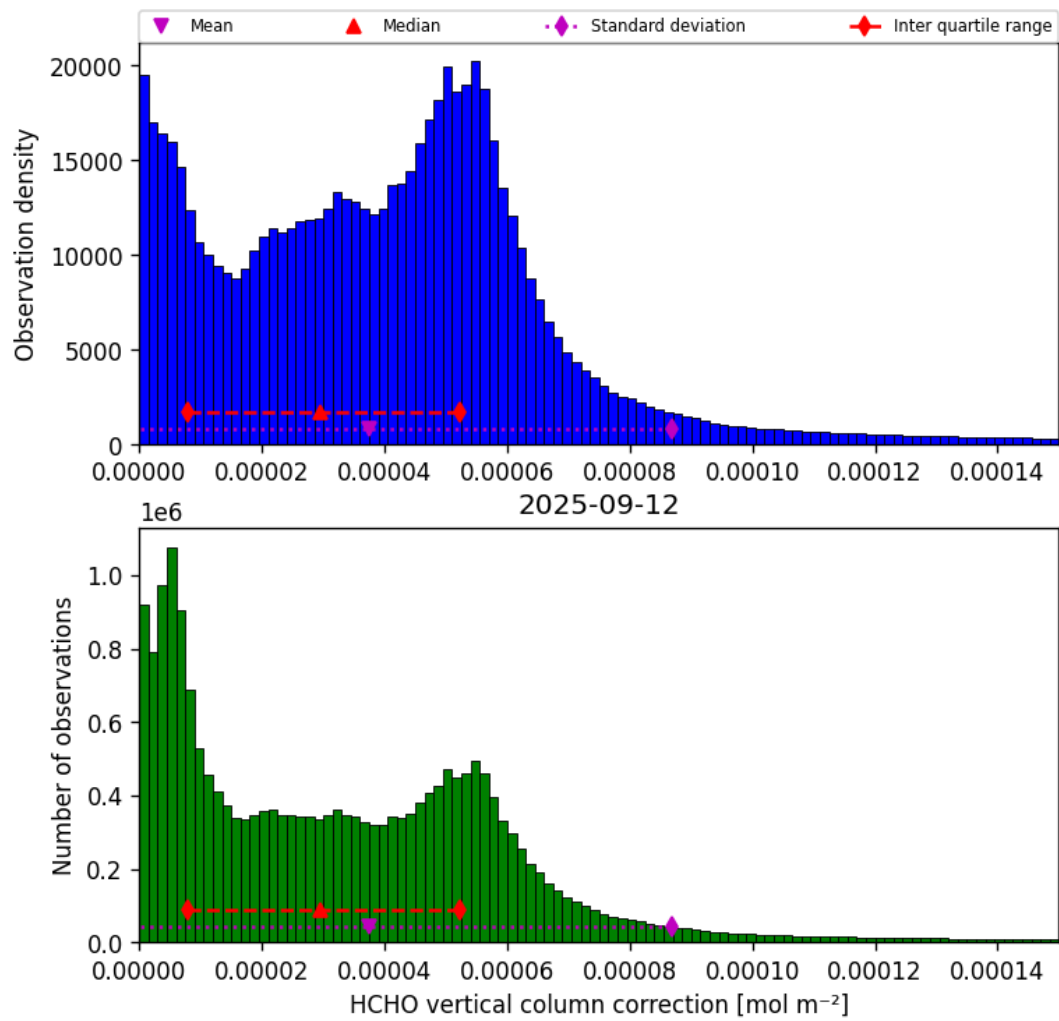
Figure 35: Histogram of “HCHO vertical column correction” for 2025-09-12 to 2025-09-13
