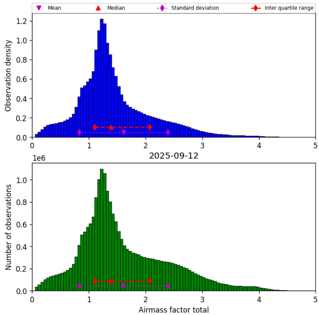
Figure 38: Histogram of “Airmass factor total” for 2025-09-12 to 2025-09-13
