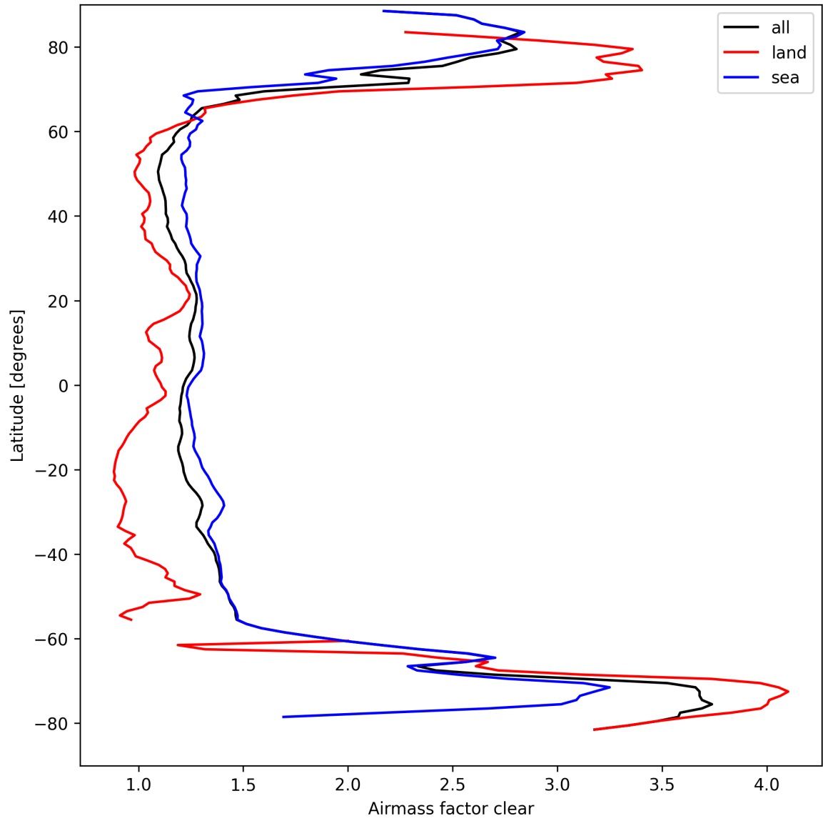
Figure 26: Zonal average of “Airmass factor clear” for 2025-09-14 to 2025-09-15.
