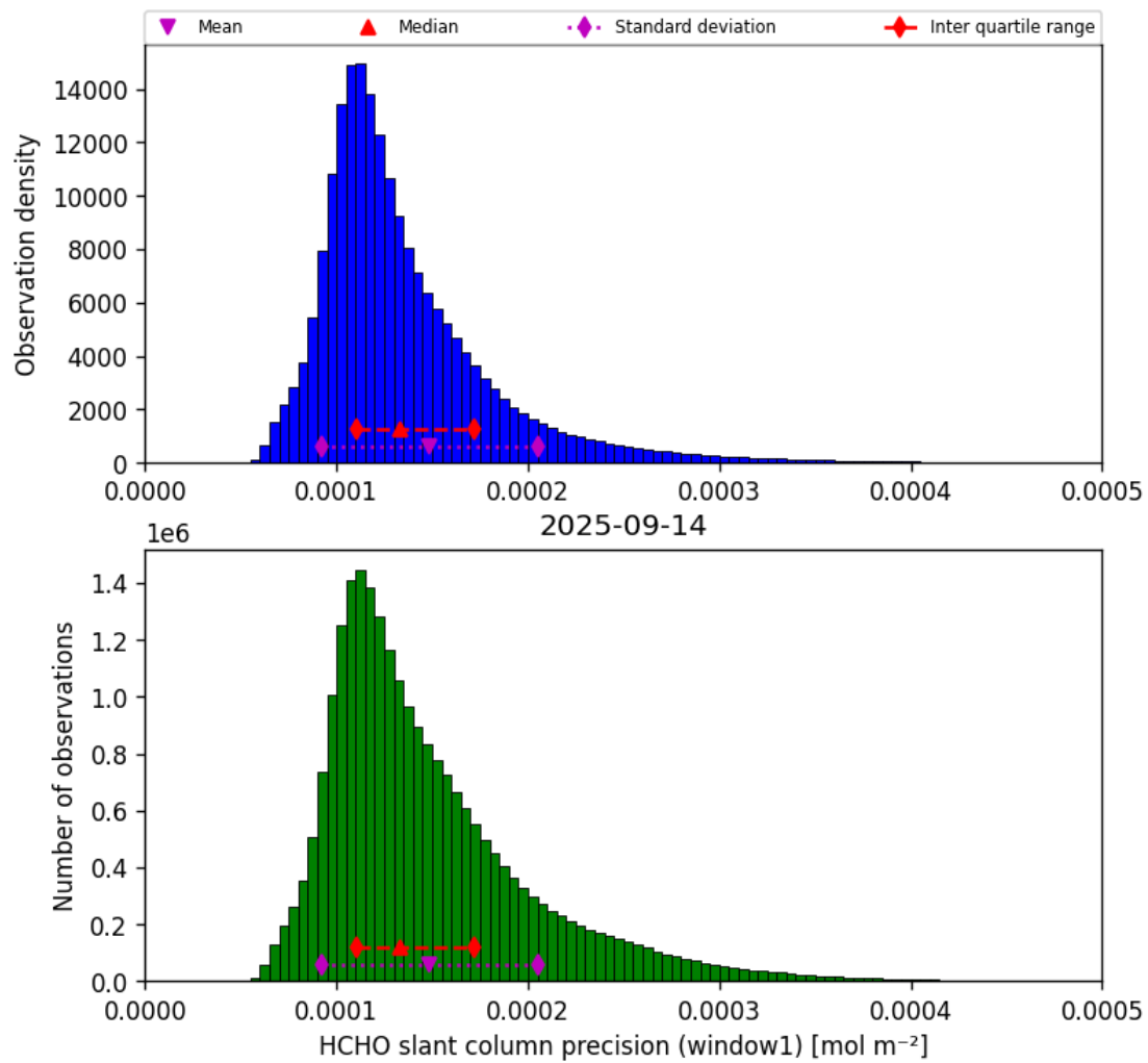
Figure 37: Histogram of “HCHO slant column precision (window1)” for 2025-09-14 to 2025-09-15
