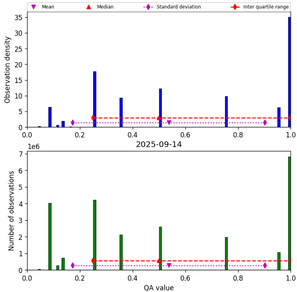
Figure 32: Histogram of “QA value” for 2025-09-14 to 2025-09-15
