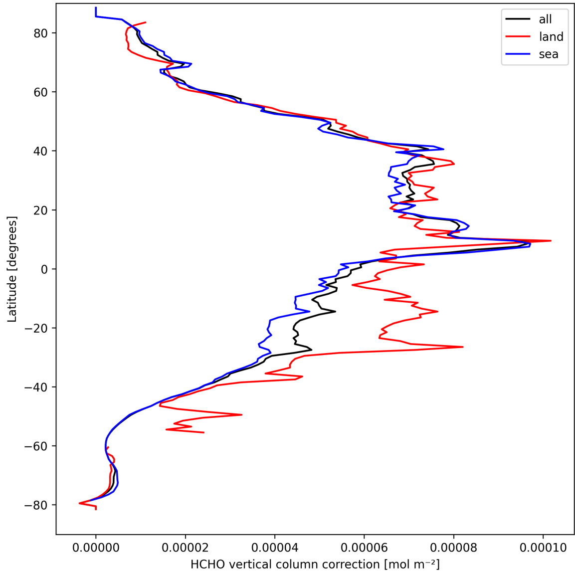
Figure 21: Zonal average of “HCHO vertical column correction” for 2025-09-14 to 2025-09-15.
