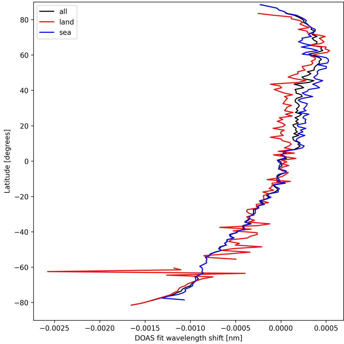
Figure 28: Zonal average of “DOAS fit wavelength shift” for 2025-09-14 to 2025-09-15.
