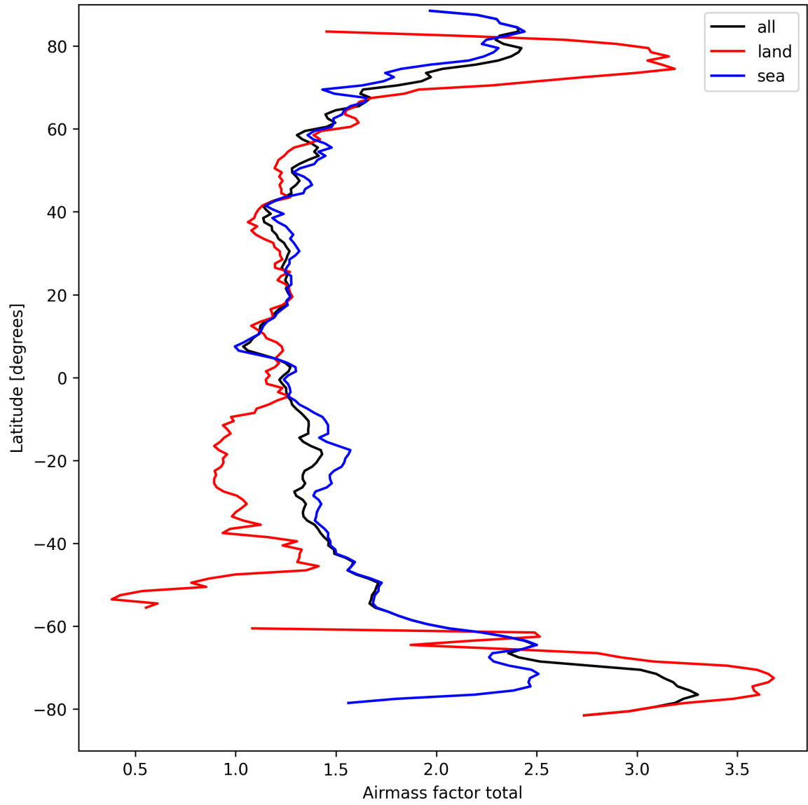
Figure 24: Zonal average of “Airmass factor total” for 2025-09-14 to 2025-09-15.
