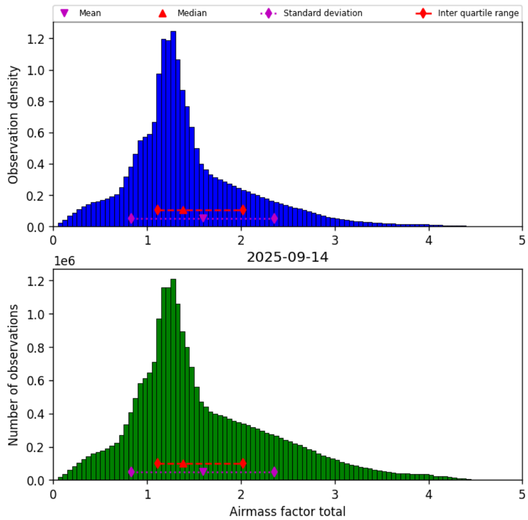
Figure 38: Histogram of “Airmass factor total” for 2025-09-14 to 2025-09-15
