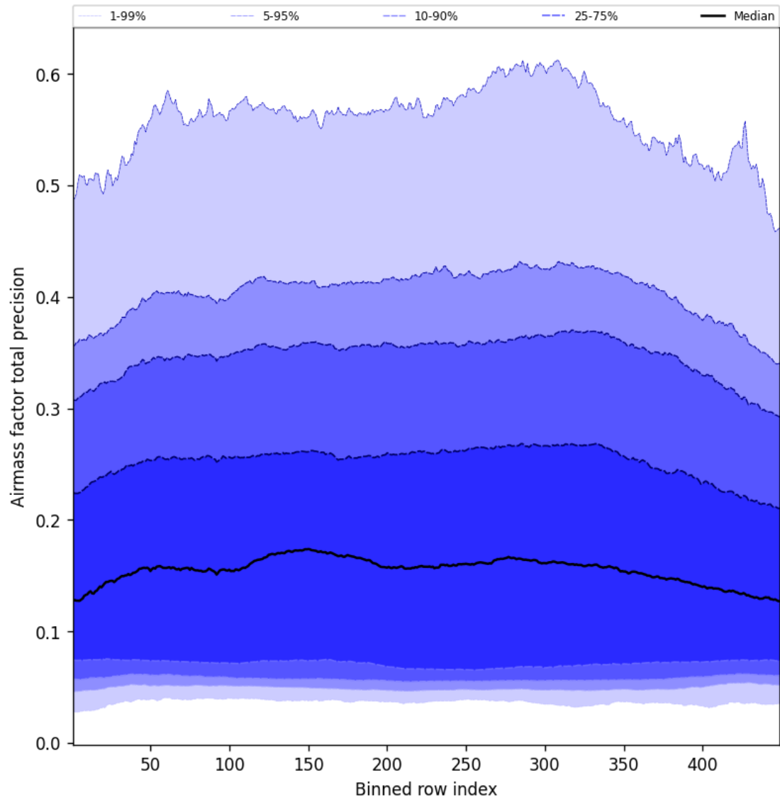
Figure 53: Along track statistics of “Airmass factor total precision” for 2025-09-14 to 2025-09-15
