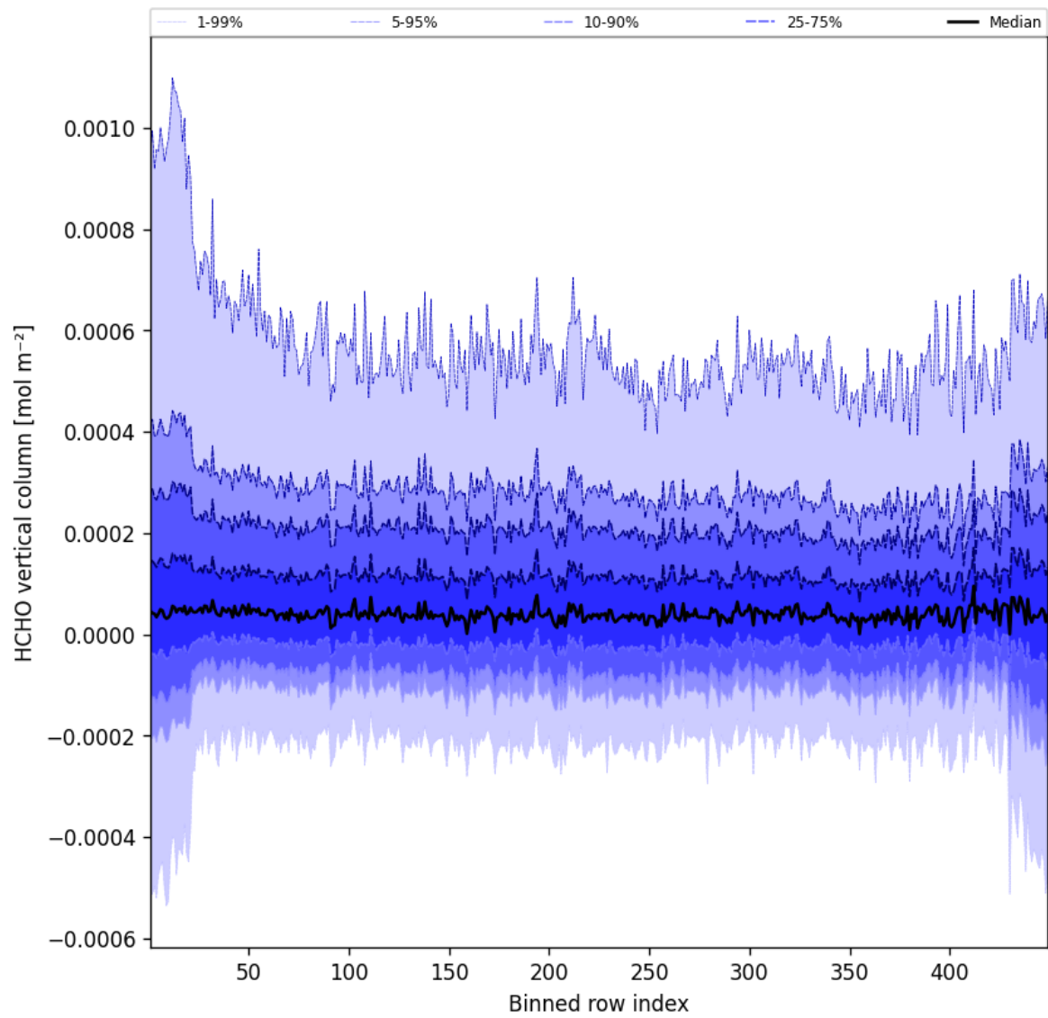
Figure 47: Along track statistics of “HCHO vertical column” for 2025-09-14 to 2025-09-15
