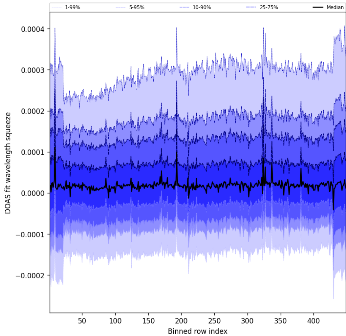
Figure 57: Along track statistics of “DOAS fit wavelength squeeze” for 2025-09-14 to 2025-09-15
