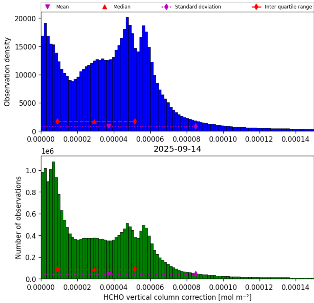
Figure 35: Histogram of “HCHO vertical column correction” for 2025-09-14 to 2025-09-15
