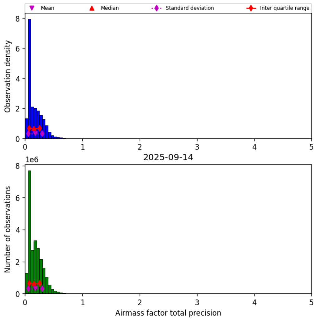
Figure 39: Histogram of “Airmass factor total precision” for 2025-09-14 to 2025-09-15
