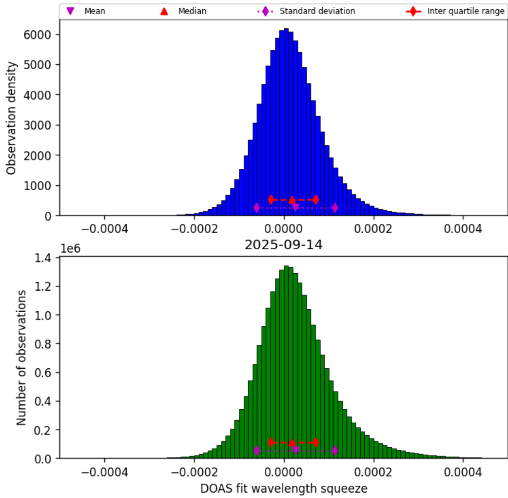
Figure 43: Histogram of “DOAS fit wavelength squeeze” for 2025-09-14 to 2025-09-15
