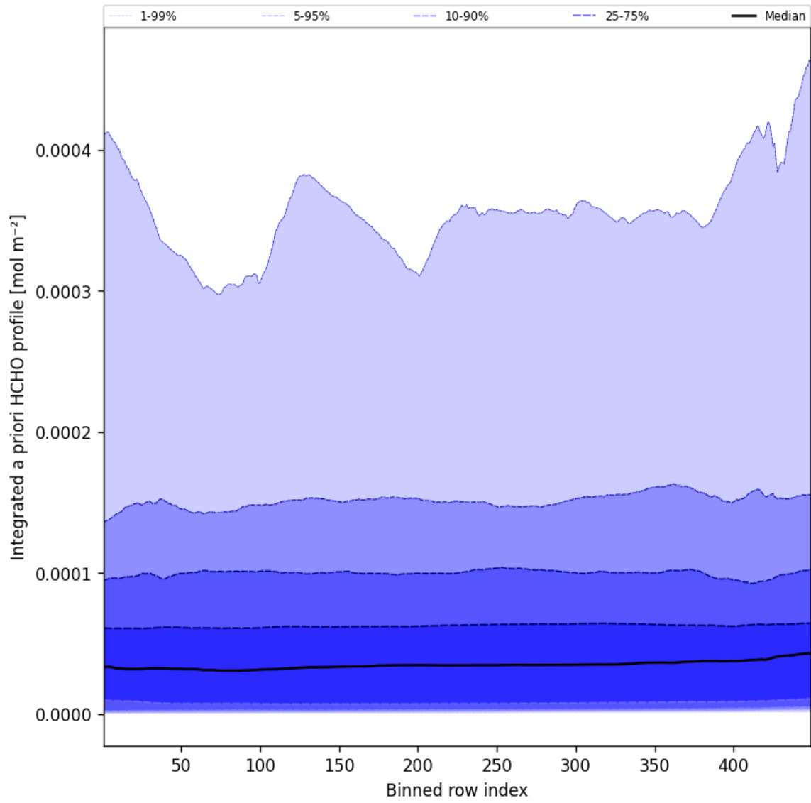
Figure 55: Along track statistics of “Integrated a priori HCHO profile” for 2025-09-14 to 2025-09-15
