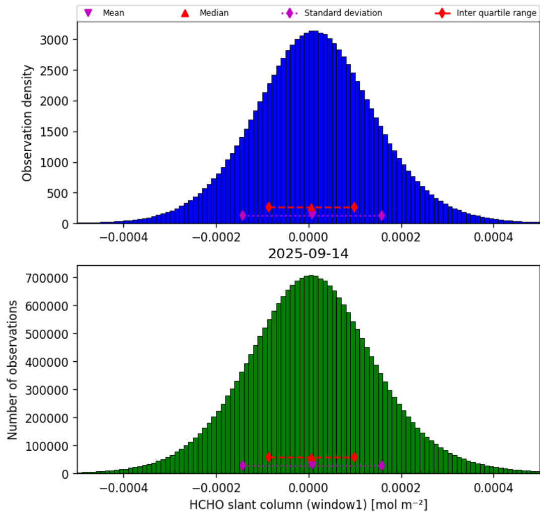
Figure 36: Histogram of “HCHO slant column (window1)” for 2025-09-14 to 2025-09-15
