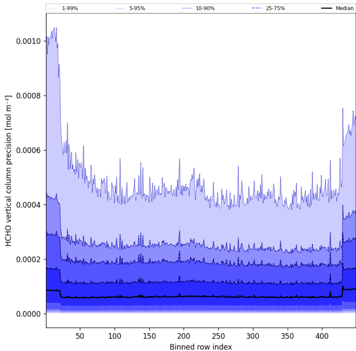
Figure 48: Along track statistics of “HCHO vertical column precision” for 2025-09-14 to 2025-09-15
