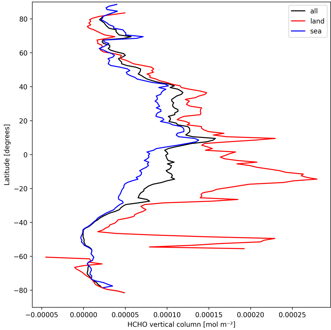
Figure 19: Zonal average of “HCHO vertical column” for 2025-09-14 to 2025-09-15.
