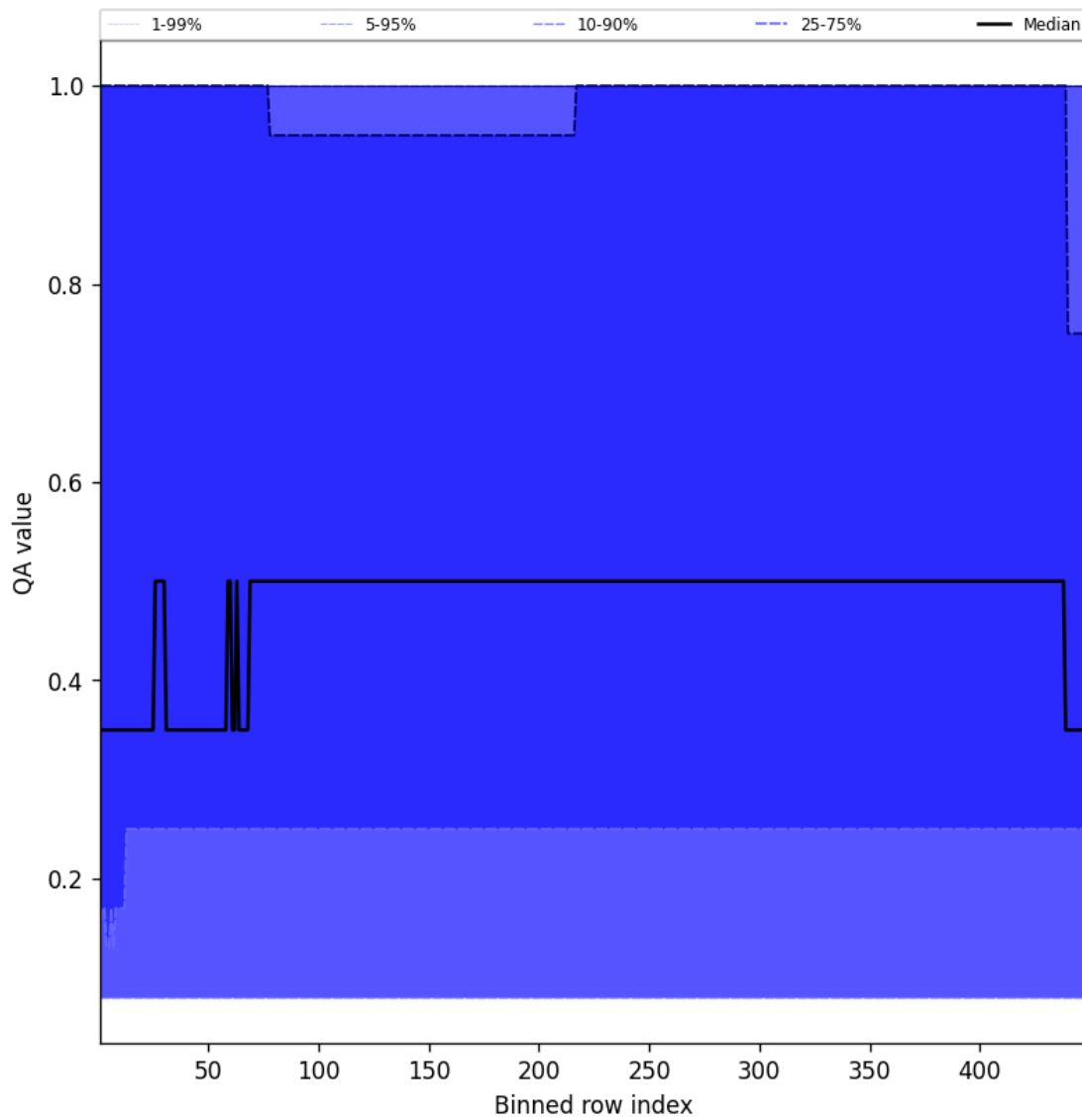
Figure 46: Along track statistics of “QA value” for 2025-09-14 to 2025-09-15
