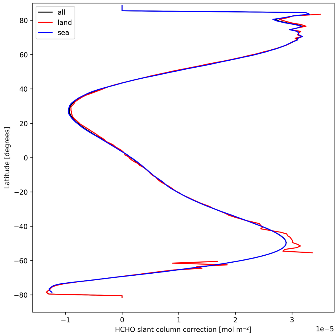
Figure 31: Zonal average of “HCHO slant column correction” for 2025-09-14 to 2025-09-15.
