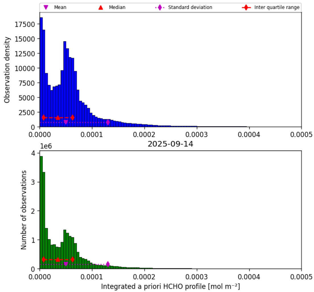
Figure 41: Histogram of “Integrated a priori HCHO profile” for 2025-09-14 to 2025-09-15
