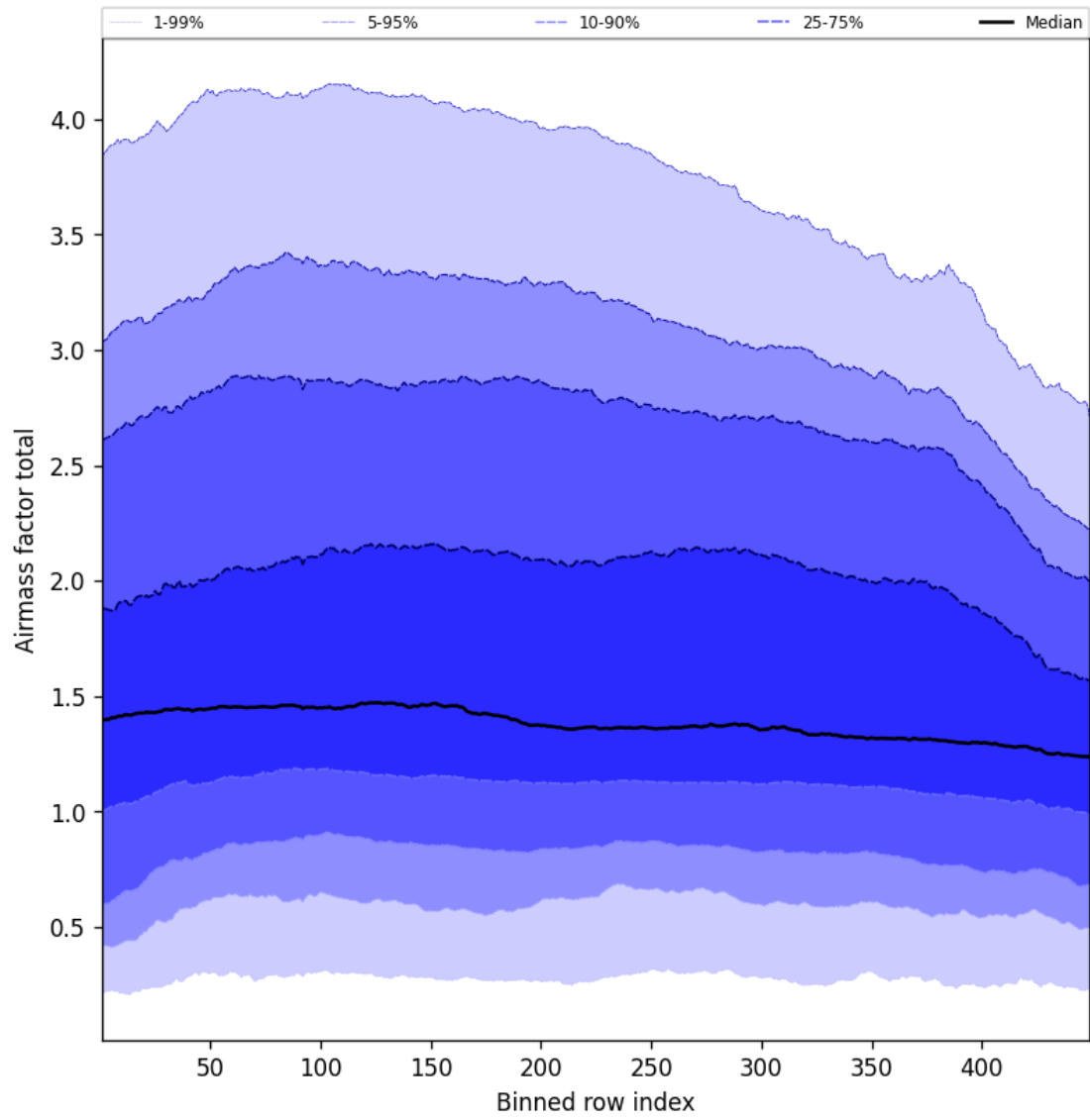
Figure 52: Along track statistics of “Airmass factor total” for 2025-09-14 to 2025-09-15
