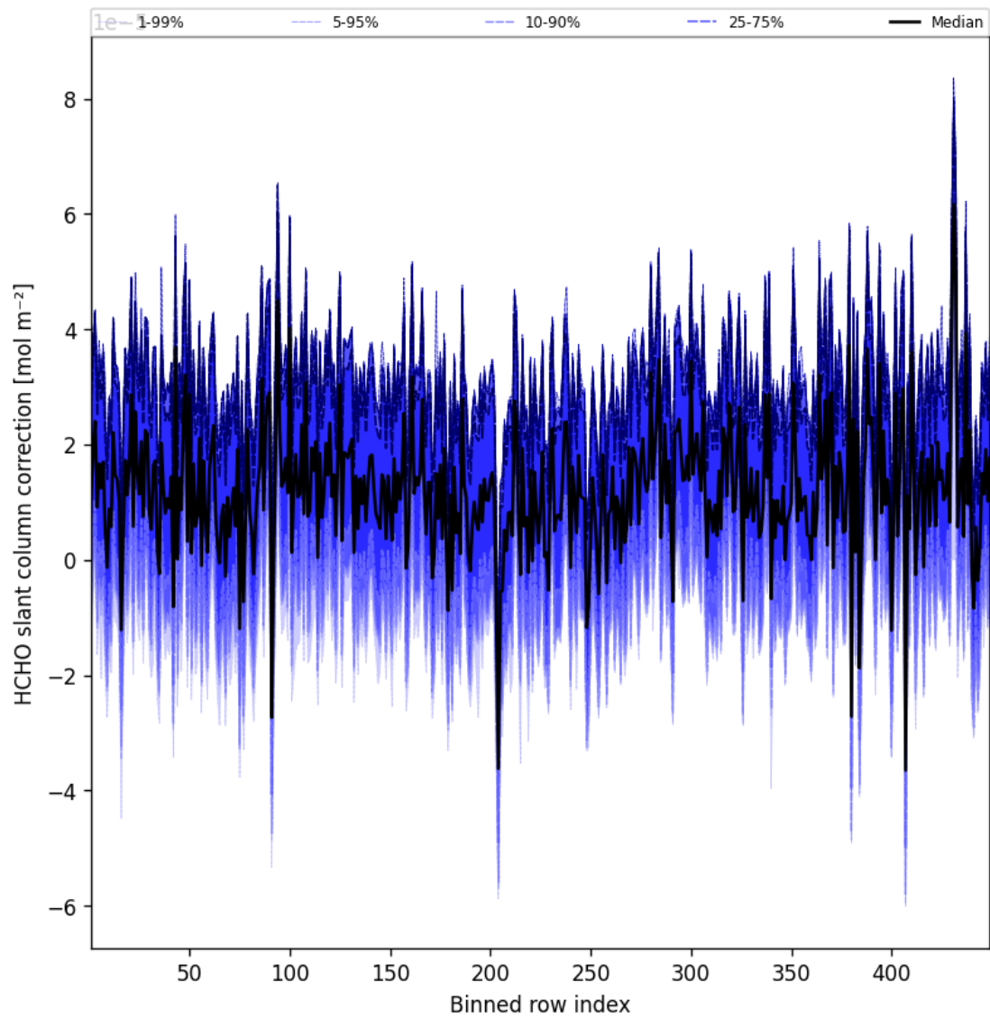
Figure 59: Along track statistics of “HCHO slant column correction” for 2025-09-14 to 2025-09-15
