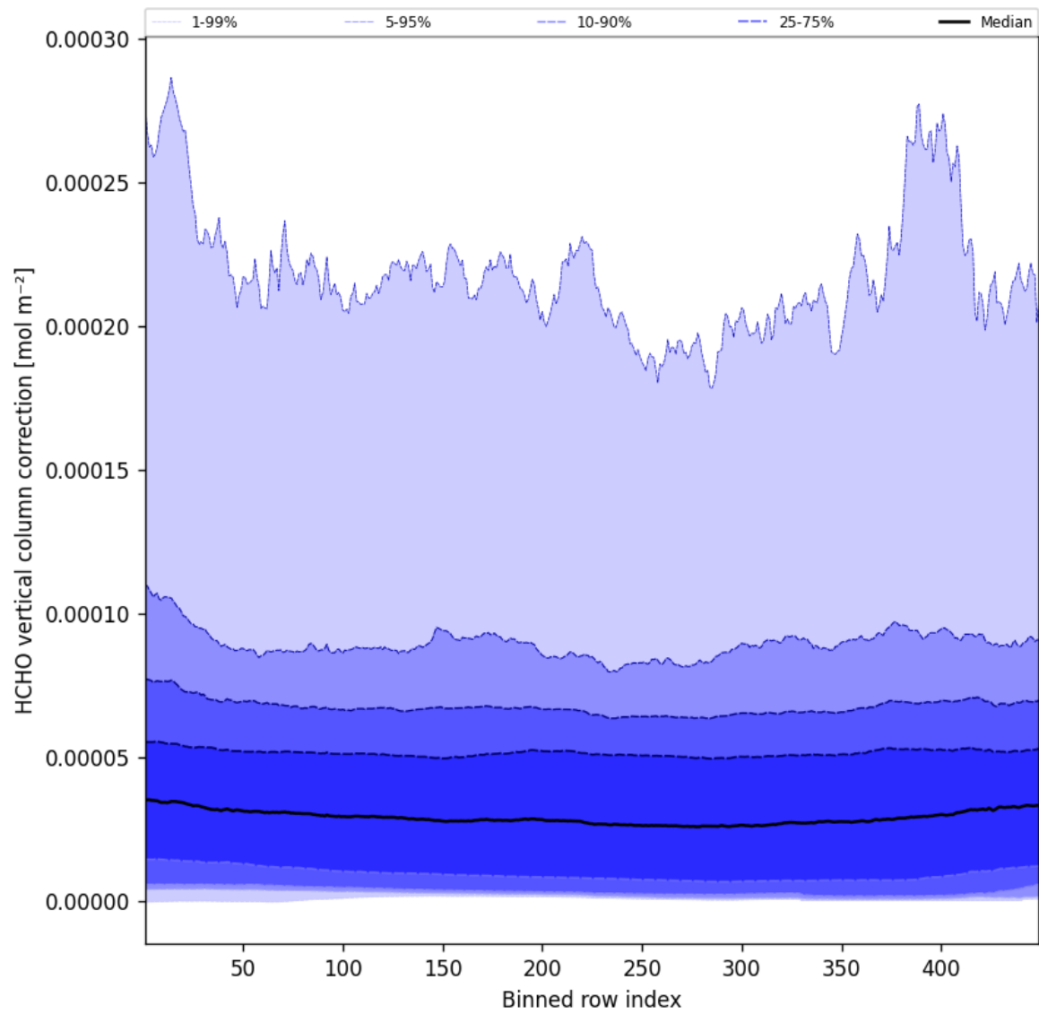
Figure 49: Along track statistics of "HCHO vertical column correction" for 2025-09-14 to 2025-09-15
