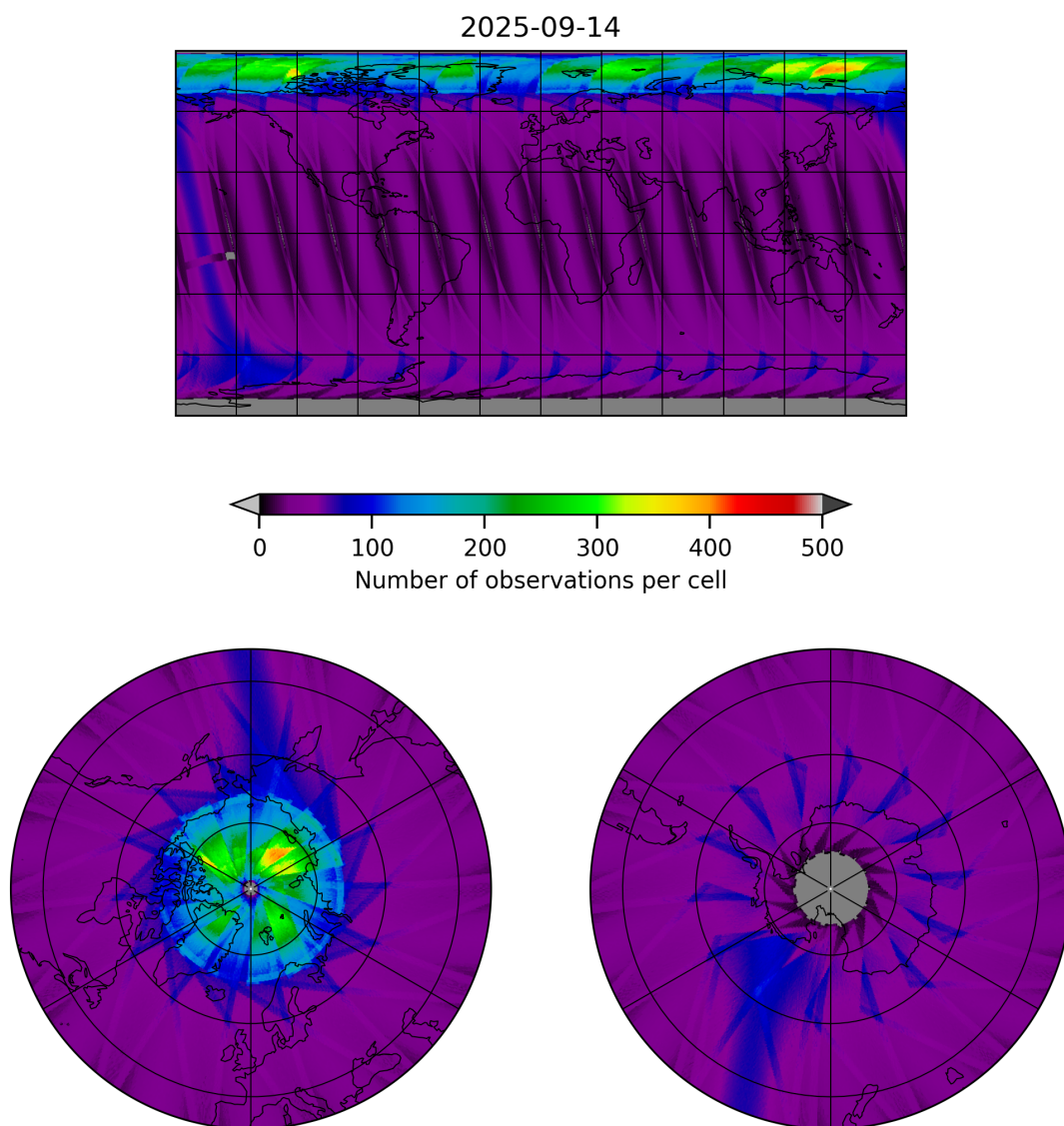
Figure 17: Map of the number of observations for 2025-09-14 to 2025-09-15
