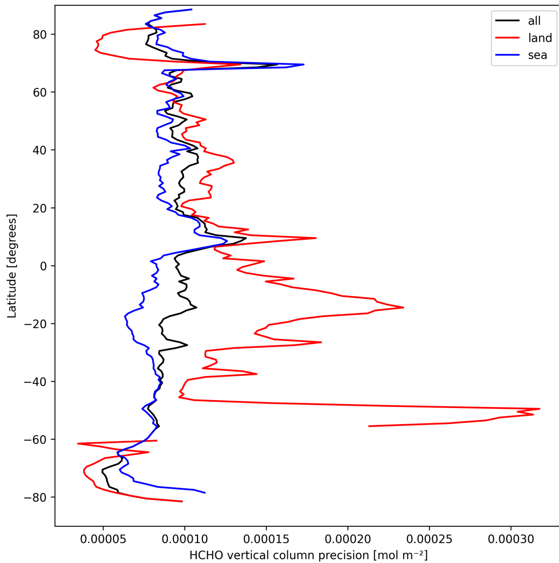
Figure 20: Zonal average of “HCHO vertical column precision” for 2025-09-14 to 2025-09-15.
