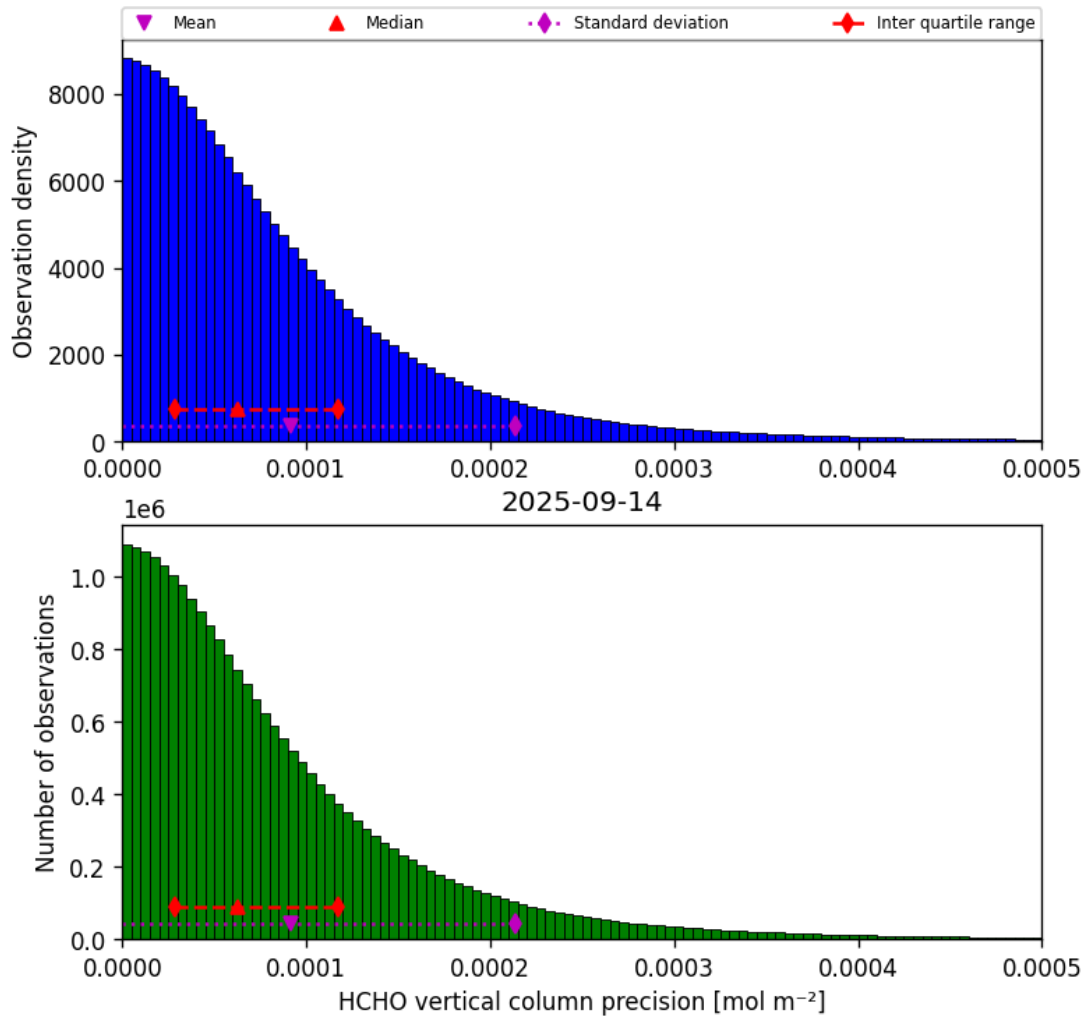
Figure 34: Histogram of “HCHO vertical column precision” for 2025-09-14 to 2025-09-15
