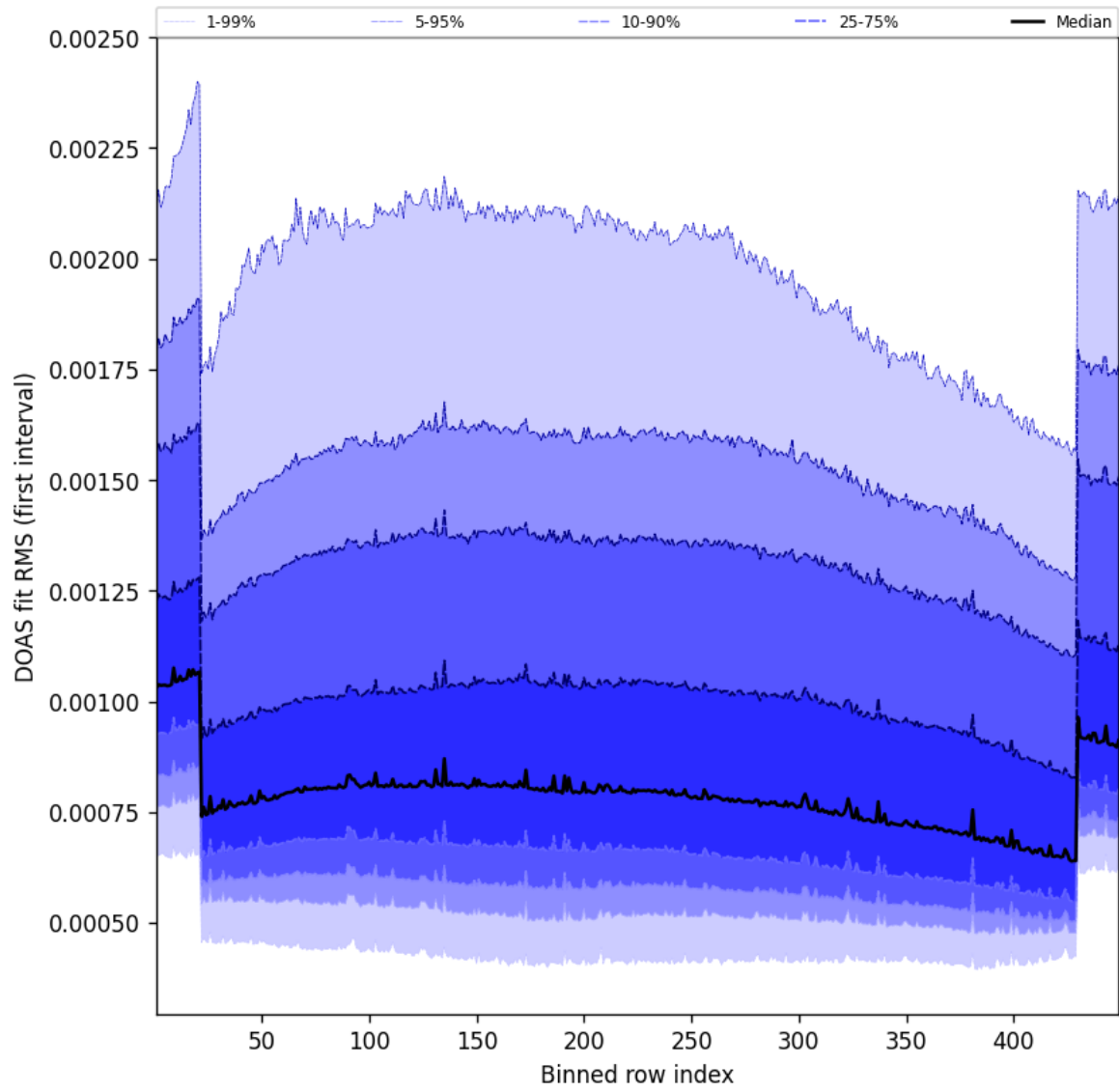
Figure 58: Along track statistics of “DOAS fit RMS (first interval)” for 2025-09-14 to 2025-09-15
