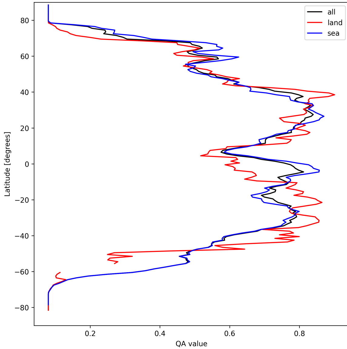
Figure 18: Zonal average of “QA value” for 2025-09-14 to 2025-09-15.
