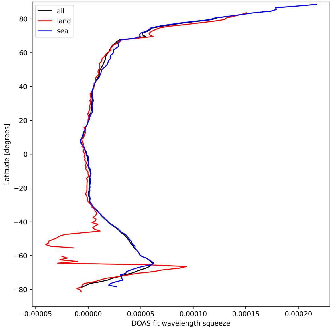
Figure 29: Zonal average of “DOAS fit wavelength squeeze” for 2025-09-14 to 2025-09-15.
