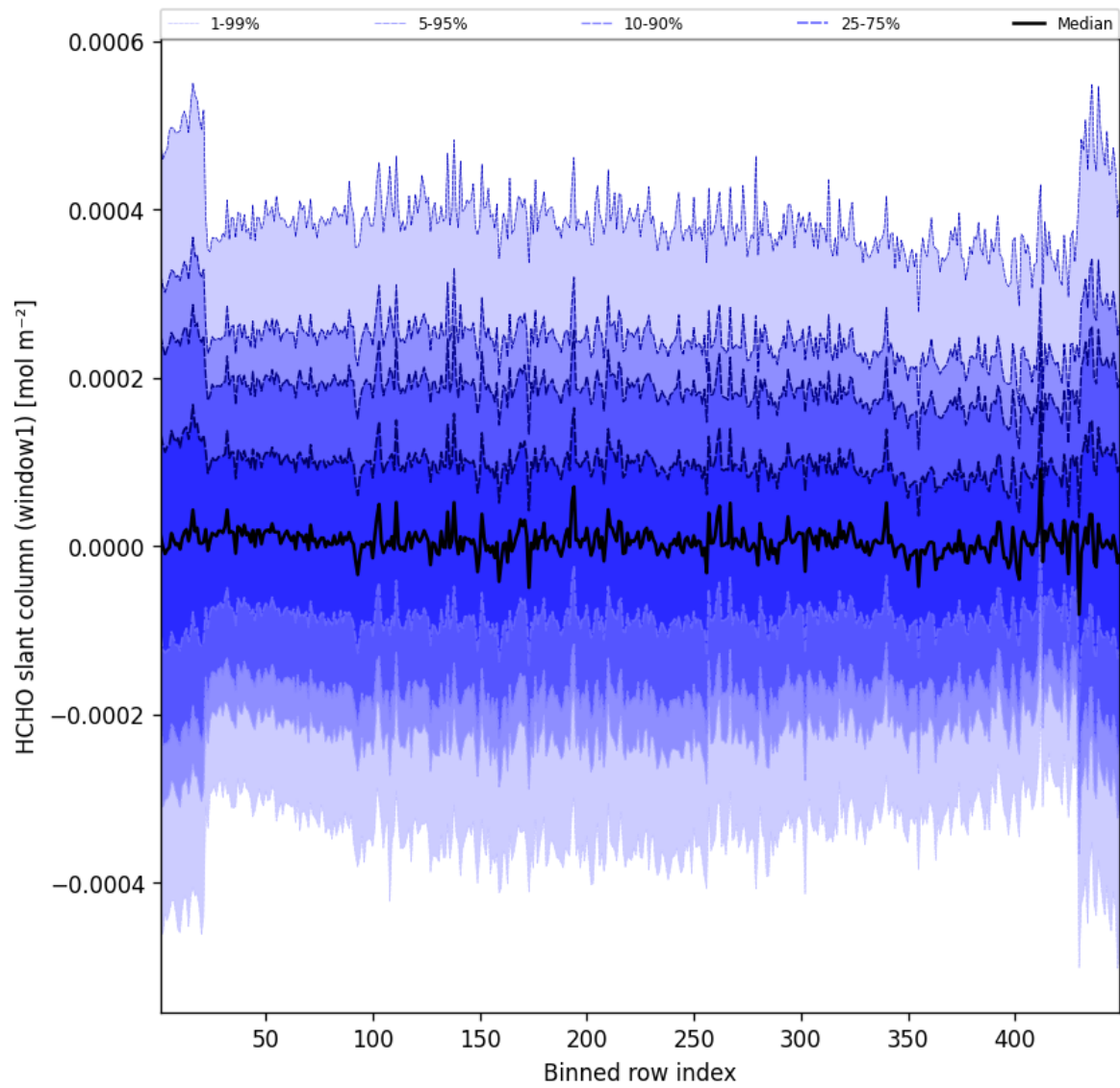
Figure 50: Along track statistics of “HCHO slant column (window1)” for 2025-09-14 to 2025-09-15
