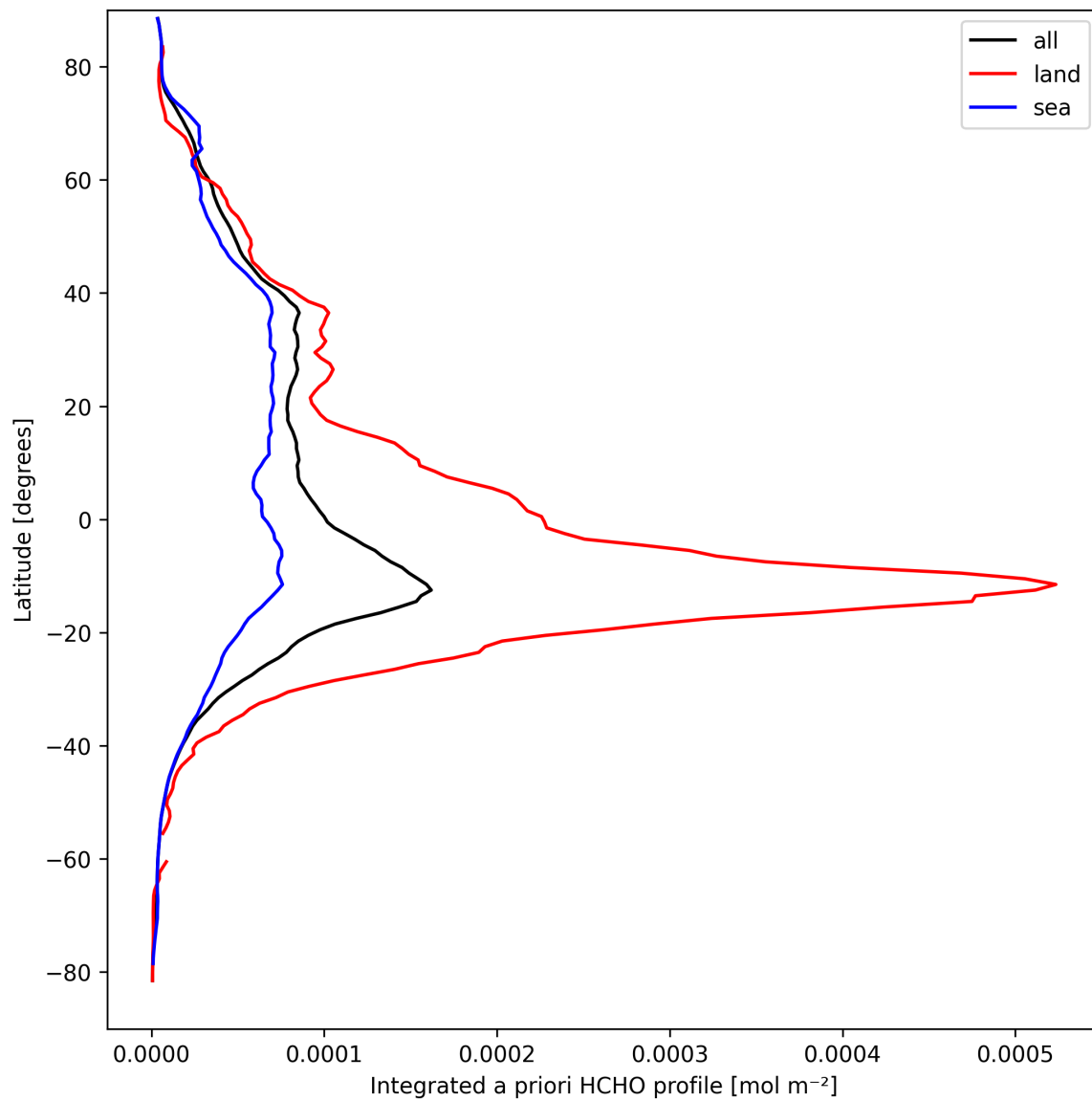
Figure 27: Zonal average of “Integrated a priori HCHO profile” for 2025-09-14 to 2025-09-15.
