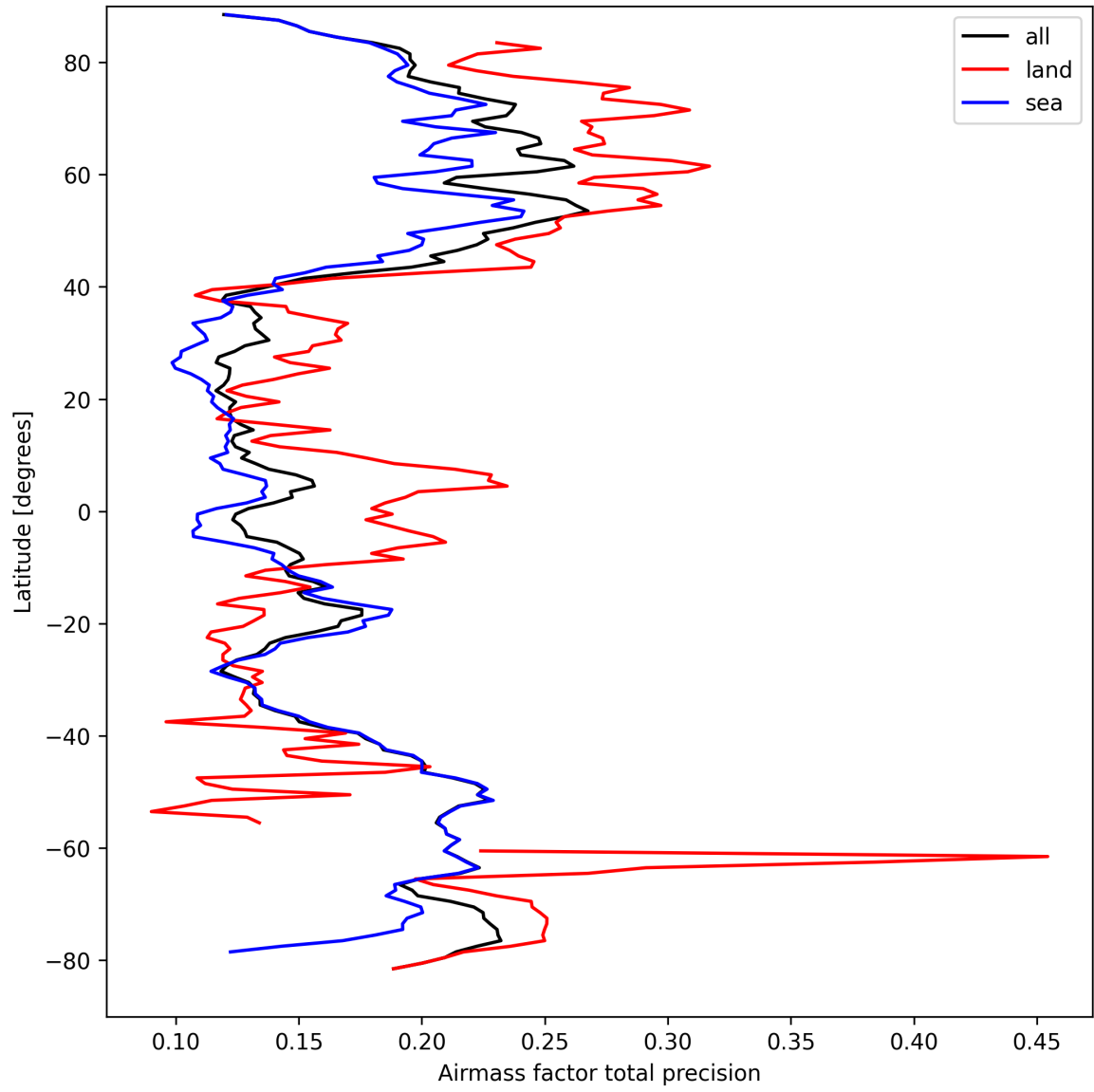
Figure 25: Zonal average of “Airmass factor total precision” for 2025-09-14 to 2025-09-15.
