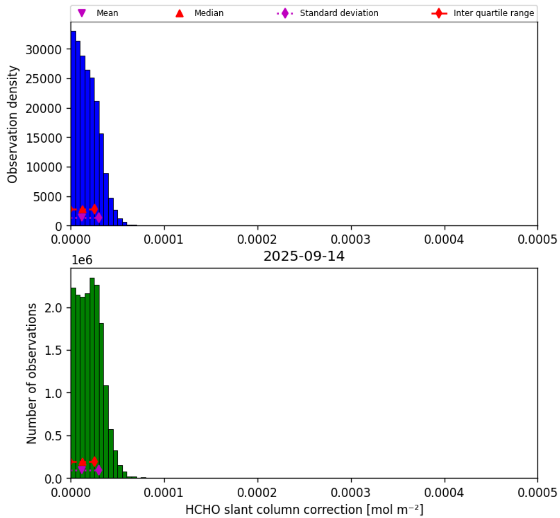
Figure 45: Histogram of “HCHO slant column correction” for 2025-09-14 to 2025-09-15
