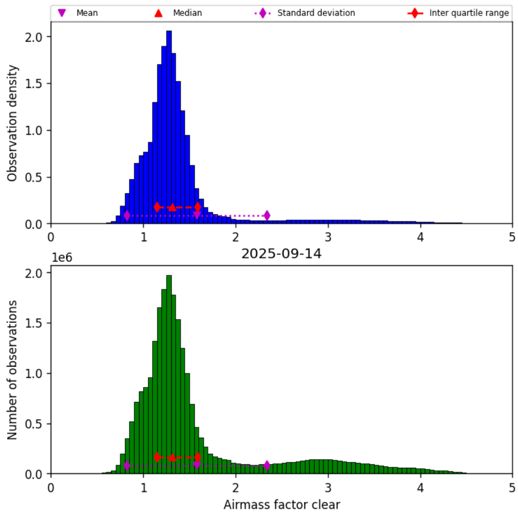
Figure 40: Histogram of “Airmass factor clear” for 2025-09-14 to 2025-09-15
