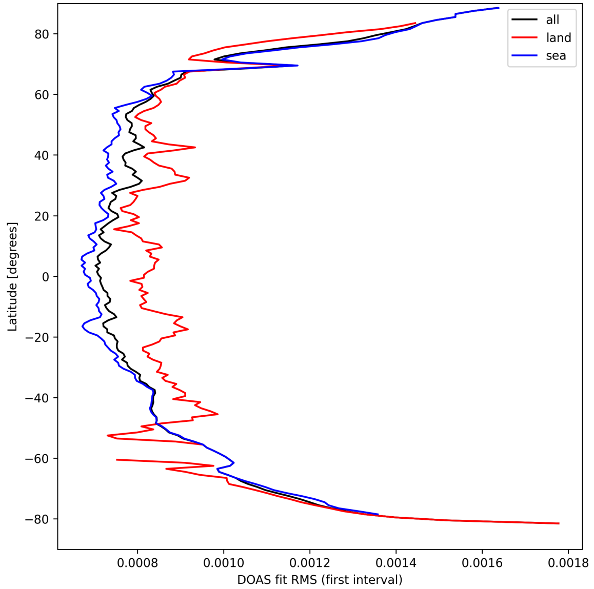
Figure 30: Zonal average of “DOAS fit RMS (first interval)” for 2025-09-14 to 2025-09-15.
