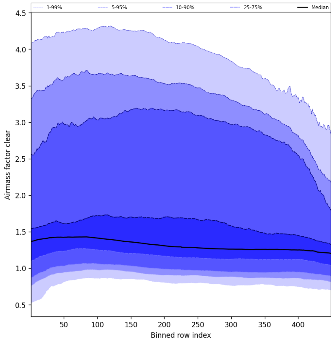
Figure 54: Along track statistics of “Airmass factor clear” for 2025-09-14 to 2025-09-15
