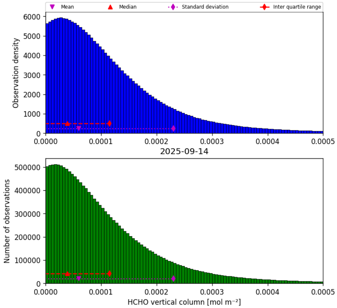
Figure 33: Histogram of “HCHO vertical column” for 2025-09-14 to 2025-09-15
