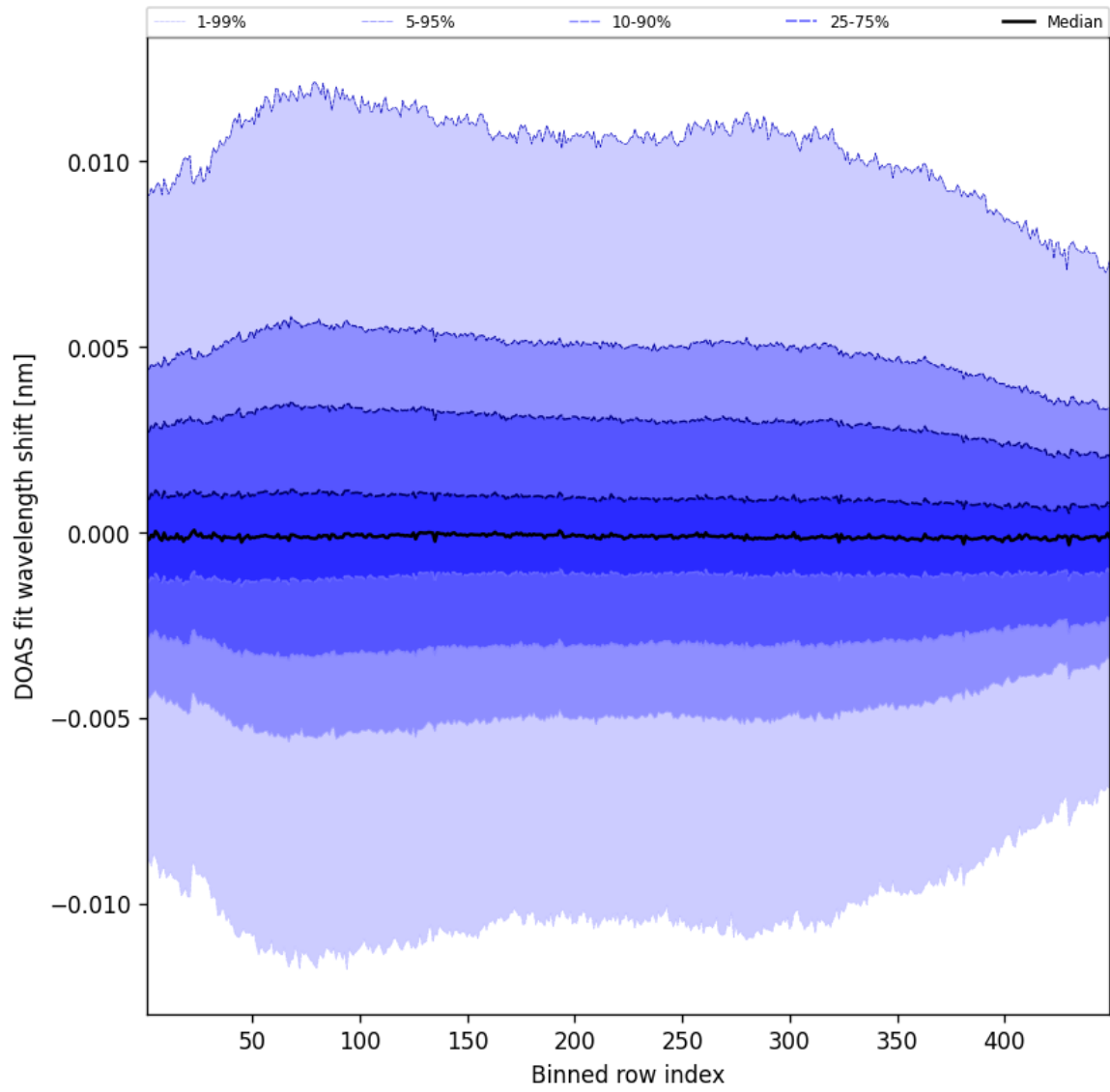
Figure 56: Along track statistics of “DOAS fit wavelength shift” for 2025-09-14 to 2025-09-15
