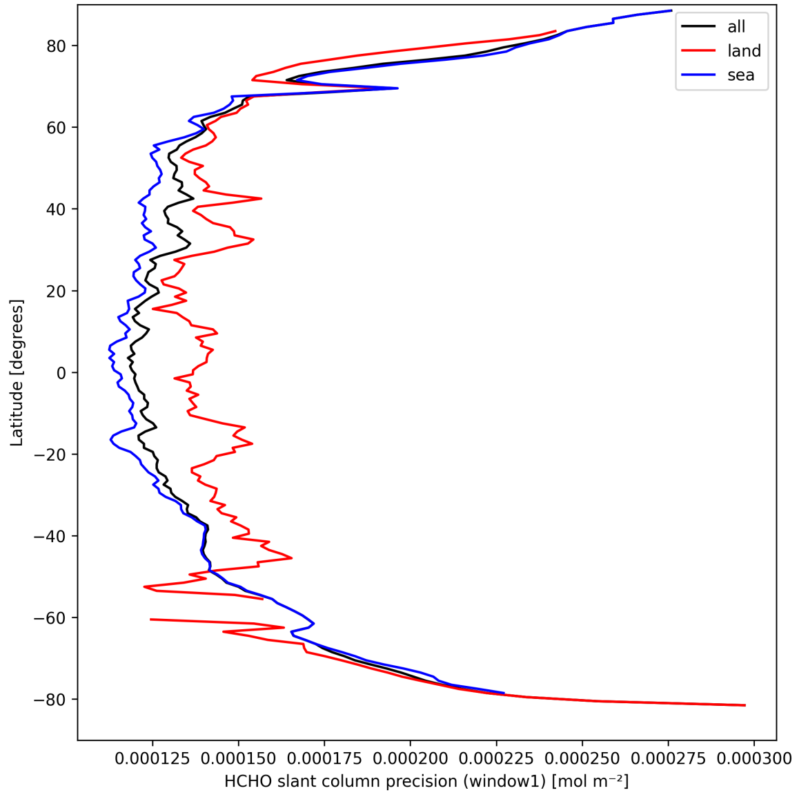
Figure 23: Zonal average of “HCHO slant column precision (window1)” for 2025-09-14 to 2025-09-15.
