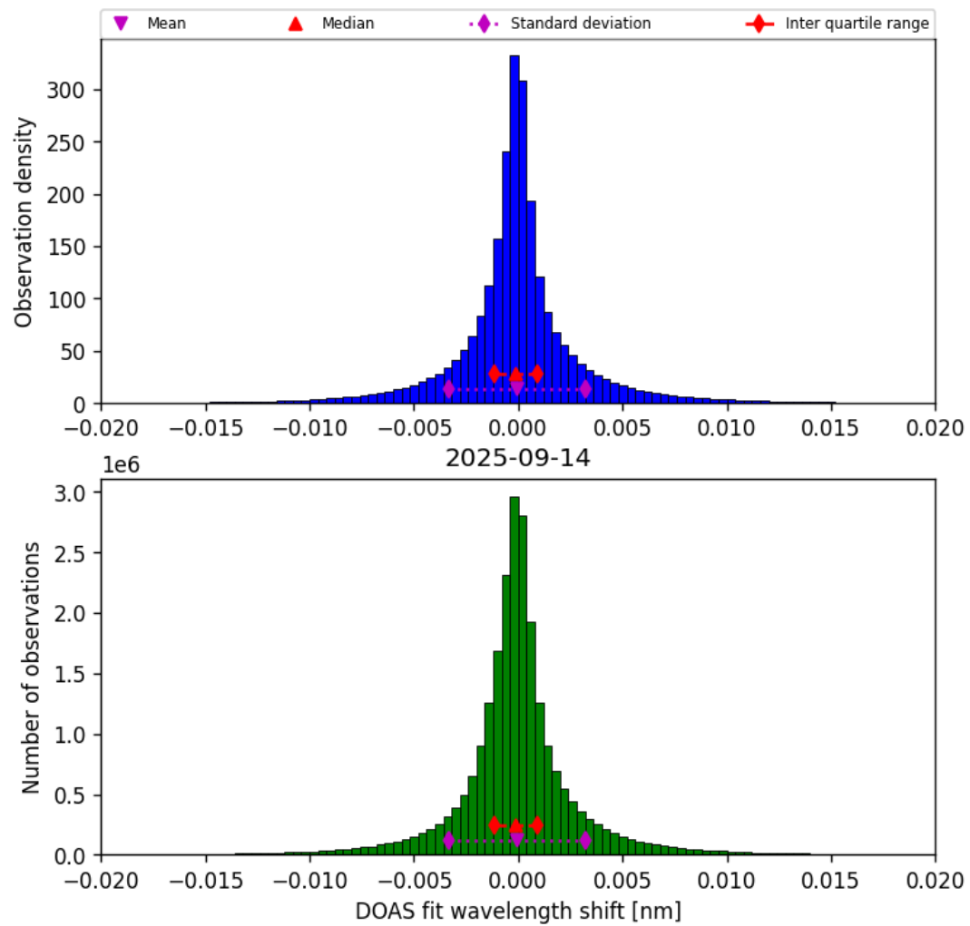
Figure 42: Histogram of “DOAS fit wavelength shift” for 2025-09-14 to 2025-09-15
