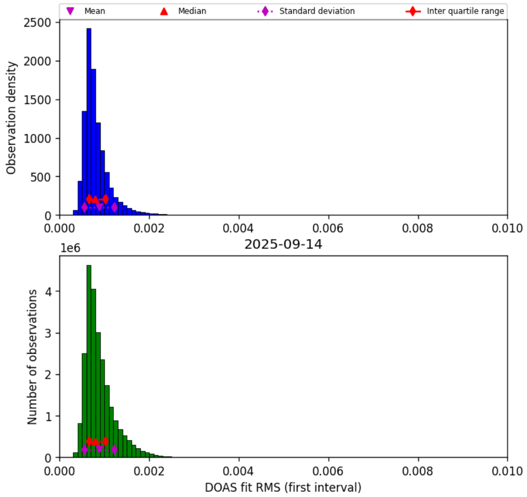
Figure 44: Histogram of “DOAS fit RMS (first interval)” for 2025-09-14 to 2025-09-15
