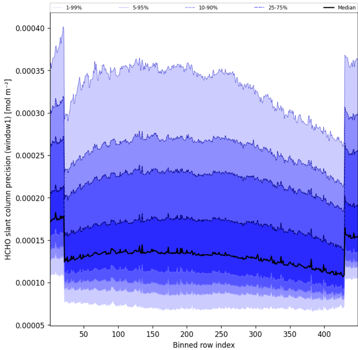
Figure 51: Along track statistics of “HCHO slant column precision (window1)” for 2025-09-14 to 2025-09-15
