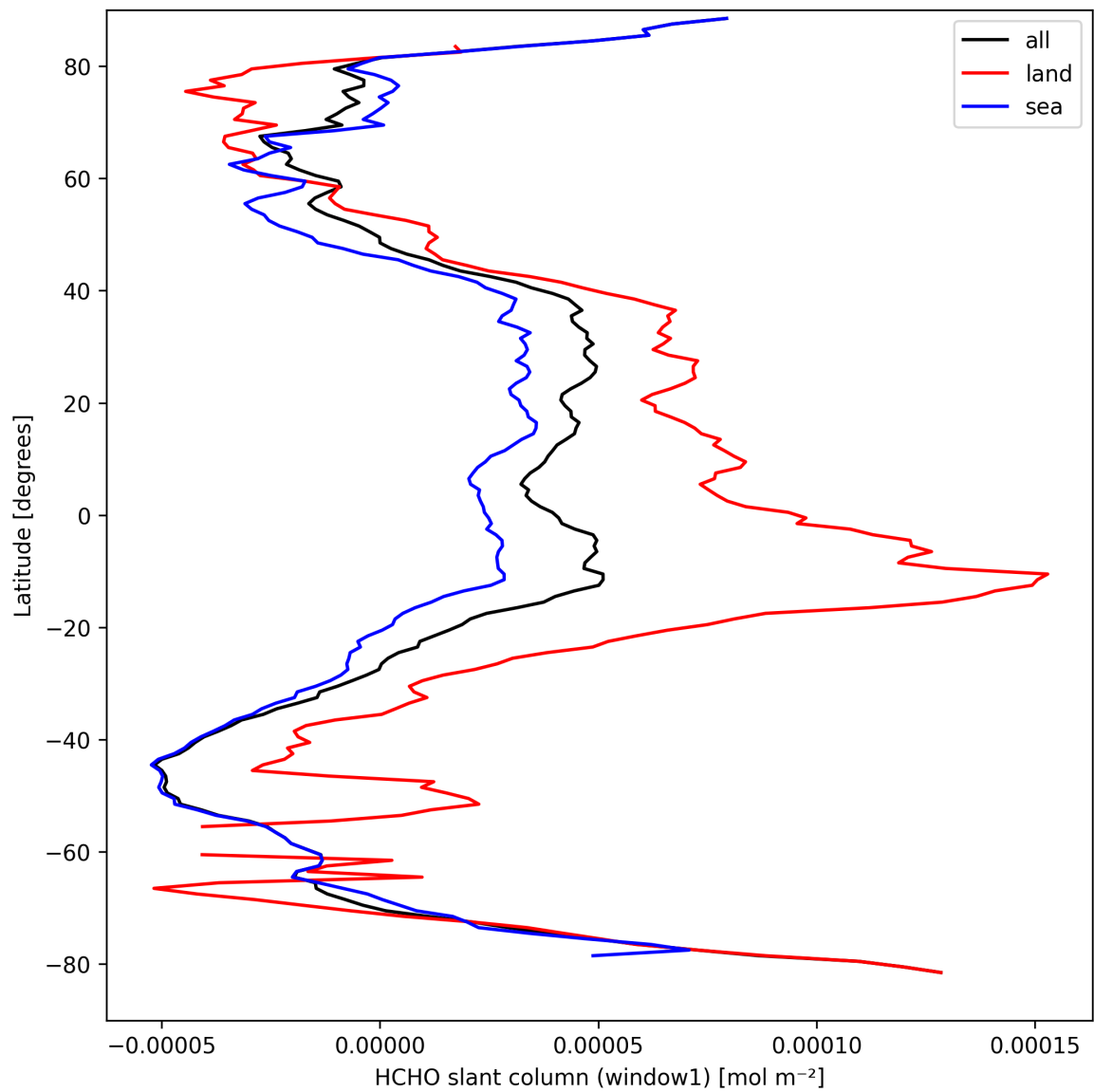
Figure 22: Zonal average of “HCHO slant column (window1)” for 2025-09-14 to 2025-09-15.
