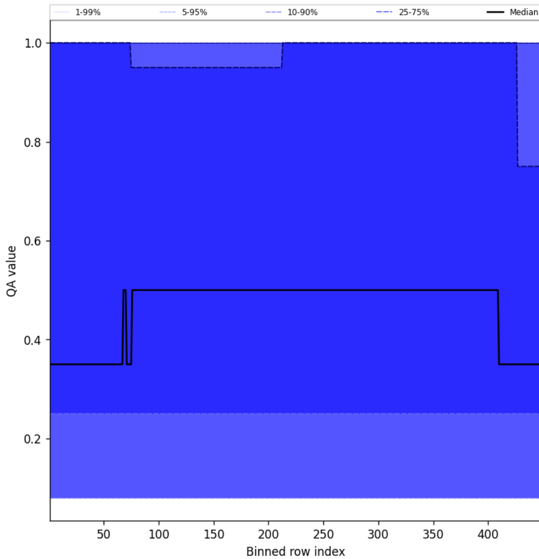
Figure 46: Along track statistics of “QA value” for 2025-09-16 to 2025-09-17
