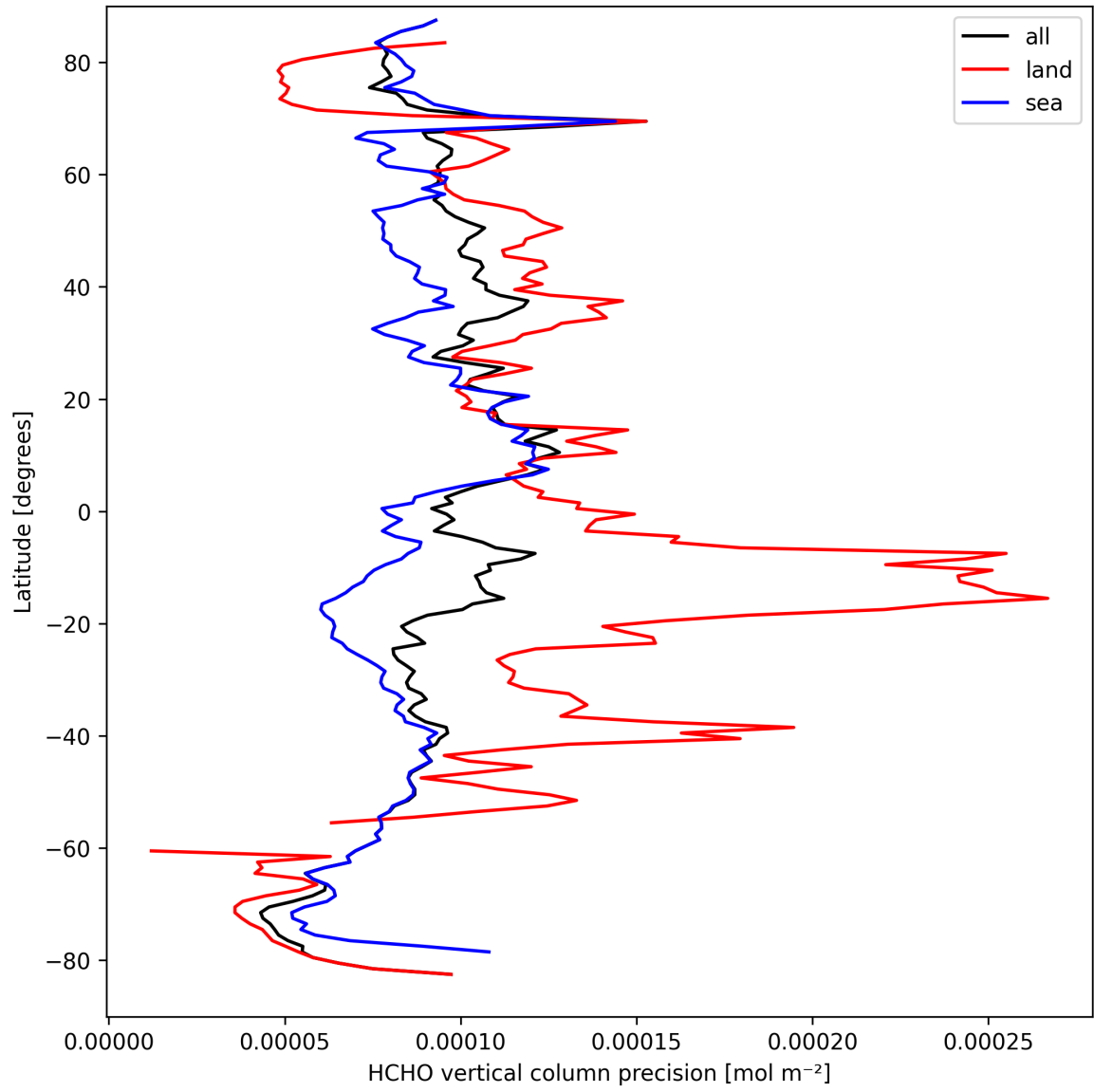
Figure 20: Zonal average of “HCHO vertical column precision” for 2025-09-16 to 2025-09-17.
