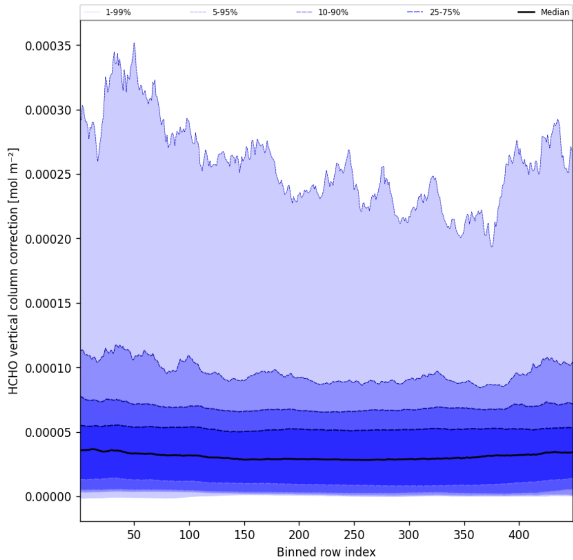
Figure 49: Along track statistics of “HCHO vertical column correction” for 2025-09-16 to 2025-09-17
