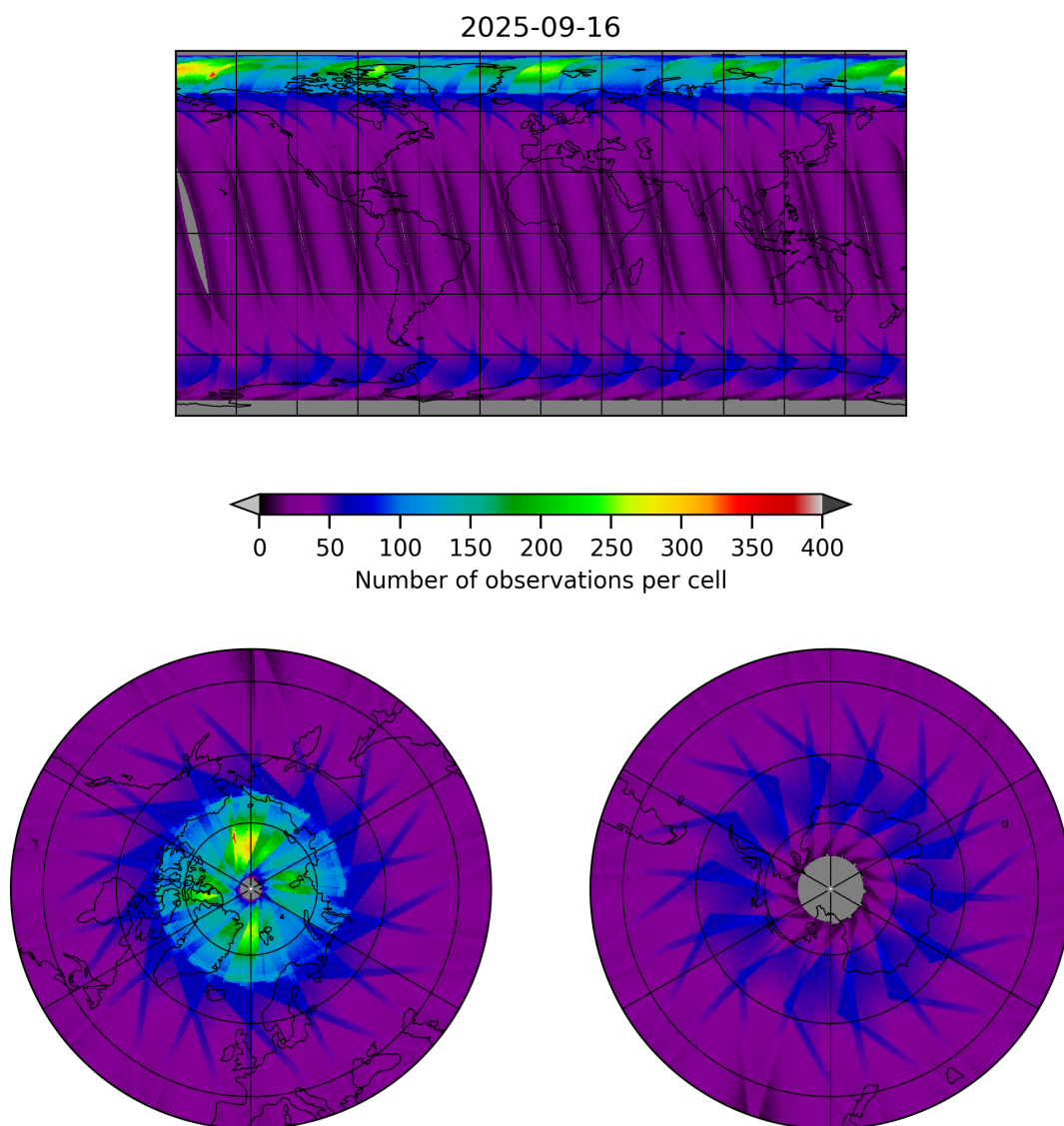
Figure 17: Map of the number of observations for 2025-09-16 to 2025-09-17
