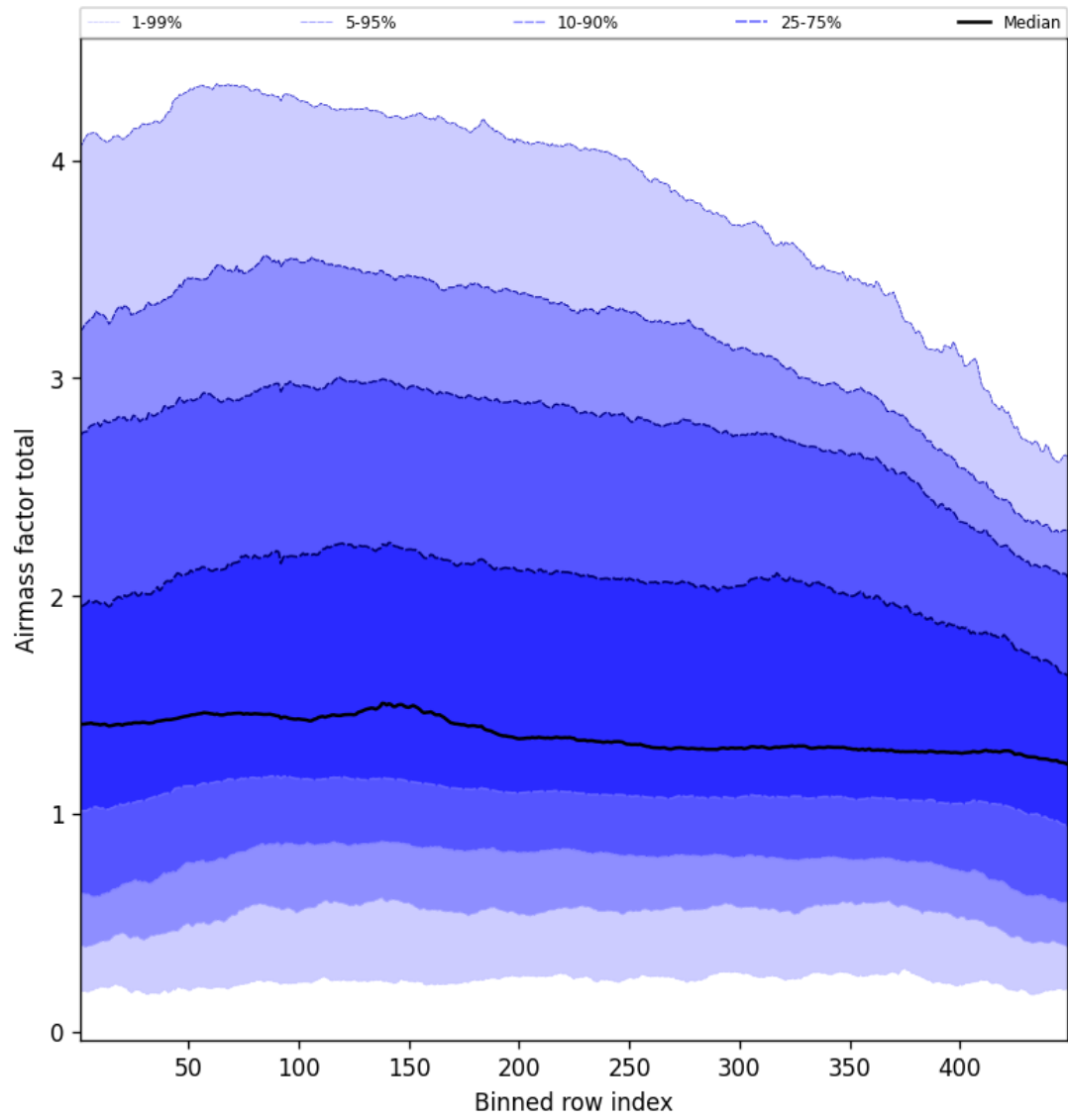
Figure 52: Along track statistics of “Airmass factor total” for 2025-09-16 to 2025-09-17
