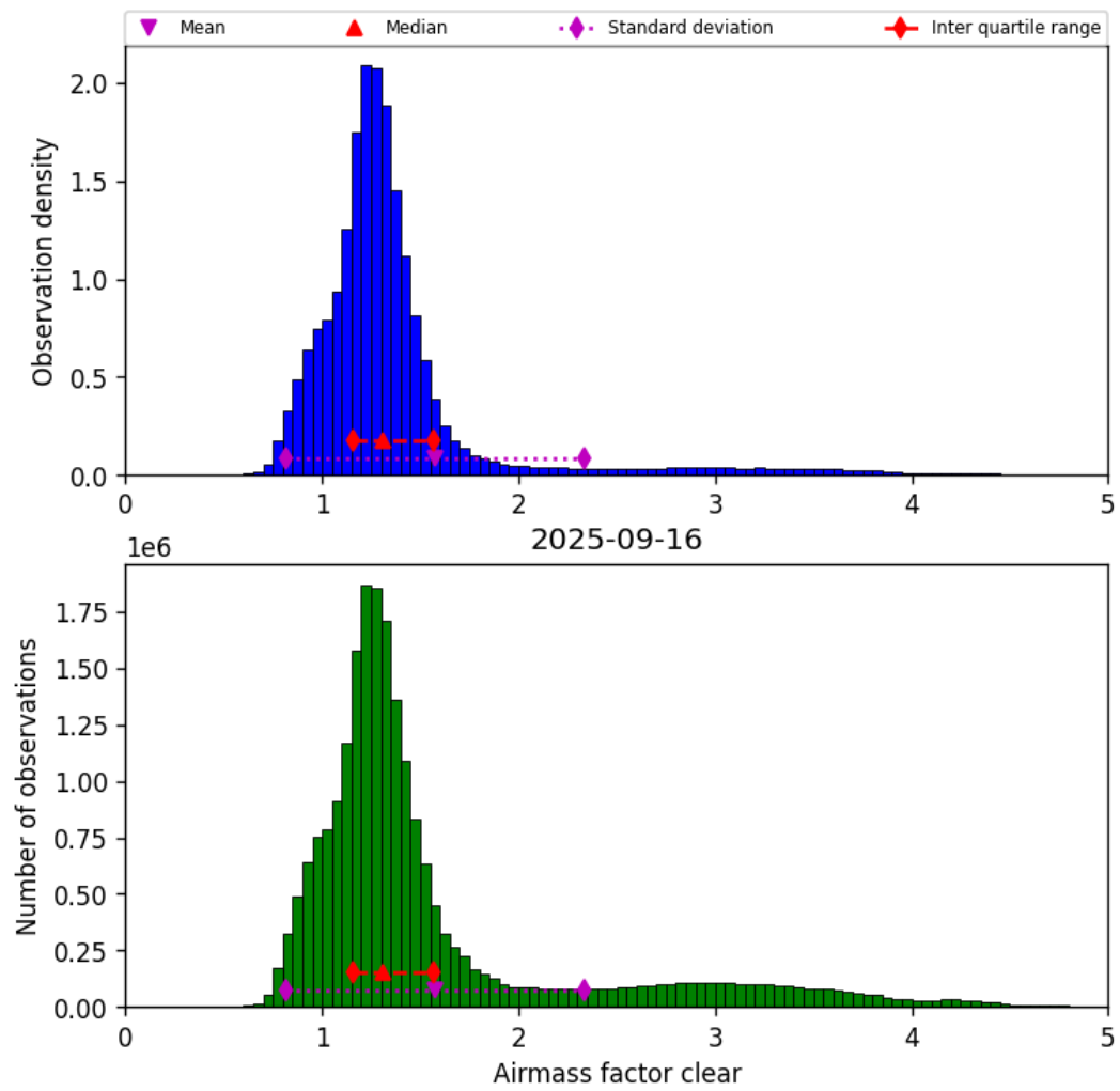
Figure 40: Histogram of “Airmass factor clear” for 2025-09-16 to 2025-09-17
