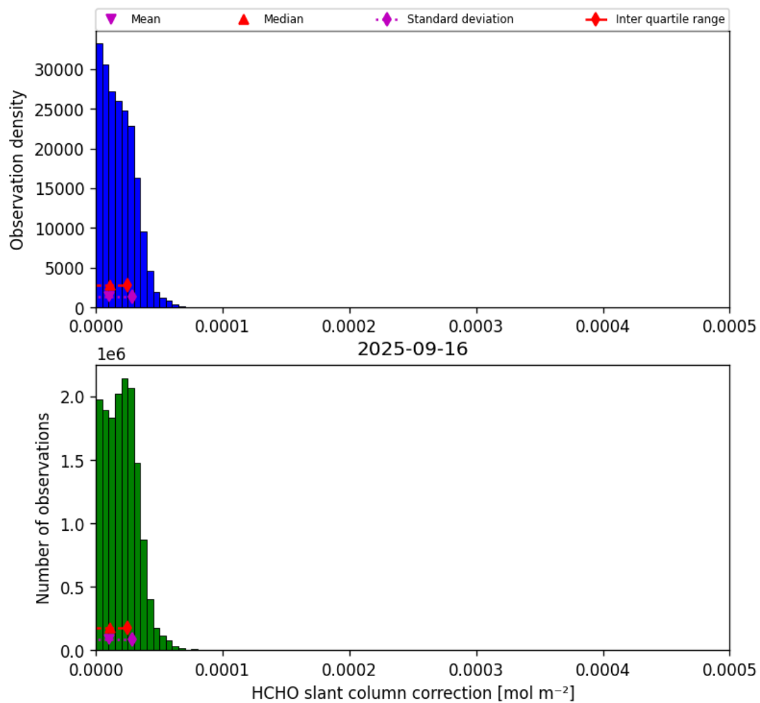
Figure 45: Histogram of “HCHO slant column correction” for 2025-09-16 to 2025-09-17
