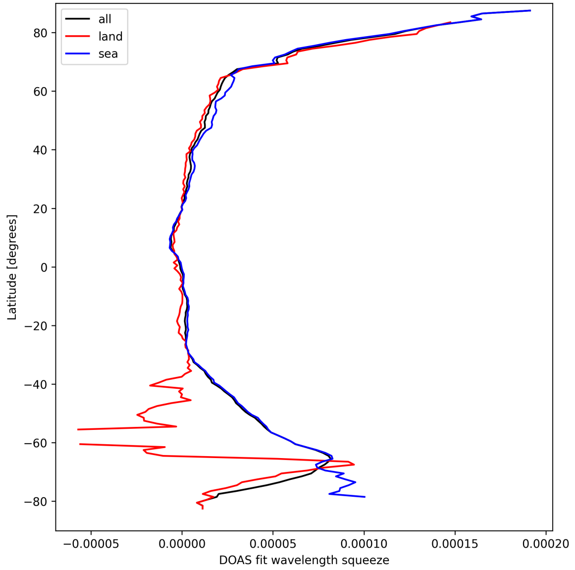
Figure 29: Zonal average of “DOAS fit wavelength squeeze” for 2025-09-16 to 2025-09-17.
