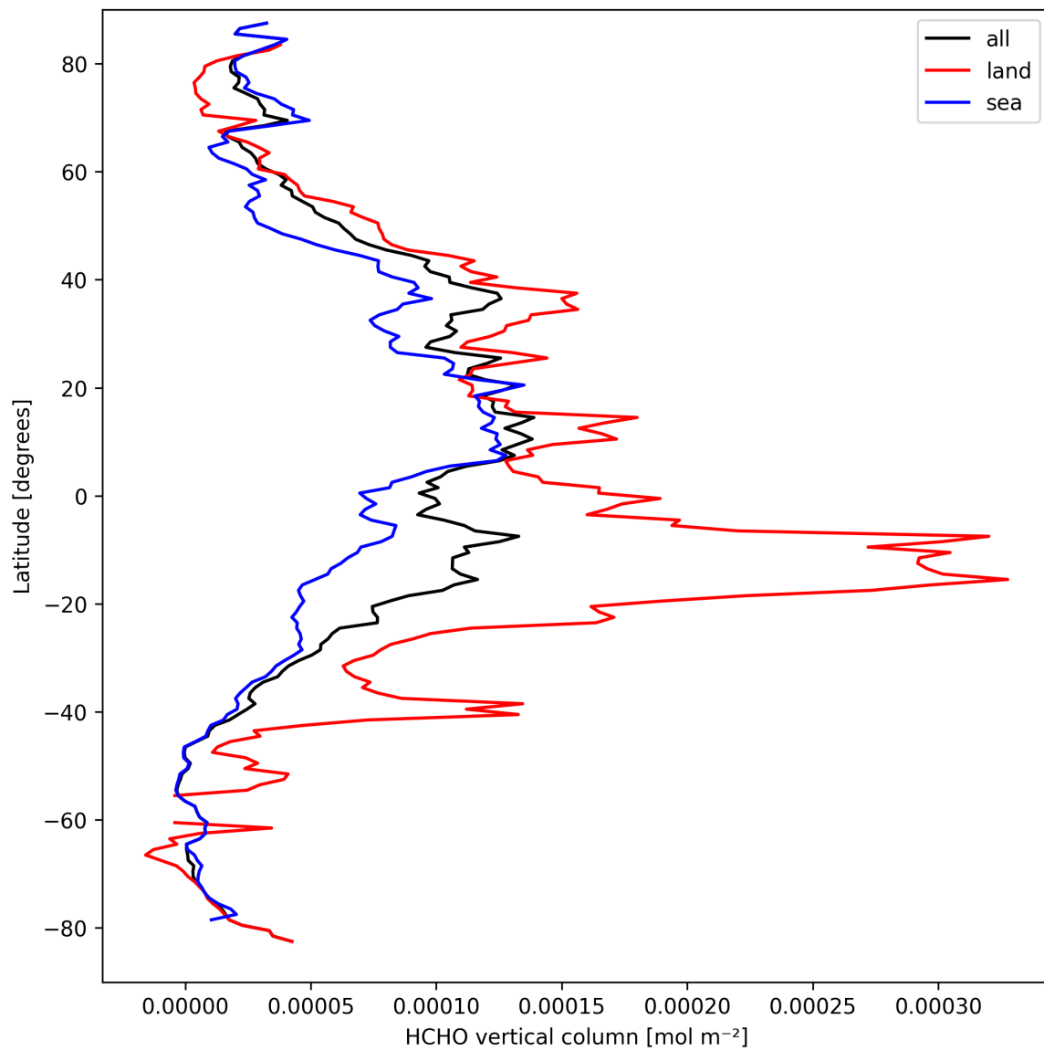
Figure 19: Zonal average of “HCHO vertical column” for 2025-09-16 to 2025-09-17.
