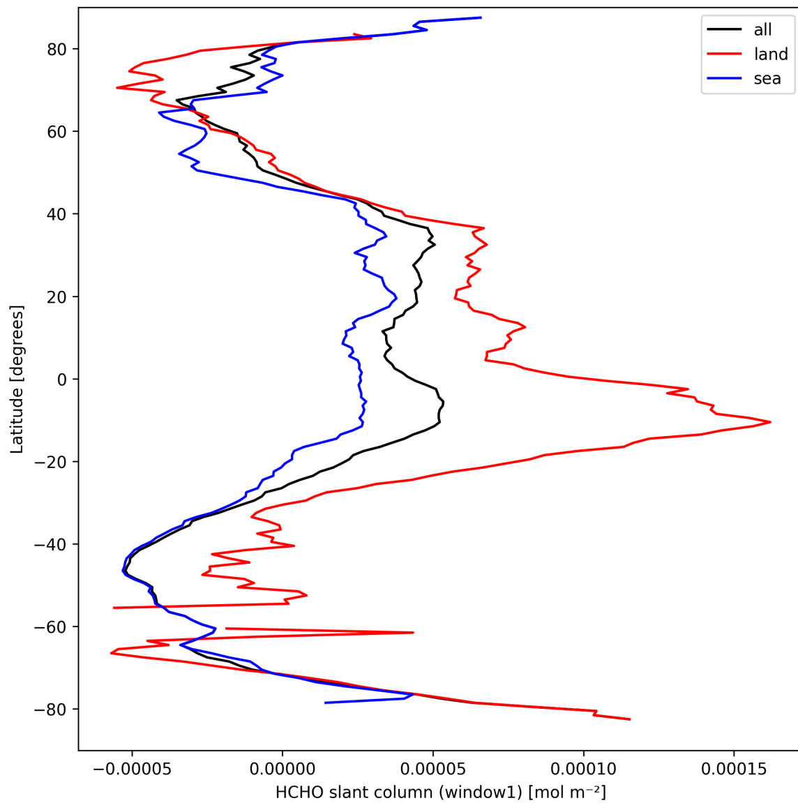
Figure 22: Zonal average of “HCHO slant column (window1)” for 2025-09-16 to 2025-09-17.
