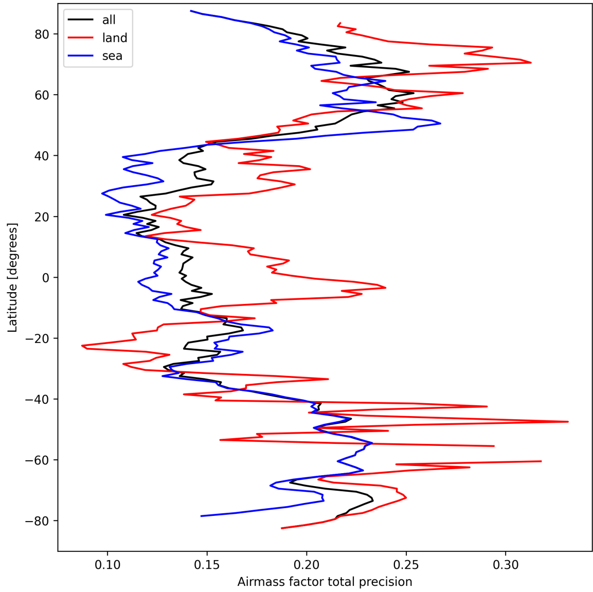
Figure 25: Zonal average of “Airmass factor total precision” for 2025-09-16 to 2025-09-17.
