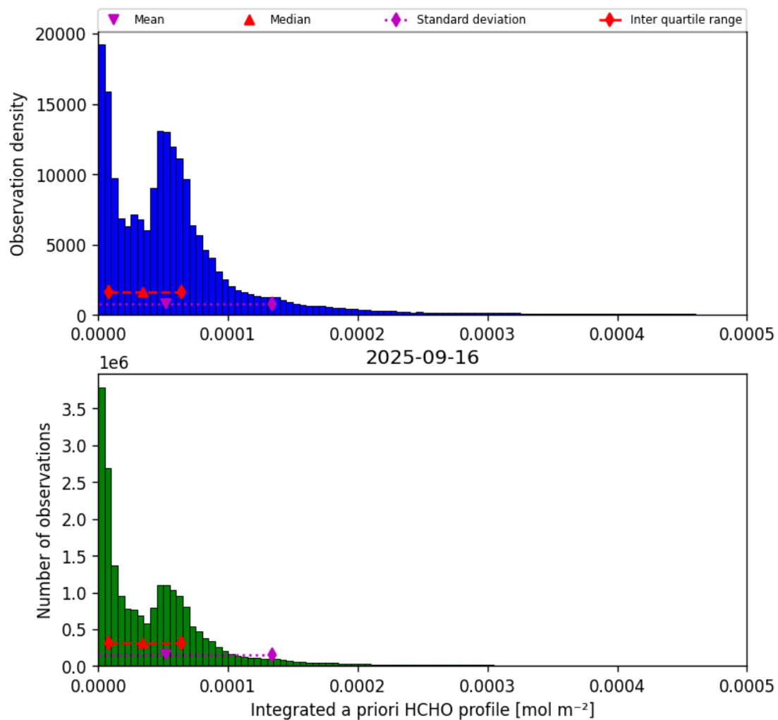
Figure 41: Histogram of “Integrated a priori HCHO profile” for 2025-09-16 to 2025-09-17
