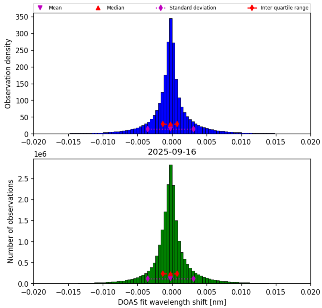
Figure 42: Histogram of “DOAS fit wavelength shift” for 2025-09-16 to 2025-09-17
