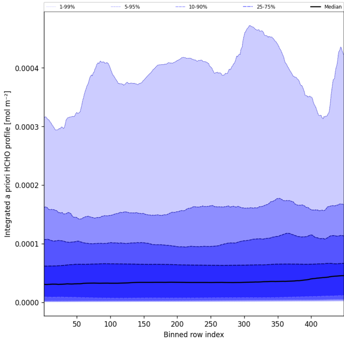
Figure 55: Along track statistics of “Integrated a priori HCHO profile” for 2025-09-16 to 2025-09-17
