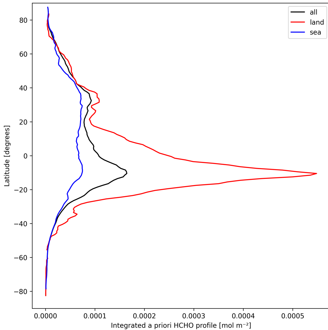
Figure 27: Zonal average of “Integrated a priori HCHO profile” for 2025-09-16 to 2025-09-17.
