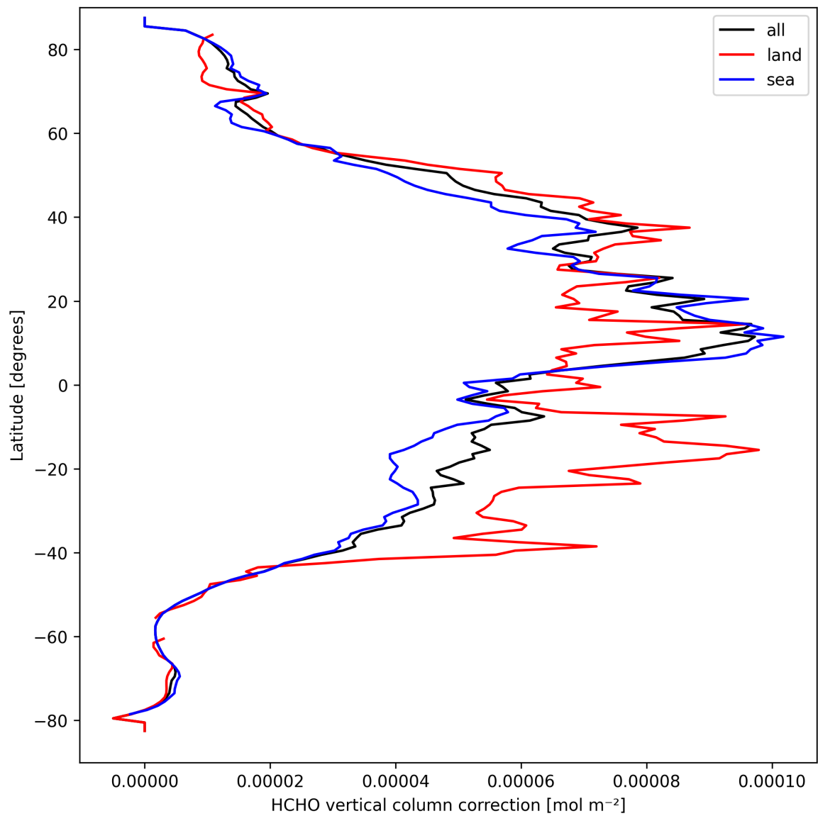
Figure 21: Zonal average of “HCHO vertical column correction” for 2025-09-16 to 2025-09-17.
