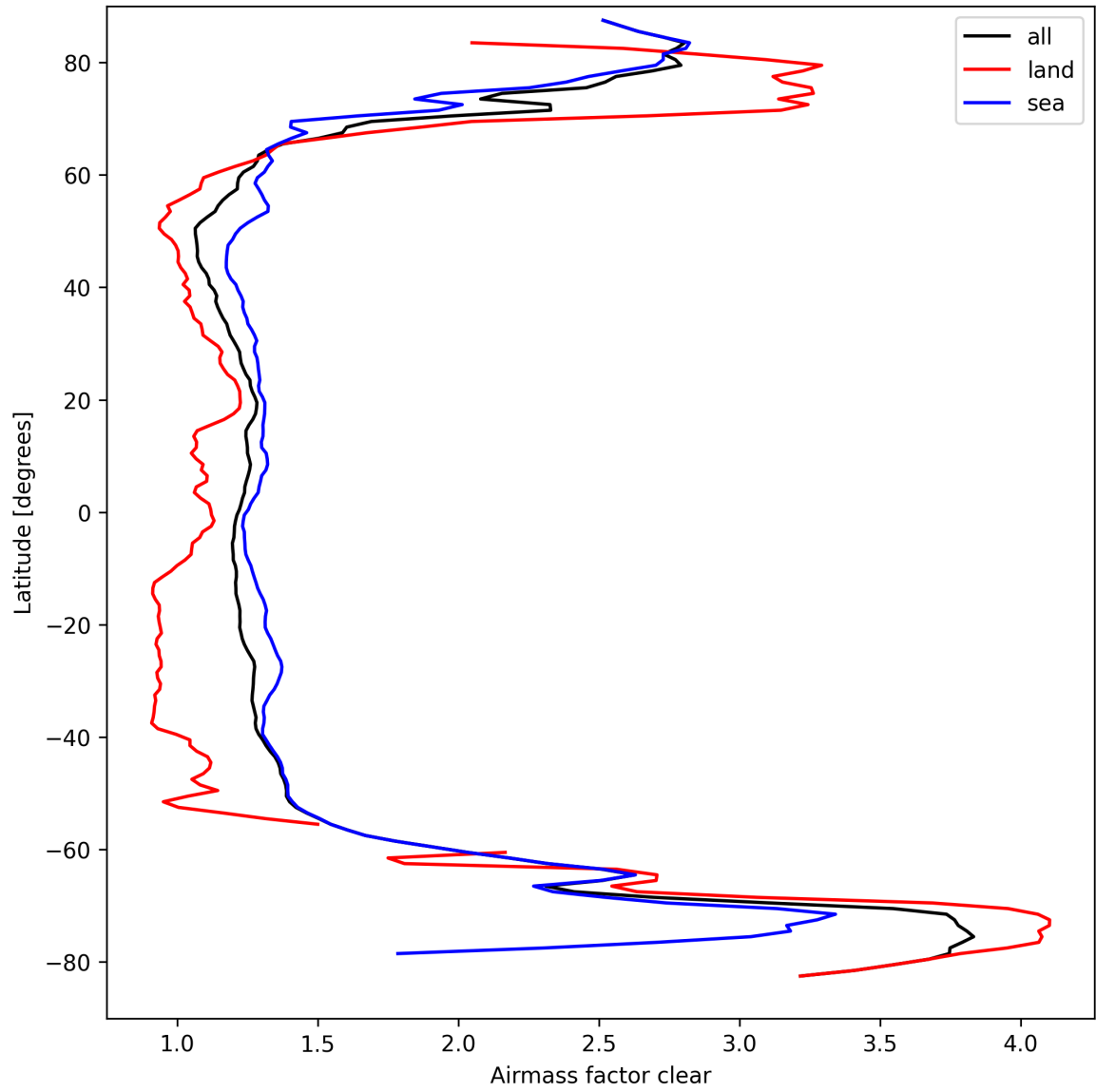
Figure 26: Zonal average of “Airmass factor clear” for 2025-09-16 to 2025-09-17.
