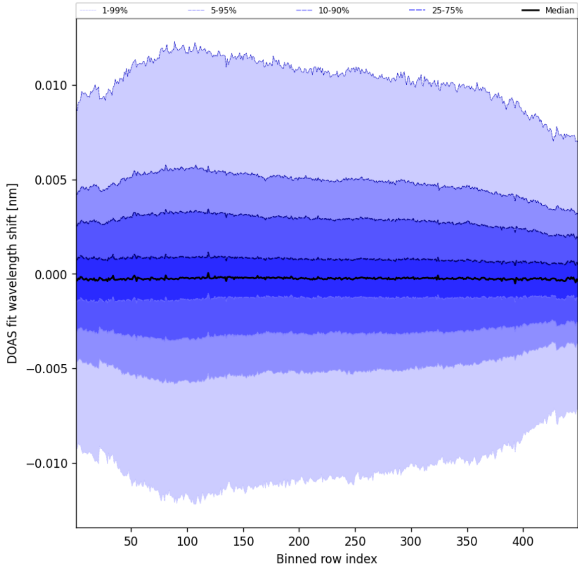
Figure 56: Along track statistics of “DOAS fit wavelength shift” for 2025-09-16 to 2025-09-17
