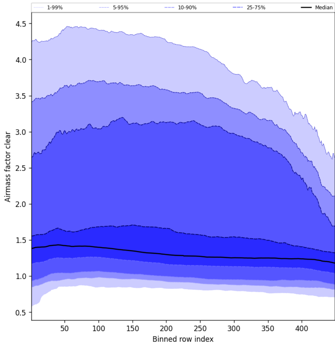
Figure 54: Along track statistics of “Airmass factor clear” for 2025-09-16 to 2025-09-17
