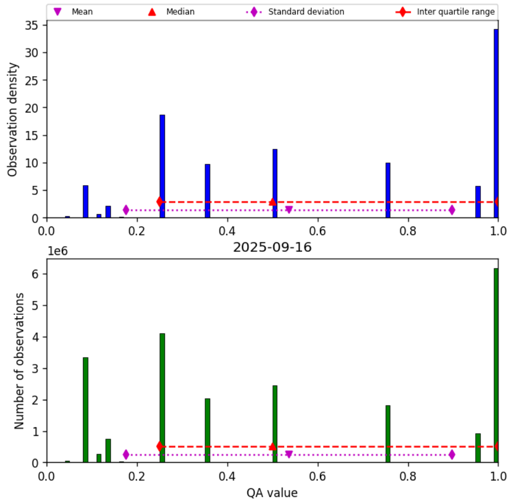
Figure 32: Histogram of “QA value” for 2025-09-16 to 2025-09-17
