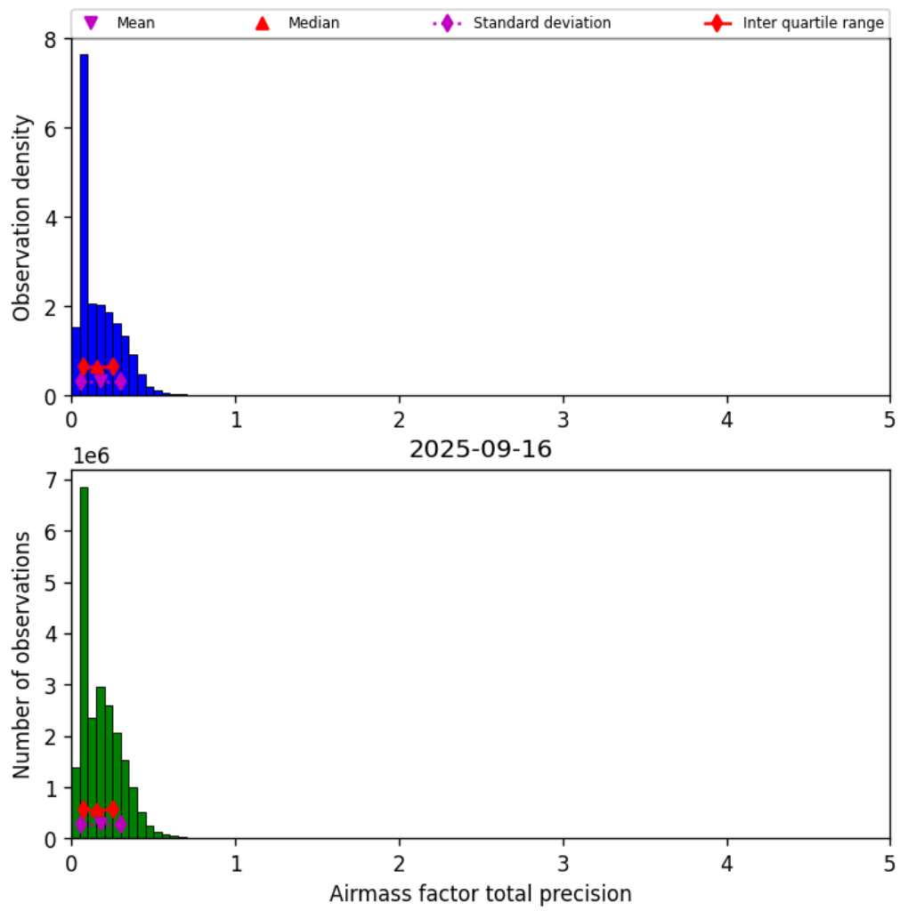
Figure 39: Histogram of “Airmass factor total precision” for 2025-09-16 to 2025-09-17
