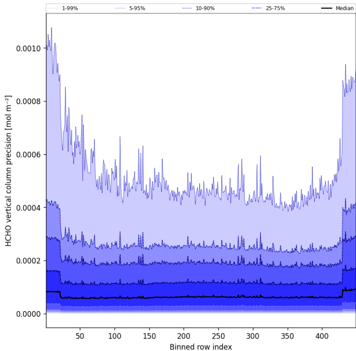
Figure 48: Along track statistics of “HCHO vertical column precision” for 2025-09-16 to 2025-09-17
