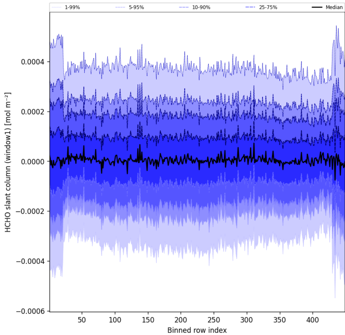
Figure 50: Along track statistics of “HCHO slant column (window1)” for 2025-09-16 to 2025-09-17
