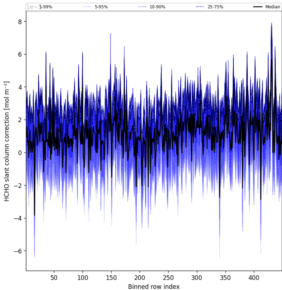
Figure 59: Along track statistics of “HCHO slant column correction” for 2025-09-16 to 2025-09-17
