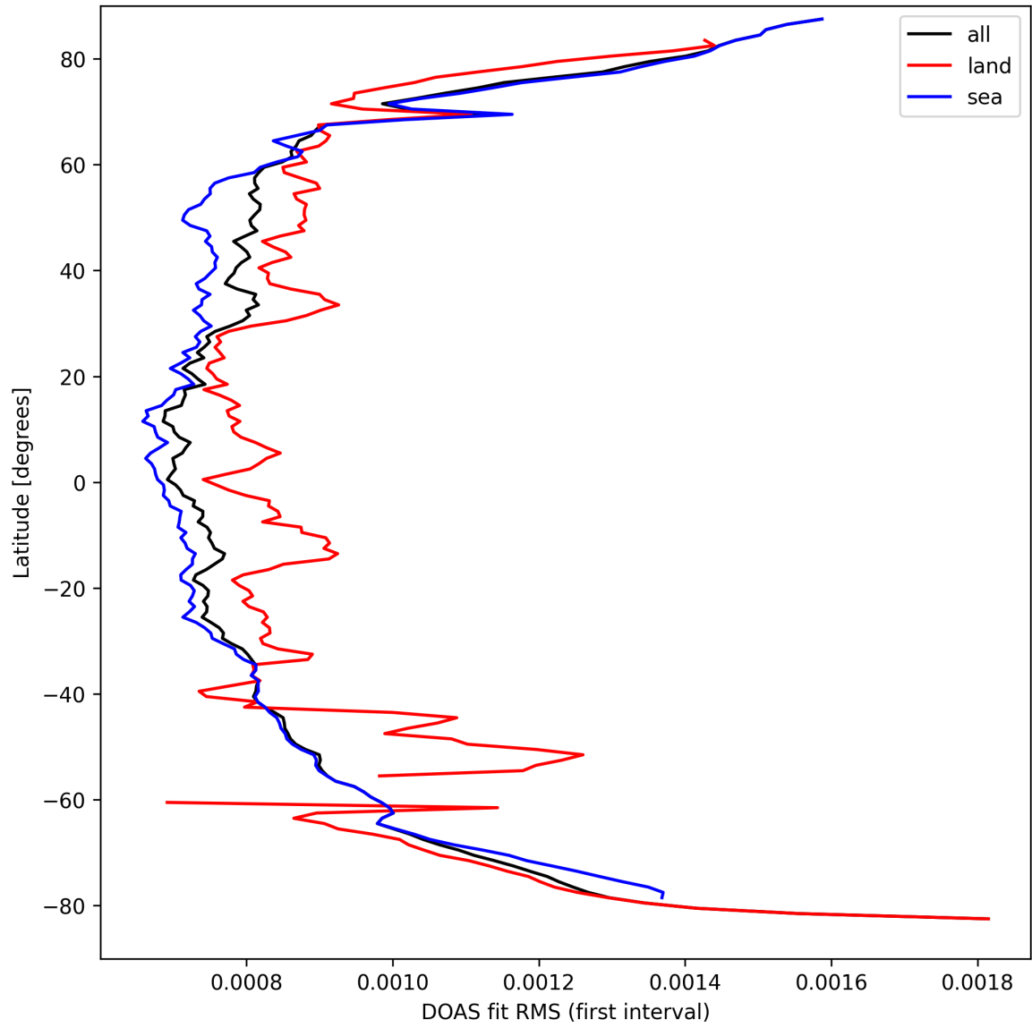
Figure 30: Zonal average of “DOAS fit RMS (first interval)” for 2025-09-16 to 2025-09-17.
