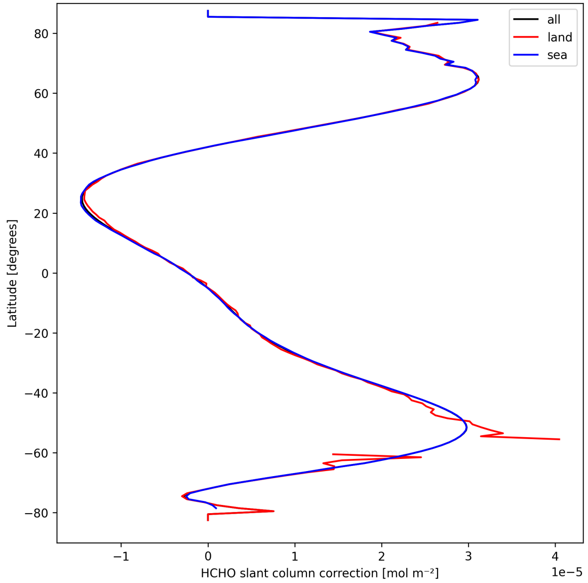
Figure 31: Zonal average of "HCHO slant column correction" for 2025-09-16 to 2025-09-17.
