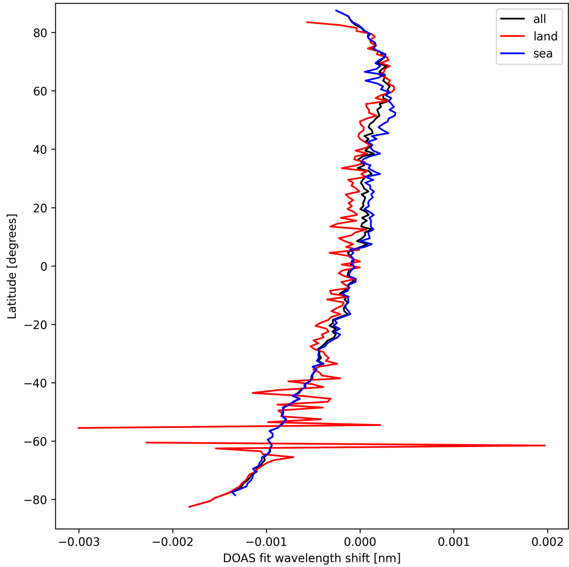
Figure 28: Zonal average of "DOAS fit wavelength shift" for 2025-09-16 to 2025-09-17.
