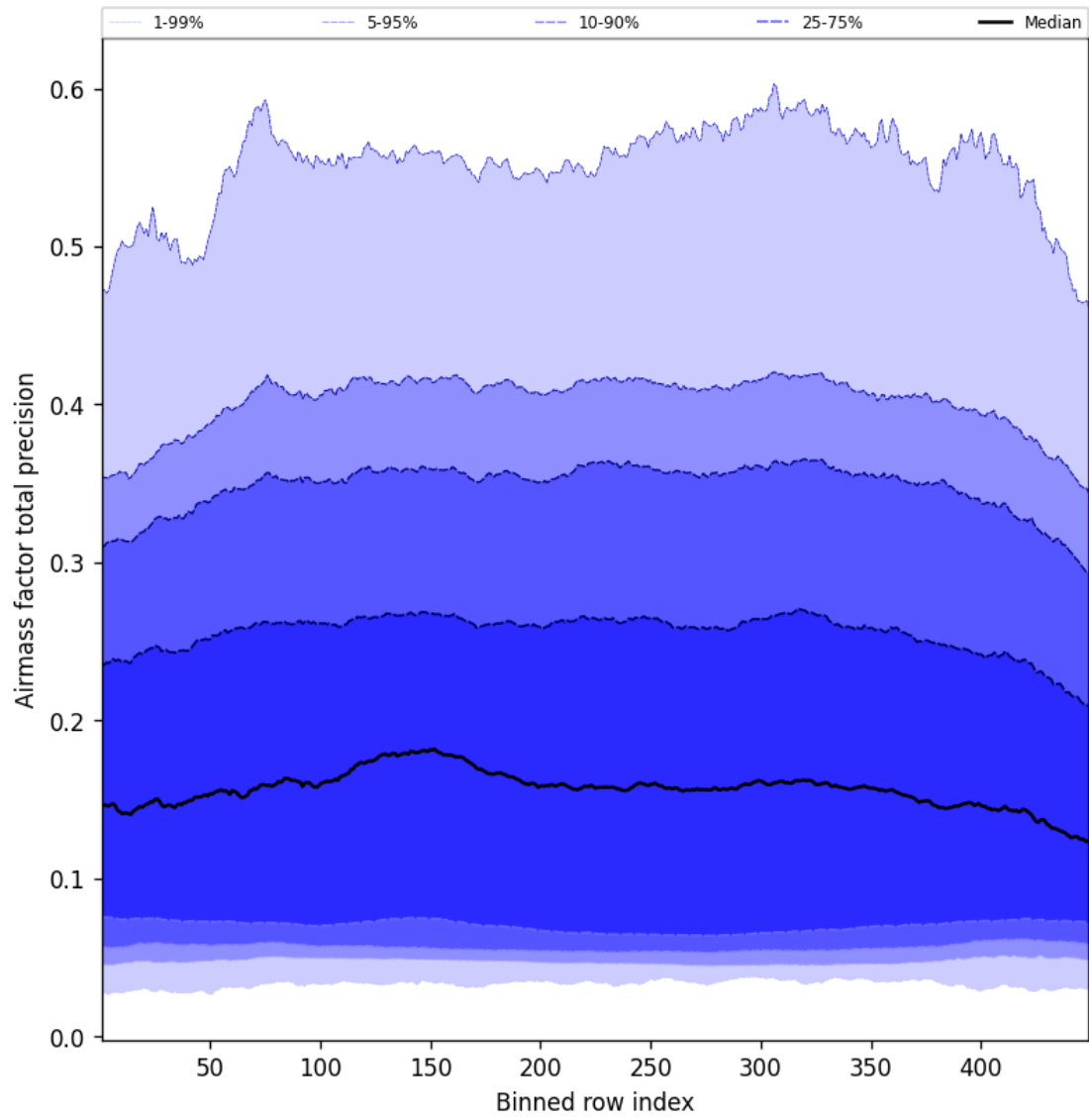
Figure 53: Along track statistics of “Airmass factor total precision” for 2025-09-16 to 2025-09-17
