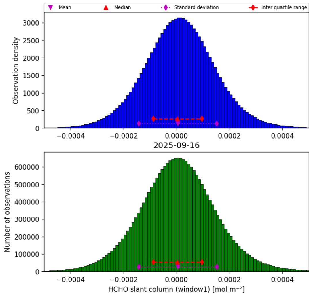
Figure 36: Histogram of “HCHO slant column (window1)” for 2025-09-16 to 2025-09-17
