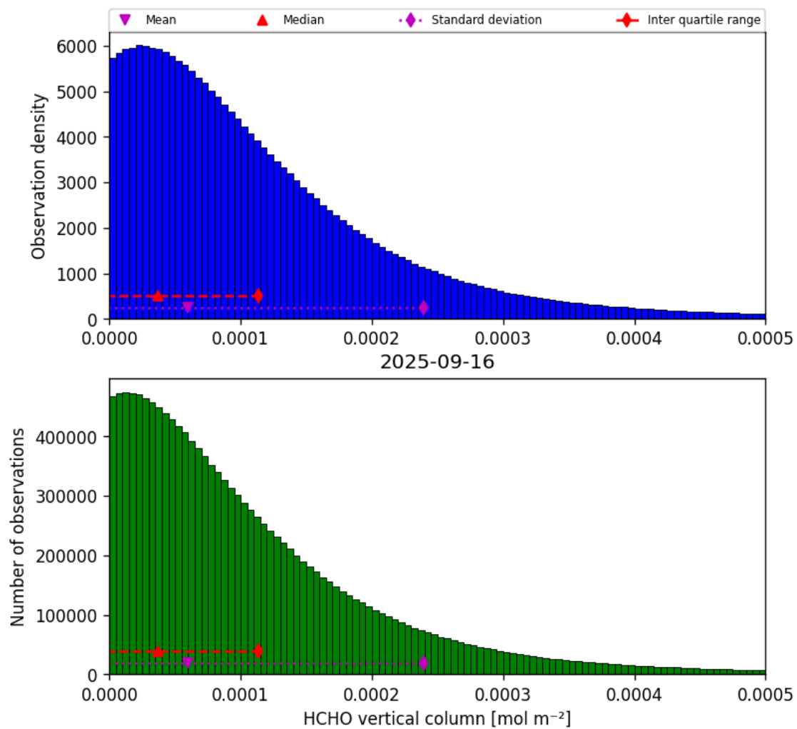
Figure 33: Histogram of “HCHO vertical column” for 2025-09-16 to 2025-09-17
