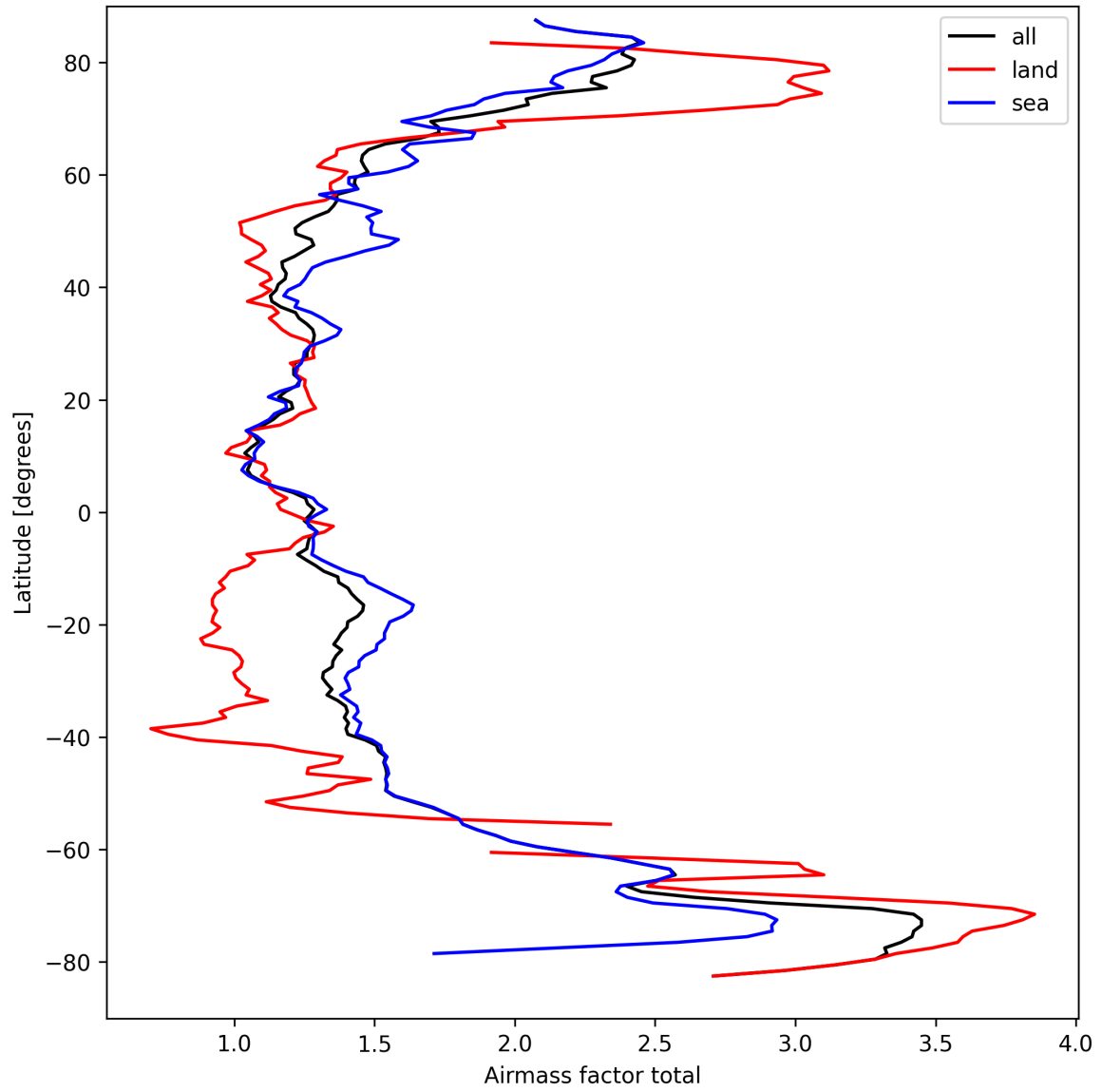
Figure 24: Zonal average of “Airmass factor total” for 2025-09-16 to 2025-09-17.
