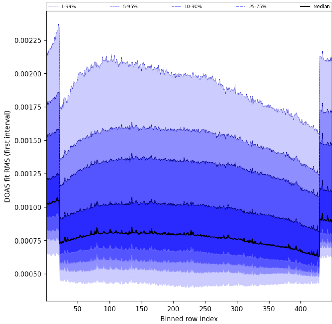
Figure 58: Along track statistics of “DOAS fit RMS (first interval)” for 2025-09-16 to 2025-09-17
