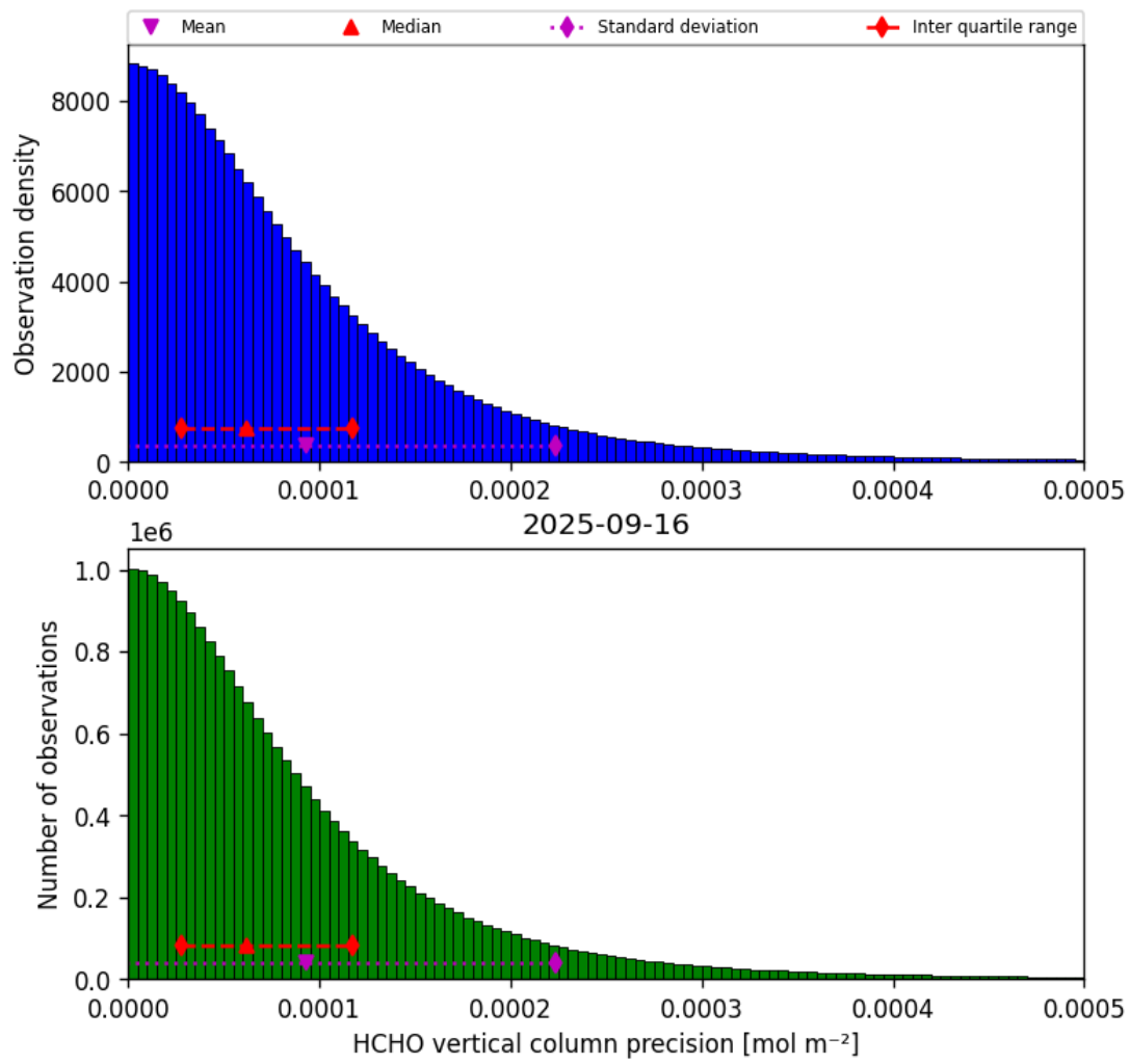
Figure 34: Histogram of “HCHO vertical column precision” for 2025-09-16 to 2025-09-17
