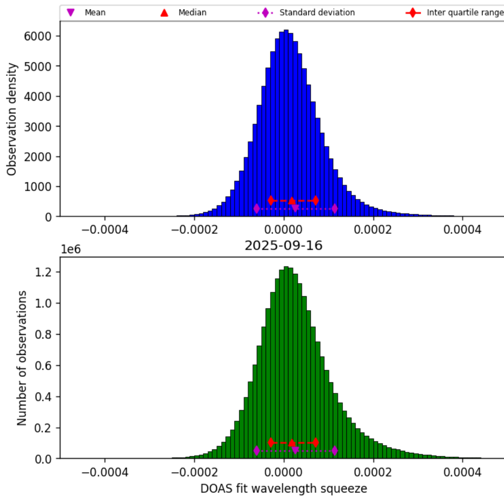
Figure 43: Histogram of “DOAS fit wavelength squeeze” for 2025-09-16 to 2025-09-17
