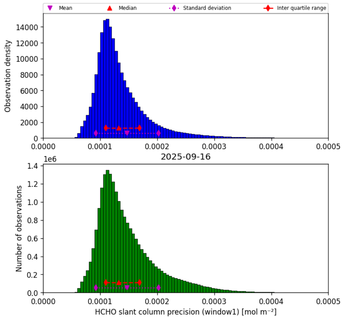
Figure 37: Histogram of “HCHO slant column precision (window1)” for 2025-09-16 to 2025-09-17
