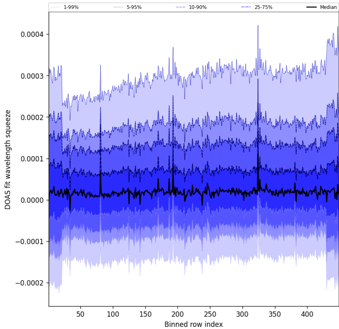
Figure 57: Along track statistics of “DOAS fit wavelength squeeze” for 2025-09-16 to 2025-09-17
