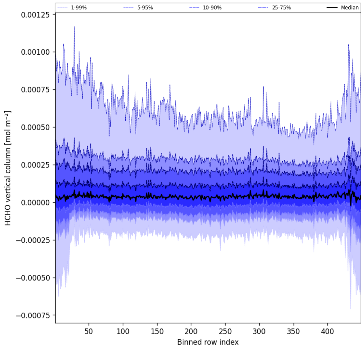
Figure 47: Along track statistics of “HCHO vertical column” for 2025-09-16 to 2025-09-17
