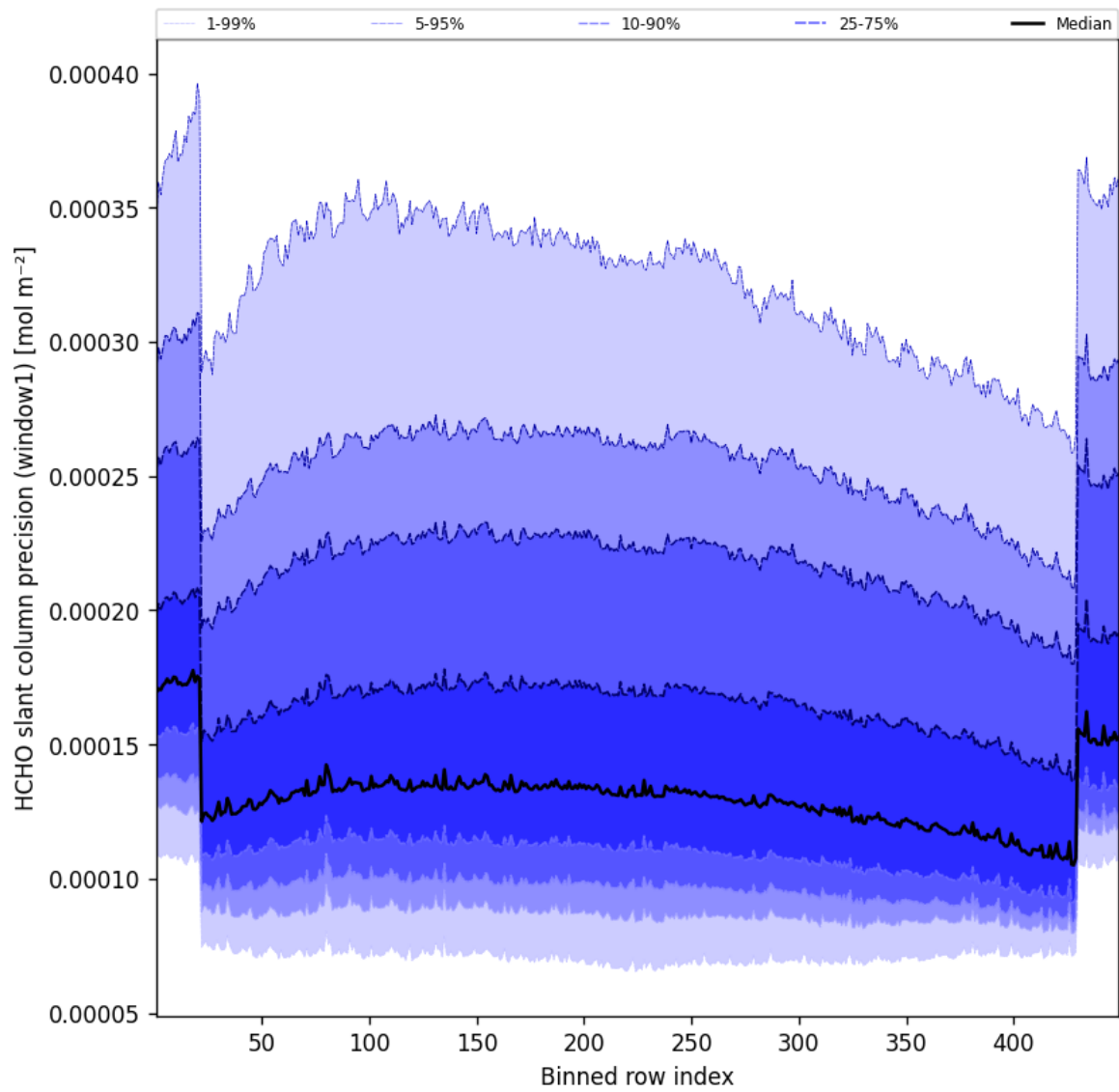
Figure 51: Along track statistics of “HCHO slant column precision (window1)” for 2025-09-16 to 2025-09-17
