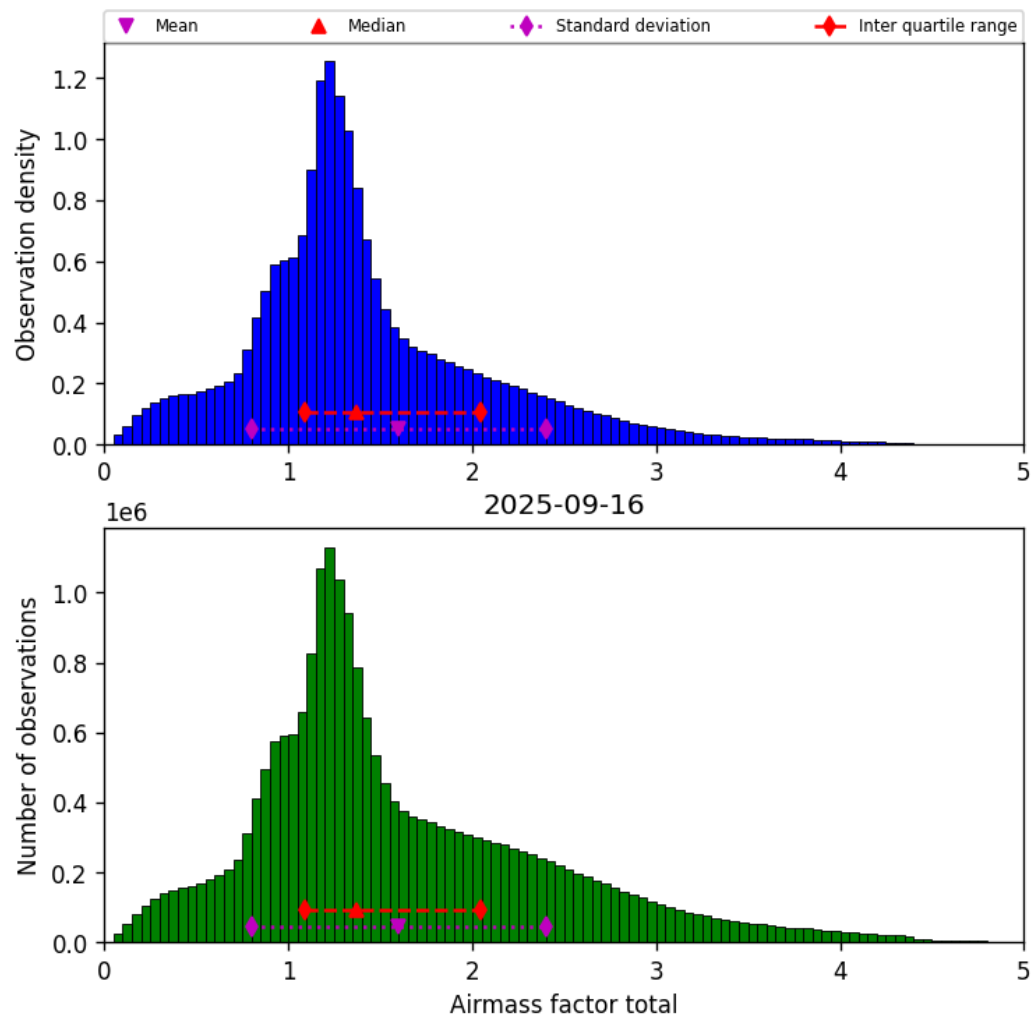
Figure 38: Histogram of “Airmass factor total” for 2025-09-16 to 2025-09-17
