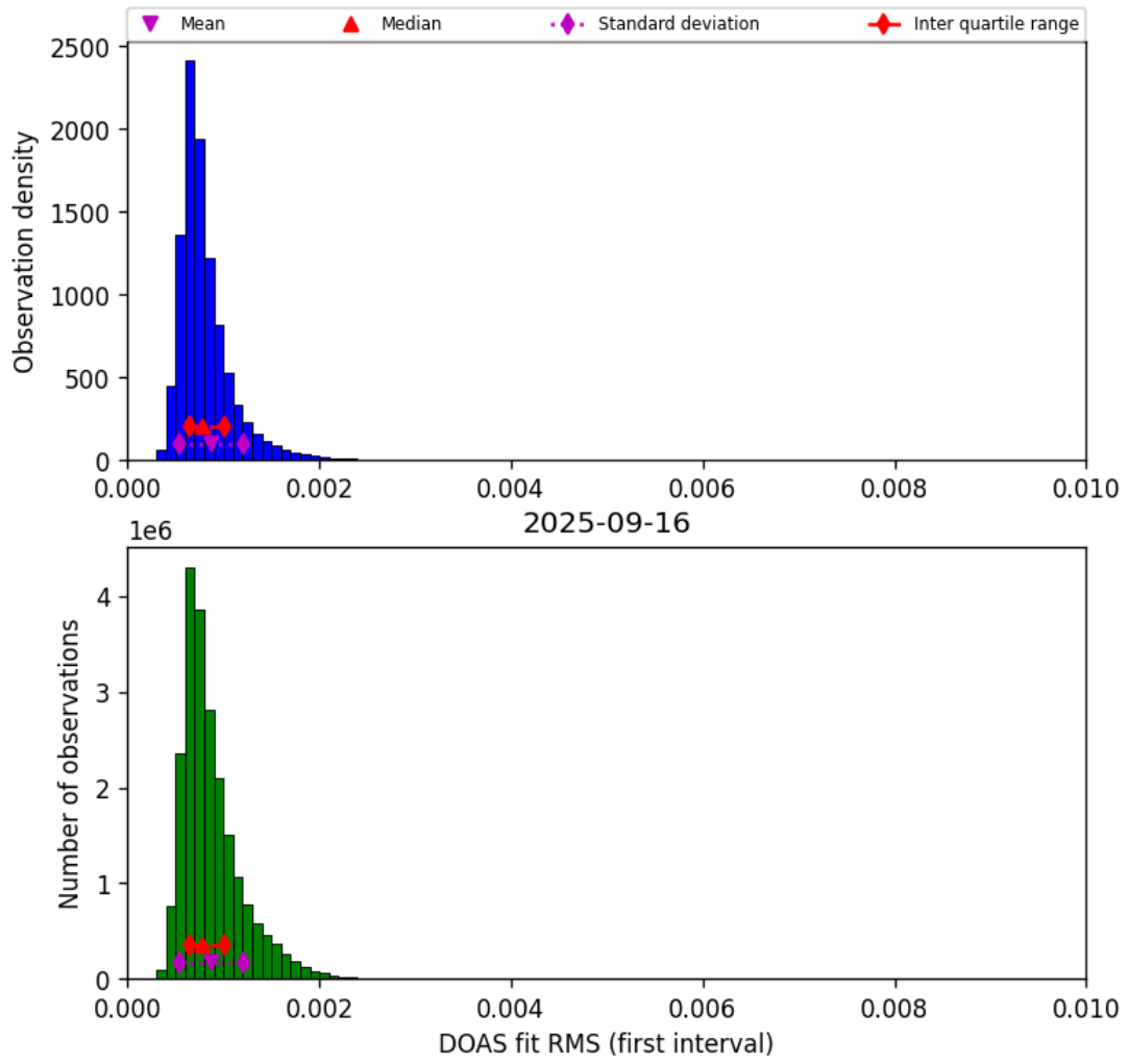
Figure 44: Histogram of “DOAS fit RMS (first interval)” for 2025-09-16 to 2025-09-17
