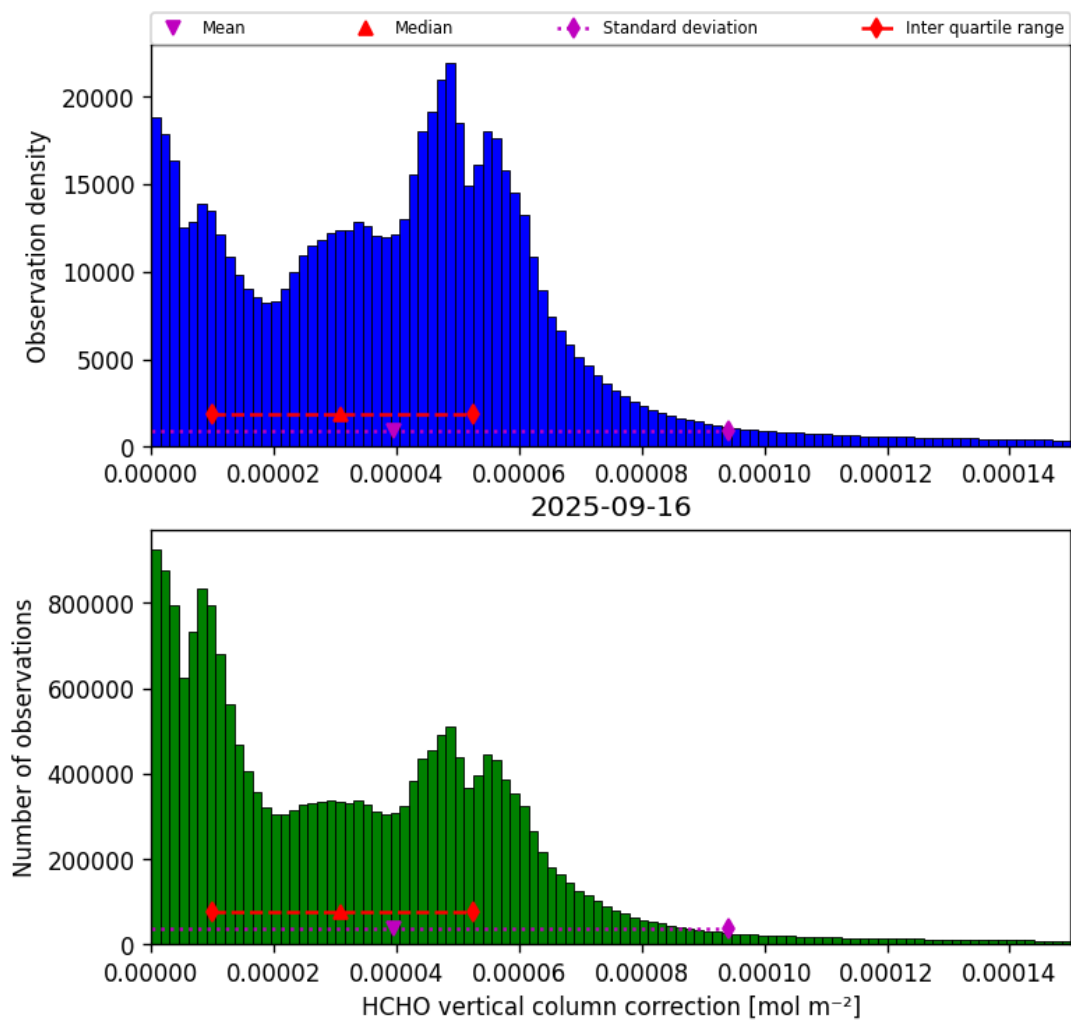
Figure 35: Histogram of “HCHO vertical column correction” for 2025-09-16 to 2025-09-17
