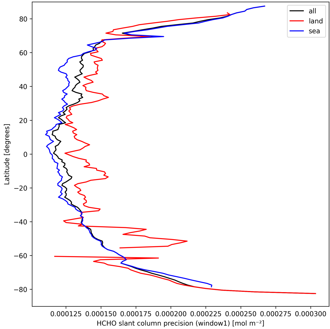
Figure 23: Zonal average of "HCHO slant column precision (window1)" for 2025-09-16 to 2025-09-17.
