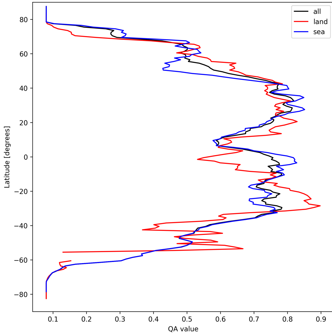
Figure 18: Zonal average of “QA value” for 2025-09-16 to 2025-09-17.
