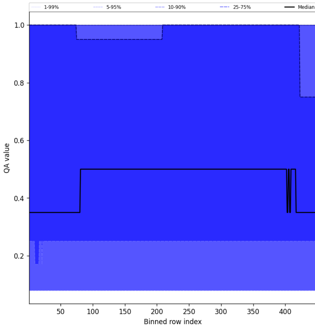
Figure 46: Along track statistics of “QA value” for 2025-09-17 to 2025-09-18
