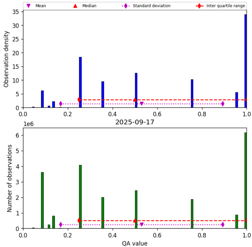
Figure 32: Histogram of “QA value” for 2025-09-17 to 2025-09-18
