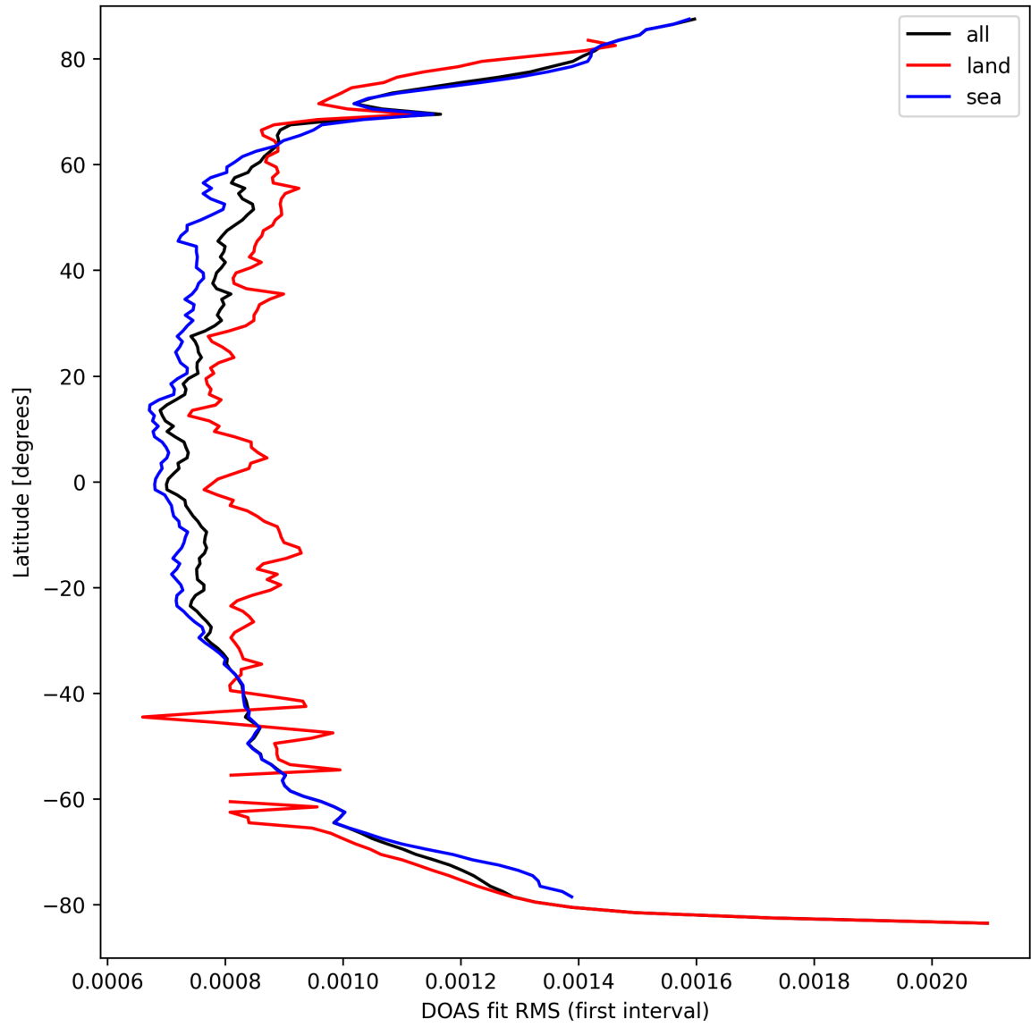
Figure 30: Zonal average of “DOAS fit RMS (first interval)” for 2025-09-17 to 2025-09-18.
