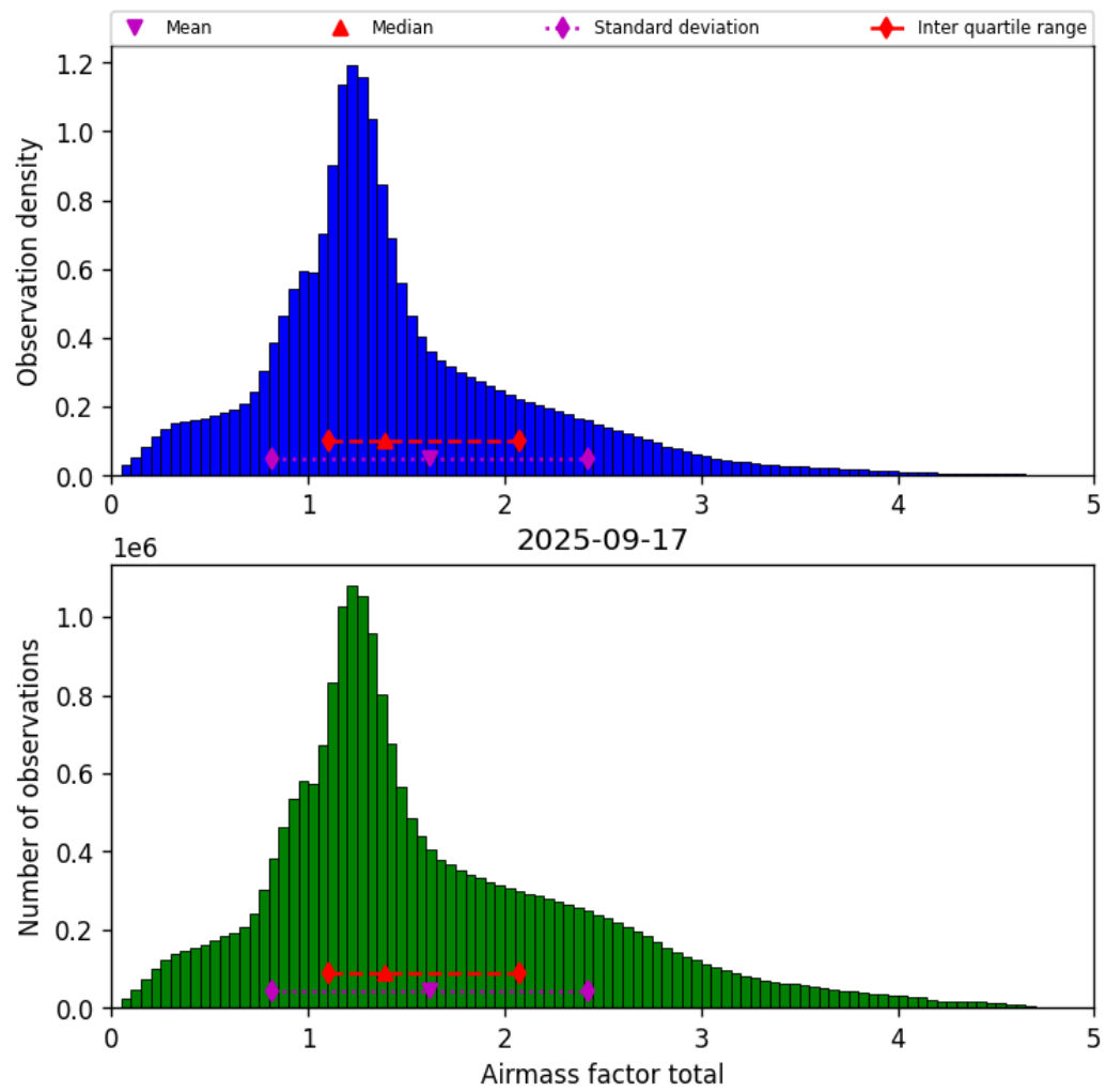
Figure 38: Histogram of “Airmass factor total” for 2025-09-17 to 2025-09-18
