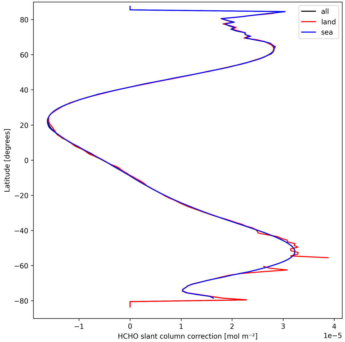
Figure 31: Zonal average of "HCHO slant column correction" for 2025-09-17 to 2025-09-18.
