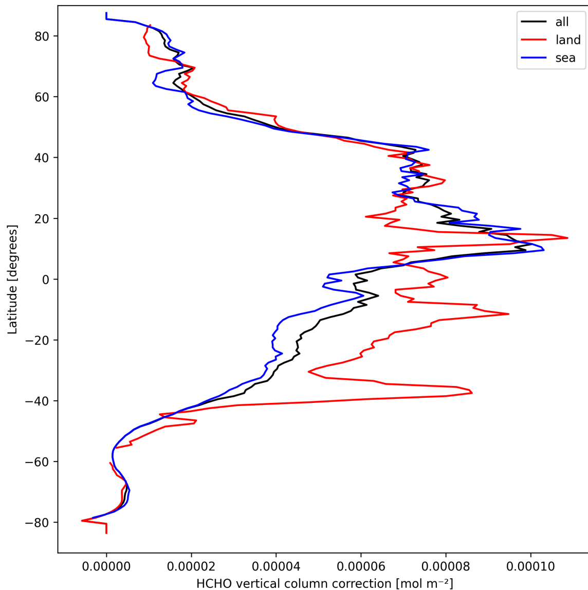
Figure 21: Zonal average of “HCHO vertical column correction” for 2025-09-17 to 2025-09-18.
