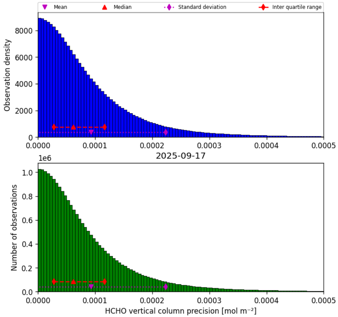
Figure 34: Histogram of “HCHO vertical column precision” for 2025-09-17 to 2025-09-18
