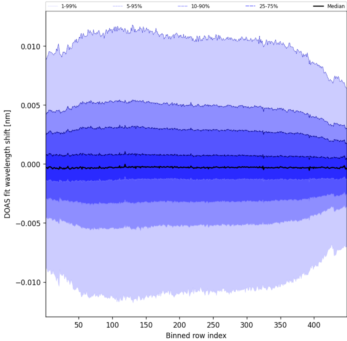
Figure 56: Along track statistics of “DOAS fit wavelength shift” for 2025-09-17 to 2025-09-18
