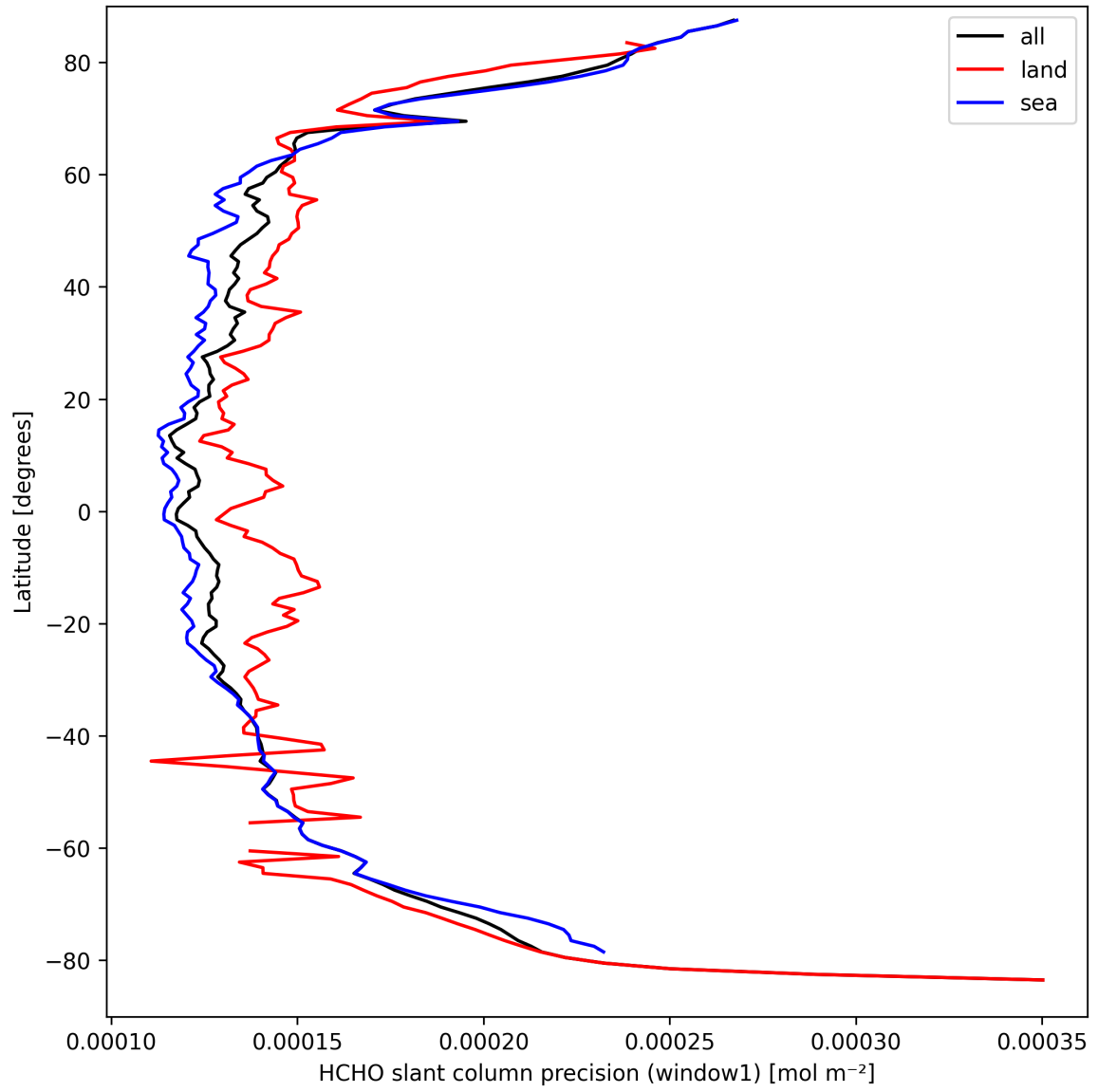
Figure 23: Zonal average of “HCHO slant column precision (window1)” for 2025-09-17 to 2025-09-18.
