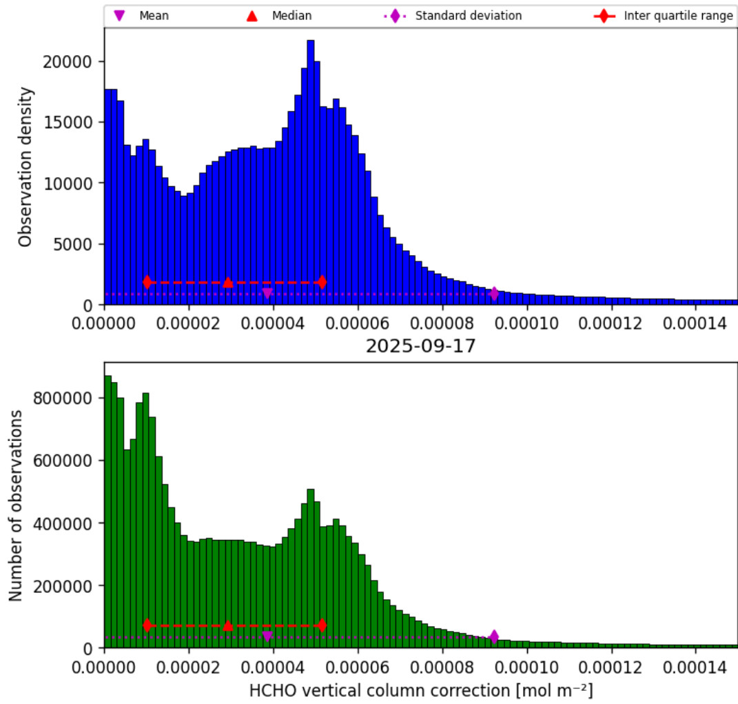
Figure 35: Histogram of “HCHO vertical column correction” for 2025-09-17 to 2025-09-18
