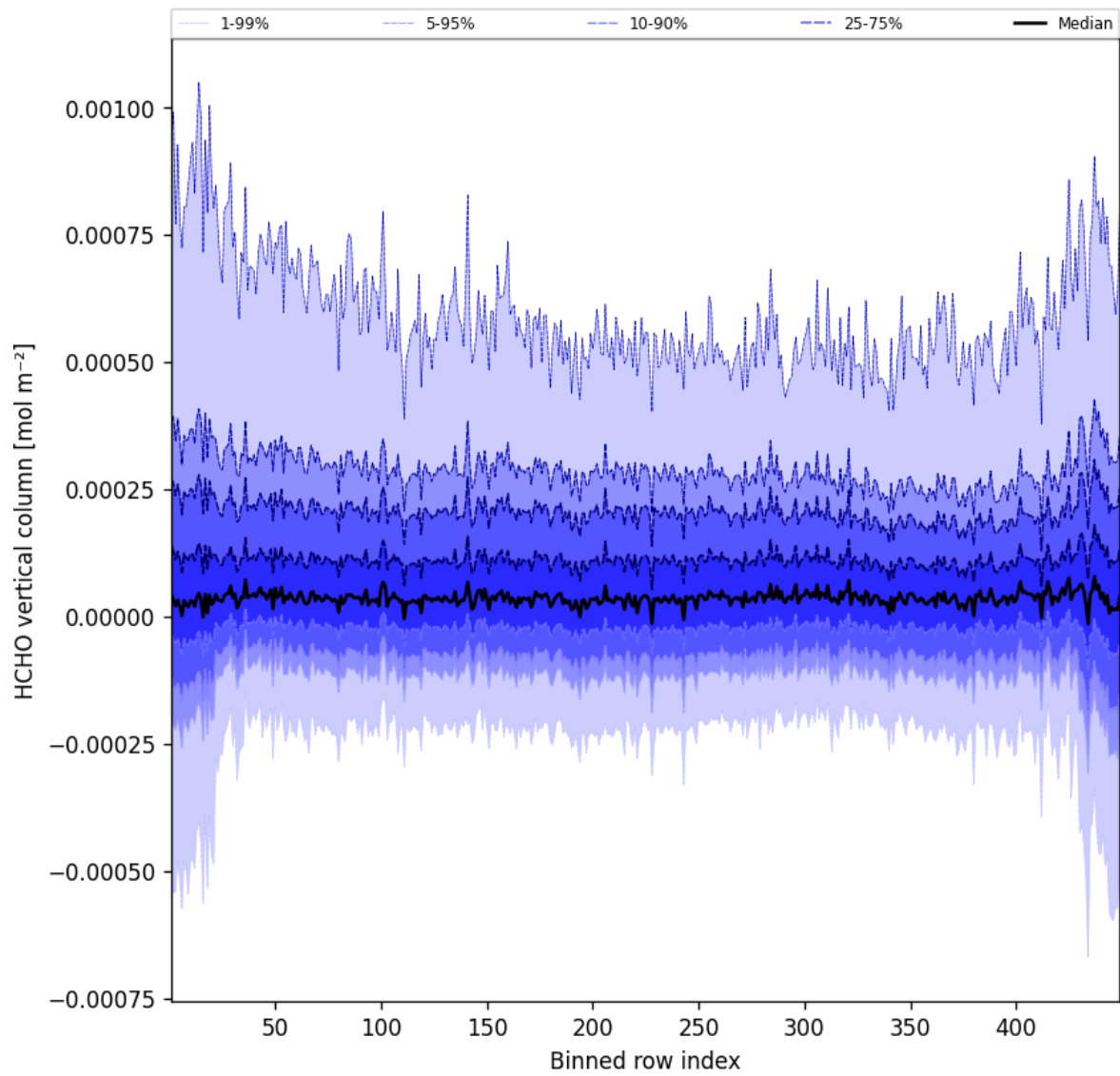
Figure 47: Along track statistics of “HCHO vertical column” for 2025-09-17 to 2025-09-18
