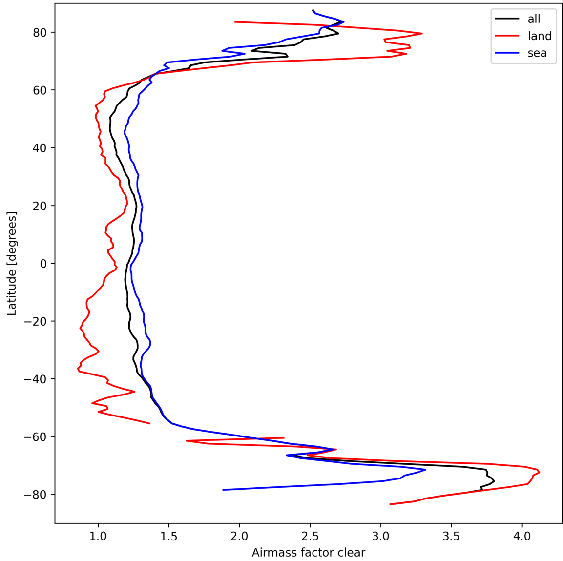
Figure 26: Zonal average of “Airmass factor clear” for 2025-09-17 to 2025-09-18.
