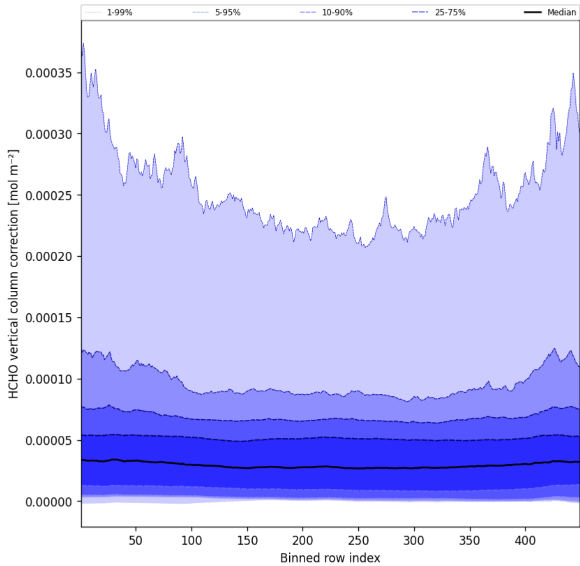
Figure 49: Along track statistics of “HCHO vertical column correction” for 2025-09-17 to 2025-09-18
