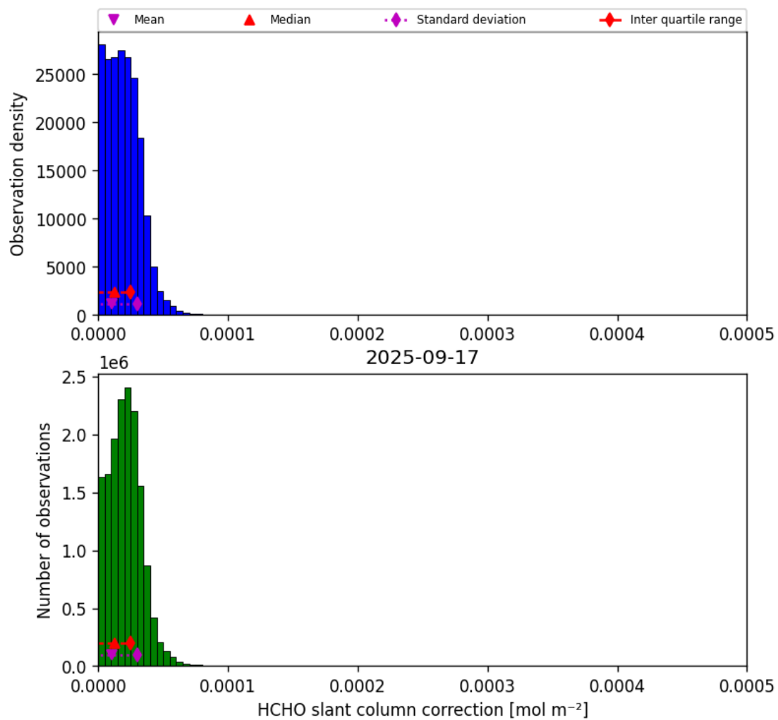
Figure 45: Histogram of “HCHO slant column correction” for 2025-09-17 to 2025-09-18
