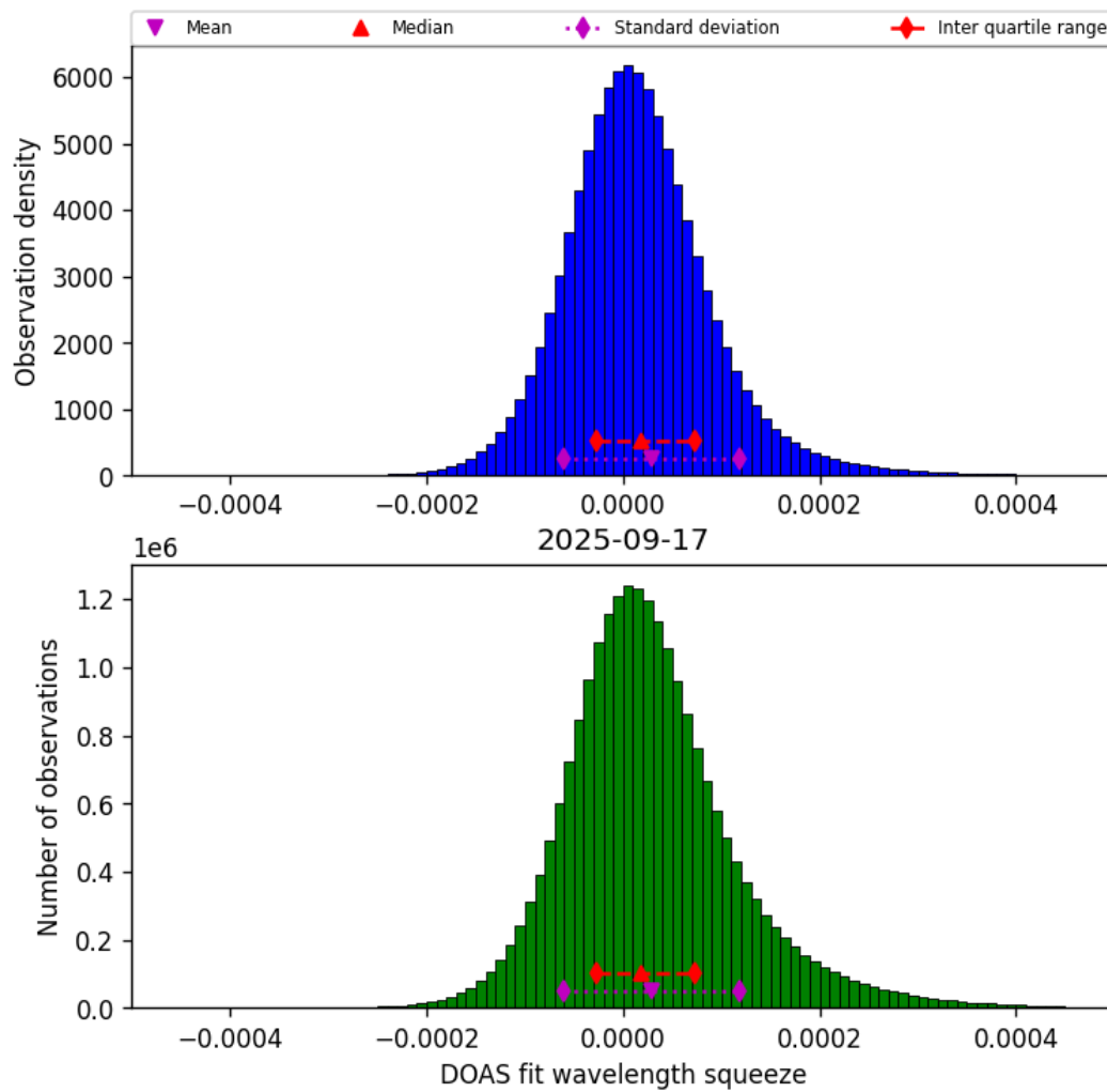
Figure 43: Histogram of “DOAS fit wavelength squeeze” for 2025-09-17 to 2025-09-18
