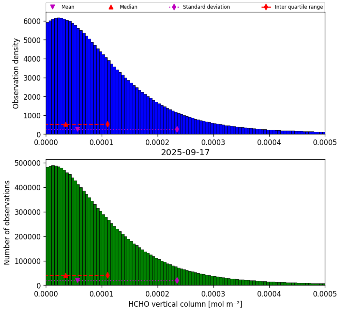
Figure 33: Histogram of “HCHO vertical column” for 2025-09-17 to 2025-09-18
