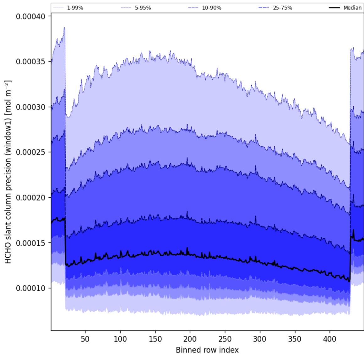
Figure 51: Along track statistics of “HCHO slant column precision (window1)” for 2025-09-17 to 2025-09-18
