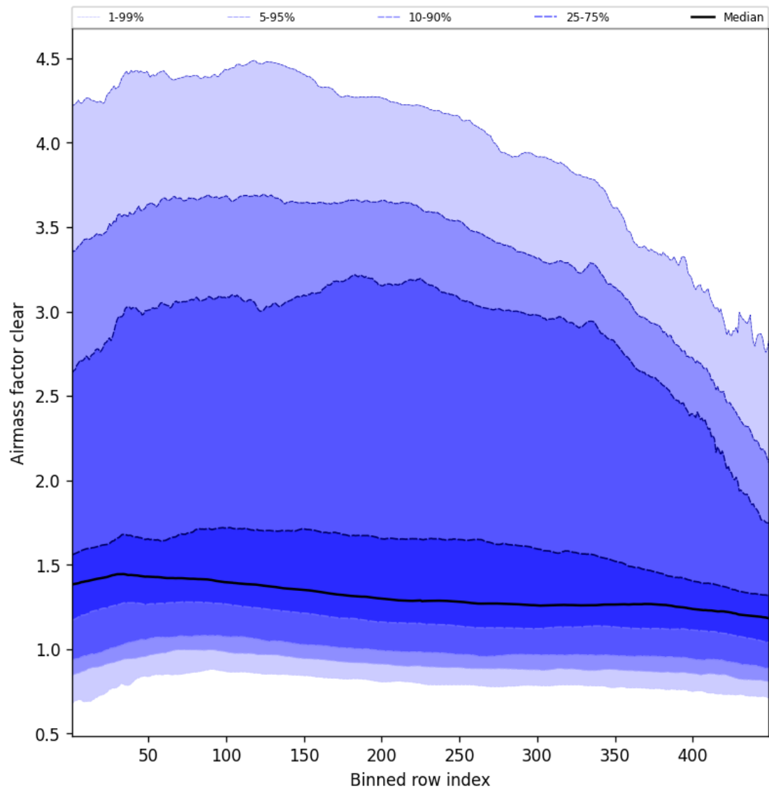
Figure 54: Along track statistics of “Air mass factor clear” for 2025-09-17 to 2025-09-18
