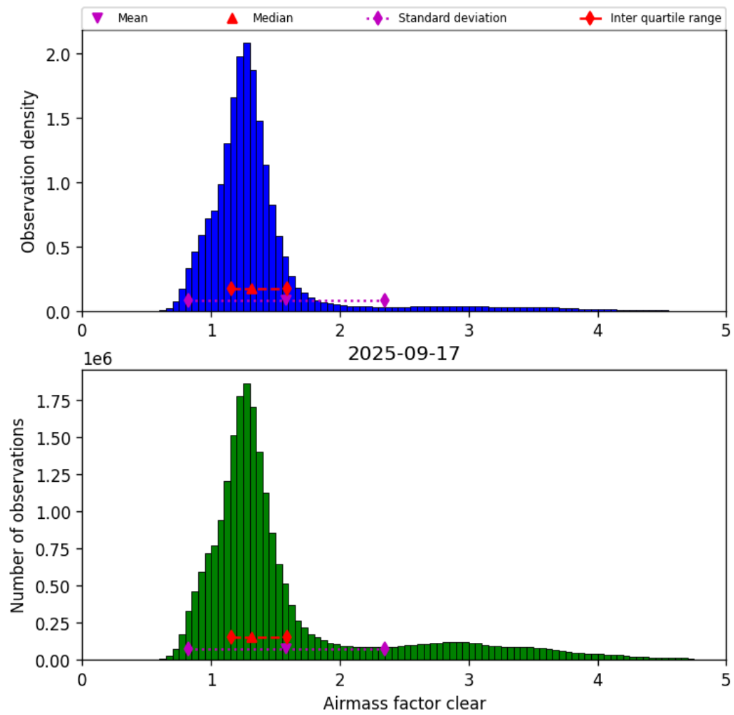
Figure 40: Histogram of “Airmass factor clear” for 2025-09-17 to 2025-09-18
