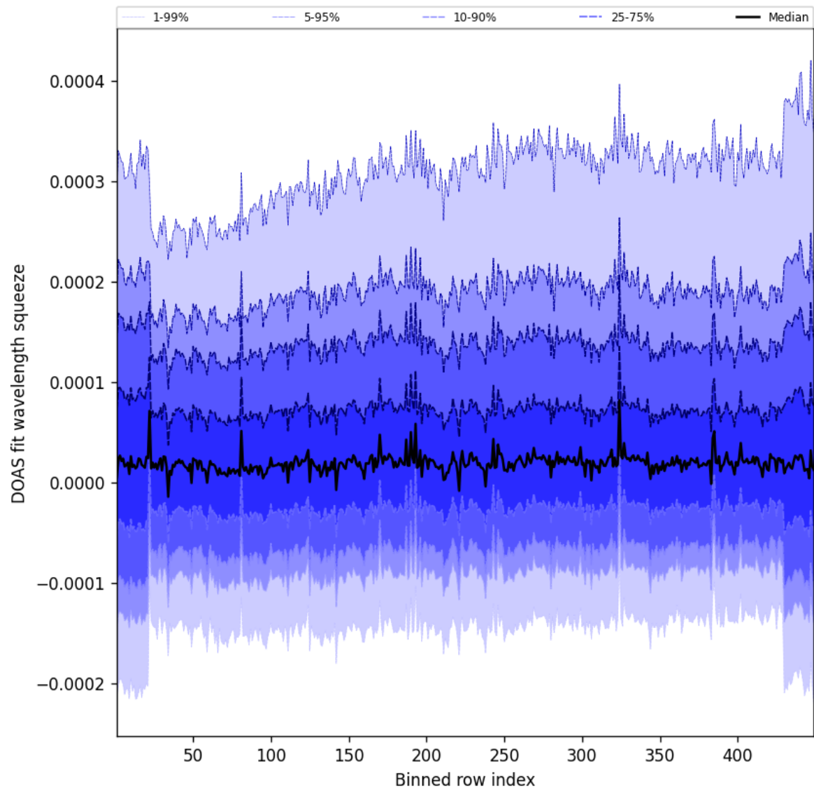
Figure 57: Along track statistics of “DOAS fit wavelength squeeze” for 2025-09-17 to 2025-09-18
