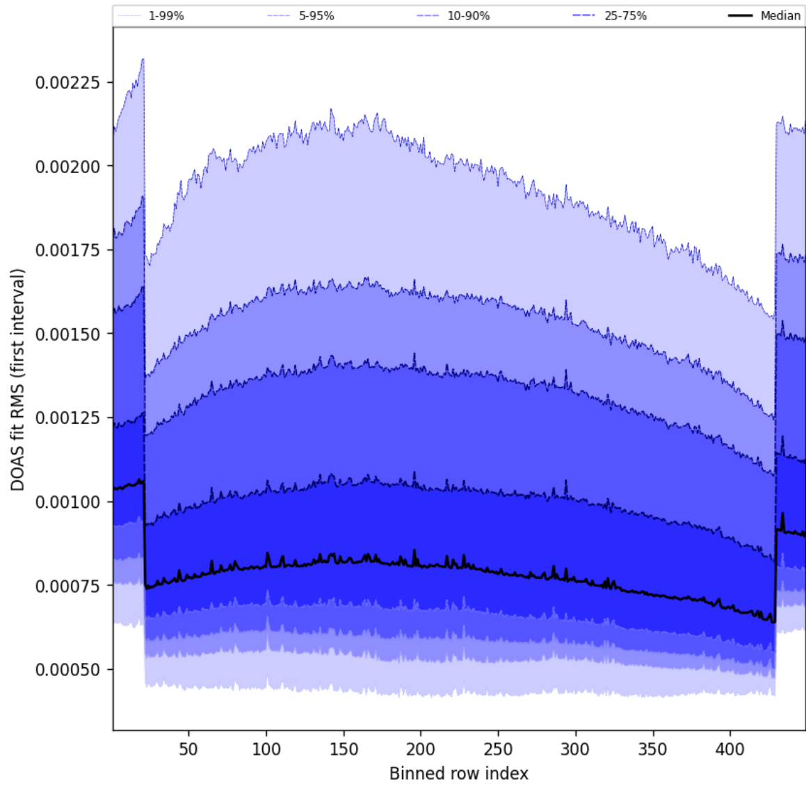
Figure 58: Along track statistics of “DOAS fit RMS (first interval)” for 2025-09-17 to 2025-09-18
