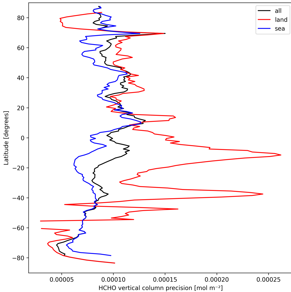
Figure 20: Zonal average of “HCHO vertical column precision” for 2025-09-17 to 2025-09-18.
