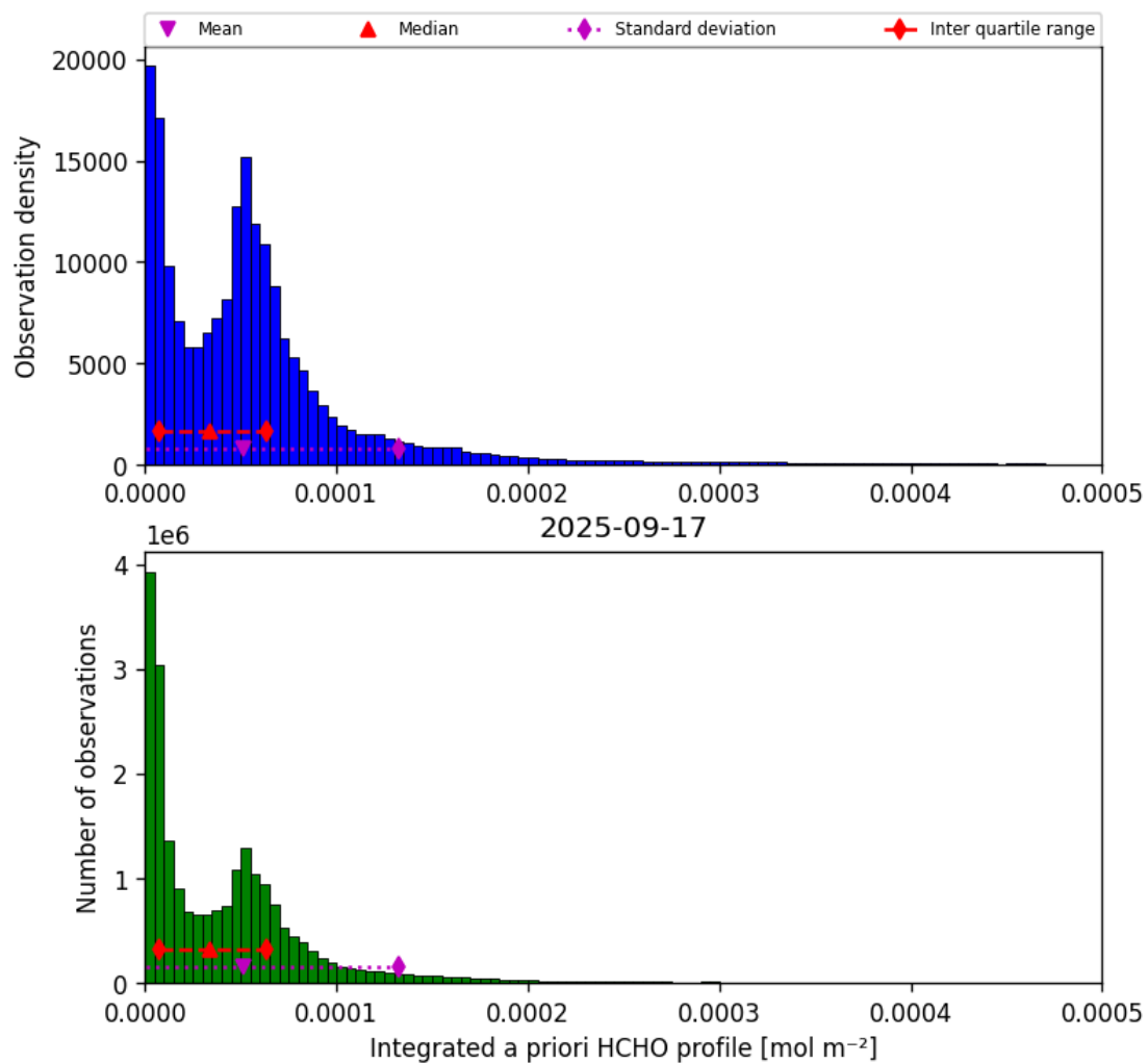
Figure 41: Histogram of “Integrated a priori HCHO profile” for 2025-09-17 to 2025-09-18
