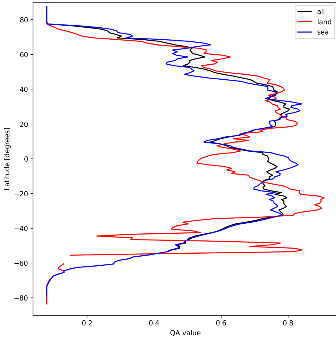
Figure 18: Zonal average of “QA value” for 2025-09-17 to 2025-09-18.
