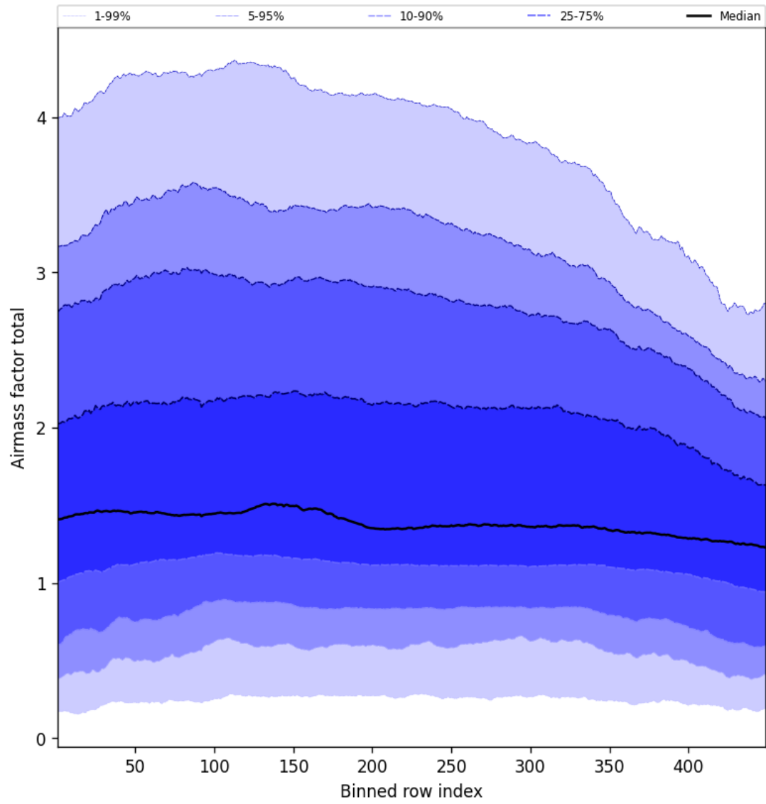
Figure 52: Along track statistics of “Airmass factor total” for 2025-09-17 to 2025-09-18
