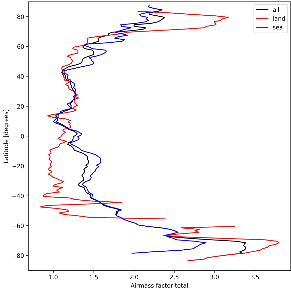
Figure 24: Zonal average of “Airmass factor total” for 2025-09-17 to 2025-09-18.
