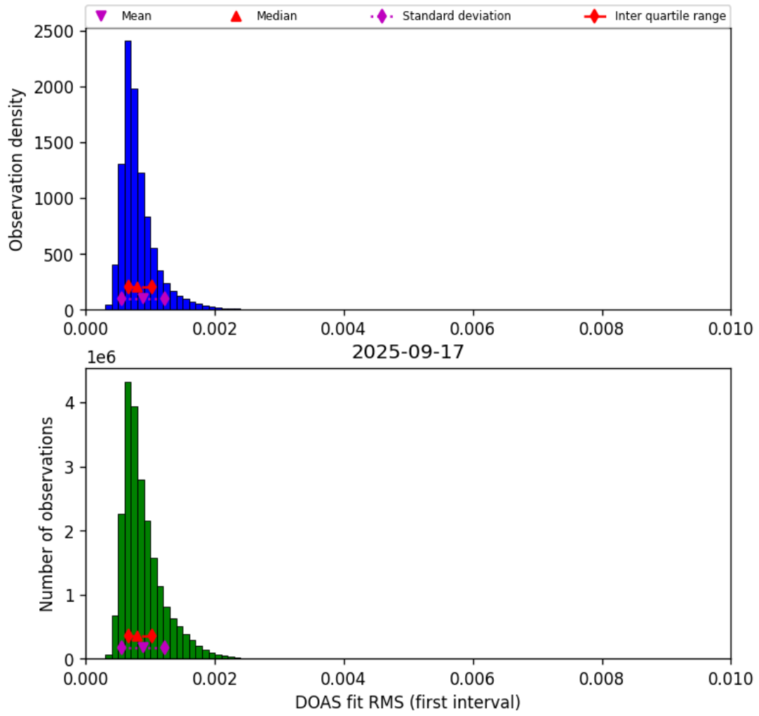
Figure 44: Histogram of “DOAS fit RMS (first interval)” for 2025-09-17 to 2025-09-18
