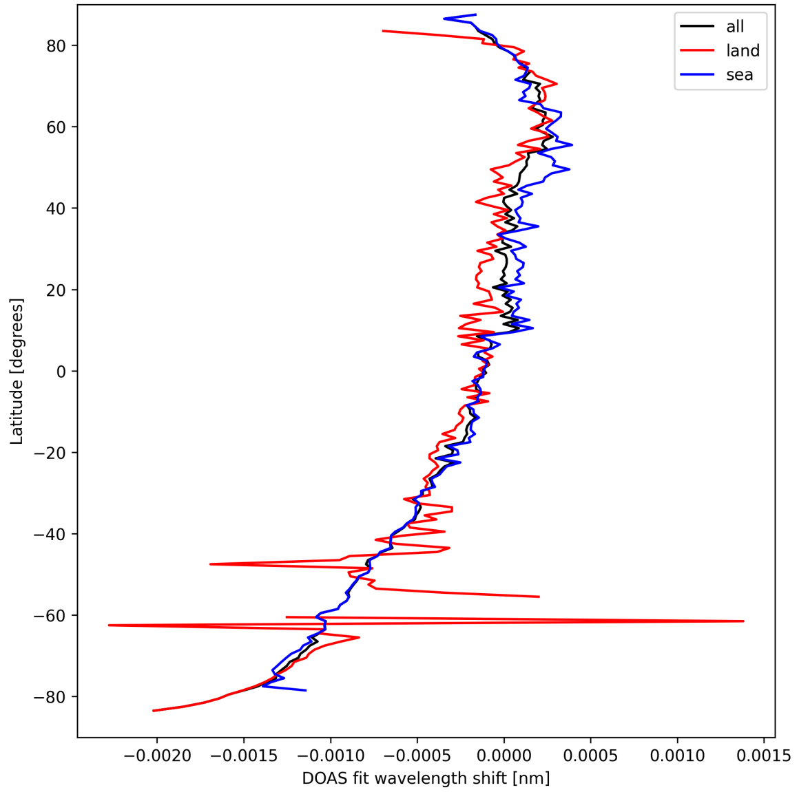
Figure 28: Zonal average of “DOAS fit wavelength shift” for 2025-09-17 to 2025-09-18.
