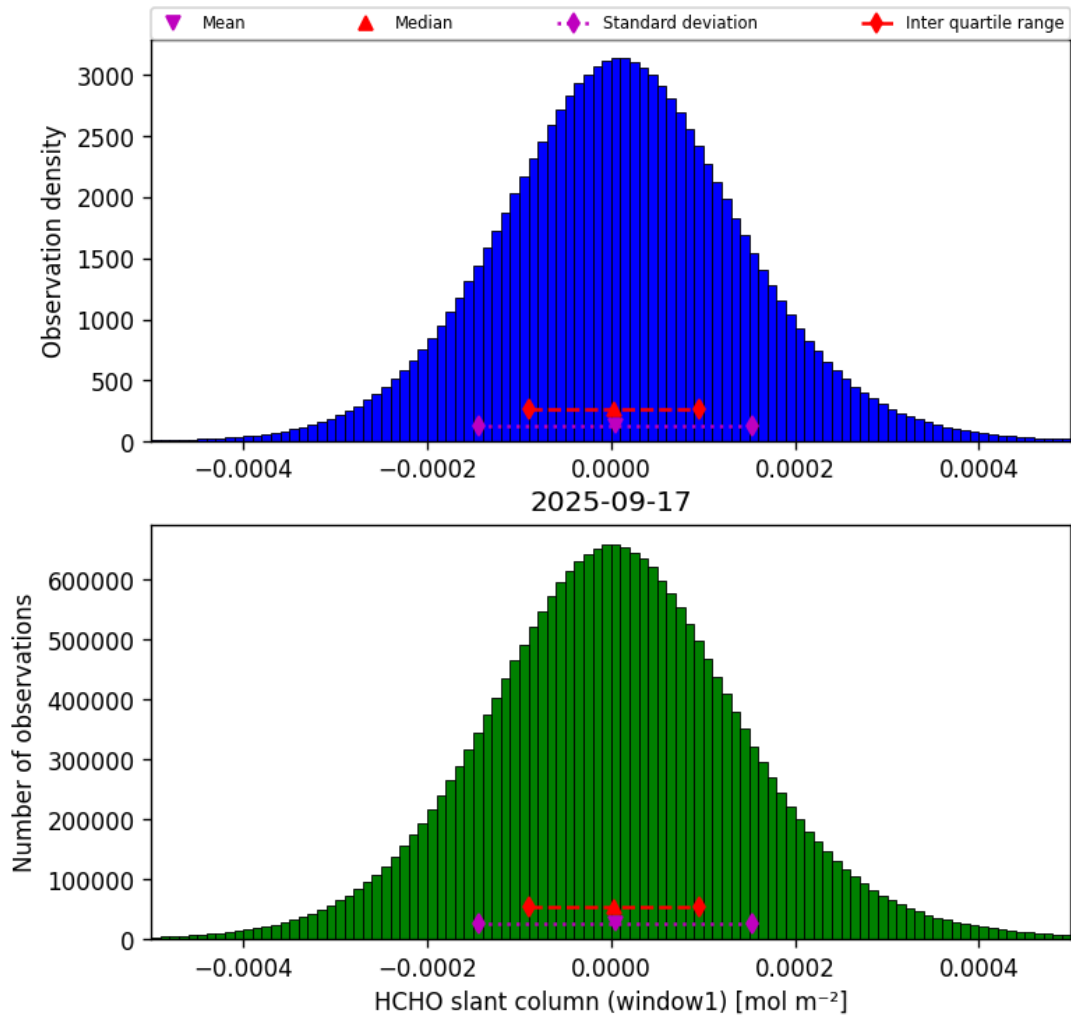
Figure 36: Histogram of “HCHO slant column (window1)” for 2025-09-17 to 2025-09-18
