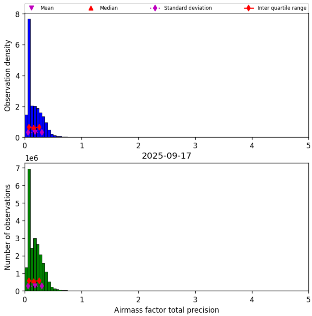
Figure 39: Histogram of “Airmass factor total precision” for 2025-09-17 to 2025-09-18
