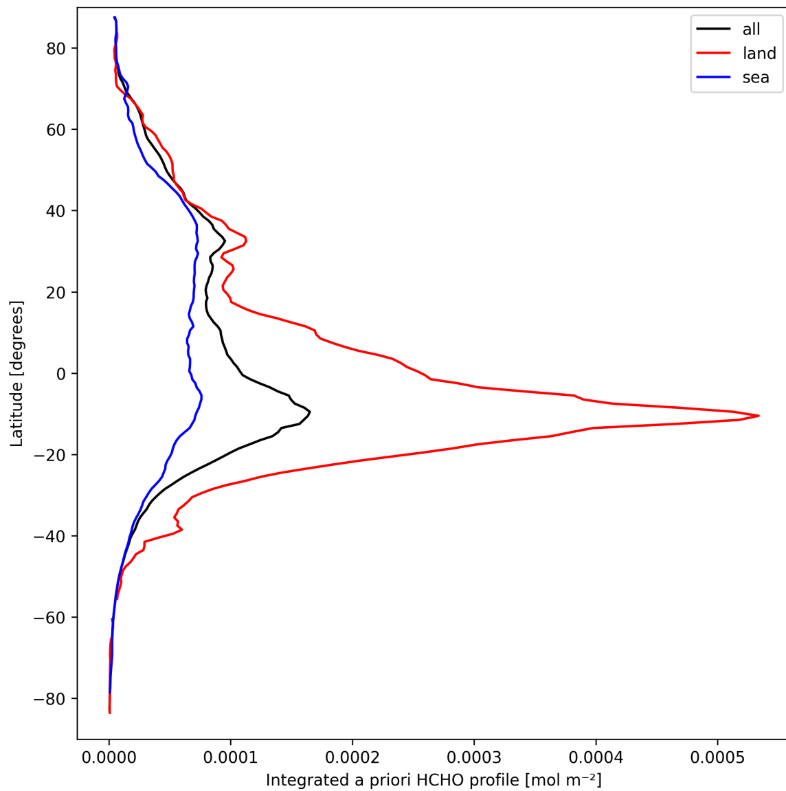
Figure 27: Zonal average of “Integrated a priori HCHO profile” for 2025-09-17 to 2025-09-18.
