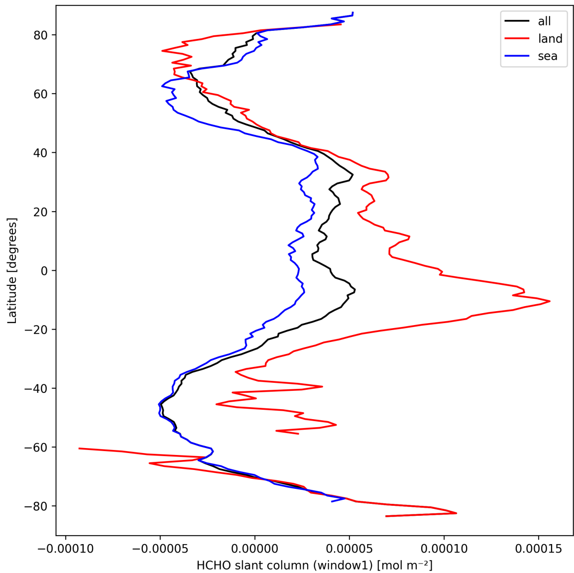
Figure 22: Zonal average of “HCHO slant column (window1)” for 2025-09-17 to 2025-09-18.
