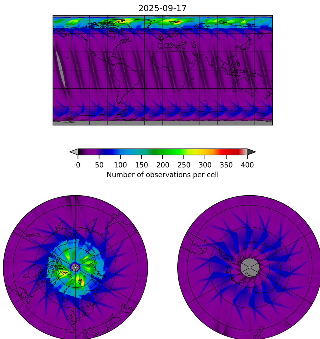
Figure 17: Map of the number of observations for 2025-09-17 to 2025-09-18
