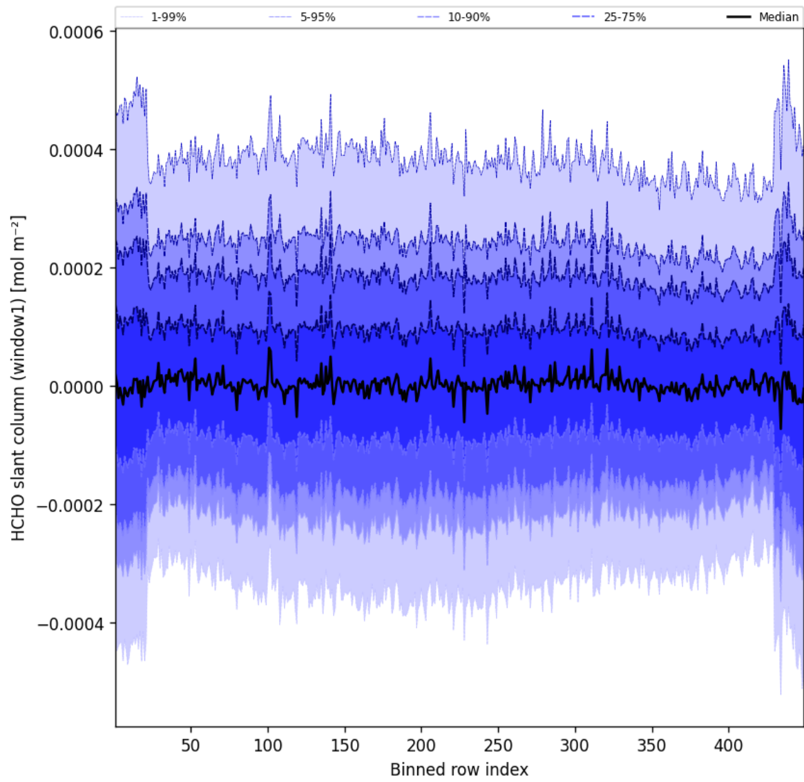
Figure 50: Along track statistics of “HCHO slant column (window1)” for 2025-09-17 to 2025-09-18
