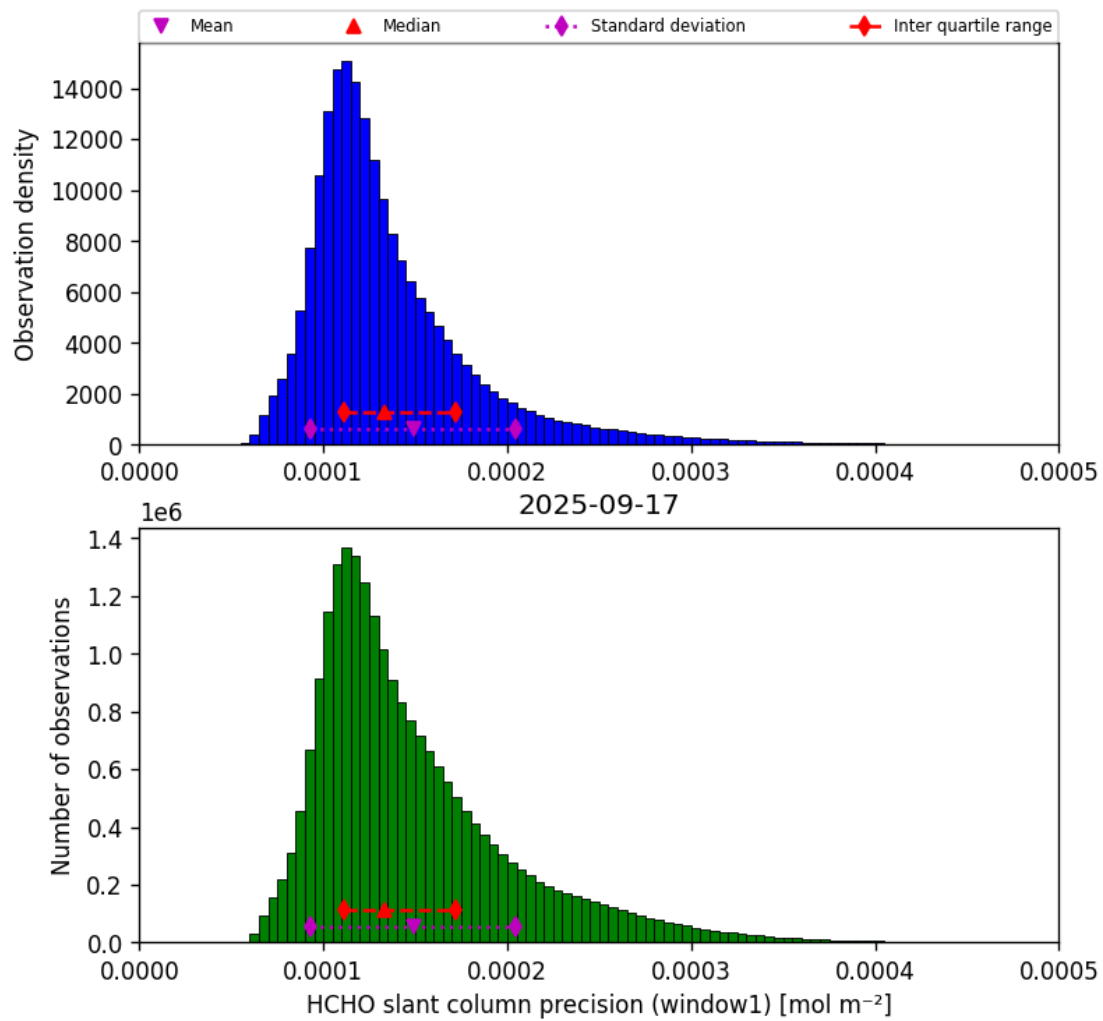
Figure 37: Histogram of “HCHO slant column precision (window1)” for 2025-09-17 to 2025-09-18
