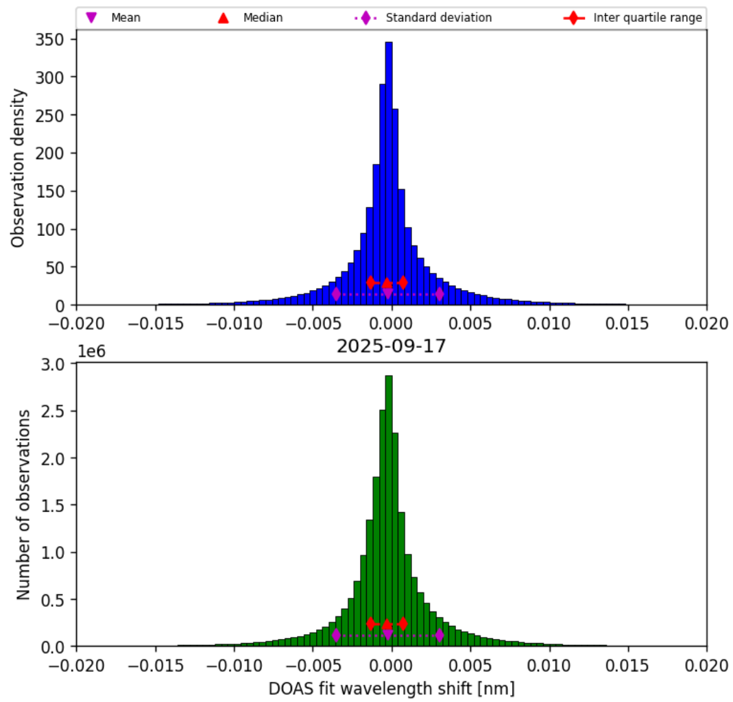
Figure 42: Histogram of “DOAS fit wavelength shift” for 2025-09-17 to 2025-09-18
