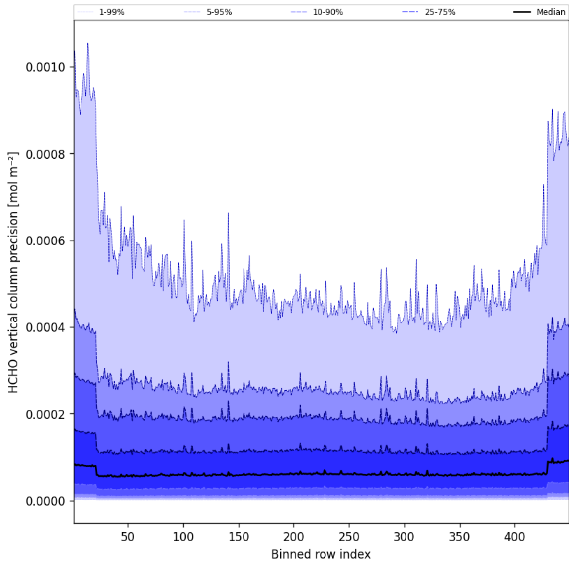
Figure 48: Along track statistics of “HCHO vertical column precision” for 2025-09-17 to 2025-09-18
