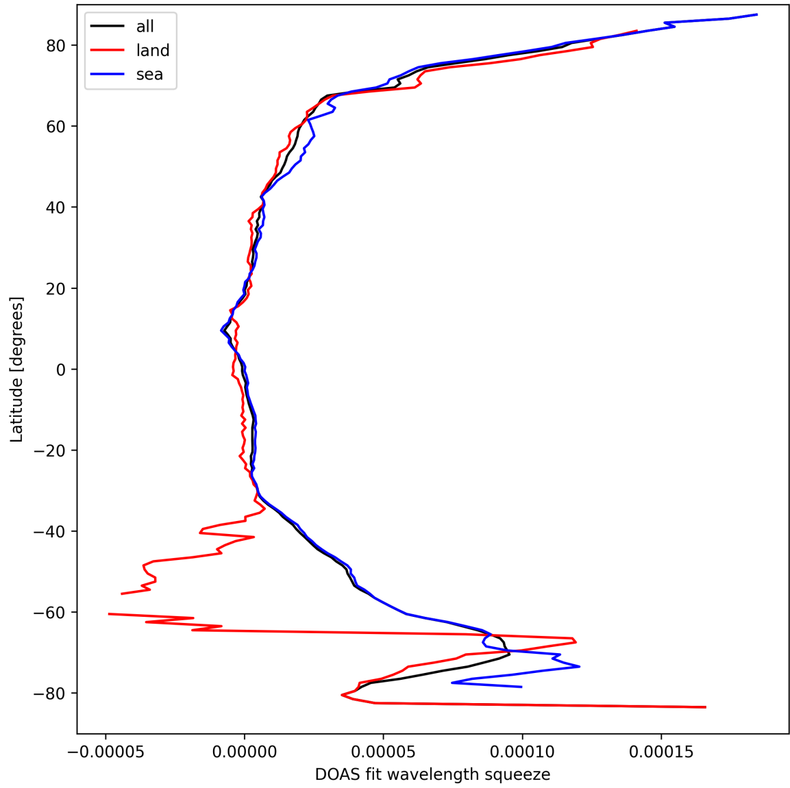
Figure 29: Zonal average of “DOAS fit wavelength squeeze” for 2025-09-17 to 2025-09-18.
