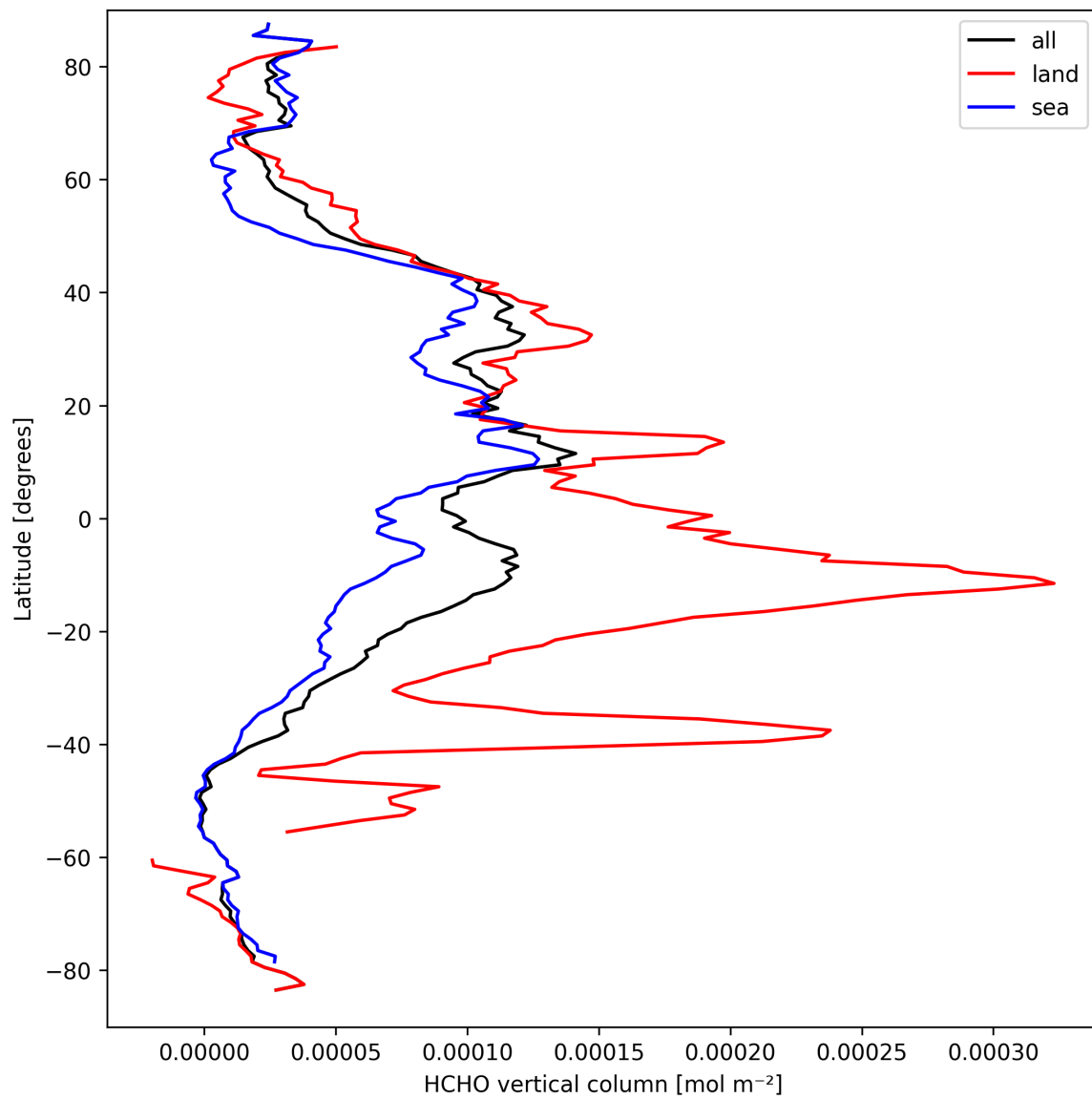
Figure 19: Zonal average of “HCHO vertical column” for 2025-09-17 to 2025-09-18.
