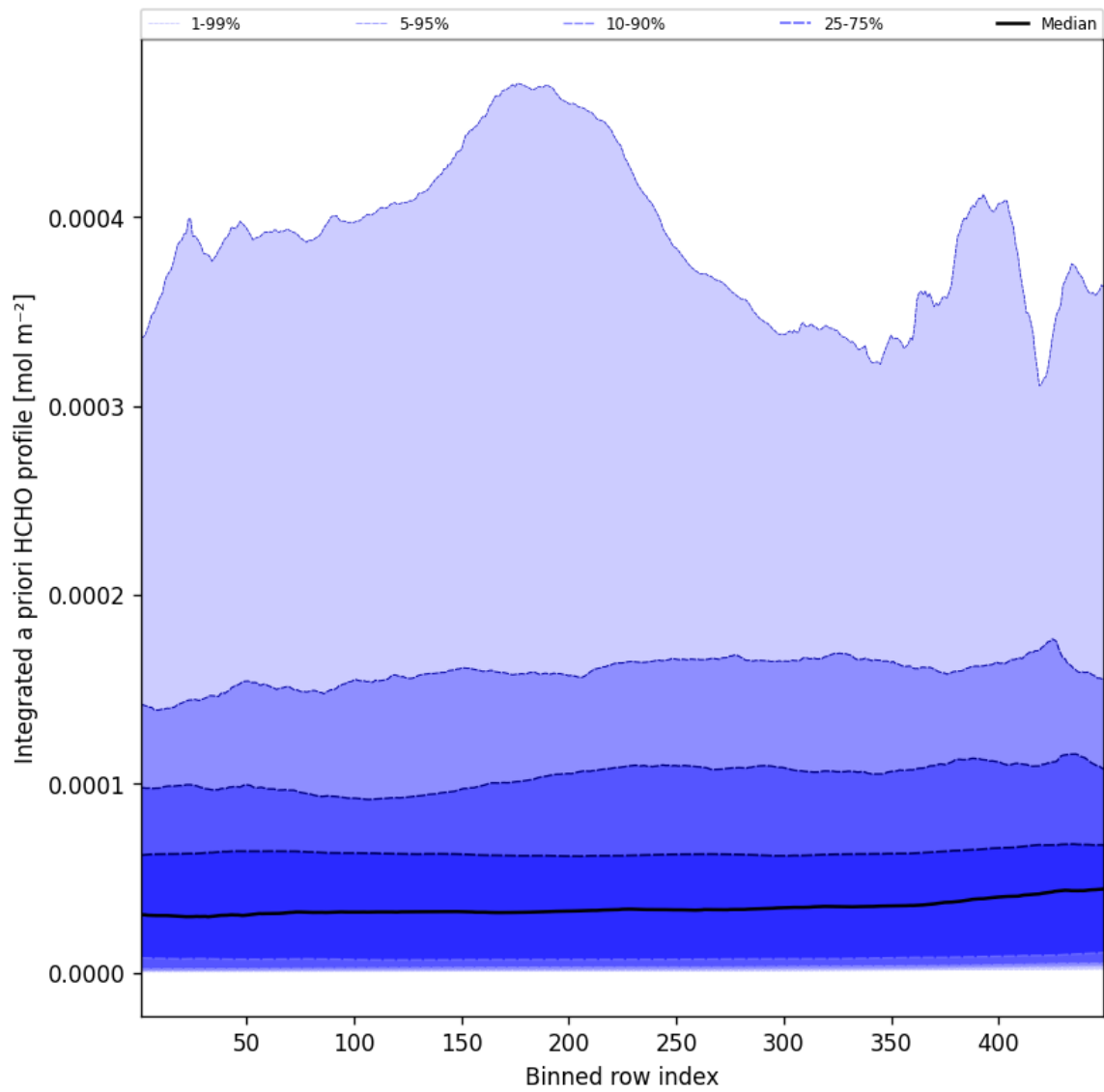
Figure 55: Along track statistics of "Integrated a priori HCHO profile" for 2025-09-17 to 2025-09-18
