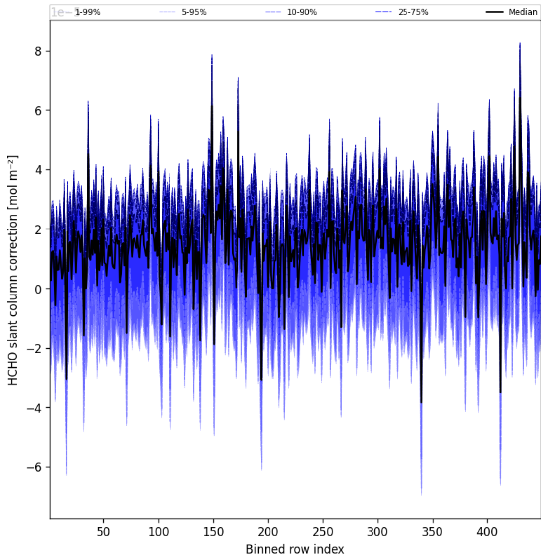
Figure 59: Along track statistics of “HCHO slant column correction” for 2025-09-17 to 2025-09-18
