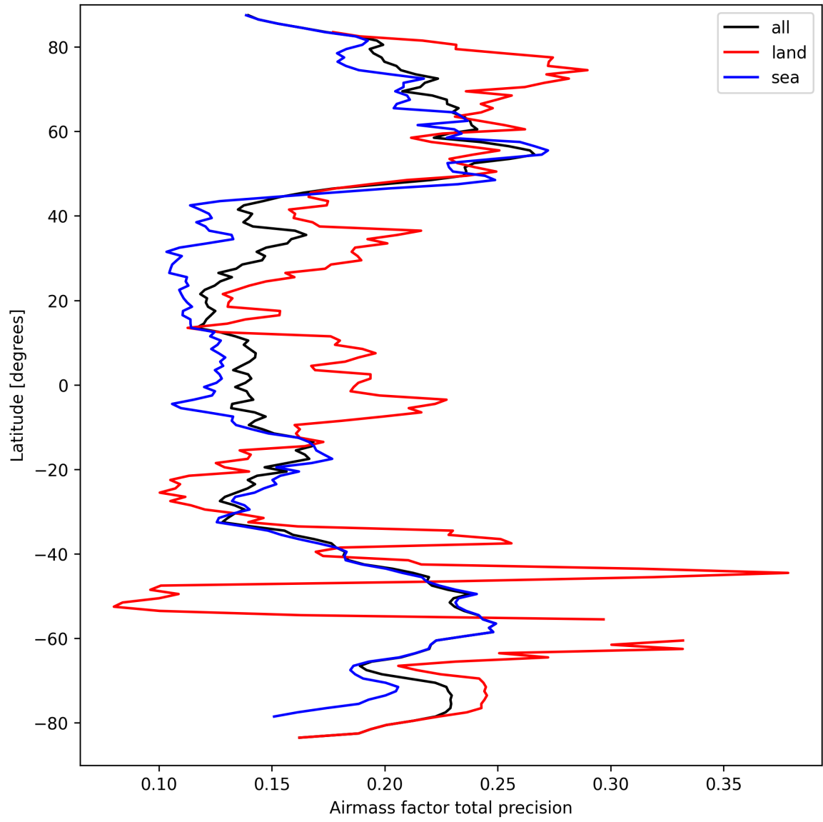
Figure 25: Zonal average of “Airmass factor total precision” for 2025-09-17 to 2025-09-18.
