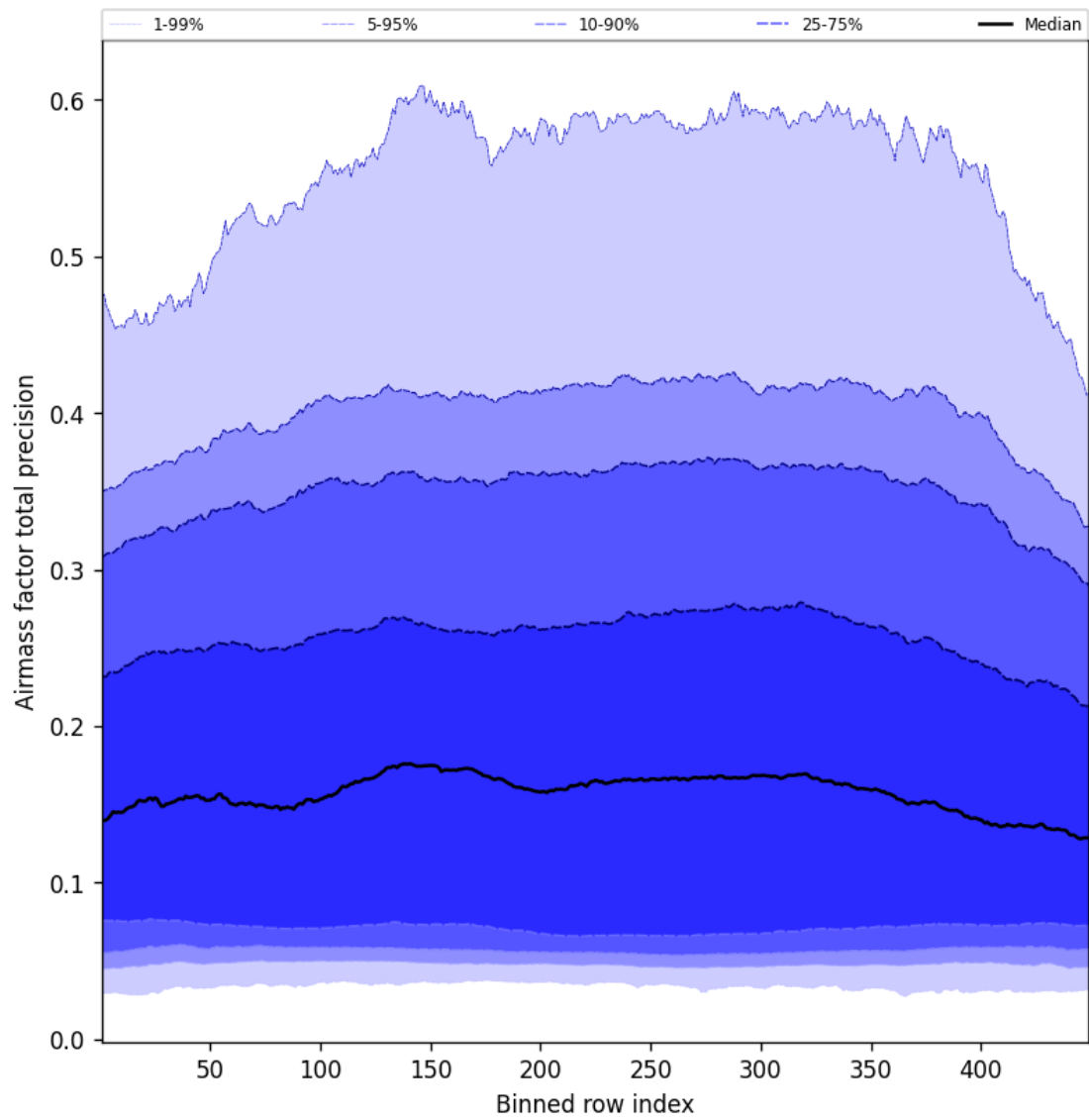
Figure 53: Along track statistics of “Airmass factor total precision” for 2025-09-17 to 2025-09-18
