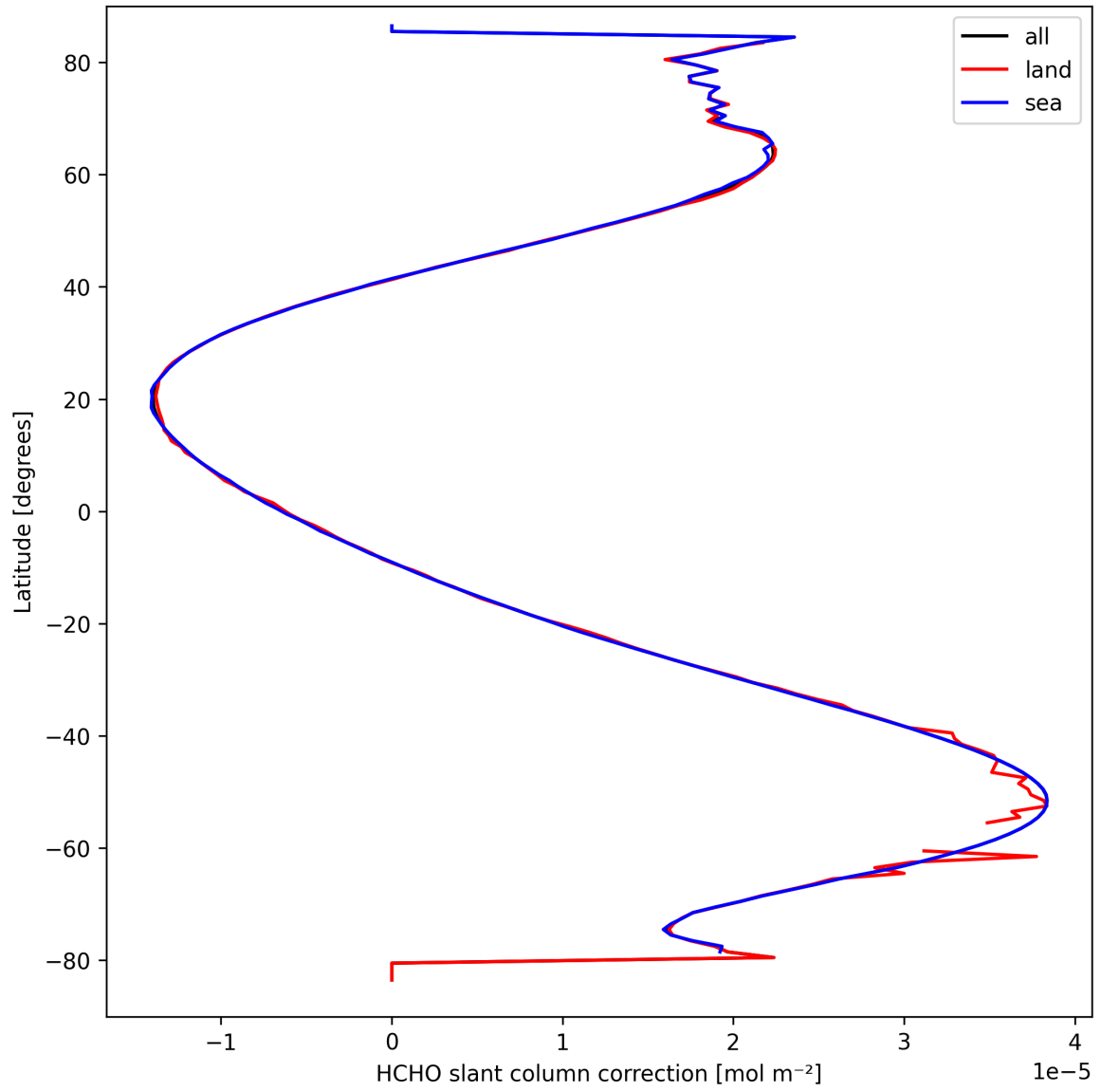
Figure 31: Zonal average of "HCHO slant column correction" for 2025-09-18 to 2025-09-18.
