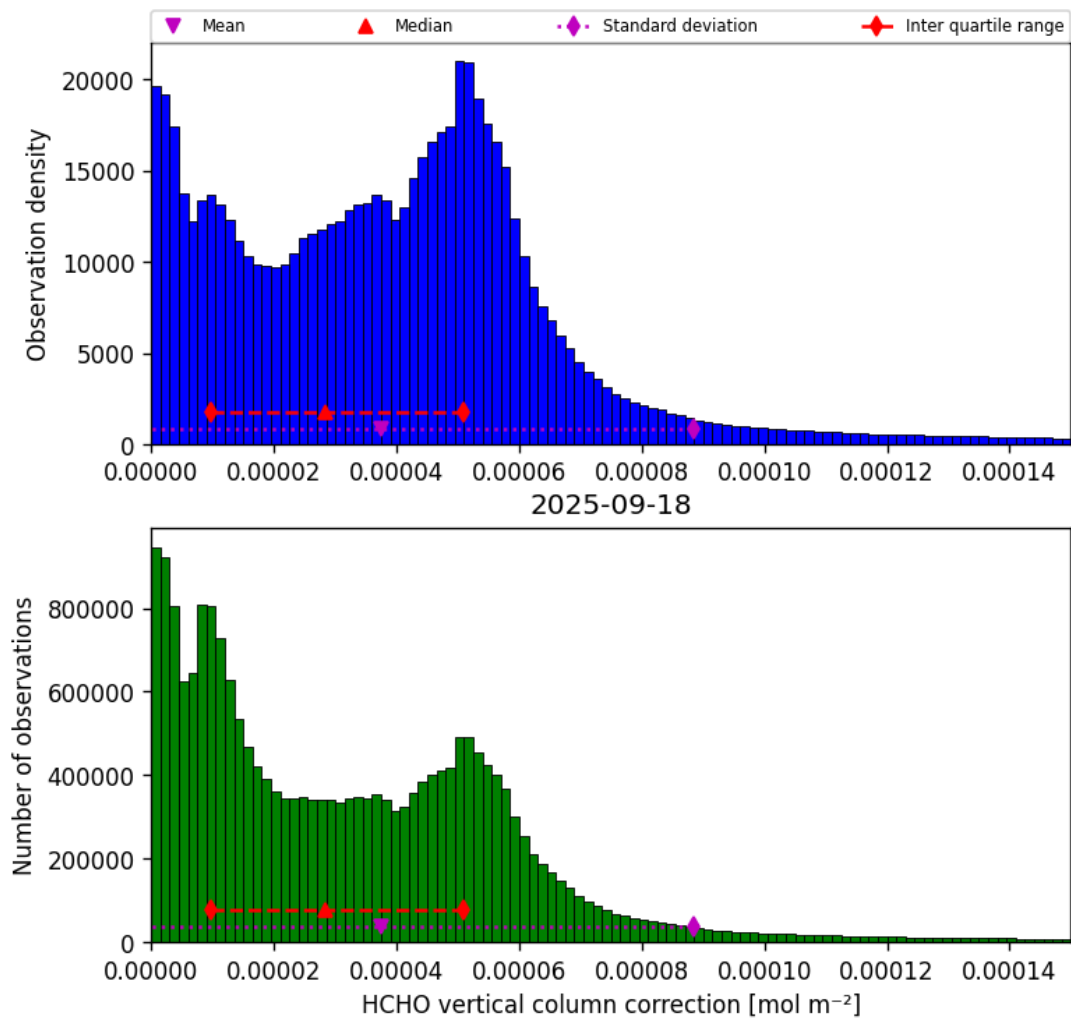
Figure 35: Histogram of “HCHO vertical column correction” for 2025-09-18 to 2025-09-18
