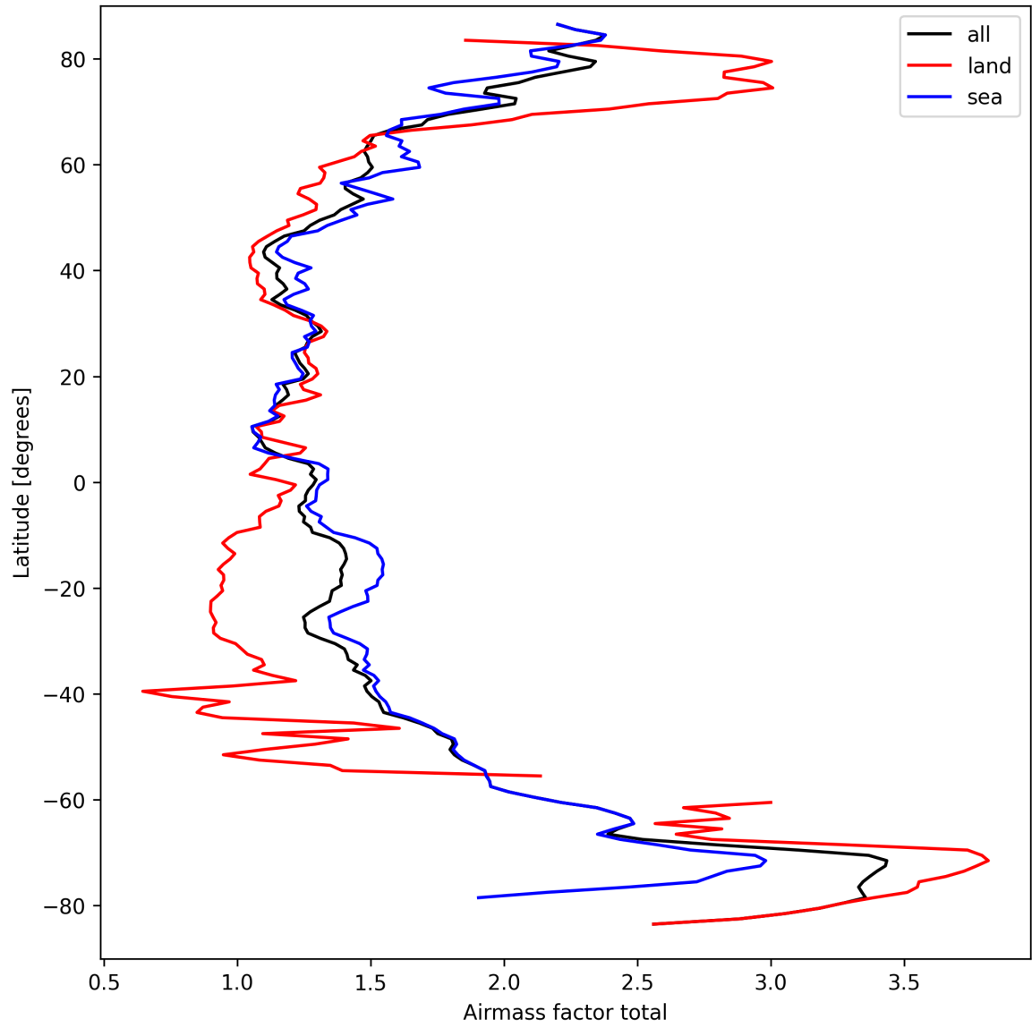
Figure 24: Zonal average of “Airmass factor total” for 2025-09-18 to 2025-09-18.
