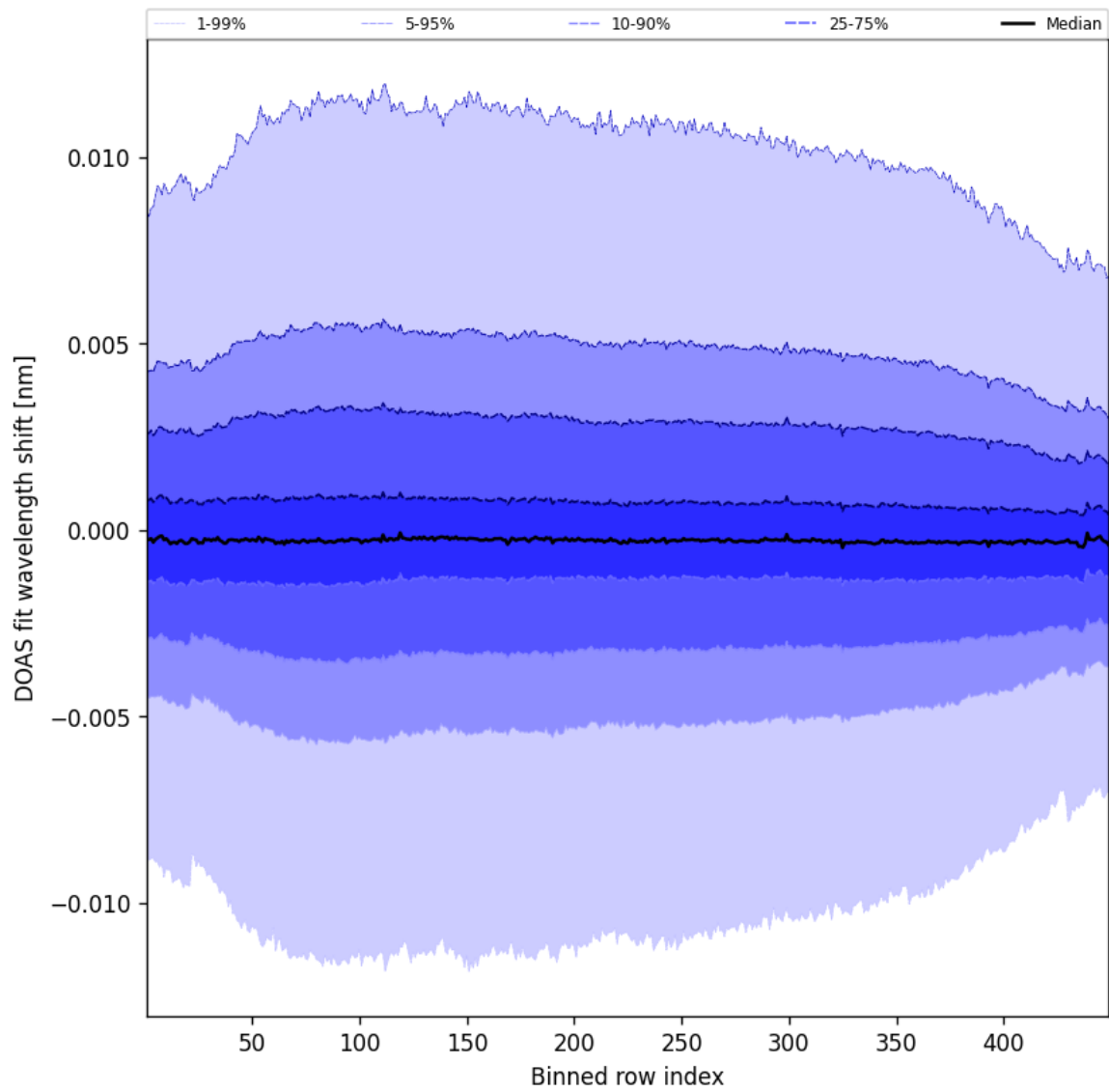
Figure 56: Along track statistics of “DOAS fit wavelength shift” for 2025-09-18 to 2025-09-18
