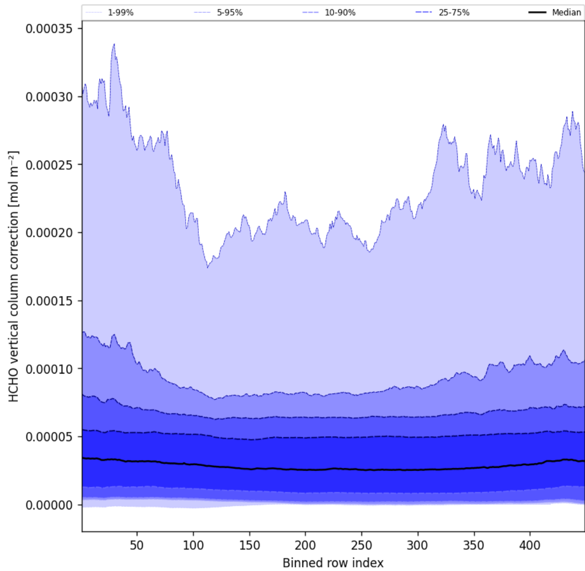
Figure 49: Along track statistics of “HCHO vertical column correction” for 2025-09-18 to 2025-09-18
