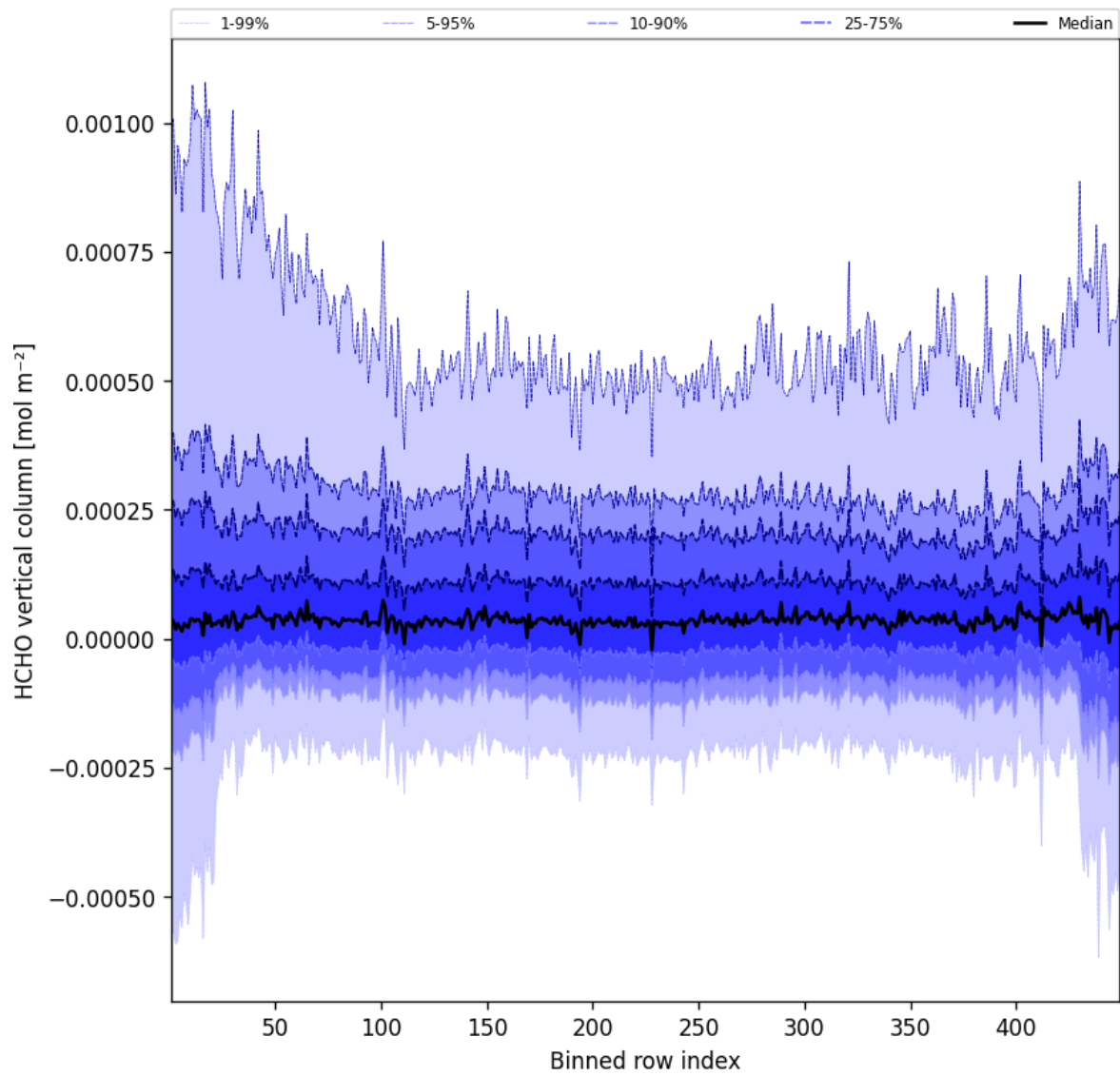
Figure 47: Along track statistics of “HCHO vertical column” for 2025-09-18 to 2025-09-18
