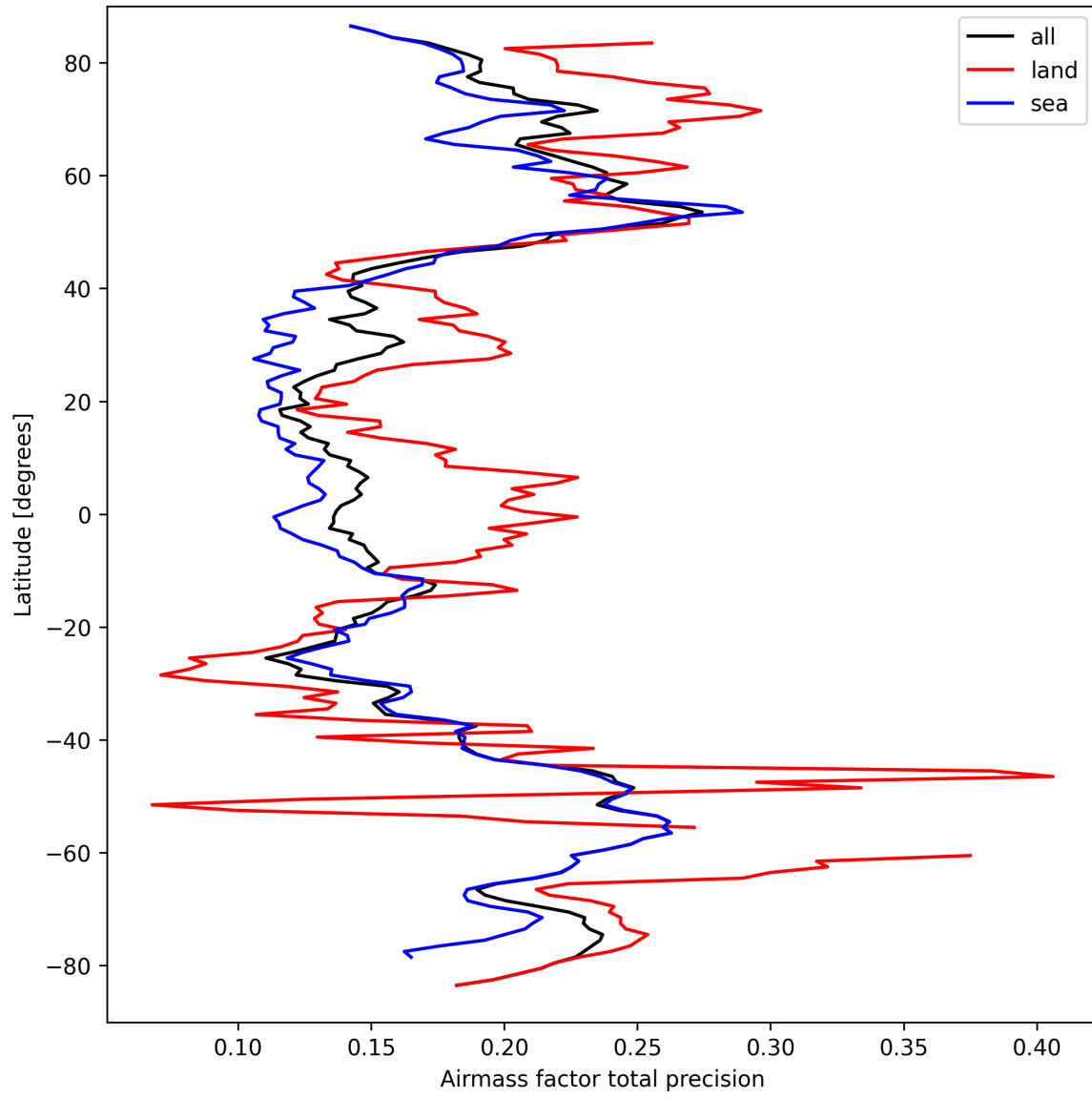
Figure 25: Zonal average of “Airmass factor total precision” for 2025-09-18 to 2025-09-18.
