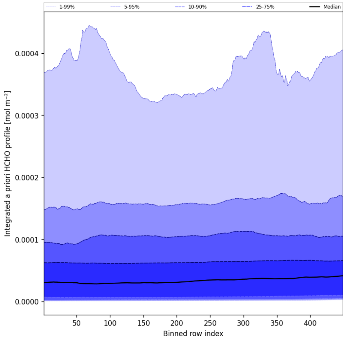
Figure 55: Along track statistics of “Integrated a priori HCHO profile” for 2025-09-18 to 2025-09-18
