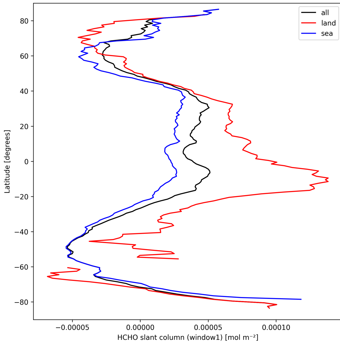
Figure 22: Zonal average of “HCHO slant column (window1)” for 2025-09-18 to 2025-09-18.
