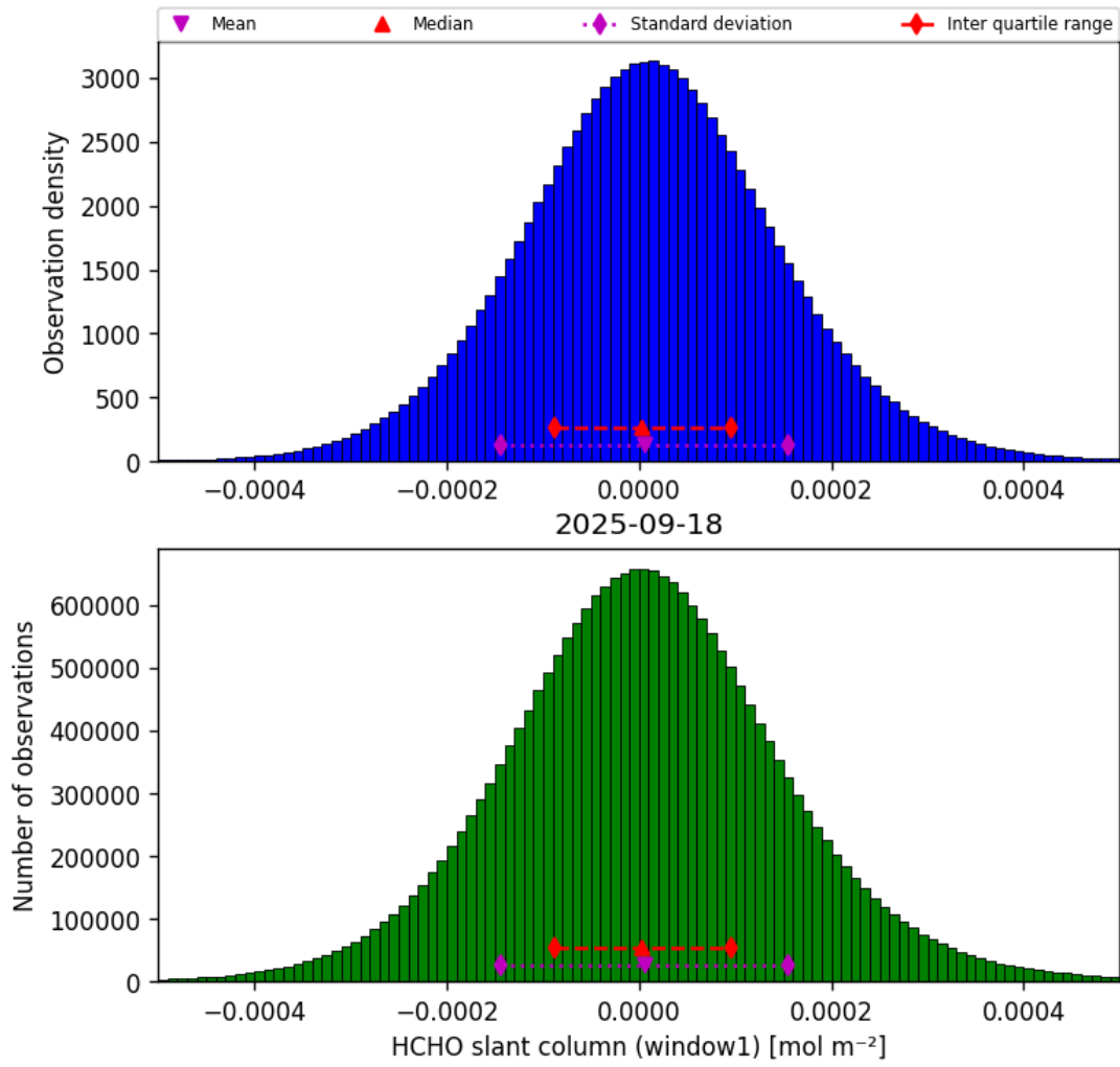
Figure 36: Histogram of “HCHO slant column (window1)” for 2025-09-18 to 2025-09-18
