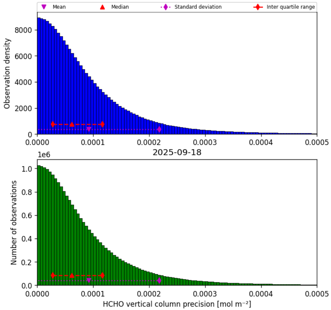
Figure 34: Histogram of “HCHO vertical column precision” for 2025-09-18 to 2025-09-18
