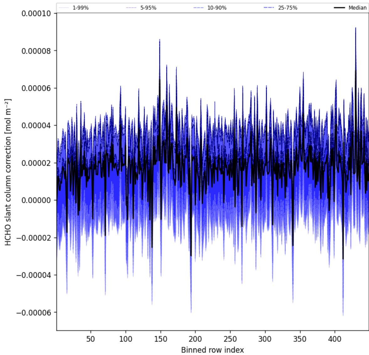
Figure 59: Along track statistics of “HCHO slant column correction” for 2025-09-18 to 2025-09-18
