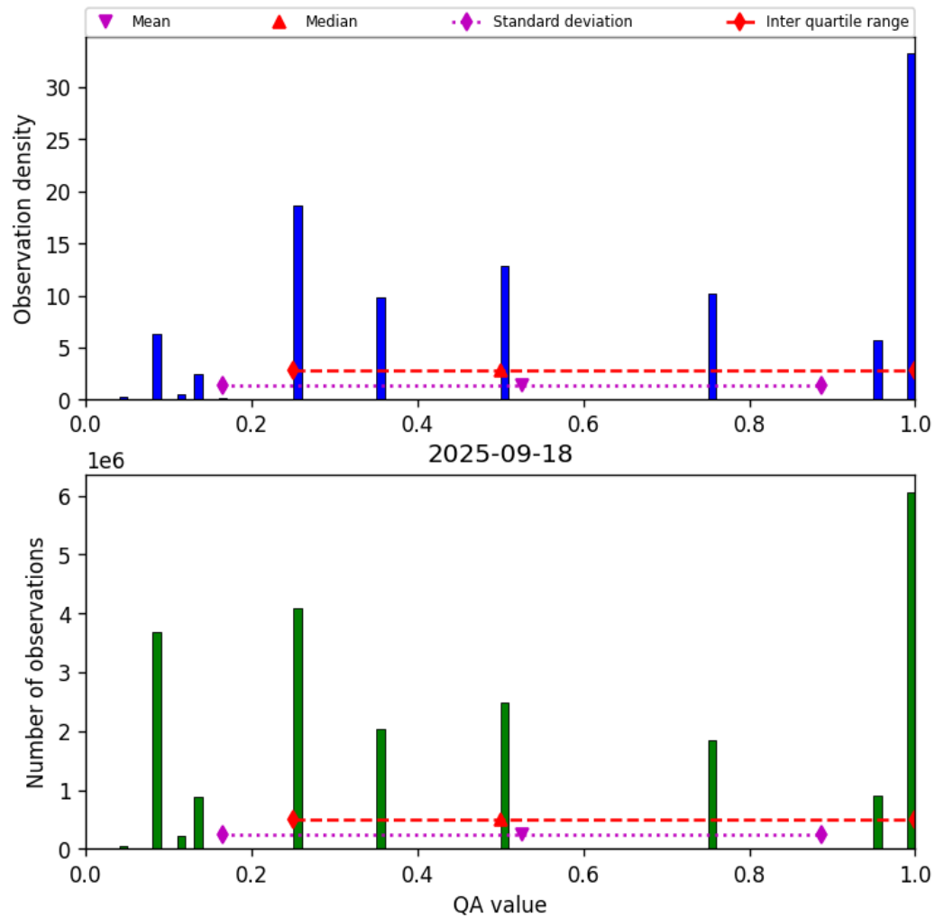
Figure 32: Histogram of “QA value” for 2025-09-18 to 2025-09-18
