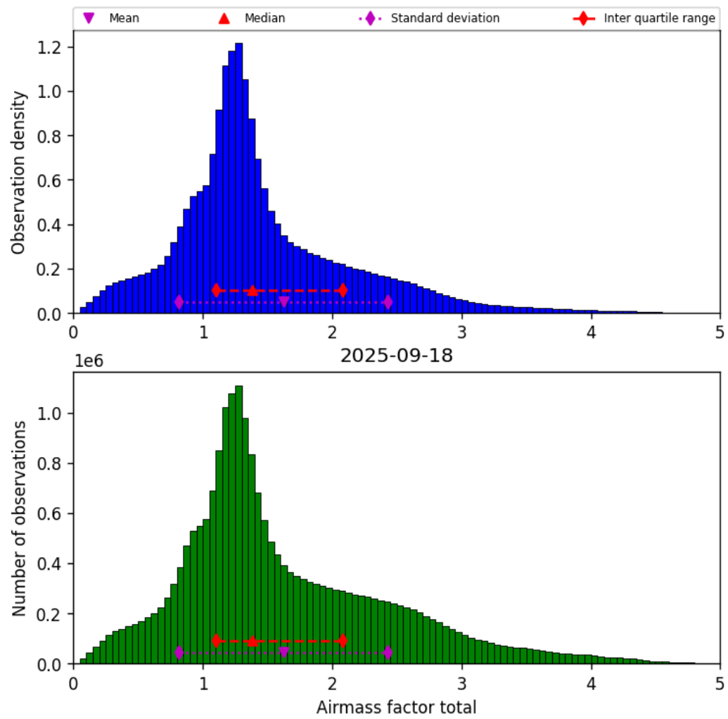
Figure 38: Histogram of “Airmass factor total” for 2025-09-18 to 2025-09-18
