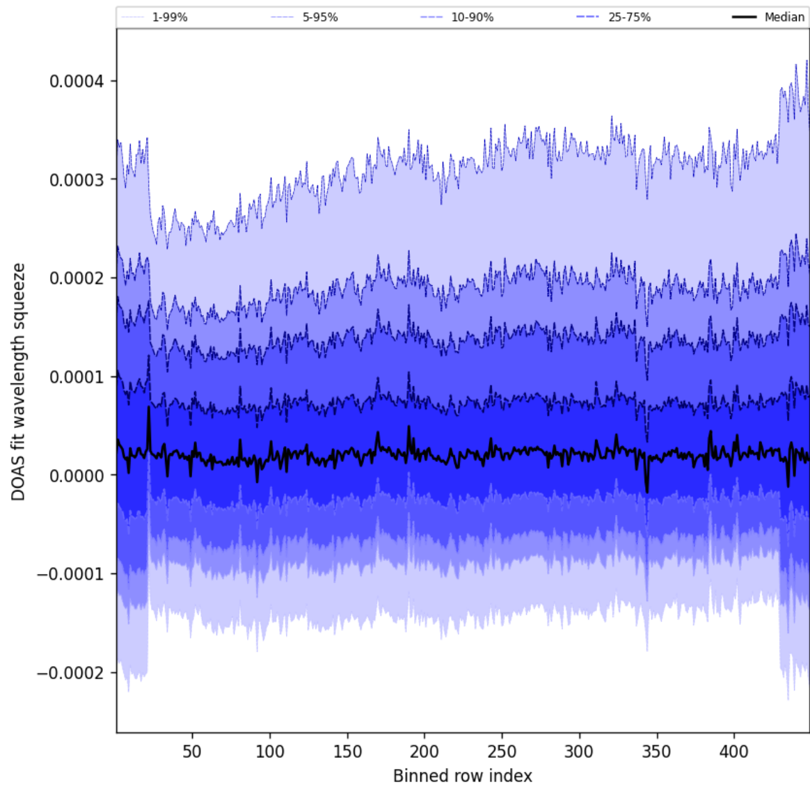
Figure 57: Along track statistics of “DOAS fit wavelength squeeze” for 2025-09-18 to 2025-09-18
