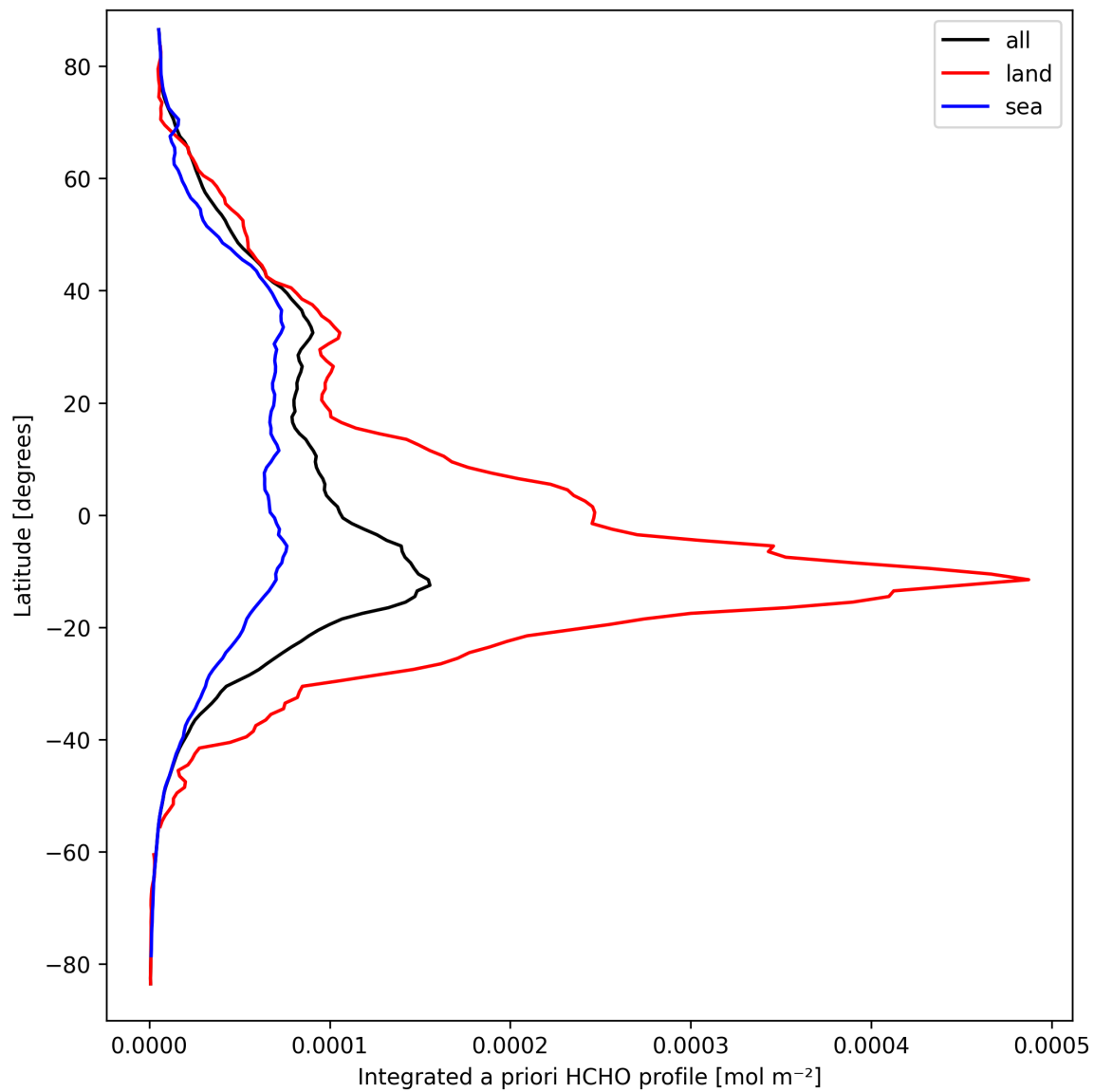
Figure 27: Zonal average of “Integrated a priori HCHO profile” for 2025-09-18 to 2025-09-18.
