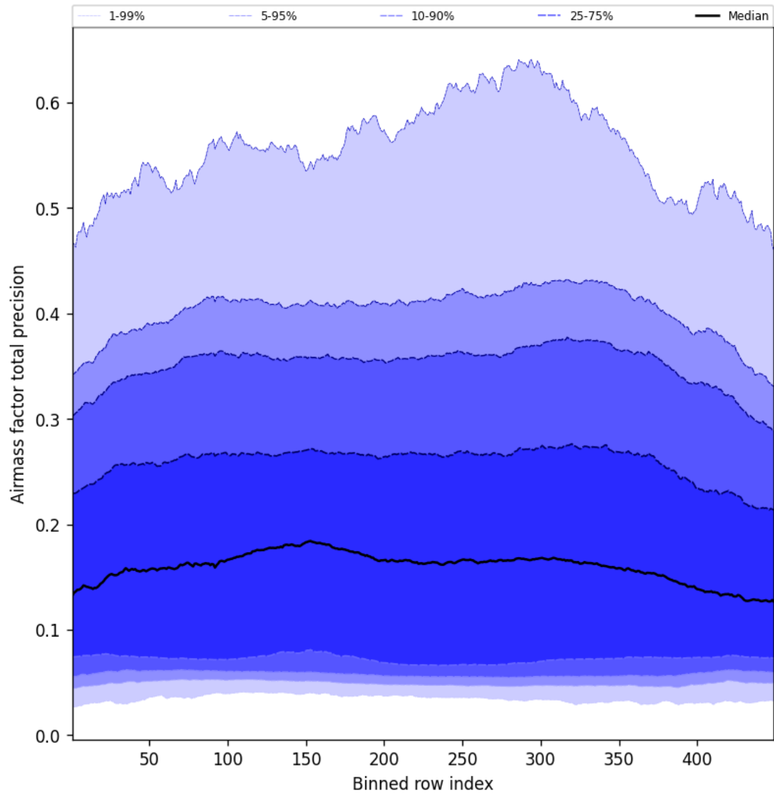
Figure 53: Along track statistics of “Airmass factor total precision” for 2025-09-18 to 2025-09-18
