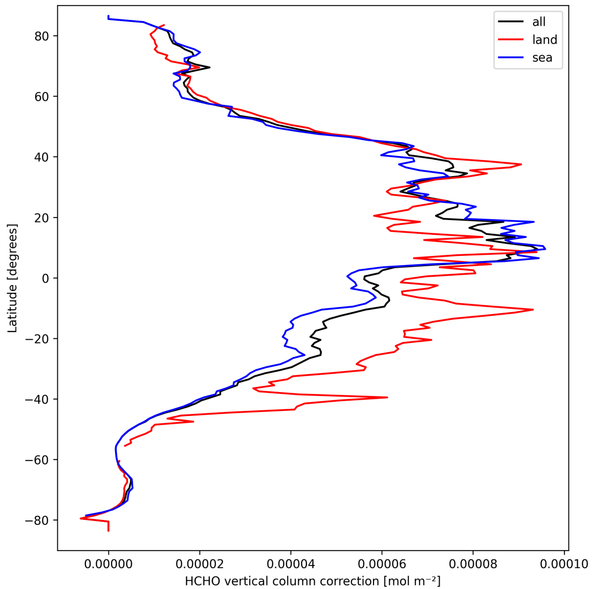
Figure 21: Zonal average of “HCHO vertical column correction” for 2025-09-18 to 2025-09-18.
