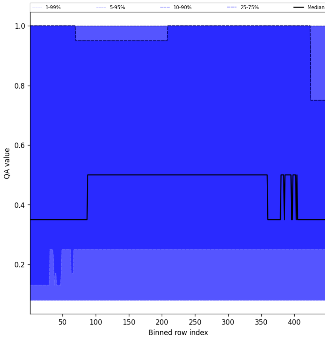
Figure 46: Along track statistics of “QA value” for 2025-09-18 to 2025-09-18
