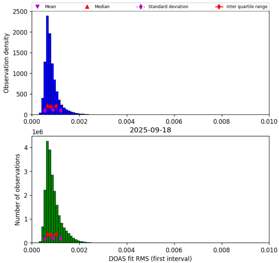
Figure 44: Histogram of “DOAS fit RMS (first interval)” for 2025-09-18 to 2025-09-18
