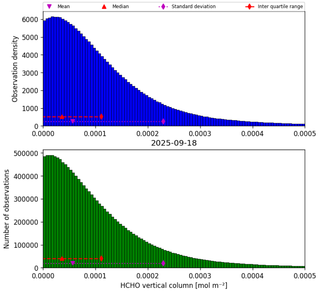
Figure 33: Histogram of “HCHO vertical column” for 2025-09-18 to 2025-09-18
