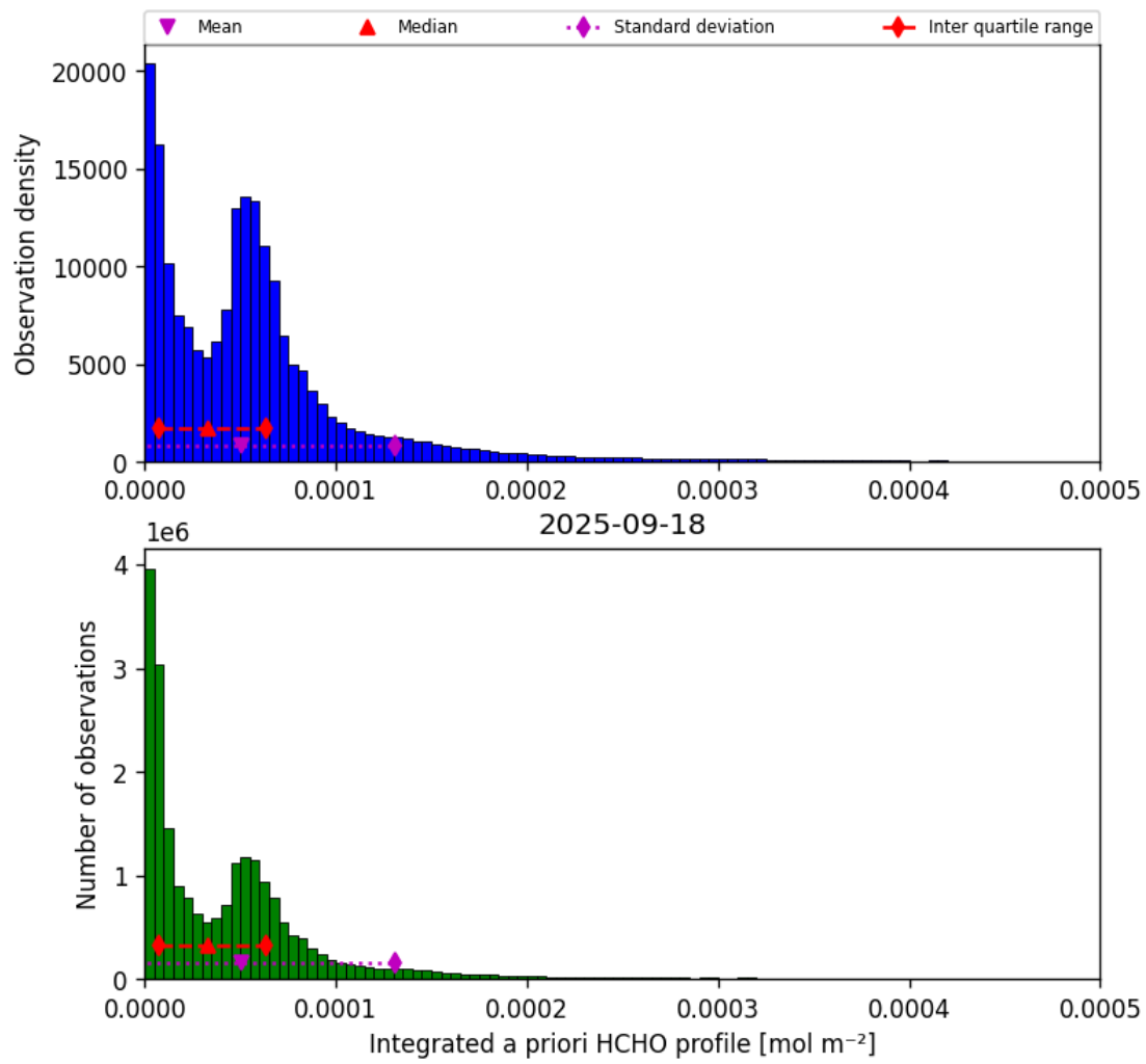
Figure 41: Histogram of “Integrated a priori HCHO profile” for 2025-09-18 to 2025-09-18
