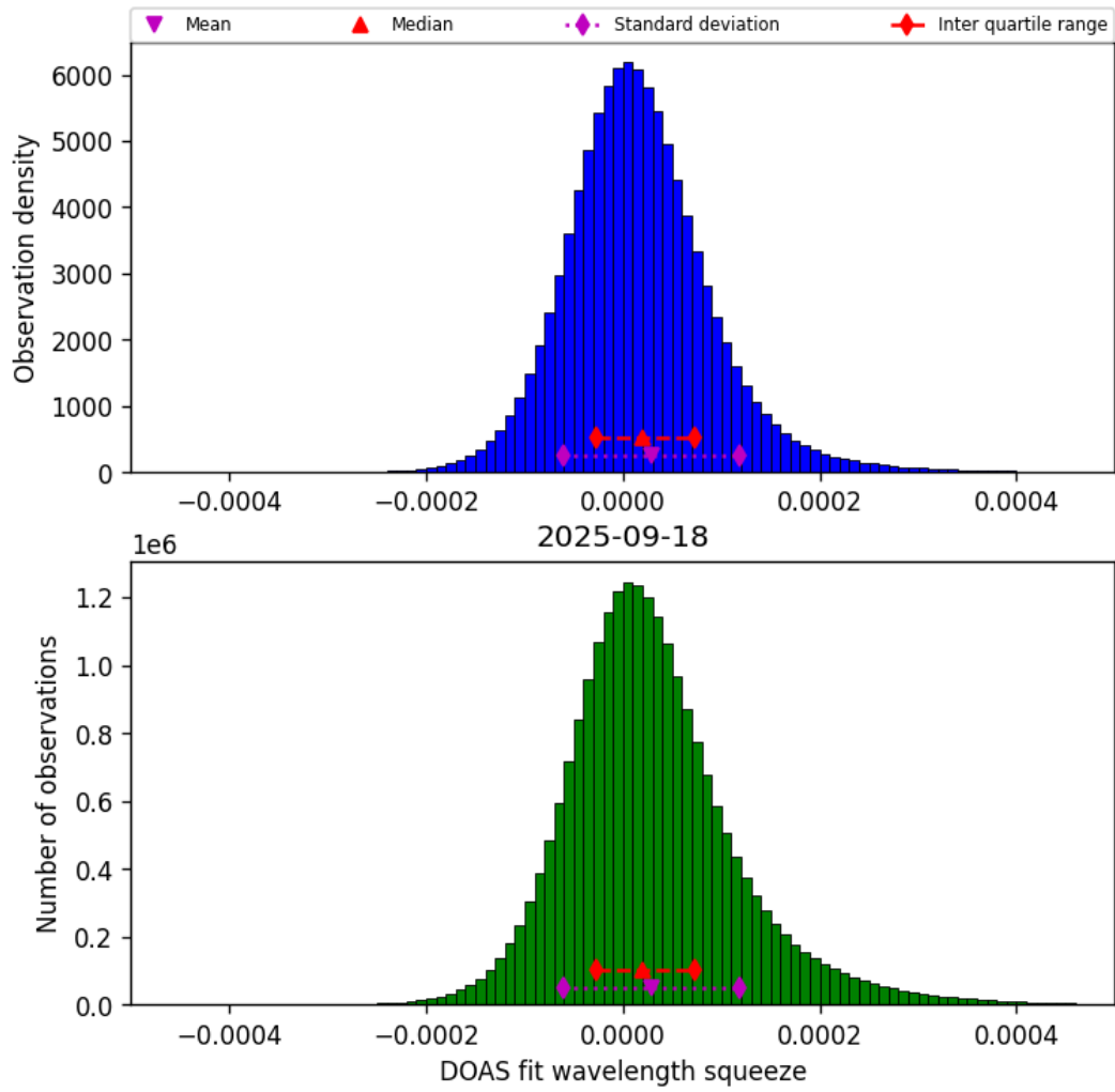
Figure 43: Histogram of “DOAS fit wavelength squeeze” for 2025-09-18 to 2025-09-18
