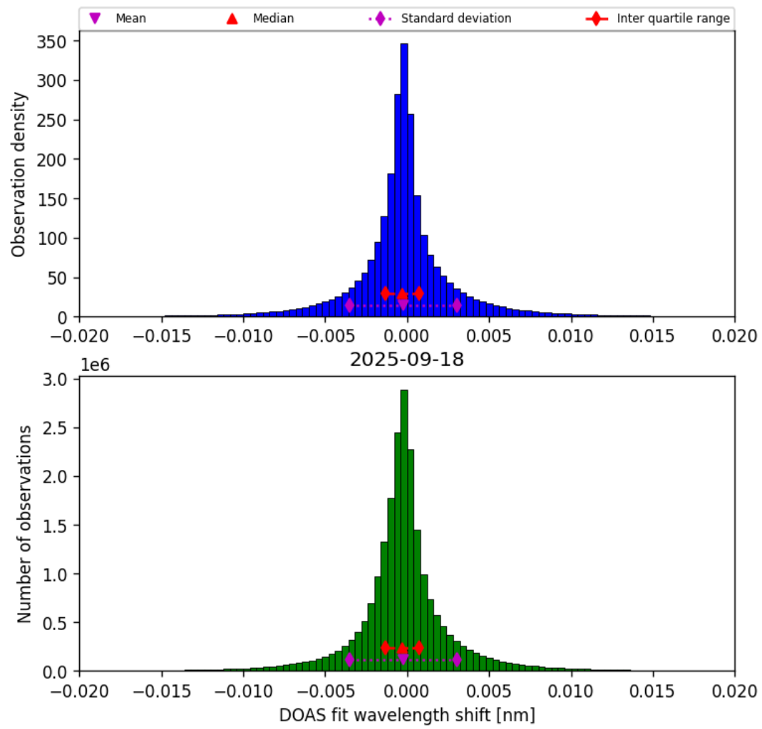
Figure 42: Histogram of “DOAS fit wavelength shift” for 2025-09-18 to 2025-09-18
