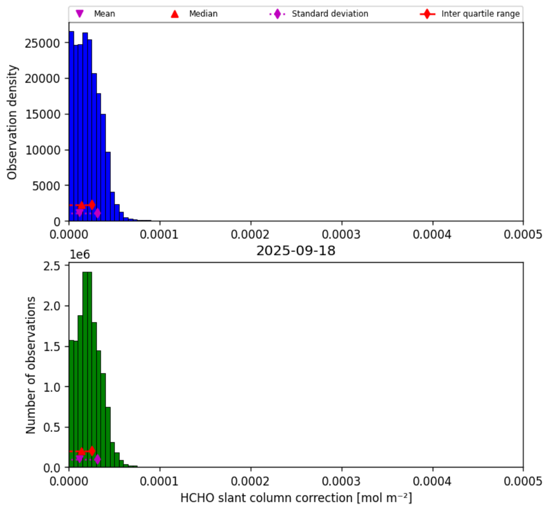
Figure 45: Histogram of “HCHO slant column correction” for 2025-09-18 to 2025-09-18
