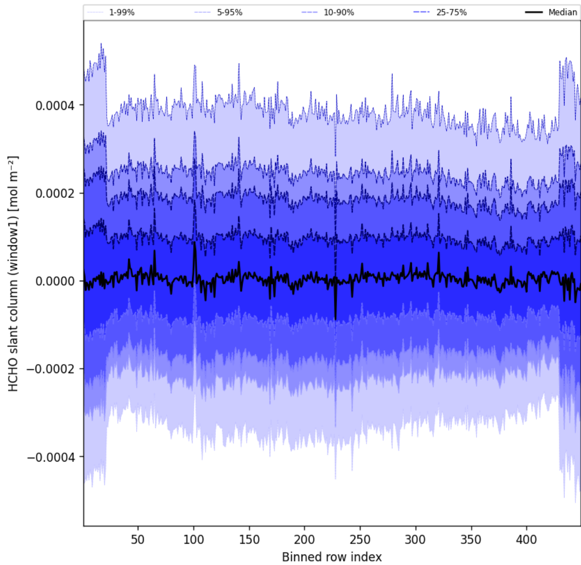
Figure 50: Along track statistics of “HCHO slant column (window1)” for 2025-09-18 to 2025-09-18
