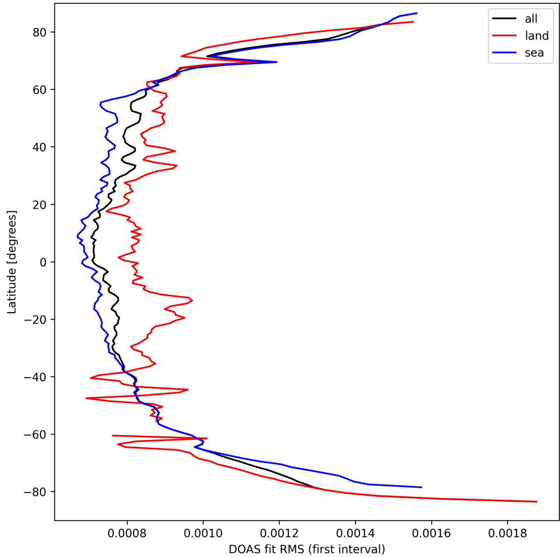
Figure 30: Zonal average of “DOAS fit RMS (first interval)” for 2025-09-18 to 2025-09-18.
