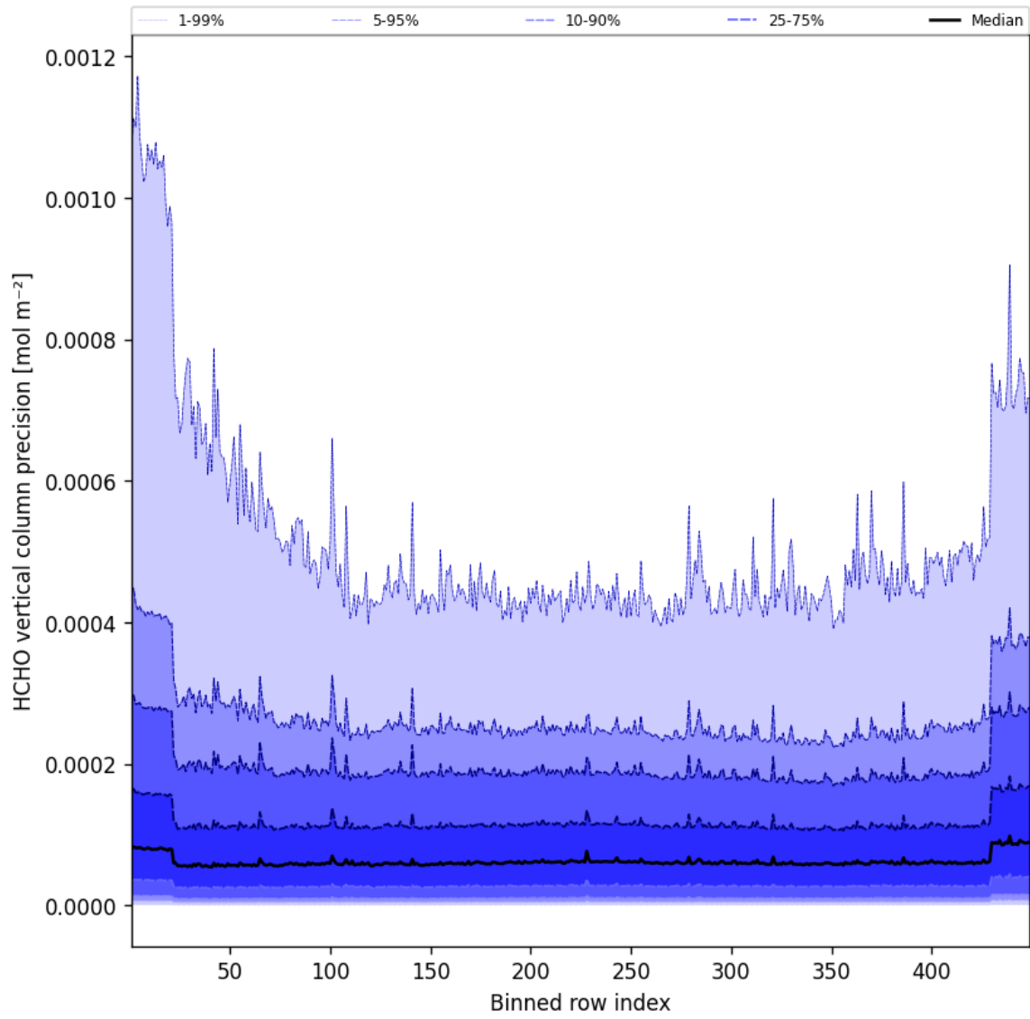
Figure 48: Along track statistics of “HCHO vertical column precision” for 2025-09-18 to 2025-09-18
