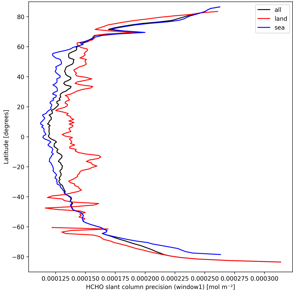
Figure 23: Zonal average of “HCHO slant column precision (window1)” for 2025-09-18 to 2025-09-18.
