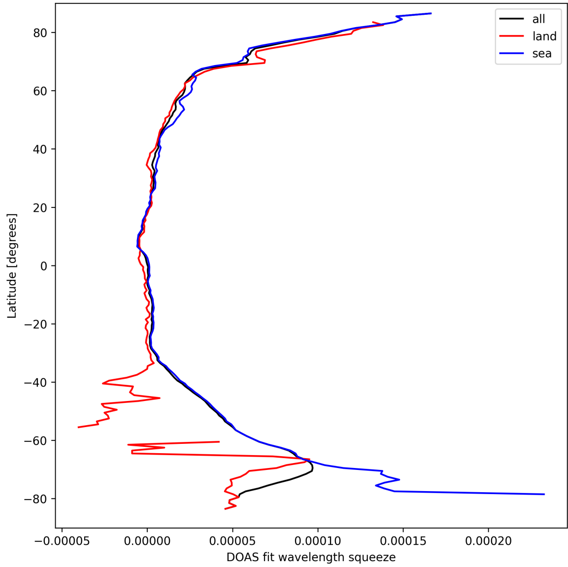
Figure 29: Zonal average of “DOAS fit wavelength squeeze” for 2025-09-18 to 2025-09-18.
