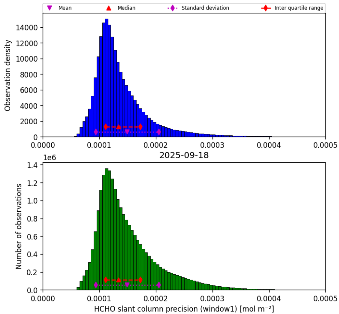
Figure 37: Histogram of “HCHO slant column precision (window1)” for 2025-09-18 to 2025-09-18
