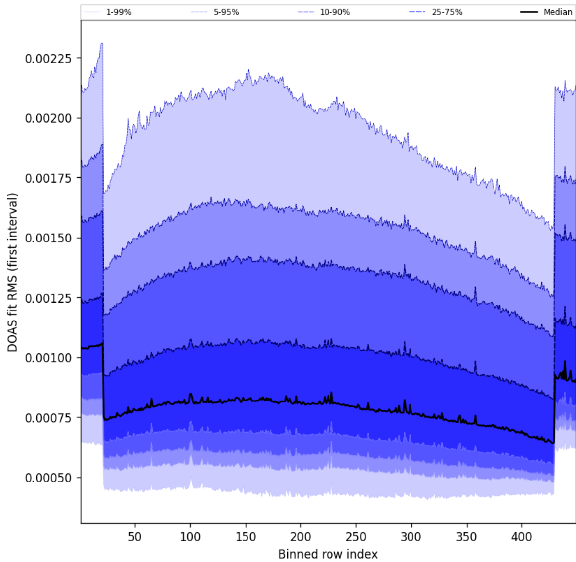
Figure 58: Along track statistics of “DOAS fit RMS (first interval)” for 2025-09-18 to 2025-09-18
