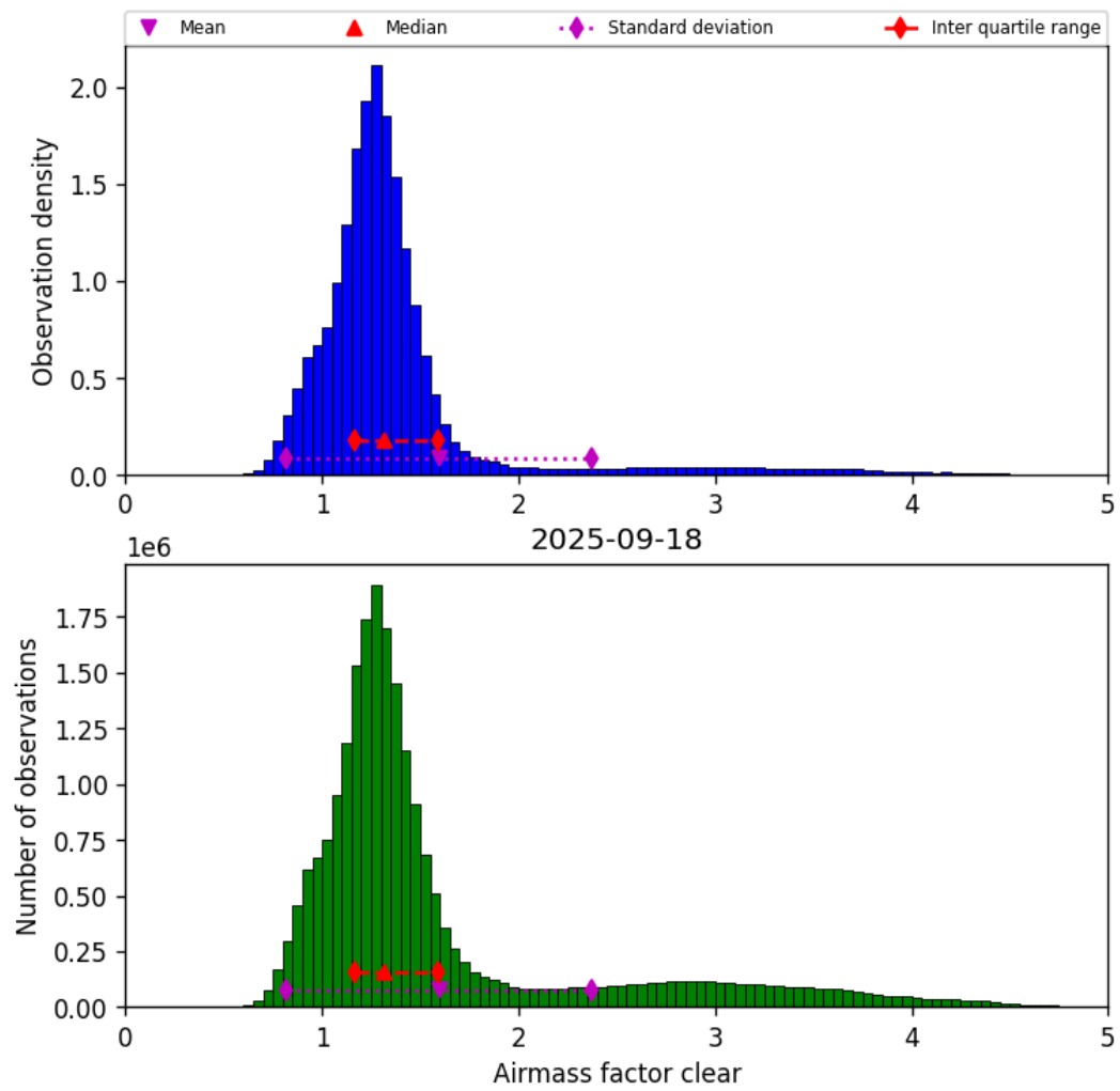
Figure 40: Histogram of “Airmass factor clear” for 2025-09-18 to 2025-09-18
