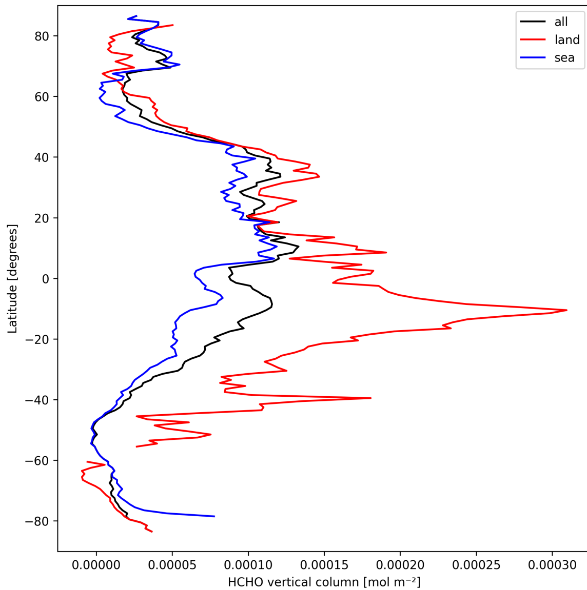
Figure 19: Zonal average of “HCHO vertical column” for 2025-09-18 to 2025-09-18.
