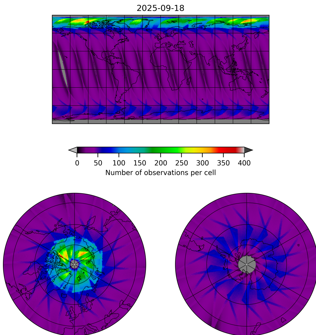
Figure 17: Map of the number of observations for 2025-09-18 to 2025-09-18
