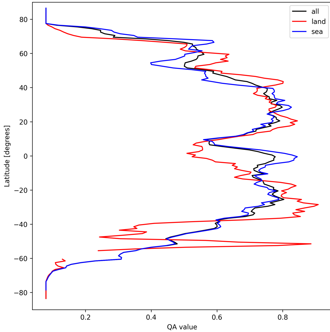
Figure 18: Zonal average of “QA value” for 2025-09-18 to 2025-09-18.
