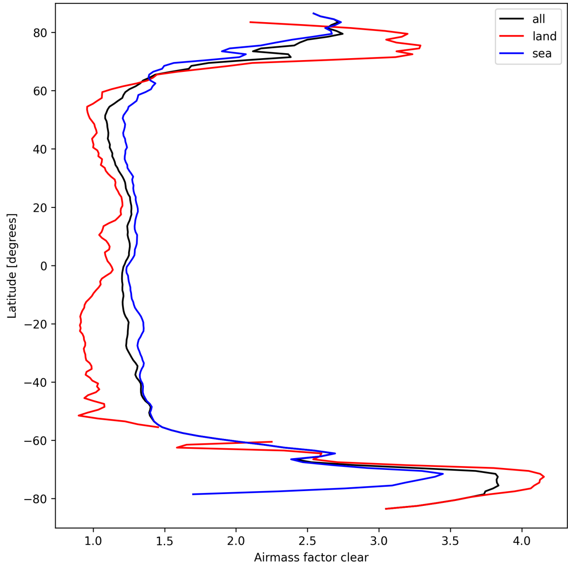
Figure 26: Zonal average of “Airmass factor clear” for 2025-09-18 to 2025-09-18.
