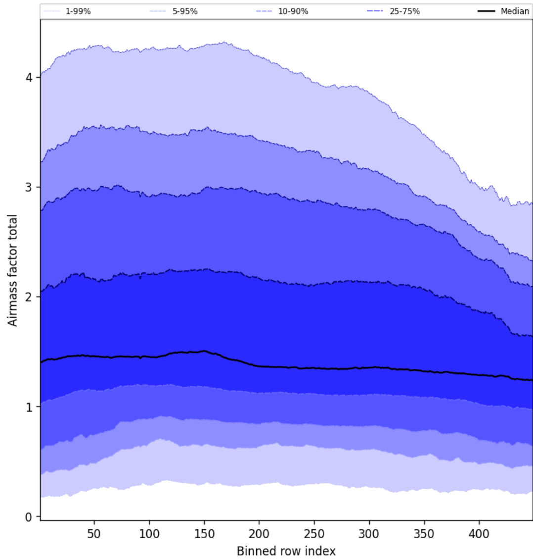
Figure 52: Along track statistics of “Airmass factor total” for 2025-09-18 to 2025-09-18
