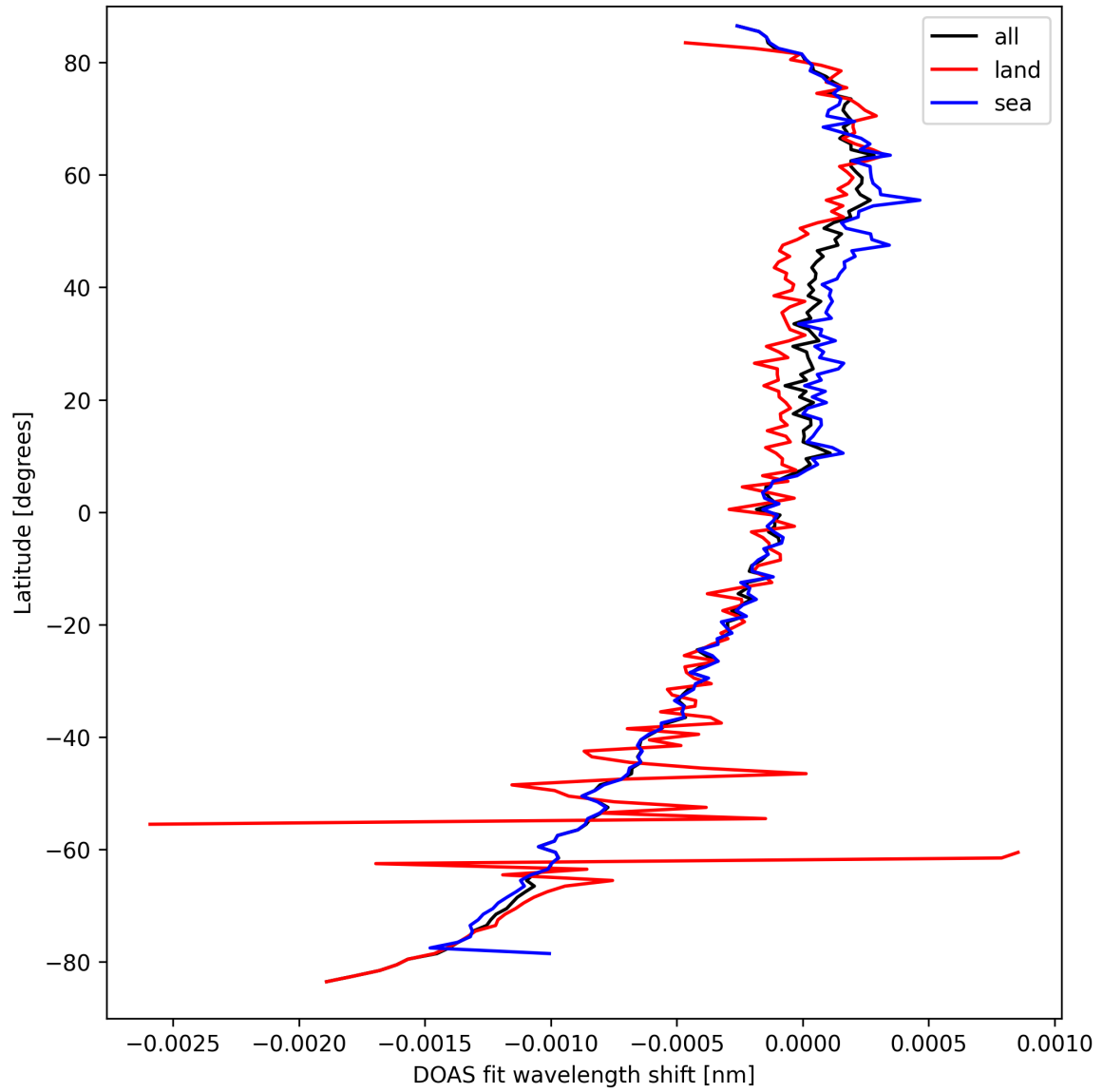
Figure 28: Zonal average of “DOAS fit wavelength shift” for 2025-09-18 to 2025-09-18.
