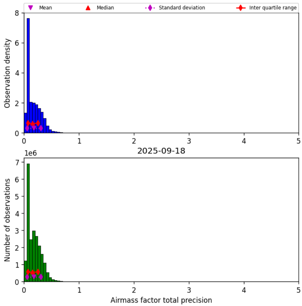
Figure 39: Histogram of “Airmass factor total precision” for 2025-09-18 to 2025-09-18
