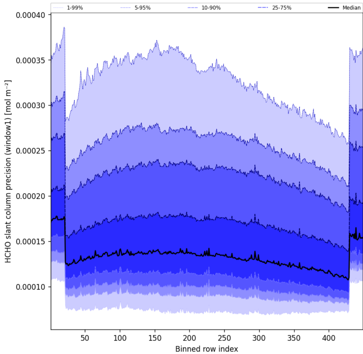
Figure 51: Along track statistics of “HCHO slant column precision (window1)” for 2025-09-18 to 2025-09-18
