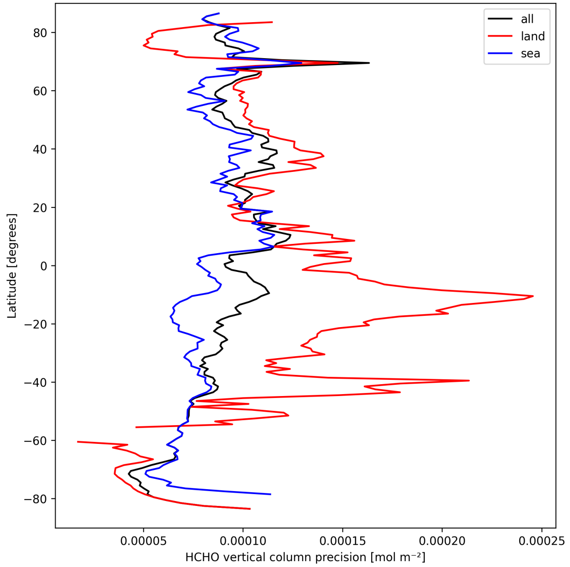
Figure 20: Zonal average of “HCHO vertical column precision” for 2025-09-18 to 2025-09-18.
