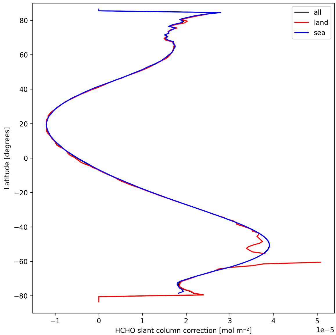
Figure 31: Zonal average of “HCHO slant column correction” for 2025-09-19 to 2025-09-20.
