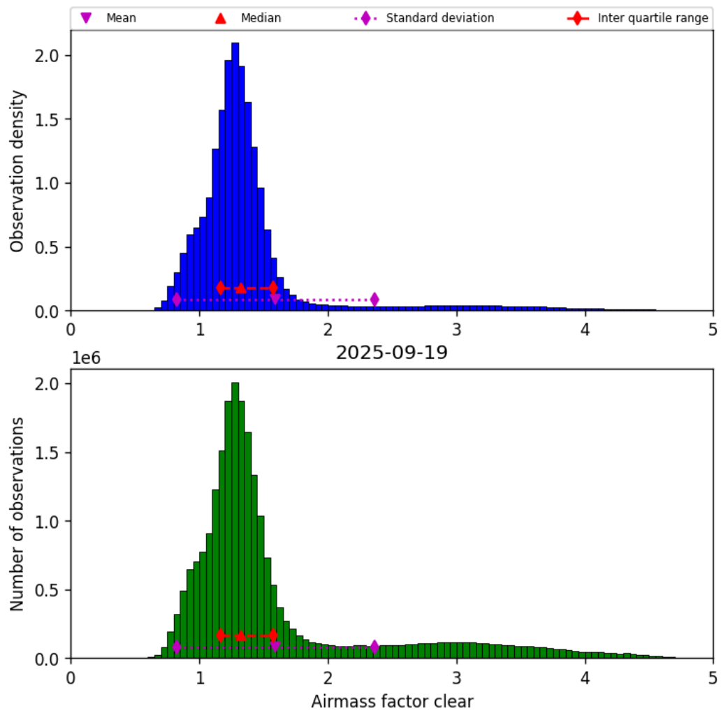
Figure 40: Histogram of “Airmass factor clear” for 2025-09-19 to 2025-09-20
