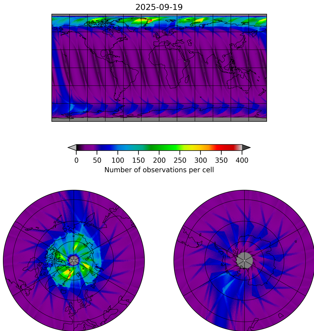
Figure 17: Map of the number of observations for 2025-09-19 to 2025-09-20
