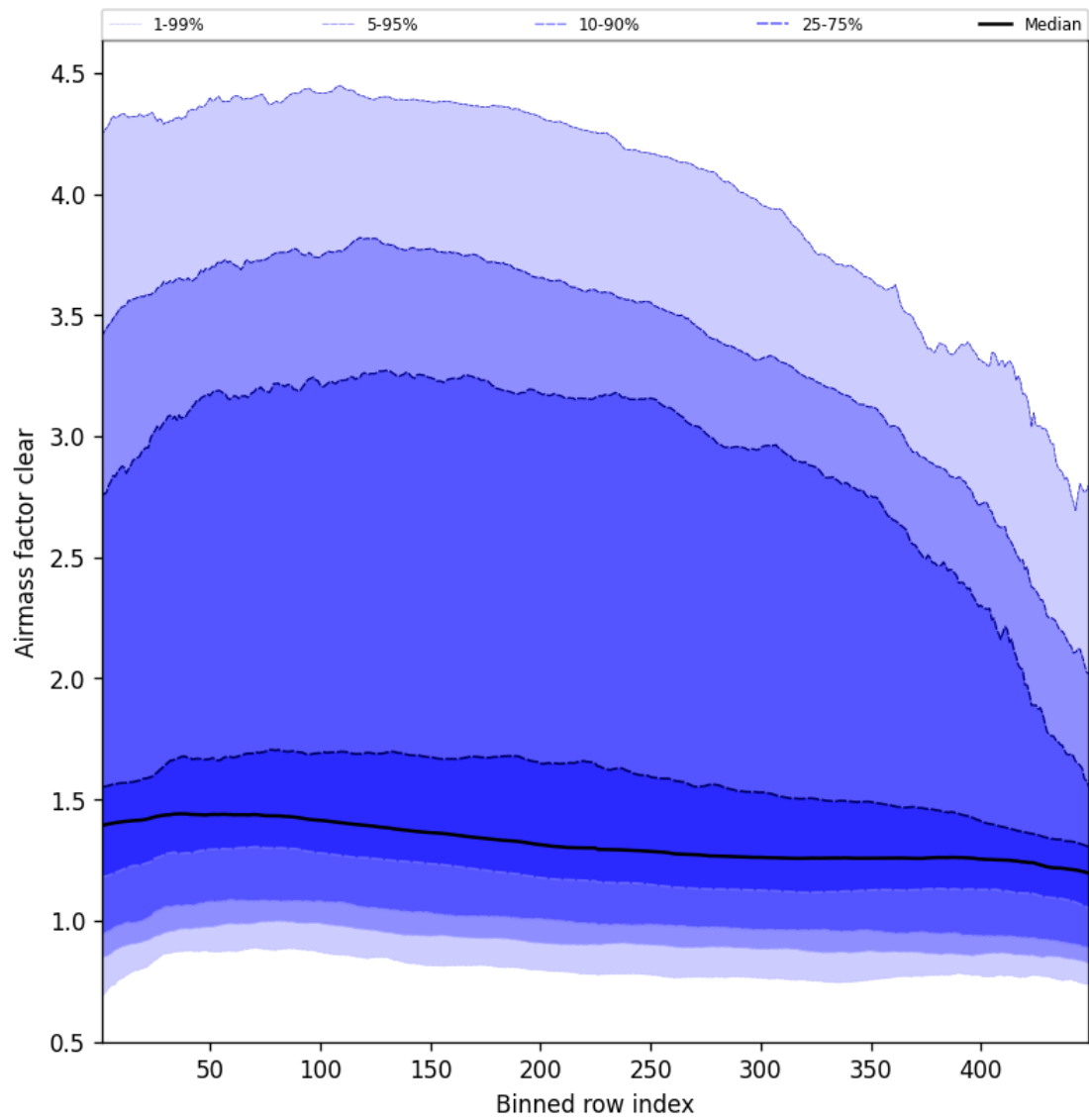
Figure 54: Along track statistics of “Airmass factor clear” for 2025-09-19 to 2025-09-20
