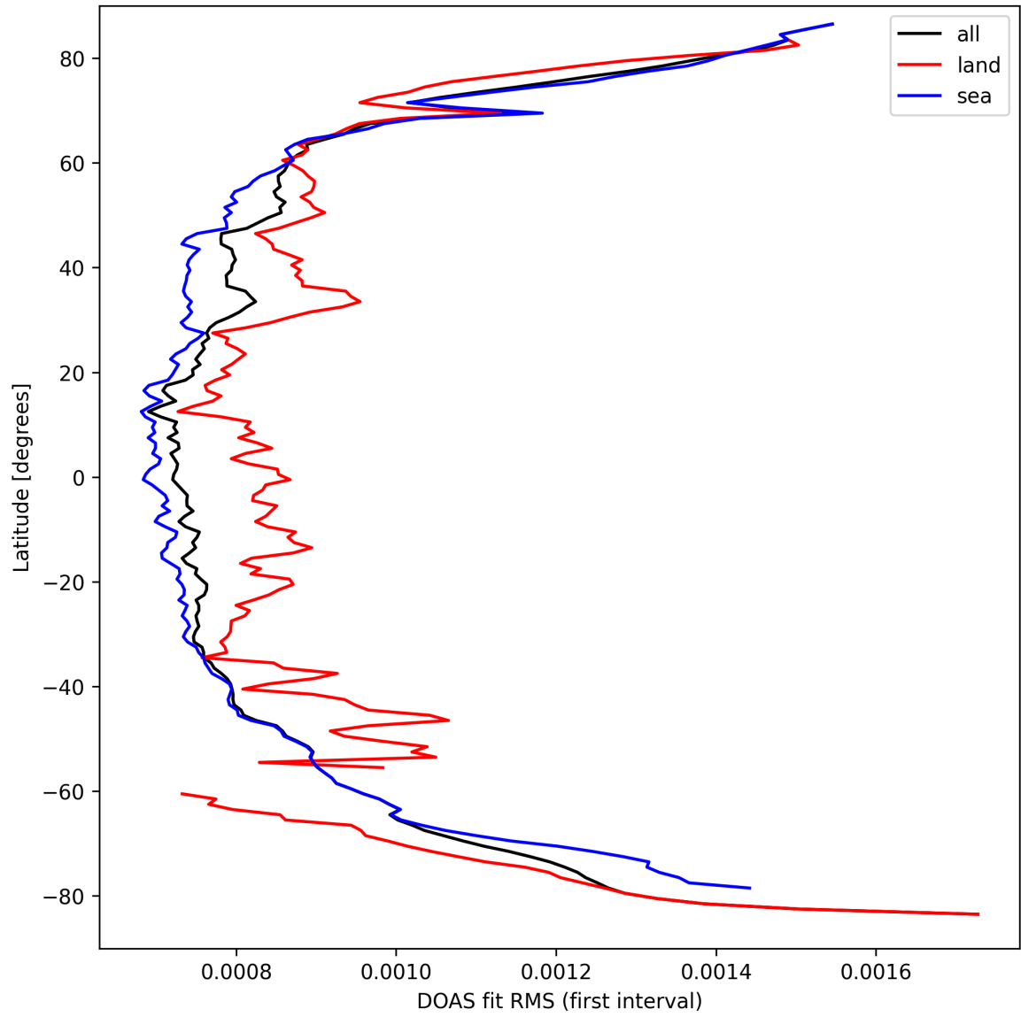
Figure 30: Zonal average of "DOAS fit RMS (first interval)" for 2025-09-19 to 2025-09-20.
