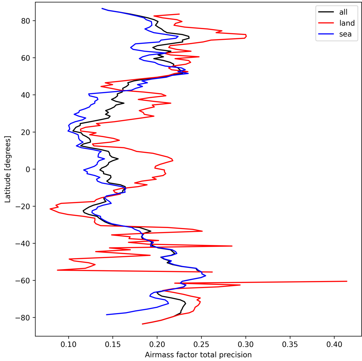
Figure 25: Zonal average of “Airmass factor total precision” for 2025-09-19 to 2025-09-20.
