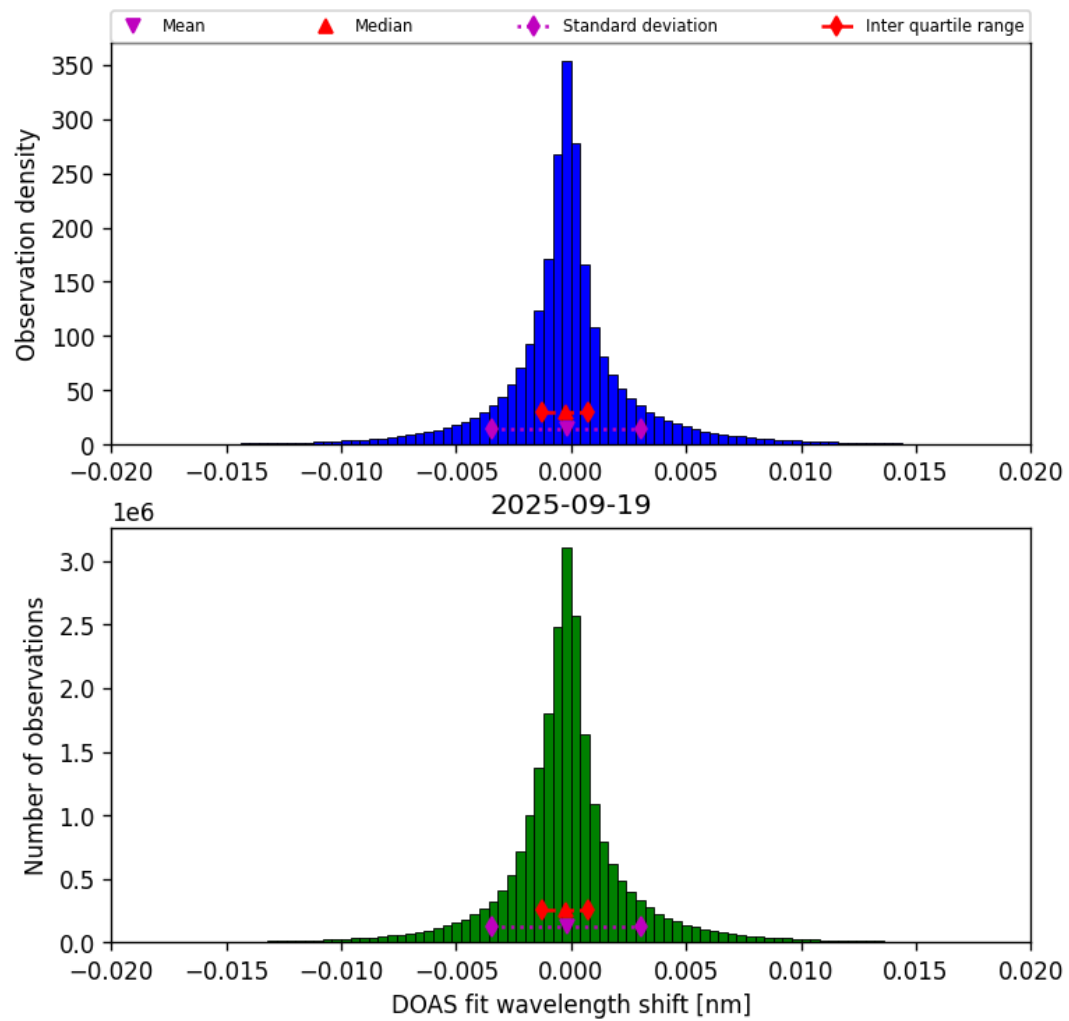
Figure 42: Histogram of “DOAS fit wavelength shift” for 2025-09-19 to 2025-09-20
