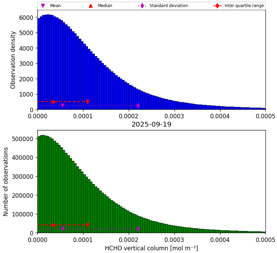
Figure 33: Histogram of “HCHO vertical column” for 2025-09-19 to 2025-09-20
