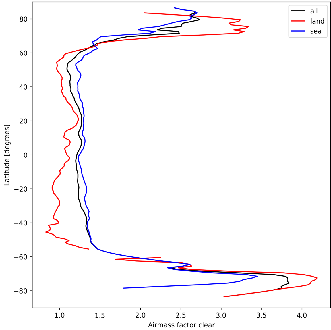
Figure 26: Zonal average of “Airmass factor clear” for 2025-09-19 to 2025-09-20.
