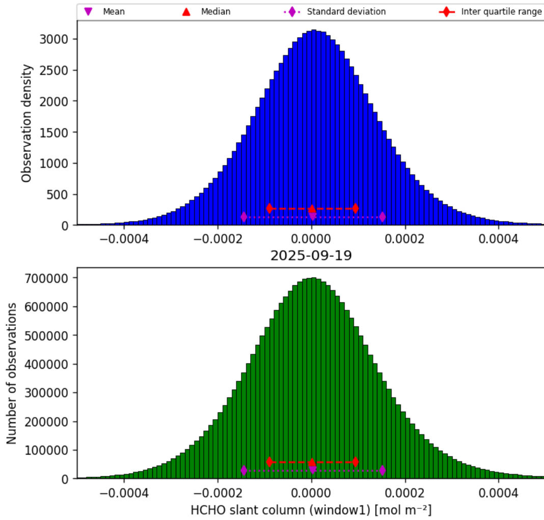
Figure 36: Histogram of “HCHO slant column (window1)” for 2025-09-19 to 2025-09-20
