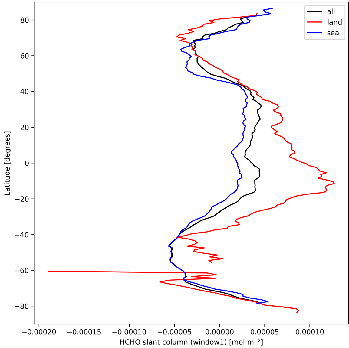
Figure 22: Zonal average of “HCHO slant column (window1)” for 2025-09-19 to 2025-09-20.
