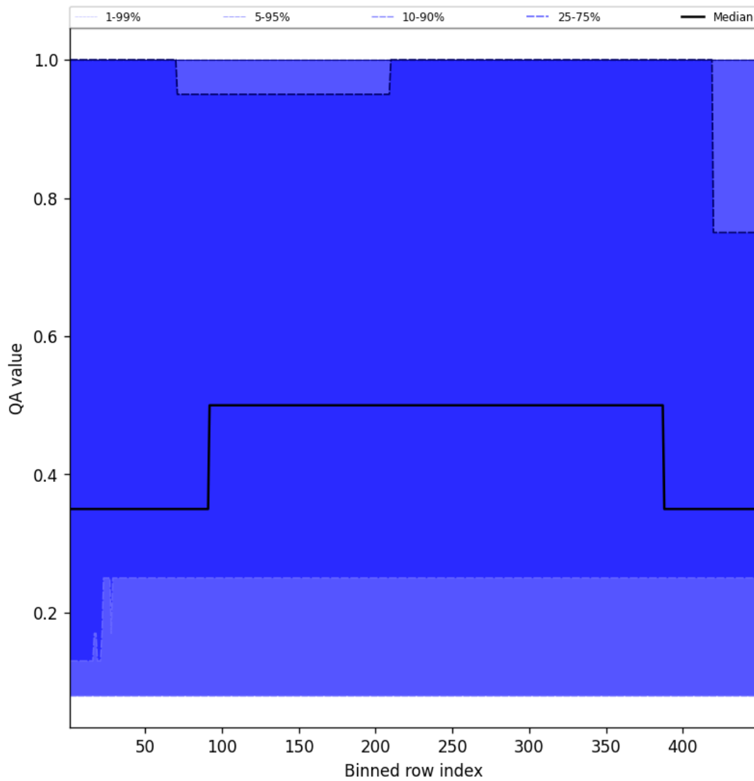
Figure 46: Along track statistics of “QA value” for 2025-09-19 to 2025-09-20
