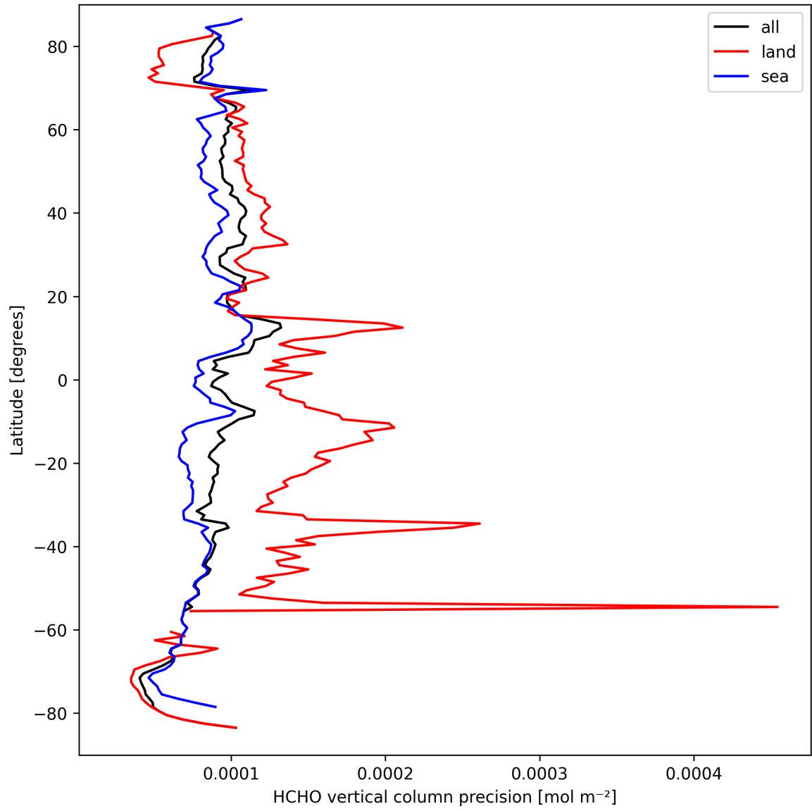
Figure 20: Zonal average of “HCHO vertical column precision” for 2025-09-19 to 2025-09-20.
