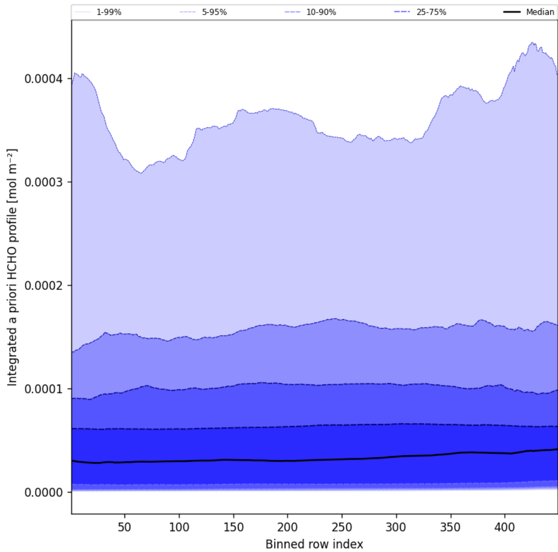
Figure 55: Along track statistics of "Integrated a priori HCHO profile" for 2025-09-19 to 2025-09-20
