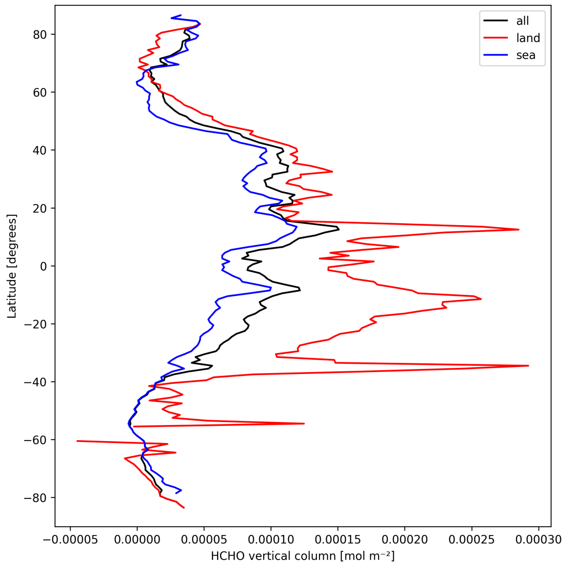
Figure 19: Zonal average of “HCHO vertical column” for 2025-09-19 to 2025-09-20.
