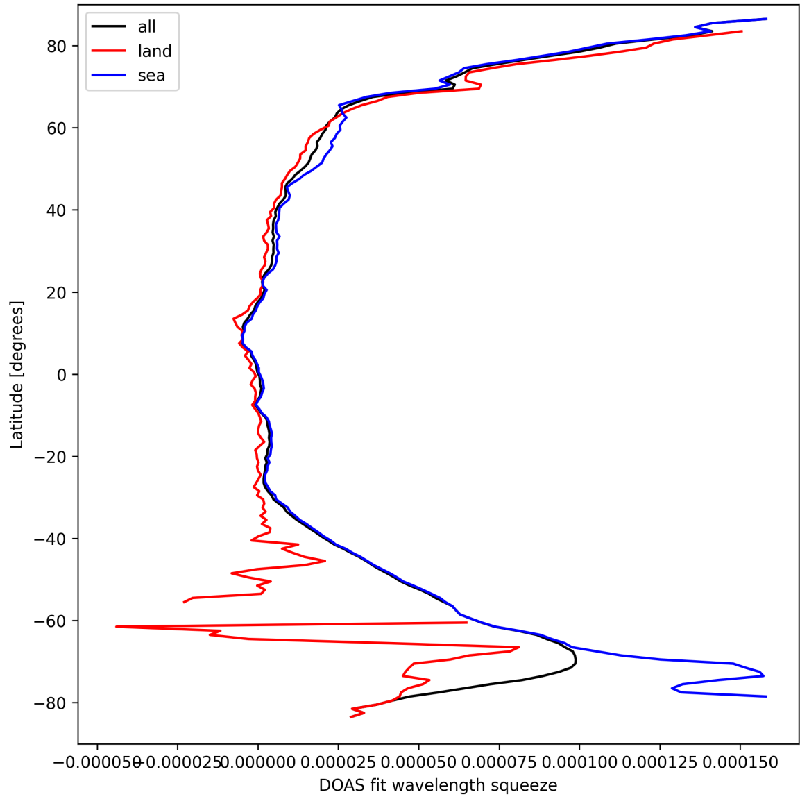
Figure 29: Zonal average of “DOAS fit wavelength squeeze” for 2025-09-19 to 2025-09-20.
