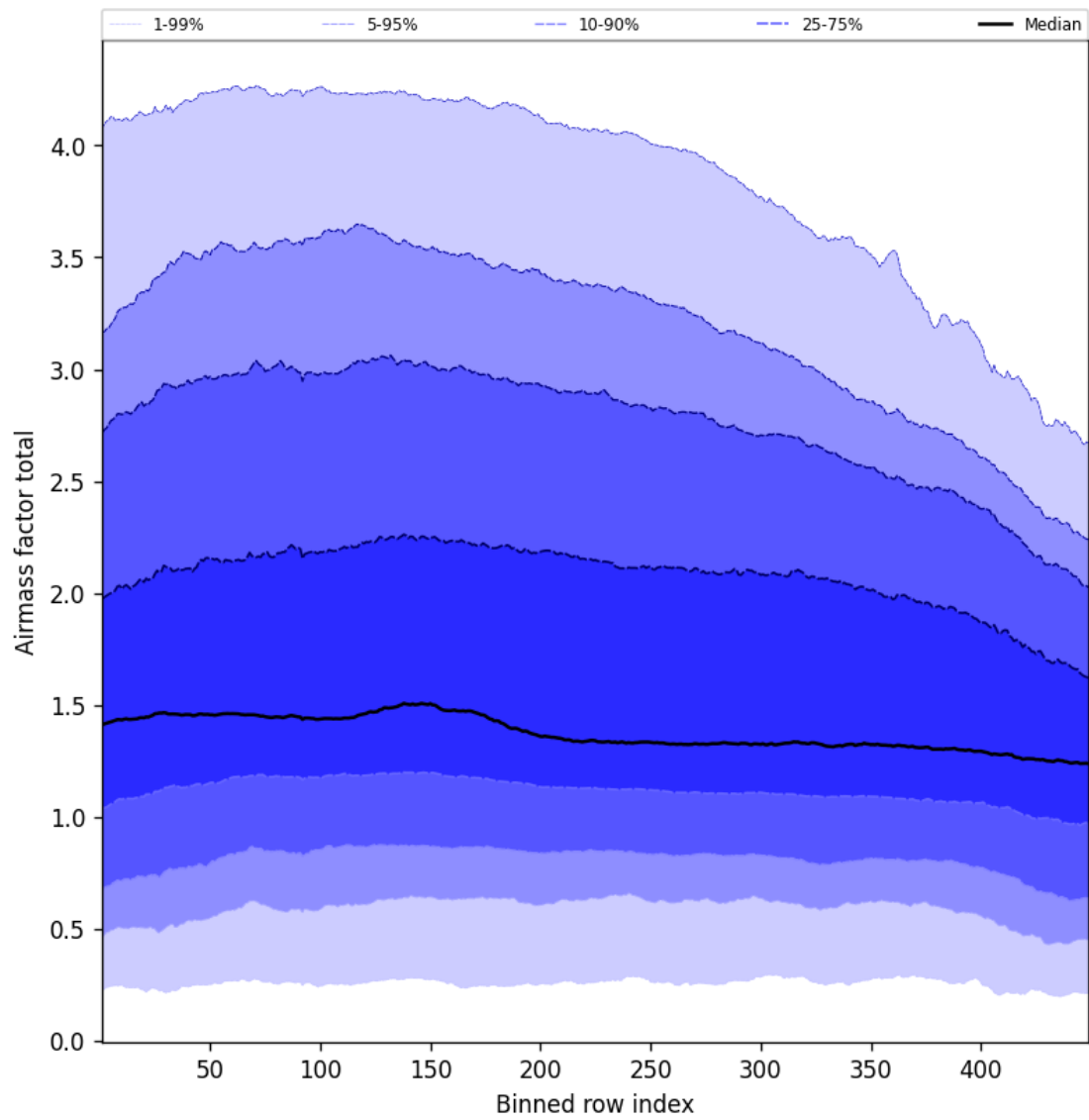
Figure 52: Along track statistics of “Airmass factor total” for 2025-09-19 to 2025-09-20
