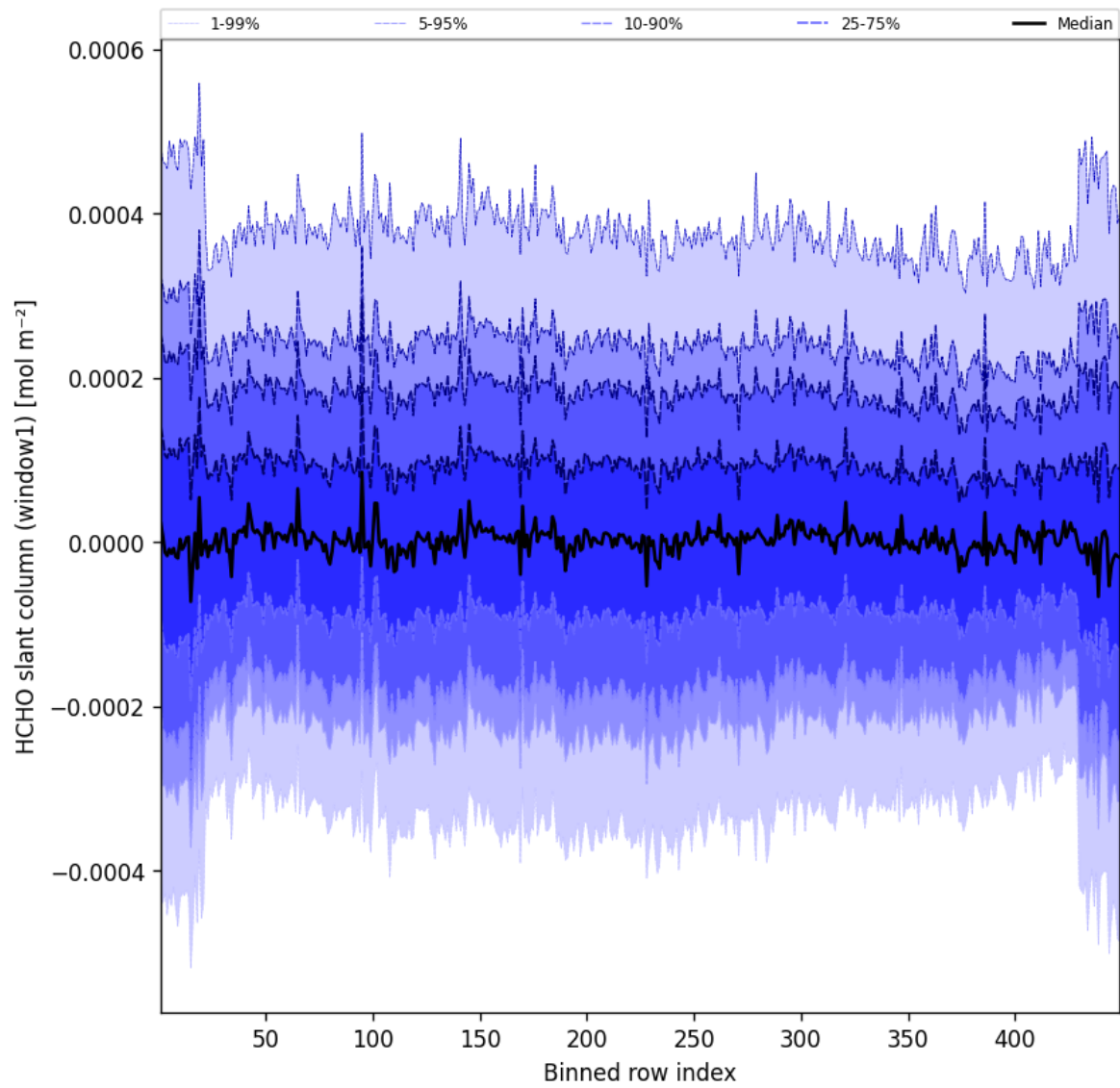
Figure 50: Along track statistics of “HCHO slant column (window1)” for 2025-09-19 to 2025-09-20
