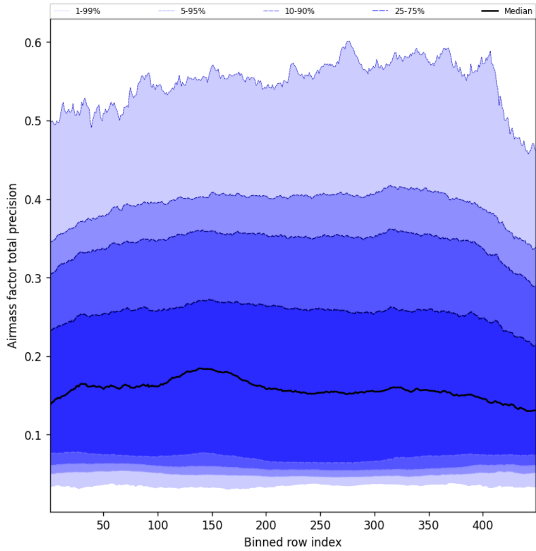
Figure 53: Along track statistics of “Airmass factor total precision” for 2025-09-19 to 2025-09-20
