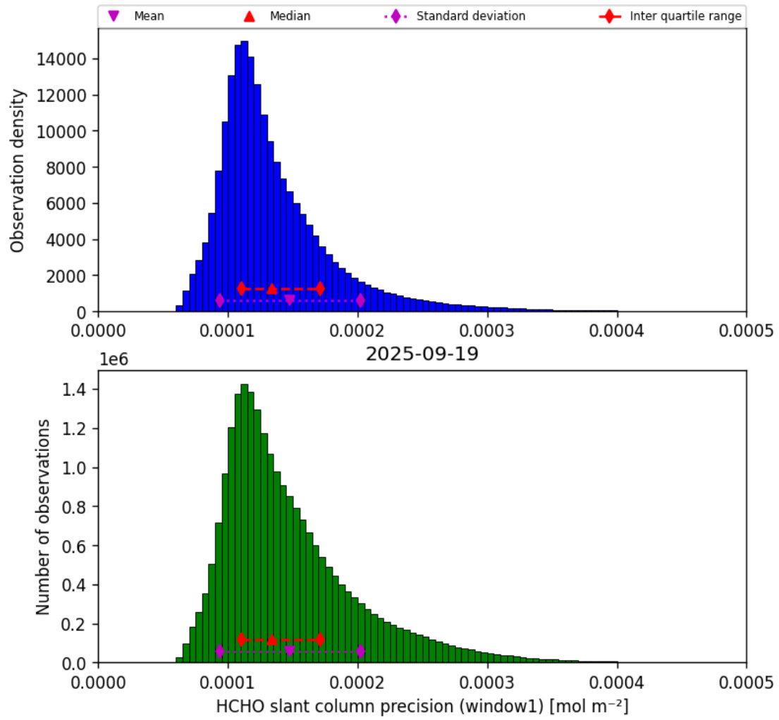
Figure 37: Histogram of “HCHO slant column precision (window1)” for 2025-09-19 to 2025-09-20
