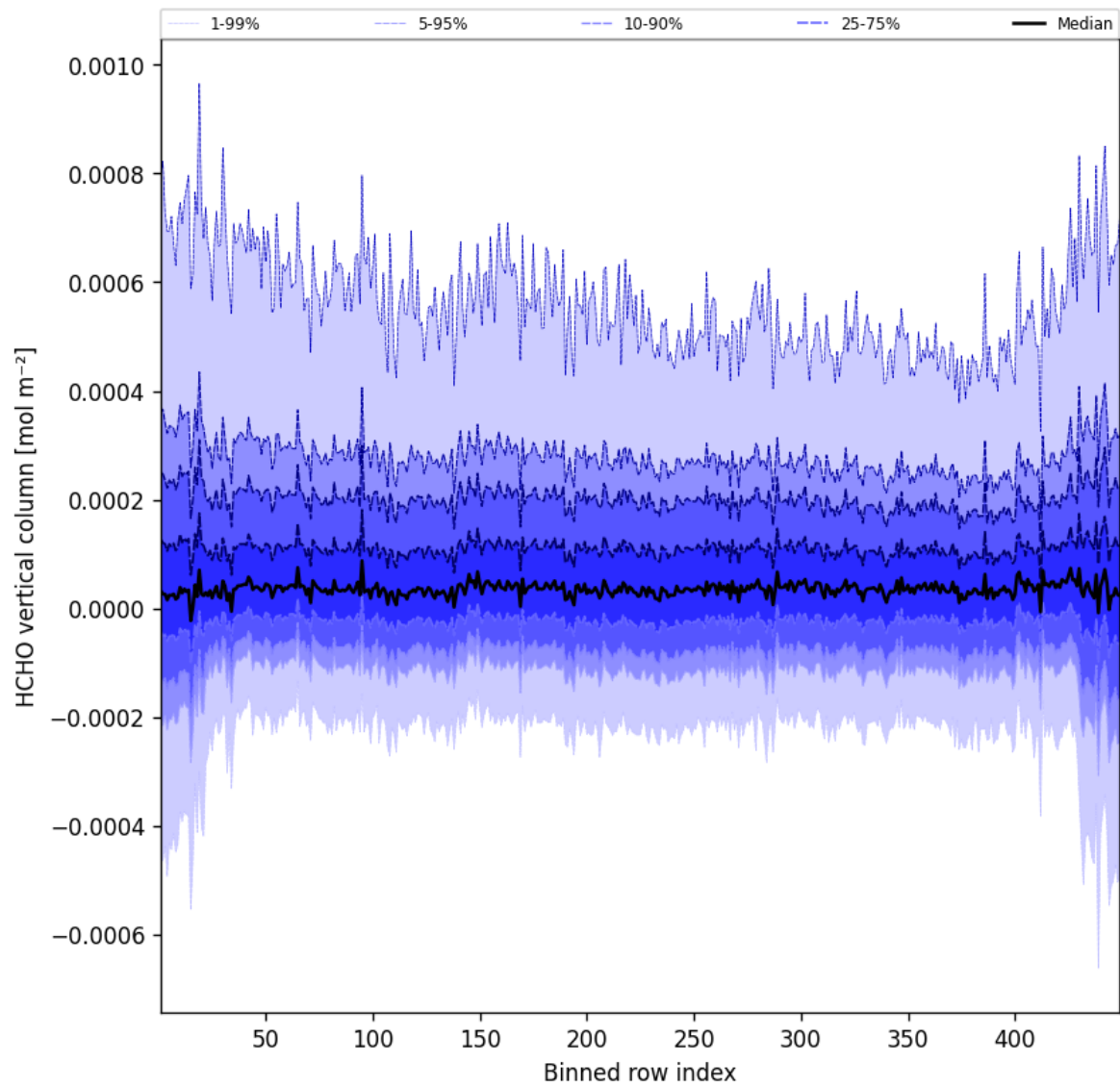
Figure 47: Along track statistics of “HCHO vertical column” for 2025-09-19 to 2025-09-20
