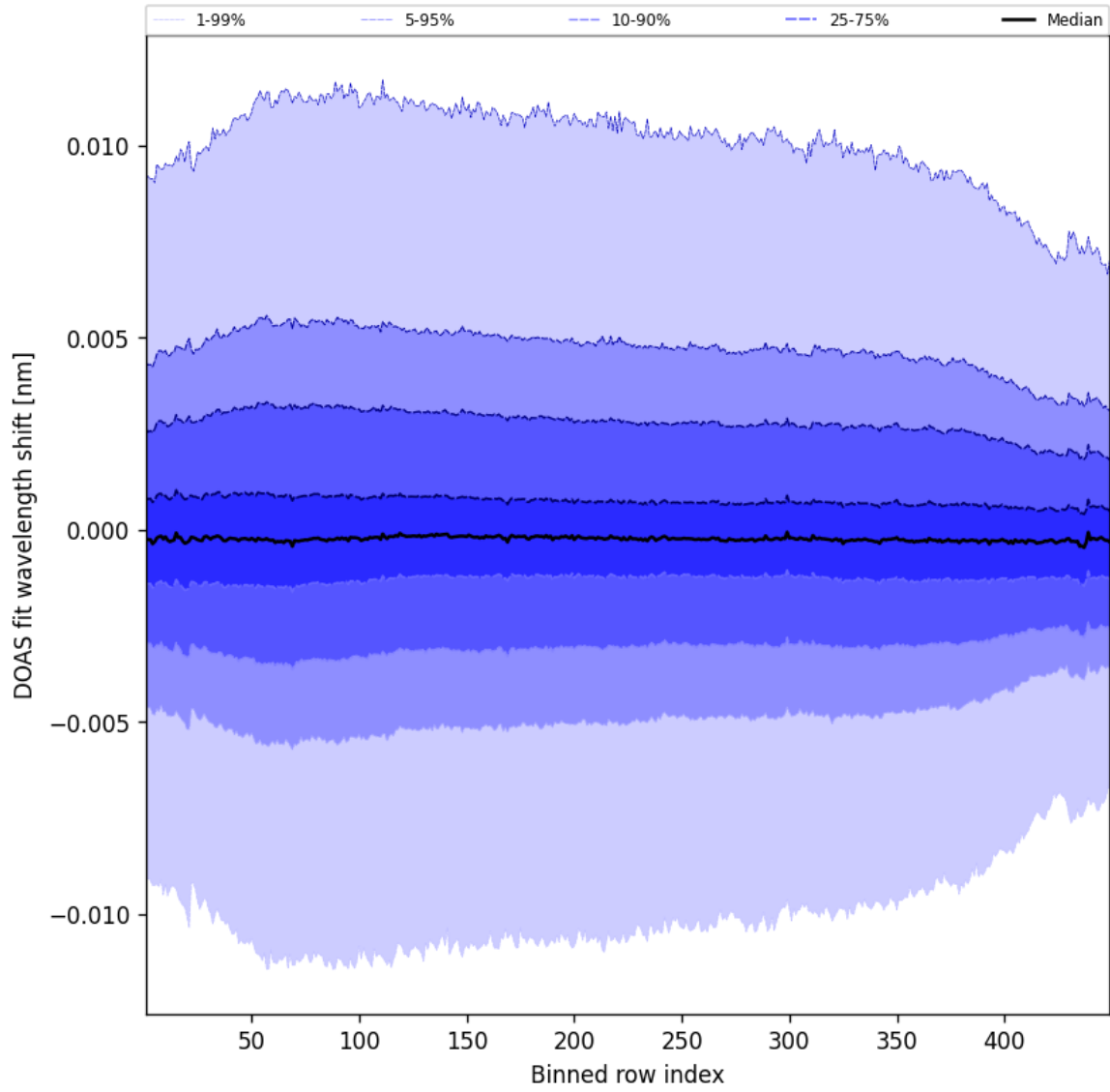
Figure 56: Along track statistics of “DOAS fit wavelength shift” for 2025-09-19 to 2025-09-20
