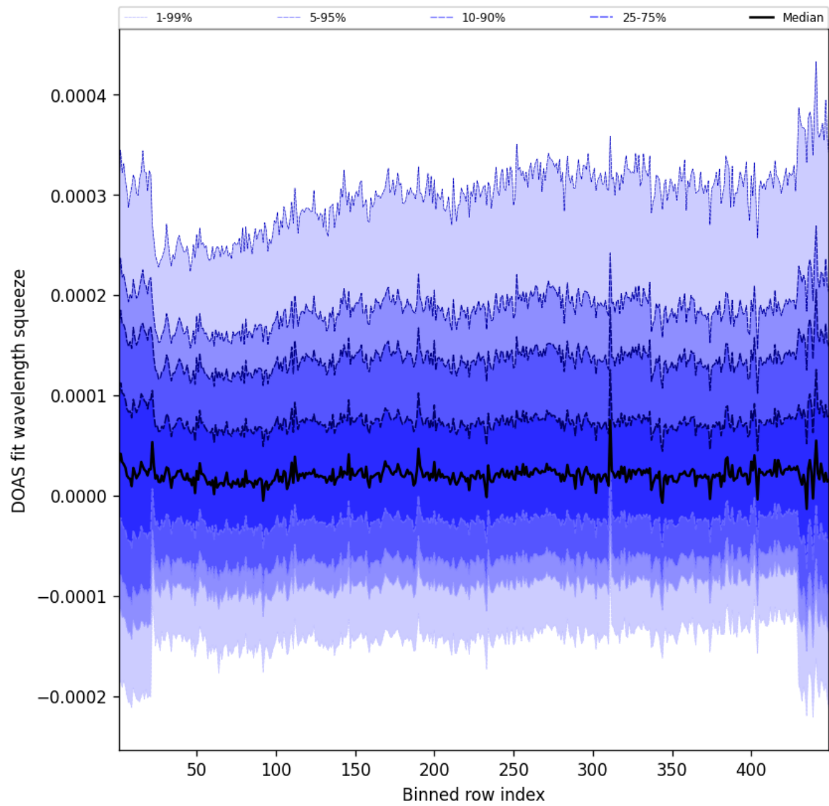
Figure 57: Along track statistics of “DOAS fit wavelength squeeze” for 2025-09-19 to 2025-09-20
