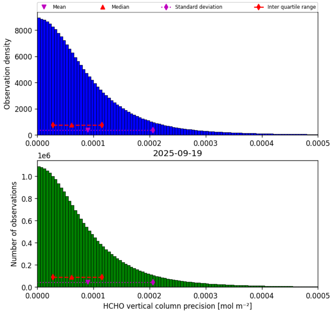
Figure 34: Histogram of “HCHO vertical column precision” for 2025-09-19 to 2025-09-20
