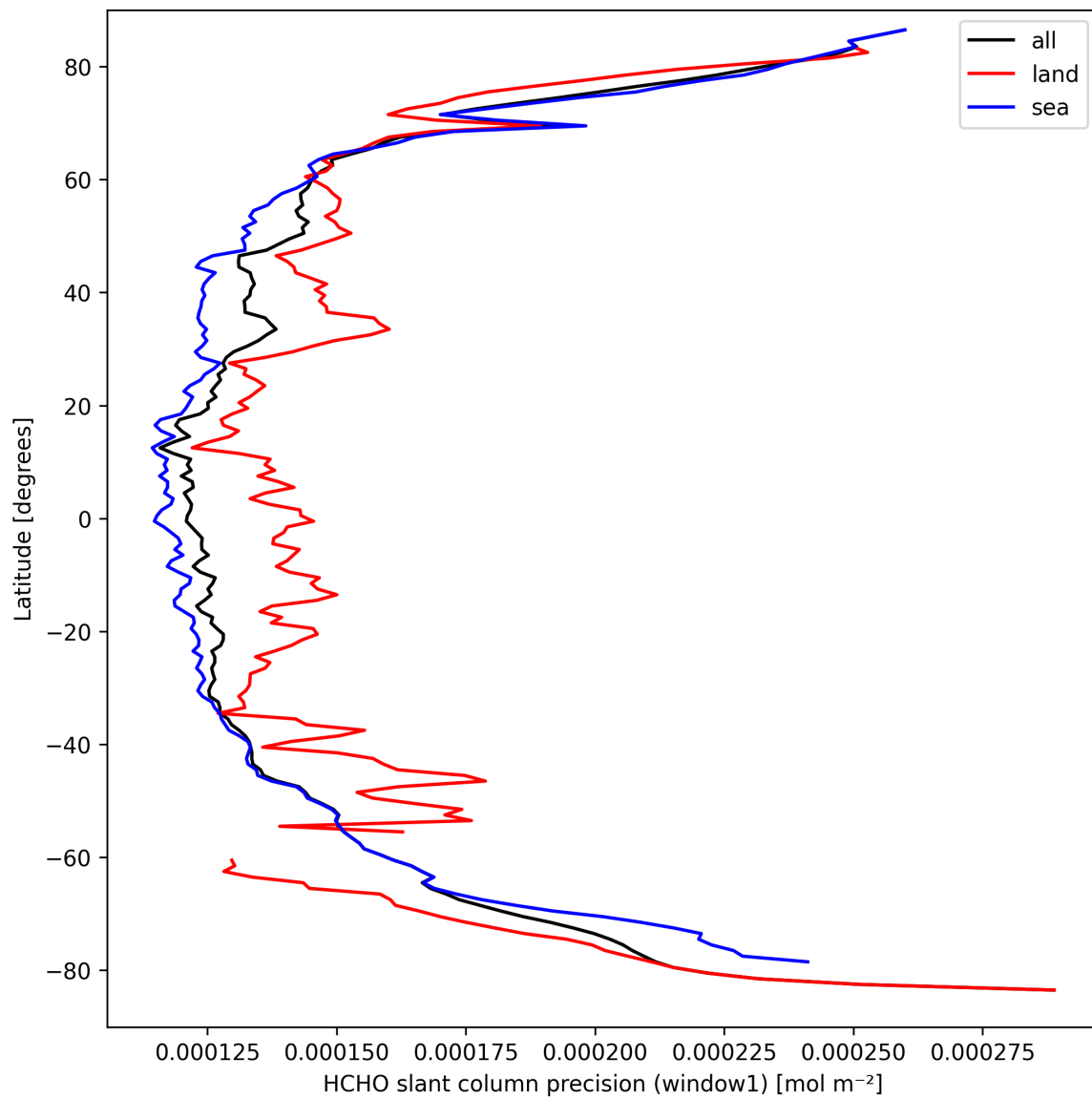
Figure 23: Zonal average of “HCHO slant column precision (window1)” for 2025-09-19 to 2025-09-20.
