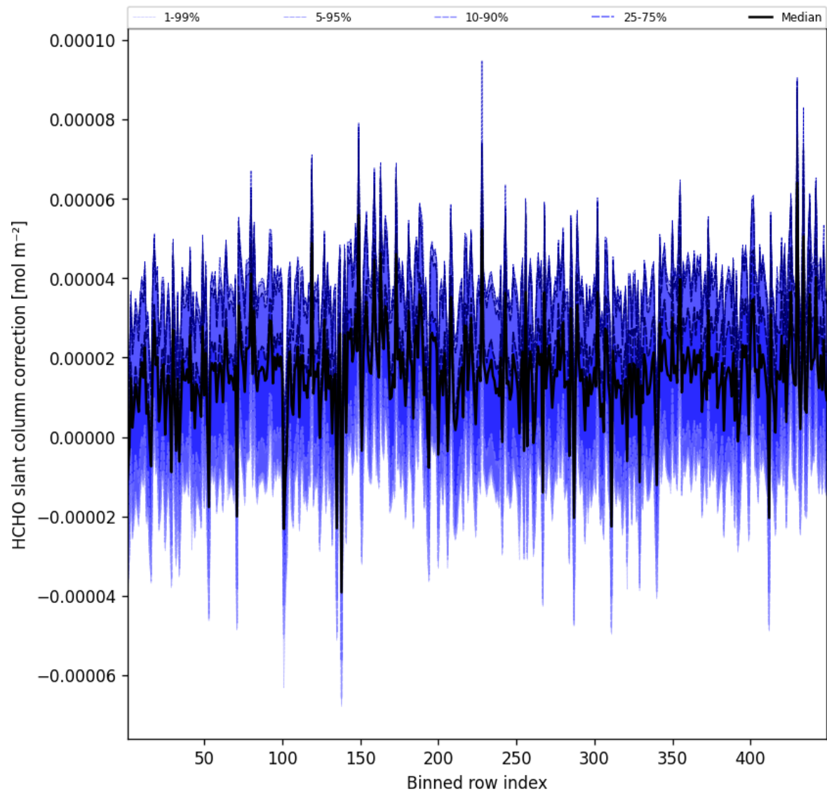
Figure 59: Along track statistics of “HCHO slant column correction” for 2025-09-19 to 2025-09-20
