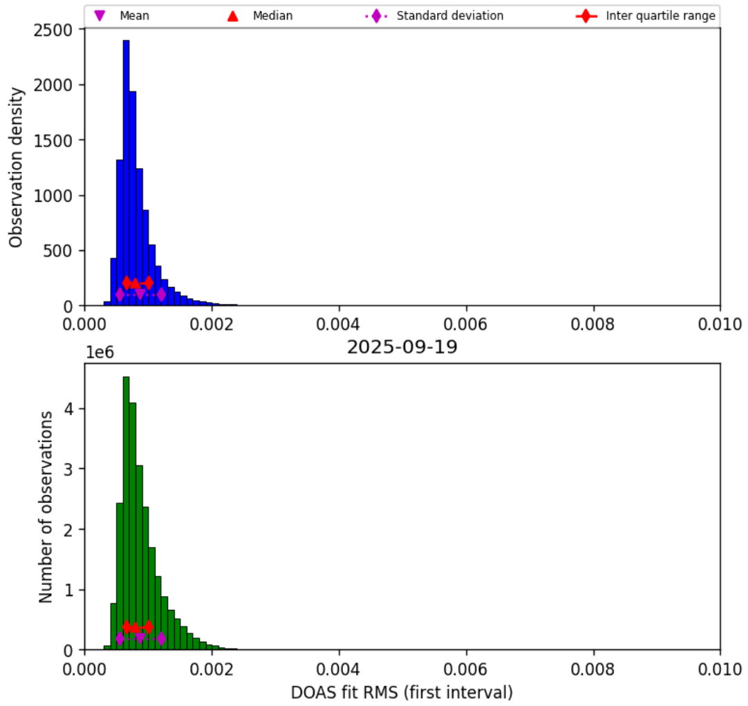
Figure 44: Histogram of “DOAS fit RMS (first interval)” for 2025-09-19 to 2025-09-20
