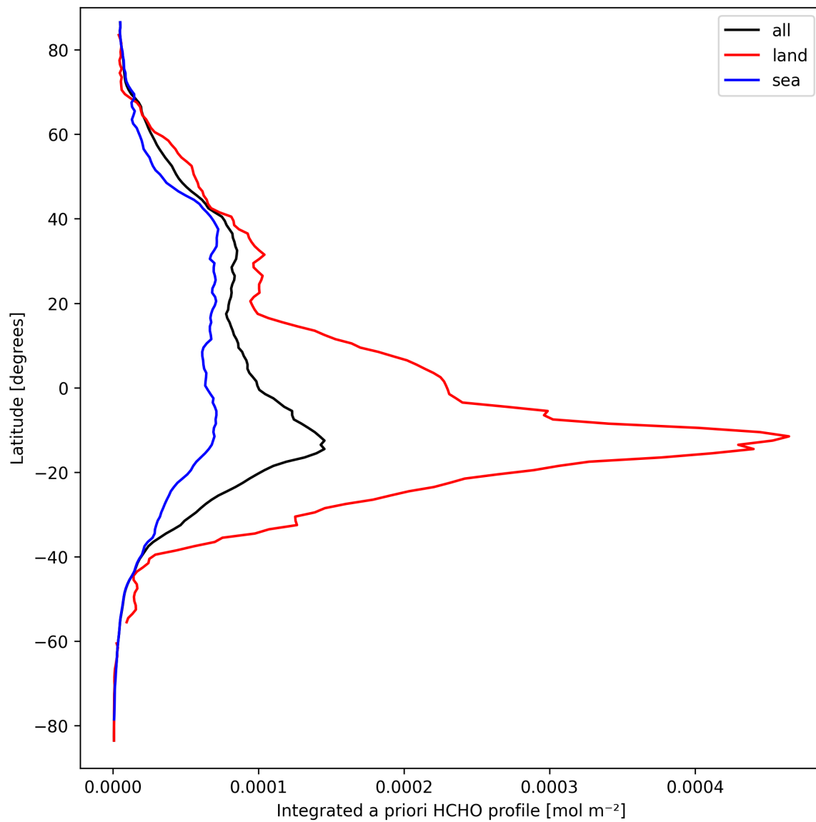
Figure 27: Zonal average of “Integrated a priori HCHO profile” for 2025-09-19 to 2025-09-20.
