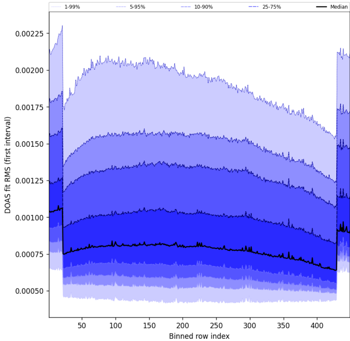
Figure 58: Along track statistics of “DOAS fit RMS (first interval)” for 2025-09-19 to 2025-09-20
