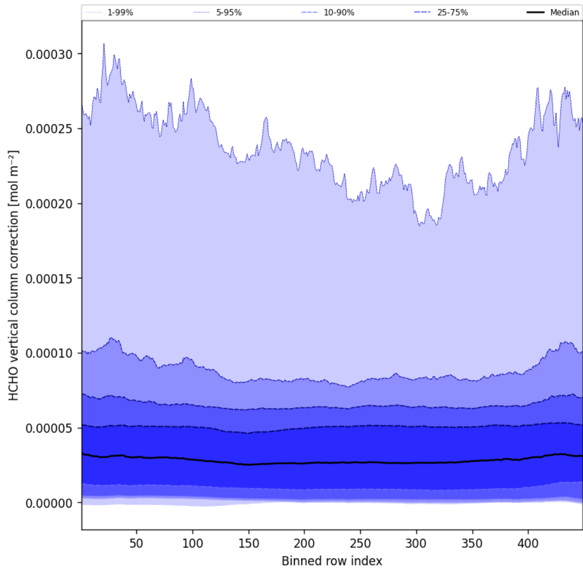
Figure 49: Along track statistics of “HCHO vertical column correction” for 2025-09-19 to 2025-09-20
