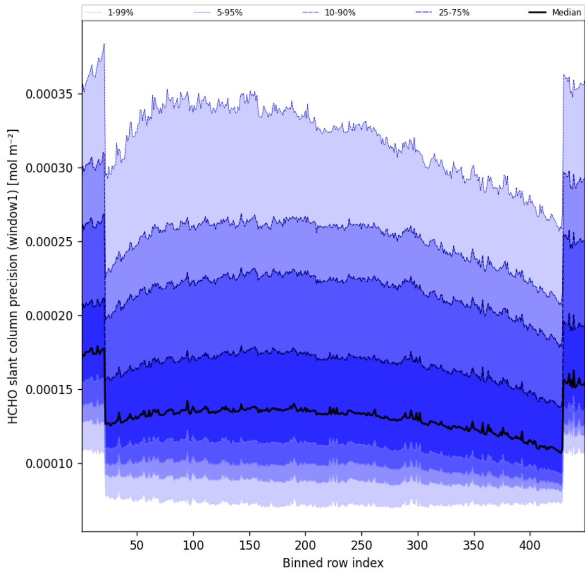
Figure 51: Along track statistics of “HCHO slant column precision (window1)” for 2025-09-19 to 2025-09-20
