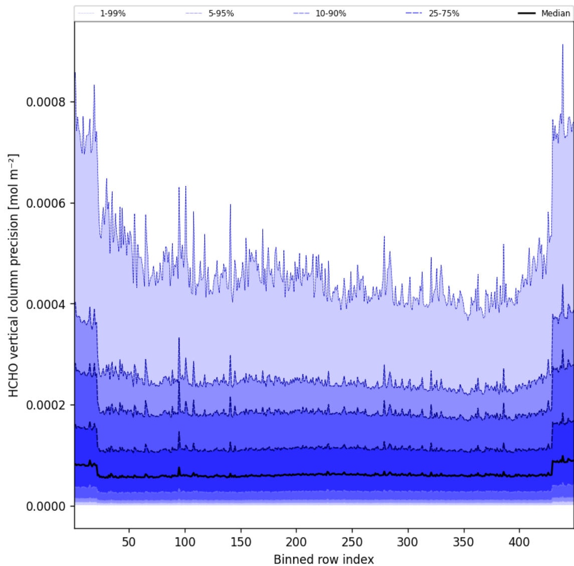
Figure 48: Along track statistics of “HCHO vertical column precision” for 2025-09-19 to 2025-09-20
