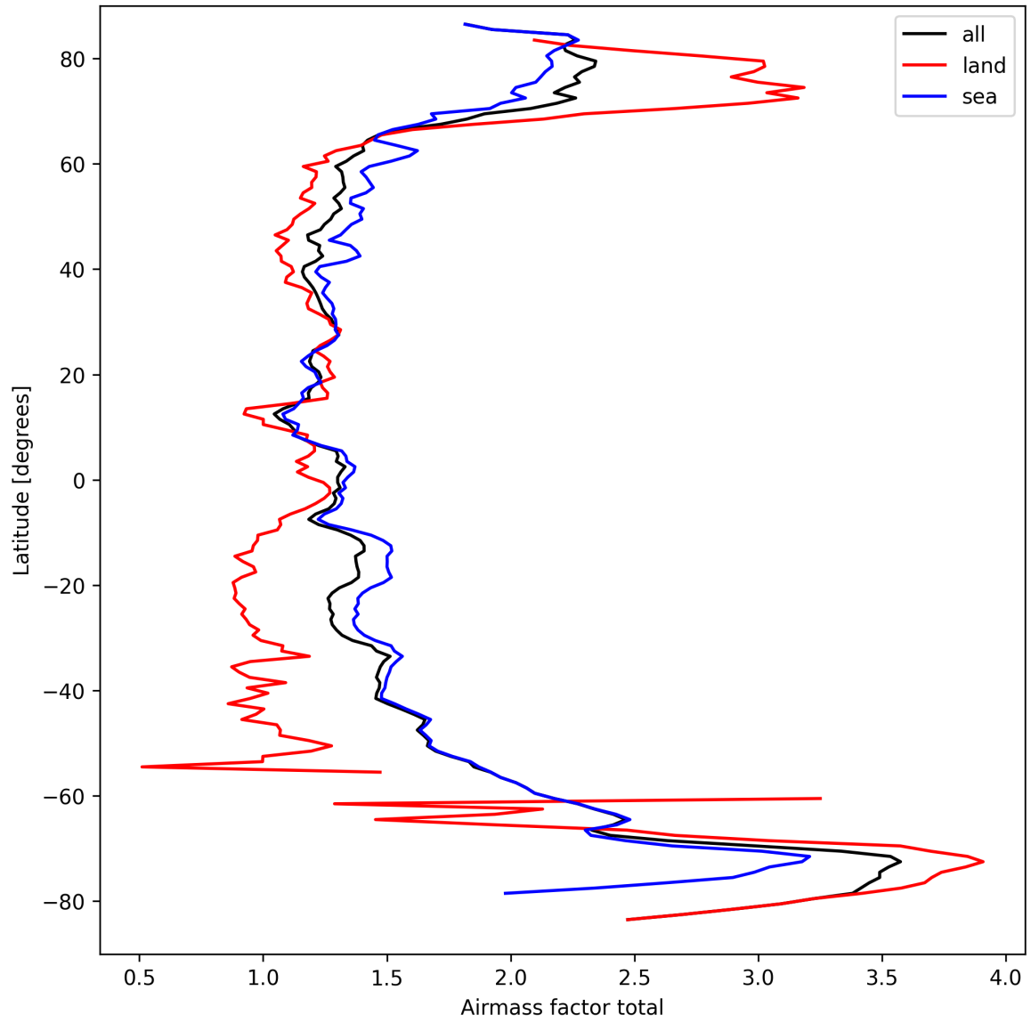
Figure 24: Zonal average of “Airmass factor total” for 2025-09-19 to 2025-09-20.
