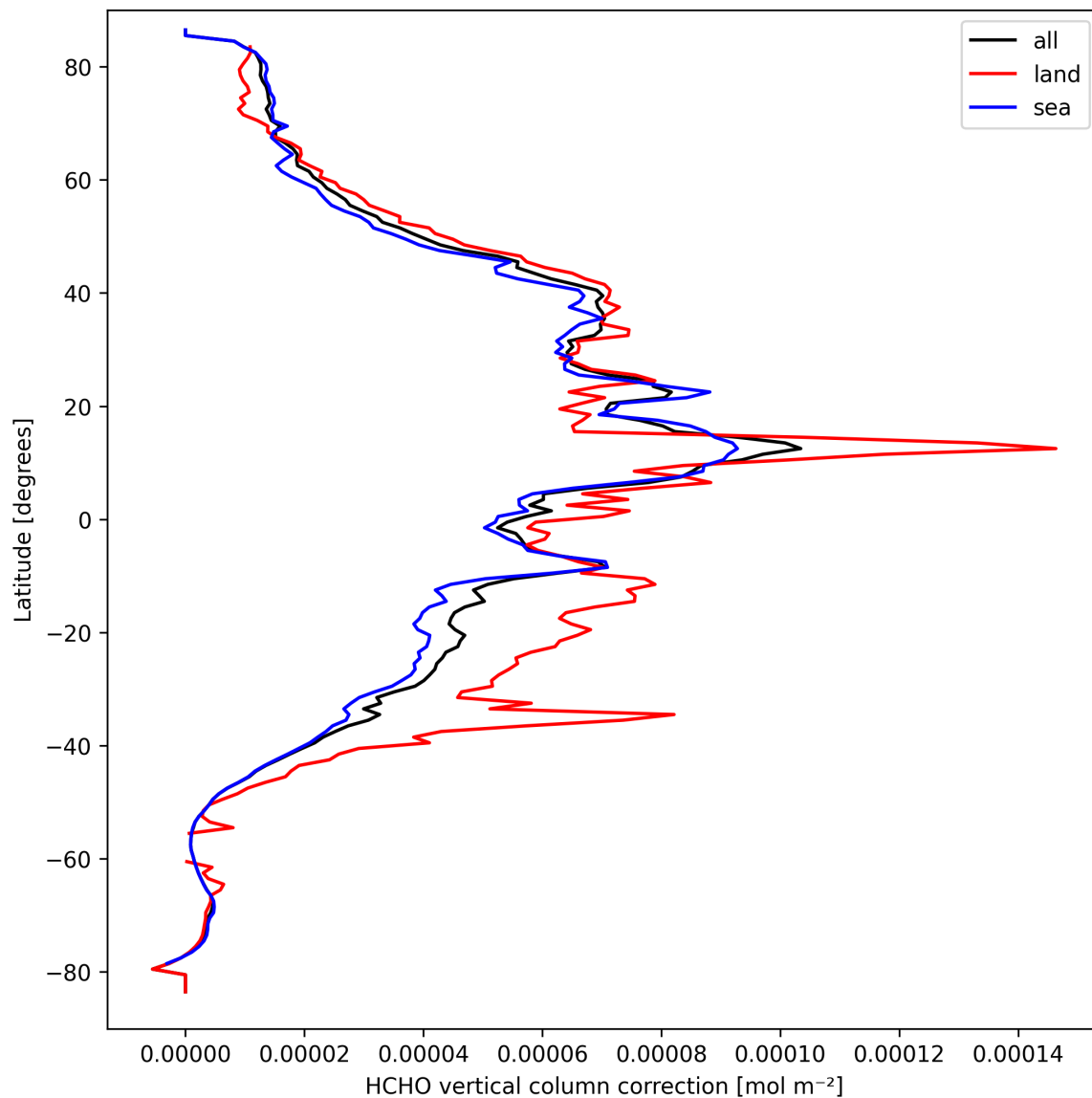
Figure 21: Zonal average of “HCHO vertical column correction” for 2025-09-19 to 2025-09-20.
