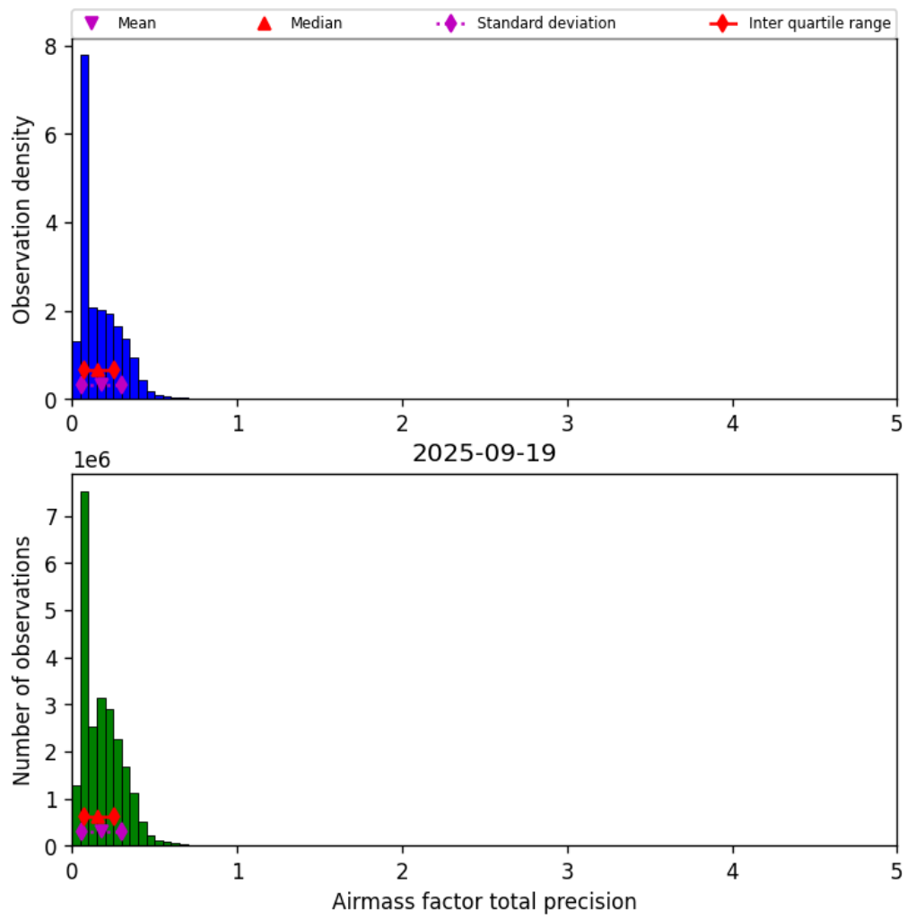
Figure 39: Histogram of “Airmass factor total precision” for 2025-09-19 to 2025-09-20
