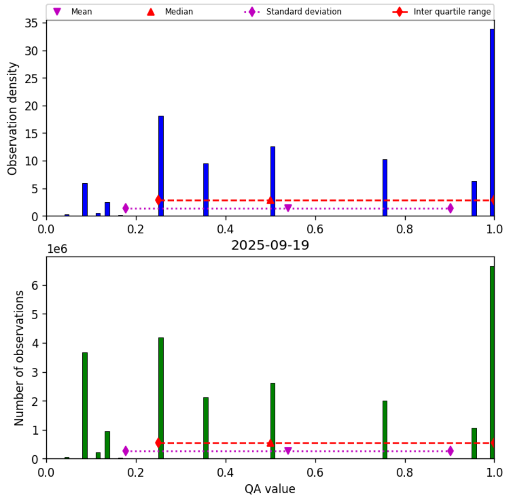
Figure 32: Histogram of “QA value” for 2025-09-19 to 2025-09-20
