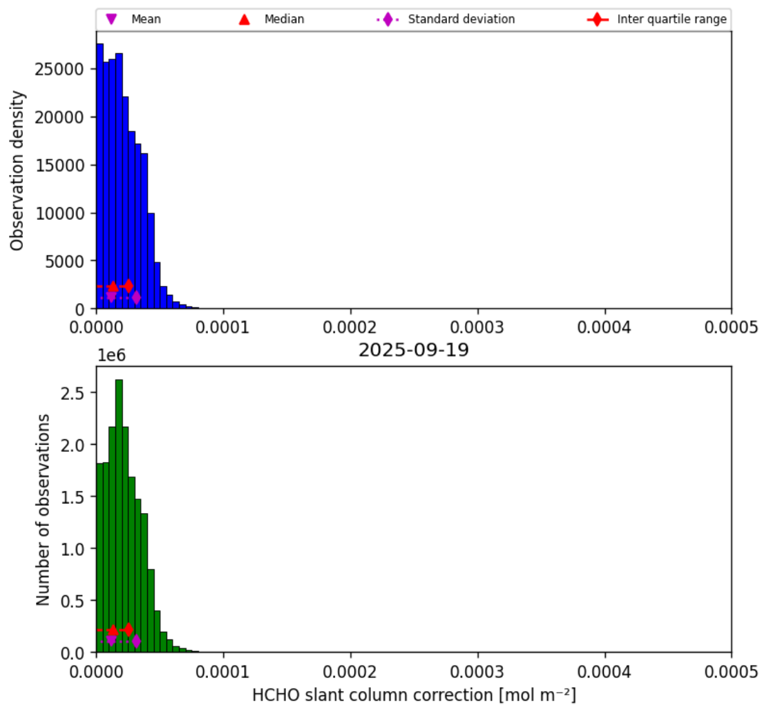
Figure 45: Histogram of “HCHO slant column correction” for 2025-09-19 to 2025-09-20
