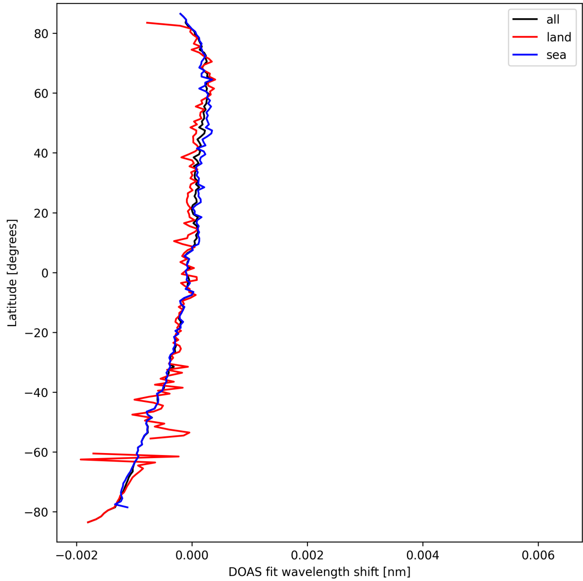
Figure 28: Zonal average of “DOAS fit wavelength shift” for 2025-09-19 to 2025-09-20.
