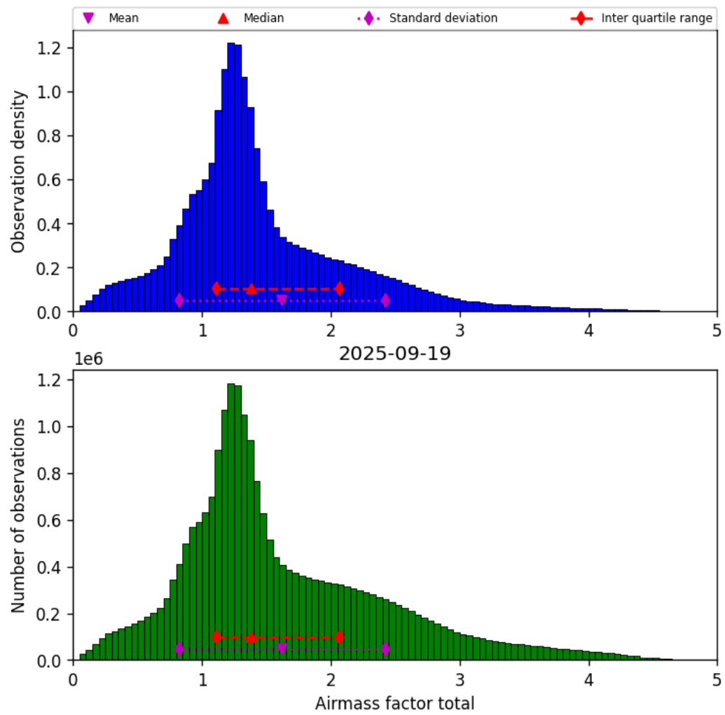
Figure 38: Histogram of “Airmass factor total” for 2025-09-19 to 2025-09-20
