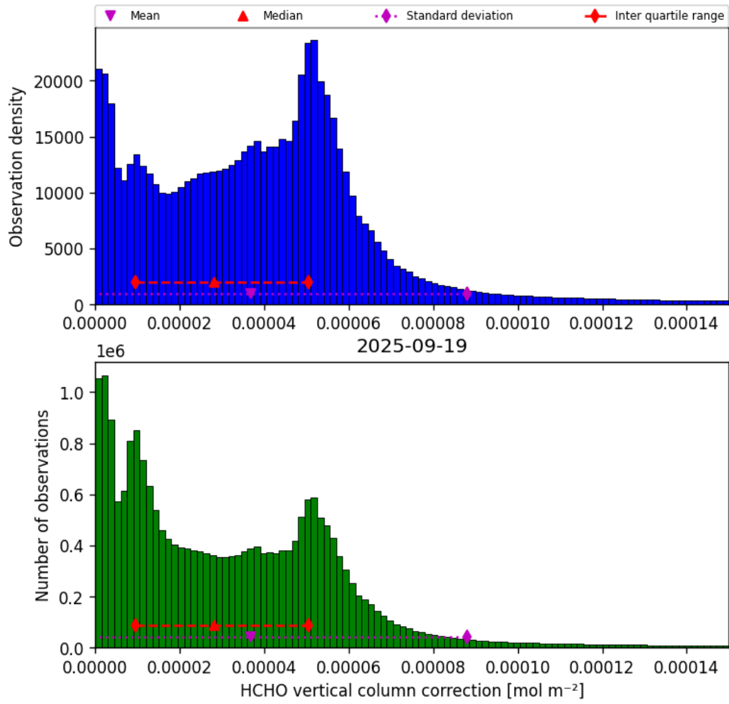
Figure 35: Histogram of “HCHO vertical column correction” for 2025-09-19 to 2025-09-20
