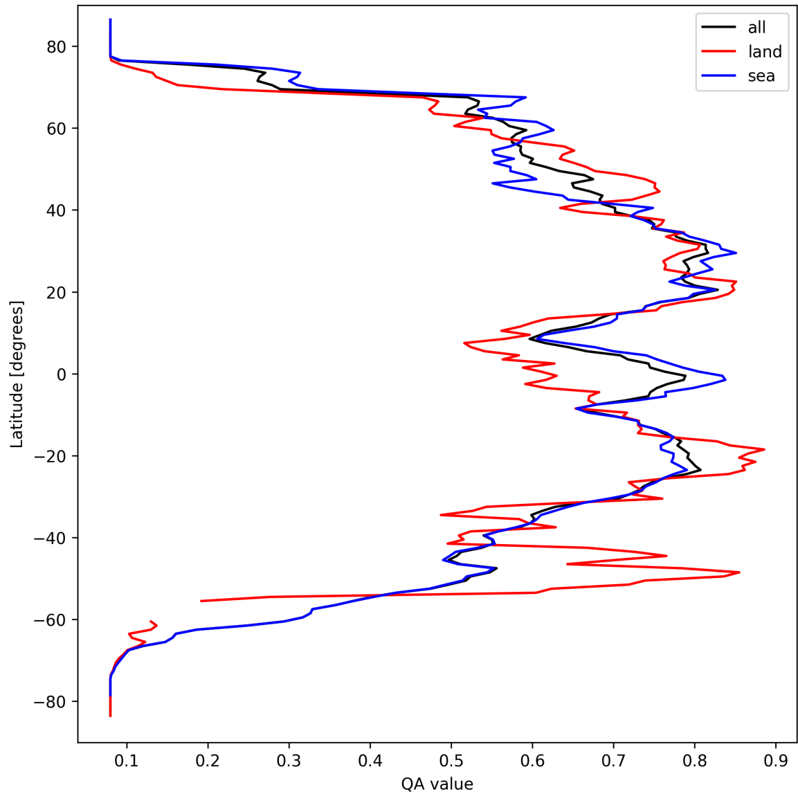
Figure 18: Zonal average of “QA value” for 2025-09-19 to 2025-09-20.
