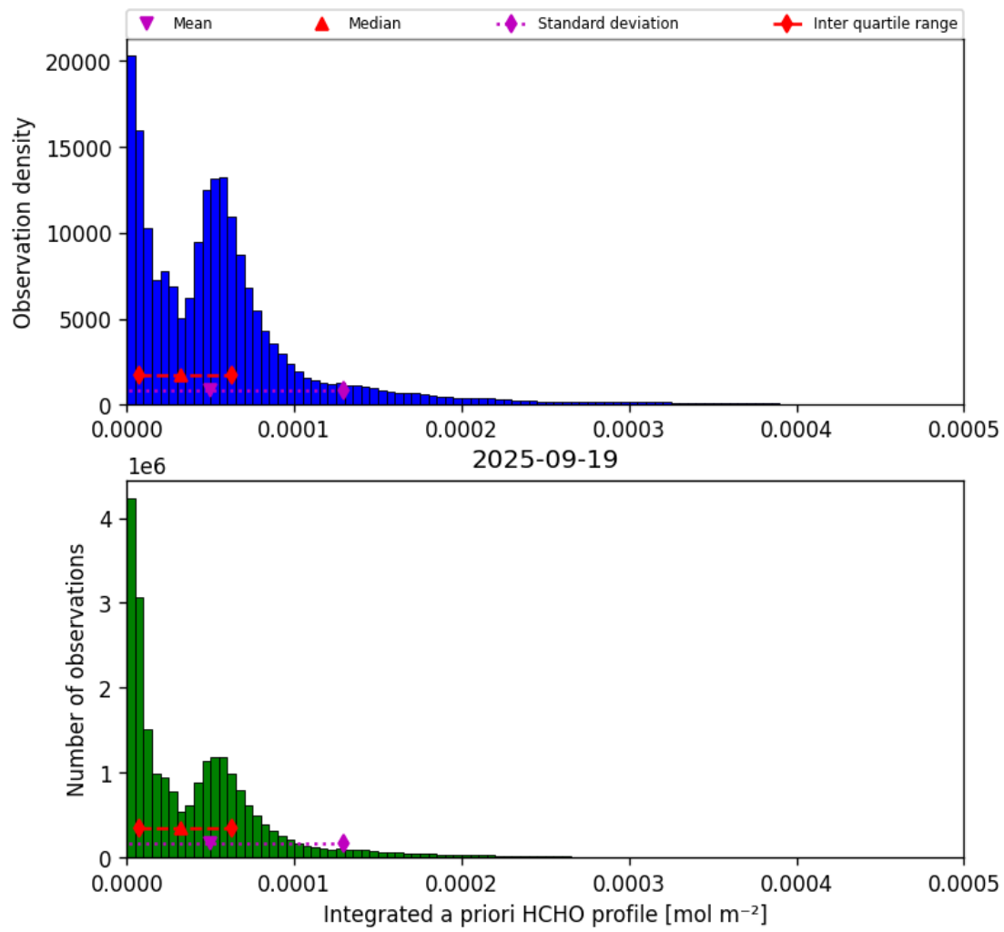
Figure 41: Histogram of “Integrated a priori HCHO profile” for 2025-09-19 to 2025-09-20
