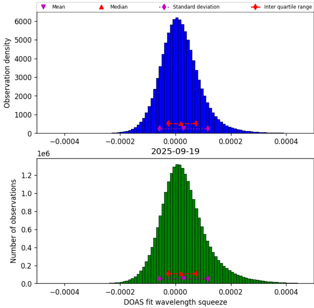
Figure 43: Histogram of “DOAS fit wavelength squeeze” for 2025-09-19 to 2025-09-20
