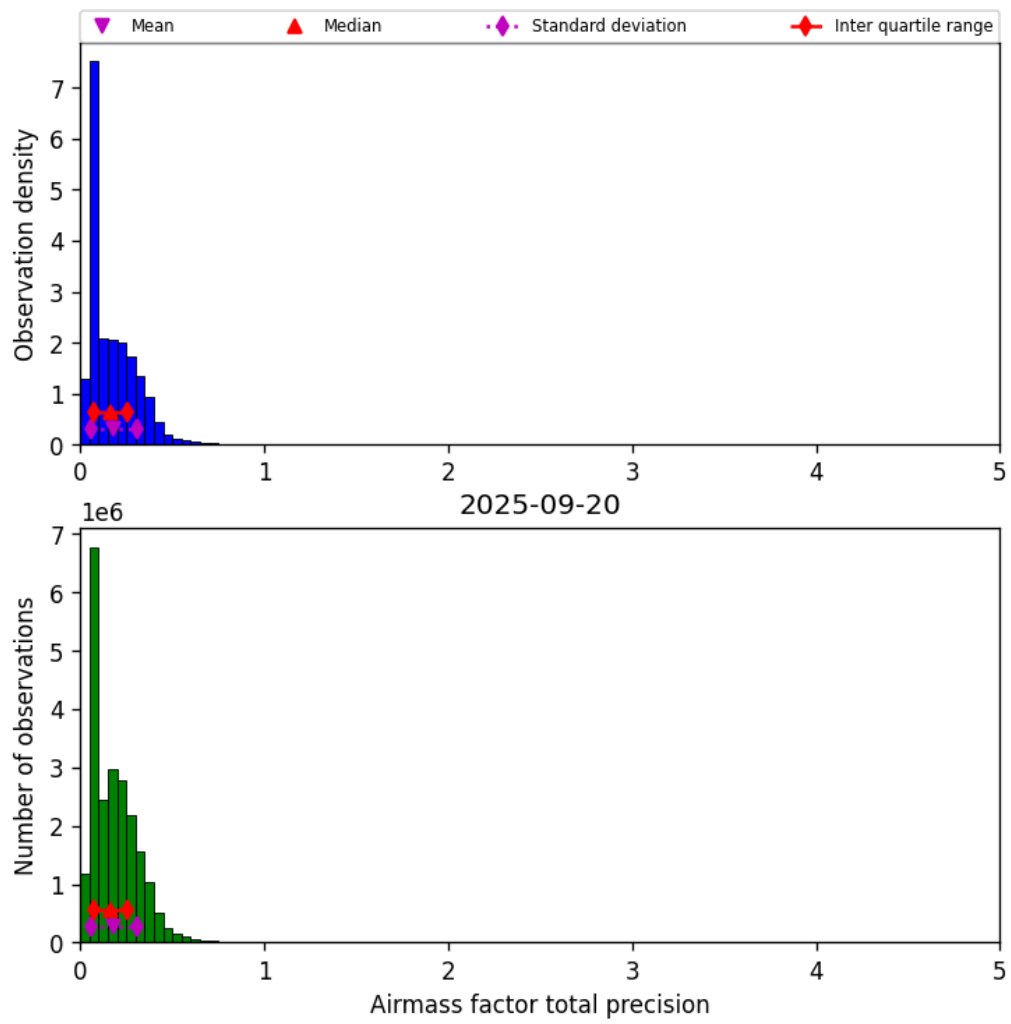
Figure 39: Histogram of “Airmass factor total precision” for 2025-09-20 to 2025-09-21
