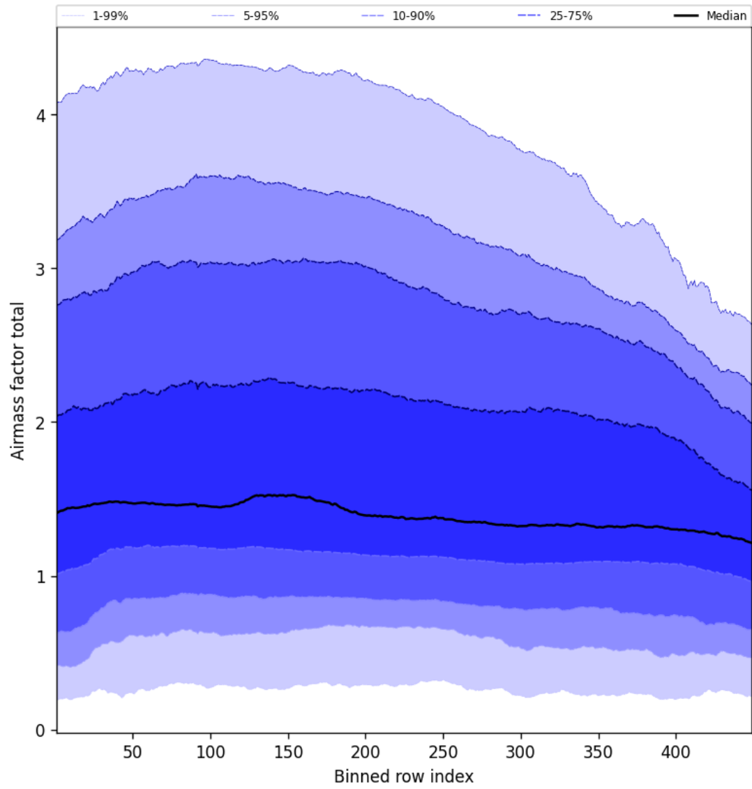
Figure 52: Along track statistics of “Airmass factor total” for 2025-09-20 to 2025-09-21
