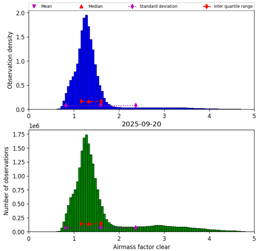
Figure 40: Histogram of “Airmass factor clear” for 2025-09-20 to 2025-09-21
