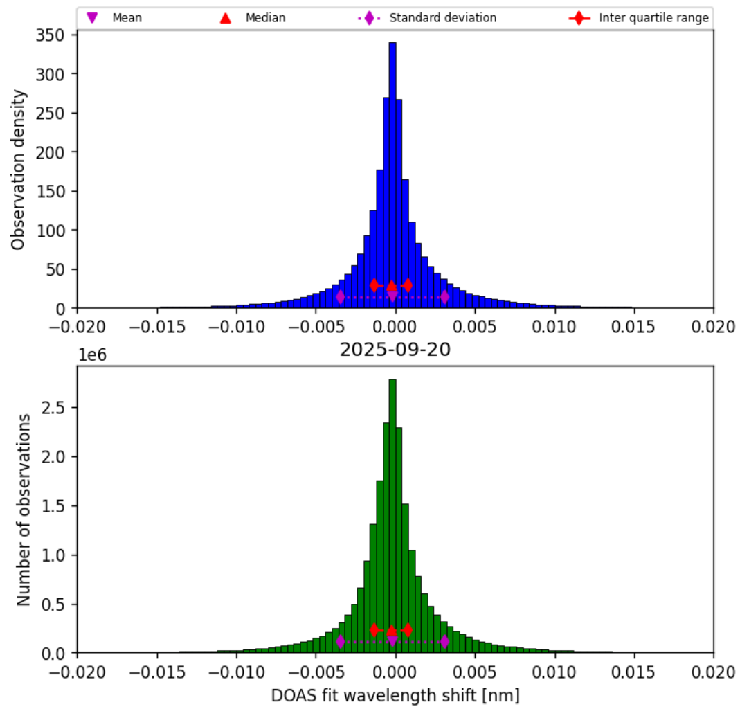
Figure 42: Histogram of “DOAS fit wavelength shift” for 2025-09-20 to 2025-09-21
