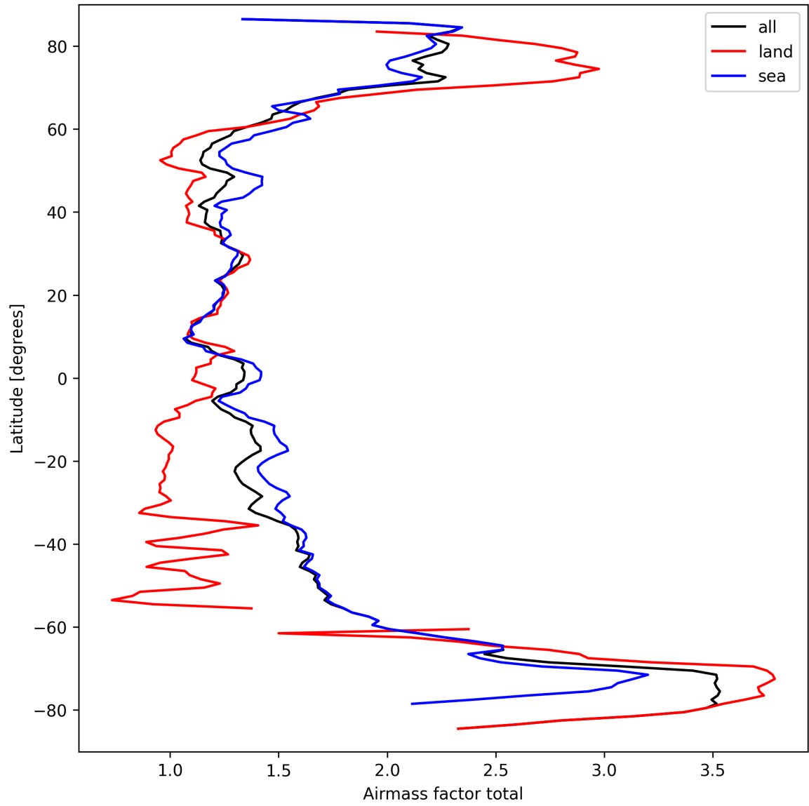
Figure 24: Zonal average of “Airmass factor total” for 2025-09-20 to 2025-09-21.
