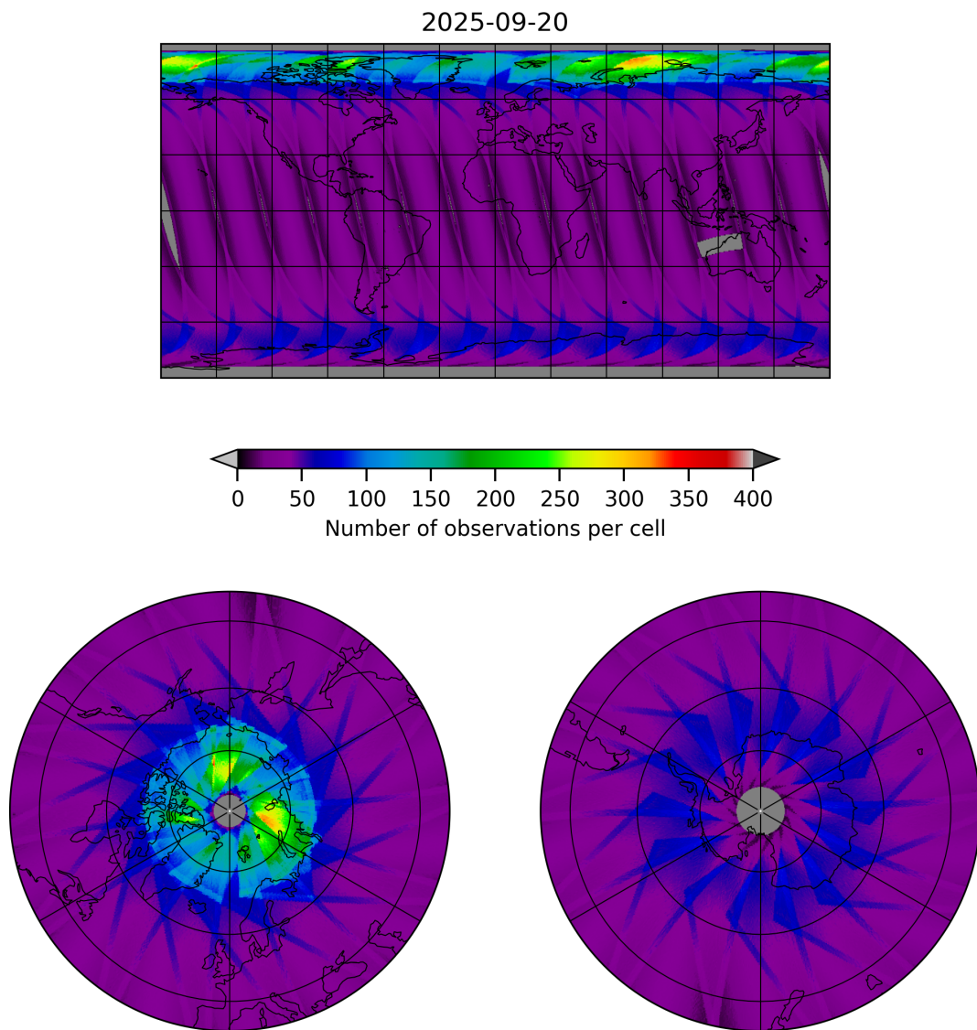
Figure 17: Map of the number of observations for 2025-09-20 to 2025-09-21
