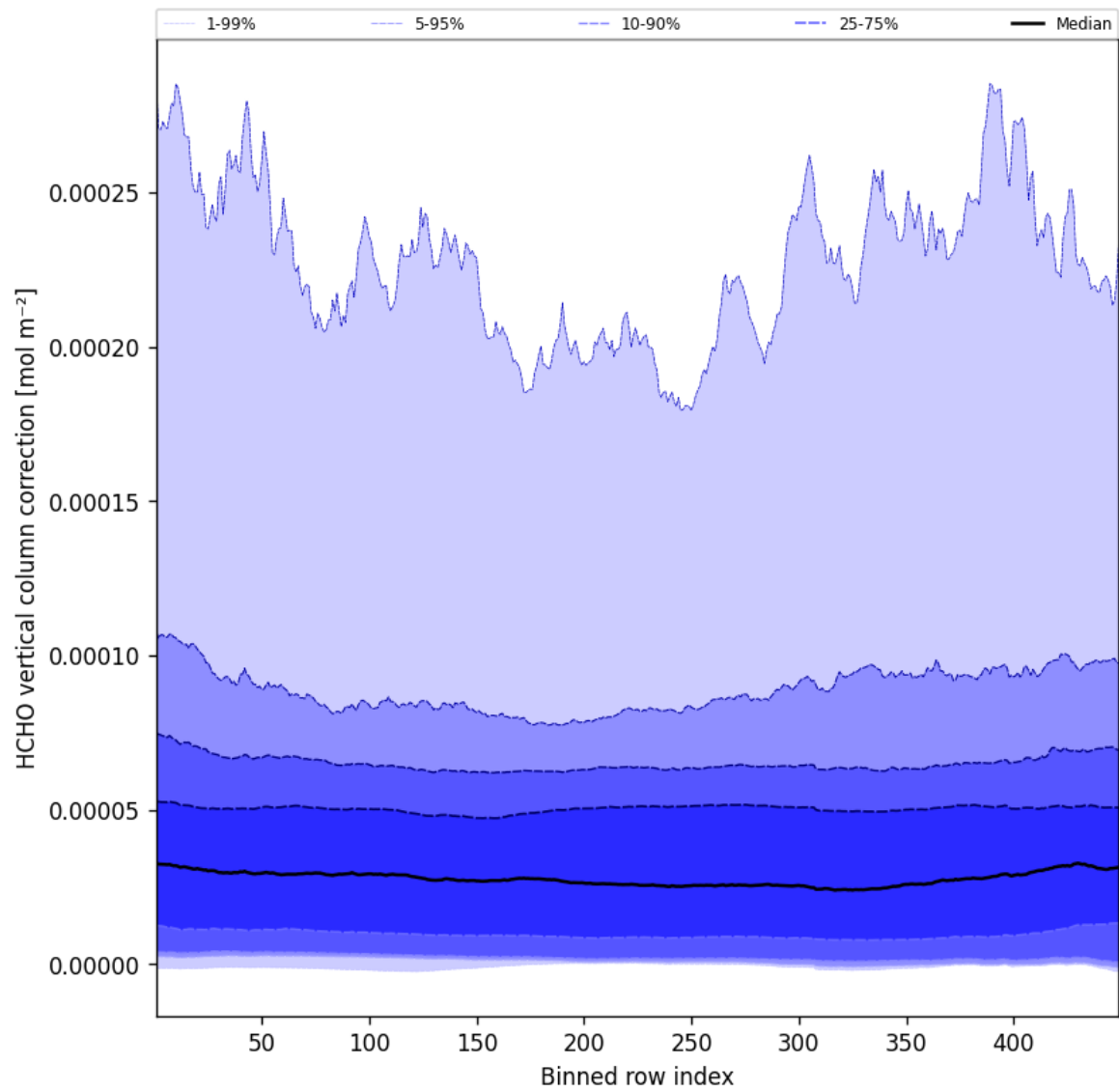
Figure 49: Along track statistics of “HCHO vertical column correction” for 2025-09-20 to 2025-09-21
