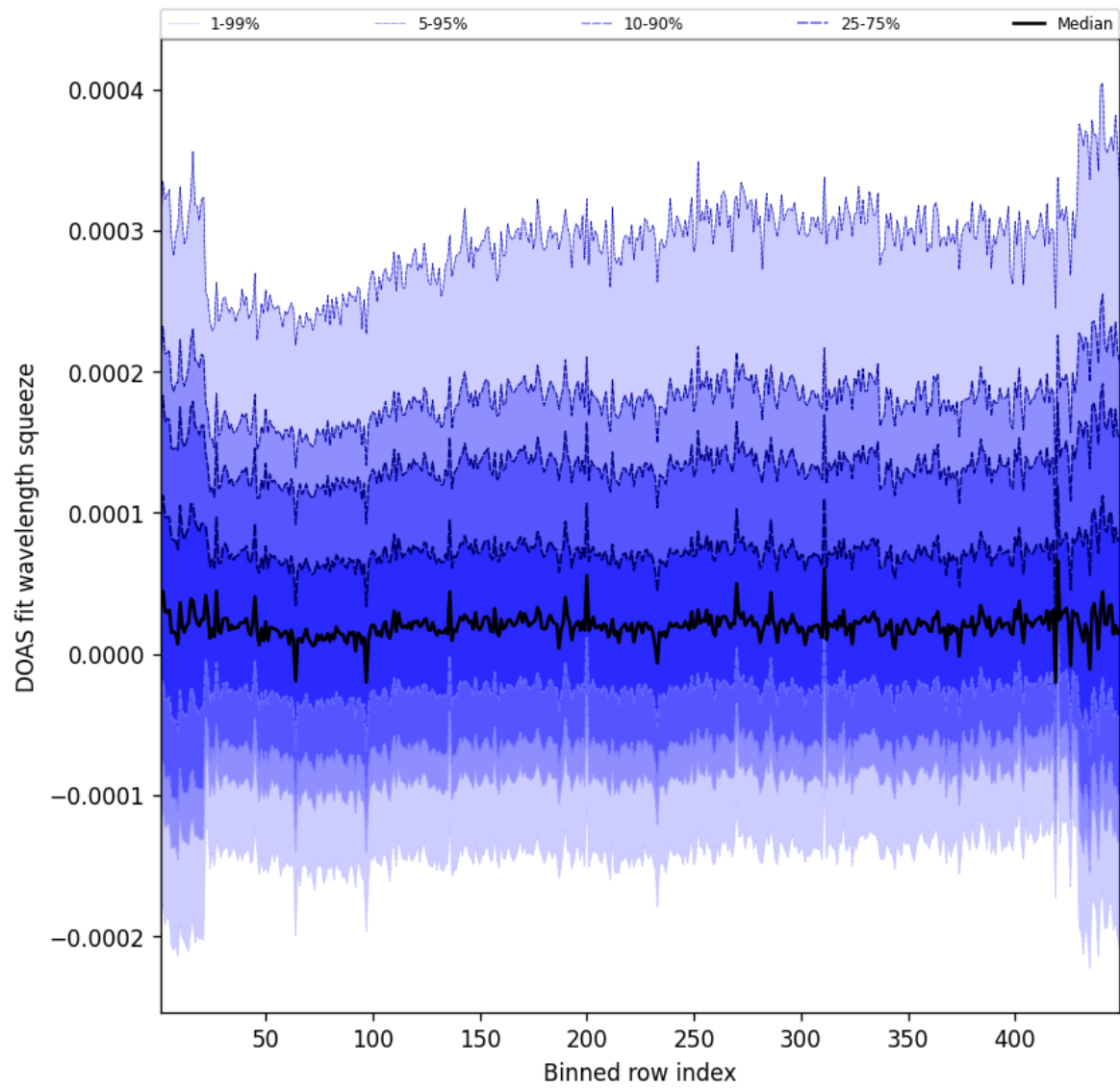
Figure 57: Along track statistics of “DOAS fit wavelength squeeze” for 2025-09-20 to 2025-09-21
