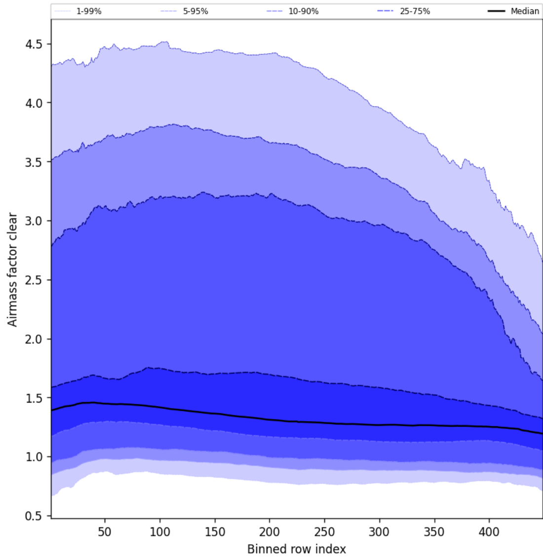
Figure 54: Along track statistics of “Air mass factor clear” for 2025-09-20 to 2025-09-21
