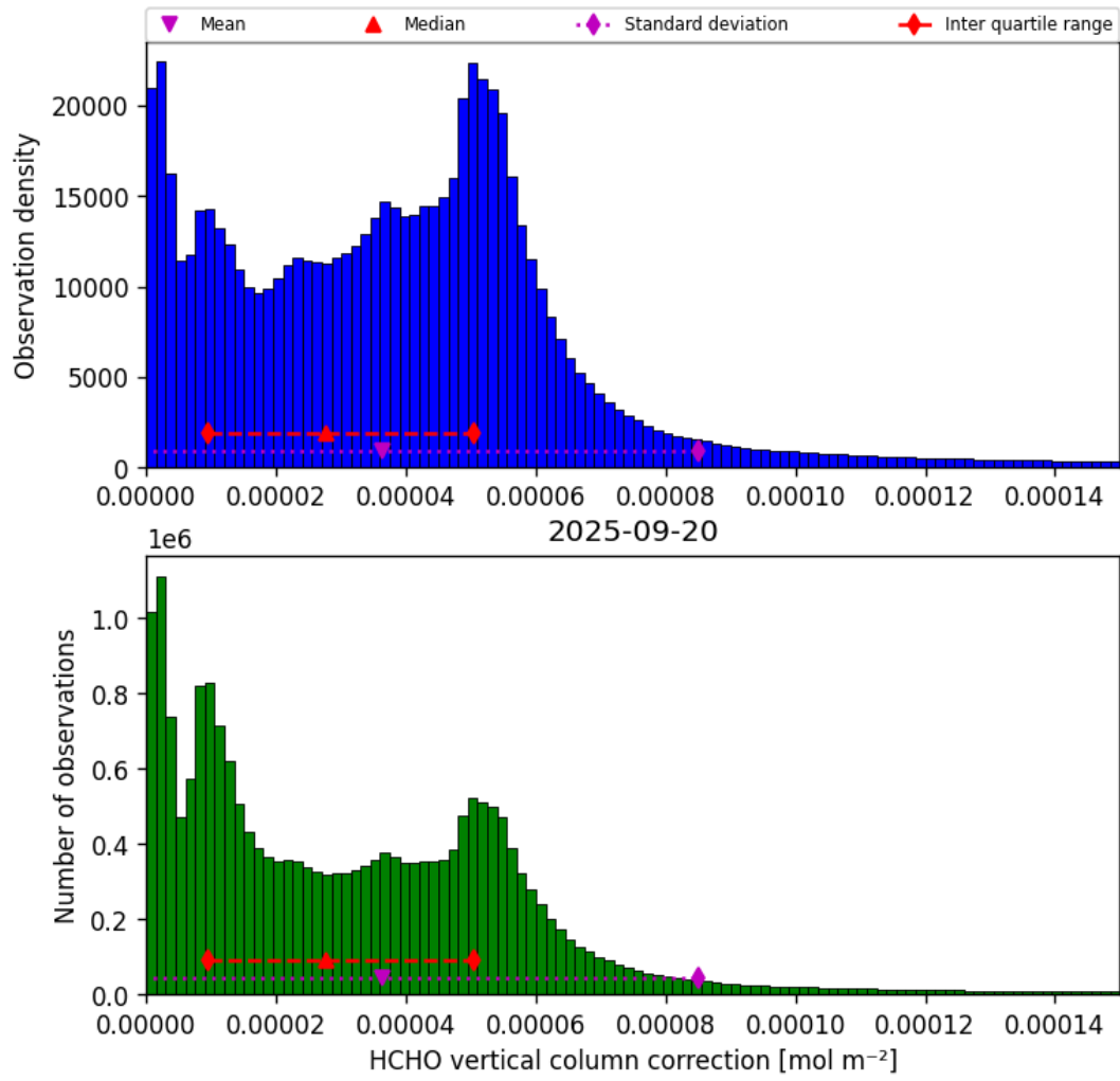
Figure 35: Histogram of “HCHO vertical column correction” for 2025-09-20 to 2025-09-21
