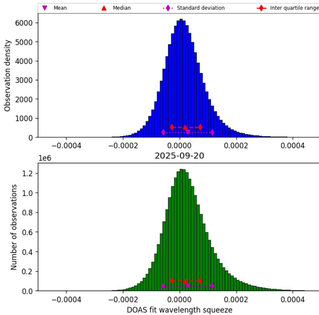
Figure 43: Histogram of “DOAS fit wavelength squeeze” for 2025-09-20 to 2025-09-21
