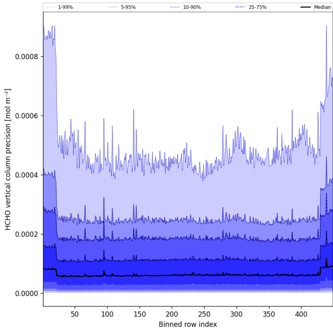
Figure 48: Along track statistics of “HCHO vertical column precision” for 2025-09-20 to 2025-09-21
