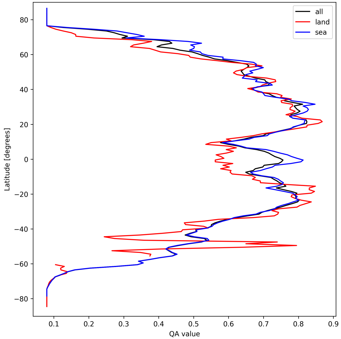
Figure 18: Zonal average of “QA value” for 2025-09-20 to 2025-09-21.
