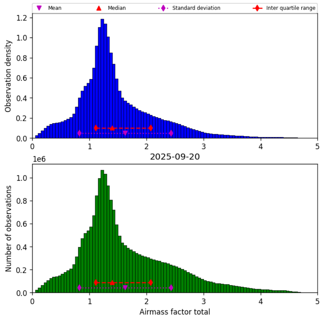
Figure 38: Histogram of “Airmass factor total” for 2025-09-20 to 2025-09-21
