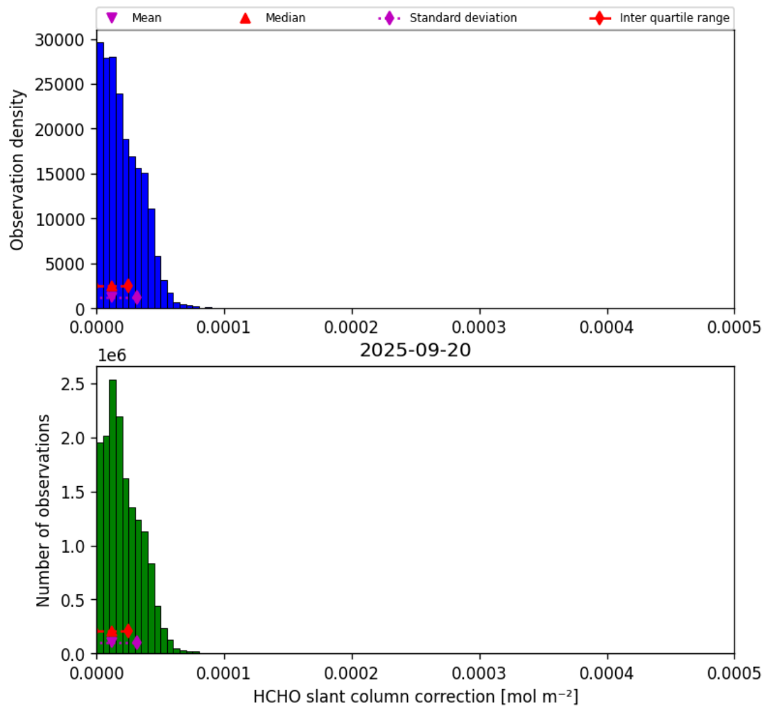
Figure 45: Histogram of “HCHO slant column correction” for 2025-09-20 to 2025-09-21
