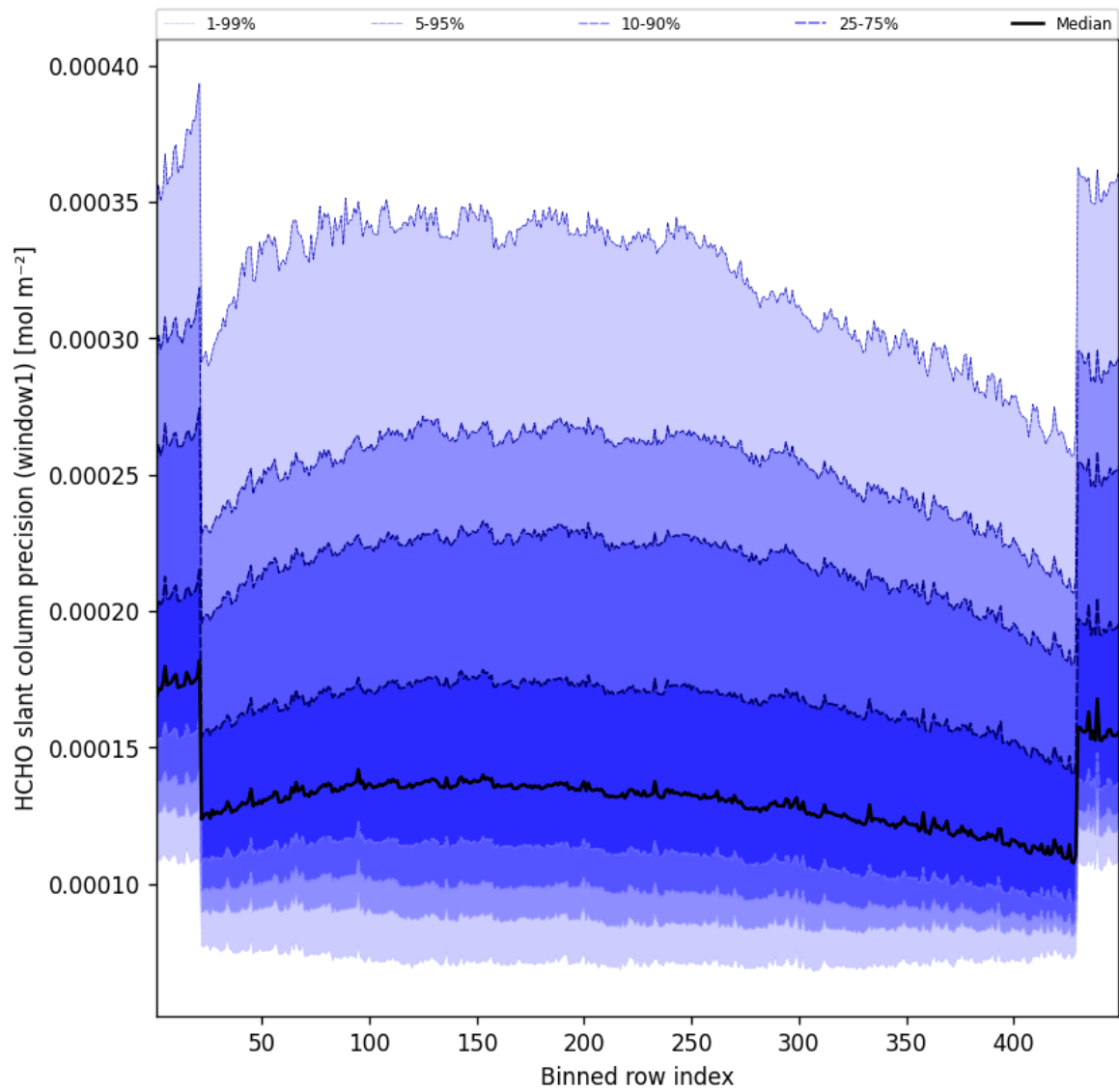
Figure 51: Along track statistics of “HCHO slant column precision (window1)” for 2025-09-20 to 2025-09-21
