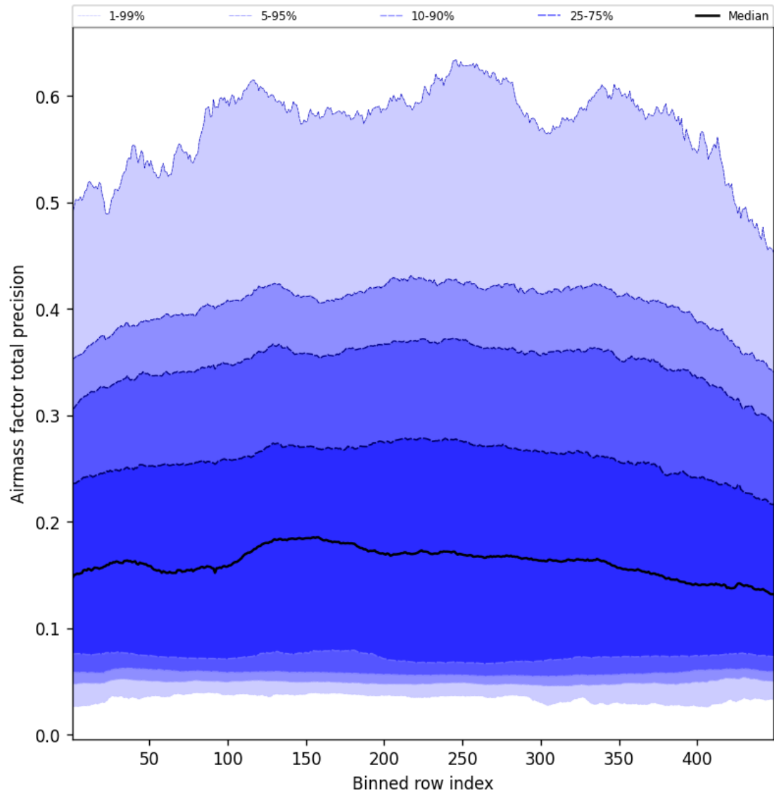
Figure 53: Along track statistics of “Airmass factor total precision” for 2025-09-20 to 2025-09-21
