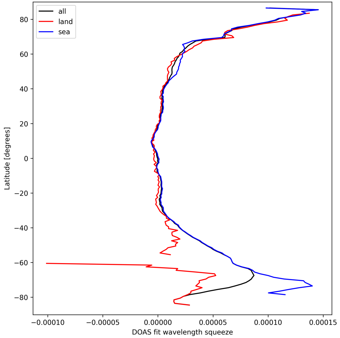
Figure 29: Zonal average of “DOAS fit wavelength squeeze” for 2025-09-20 to 2025-09-21.
