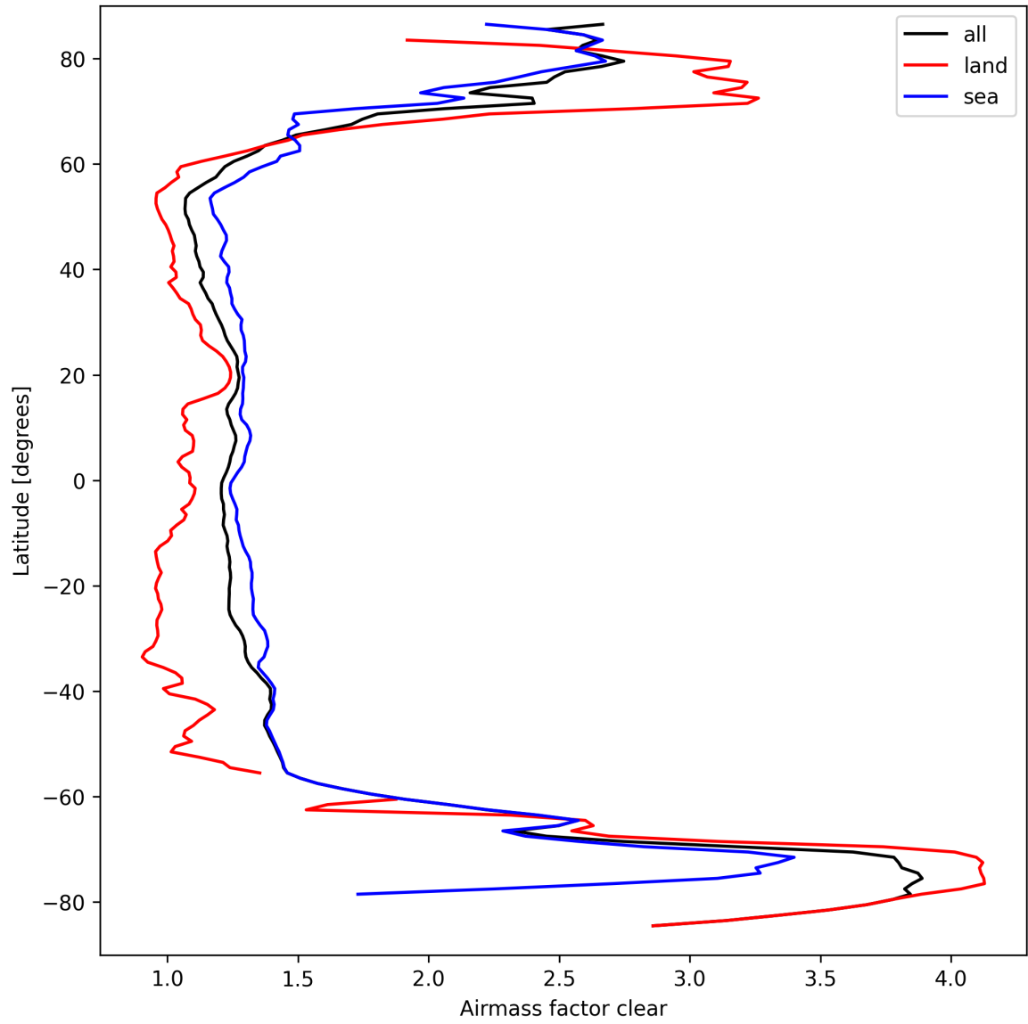
Figure 26: Zonal average of “Airmass factor clear” for 2025-09-20 to 2025-09-21.
