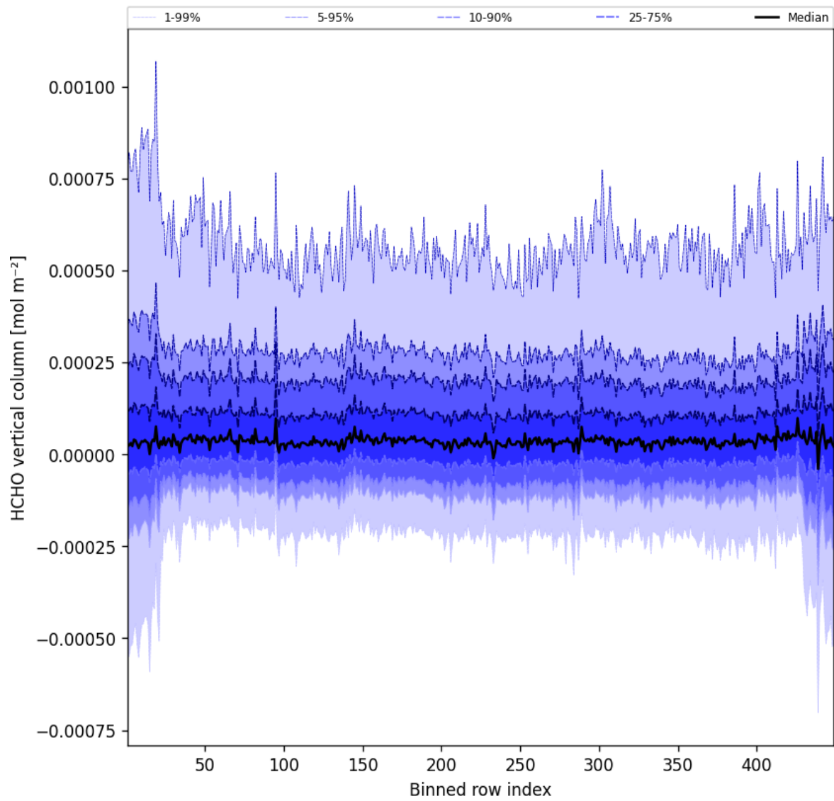
Figure 47: Along track statistics of “HCHO vertical column” for 2025-09-20 to 2025-09-21
