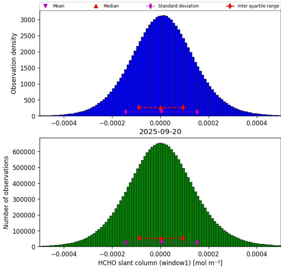
Figure 36: Histogram of “HCHO slant column (window1)” for 2025-09-20 to 2025-09-21
