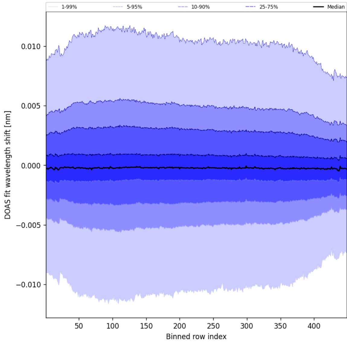
Figure 56: Along track statistics of “DOAS fit wavelength shift” for 2025-09-20 to 2025-09-21
