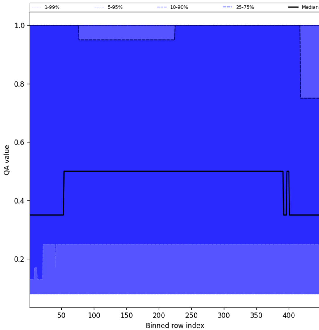
Figure 46: Along track statistics of “QA value” for 2025-09-20 to 2025-09-21
