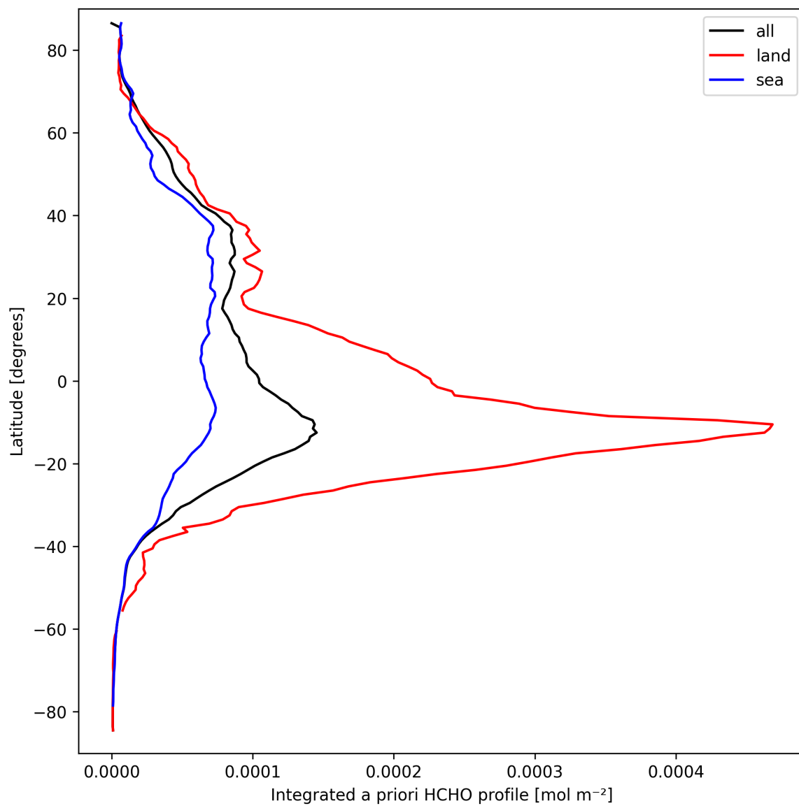
Figure 27: Zonal average of “Integrated a priori HCHO profile” for 2025-09-20 to 2025-09-21.
