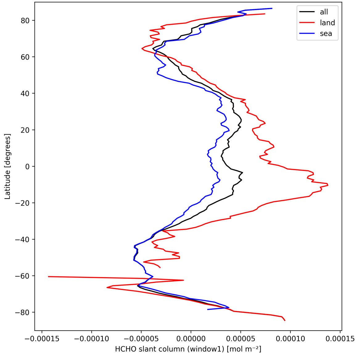
Figure 22: Zonal average of “HCHO slant column (window1)” for 2025-09-20 to 2025-09-21.
