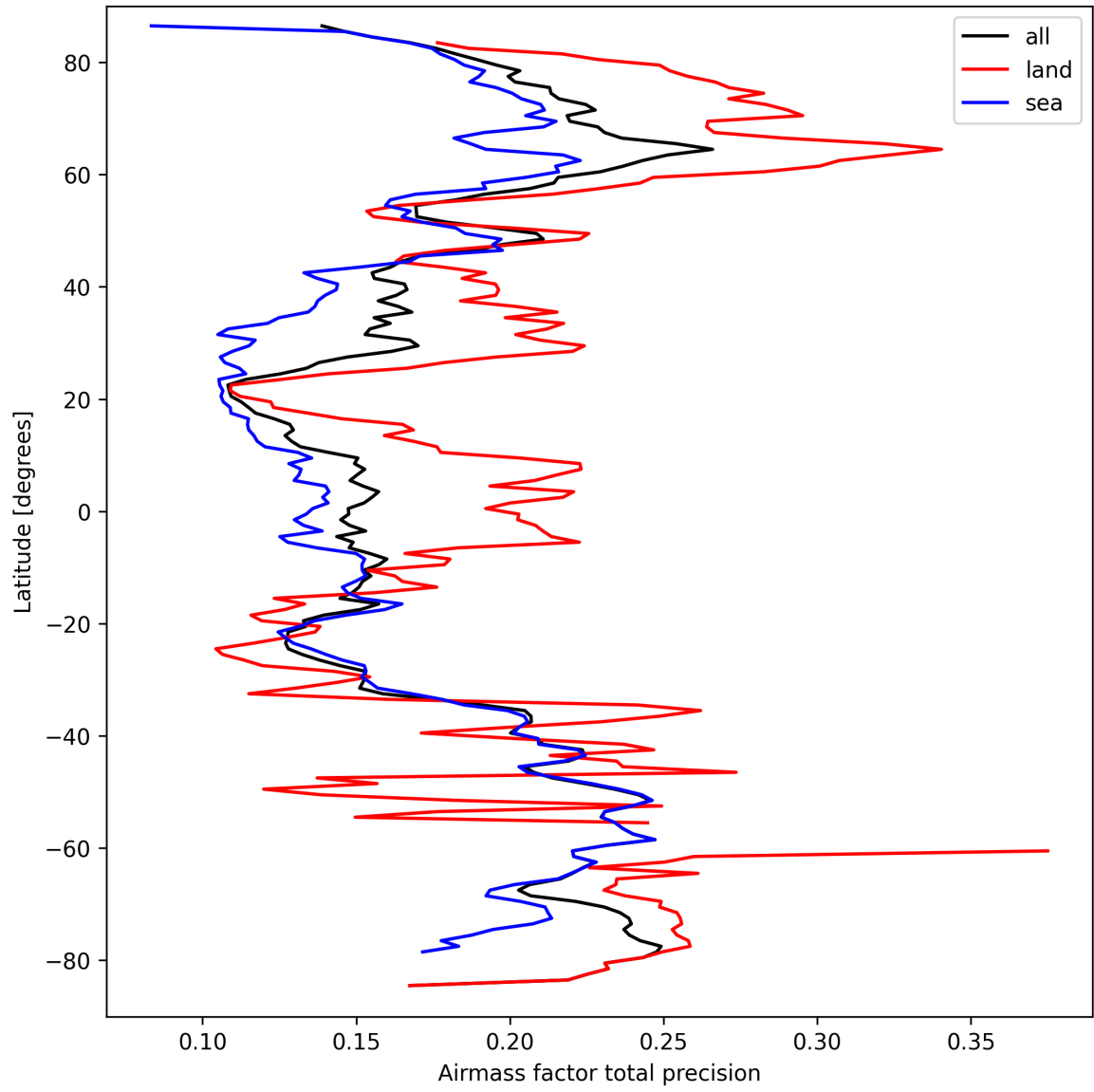
Figure 25: Zonal average of “Airmass factor total precision” for 2025-09-20 to 2025-09-21.
