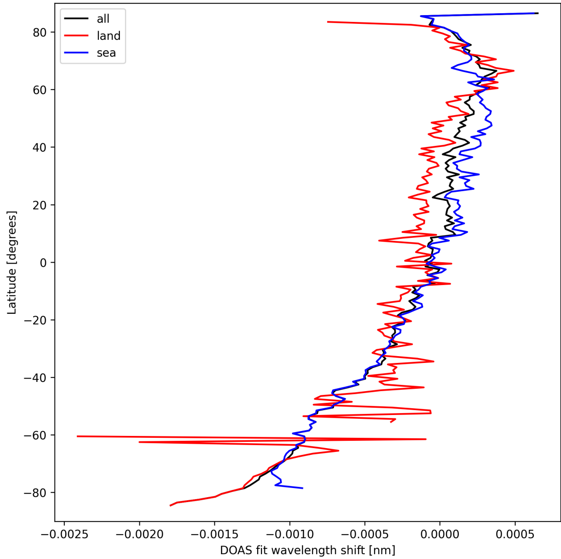
Figure 28: Zonal average of "DOAS fit wavelength shift" for 2025-09-20 to 2025-09-21.
