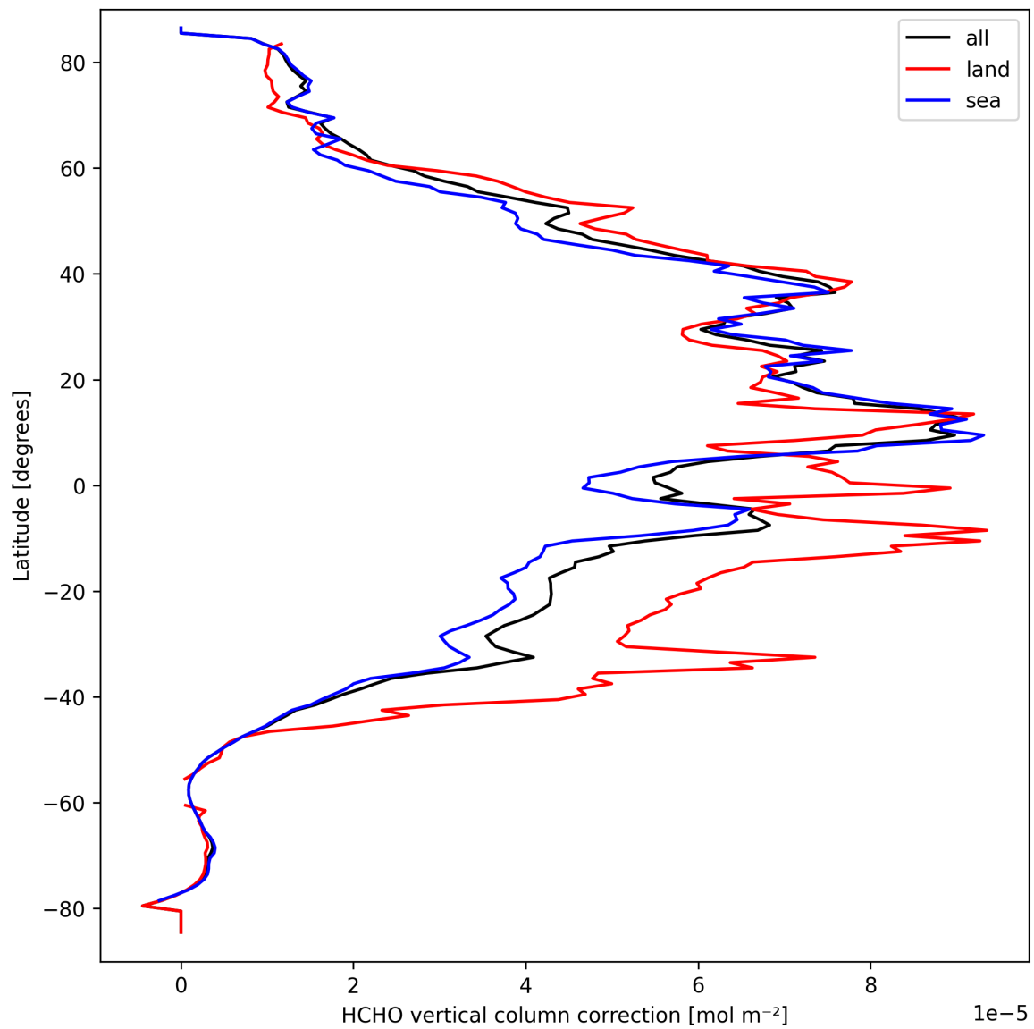
Figure 21: Zonal average of "HCHO vertical column correction" for 2025-09-20 to 2025-09-21.
