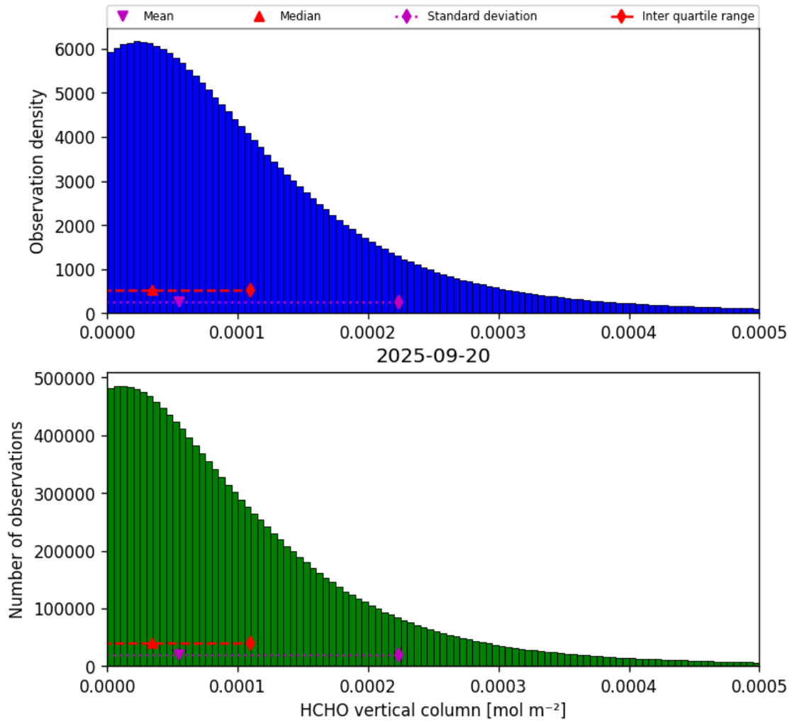
Figure 33: Histogram of “HCHO vertical column” for 2025-09-20 to 2025-09-21
