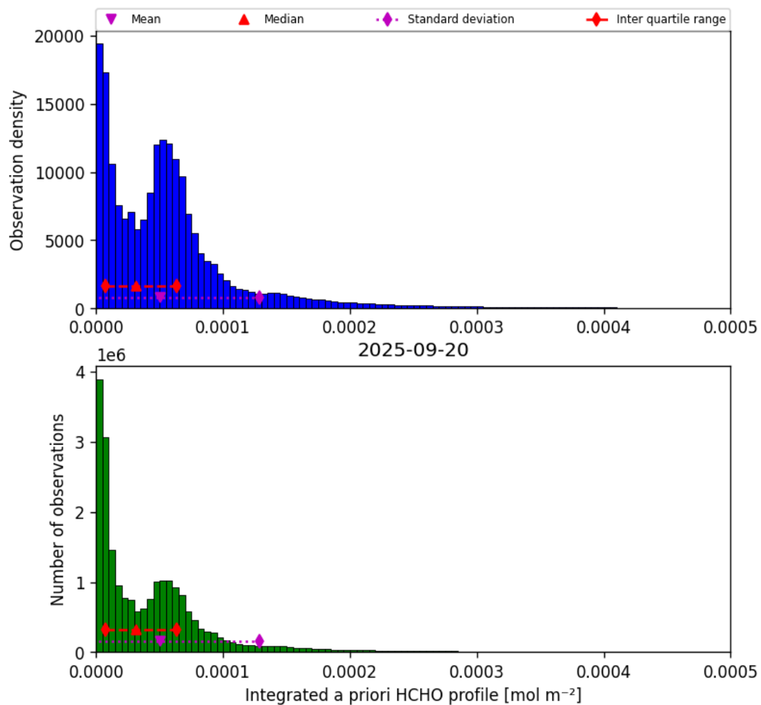
Figure 41: Histogram of “Integrated a priori HCHO profile” for 2025-09-20 to 2025-09-21
