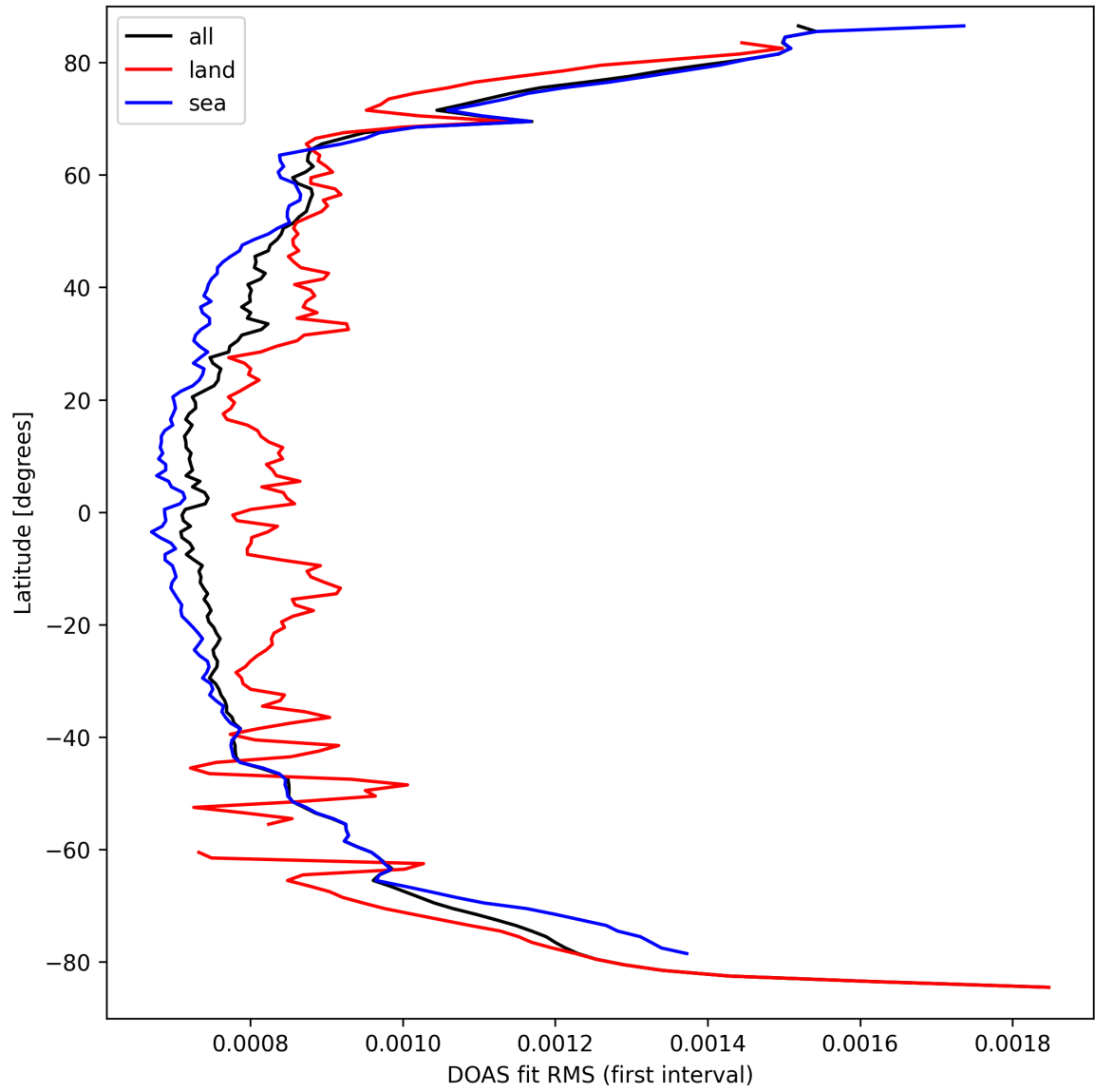
Figure 30: Zonal average of “DOAS fit RMS (first interval)” for 2025-09-20 to 2025-09-21.
