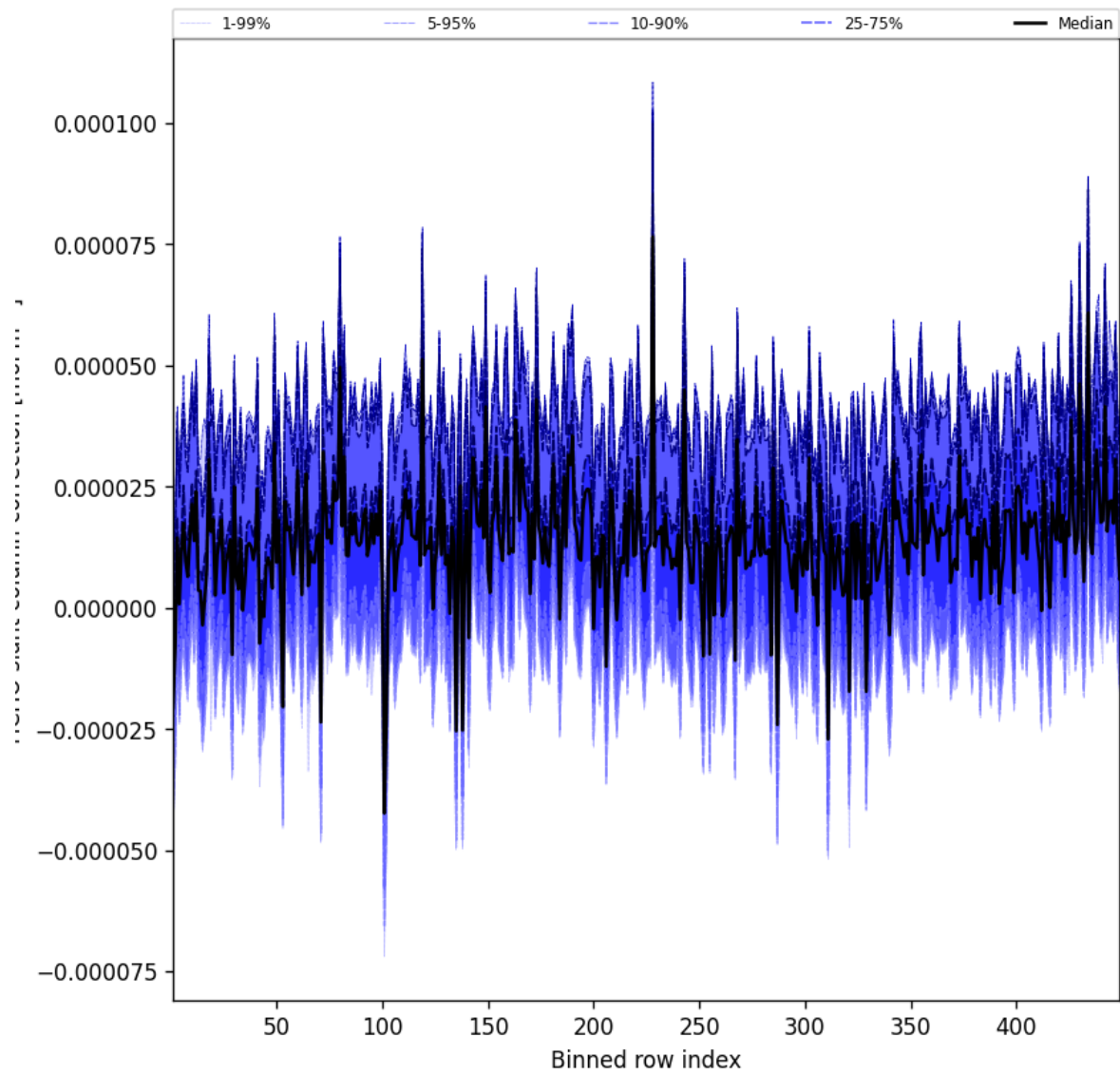
Figure 59: Along track statistics of “HCHO slant column correction” for 2025-09-20 to 2025-09-21
