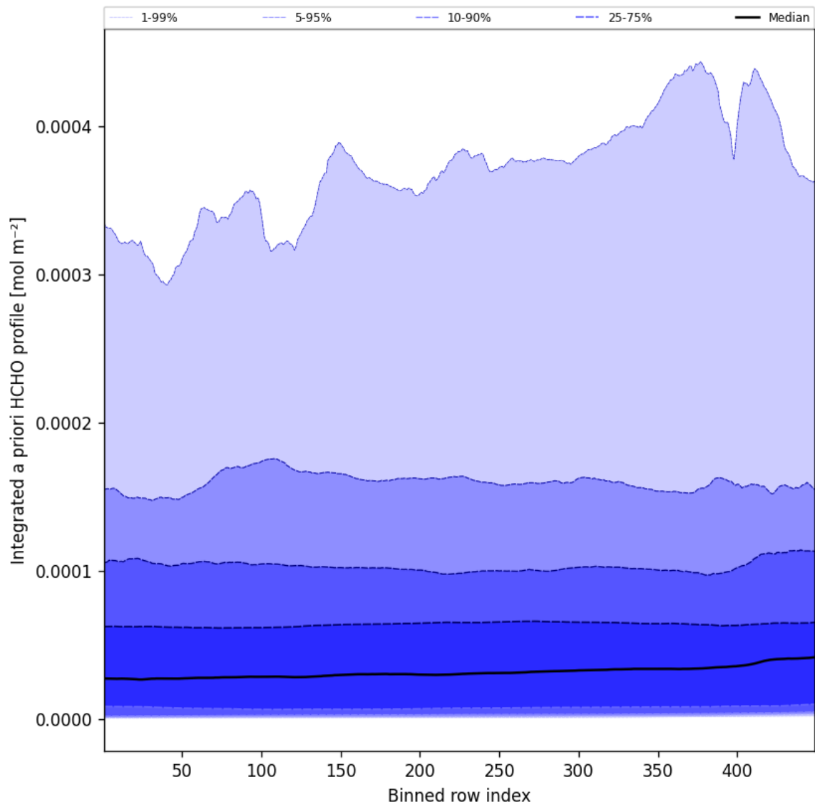
Figure 55: Along track statistics of “Integrated a priori HCHO profile” for 2025-09-20 to 2025-09-21
