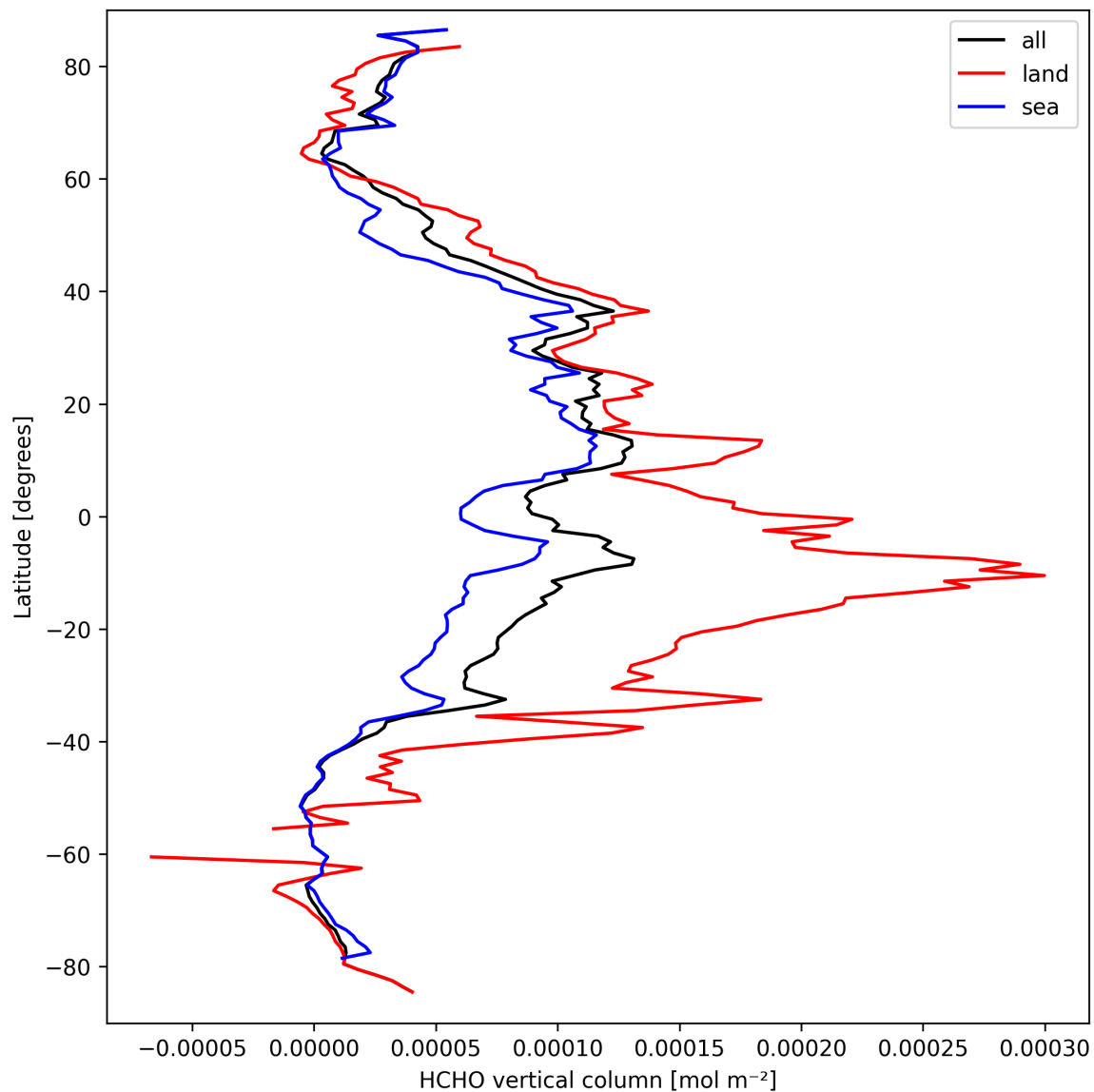
Figure 19: Zonal average of “HCHO vertical column” for 2025-09-20 to 2025-09-21.
