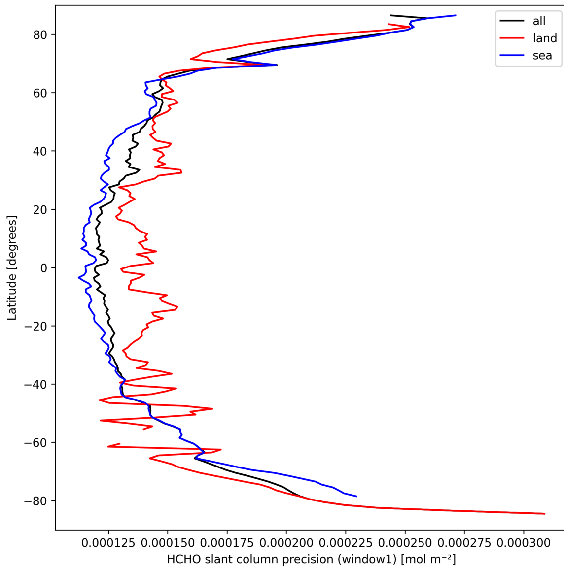
Figure 23: Zonal average of “HCHO slant column precision (window1)” for 2025-09-20 to 2025-09-21.
