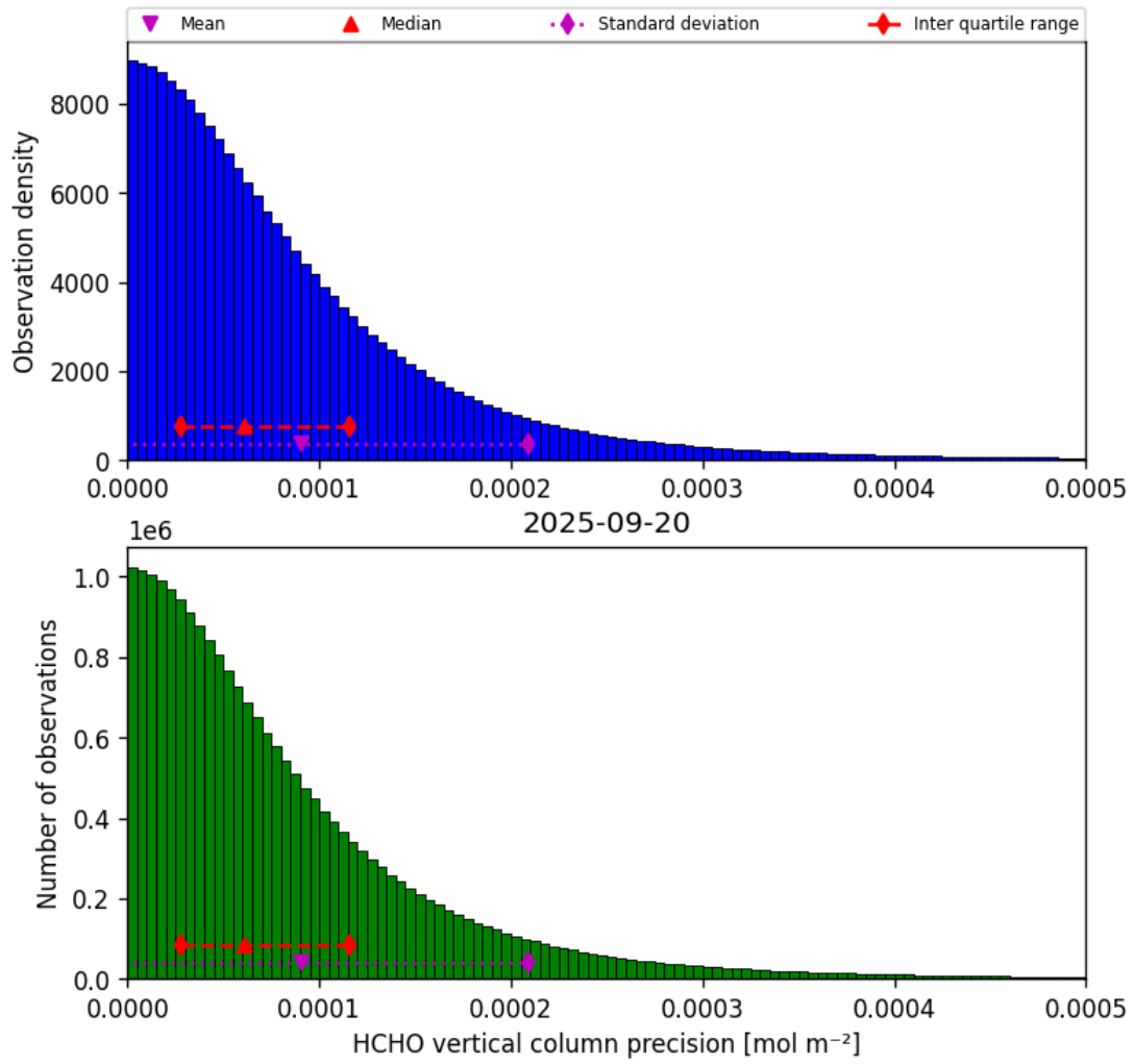
Figure 34: Histogram of “HCHO vertical column precision” for 2025-09-20 to 2025-09-21
