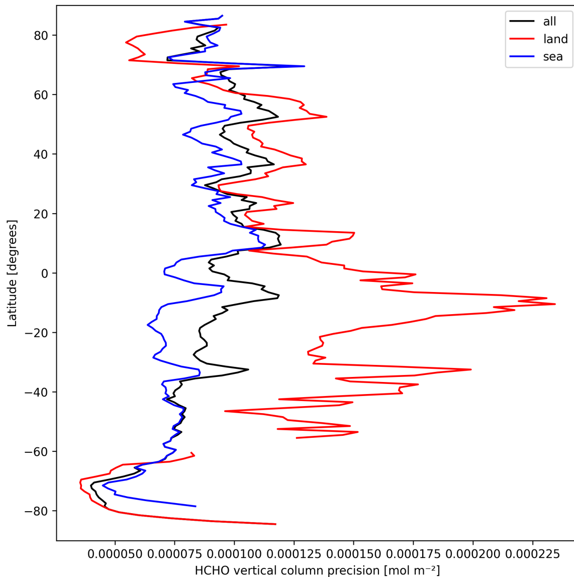
Figure 20: Zonal average of “HCHO vertical column precision” for 2025-09-20 to 2025-09-21.
