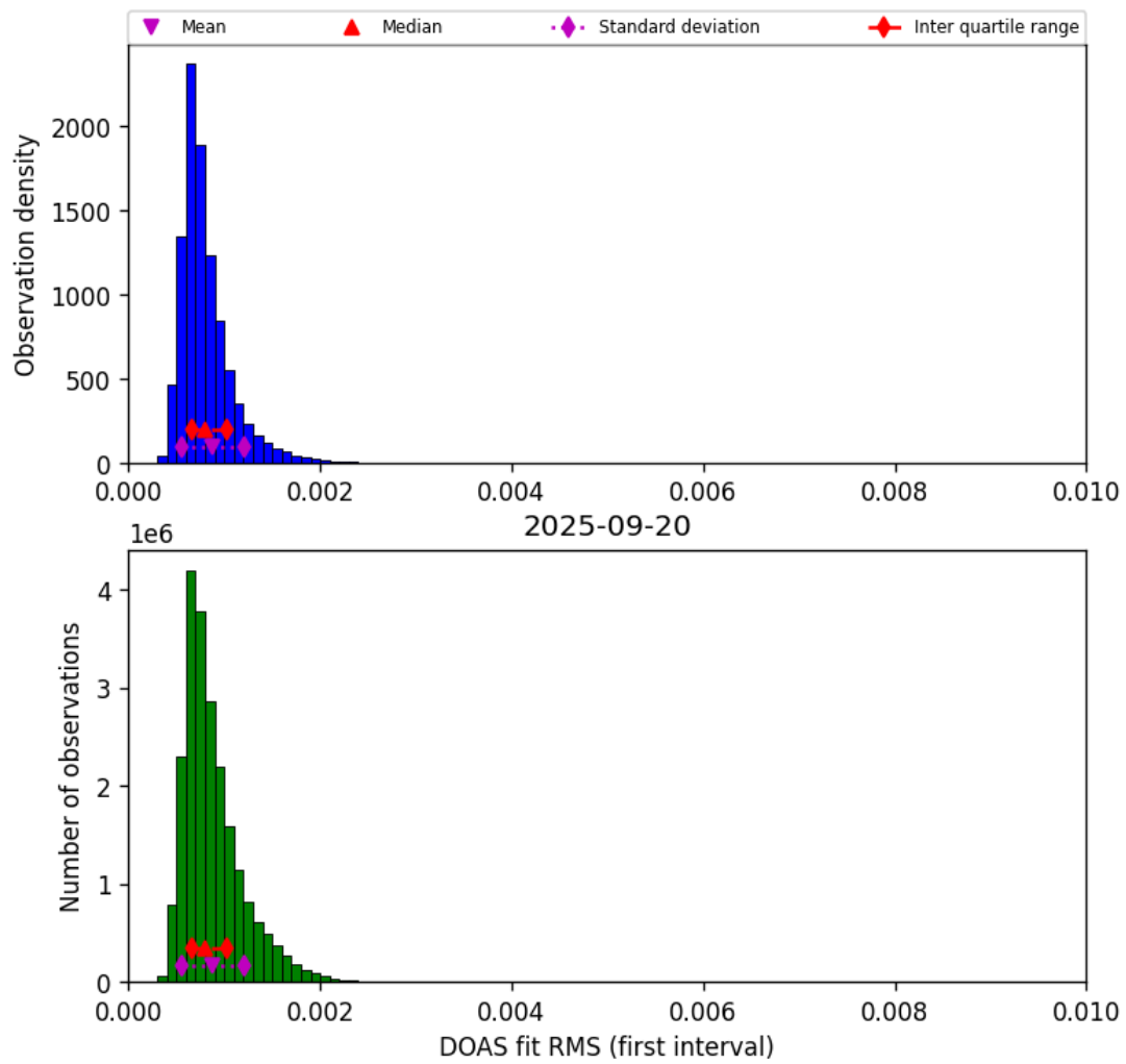
Figure 44: Histogram of “DOAS fit RMS (first interval)” for 2025-09-20 to 2025-09-21
