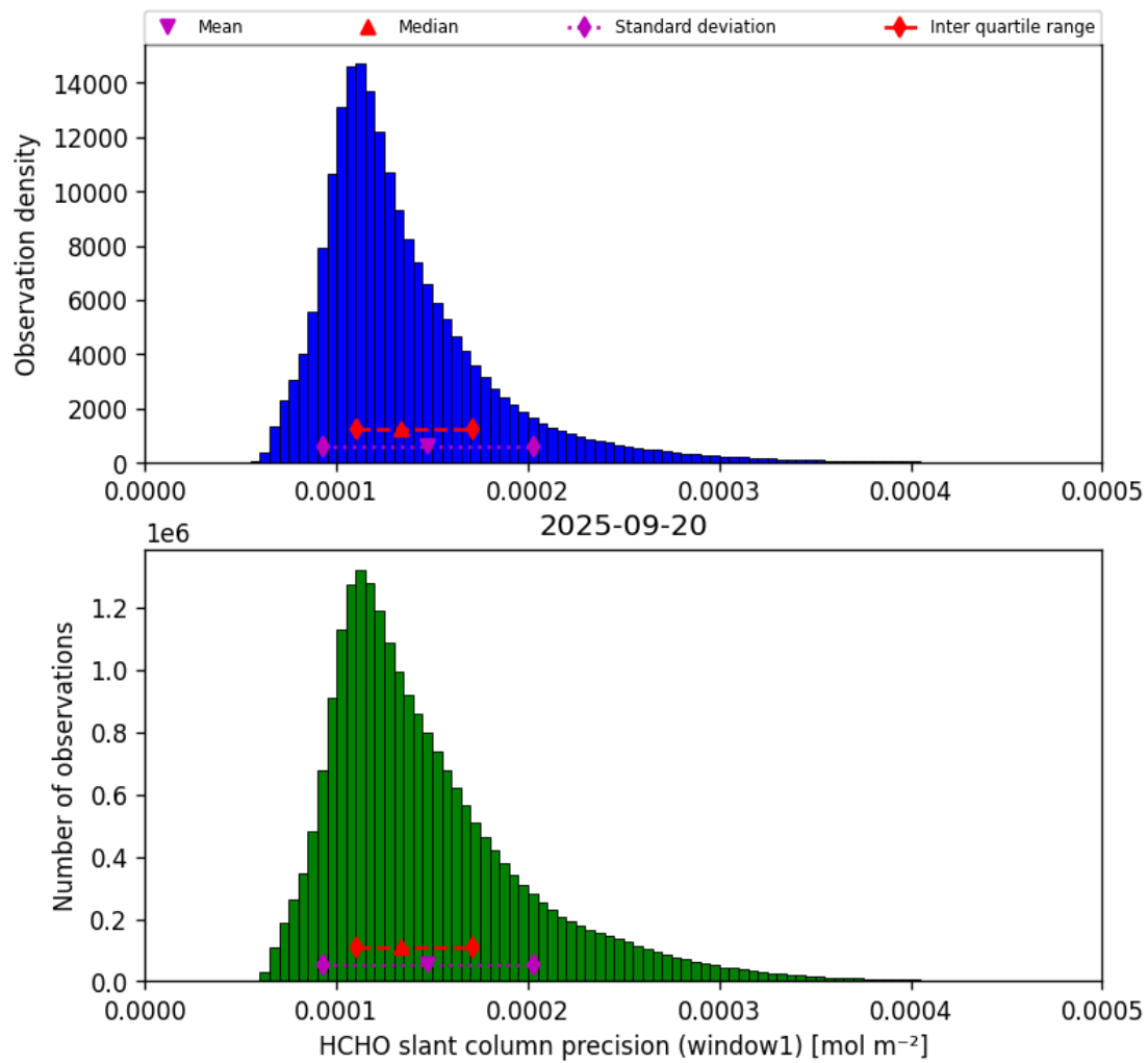
Figure 37: Histogram of “HCHO slant column precision (window1)” for 2025-09-20 to 2025-09-21
