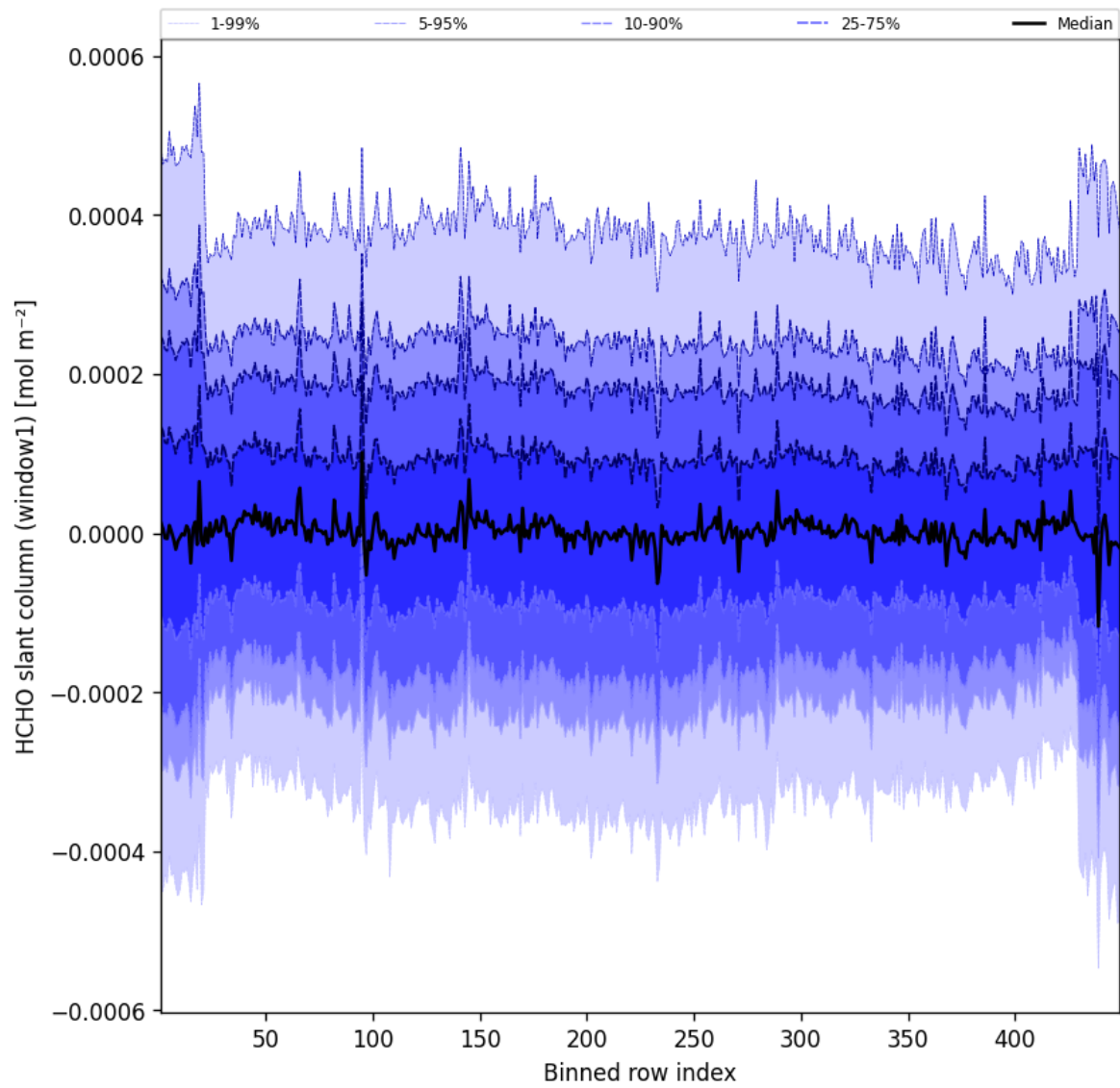
Figure 50: Along track statistics of “HCHO slant column (window1)” for 2025-09-20 to 2025-09-21
