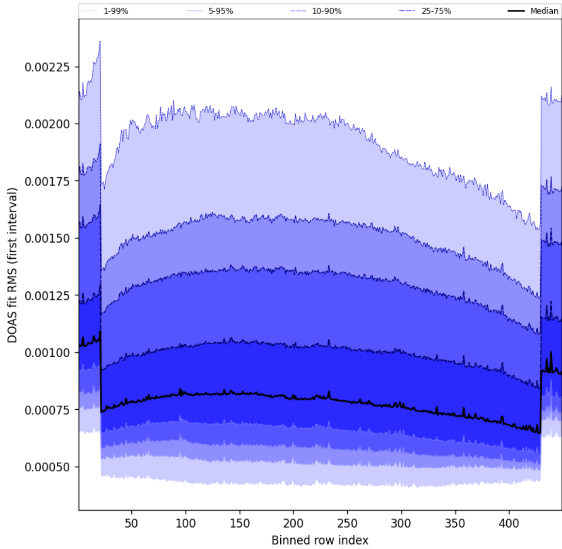
Figure 58: Along track statistics of “DOAS fit RMS (first interval)” for 2025-09-20 to 2025-09-21
