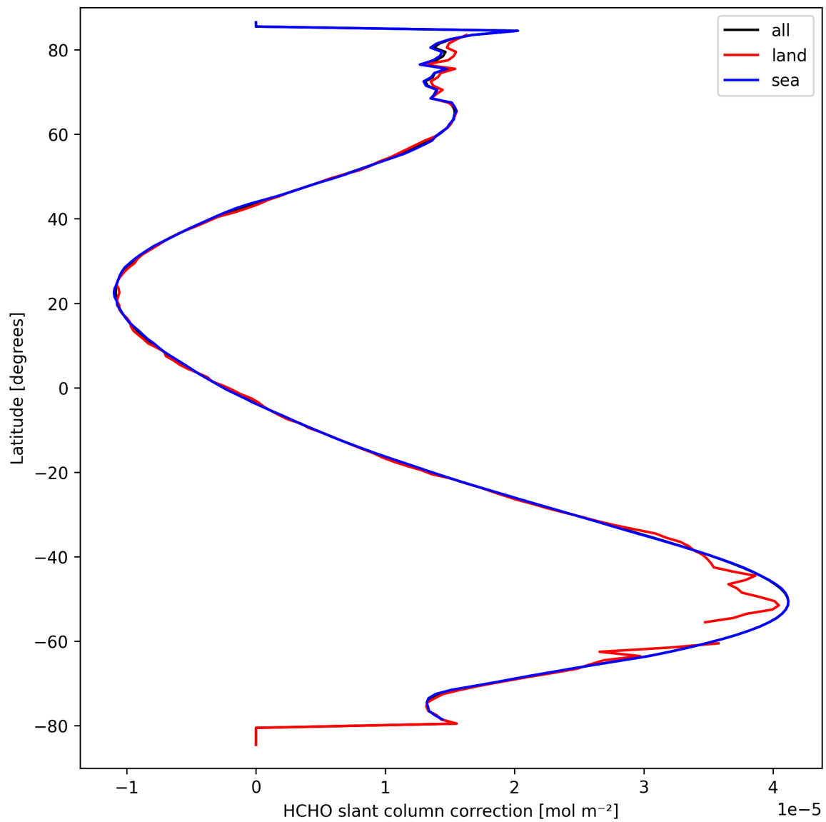
Figure 31: Zonal average of “HCHO slant column correction” for 2025-09-20 to 2025-09-21.
