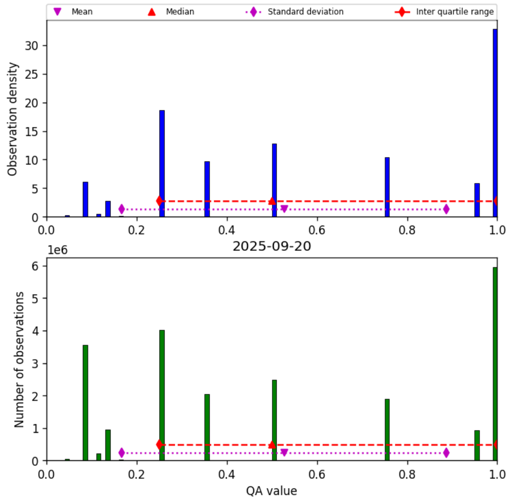
Figure 32: Histogram of “QA value” for 2025-09-20 to 2025-09-21
