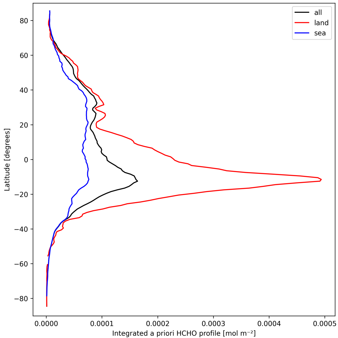
Figure 27: Zonal average of “Integrated a priori HCHO profile” for 2025-09-21 to 2025-09-22.
