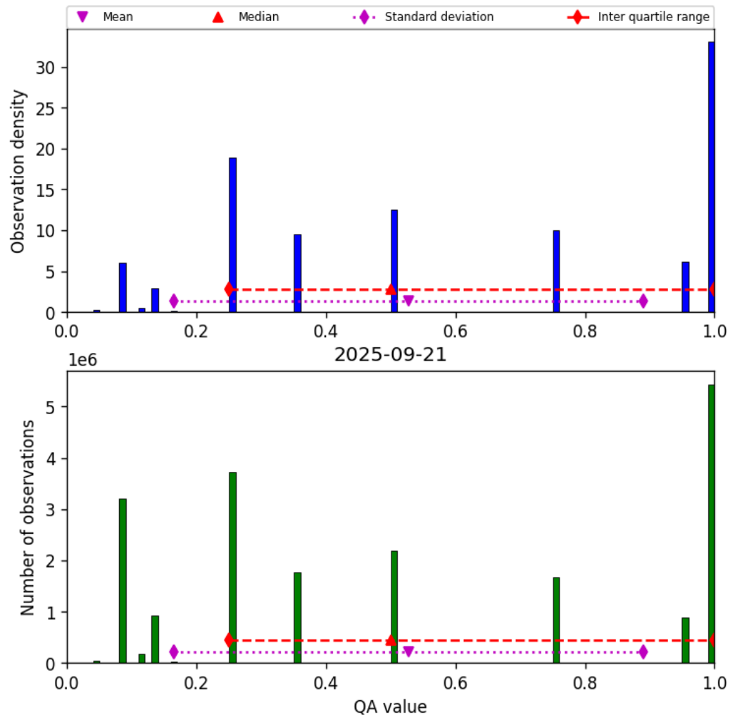
Figure 32: Histogram of “QA value” for 2025-09-21 to 2025-09-22
