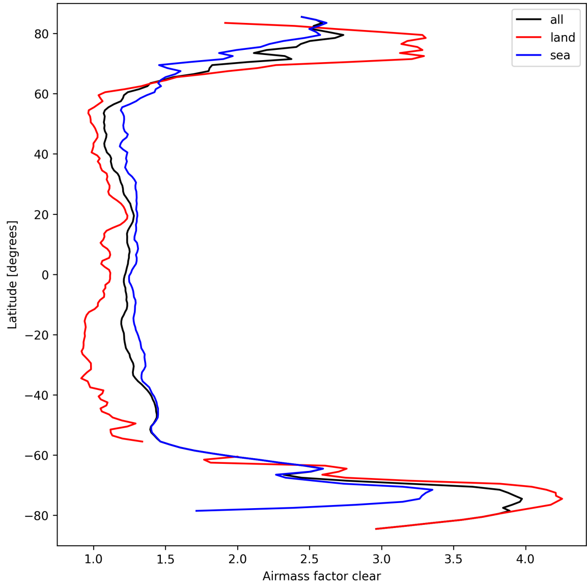
Figure 26: Zonal average of “Airmass factor clear” for 2025-09-21 to 2025-09-22.
