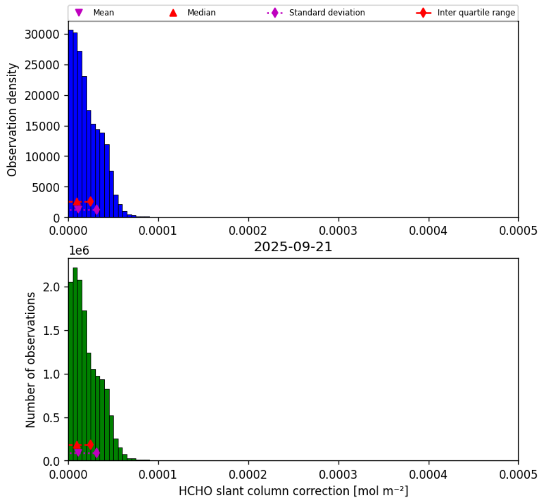
Figure 45: Histogram of “HCHO slant column correction” for 2025-09-21 to 2025-09-22
