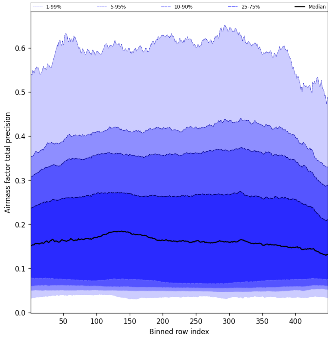
Figure 53: Along track statistics of “Airmass factor total precision” for 2025-09-21 to 2025-09-22
