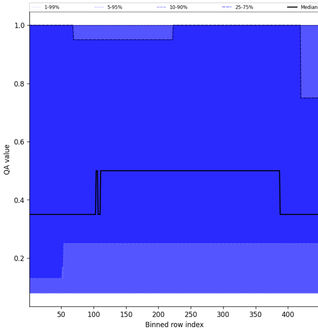
Figure 46: Along track statistics of “QA value” for 2025-09-21 to 2025-09-22
