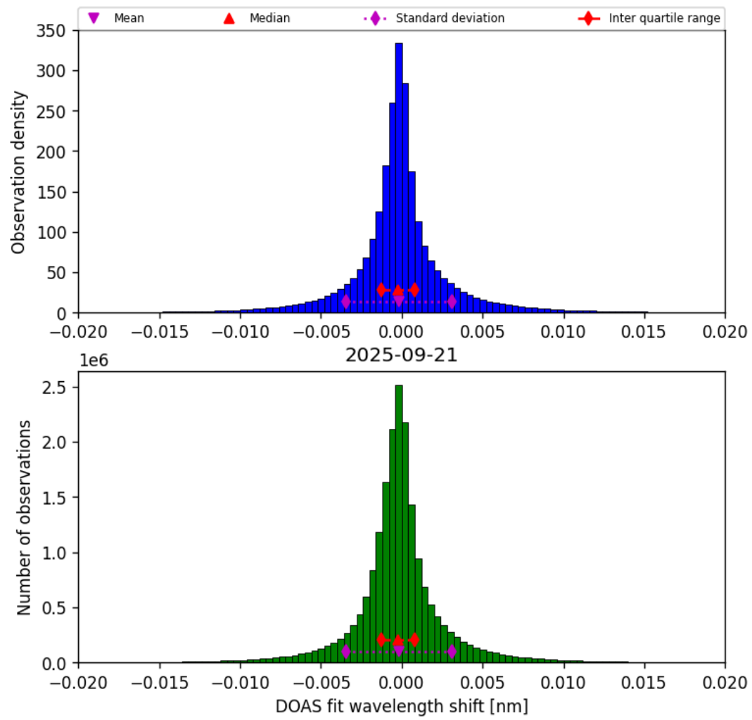
Figure 42: Histogram of “DOAS fit wavelength shift” for 2025-09-21 to 2025-09-22
