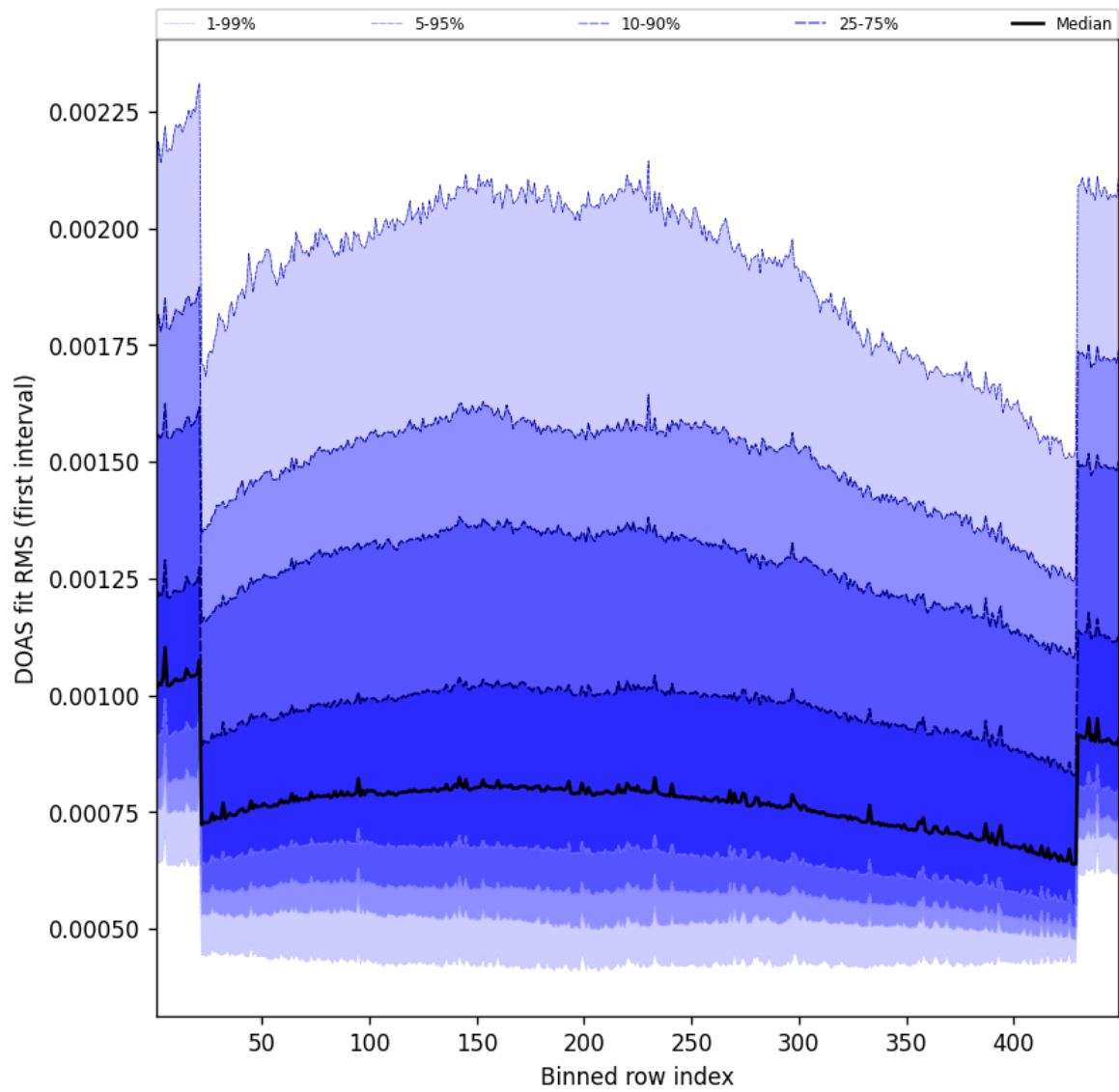
Figure 58: Along track statistics of “DOAS fit RMS (first interval)” for 2025-09-21 to 2025-09-22
