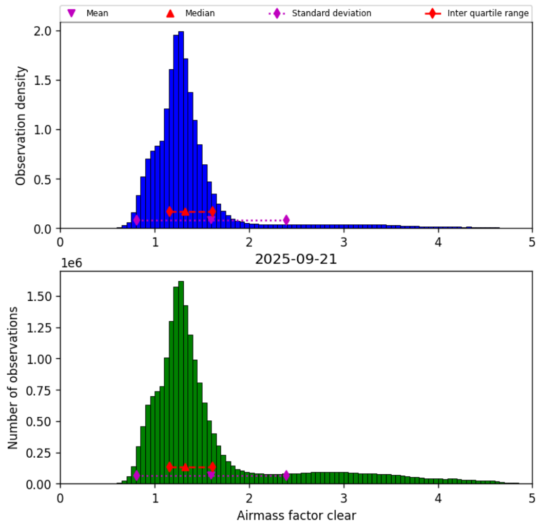
Figure 40: Histogram of “Airmass factor clear” for 2025-09-21 to 2025-09-22
