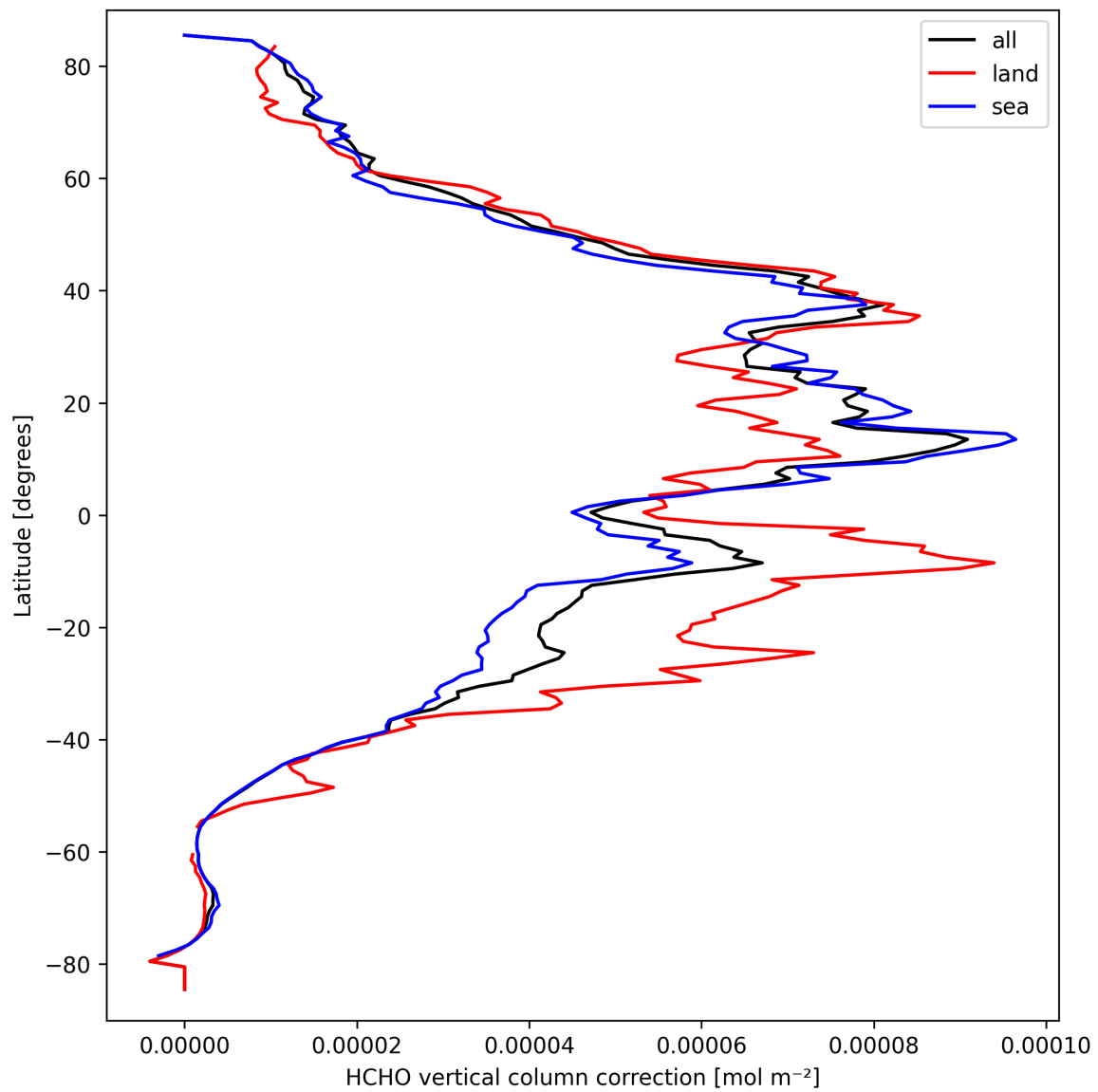
Figure 21: Zonal average of “HCHO vertical column correction” for 2025-09-21 to 2025-09-22.
