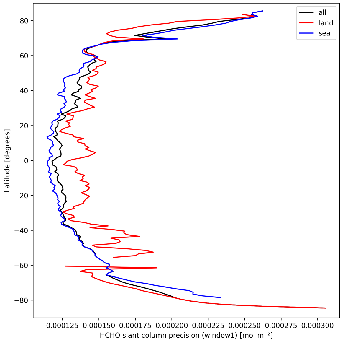
Figure 23: Zonal average of “HCHO slant column precision (window1)” for 2025-09-21 to 2025-09-22.
