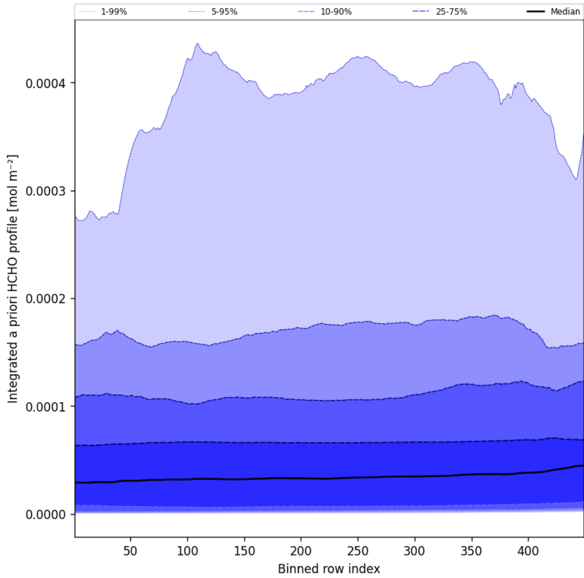
Figure 55: Along track statistics of “Integrated a priori HCHO profile” for 2025-09-21 to 2025-09-22
