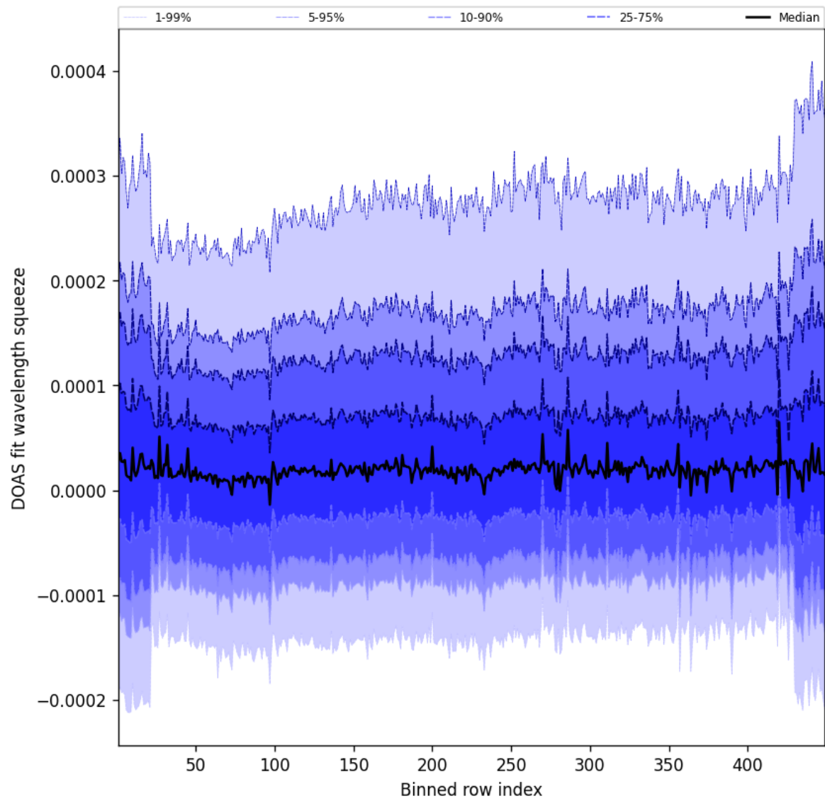
Figure 57: Along track statistics of “DOAS fit wavelength squeeze” for 2025-09-21 to 2025-09-22
