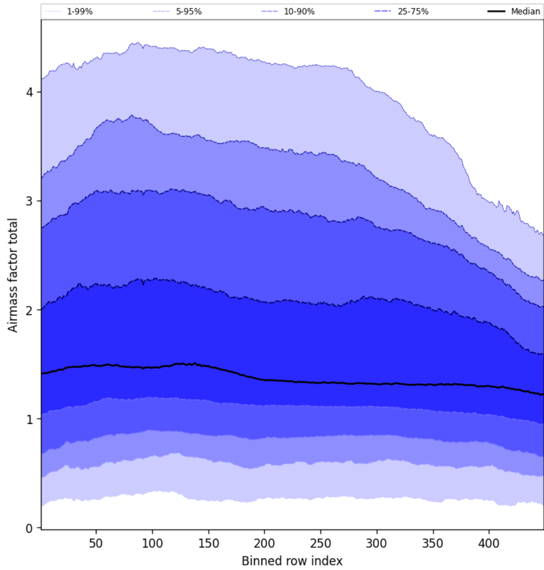
Figure 52: Along track statistics of “Airmass factor total” for 2025-09-21 to 2025-09-22
