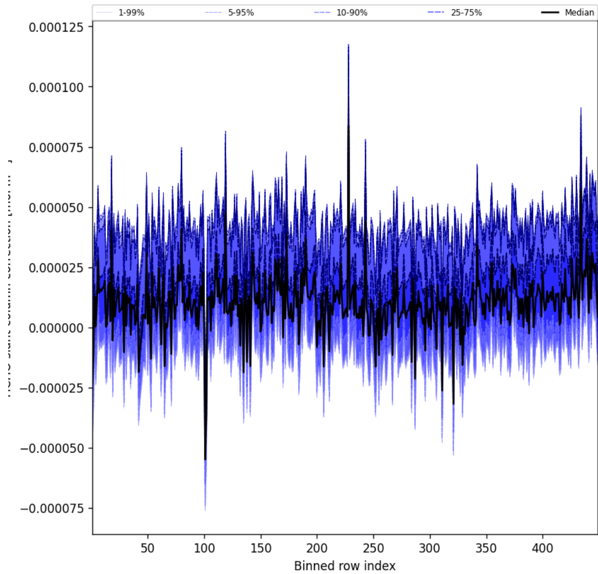
Figure 59: Along track statistics of “HCHO slant column correction” for 2025-09-21 to 2025-09-22
