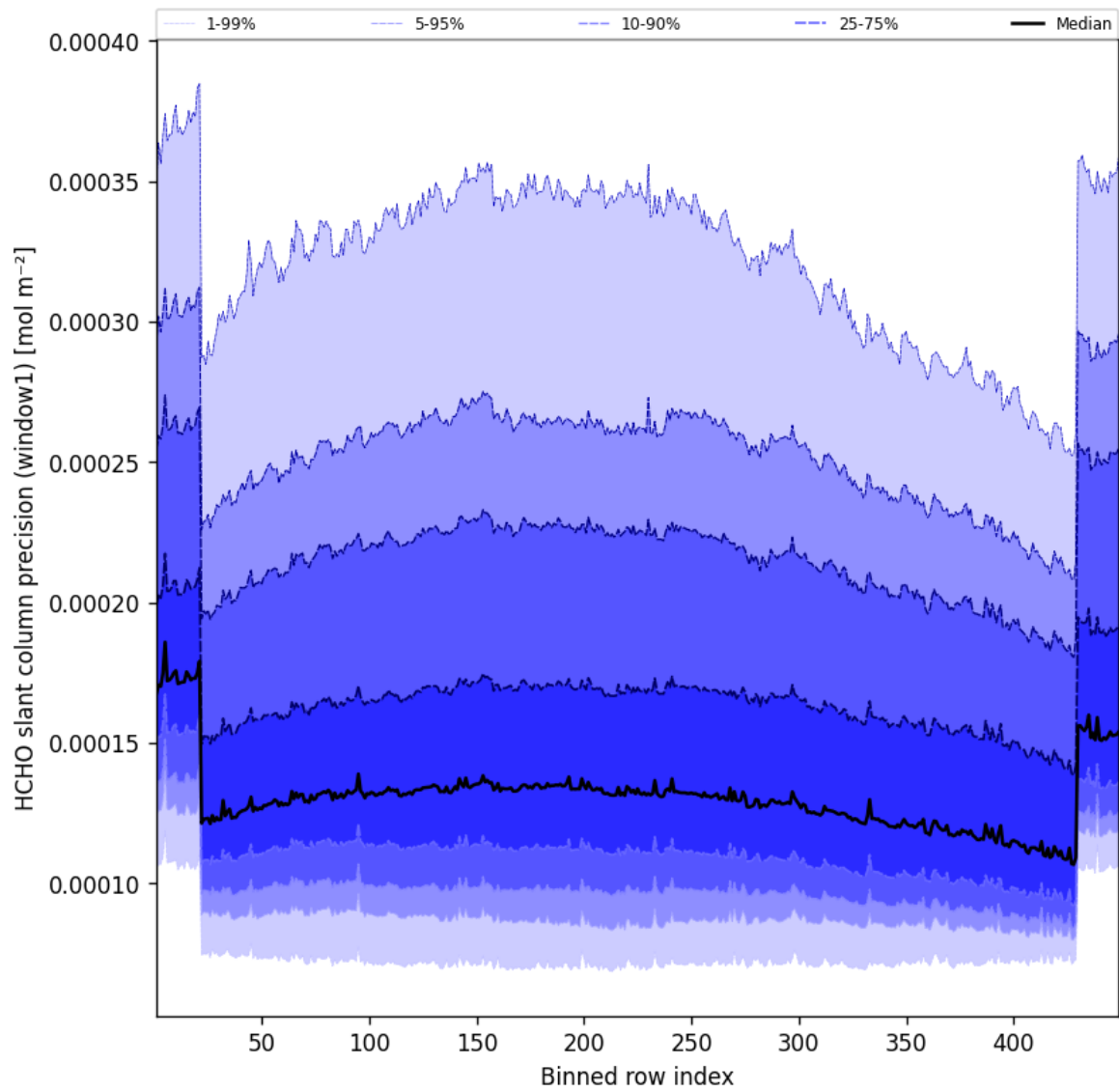
Figure 51: Along track statistics of “HCHO slant column precision (window1)” for 2025-09-21 to 2025-09-22
