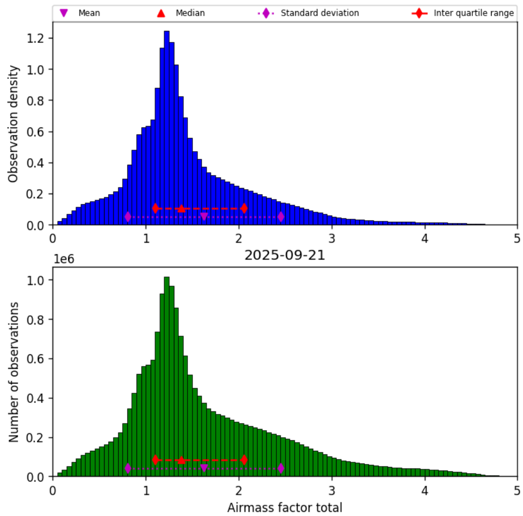
Figure 38: Histogram of “Airmass factor total” for 2025-09-21 to 2025-09-22
