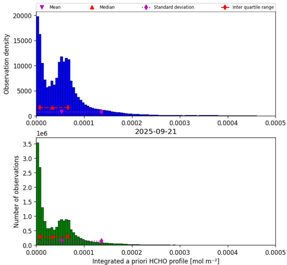
Figure 41: Histogram of “Integrated a priori HCHO profile” for 2025-09-21 to 2025-09-22
