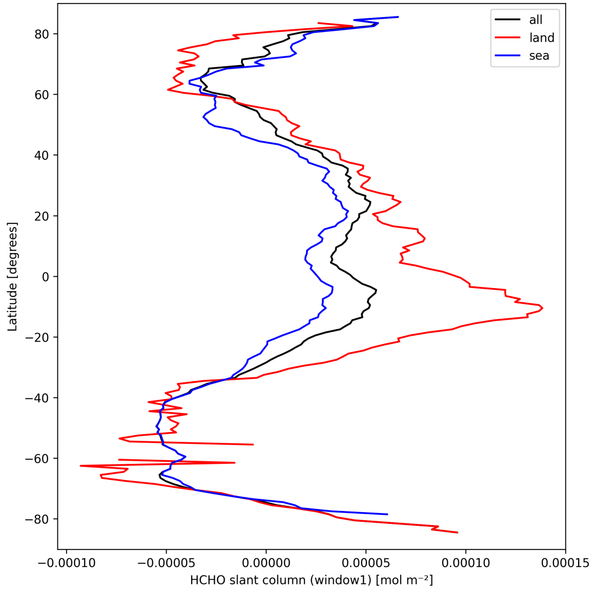
Figure 22: Zonal average of “HCHO slant column (window1)” for 2025-09-21 to 2025-09-22.
