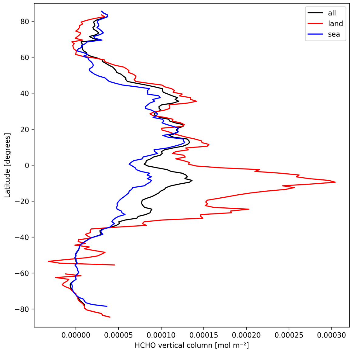
Figure 19: Zonal average of “HCHO vertical column” for 2025-09-21 to 2025-09-22.
