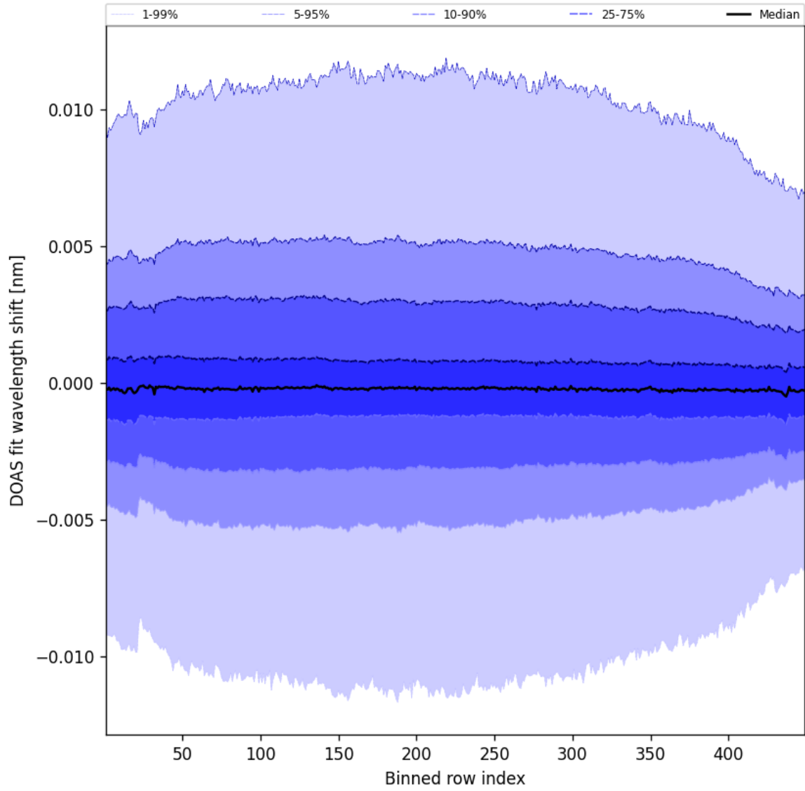
Figure 56: Along track statistics of “DOAS fit wavelength shift” for 2025-09-21 to 2025-09-22
