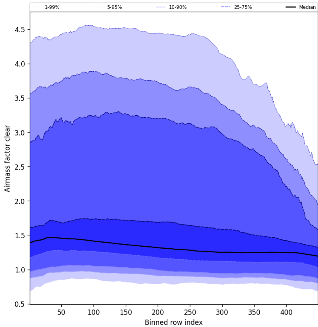
Figure 54: Along track statistics of “Air mass factor clear” for 2025-09-21 to 2025-09-22
