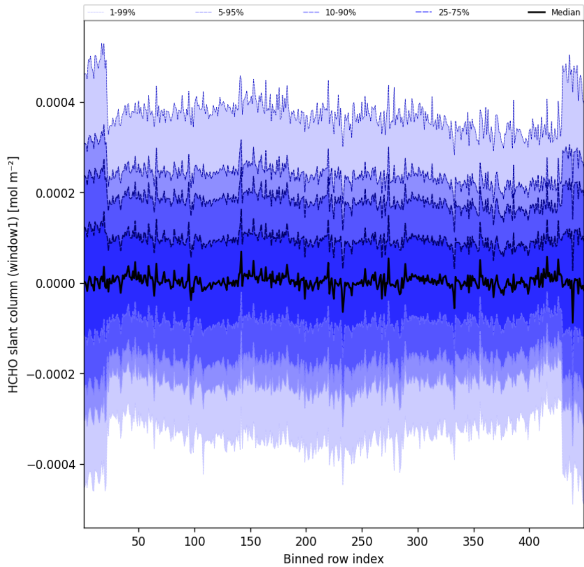
Figure 50: Along track statistics of “HCHO slant column (window1)” for 2025-09-21 to 2025-09-22
