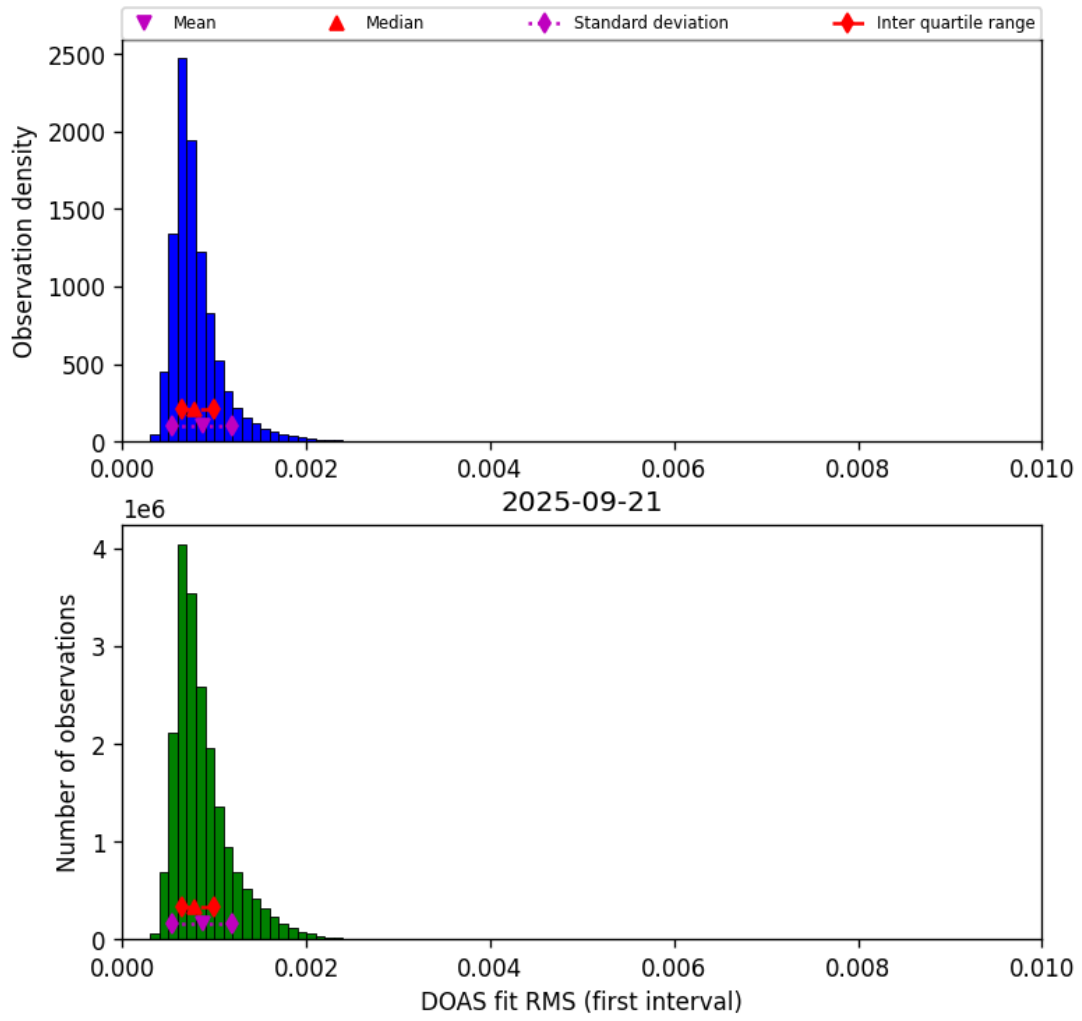
Figure 44: Histogram of “DOAS fit RMS (first interval)” for 2025-09-21 to 2025-09-22
