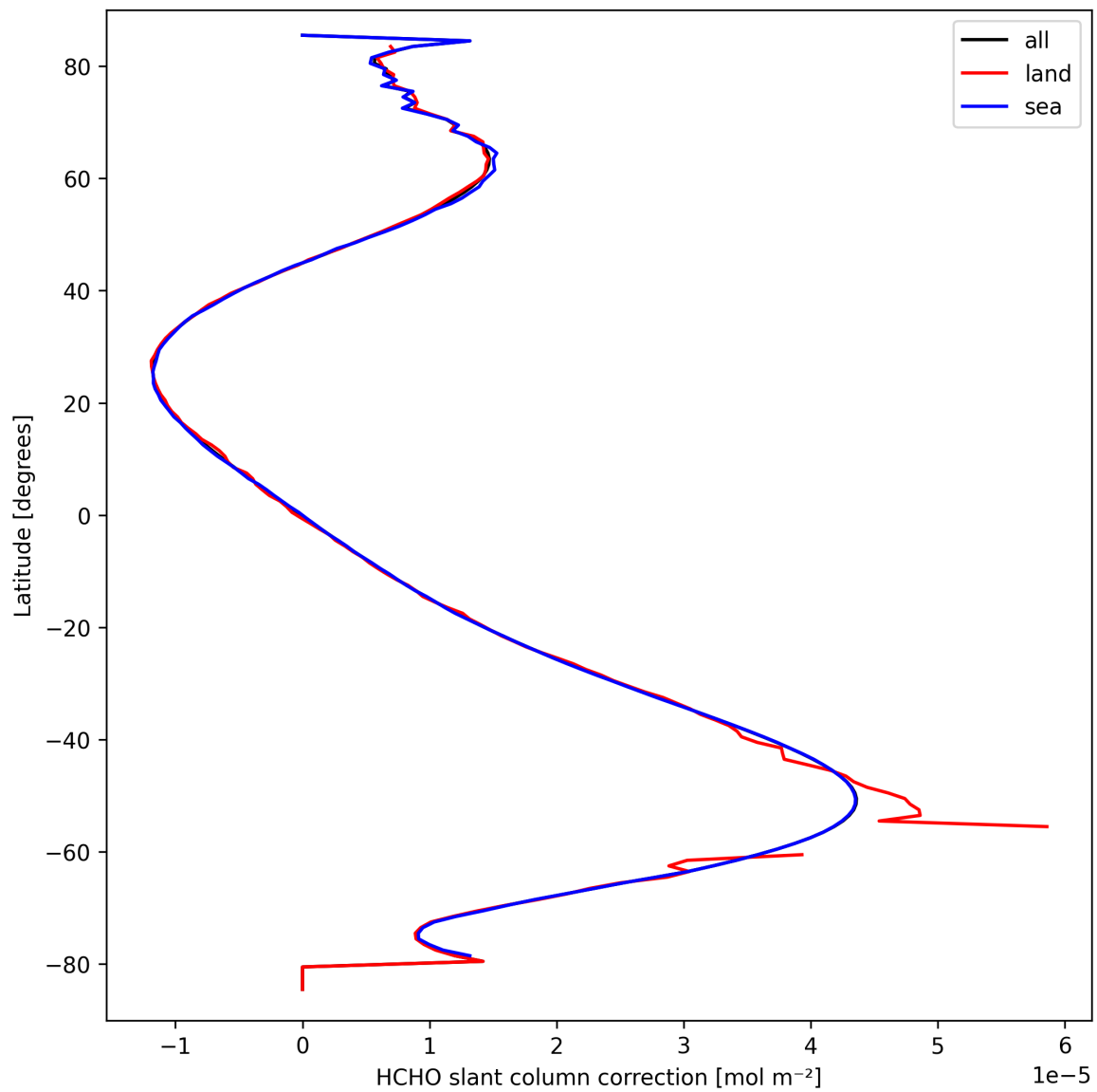
Figure 31: Zonal average of “HCHO slant column correction” for 2025-09-21 to 2025-09-22.
