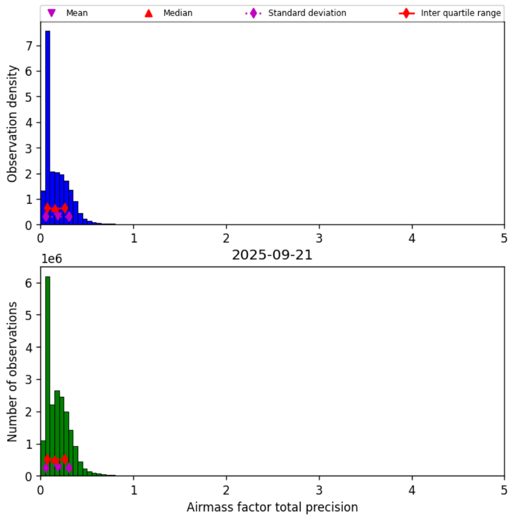
Figure 39: Histogram of “Airmass factor total precision” for 2025-09-21 to 2025-09-22
