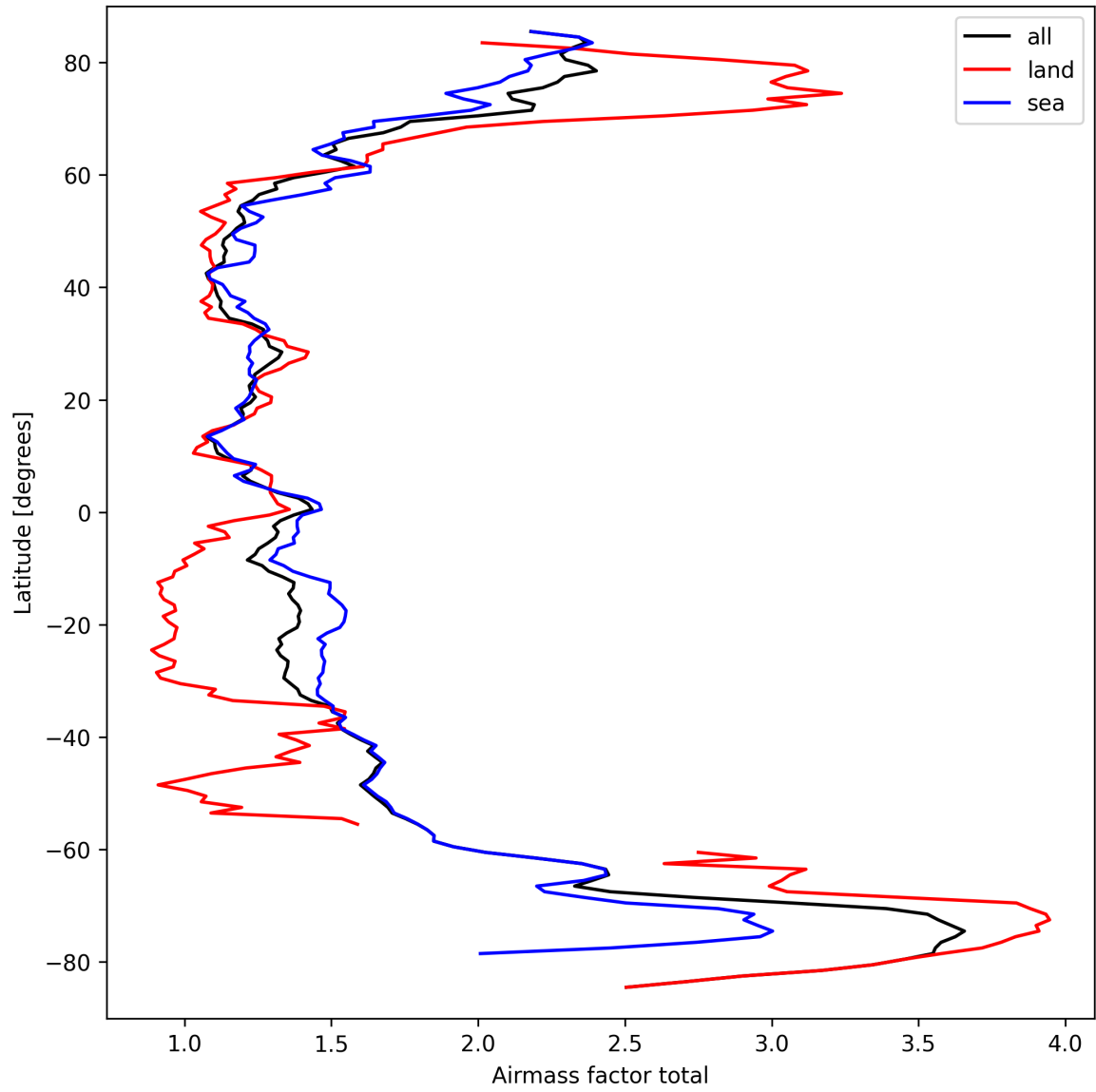
Figure 24: Zonal average of “Airmass factor total” for 2025-09-21 to 2025-09-22.
