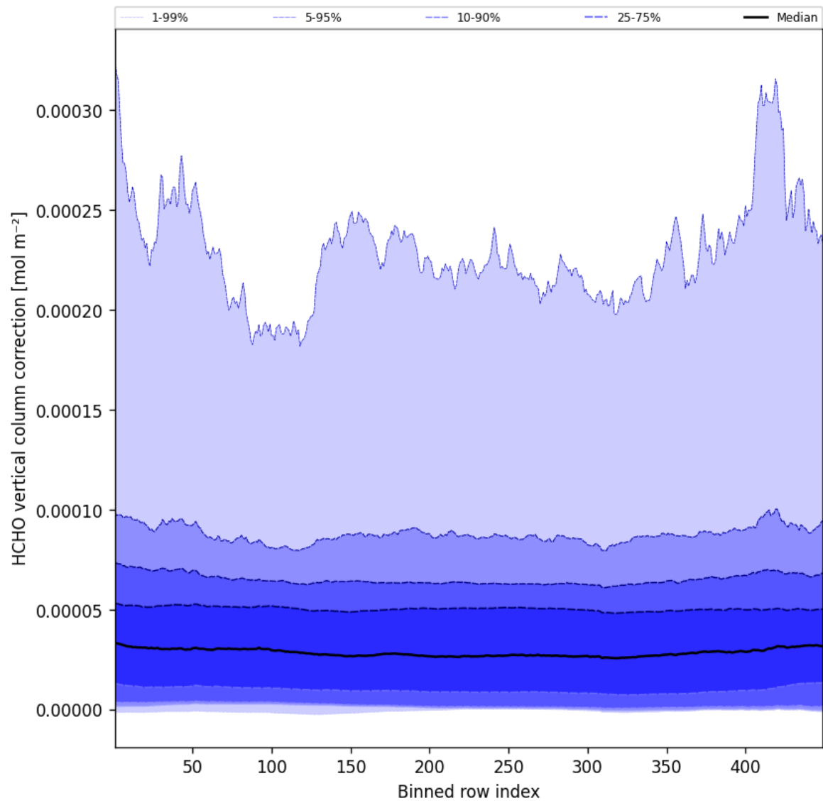
Figure 49: Along track statistics of “HCHO vertical column correction” for 2025-09-21 to 2025-09-22
