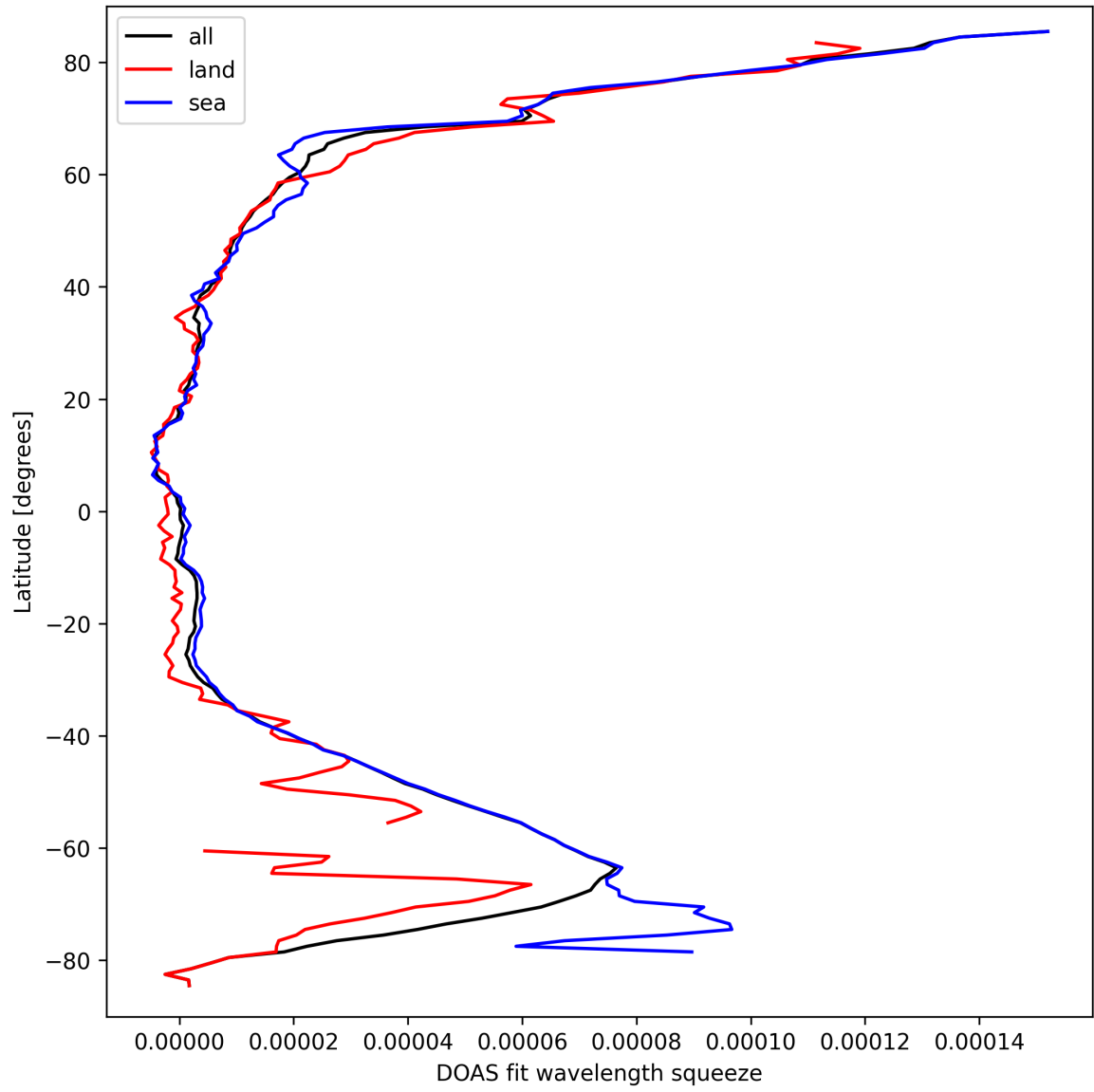
Figure 29: Zonal average of “DOAS fit wavelength squeeze” for 2025-09-21 to 2025-09-22.
