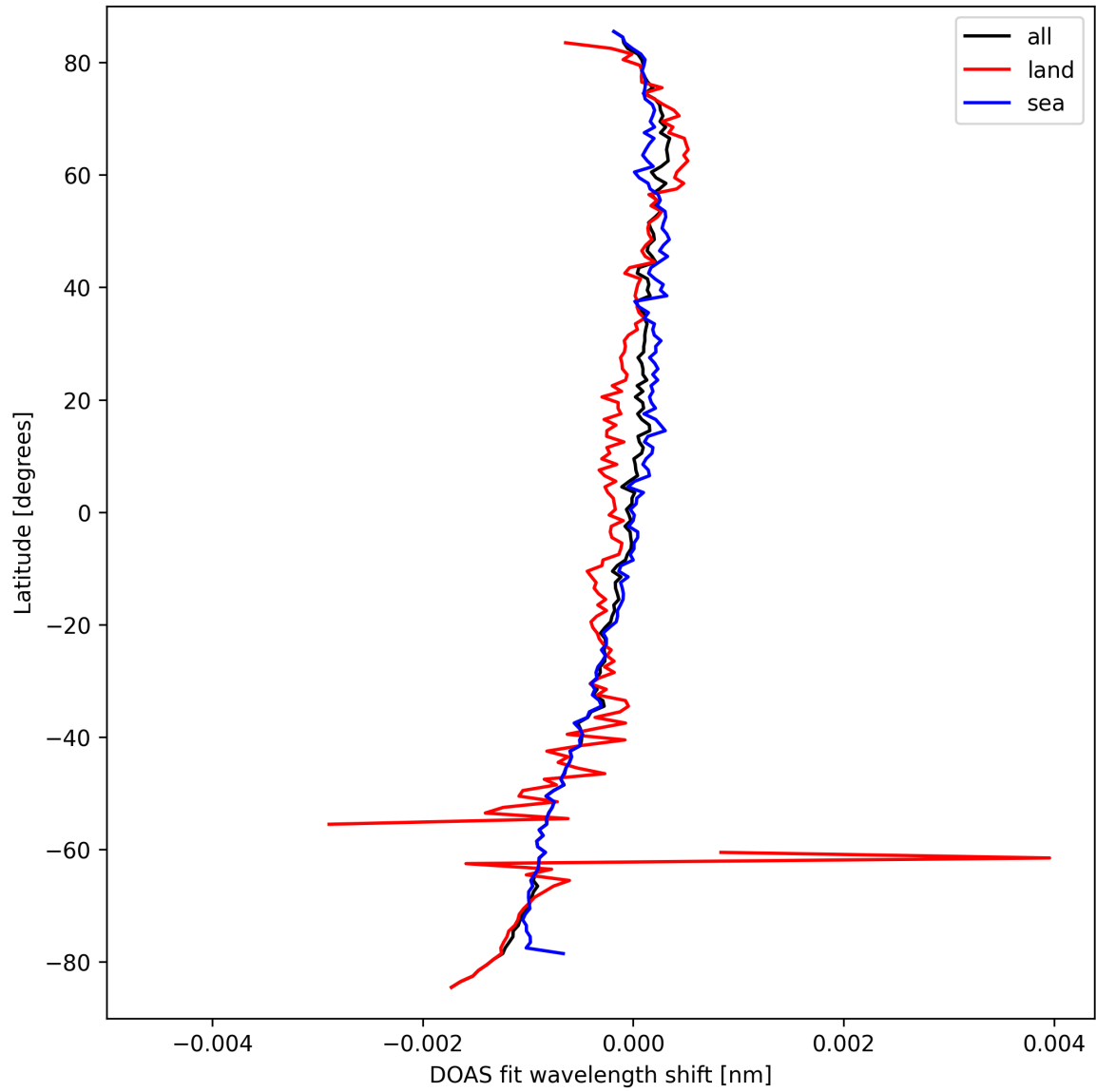
Figure 28: Zonal average of “DOAS fit wavelength shift” for 2025-09-21 to 2025-09-22.
