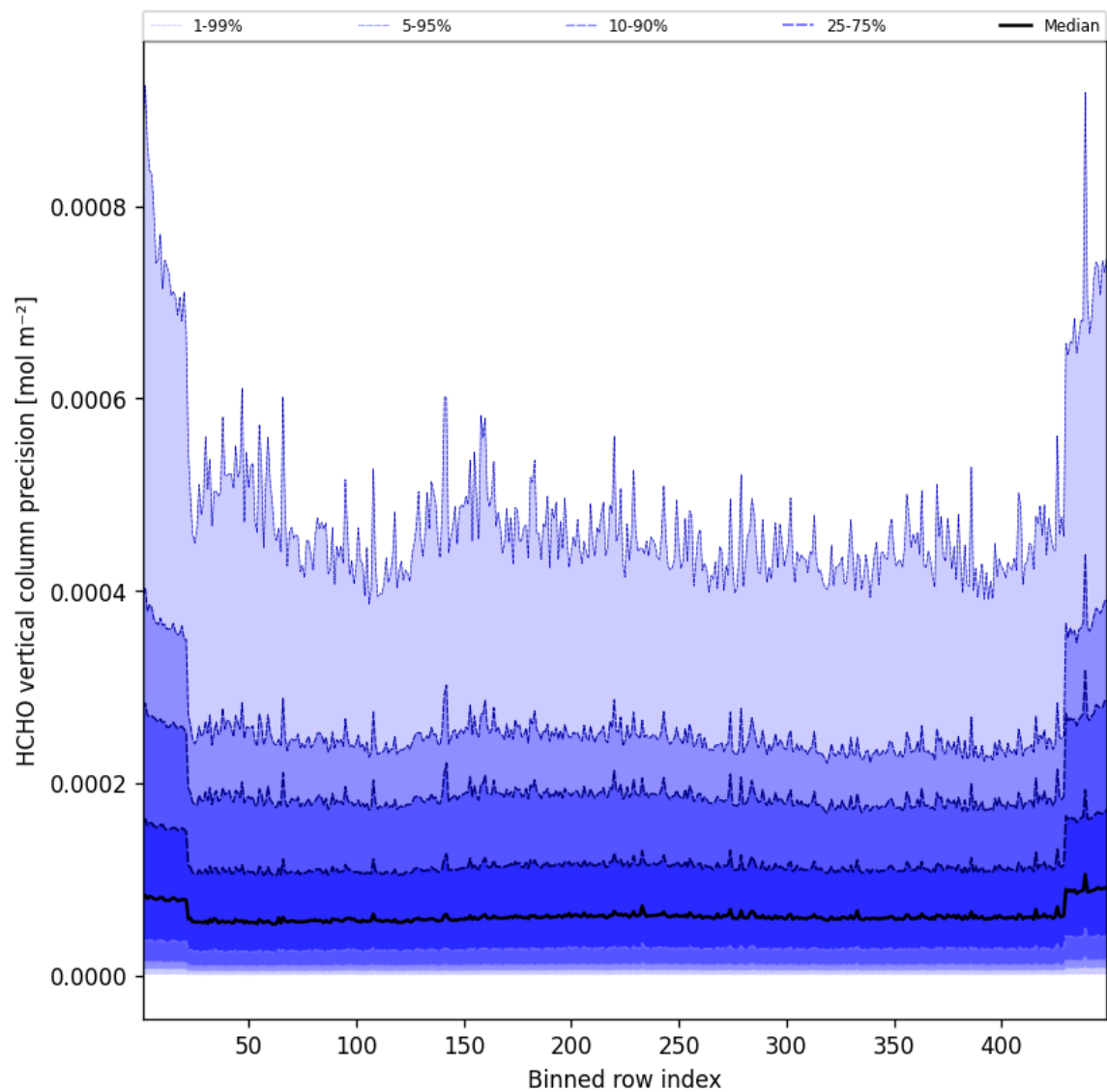
Figure 48: Along track statistics of “HCHO vertical column precision” for 2025-09-21 to 2025-09-22
