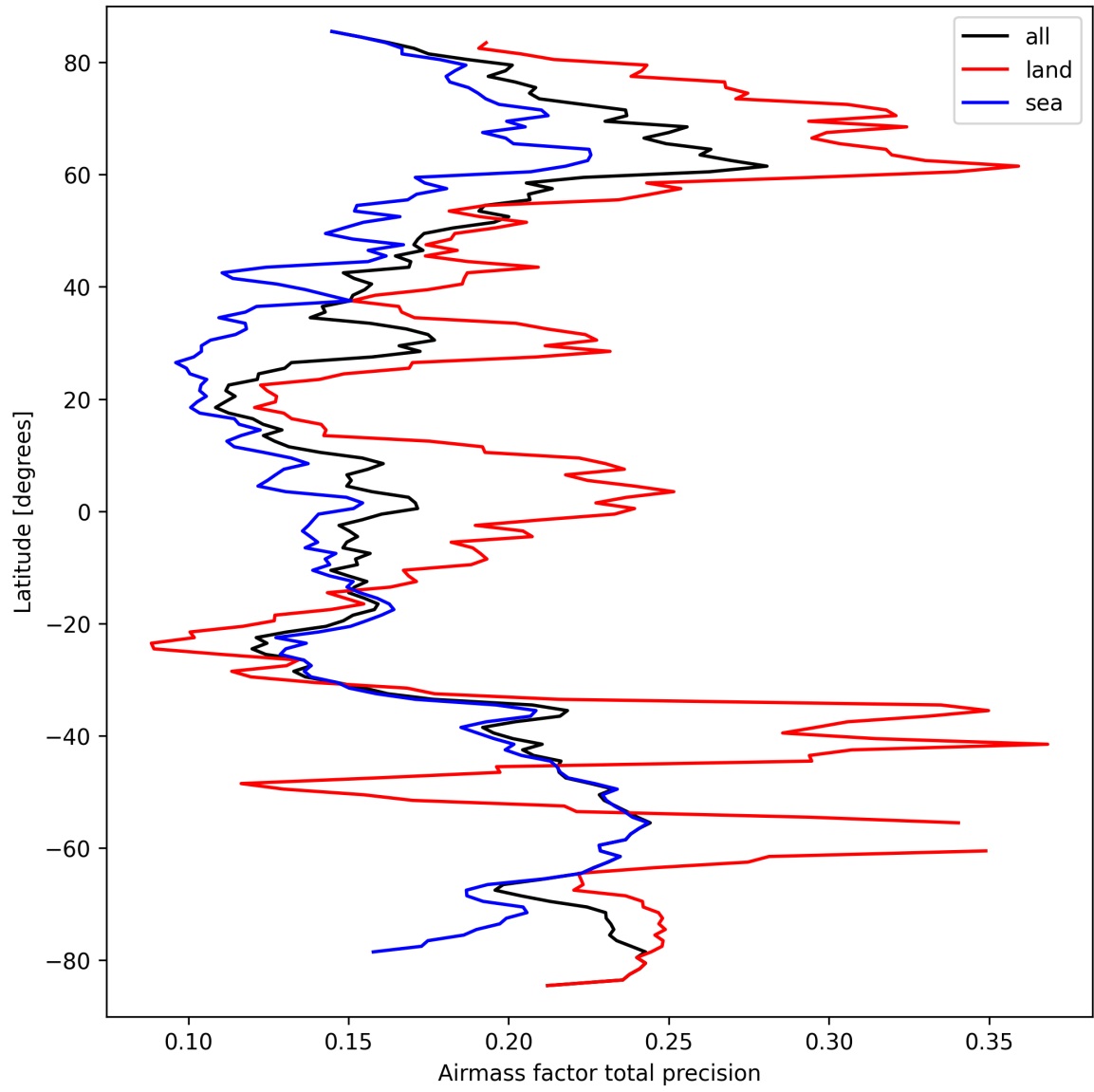
Figure 25: Zonal average of “Airmass factor total precision” for 2025-09-21 to 2025-09-22.
