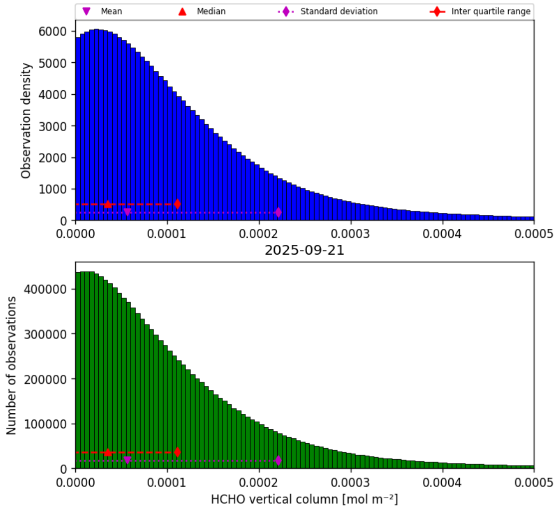
Figure 33: Histogram of “HCHO vertical column” for 2025-09-21 to 2025-09-22
