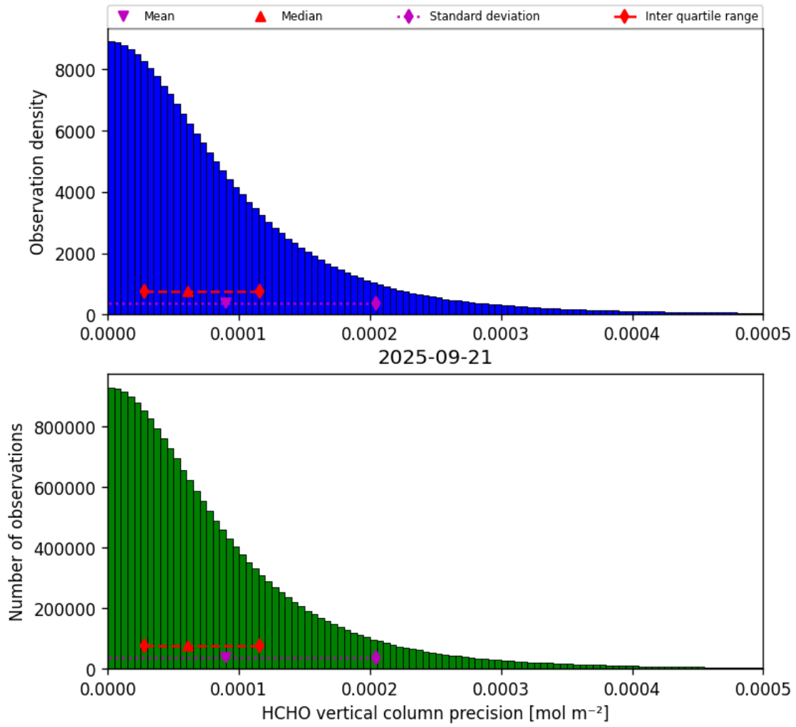
Figure 34: Histogram of “HCHO vertical column precision” for 2025-09-21 to 2025-09-22
