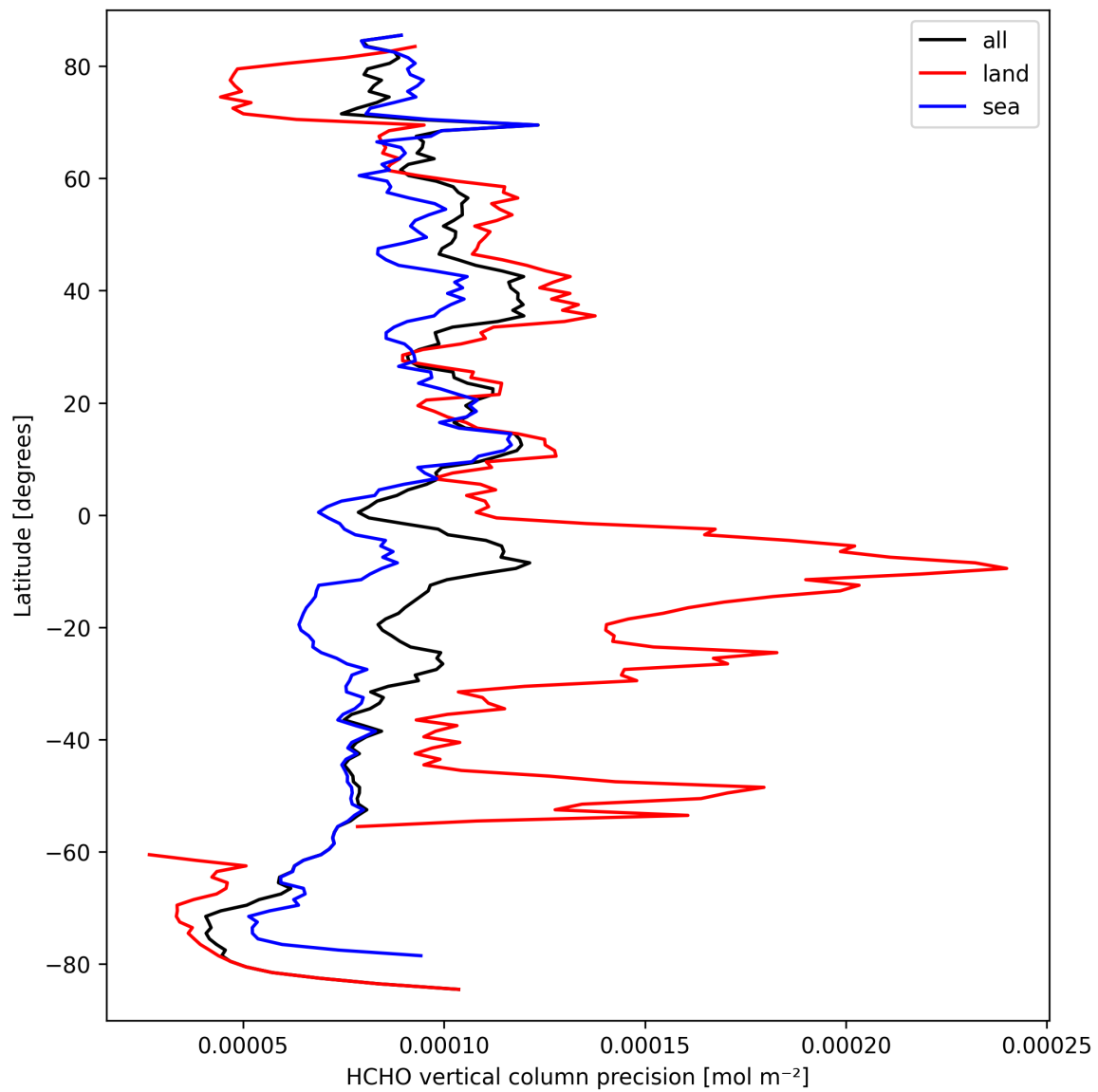
Figure 20: Zonal average of “HCHO vertical column precision” for 2025-09-21 to 2025-09-22.
