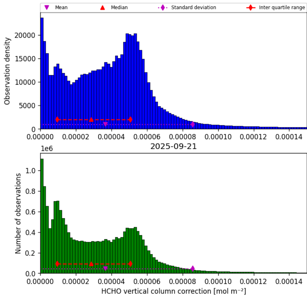
Figure 35: Histogram of “HCHO vertical column correction” for 2025-09-21 to 2025-09-22
