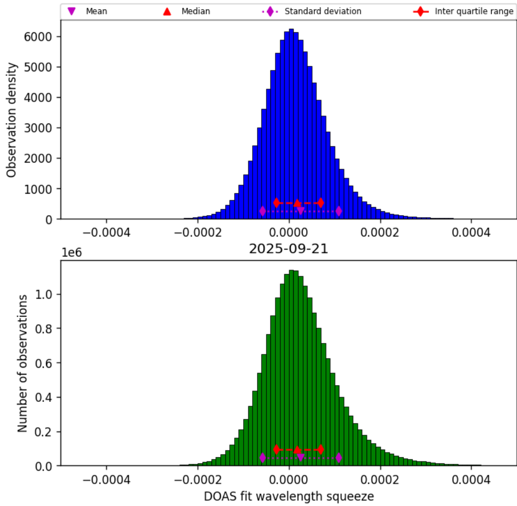
Figure 43: Histogram of “DOAS fit wavelength squeeze” for 2025-09-21 to 2025-09-22
