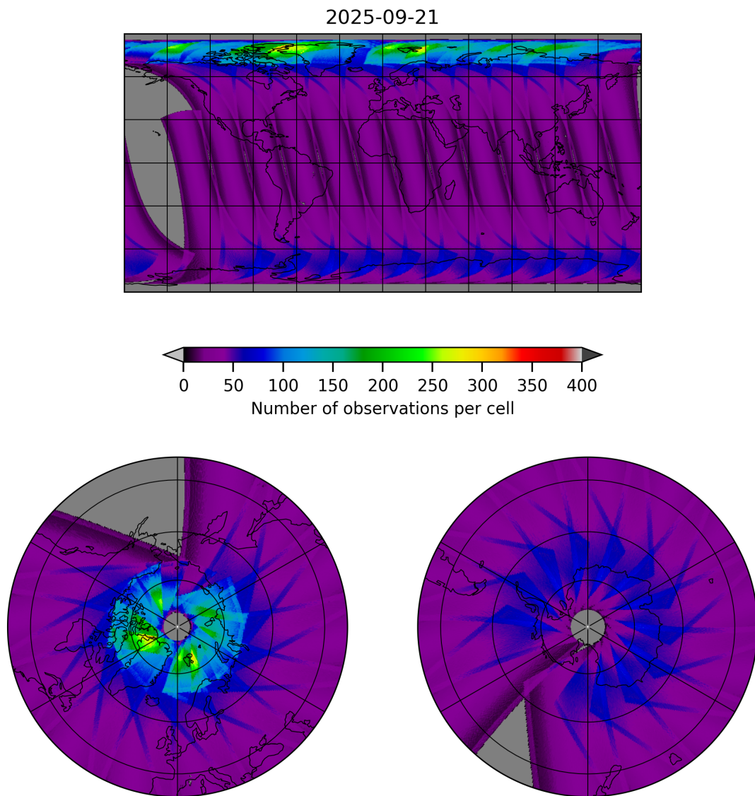
Figure 17: Map of the number of observations for 2025-09-21 to 2025-09-22
