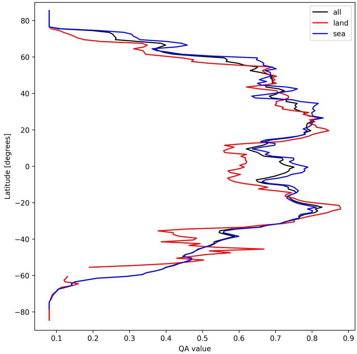
Figure 18: Zonal average of “QA value” for 2025-09-21 to 2025-09-22.
