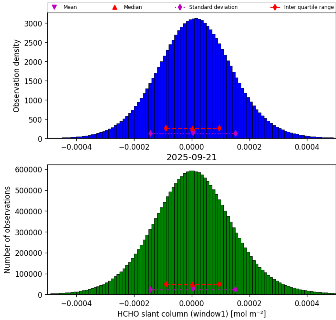
Figure 36: Histogram of “HCHO slant column (window1)” for 2025-09-21 to 2025-09-22
