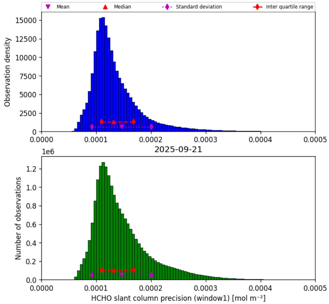
Figure 37: Histogram of “HCHO slant column precision (window1)” for 2025-09-21 to 2025-09-22
