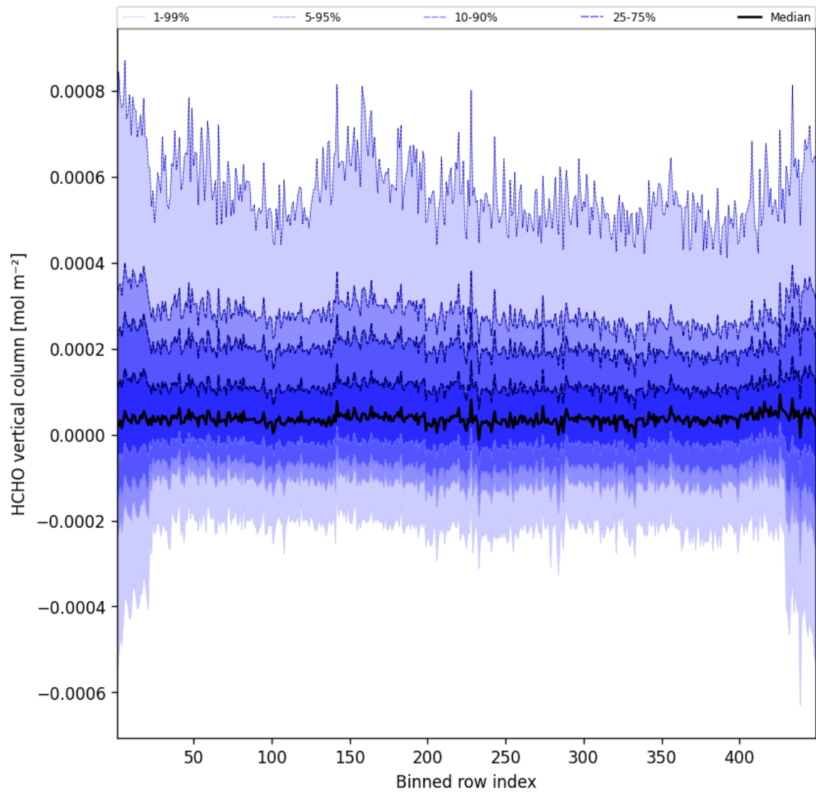
Figure 47: Along track statistics of “HCHO vertical column” for 2025-09-21 to 2025-09-22
