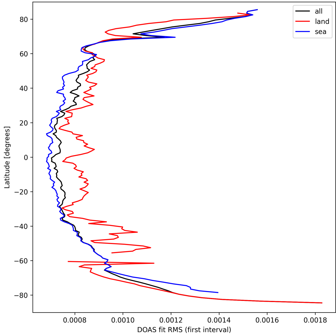
Figure 30: Zonal average of "DOAS fit RMS (first interval)" for 2025-09-21 to 2025-09-22.
