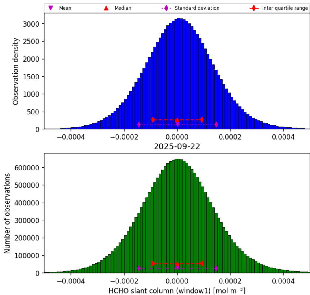
Figure 36: Histogram of “HCHO slant column (window1)” for 2025-09-22 to 2025-09-23
