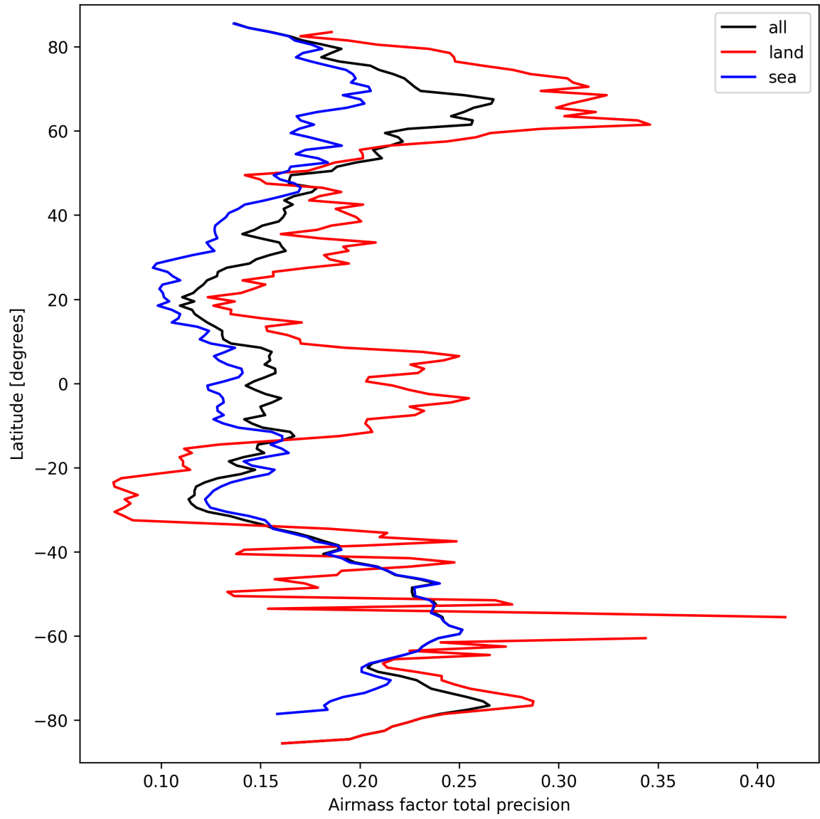
Figure 25: Zonal average of “Airmass factor total precision” for 2025-09-22 to 2025-09-23.
