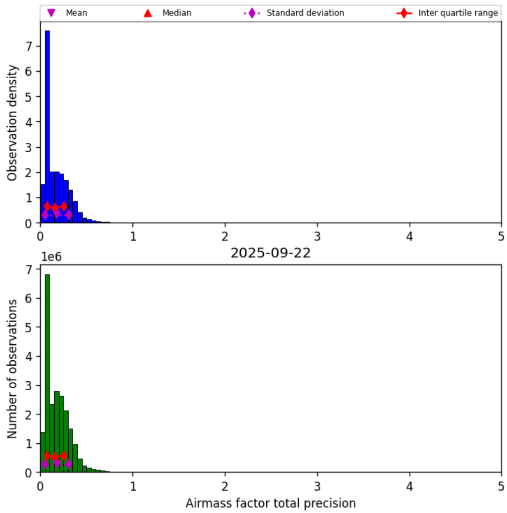
Figure 39: Histogram of “Airmass factor total precision” for 2025-09-22 to 2025-09-23
