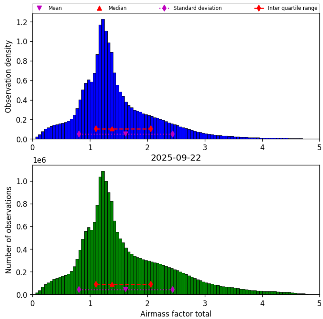
Figure 38: Histogram of “Airmass factor total” for 2025-09-22 to 2025-09-23
