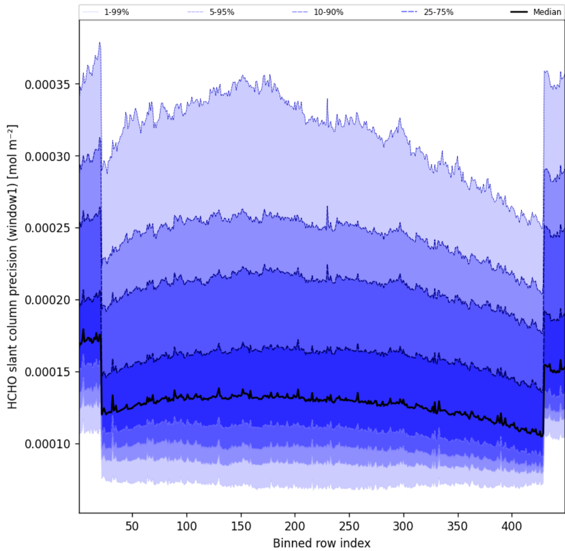
Figure 51: Along track statistics of “HCHO slant column precision (window1)” for 2025-09-22 to 2025-09-23
