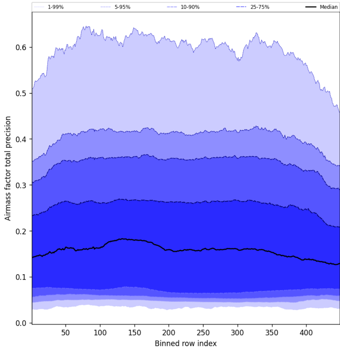
Figure 53: Along track statistics of “Airmass factor total precision” for 2025-09-22 to 2025-09-23
