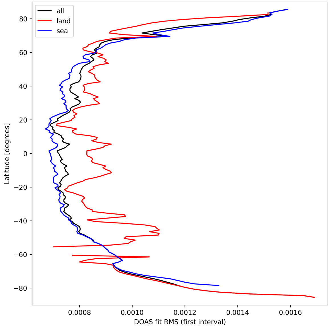
Figure 30: Zonal average of "DOAS fit RMS (first interval)" for 2025-09-22 to 2025-09-23.
