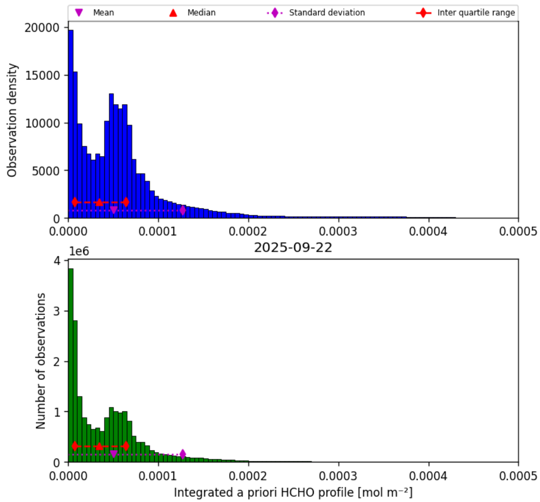
Figure 41: Histogram of “Integrated a priori HCHO profile” for 2025-09-22 to 2025-09-23
