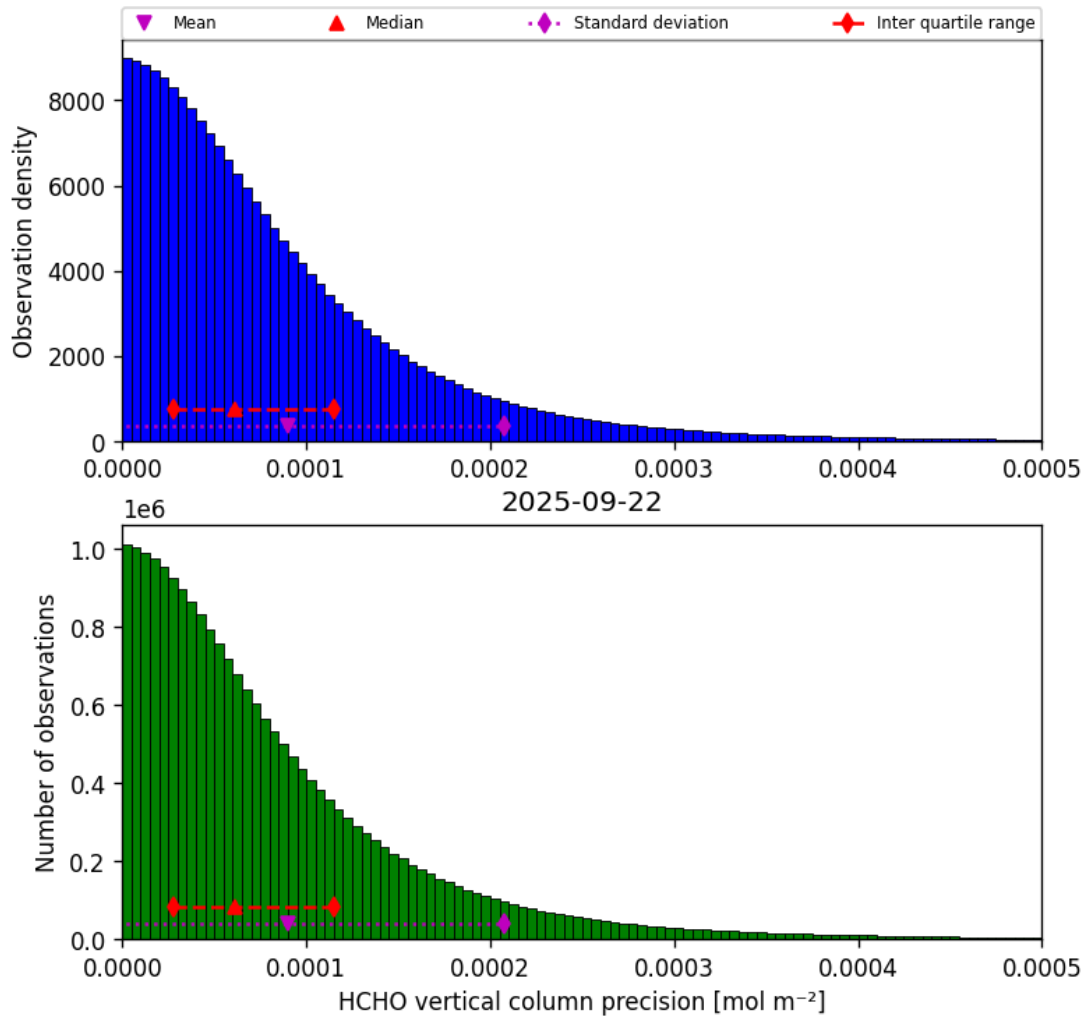
Figure 34: Histogram of “HCHO vertical column precision” for 2025-09-22 to 2025-09-23
