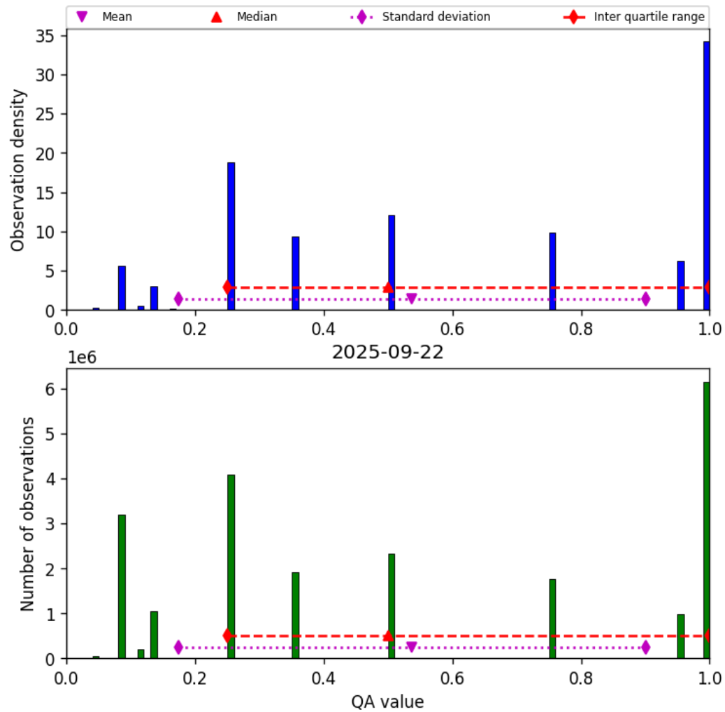
Figure 32: Histogram of “QA value” for 2025-09-22 to 2025-09-23
