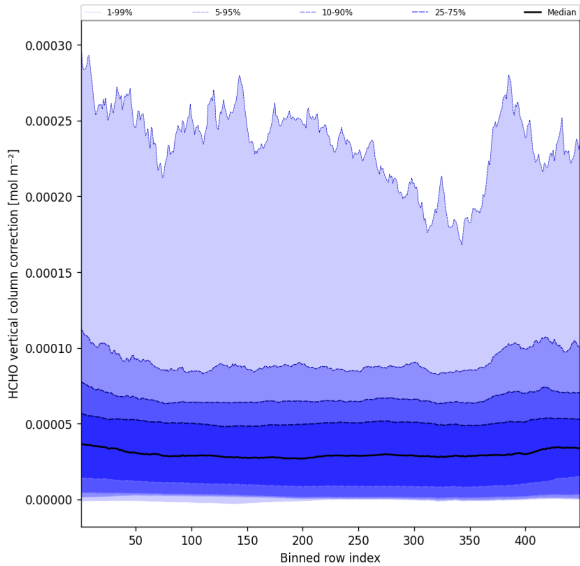
Figure 49: Along track statistics of “HCHO vertical column correction” for 2025-09-22 to 2025-09-23
