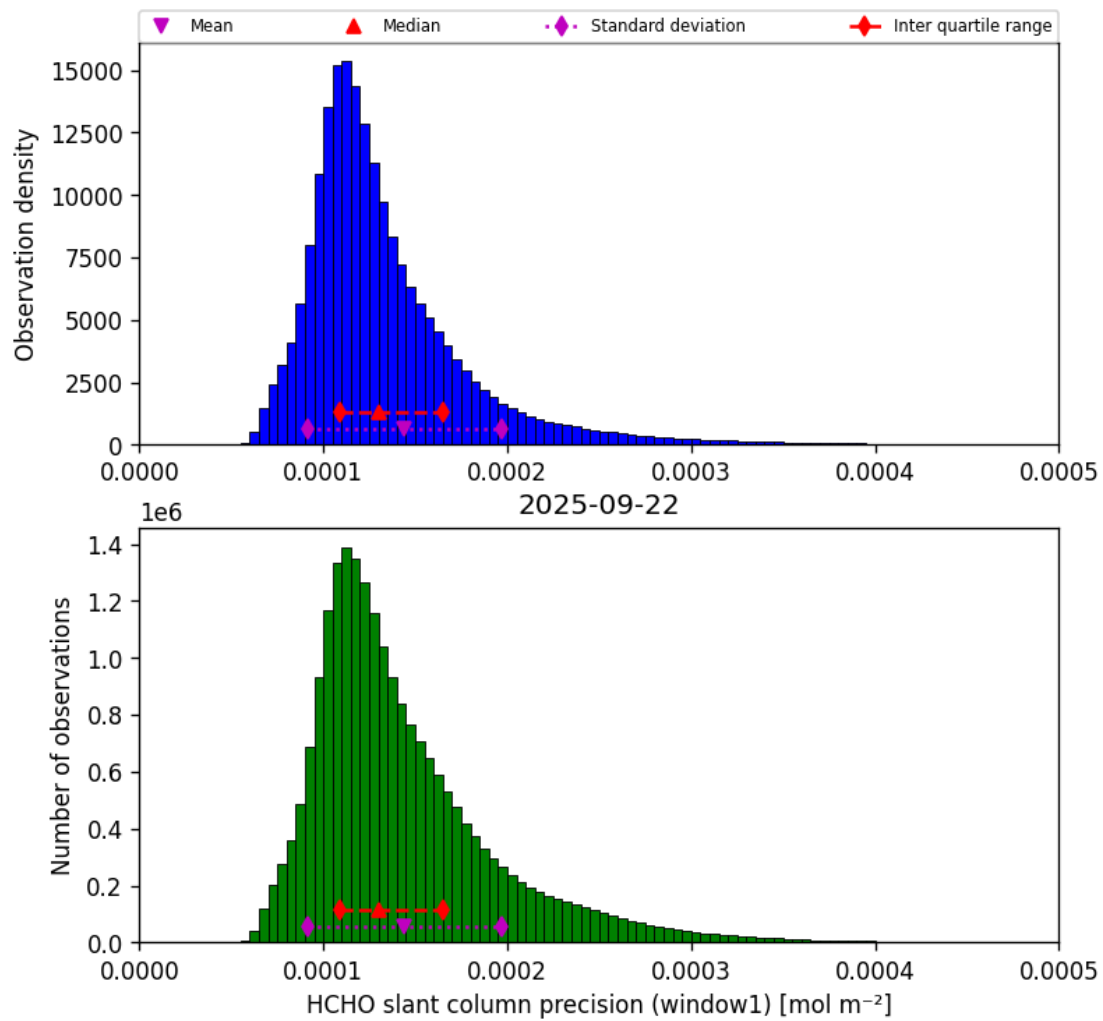
Figure 37: Histogram of “HCHO slant column precision (window1)” for 2025-09-22 to 2025-09-23
