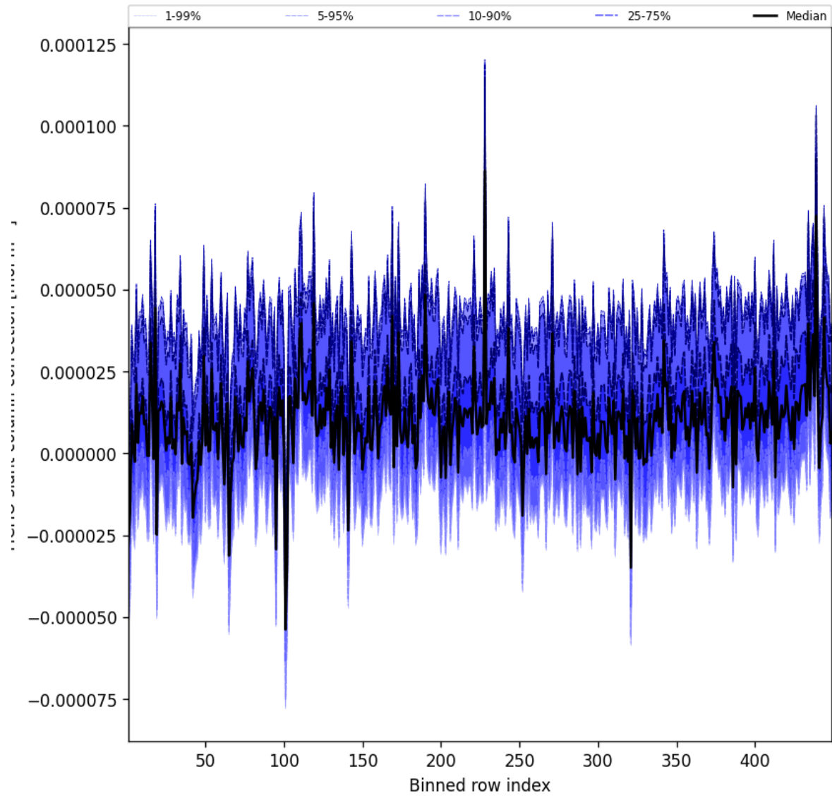
Figure 59: Along track statistics of “HCHO slant column correction” for 2025-09-22 to 2025-09-23
