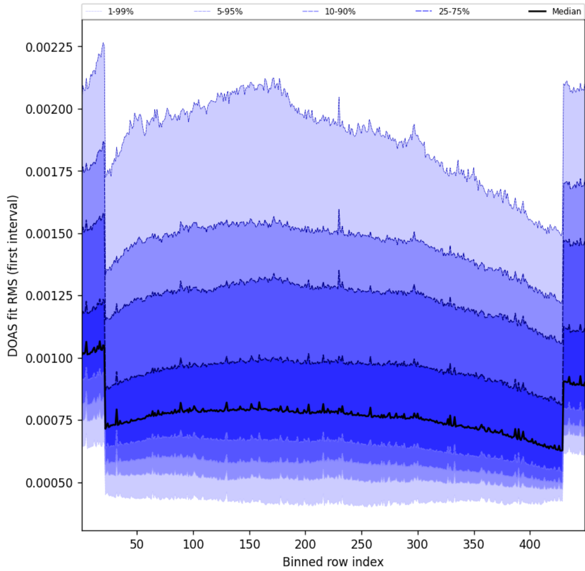
Figure 58: Along track statistics of “DOAS fit RMS (first interval)” for 2025-09-22 to 2025-09-23
