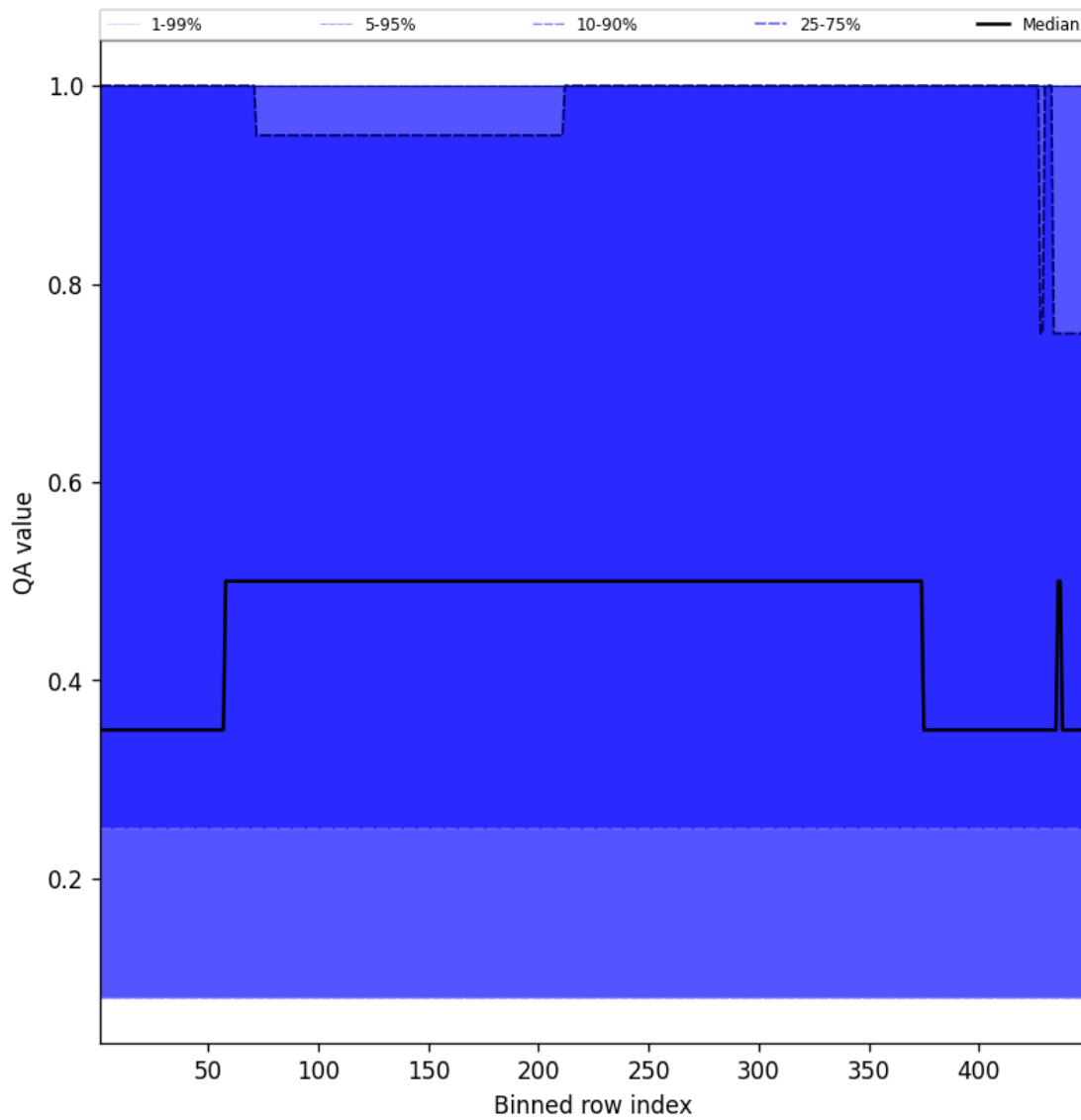
Figure 46: Along track statistics of “QA value” for 2025-09-22 to 2025-09-23
