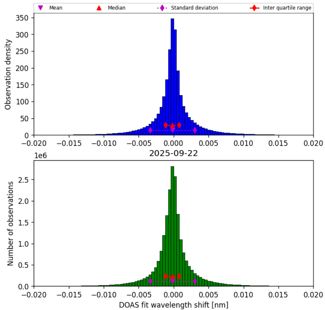
Figure 42: Histogram of “DOAS fit wavelength shift” for 2025-09-22 to 2025-09-23
