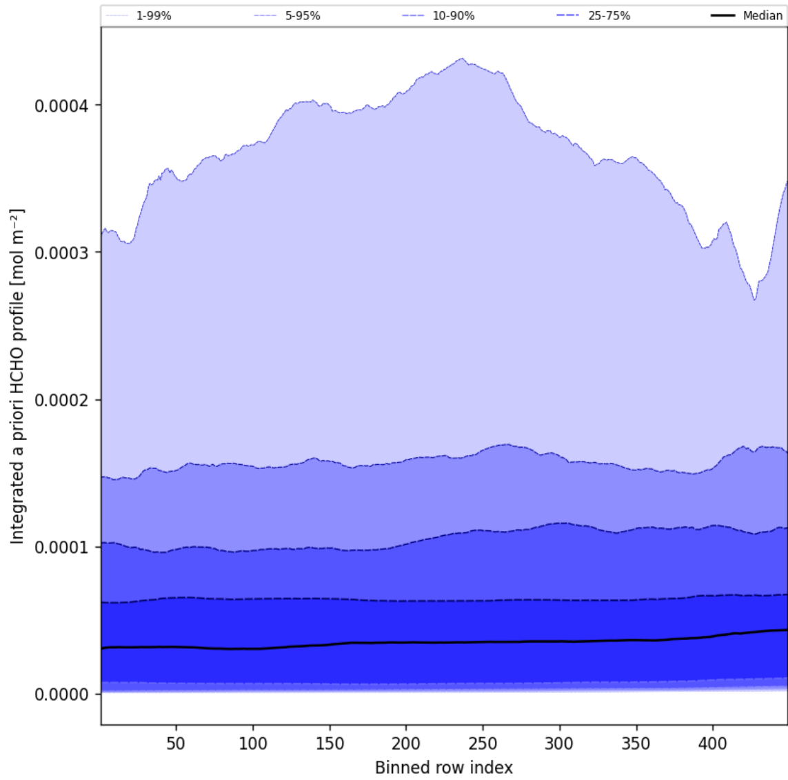
Figure 55: Along track statistics of “Integrated a priori HCHO profile” for 2025-09-22 to 2025-09-23
