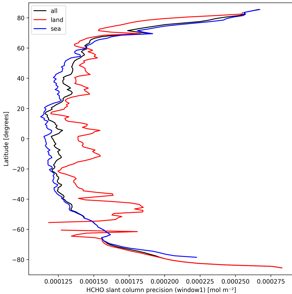
Figure 23: Zonal average of “HCHO slant column precision (window1)” for 2025-09-22 to 2025-09-23.
