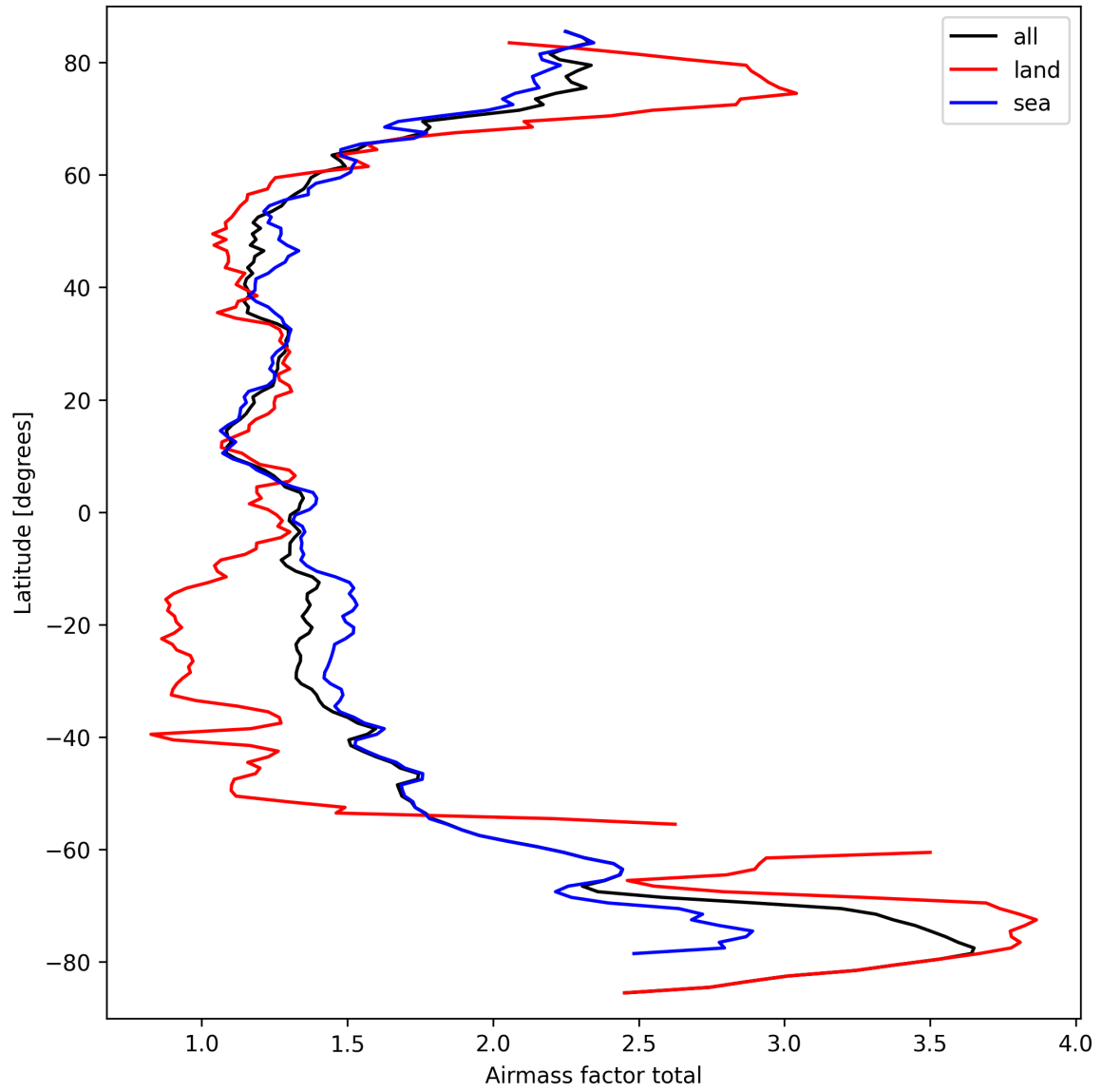
Figure 24: Zonal average of “Airmass factor total” for 2025-09-22 to 2025-09-23.
