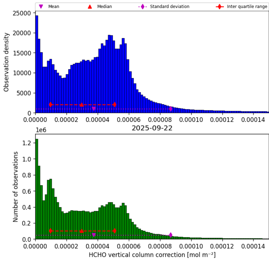
Figure 35: Histogram of “HCHO vertical column correction” for 2025-09-22 to 2025-09-23
