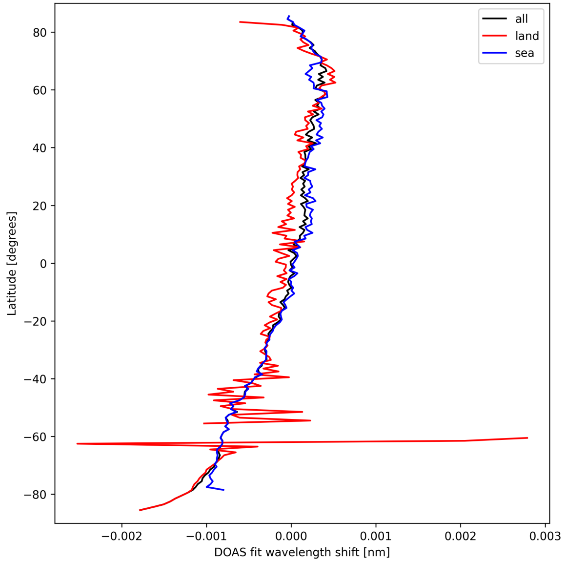
Figure 28: Zonal average of “DOAS fit wavelength shift” for 2025-09-22 to 2025-09-23.
