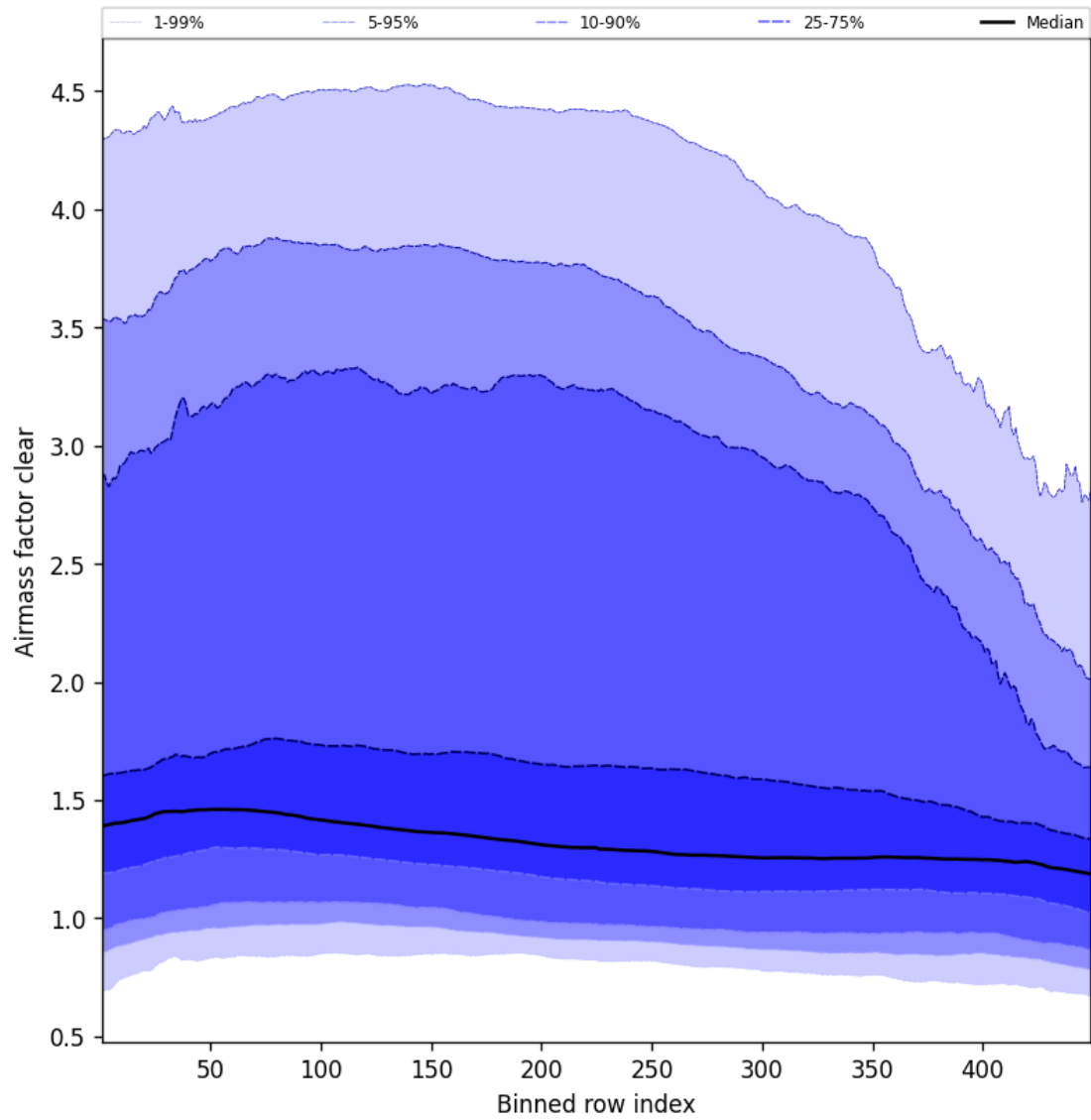
Figure 54: Along track statistics of “Airmass factor clear” for 2025-09-22 to 2025-09-23
