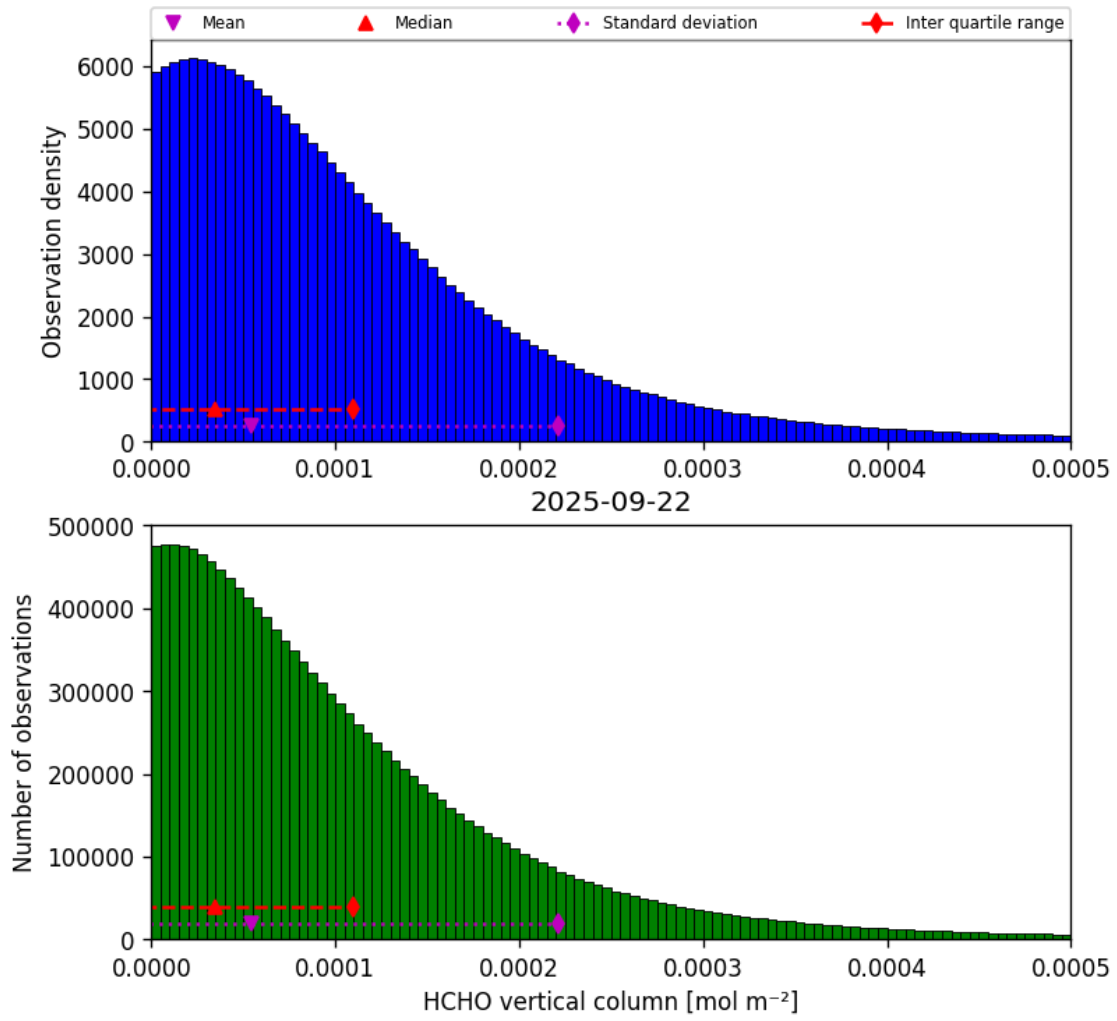
Figure 33: Histogram of “HCHO vertical column” for 2025-09-22 to 2025-09-23
