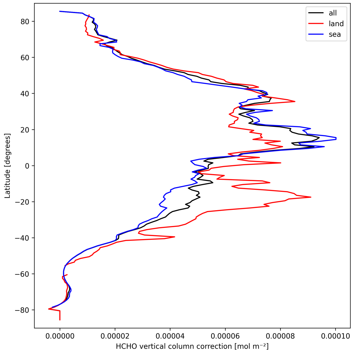
Figure 21: Zonal average of “HCHO vertical column correction” for 2025-09-22 to 2025-09-23.
