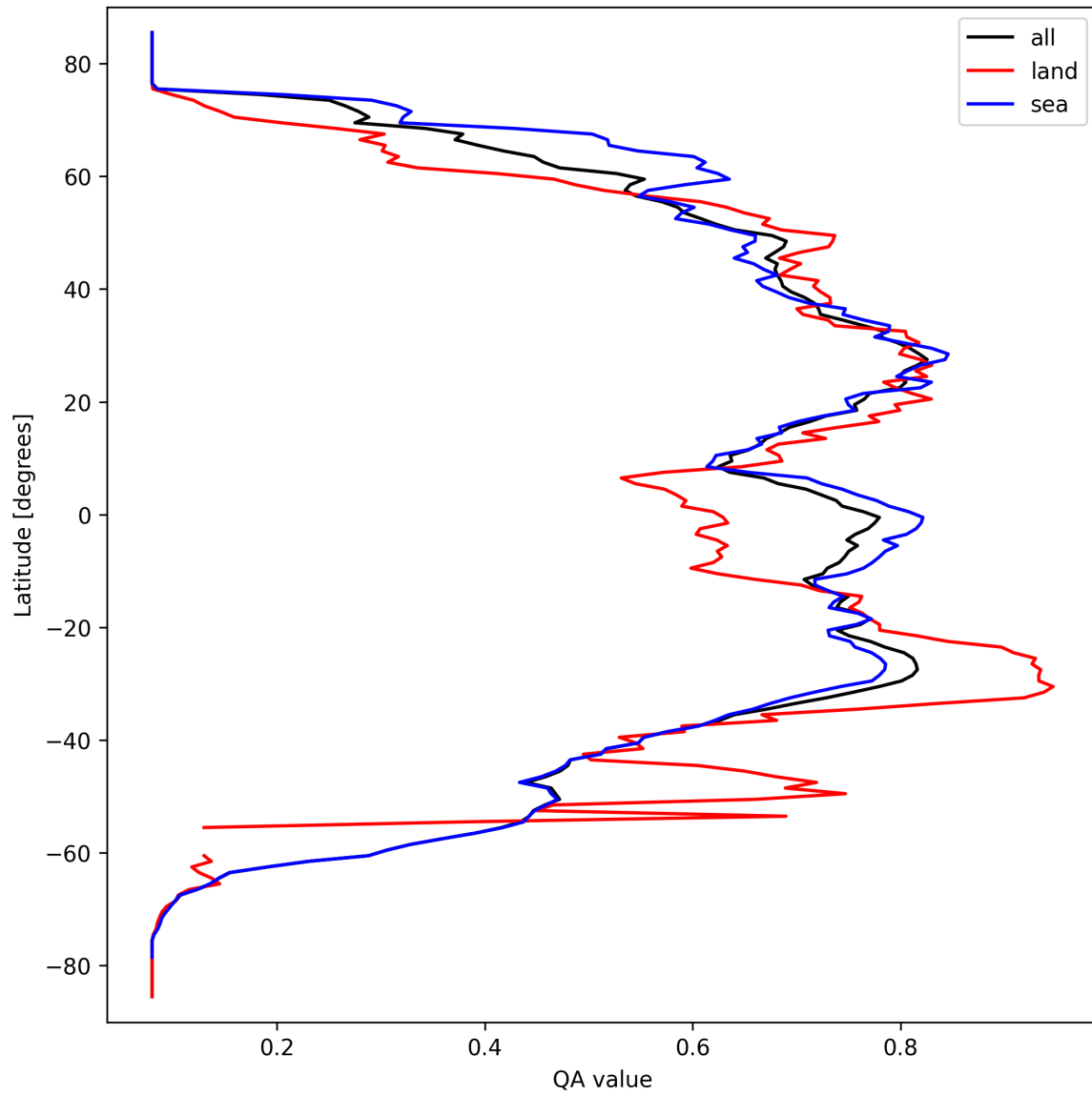
Figure 18: Zonal average of “QA value” for 2025-09-22 to 2025-09-23.
