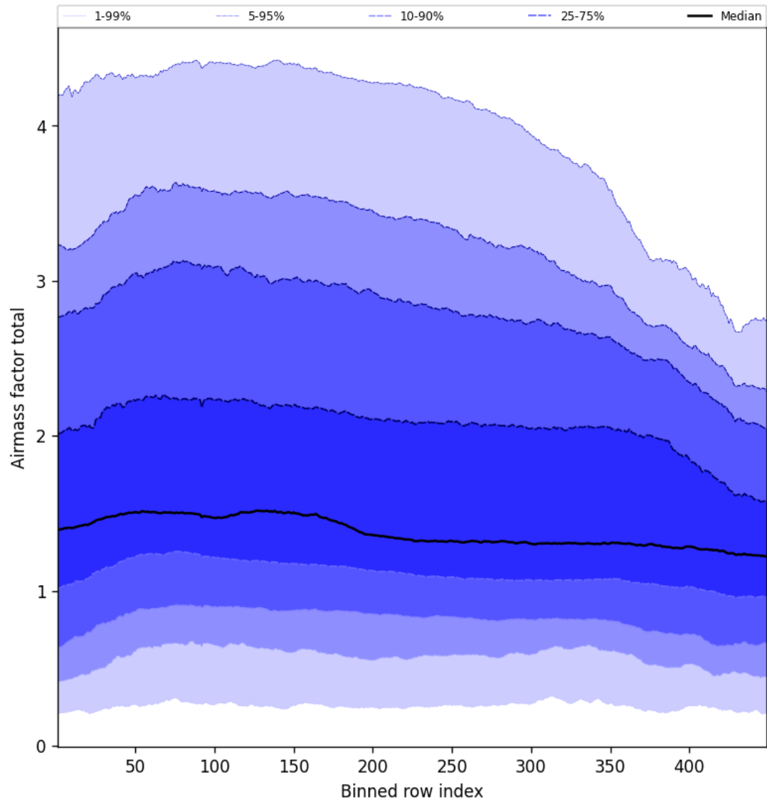
Figure 52: Along track statistics of “Airmass factor total” for 2025-09-22 to 2025-09-23
