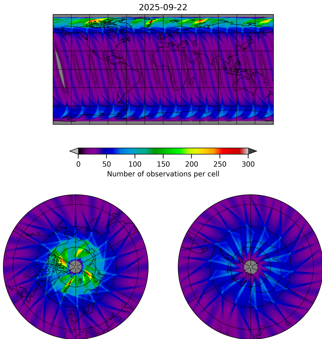
Figure 17: Map of the number of observations for 2025-09-22 to 2025-09-23
