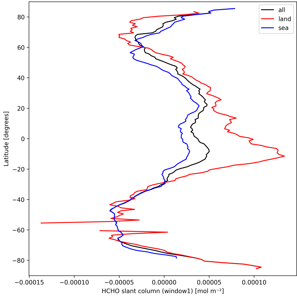
Figure 22: Zonal average of “HCHO slant column (window1)” for 2025-09-22 to 2025-09-23.
