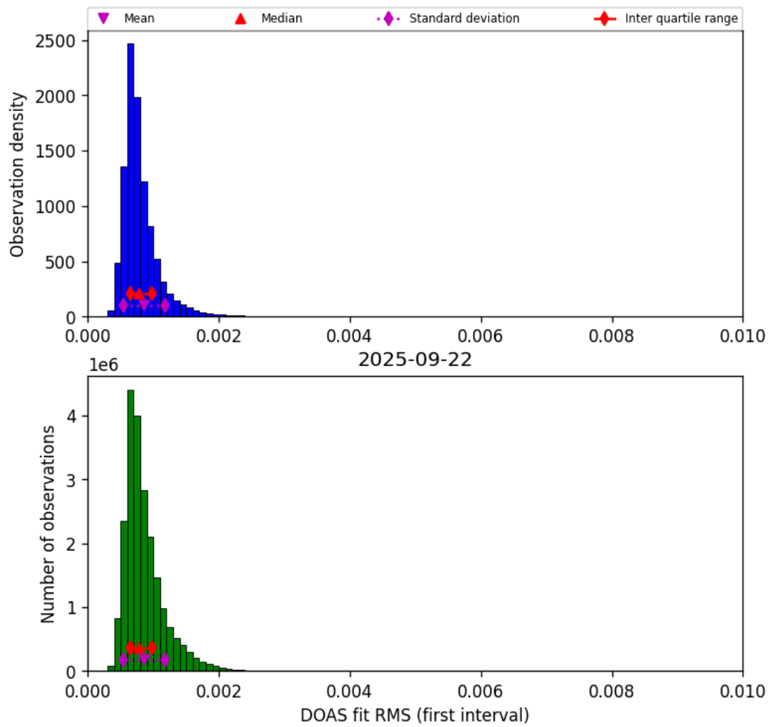
Figure 44: Histogram of “DOAS fit RMS (first interval)” for 2025-09-22 to 2025-09-23
