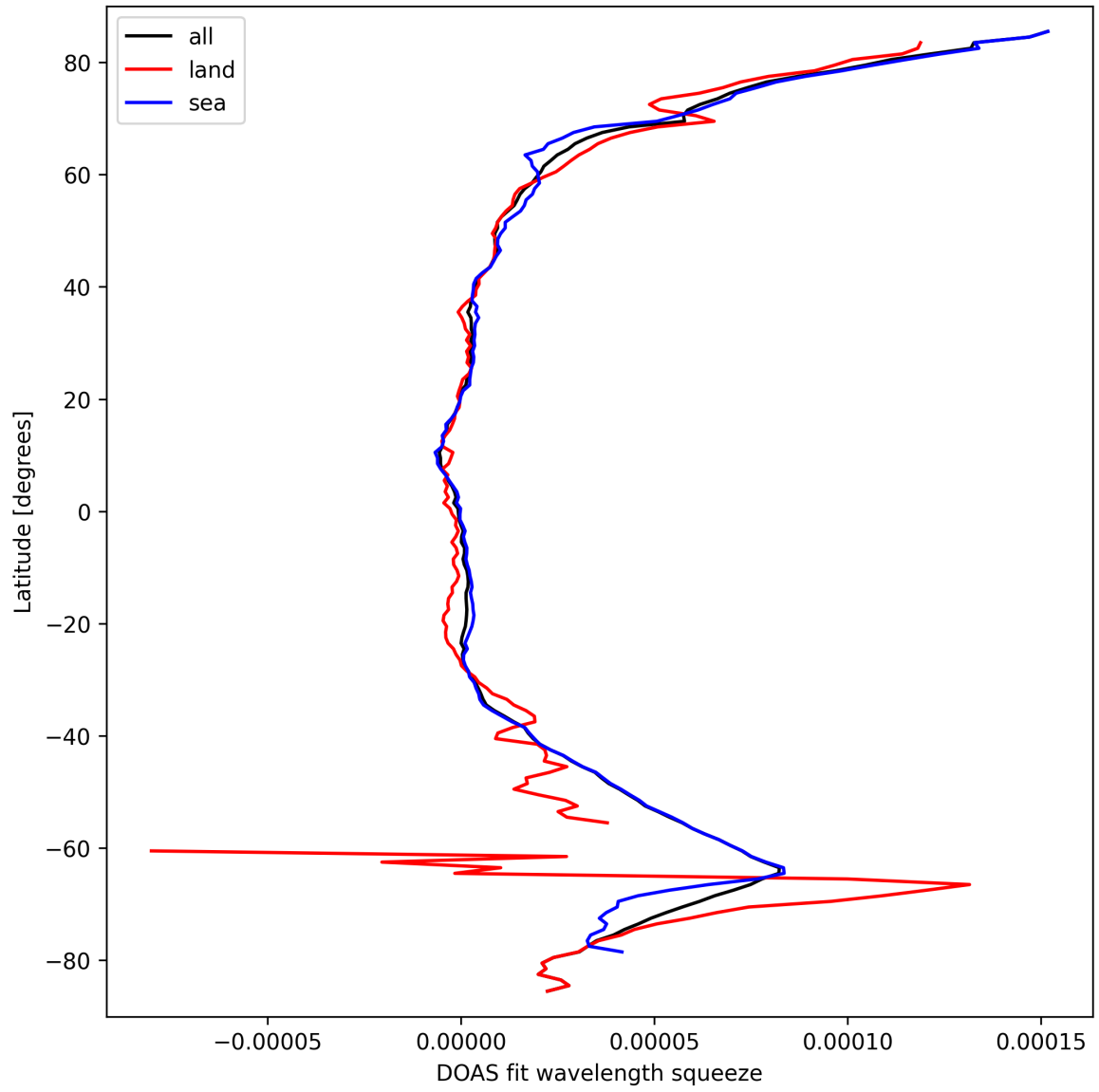
Figure 29: Zonal average of “DOAS fit wavelength squeeze” for 2025-09-22 to 2025-09-23.
