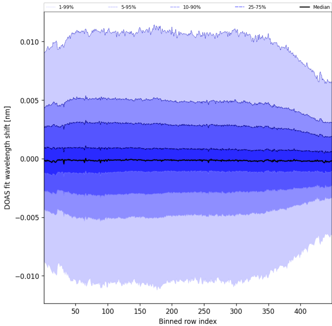
Figure 56: Along track statistics of “DOAS fit wavelength shift” for 2025-09-22 to 2025-09-23
