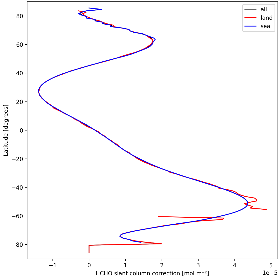
Figure 31: Zonal average of "HCHO slant column correction" for 2025-09-22 to 2025-09-23.
