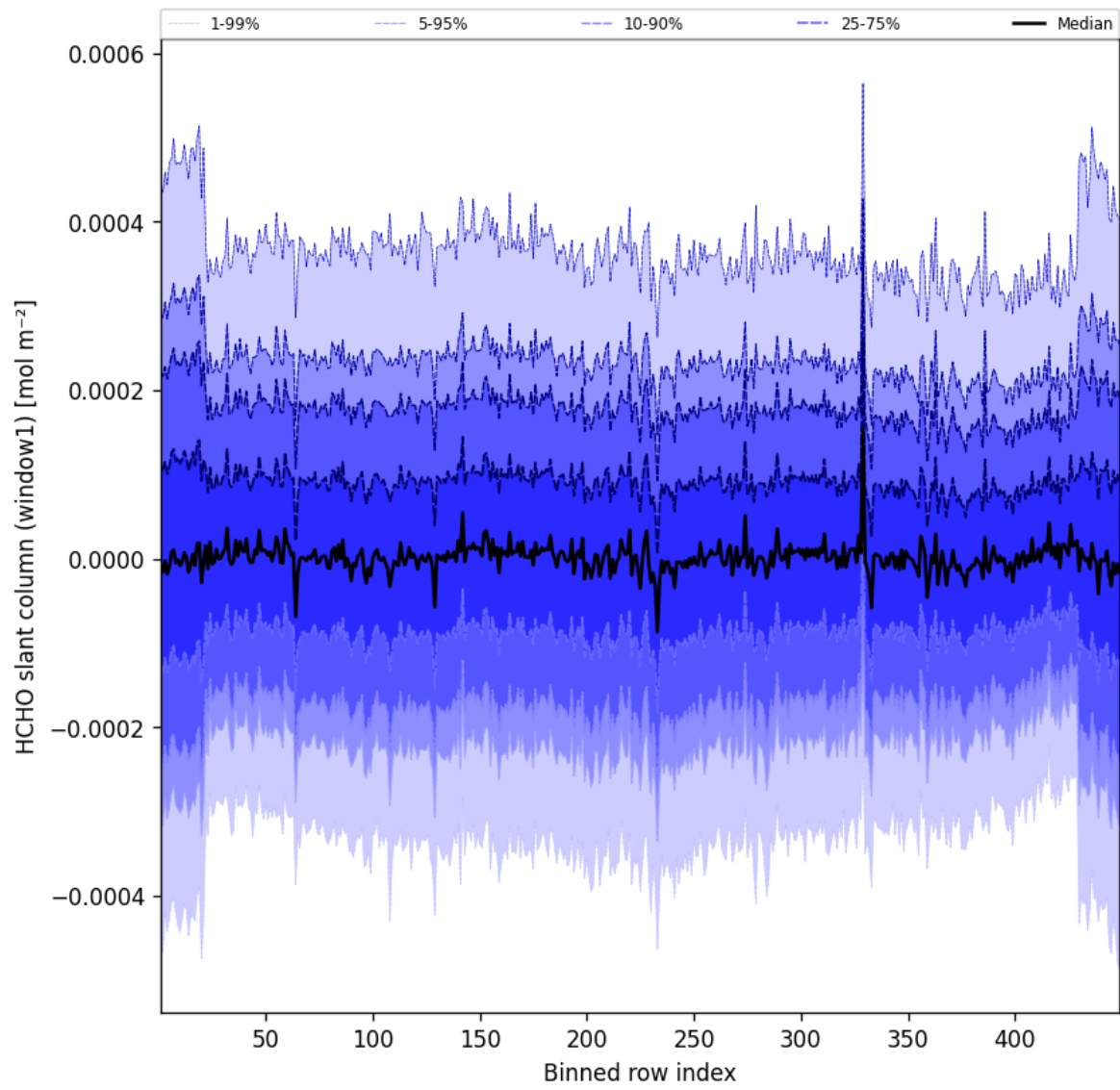
Figure 50: Along track statistics of “HCHO slant column (window1)” for 2025-09-22 to 2025-09-23
