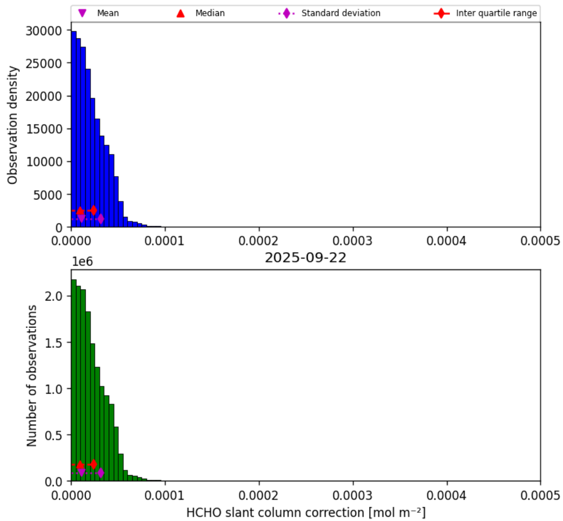
Figure 45: Histogram of “HCHO slant column correction” for 2025-09-22 to 2025-09-23
