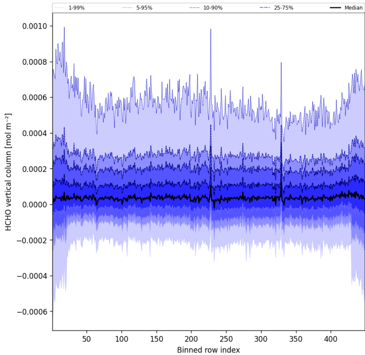
Figure 47: Along track statistics of “HCHO vertical column” for 2025-09-22 to 2025-09-23
