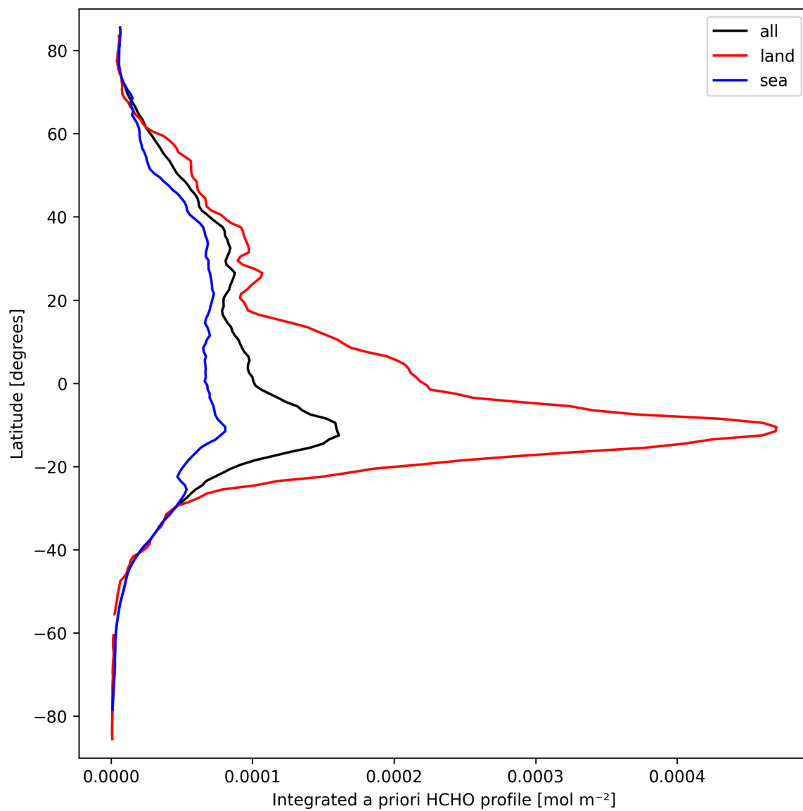
Figure 27: Zonal average of “Integrated a priori HCHO profile” for 2025-09-22 to 2025-09-23.
