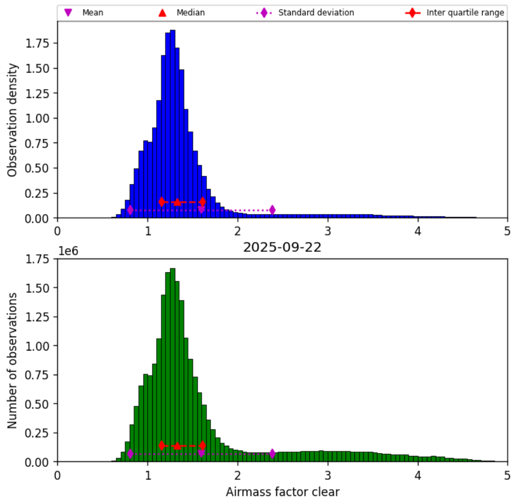
Figure 40: Histogram of “Airmass factor clear” for 2025-09-22 to 2025-09-23
