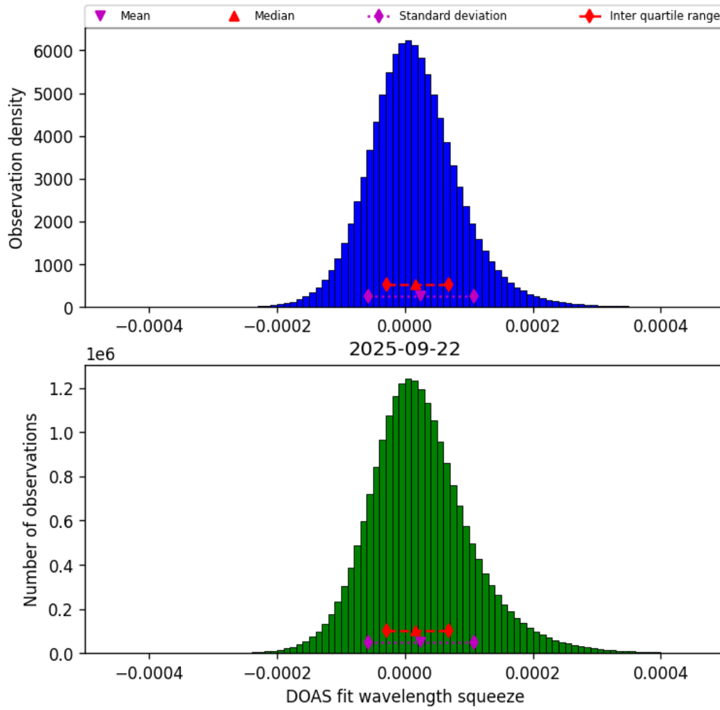
Figure 43: Histogram of “DOAS fit wavelength squeeze” for 2025-09-22 to 2025-09-23
