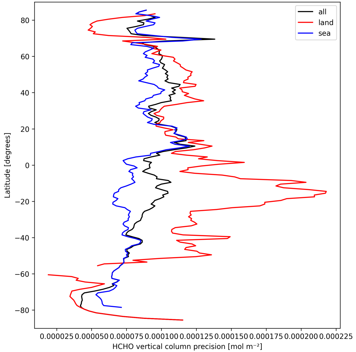
Figure 20: Zonal average of “HCHO vertical column precision” for 2025-09-22 to 2025-09-23.
