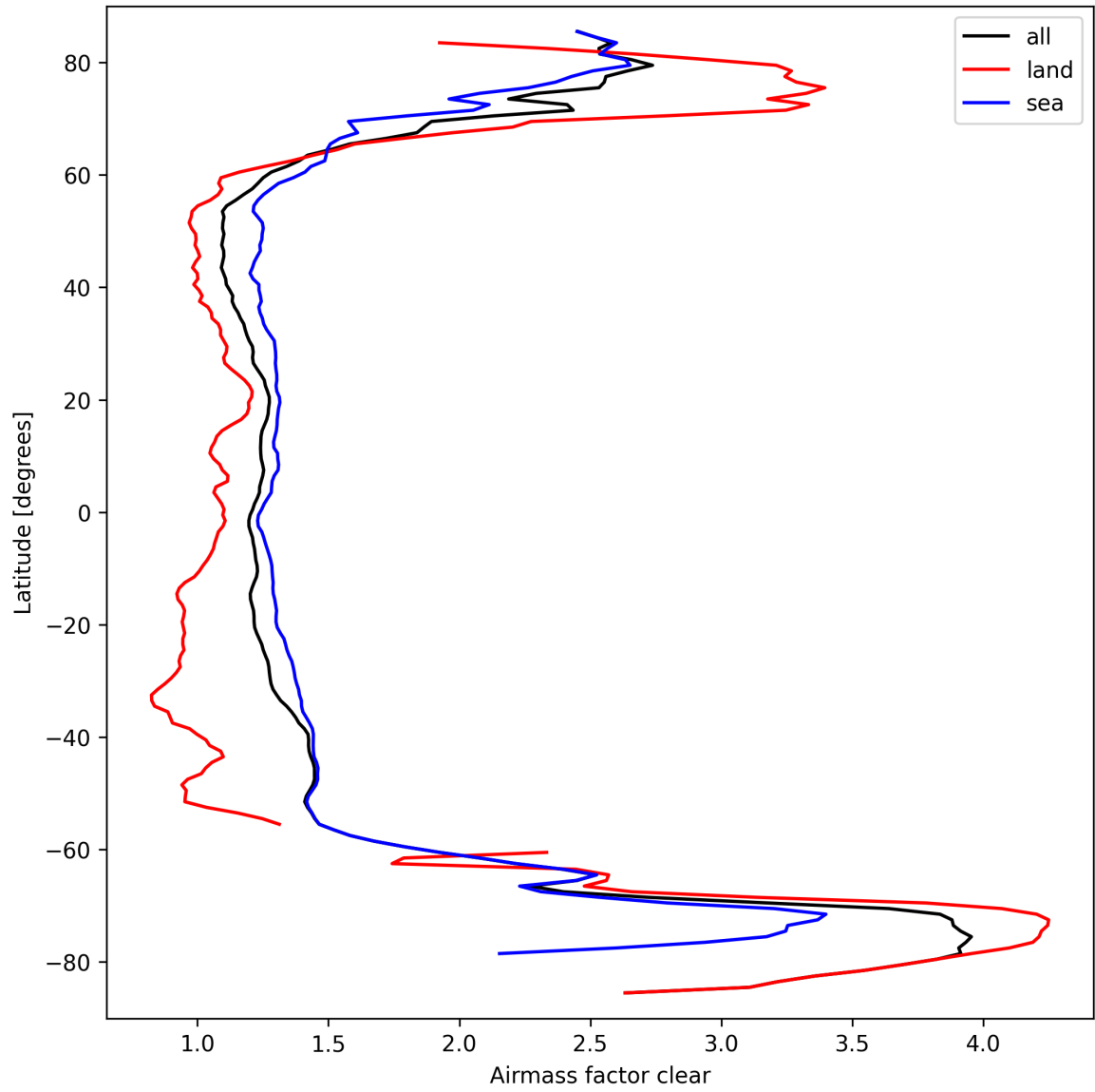
Figure 26: Zonal average of “Airmass factor clear” for 2025-09-22 to 2025-09-23.
