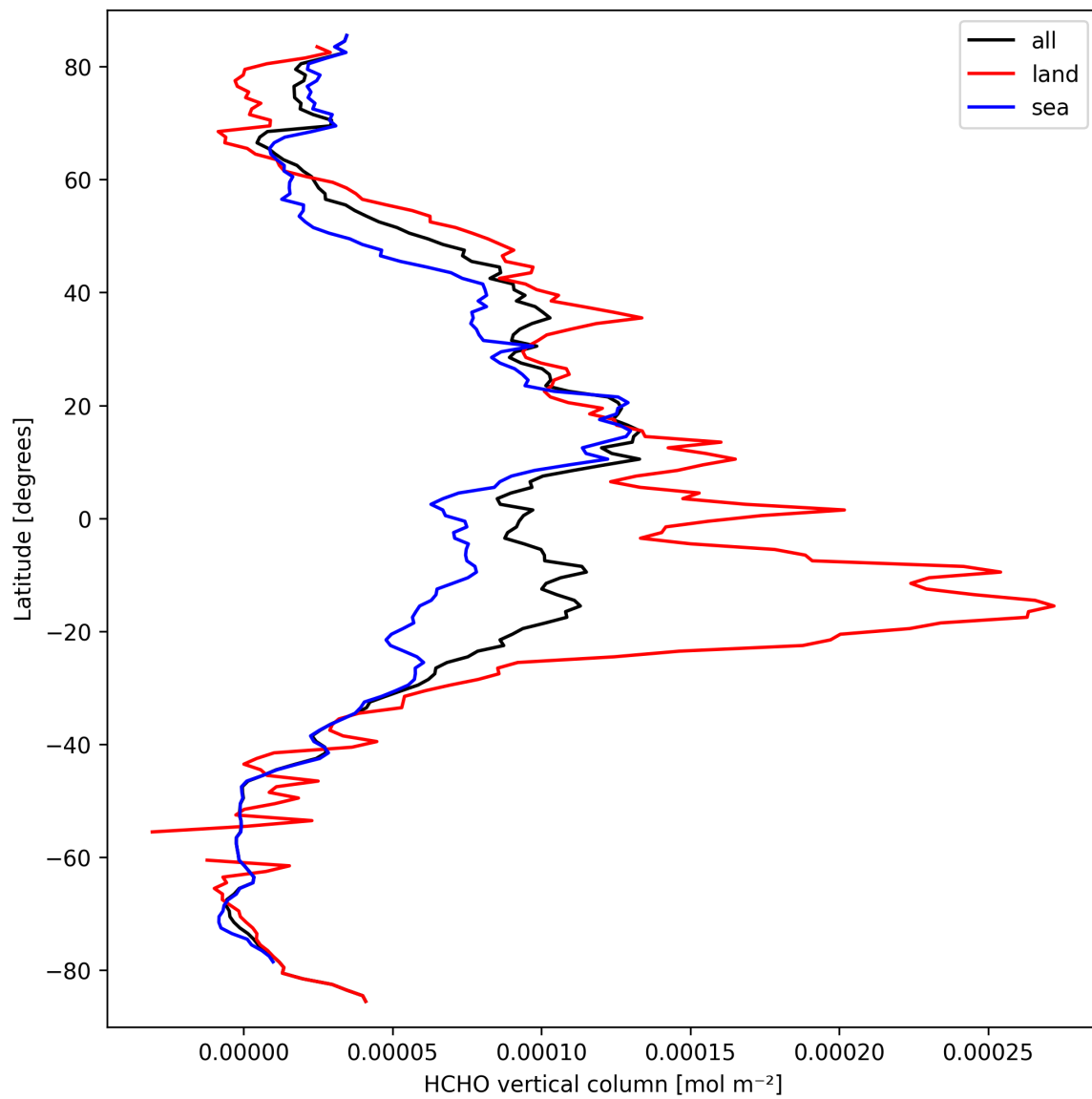
Figure 19: Zonal average of “HCHO vertical column” for 2025-09-22 to 2025-09-23.
