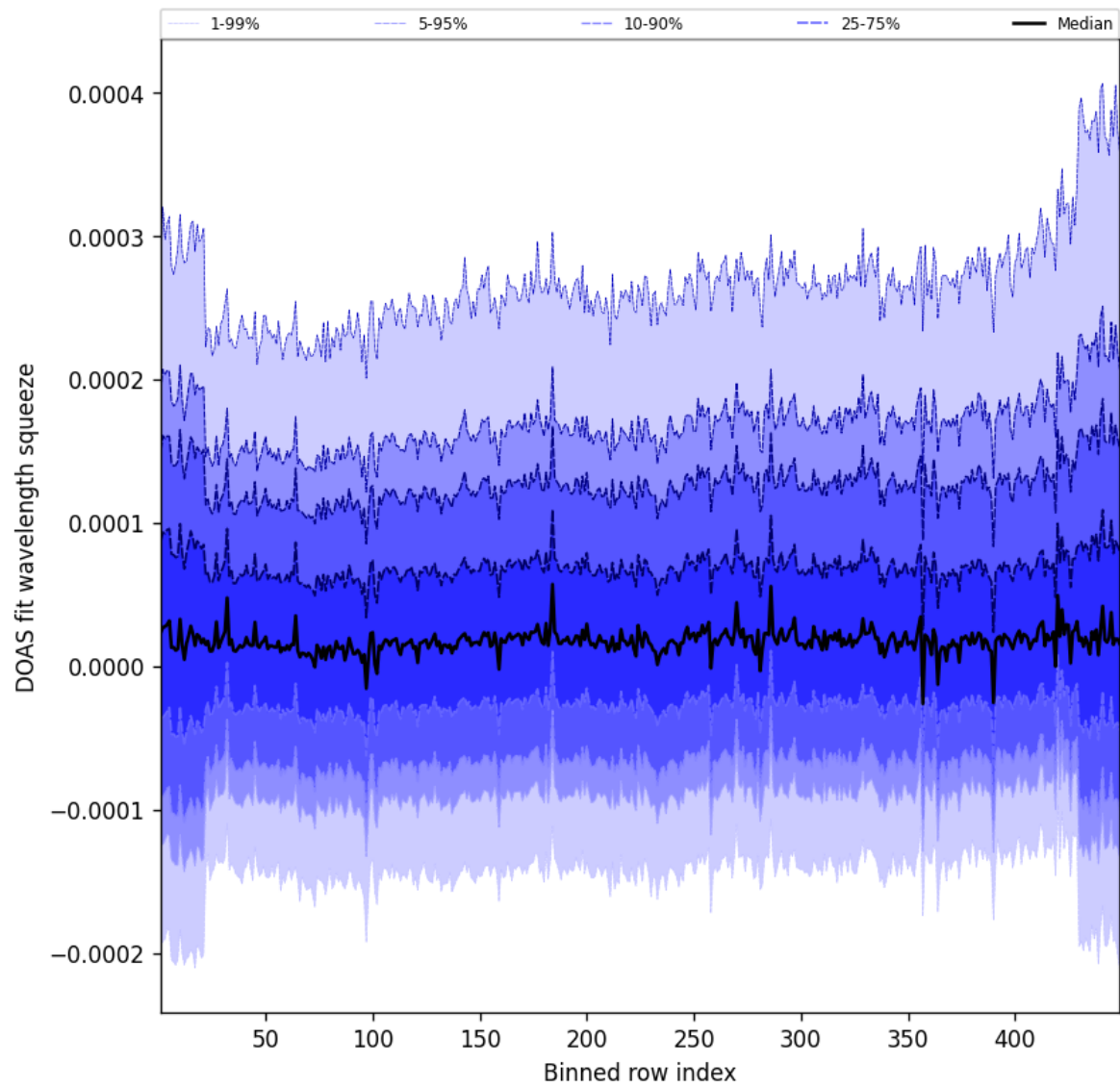
Figure 57: Along track statistics of “DOAS fit wavelength squeeze” for 2025-09-22 to 2025-09-23
