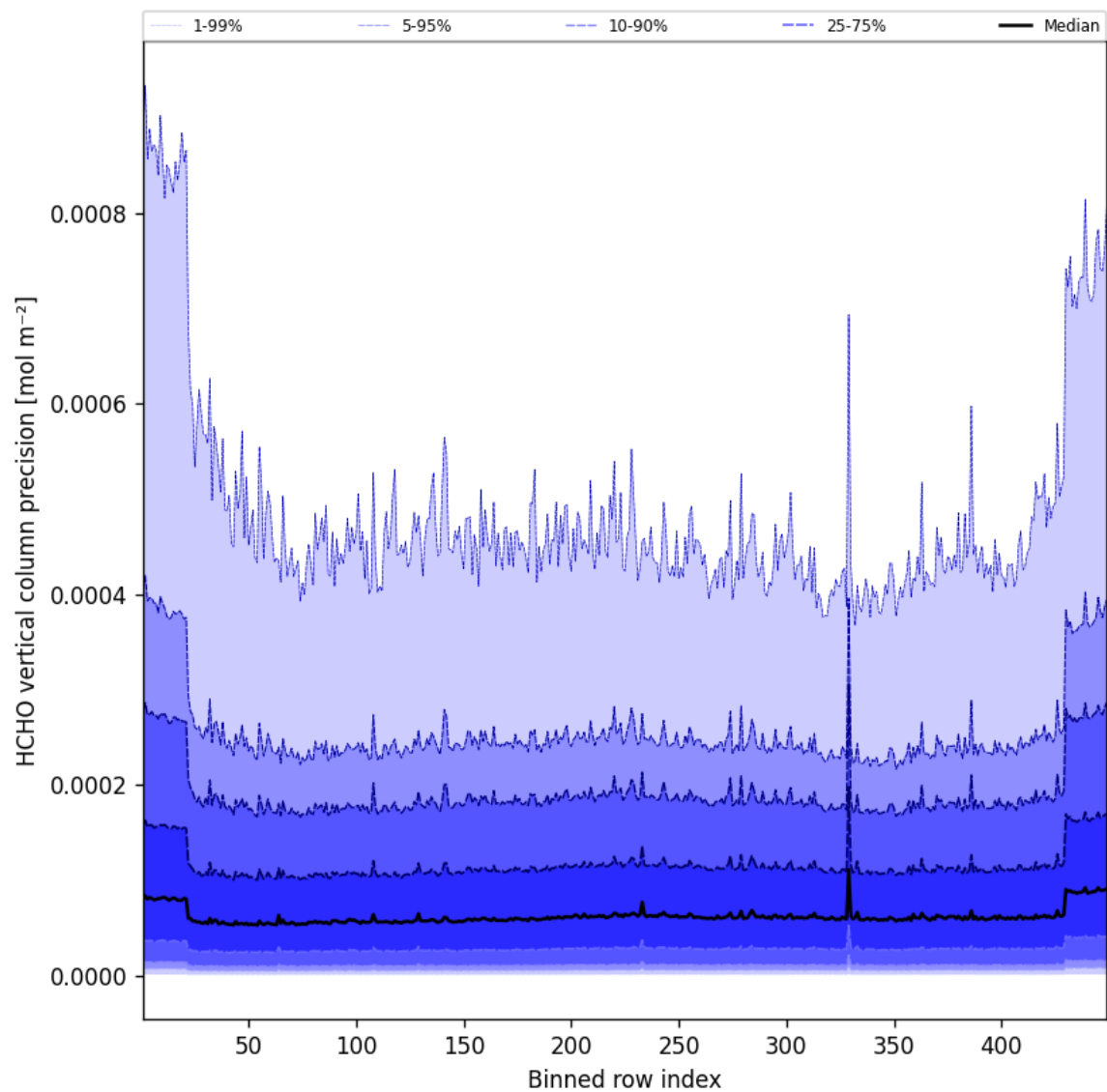
Figure 48: Along track statistics of “HCHO vertical column precision” for 2025-09-22 to 2025-09-23
