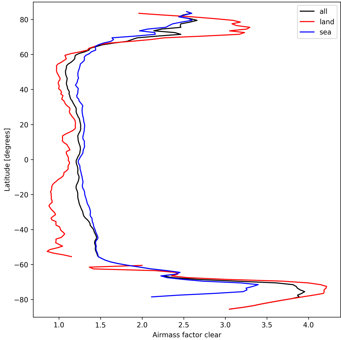
Figure 26: Zonal average of “Airmass factor clear” for 2025-09-23 to 2025-09-23.
