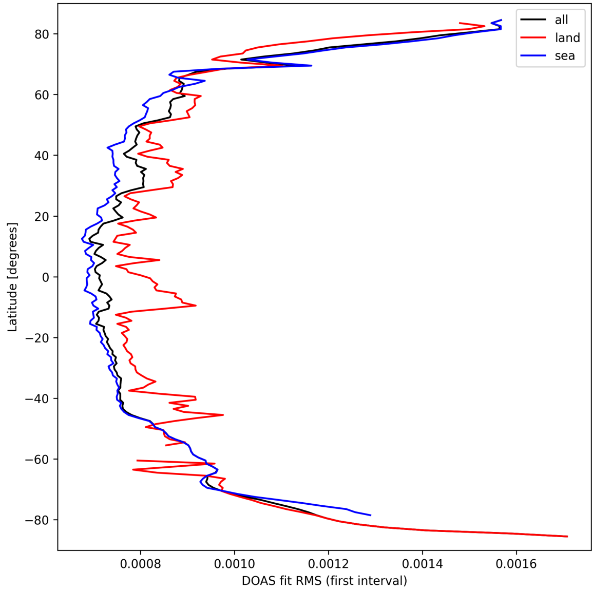
Figure 30: Zonal average of “DOAS fit RMS (first interval)” for 2025-09-23 to 2025-09-23.
