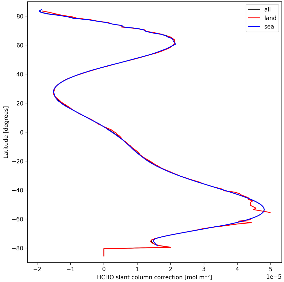
Figure 31: Zonal average of “HCHO slant column correction” for 2025-09-23 to 2025-09-23.
