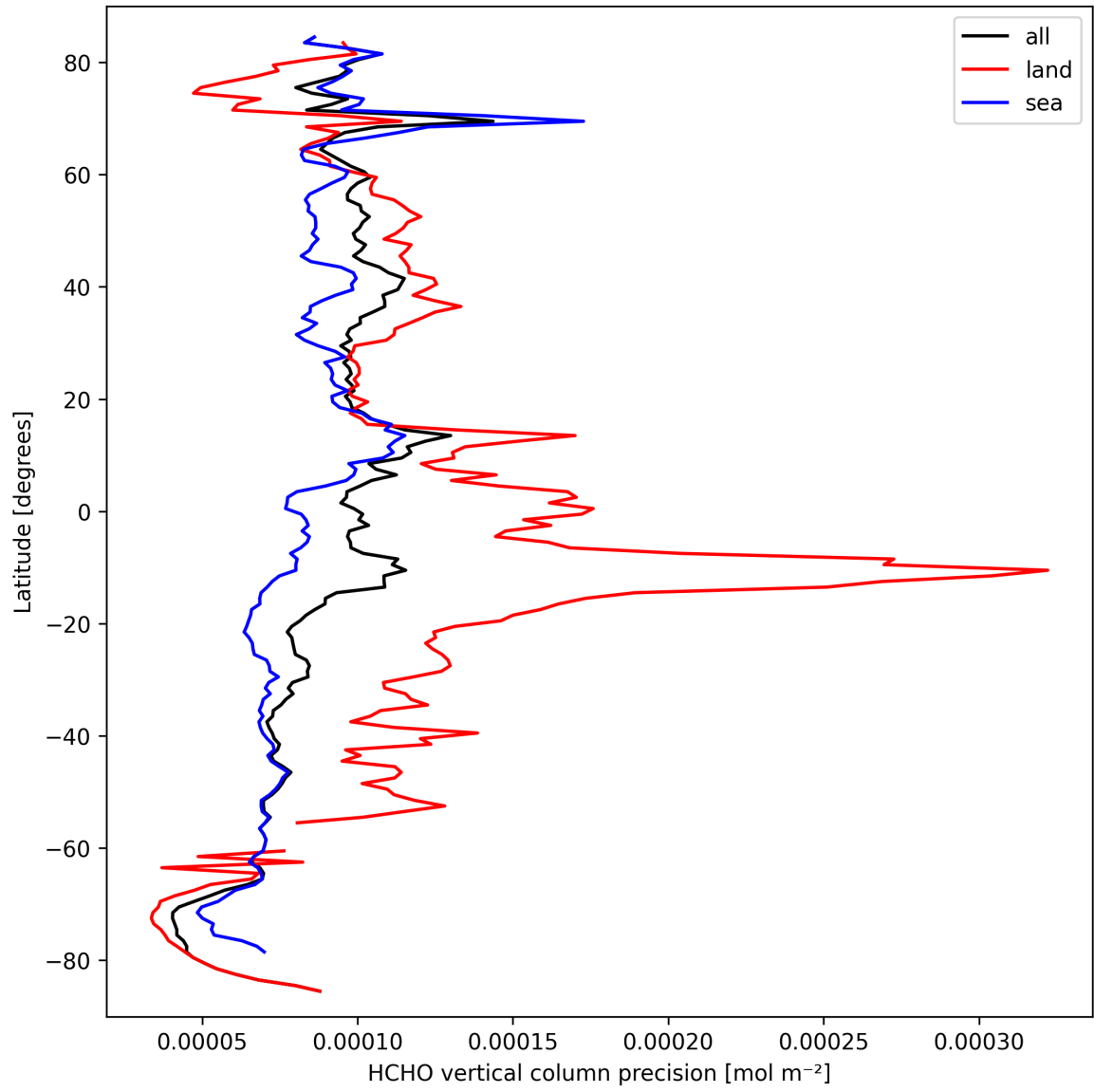
Figure 20: Zonal average of “HCHO vertical column precision” for 2025-09-23 to 2025-09-23.
