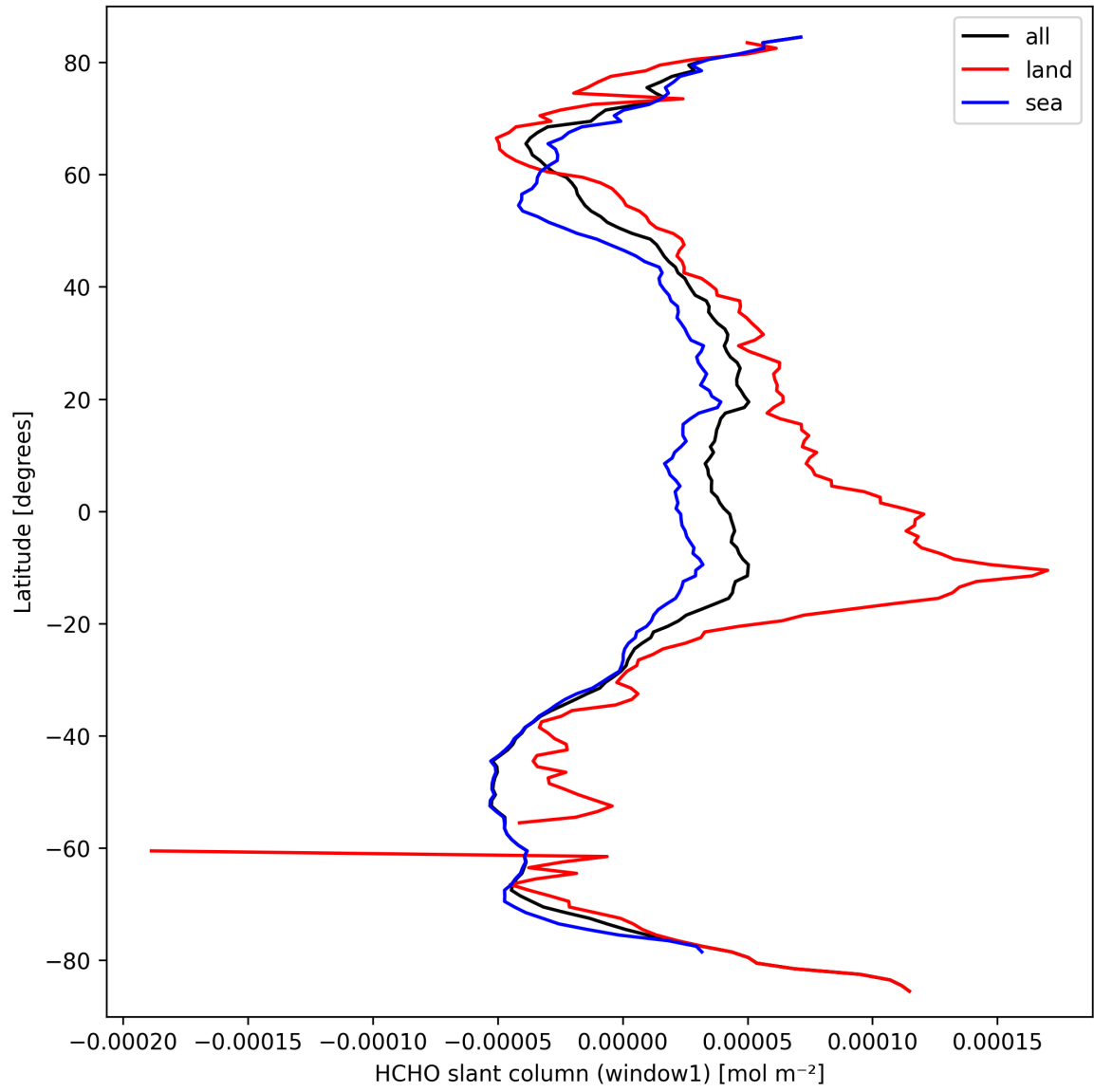
Figure 22: Zonal average of “HCHO slant column (window1)” for 2025-09-23 to 2025-09-23.
