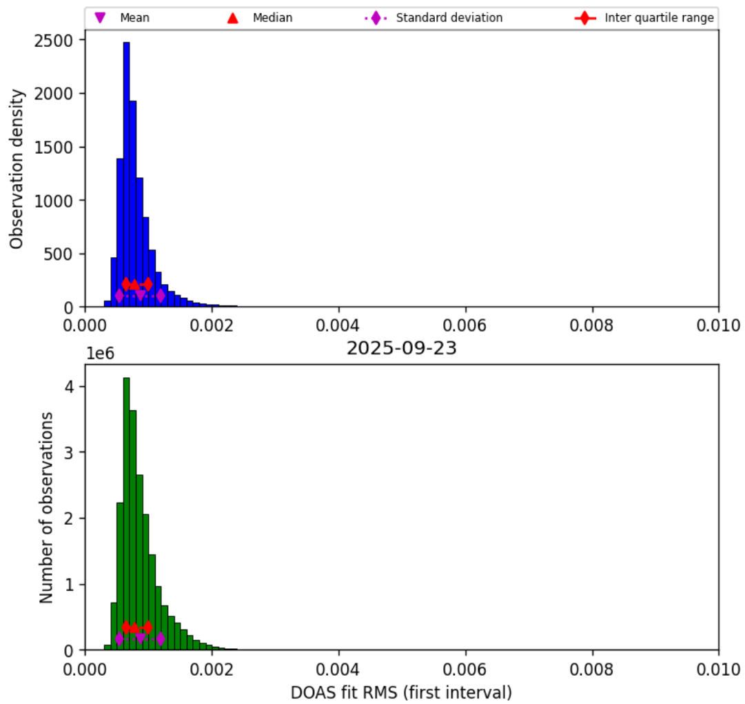
Figure 44: Histogram of “DOAS fit RMS (first interval)” for 2025-09-23 to 2025-09-23
