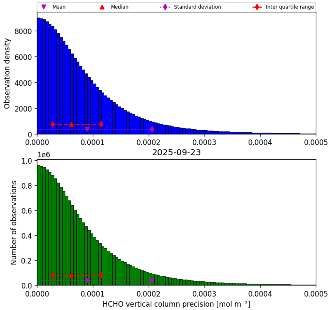
Figure 34: Histogram of “HCHO vertical column precision” for 2025-09-23 to 2025-09-23
