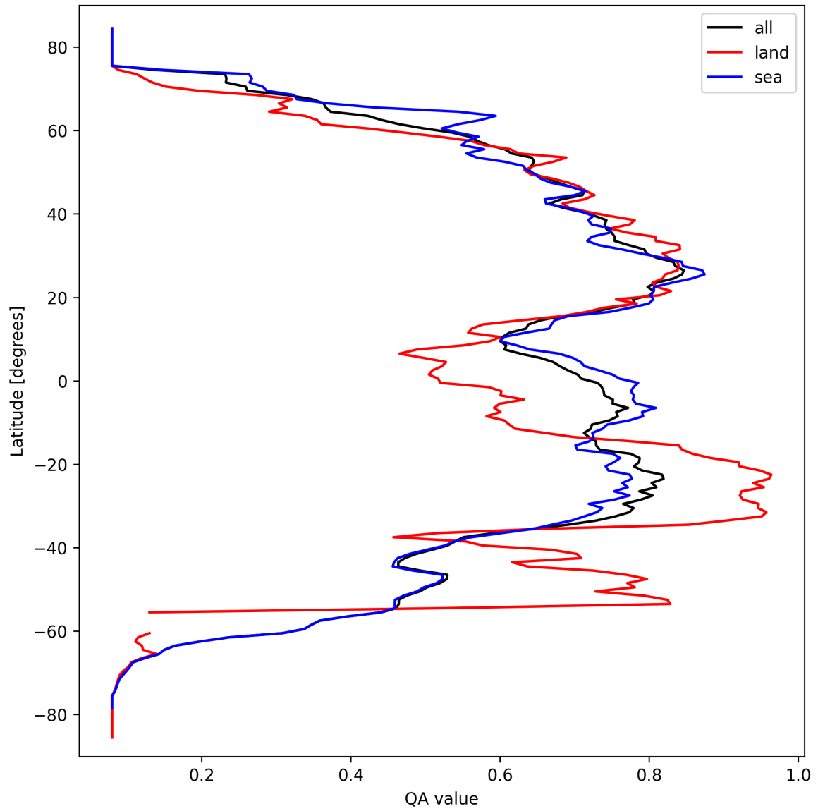
Figure 18: Zonal average of “QA value” for 2025-09-23 to 2025-09-23.
