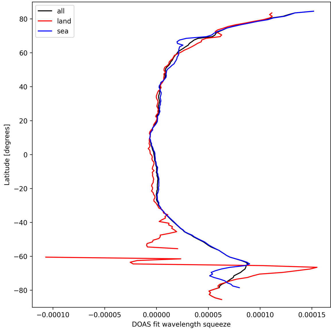
Figure 29: Zonal average of “DOAS fit wavelength squeeze” for 2025-09-23 to 2025-09-23.
