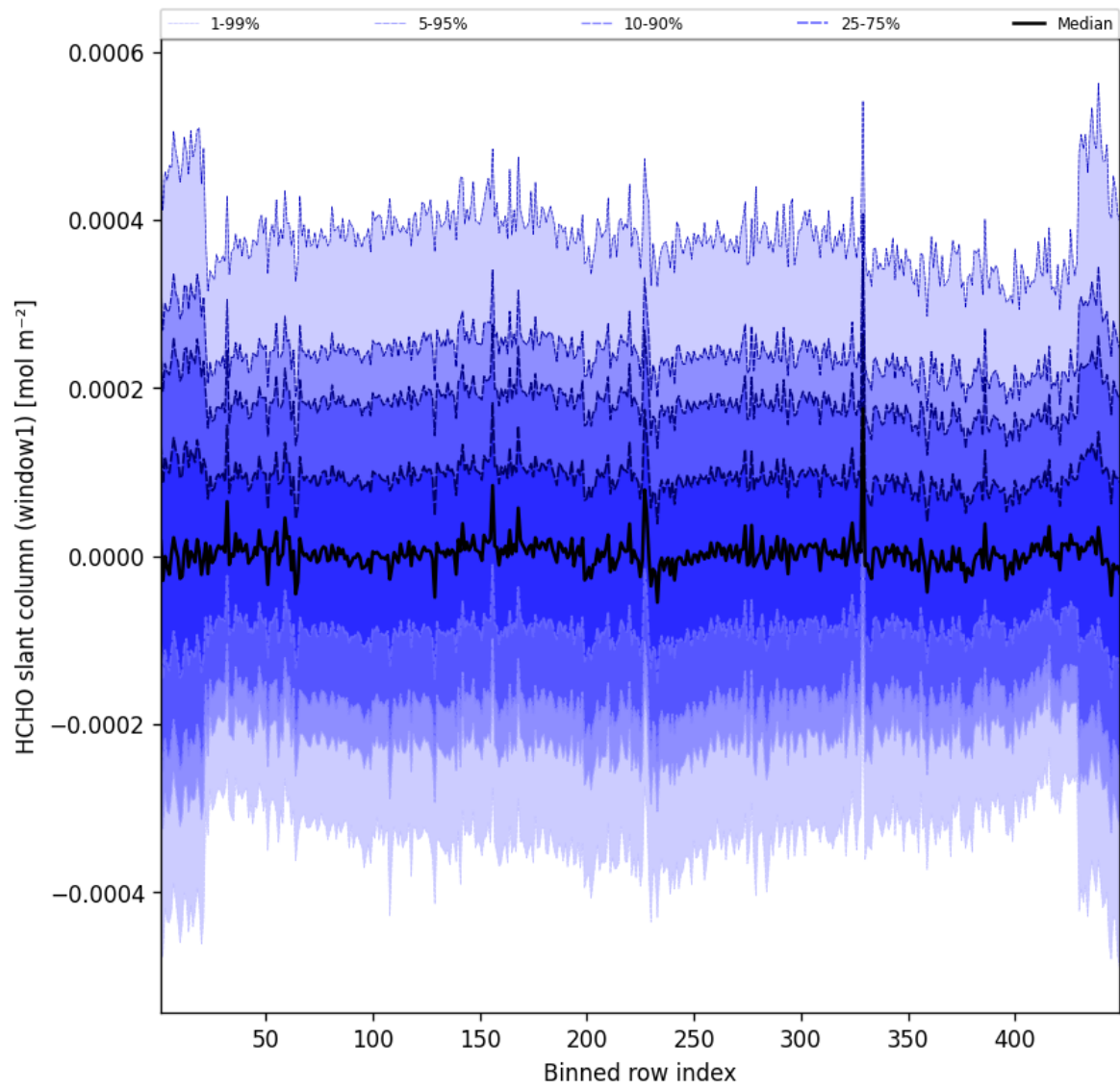
Figure 50: Along track statistics of “HCHO slant column (window1)” for 2025-09-23 to 2025-09-23
