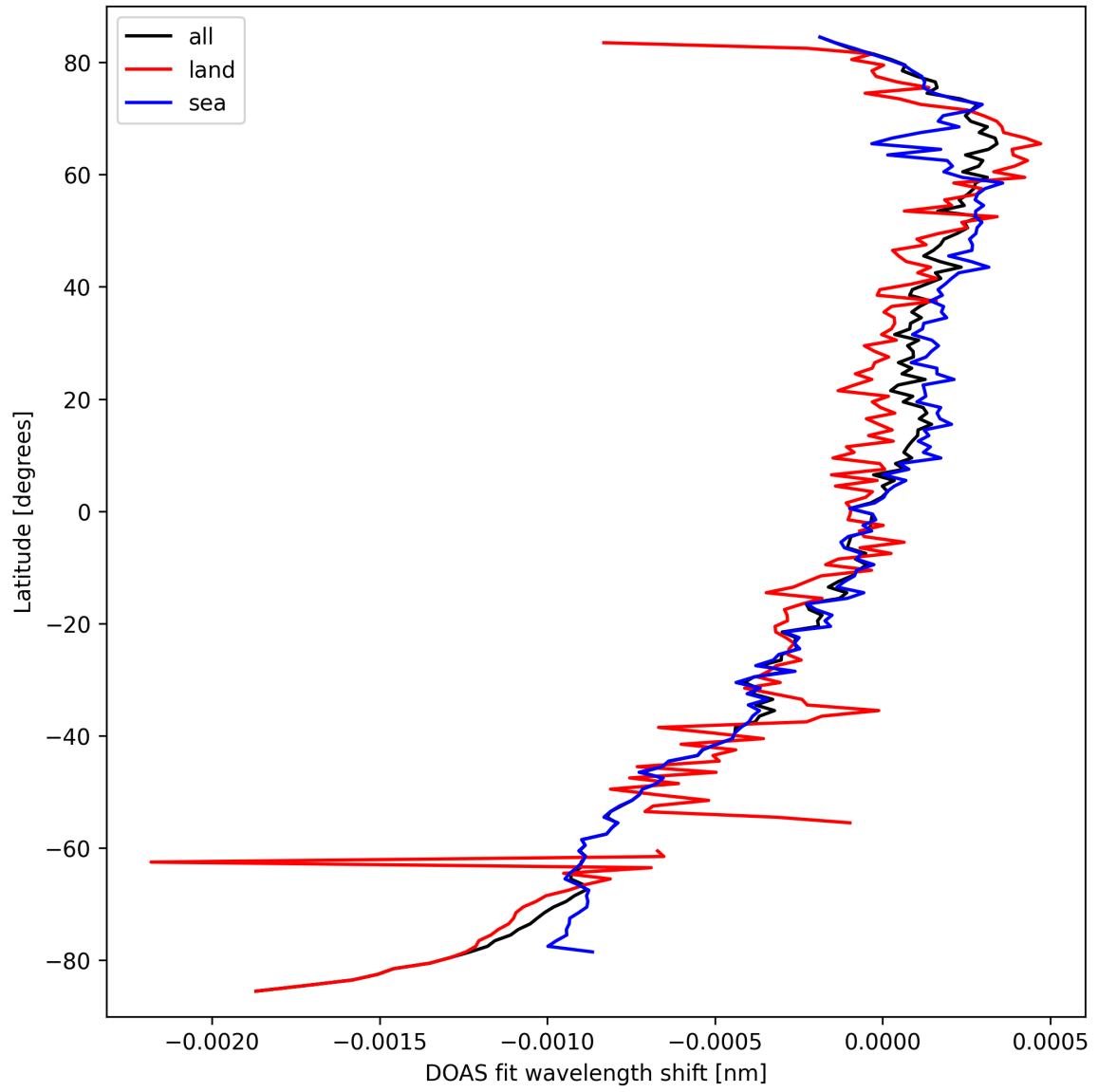
Figure 28: Zonal average of “DOAS fit wavelength shift” for 2025-09-23 to 2025-09-23.
