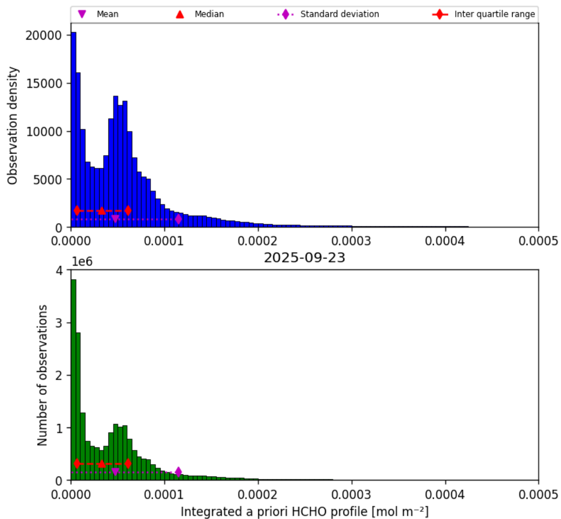
Figure 41: Histogram of “Integrated a priori HCHO profile” for 2025-09-23 to 2025-09-23
