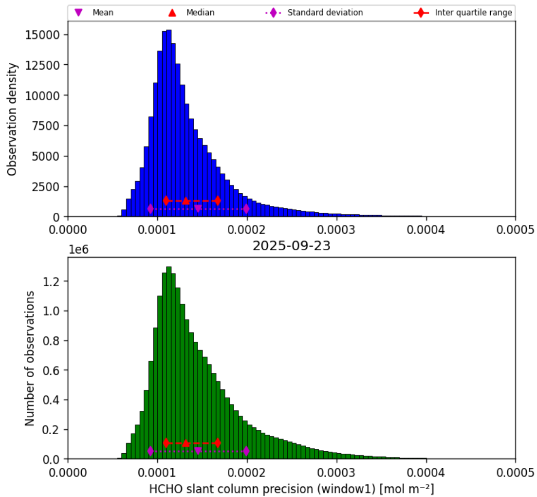
Figure 37: Histogram of “HCHO slant column precision (window1)” for 2025-09-23 to 2025-09-23
