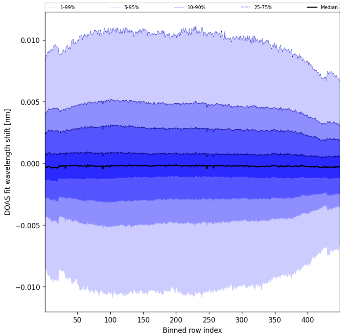
Figure 56: Along track statistics of “DOAS fit wavelength shift” for 2025-09-23 to 2025-09-23
