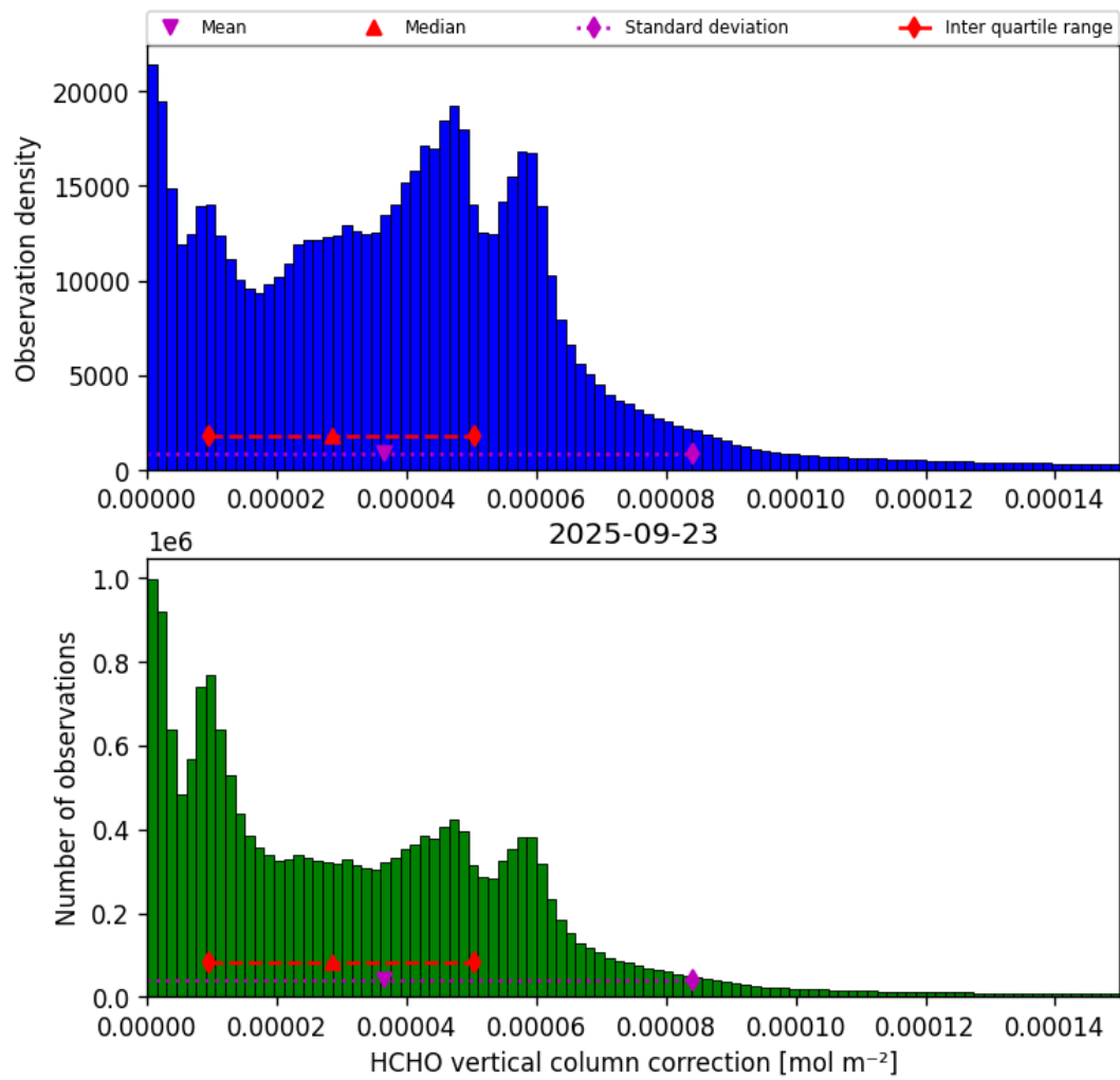
Figure 35: Histogram of “HCHO vertical column correction” for 2025-09-23 to 2025-09-23
