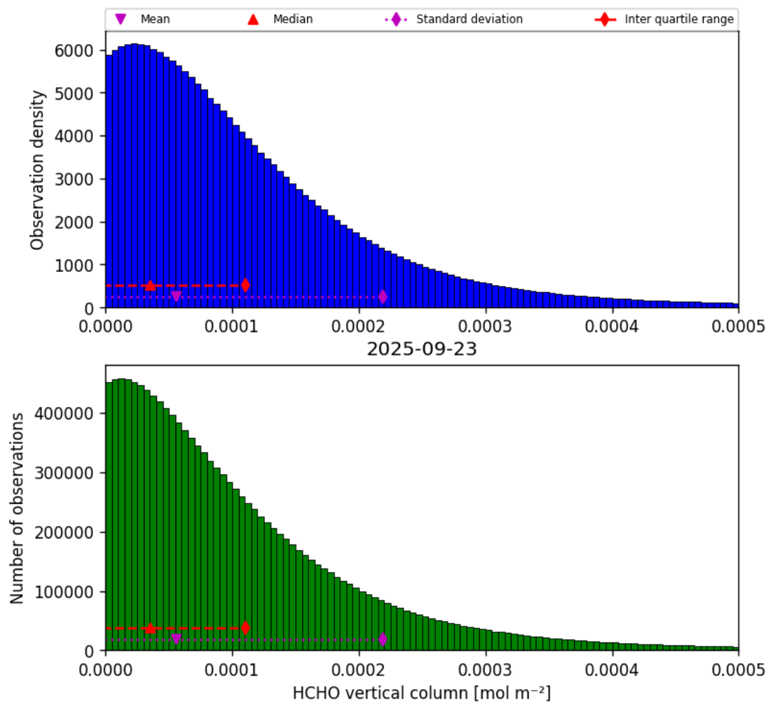
Figure 33: Histogram of “HCHO vertical column” for 2025-09-23 to 2025-09-23
