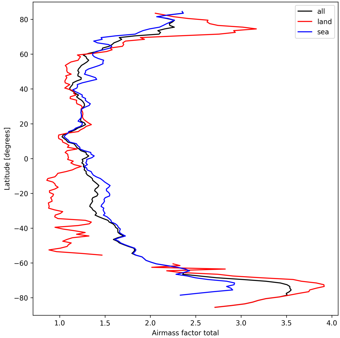
Figure 24: Zonal average of “Airmass factor total” for 2025-09-23 to 2025-09-23.
