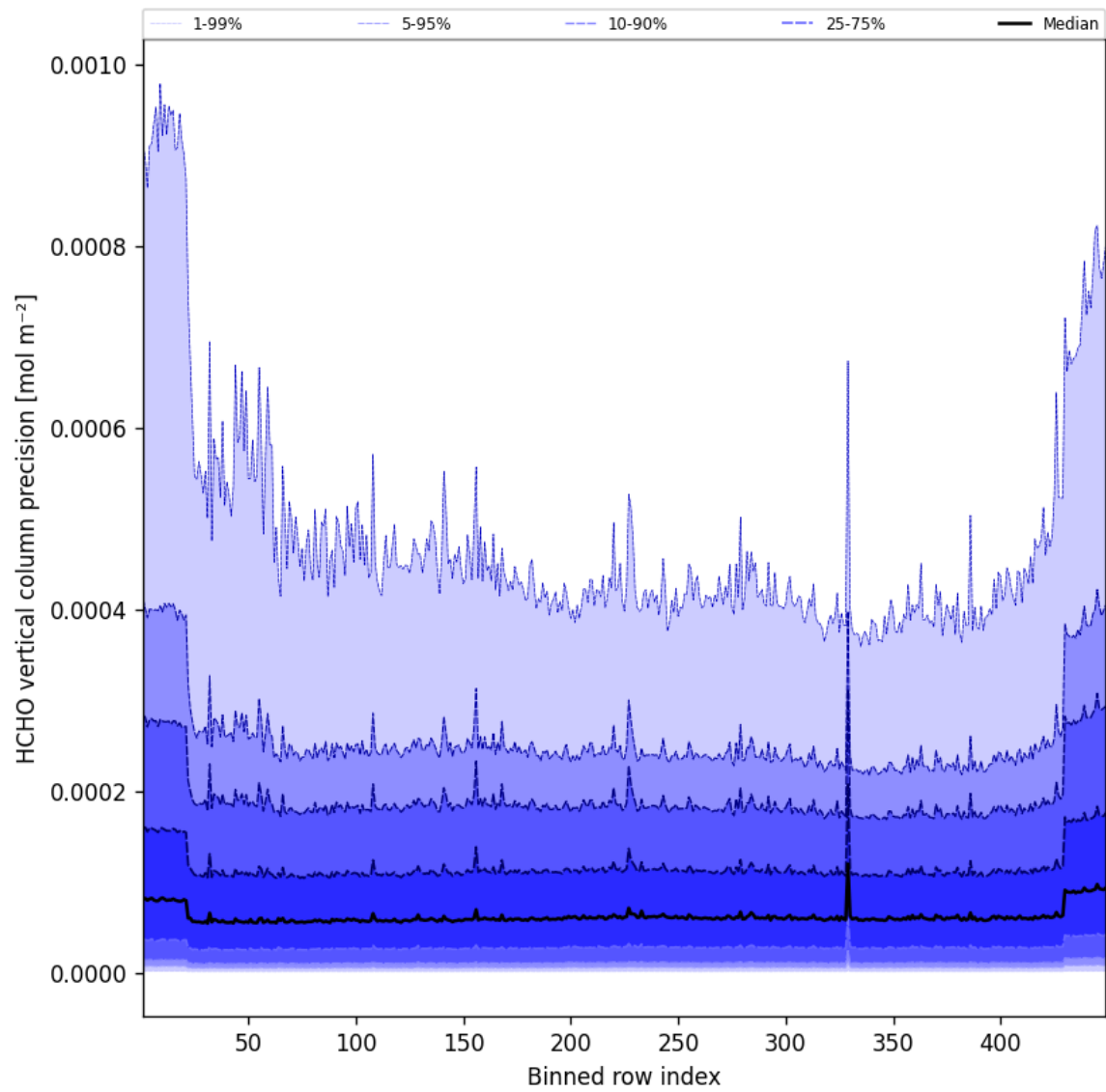
Figure 48: Along track statistics of “HCHO vertical column precision” for 2025-09-23 to 2025-09-23
