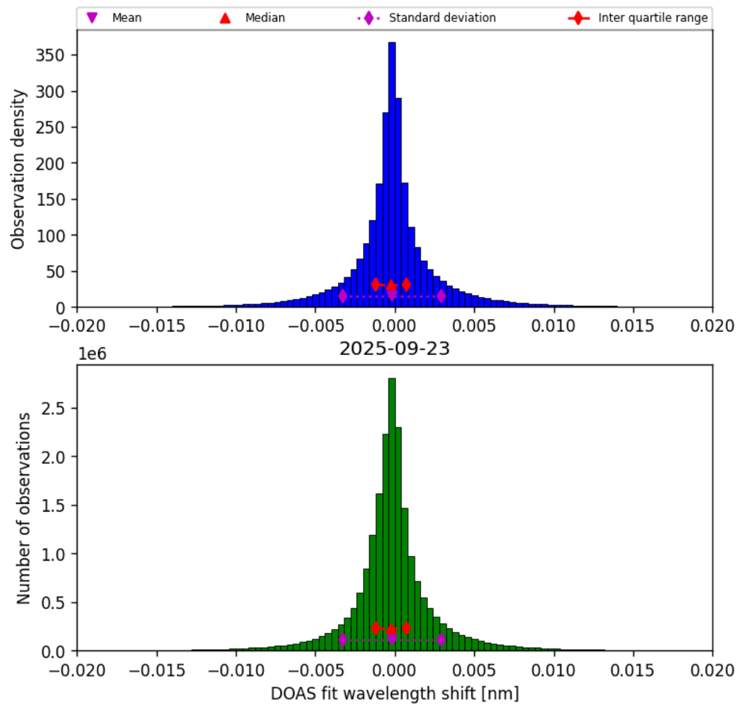
Figure 42: Histogram of “DOAS fit wavelength shift” for 2025-09-23 to 2025-09-23
