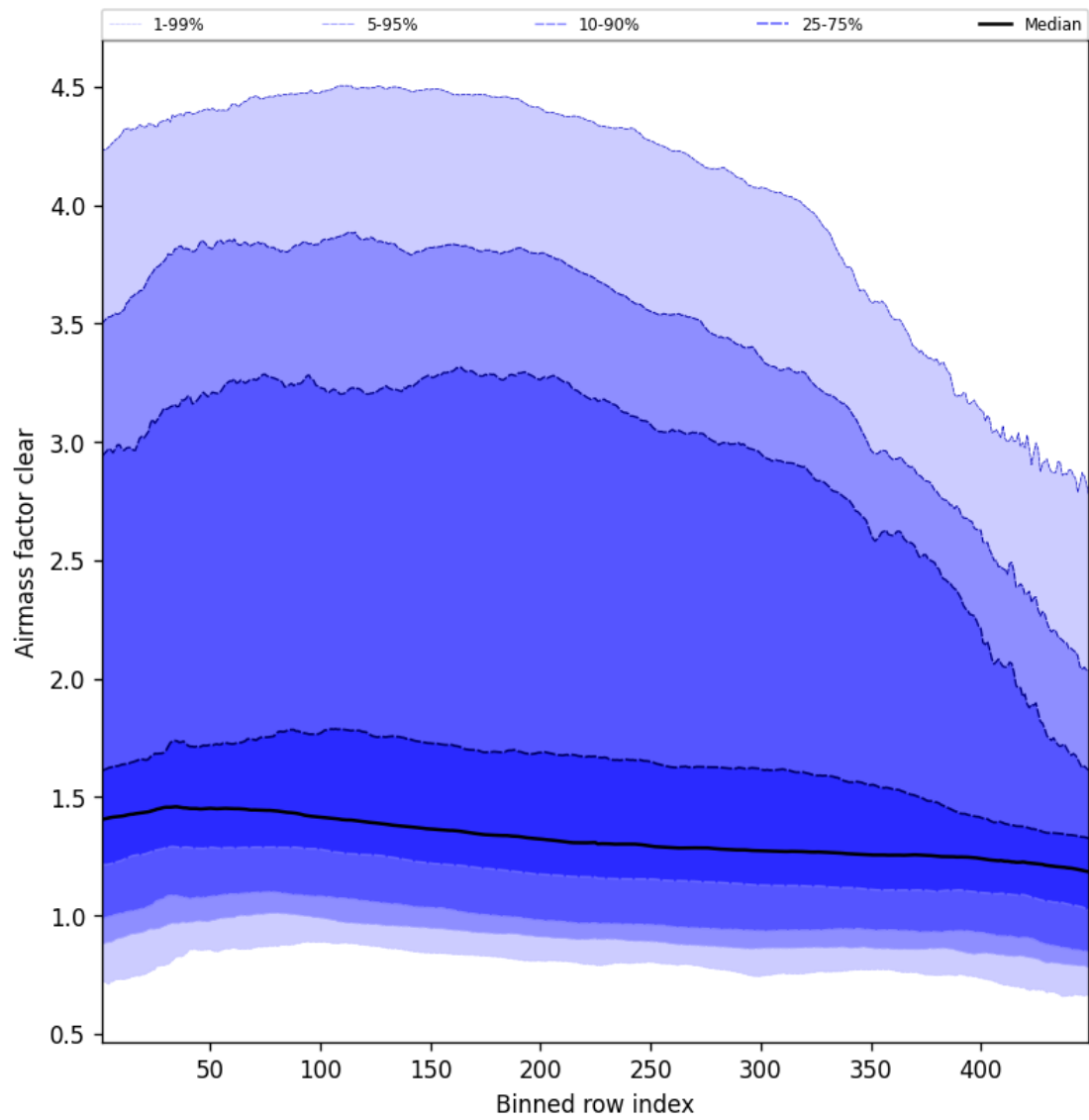
Figure 54: Along track statistics of “Airmass factor clear” for 2025-09-23 to 2025-09-23
