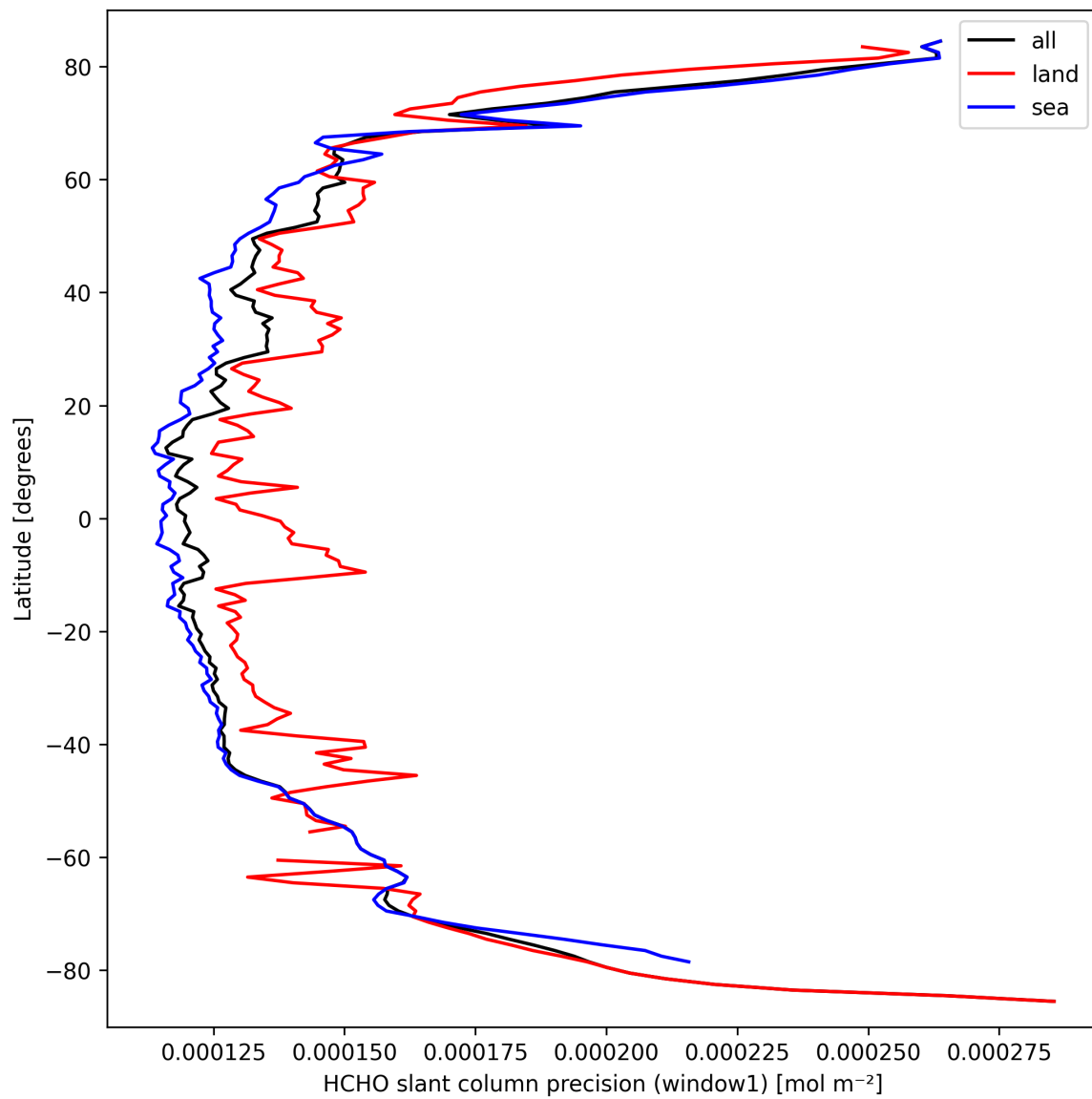
Figure 23: Zonal average of “HCHO slant column precision (window1)” for 2025-09-23 to 2025-09-23.
