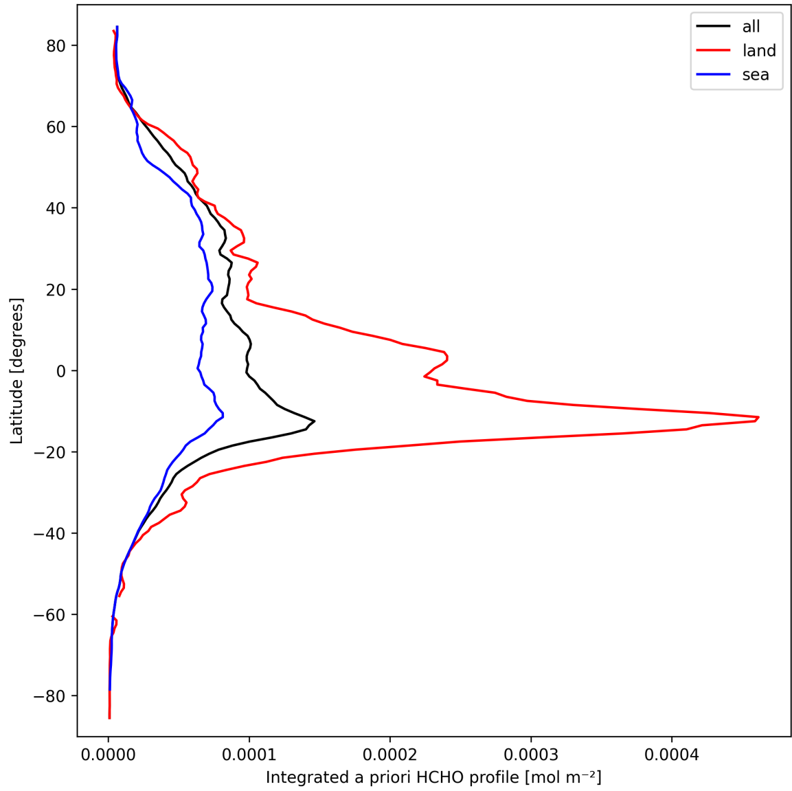
Figure 27: Zonal average of “Integrated a priori HCHO profile” for 2025-09-23 to 2025-09-23.
