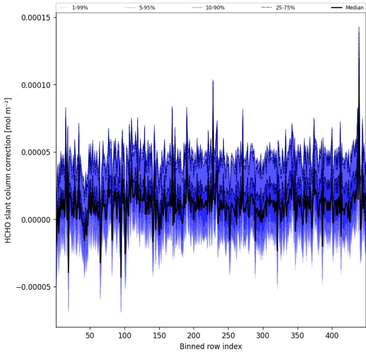
Figure 59: Along track statistics of “HCHO slant column correction” for 2025-09-23 to 2025-09-23
