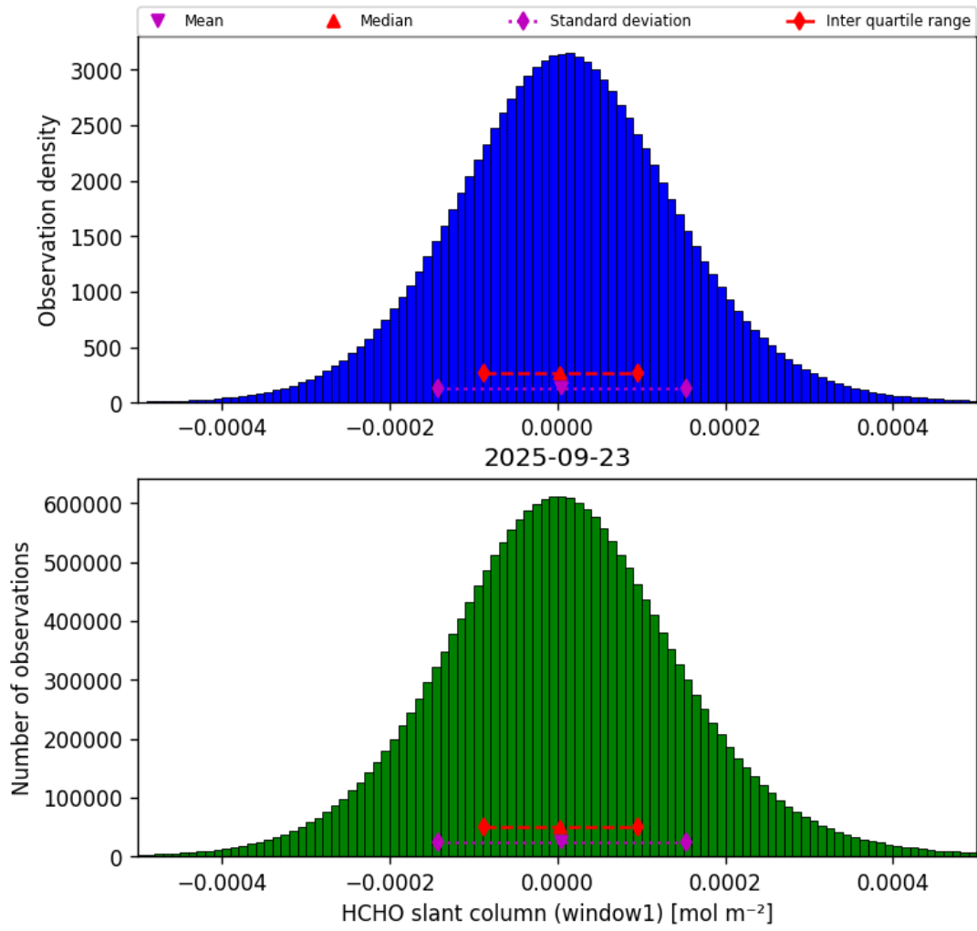
Figure 36: Histogram of “HCHO slant column (window1)” for 2025-09-23 to 2025-09-23
