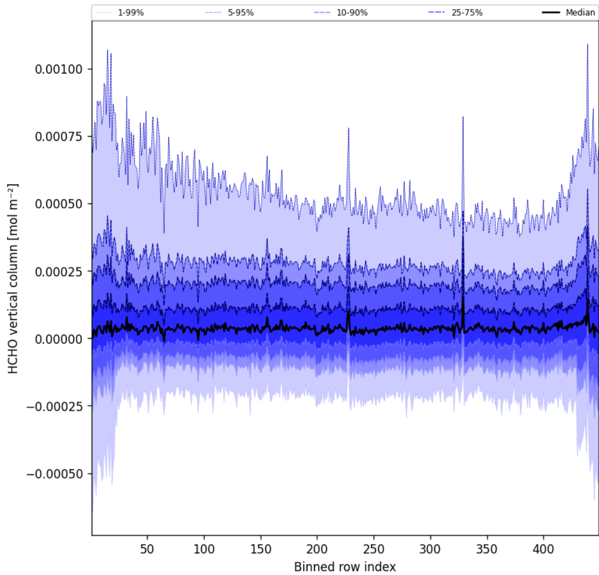
Figure 47: Along track statistics of “HCHO vertical column” for 2025-09-23 to 2025-09-23
