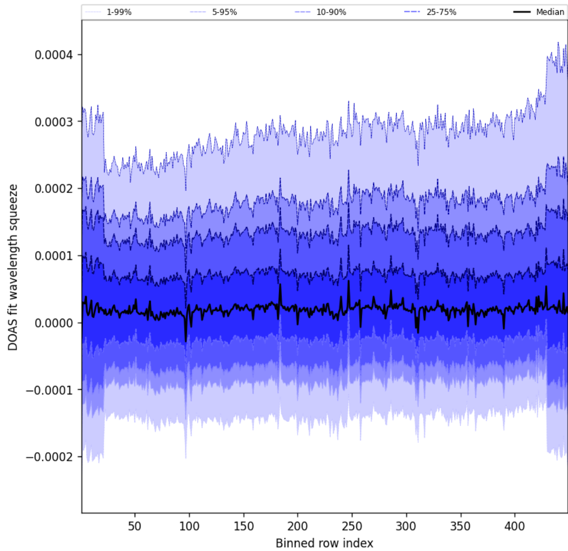
Figure 57: Along track statistics of “DOAS fit wavelength squeeze” for 2025-09-23 to 2025-09-23
