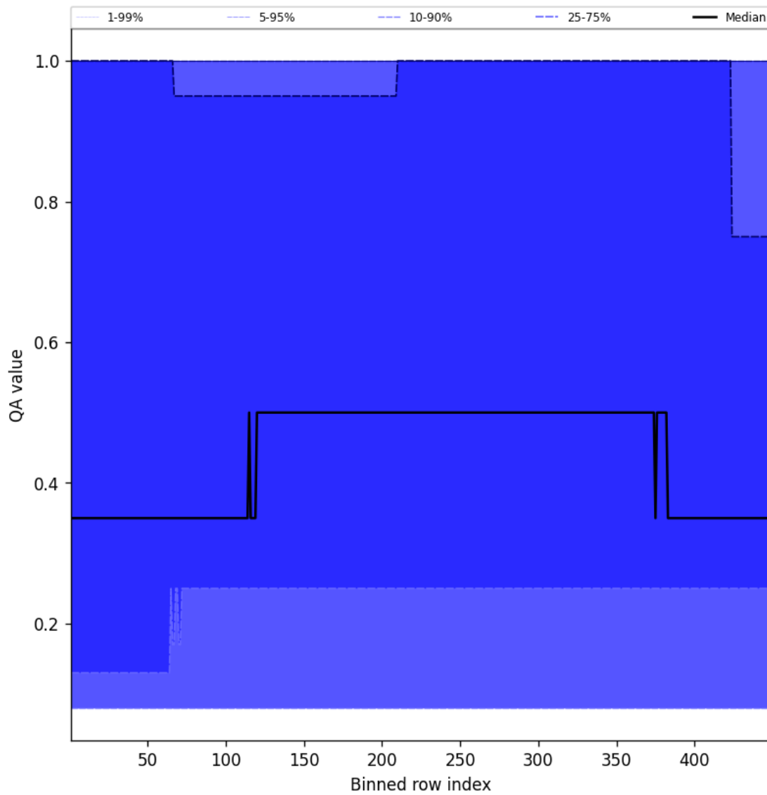
Figure 46: Along track statistics of “QA value” for 2025-09-23 to 2025-09-23
