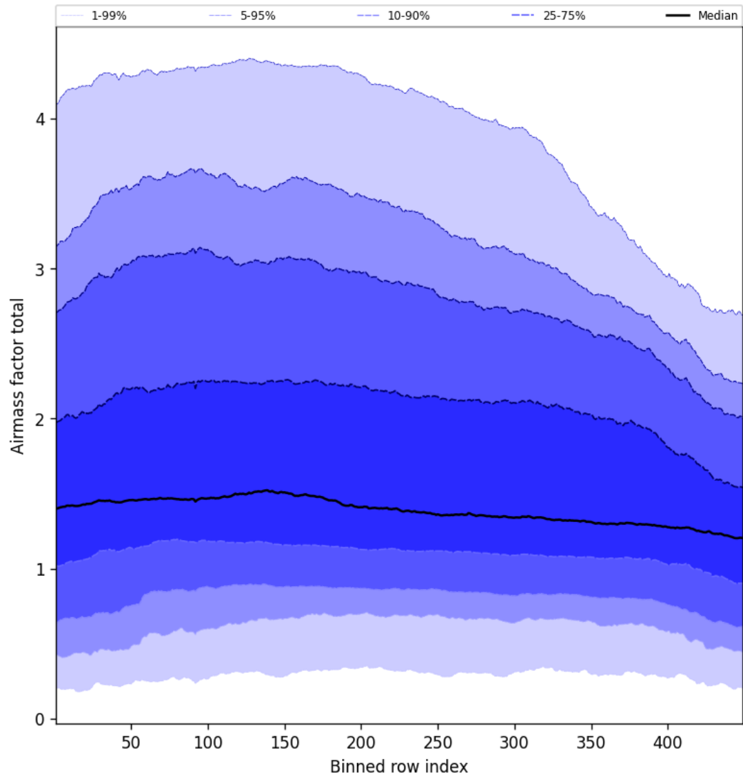
Figure 52: Along track statistics of “Airmass factor total” for 2025-09-23 to 2025-09-23
