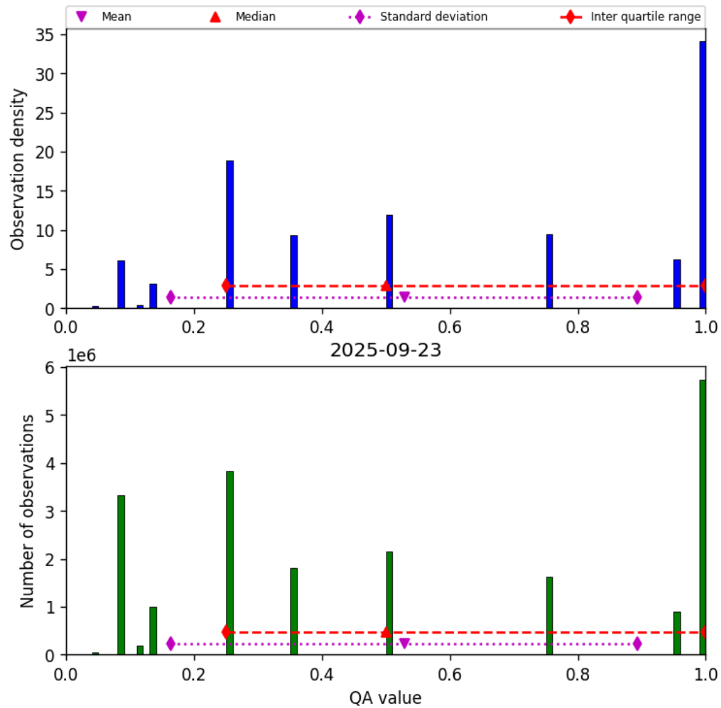
Figure 32: Histogram of “QA value” for 2025-09-23 to 2025-09-23
