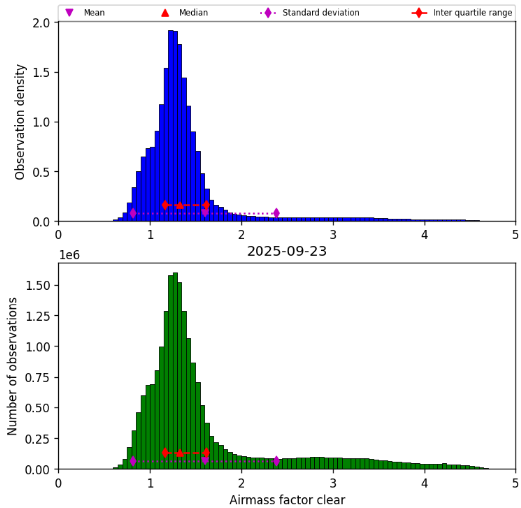
Figure 40: Histogram of “Airmass factor clear” for 2025-09-23 to 2025-09-23
