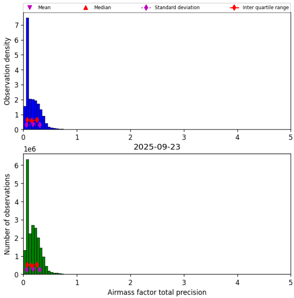
Figure 39: Histogram of “Airmass factor total precision” for 2025-09-23 to 2025-09-23
