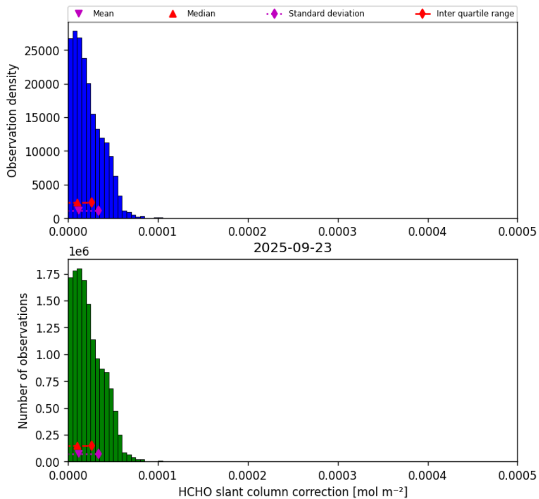
Figure 45: Histogram of “HCHO slant column correction” for 2025-09-23 to 2025-09-23
