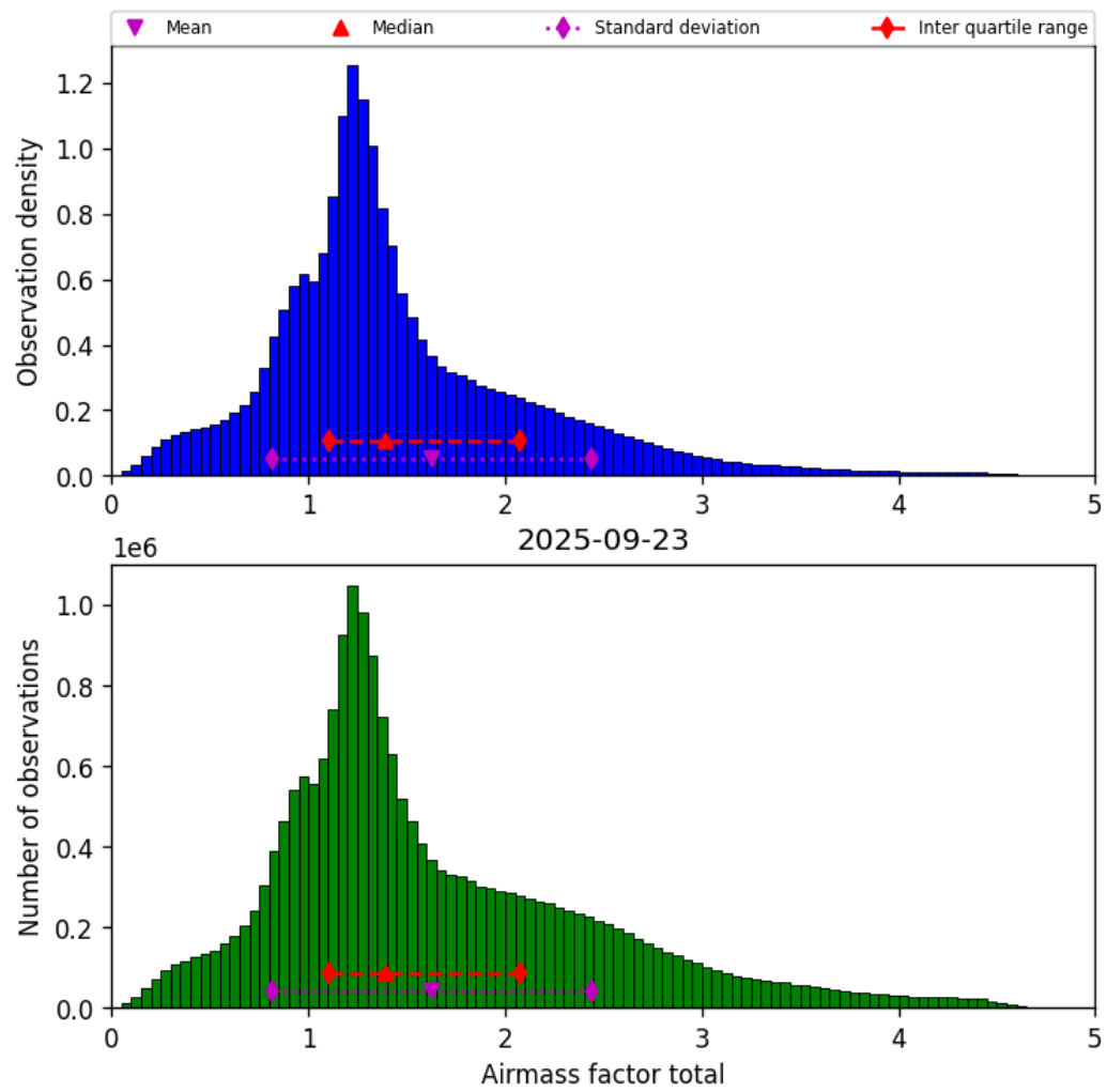
Figure 38: Histogram of “Airmass factor total” for 2025-09-23 to 2025-09-23
