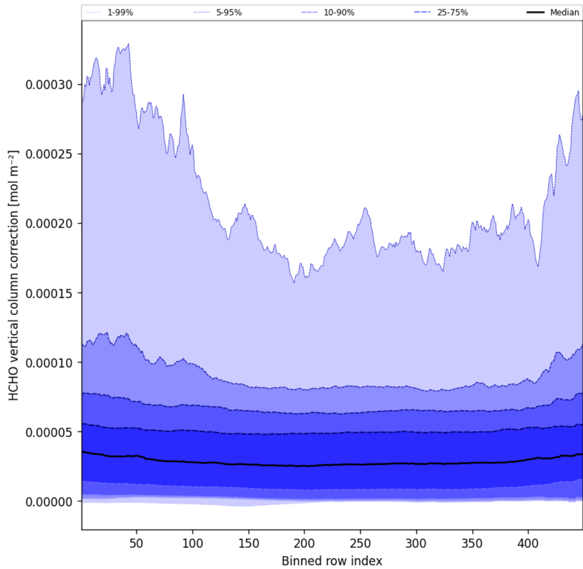
Figure 49: Along track statistics of “HCHO vertical column correction” for 2025-09-23 to 2025-09-23
