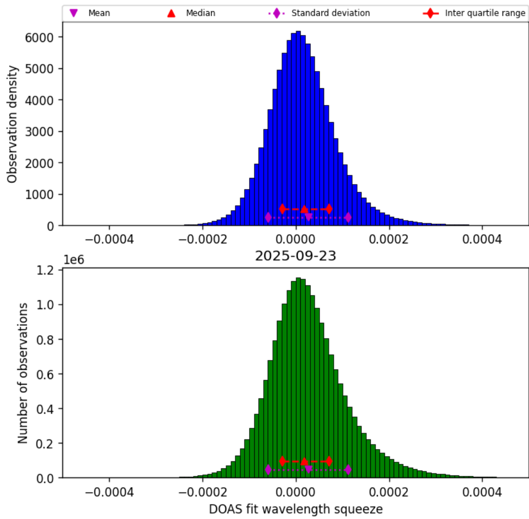
Figure 43: Histogram of “DOAS fit wavelength squeeze” for 2025-09-23 to 2025-09-23
