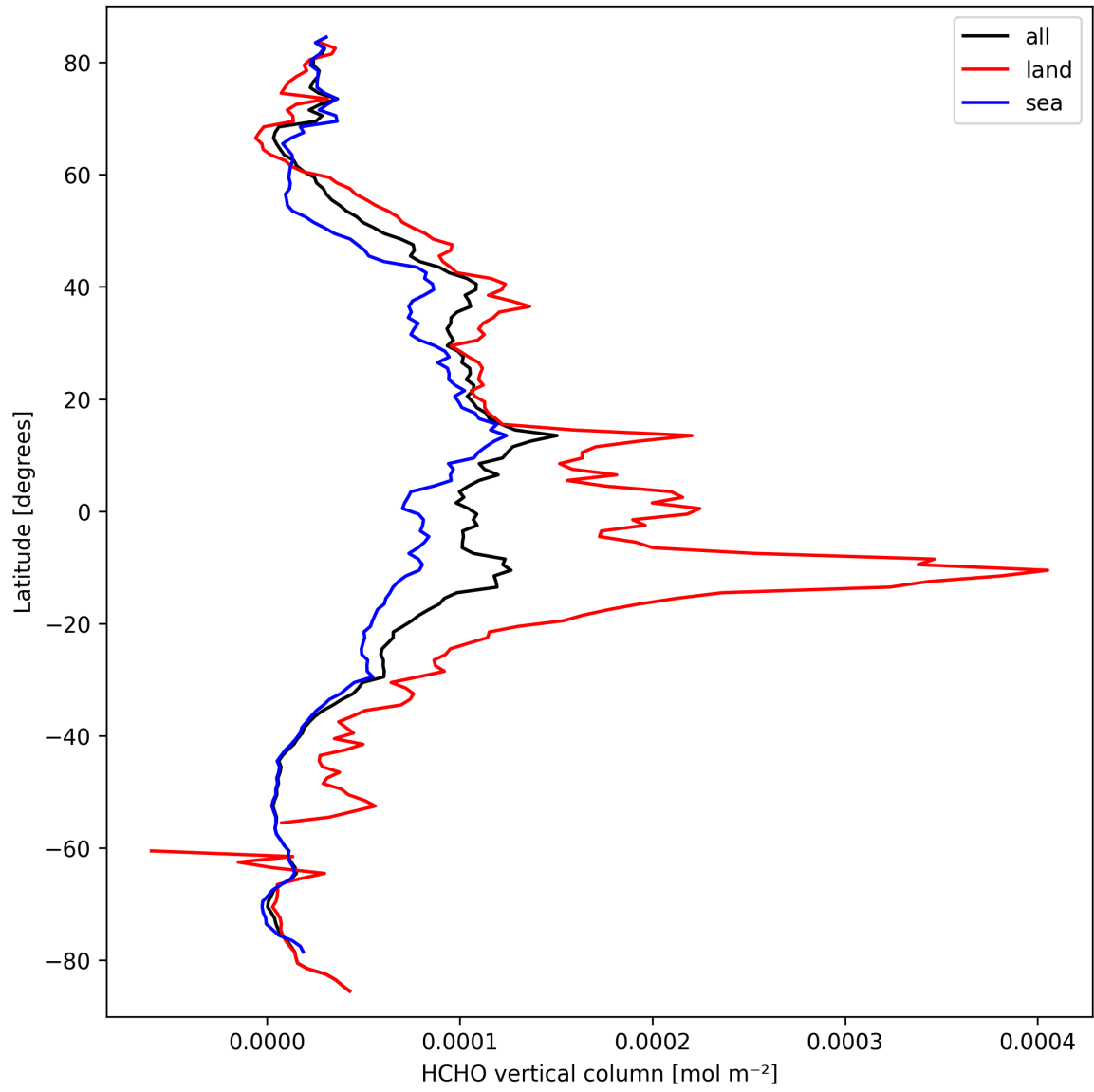
Figure 19: Zonal average of “HCHO vertical column” for 2025-09-23 to 2025-09-23.
