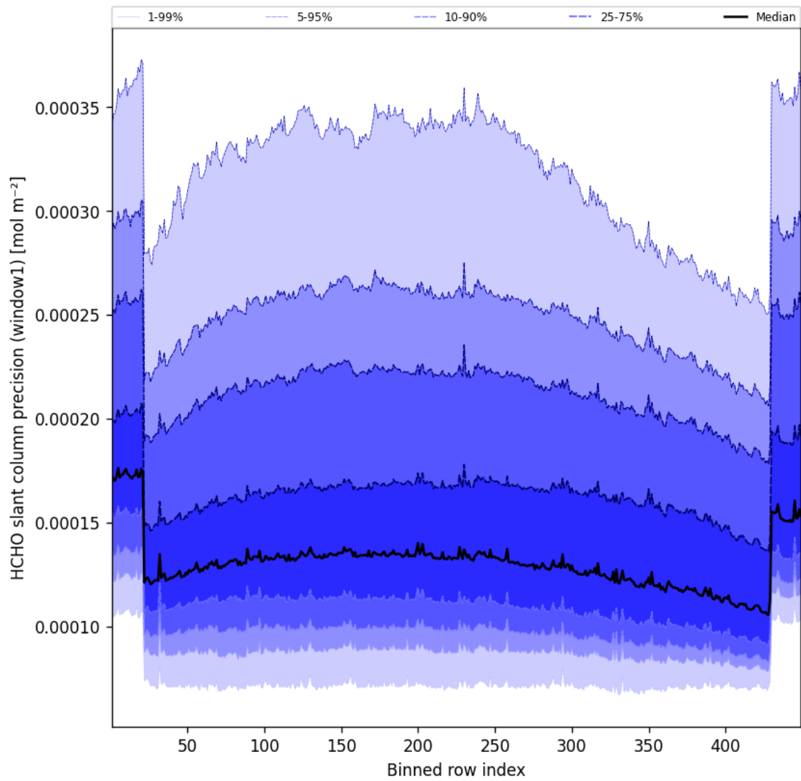
Figure 51: Along track statistics of “HCHO slant column precision (window1)” for 2025-09-23 to 2025-09-23
