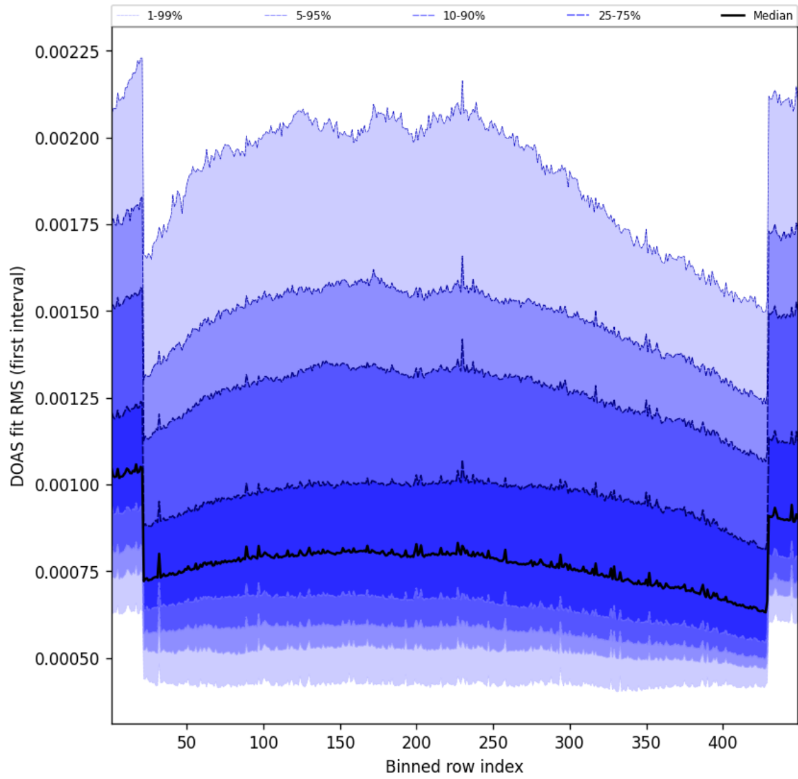
Figure 58: Along track statistics of “DOAS fit RMS (first interval)” for 2025-09-23 to 2025-09-23
