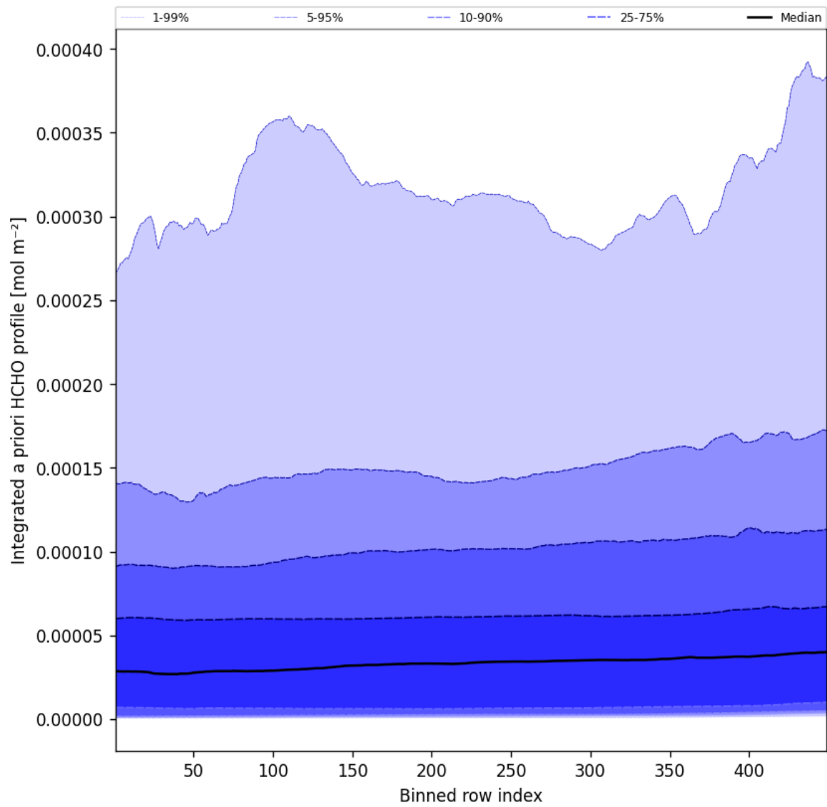
Figure 55: Along track statistics of “Integrated a priori HCHO profile” for 2025-09-23 to 2025-09-23
