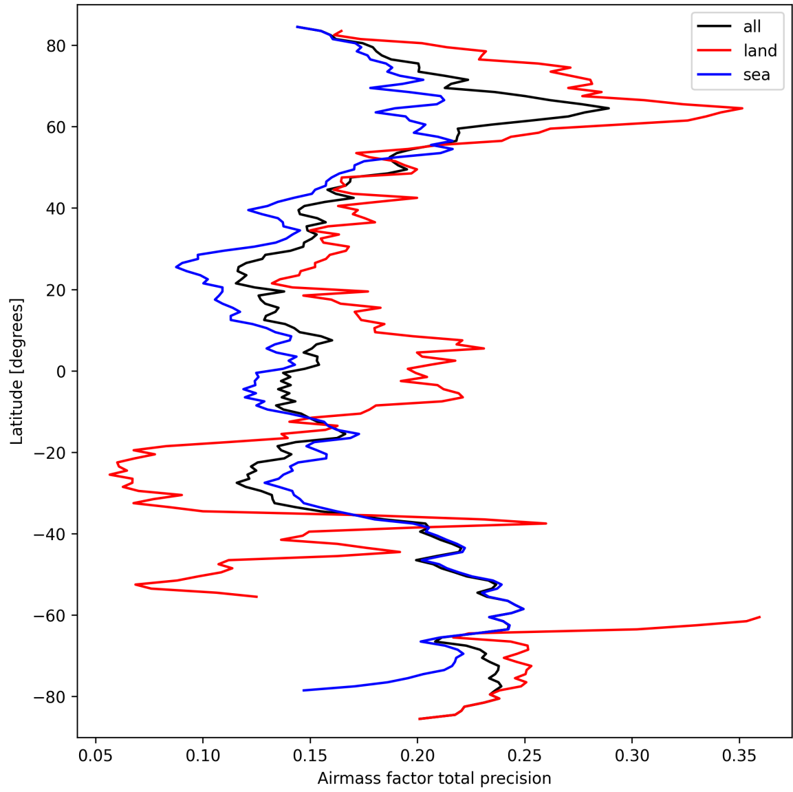
Figure 25: Zonal average of “Airmass factor total precision” for 2025-09-23 to 2025-09-23.
