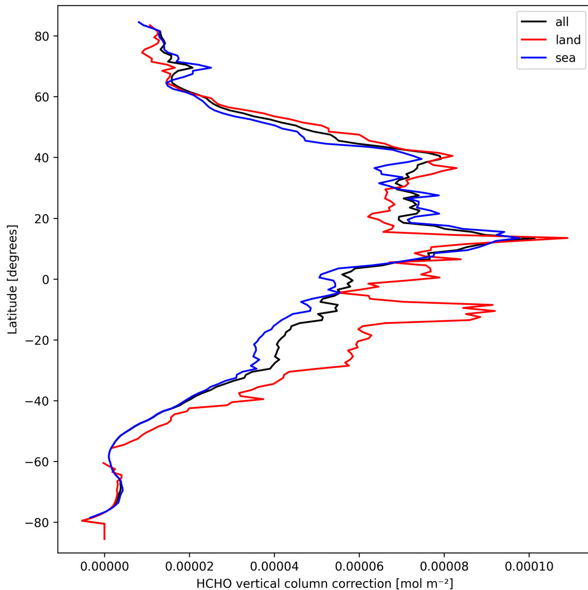
Figure 21: Zonal average of “HCHO vertical column correction” for 2025-09-23 to 2025-09-23.
