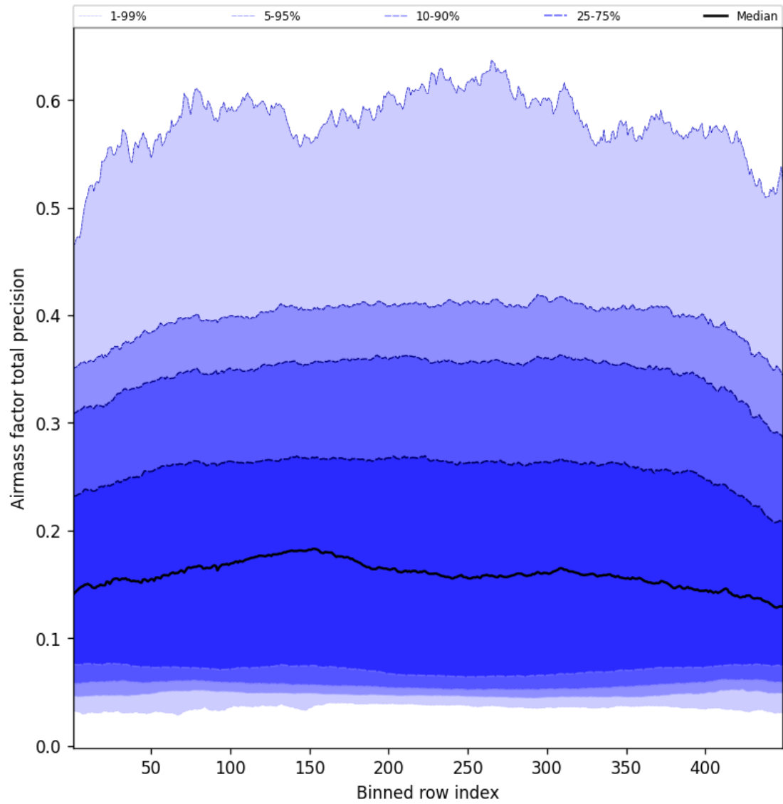
Figure 53: Along track statistics of “Airmass factor total precision” for 2025-09-23 to 2025-09-23
