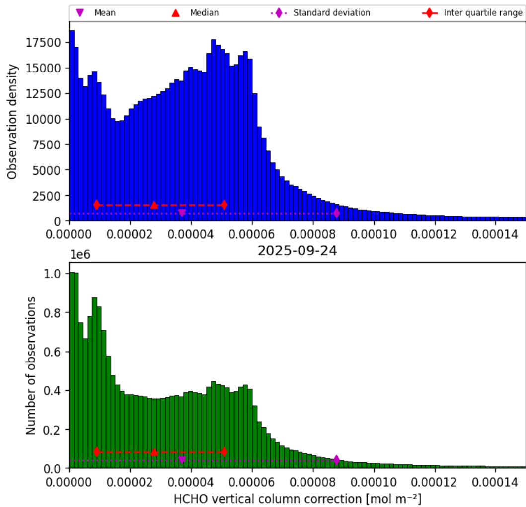
Figure 35: Histogram of “HCHO vertical column correction” for 2025-09-24 to 2025-09-25
