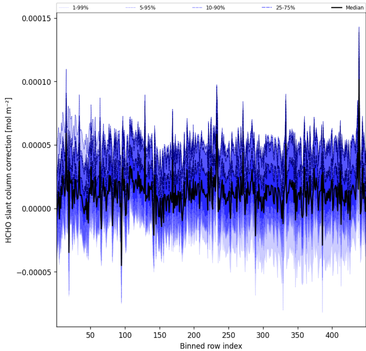
Figure 59: Along track statistics of “HCHO slant column correction” for 2025-09-24 to 2025-09-25
