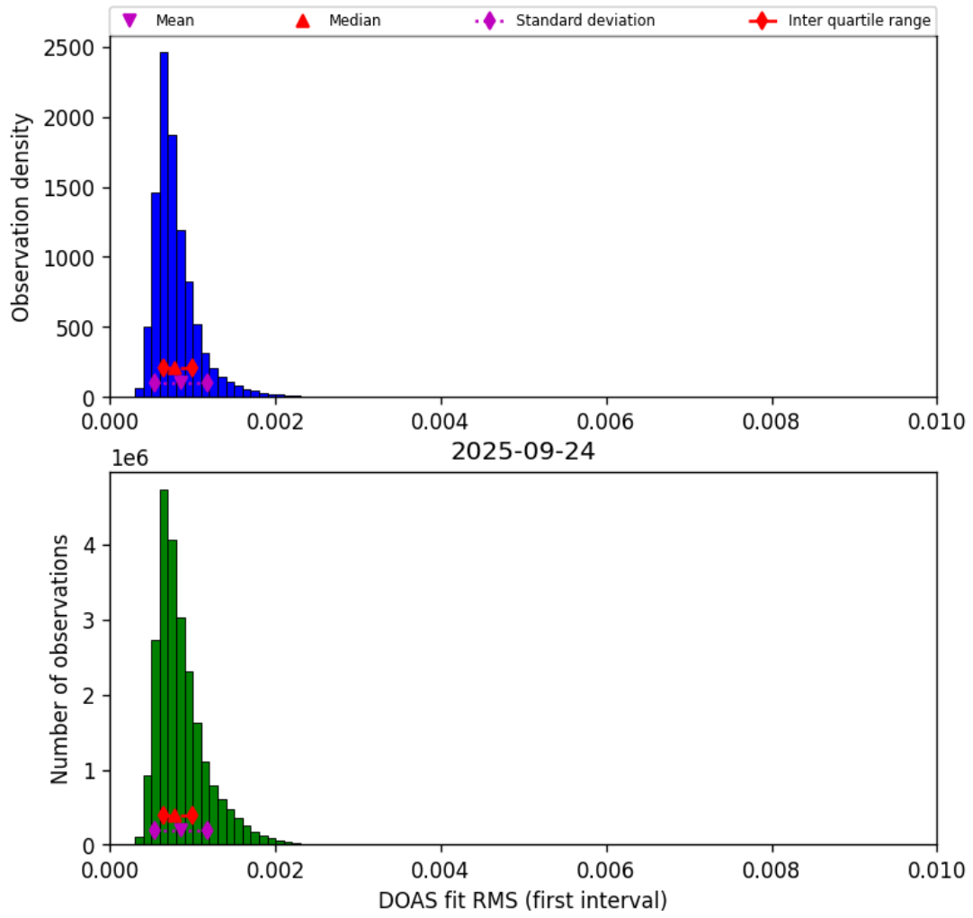
Figure 44: Histogram of “DOAS fit RMS (first interval)” for 2025-09-24 to 2025-09-25
