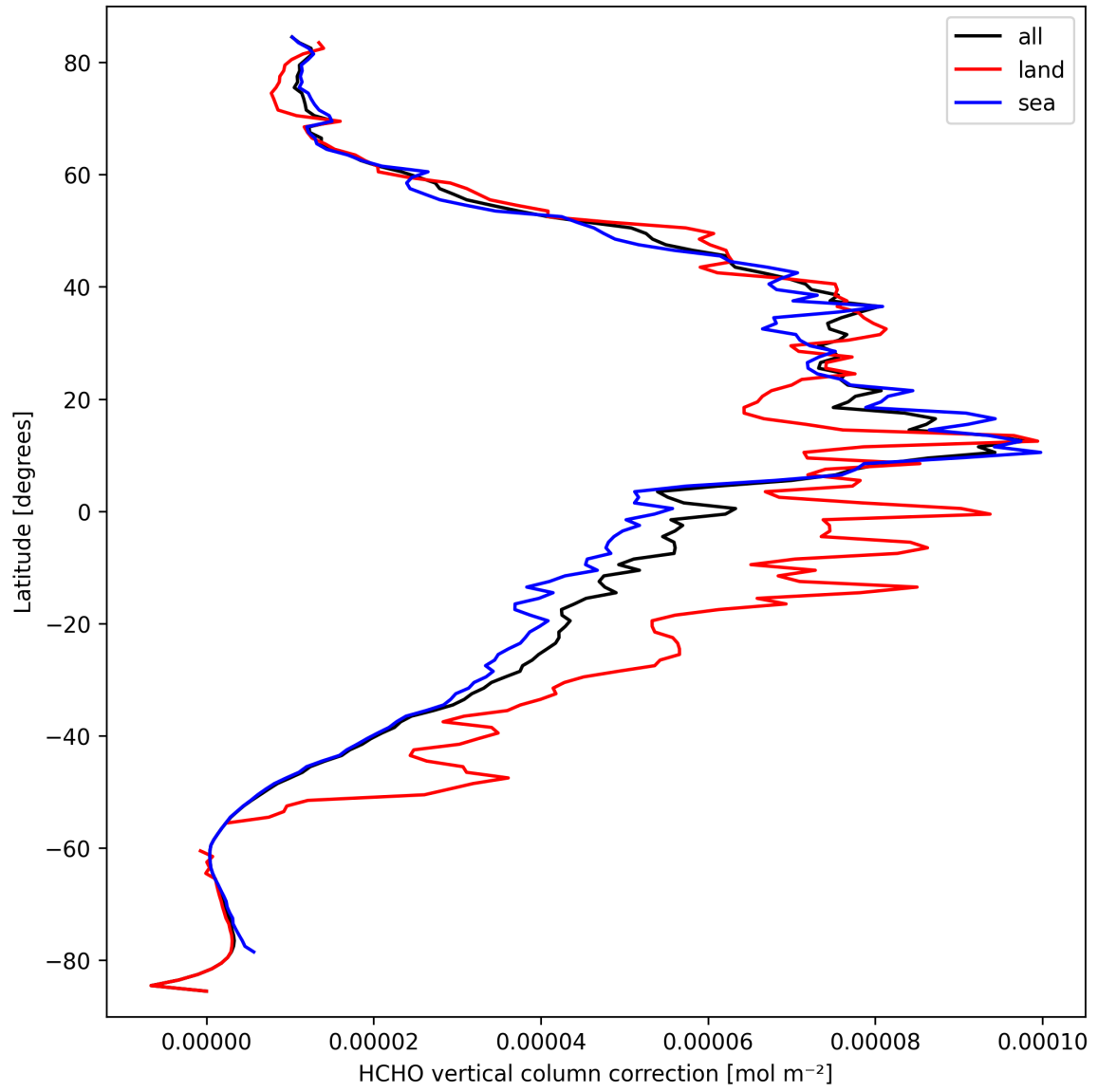
Figure 21: Zonal average of “HCHO vertical column correction” for 2025-09-24 to 2025-09-25.
