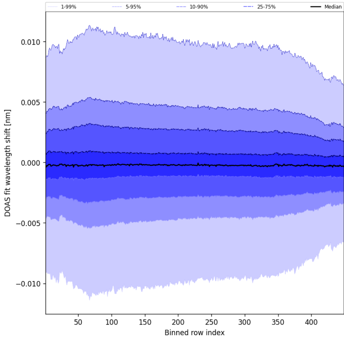
Figure 56: Along track statistics of “DOAS fit wavelength shift” for 2025-09-24 to 2025-09-25
