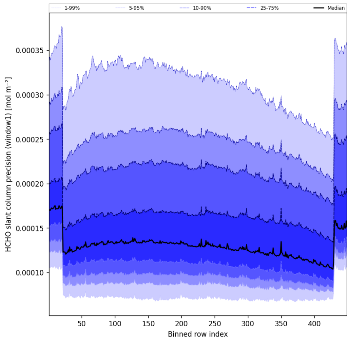
Figure 51: Along track statistics of “HCHO slant column precision (window1)” for 2025-09-24 to 2025-09-25
