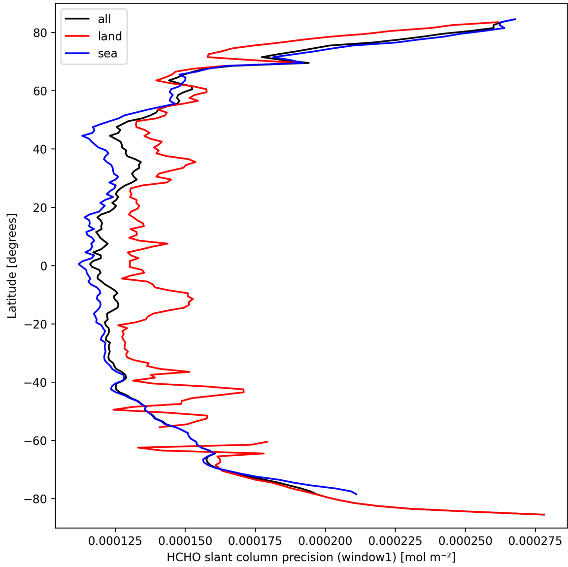
Figure 23: Zonal average of “HCHO slant column precision (window1)” for 2025-09-24 to 2025-09-25.
