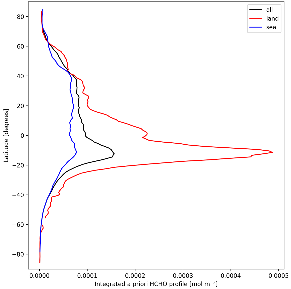
Figure 27: Zonal average of “Integrated a priori HCHO profile” for 2025-09-24 to 2025-09-25.
