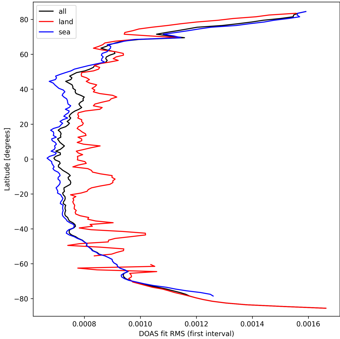
Figure 30: Zonal average of “DOAS fit RMS (first interval)” for 2025-09-24 to 2025-09-25.
