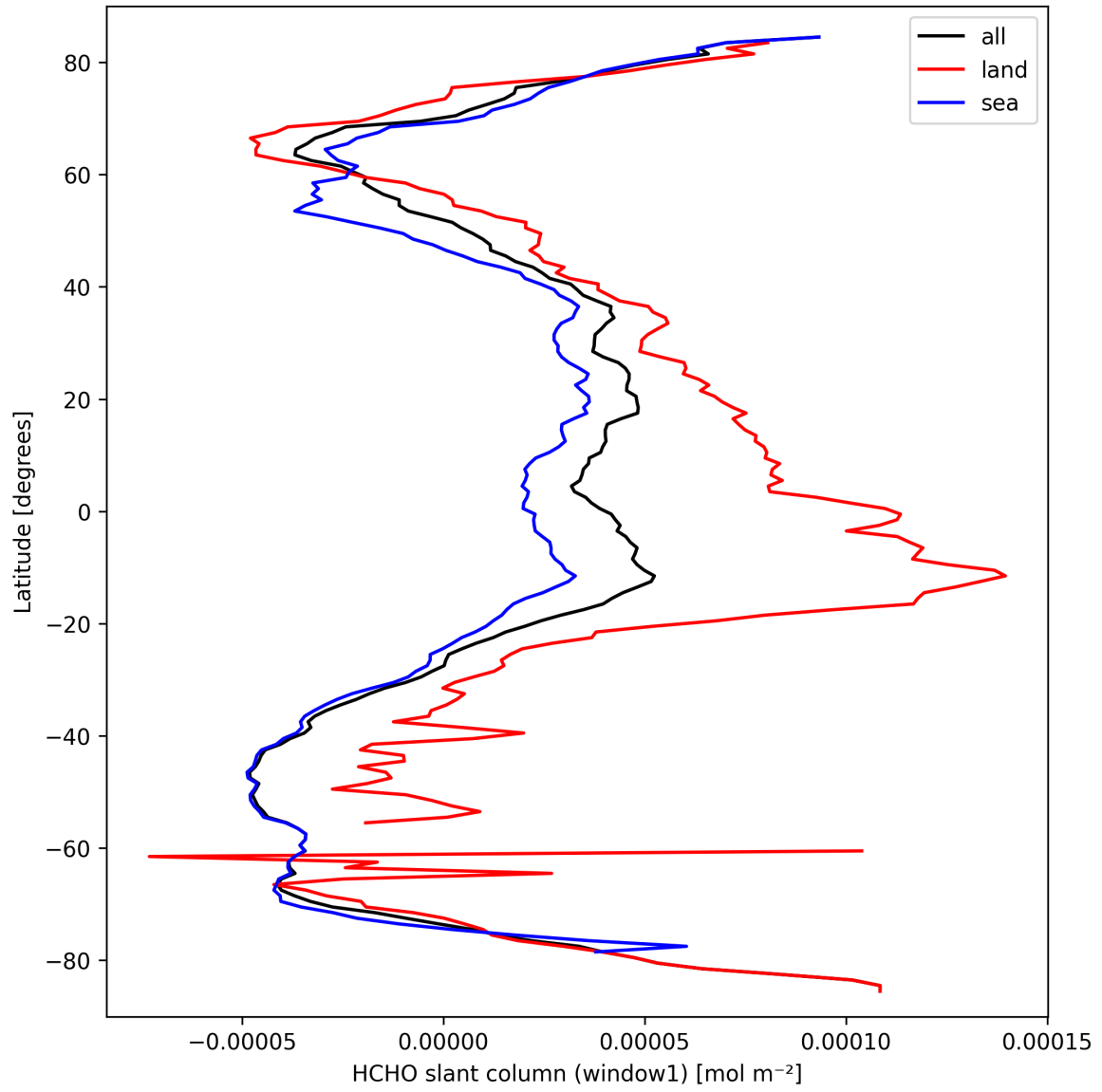
Figure 22: Zonal average of “HCHO slant column (window1)” for 2025-09-24 to 2025-09-25.
