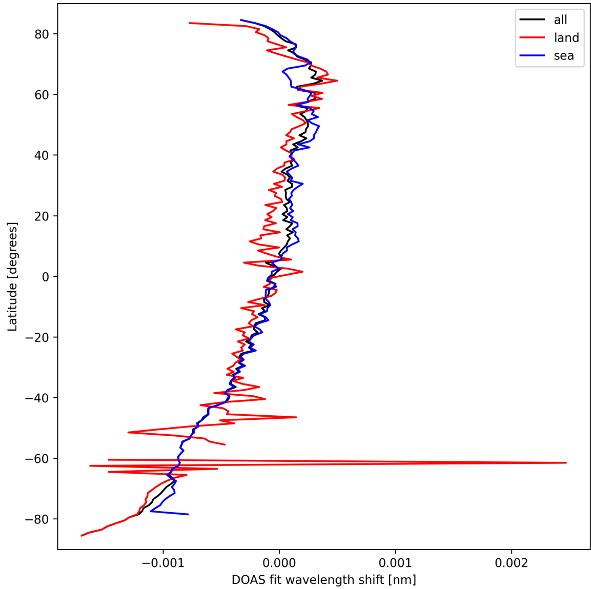
Figure 28: Zonal average of "DOAS fit wavelength shift" for 2025-09-24 to 2025-09-25.
