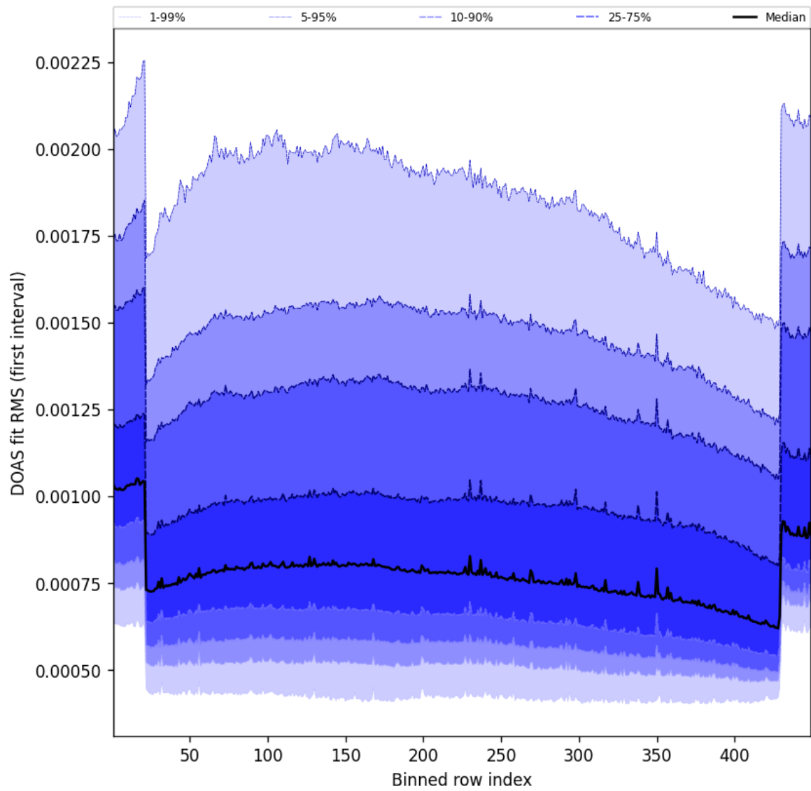
Figure 58: Along track statistics of “DOAS fit RMS (first interval)” for 2025-09-24 to 2025-09-25
