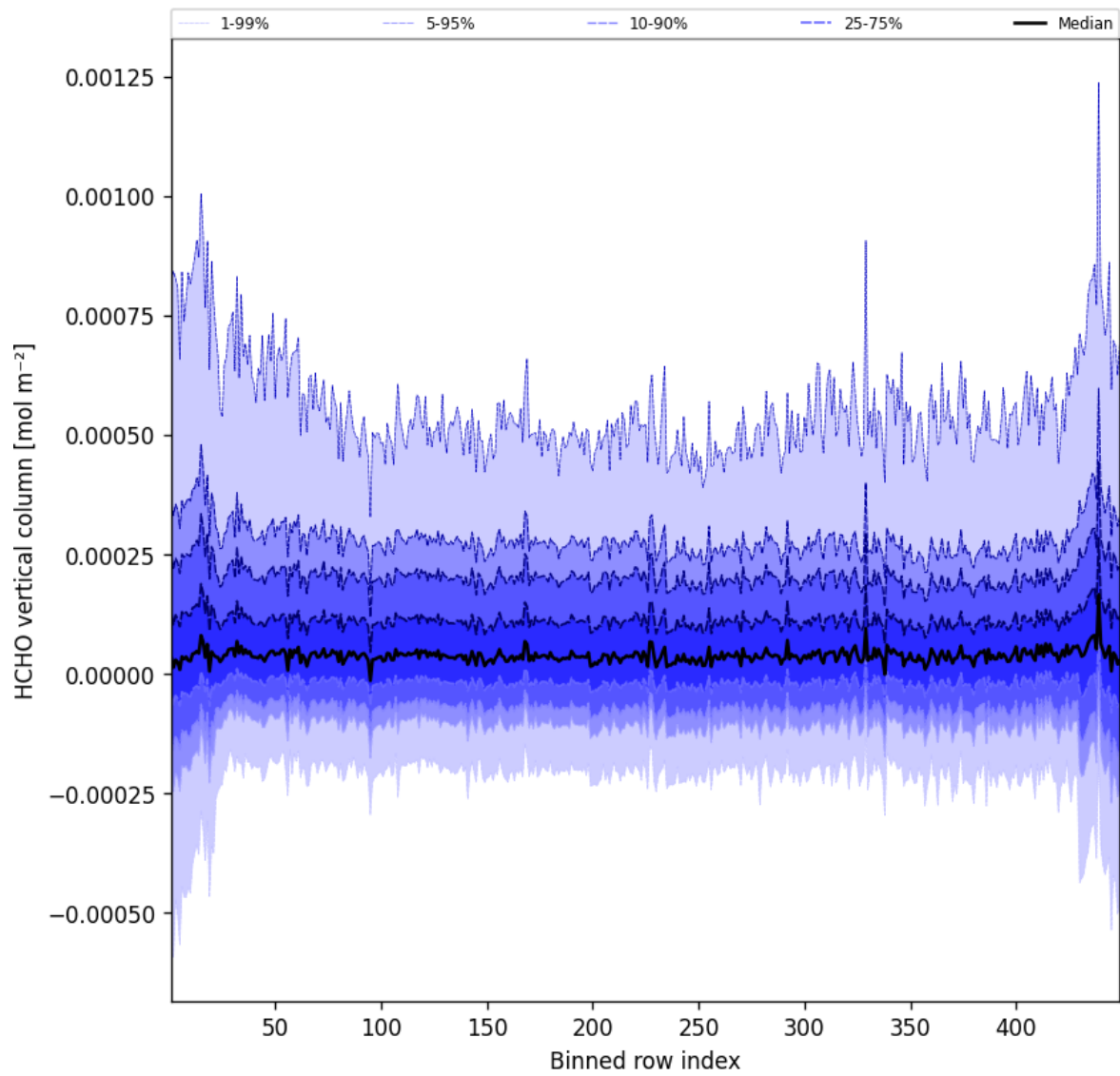
Figure 47: Along track statistics of “HCHO vertical column” for 2025-09-24 to 2025-09-25
