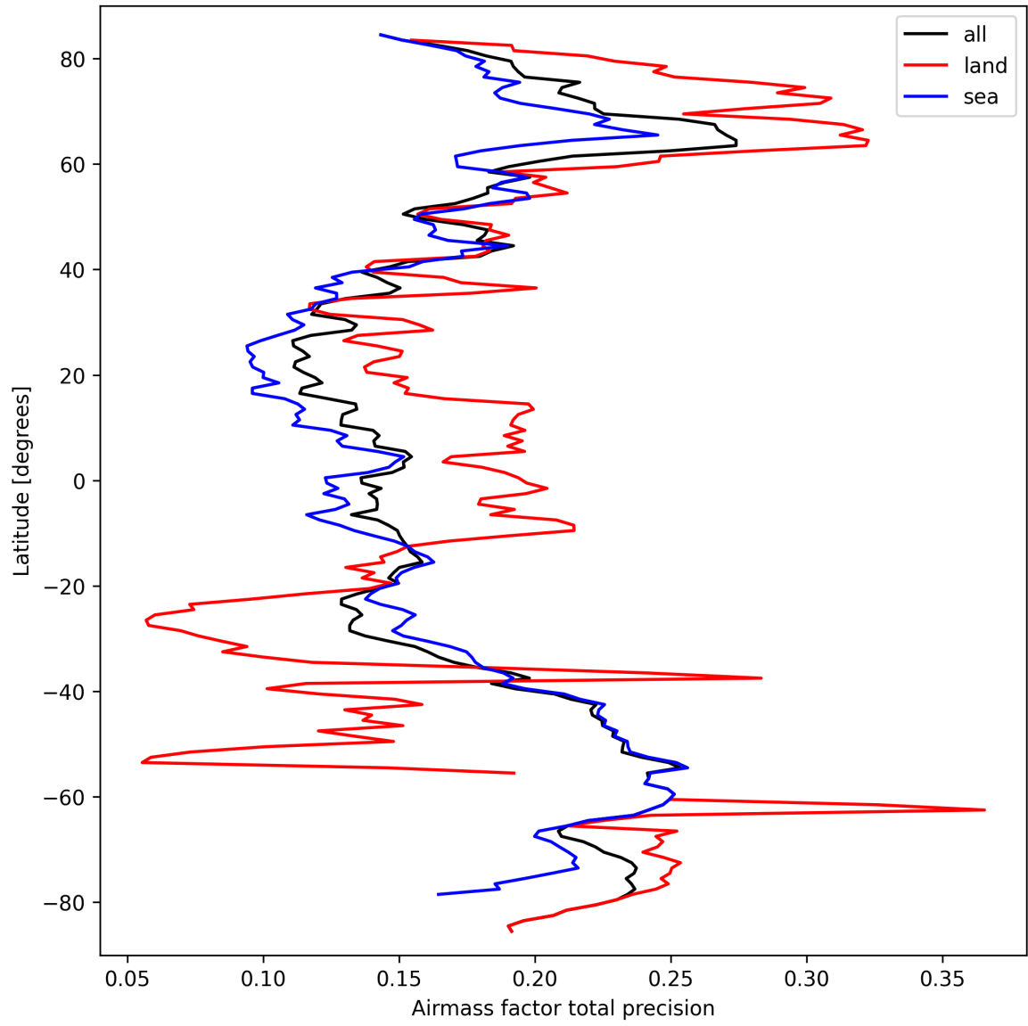
Figure 25: Zonal average of “Airmass factor total precision” for 2025-09-24 to 2025-09-25.
