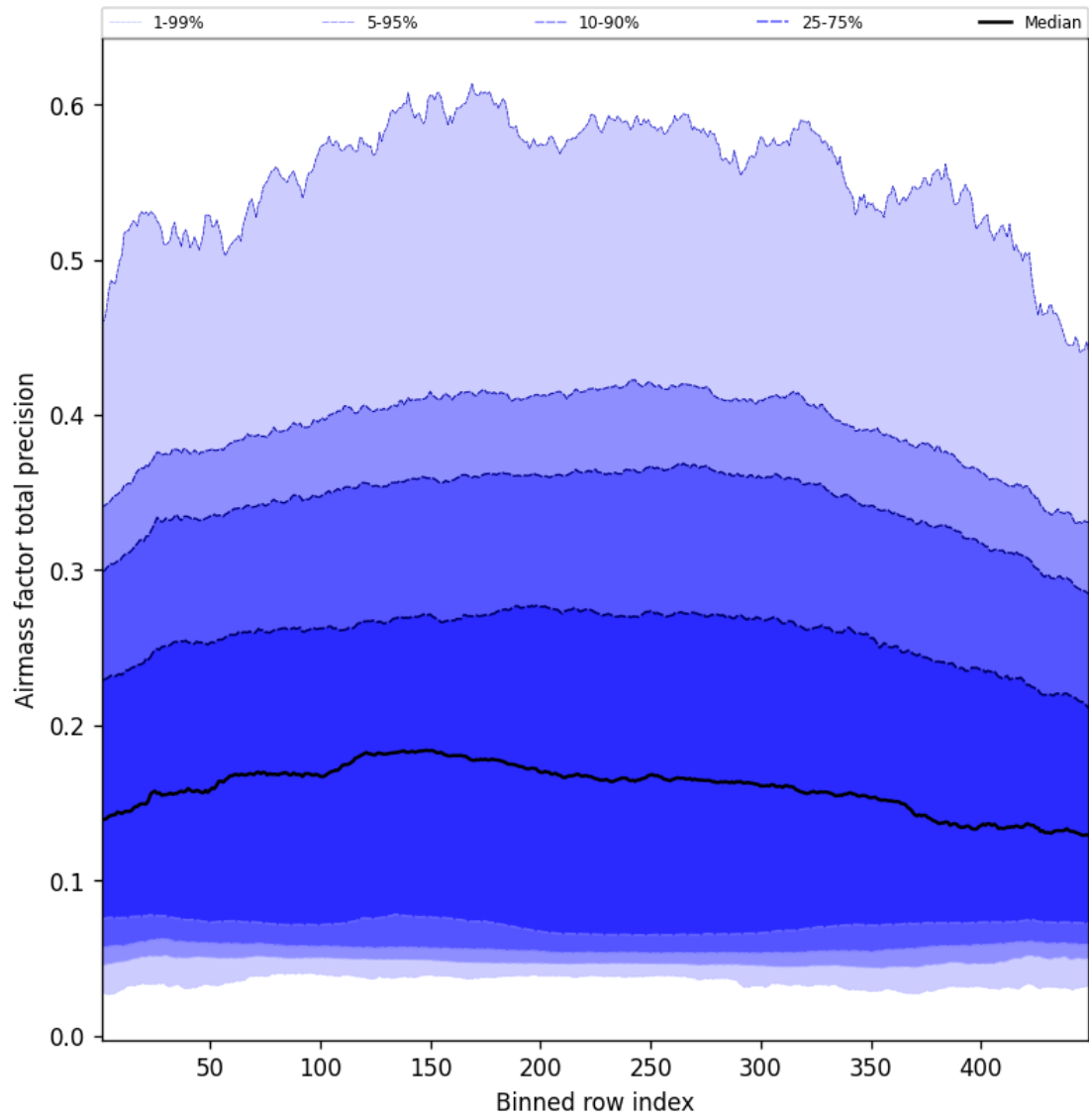
Figure 53: Along track statistics of “Airmass factor total precision” for 2025-09-24 to 2025-09-25
