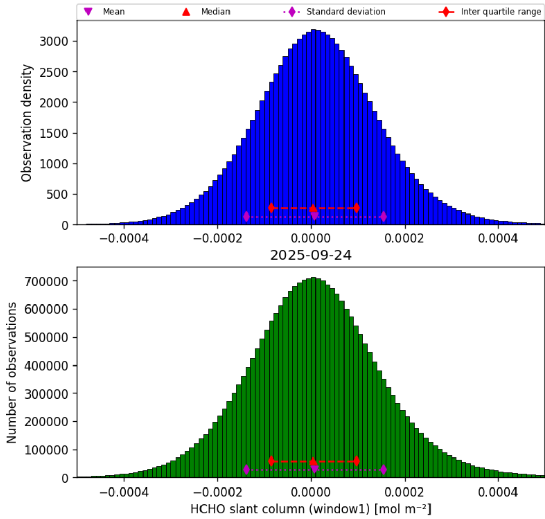
Figure 36: Histogram of “HCHO slant column (window1)” for 2025-09-24 to 2025-09-25
