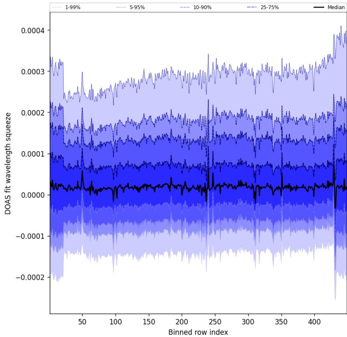
Figure 57: Along track statistics of “DOAS fit wavelength squeeze” for 2025-09-24 to 2025-09-25
