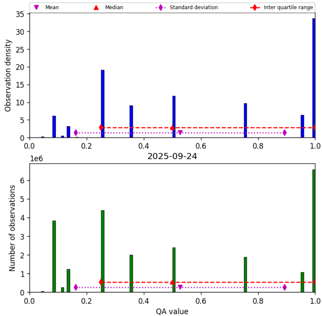
Figure 32: Histogram of “QA value” for 2025-09-24 to 2025-09-25
