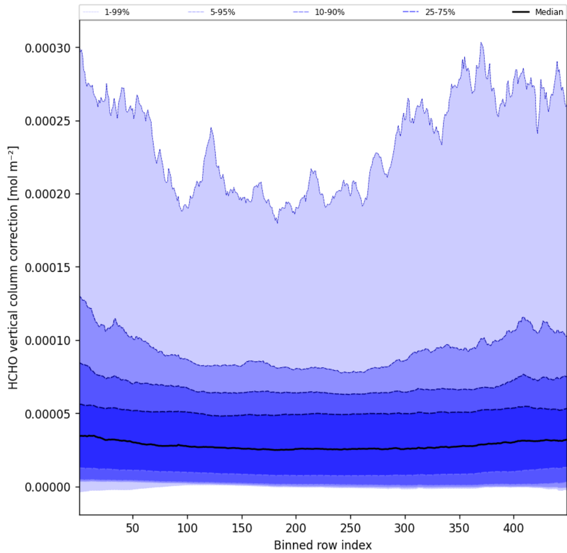
Figure 49: Along track statistics of “HCHO vertical column correction” for 2025-09-24 to 2025-09-25
