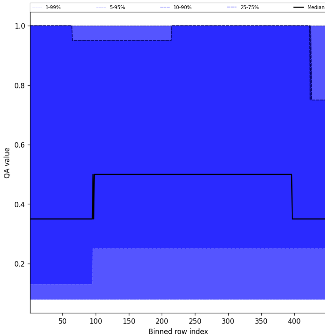
Figure 46: Along track statistics of “QA value” for 2025-09-24 to 2025-09-25
