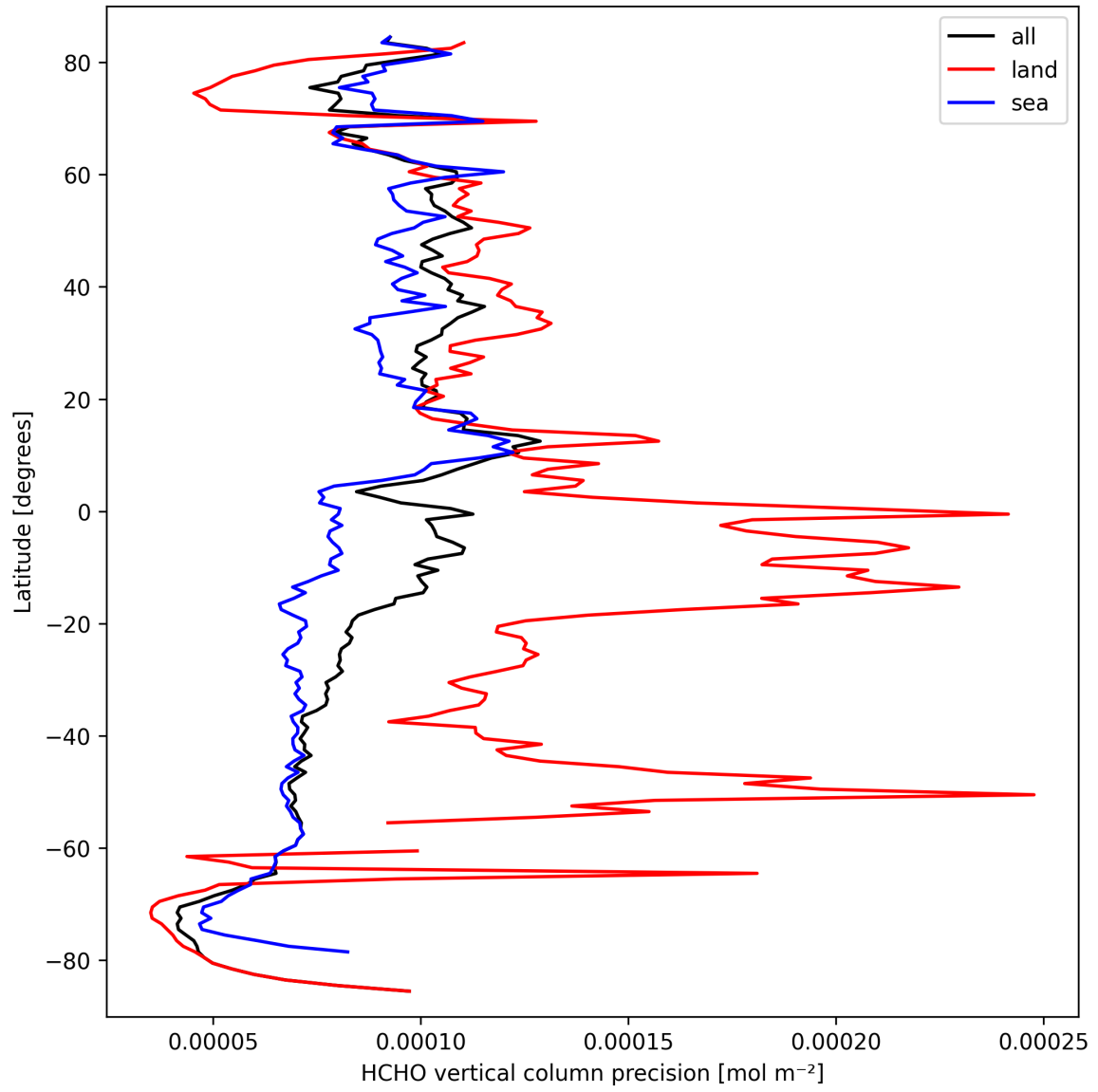
Figure 20: Zonal average of “HCHO vertical column precision” for 2025-09-24 to 2025-09-25.
