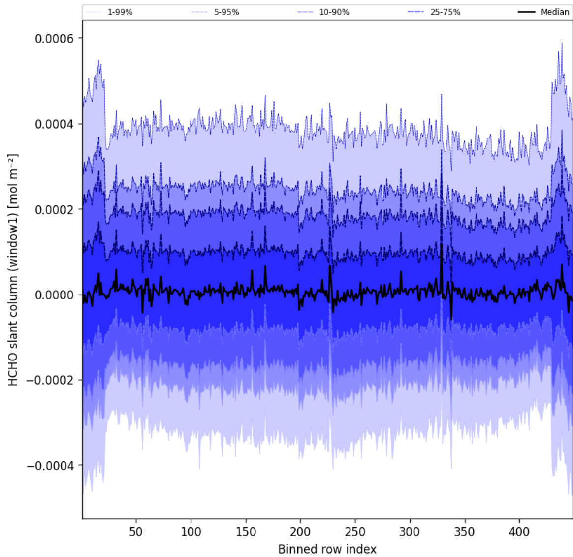
Figure 50: Along track statistics of “HCHO slant column (window1)” for 2025-09-24 to 2025-09-25
