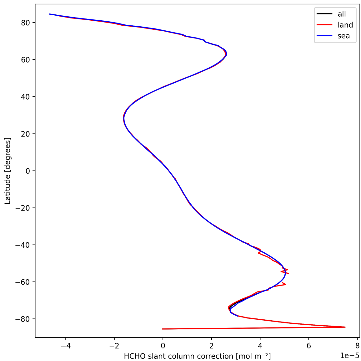
Figure 31: Zonal average of “HCHO slant column correction” for 2025-09-24 to 2025-09-25.
