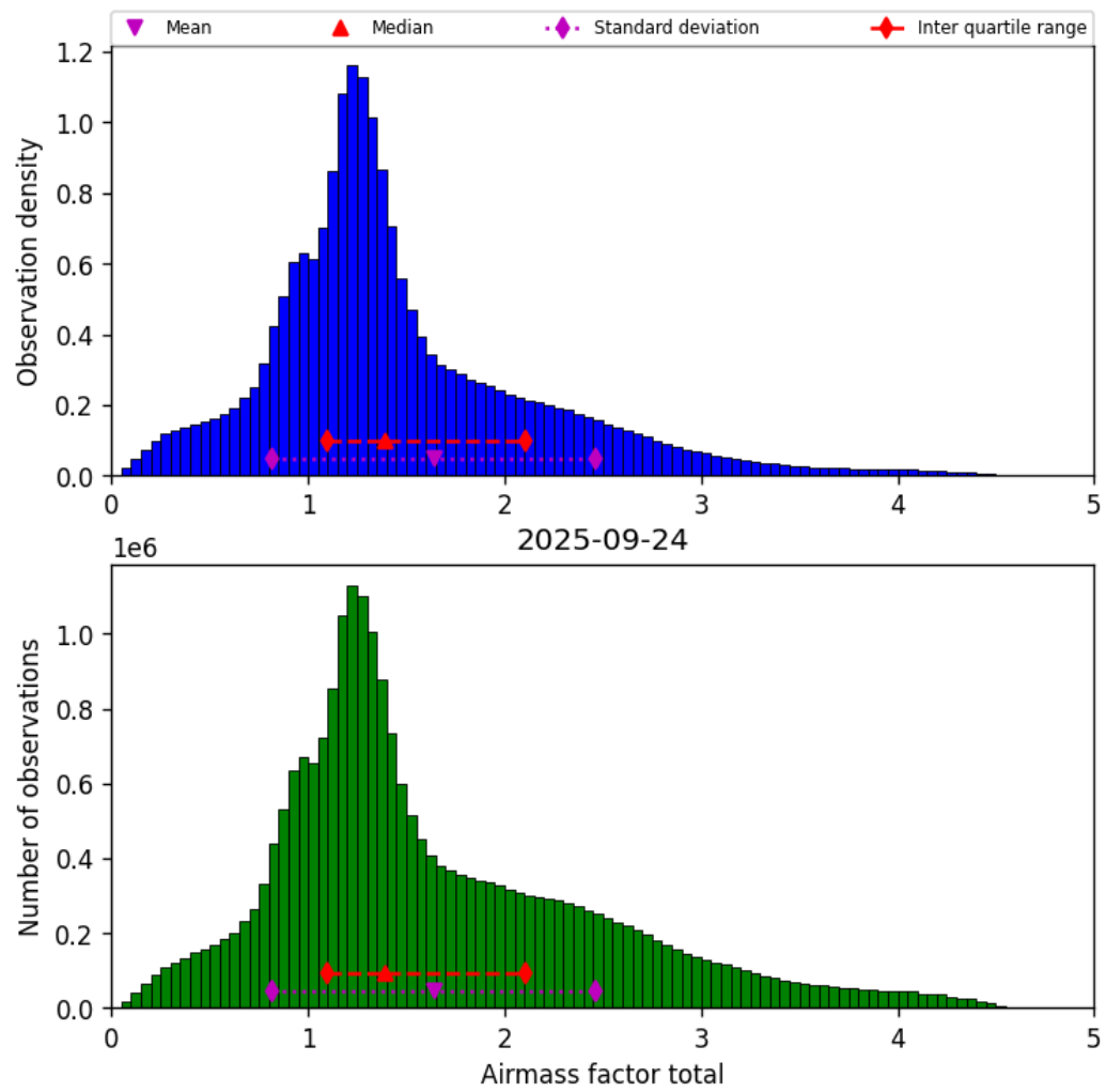
Figure 38: Histogram of “Airmass factor total” for 2025-09-24 to 2025-09-25
