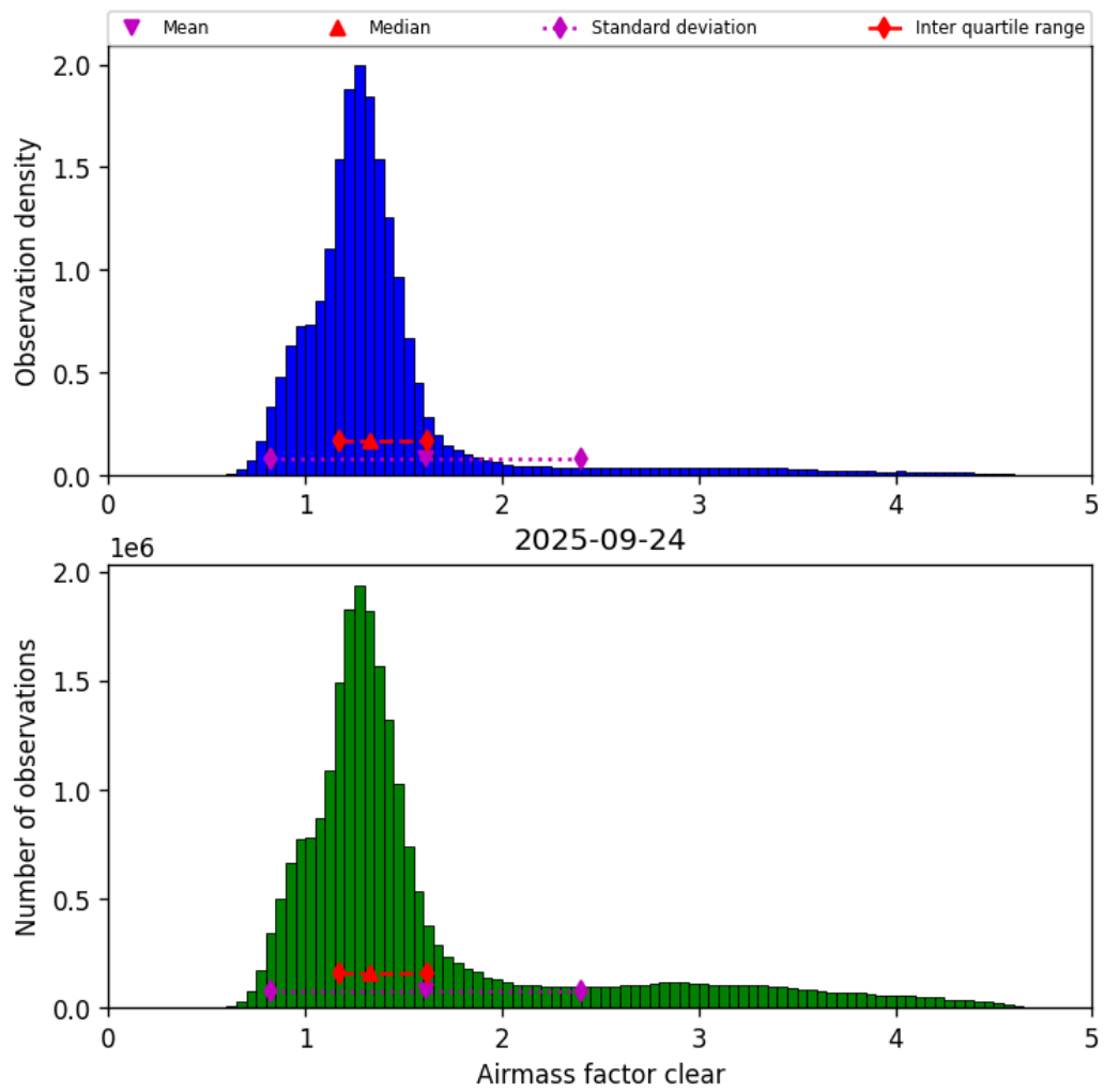
Figure 40: Histogram of “Airmass factor clear” for 2025-09-24 to 2025-09-25
