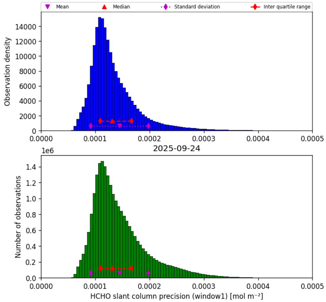
Figure 37: Histogram of “HCHO slant column precision (window1)” for 2025-09-24 to 2025-09-25
