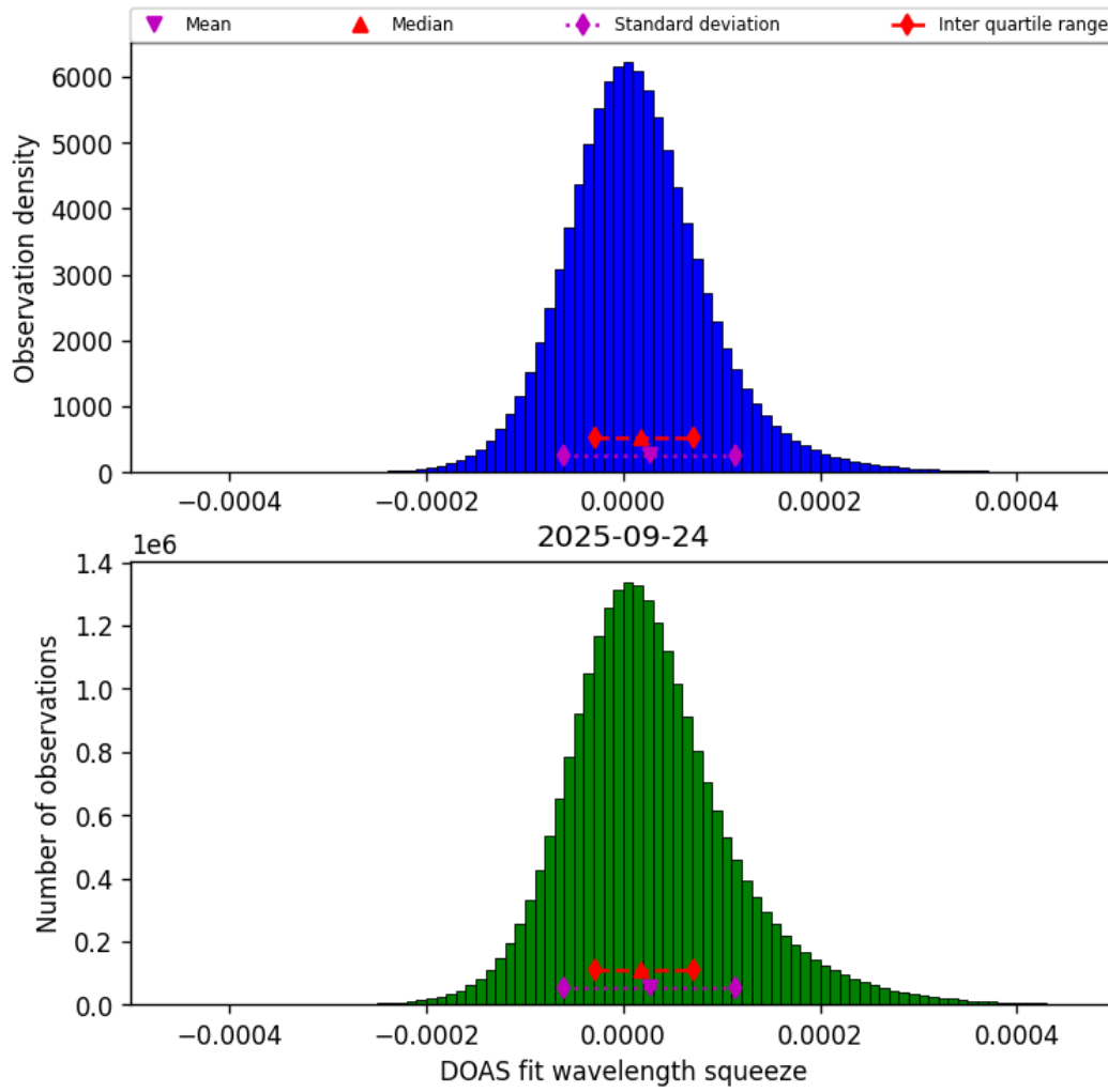
Figure 43: Histogram of “DOAS fit wavelength squeeze” for 2025-09-24 to 2025-09-25
