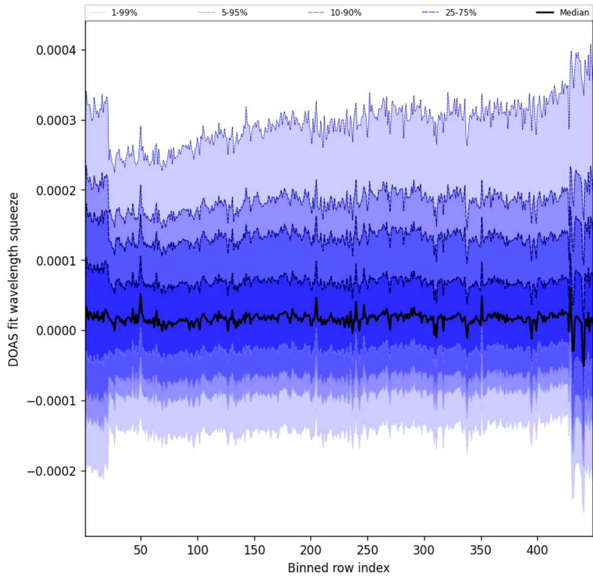
Figure 57: Along track statistics of “DOAS fit wavelength squeeze” for 2025-09-25 to 2025-09-26
