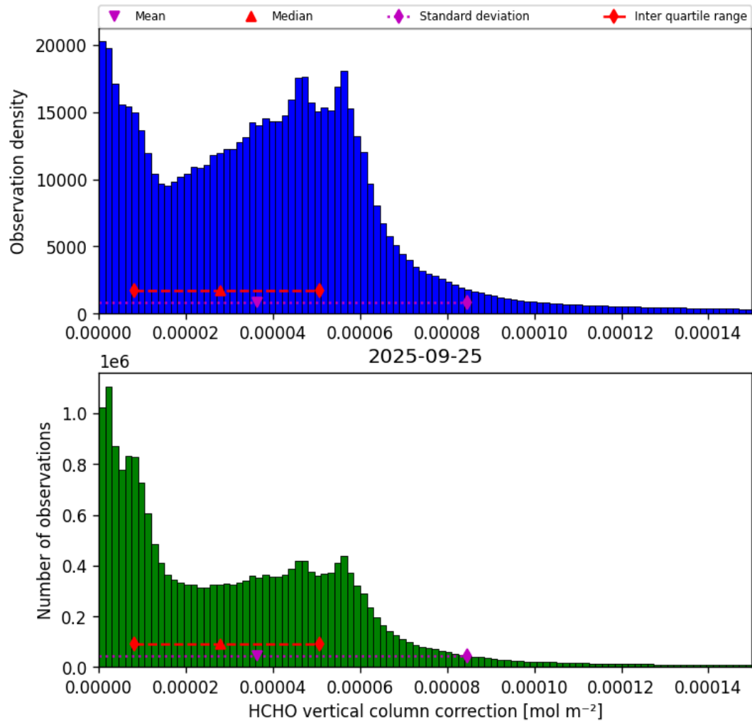
Figure 35: Histogram of “HCHO vertical column correction” for 2025-09-25 to 2025-09-26
