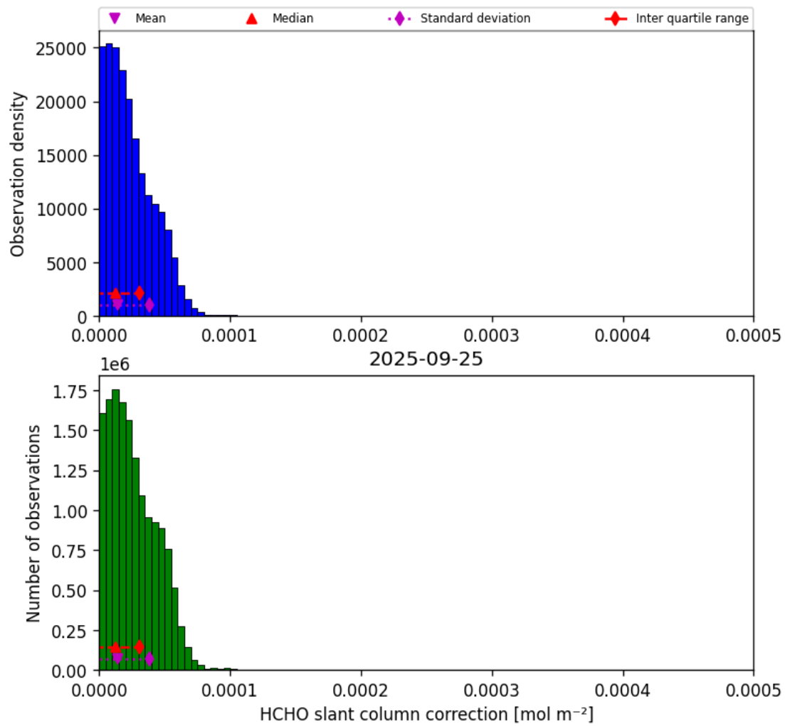
Figure 45: Histogram of “HCHO slant column correction” for 2025-09-25 to 2025-09-26
