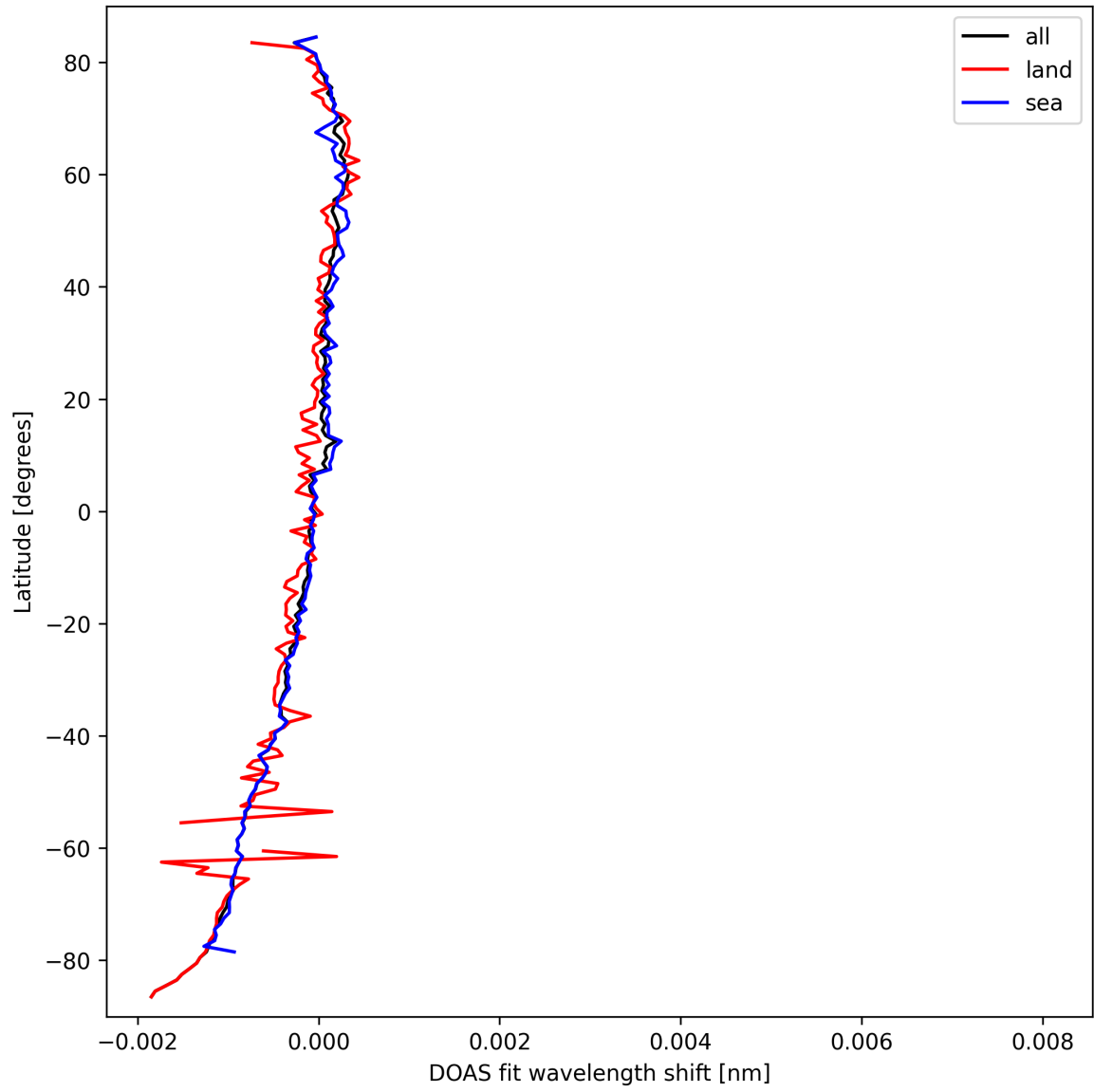
Figure 28: Zonal average of "DOAS fit wavelength shift" for 2025-09-25 to 2025-09-26.
