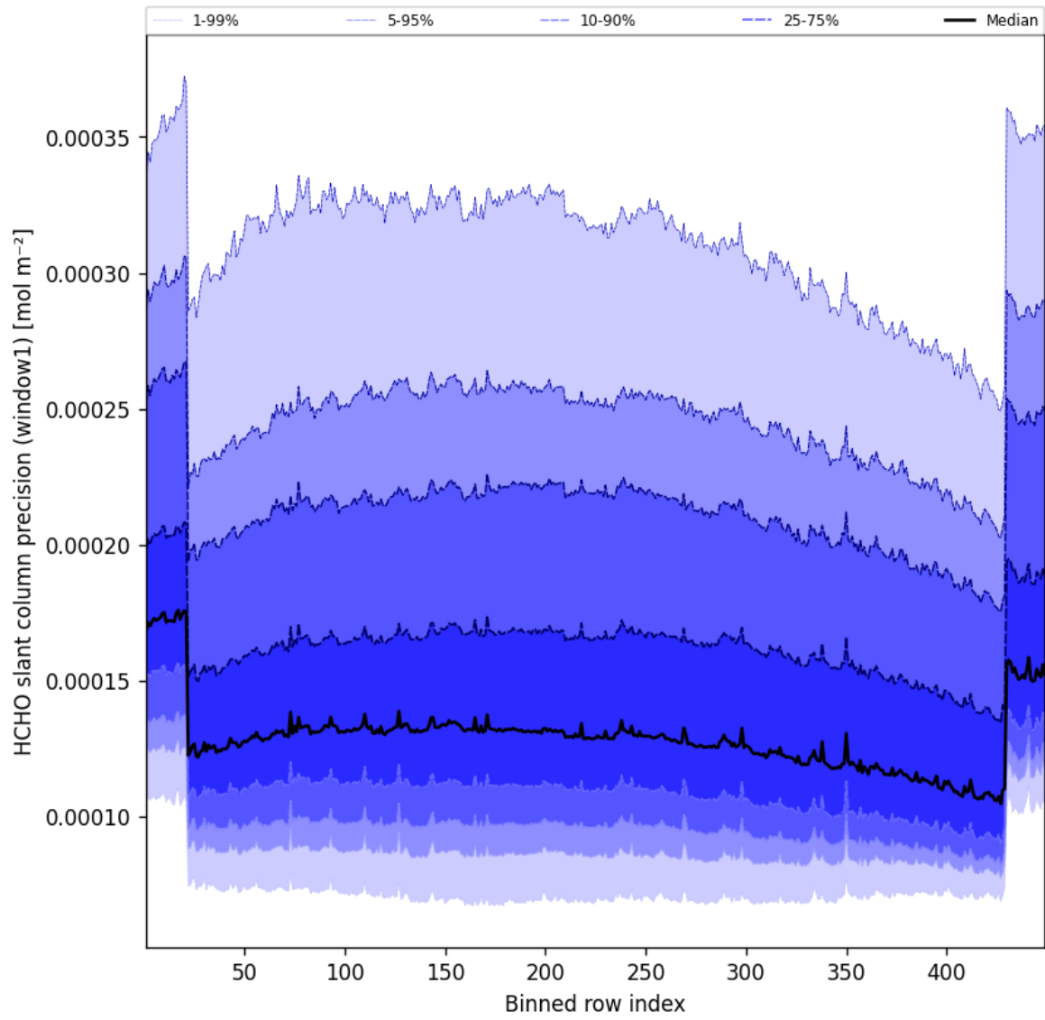
Figure 51: Along track statistics of “HCHO slant column precision (window1)” for 2025-09-25 to 2025-09-26
