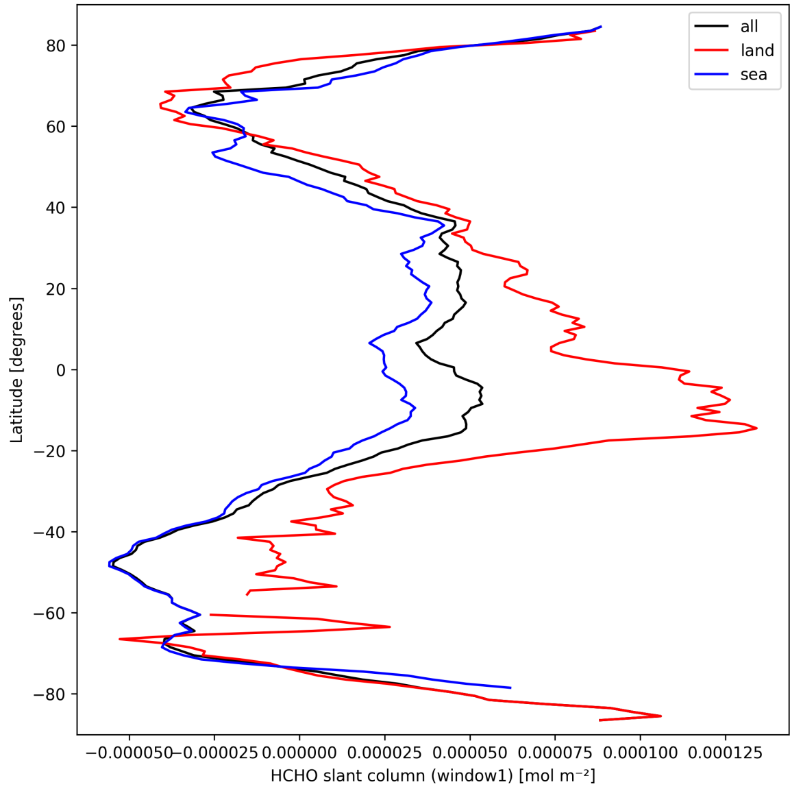
Figure 22: Zonal average of “HCHO slant column (window1)” for 2025-09-25 to 2025-09-26.
