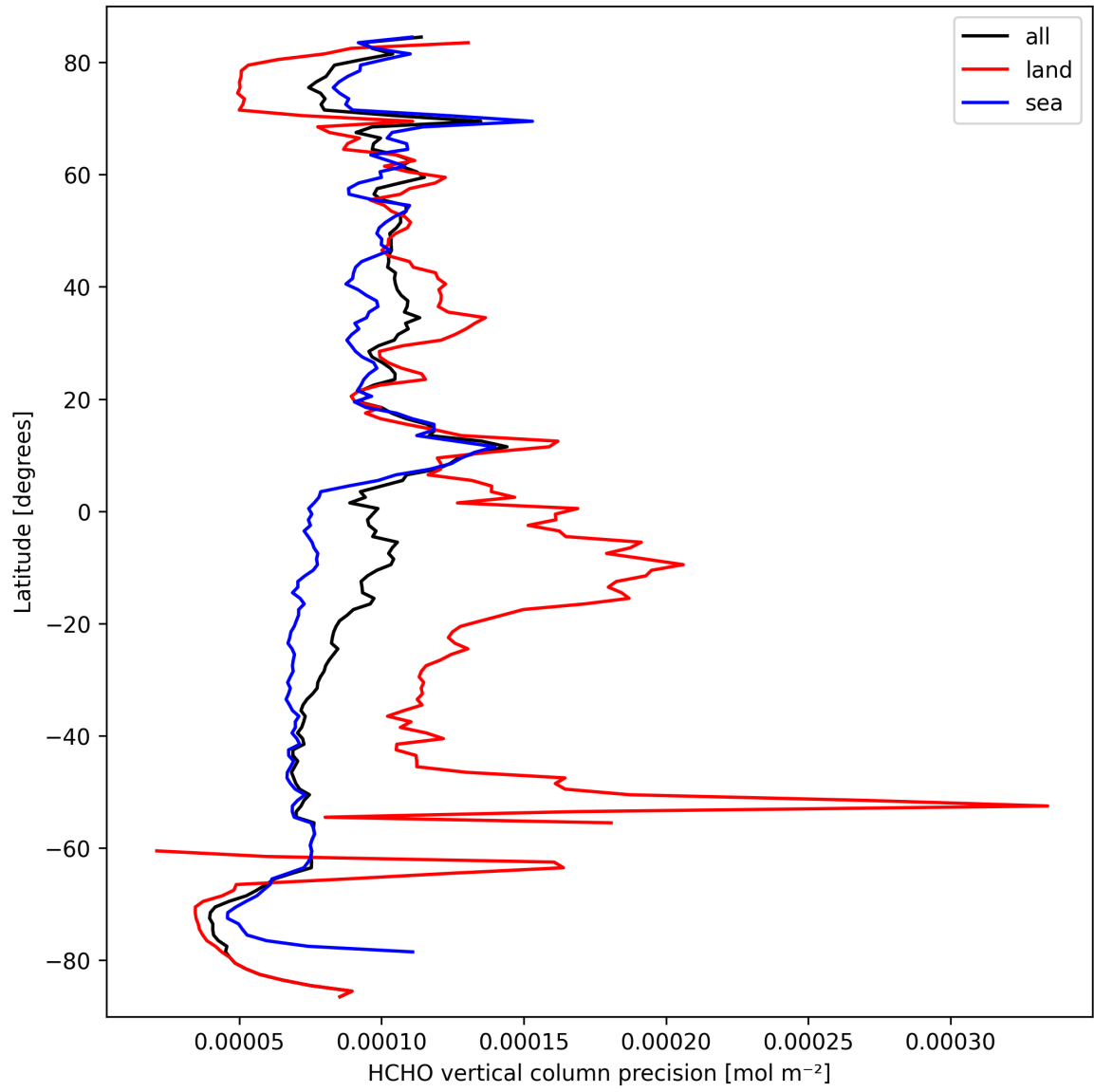
Figure 20: Zonal average of “HCHO vertical column precision” for 2025-09-25 to 2025-09-26.
