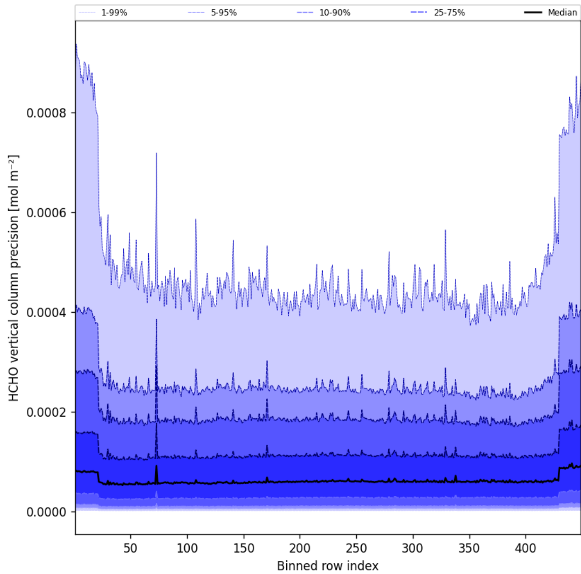
Figure 48: Along track statistics of “HCHO vertical column precision” for 2025-09-25 to 2025-09-26
