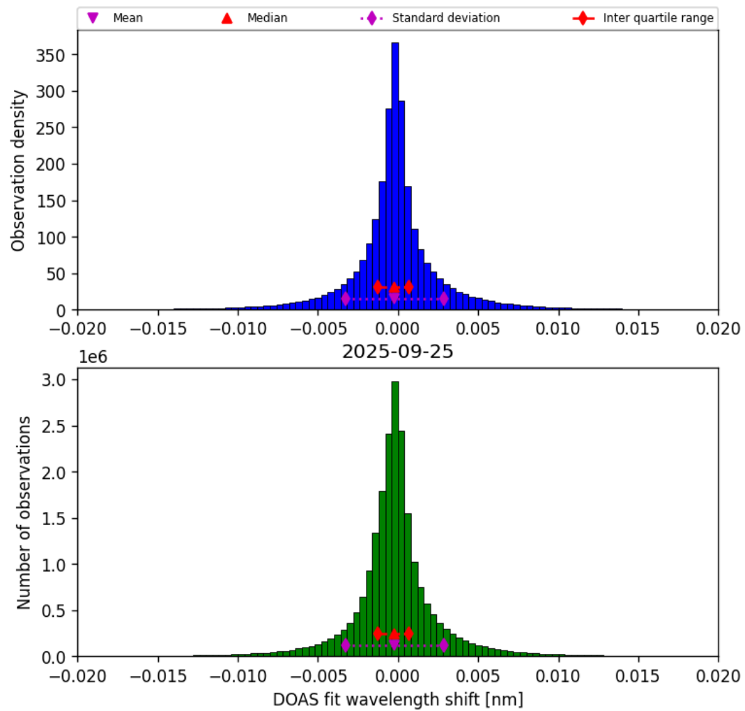
Figure 42: Histogram of “DOAS fit wavelength shift” for 2025-09-25 to 2025-09-26
