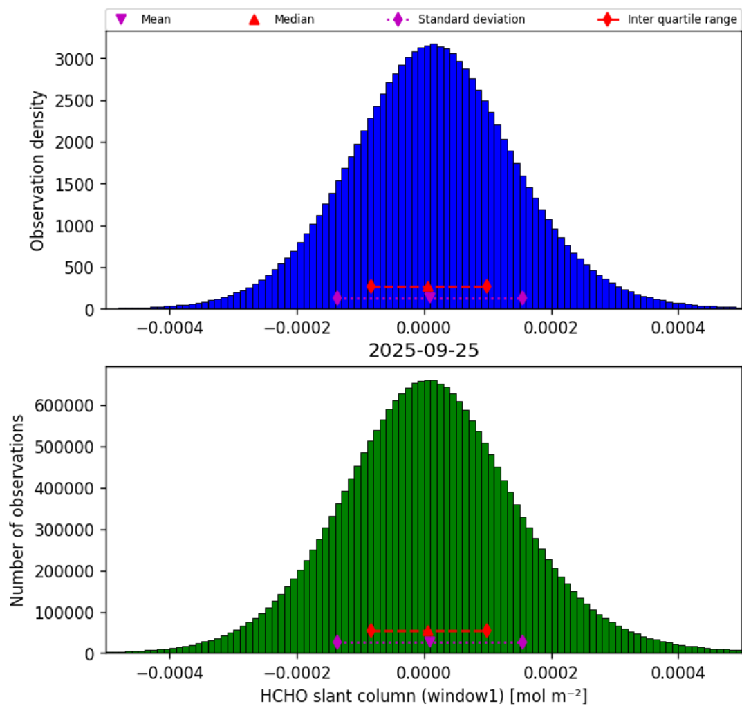
Figure 36: Histogram of “HCHO slant column (window1)” for 2025-09-25 to 2025-09-26
