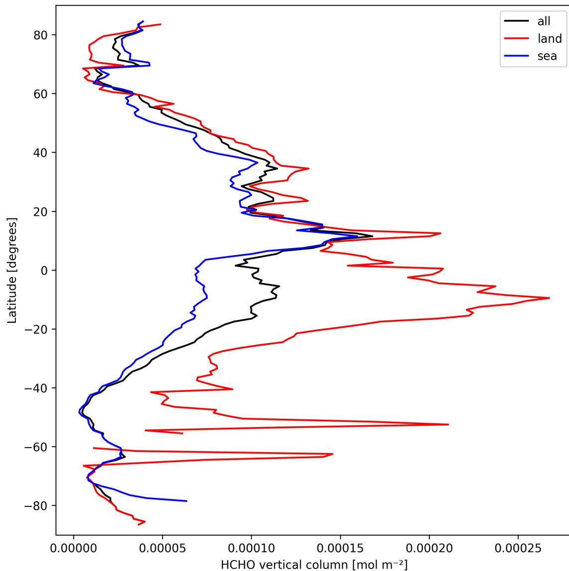
Figure 19: Zonal average of “HCHO vertical column” for 2025-09-25 to 2025-09-26.
