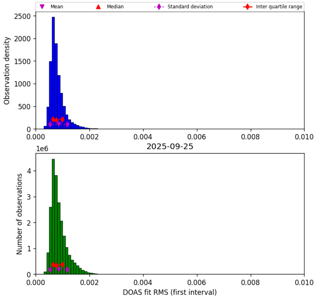
Figure 44: Histogram of “DOAS fit RMS (first interval)” for 2025-09-25 to 2025-09-26
