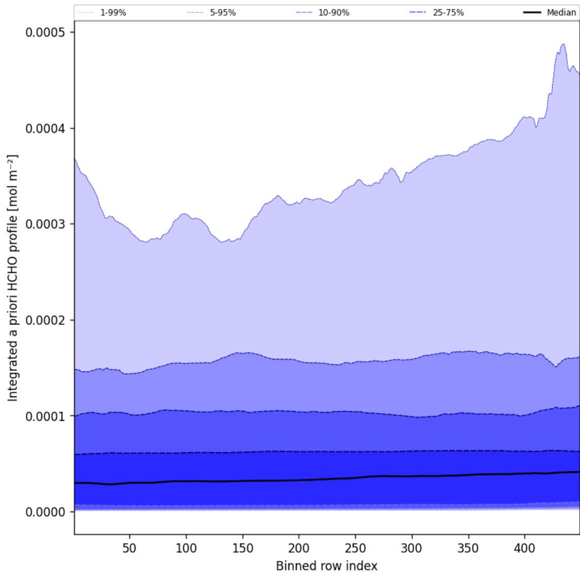
Figure 55: Along track statistics of “Integrated a priori HCHO profile” for 2025-09-25 to 2025-09-26
