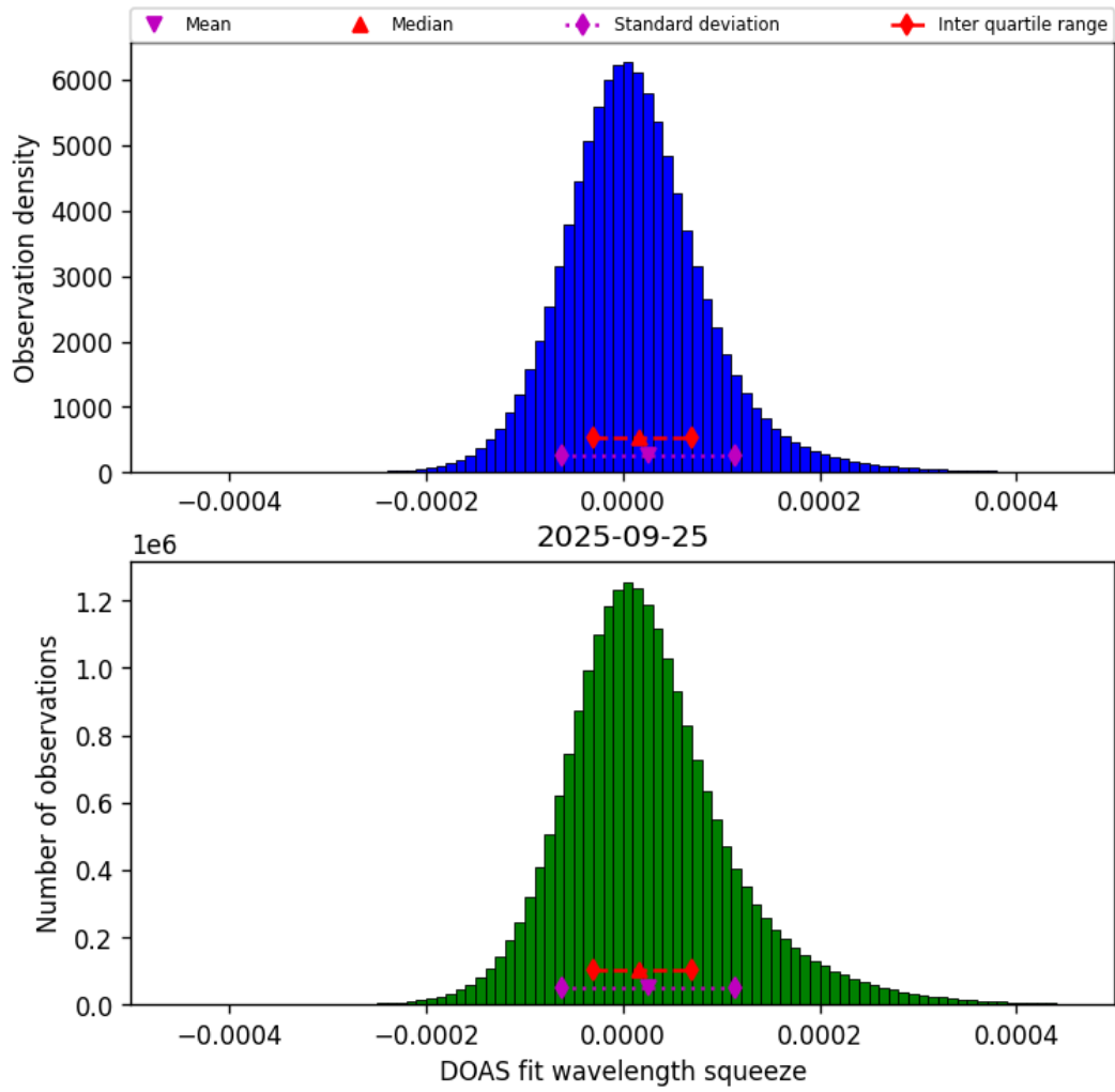
Figure 43: Histogram of “DOAS fit wavelength squeeze” for 2025-09-25 to 2025-09-26
