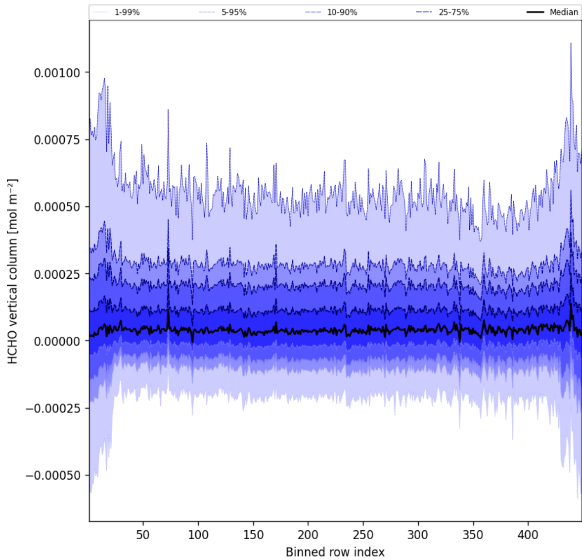
Figure 47: Along track statistics of “HCHO vertical column” for 2025-09-25 to 2025-09-26
