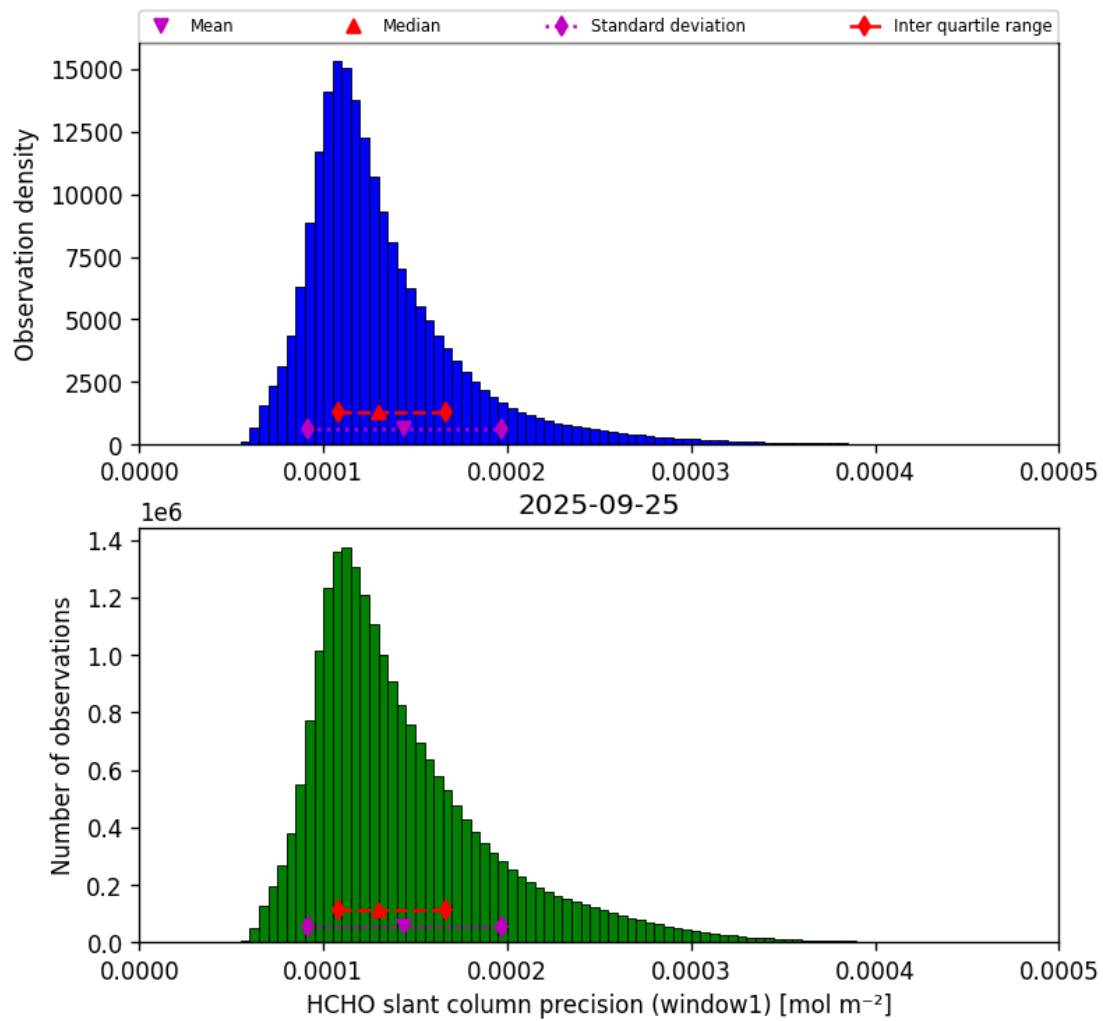
Figure 37: Histogram of “HCHO slant column precision (window1)” for 2025-09-25 to 2025-09-26
