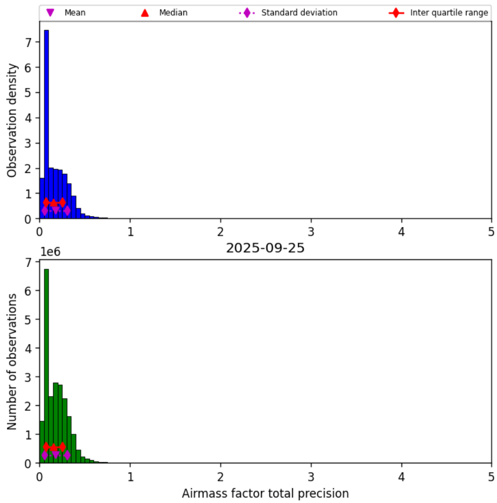
Figure 39: Histogram of “Airmass factor total precision” for 2025-09-25 to 2025-09-26
