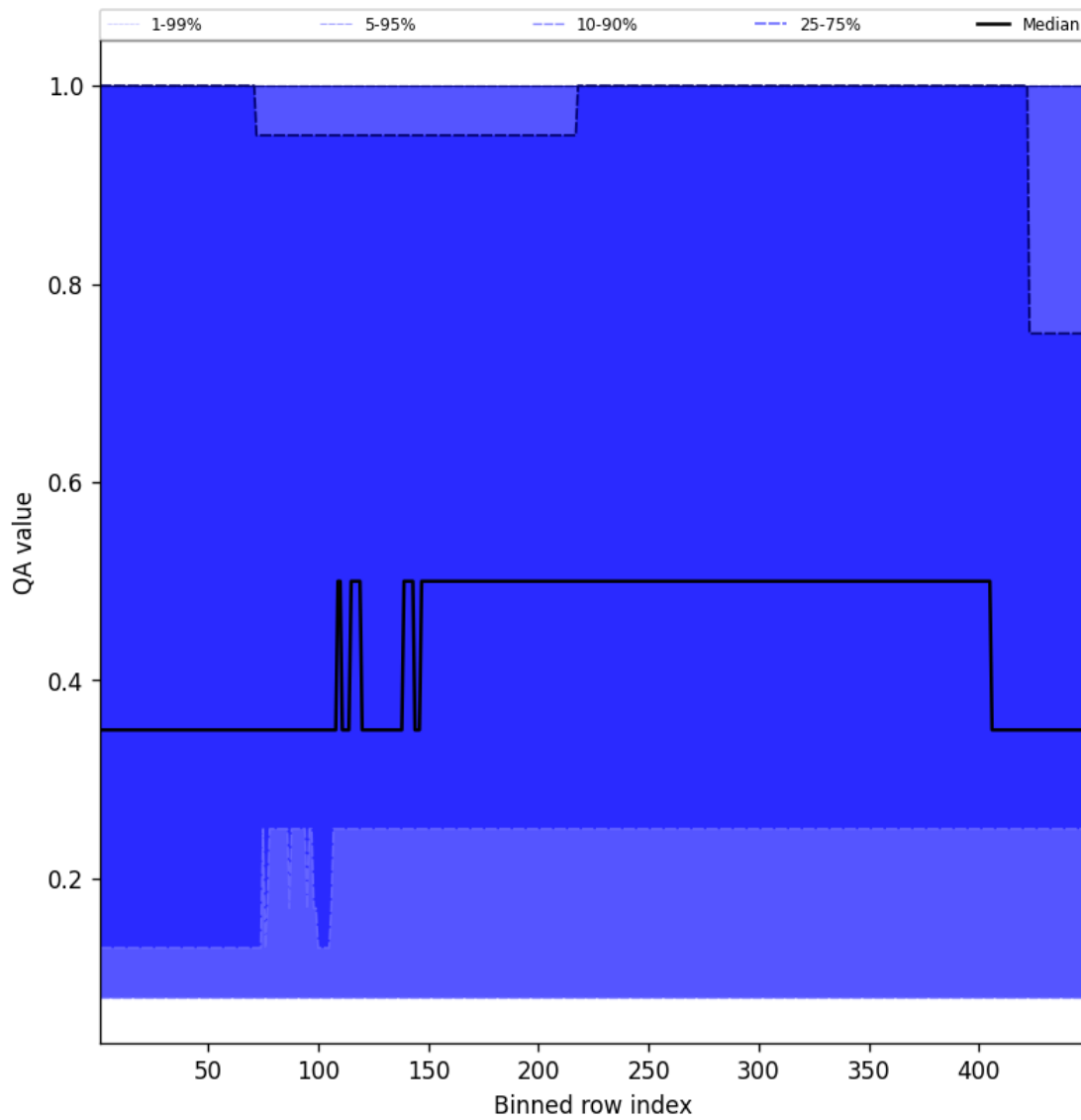
Figure 46: Along track statistics of “QA value” for 2025-09-25 to 2025-09-26
