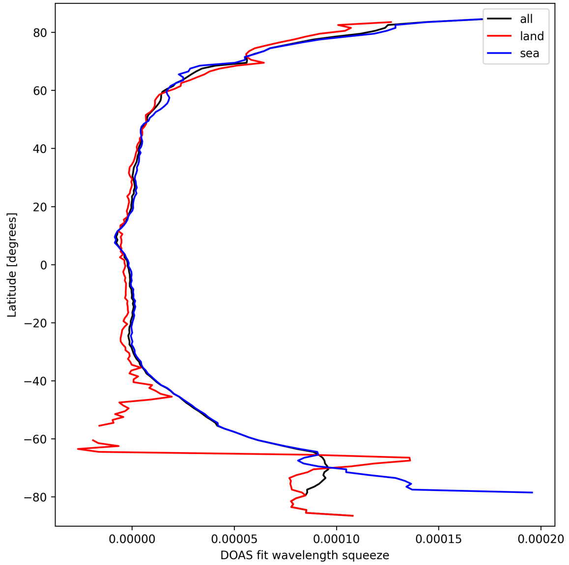
Figure 29: Zonal average of “DOAS fit wavelength squeeze” for 2025-09-25 to 2025-09-26.
