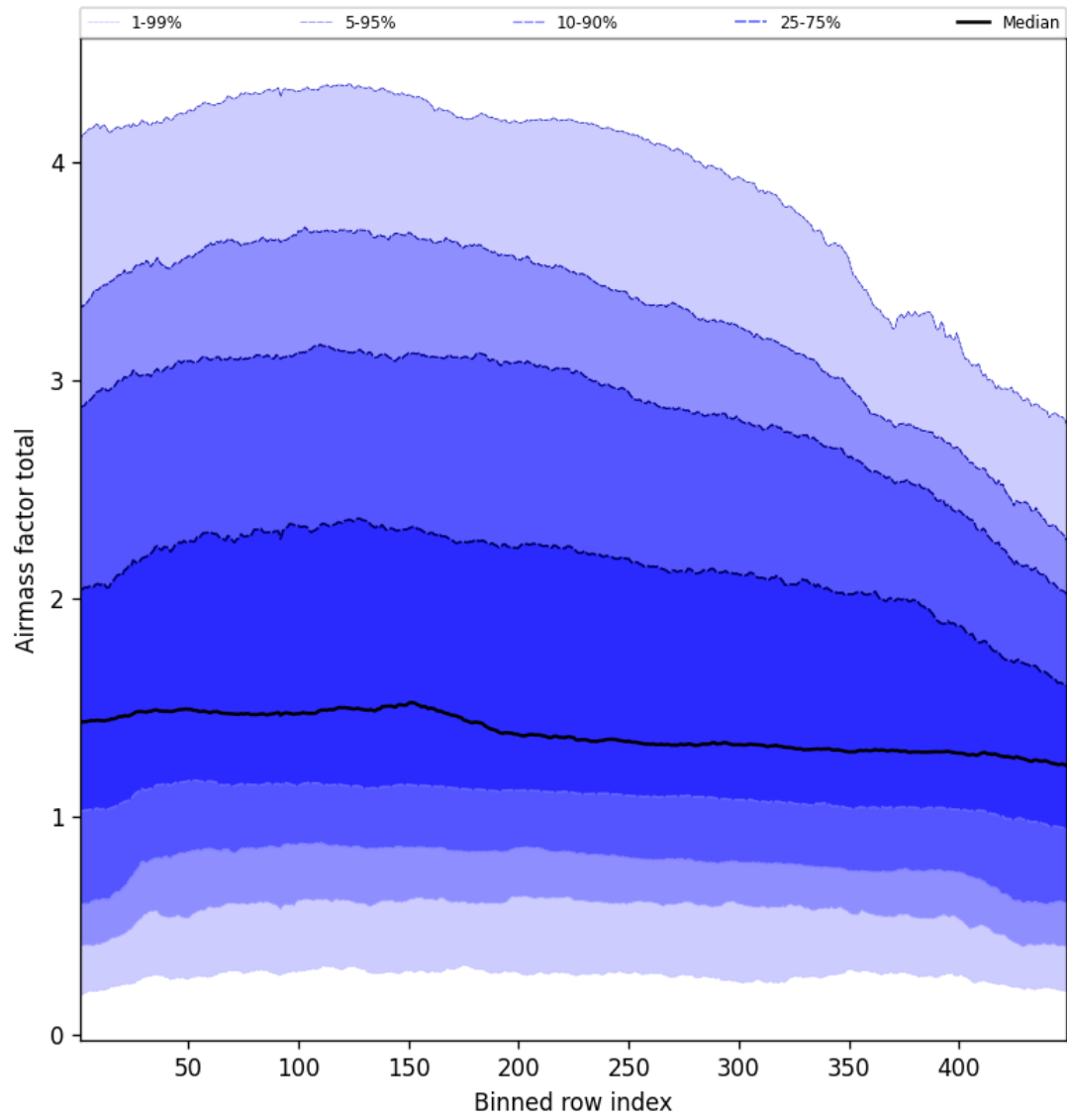
Figure 52: Along track statistics of “Airmass factor total” for 2025-09-25 to 2025-09-26
