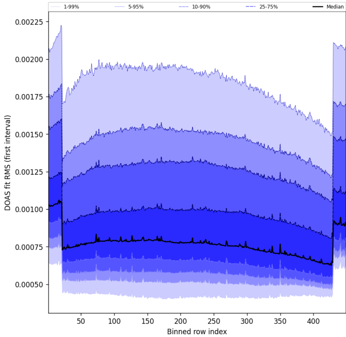
Figure 58: Along track statistics of “DOAS fit RMS (first interval)” for 2025-09-25 to 2025-09-26
