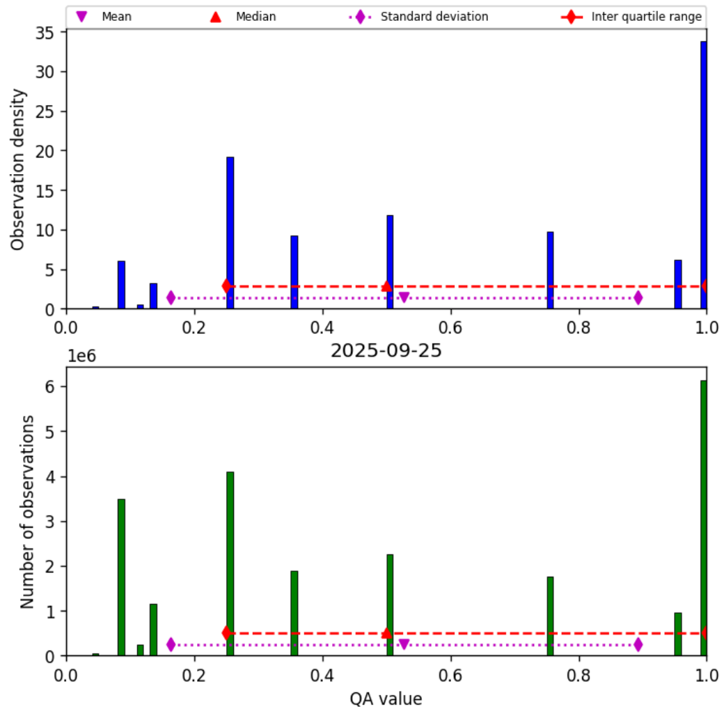
Figure 32: Histogram of “QA value” for 2025-09-25 to 2025-09-26
