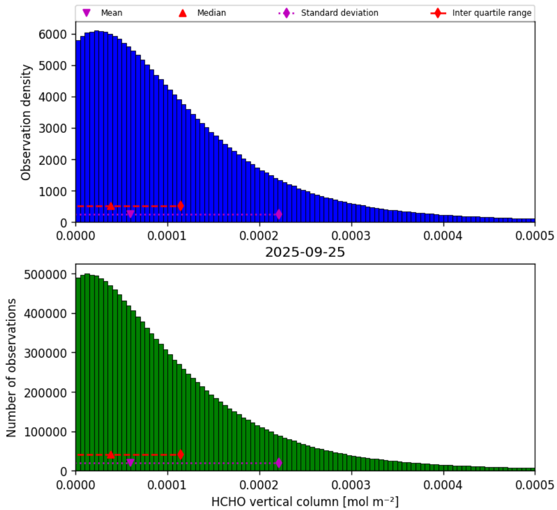
Figure 33: Histogram of “HCHO vertical column” for 2025-09-25 to 2025-09-26
