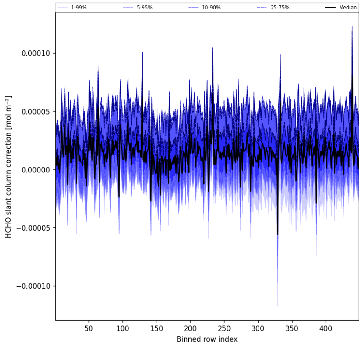
Figure 59: Along track statistics of “HCHO slant column correction” for 2025-09-25 to 2025-09-26
