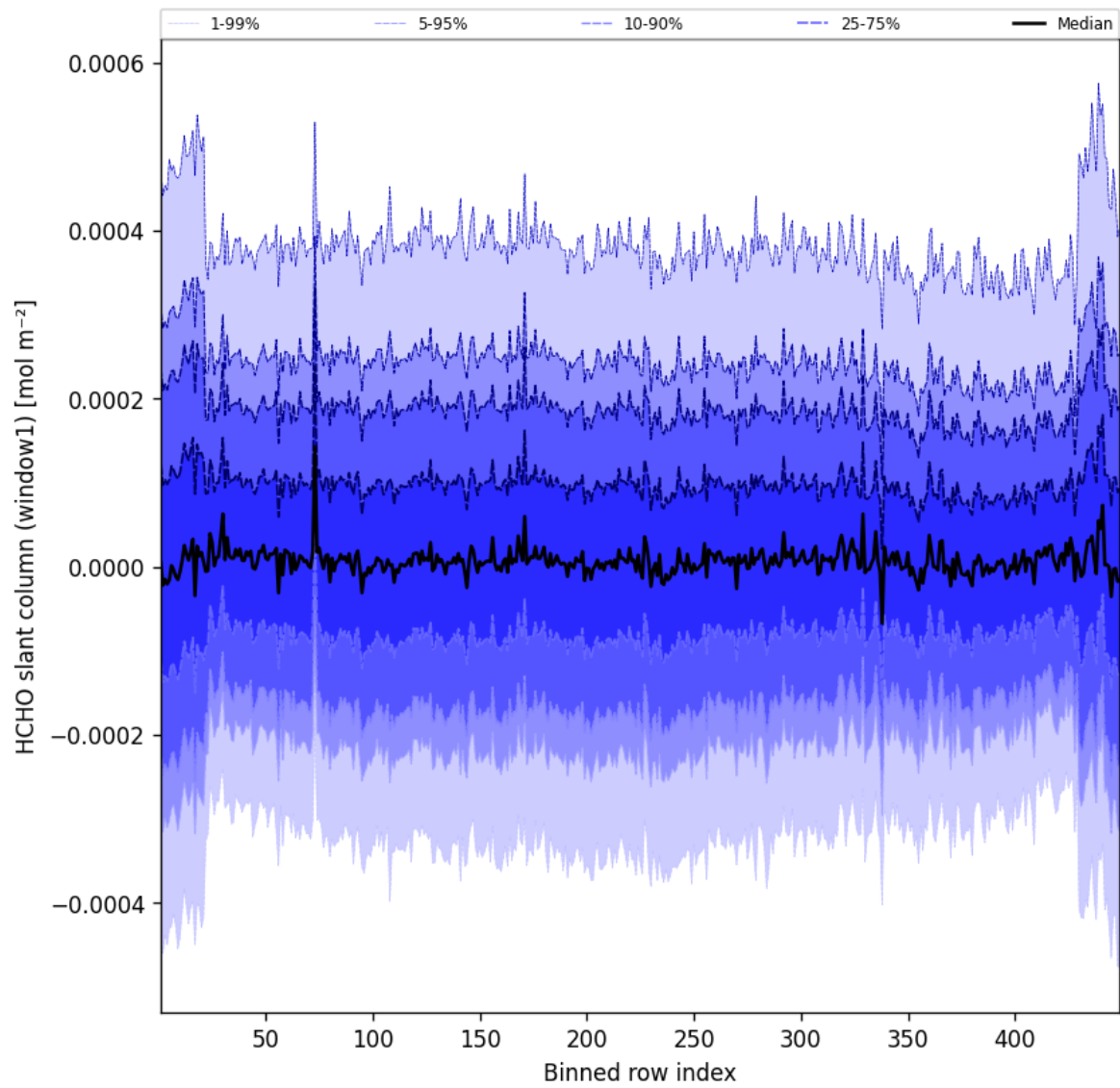
Figure 50: Along track statistics of “HCHO slant column (window1)” for 2025-09-25 to 2025-09-26
