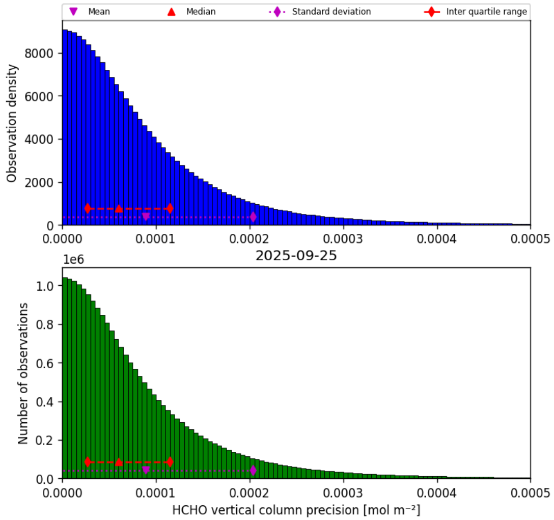
Figure 34: Histogram of “HCHO vertical column precision” for 2025-09-25 to 2025-09-26
