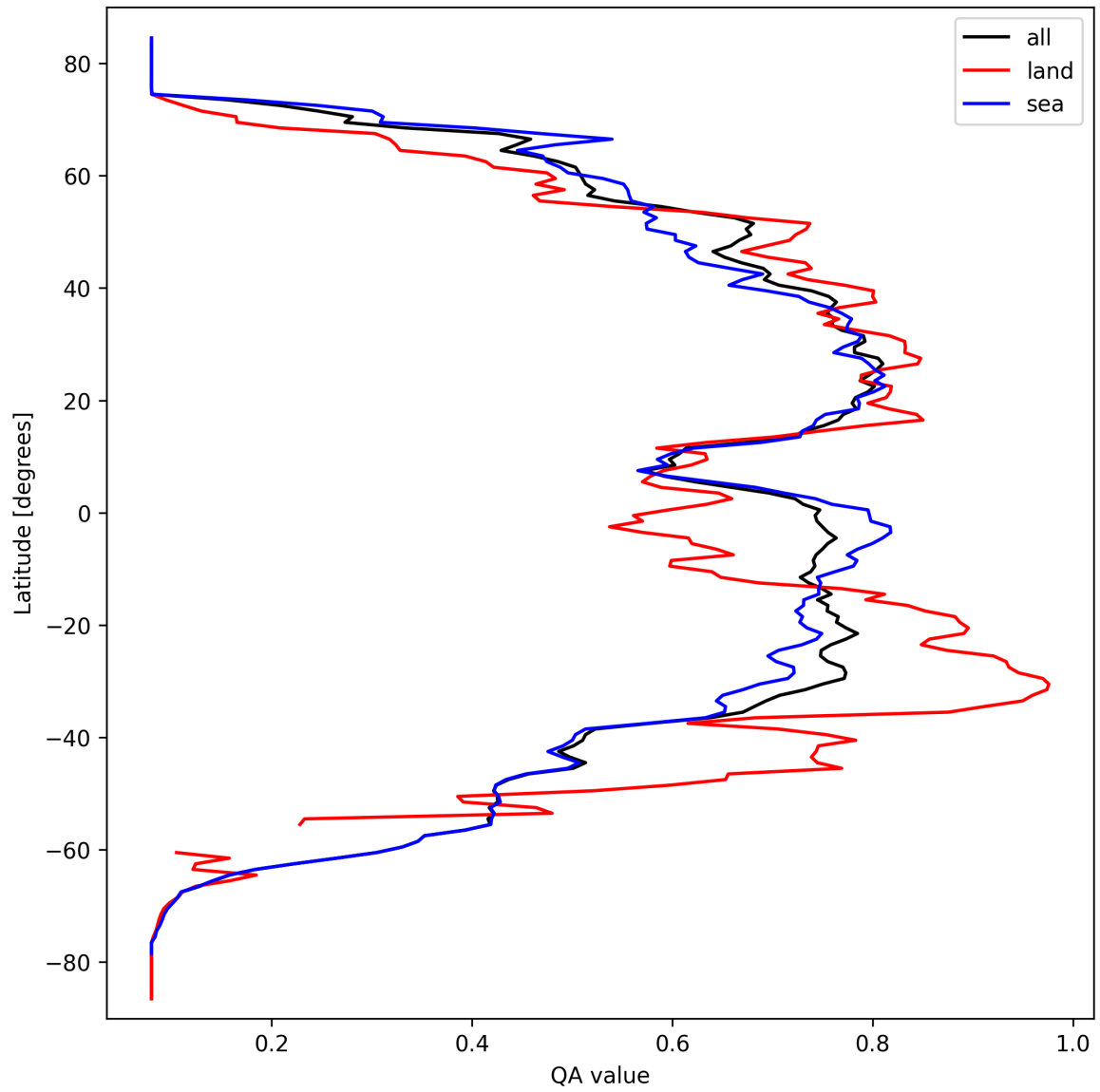
Figure 18: Zonal average of “QA value” for 2025-09-25 to 2025-09-26.
