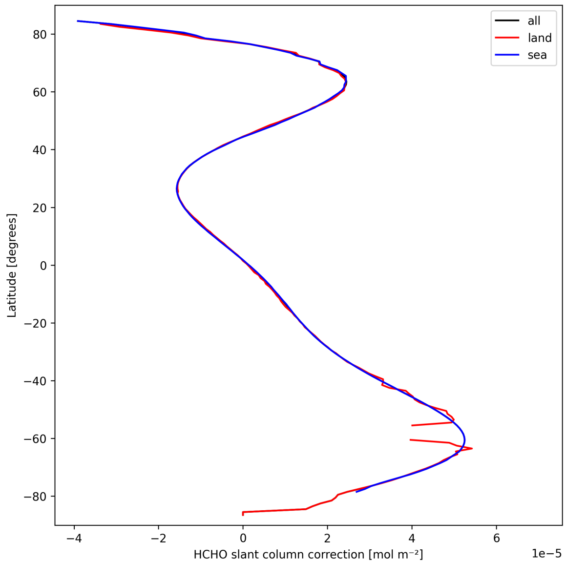
Figure 31: Zonal average of “HCHO slant column correction” for 2025-09-25 to 2025-09-26.
