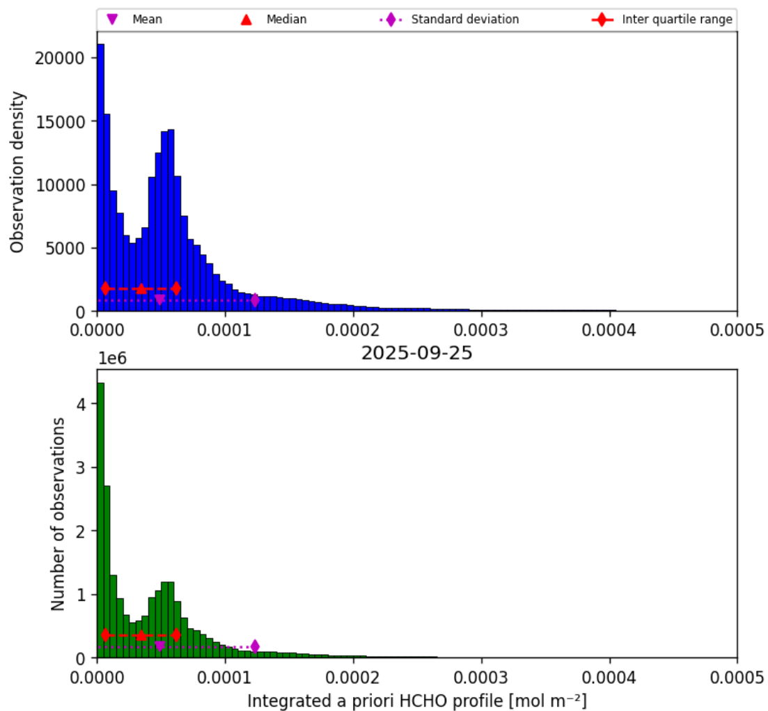
Figure 41: Histogram of “Integrated a priori HCHO profile” for 2025-09-25 to 2025-09-26
