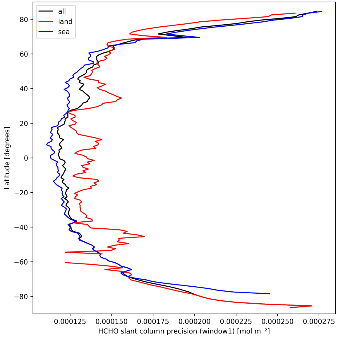
Figure 23: Zonal average of “HCHO slant column precision (window1)” for 2025-09-25 to 2025-09-26.
