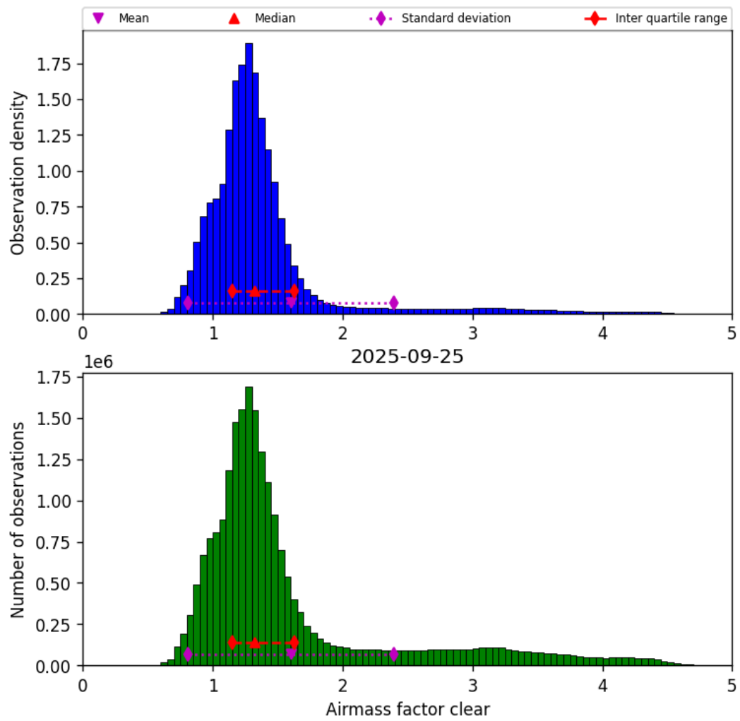
Figure 40: Histogram of “Airmass factor clear” for 2025-09-25 to 2025-09-26
