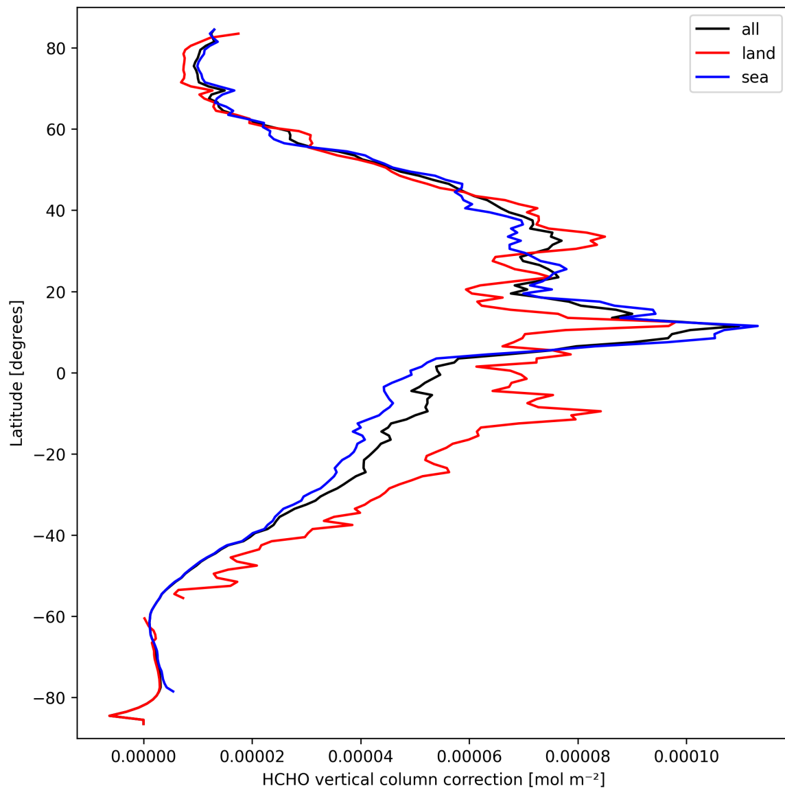
Figure 21: Zonal average of “HCHO vertical column correction” for 2025-09-25 to 2025-09-26.
