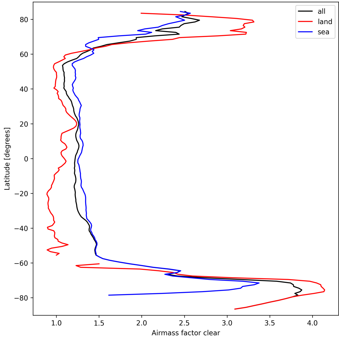
Figure 26: Zonal average of “Airmass factor clear” for 2025-09-25 to 2025-09-26.
