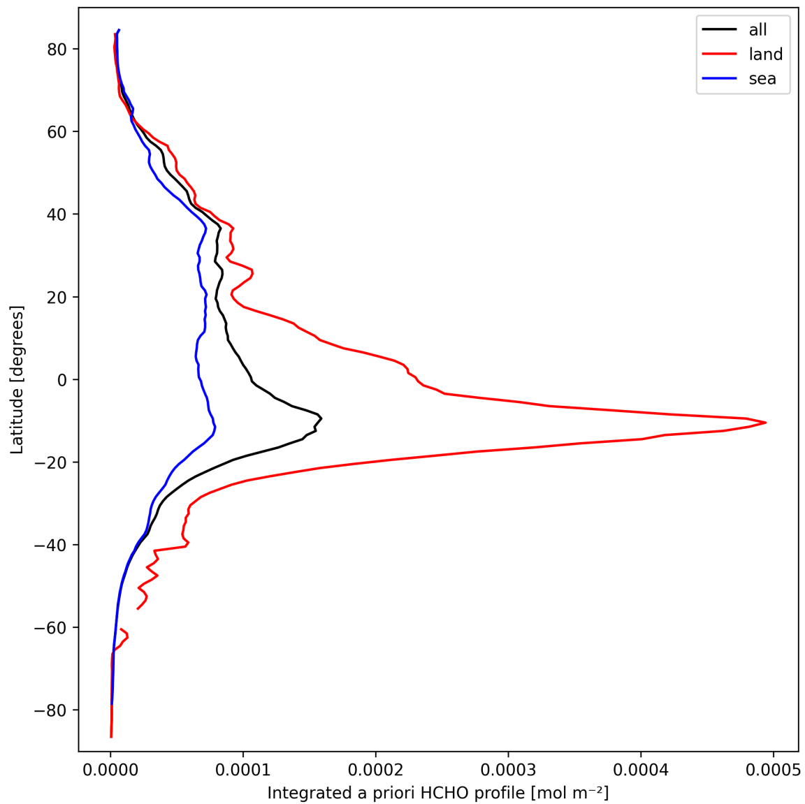
Figure 27: Zonal average of “Integrated a priori HCHO profile” for 2025-09-25 to 2025-09-26.
