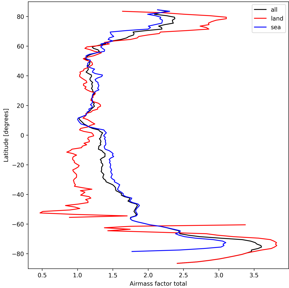
Figure 24: Zonal average of “Airmass factor total” for 2025-09-25 to 2025-09-26.
