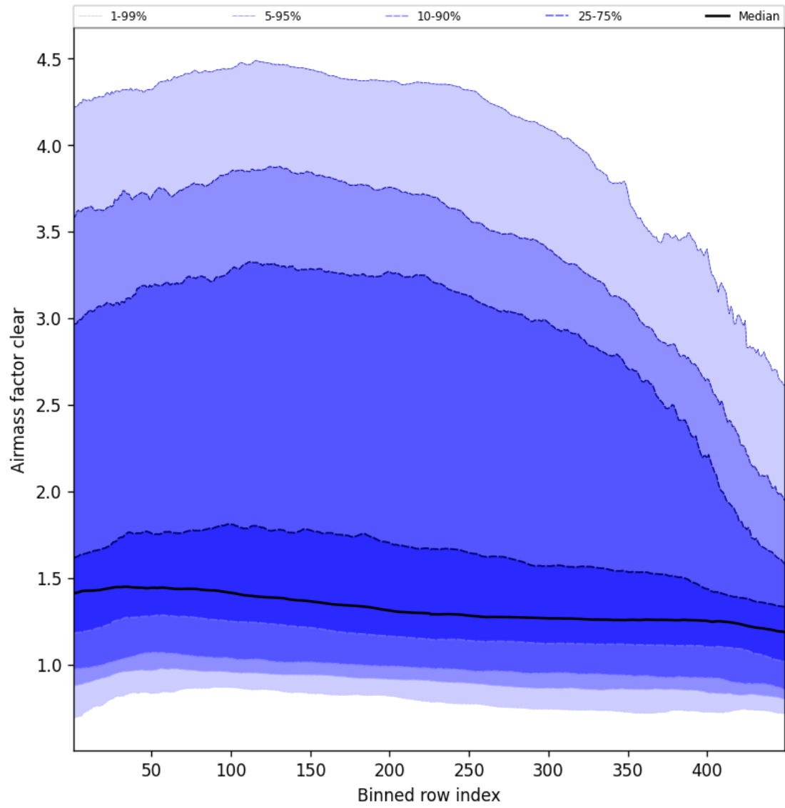
Figure 54: Along track statistics of “Airmass factor clear” for 2025-09-25 to 2025-09-26
