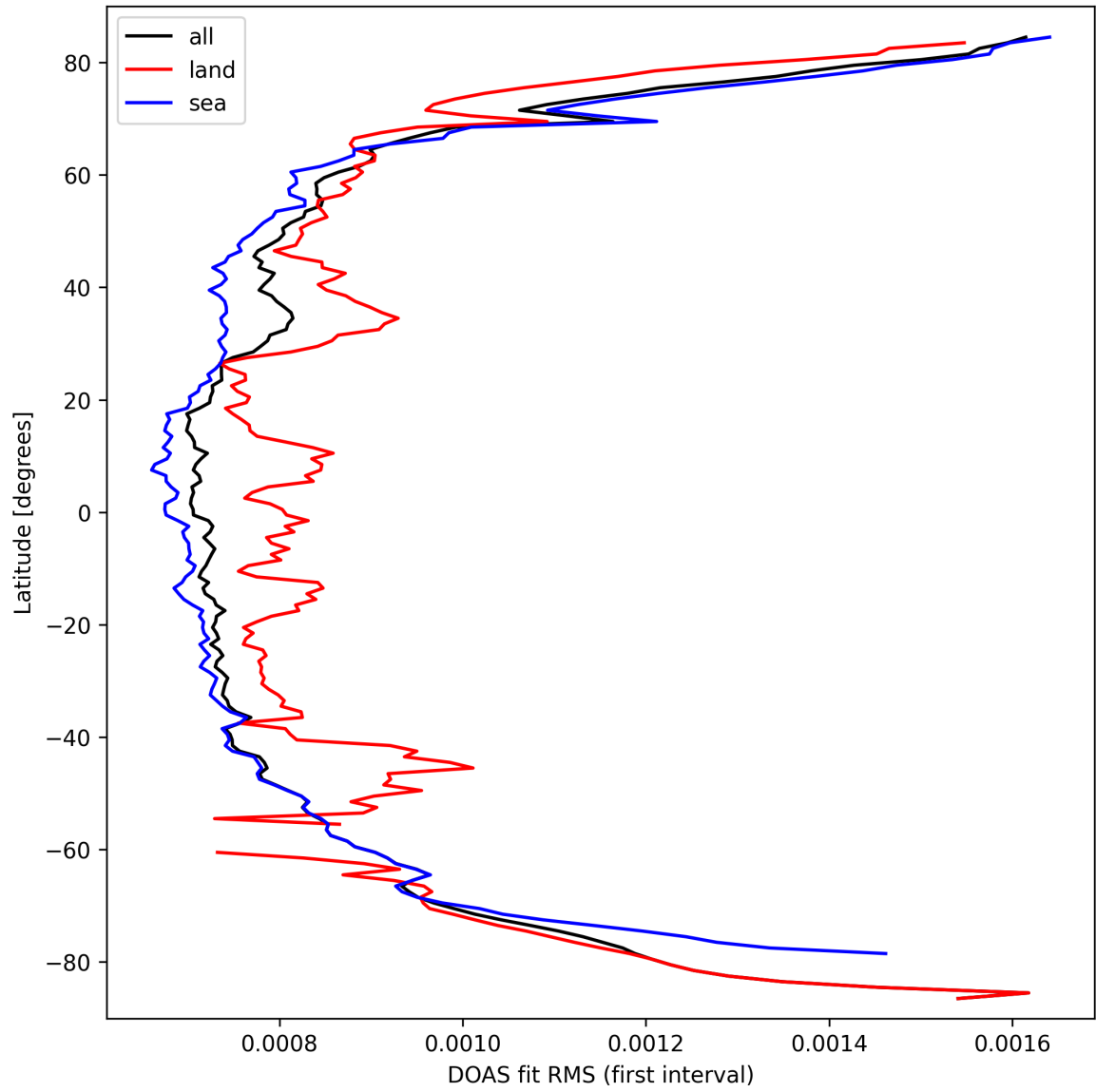
Figure 30: Zonal average of “DOAS fit RMS (first interval)” for 2025-09-25 to 2025-09-26.
