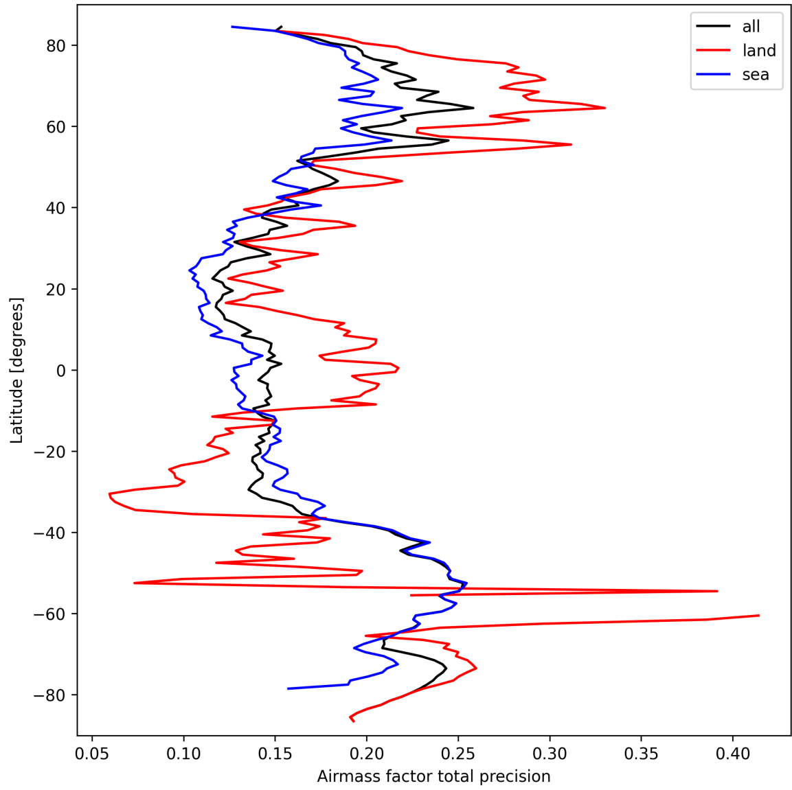
Figure 25: Zonal average of “Airmass factor total precision” for 2025-09-25 to 2025-09-26.
