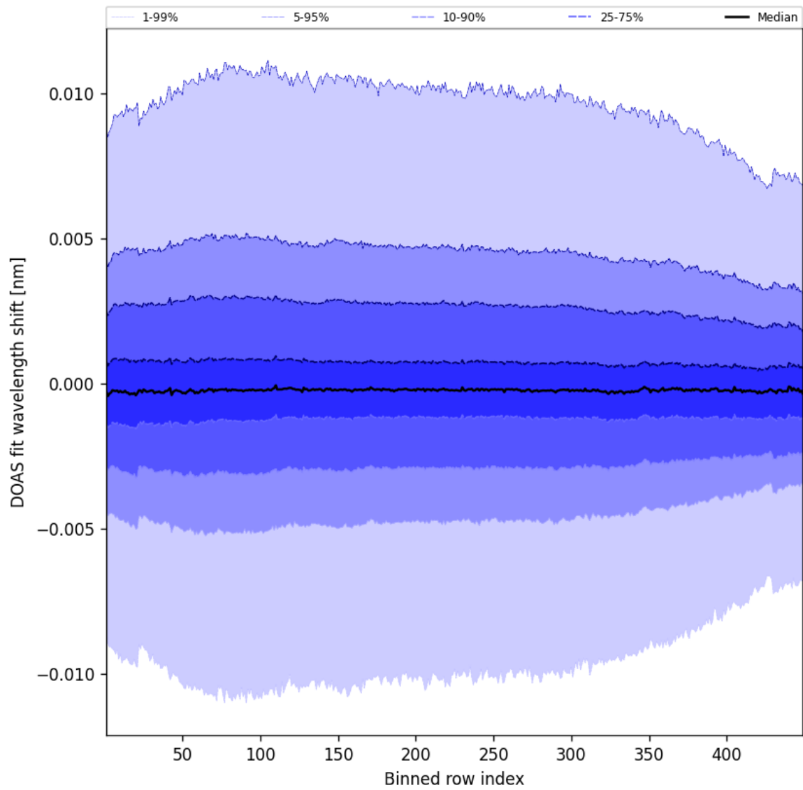
Figure 56: Along track statistics of “DOAS fit wavelength shift” for 2025-09-25 to 2025-09-26
