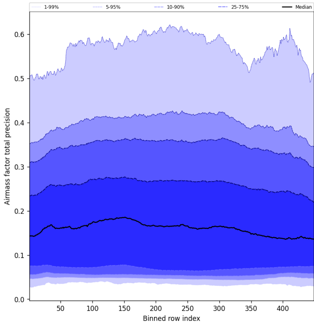
Figure 53: Along track statistics of “Airmass factor total precision” for 2025-09-25 to 2025-09-26
