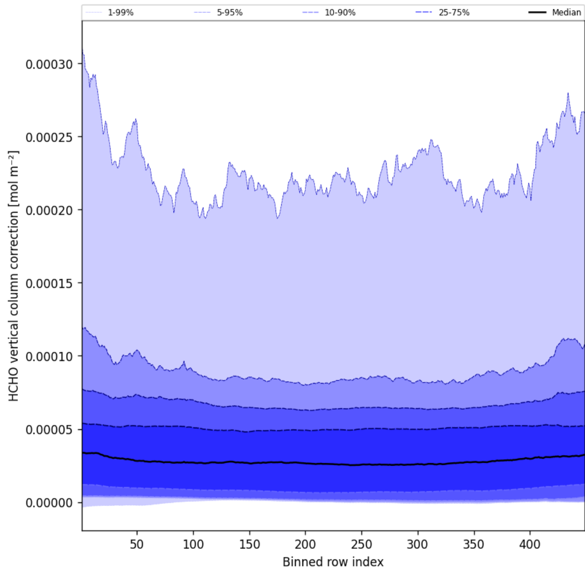
Figure 49: Along track statistics of “HCHO vertical column correction” for 2025-09-25 to 2025-09-26
