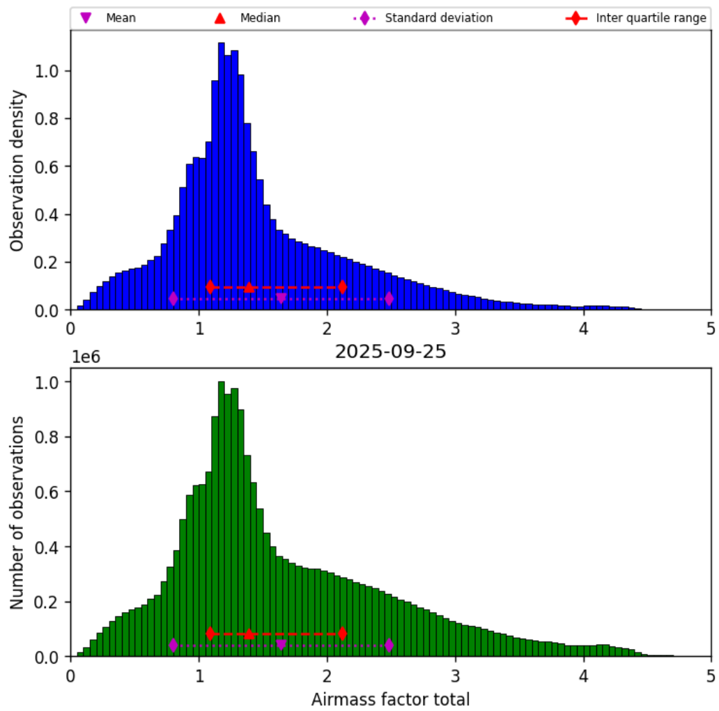
Figure 38: Histogram of “Airmass factor total” for 2025-09-25 to 2025-09-26
