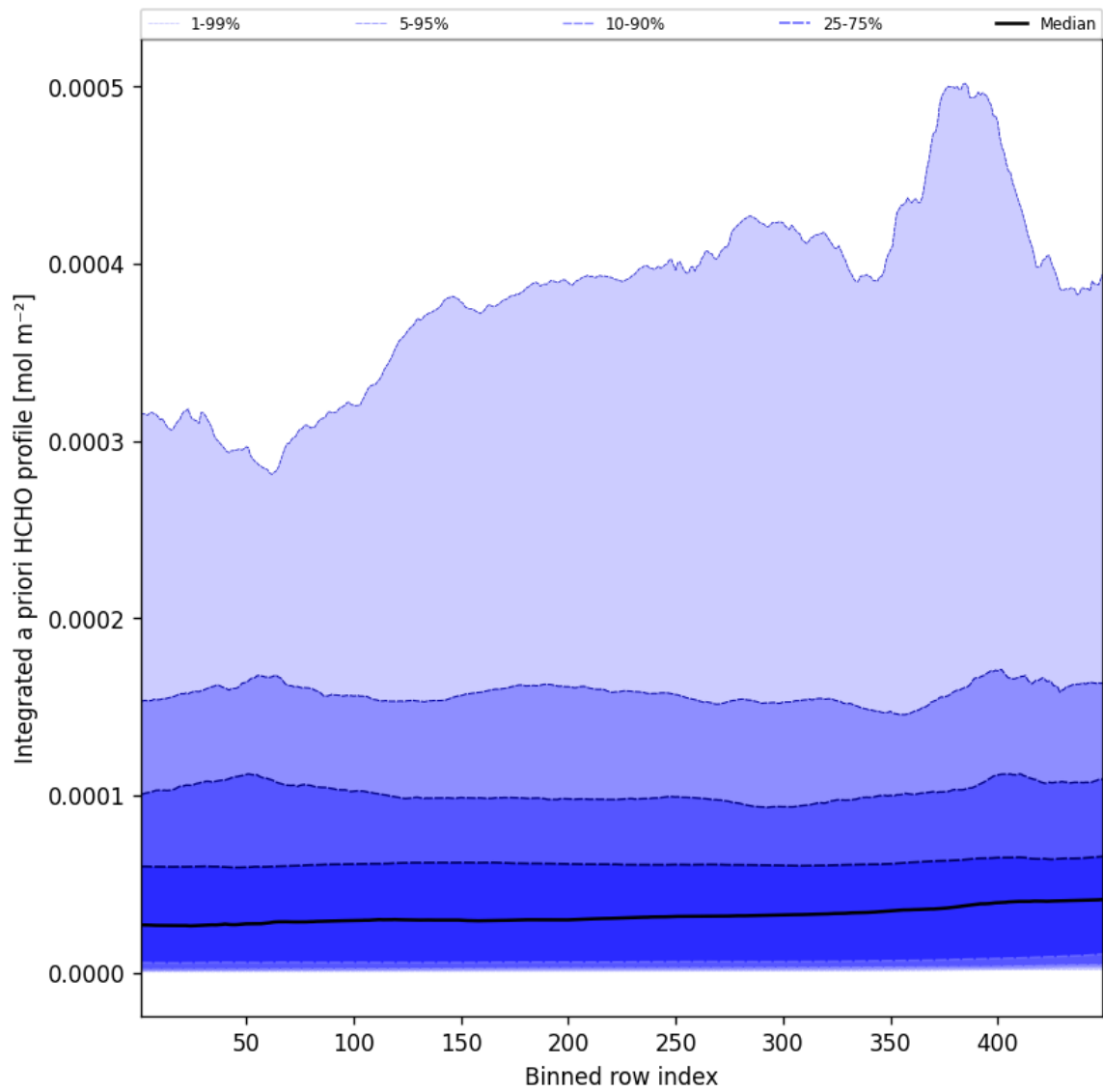
Figure 55: Along track statistics of “Integrated a priori HCHO profile” for 2025-09-26 to 2025-09-27
