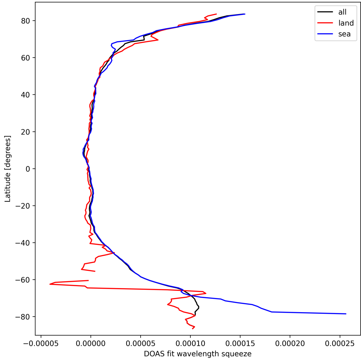
Figure 29: Zonal average of “DOAS fit wavelength squeeze” for 2025-09-26 to 2025-09-27.
