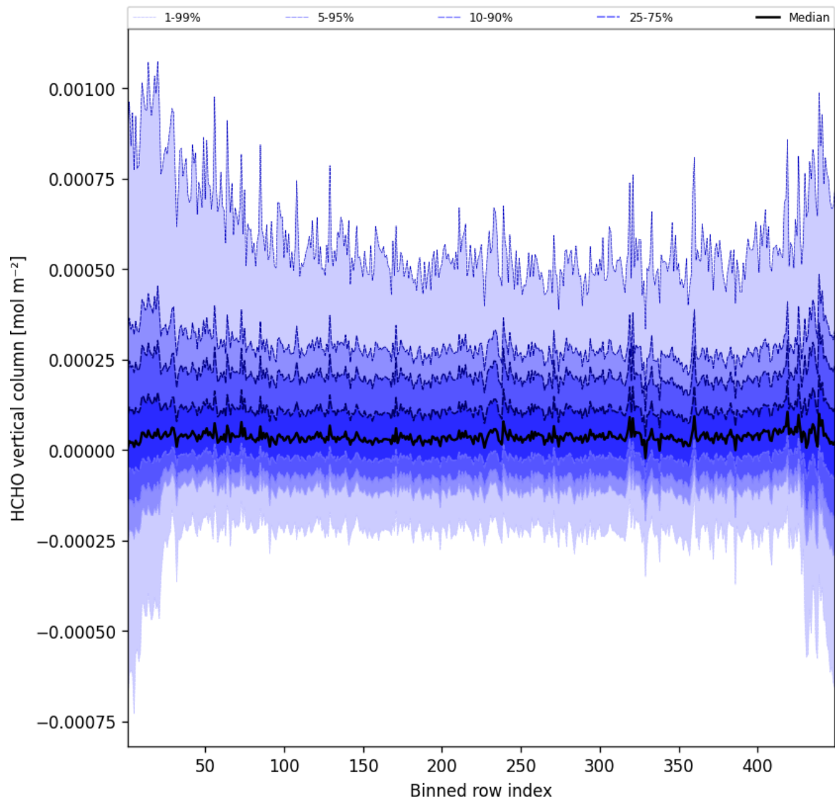
Figure 47: Along track statistics of “HCHO vertical column” for 2025-09-26 to 2025-09-27
