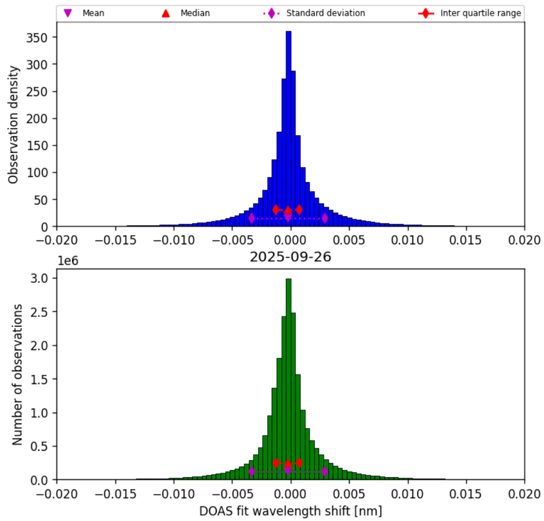
Figure 42: Histogram of “DOAS fit wavelength shift” for 2025-09-26 to 2025-09-27
