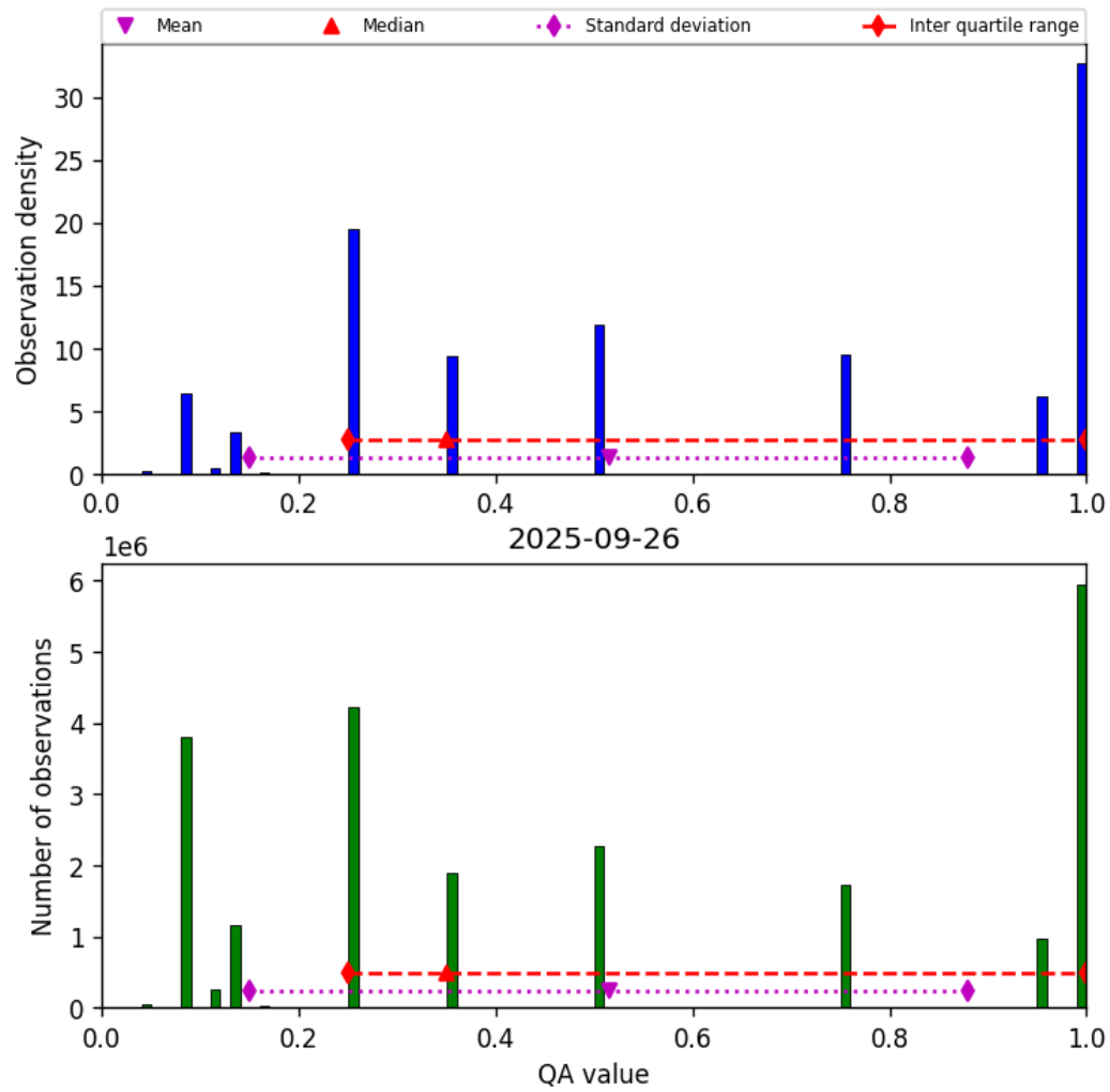
Figure 32: Histogram of “QA value” for 2025-09-26 to 2025-09-27
