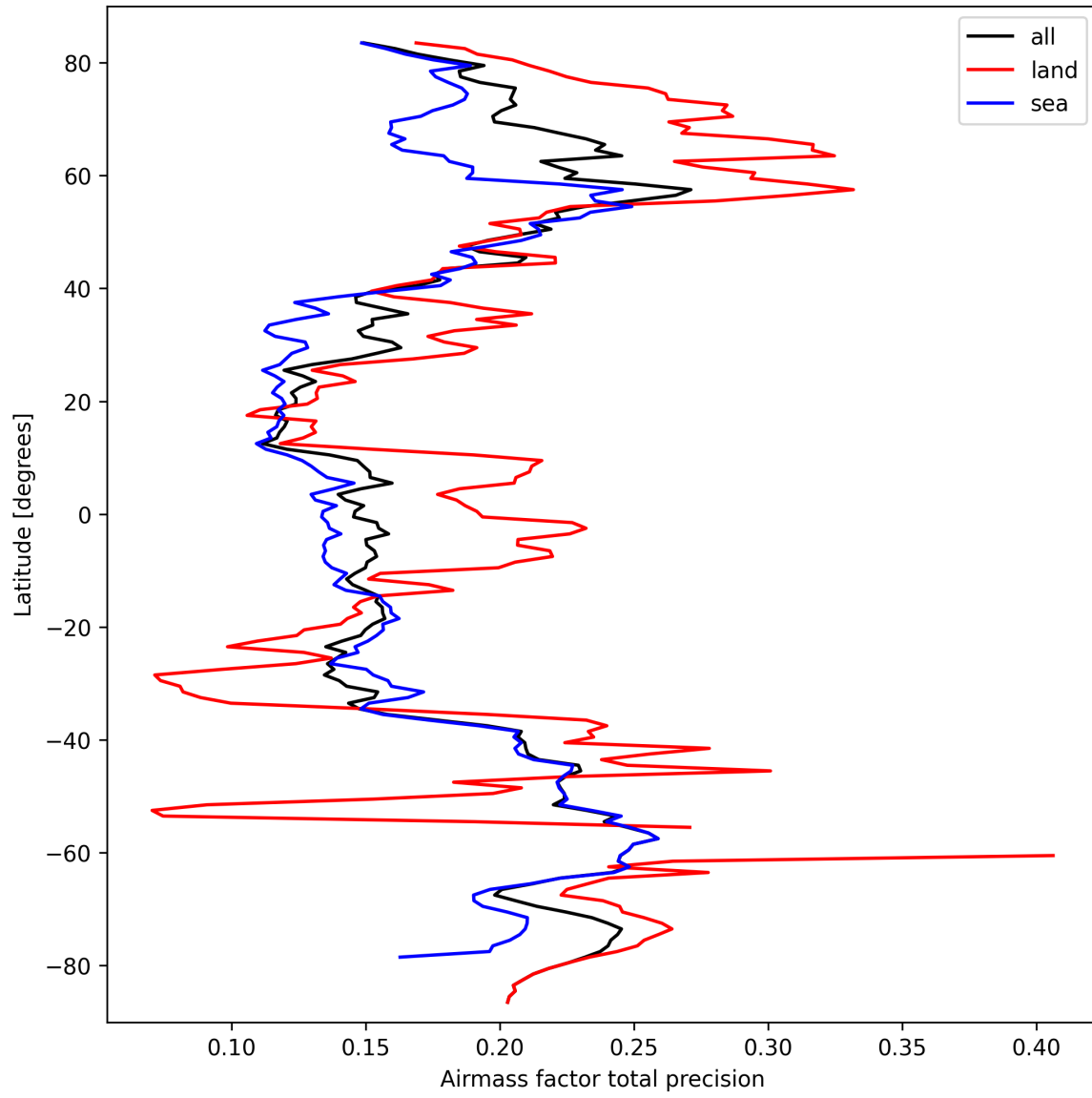
Figure 25: Zonal average of “Airmass factor total precision” for 2025-09-26 to 2025-09-27.
