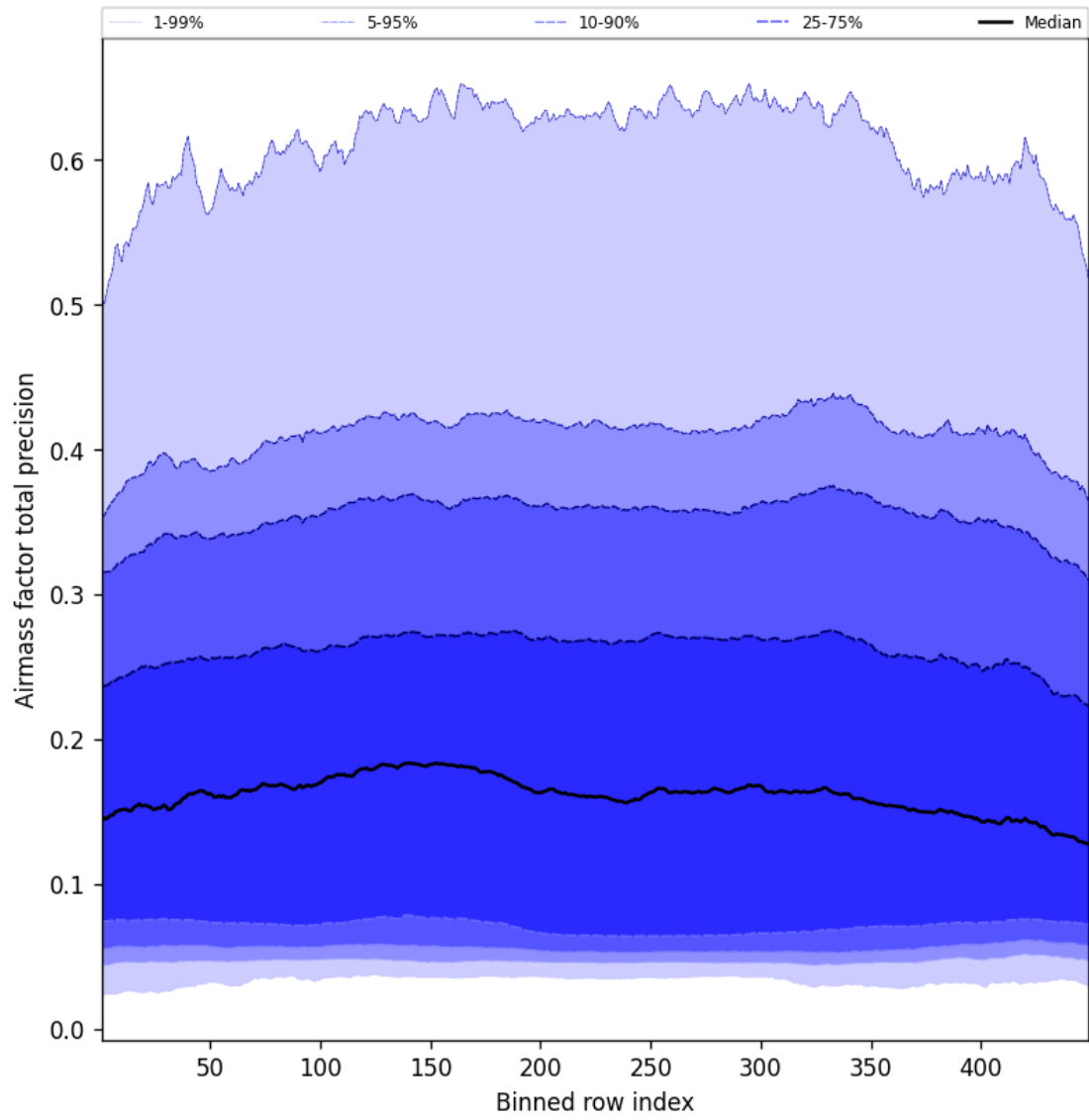
Figure 53: Along track statistics of “Airmass factor total precision” for 2025-09-26 to 2025-09-27
