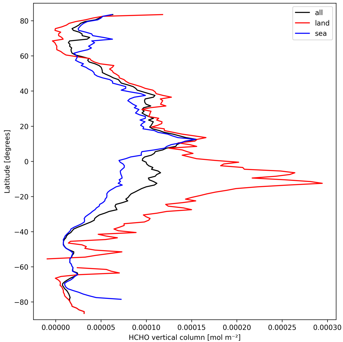
Figure 19: Zonal average of “HCHO vertical column” for 2025-09-26 to 2025-09-27.
