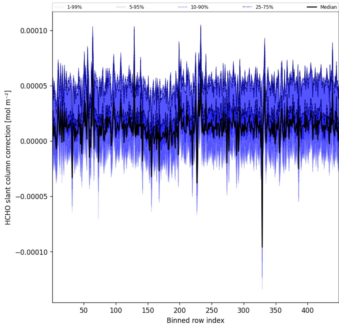
Figure 59: Along track statistics of “HCHO slant column correction” for 2025-09-26 to 2025-09-27
