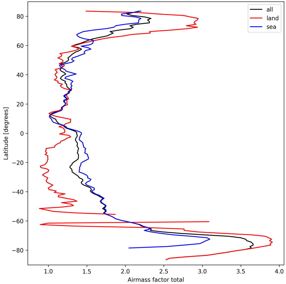
Figure 24: Zonal average of “Airmass factor total” for 2025-09-26 to 2025-09-27.
