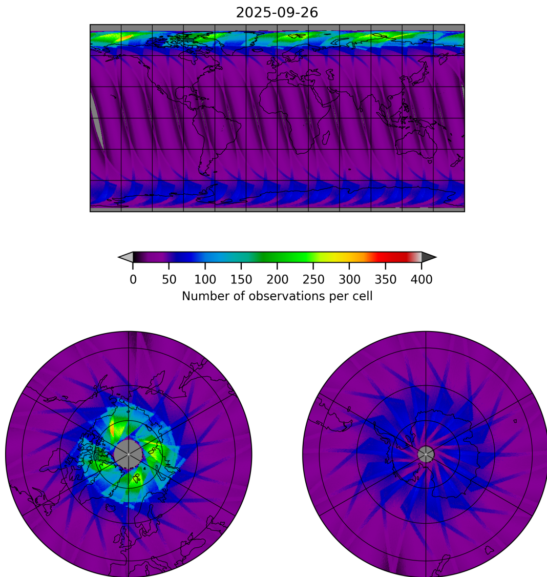
Figure 17: Map of the number of observations for 2025-09-26 to 2025-09-27
