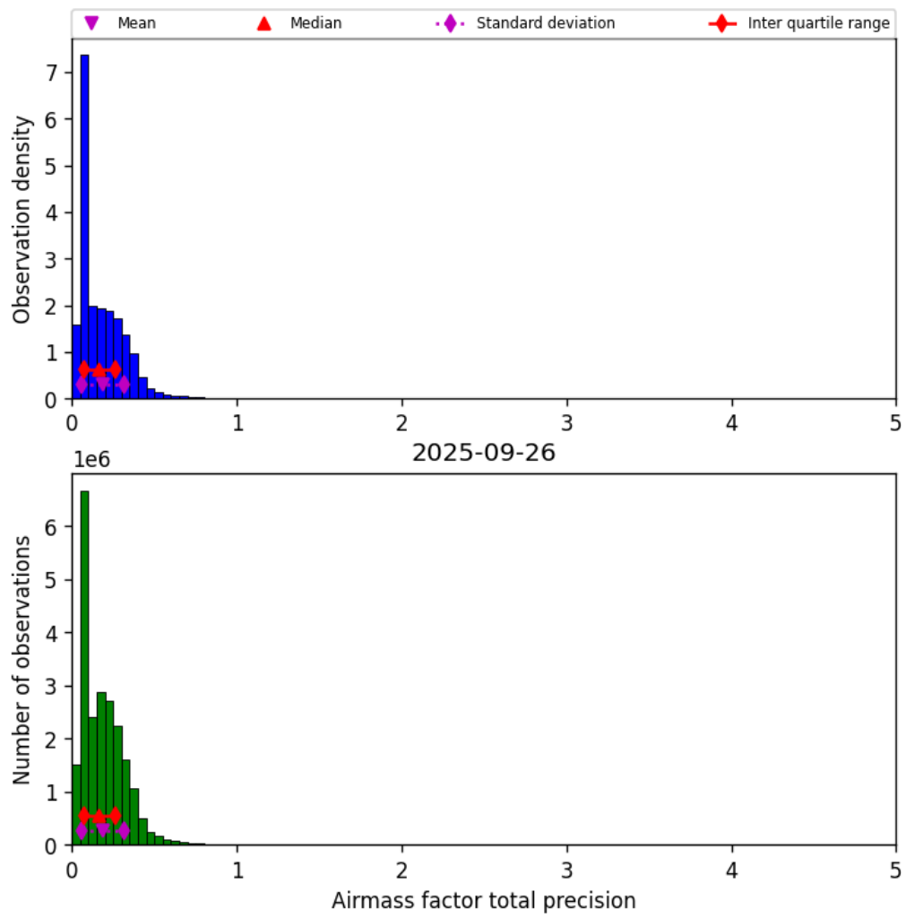
Figure 39: Histogram of “Airmass factor total precision” for 2025-09-26 to 2025-09-27
