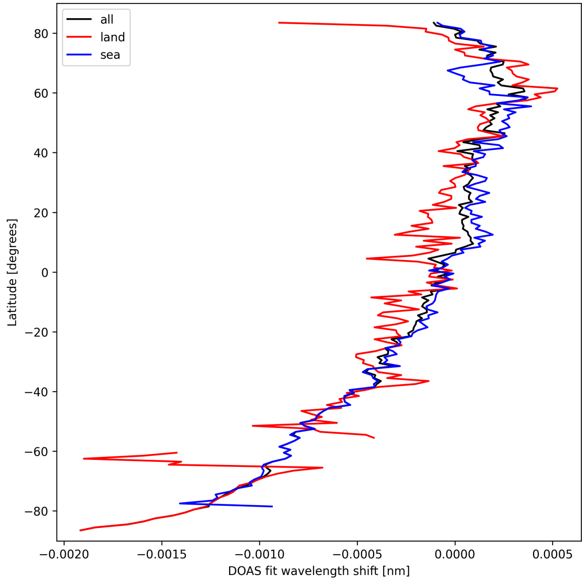
Figure 28: Zonal average of “DOAS fit wavelength shift” for 2025-09-26 to 2025-09-27.
