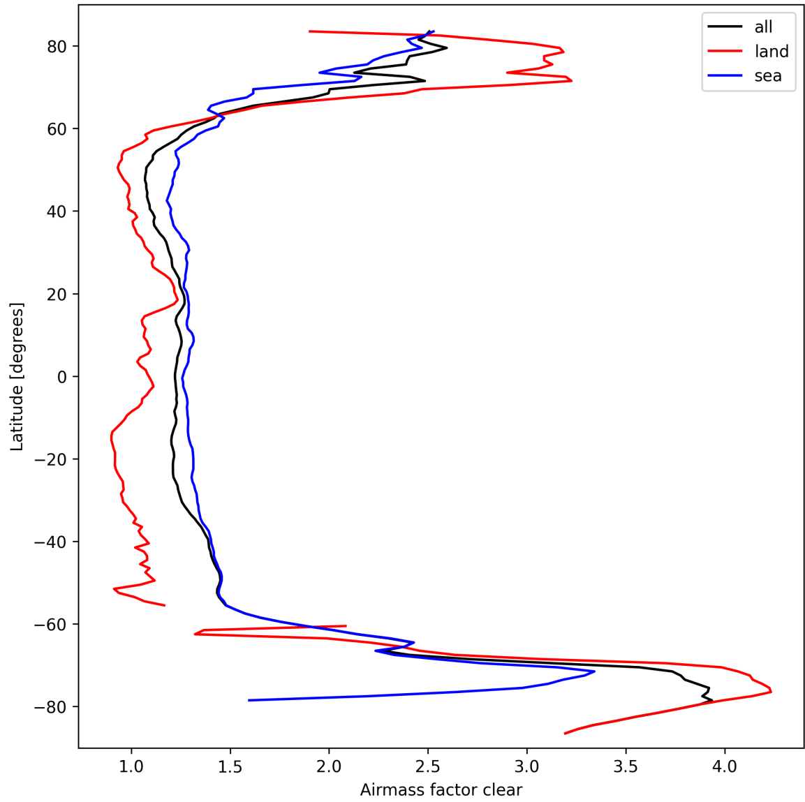
Figure 26: Zonal average of “Airmass factor clear” for 2025-09-26 to 2025-09-27.
