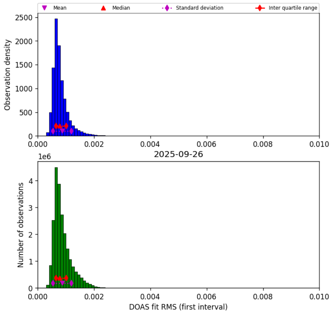
Figure 44: Histogram of “DOAS fit RMS (first interval)” for 2025-09-26 to 2025-09-27
