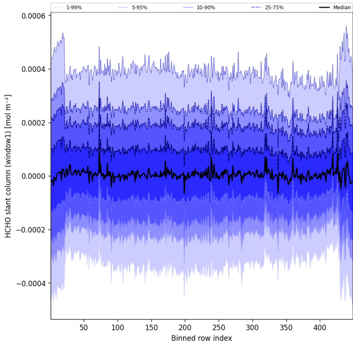
Figure 50: Along track statistics of “HCHO slant column (window1)” for 2025-09-26 to 2025-09-27
