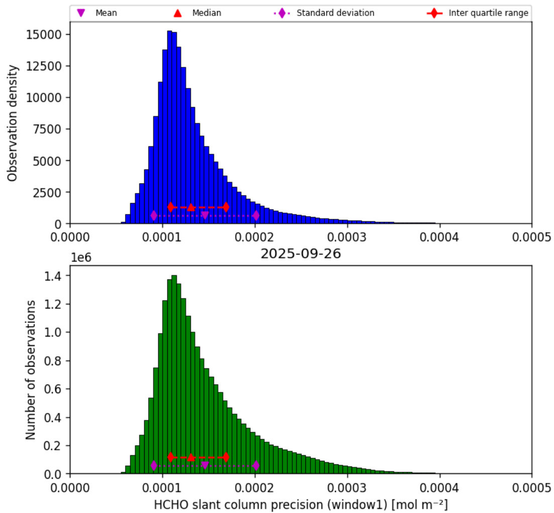
Figure 37: Histogram of “HCHO slant column precision (window1)” for 2025-09-26 to 2025-09-27
