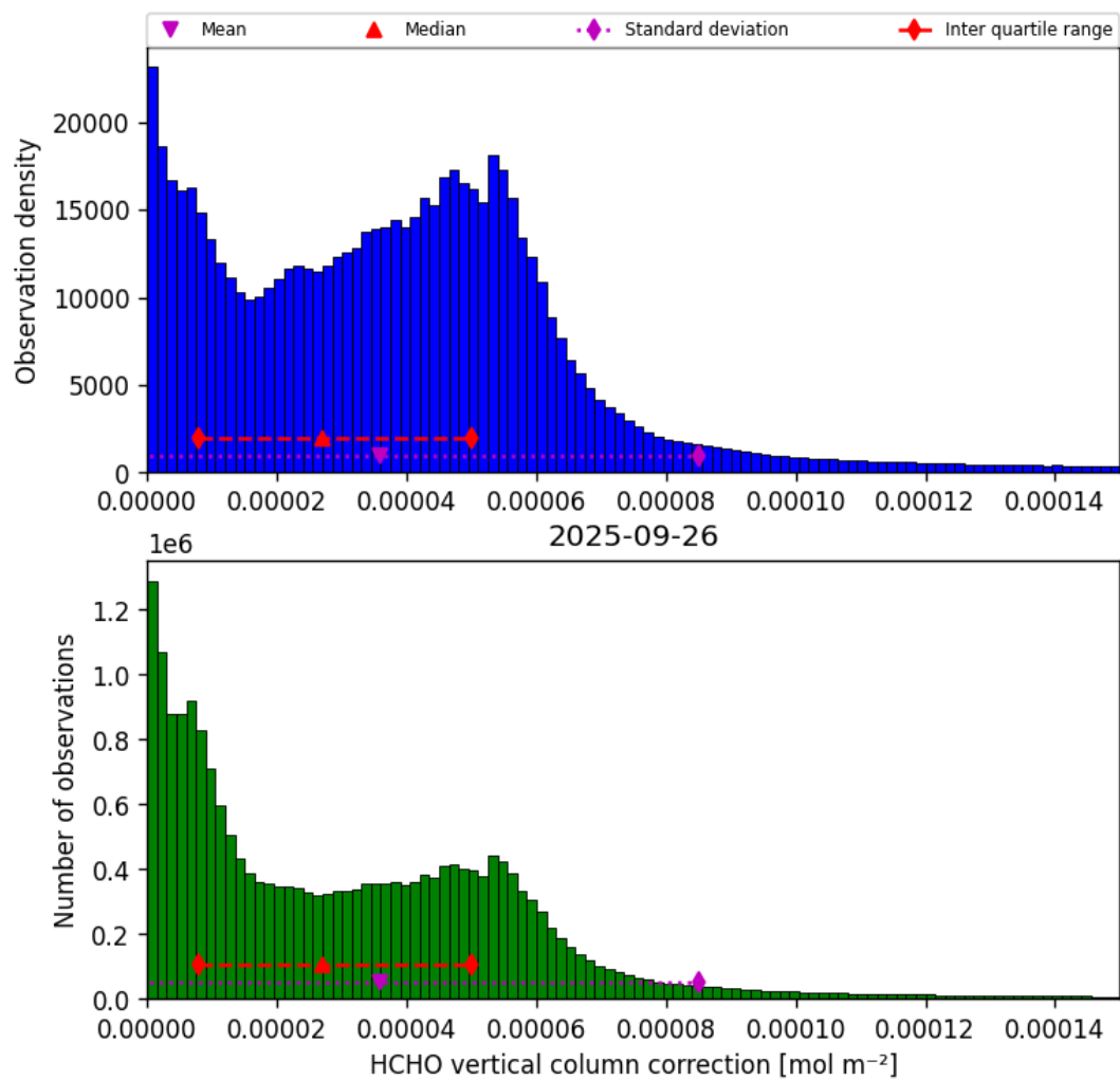
Figure 35: Histogram of “HCHO vertical column correction” for 2025-09-26 to 2025-09-27
