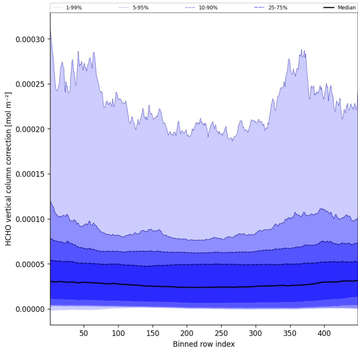
Figure 49: Along track statistics of “HCHO vertical column correction” for 2025-09-26 to 2025-09-27
