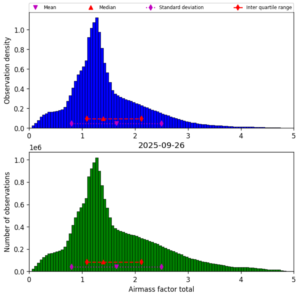
Figure 38: Histogram of “Airmass factor total” for 2025-09-26 to 2025-09-27
