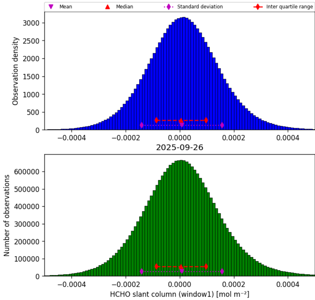
Figure 36: Histogram of “HCHO slant column (window1)” for 2025-09-26 to 2025-09-27
