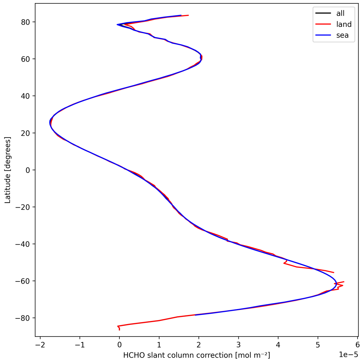
Figure 31: Zonal average of “HCHO slant column correction” for 2025-09-26 to 2025-09-27.
