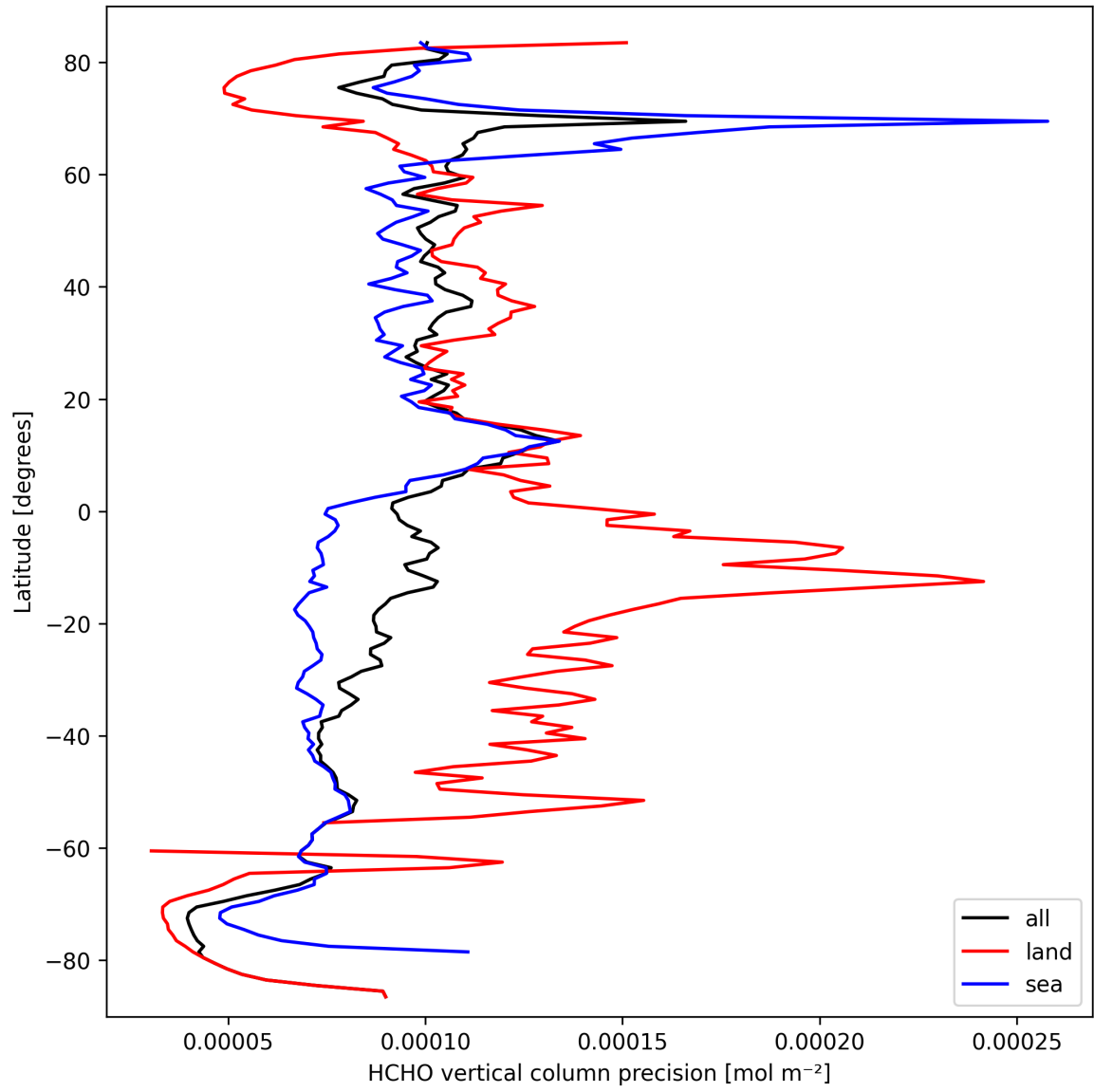
Figure 20: Zonal average of “HCHO vertical column precision” for 2025-09-26 to 2025-09-27.
