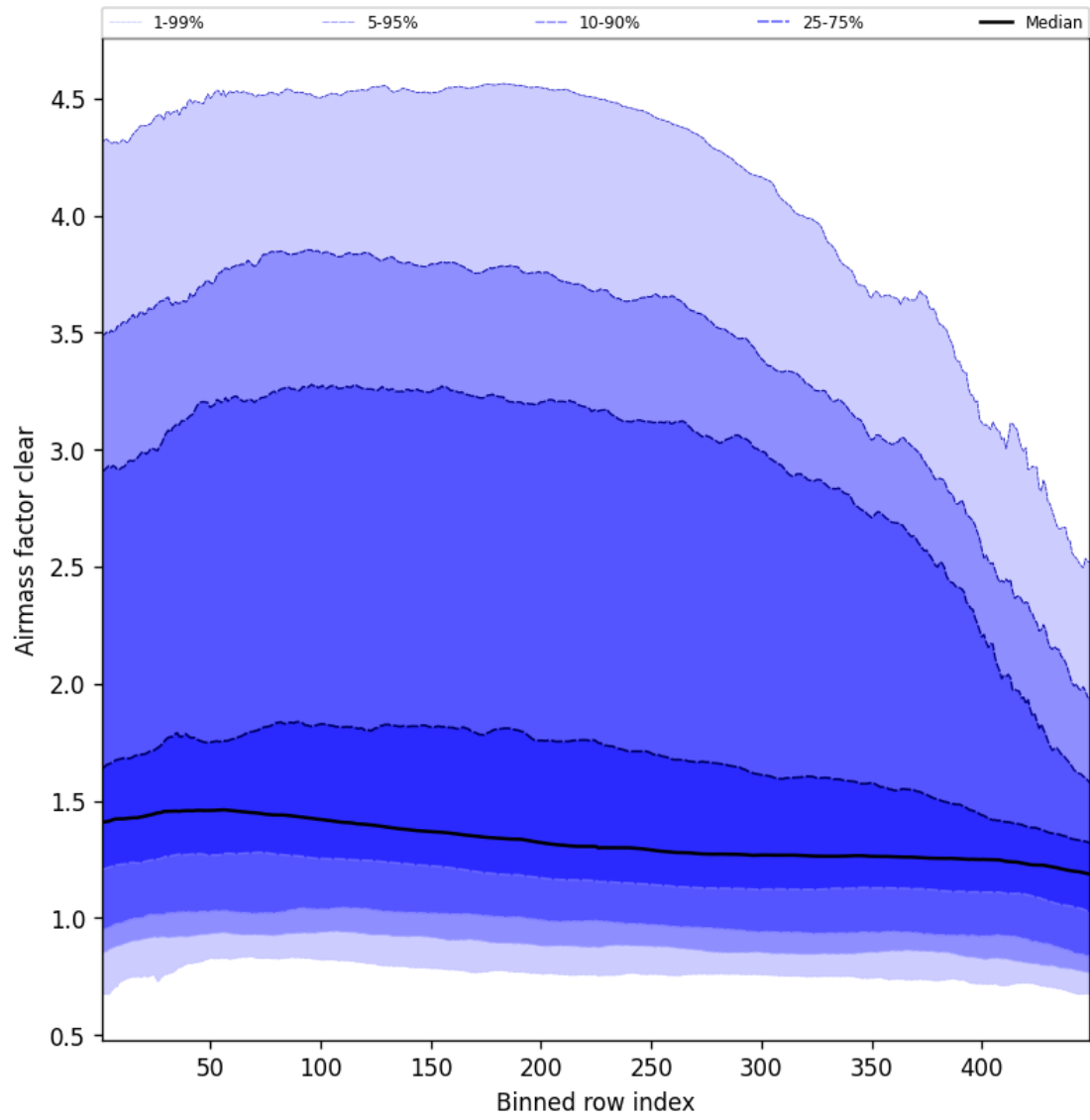
Figure 54: Along track statistics of “Airmass factor clear” for 2025-09-26 to 2025-09-27
