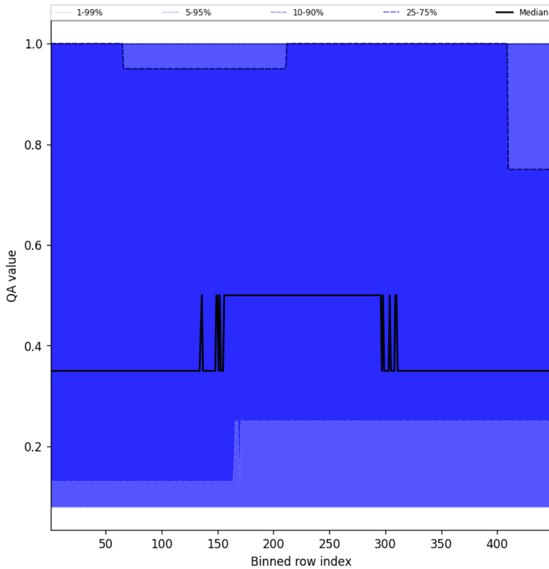
Figure 46: Along track statistics of “QA value” for 2025-09-26 to 2025-09-27
