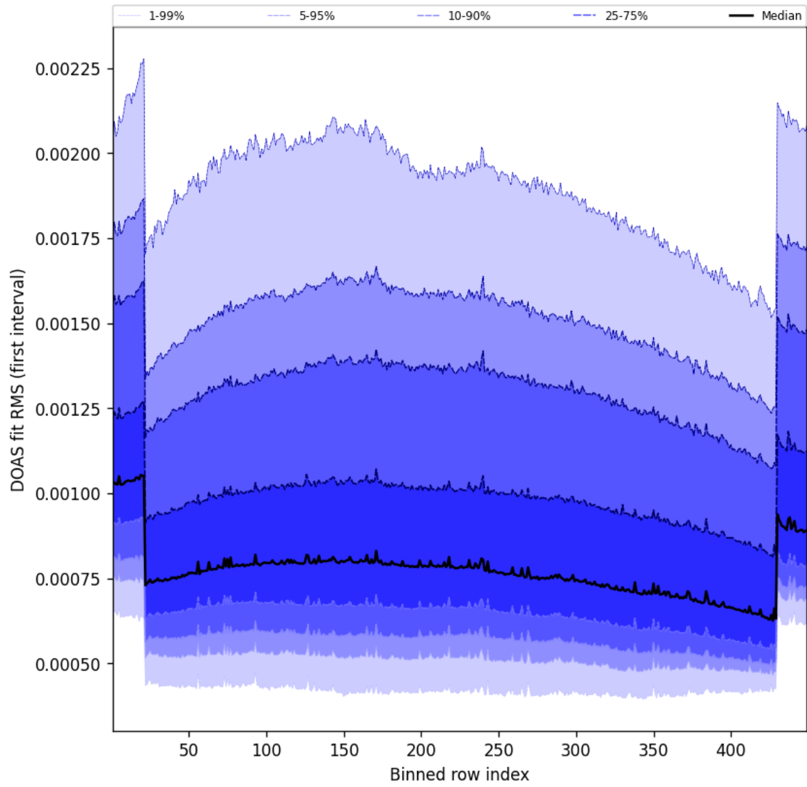
Figure 58: Along track statistics of “DOAS fit RMS (first interval)” for 2025-09-26 to 2025-09-27
