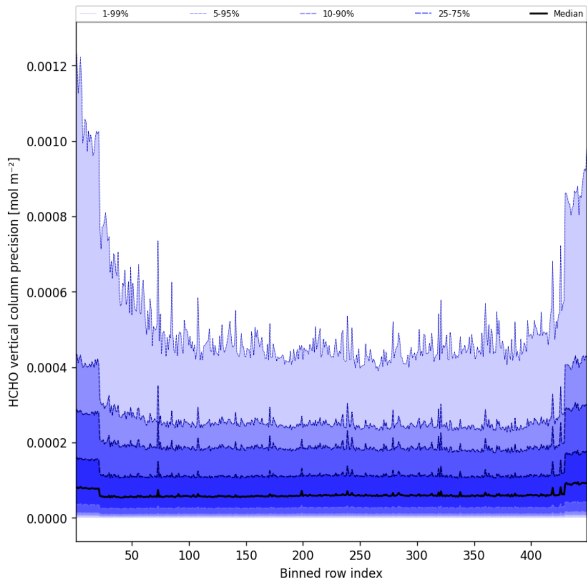
Figure 48: Along track statistics of “HCHO vertical column precision” for 2025-09-26 to 2025-09-27
