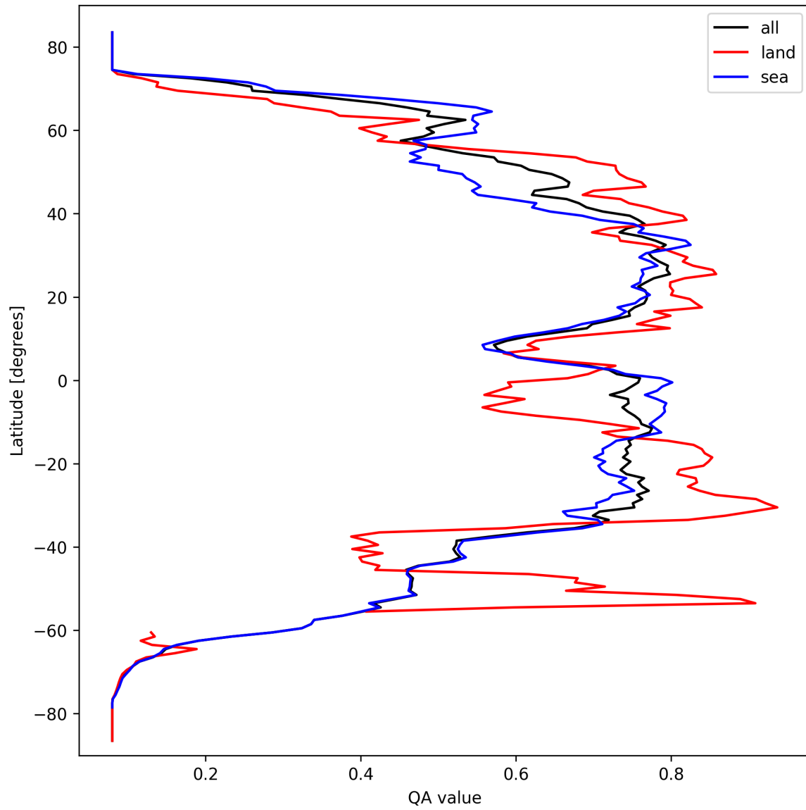
Figure 18: Zonal average of “QA value” for 2025-09-26 to 2025-09-27.
