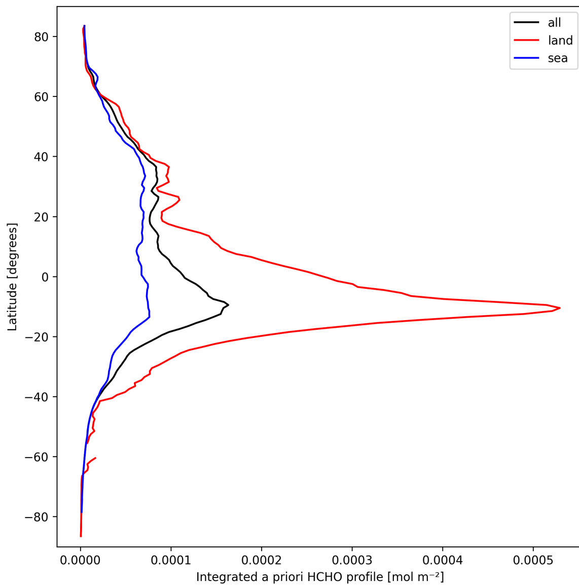
Figure 27: Zonal average of “Integrated a priori HCHO profile” for 2025-09-26 to 2025-09-27.
