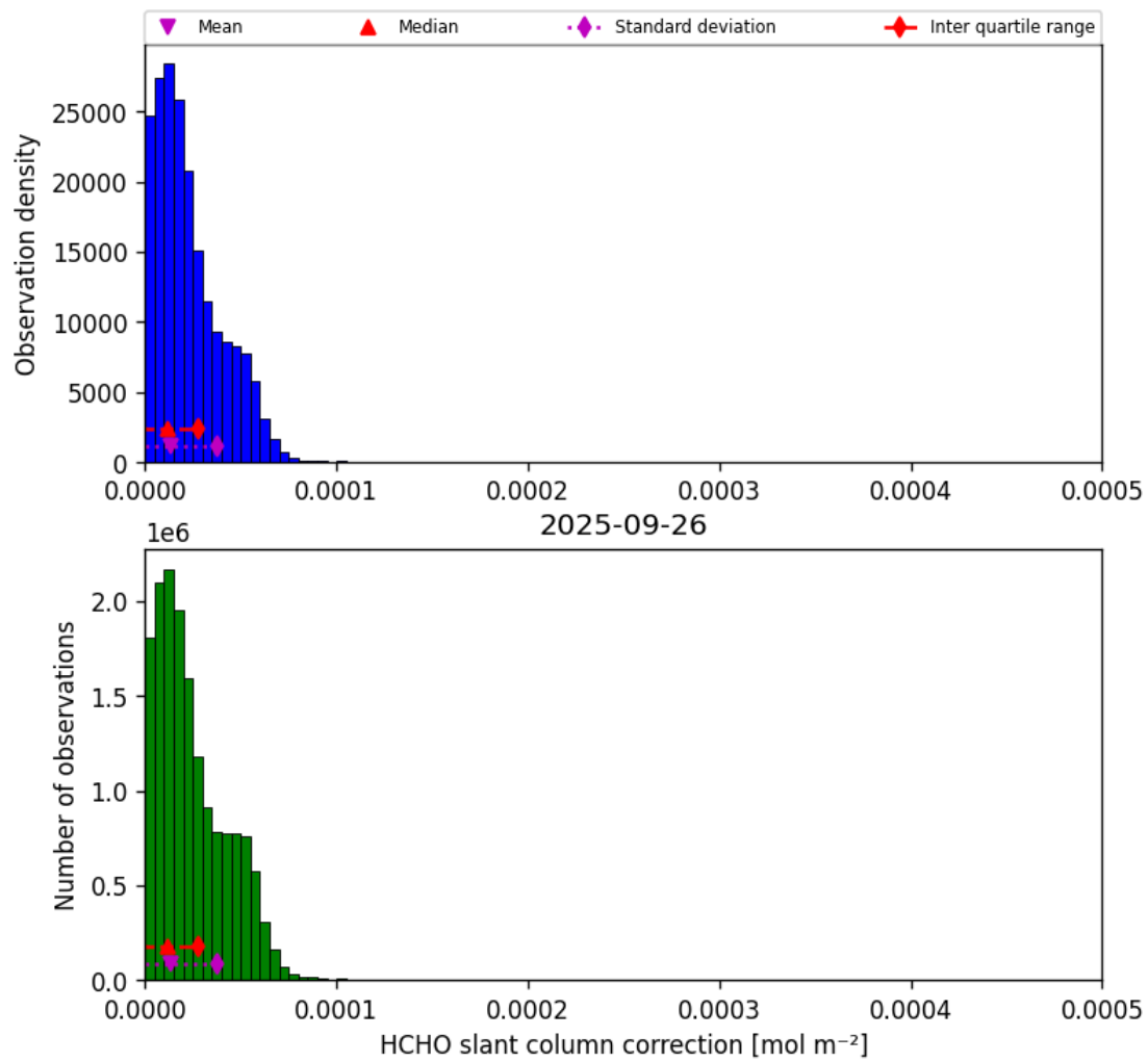
Figure 45: Histogram of “HCHO slant column correction” for 2025-09-26 to 2025-09-27
