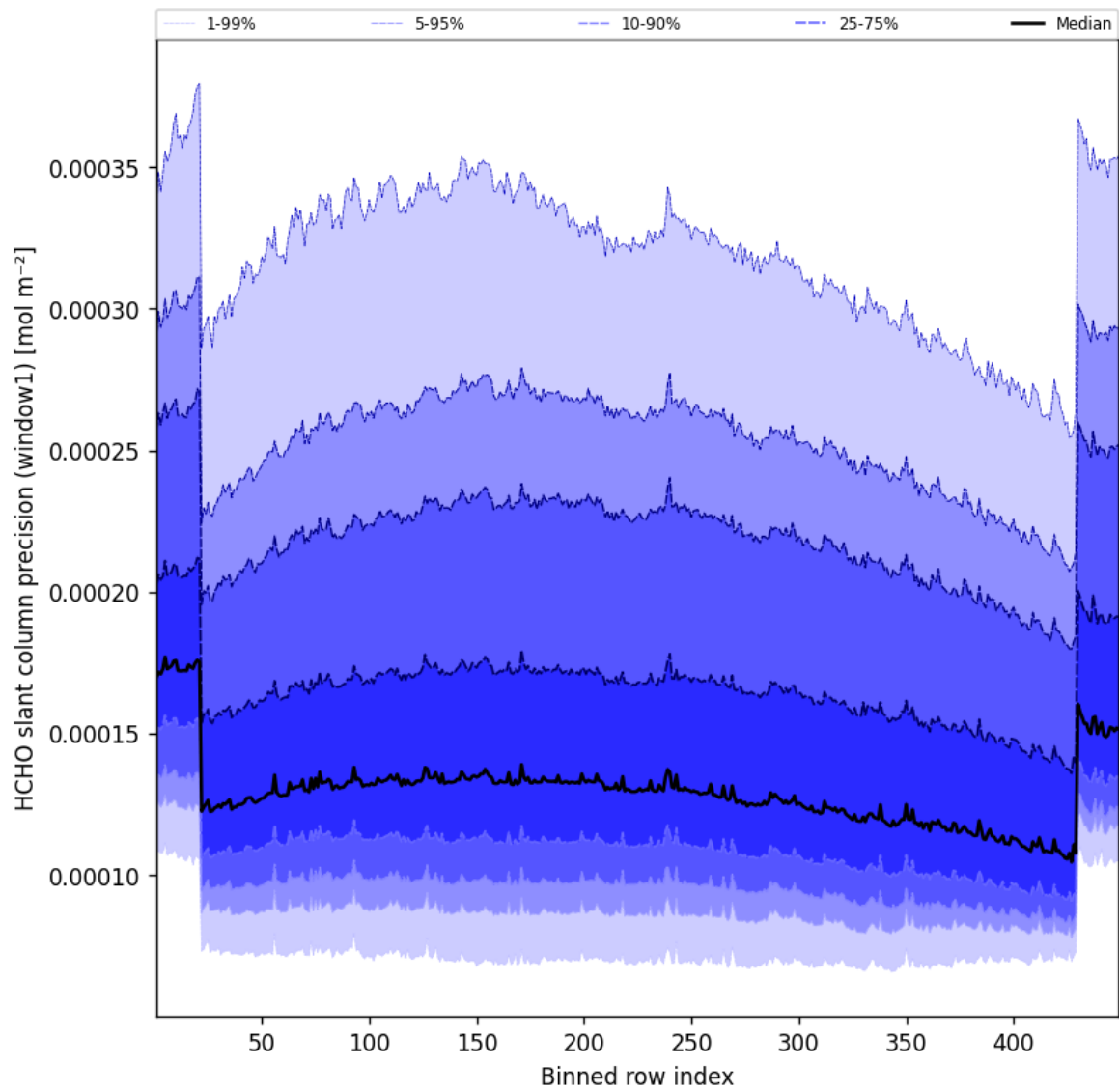
Figure 51: Along track statistics of “HCHO slant column precision (window1)” for 2025-09-26 to 2025-09-27
