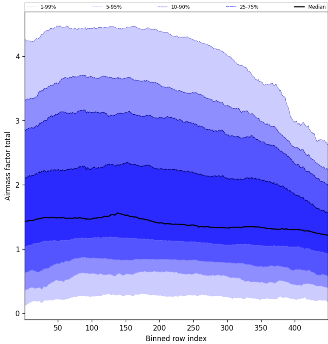
Figure 52: Along track statistics of “Airmass factor total” for 2025-09-26 to 2025-09-27
