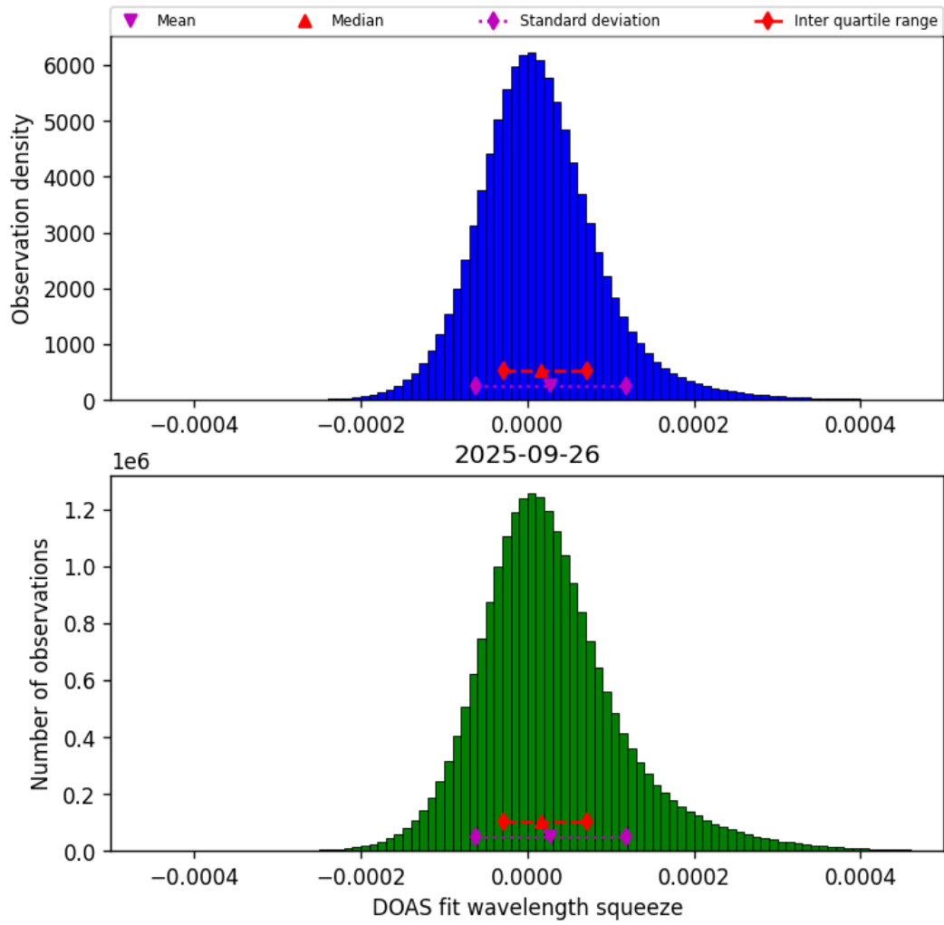
Figure 43: Histogram of “DOAS fit wavelength squeeze” for 2025-09-26 to 2025-09-27
