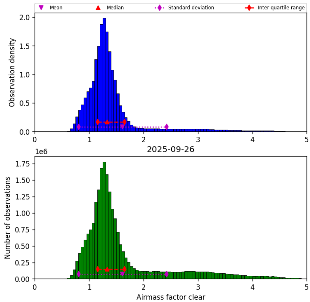
Figure 40: Histogram of “Airmass factor clear” for 2025-09-26 to 2025-09-27
