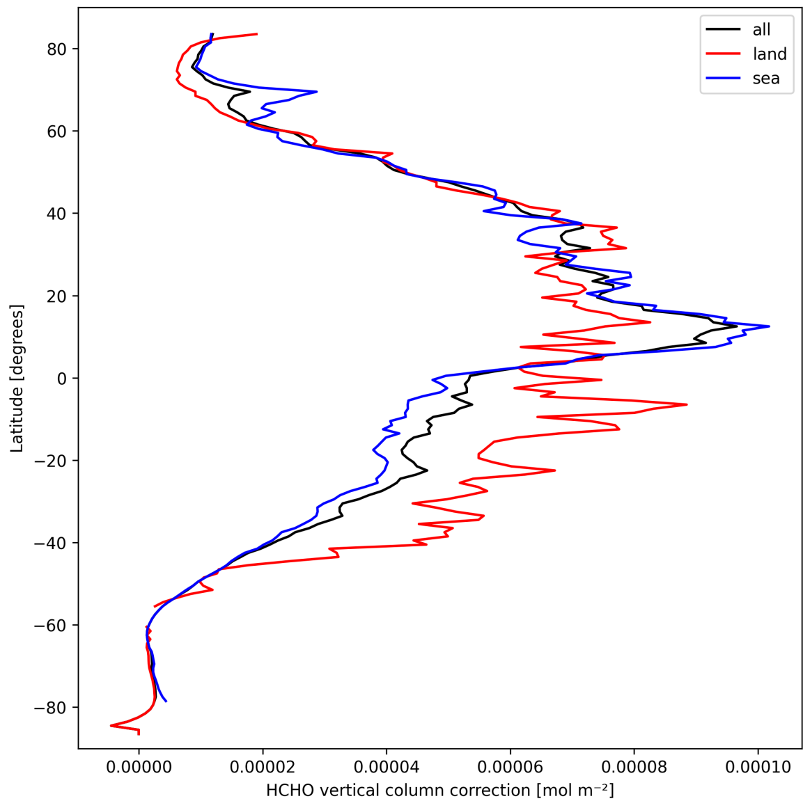
Figure 21: Zonal average of “HCHO vertical column correction” for 2025-09-26 to 2025-09-27.
