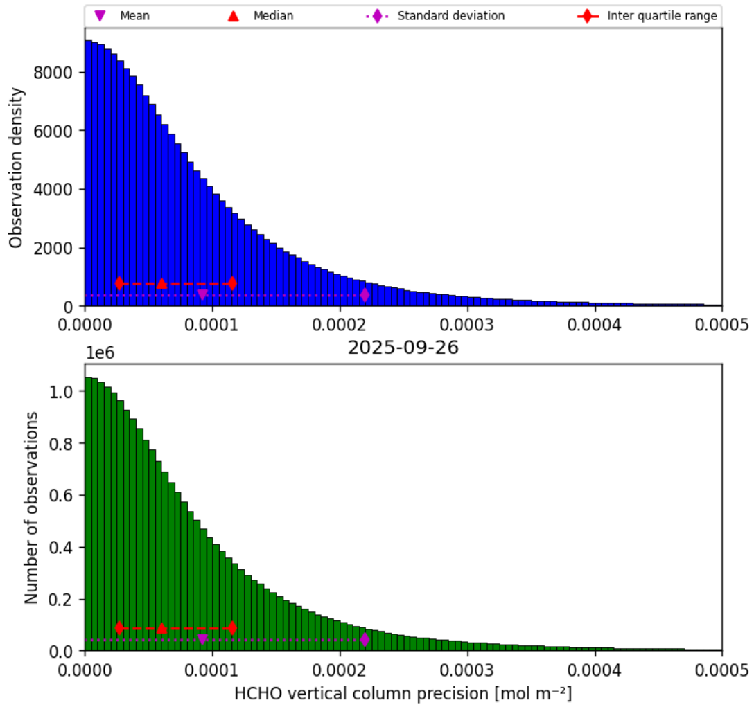
Figure 34: Histogram of “HCHO vertical column precision” for 2025-09-26 to 2025-09-27
