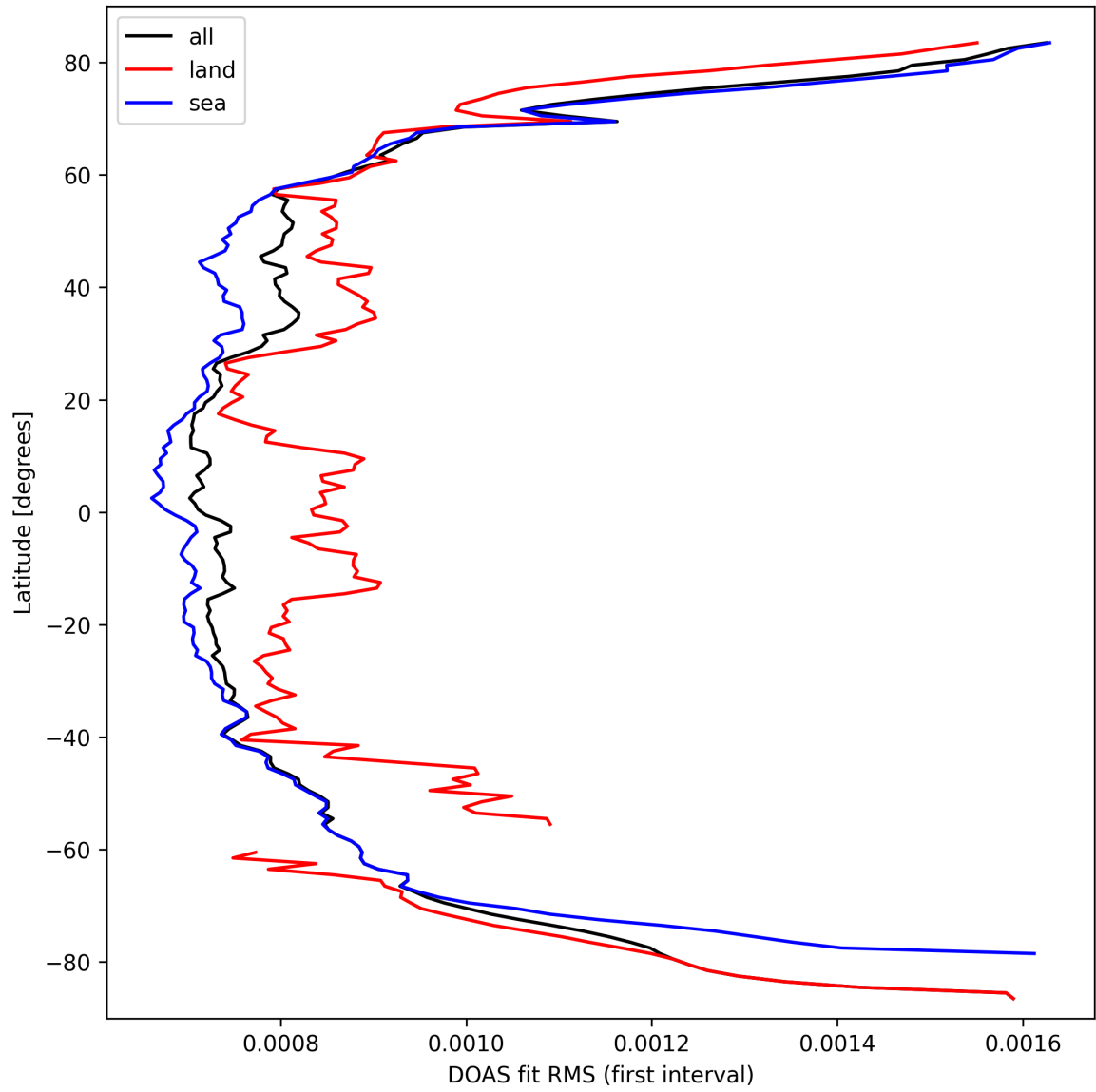
Figure 30: Zonal average of "DOAS fit RMS (first interval)" for 2025-09-26 to 2025-09-27.
