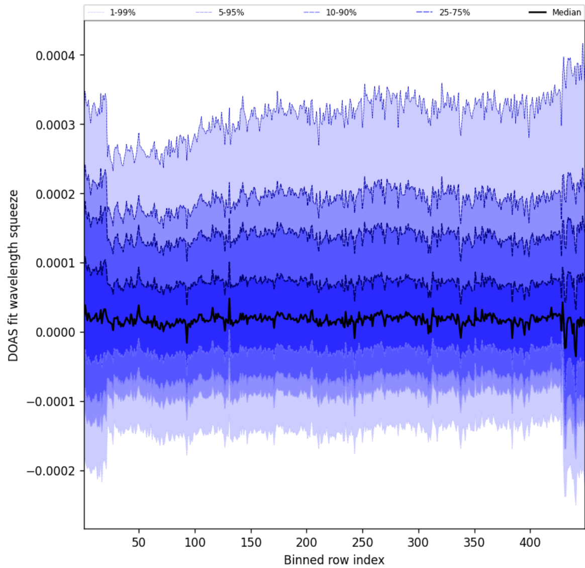
Figure 57: Along track statistics of “DOAS fit wavelength squeeze” for 2025-09-26 to 2025-09-27
