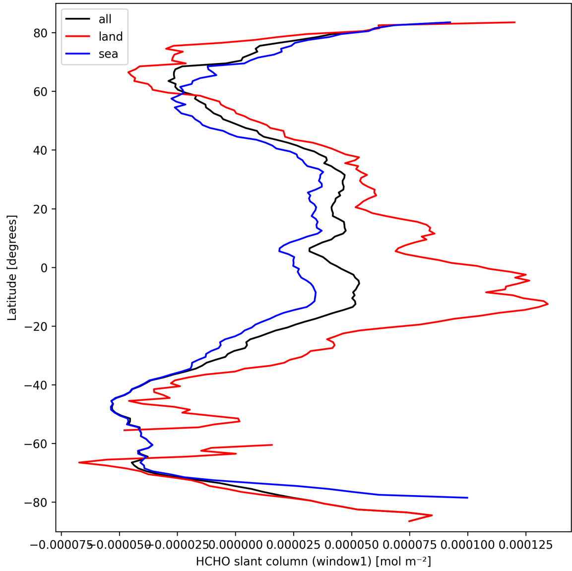
Figure 22: Zonal average of “HCHO slant column (window1)” for 2025-09-26 to 2025-09-27.
