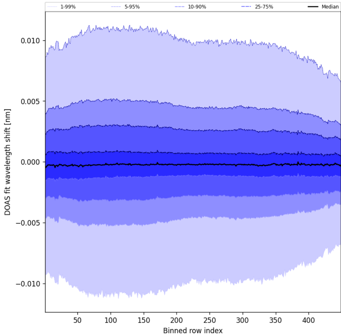
Figure 56: Along track statistics of “DOAS fit wavelength shift” for 2025-09-26 to 2025-09-27
