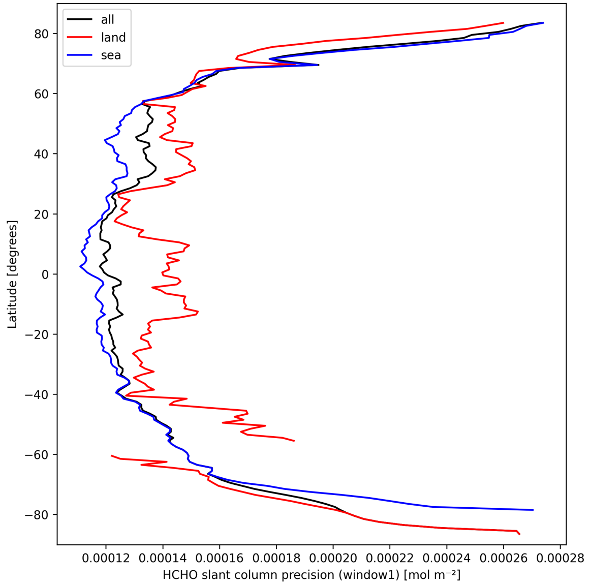
Figure 23: Zonal average of “HCHO slant column precision (window1)” for 2025-09-26 to 2025-09-27.
