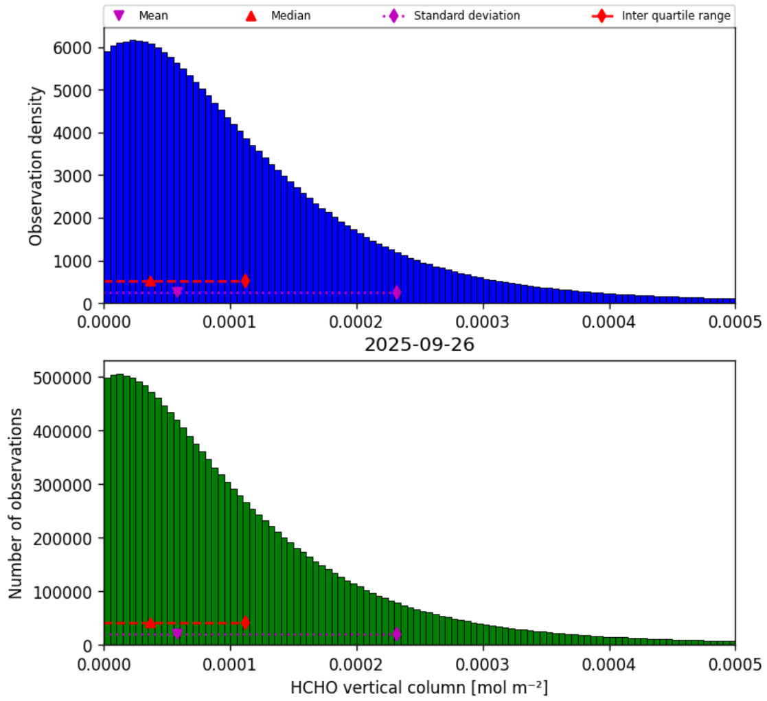
Figure 33: Histogram of “HCHO vertical column” for 2025-09-26 to 2025-09-27
