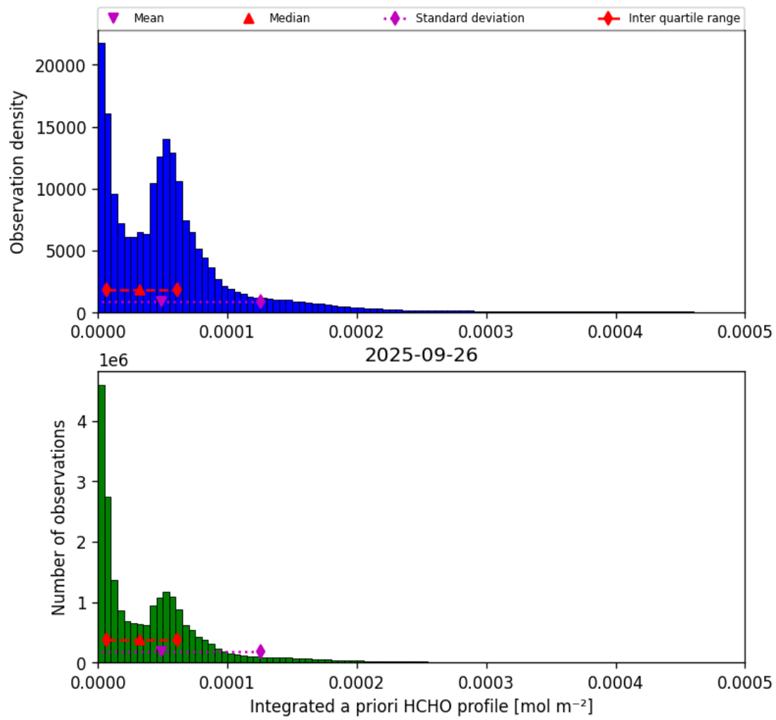
Figure 41: Histogram of “Integrated a priori HCHO profile” for 2025-09-26 to 2025-09-27
