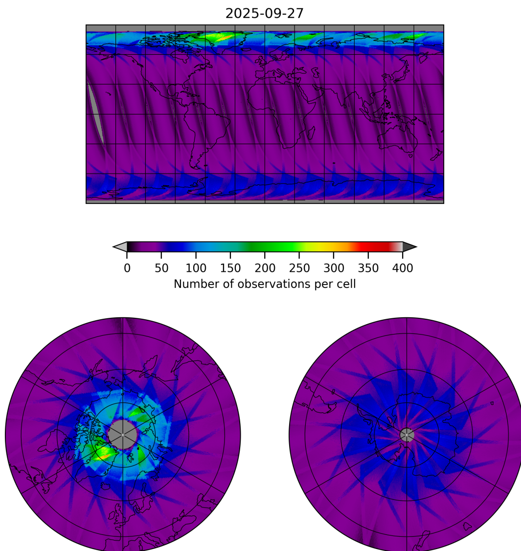
Figure 17: Map of the number of observations for 2025-09-27 to 2025-09-28
