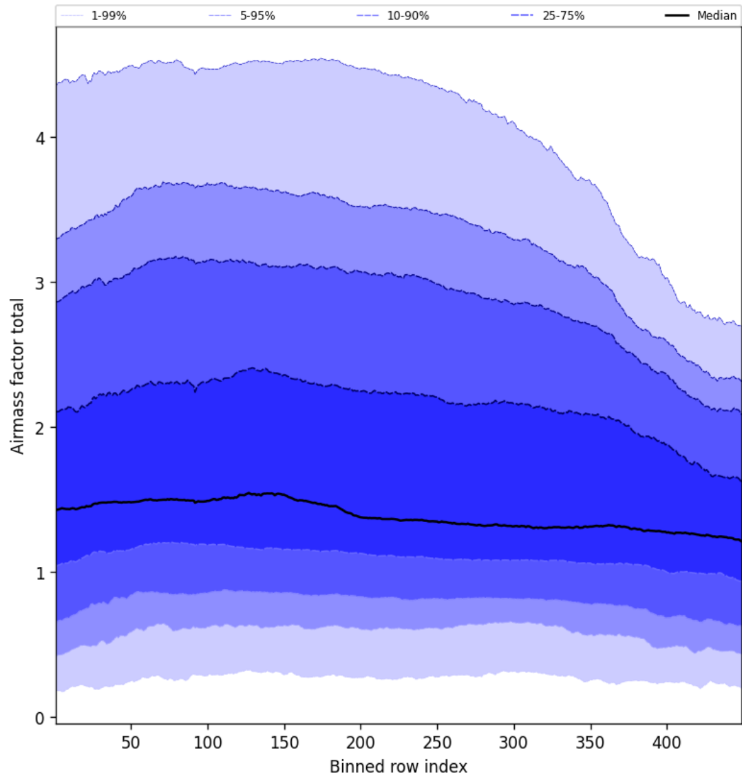
Figure 52: Along track statistics of “Airmass factor total” for 2025-09-27 to 2025-09-28
