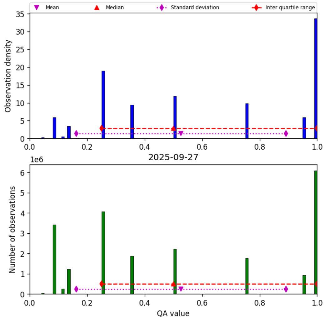
Figure 32: Histogram of “QA value” for 2025-09-27 to 2025-09-28
