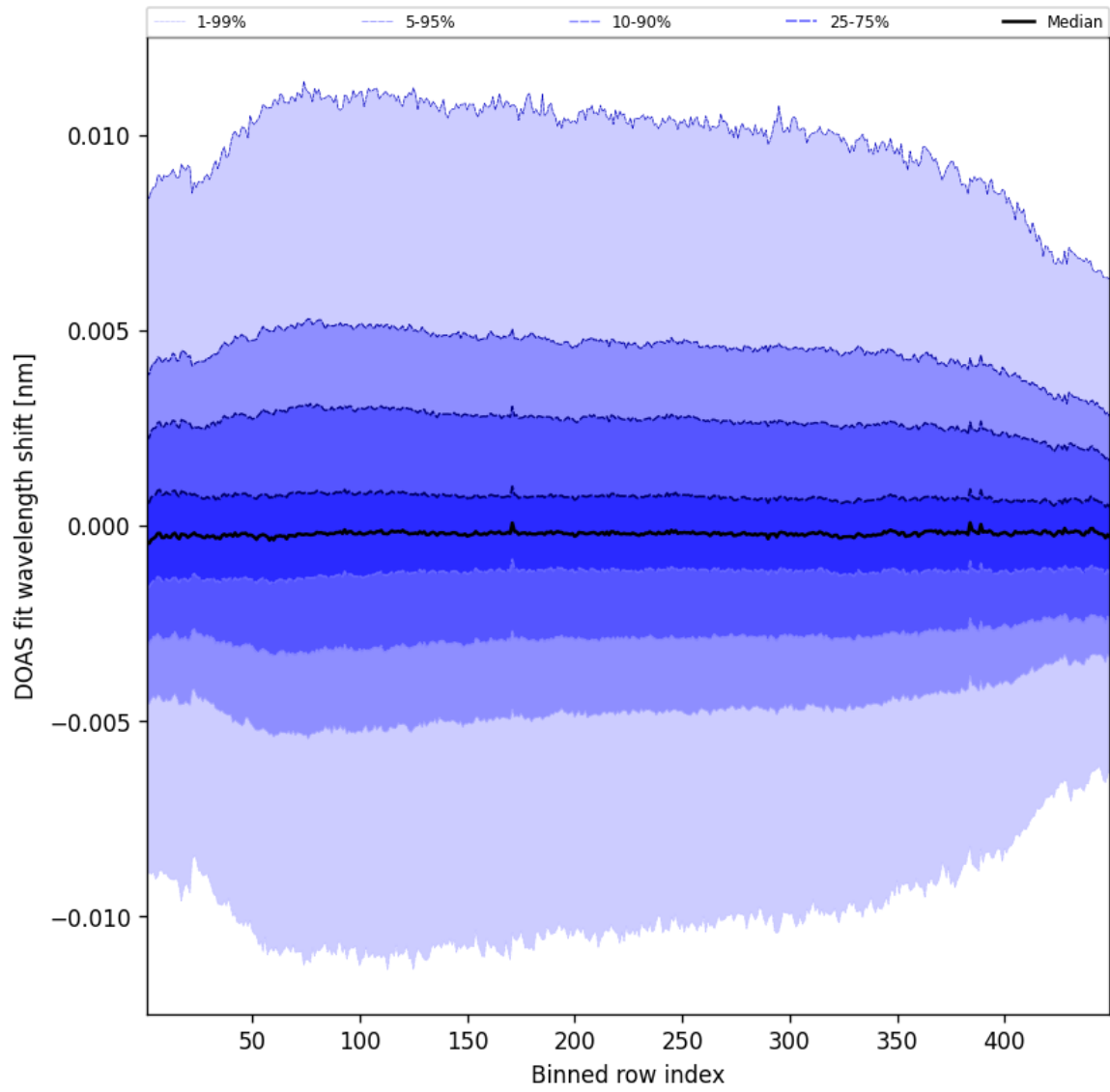
Figure 56: Along track statistics of “DOAS fit wavelength shift” for 2025-09-27 to 2025-09-28
