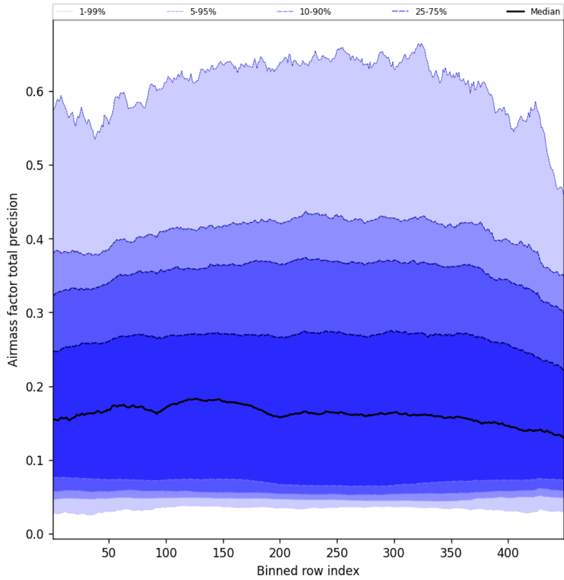
Figure 53: Along track statistics of “Airmass factor total precision” for 2025-09-27 to 2025-09-28
