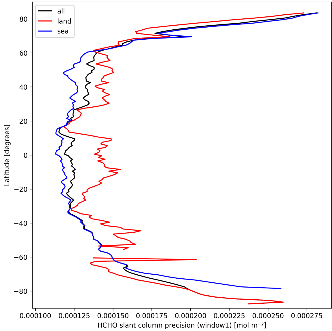
Figure 23: Zonal average of “HCHO slant column precision (window1)” for 2025-09-27 to 2025-09-28.
