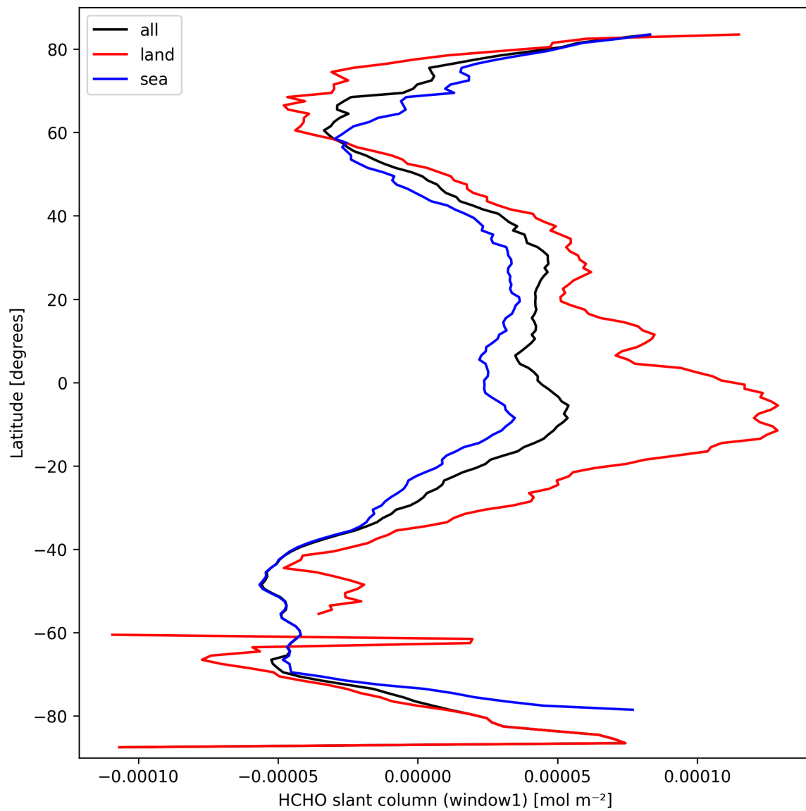
Figure 22: Zonal average of “HCHO slant column (window1)” for 2025-09-27 to 2025-09-28.
