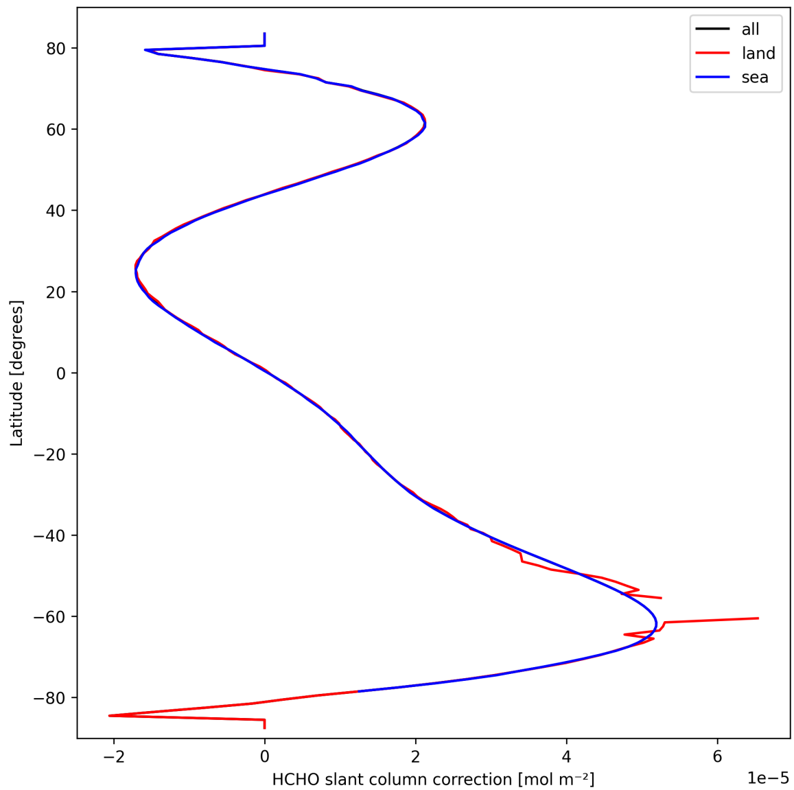
Figure 31: Zonal average of “HCHO slant column correction” for 2025-09-27 to 2025-09-28.
