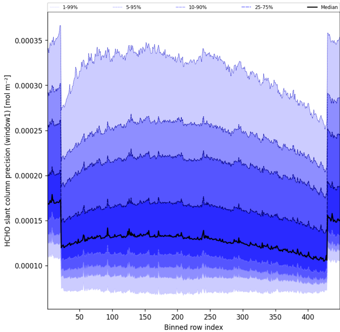
Figure 51: Along track statistics of “HCHO slant column precision (window1)” for 2025-09-27 to 2025-09-28
