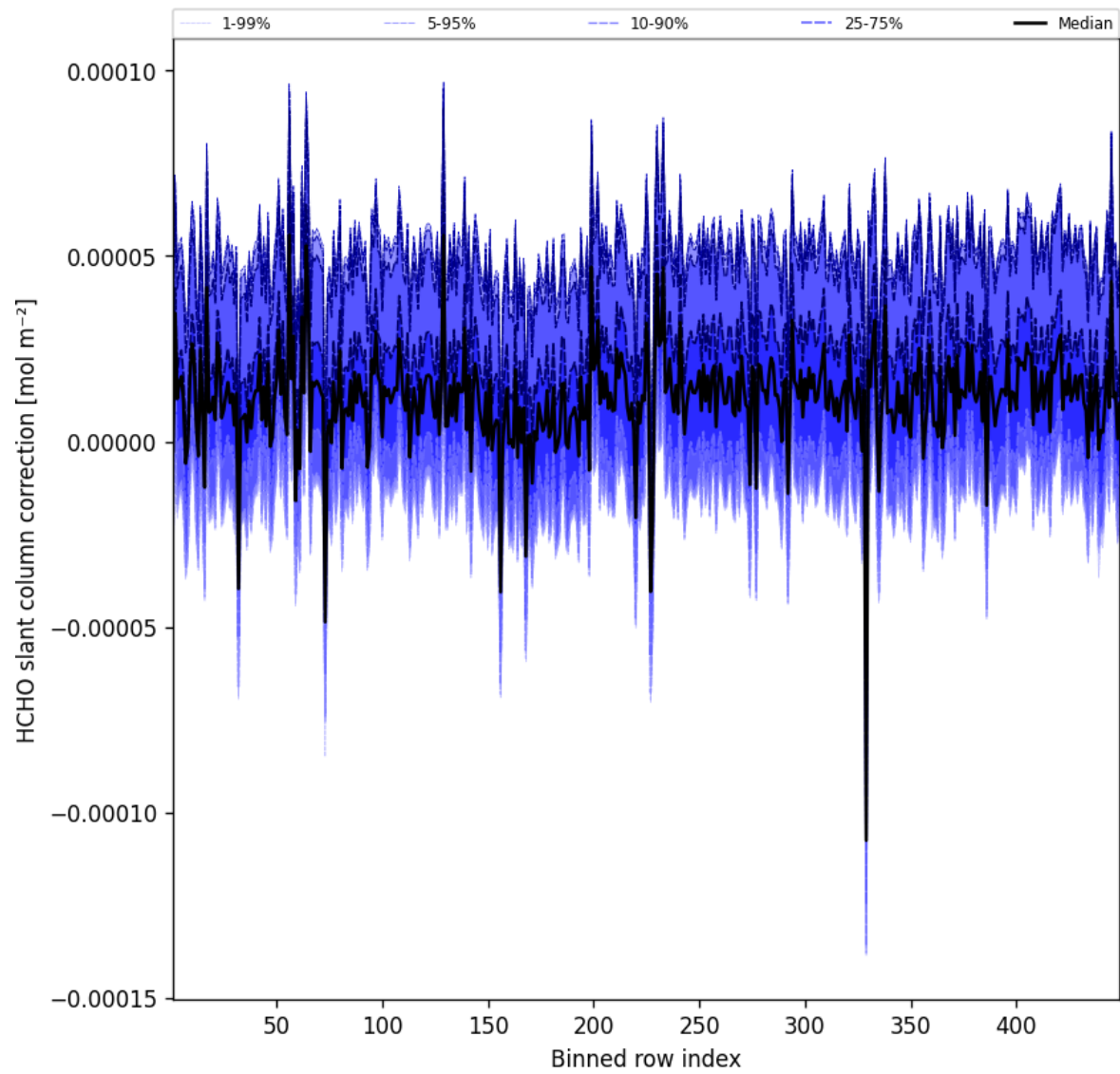
Figure 59: Along track statistics of “HCHO slant column correction” for 2025-09-27 to 2025-09-28
