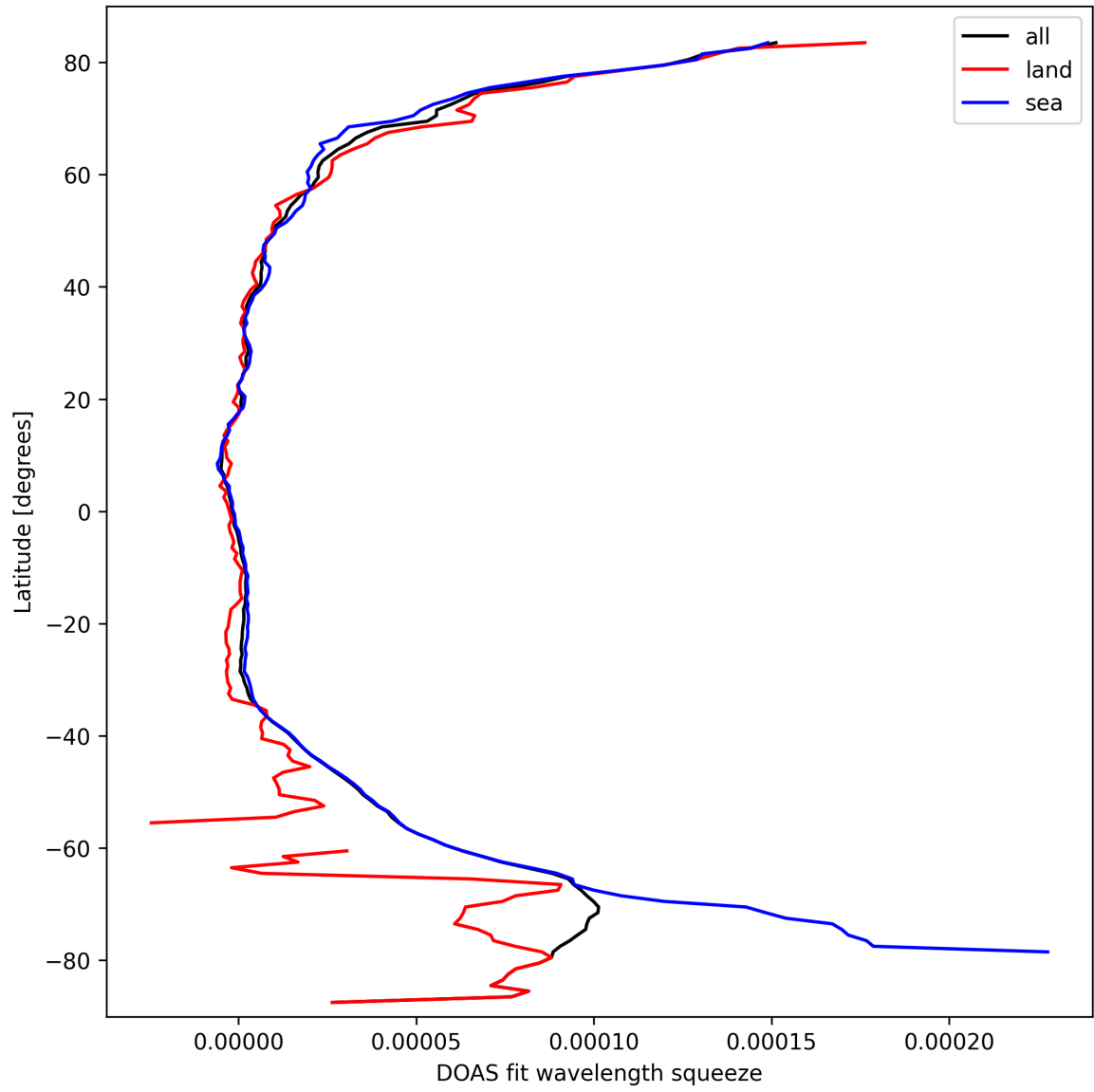
Figure 29: Zonal average of “DOAS fit wavelength squeeze” for 2025-09-27 to 2025-09-28.
