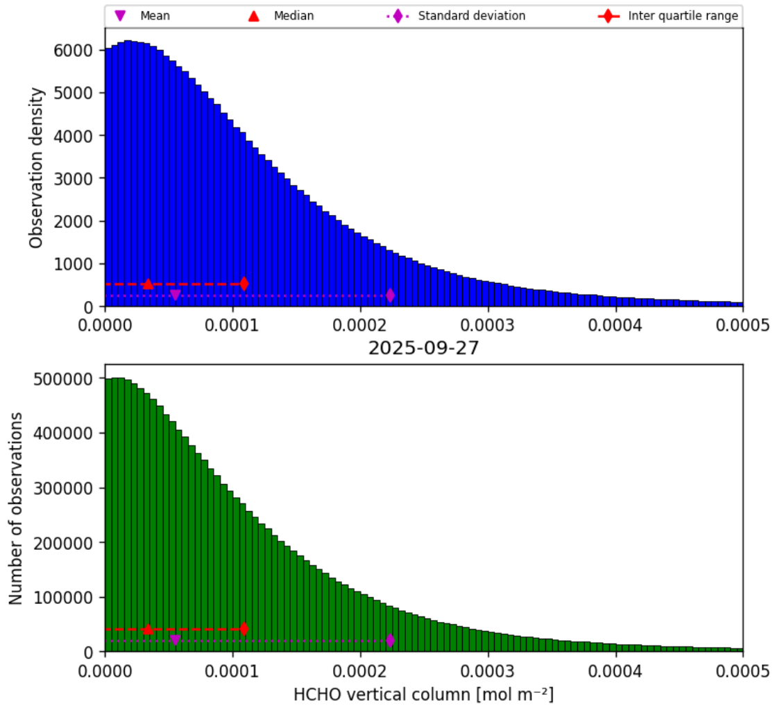
Figure 33: Histogram of “HCHO vertical column” for 2025-09-27 to 2025-09-28
