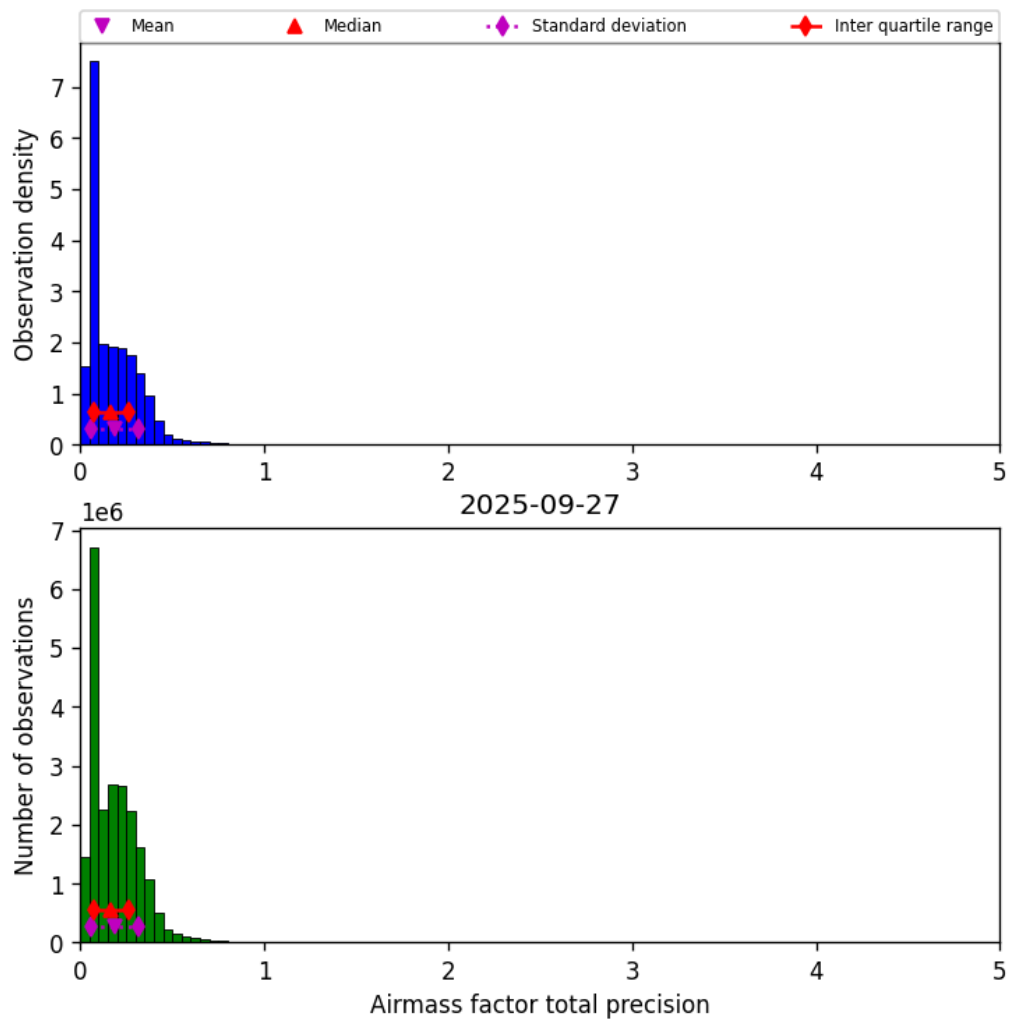
Figure 39: Histogram of “Airmass factor total precision” for 2025-09-27 to 2025-09-28
