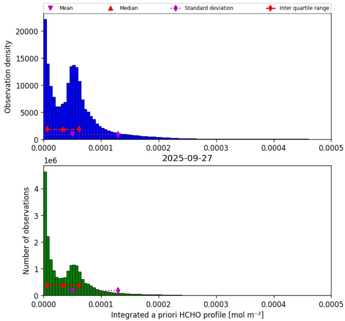
Figure 41: Histogram of “Integrated a priori HCHO profile” for 2025-09-27 to 2025-09-28
