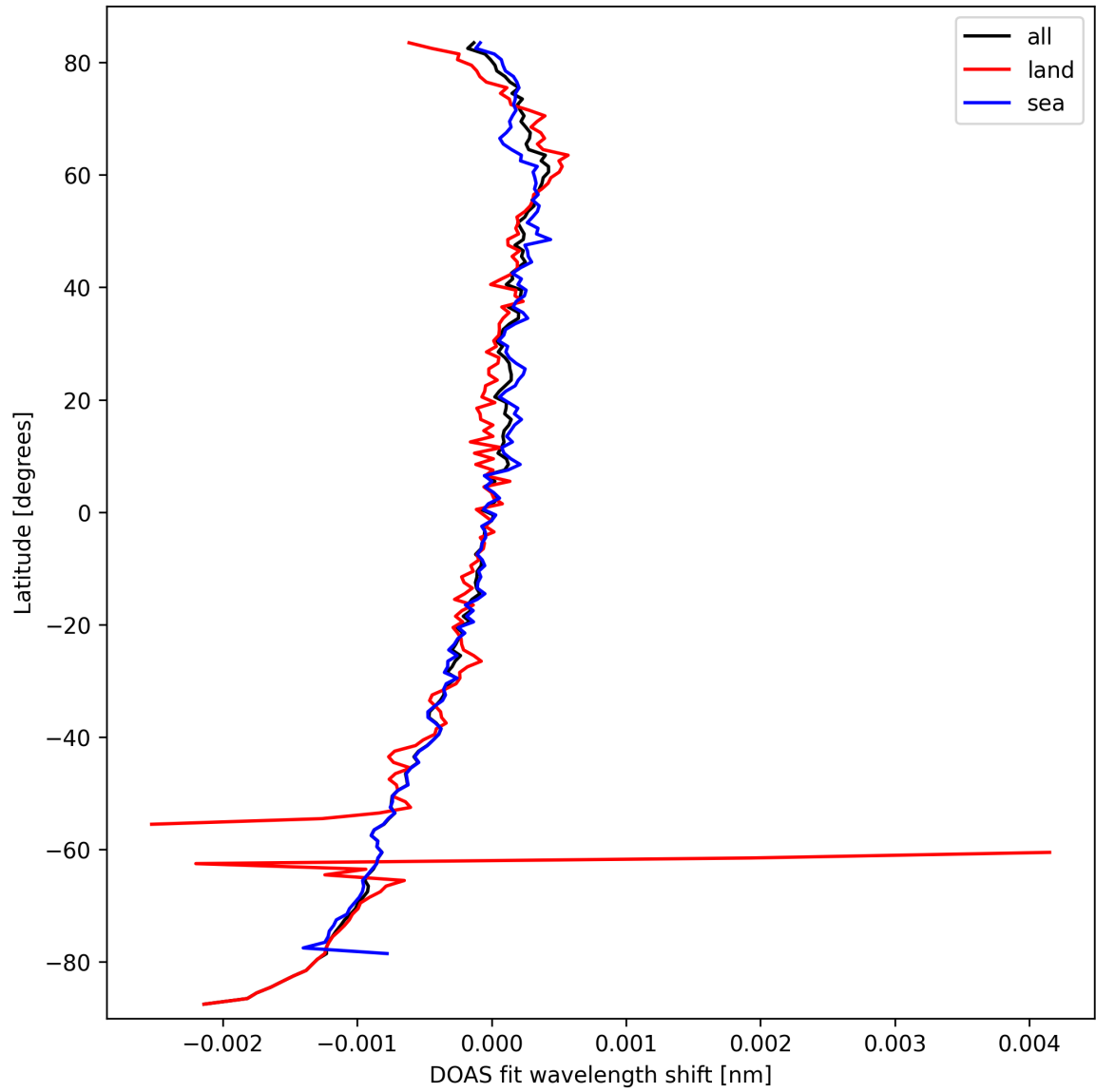
Figure 28: Zonal average of “DOAS fit wavelength shift” for 2025-09-27 to 2025-09-28.
