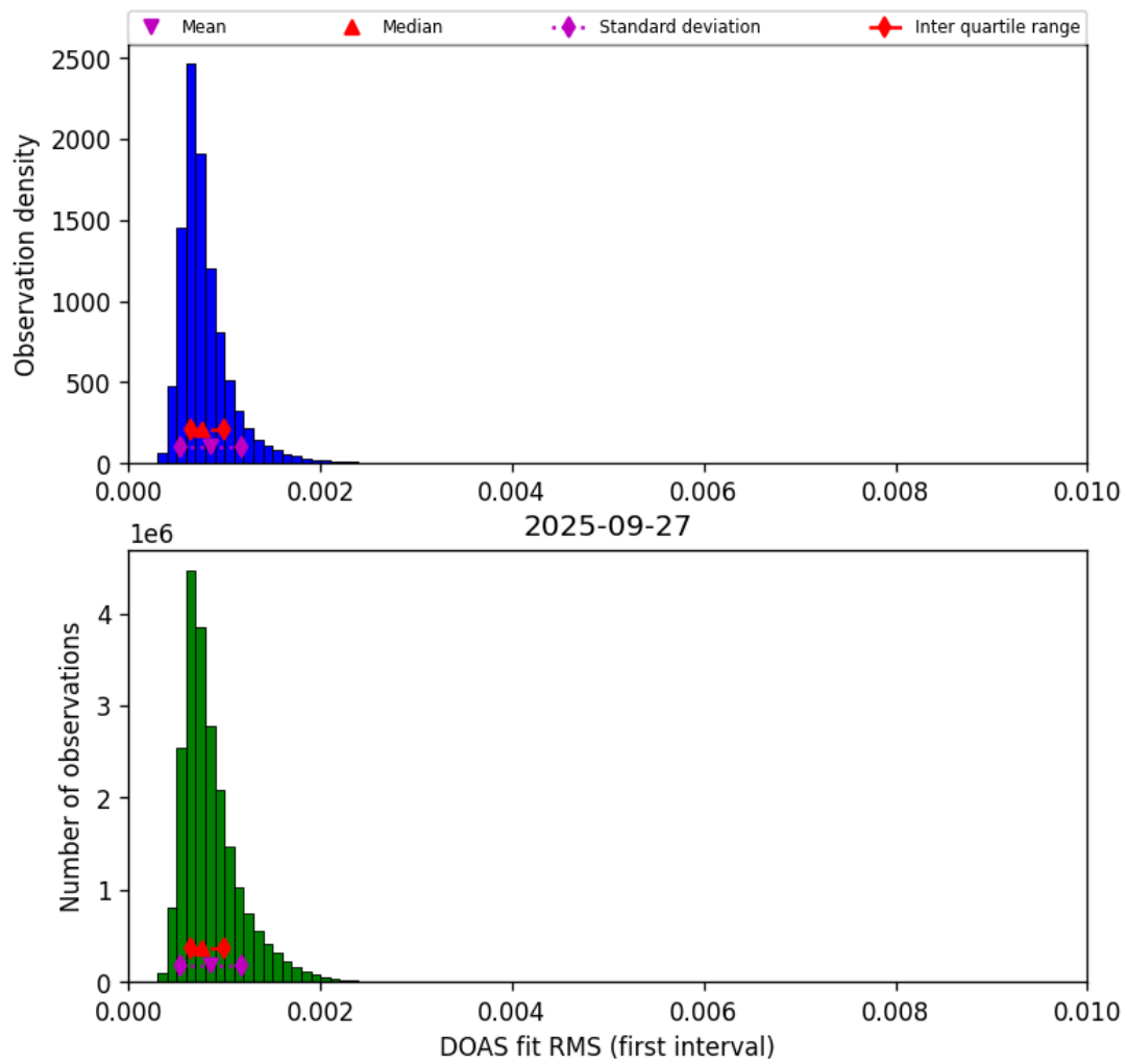
Figure 44: Histogram of “DOAS fit RMS (first interval)” for 2025-09-27 to 2025-09-28
