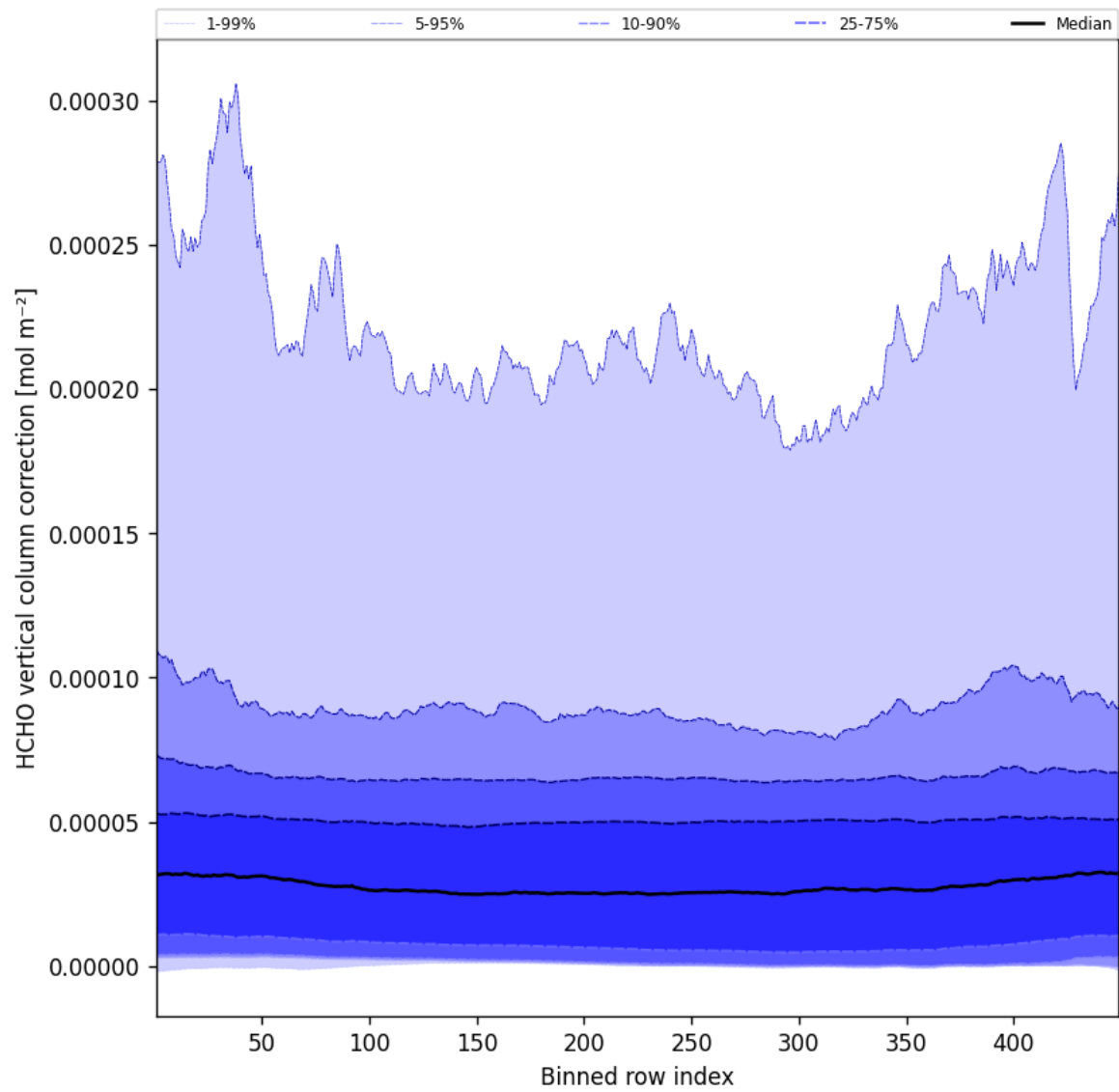
Figure 49: Along track statistics of “HCHO vertical column correction” for 2025-09-27 to 2025-09-28
