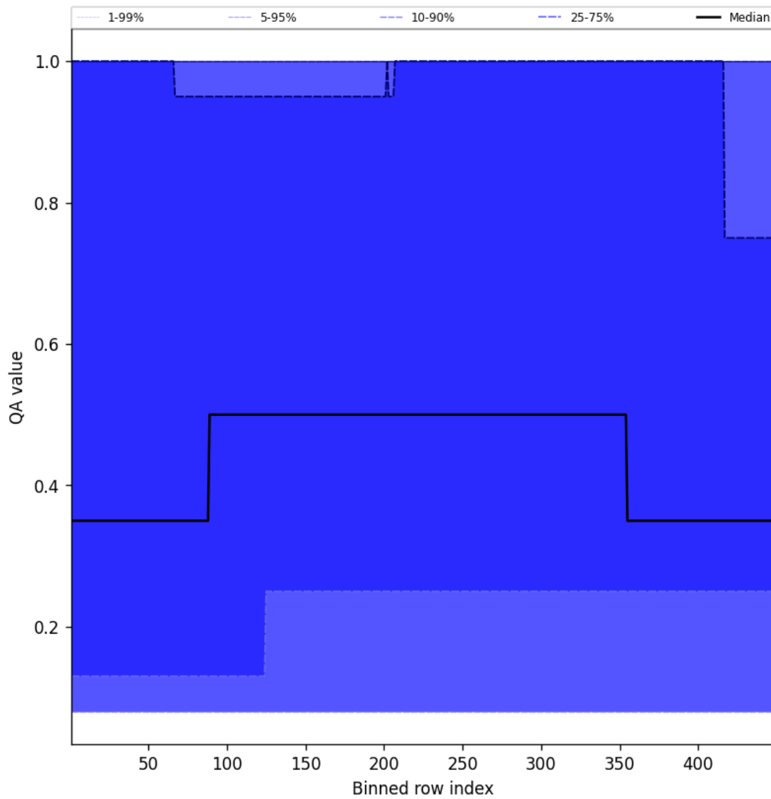
Figure 46: Along track statistics of “QA value” for 2025-09-27 to 2025-09-28
