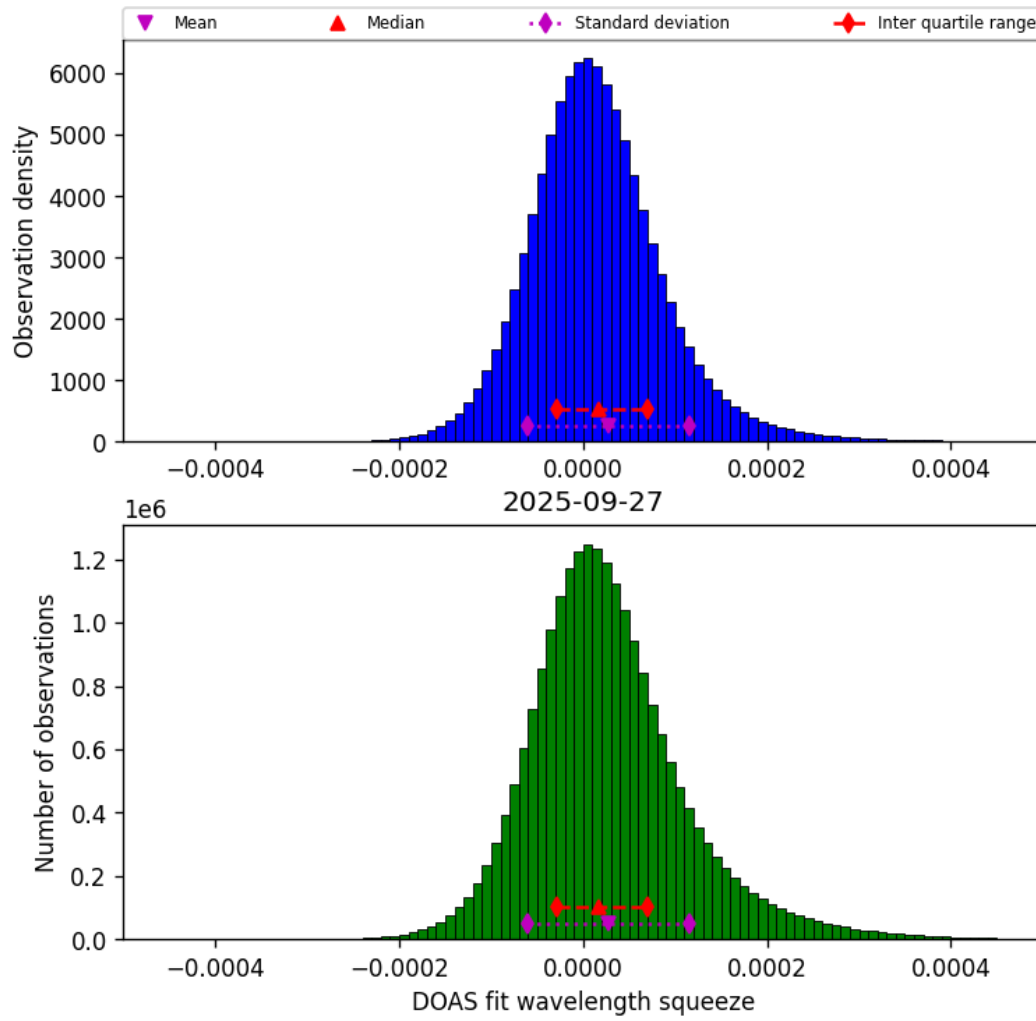
Figure 43: Histogram of “DOAS fit wavelength squeeze” for 2025-09-27 to 2025-09-28
