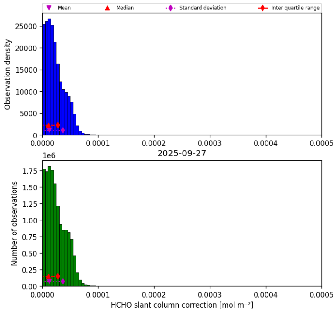
Figure 45: Histogram of “HCHO slant column correction” for 2025-09-27 to 2025-09-28
