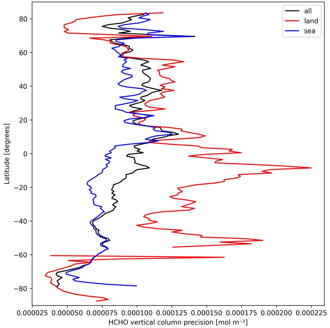
Figure 20: Zonal average of “HCHO vertical column precision” for 2025-09-27 to 2025-09-28.
