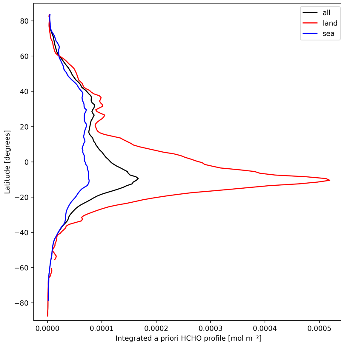
Figure 27: Zonal average of “Integrated a priori HCHO profile” for 2025-09-27 to 2025-09-28.
