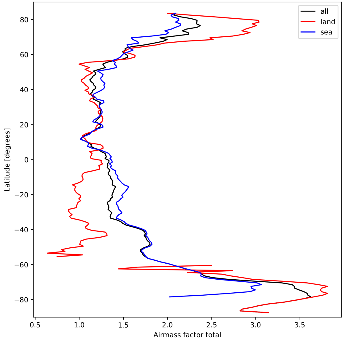
Figure 24: Zonal average of “Airmass factor total” for 2025-09-27 to 2025-09-28.
