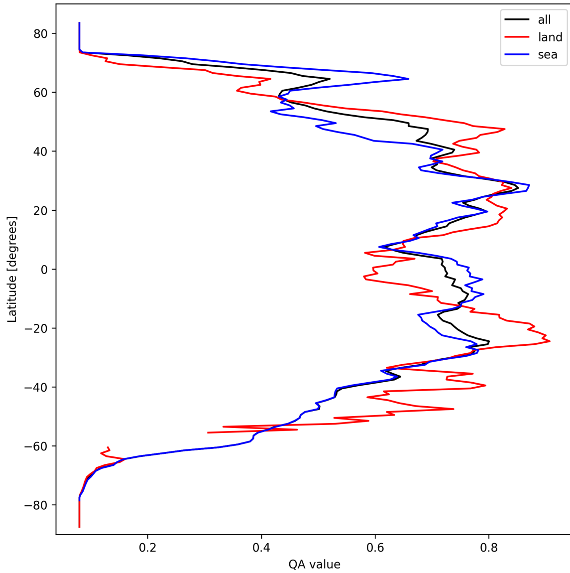
Figure 18: Zonal average of “QA value” for 2025-09-27 to 2025-09-28.
