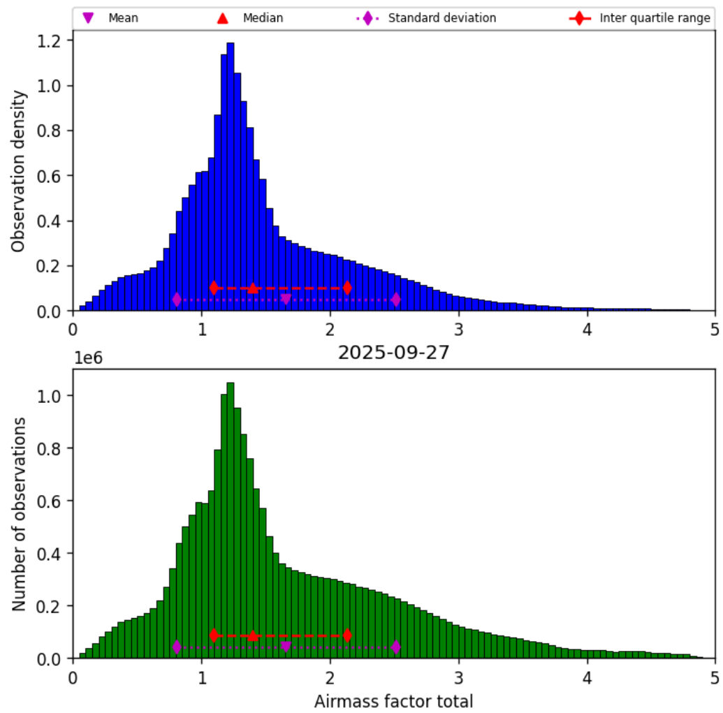
Figure 38: Histogram of “Airmass factor total” for 2025-09-27 to 2025-09-28
