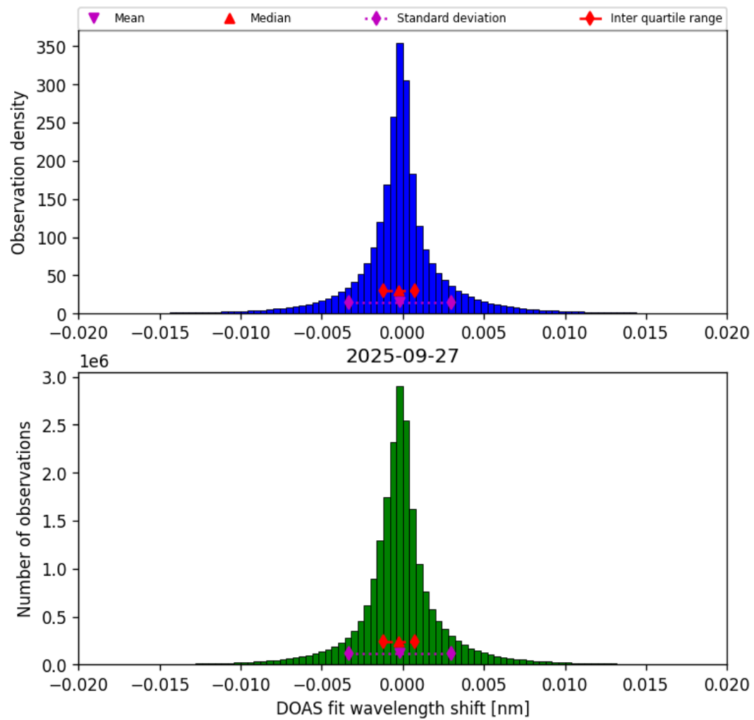
Figure 42: Histogram of “DOAS fit wavelength shift” for 2025-09-27 to 2025-09-28
