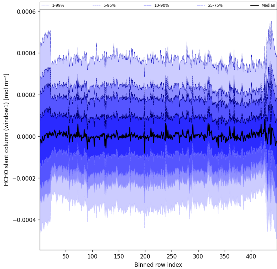
Figure 50: Along track statistics of “HCHO slant column (window1)” for 2025-09-27 to 2025-09-28
