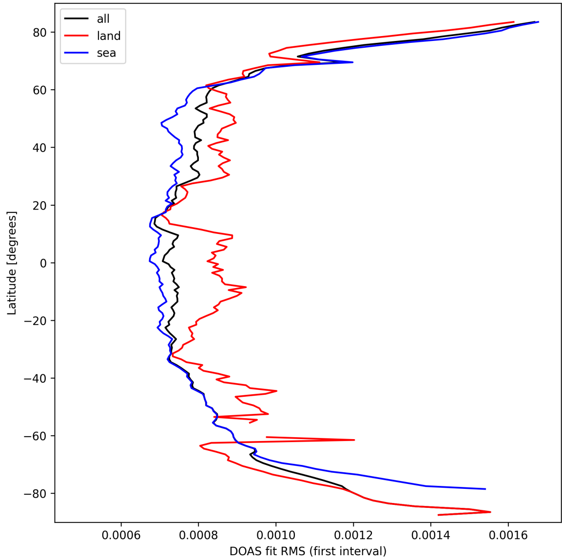
Figure 30: Zonal average of “DOAS fit RMS (first interval)” for 2025-09-27 to 2025-09-28.
