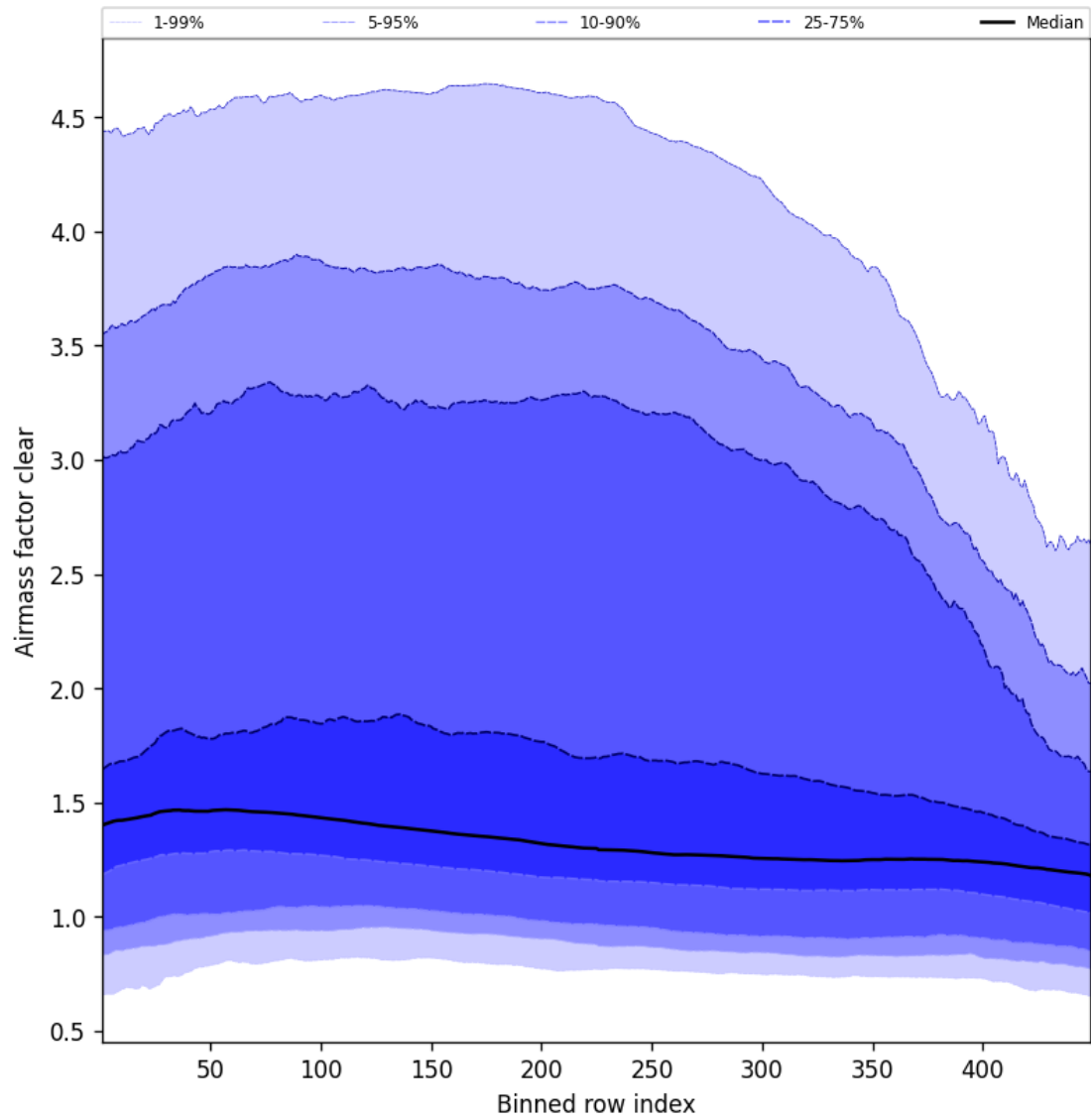
Figure 54: Along track statistics of “Air mass factor clear” for 2025-09-27 to 2025-09-28
