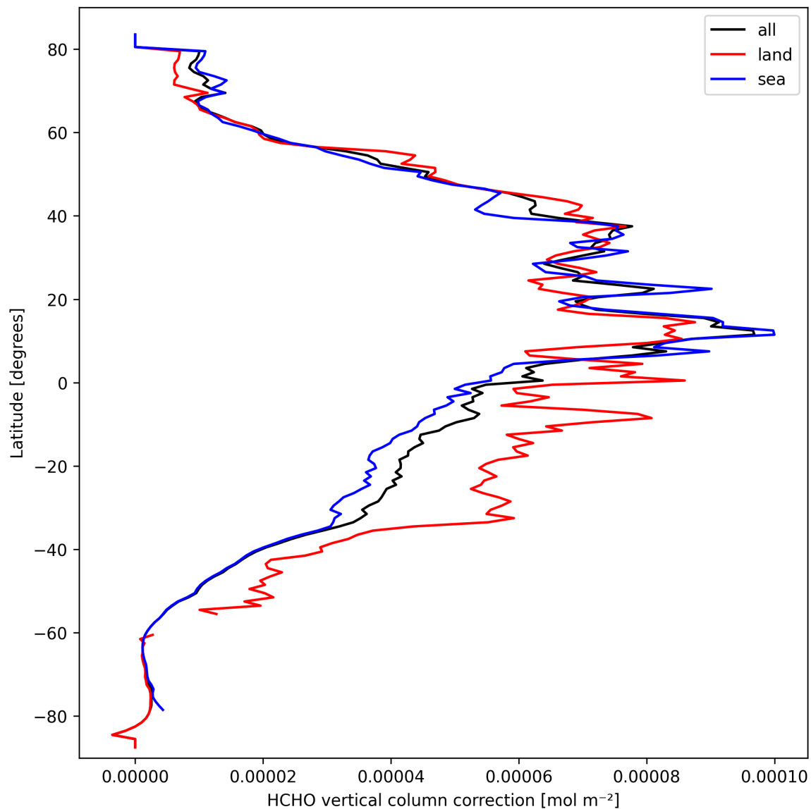
Figure 21: Zonal average of “HCHO vertical column correction” for 2025-09-27 to 2025-09-28.
