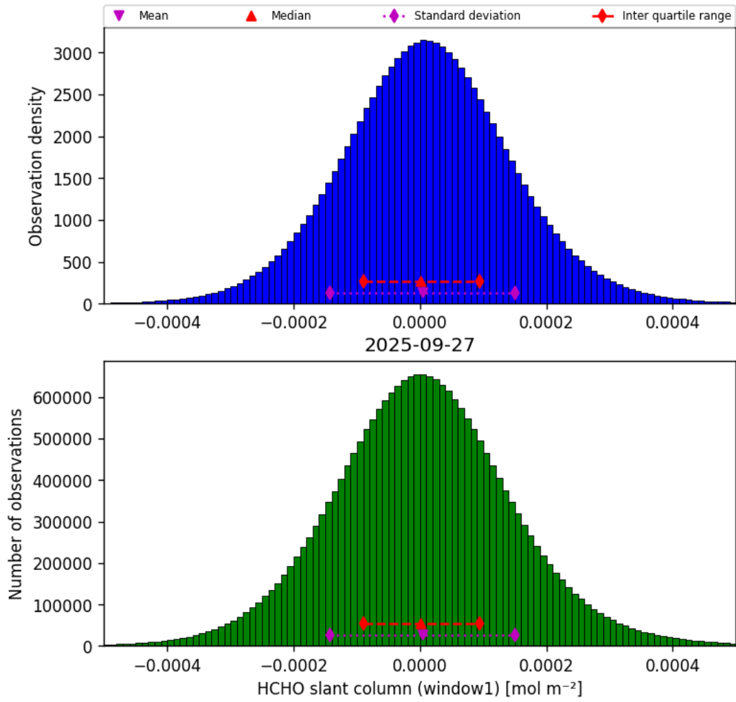
Figure 36: Histogram of “HCHO slant column (window1)” for 2025-09-27 to 2025-09-28
