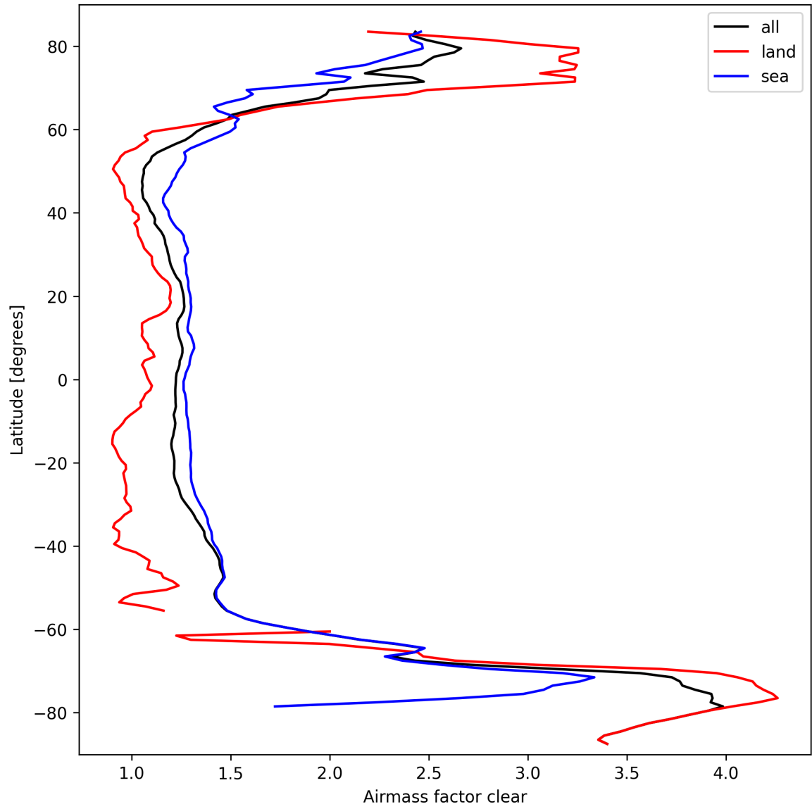
Figure 26: Zonal average of “Airmass factor clear” for 2025-09-27 to 2025-09-28.
