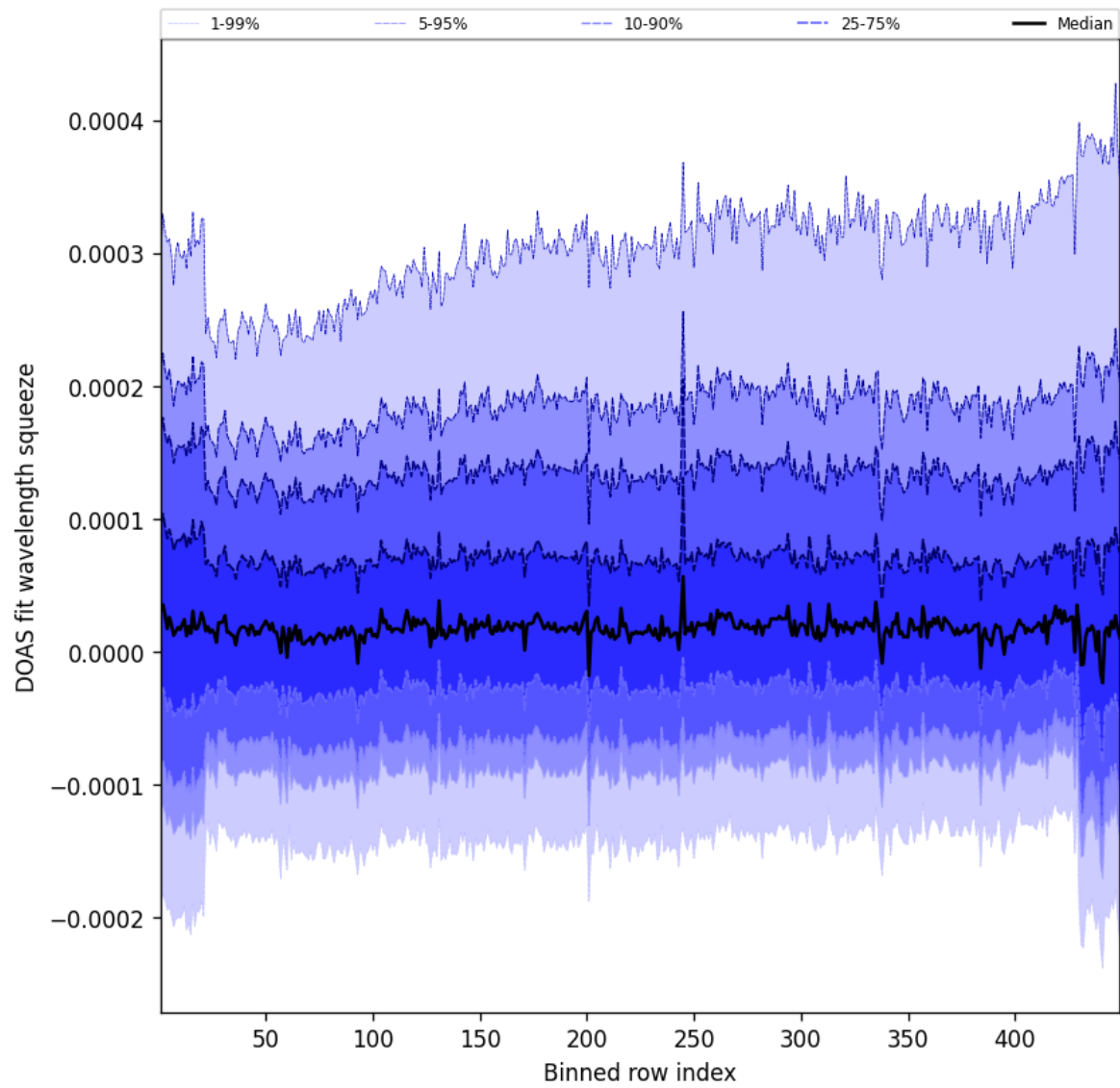
Figure 57: Along track statistics of “DOAS fit wavelength squeeze” for 2025-09-27 to 2025-09-28
