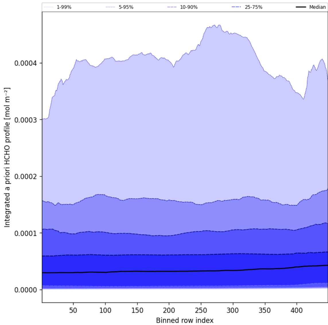
Figure 55: Along track statistics of “Integrated a priori HCHO profile” for 2025-09-27 to 2025-09-28
