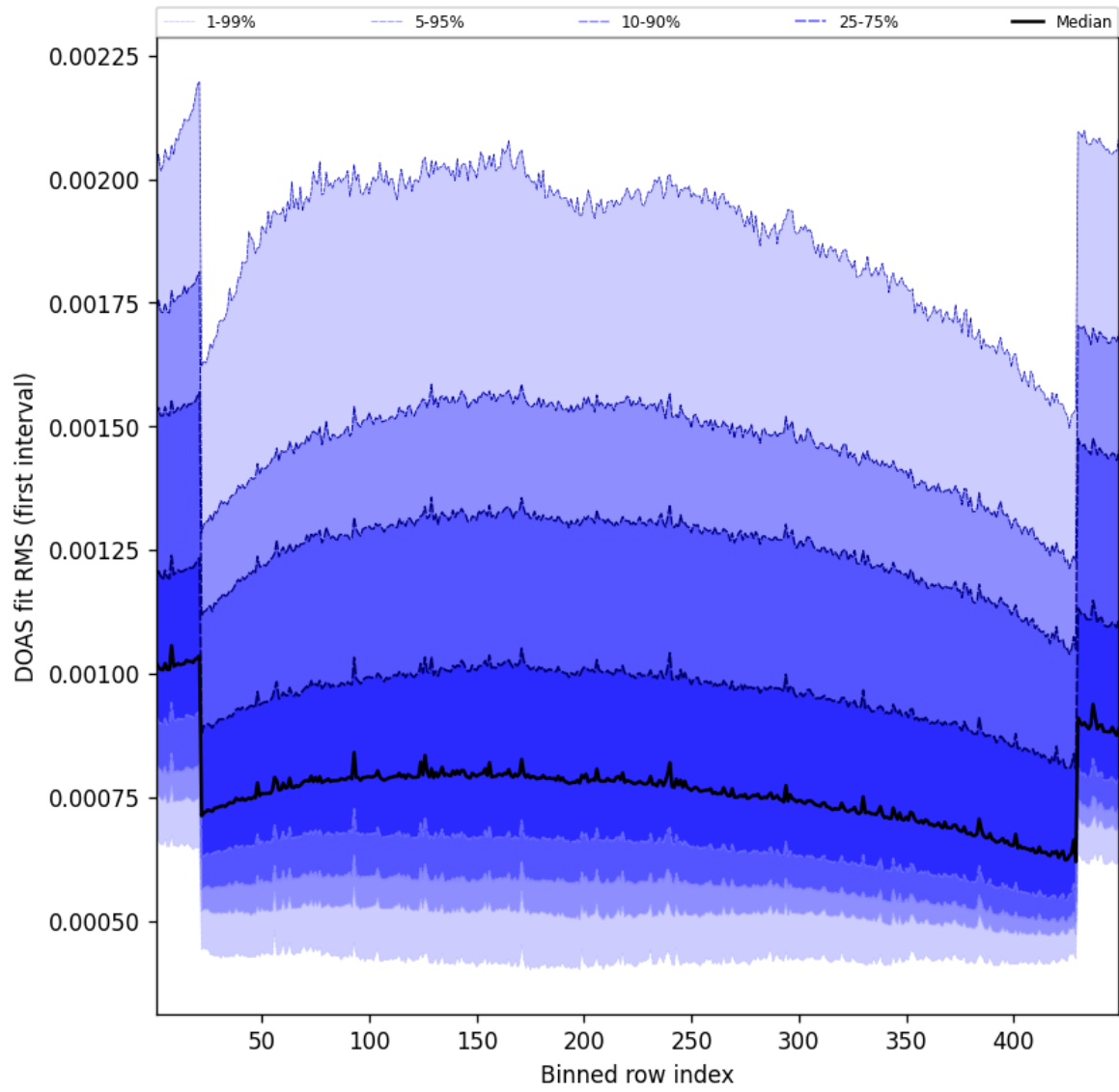
Figure 58: Along track statistics of “DOAS fit RMS (first interval)” for 2025-09-27 to 2025-09-28
