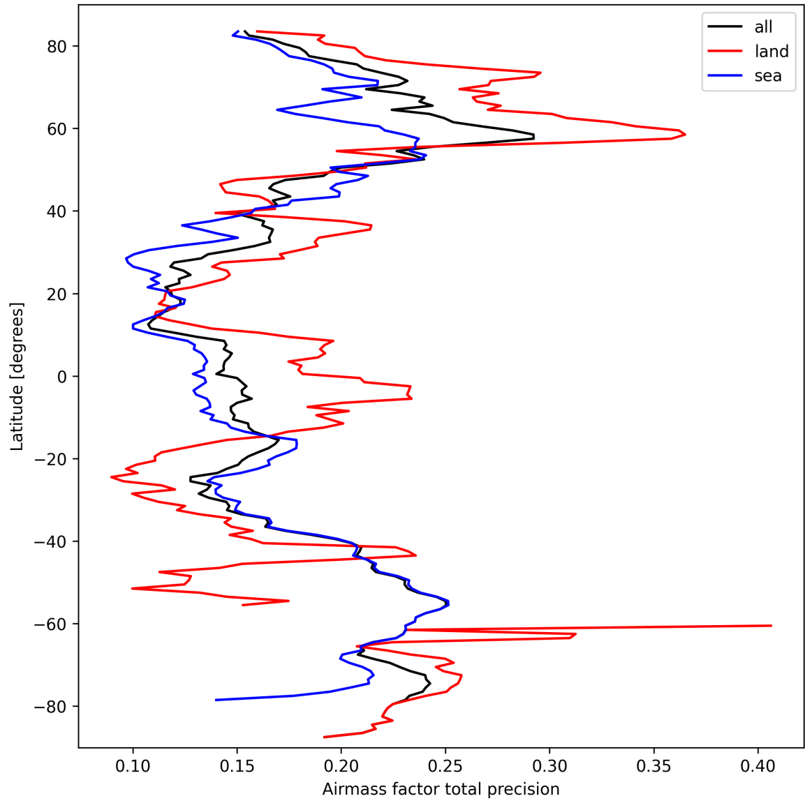
Figure 25: Zonal average of “Airmass factor total precision” for 2025-09-27 to 2025-09-28.
