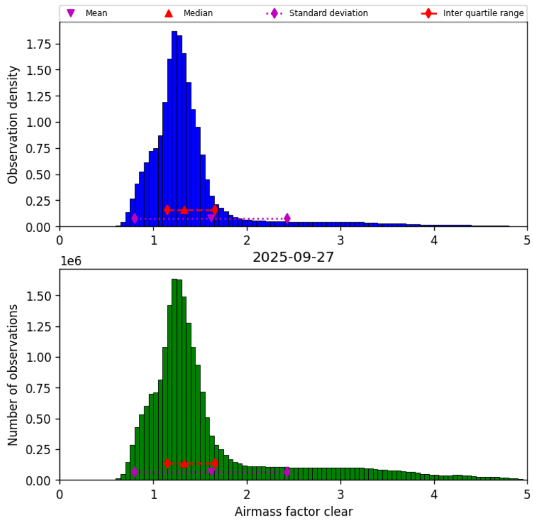
Figure 40: Histogram of “Airmass factor clear” for 2025-09-27 to 2025-09-28
