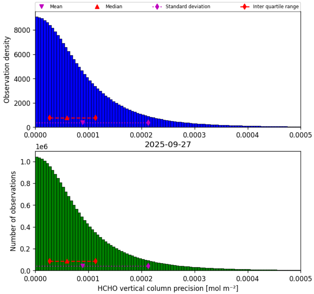
Figure 34: Histogram of “HCHO vertical column precision” for 2025-09-27 to 2025-09-28
