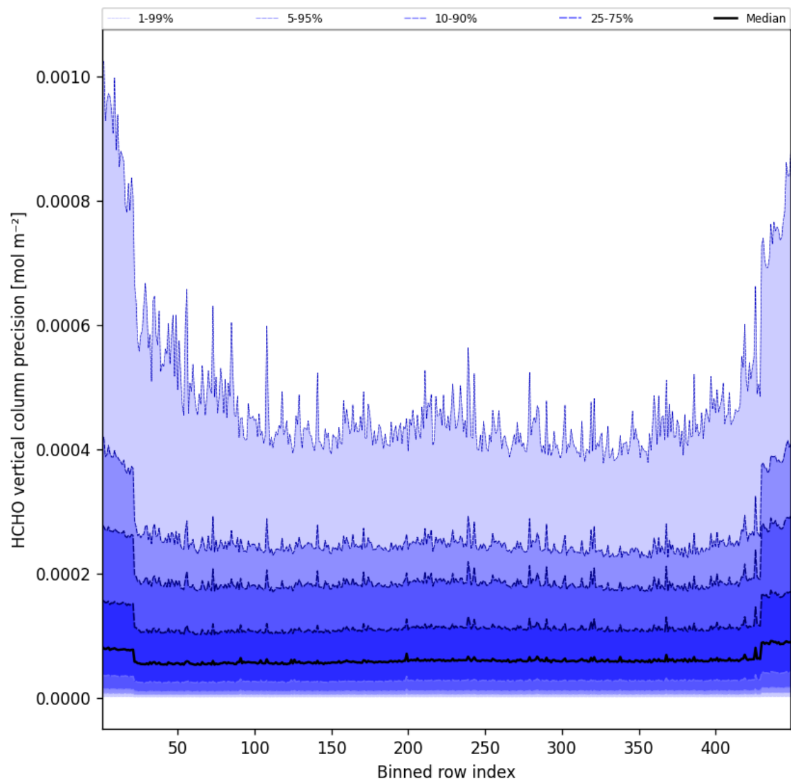
Figure 48: Along track statistics of “HCHO vertical column precision” for 2025-09-27 to 2025-09-28
