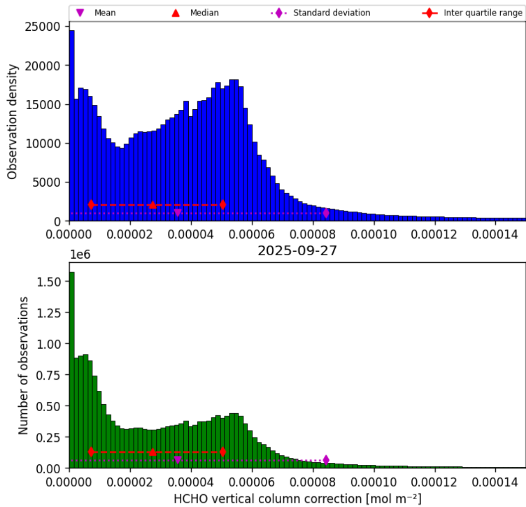
Figure 35: Histogram of “HCHO vertical column correction” for 2025-09-27 to 2025-09-28
