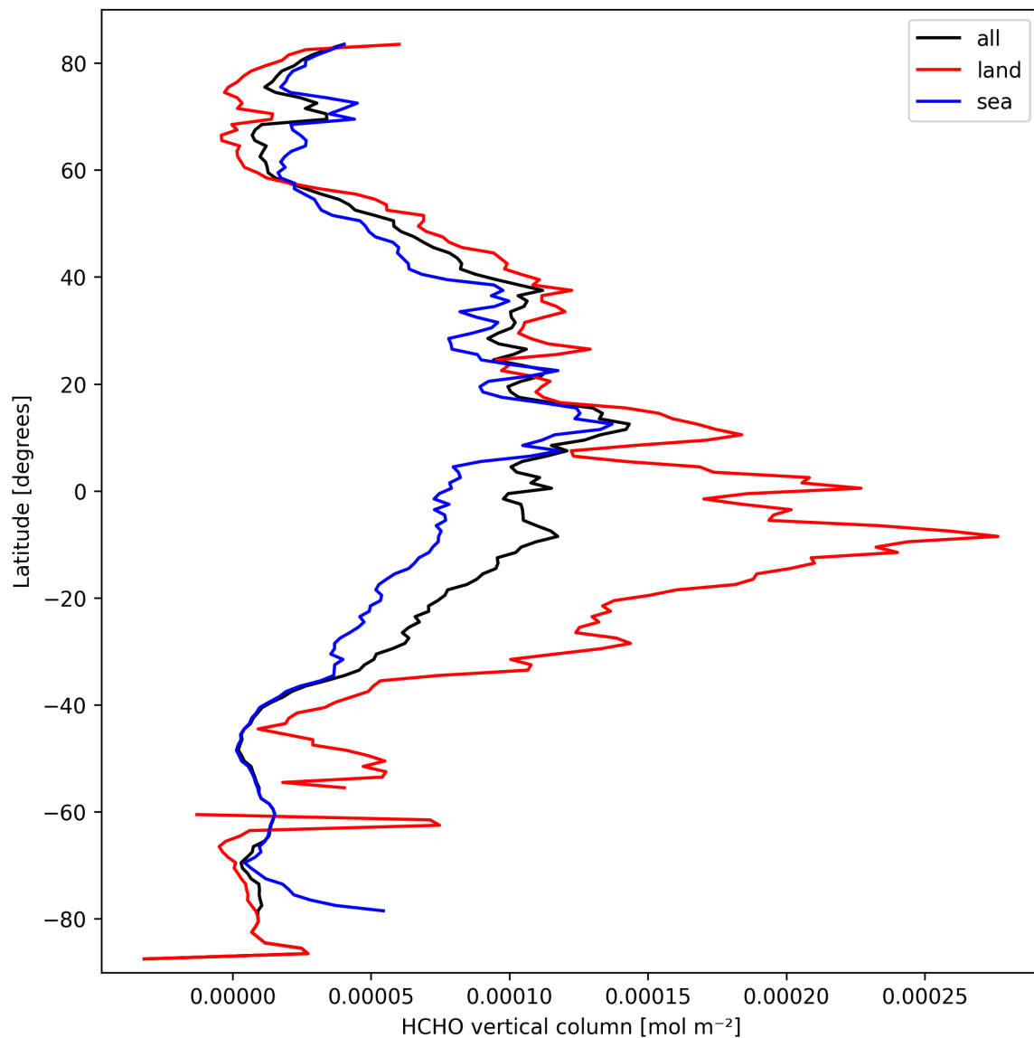
Figure 19: Zonal average of “HCHO vertical column” for 2025-09-27 to 2025-09-28.
