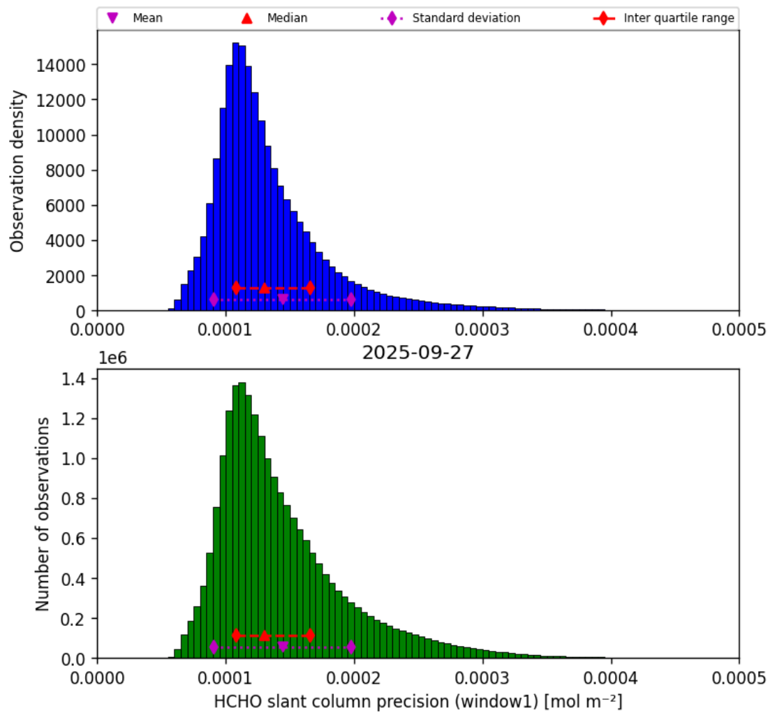
Figure 37: Histogram of “HCHO slant column precision (window1)” for 2025-09-27 to 2025-09-28
