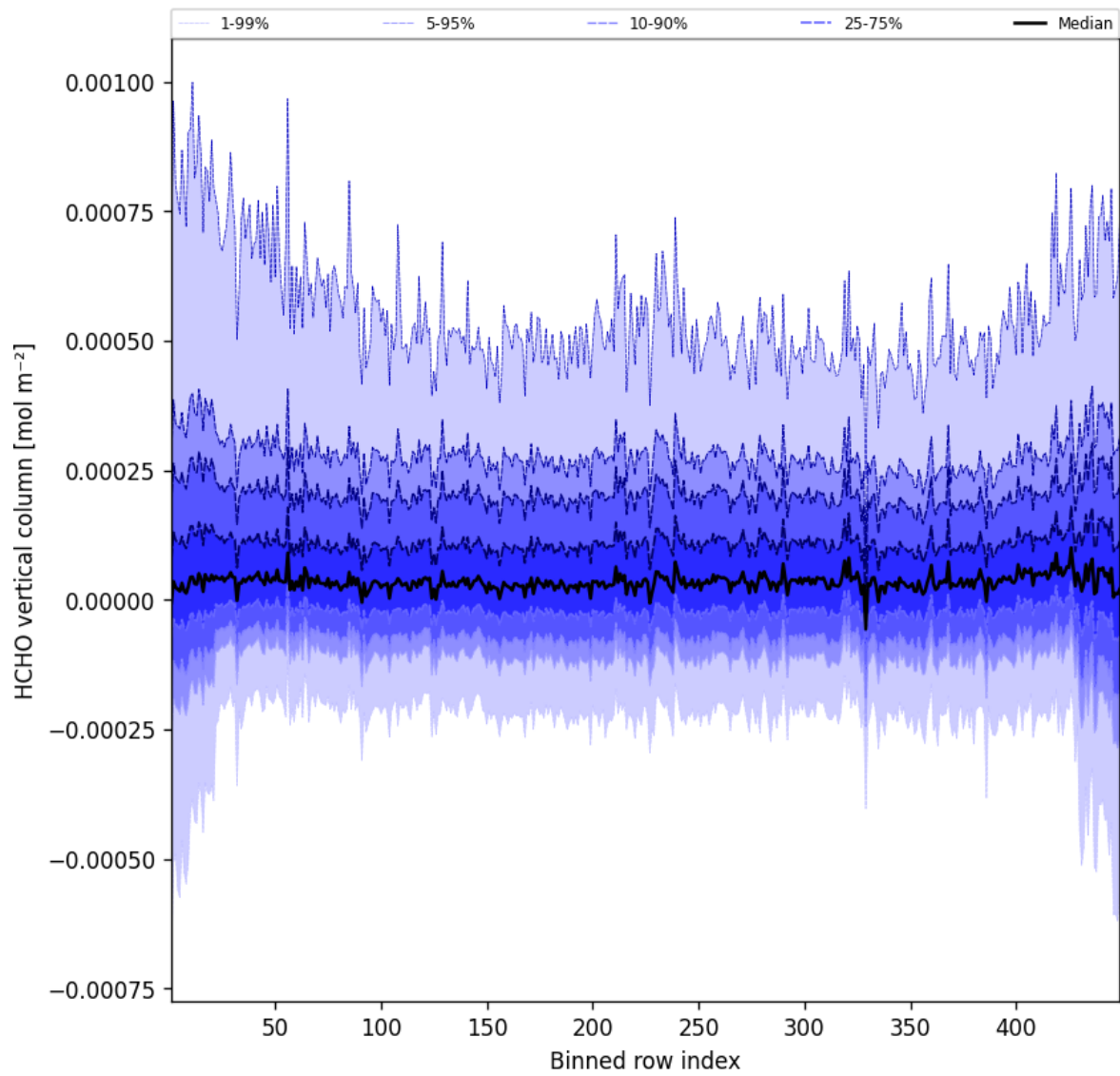
Figure 47: Along track statistics of “HCHO vertical column” for 2025-09-27 to 2025-09-28
