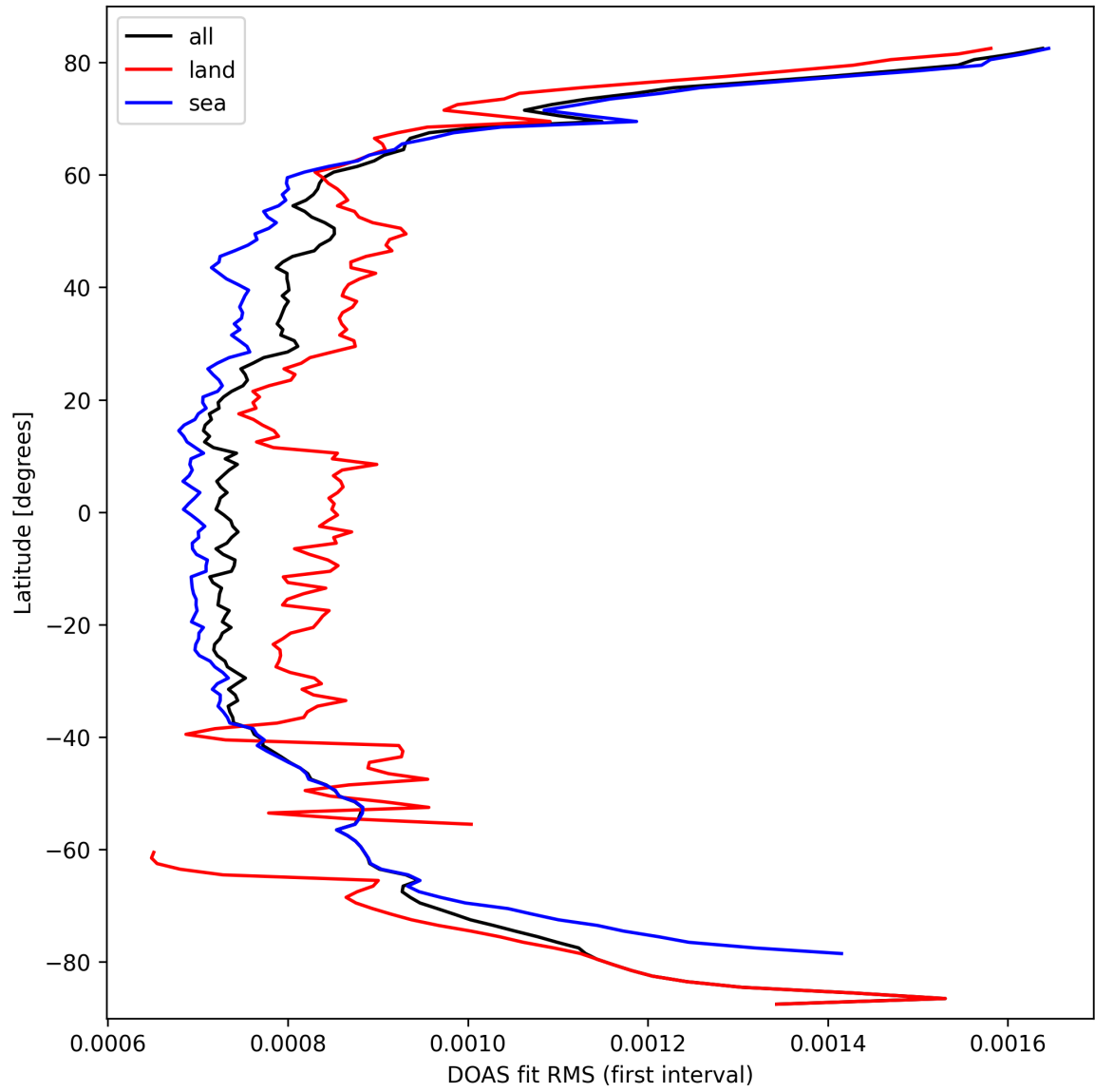
Figure 30: Zonal average of “DOAS fit RMS (first interval)” for 2025-09-28 to 2025-09-29.
