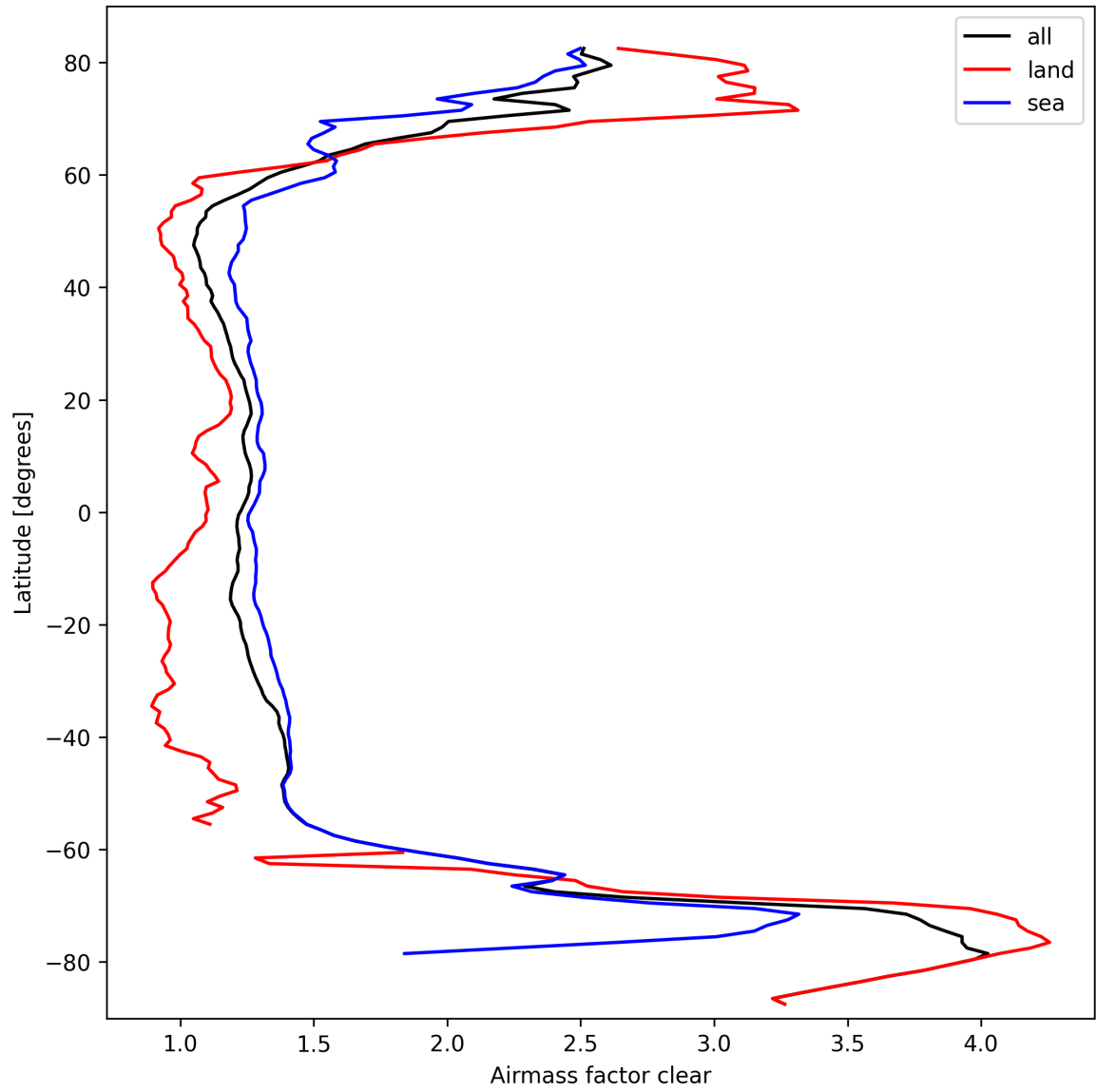
Figure 26: Zonal average of “Airmass factor clear” for 2025-09-28 to 2025-09-29.
