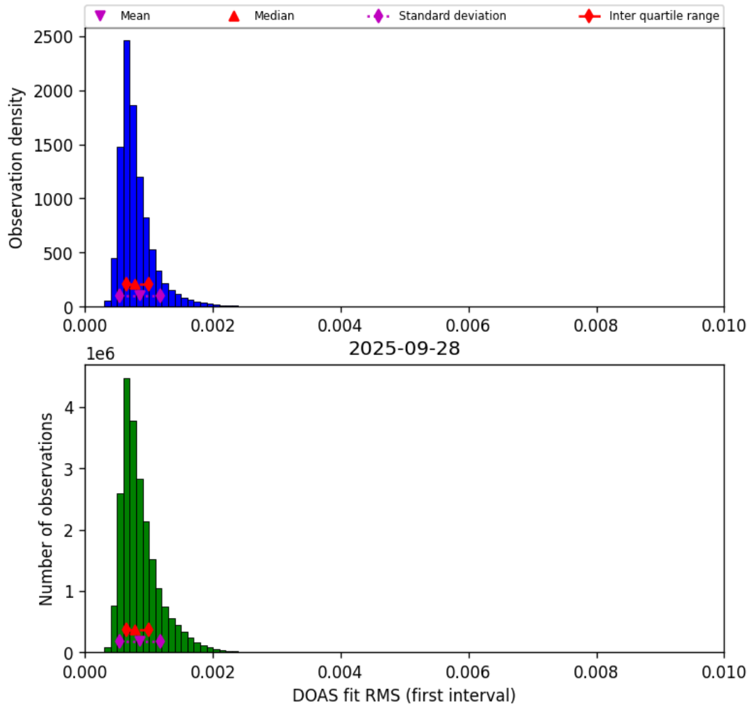
Figure 44: Histogram of “DOAS fit RMS (first interval)” for 2025-09-28 to 2025-09-29
