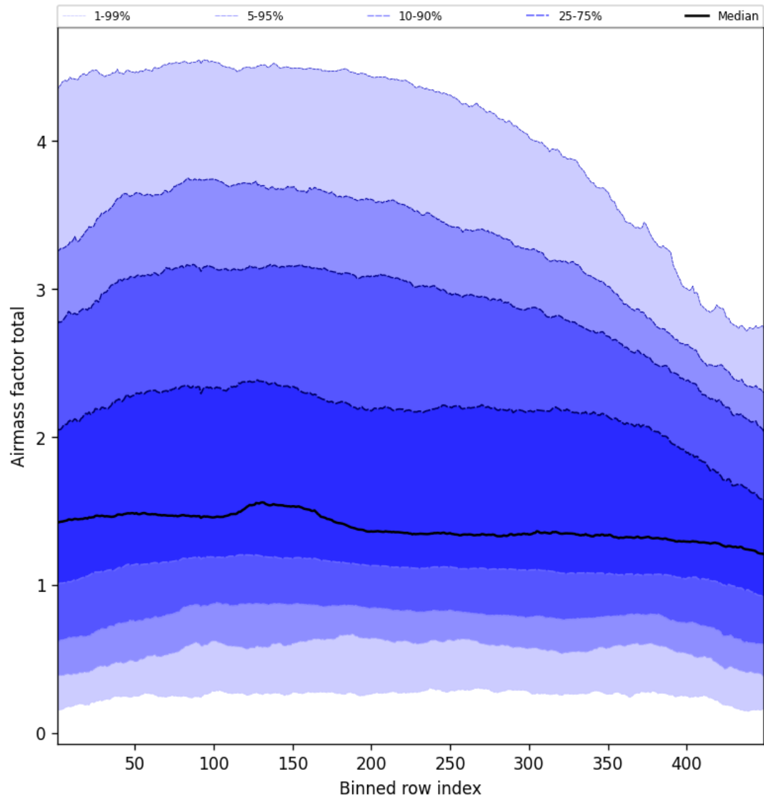
Figure 52: Along track statistics of “Airmass factor total” for 2025-09-28 to 2025-09-29
