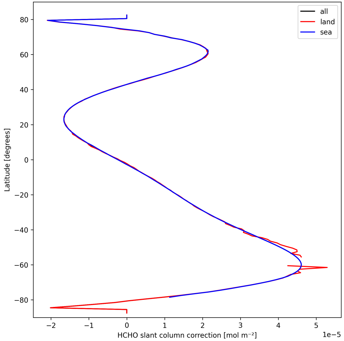
Figure 31: Zonal average of "HCHO slant column correction" for 2025-09-28 to 2025-09-29.
