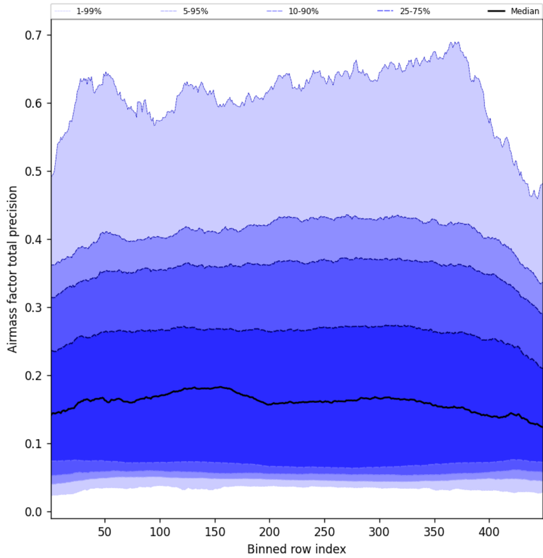
Figure 53: Along track statistics of “Airmass factor total precision” for 2025-09-28 to 2025-09-29
