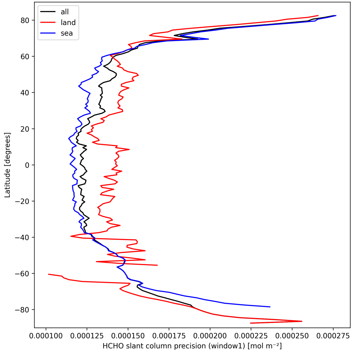
Figure 23: Zonal average of “HCHO slant column precision (window1)” for 2025-09-28 to 2025-09-29.
