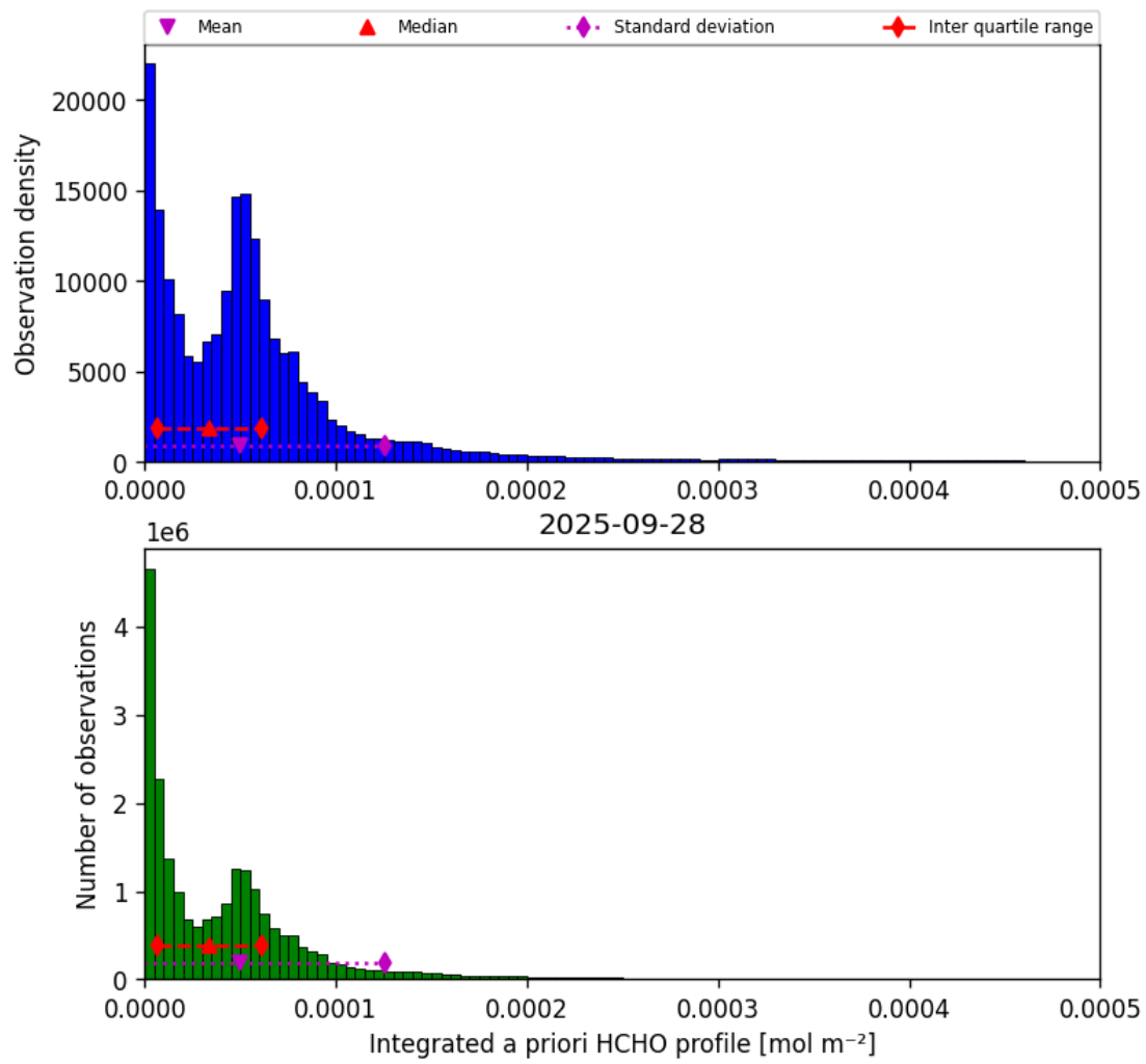
Figure 41: Histogram of “Integrated a priori HCHO profile” for 2025-09-28 to 2025-09-29
