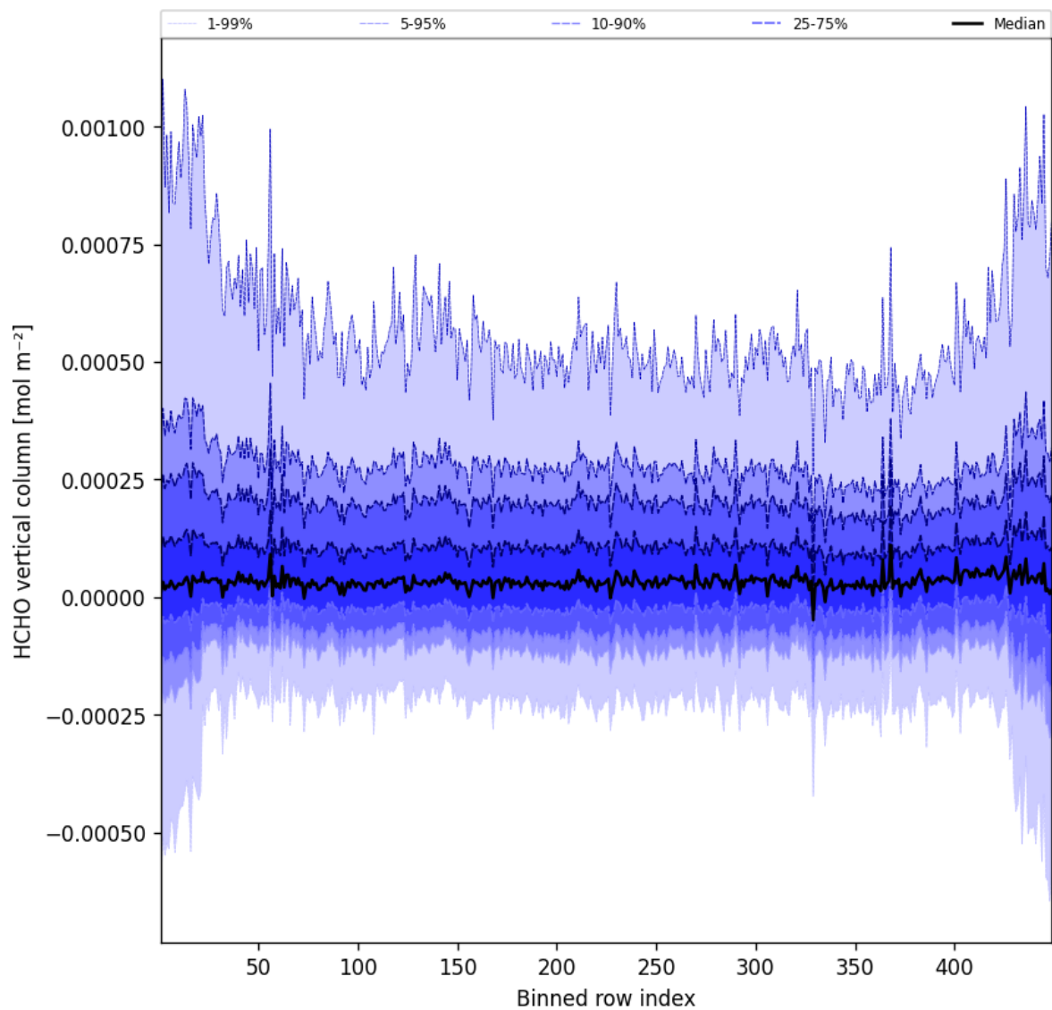
Figure 47: Along track statistics of “HCHO vertical column” for 2025-09-28 to 2025-09-29
