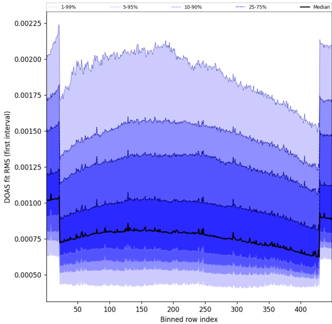
Figure 58: Along track statistics of “DOAS fit RMS (first interval)” for 2025-09-28 to 2025-09-29
