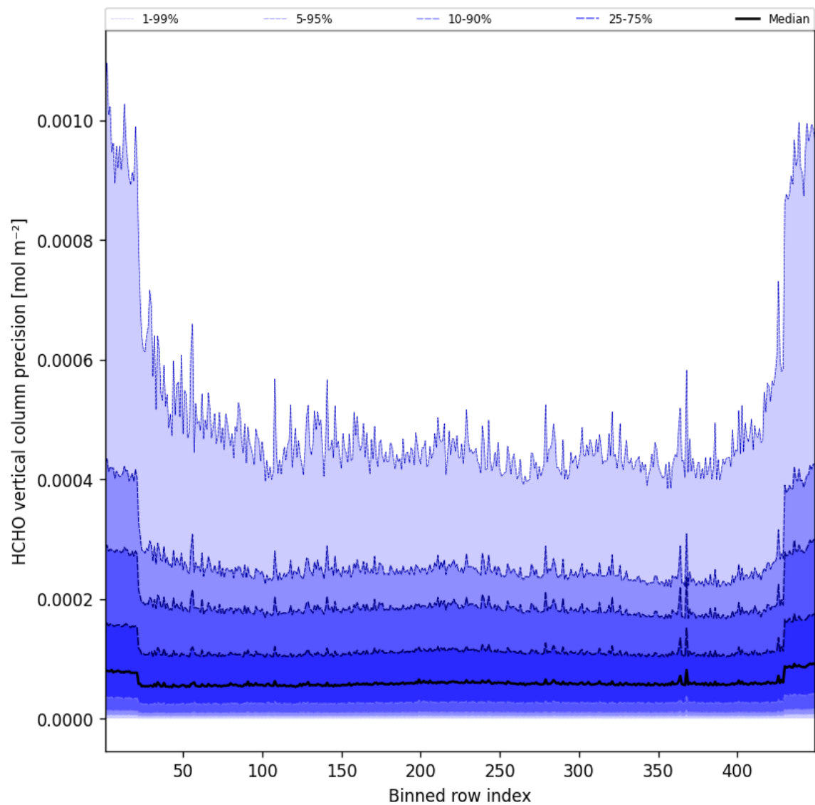
Figure 48: Along track statistics of “HCHO vertical column precision” for 2025-09-28 to 2025-09-29
