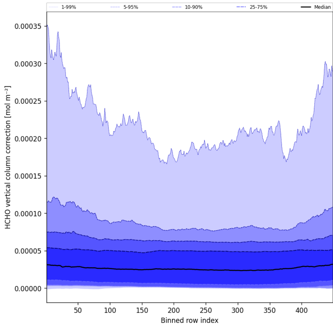
Figure 49: Along track statistics of “HCHO vertical column correction” for 2025-09-28 to 2025-09-29
