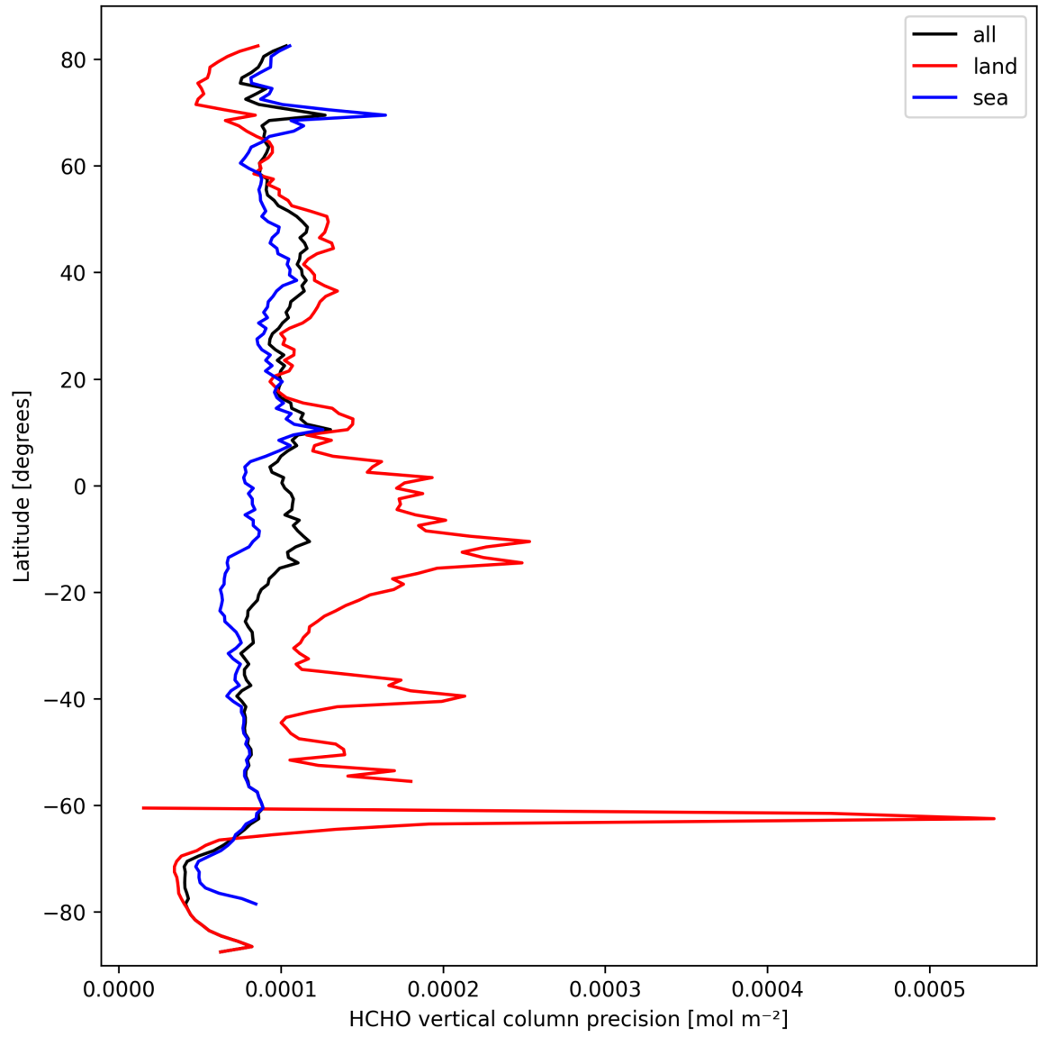
Figure 20: Zonal average of “HCHO vertical column precision” for 2025-09-28 to 2025-09-29.
