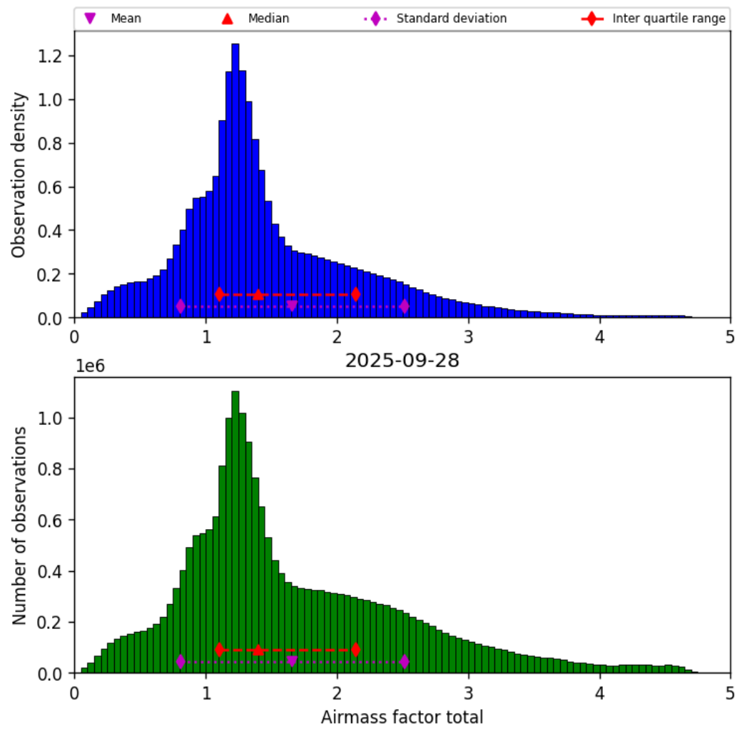
Figure 38: Histogram of “Airmass factor total” for 2025-09-28 to 2025-09-29
