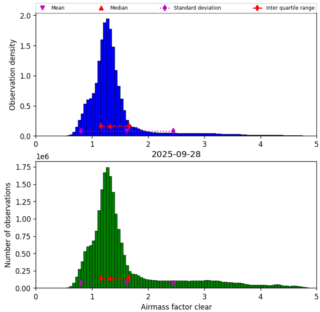
Figure 40: Histogram of “Airmass factor clear” for 2025-09-28 to 2025-09-29
