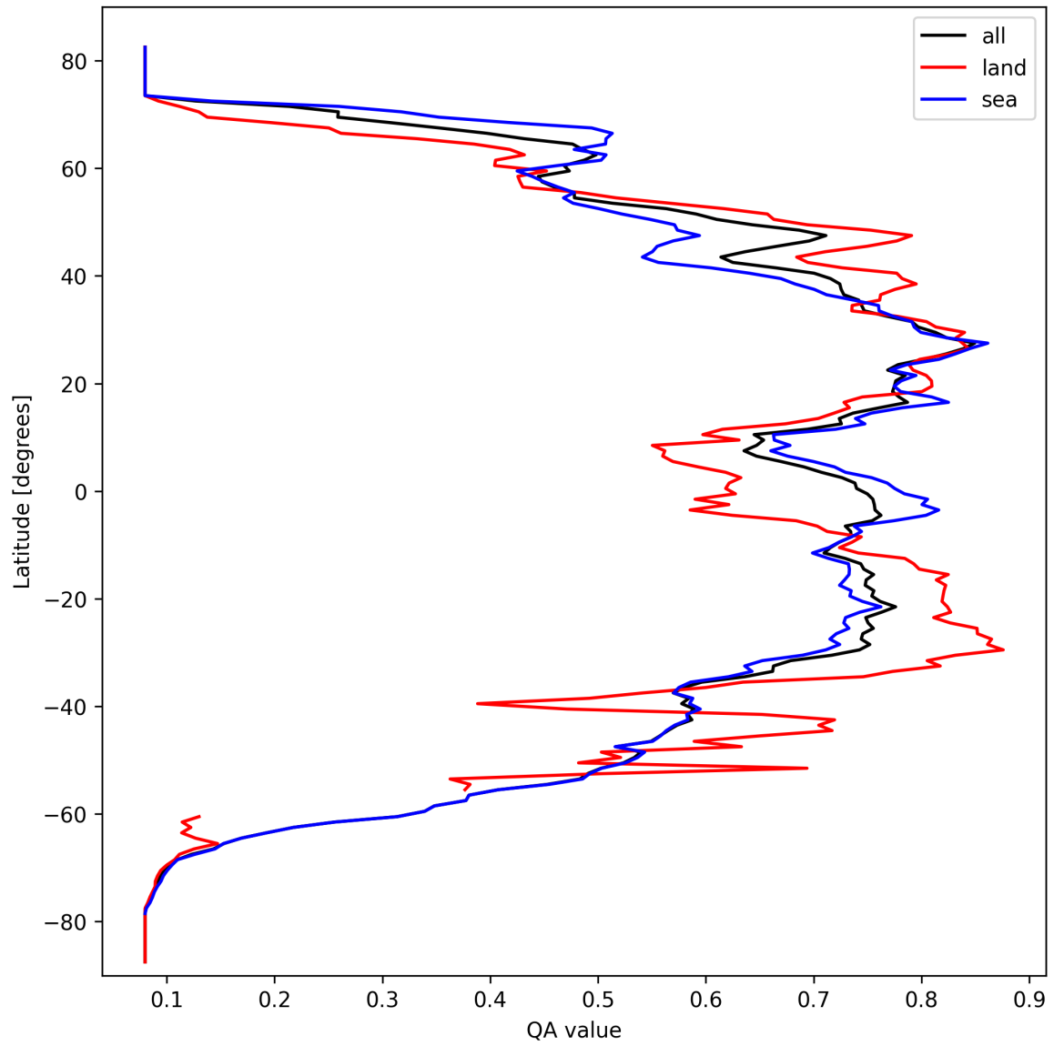
Figure 18: Zonal average of “QA value” for 2025-09-28 to 2025-09-29.
