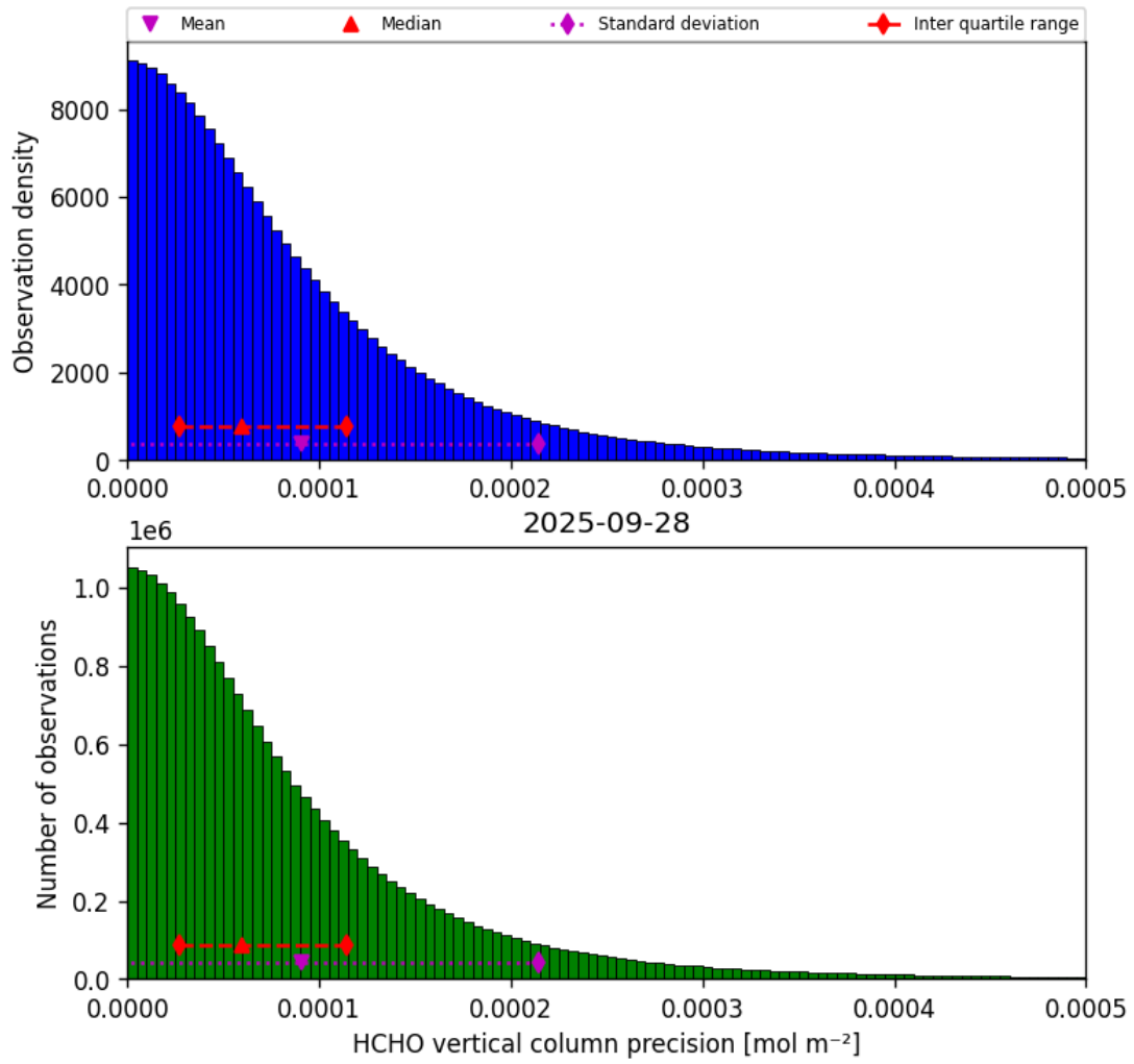
Figure 34: Histogram of “HCHO vertical column precision” for 2025-09-28 to 2025-09-29
