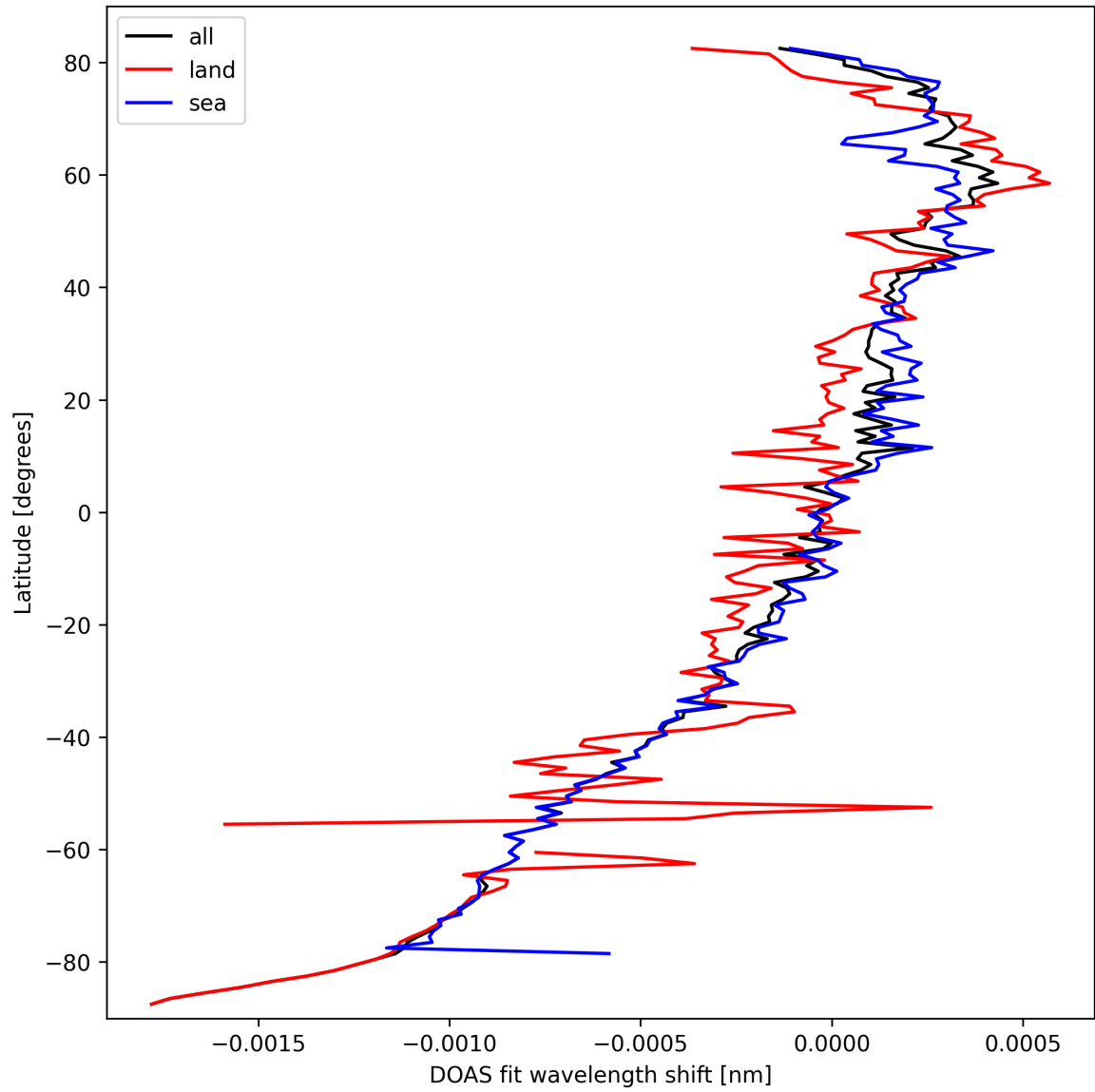
Figure 28: Zonal average of "DOAS fit wavelength shift" for 2025-09-28 to 2025-09-29.
