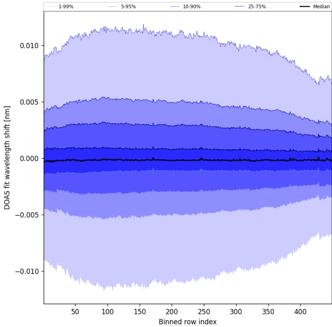
Figure 56: Along track statistics of “DOAS fit wavelength shift” for 2025-09-28 to 2025-09-29
