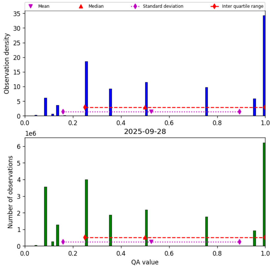
Figure 32: Histogram of “QA value” for 2025-09-28 to 2025-09-29
