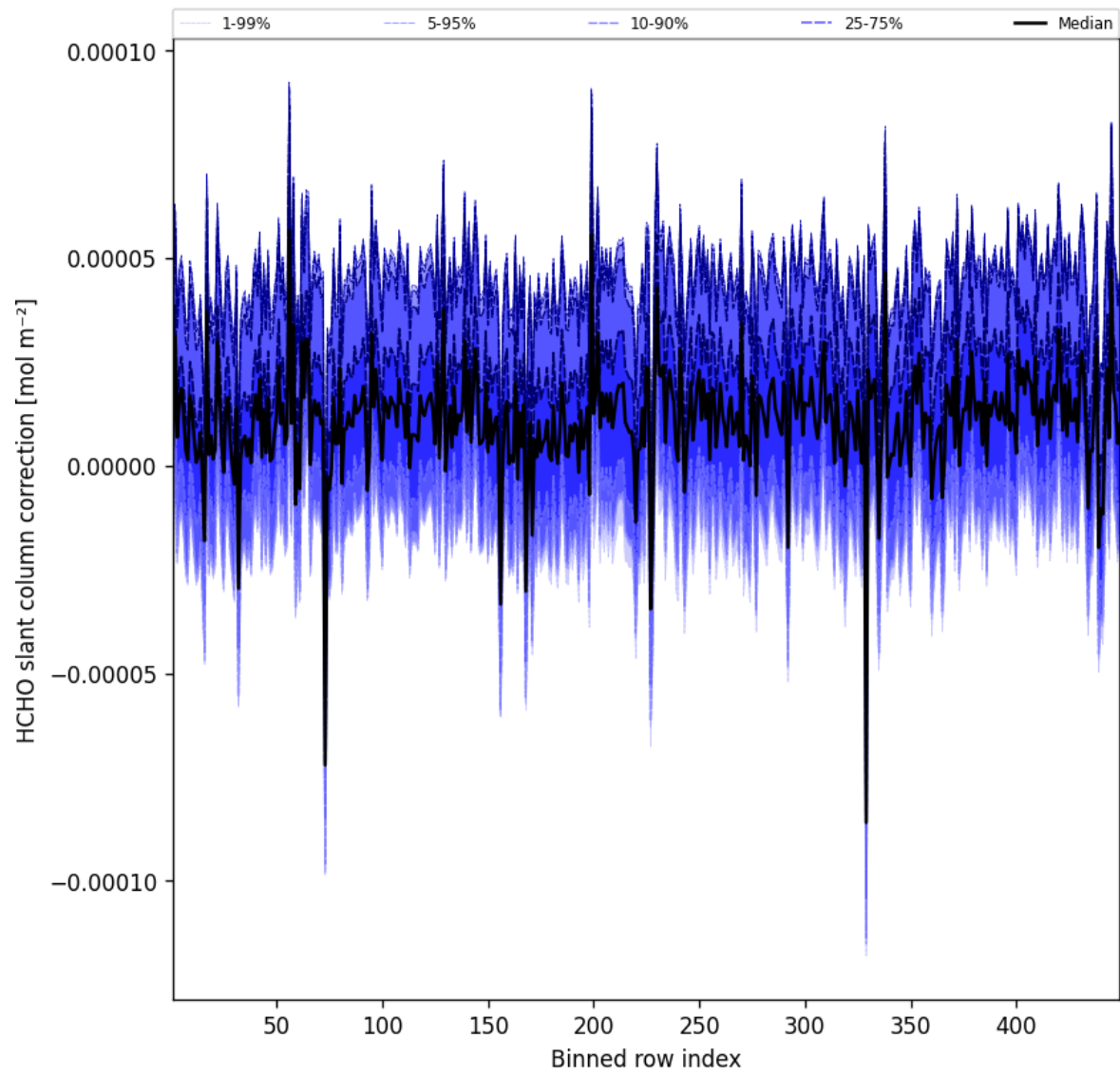
Figure 59: Along track statistics of “HCHO slant column correction” for 2025-09-28 to 2025-09-29
