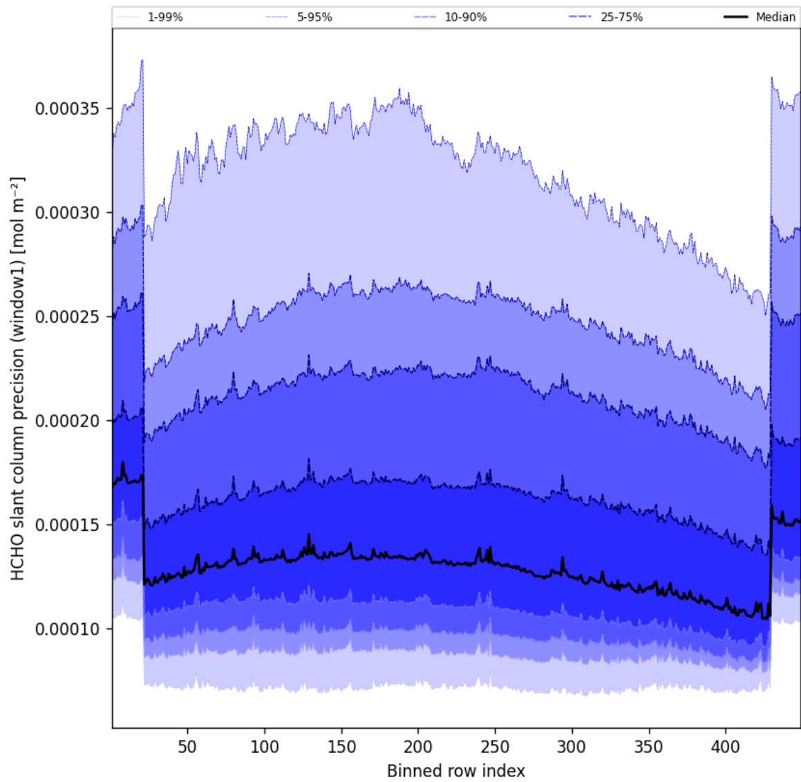
Figure 51: Along track statistics of “HCHO slant column precision (window1)” for 2025-09-28 to 2025-09-29
