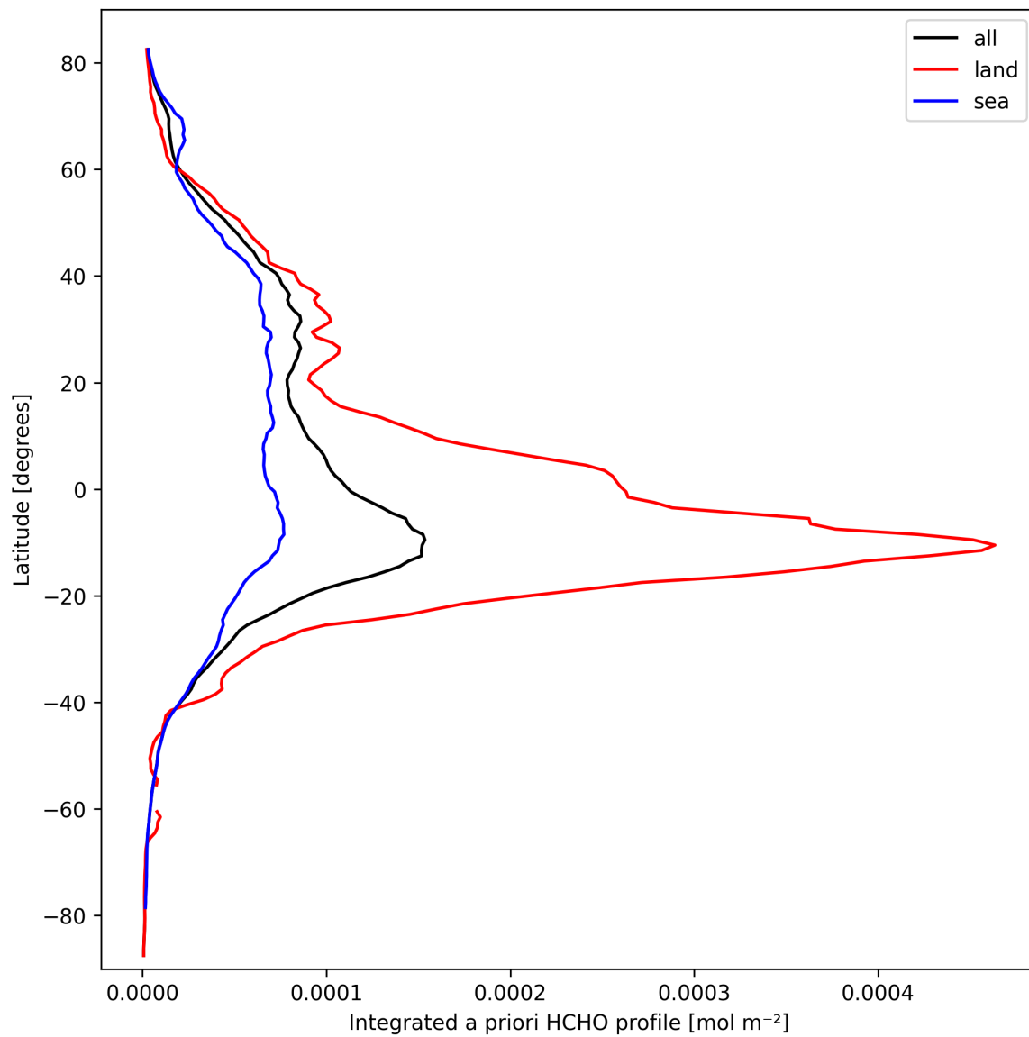
Figure 27: Zonal average of “Integrated a priori HCHO profile” for 2025-09-28 to 2025-09-29.
