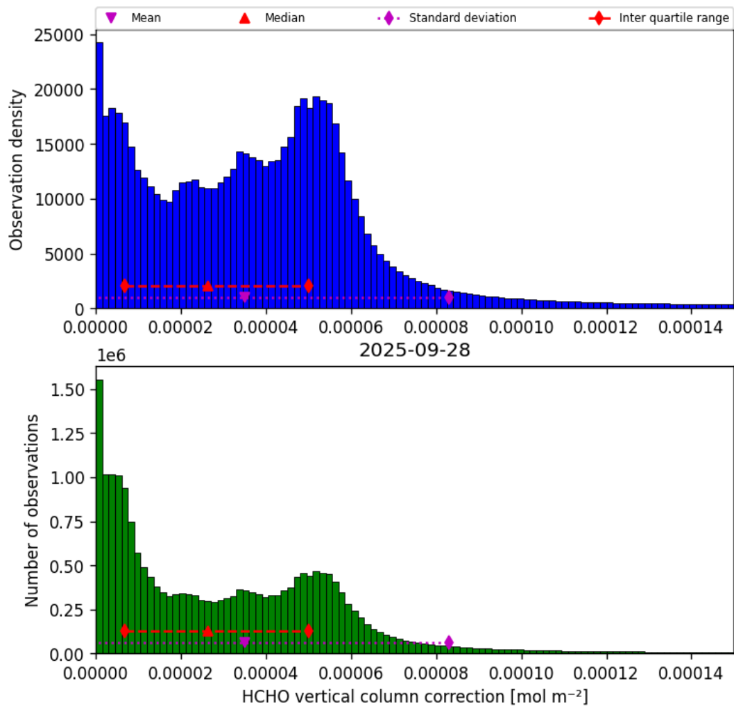
Figure 35: Histogram of “HCHO vertical column correction” for 2025-09-28 to 2025-09-29
