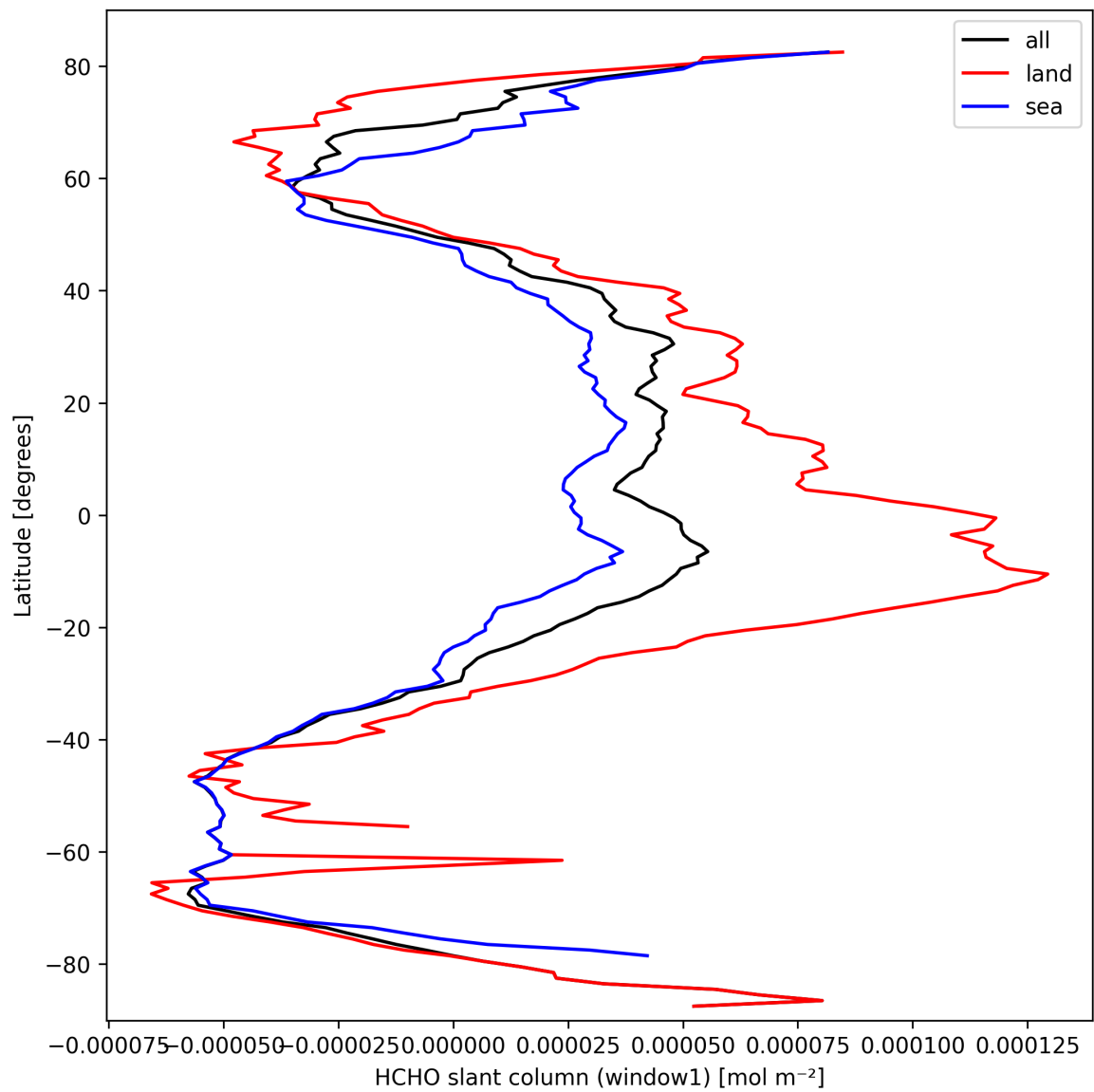
Figure 22: Zonal average of “HCHO slant column (window1)” for 2025-09-28 to 2025-09-29.
