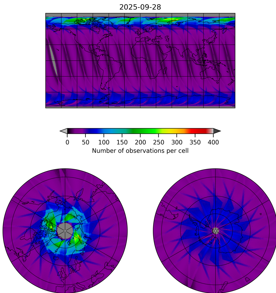
Figure 17: Map of the number of observations for 2025-09-28 to 2025-09-29
