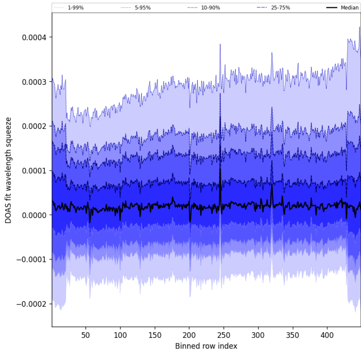
Figure 57: Along track statistics of “DOAS fit wavelength squeeze” for 2025-09-28 to 2025-09-29
