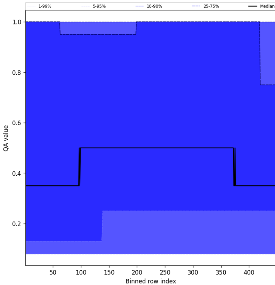
Figure 46: Along track statistics of “QA value” for 2025-09-28 to 2025-09-29
