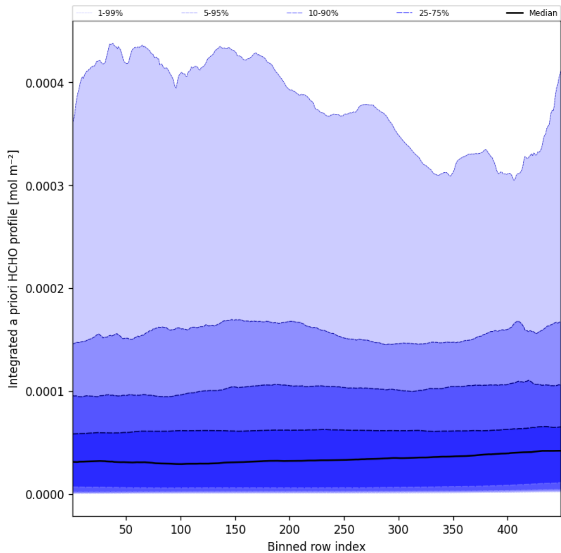
Figure 55: Along track statistics of “Integrated a priori HCHO profile” for 2025-09-28 to 2025-09-29
