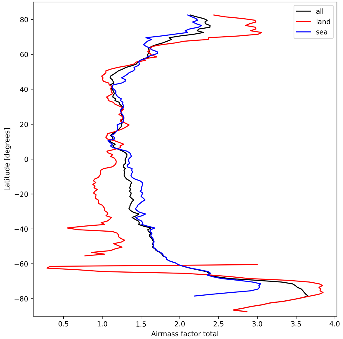
Figure 24: Zonal average of “Airmass factor total” for 2025-09-28 to 2025-09-29.
