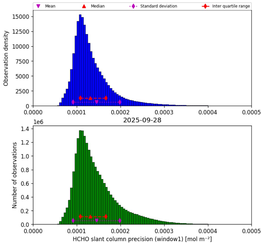
Figure 37: Histogram of “HCHO slant column precision (window1)” for 2025-09-28 to 2025-09-29
