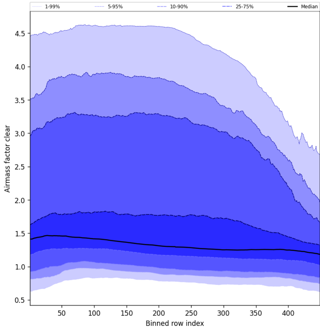
Figure 54: Along track statistics of “Airmass factor clear” for 2025-09-28 to 2025-09-29
