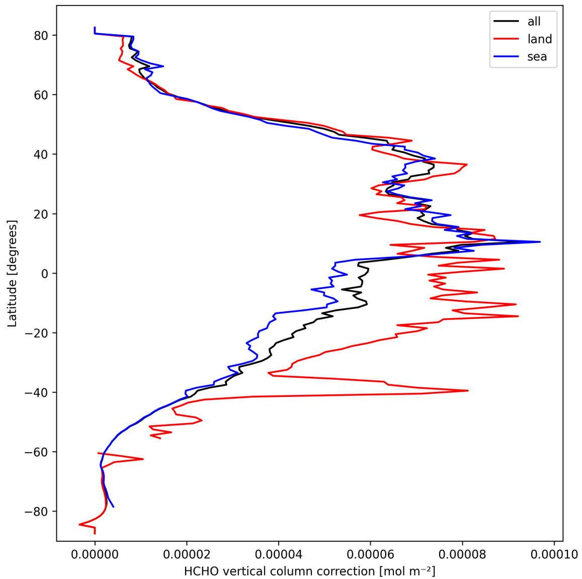
Figure 21: Zonal average of “HCHO vertical column correction” for 2025-09-28 to 2025-09-29.
