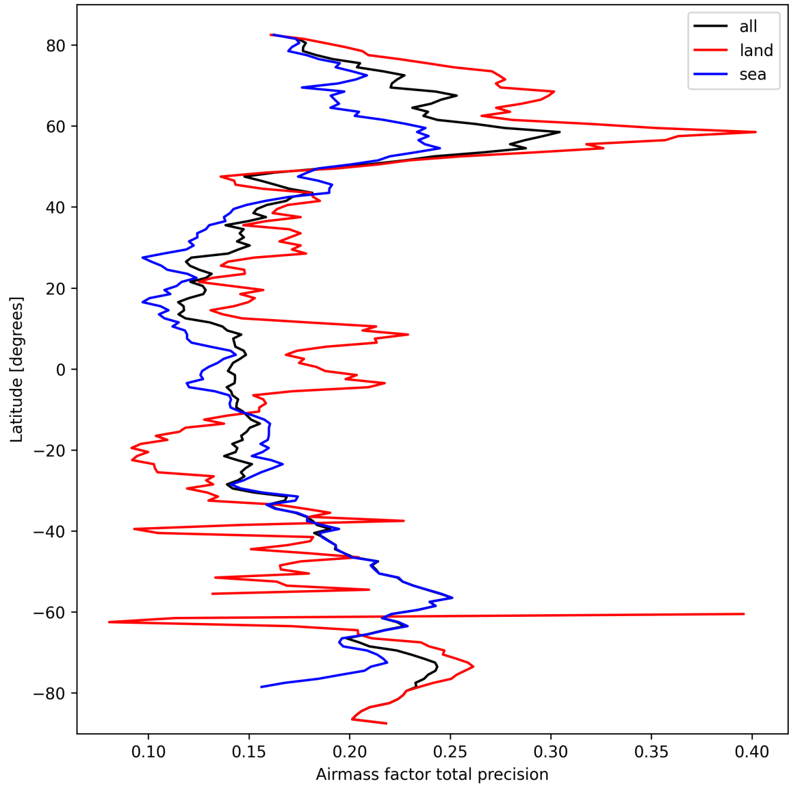
Figure 25: Zonal average of “Airmass factor total precision” for 2025-09-28 to 2025-09-29.
