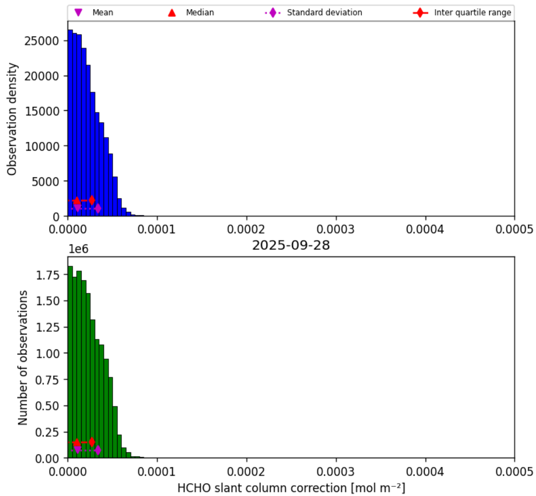
Figure 45: Histogram of “HCHO slant column correction” for 2025-09-28 to 2025-09-29
