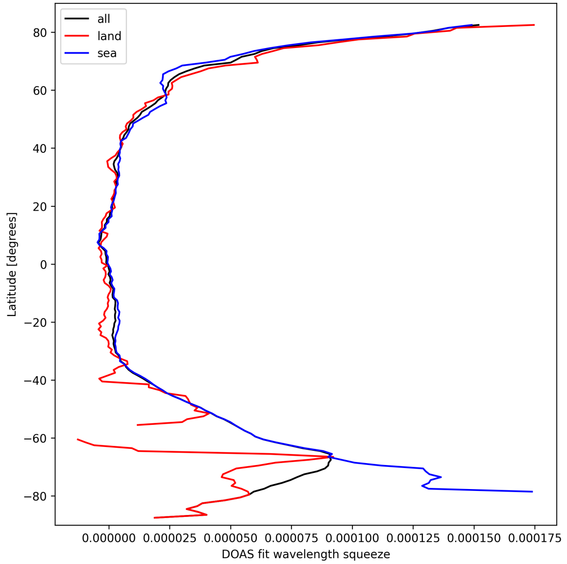
Figure 29: Zonal average of “DOAS fit wavelength squeeze” for 2025-09-28 to 2025-09-29.
