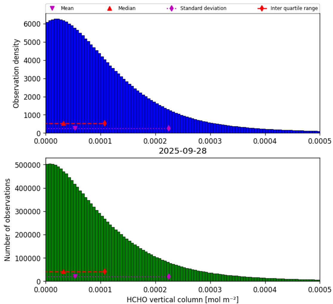
Figure 33: Histogram of “HCHO vertical column” for 2025-09-28 to 2025-09-29
