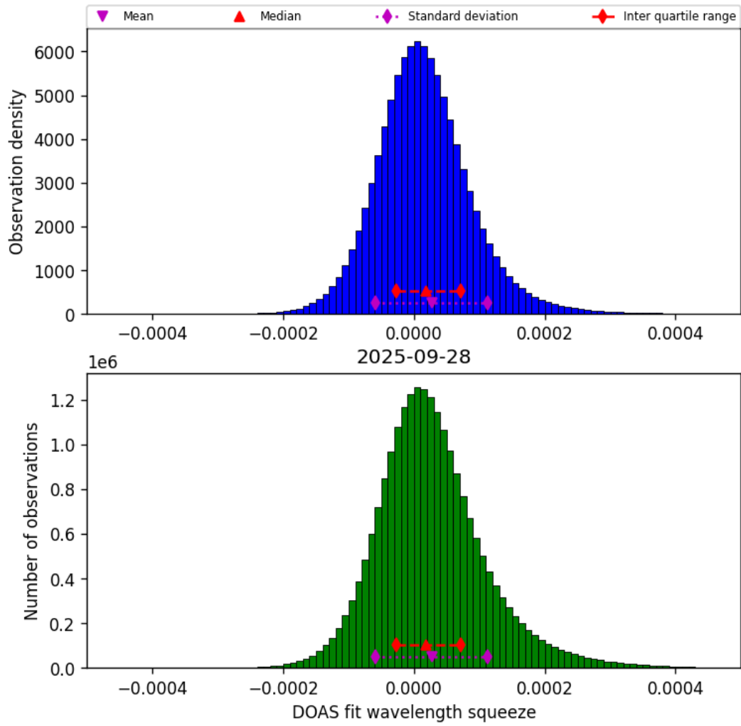
Figure 43: Histogram of “DOAS fit wavelength squeeze” for 2025-09-28 to 2025-09-29
