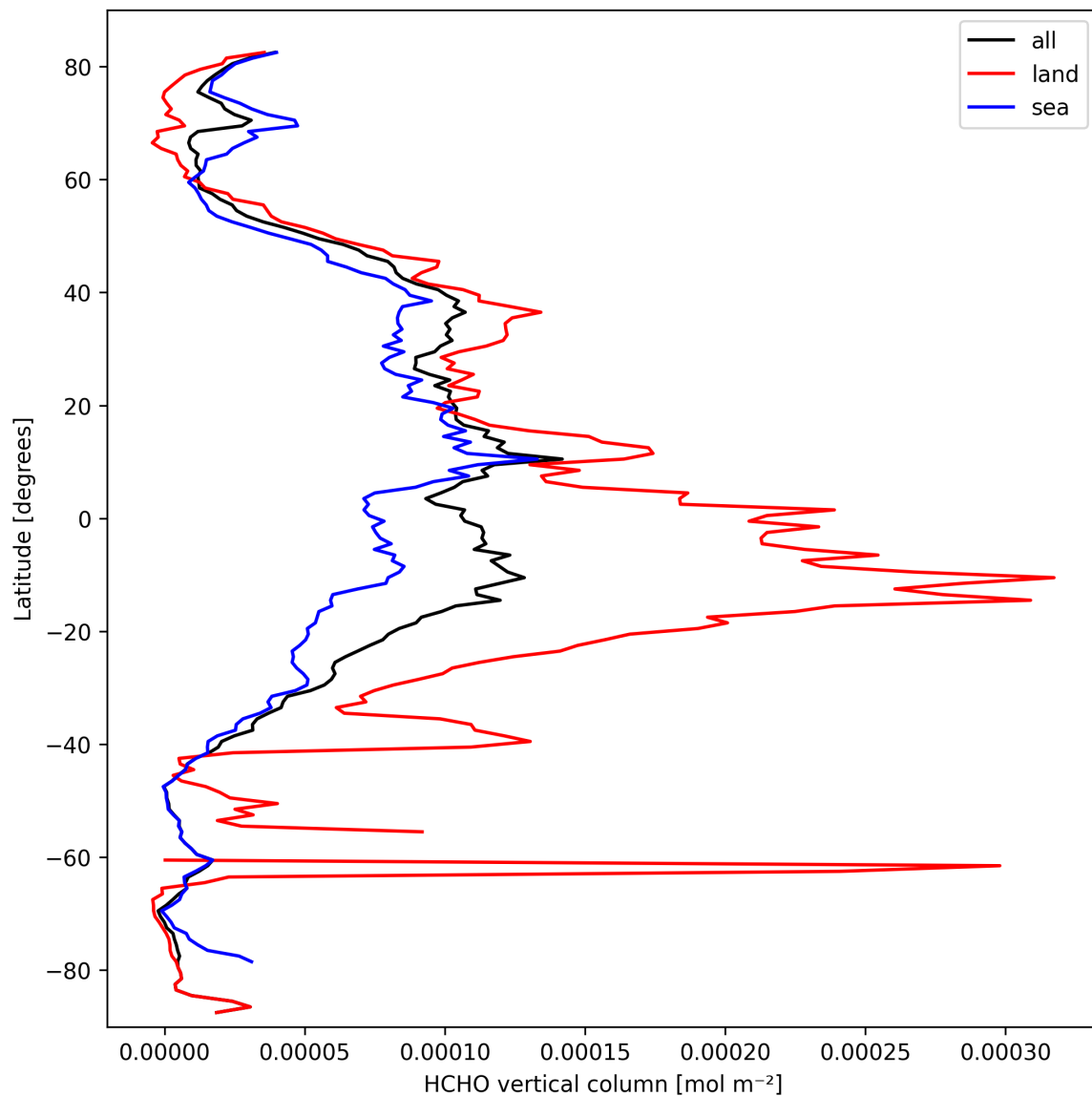
Figure 19: Zonal average of “HCHO vertical column” for 2025-09-28 to 2025-09-29.
