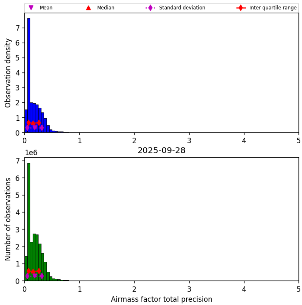
Figure 39: Histogram of “Airmass factor total precision” for 2025-09-28 to 2025-09-29
