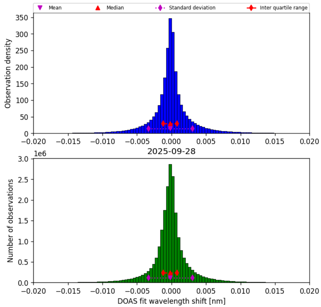
Figure 42: Histogram of “DOAS fit wavelength shift” for 2025-09-28 to 2025-09-29
