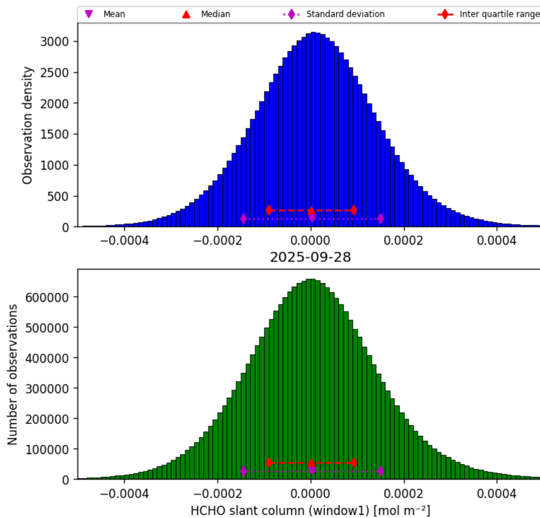
Figure 36: Histogram of “HCHO slant column (window1)” for 2025-09-28 to 2025-09-29
