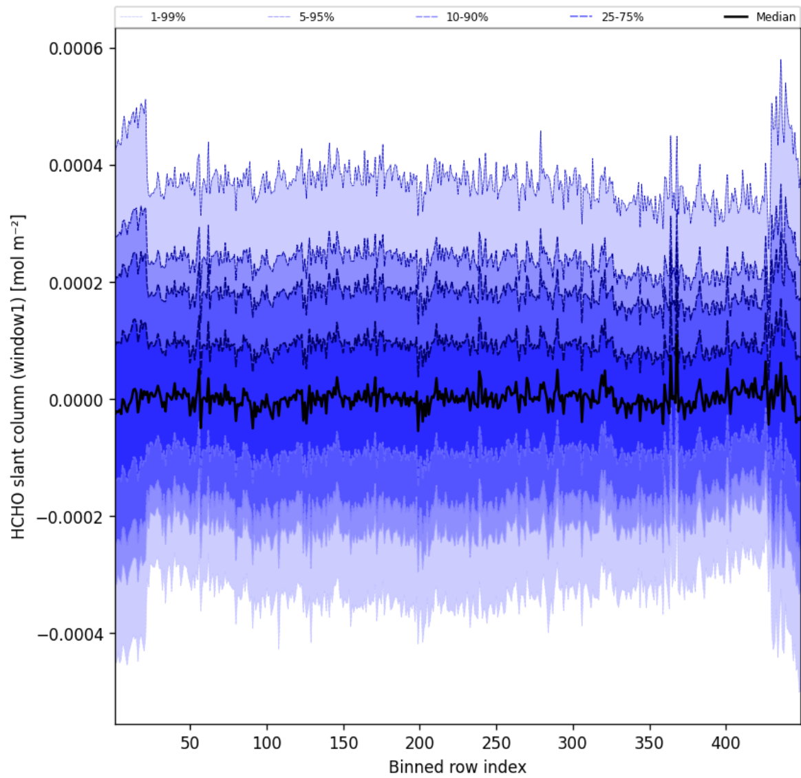
Figure 50: Along track statistics of “HCHO slant column (window1)” for 2025-09-28 to 2025-09-29
