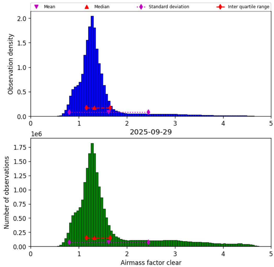
Figure 40: Histogram of “Airmass factor clear” for 2025-09-29 to 2025-09-29
