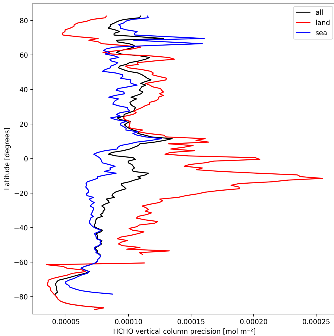
Figure 20: Zonal average of "HCHO vertical column precision" for 2025-09-29 to 2025-09-29.
