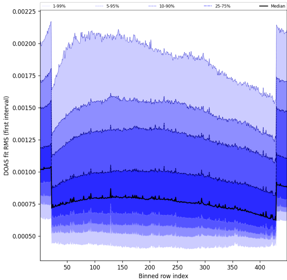
Figure 58: Along track statistics of “DOAS fit RMS (first interval)” for 2025-09-29 to 2025-09-29
