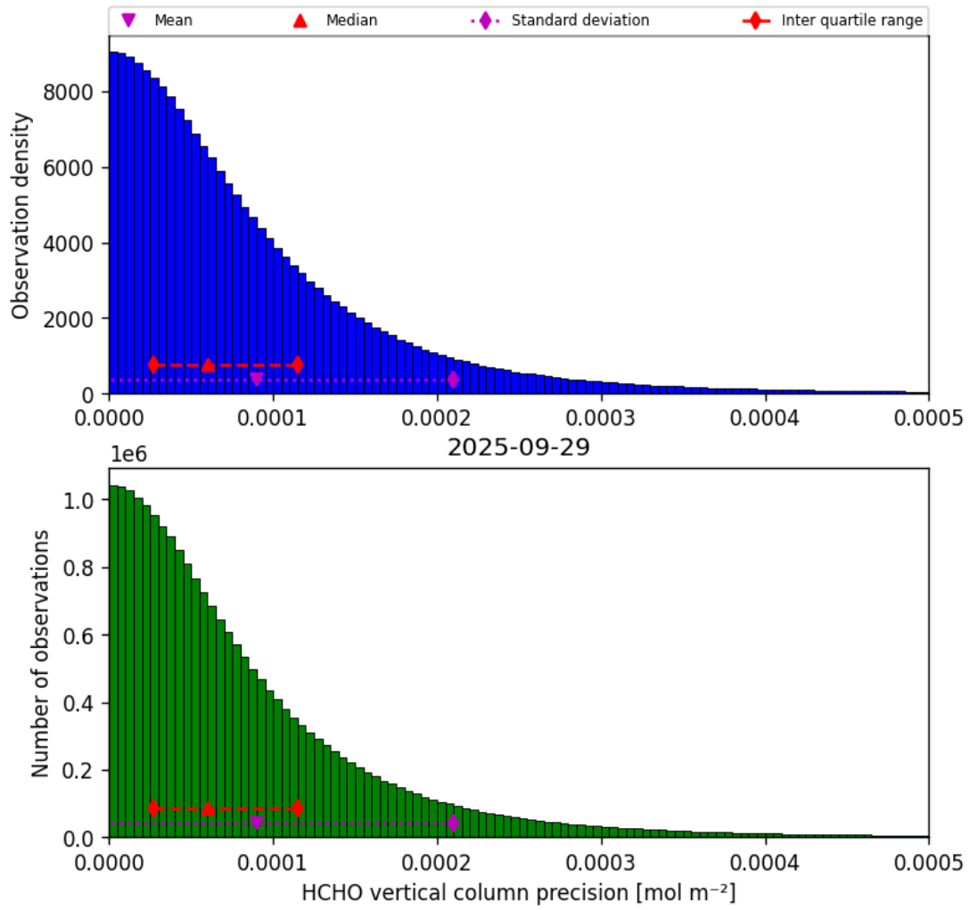
Figure 34: Histogram of “HCHO vertical column precision” for 2025-09-29 to 2025-09-29
