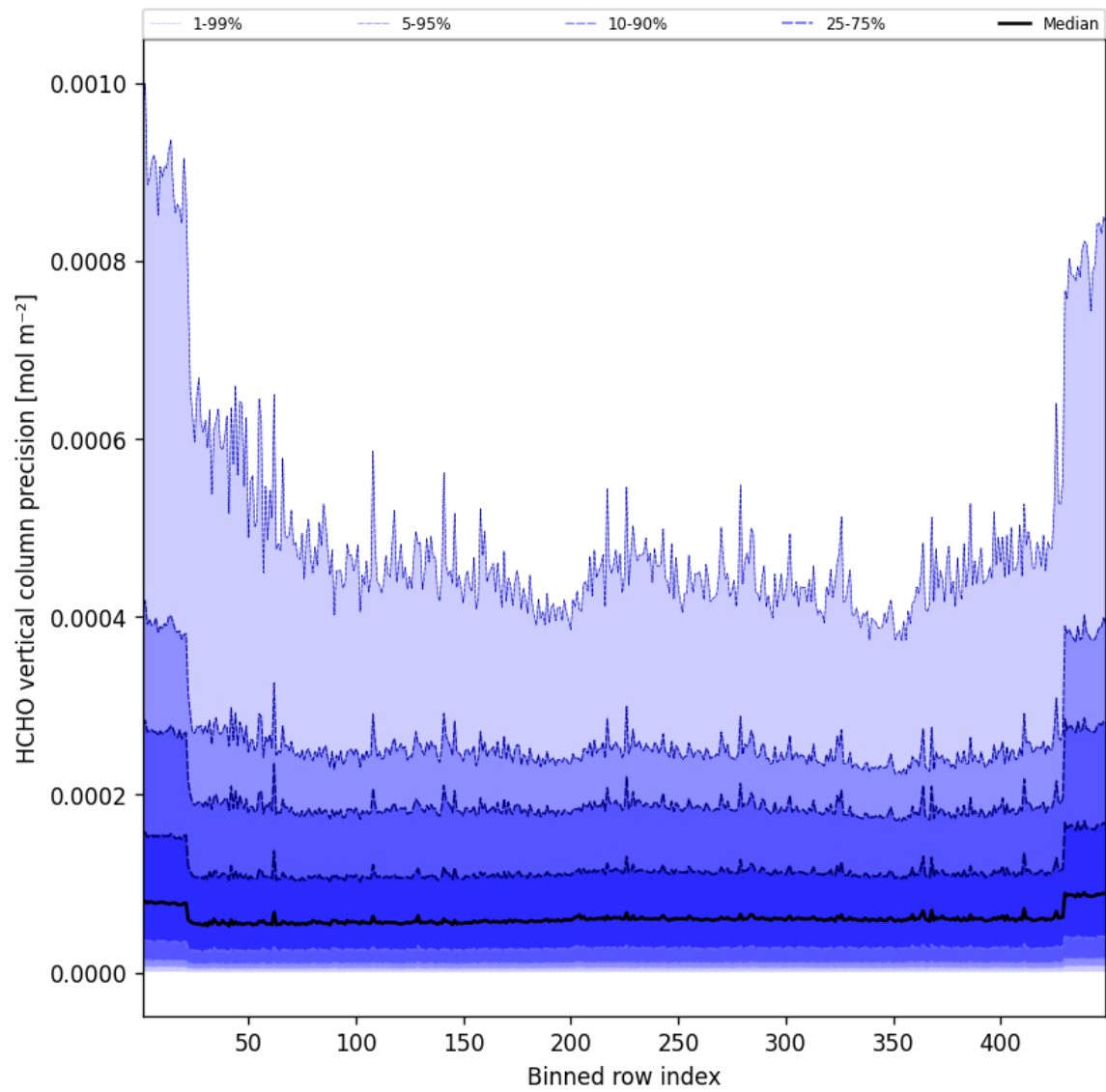
Figure 48: Along track statistics of “HCHO vertical column precision” for 2025-09-29 to 2025-09-29
