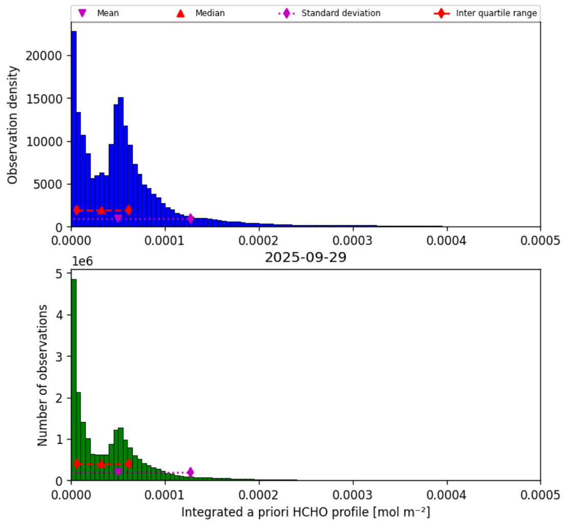
Figure 41: Histogram of “Integrated a priori HCHO profile” for 2025-09-29 to 2025-09-29
