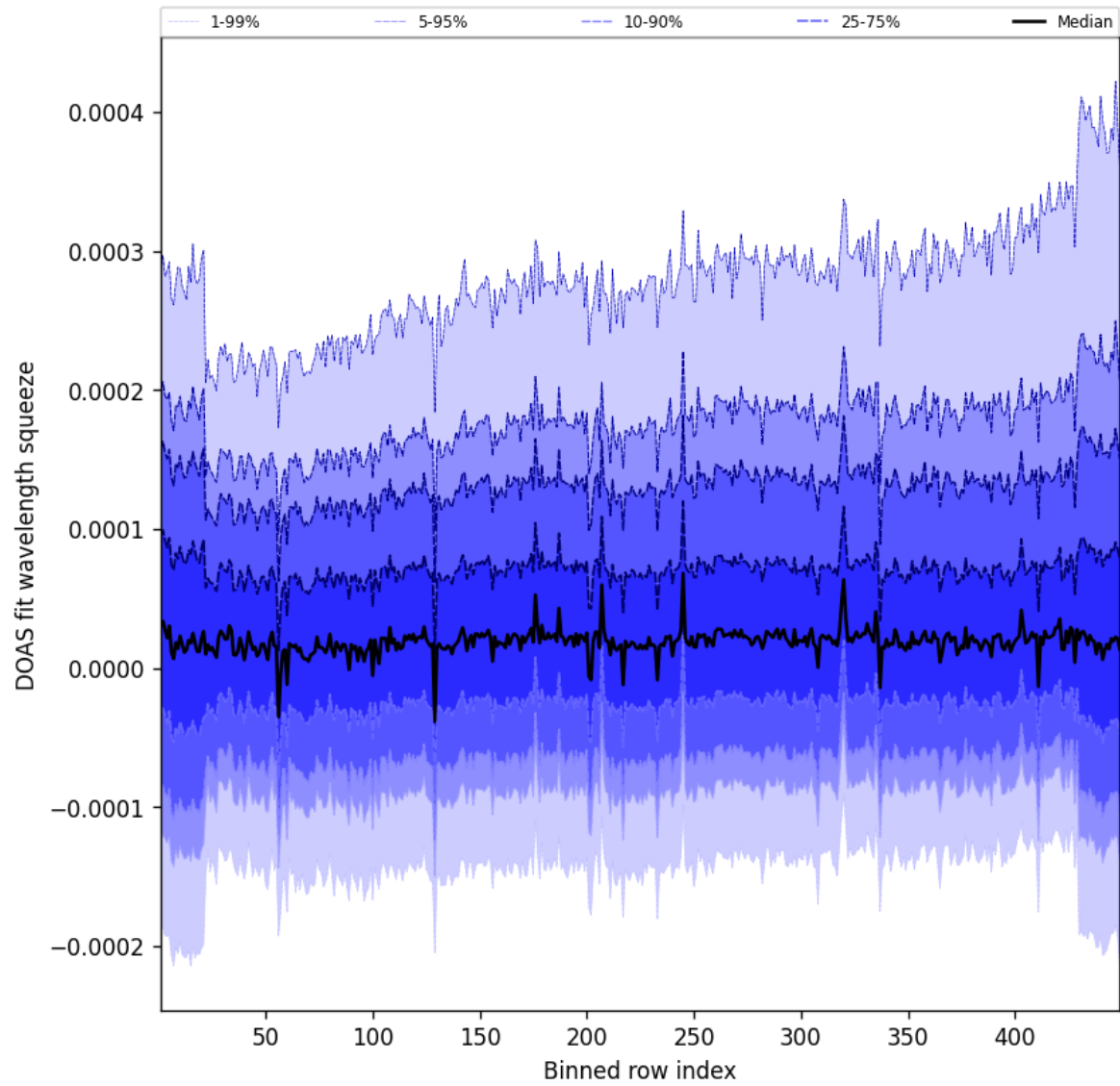
Figure 57: Along track statistics of “DOAS fit wavelength squeeze” for 2025-09-29 to 2025-09-29
