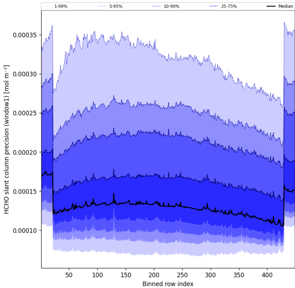
Figure 51: Along track statistics of “HCHO slant column precision (window1)” for 2025-09-29 to 2025-09-29
