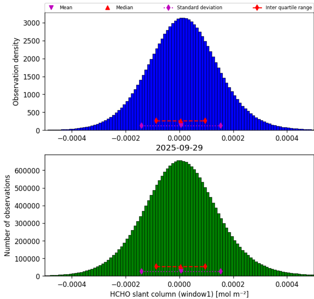
Figure 36: Histogram of “HCHO slant column (window1)” for 2025-09-29 to 2025-09-29
