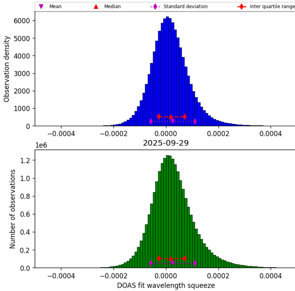
Figure 43: Histogram of “DOAS fit wavelength squeeze” for 2025-09-29 to 2025-09-29
