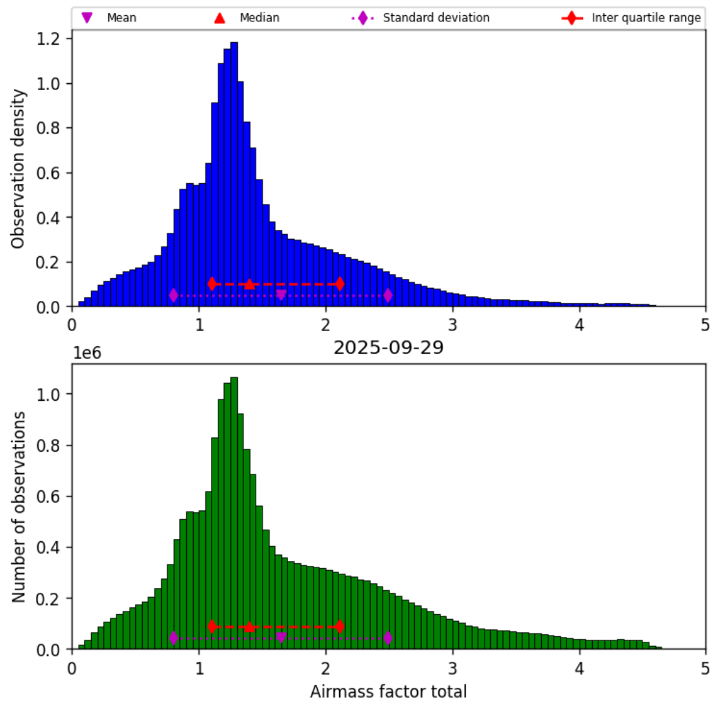
Figure 38: Histogram of “Airmass factor total” for 2025-09-29 to 2025-09-29
