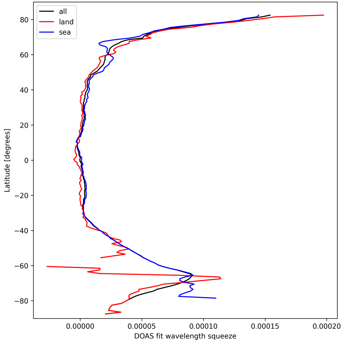
Figure 29: Zonal average of “DOAS fit wavelength squeeze” for 2025-09-29 to 2025-09-29.
