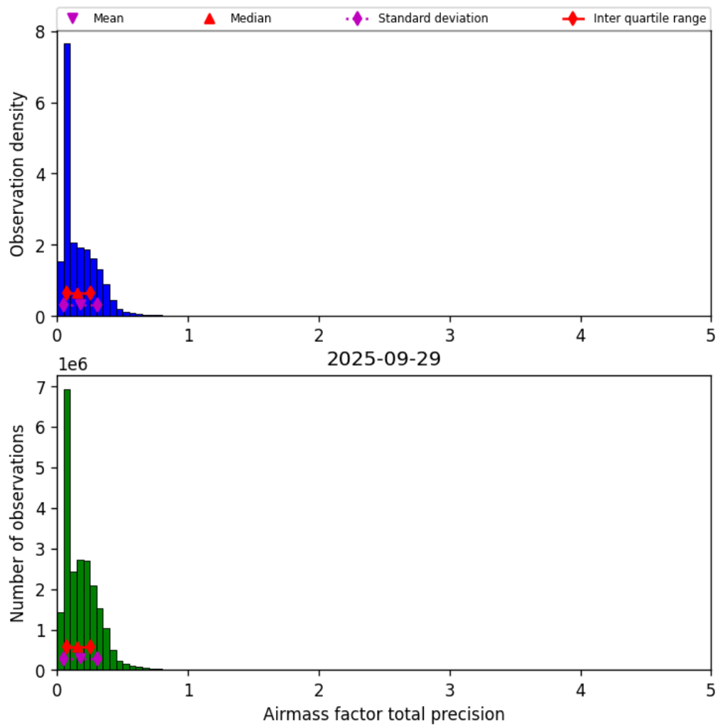
Figure 39: Histogram of “Airmass factor total precision” for 2025-09-29 to 2025-09-29
