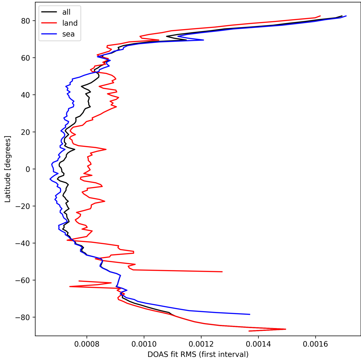
Figure 30: Zonal average of “DOAS fit RMS (first interval)” for 2025-09-29 to 2025-09-29.
