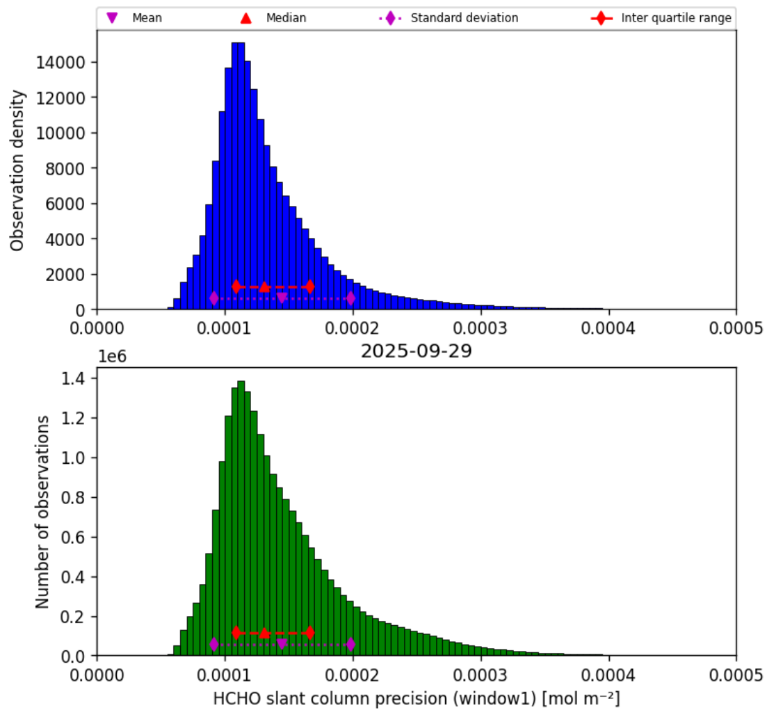
Figure 37: Histogram of “HCHO slant column precision (window1)” for 2025-09-29 to 2025-09-29
