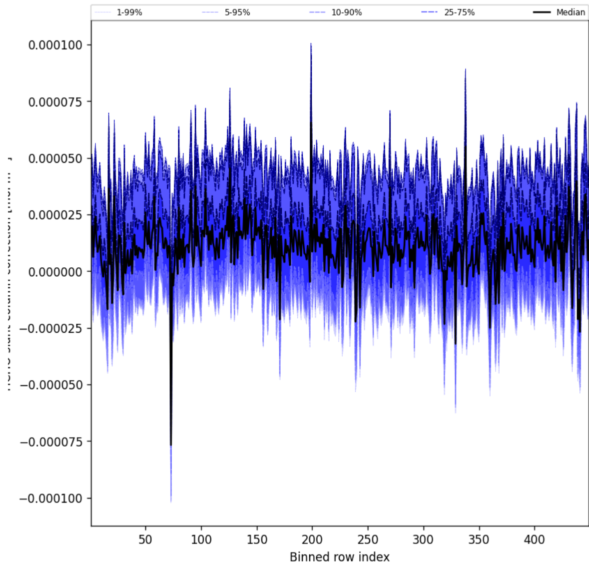
Figure 59: Along track statistics of “HCHO slant column correction” for 2025-09-29 to 2025-09-29
