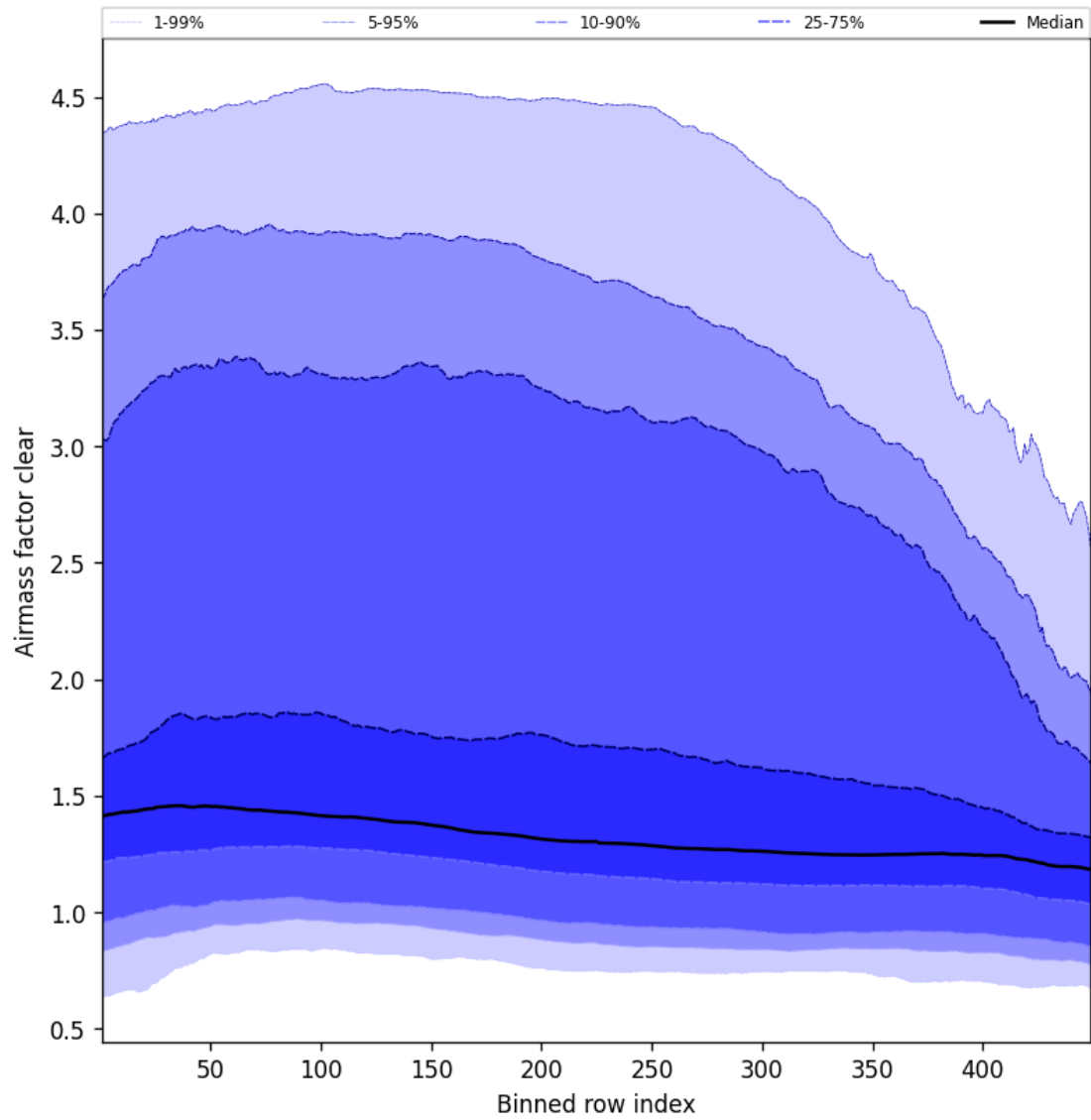
Figure 54: Along track statistics of “Airmass factor clear” for 2025-09-29 to 2025-09-29
