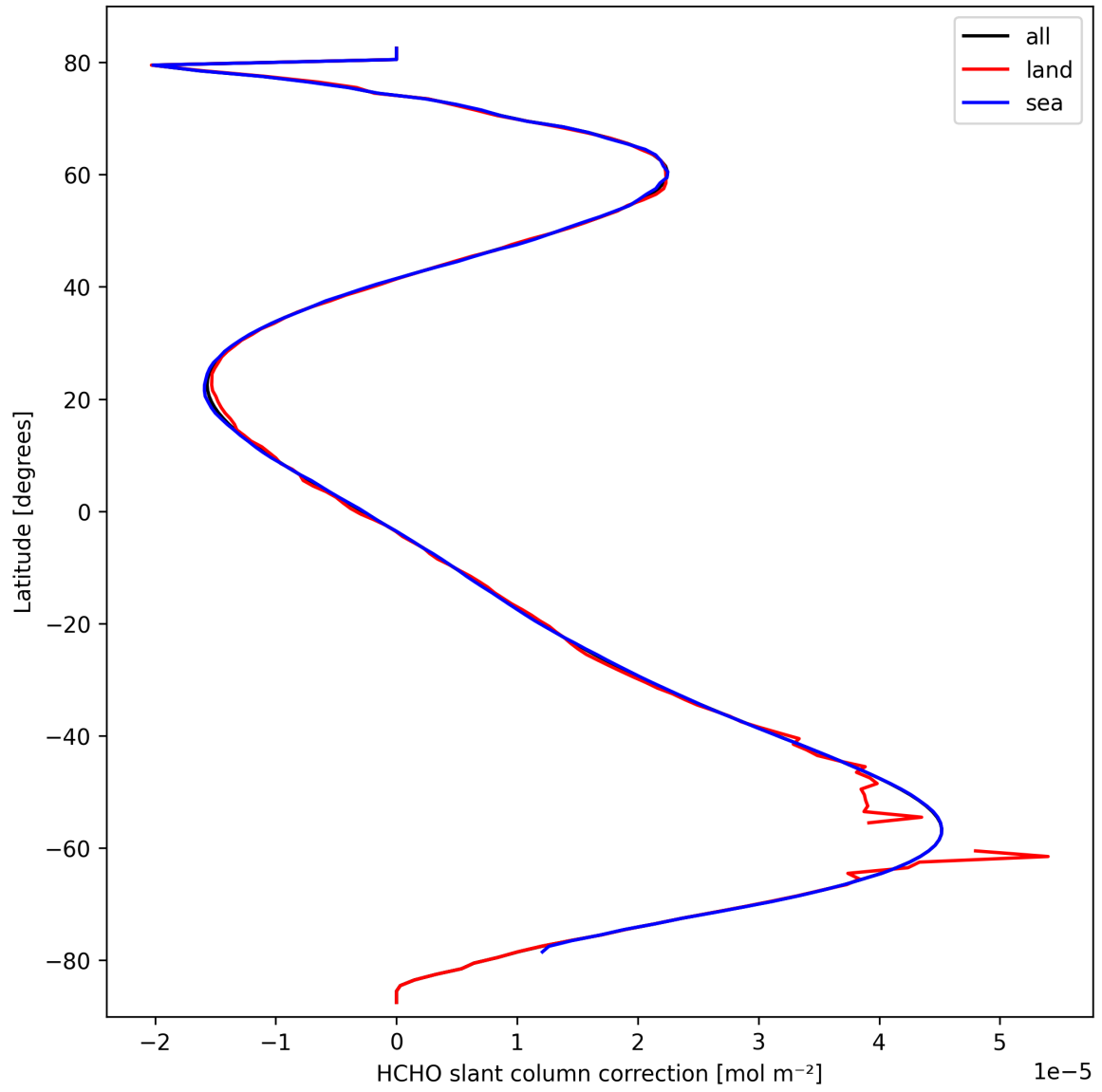
Figure 31: Zonal average of “HCHO slant column correction” for 2025-09-29 to 2025-09-29.
