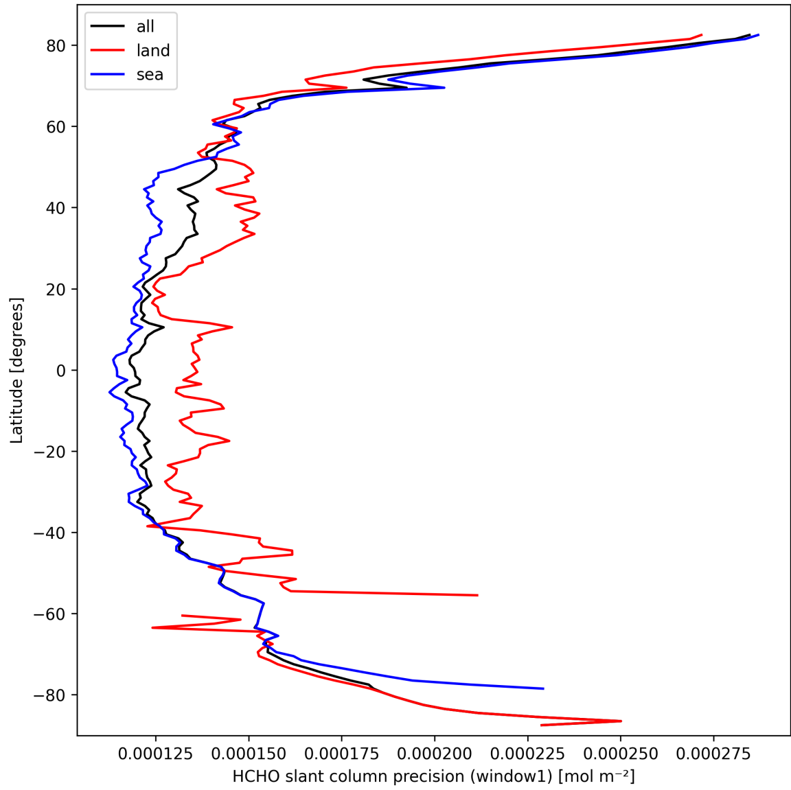
Figure 23: Zonal average of “HCHO slant column precision (window1)” for 2025-09-29 to 2025-09-29.
