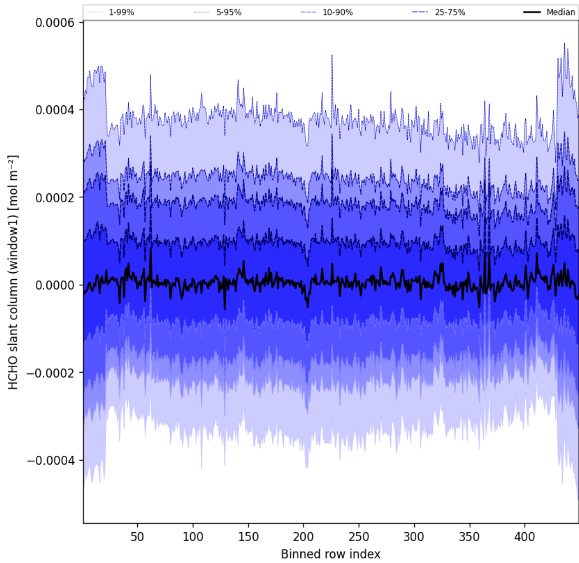
Figure 50: Along track statistics of "HCHO slant column (window1)" for 2025-09-29 to 2025-09-29
