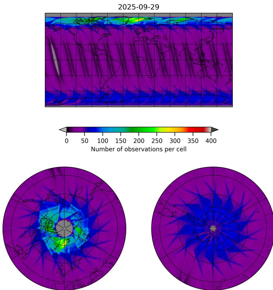
Figure 17: Map of the number of observations for 2025-09-29 to 2025-09-29
