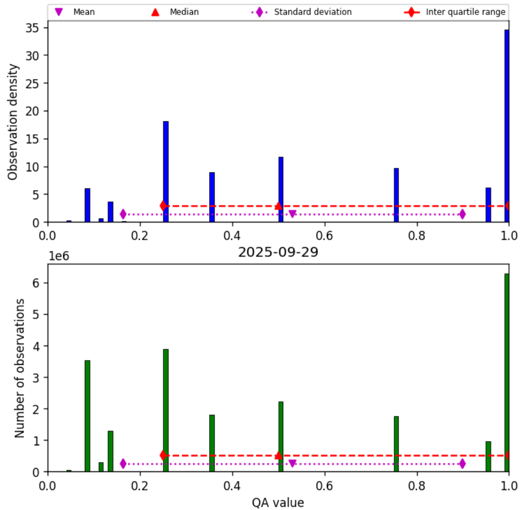
Figure 32: Histogram of “QA value” for 2025-09-29 to 2025-09-29
