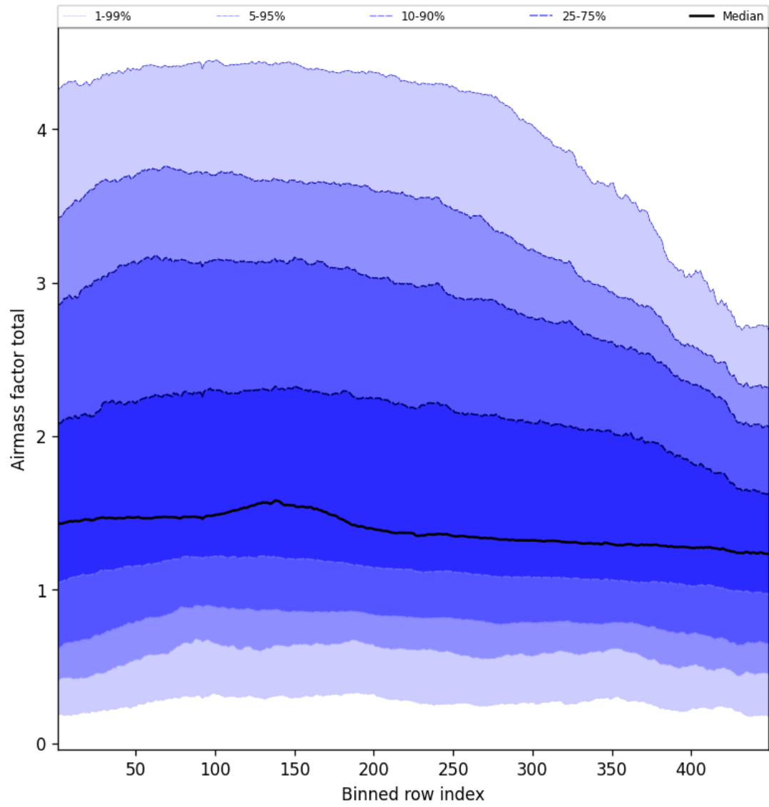
Figure 52: Along track statistics of “Airmass factor total” for 2025-09-29 to 2025-09-29
