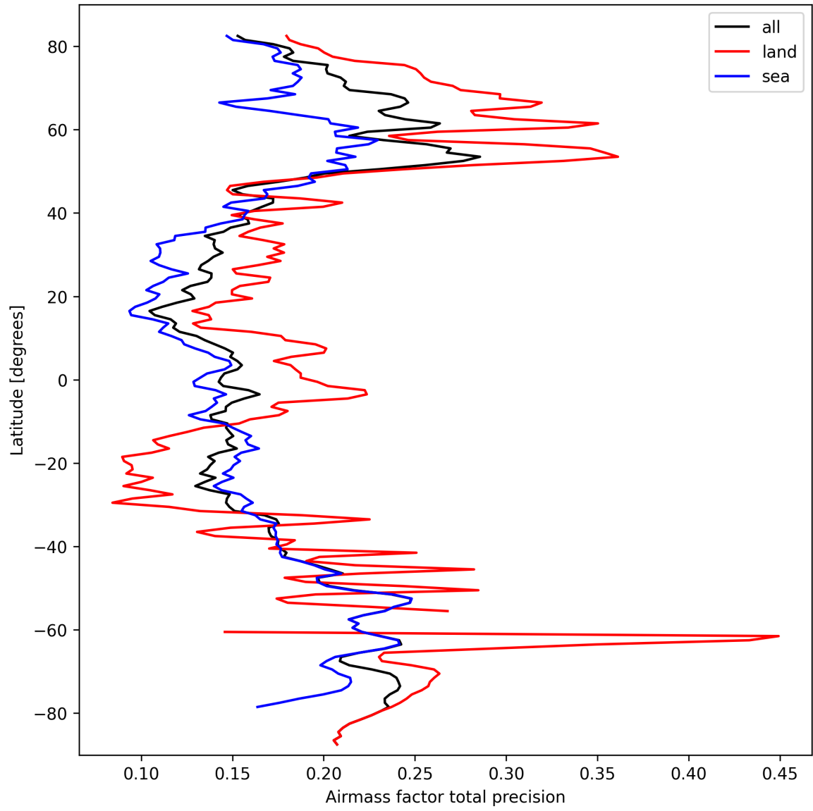
Figure 25: Zonal average of “Airmass factor total precision” for 2025-09-29 to 2025-09-29.
