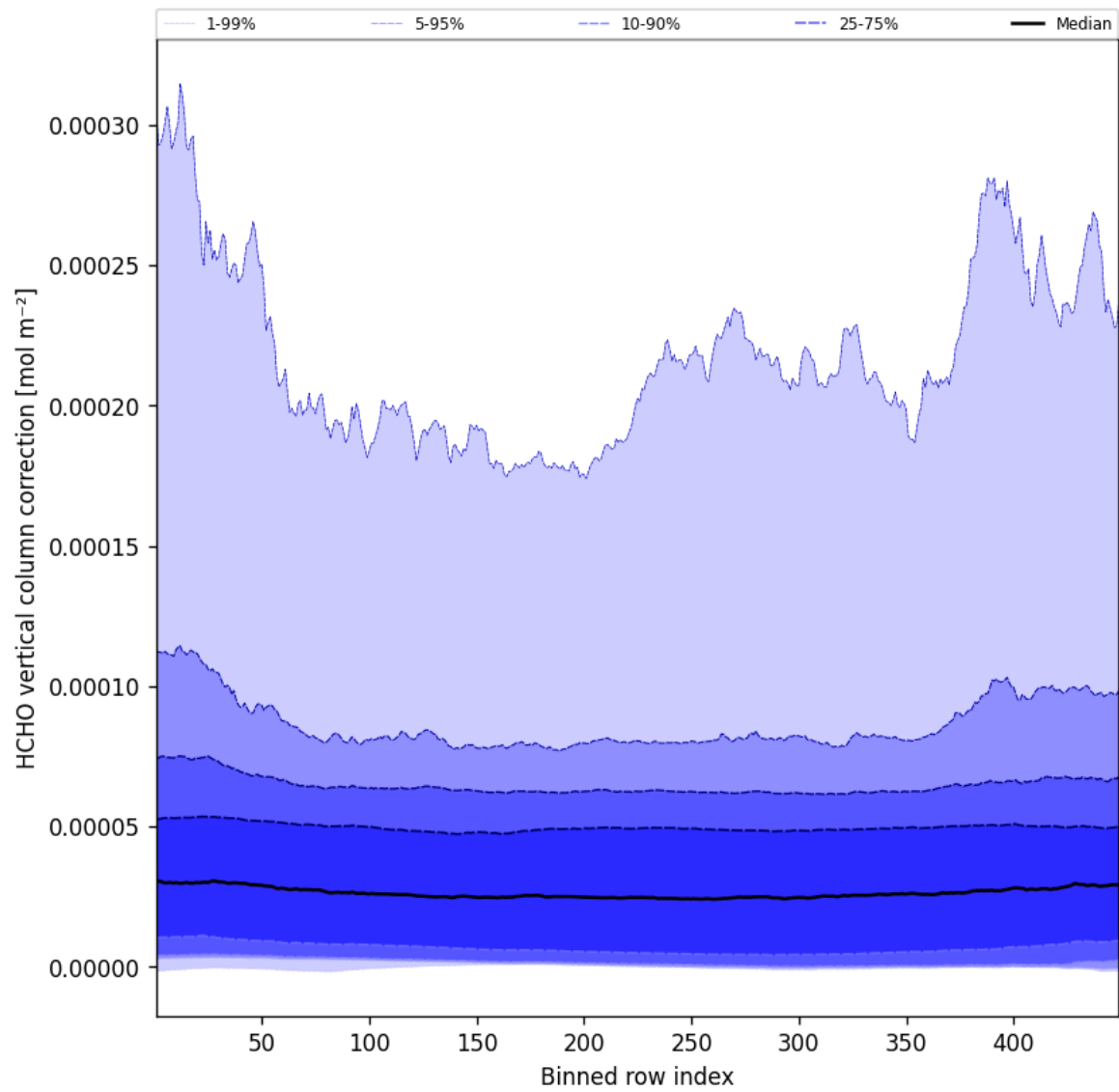
Figure 49: Along track statistics of “HCHO vertical column correction” for 2025-09-29 to 2025-09-29
