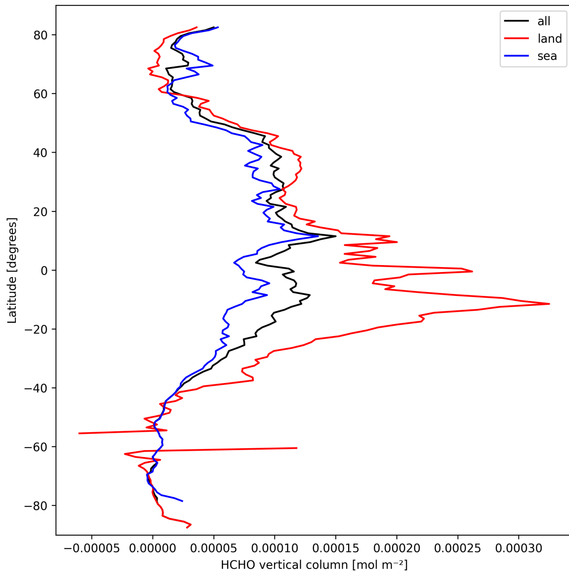
Figure 19: Zonal average of “HCHO vertical column” for 2025-09-29 to 2025-09-29.
