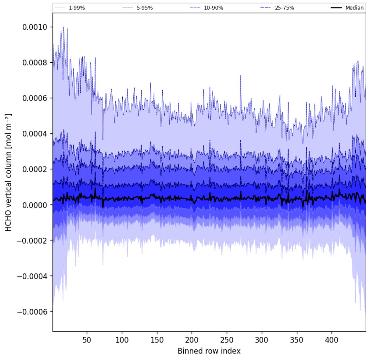
Figure 47: Along track statistics of “HCHO vertical column” for 2025-09-29 to 2025-09-29
