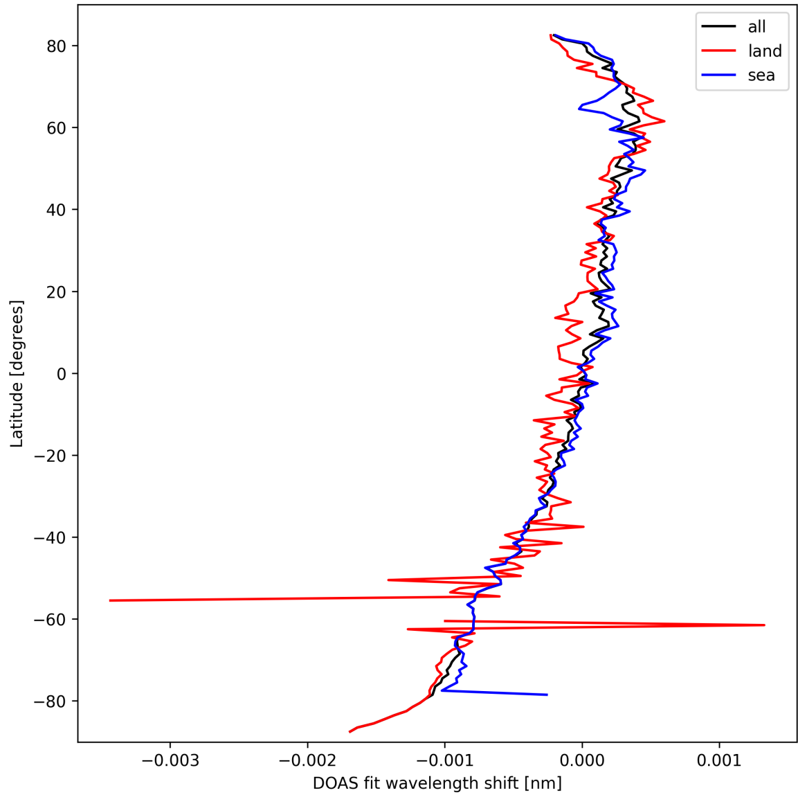
Figure 28: Zonal average of “DOAS fit wavelength shift” for 2025-09-29 to 2025-09-29.
