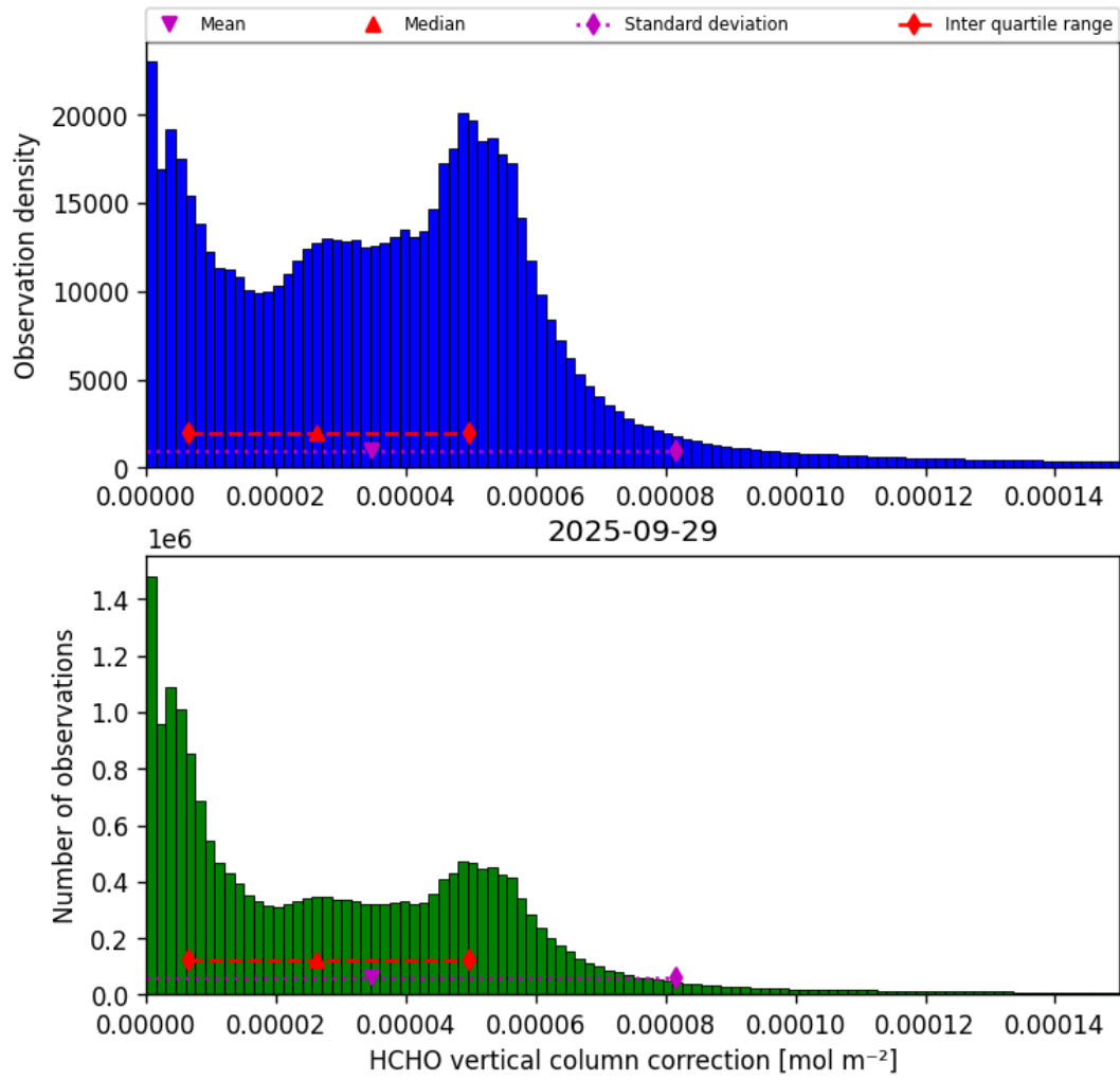
Figure 35: Histogram of “HCHO vertical column correction” for 2025-09-29 to 2025-09-29
