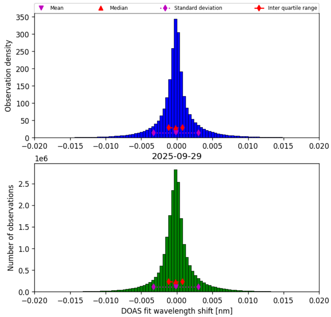
Figure 42: Histogram of “DOAS fit wavelength shift” for 2025-09-29 to 2025-09-29
