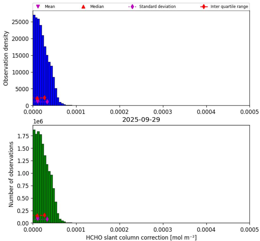
Figure 45: Histogram of “HCHO slant column correction” for 2025-09-29 to 2025-09-29
