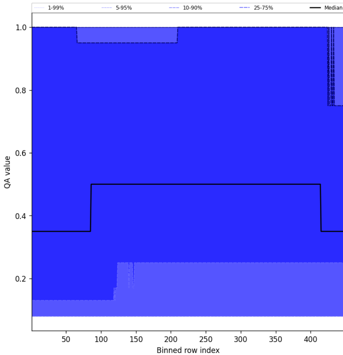
Figure 46: Along track statistics of "QA value" for 2025-09-29 to 2025-09-29
