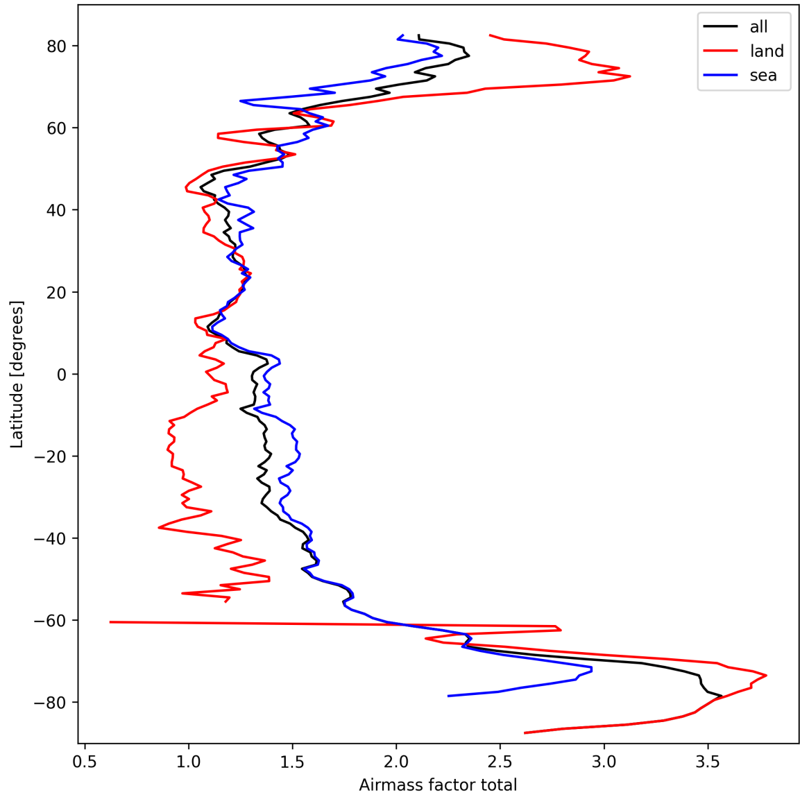
Figure 24: Zonal average of “Airmass factor total” for 2025-09-29 to 2025-09-29.
