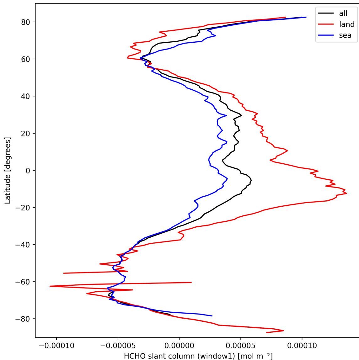
Figure 22: Zonal average of “HCHO slant column (window1)” for 2025-09-29 to 2025-09-29.
