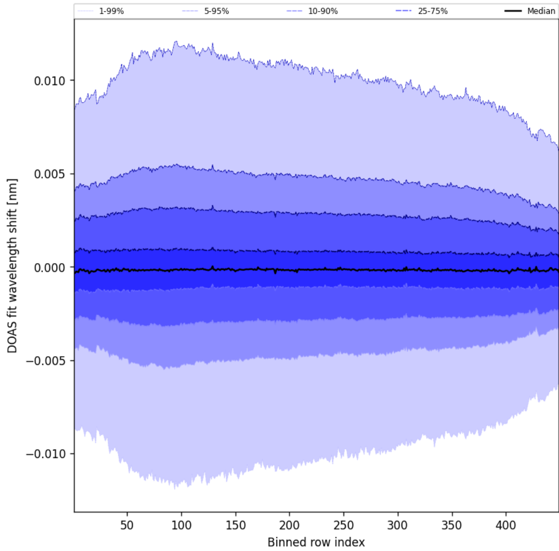
Figure 56: Along track statistics of “DOAS fit wavelength shift” for 2025-09-29 to 2025-09-29
