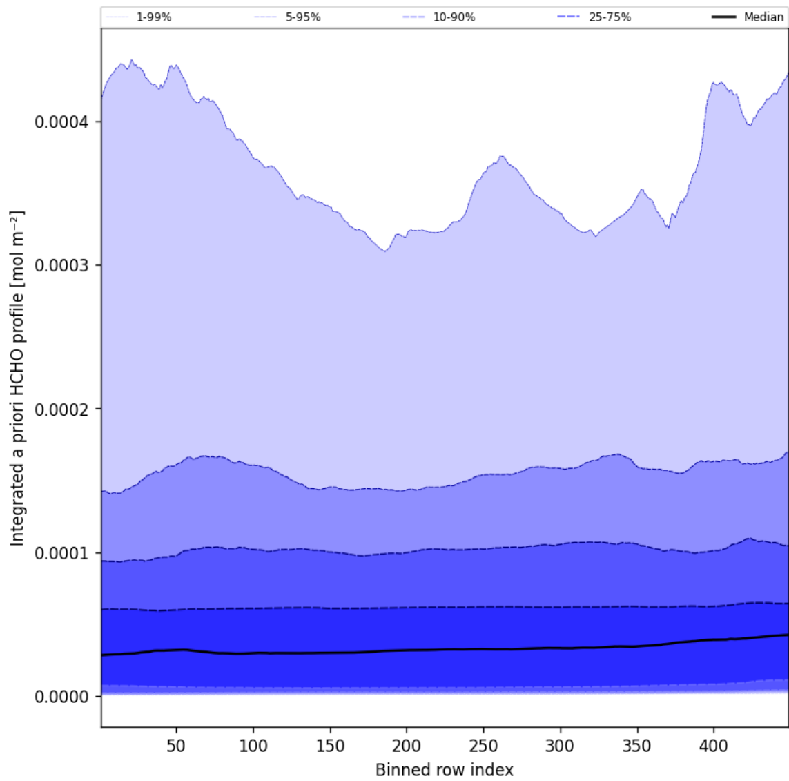
Figure 55: Along track statistics of “Integrated a priori HCHO profile” for 2025-09-29 to 2025-09-29
