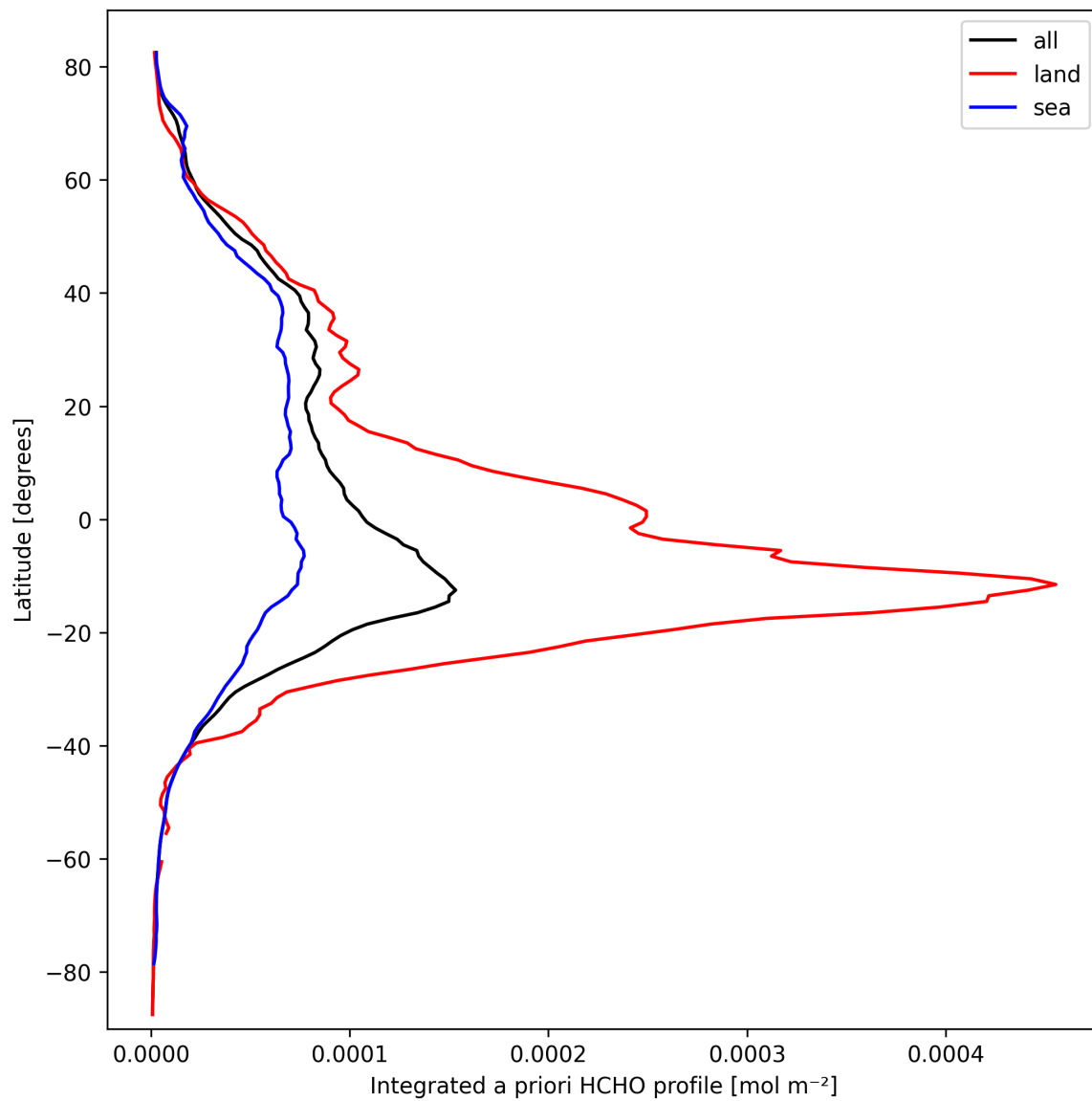
Figure 27: Zonal average of “Integrated a priori HCHO profile” for 2025-09-29 to 2025-09-29.
