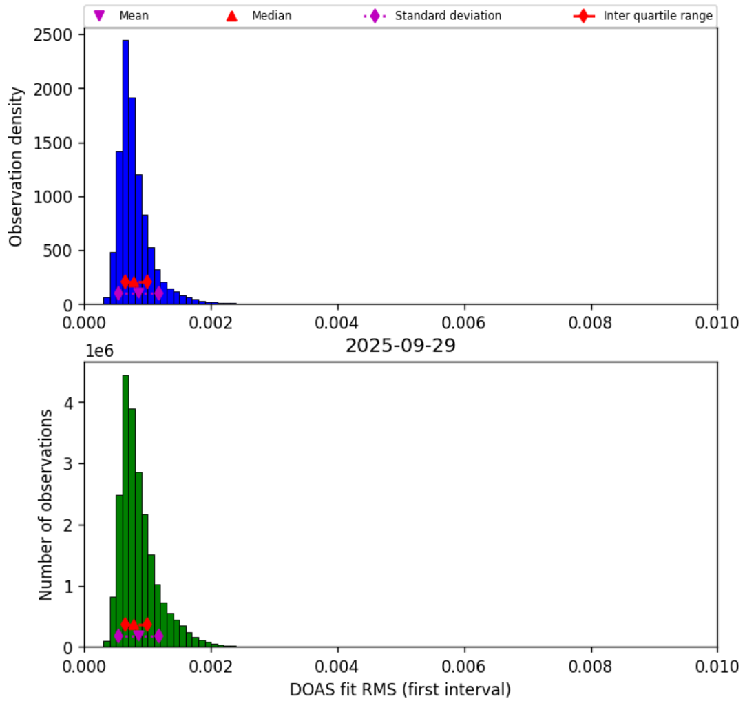
Figure 44: Histogram of “DOAS fit RMS (first interval)” for 2025-09-29 to 2025-09-29
