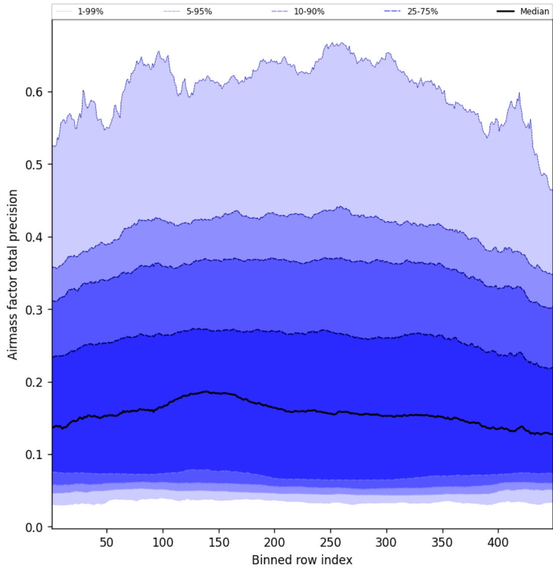
Figure 53: Along track statistics of “Airmass factor total precision” for 2025-09-29 to 2025-09-29
