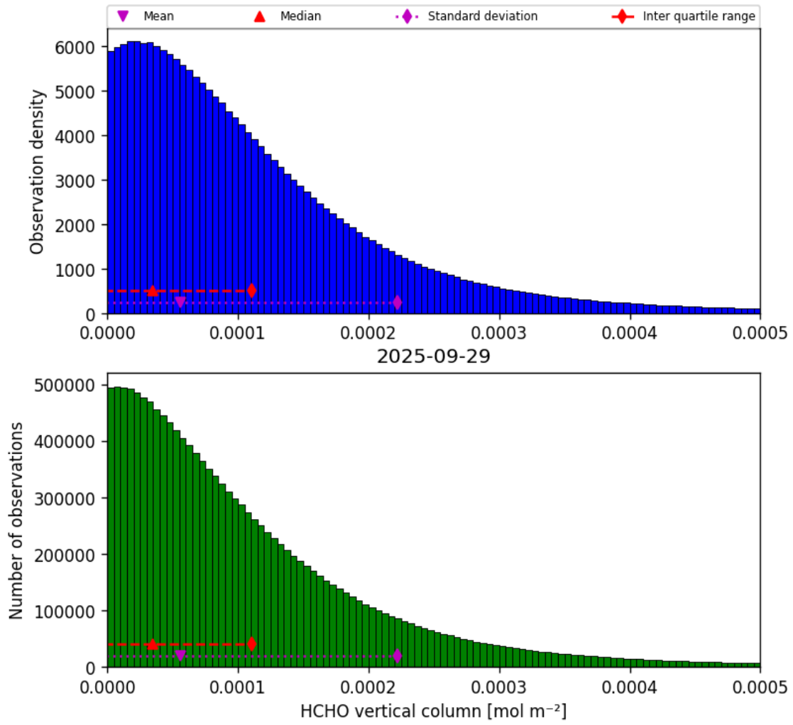
Figure 33: Histogram of “HCHO vertical column” for 2025-09-29 to 2025-09-29
