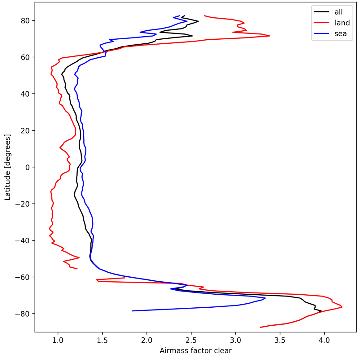
Figure 26: Zonal average of “Airmass factor clear” for 2025-09-29 to 2025-09-29.
