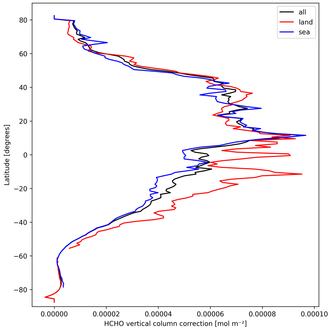
Figure 21: Zonal average of “HCHO vertical column correction” for 2025-09-29 to 2025-09-29.
