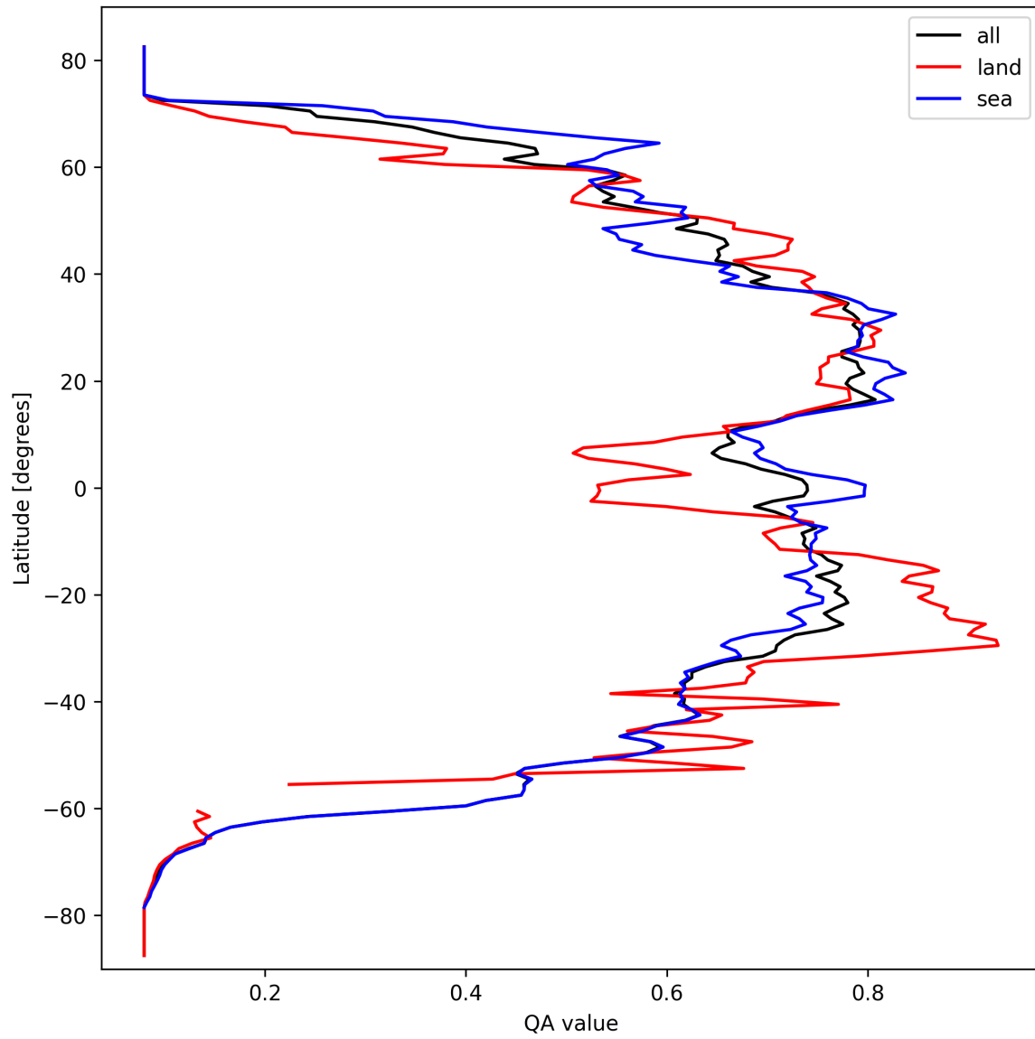
Figure 18: Zonal average of “QA value” for 2025-09-29 to 2025-09-29.
