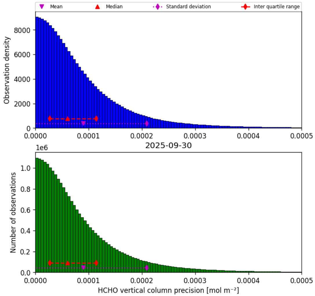
Figure 34: Histogram of “HCHO vertical column precision” for 2025-09-30 to 2025-10-01
