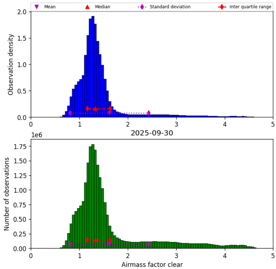
Figure 40: Histogram of “Airmass factor clear” for 2025-09-30 to 2025-10-01
