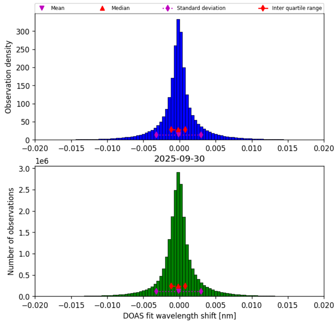
Figure 42: Histogram of “DOAS fit wavelength shift” for 2025-09-30 to 2025-10-01
