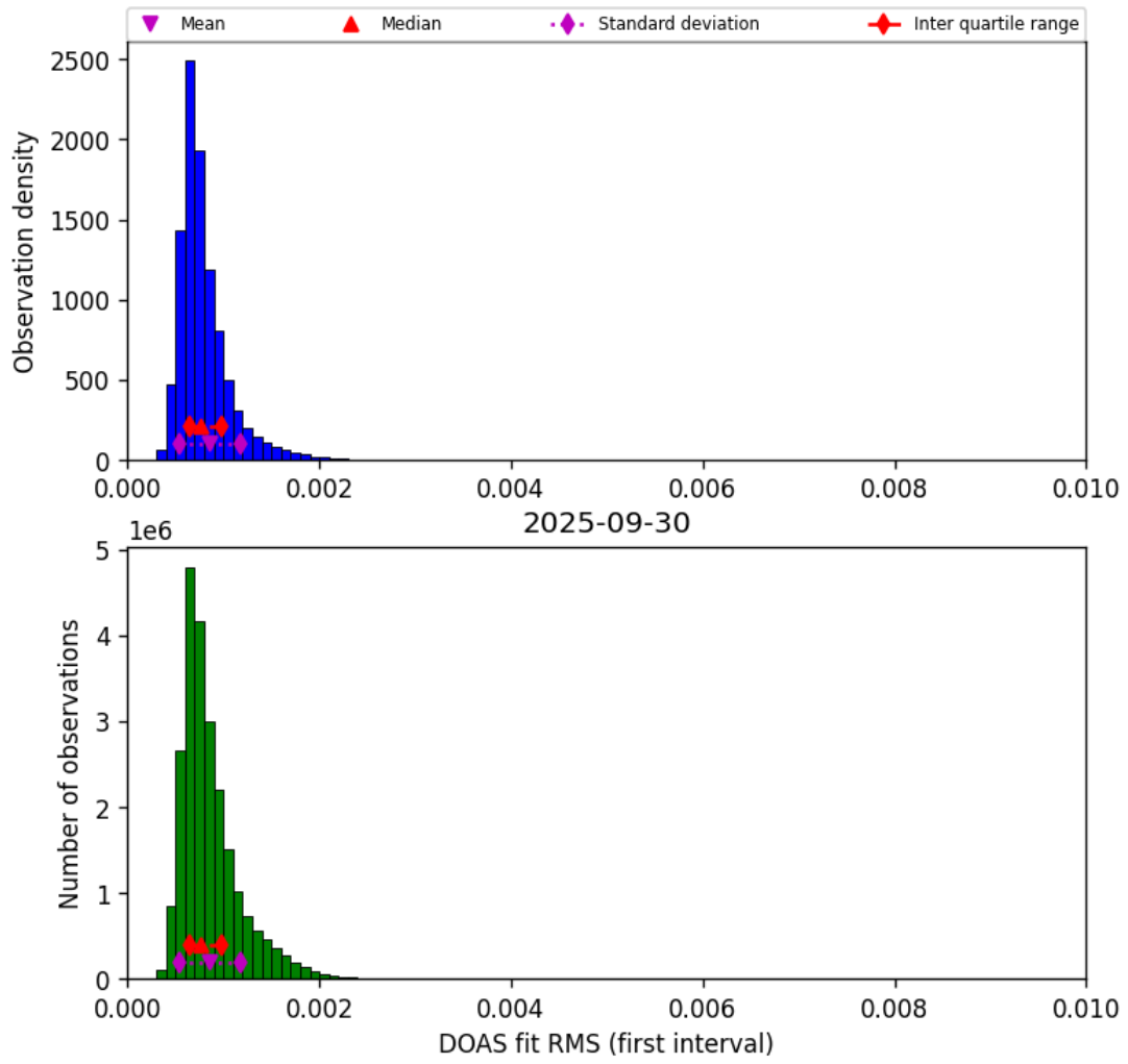
Figure 44: Histogram of “DOAS fit RMS (first interval)” for 2025-09-30 to 2025-10-01
