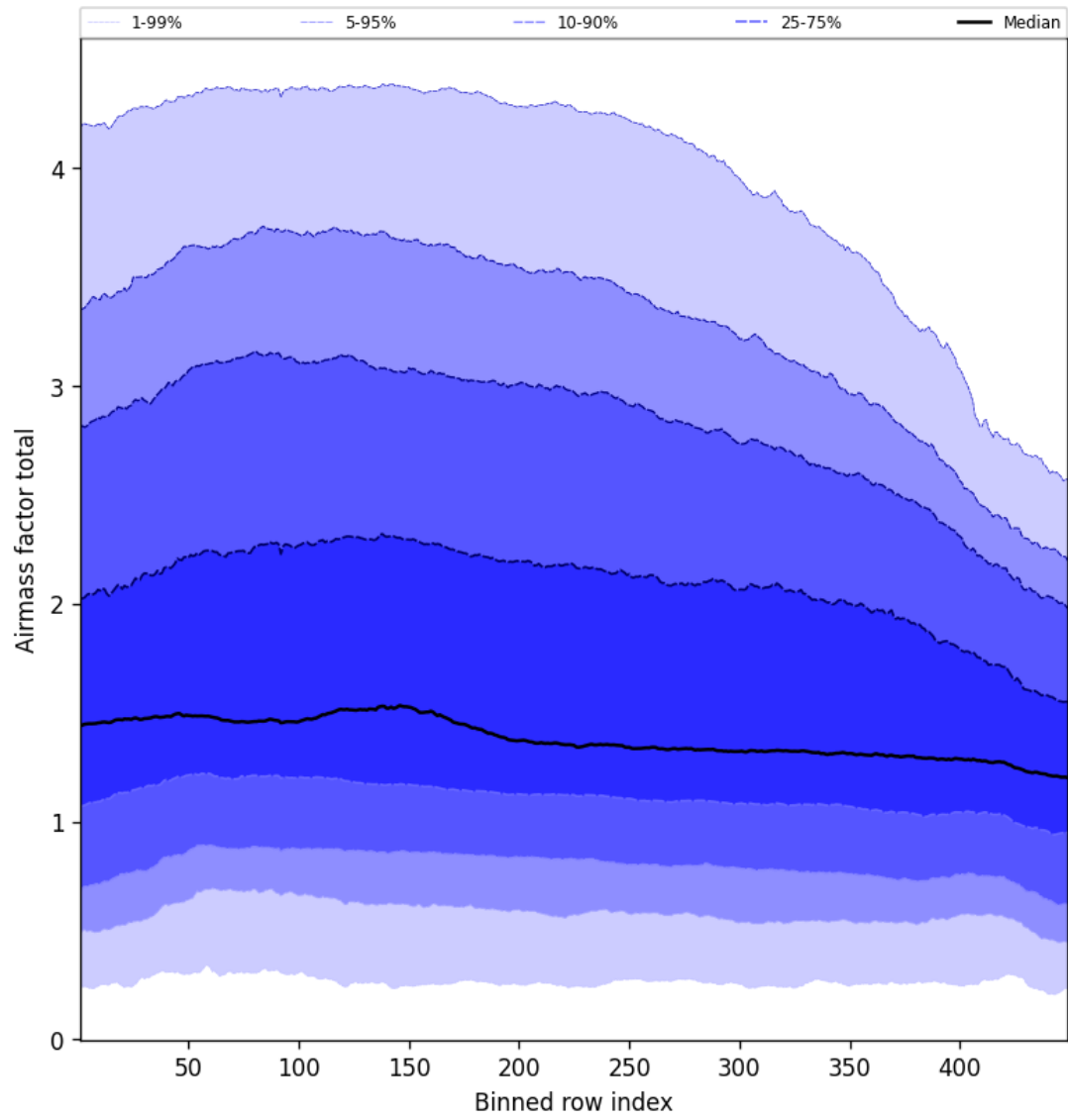
Figure 52: Along track statistics of “Airmass factor total” for 2025-09-30 to 2025-10-01
