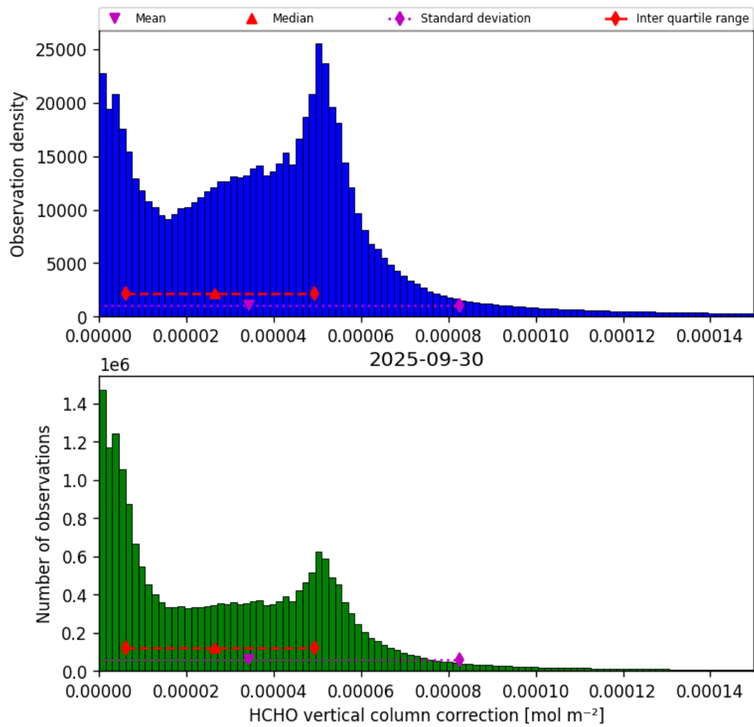
Figure 35: Histogram of “HCHO vertical column correction” for 2025-09-30 to 2025-10-01
