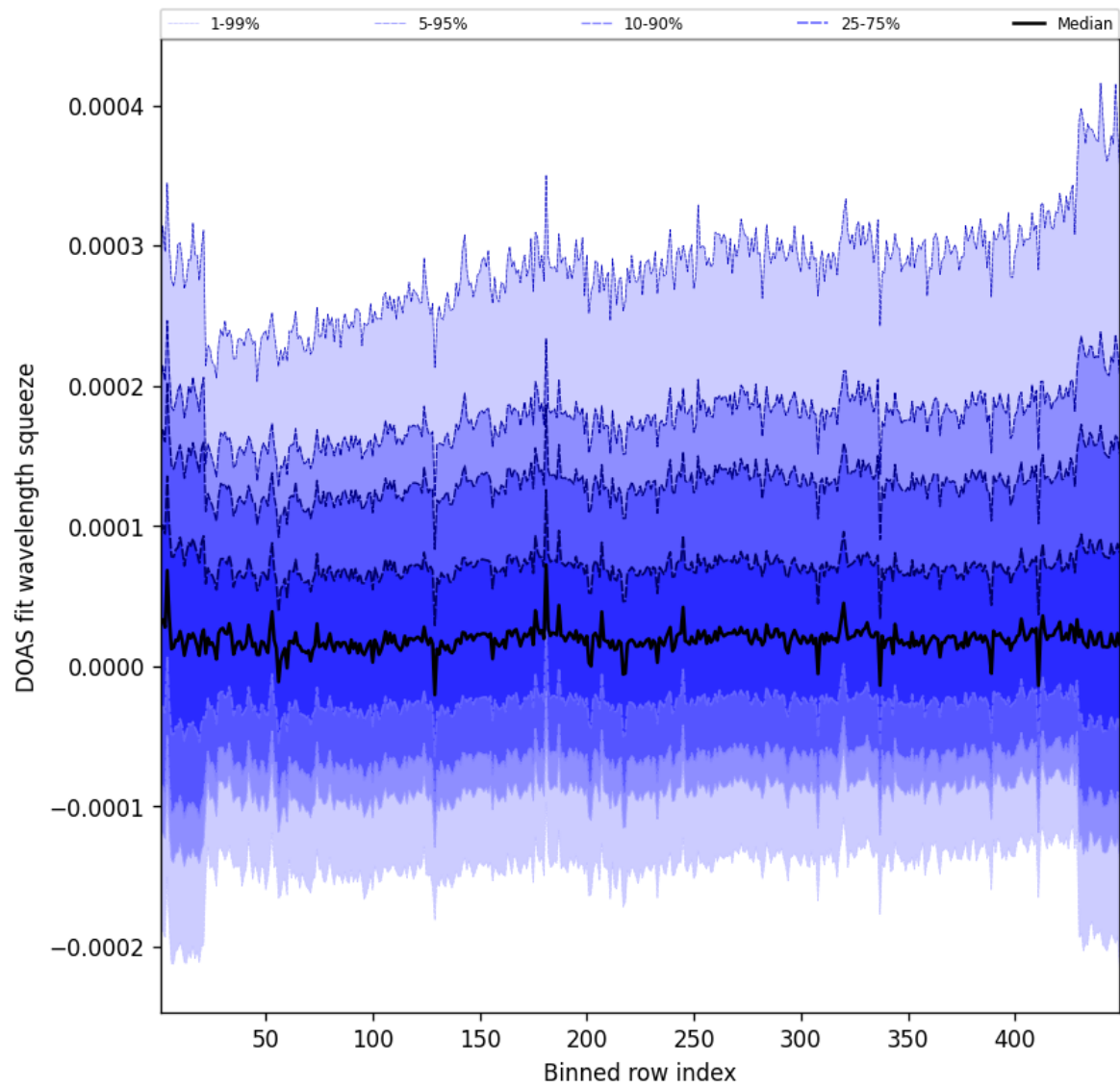
Figure 57: Along track statistics of “DOAS fit wavelength squeeze” for 2025-09-30 to 2025-10-01
