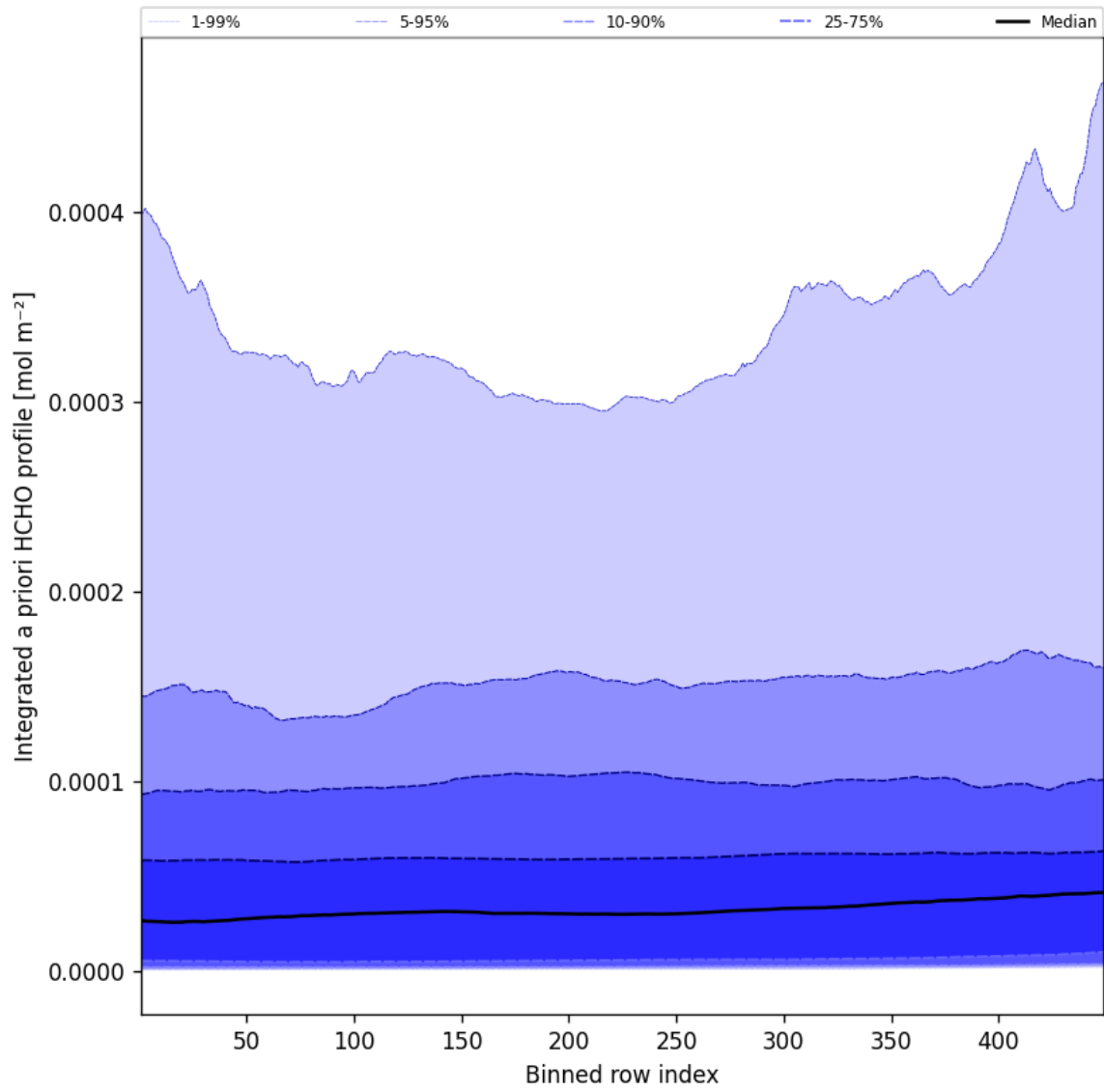
Figure 55: Along track statistics of “Integrated a priori HCHO profile” for 2025-09-30 to 2025-10-01
