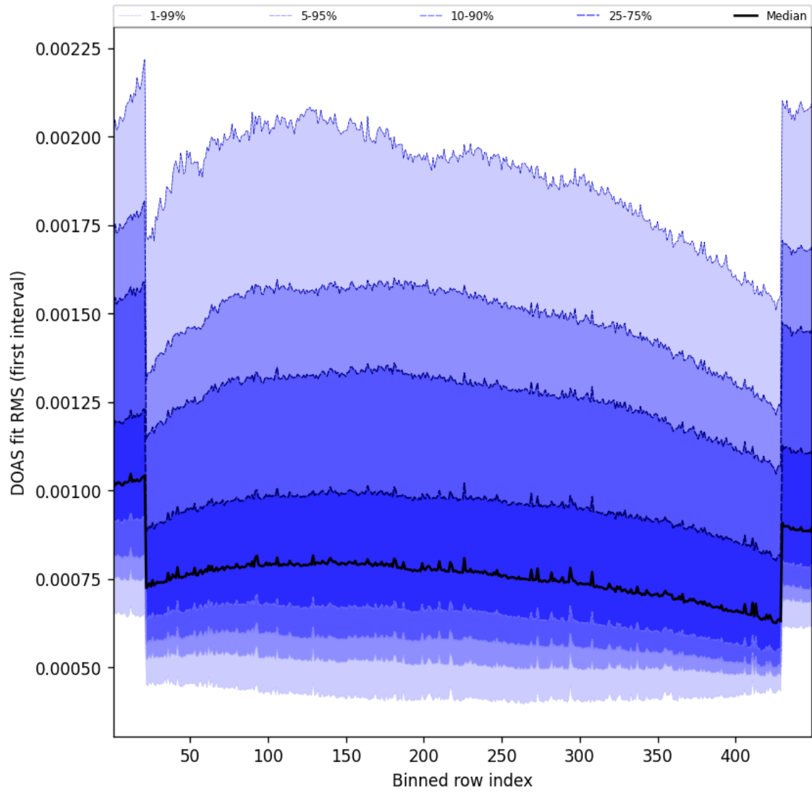
Figure 58: Along track statistics of “DOAS fit RMS (first interval)” for 2025-09-30 to 2025-10-01
