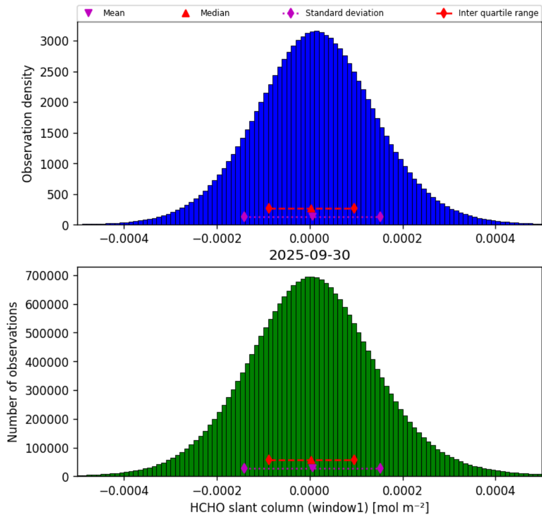
Figure 36: Histogram of “HCHO slant column (window1)” for 2025-09-30 to 2025-10-01
