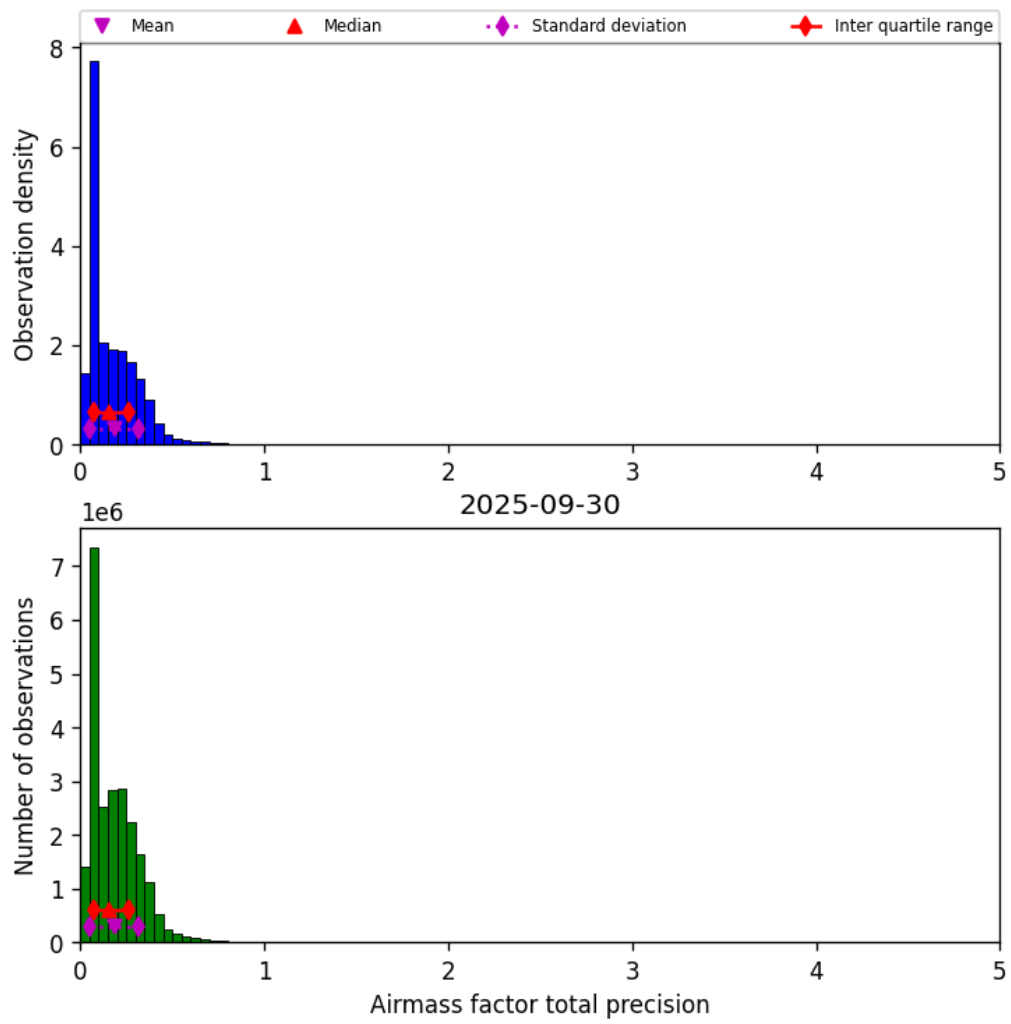
Figure 39: Histogram of “Airmass factor total precision” for 2025-09-30 to 2025-10-01
