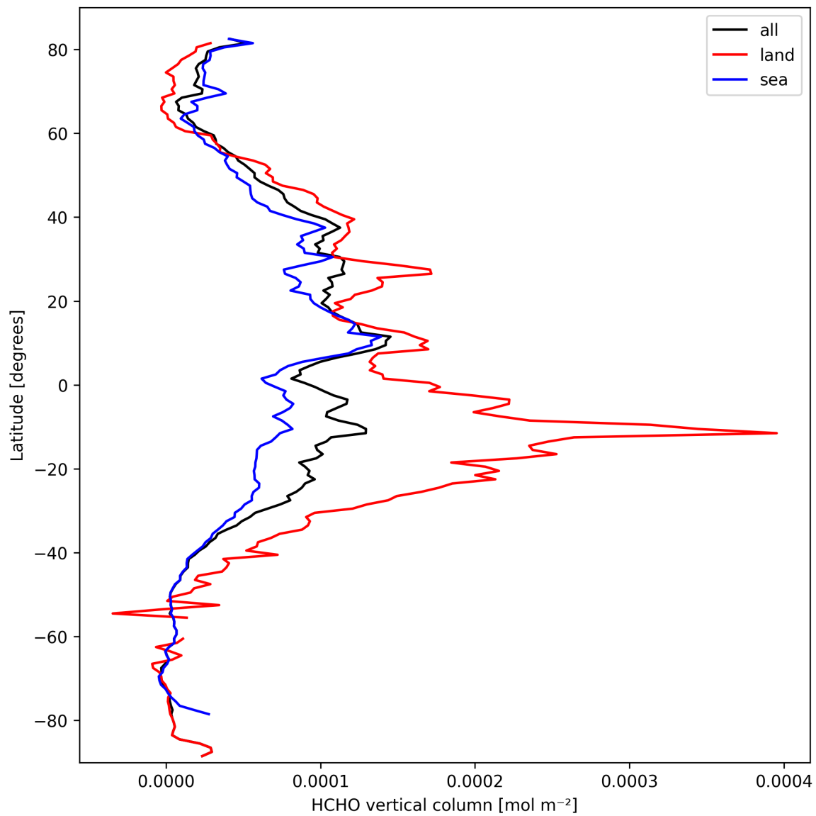
Figure 19: Zonal average of “HCHO vertical column” for 2025-09-30 to 2025-10-01.
