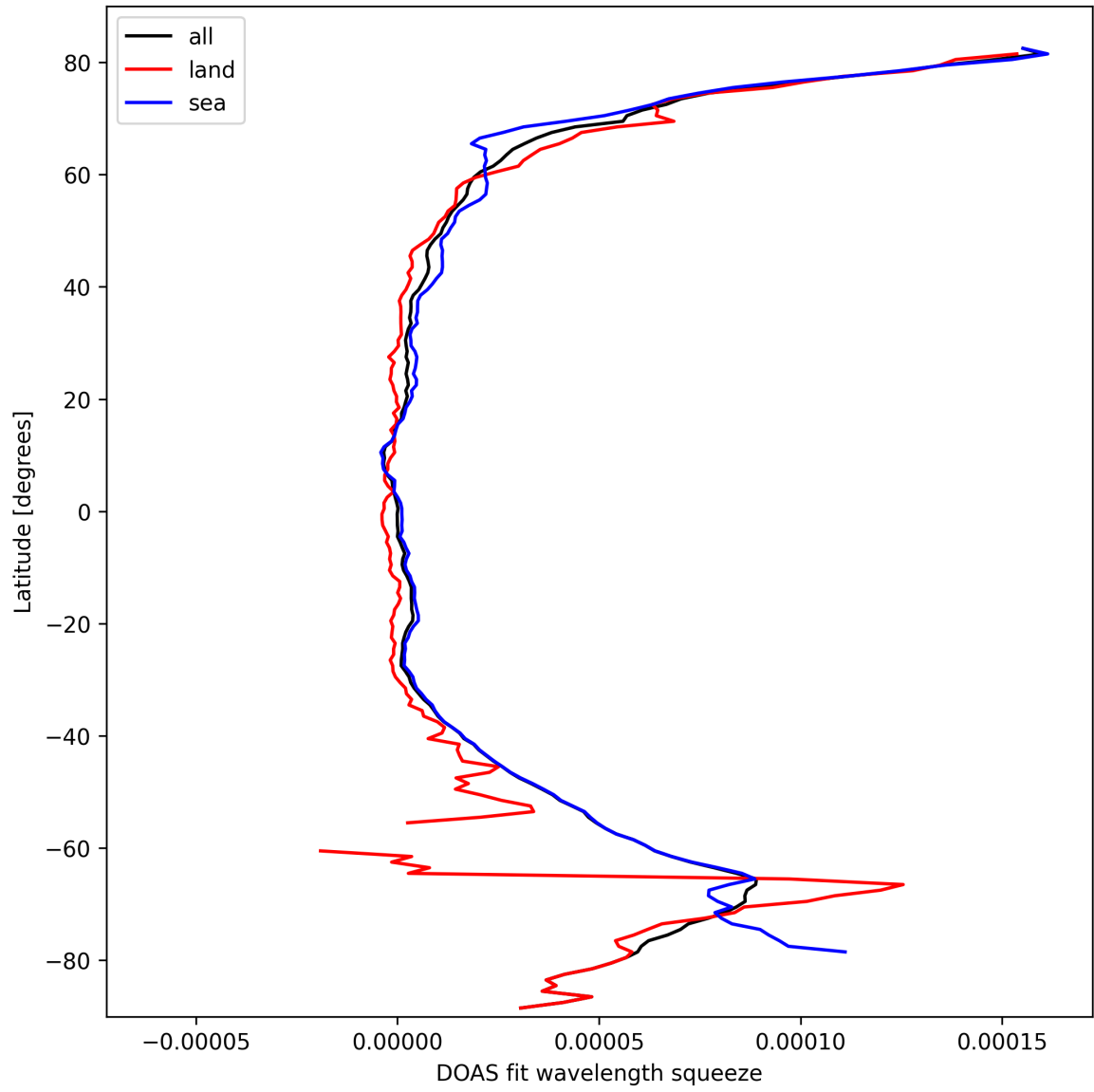
Figure 29: Zonal average of “DOAS fit wavelength squeeze” for 2025-09-30 to 2025-10-01.
