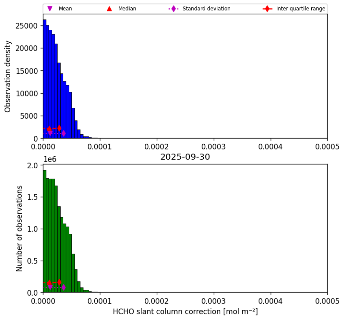
Figure 45: Histogram of “HCHO slant column correction” for 2025-09-30 to 2025-10-01
