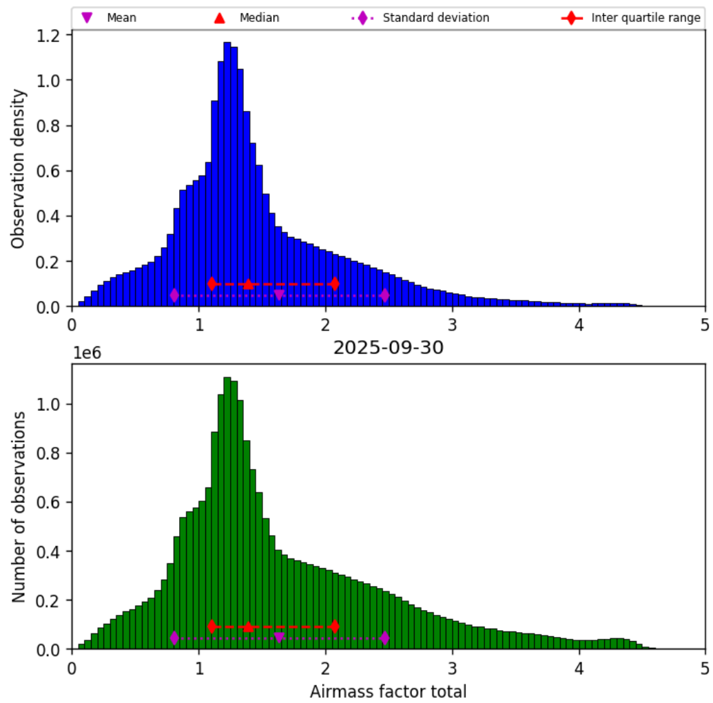
Figure 38: Histogram of “Airmass factor total” for 2025-09-30 to 2025-10-01
