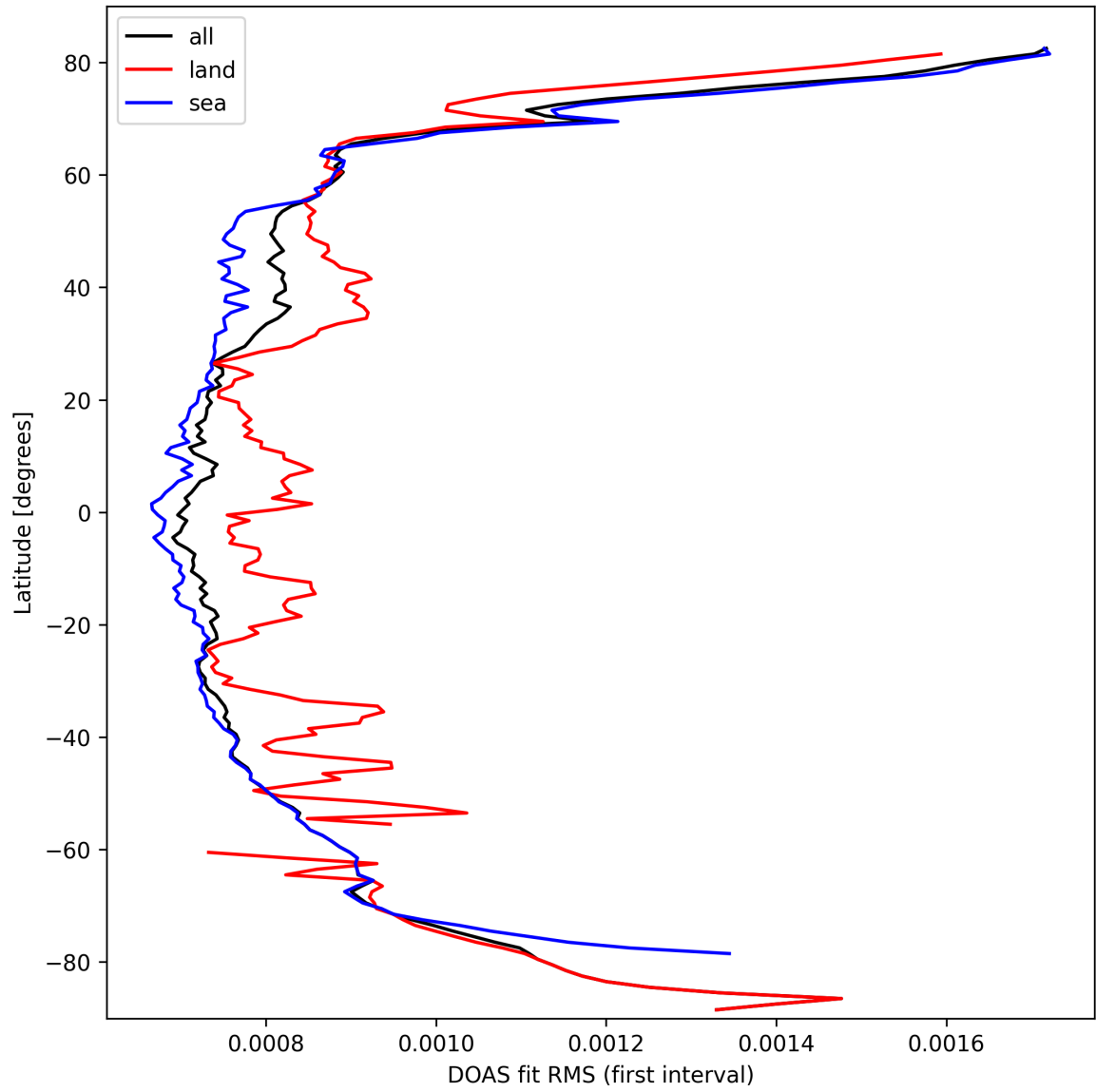
Figure 30: Zonal average of “DOAS fit RMS (first interval)” for 2025-09-30 to 2025-10-01.
