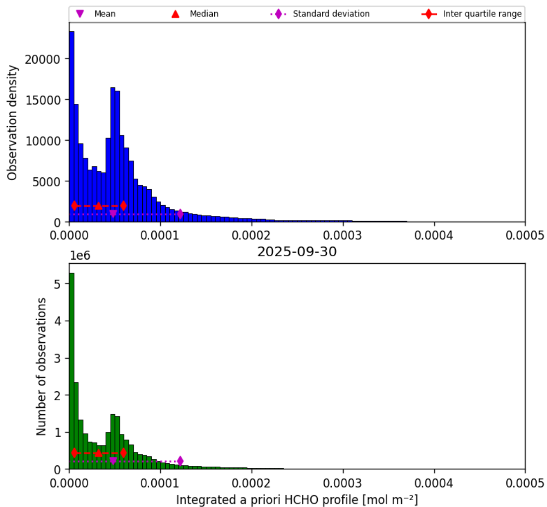
Figure 41: Histogram of “Integrated a priori HCHO profile” for 2025-09-30 to 2025-10-01
