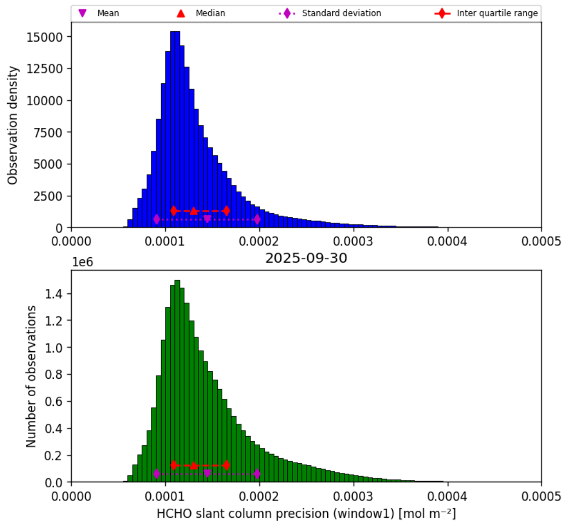
Figure 37: Histogram of “HCHO slant column precision (window1)” for 2025-09-30 to 2025-10-01
