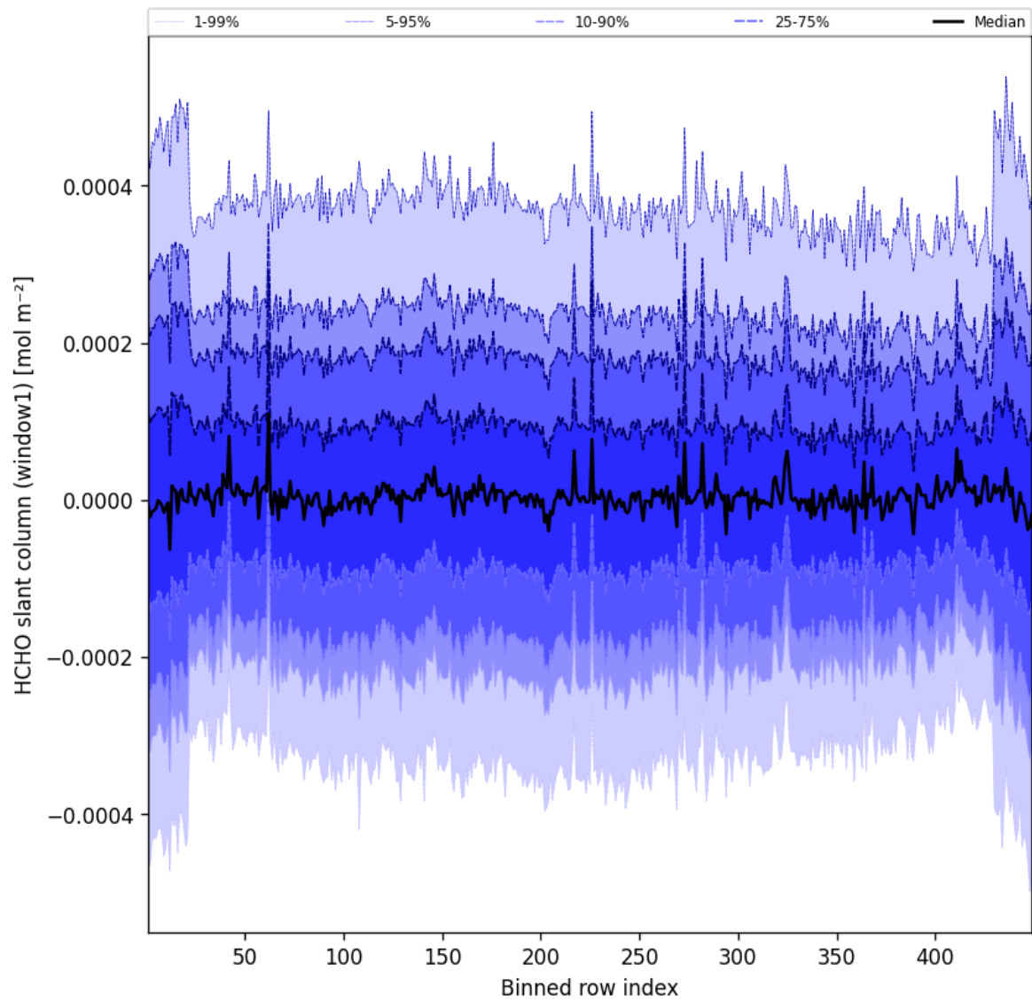
Figure 50: Along track statistics of “HCHO slant column (window1)” for 2025-09-30 to 2025-10-01
