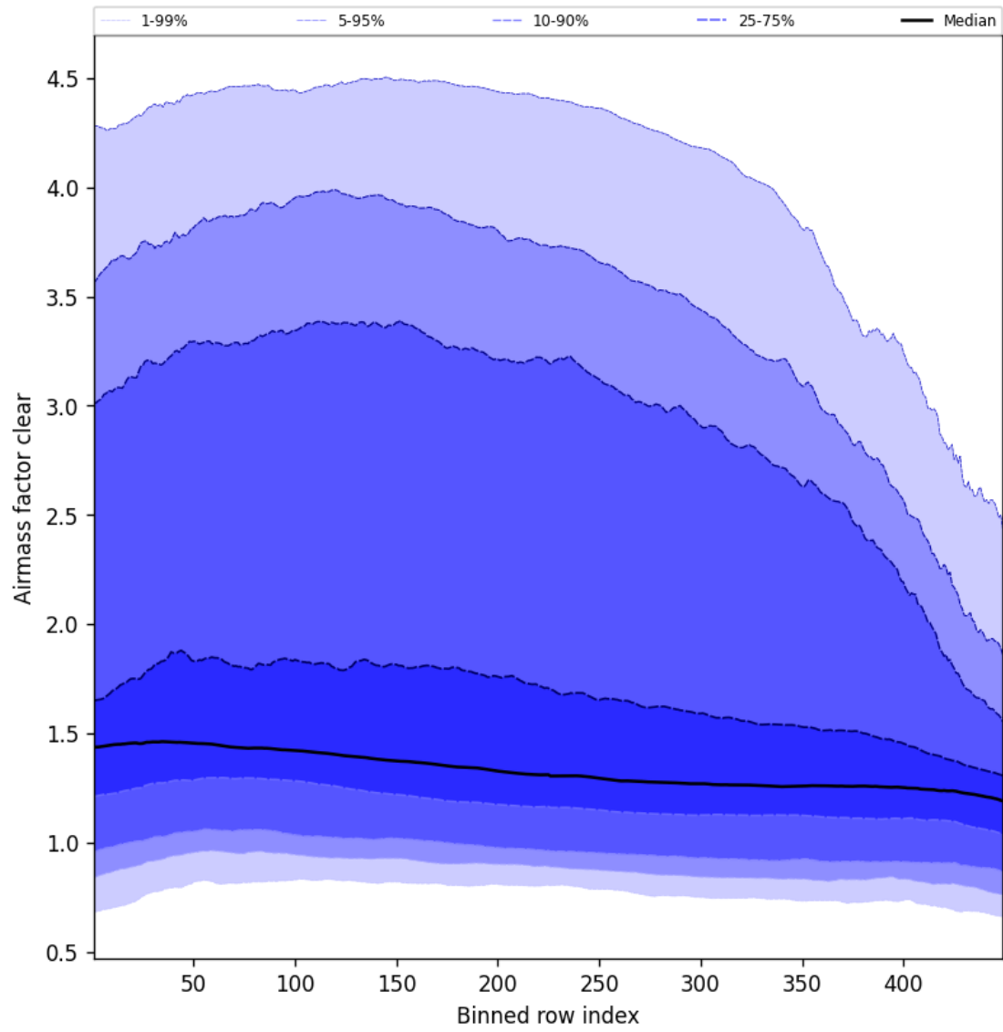
Figure 54: Along track statistics of “Airmass factor clear” for 2025-09-30 to 2025-10-01
