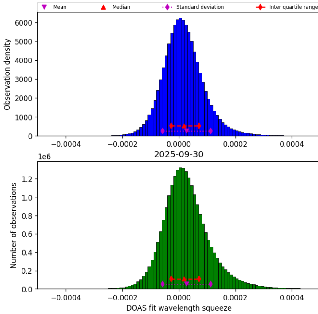
Figure 43: Histogram of “DOAS fit wavelength squeeze” for 2025-09-30 to 2025-10-01
