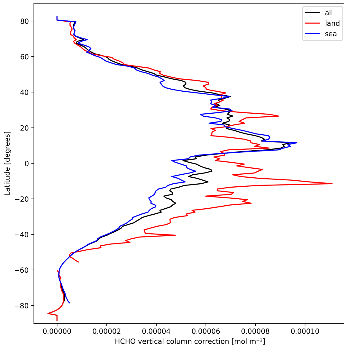
Figure 21: Zonal average of “HCHO vertical column correction” for 2025-09-30 to 2025-10-01.
