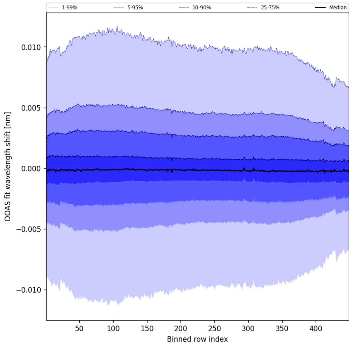
Figure 56: Along track statistics of “DOAS fit wavelength shift” for 2025-09-30 to 2025-10-01
