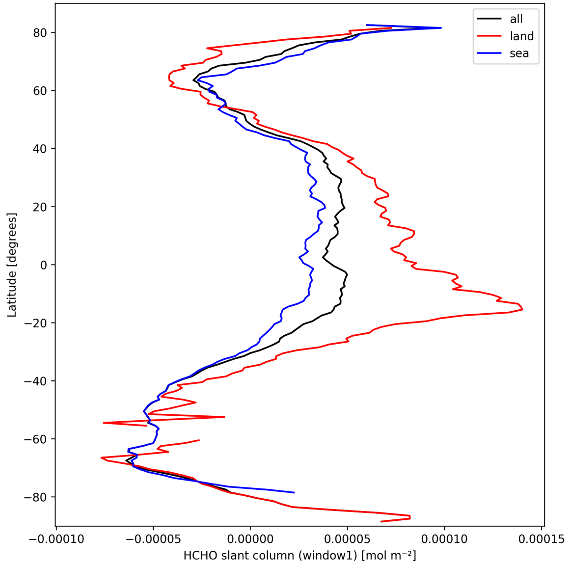
Figure 22: Zonal average of “HCHO slant column (window1)” for 2025-09-30 to 2025-10-01.
