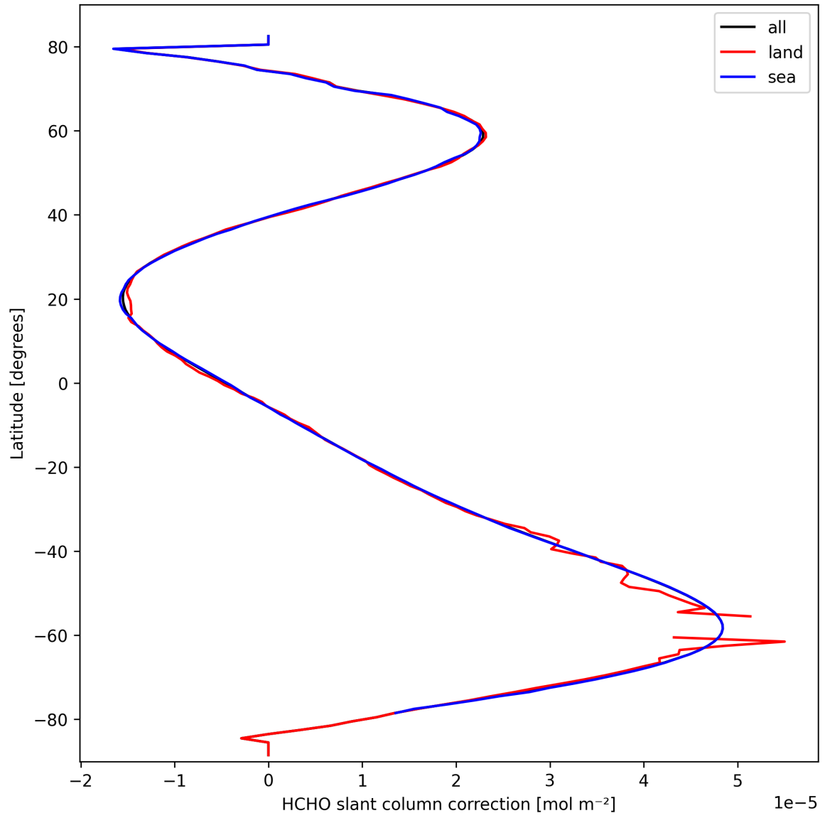
Figure 31: Zonal average of “HCHO slant column correction” for 2025-09-30 to 2025-10-01.
