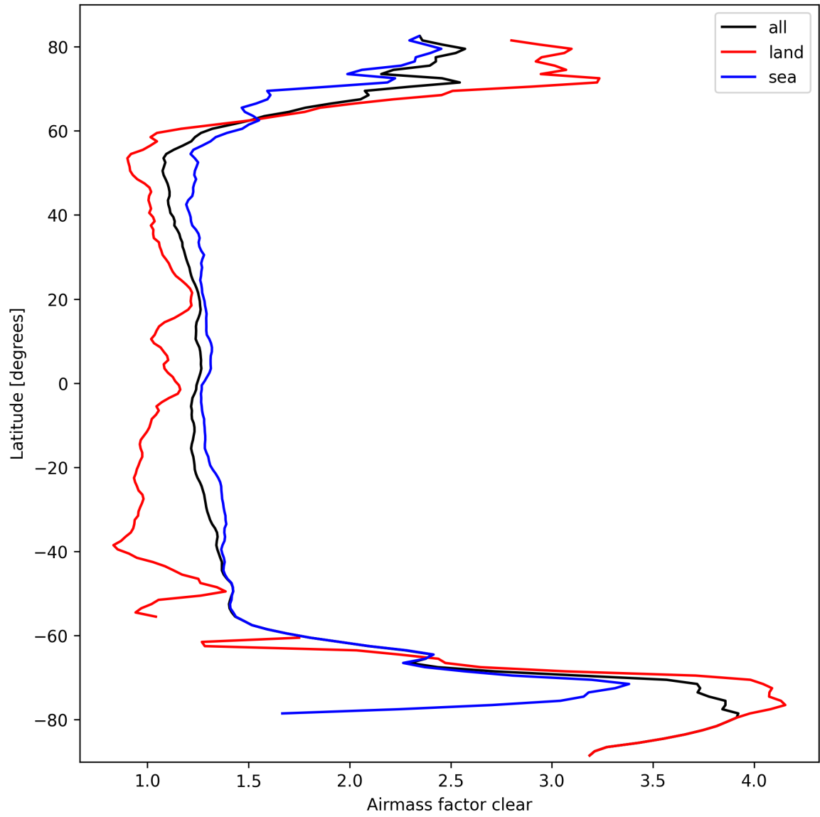
Figure 26: Zonal average of “Airmass factor clear” for 2025-09-30 to 2025-10-01.
