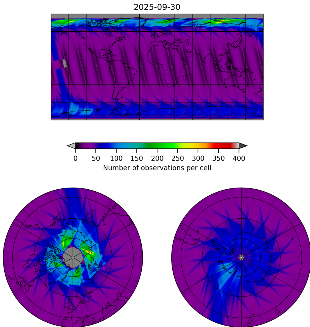
Figure 17: Map of the number of observations for 2025-09-30 to 2025-10-01
