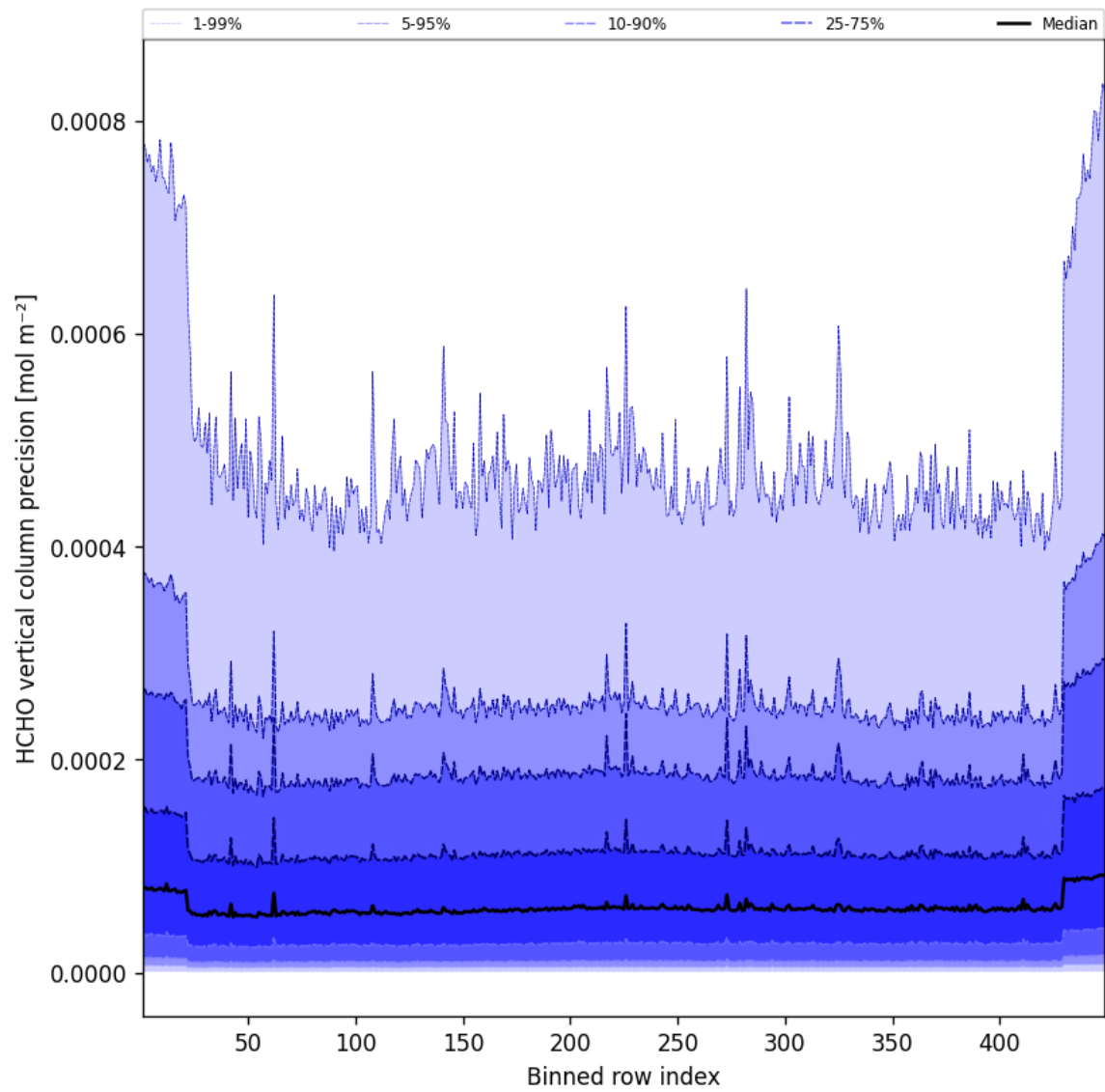
Figure 48: Along track statistics of “HCHO vertical column precision” for 2025-09-30 to 2025-10-01
