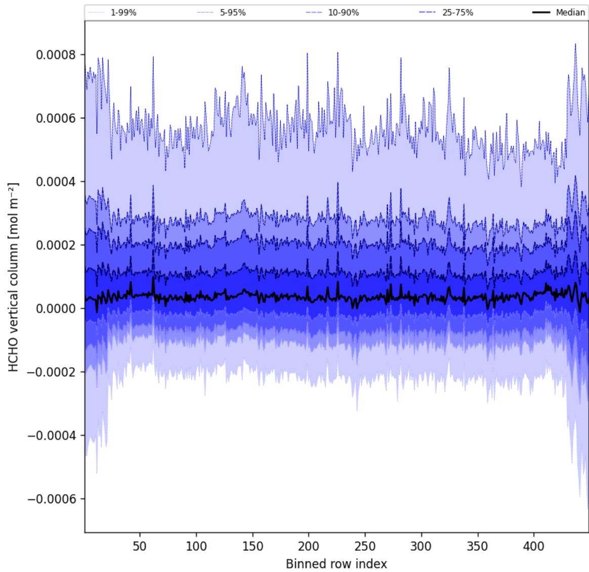
Figure 47: Along track statistics of “HCHO vertical column” for 2025-09-30 to 2025-10-01
