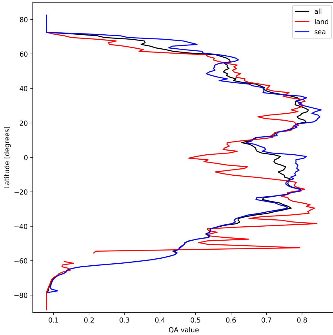
Figure 18: Zonal average of “QA value” for 2025-09-30 to 2025-10-01.
