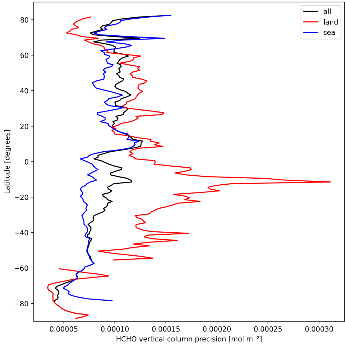
Figure 20: Zonal average of “HCHO vertical column precision” for 2025-09-30 to 2025-10-01.
