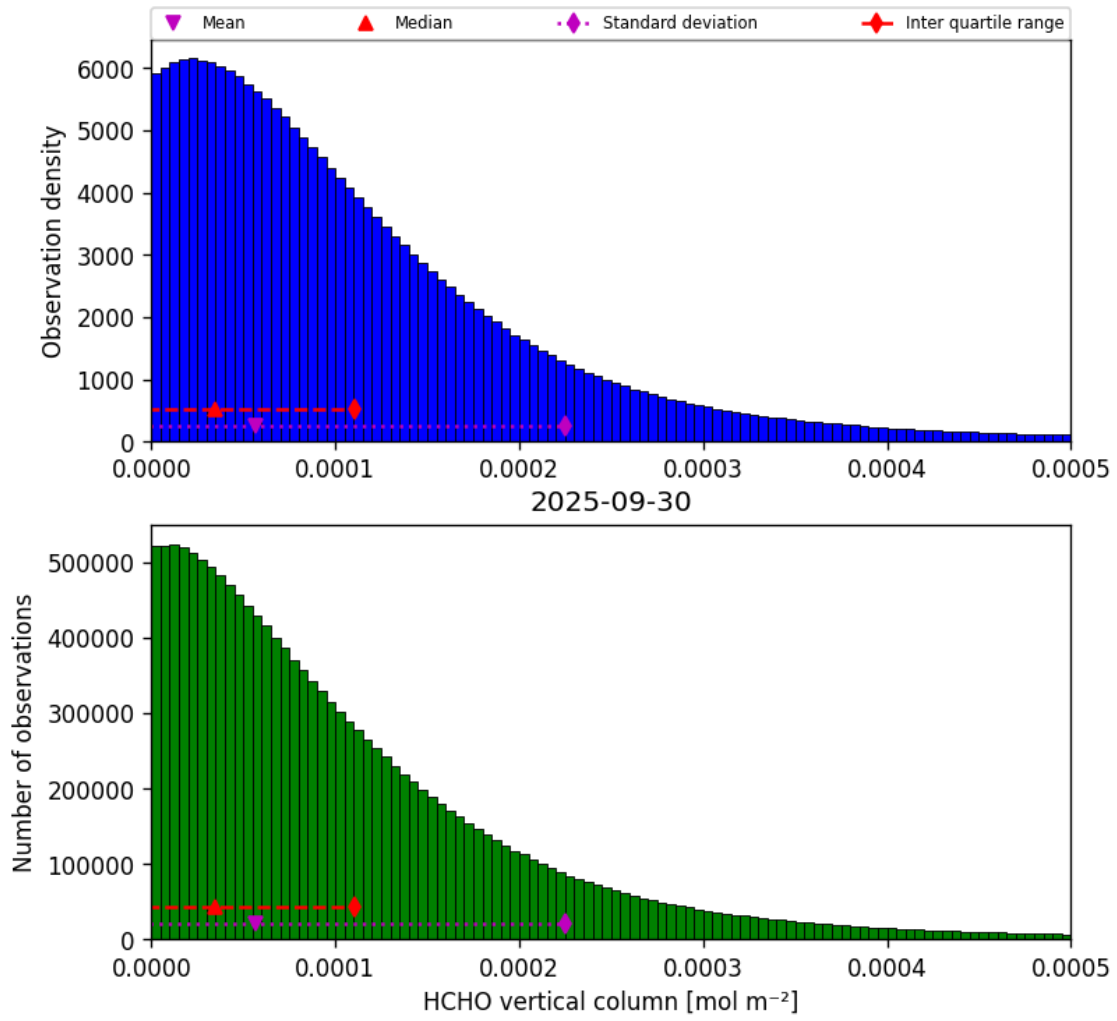
Figure 33: Histogram of “HCHO vertical column” for 2025-09-30 to 2025-10-01
