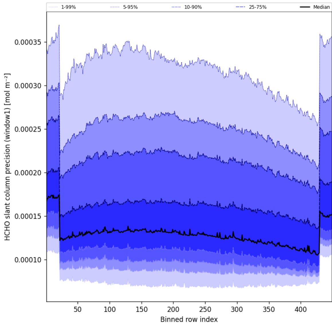
Figure 51: Along track statistics of “HCHO slant column precision (window1)” for 2025-09-30 to 2025-10-01
