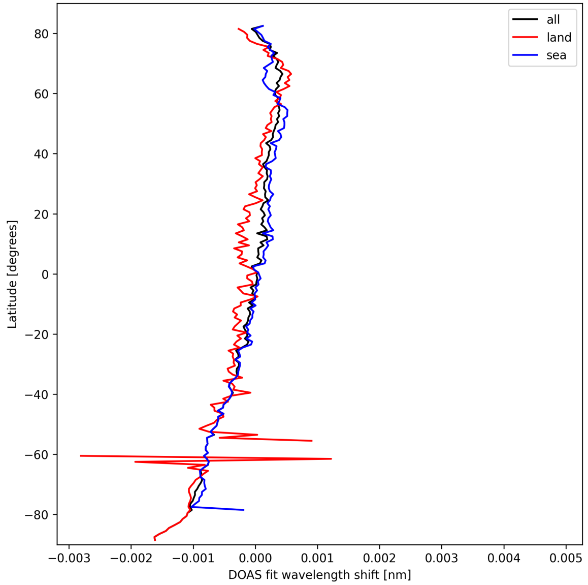
Figure 28: Zonal average of "DOAS fit wavelength shift" for 2025-09-30 to 2025-10-01.
