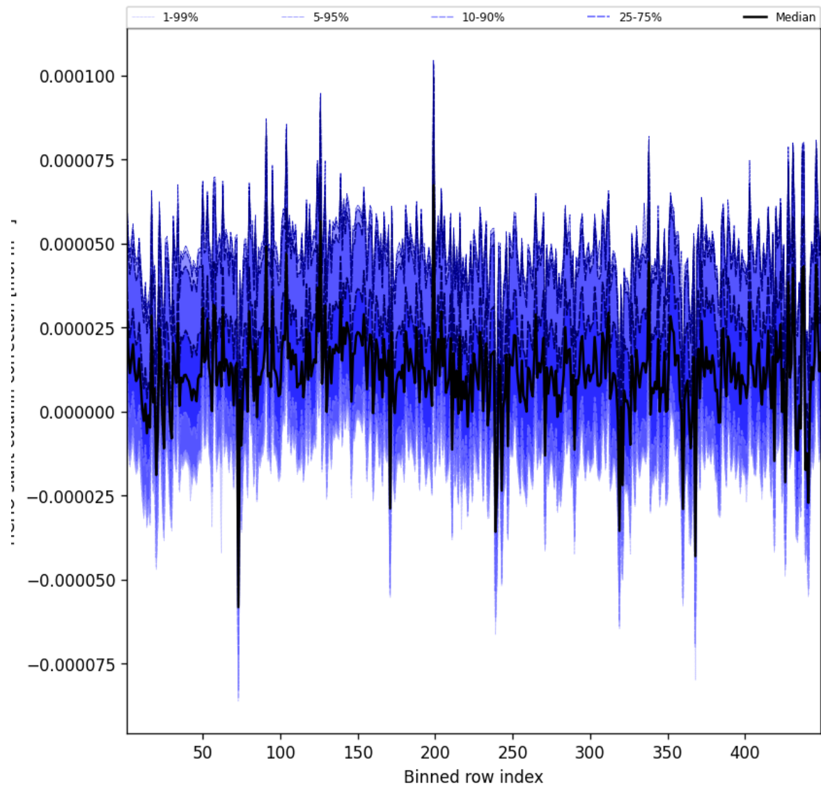
Figure 59: Along track statistics of “HCHO slant column correction” for 2025-09-30 to 2025-10-01
