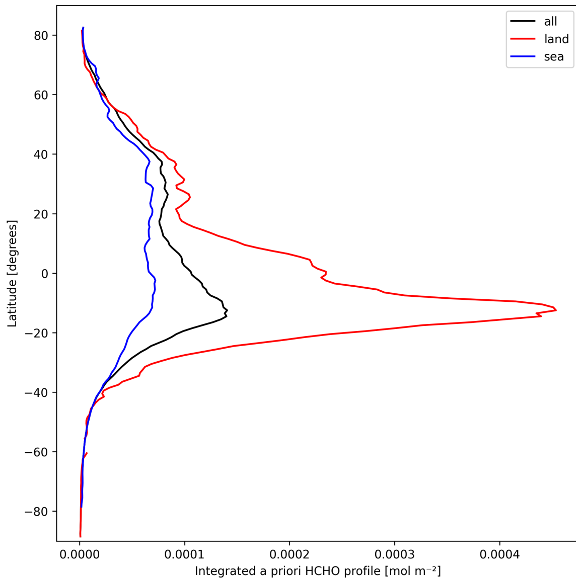
Figure 27: Zonal average of “Integrated a priori HCHO profile” for 2025-09-30 to 2025-10-01.
