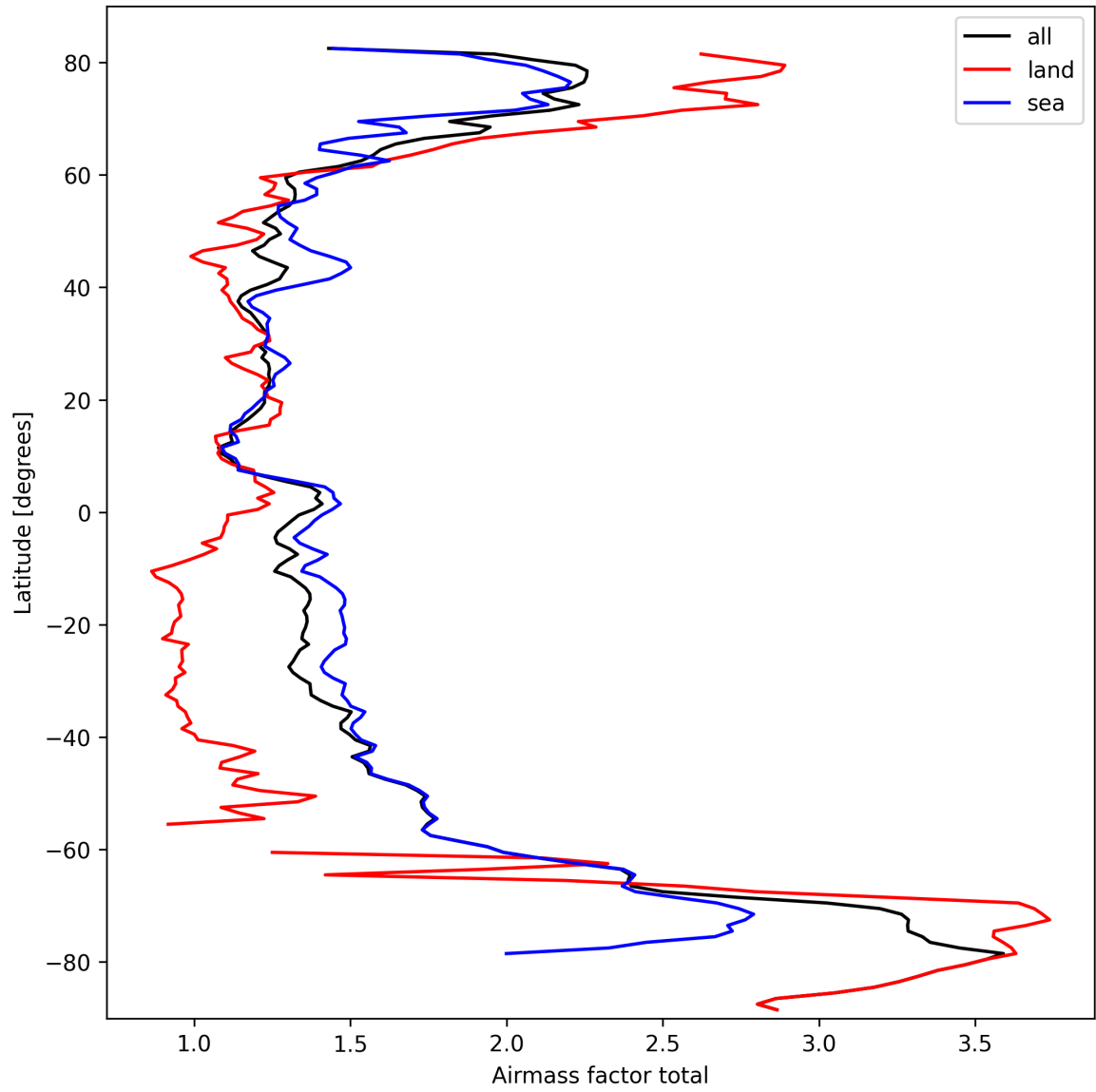
Figure 24: Zonal average of “Airmass factor total” for 2025-09-30 to 2025-10-01.
