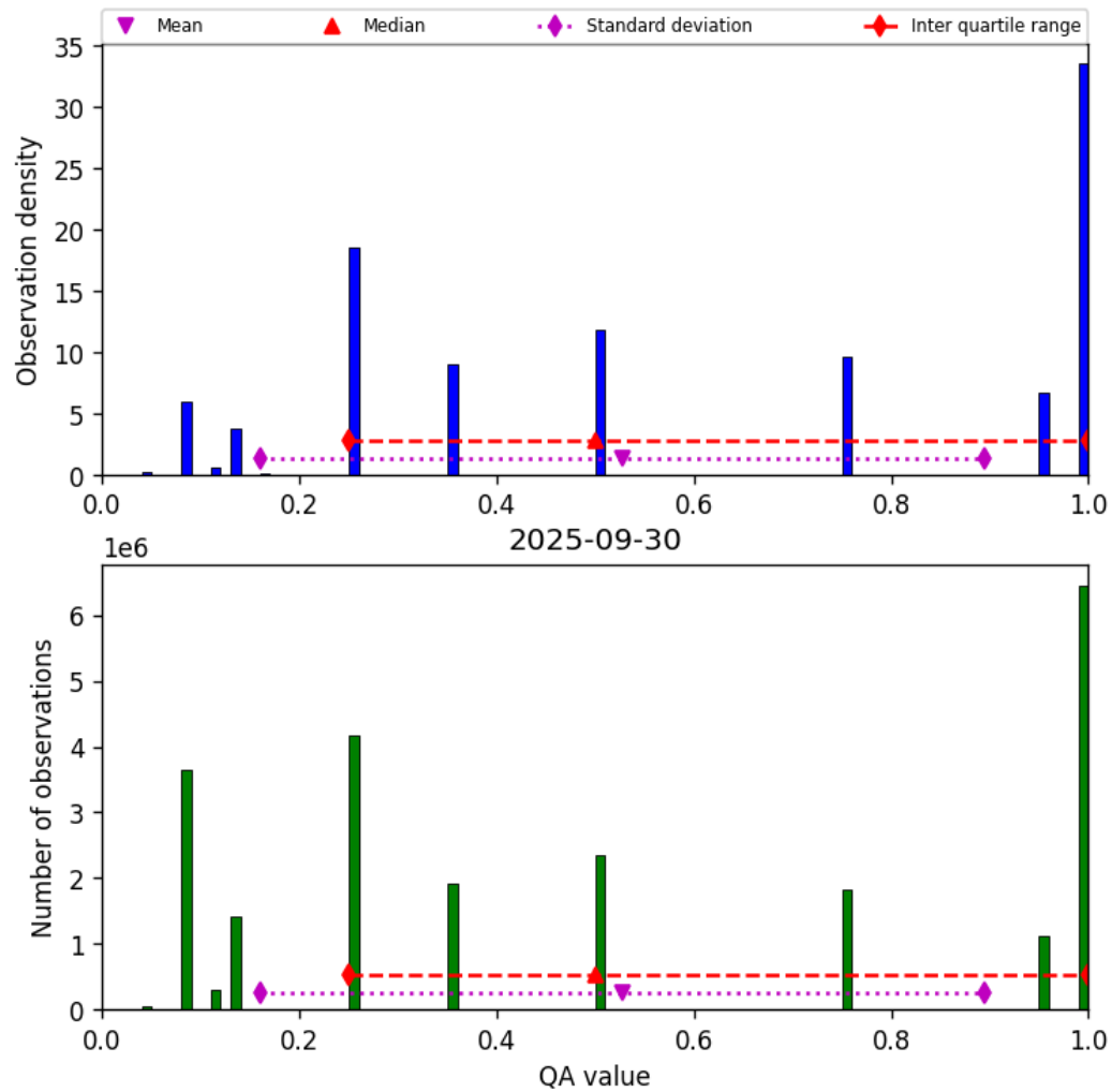
Figure 32: Histogram of “QA value” for 2025-09-30 to 2025-10-01
