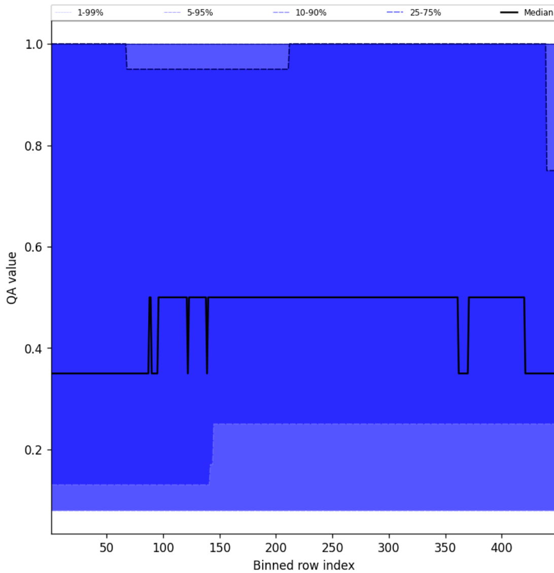
Figure 46: Along track statistics of “QA value” for 2025-09-30 to 2025-10-01
