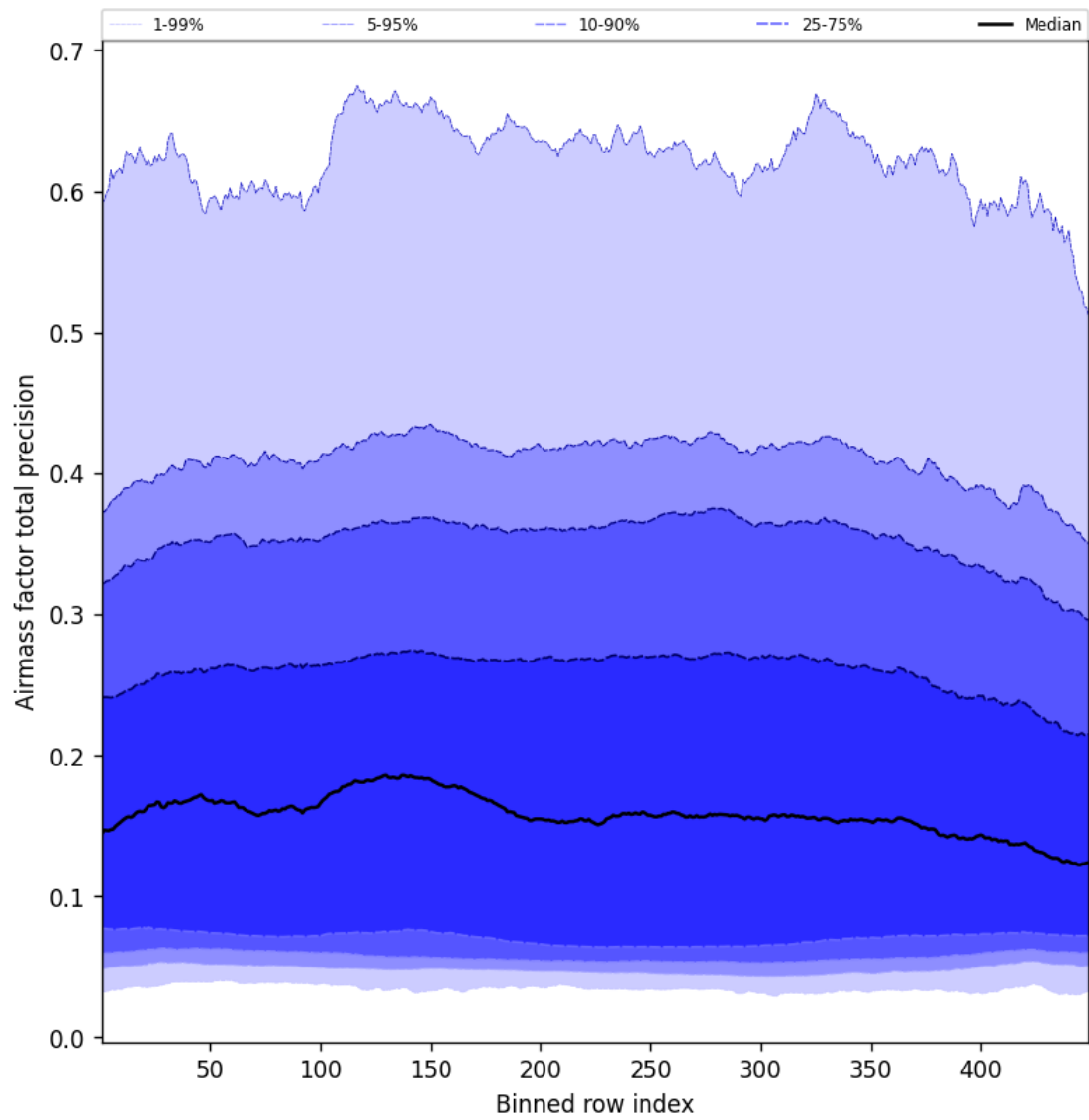
Figure 53: Along track statistics of “Airmass factor total precision” for 2025-09-30 to 2025-10-01
