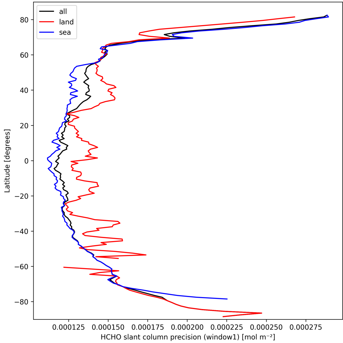
Figure 23: Zonal average of “HCHO slant column precision (window1)” for 2025-09-30 to 2025-10-01.
