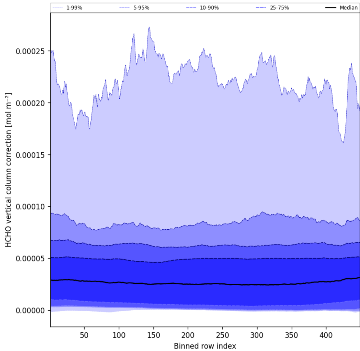
Figure 49: Along track statistics of “HCHO vertical column correction” for 2025-09-30 to 2025-10-01
