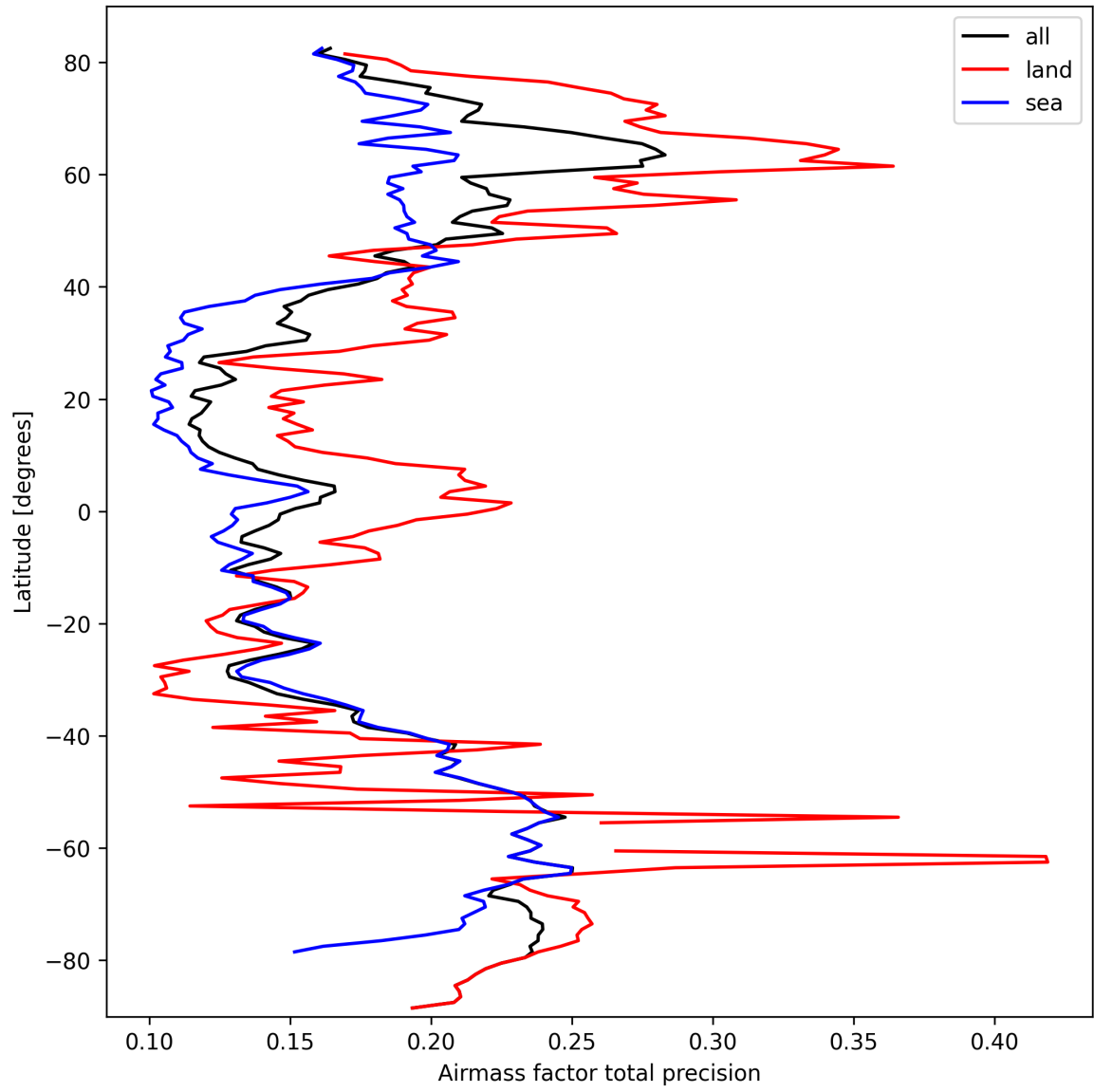
Figure 25: Zonal average of “Airmass factor total precision” for 2025-09-30 to 2025-10-01.
