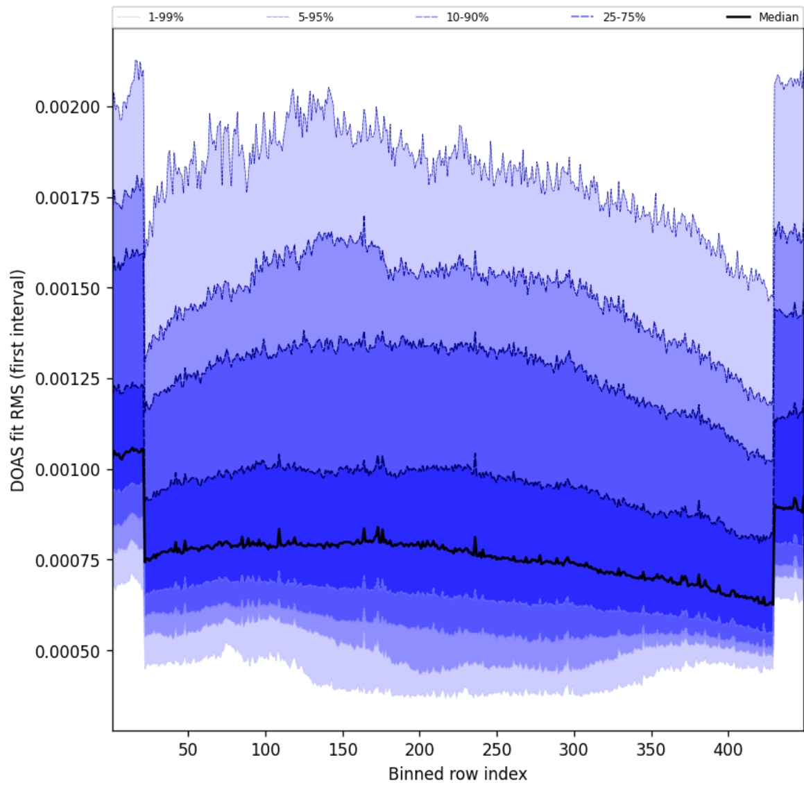
Figure 58: Along track statistics of “DOAS fit RMS (first interval)” for 2025-10-02 to 2025-10-03
