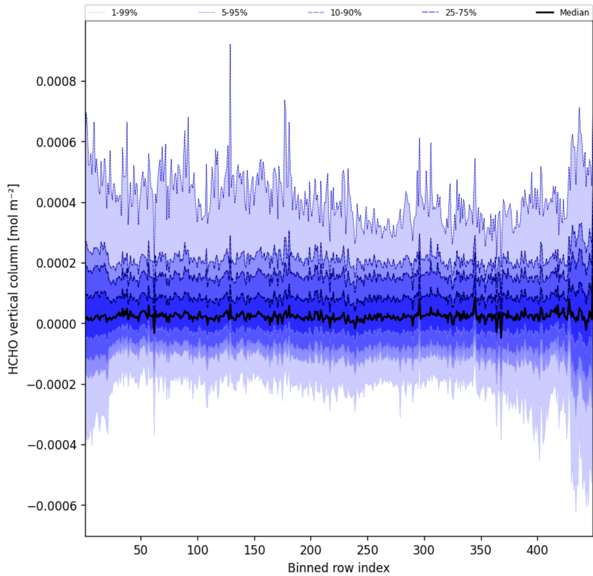
Figure 47: Along track statistics of “HCHO vertical column” for 2025-10-02 to 2025-10-03
