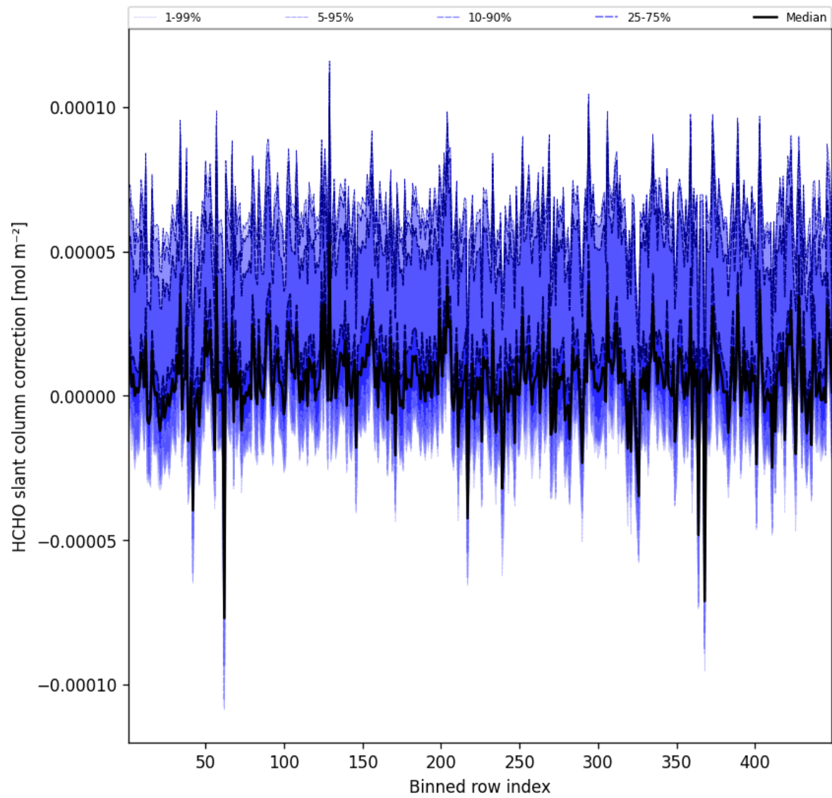
Figure 59: Along track statistics of “HCHO slant column correction” for 2025-10-02 to 2025-10-03
