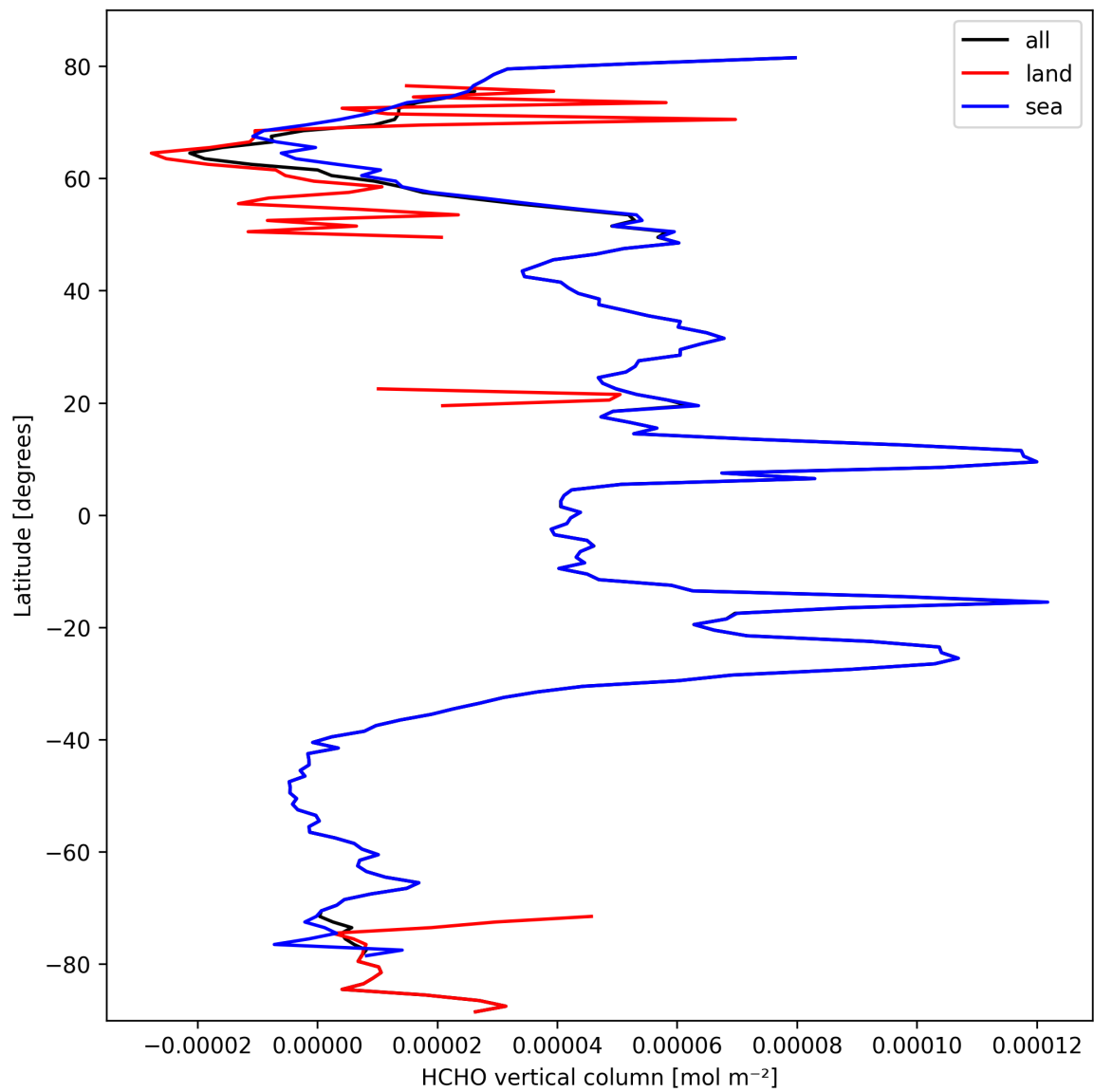
Figure 19: Zonal average of “HCHO vertical column” for 2025-10-02 to 2025-10-03.
