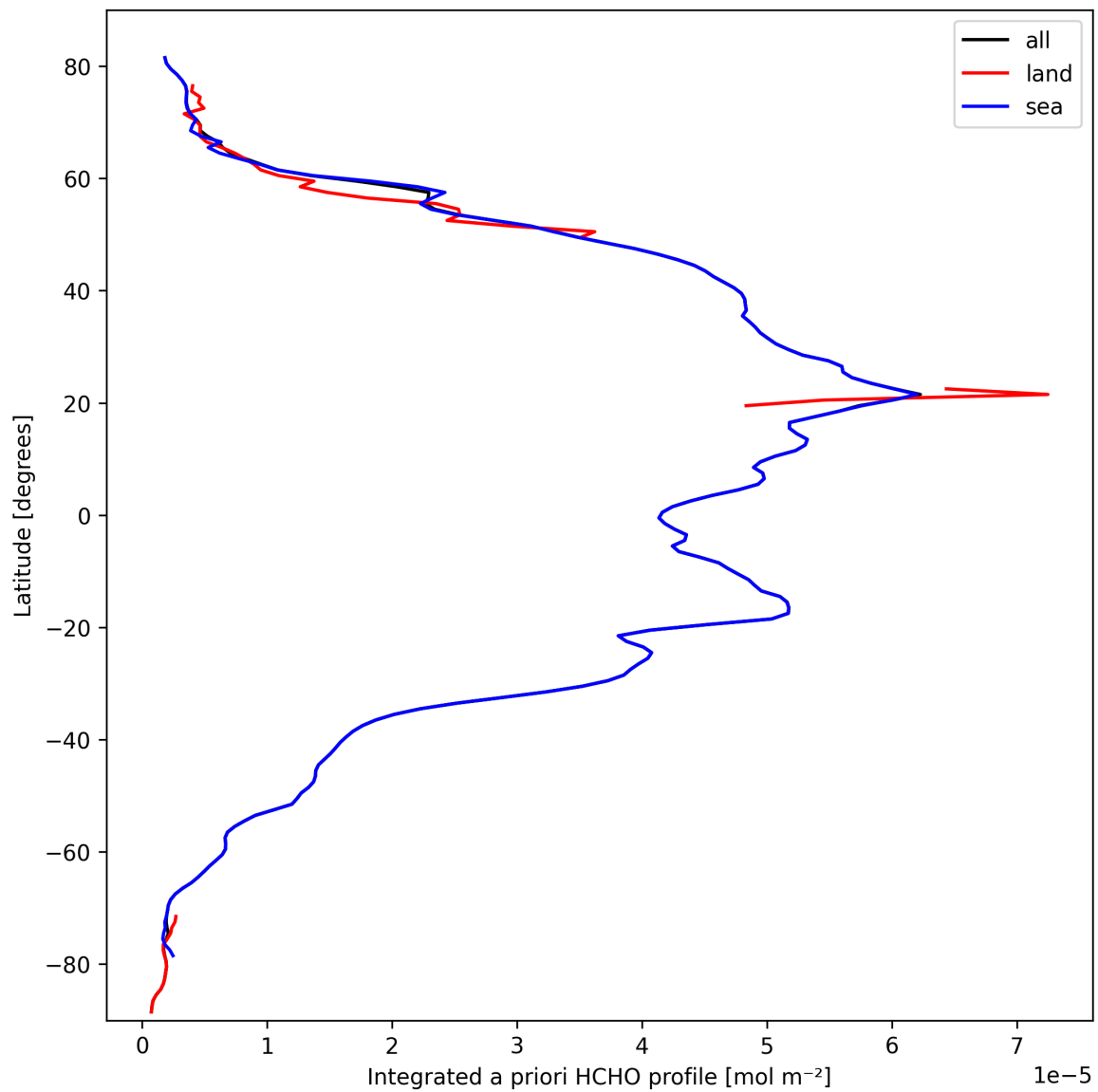
Figure 27: Zonal average of “Integrated a priori HCHO profile” for 2025-10-02 to 2025-10-03.
