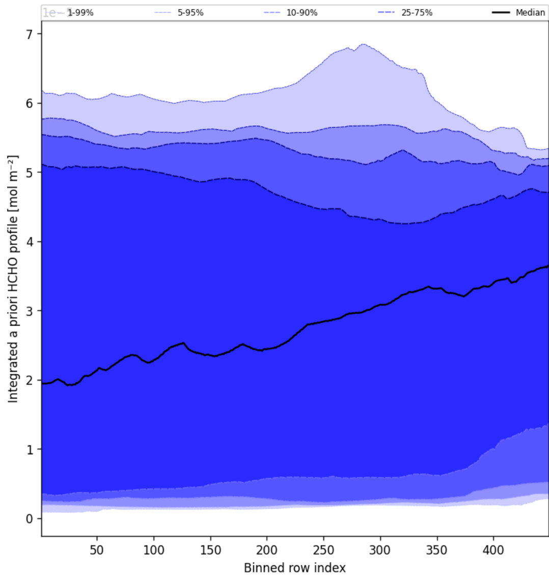
Figure 55: Along track statistics of “Integrated a priori HCHO profile” for 2025-10-02 to 2025-10-03
