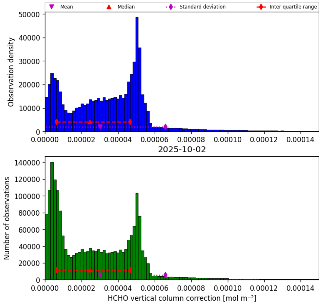
Figure 35: Histogram of “HCHO vertical column correction” for 2025-10-02 to 2025-10-03
