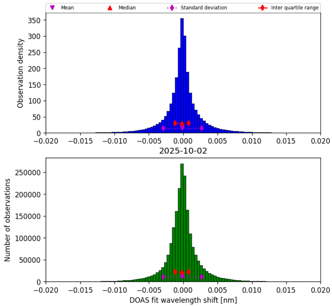
Figure 42: Histogram of “DOAS fit wavelength shift” for 2025-10-02 to 2025-10-03
