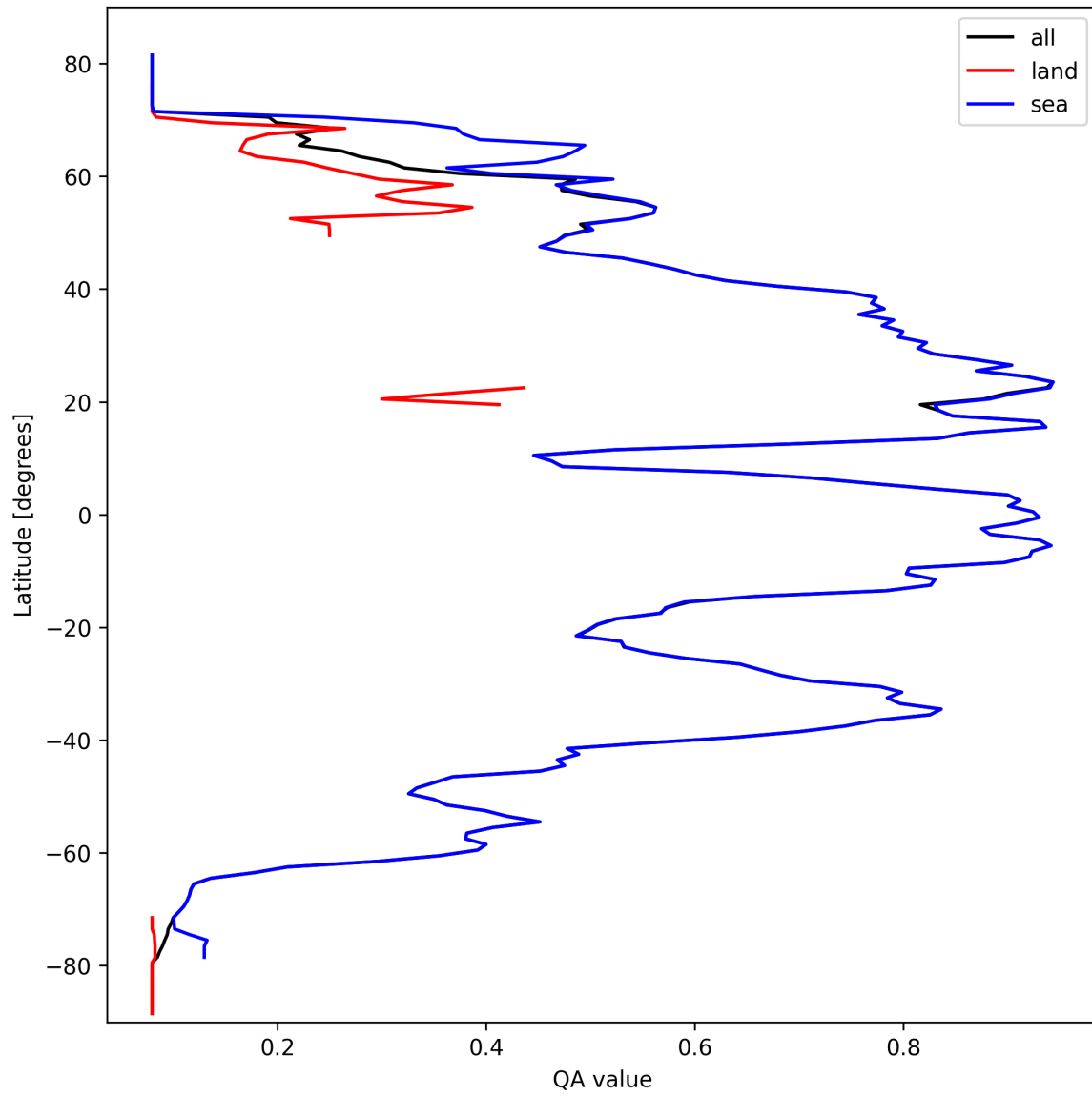
Figure 18: Zonal average of "QA value" for 2025-10-02 to 2025-10-03.
