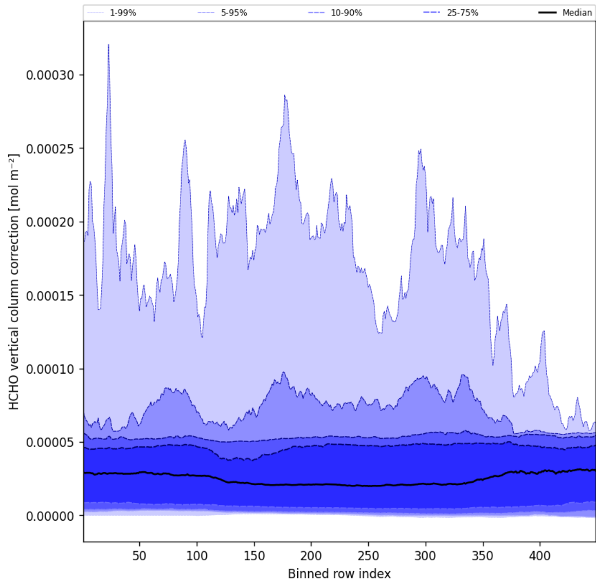
Figure 49: Along track statistics of "HCHO vertical column correction" for 2025-10-02 to 2025-10-03
