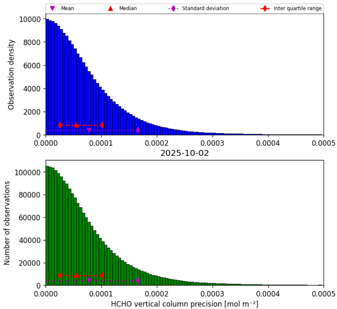
Figure 34: Histogram of “HCHO vertical column precision” for 2025-10-02 to 2025-10-03
