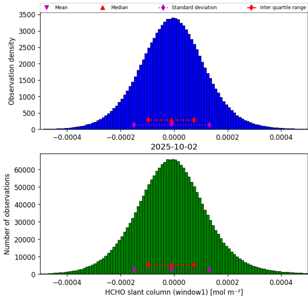
Figure 36: Histogram of “HCHO slant column (window1)” for 2025-10-02 to 2025-10-03
