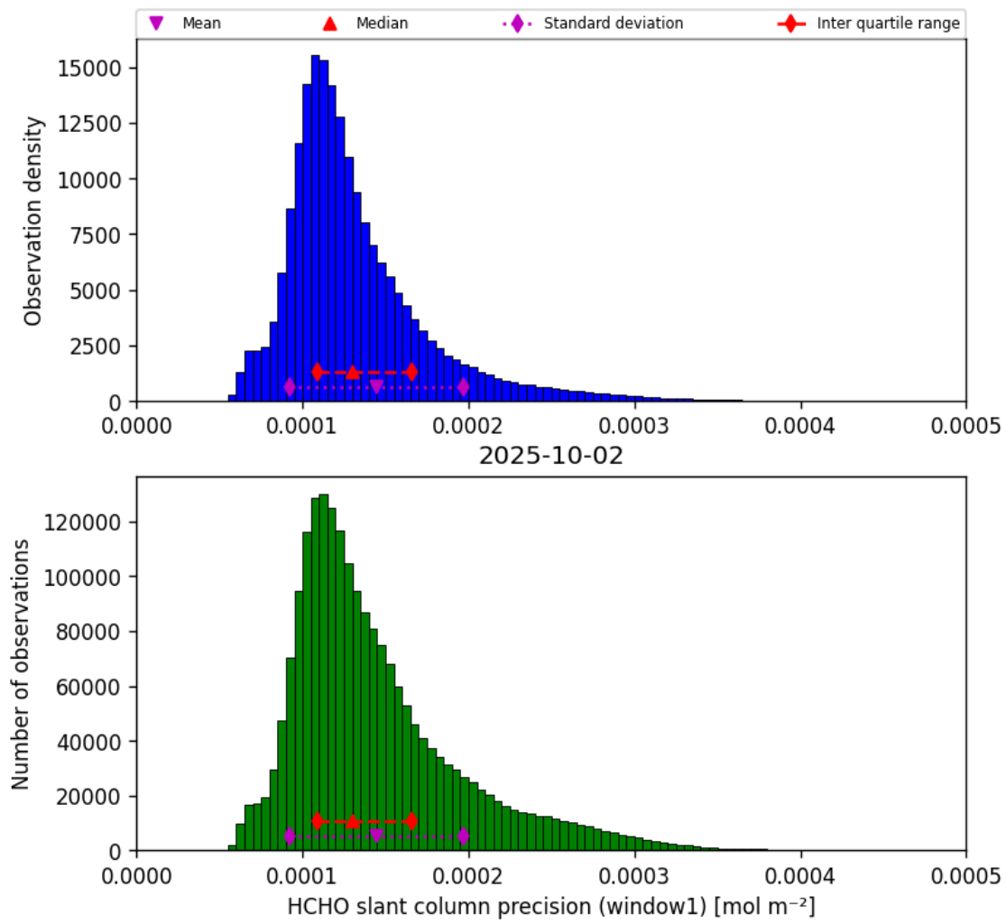
Figure 37: Histogram of “HCHO slant column precision (window1)” for 2025-10-02 to 2025-10-03
