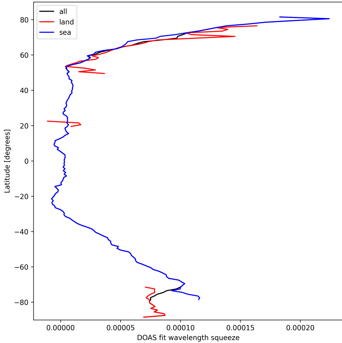
Figure 29: Zonal average of “DOAS fit wavelength squeeze” for 2025-10-02 to 2025-10-03.
