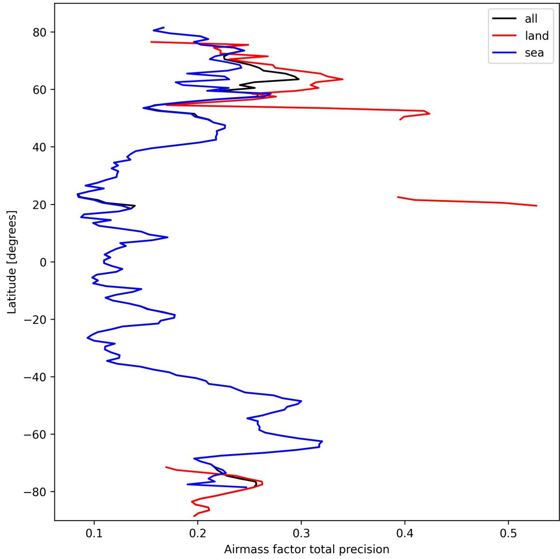
Figure 25: Zonal average of “Airmass factor total precision” for 2025-10-02 to 2025-10-03.
