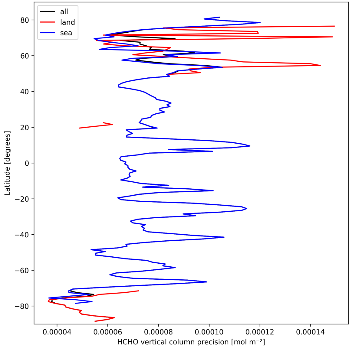
Figure 20: Zonal average of “HCHO vertical column precision” for 2025-10-02 to 2025-10-03.
