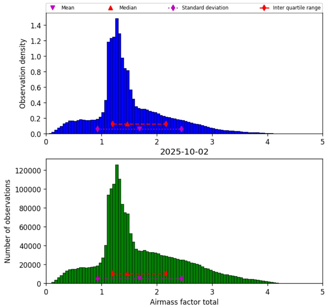
Figure 38: Histogram of “Airmass factor total” for 2025-10-02 to 2025-10-03
