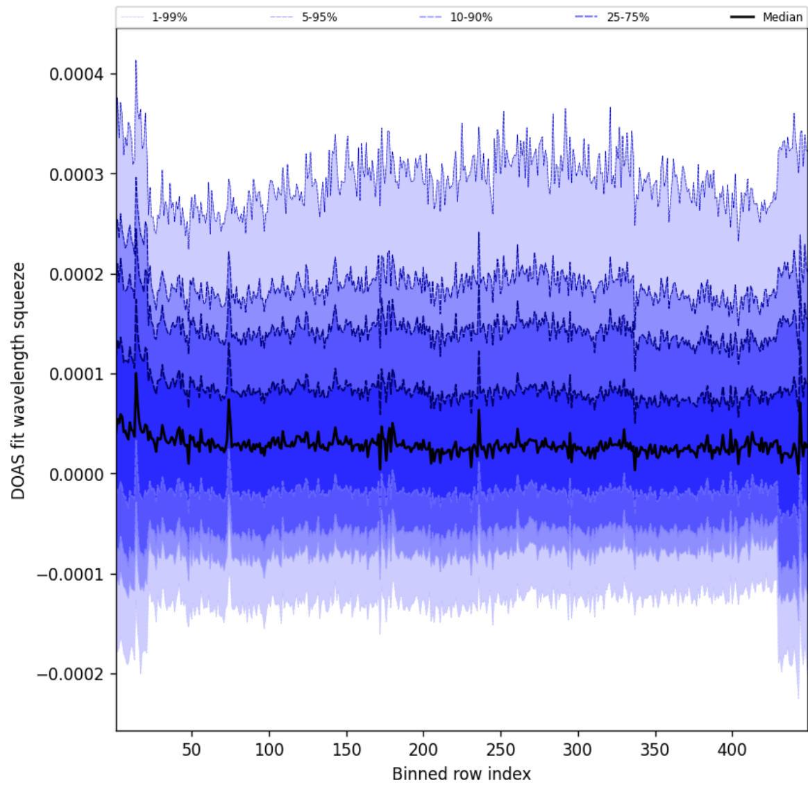
Figure 57: Along track statistics of “DOAS fit wavelength squeeze” for 2025-10-02 to 2025-10-03
