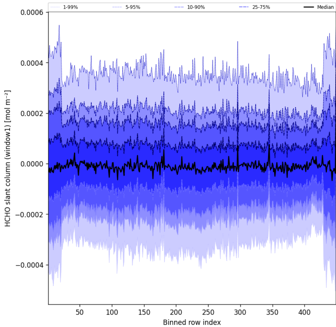
Figure 50: Along track statistics of “HCHO slant column (window1)” for 2025-10-02 to 2025-10-03
