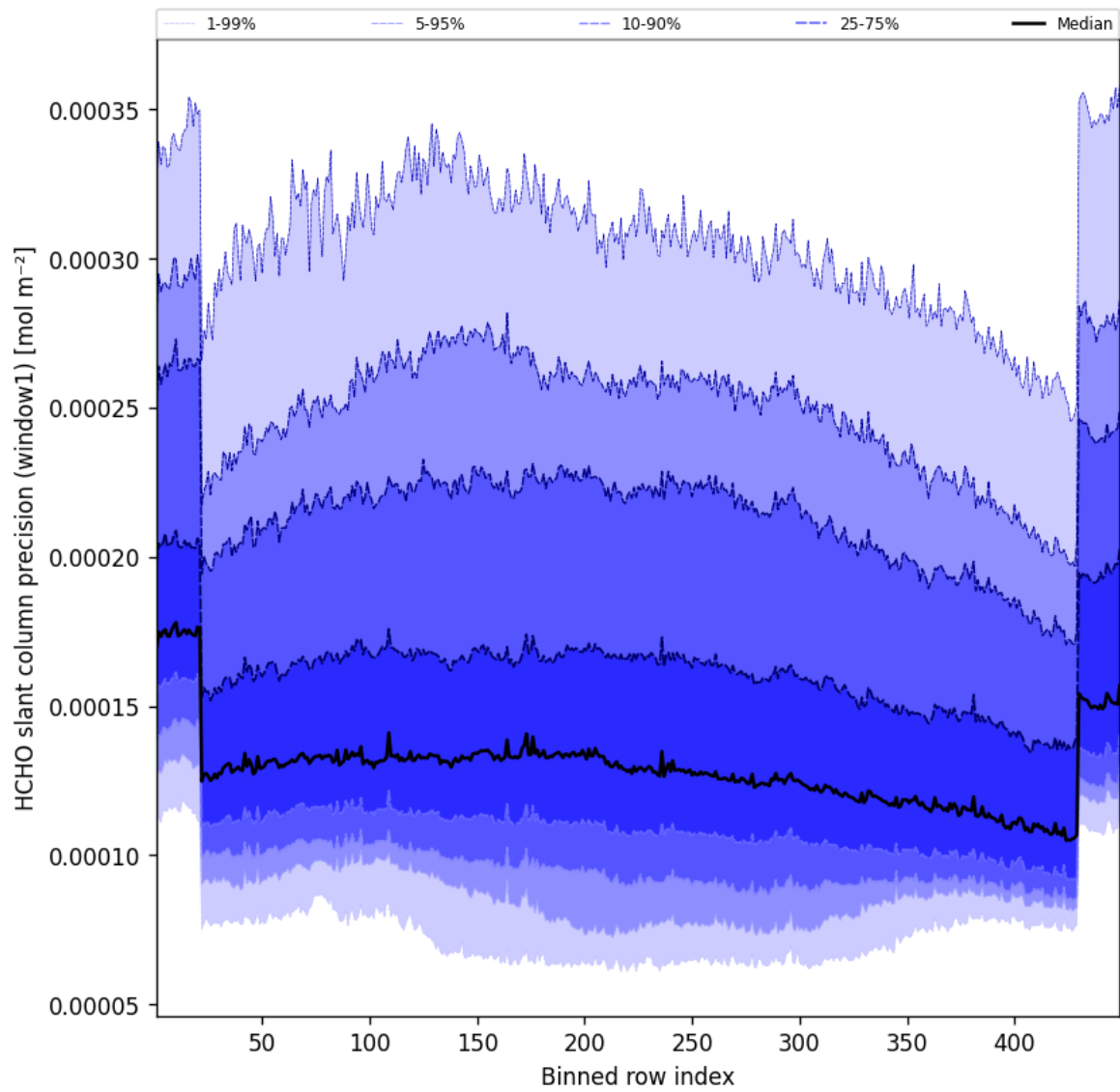
Figure 51: Along track statistics of “HCHO slant column precision (window1)” for 2025-10-02 to 2025-10-03
