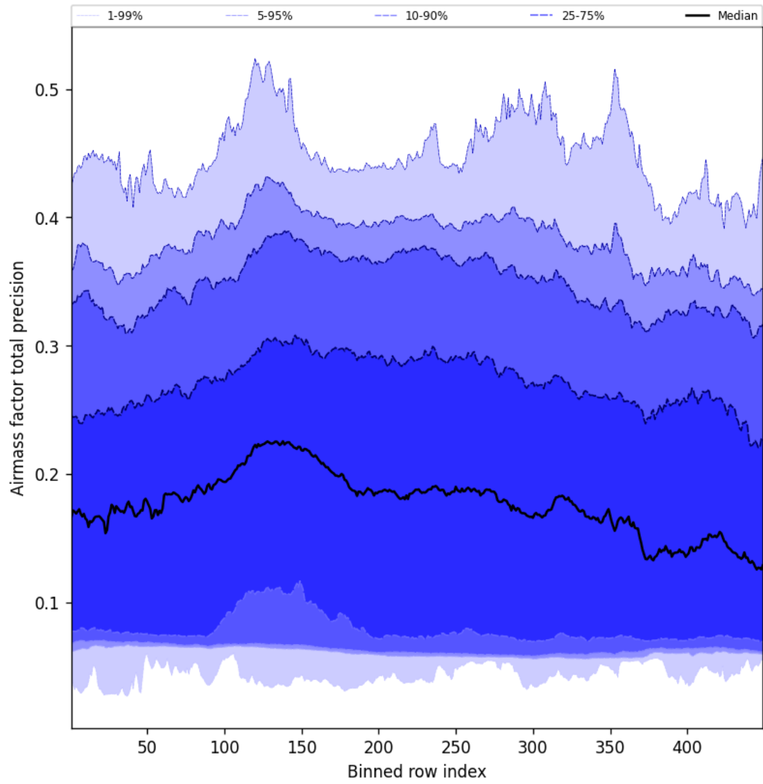
Figure 53: Along track statistics of “Airmass factor total precision” for 2025-10-02 to 2025-10-03
