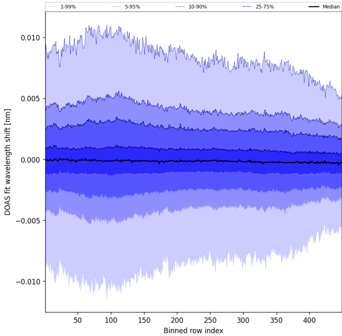
Figure 56: Along track statistics of “DOAS fit wavelength shift” for 2025-10-02 to 2025-10-03
