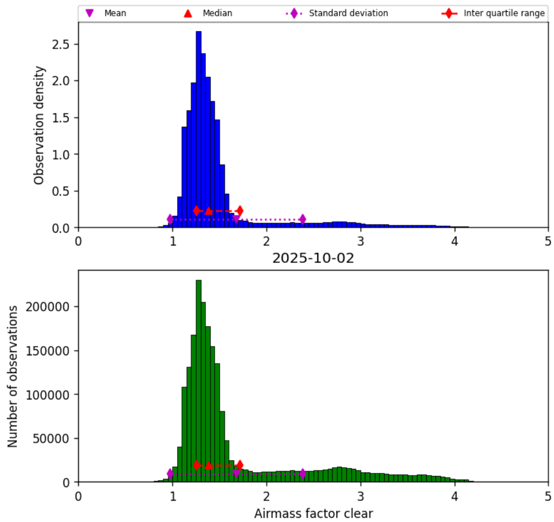
Figure 40: Histogram of “Airmass factor clear” for 2025-10-02 to 2025-10-03
