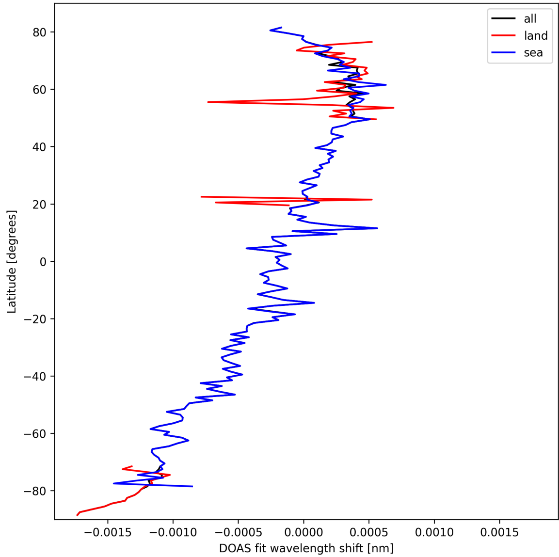
Figure 28: Zonal average of “DOAS fit wavelength shift” for 2025-10-02 to 2025-10-03.
