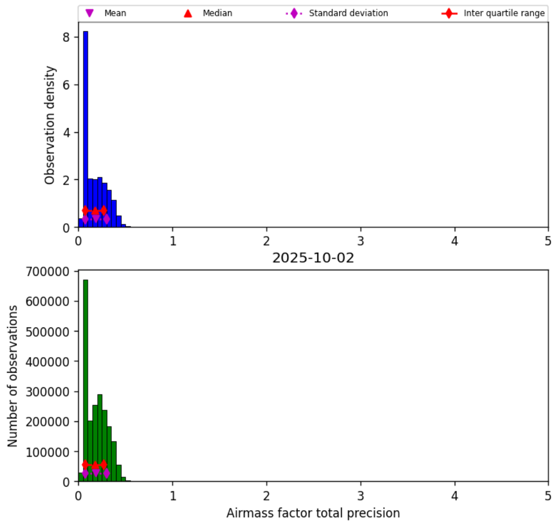
Figure 39: Histogram of “Airmass factor total precision” for 2025-10-02 to 2025-10-03
