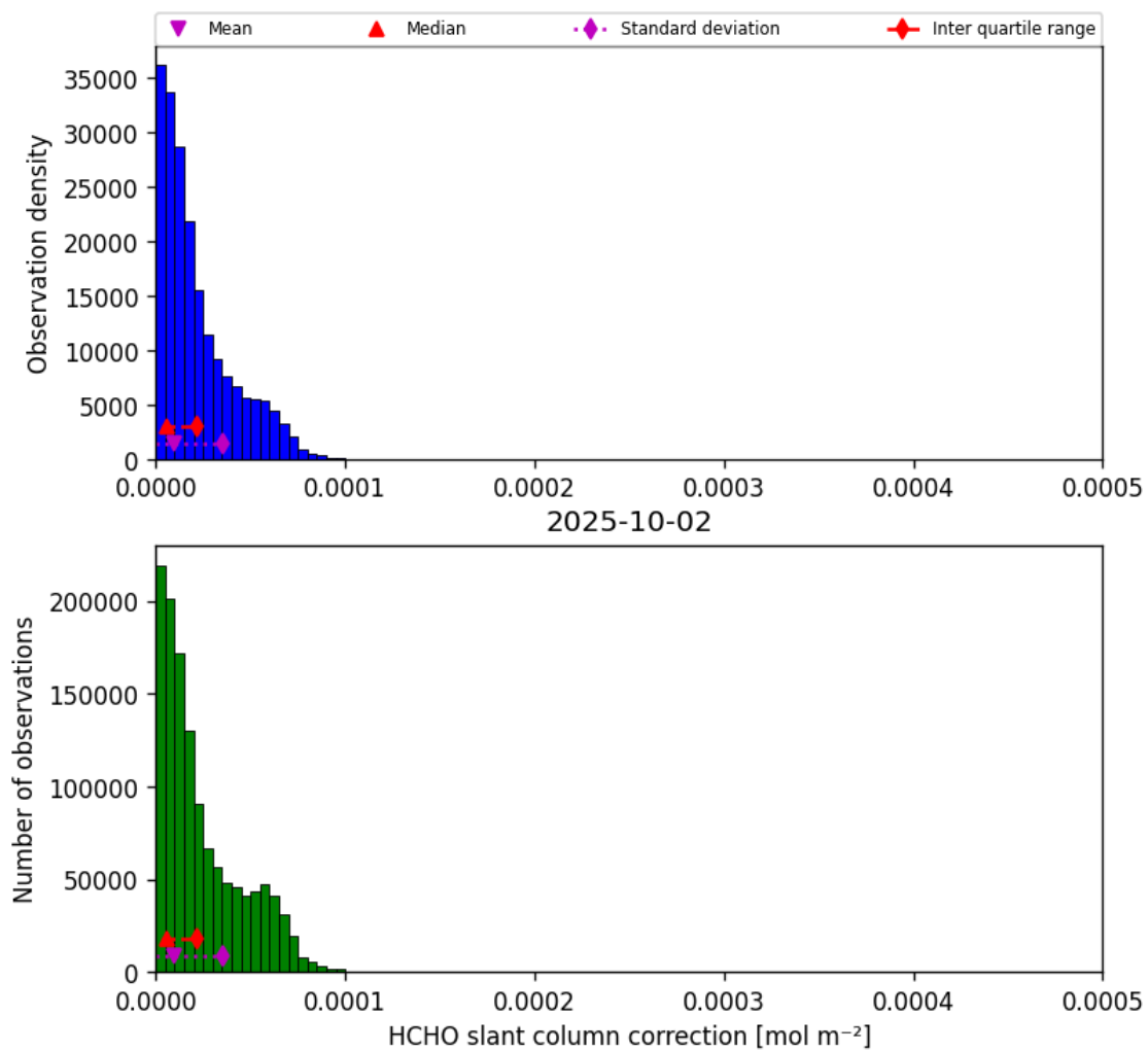
Figure 45: Histogram of “HCHO slant column correction” for 2025-10-02 to 2025-10-03
