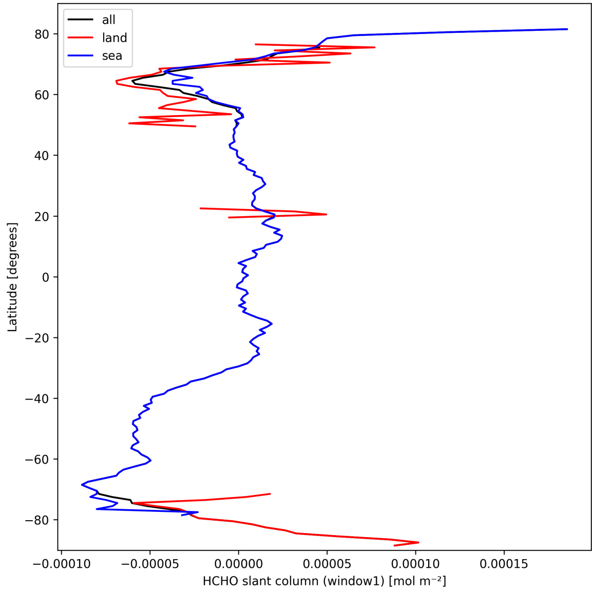
Figure 22: Zonal average of “HCHO slant column (window1)” for 2025-10-02 to 2025-10-03.
