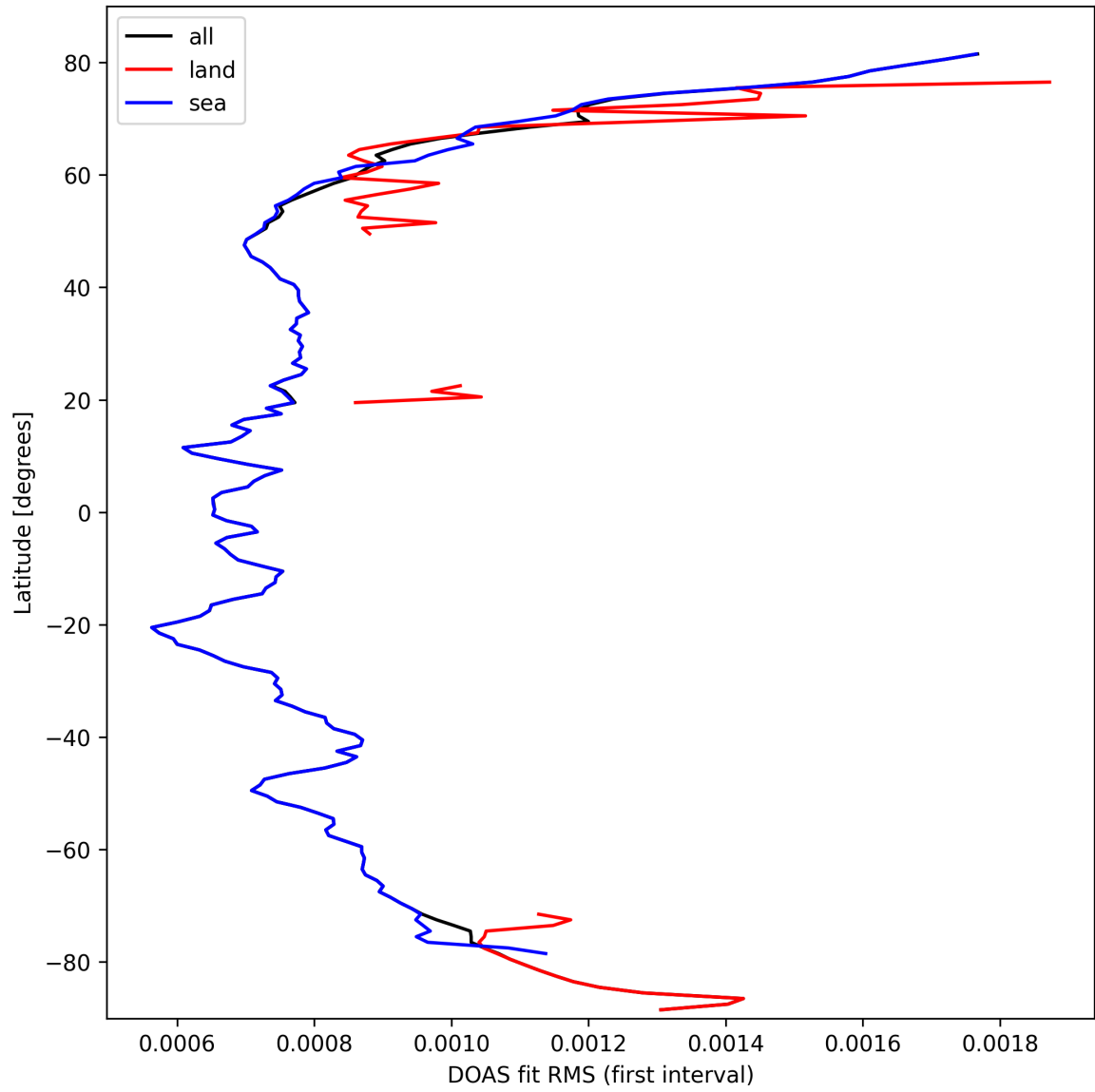
Figure 30: Zonal average of "DOAS fit RMS (first interval)" for 2025-10-02 to 2025-10-03.
