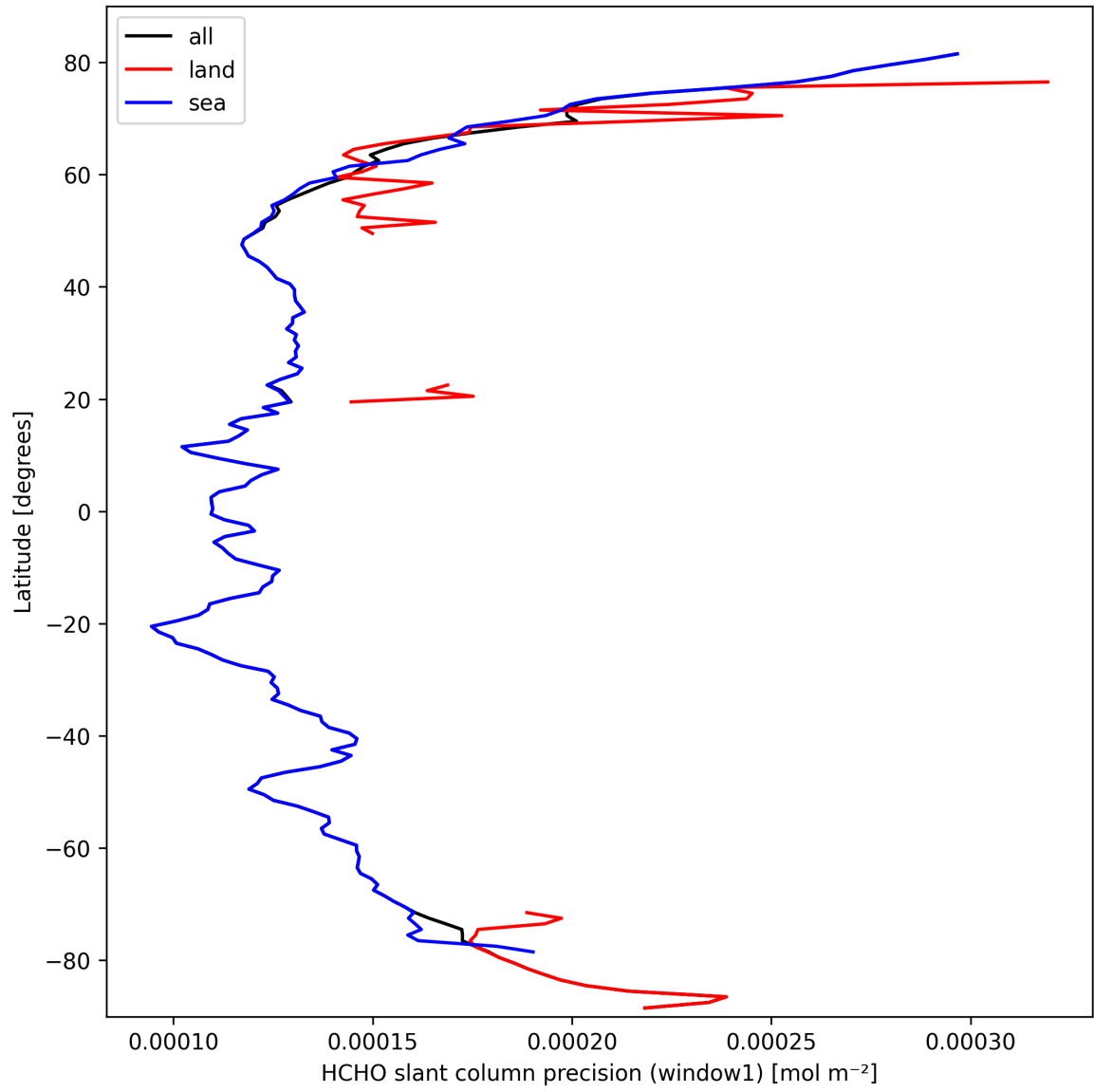
Figure 23: Zonal average of “HCHO slant column precision (window1)” for 2025-10-02 to 2025-10-03.
