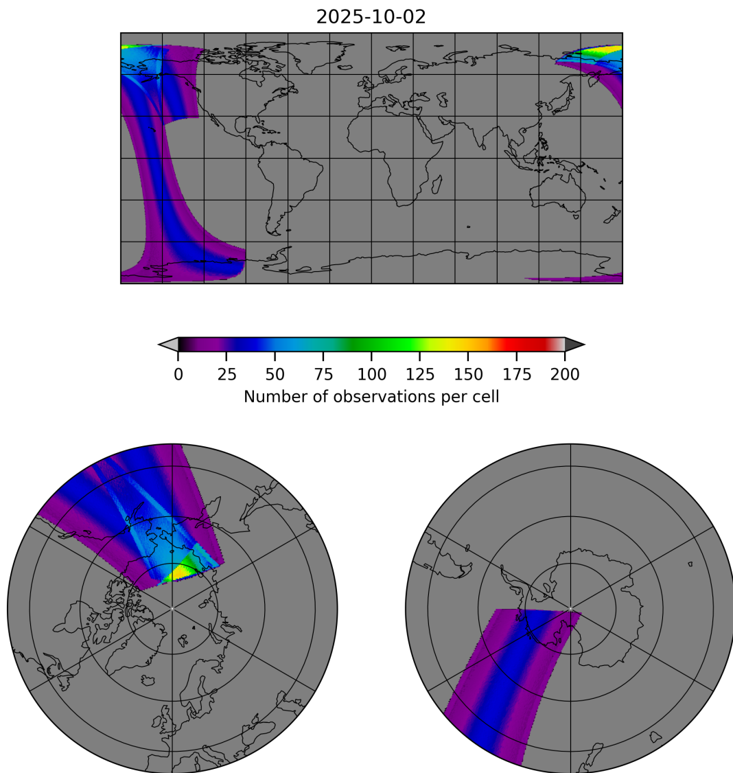
Figure 17: Map of the number of observations for 2025-10-02 to 2025-10-03
