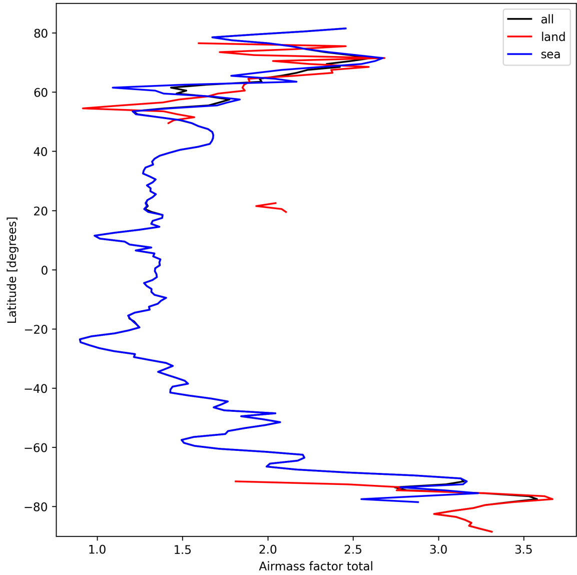
Figure 24: Zonal average of "Airmass factor total" for 2025-10-02 to 2025-10-03.
