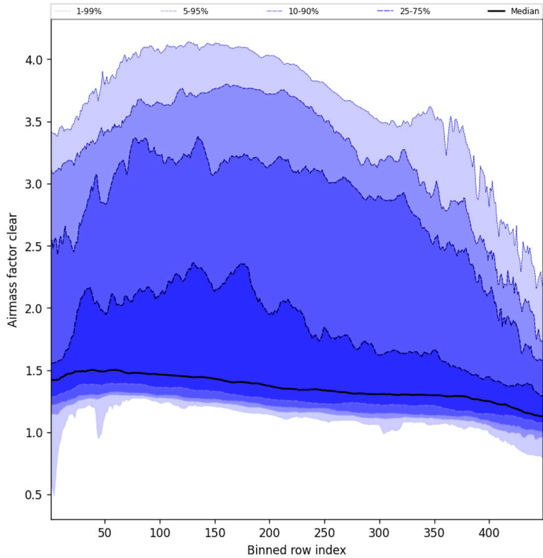
Figure 54: Along track statistics of “Airmass factor clear” for 2025-10-02 to 2025-10-03
