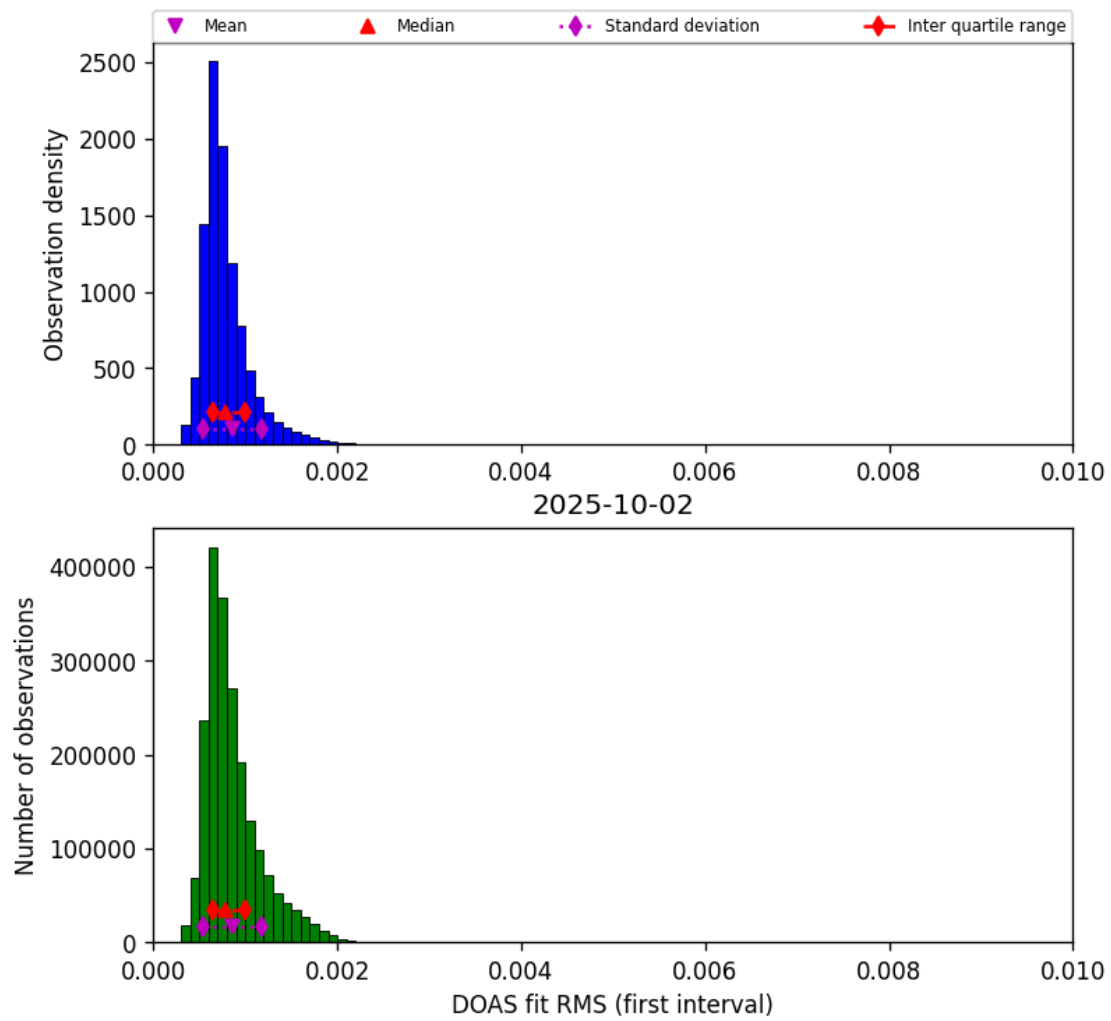
Figure 44: Histogram of “DOAS fit RMS (first interval)” for 2025-10-02 to 2025-10-03
