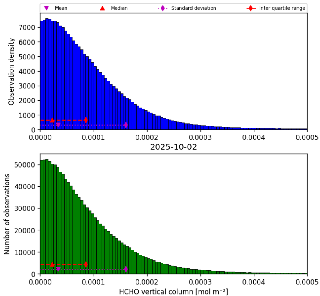
Figure 33: Histogram of “HCHO vertical column” for 2025-10-02 to 2025-10-03
