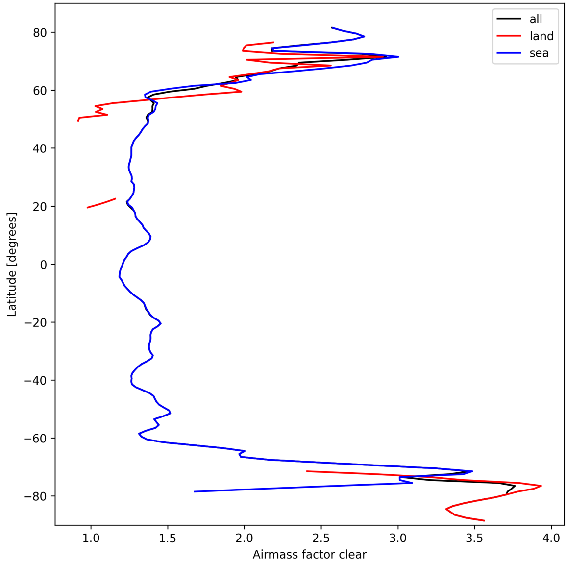
Figure 26: Zonal average of “Airmass factor clear” for 2025-10-02 to 2025-10-03.
