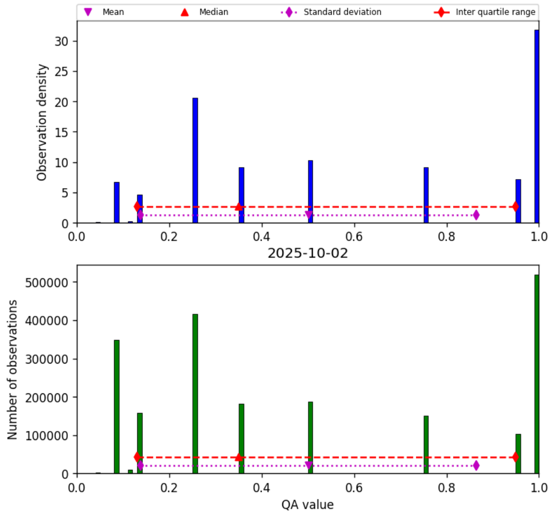
Figure 32: Histogram of “QA value” for 2025-10-02 to 2025-10-03
