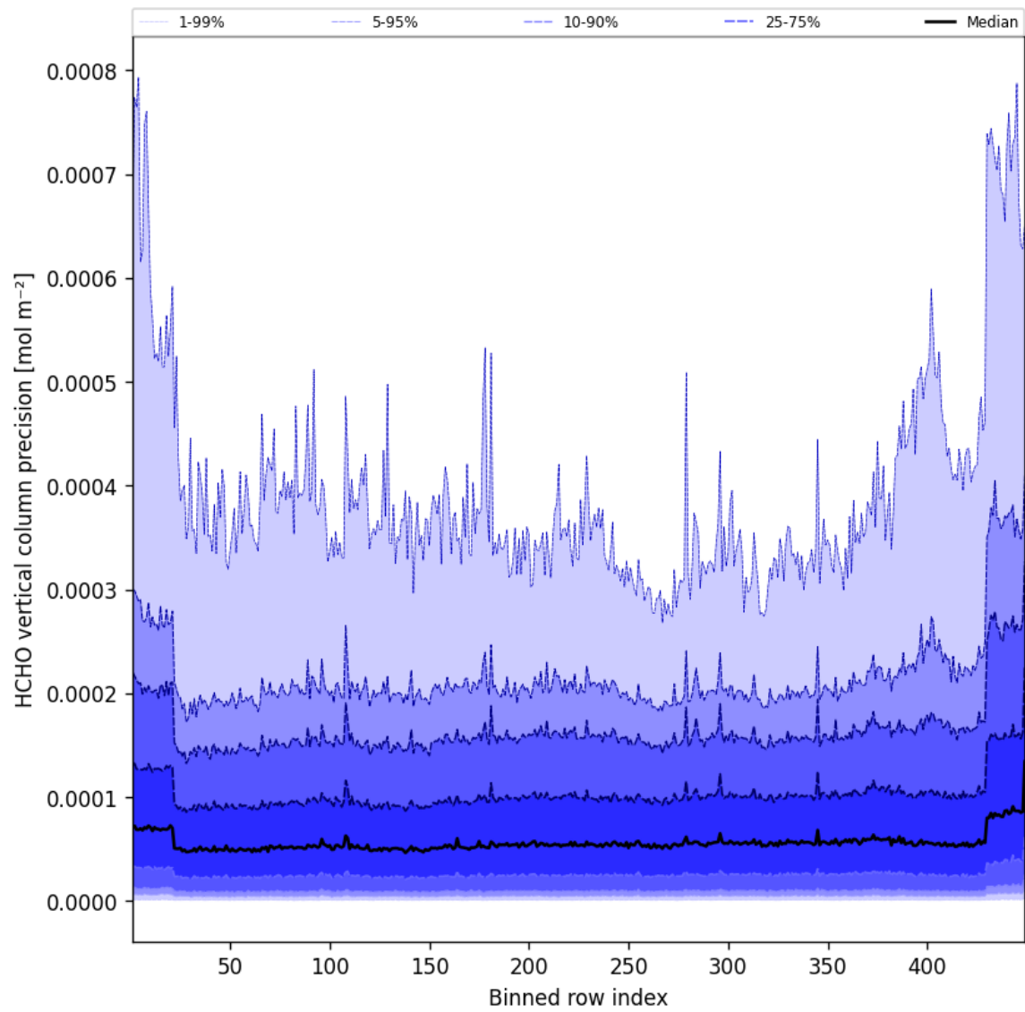
Figure 48: Along track statistics of “HCHO vertical column precision” for 2025-10-02 to 2025-10-03
