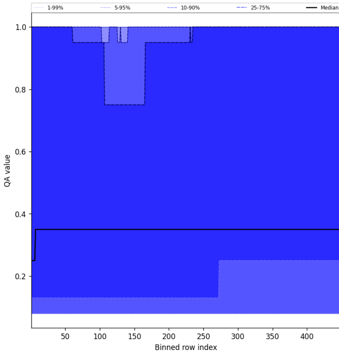
Figure 46: Along track statistics of "QA value" for 2025-10-02 to 2025-10-03
