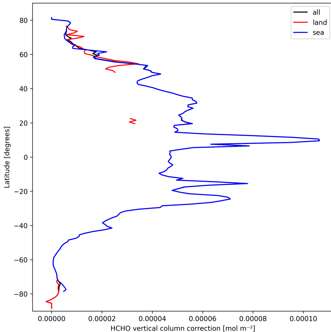
Figure 21: Zonal average of “HCHO vertical column correction” for 2025-10-02 to 2025-10-03.
