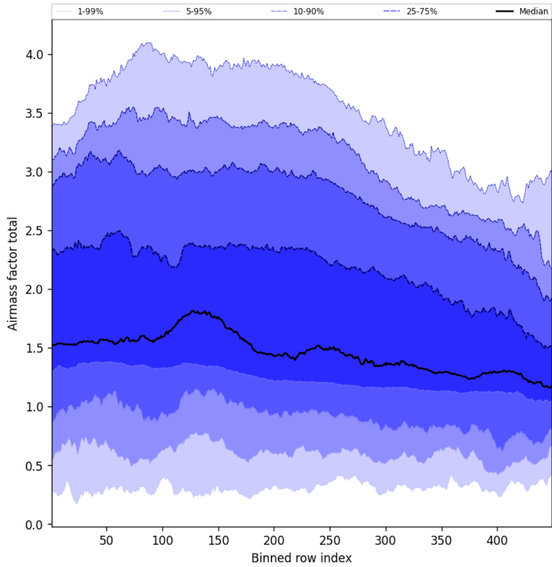
Figure 52: Along track statistics of “Airmass factor total” for 2025-10-02 to 2025-10-03
