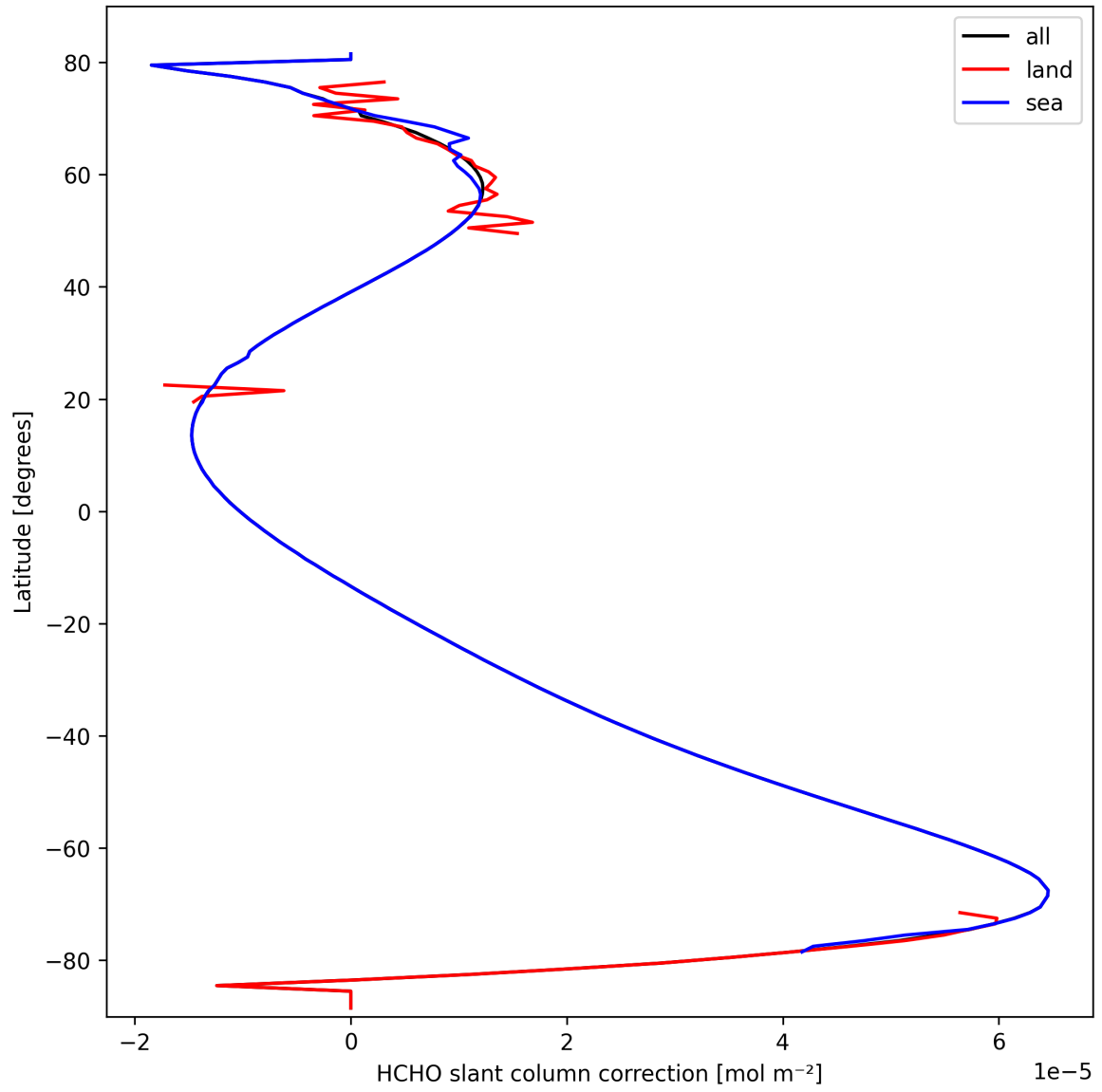
Figure 31: Zonal average of “HCHO slant column correction” for 2025-10-02 to 2025-10-03.
