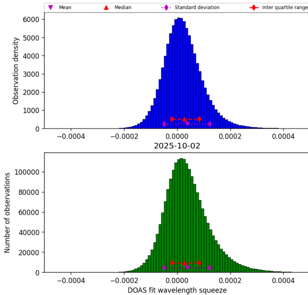
Figure 43: Histogram of “DOAS fit wavelength squeeze” for 2025-10-02 to 2025-10-03
