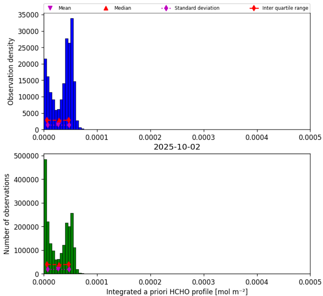
Figure 41: Histogram of “Integrated a priori HCHO profile” for 2025-10-02 to 2025-10-03
