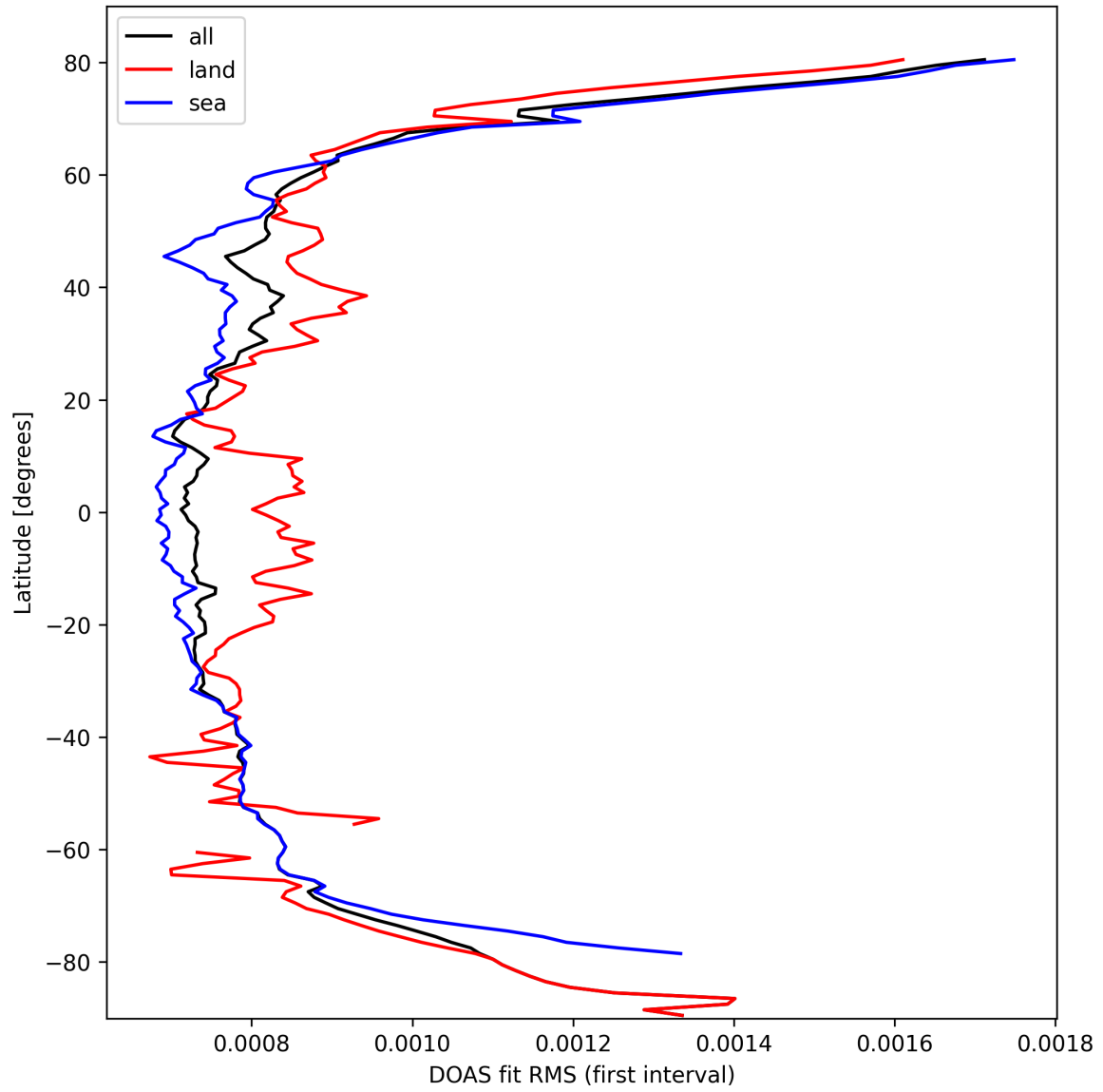
Figure 30: Zonal average of "DOAS fit RMS (first interval)" for 2025-10-03 to 2025-10-04.
