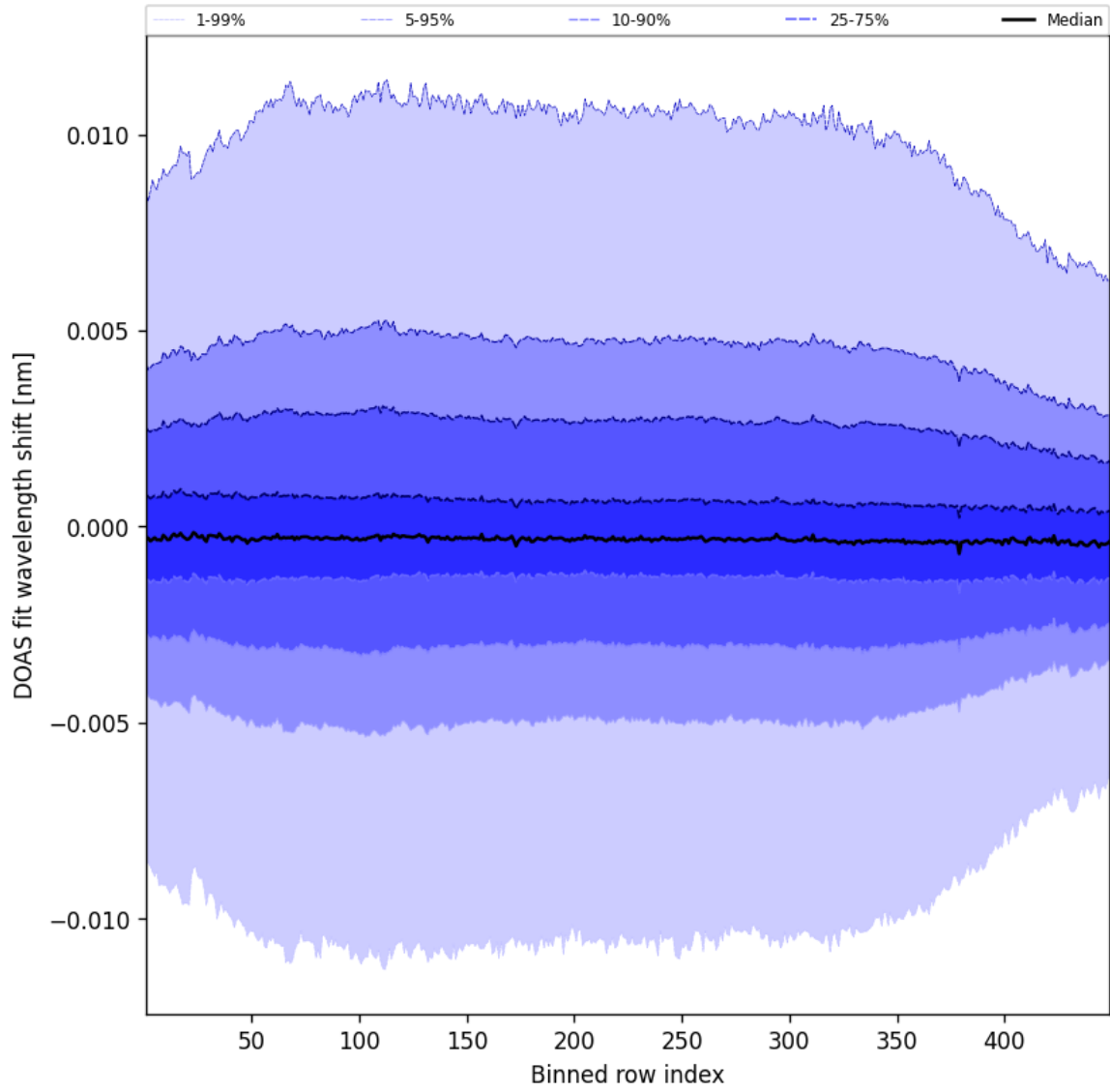
Figure 56: Along track statistics of “DOAS fit wavelength shift” for 2025-10-03 to 2025-10-04
