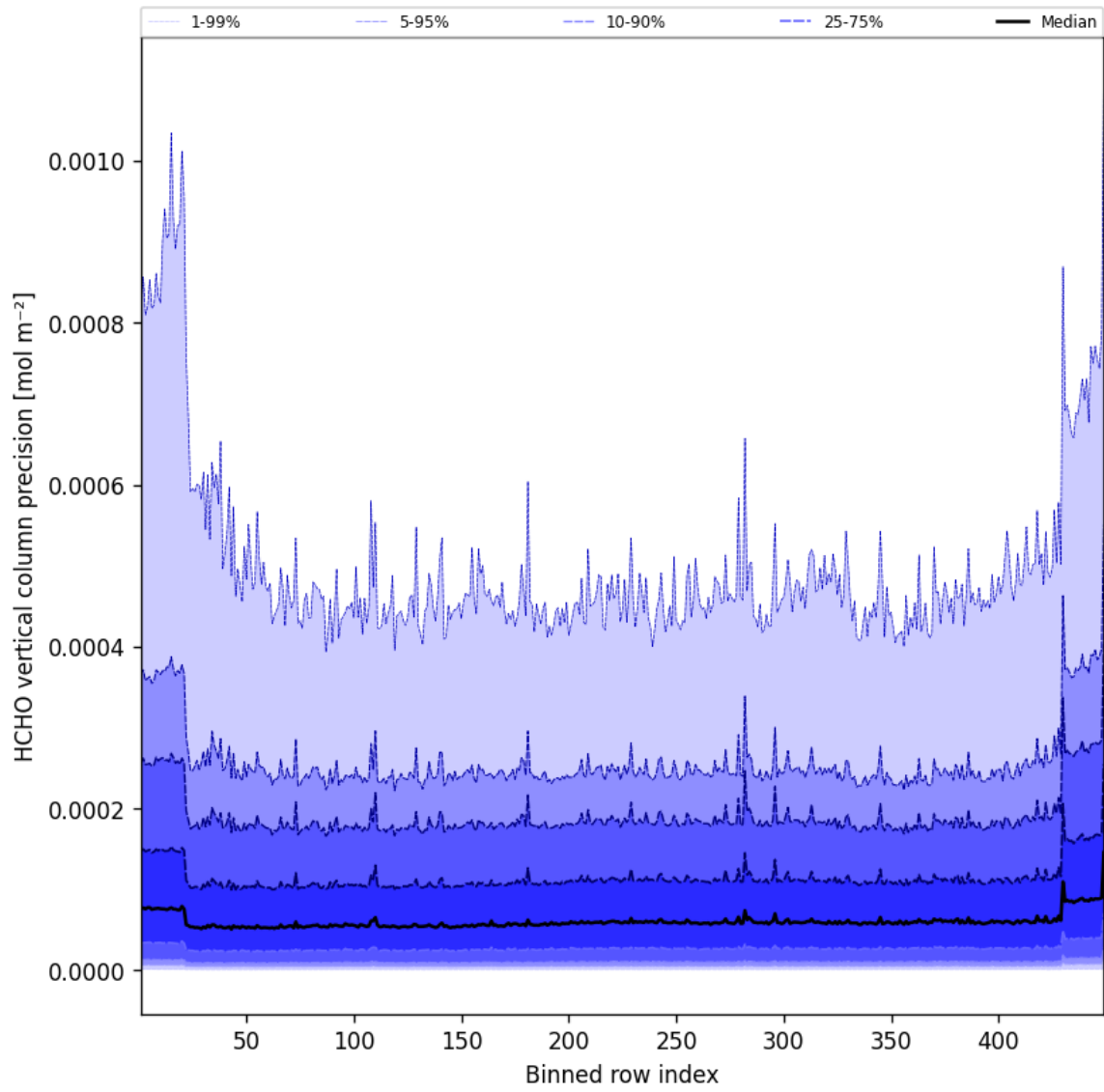
Figure 48: Along track statistics of “HCHO vertical column precision” for 2025-10-03 to 2025-10-04
