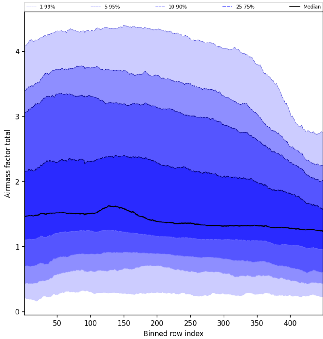
Figure 52: Along track statistics of “Airmass factor total” for 2025-10-03 to 2025-10-04
