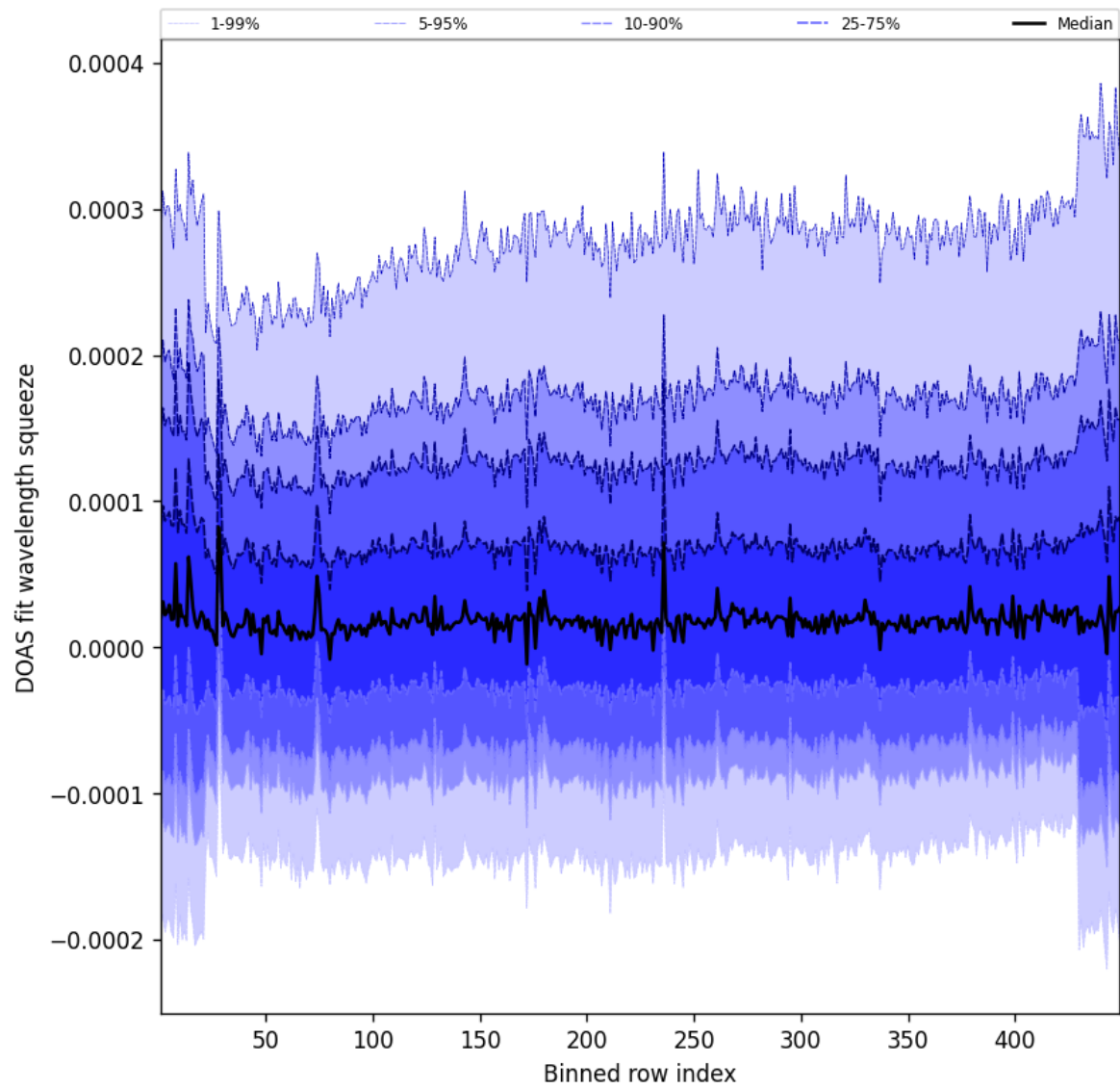
Figure 57: Along track statistics of “DOAS fit wavelength squeeze” for 2025-10-03 to 2025-10-04
