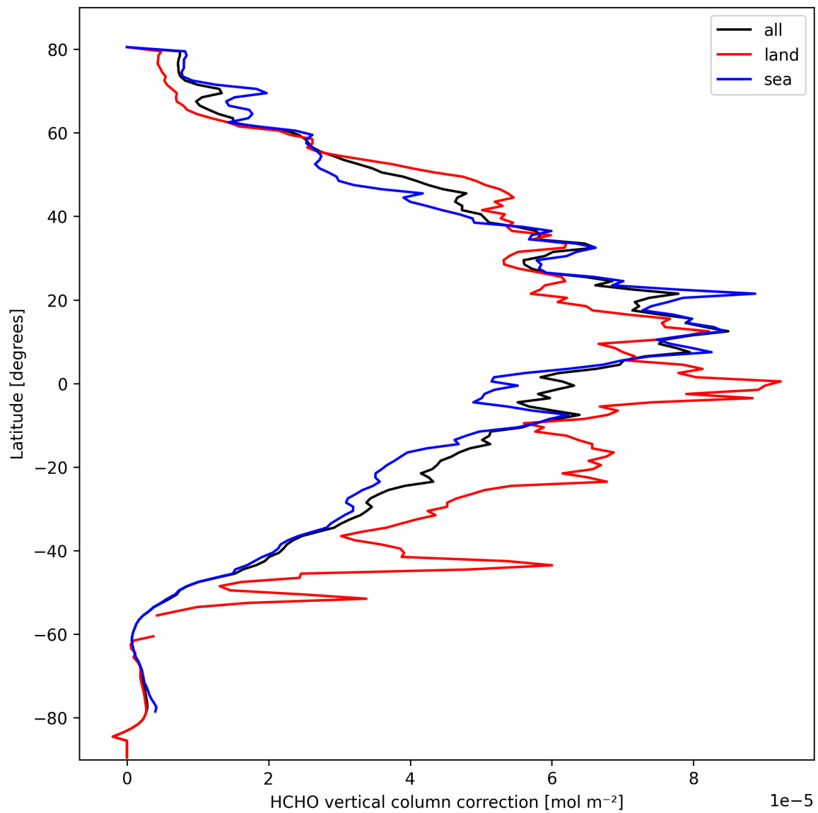
Figure 21: Zonal average of "HCHO vertical column correction" for 2025-10-03 to 2025-10-04.
