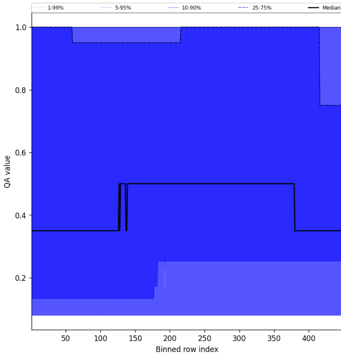
Figure 46: Along track statistics of “QA value” for 2025-10-03 to 2025-10-04
