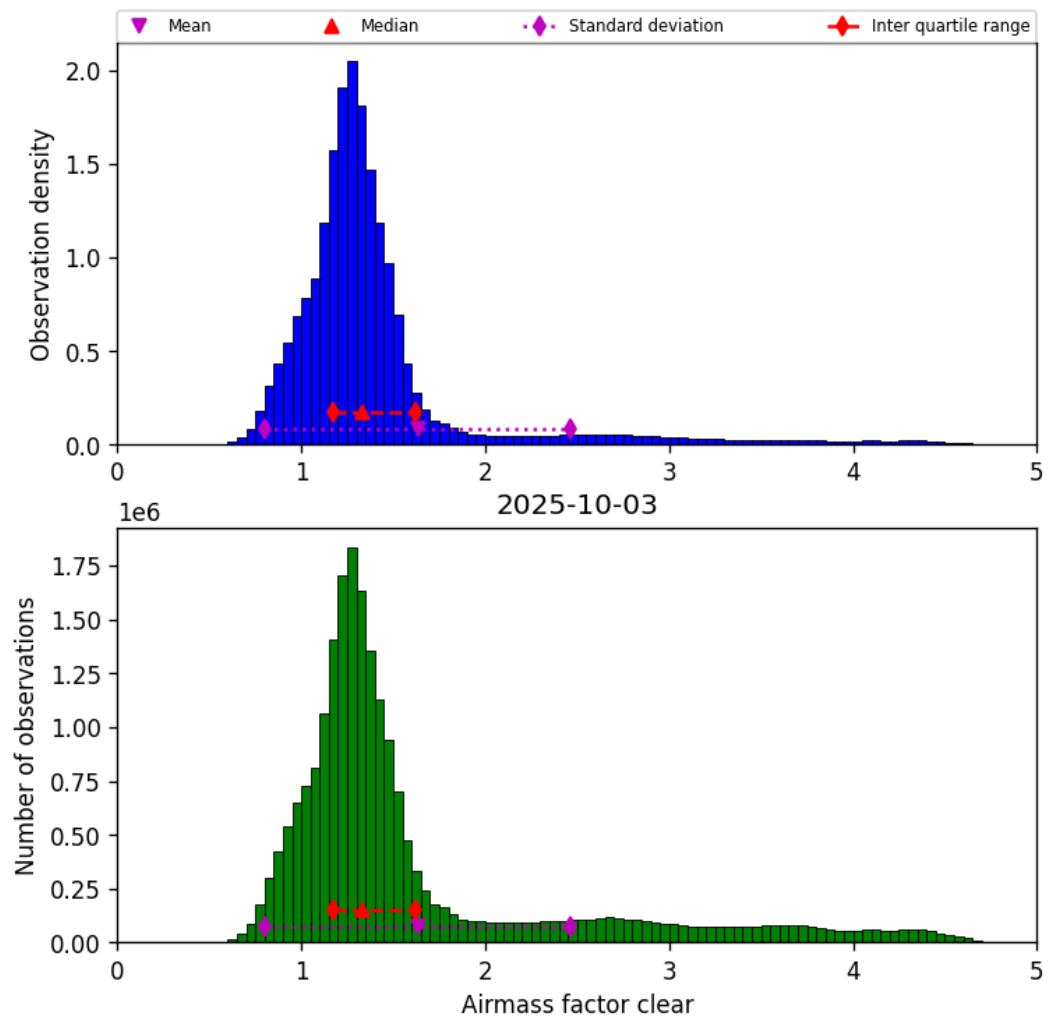
Figure 40: Histogram of “Airmass factor clear” for 2025-10-03 to 2025-10-04
