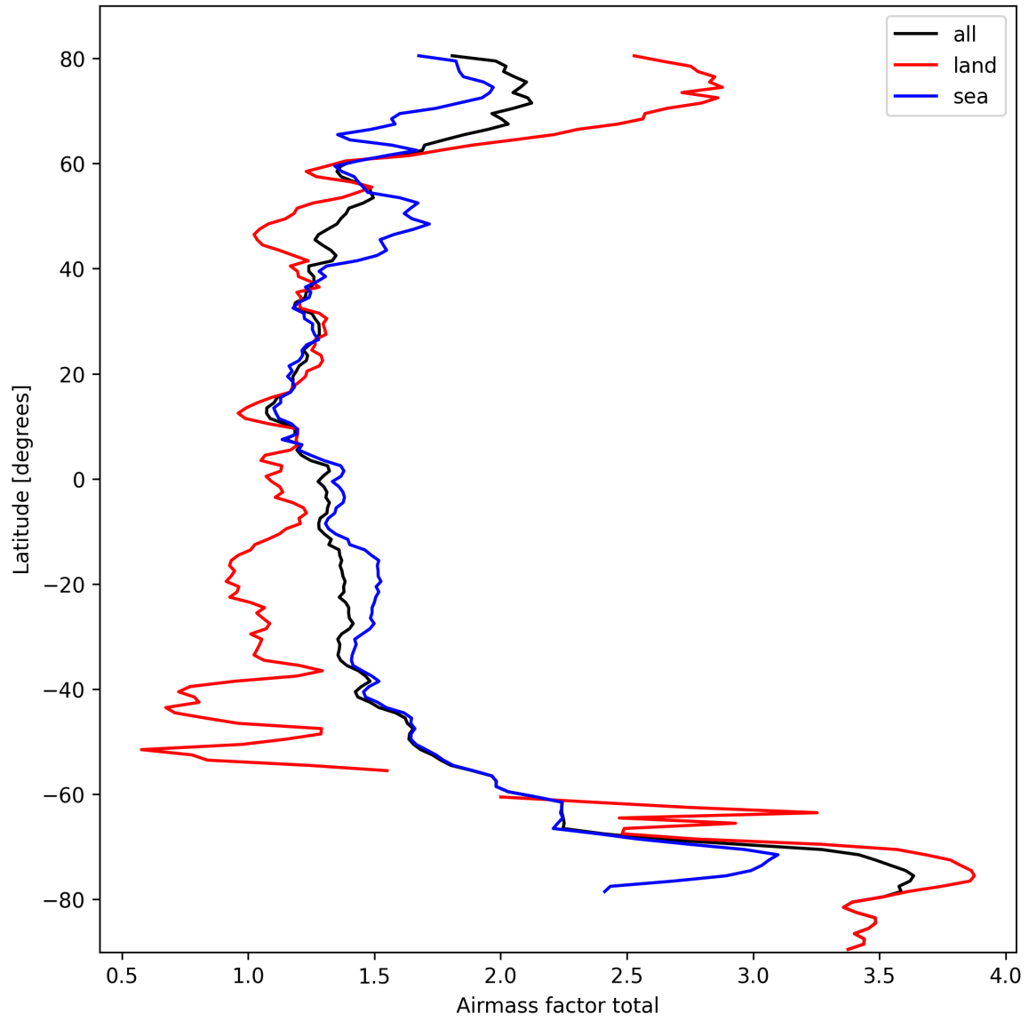
Figure 24: Zonal average of “Airmass factor total” for 2025-10-03 to 2025-10-04.
