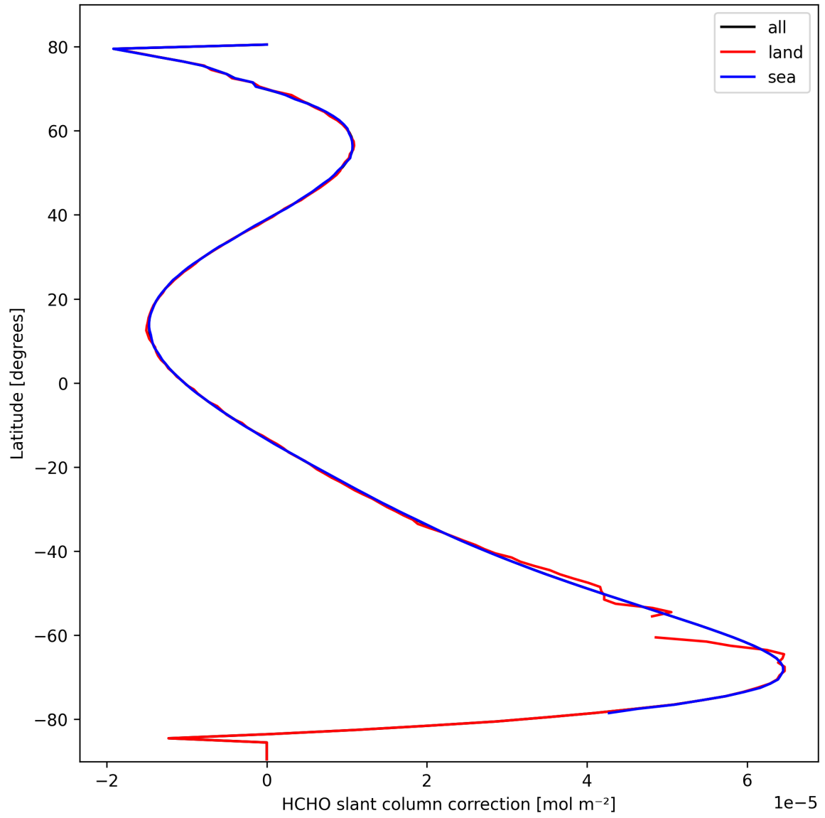
Figure 31: Zonal average of “HCHO slant column correction” for 2025-10-03 to 2025-10-04.
