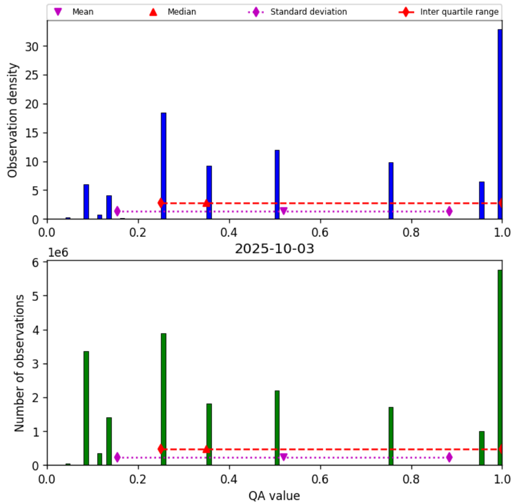
Figure 32: Histogram of “QA value” for 2025-10-03 to 2025-10-04
