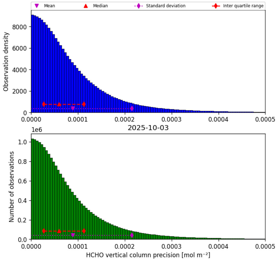
Figure 34: Histogram of “HCHO vertical column precision” for 2025-10-03 to 2025-10-04
