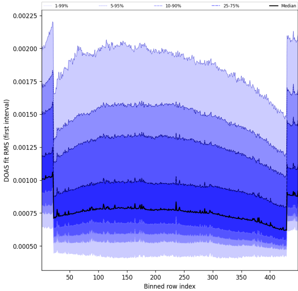
Figure 58: Along track statistics of “DOAS fit RMS (first interval)” for 2025-10-03 to 2025-10-04
