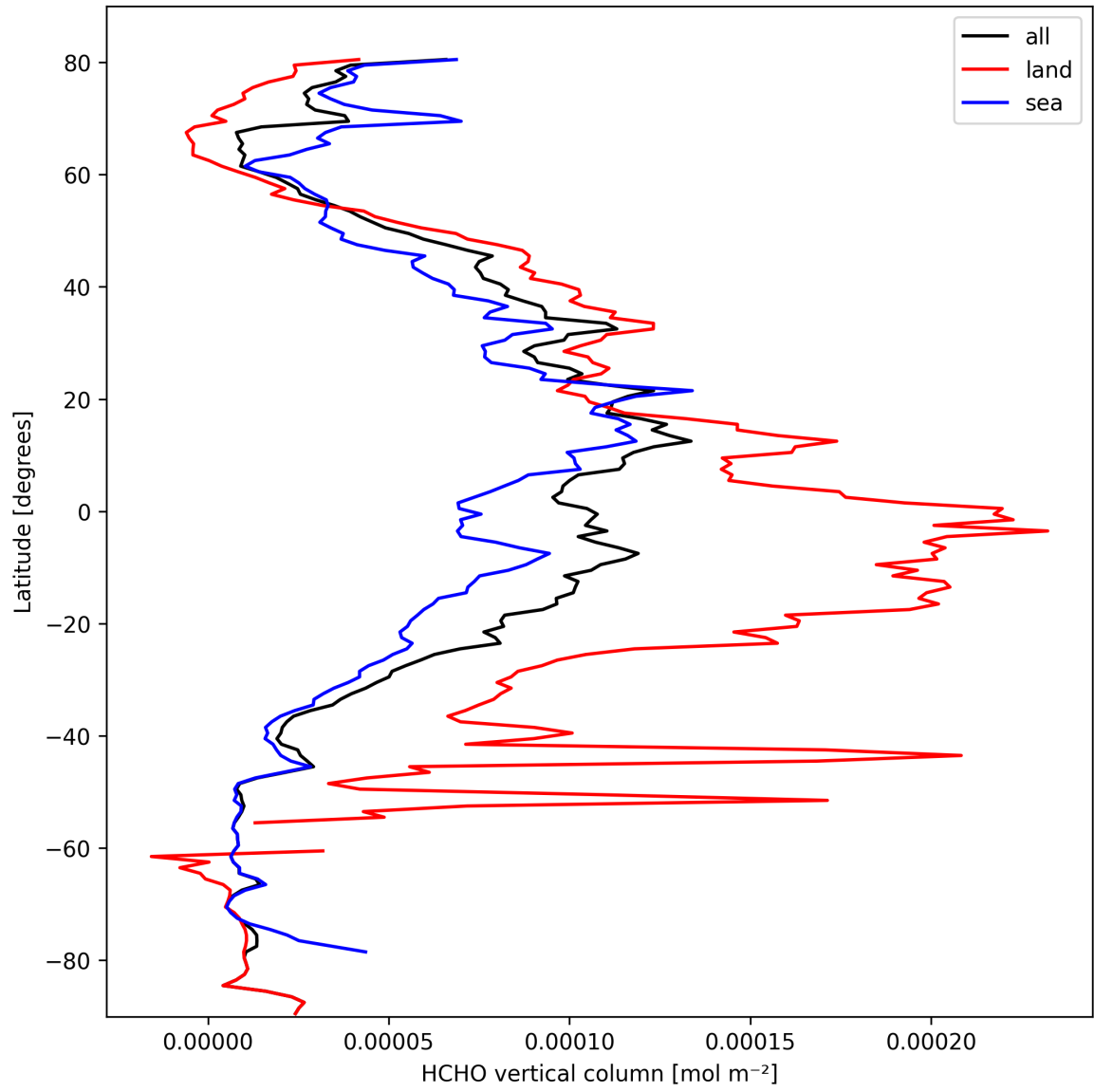
Figure 19: Zonal average of “HCHO vertical column” for 2025-10-03 to 2025-10-04.
