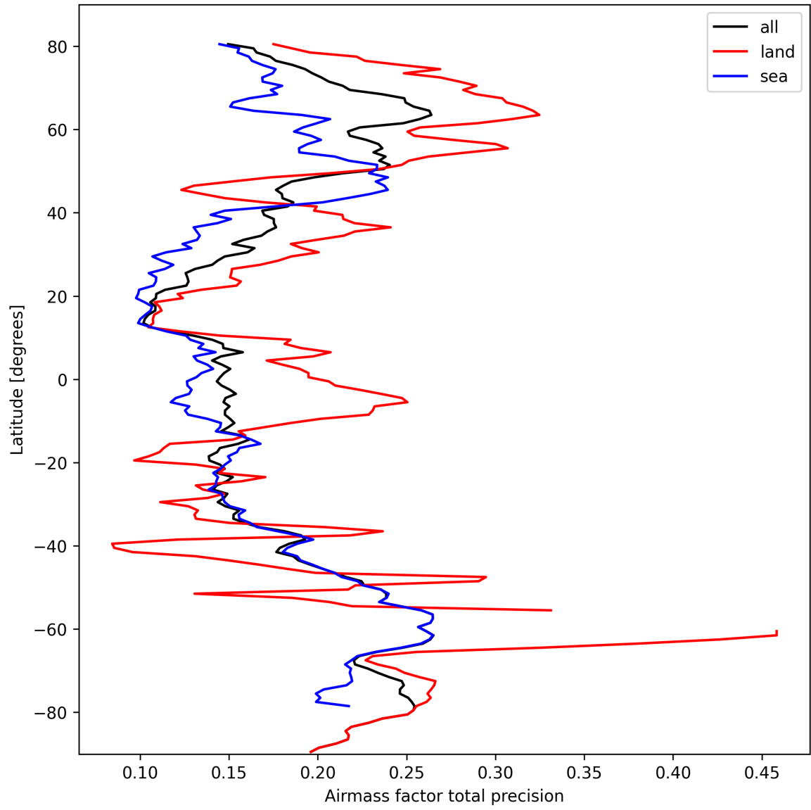
Figure 25: Zonal average of “Airmass factor total precision” for 2025-10-03 to 2025-10-04.
