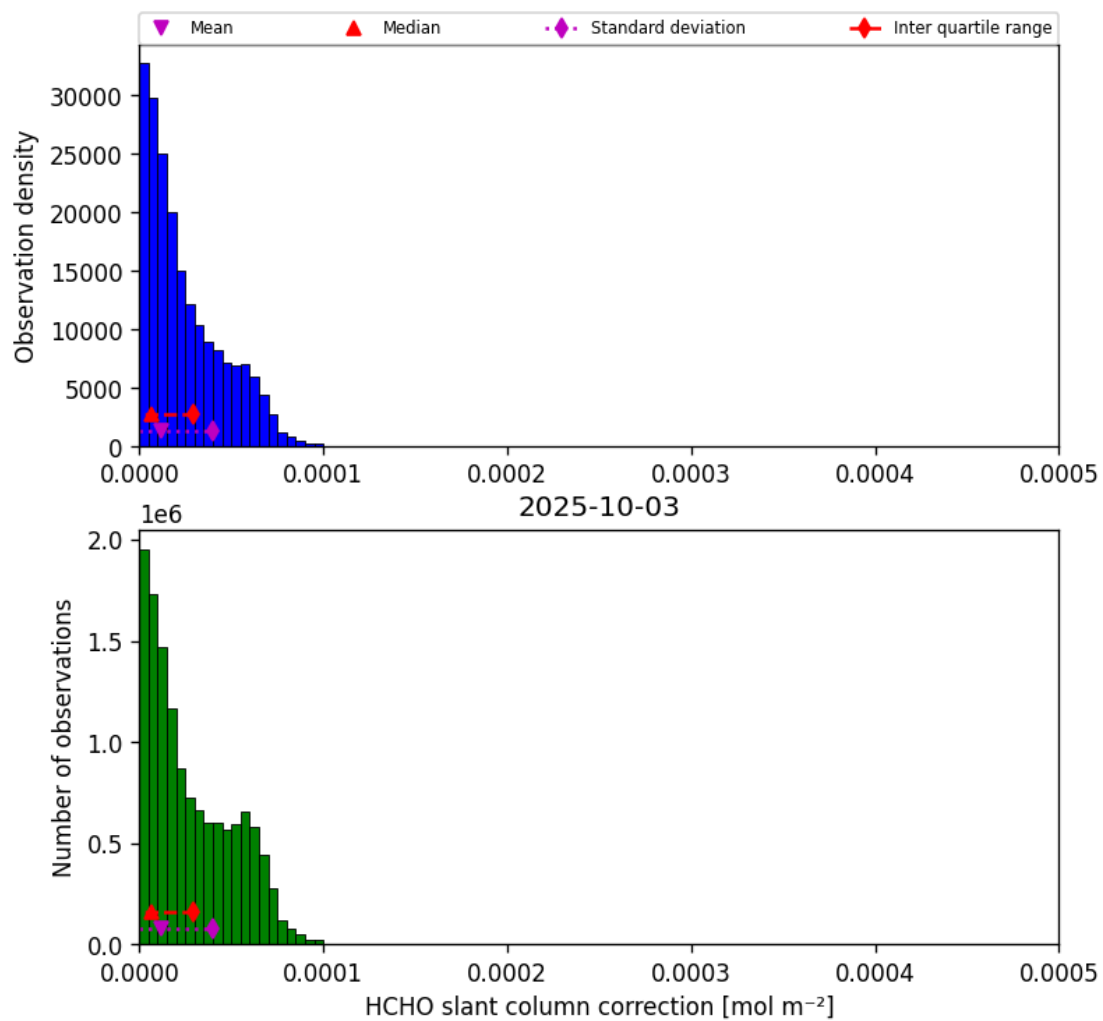
Figure 45: Histogram of “HCHO slant column correction” for 2025-10-03 to 2025-10-04
