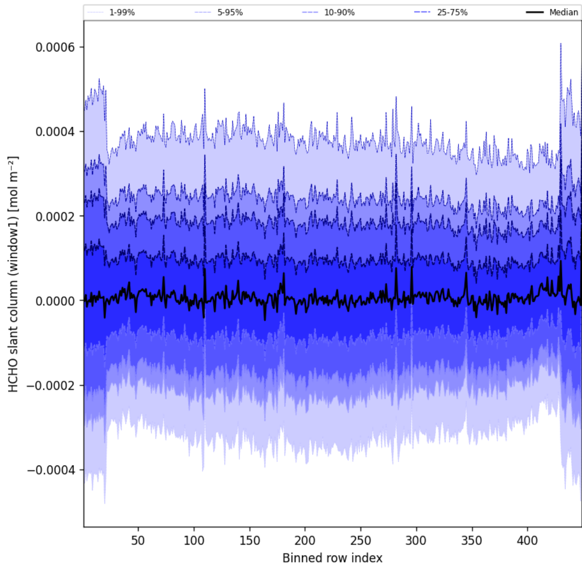
Figure 50: Along track statistics of “HCHO slant column (window1)” for 2025-10-03 to 2025-10-04
