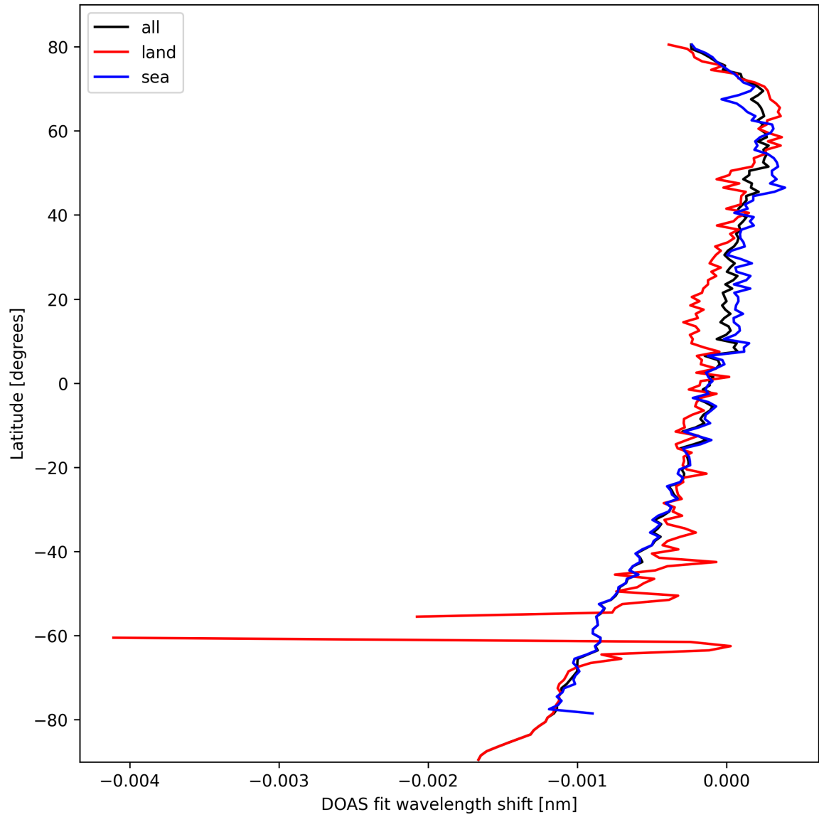
Figure 28: Zonal average of “DOAS fit wavelength shift” for 2025-10-03 to 2025-10-04.
