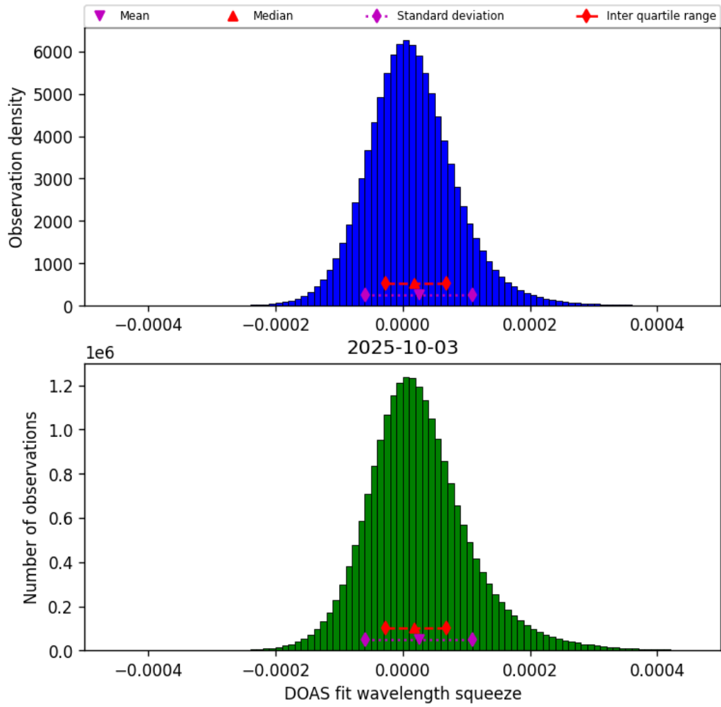
Figure 43: Histogram of “DOAS fit wavelength squeeze” for 2025-10-03 to 2025-10-04
