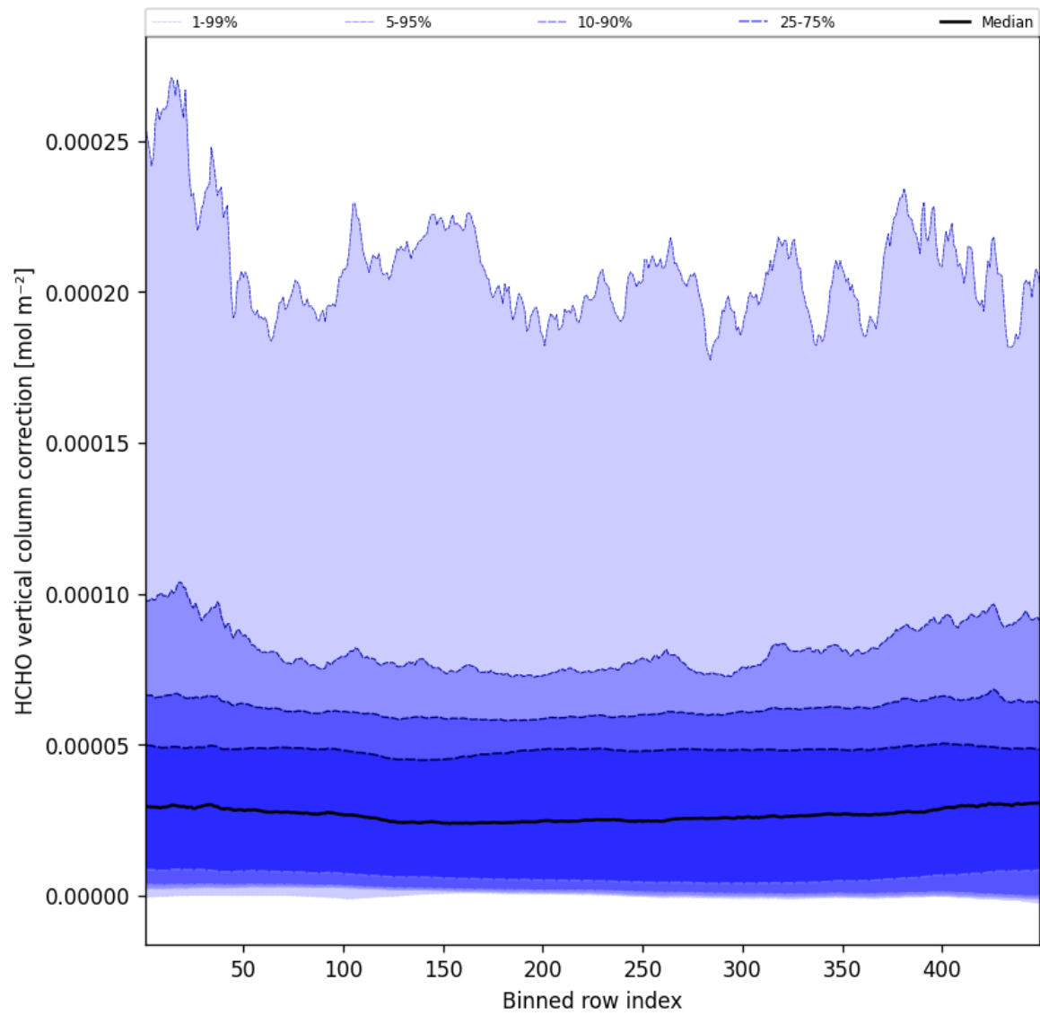
Figure 49: Along track statistics of "HCHO vertical column correction" for 2025-10-03 to 2025-10-04
