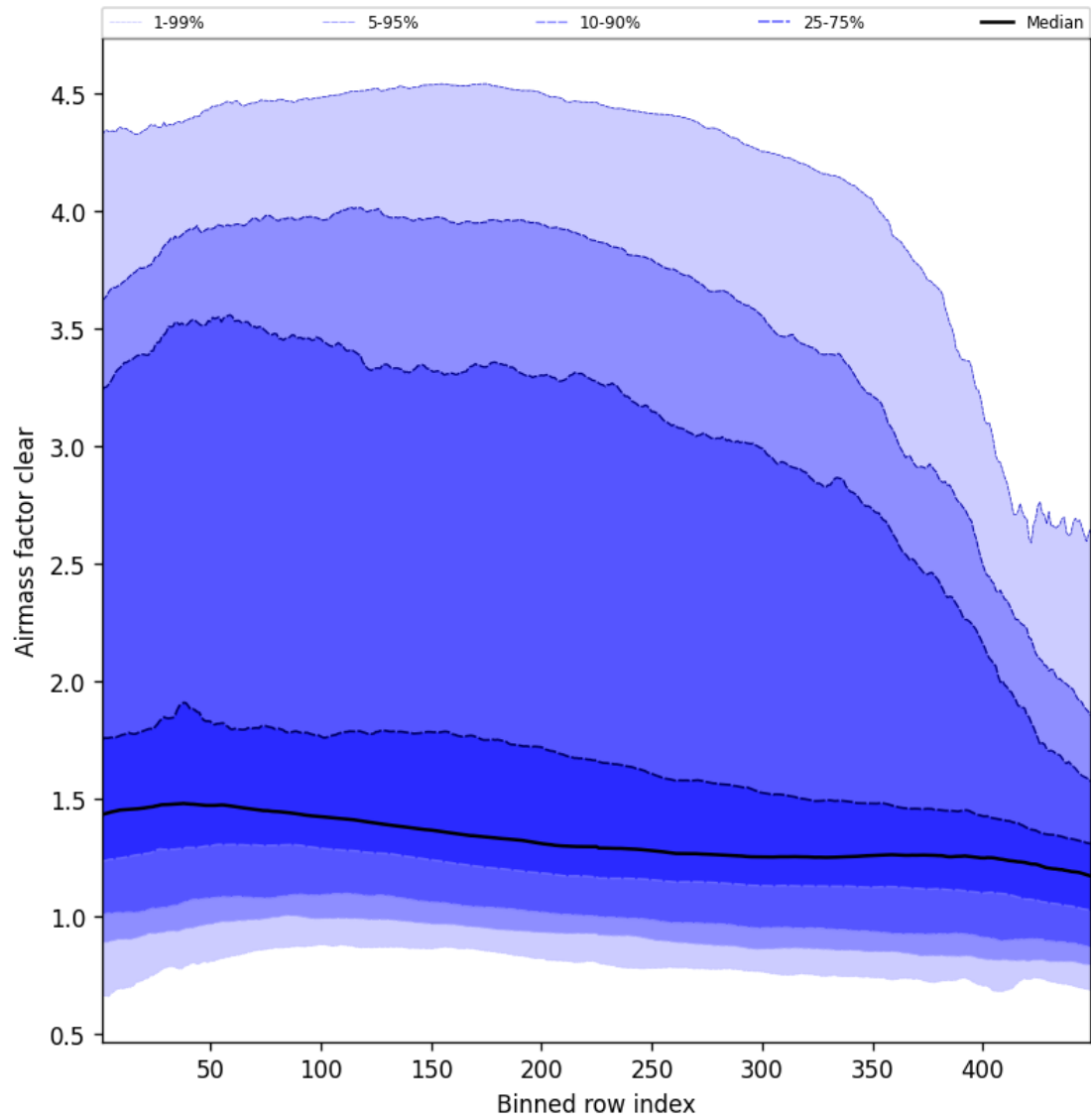
Figure 54: Along track statistics of “Airmass factor clear” for 2025-10-03 to 2025-10-04
