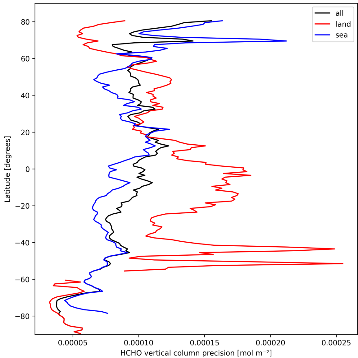
Figure 20: Zonal average of “HCHO vertical column precision” for 2025-10-03 to 2025-10-04.
