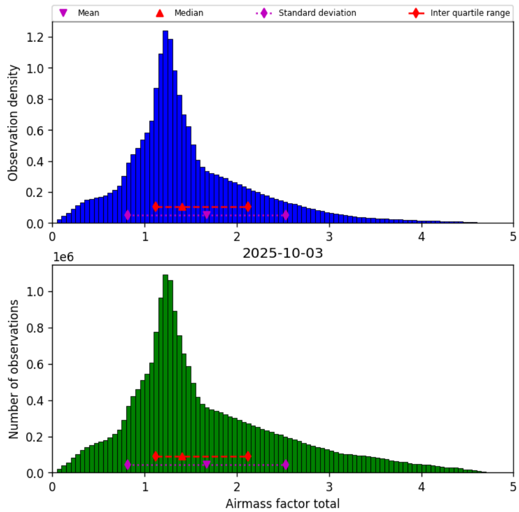
Figure 38: Histogram of “Airmass factor total” for 2025-10-03 to 2025-10-04
