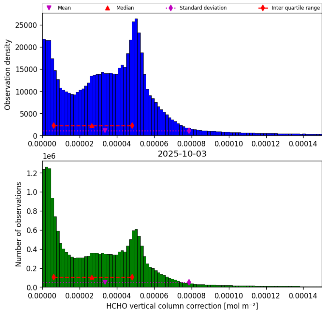
Figure 35: Histogram of “HCHO vertical column correction” for 2025-10-03 to 2025-10-04
