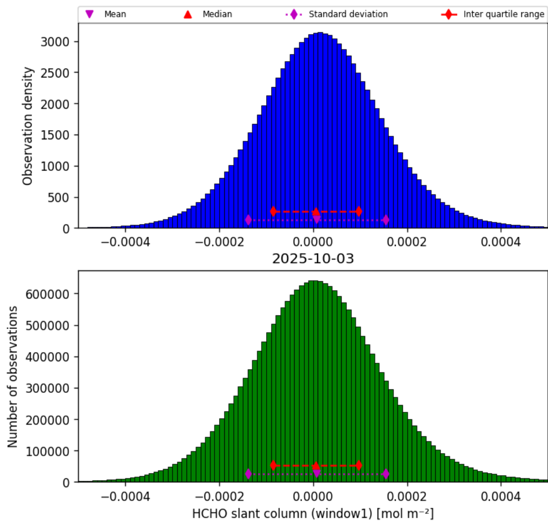
Figure 36: Histogram of “HCHO slant column (window1)” for 2025-10-03 to 2025-10-04
