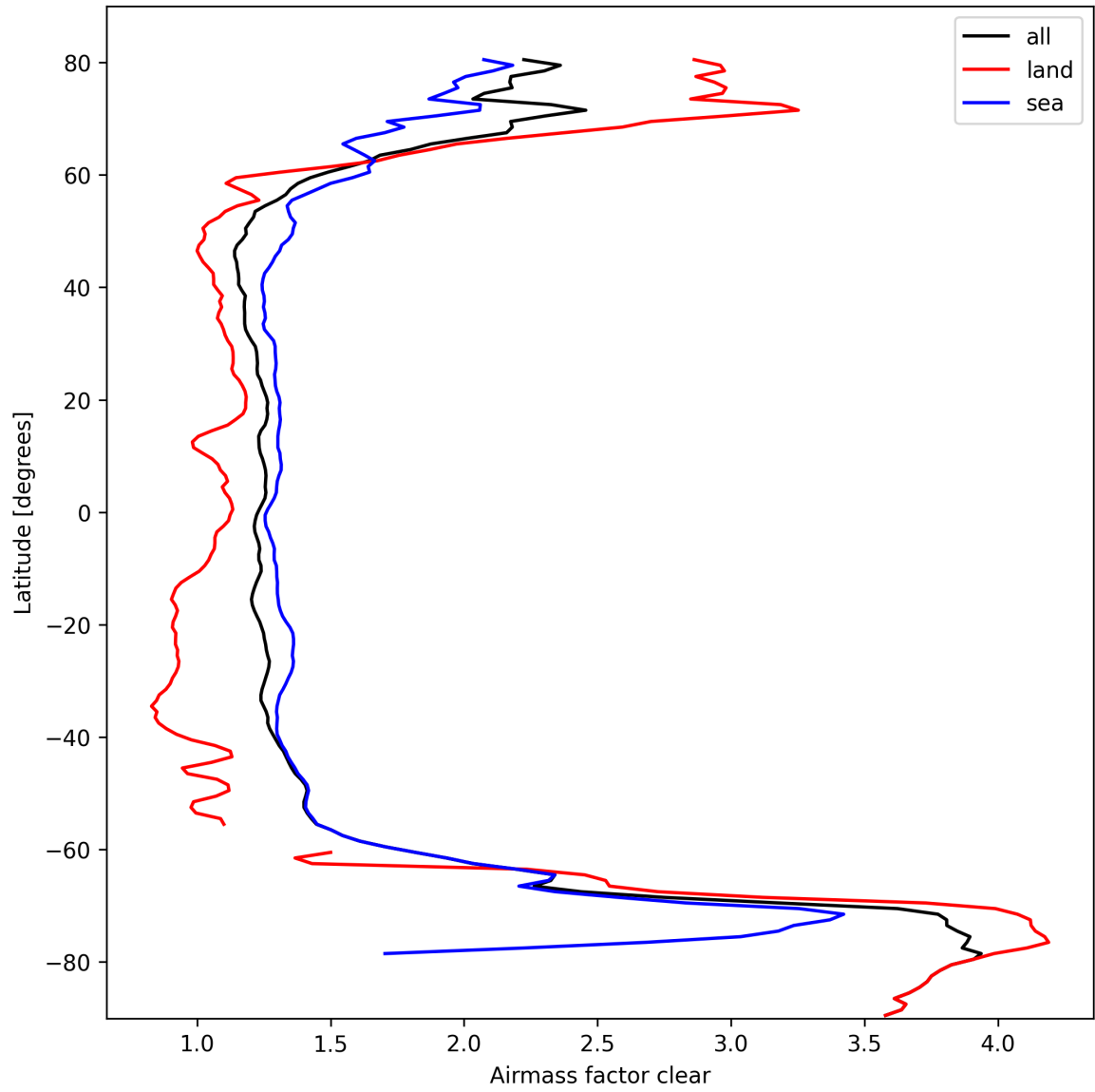
Figure 26: Zonal average of “Airmass factor clear” for 2025-10-03 to 2025-10-04.
