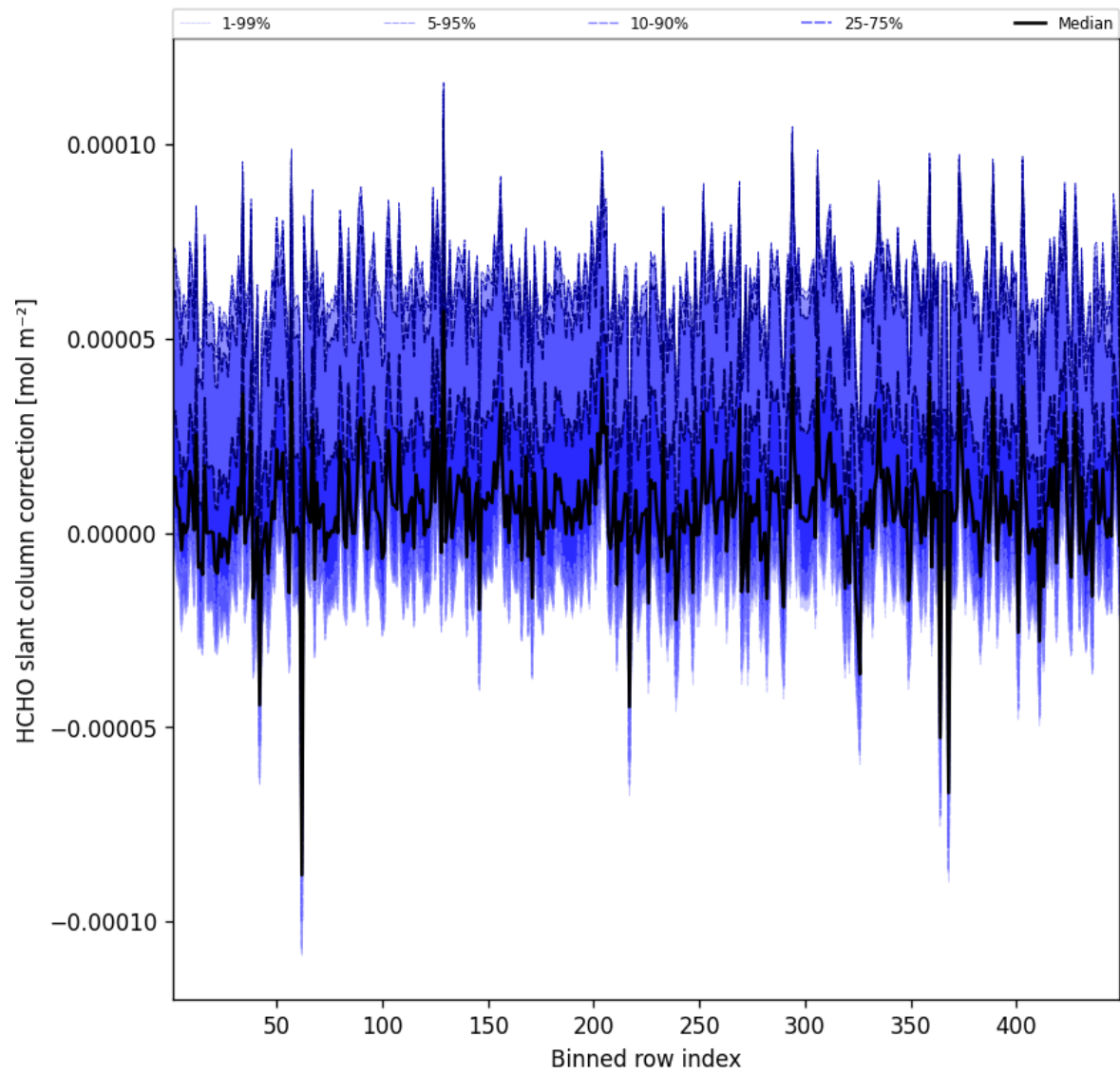
Figure 59: Along track statistics of “HCHO slant column correction” for 2025-10-03 to 2025-10-04
