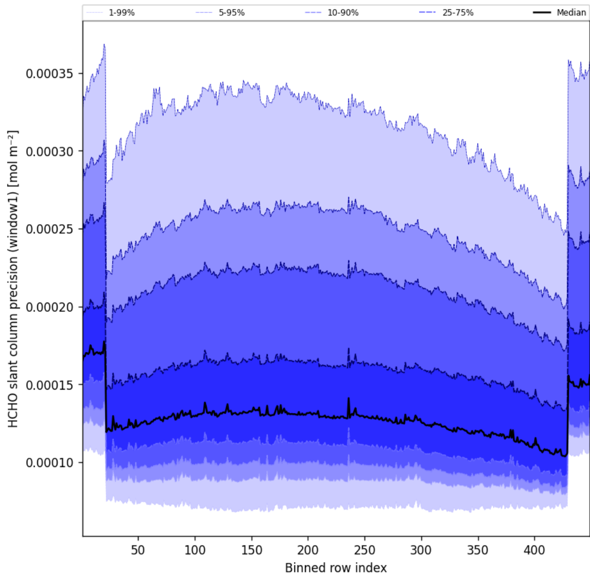
Figure 51: Along track statistics of “HCHO slant column precision (window1)” for 2025-10-03 to 2025-10-04
