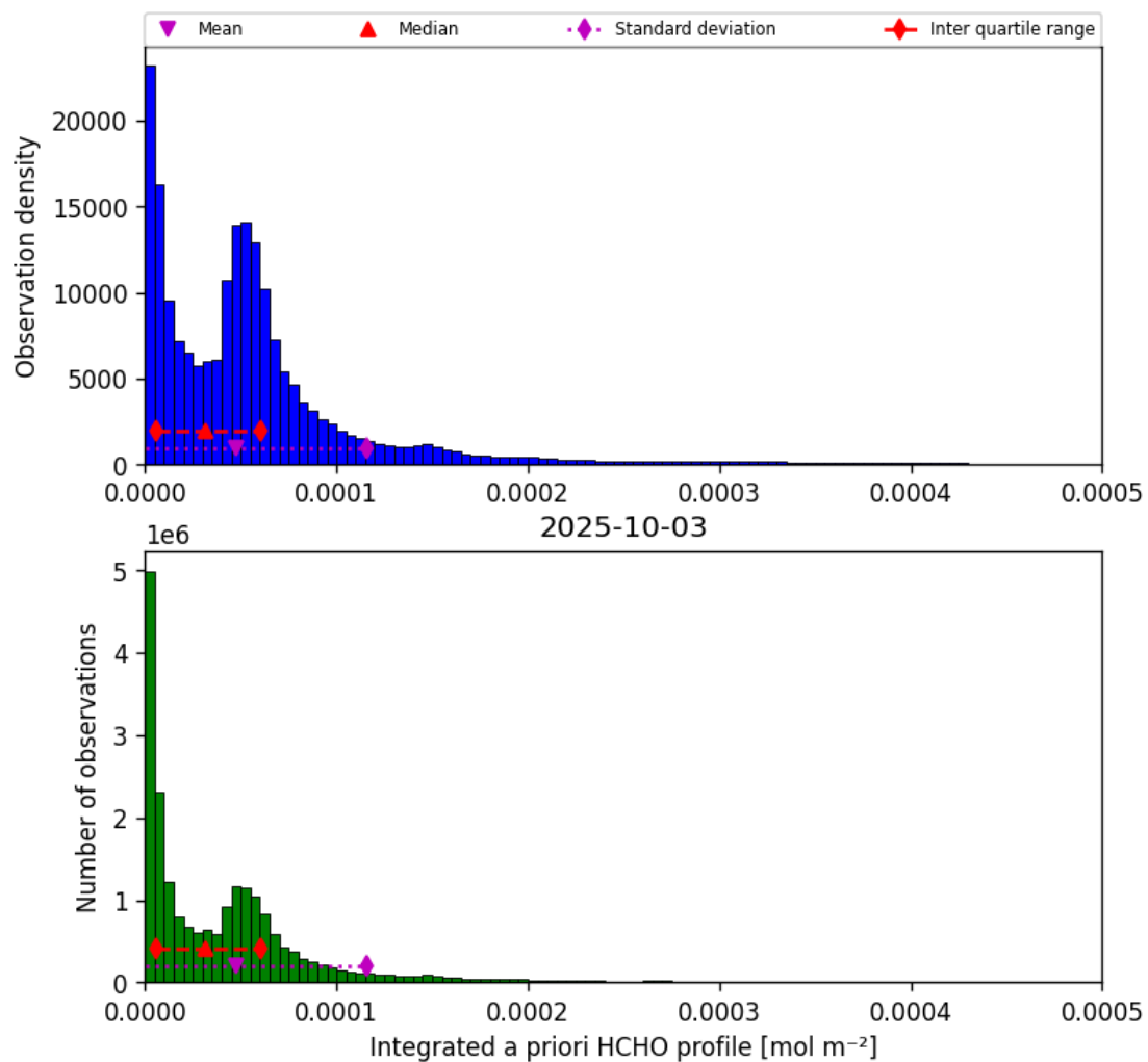
Figure 41: Histogram of “Integrated a priori HCHO profile” for 2025-10-03 to 2025-10-04
