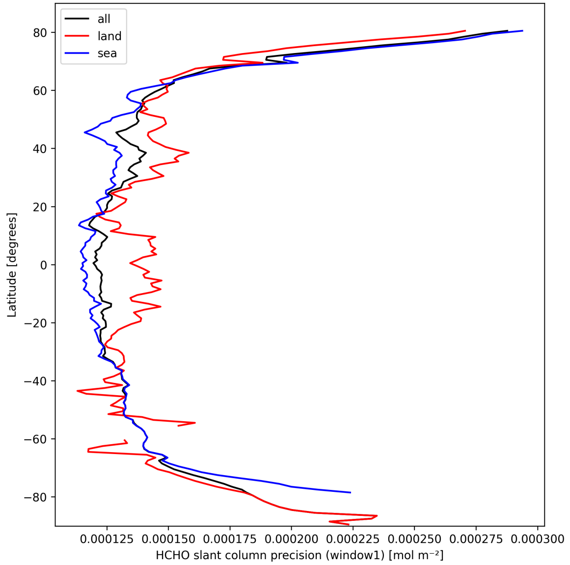
Figure 23: Zonal average of “HCHO slant column precision (window1)” for 2025-10-03 to 2025-10-04.
