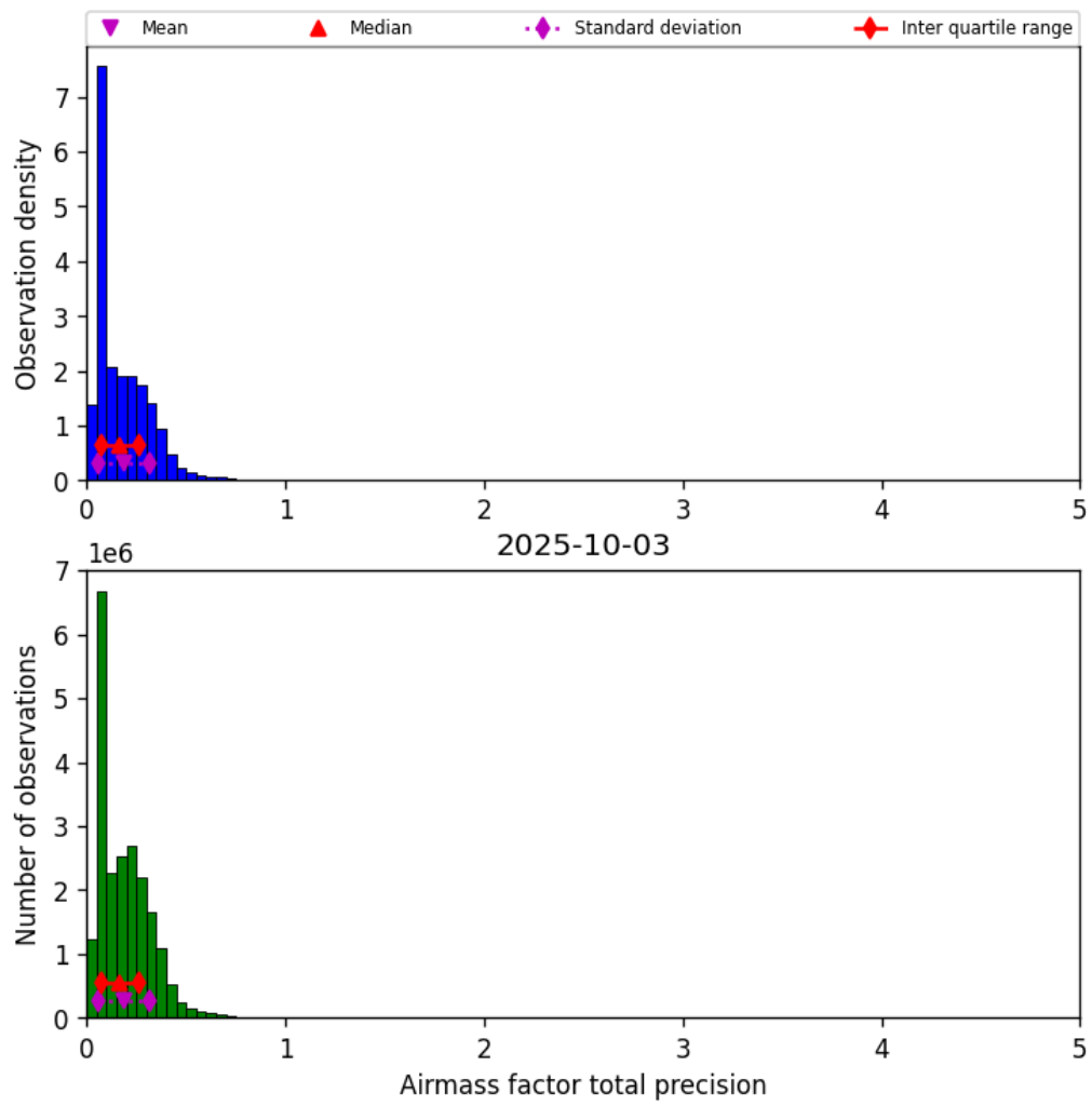
Figure 39: Histogram of “Airmass factor total precision” for 2025-10-03 to 2025-10-04
