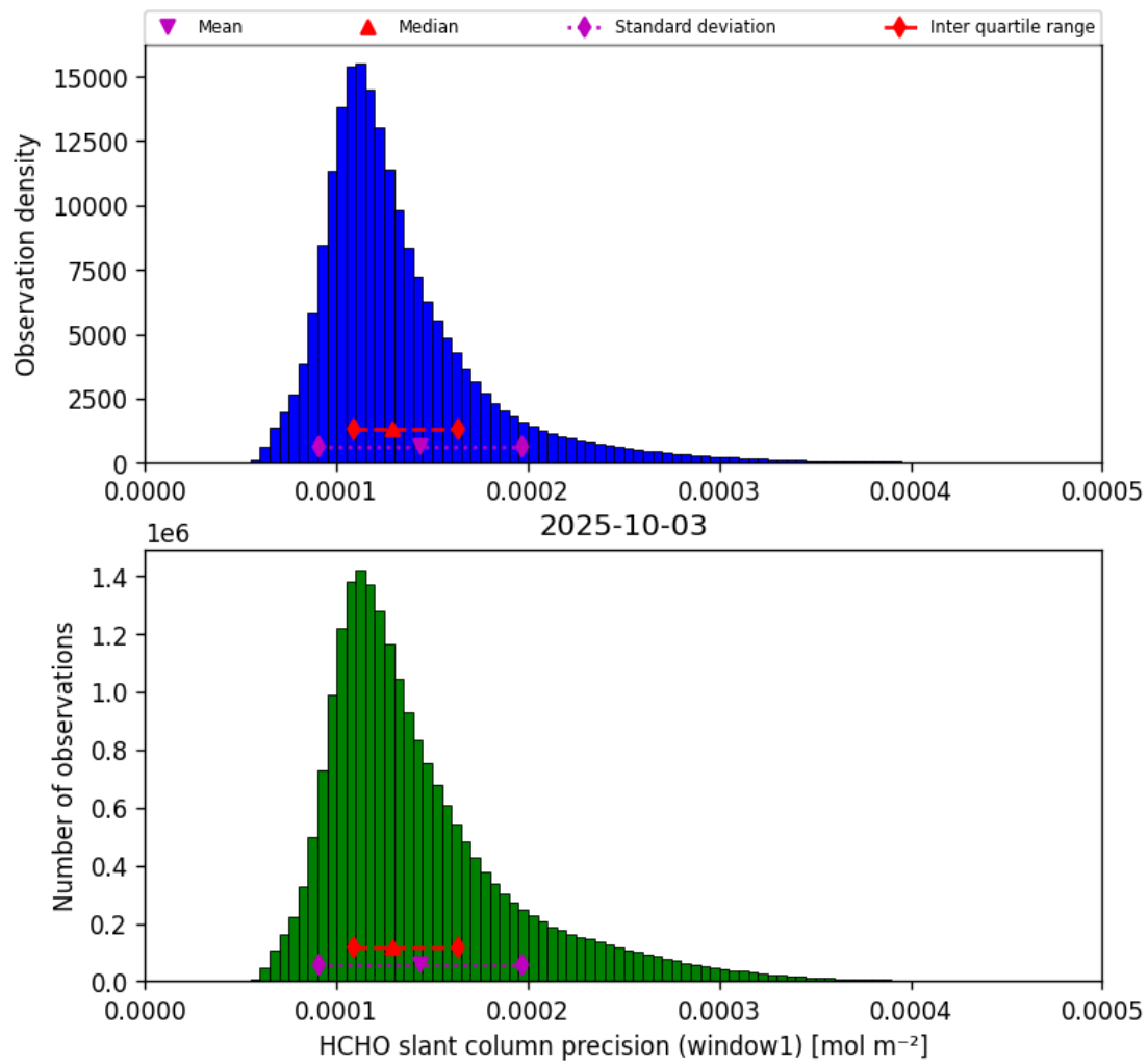
Figure 37: Histogram of “HCHO slant column precision (window1)” for 2025-10-03 to 2025-10-04
