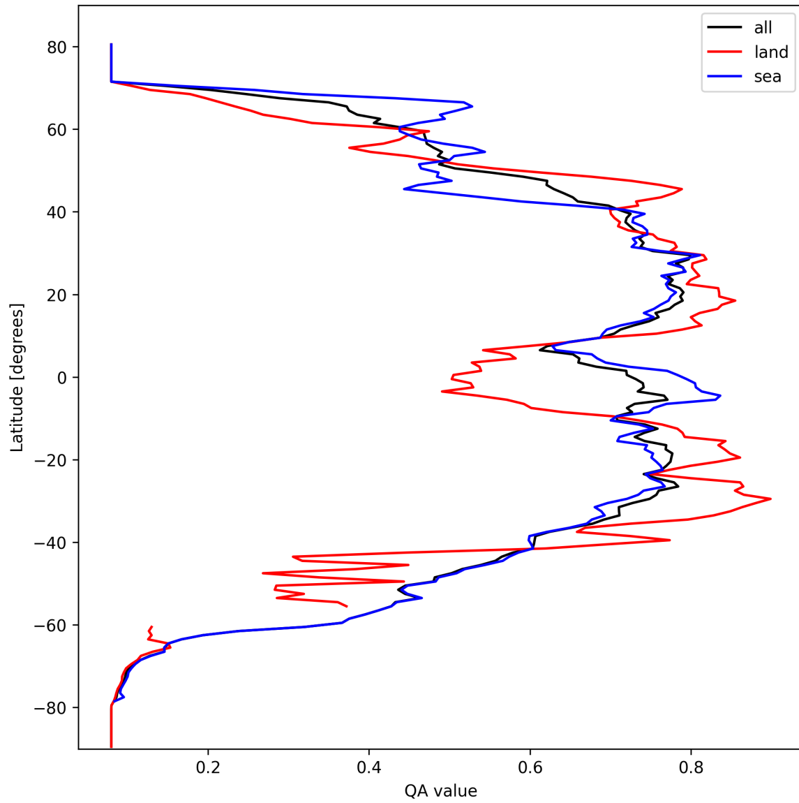
Figure 18: Zonal average of “QA value” for 2025-10-03 to 2025-10-04.
