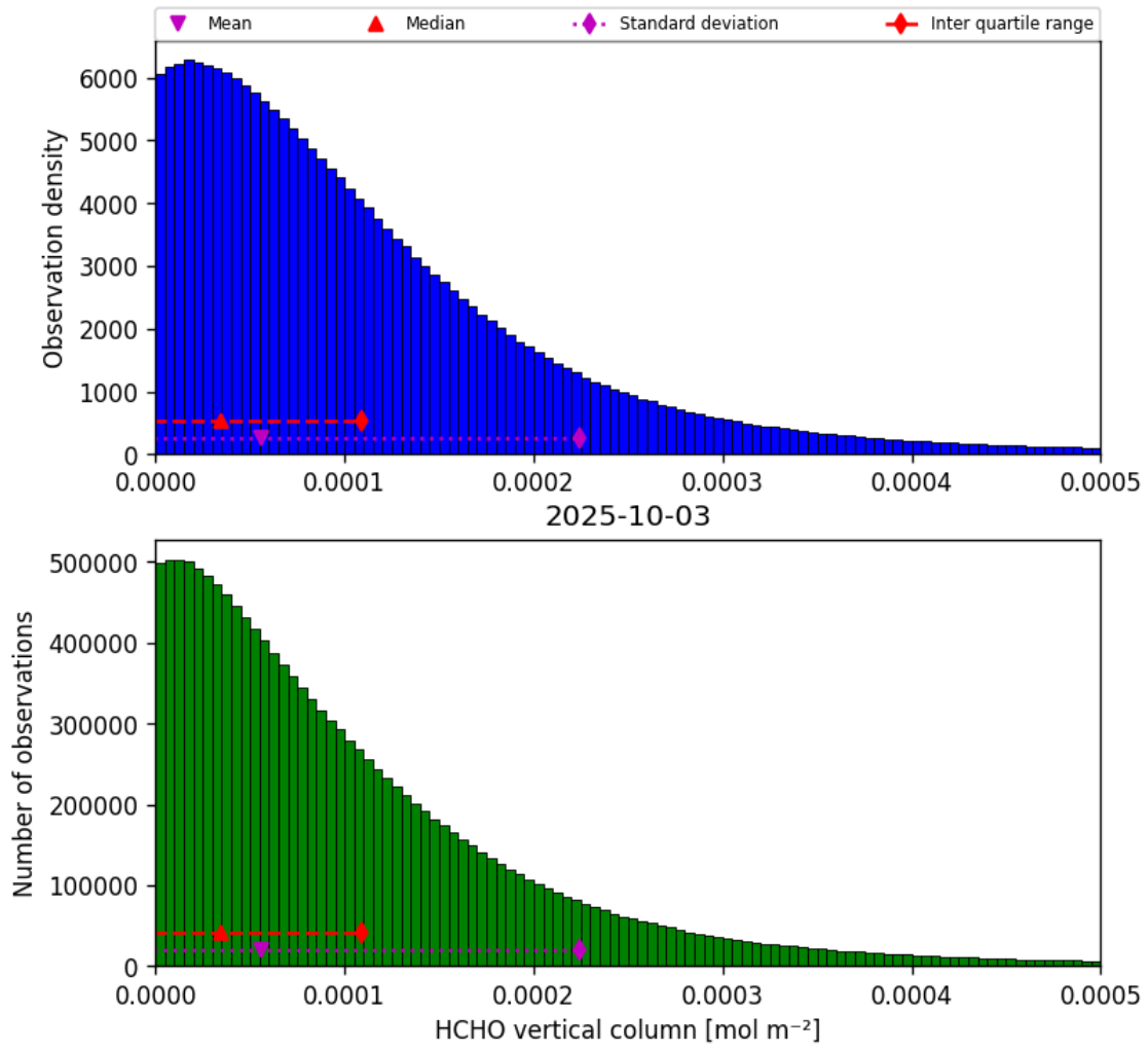
Figure 33: Histogram of “HCHO vertical column” for 2025-10-03 to 2025-10-04
