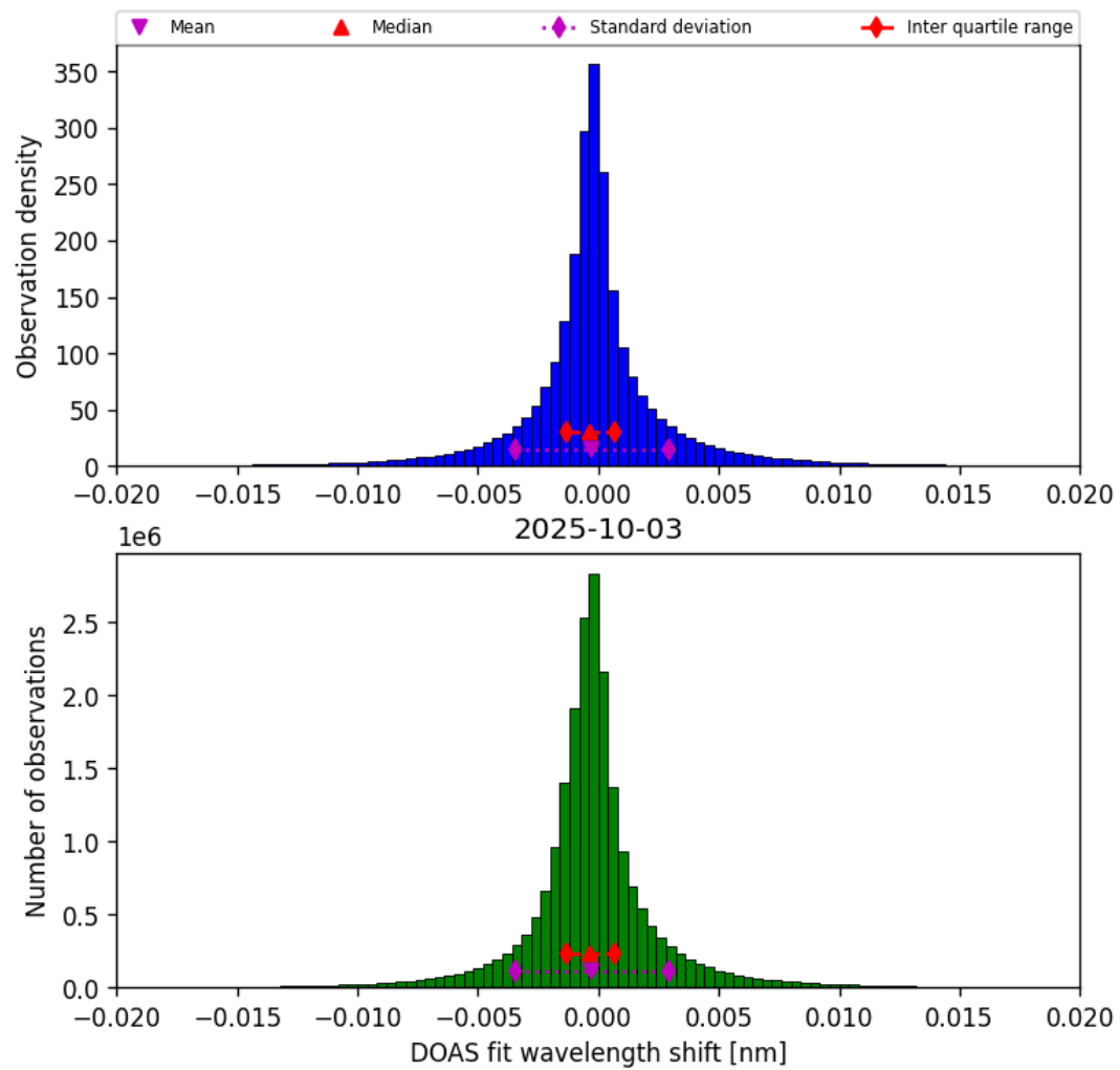
Figure 42: Histogram of “DOAS fit wavelength shift” for 2025-10-03 to 2025-10-04
