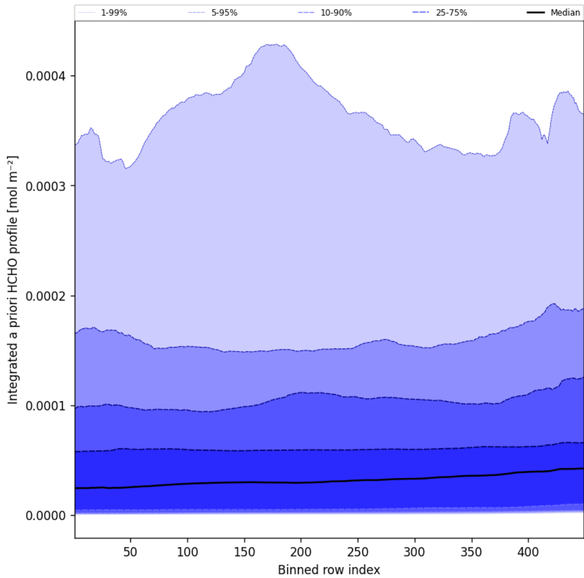
Figure 55: Along track statistics of "Integrated a priori HCHO profile" for 2025-10-03 to 2025-10-04
