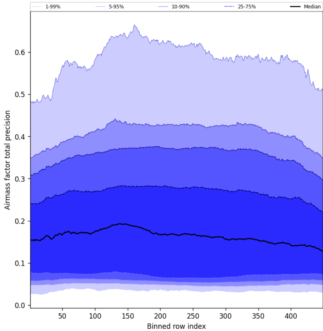
Figure 53: Along track statistics of “Airmass factor total precision” for 2025-10-03 to 2025-10-04
