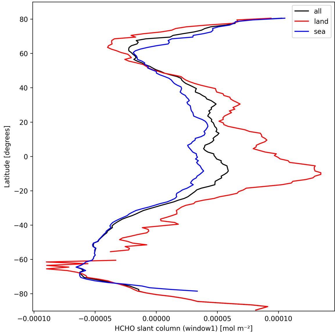
Figure 22: Zonal average of "HCHO slant column (window1)" for 2025-10-03 to 2025-10-04.
