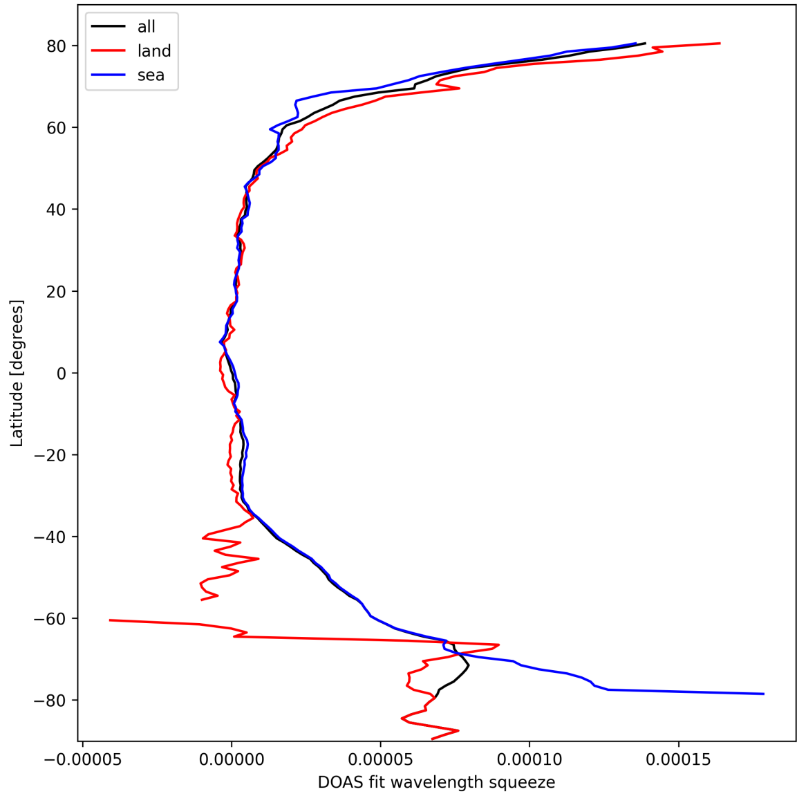
Figure 29: Zonal average of “DOAS fit wavelength squeeze” for 2025-10-03 to 2025-10-04.
