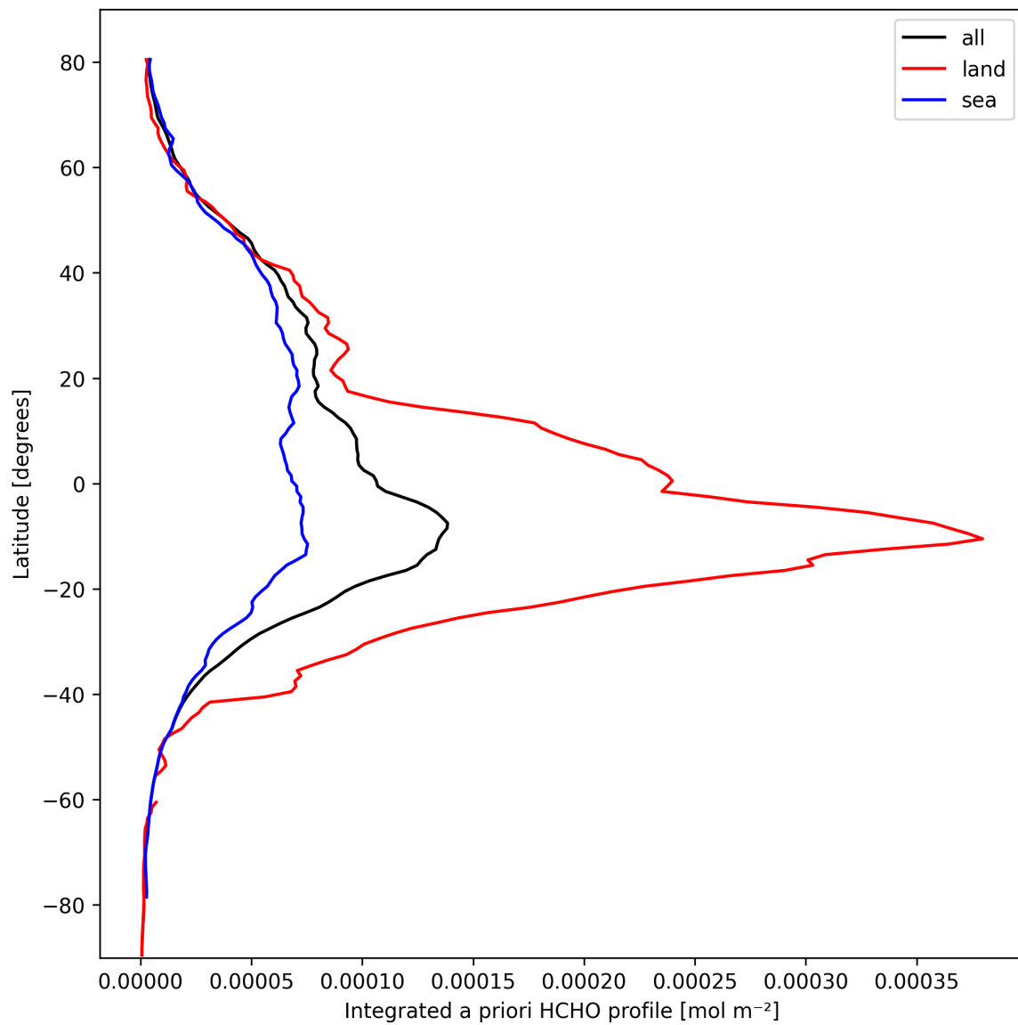
Figure 27: Zonal average of “Integrated a priori HCHO profile” for 2025-10-03 to 2025-10-04.
