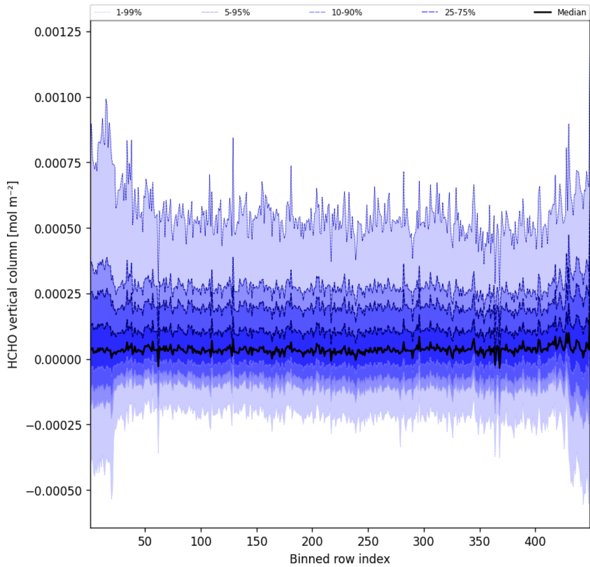
Figure 47: Along track statistics of “HCHO vertical column” for 2025-10-03 to 2025-10-04
