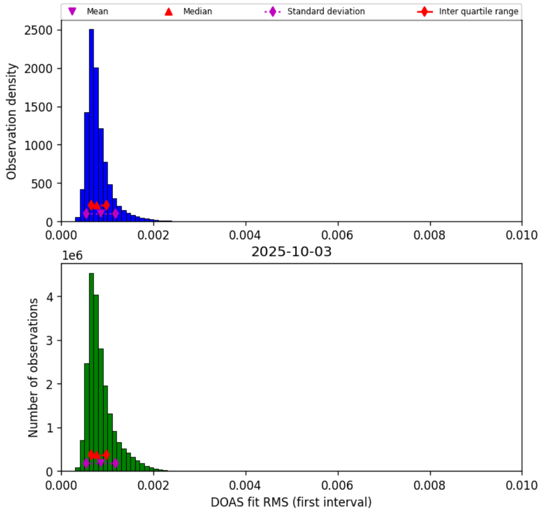
Figure 44: Histogram of “DOAS fit RMS (first interval)” for 2025-10-03 to 2025-10-04
