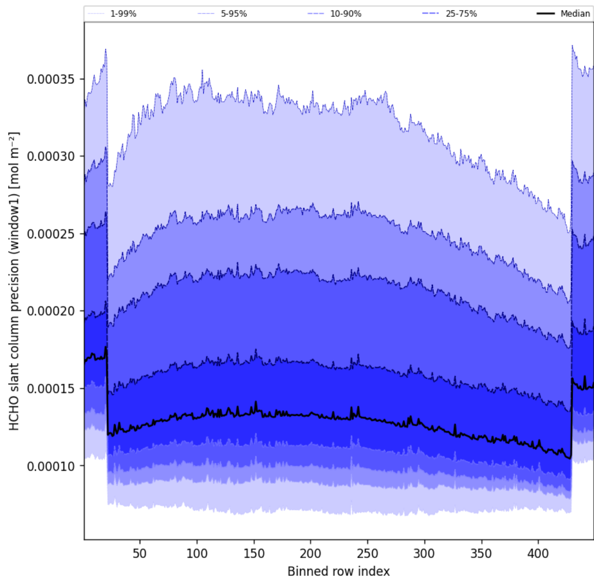
Figure 51: Along track statistics of “HCHO slant column precision (window1)” for 2025-10-04 to 2025-10-04
