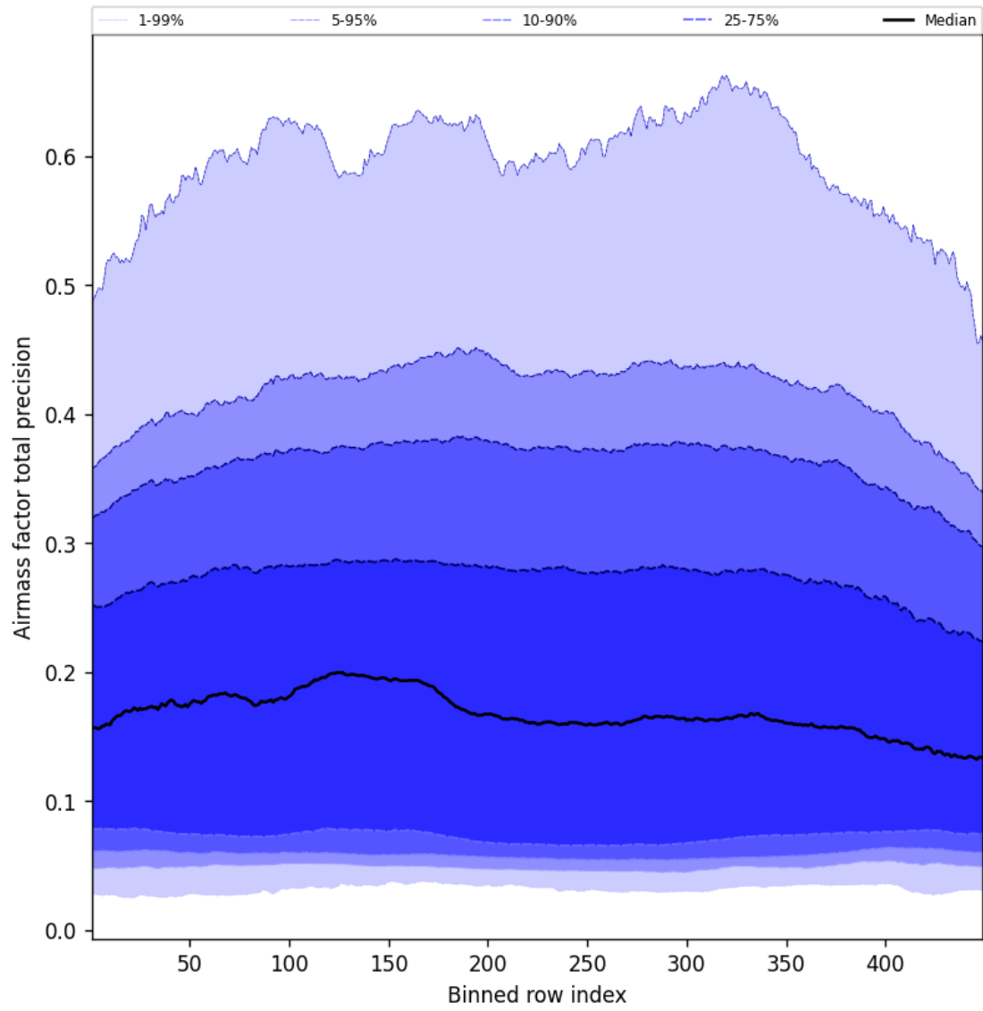
Figure 53: Along track statistics of “Airmass factor total precision” for 2025-10-04 to 2025-10-04
