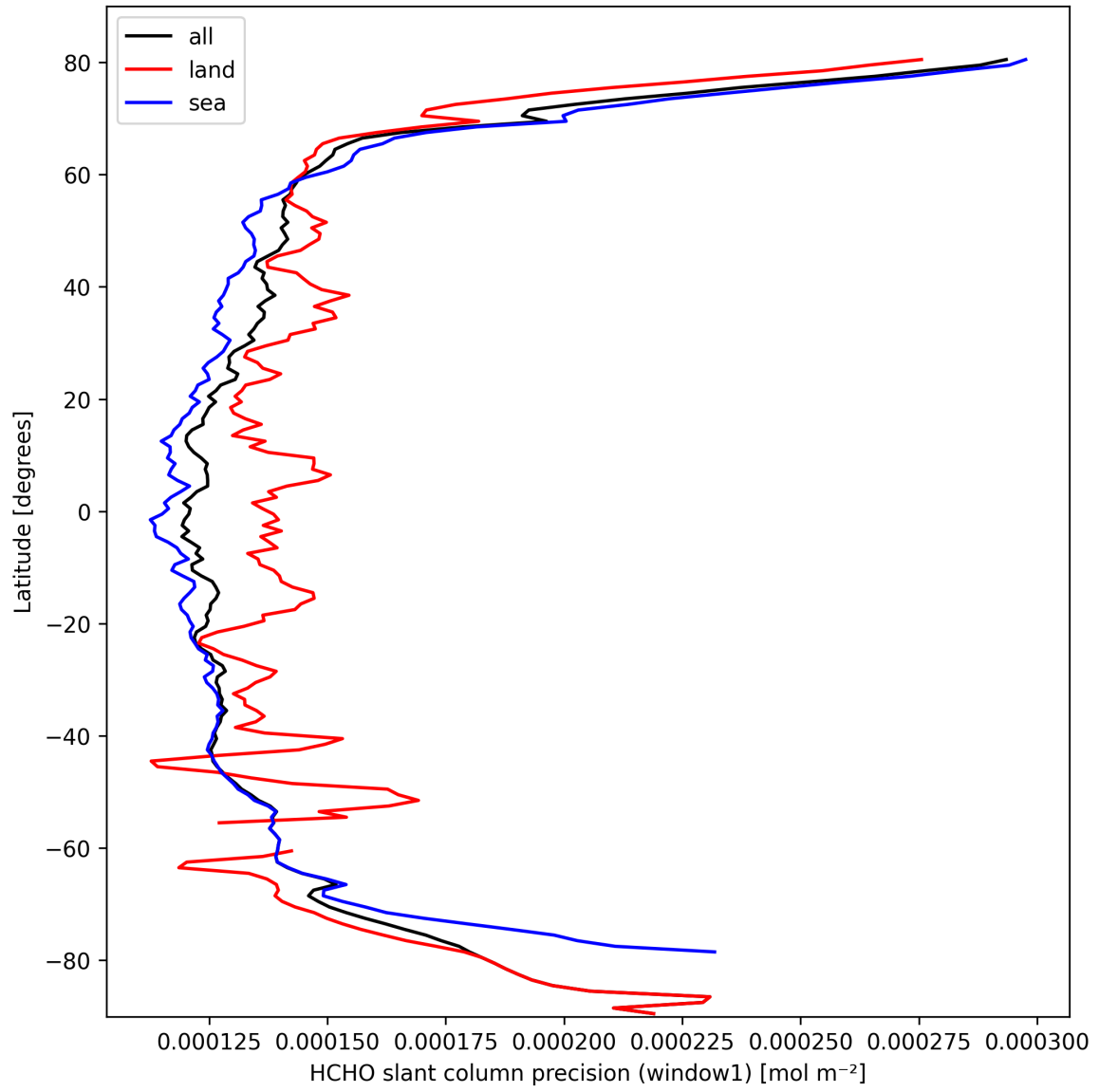
Figure 23: Zonal average of “HCHO slant column precision (window1)” for 2025-10-04 to 2025-10-04.
