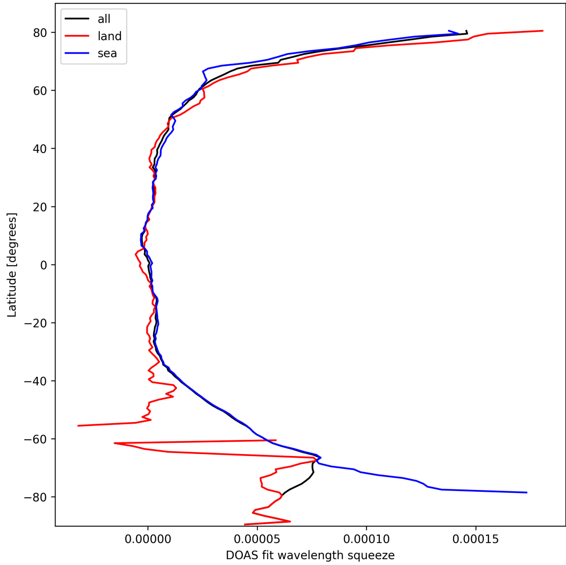
Figure 29: Zonal average of “DOAS fit wavelength squeeze” for 2025-10-04 to 2025-10-04.
