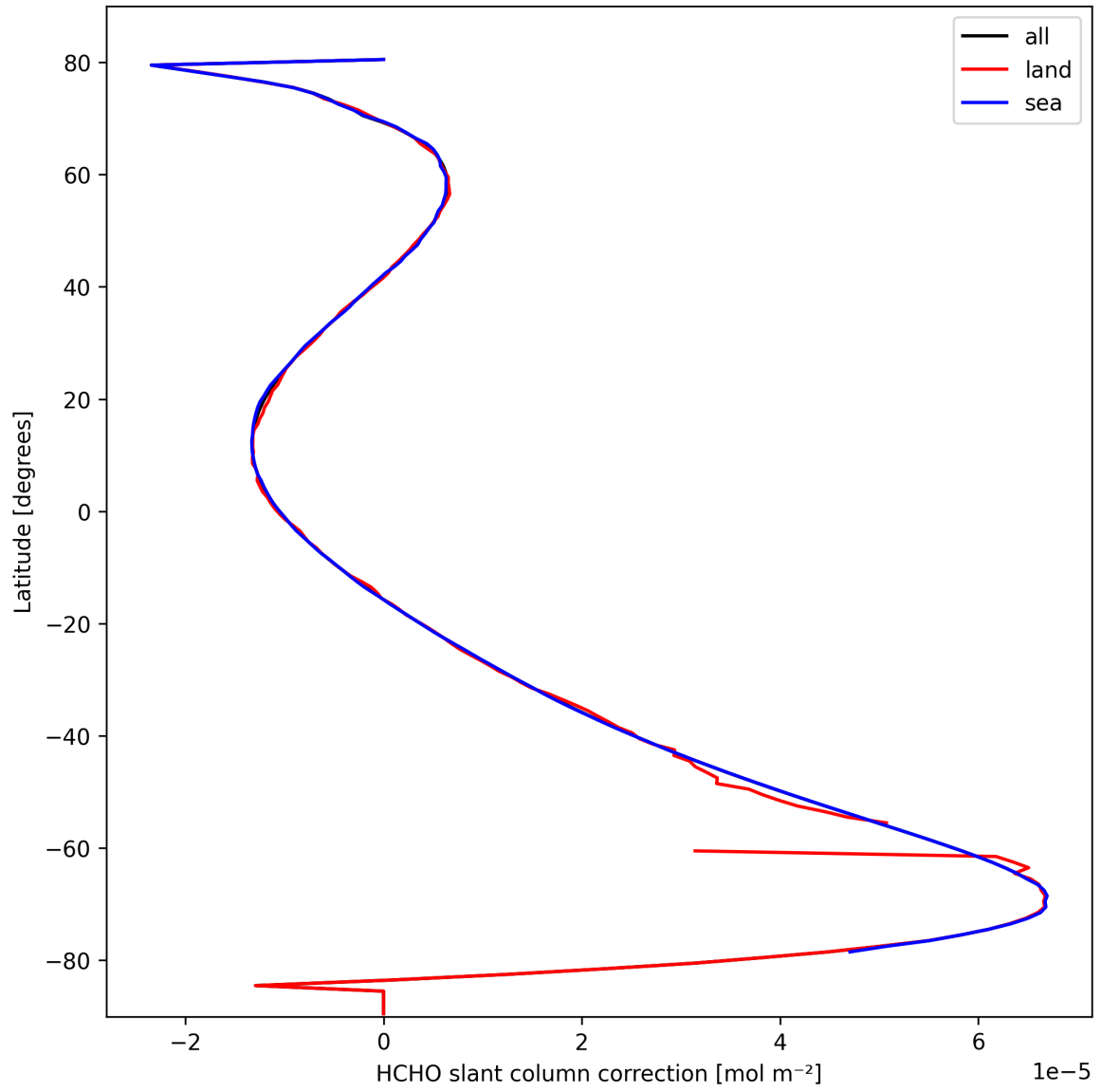
Figure 31: Zonal average of “HCHO slant column correction” for 2025-10-04 to 2025-10-04.
