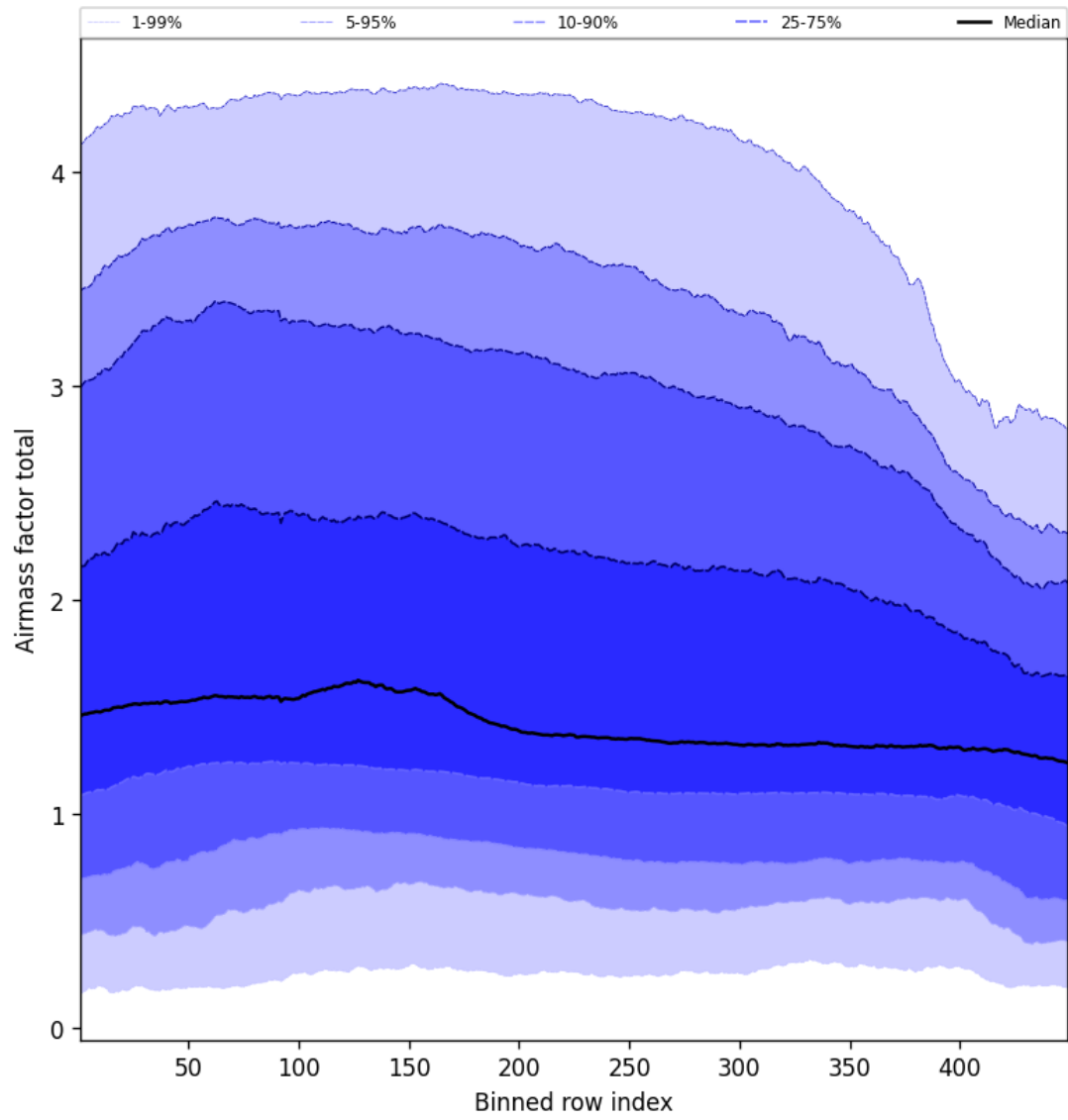
Figure 52: Along track statistics of “Airmass factor total” for 2025-10-04 to 2025-10-04
