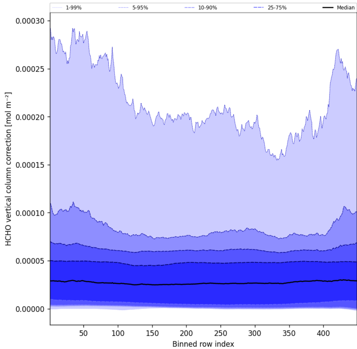
Figure 49: Along track statistics of “HCHO vertical column correction” for 2025-10-04 to 2025-10-04
