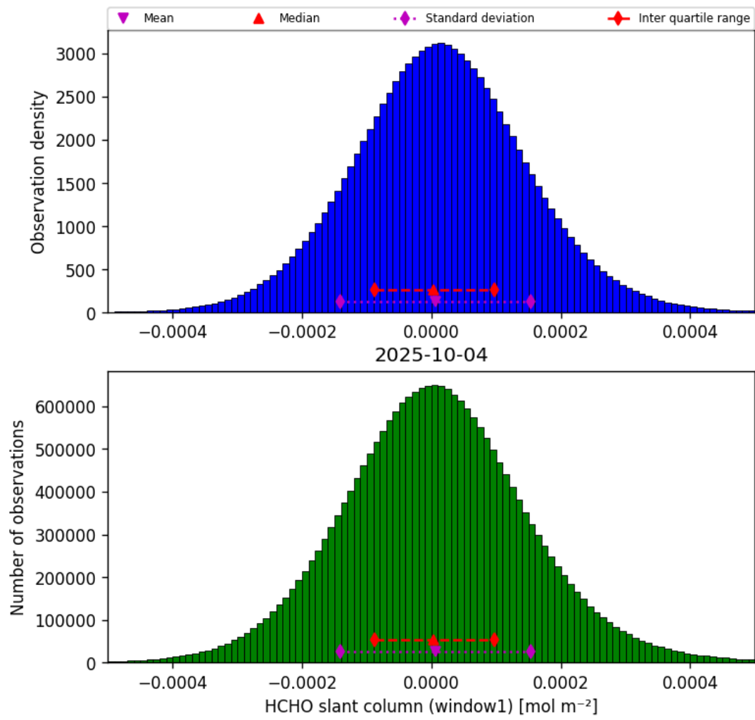
Figure 36: Histogram of “HCHO slant column (window1)” for 2025-10-04 to 2025-10-04
