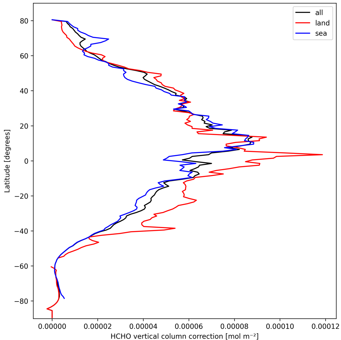
Figure 21: Zonal average of “HCHO vertical column correction” for 2025-10-04 to 2025-10-04.
