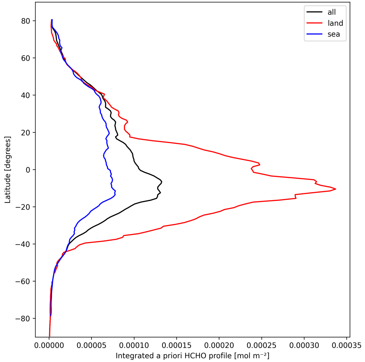
Figure 27: Zonal average of “Integrated a priori HCHO profile” for 2025-10-04 to 2025-10-04.
