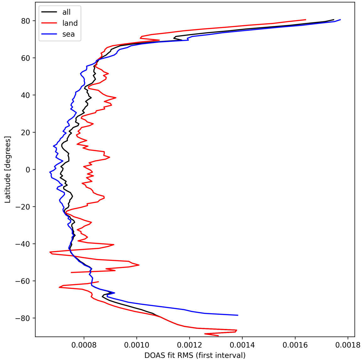
Figure 30: Zonal average of “DOAS fit RMS (first interval)” for 2025-10-04 to 2025-10-04.
