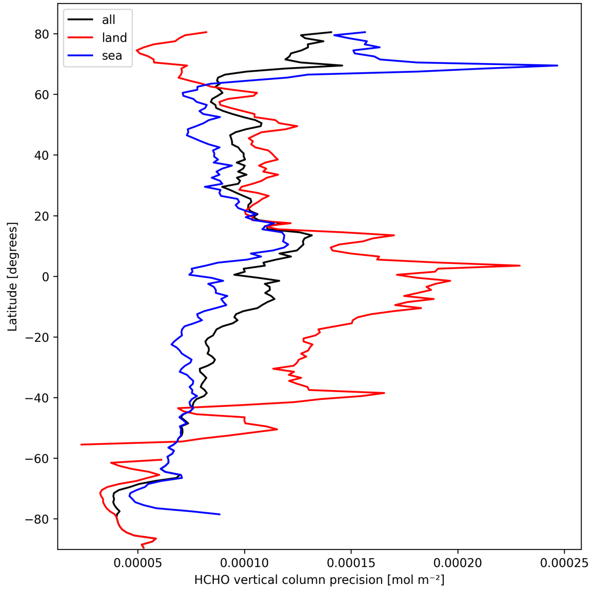
Figure 20: Zonal average of “HCHO vertical column precision” for 2025-10-04 to 2025-10-04.
