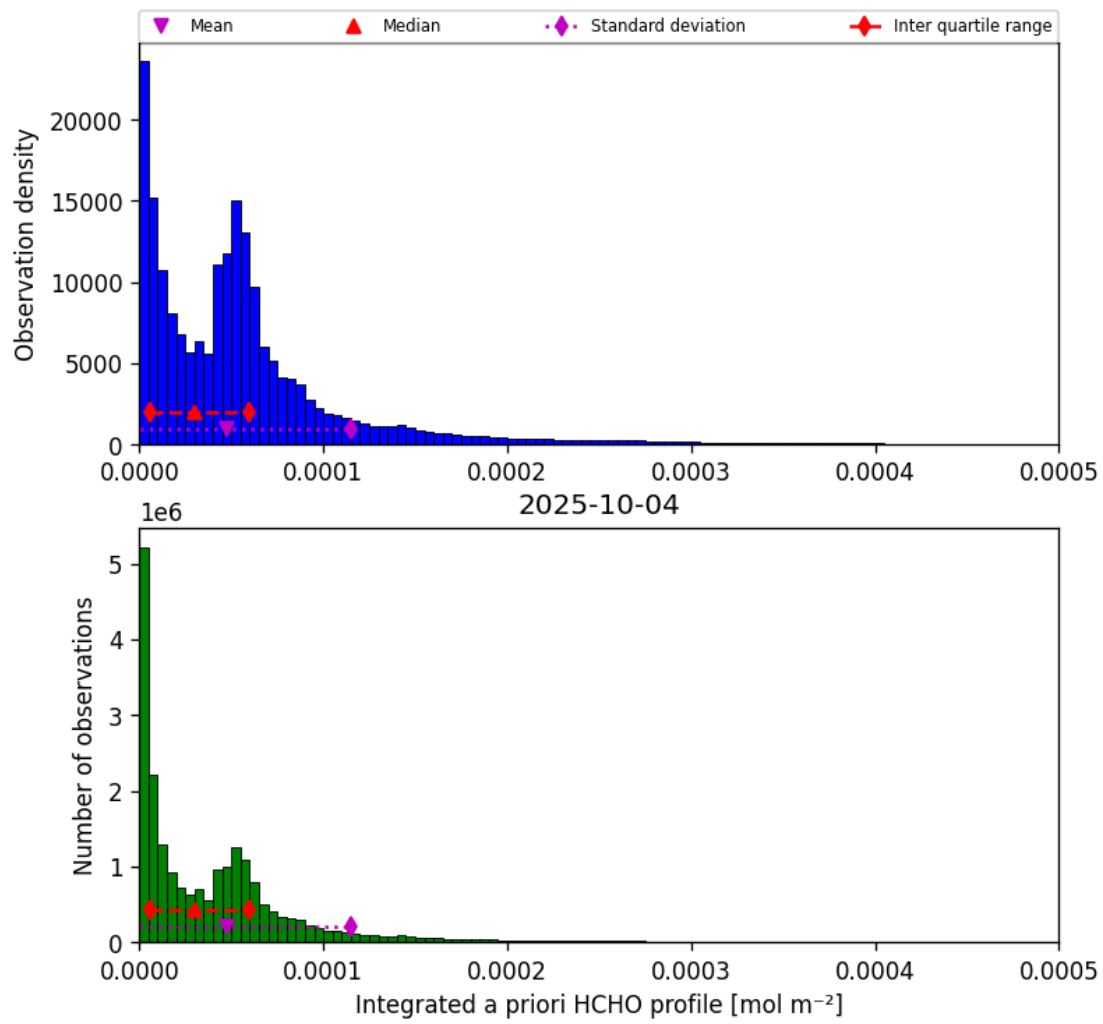
Figure 41: Histogram of “Integrated a priori HCHO profile” for 2025-10-04 to 2025-10-04
