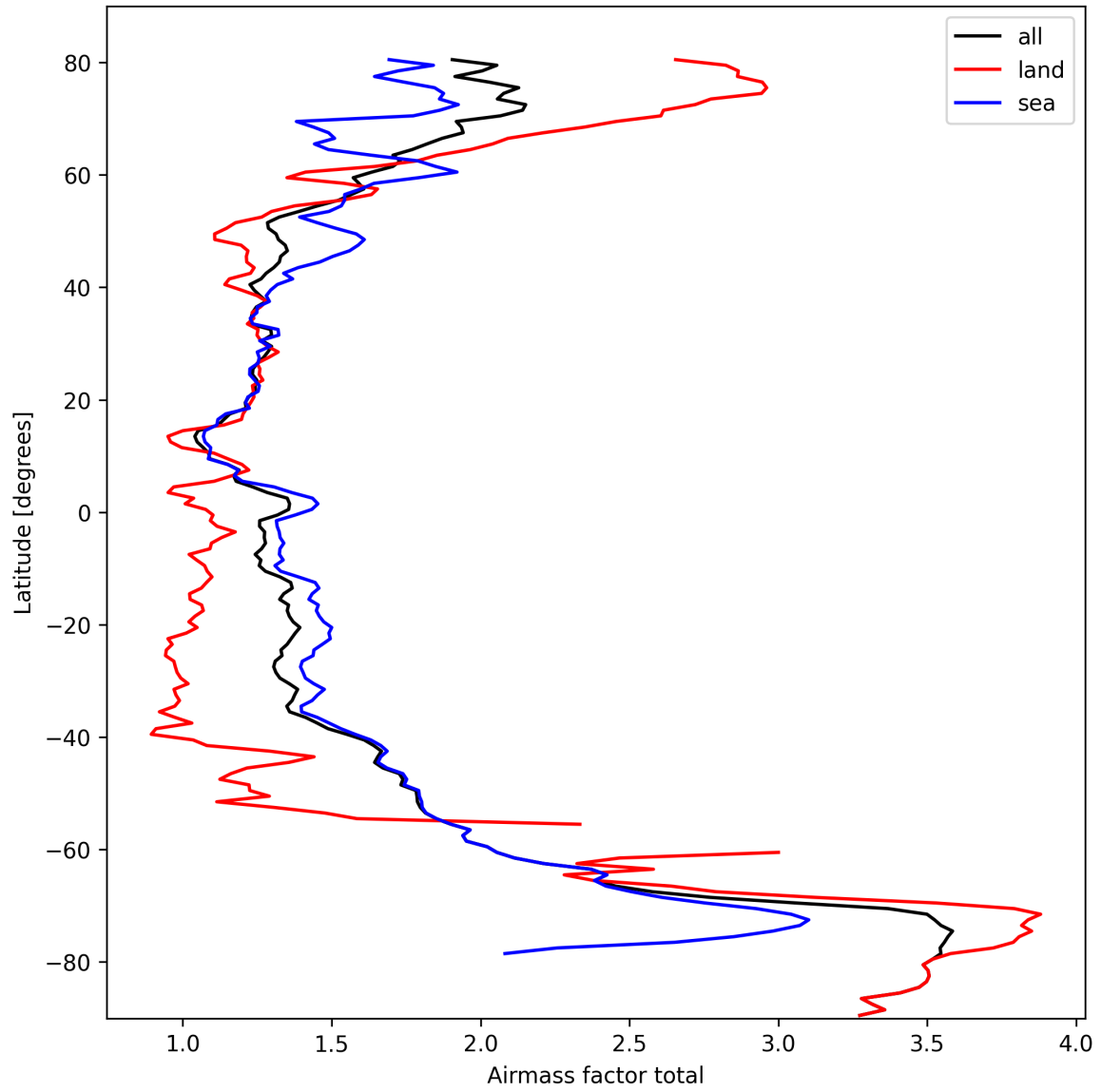
Figure 24: Zonal average of “Airmass factor total” for 2025-10-04 to 2025-10-04.
