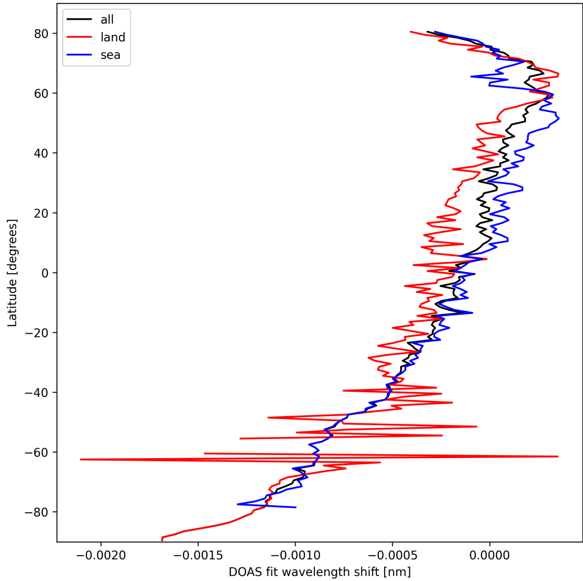
Figure 28: Zonal average of “DOAS fit wavelength shift” for 2025-10-04 to 2025-10-04.
