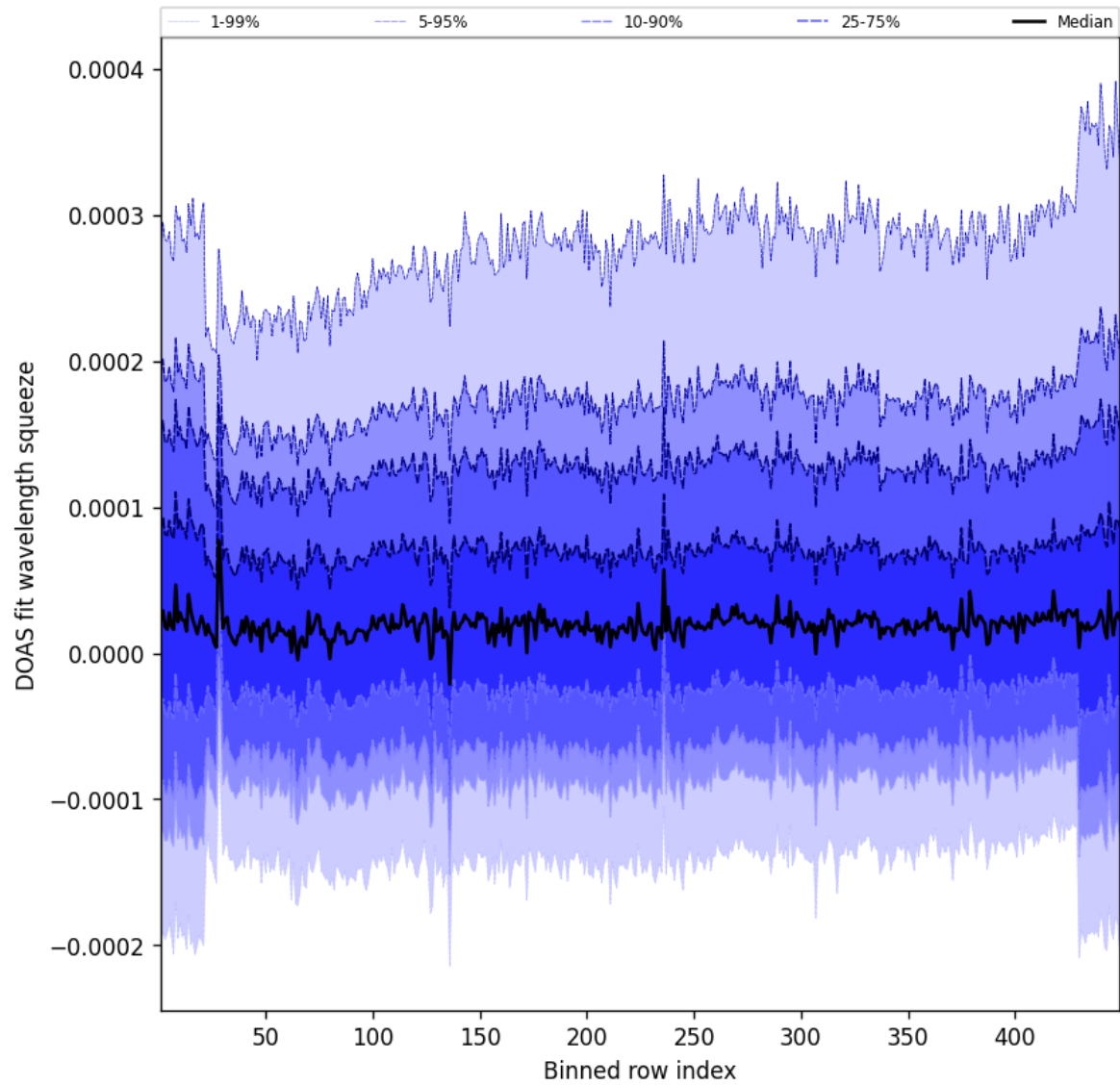
Figure 57: Along track statistics of “DOAS fit wavelength squeeze” for 2025-10-04 to 2025-10-04
