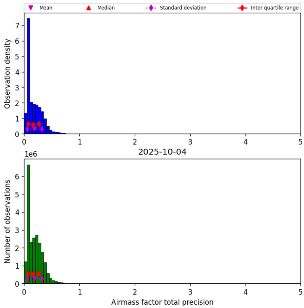
Figure 39: Histogram of “Airmass factor total precision” for 2025-10-04 to 2025-10-04
