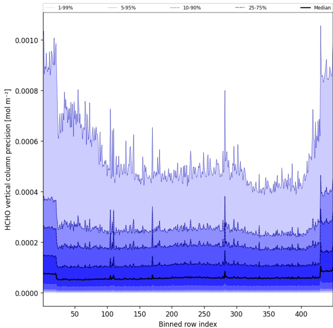
Figure 48: Along track statistics of “HCHO vertical column precision” for 2025-10-04 to 2025-10-04
