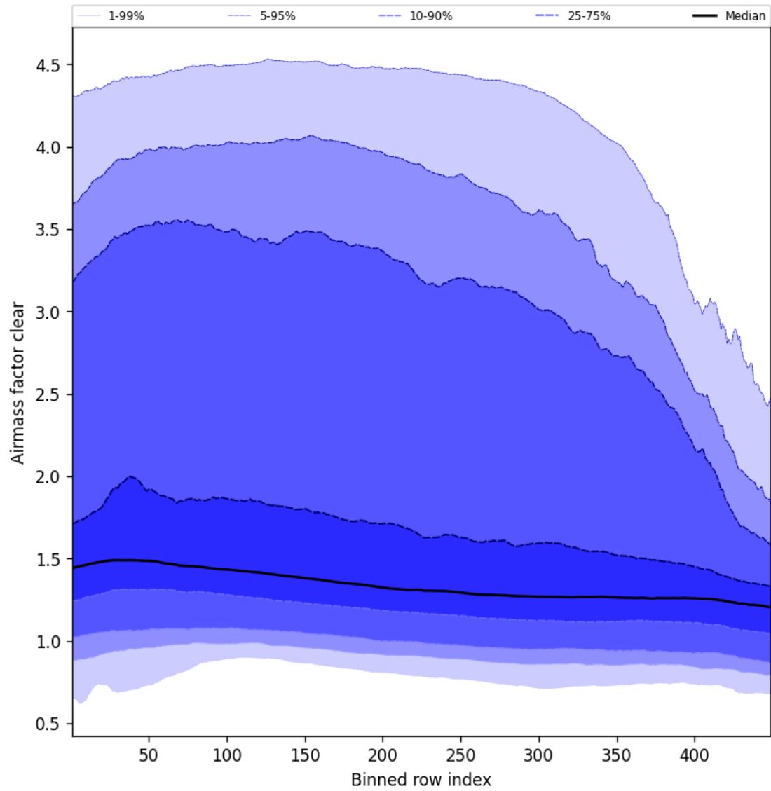
Figure 54: Along track statistics of “Airmass factor clear” for 2025-10-04 to 2025-10-04
