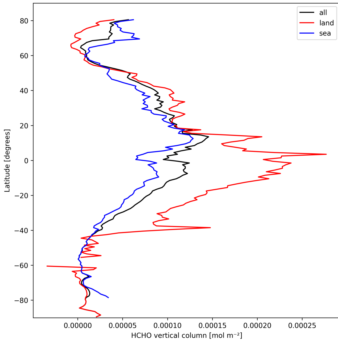
Figure 19: Zonal average of “HCHO vertical column” for 2025-10-04 to 2025-10-04.
