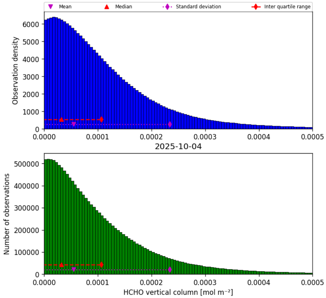
Figure 33: Histogram of “HCHO vertical column” for 2025-10-04 to 2025-10-04
