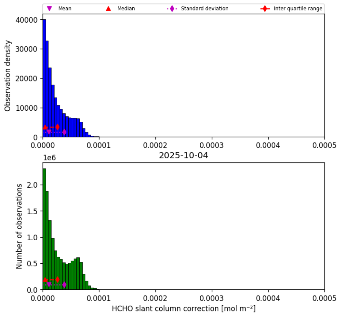
Figure 45: Histogram of “HCHO slant column correction” for 2025-10-04 to 2025-10-04
