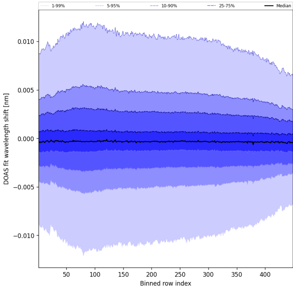
Figure 56: Along track statistics of “DOAS fit wavelength shift” for 2025-10-04 to 2025-10-04
