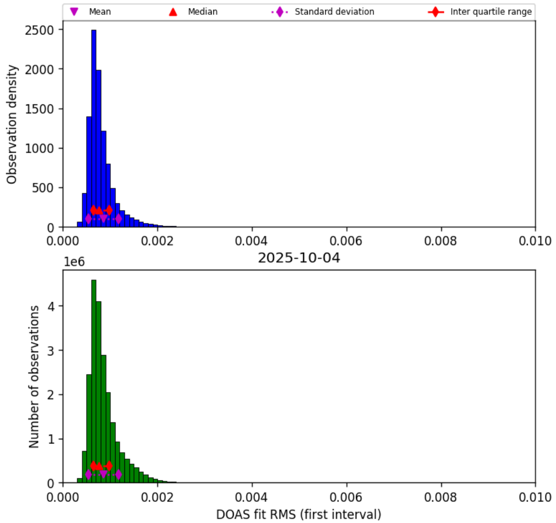
Figure 44: Histogram of “DOAS fit RMS (first interval)” for 2025-10-04 to 2025-10-04
