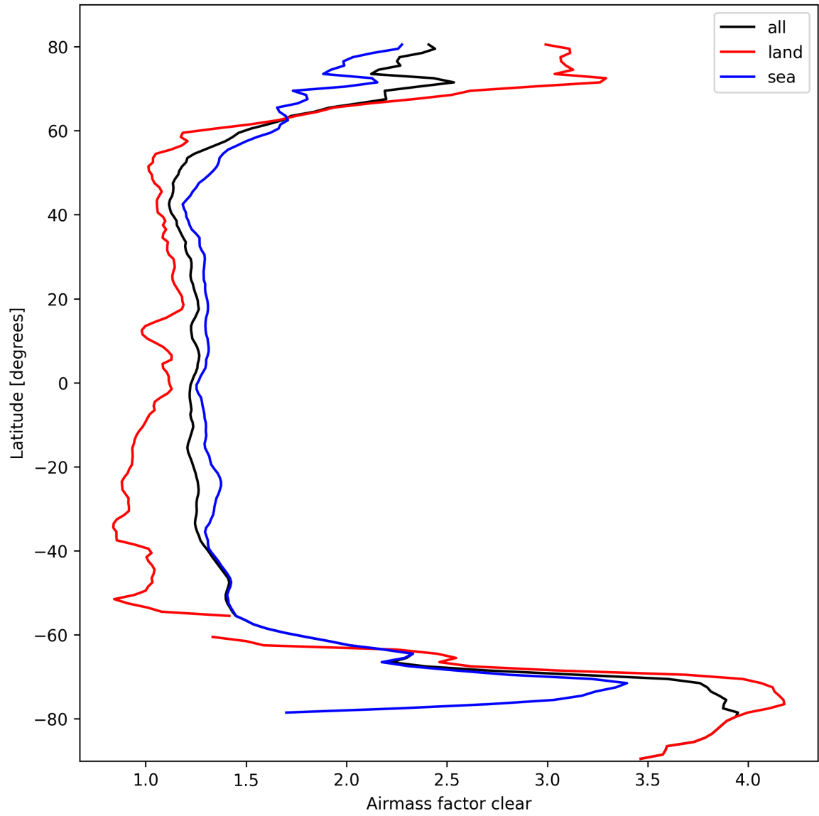
Figure 26: Zonal average of “Airmass factor clear” for 2025-10-04 to 2025-10-04.
