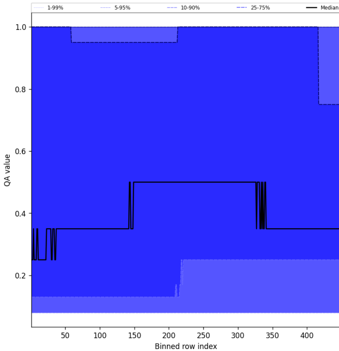
Figure 46: Along track statistics of “QA value” for 2025-10-04 to 2025-10-04
