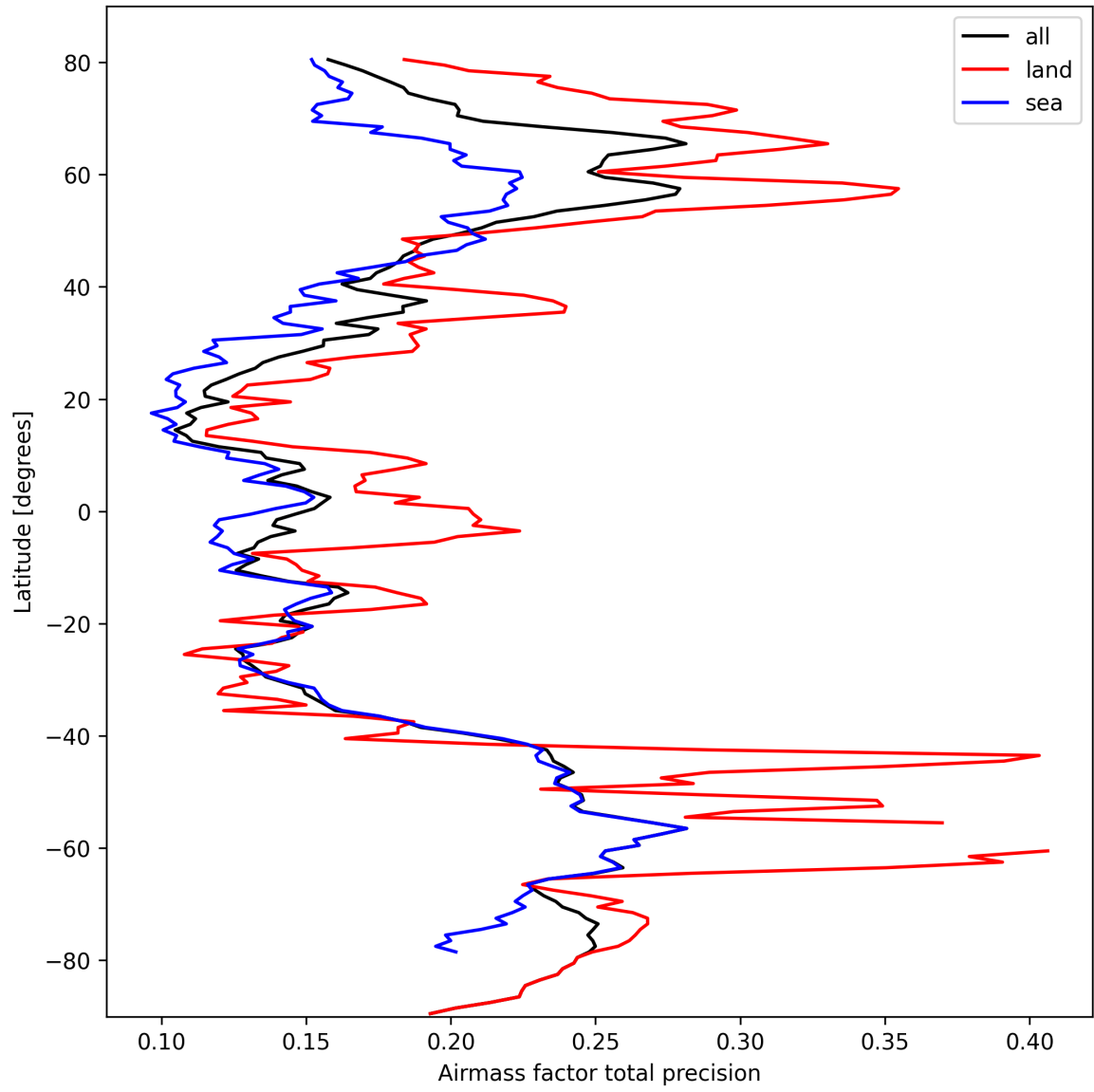
Figure 25: Zonal average of “Airmass factor total precision” for 2025-10-04 to 2025-10-04.
