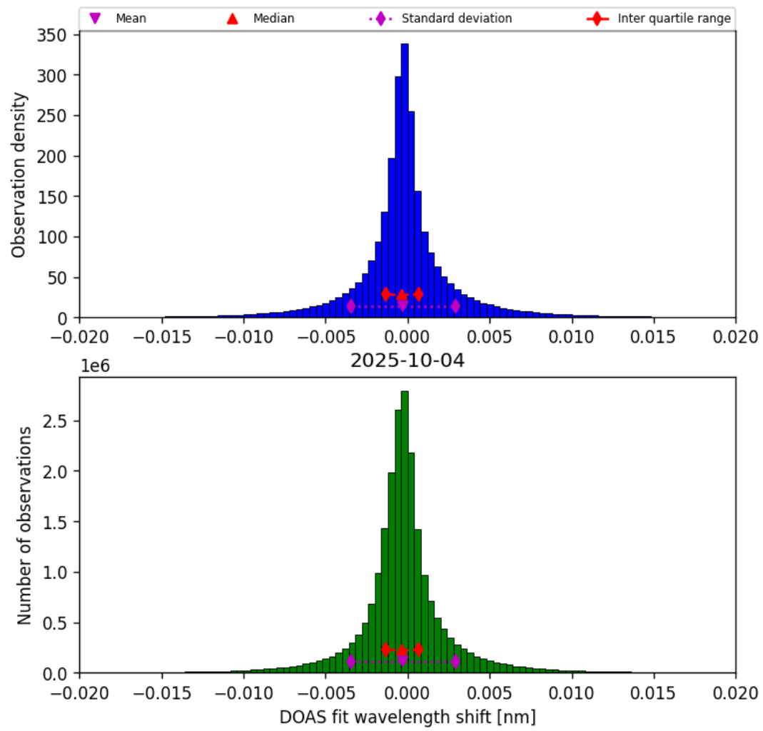
Figure 42: Histogram of “DOAS fit wavelength shift” for 2025-10-04 to 2025-10-04
