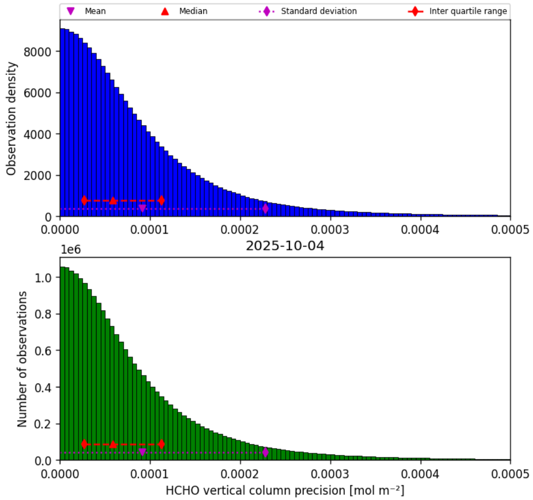
Figure 34: Histogram of “HCHO vertical column precision” for 2025-10-04 to 2025-10-04
