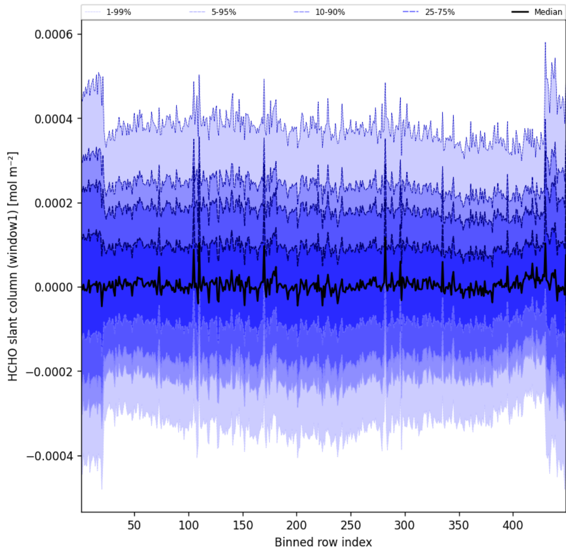
Figure 50: Along track statistics of “HCHO slant column (window1)” for 2025-10-04 to 2025-10-04
