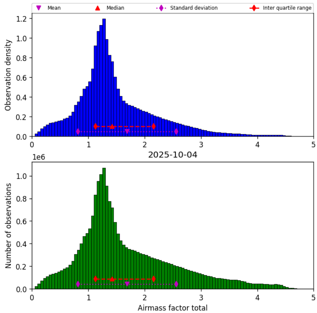
Figure 38: Histogram of “Airmass factor total” for 2025-10-04 to 2025-10-04
