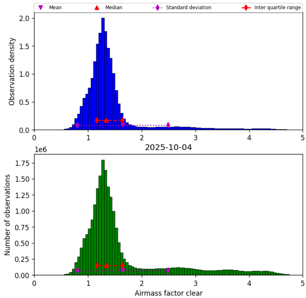
Figure 40: Histogram of “Airmass factor clear” for 2025-10-04 to 2025-10-04
