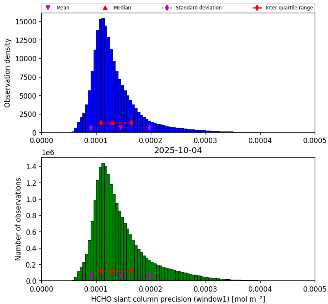
Figure 37: Histogram of “HCHO slant column precision (window1)” for 2025-10-04 to 2025-10-04
