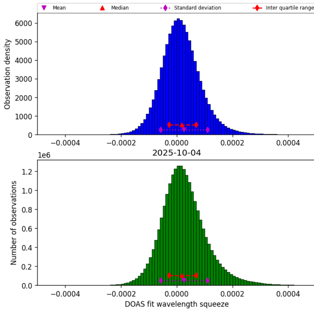
Figure 43: Histogram of “DOAS fit wavelength squeeze” for 2025-10-04 to 2025-10-04
