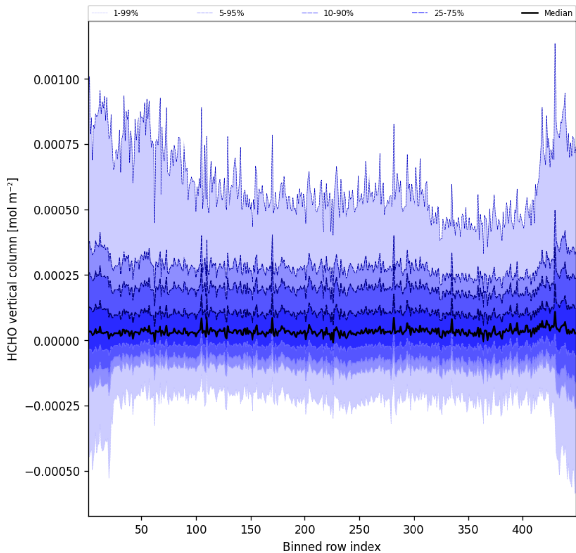
Figure 47: Along track statistics of “HCHO vertical column” for 2025-10-04 to 2025-10-04
