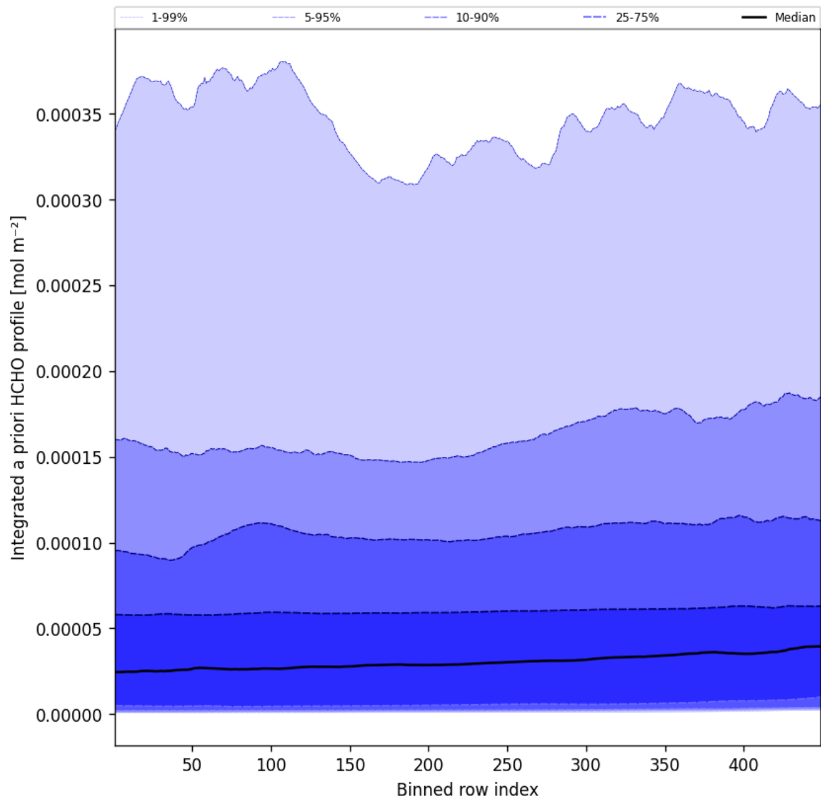
Figure 55: Along track statistics of "Integrated a priori HCHO profile" for 2025-10-04 to 2025-10-04
