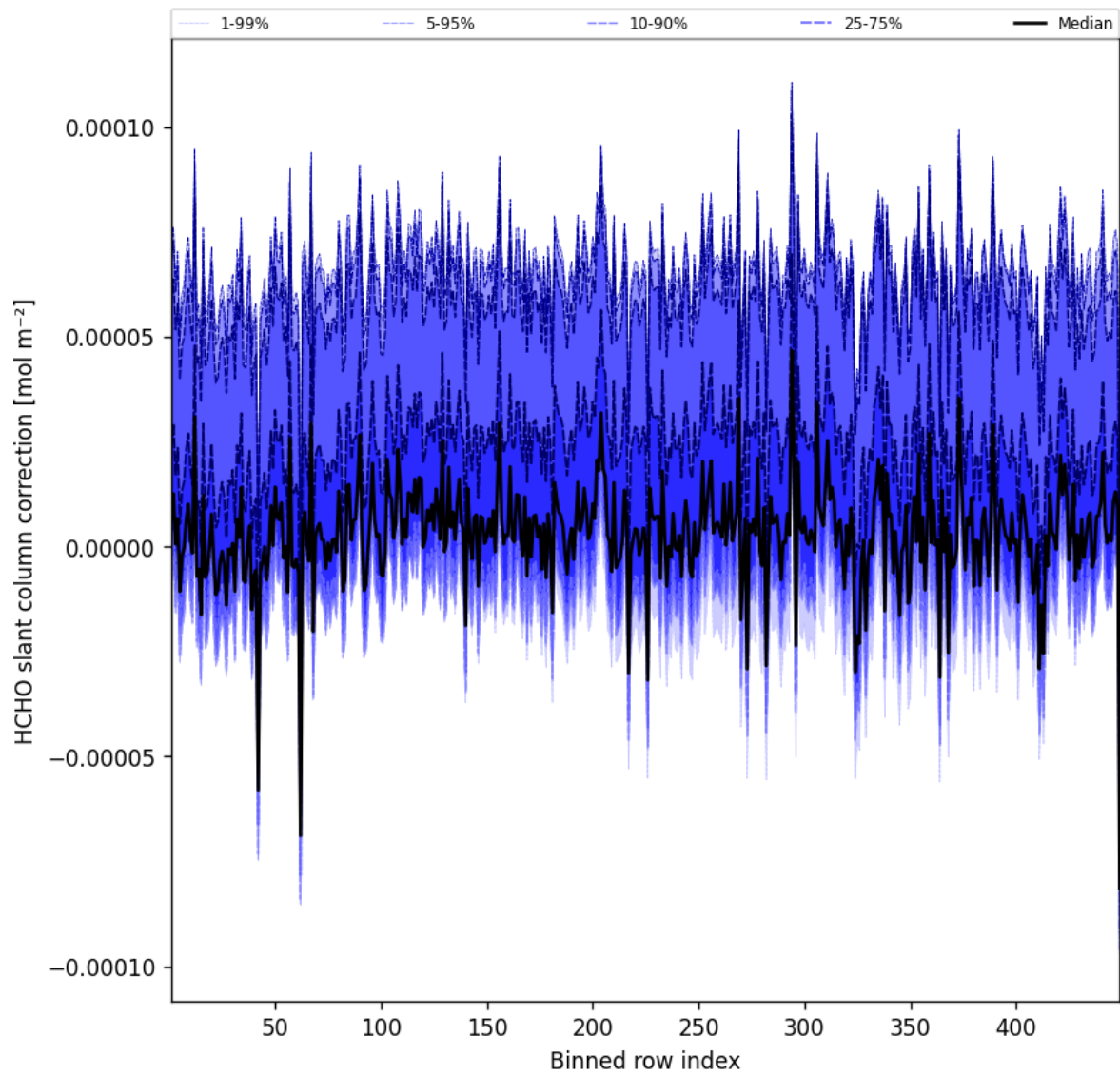
Figure 59: Along track statistics of “HCHO slant column correction” for 2025-10-04 to 2025-10-04
