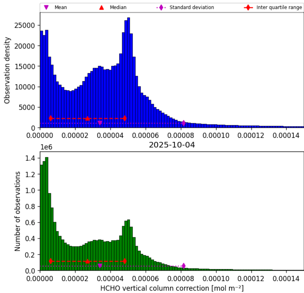
Figure 35: Histogram of “HCHO vertical column correction” for 2025-10-04 to 2025-10-04
