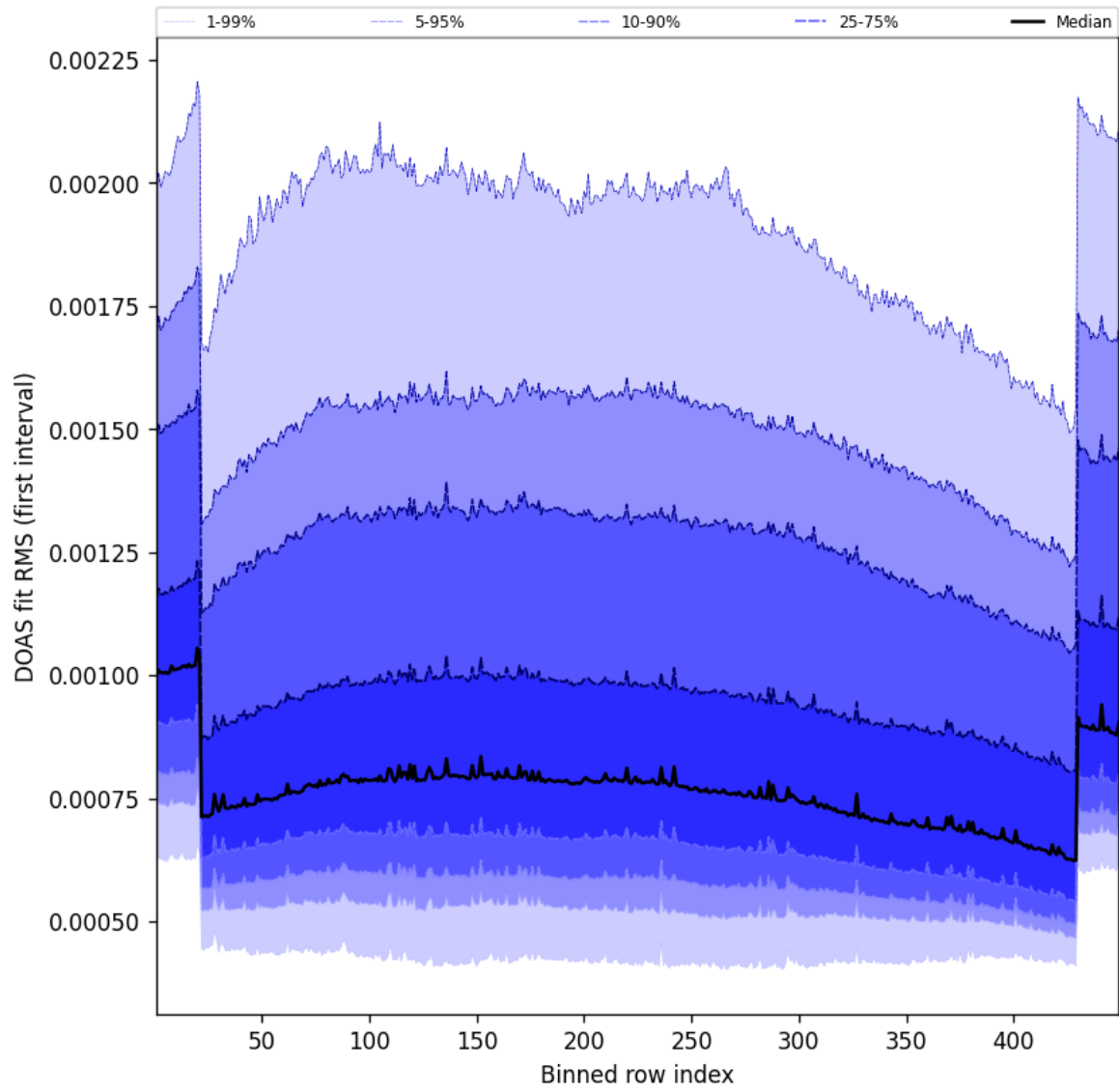
Figure 58: Along track statistics of “DOAS fit RMS (first interval)” for 2025-10-04 to 2025-10-04
