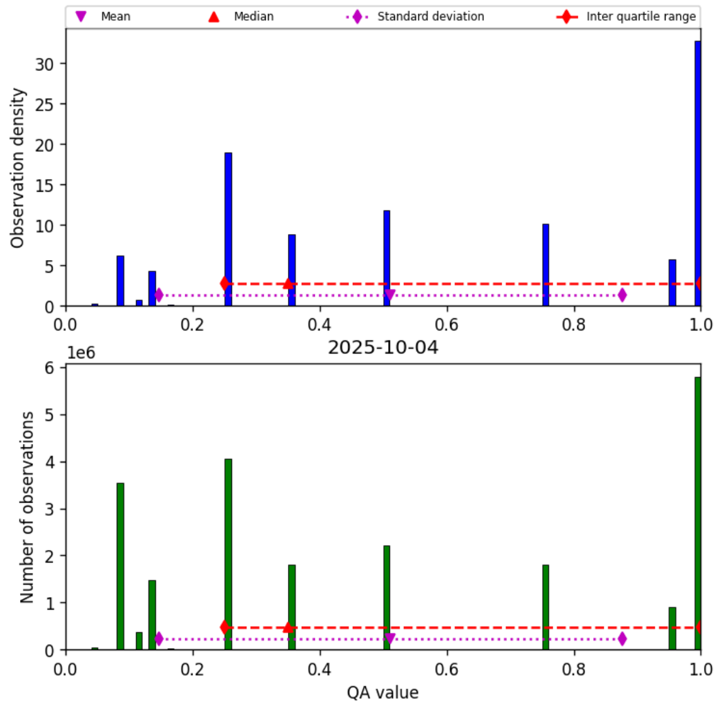
Figure 32: Histogram of “QA value” for 2025-10-04 to 2025-10-04
