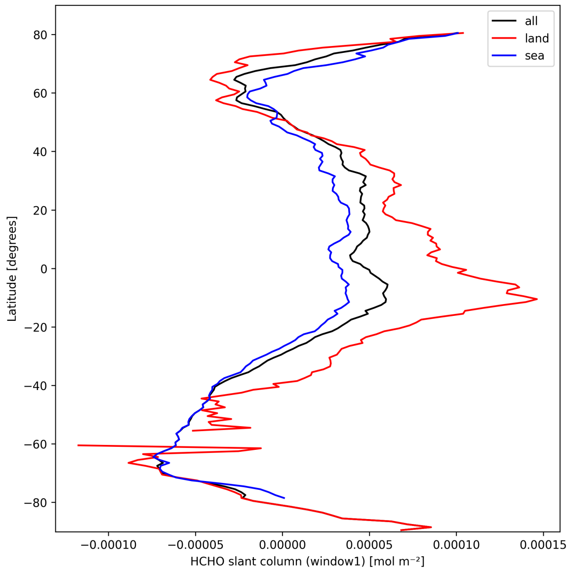
Figure 22: Zonal average of “HCHO slant column (window1)” for 2025-10-04 to 2025-10-04.
