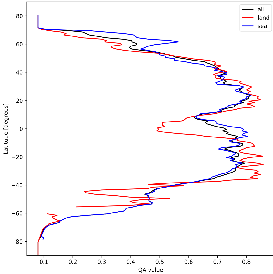
Figure 18: Zonal average of “QA value” for 2025-10-04 to 2025-10-04.
