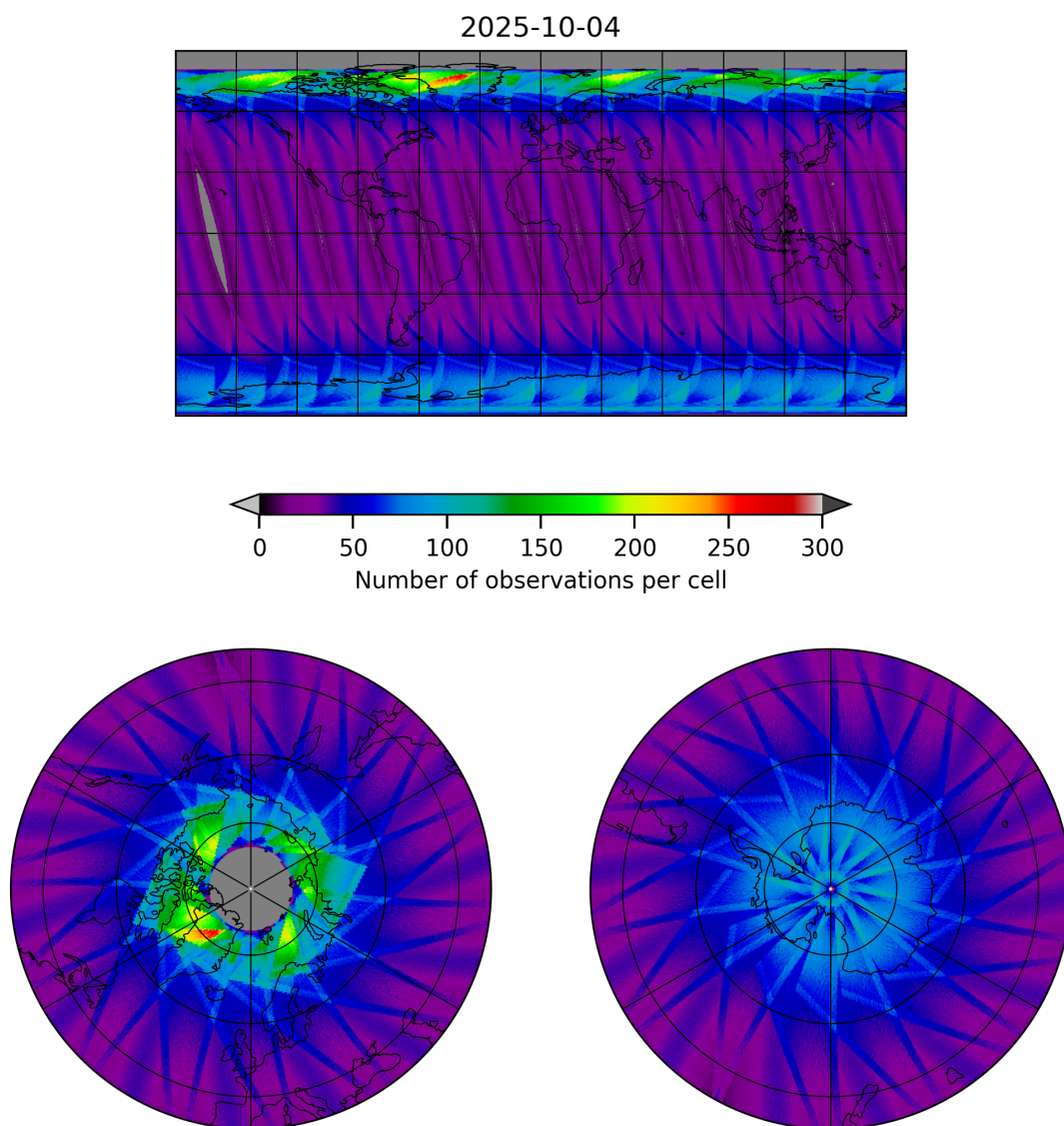
Figure 17: Map of the number of observations for 2025-10-04 to 2025-10-04
